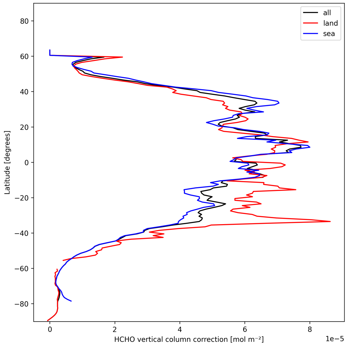
Figure 21: Zonal average of “HCHO vertical column correction” for 2024-12-01 to 2024-12-02.
