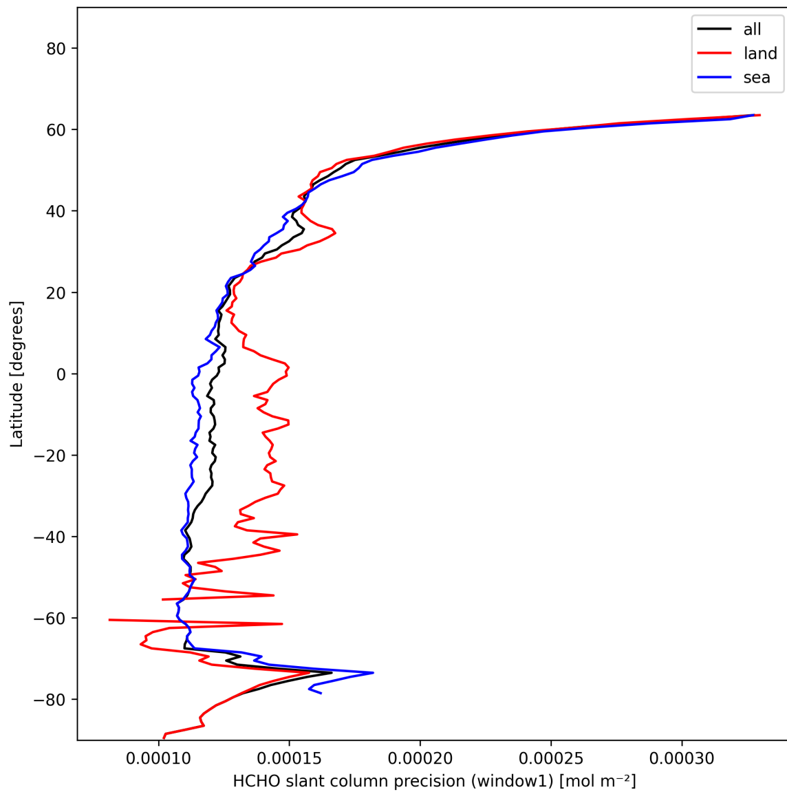
Figure 23: Zonal average of “HCHO slant column precision (window1)” for 2024-12-01 to 2024-12-02.
