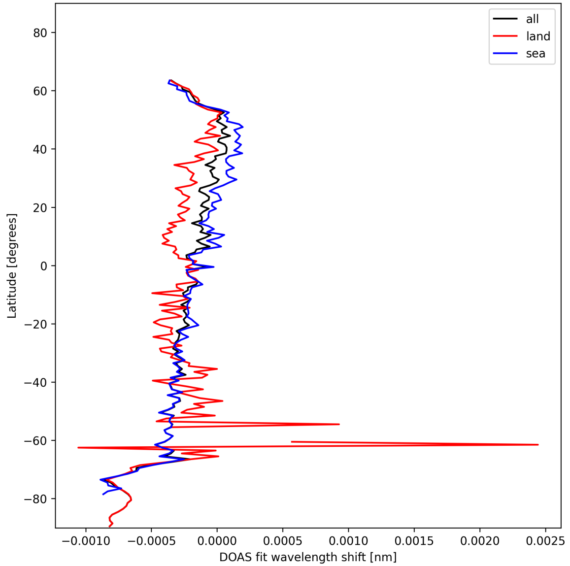
Figure 28: Zonal average of “DOAS fit wavelength shift” for 2024-12-01 to 2024-12-02.
