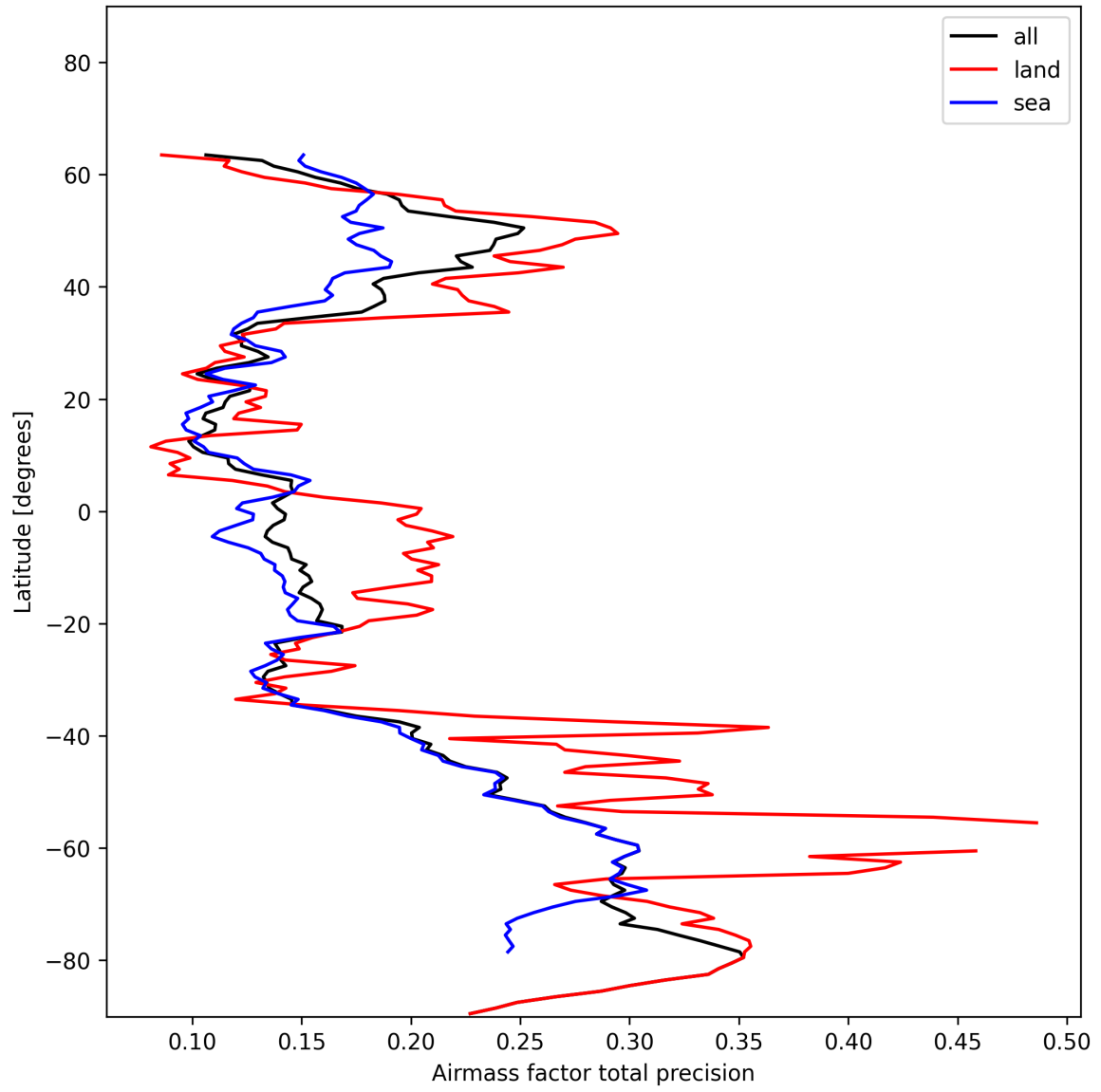
Figure 25: Zonal average of “Airmass factor total precision” for 2024-12-01 to 2024-12-02.
