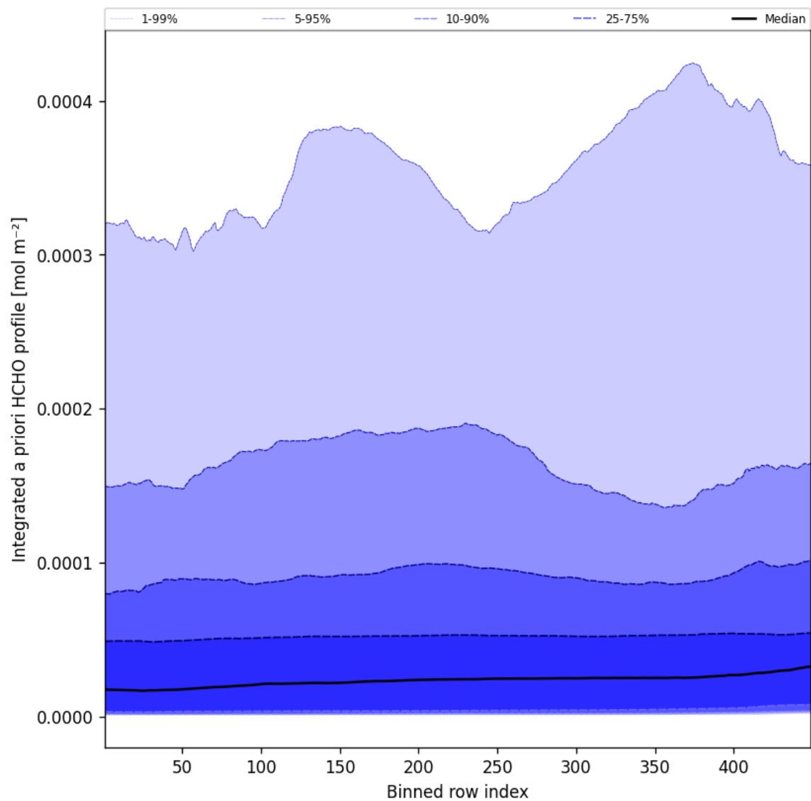
Figure 55: Along track statistics of "Integrated a priori HCHO profile" for 2024-12-01 to 2024-12-02
