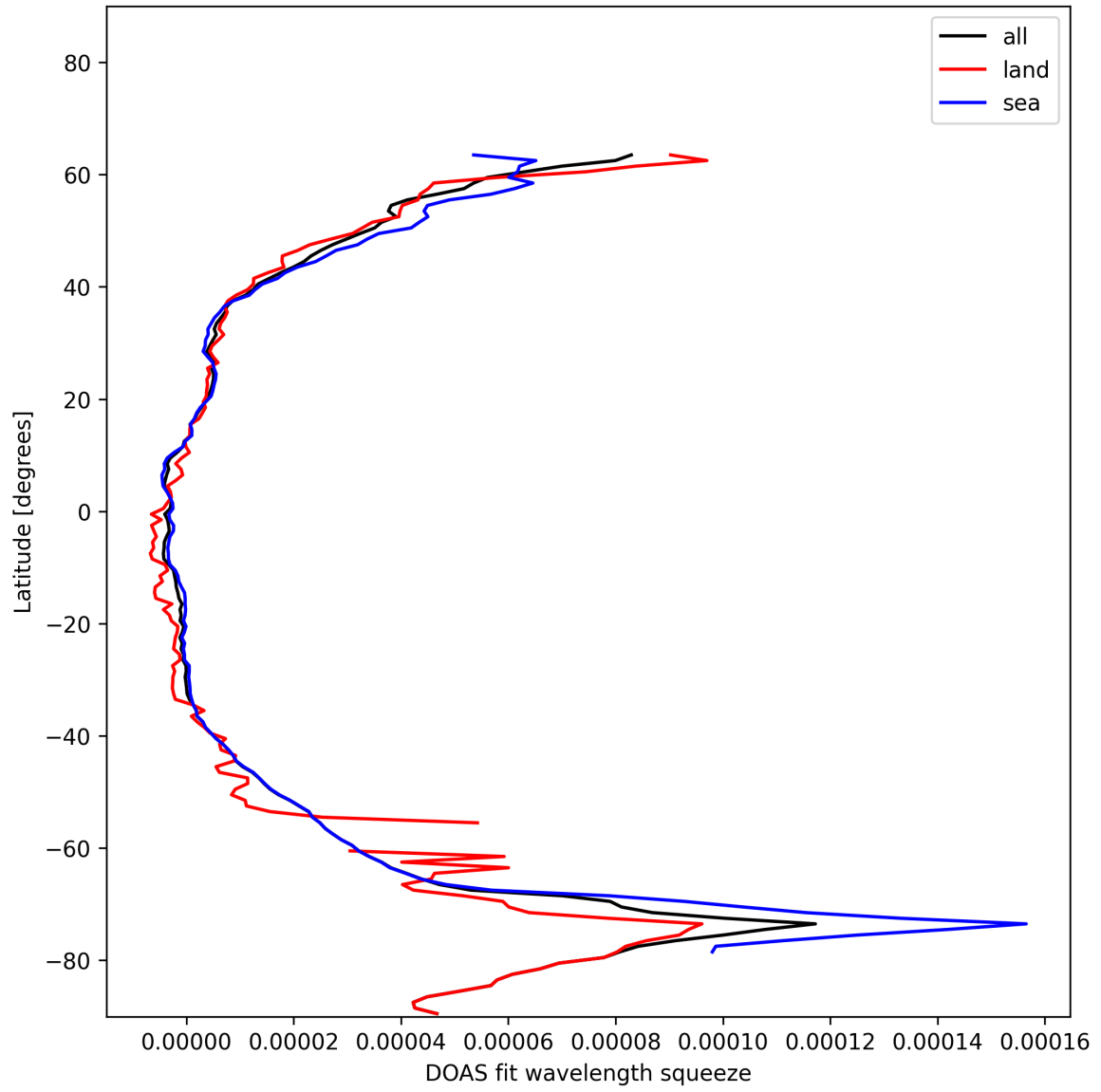
Figure 29: Zonal average of “DOAS fit wavelength squeeze” for 2024-12-01 to 2024-12-02.
