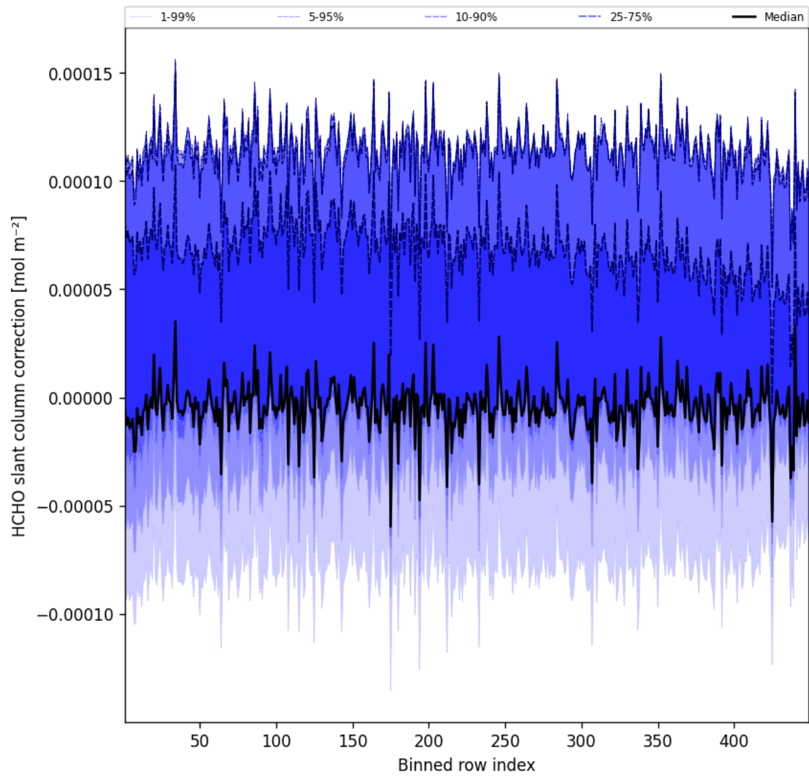
Figure 59: Along track statistics of “HCHO slant column correction” for 2024-12-01 to 2024-12-02
