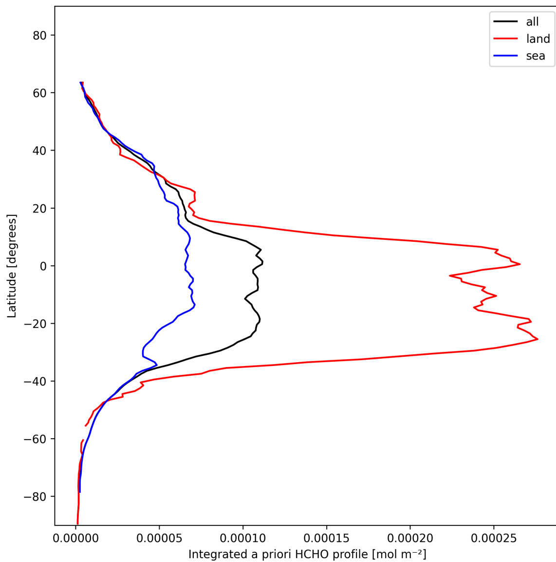
Figure 27: Zonal average of “Integrated a priori HCHO profile” for 2024-12-01 to 2024-12-02.
