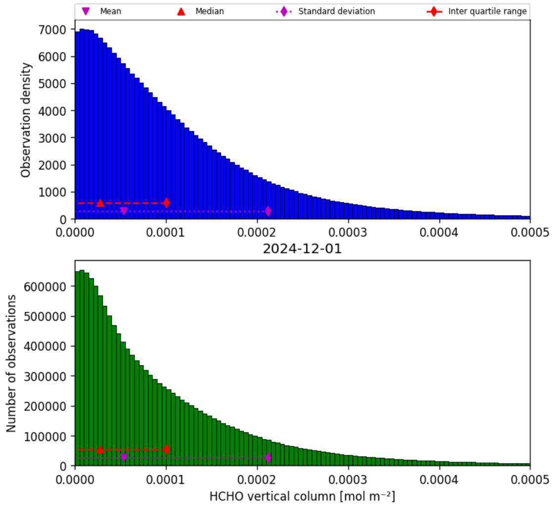
Figure 33: Histogram of “HCHO vertical column” for 2024-12-01 to 2024-12-02
