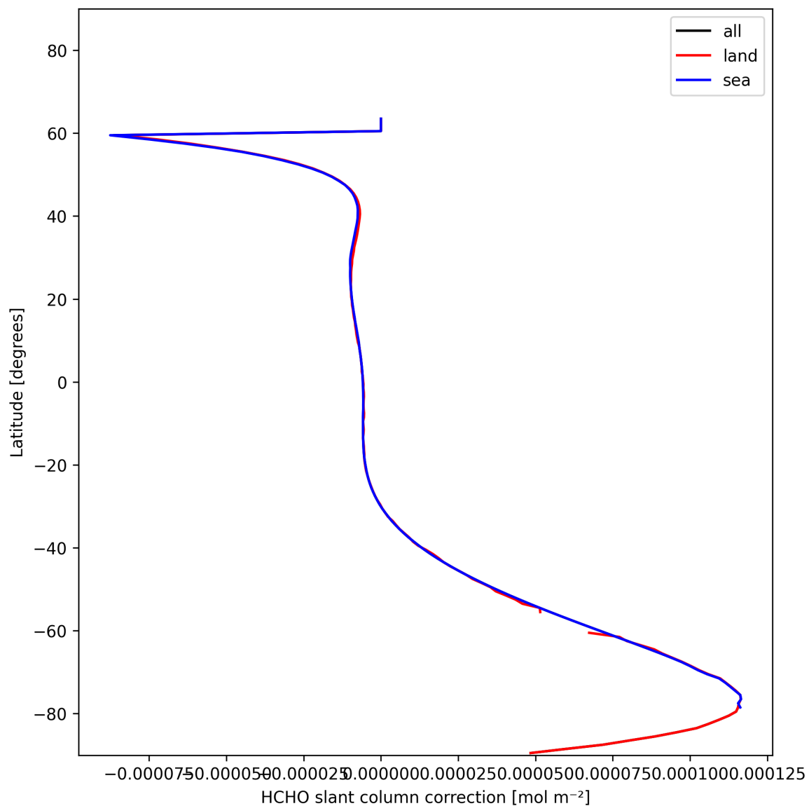
Figure 31: Zonal average of “HCHO slant column correction” for 2024-12-01 to 2024-12-02.
