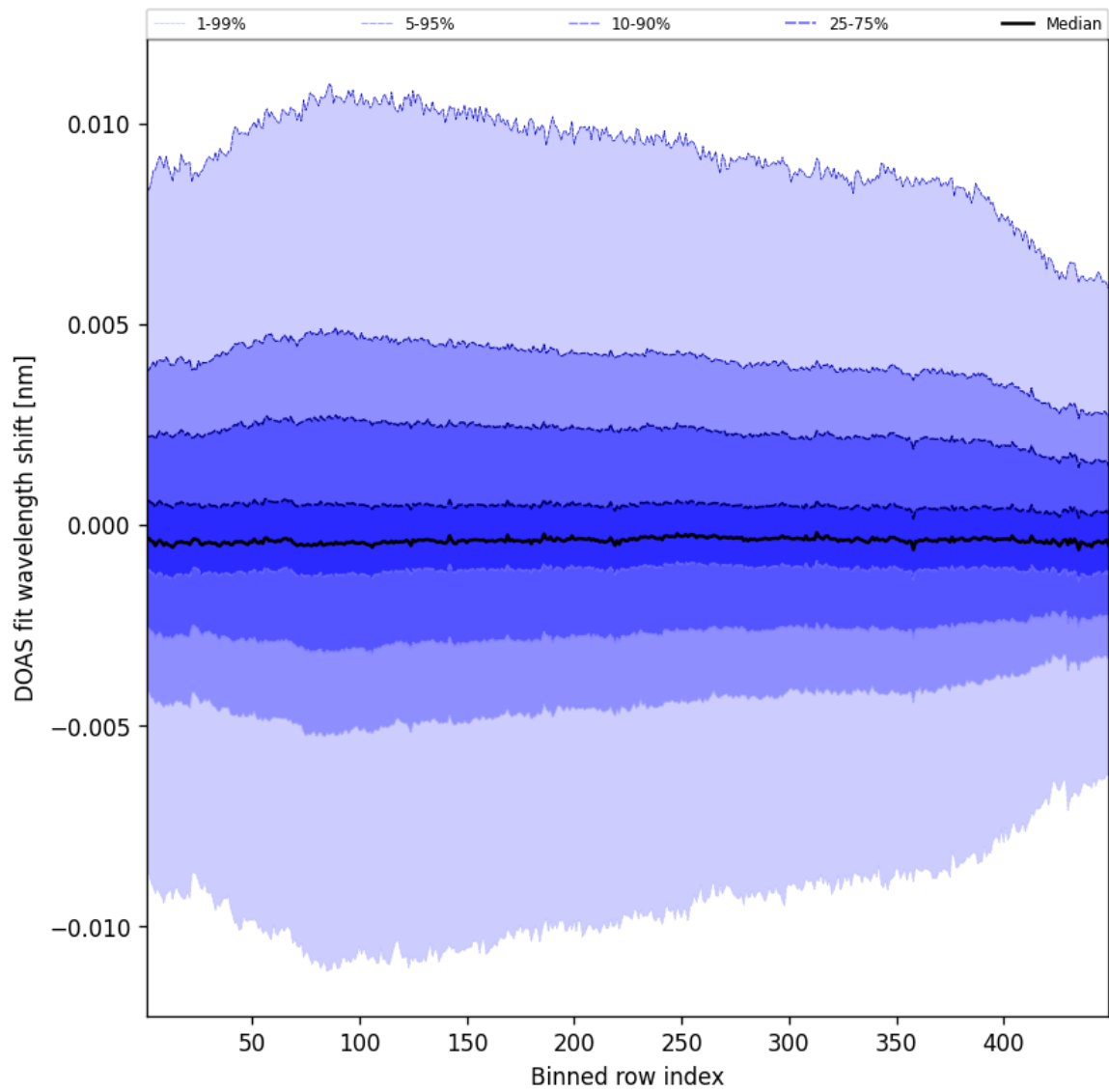
Figure 56: Along track statistics of “DOAS fit wavelength shift” for 2024-12-01 to 2024-12-02
