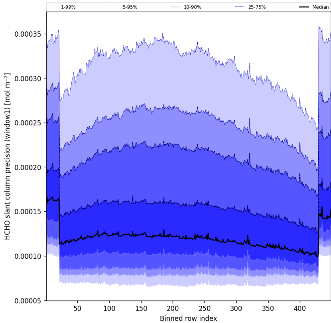
Figure 51: Along track statistics of “HCHO slant column precision (window1)” for 2024-12-01 to 2024-12-02
