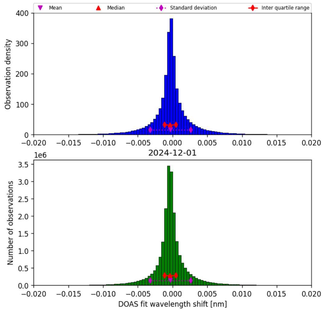
Figure 42: Histogram of “DOAS fit wavelength shift” for 2024-12-01 to 2024-12-02
