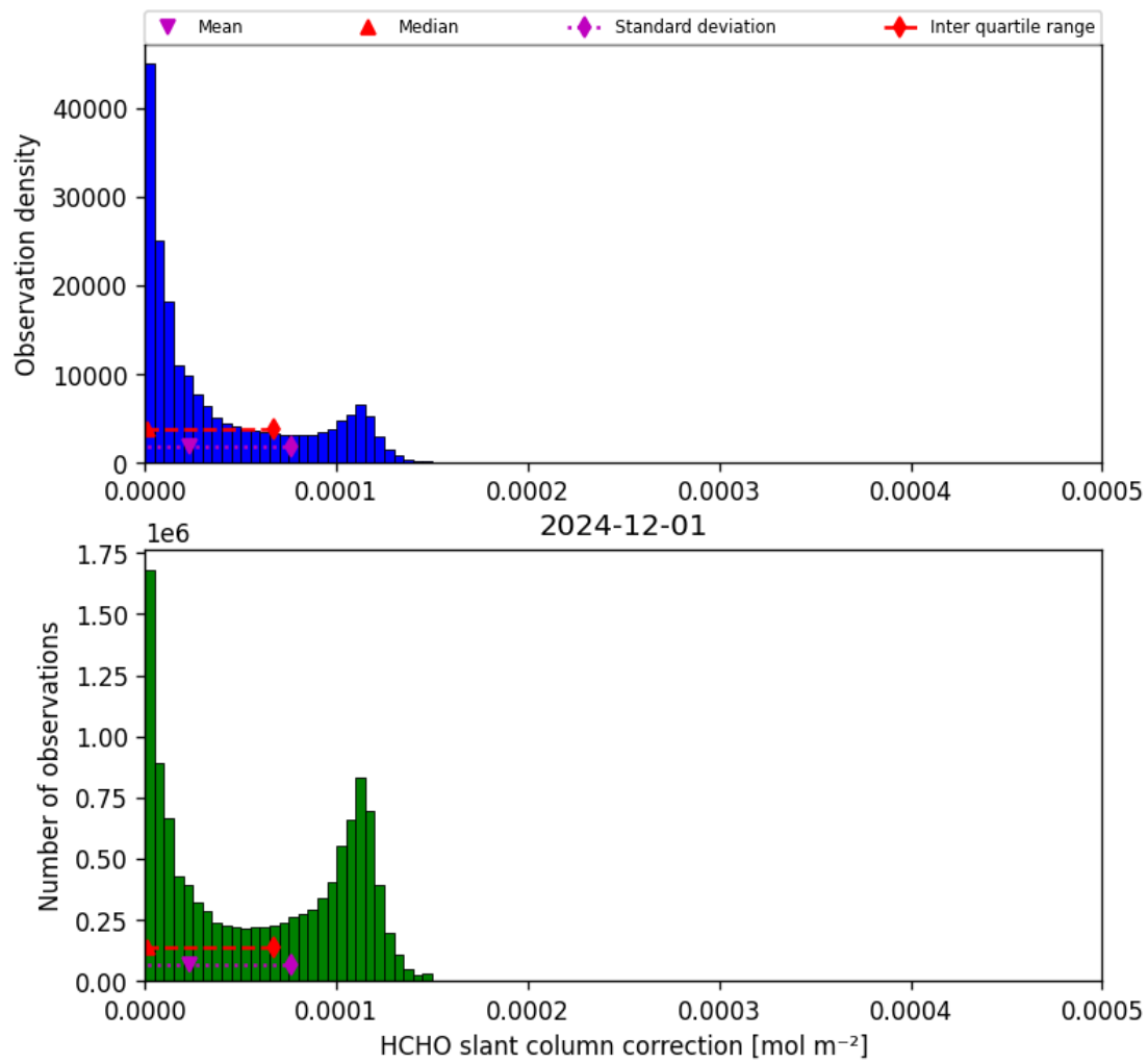
Figure 45: Histogram of “HCHO slant column correction” for 2024-12-01 to 2024-12-02
