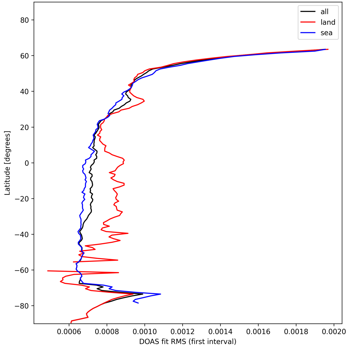
Figure 30: Zonal average of “DOAS fit RMS (first interval)” for 2024-12-01 to 2024-12-02.
