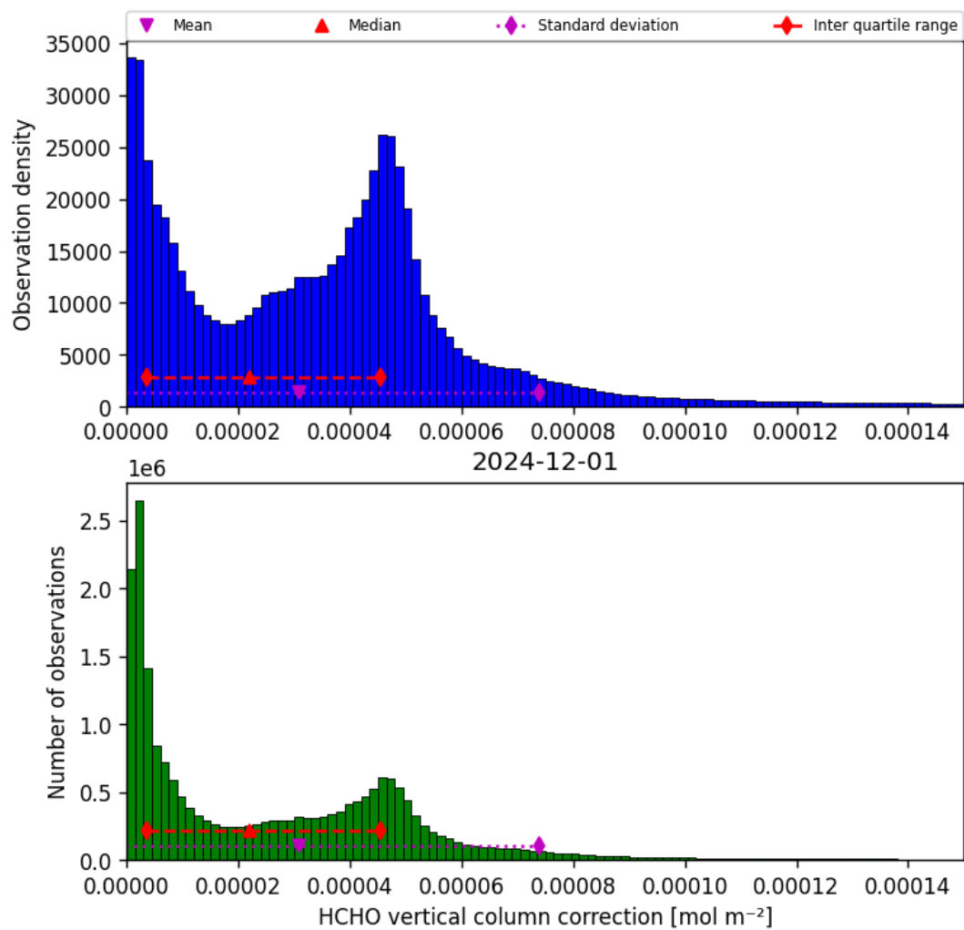
Figure 35: Histogram of “HCHO vertical column correction” for 2024-12-01 to 2024-12-02
