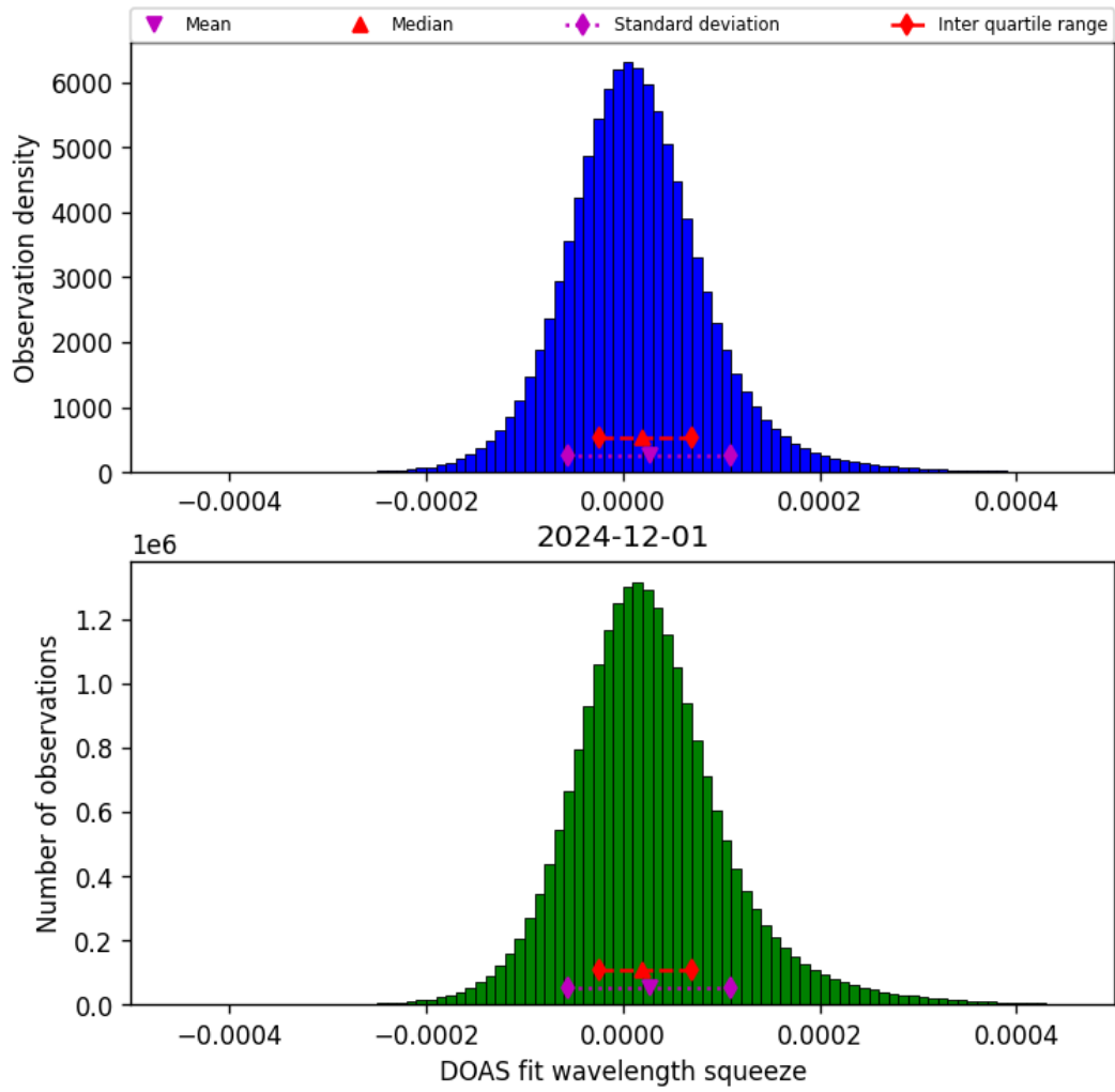
Figure 43: Histogram of “DOAS fit wavelength squeeze” for 2024-12-01 to 2024-12-02
