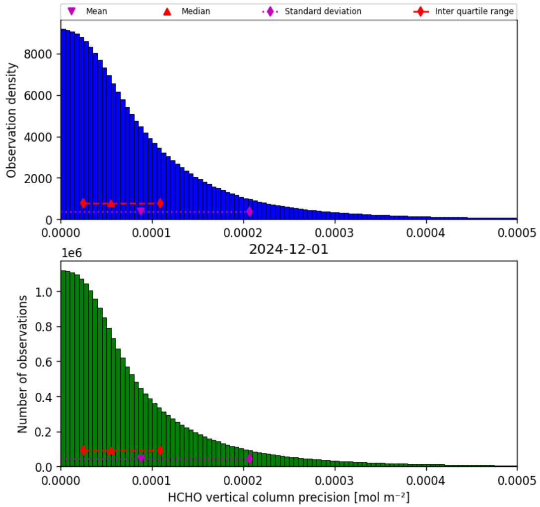
Figure 34: Histogram of “HCHO vertical column precision” for 2024-12-01 to 2024-12-02
