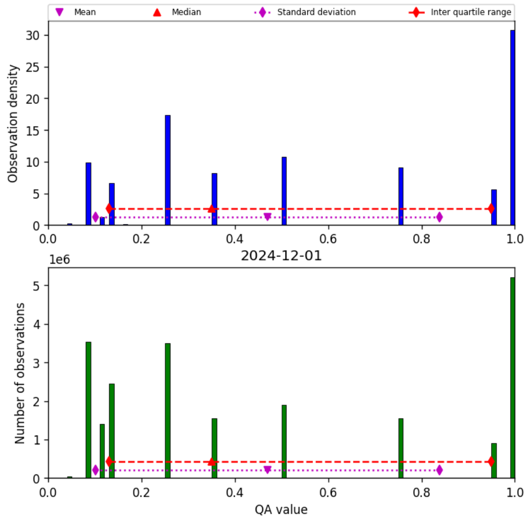
Figure 32: Histogram of “QA value” for 2024-12-01 to 2024-12-02
