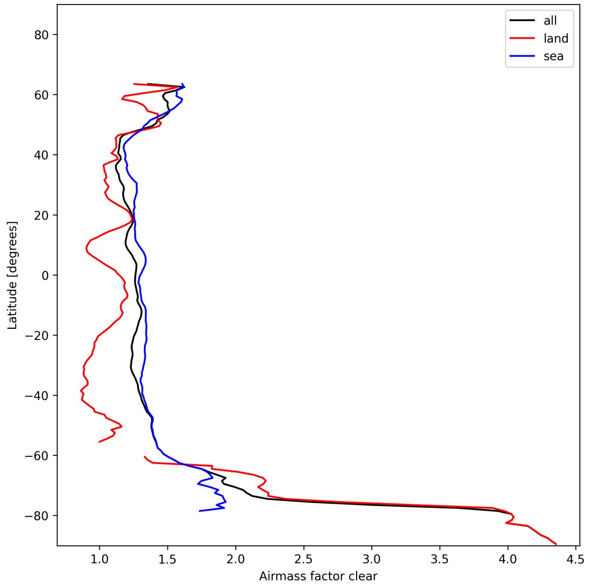
Figure 26: Zonal average of “Airmass factor clear” for 2024-12-01 to 2024-12-02.
