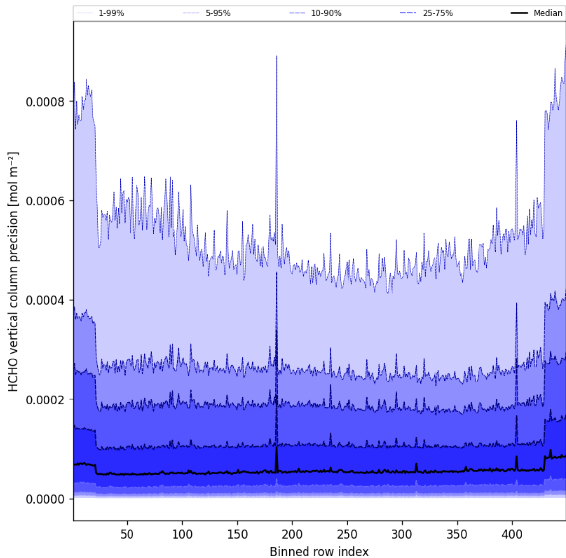
Figure 48: Along track statistics of “HCHO vertical column precision” for 2024-12-01 to 2024-12-02
