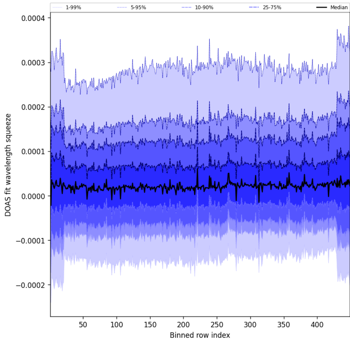
Figure 57: Along track statistics of “DOAS fit wavelength squeeze” for 2024-12-01 to 2024-12-02
