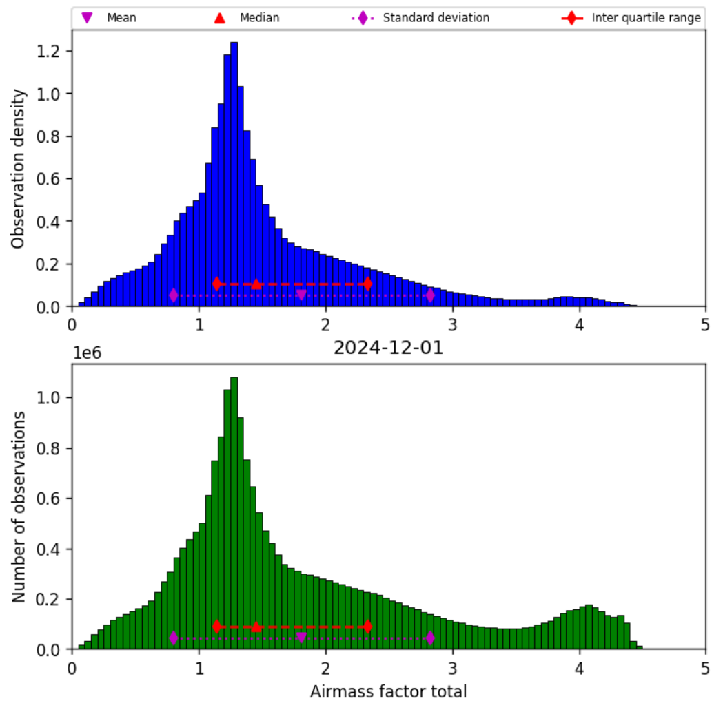
Figure 38: Histogram of “Airmass factor total” for 2024-12-01 to 2024-12-02
