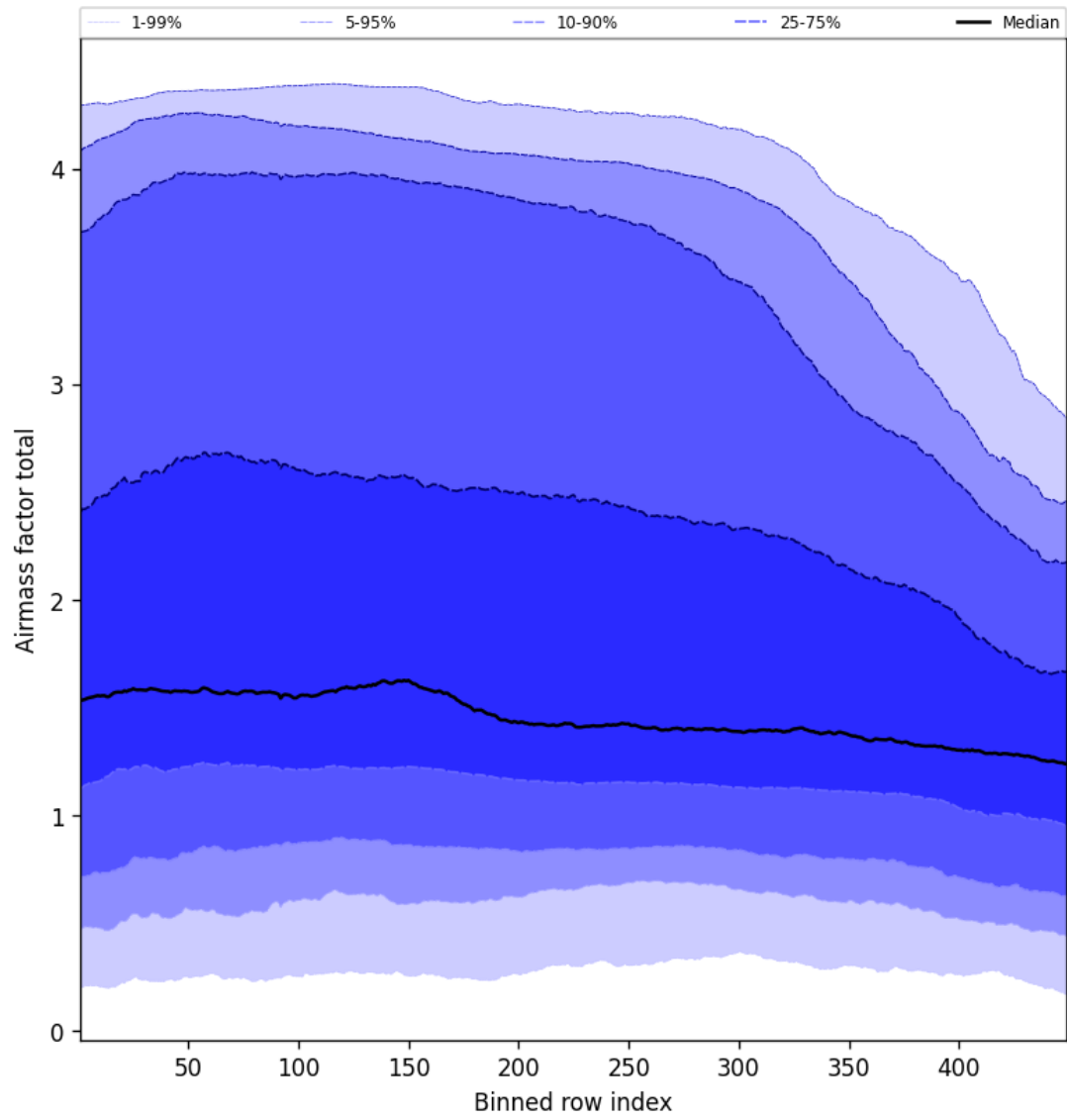
Figure 52: Along track statistics of “Airmass factor total” for 2024-12-01 to 2024-12-02
