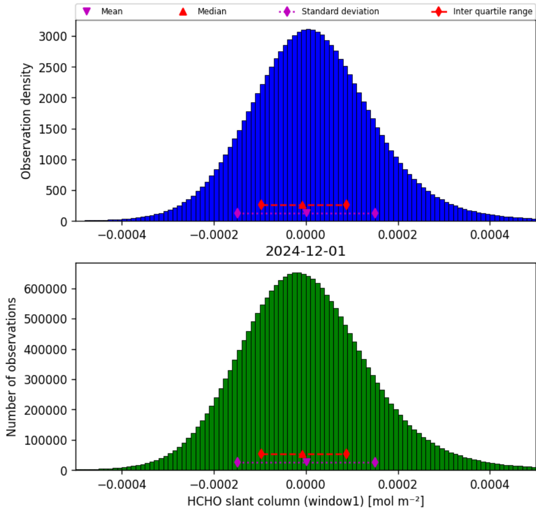
Figure 36: Histogram of “HCHO slant column (window1)” for 2024-12-01 to 2024-12-02
