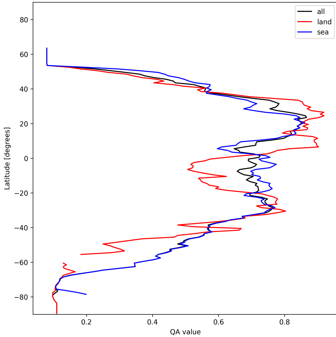
Figure 18: Zonal average of “QA value” for 2024-12-01 to 2024-12-02.
