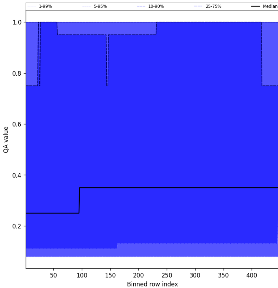
Figure 46: Along track statistics of “QA value” for 2024-12-01 to 2024-12-02
