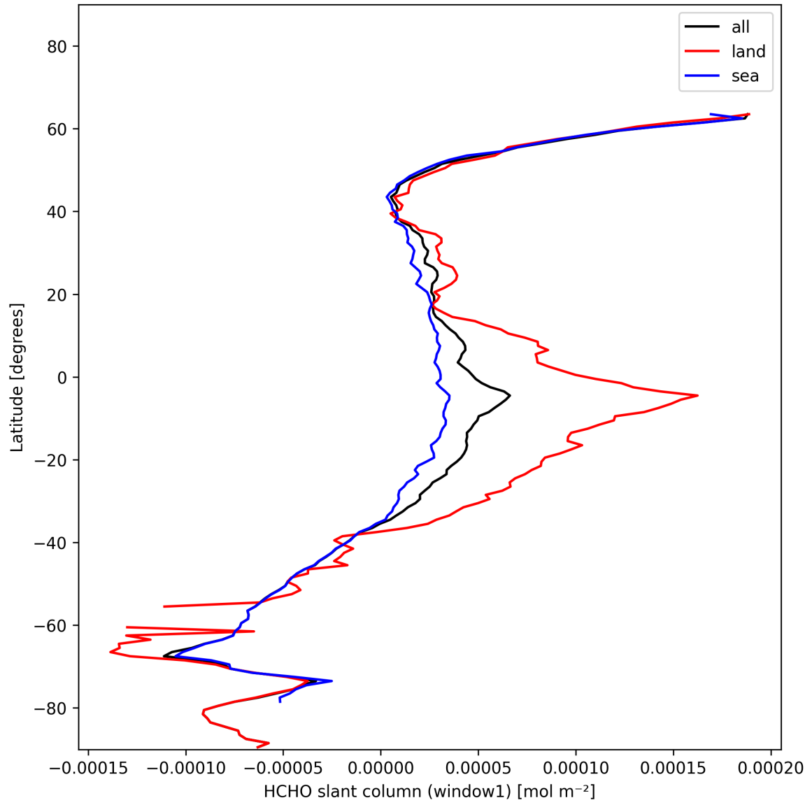
Figure 22: Zonal average of “HCHO slant column (window1)” for 2024-12-01 to 2024-12-02.
