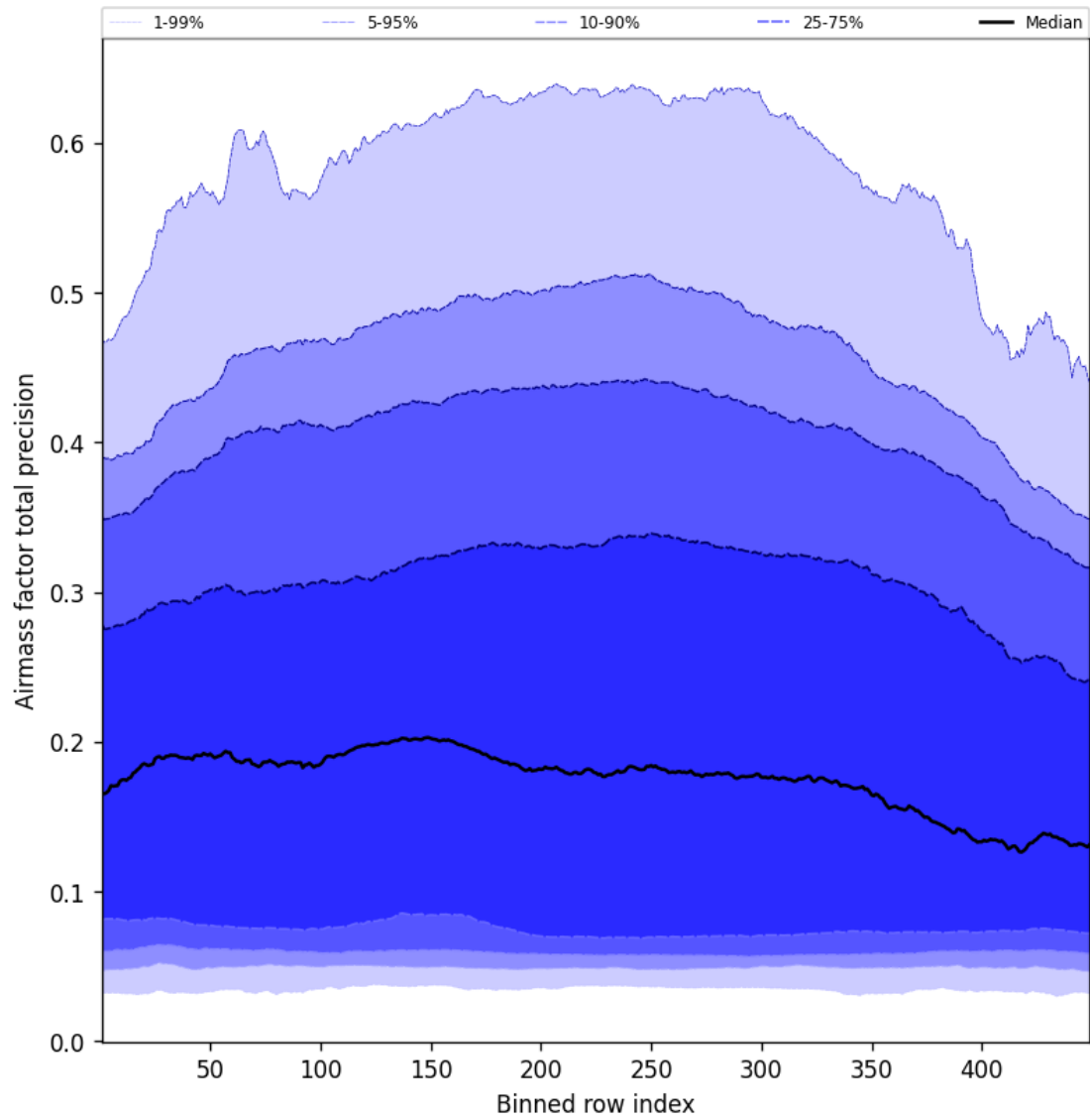
Figure 53: Along track statistics of “Airmass factor total precision” for 2024-12-01 to 2024-12-02
