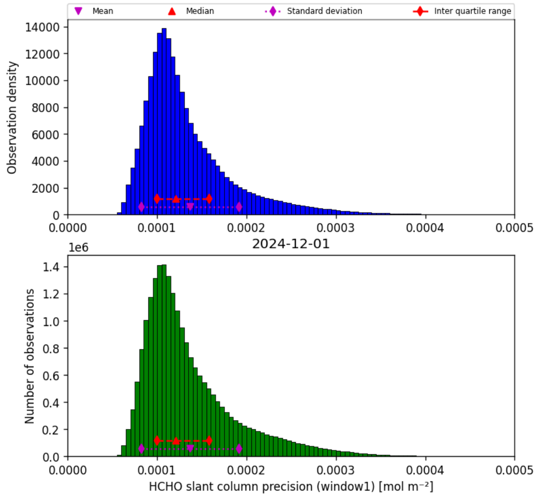
Figure 37: Histogram of “HCHO slant column precision (window1)” for 2024-12-01 to 2024-12-02
