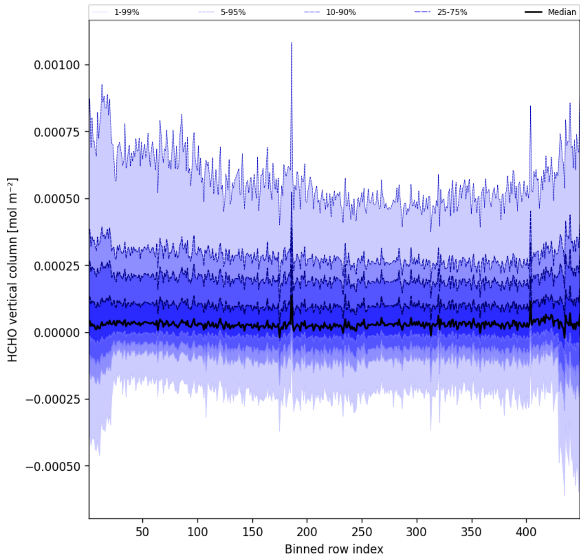
Figure 47: Along track statistics of “HCHO vertical column” for 2024-12-01 to 2024-12-02
