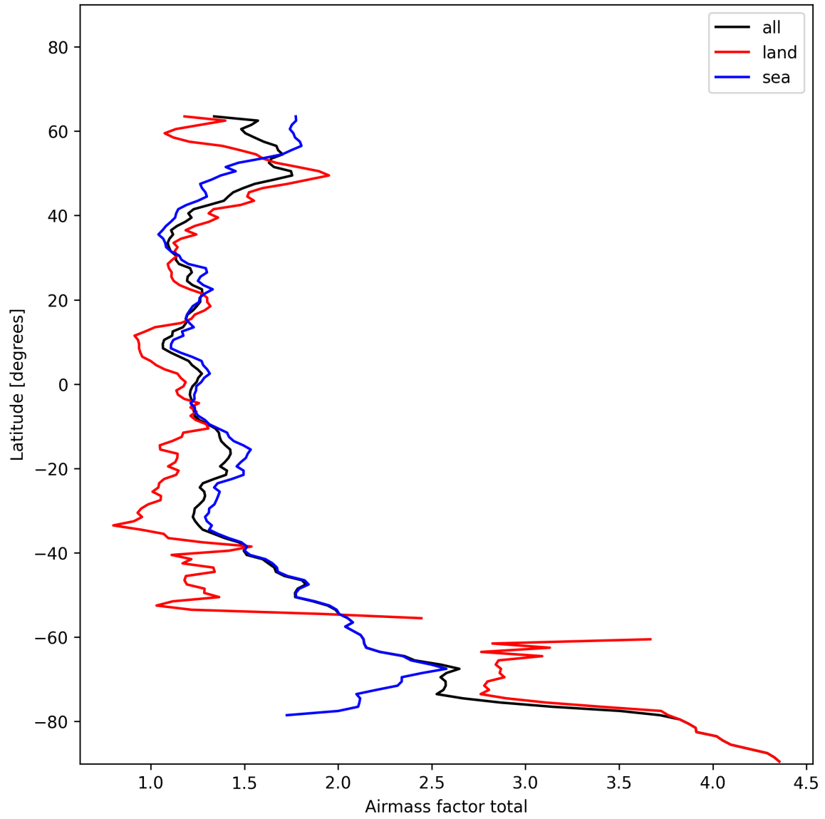
Figure 24: Zonal average of “Airmass factor total” for 2024-12-01 to 2024-12-02.
