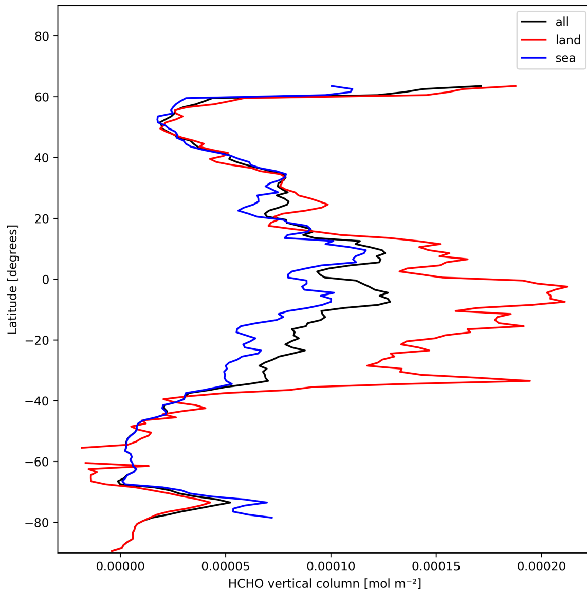
Figure 19: Zonal average of “HCHO vertical column” for 2024-12-01 to 2024-12-02.
