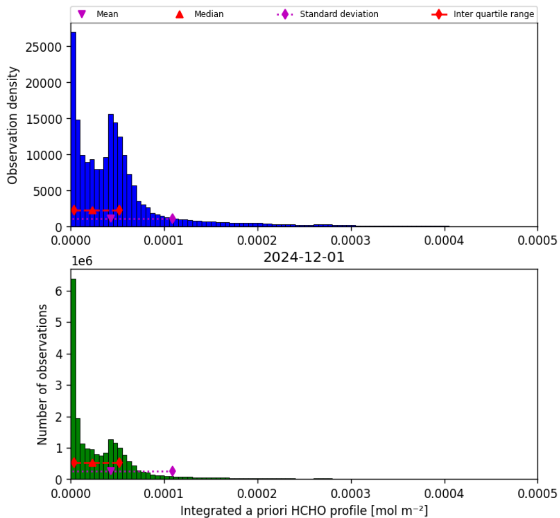
Figure 41: Histogram of “Integrated a priori HCHO profile” for 2024-12-01 to 2024-12-02
