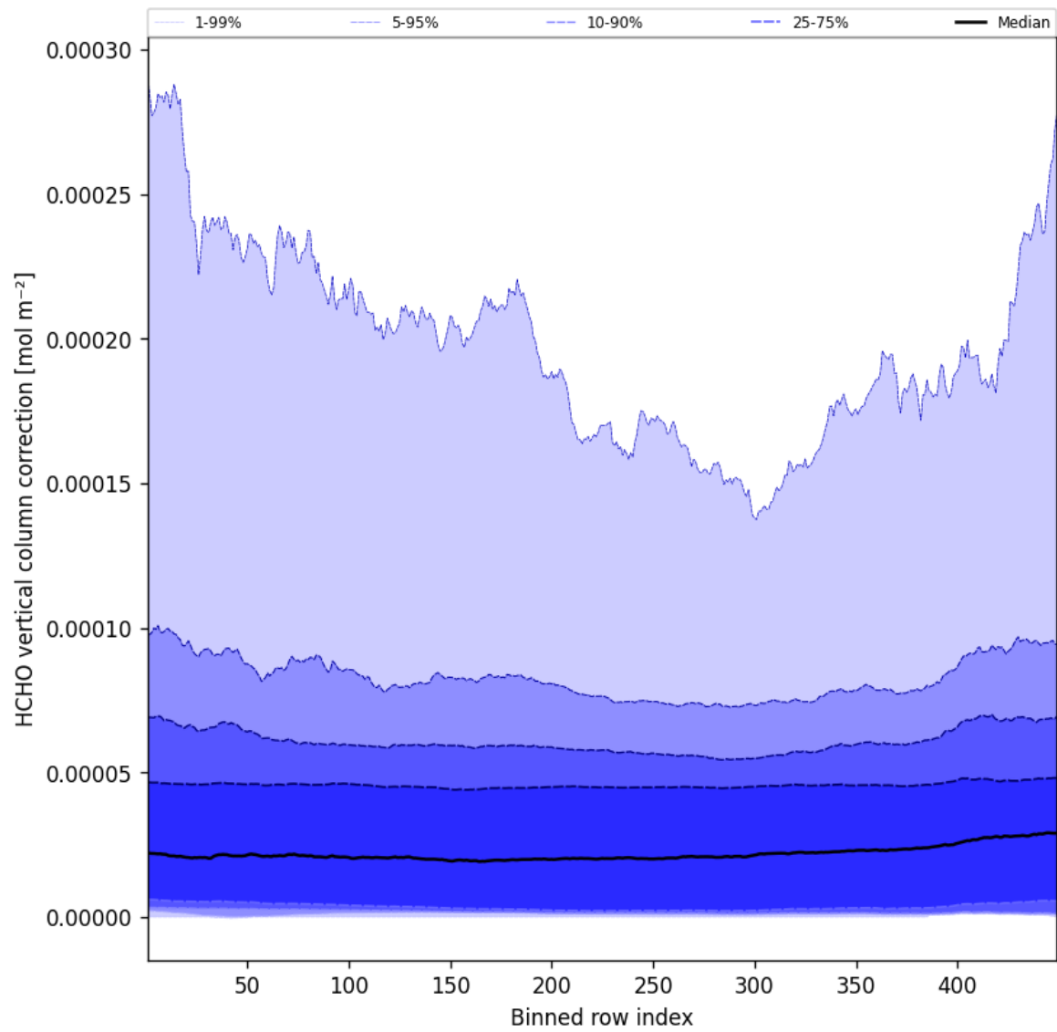
Figure 49: Along track statistics of “HCHO vertical column correction” for 2024-12-01 to 2024-12-02
