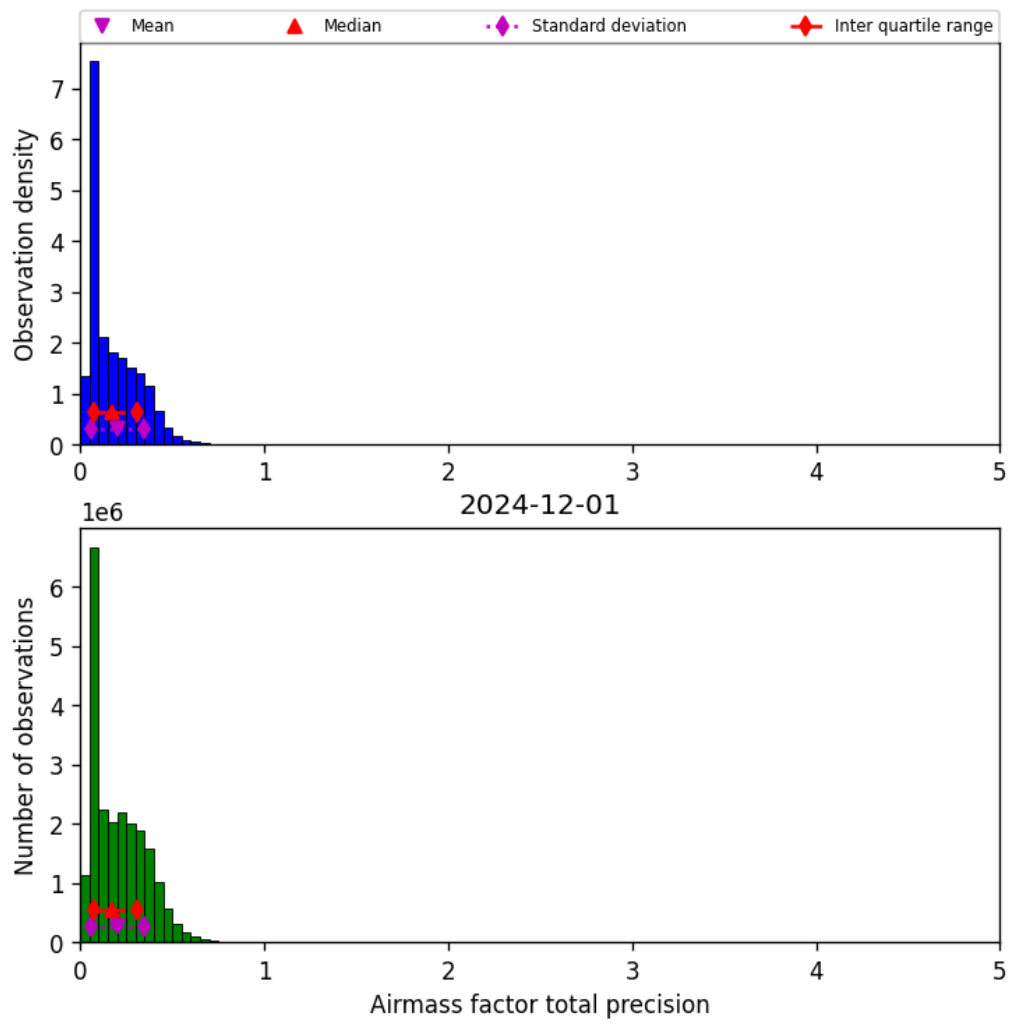
Figure 39: Histogram of “Airmass factor total precision” for 2024-12-01 to 2024-12-02
