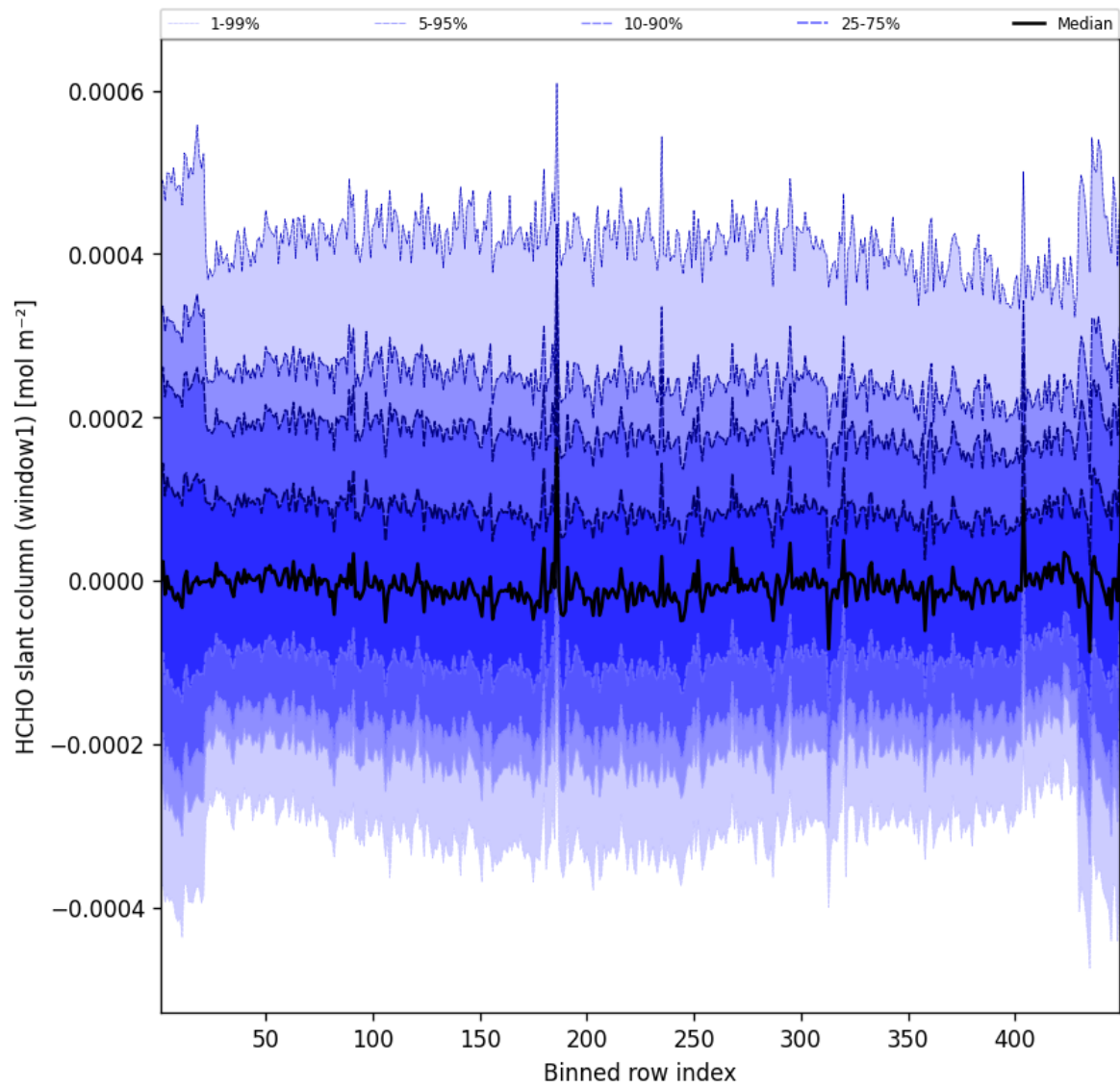
Figure 50: Along track statistics of “HCHO slant column (window1)” for 2024-12-01 to 2024-12-02
