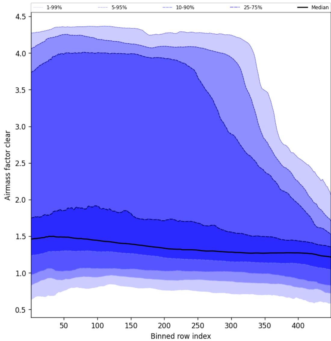
Figure 54: Along track statistics of “Airmass factor clear” for 2024-12-01 to 2024-12-02
