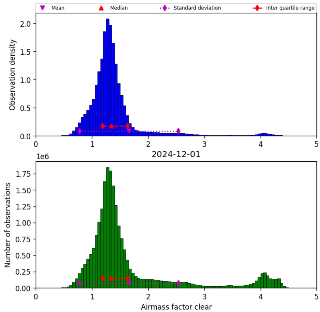
Figure 40: Histogram of “Airmass factor clear” for 2024-12-01 to 2024-12-02
