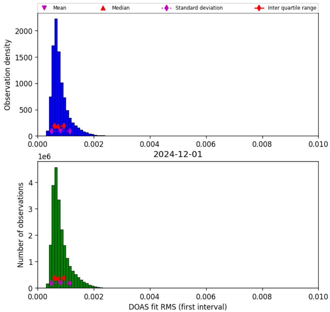
Figure 44: Histogram of “DOAS fit RMS (first interval)” for 2024-12-01 to 2024-12-02
