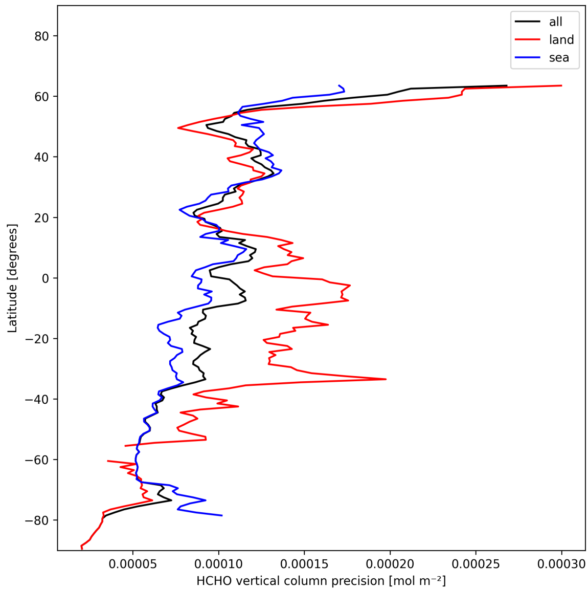
Figure 20: Zonal average of “HCHO vertical column precision” for 2024-12-01 to 2024-12-02.
