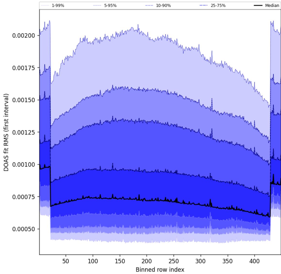
Figure 58: Along track statistics of “DOAS fit RMS (first interval)” for 2024-12-01 to 2024-12-02
