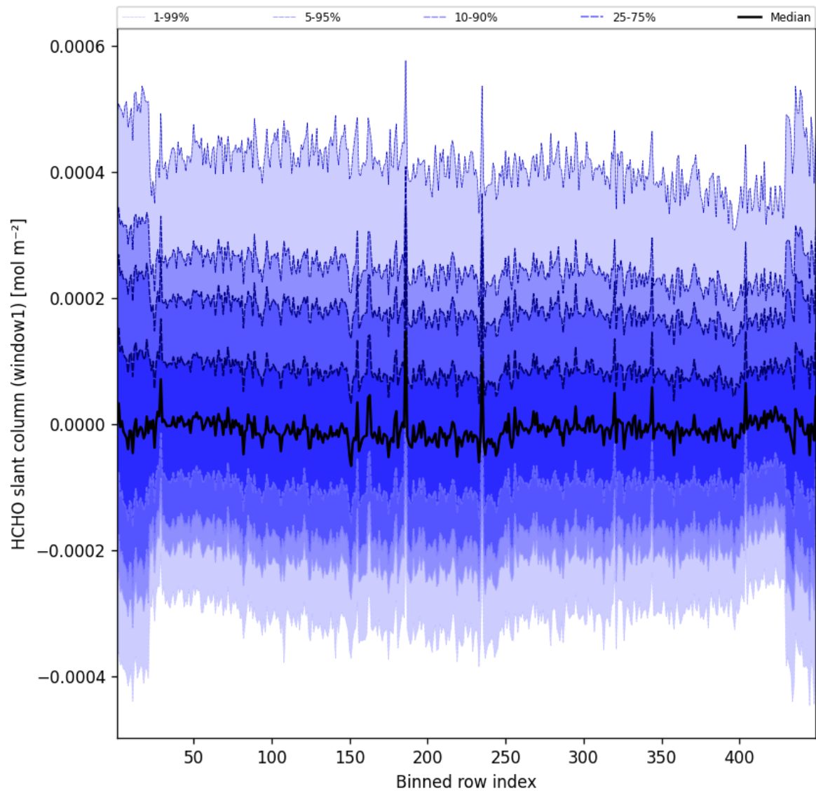
Figure 50: Along track statistics of “HCHO slant column (window1)” for 2024-12-02 to 2024-12-03
