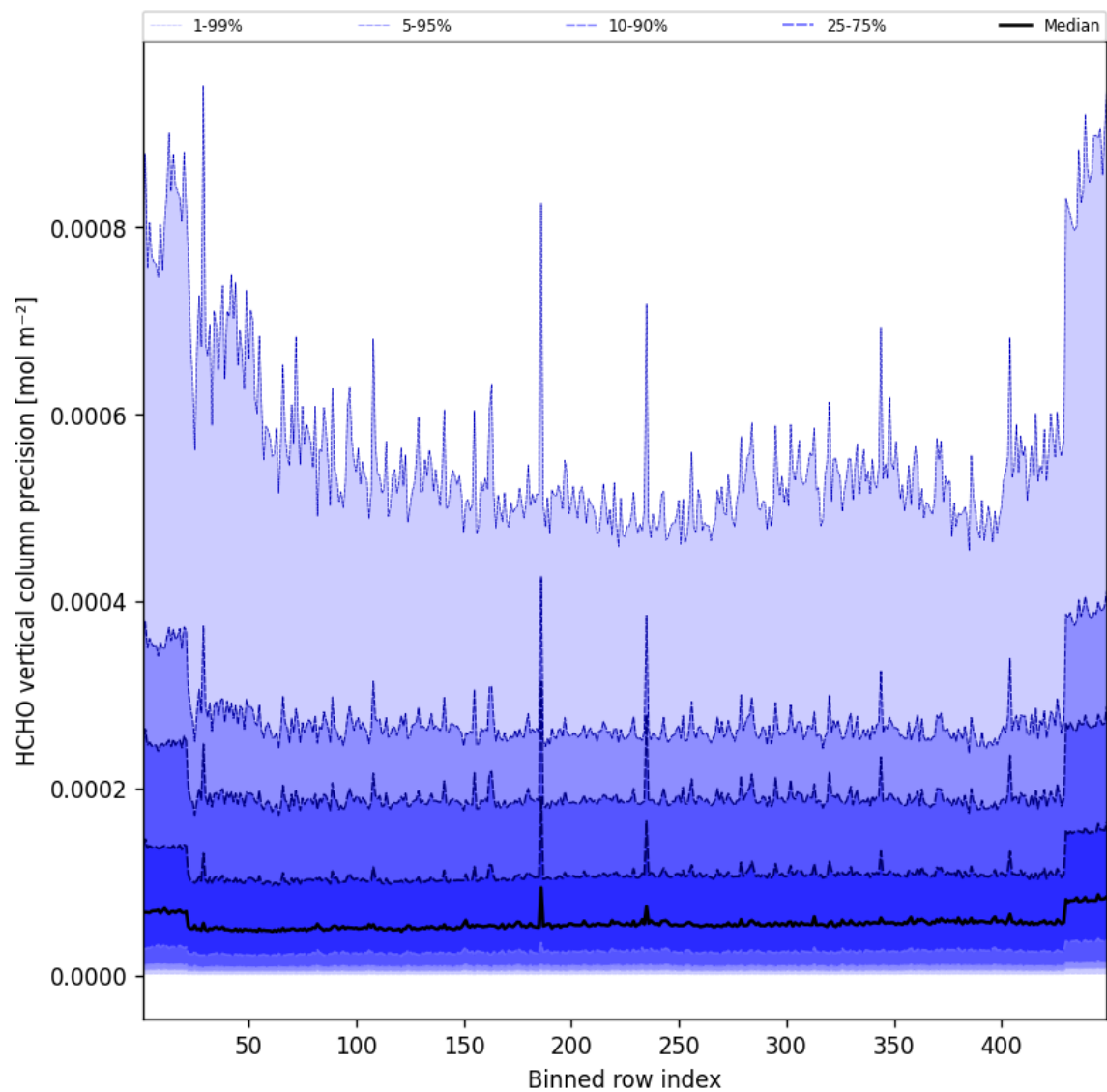
Figure 48: Along track statistics of “HCHO vertical column precision” for 2024-12-02 to 2024-12-03
