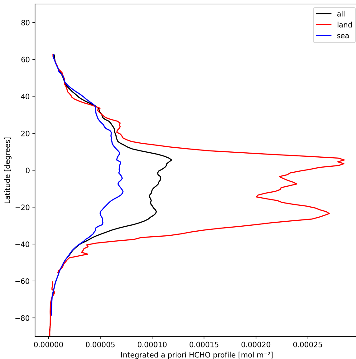
Figure 27: Zonal average of “Integrated a priori HCHO profile” for 2024-12-02 to 2024-12-03.
