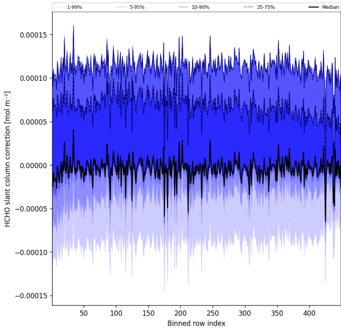
Figure 59: Along track statistics of “HCHO slant column correction” for 2024-12-02 to 2024-12-03
