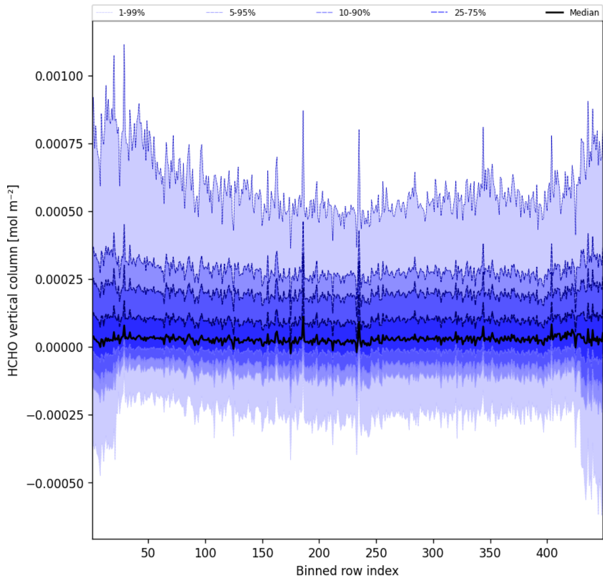
Figure 47: Along track statistics of “HCHO vertical column” for 2024-12-02 to 2024-12-03
