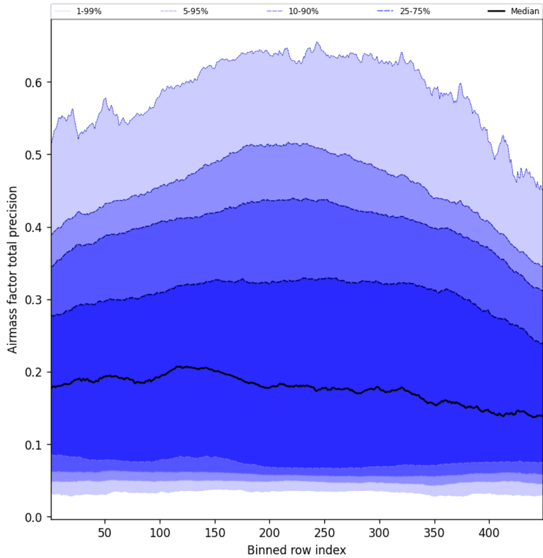
Figure 53: Along track statistics of “Airmass factor total precision” for 2024-12-02 to 2024-12-03
