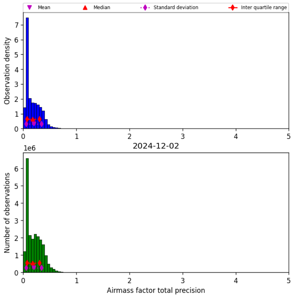
Figure 39: Histogram of “Airmass factor total precision” for 2024-12-02 to 2024-12-03
