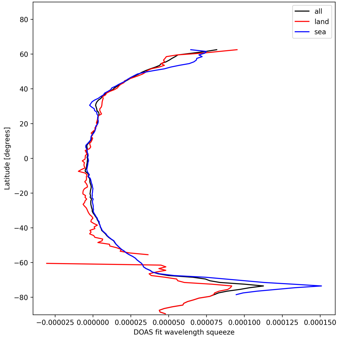
Figure 29: Zonal average of “DOAS fit wavelength squeeze” for 2024-12-02 to 2024-12-03.
