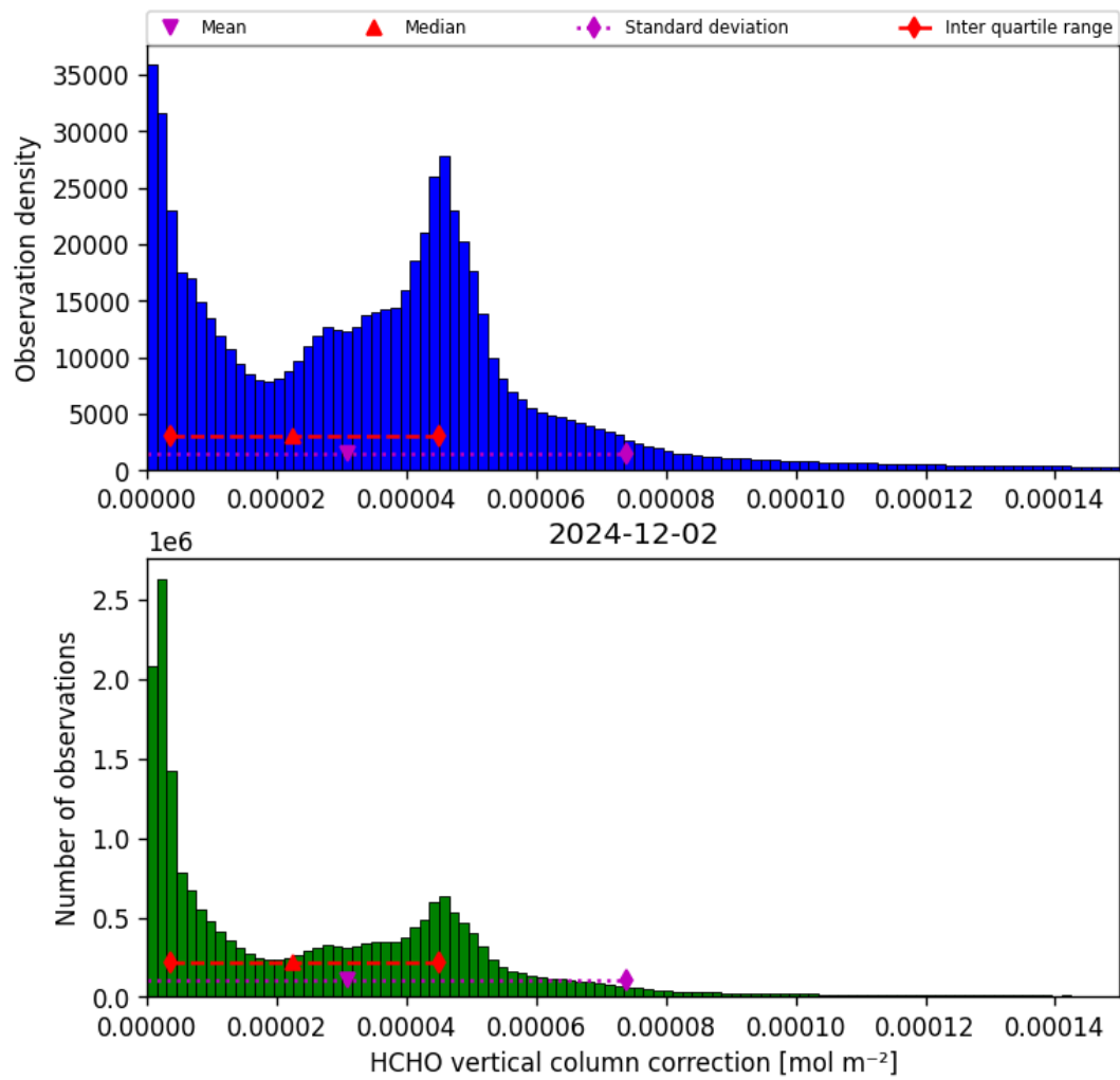
Figure 35: Histogram of “HCHO vertical column correction” for 2024-12-02 to 2024-12-03
