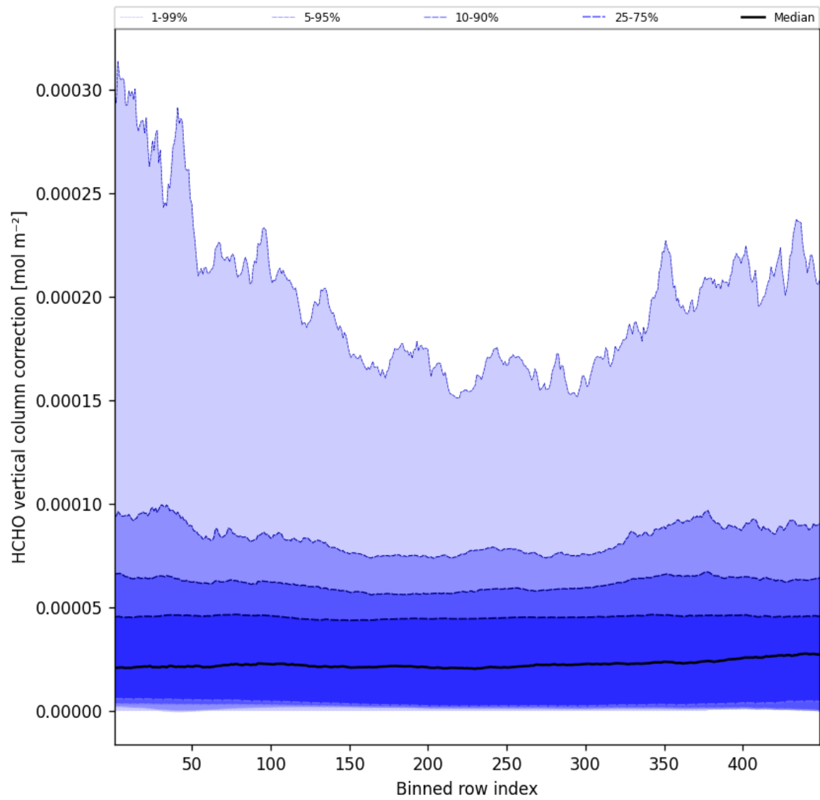
Figure 49: Along track statistics of "HCHO vertical column correction" for 2024-12-02 to 2024-12-03
