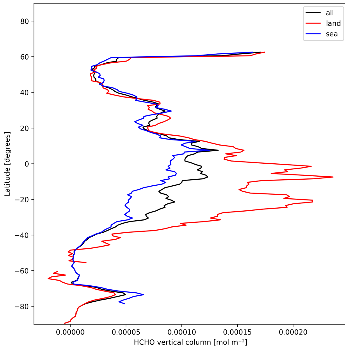
Figure 19: Zonal average of “HCHO vertical column” for 2024-12-02 to 2024-12-03.
