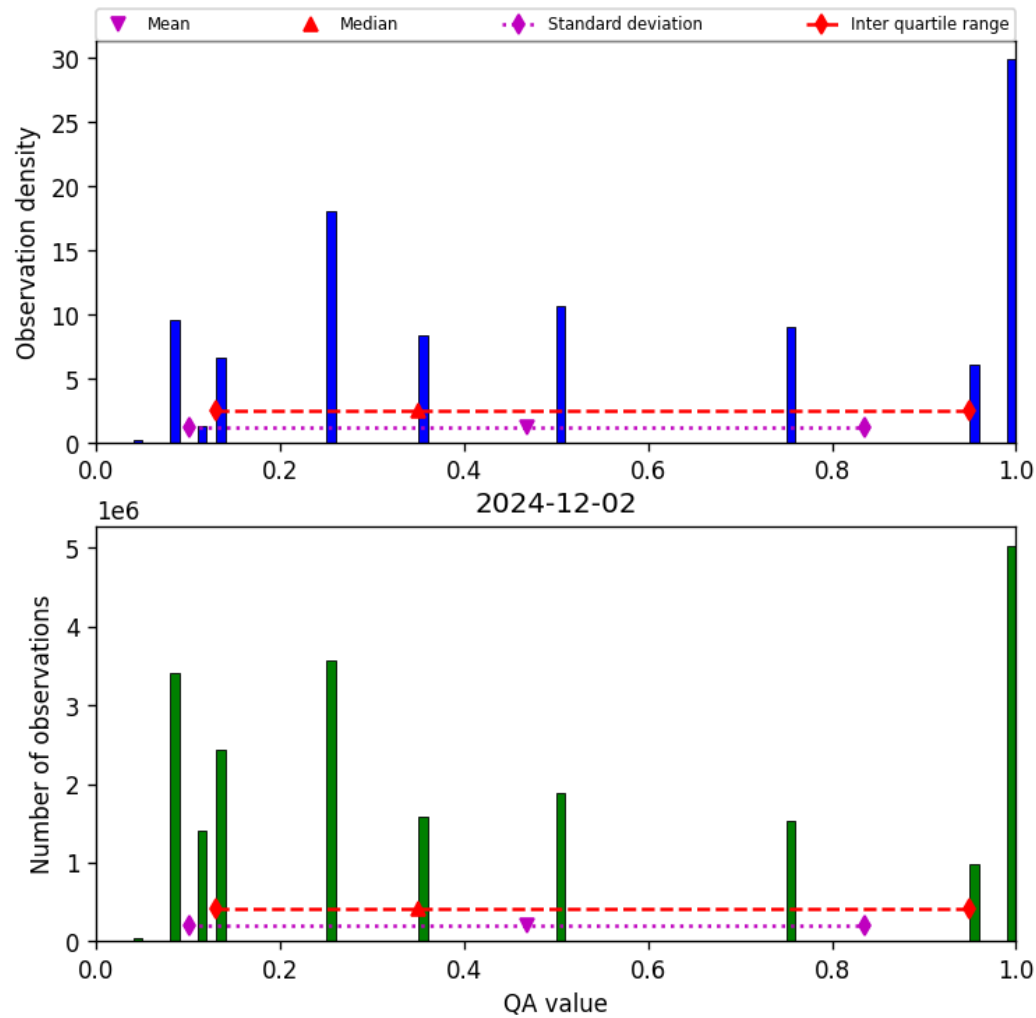
Figure 32: Histogram of “QA value” for 2024-12-02 to 2024-12-03
