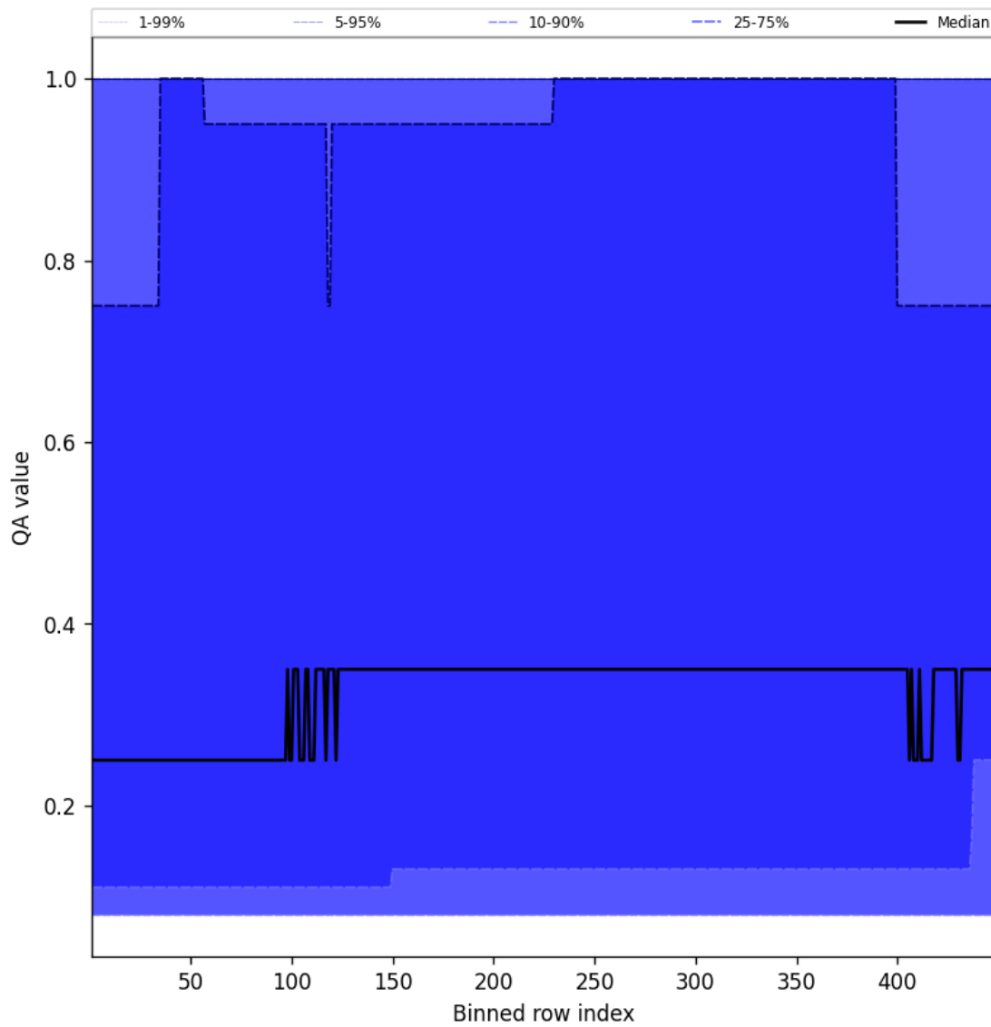
Figure 46: Along track statistics of “QA value” for 2024-12-02 to 2024-12-03
