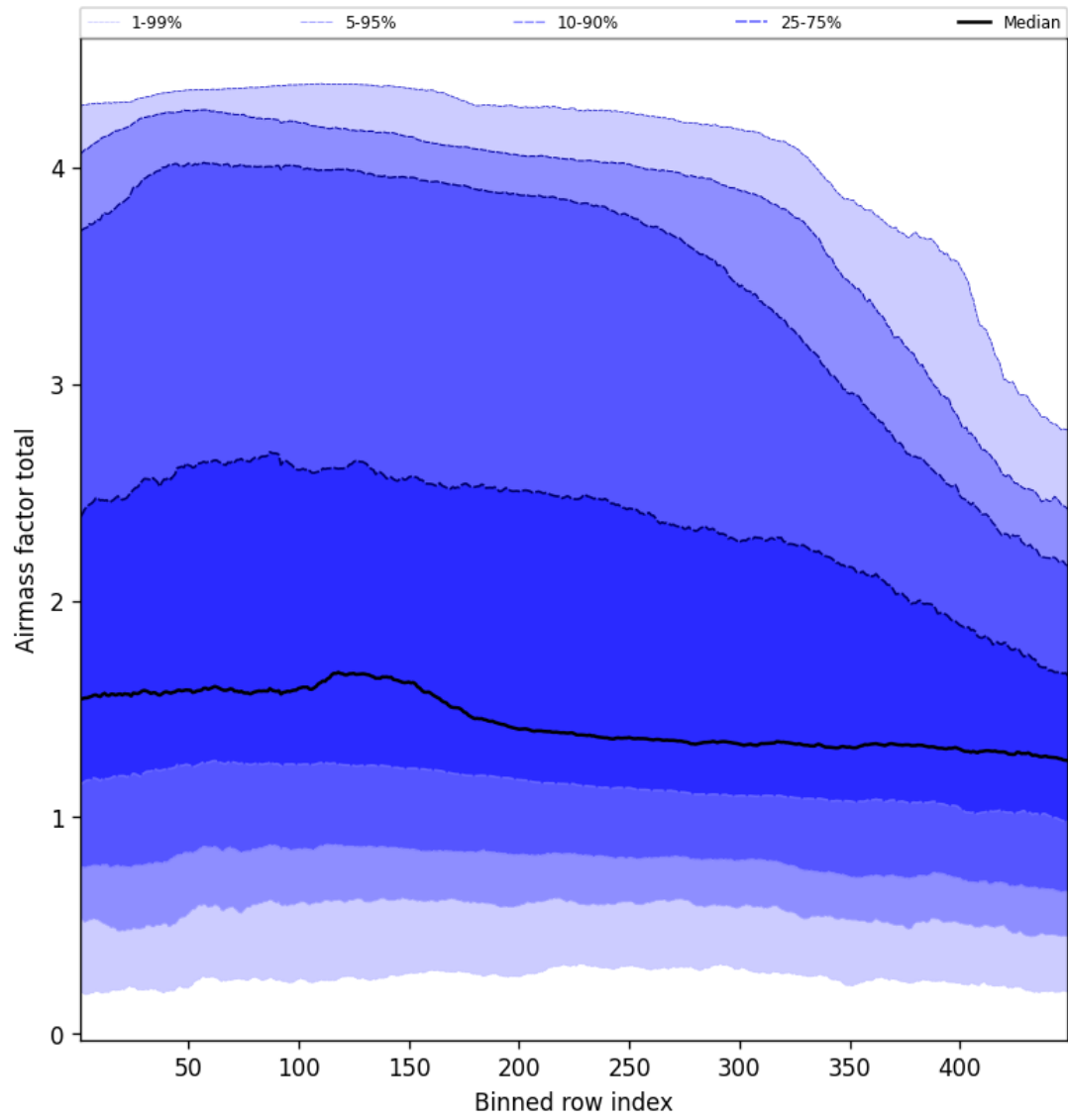
Figure 52: Along track statistics of “Airmass factor total” for 2024-12-02 to 2024-12-03
