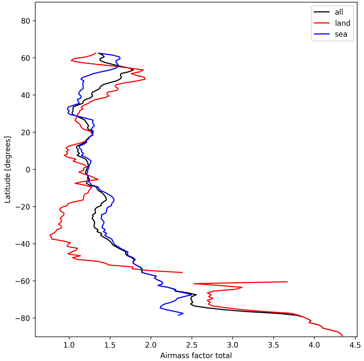
Figure 24: Zonal average of “Airmass factor total” for 2024-12-02 to 2024-12-03.
