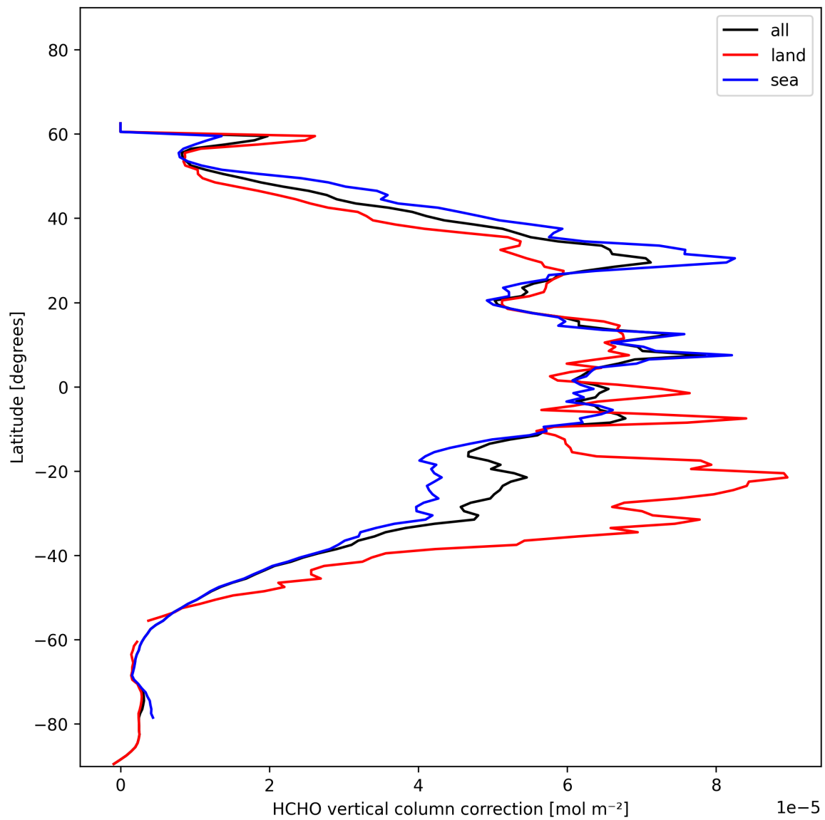
Figure 21: Zonal average of “HCHO vertical column correction” for 2024-12-02 to 2024-12-03.
