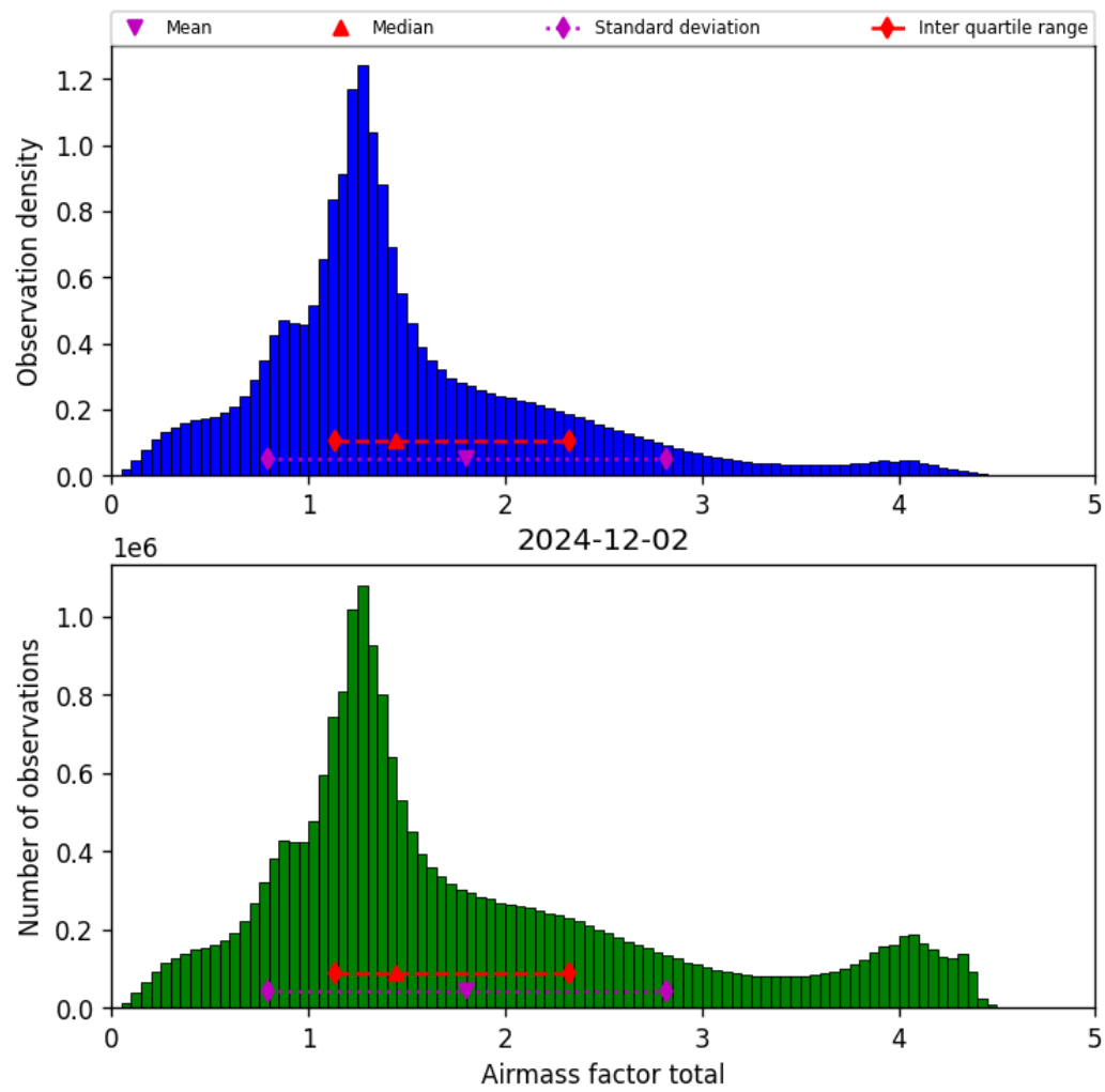
Figure 38: Histogram of “Airmass factor total” for 2024-12-02 to 2024-12-03
