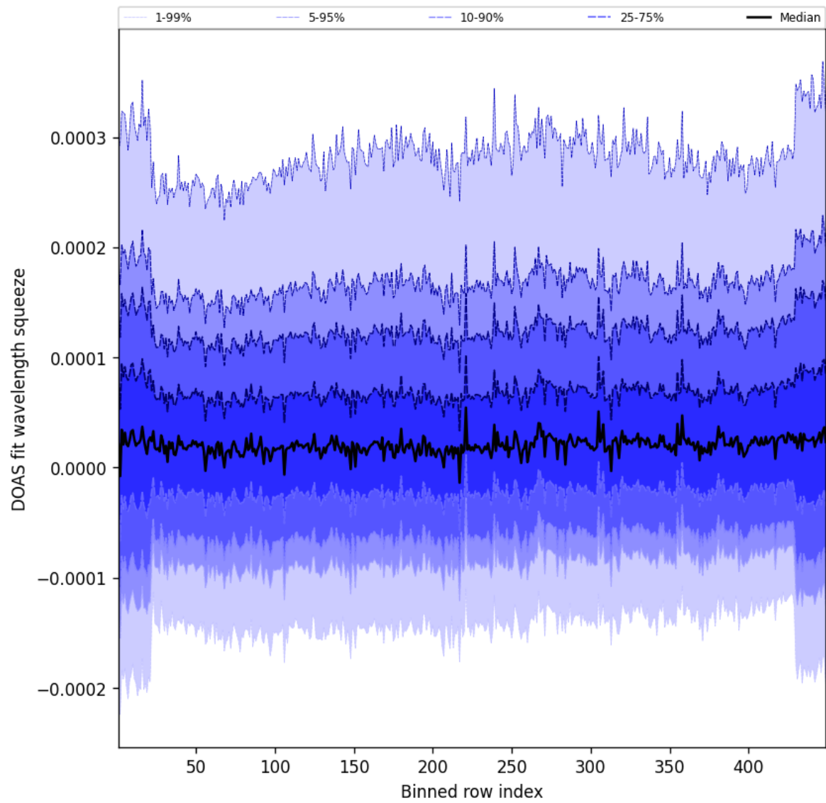
Figure 57: Along track statistics of “DOAS fit wavelength squeeze” for 2024-12-02 to 2024-12-03
