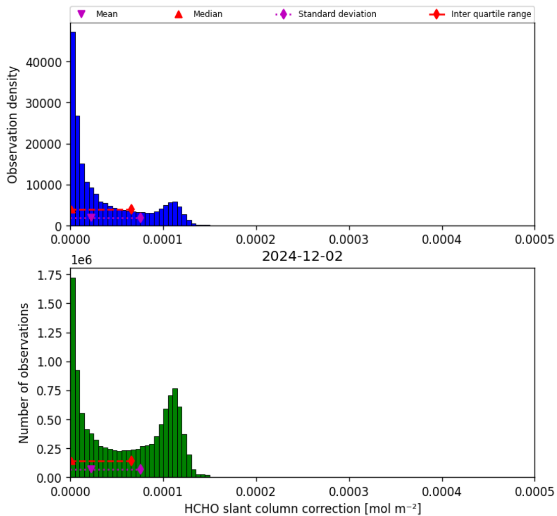
Figure 45: Histogram of “HCHO slant column correction” for 2024-12-02 to 2024-12-03
