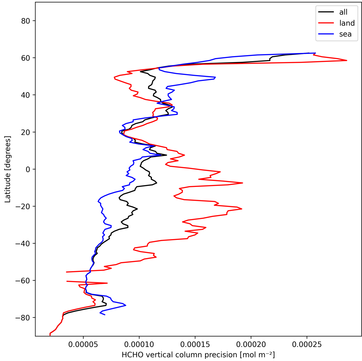
Figure 20: Zonal average of “HCHO vertical column precision” for 2024-12-02 to 2024-12-03.
