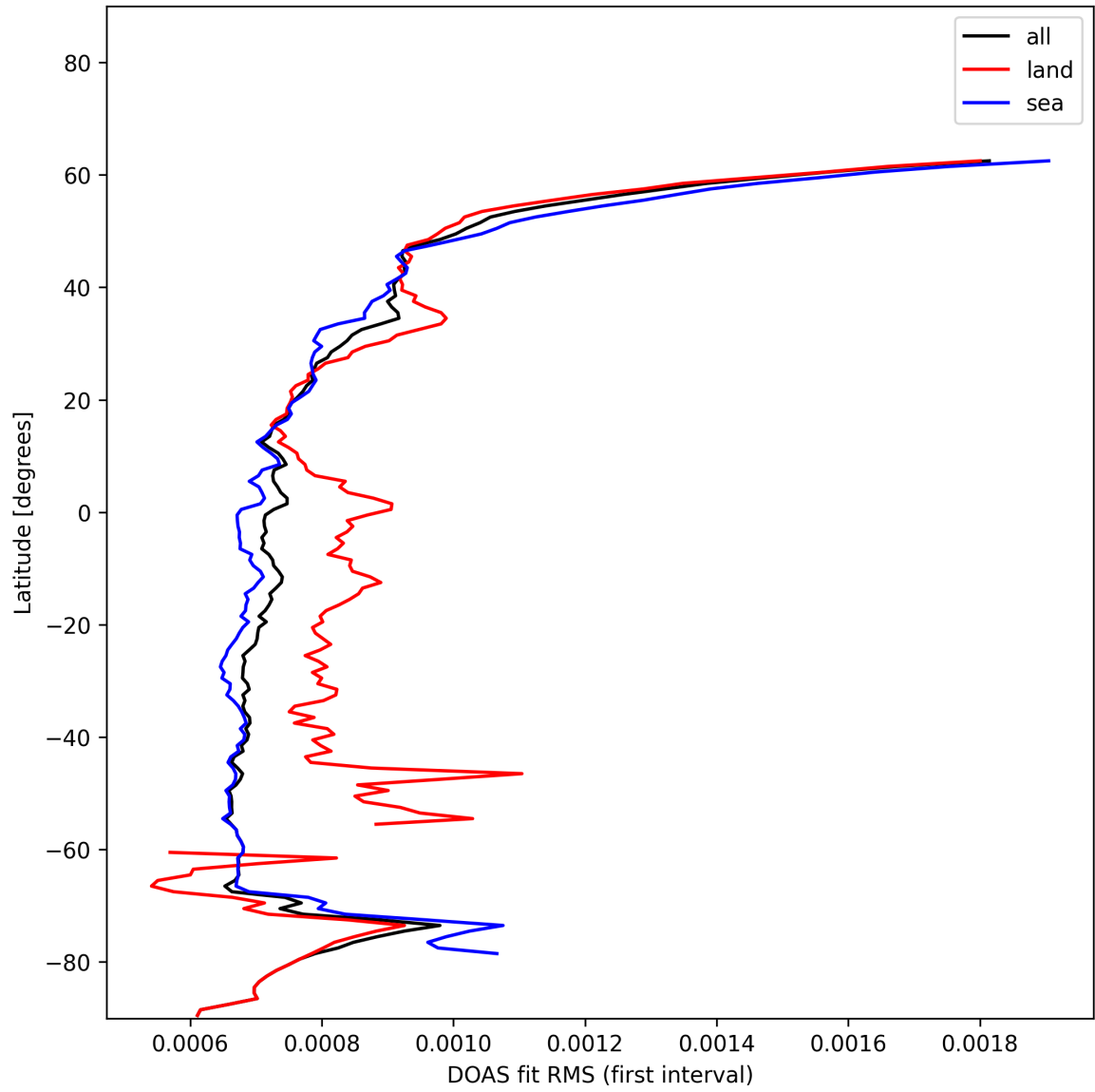
Figure 30: Zonal average of "DOAS fit RMS (first interval)" for 2024-12-02 to 2024-12-03.
