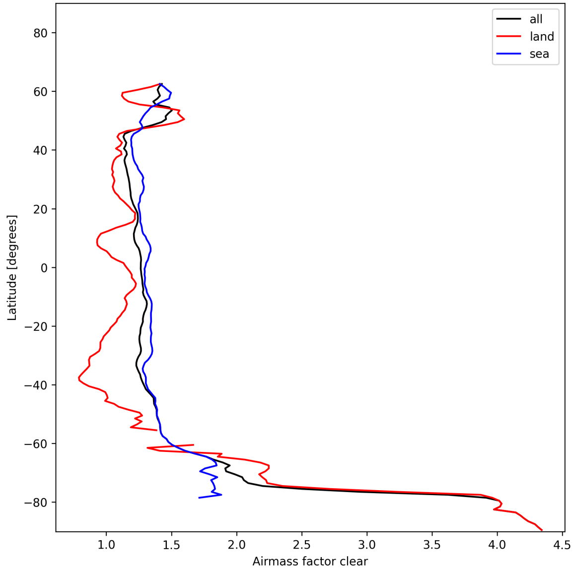
Figure 26: Zonal average of “Airmass factor clear” for 2024-12-02 to 2024-12-03.
