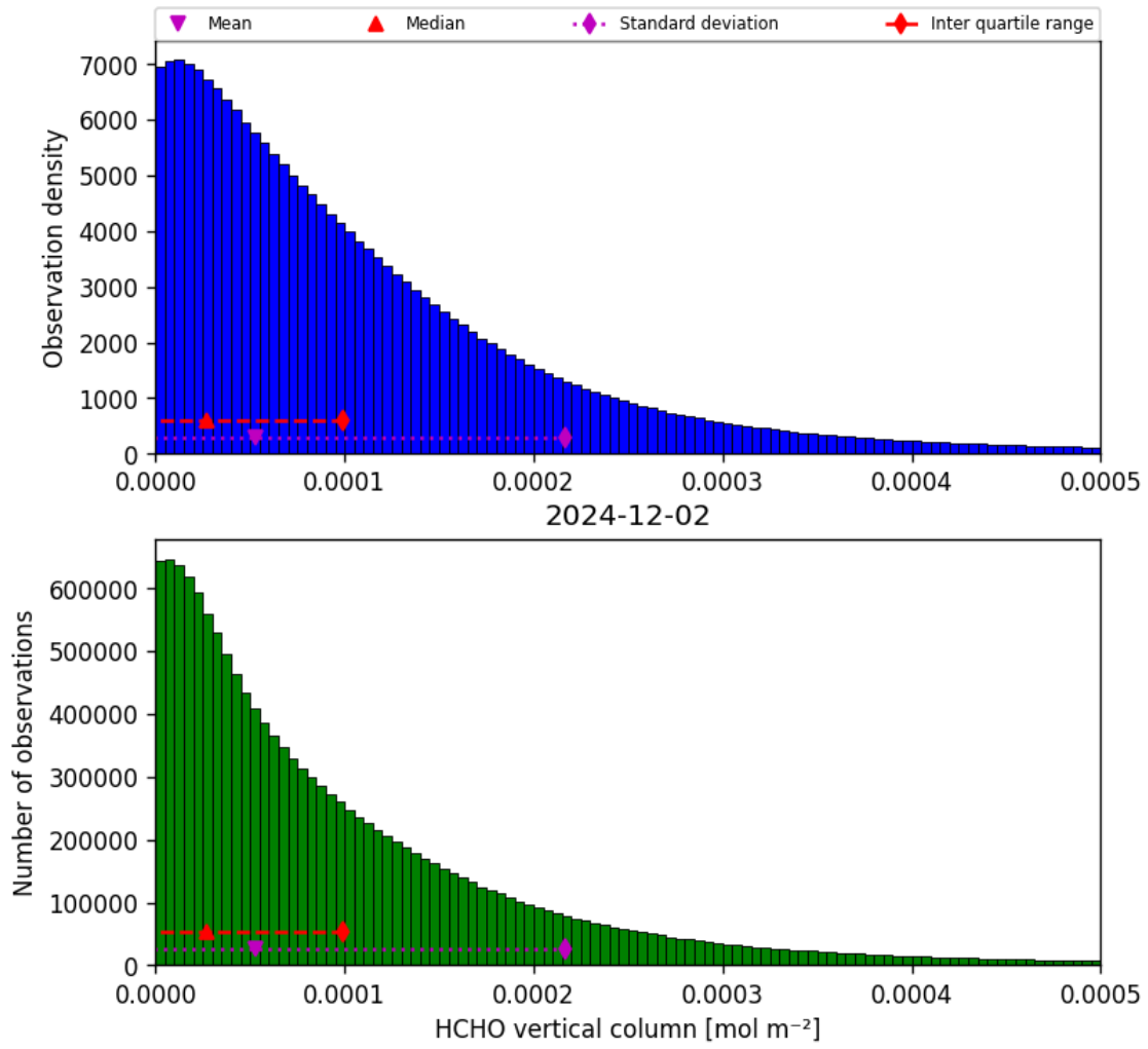
Figure 33: Histogram of “HCHO vertical column” for 2024-12-02 to 2024-12-03
