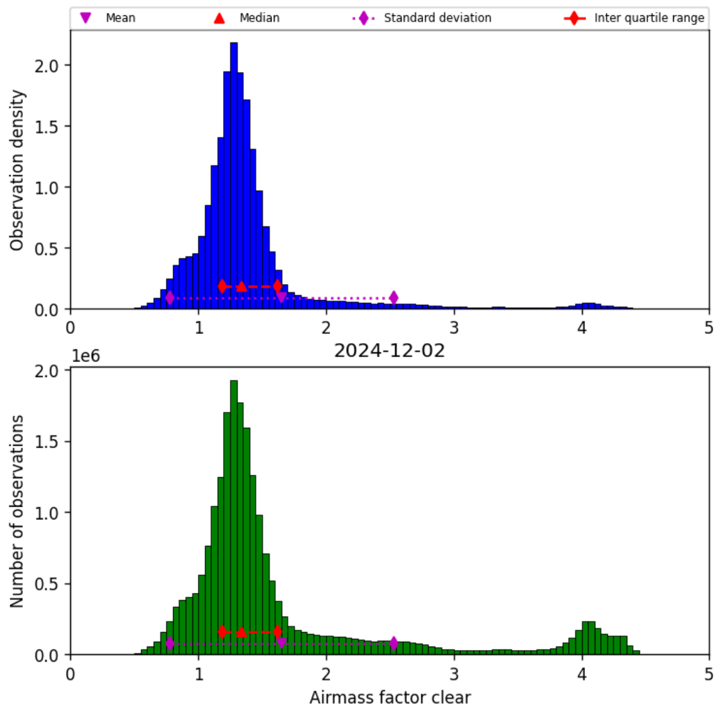
Figure 40: Histogram of “Airmass factor clear” for 2024-12-02 to 2024-12-03
