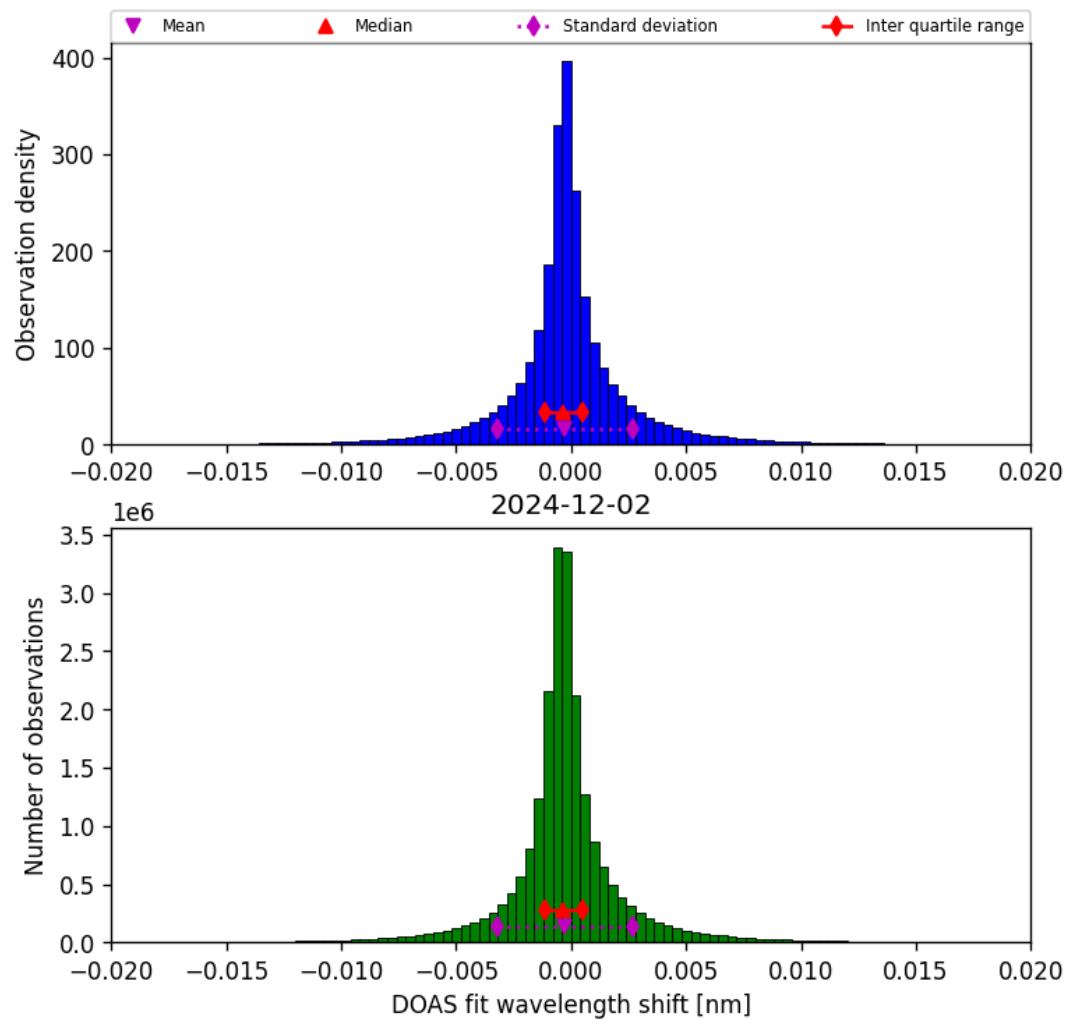
Figure 42: Histogram of “DOAS fit wavelength shift” for 2024-12-02 to 2024-12-03
