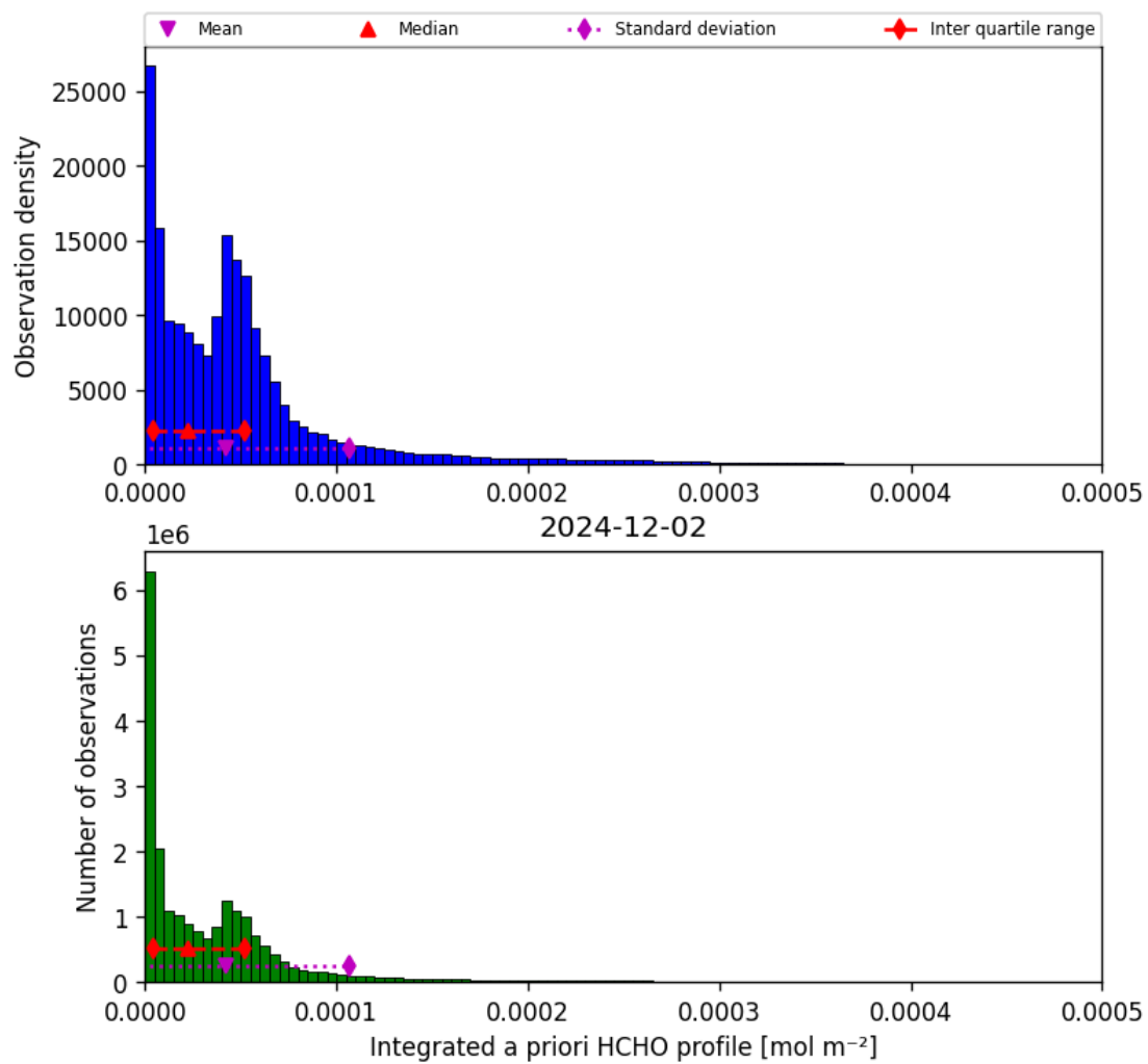
Figure 41: Histogram of “Integrated a priori HCHO profile” for 2024-12-02 to 2024-12-03
