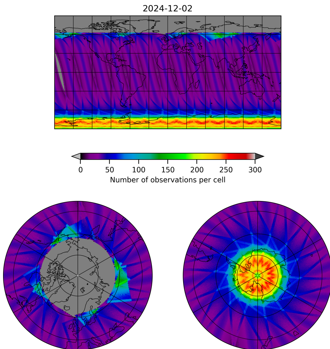
Figure 17: Map of the number of observations for 2024-12-02 to 2024-12-03
