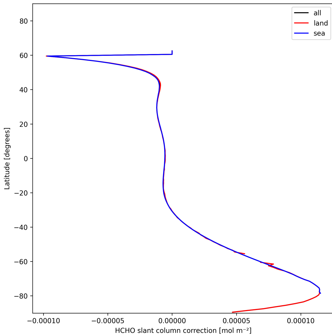
Figure 31: Zonal average of “HCHO slant column correction” for 2024-12-02 to 2024-12-03.
