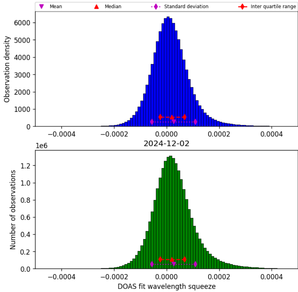
Figure 43: Histogram of “DOAS fit wavelength squeeze” for 2024-12-02 to 2024-12-03
