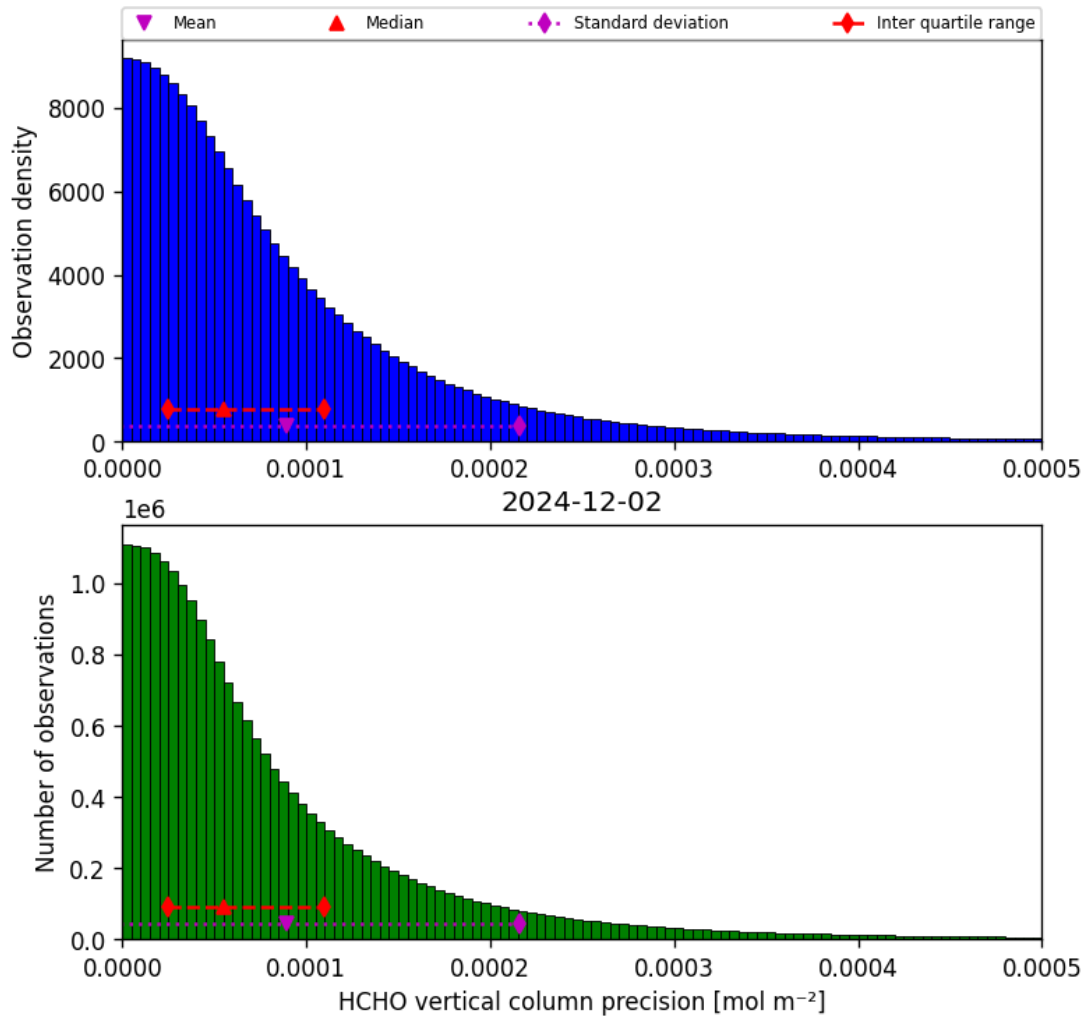
Figure 34: Histogram of “HCHO vertical column precision” for 2024-12-02 to 2024-12-03
