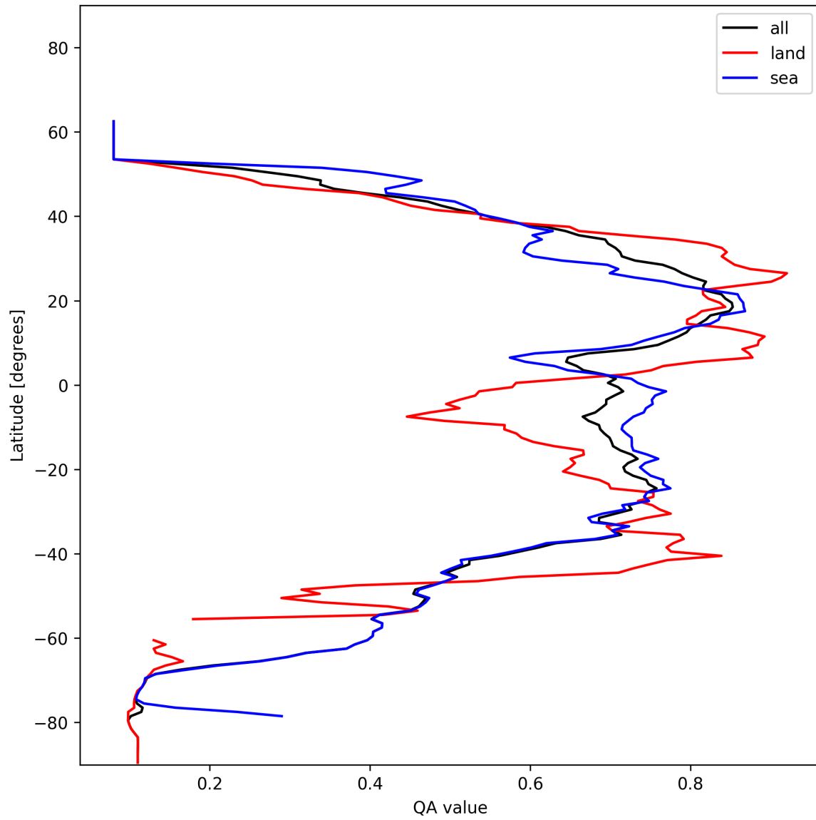
Figure 18: Zonal average of “QA value” for 2024-12-02 to 2024-12-03.
