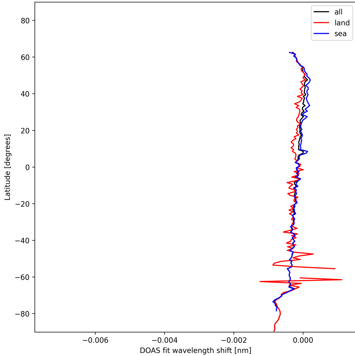
Figure 28: Zonal average of "DOAS fit wavelength shift" for 2024-12-02 to 2024-12-03.
