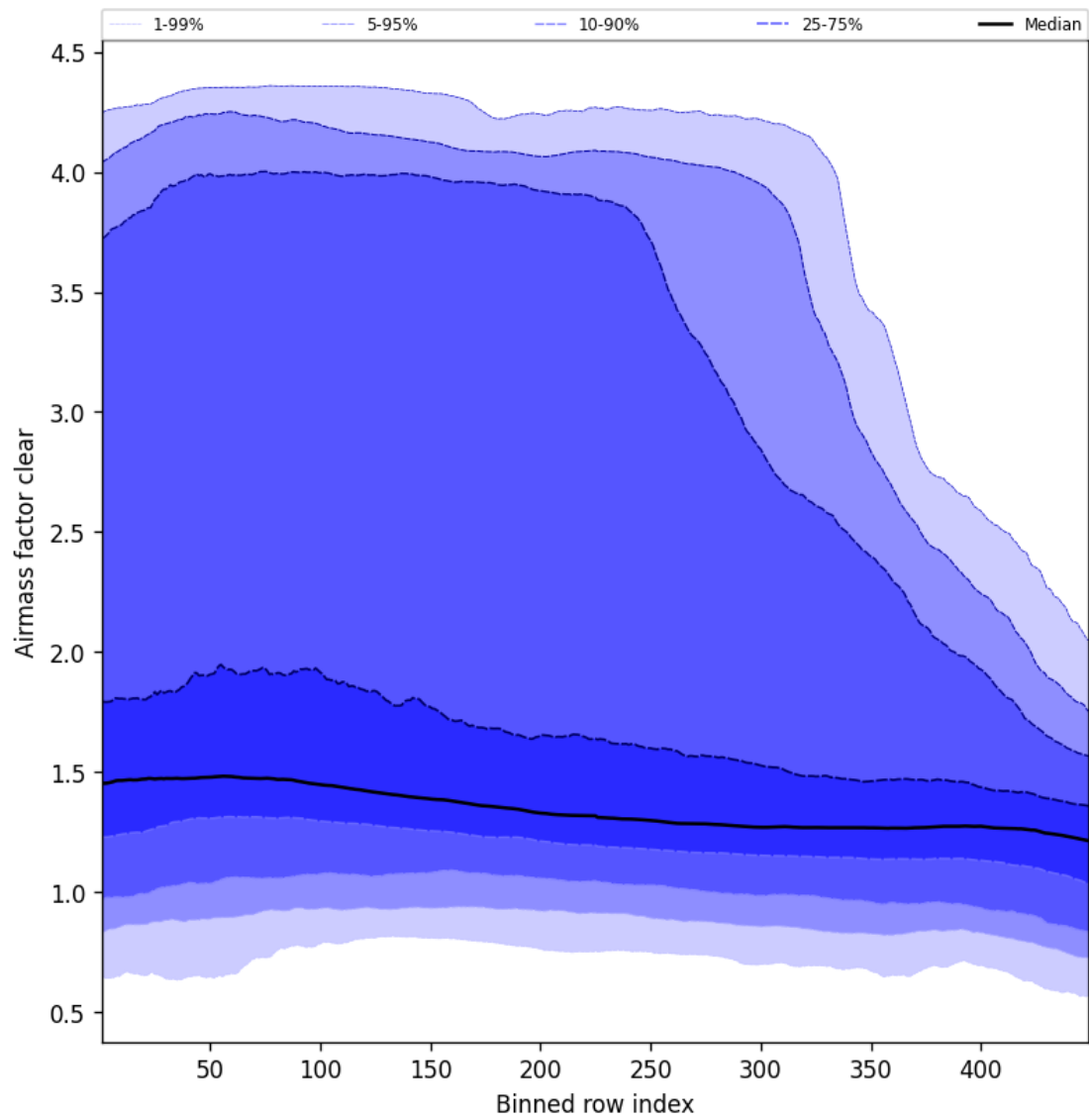
Figure 54: Along track statistics of “Airmass factor clear” for 2024-12-02 to 2024-12-03
