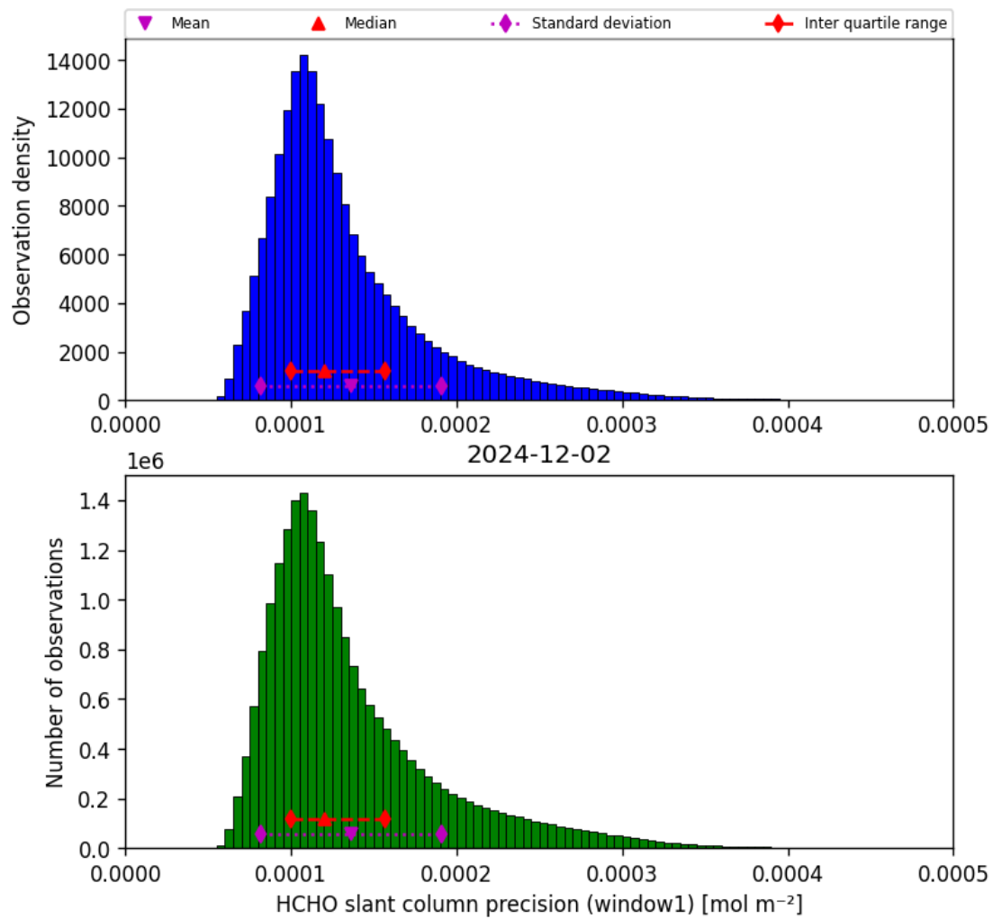
Figure 37: Histogram of “HCHO slant column precision (window1)” for 2024-12-02 to 2024-12-03
