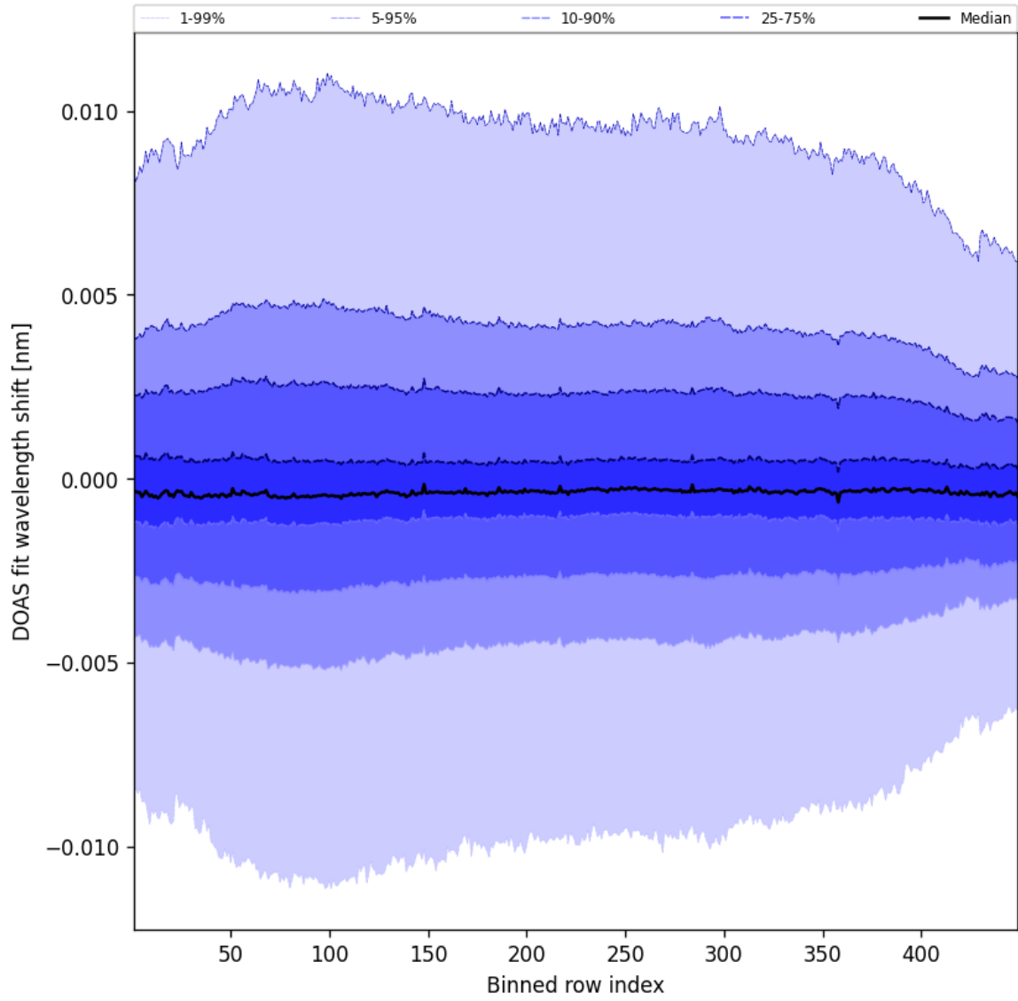
Figure 56: Along track statistics of “DOAS fit wavelength shift” for 2024-12-02 to 2024-12-03
