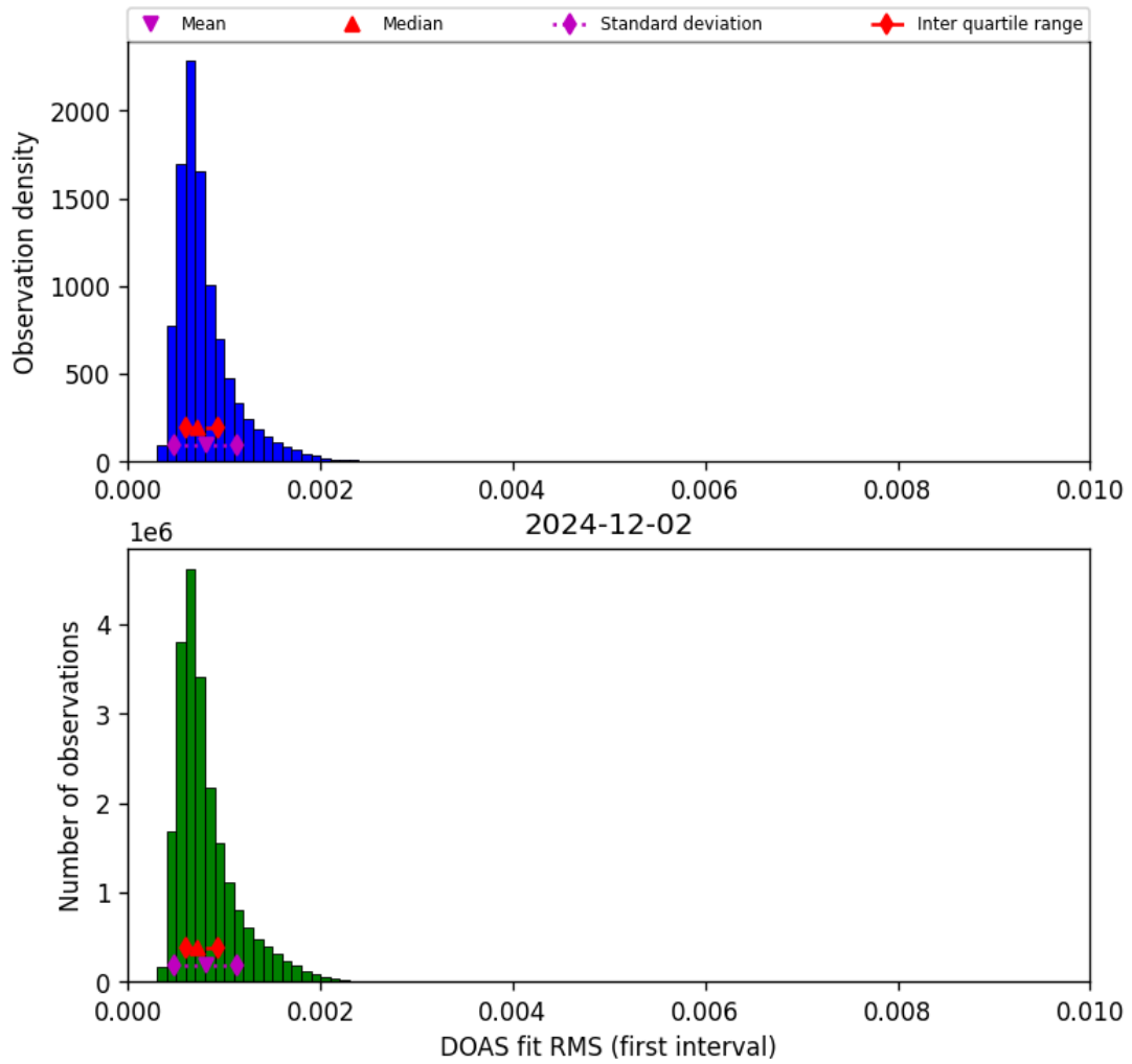
Figure 44: Histogram of “DOAS fit RMS (first interval)” for 2024-12-02 to 2024-12-03
