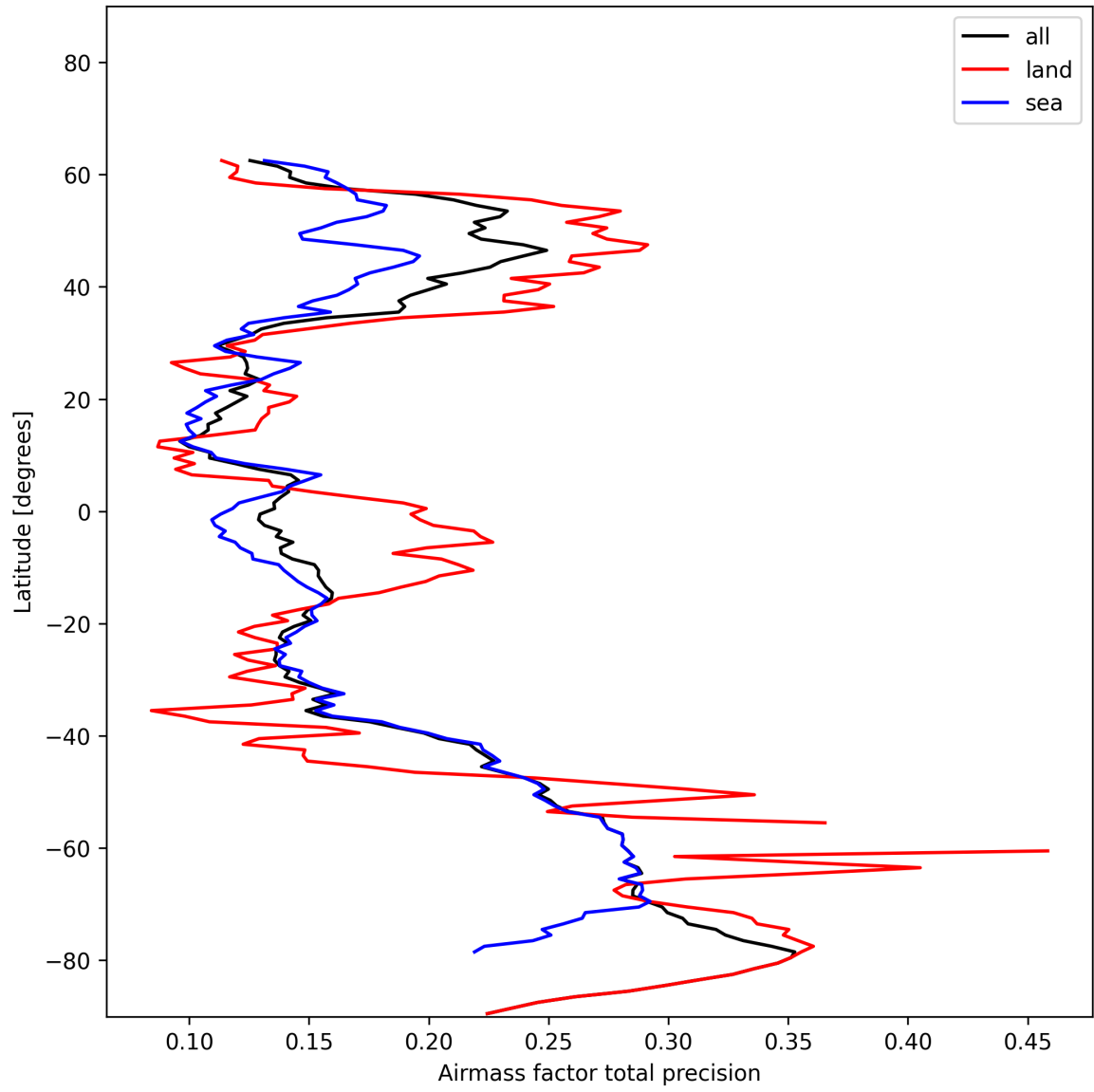
Figure 25: Zonal average of “Airmass factor total precision” for 2024-12-02 to 2024-12-03.
