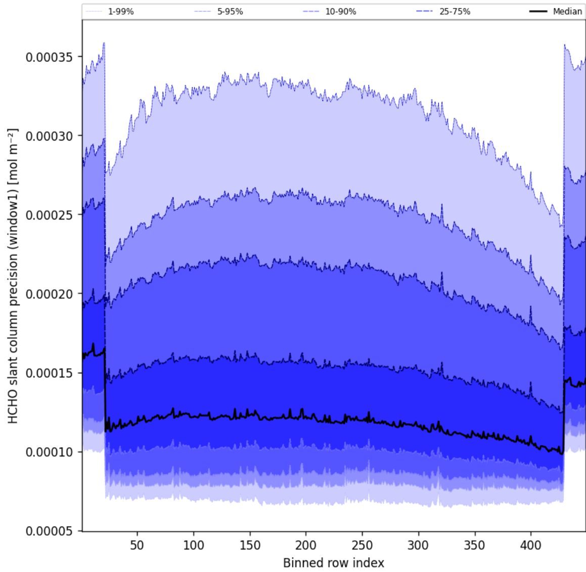
Figure 51: Along track statistics of "HCHO slant column precision (window1)" for 2024-12-02 to 2024-12-03
