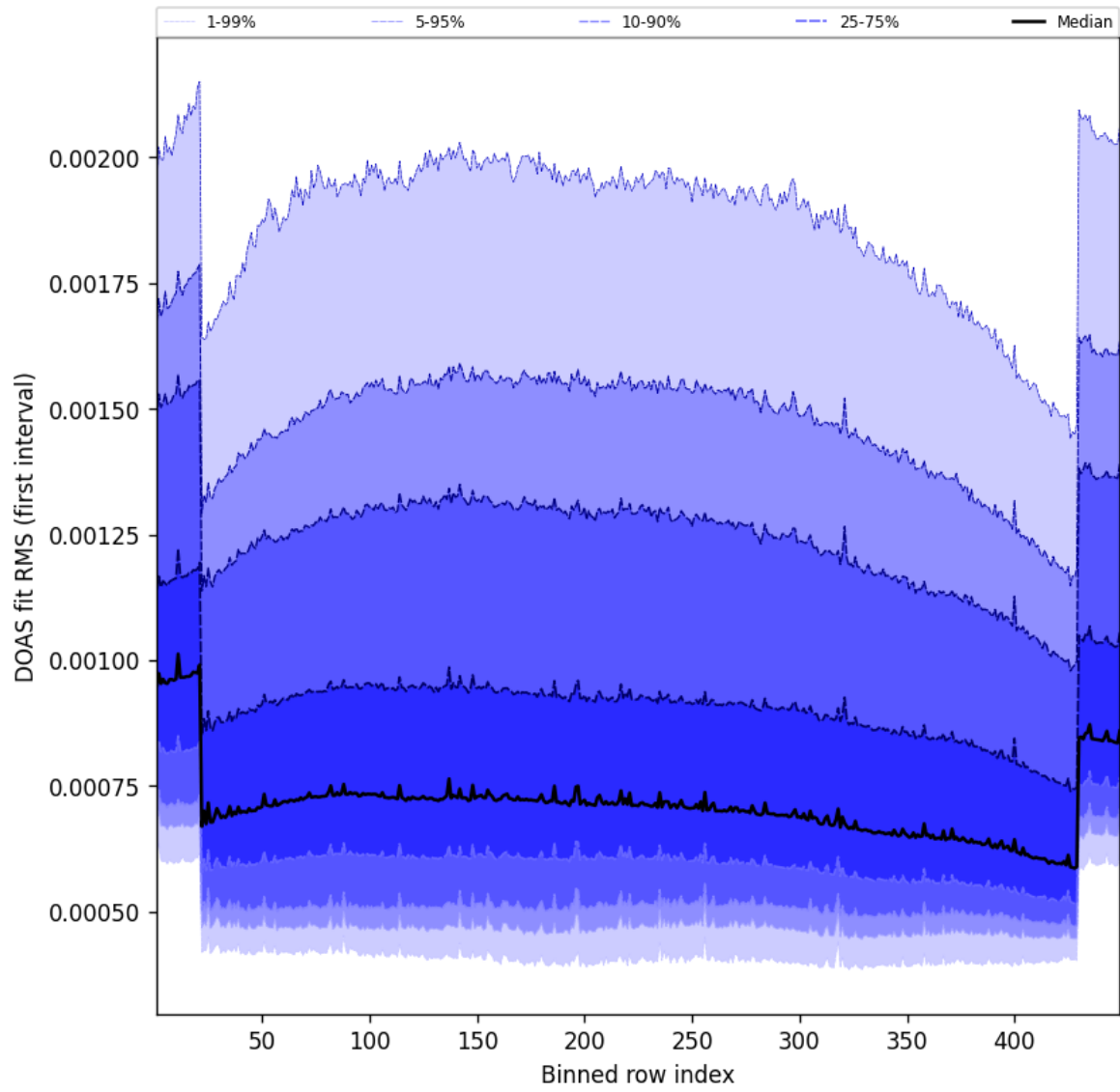
Figure 58: Along track statistics of “DOAS fit RMS (first interval)” for 2024-12-02 to 2024-12-03
