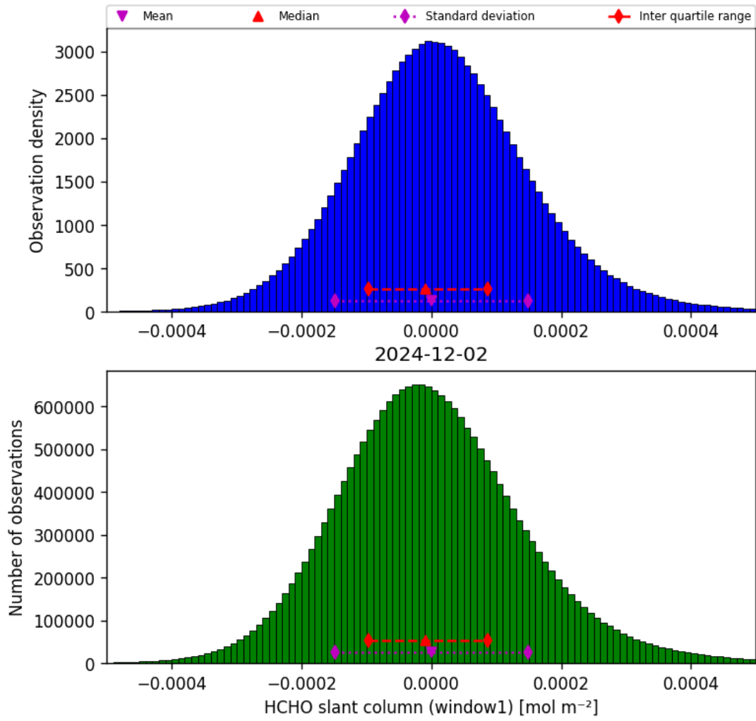
Figure 36: Histogram of “HCHO slant column (window1)” for 2024-12-02 to 2024-12-03
