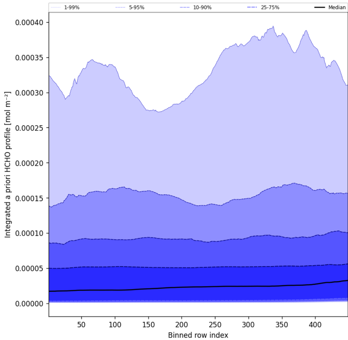
Figure 55: Along track statistics of "Integrated a priori HCHO profile" for 2024-12-02 to 2024-12-03
