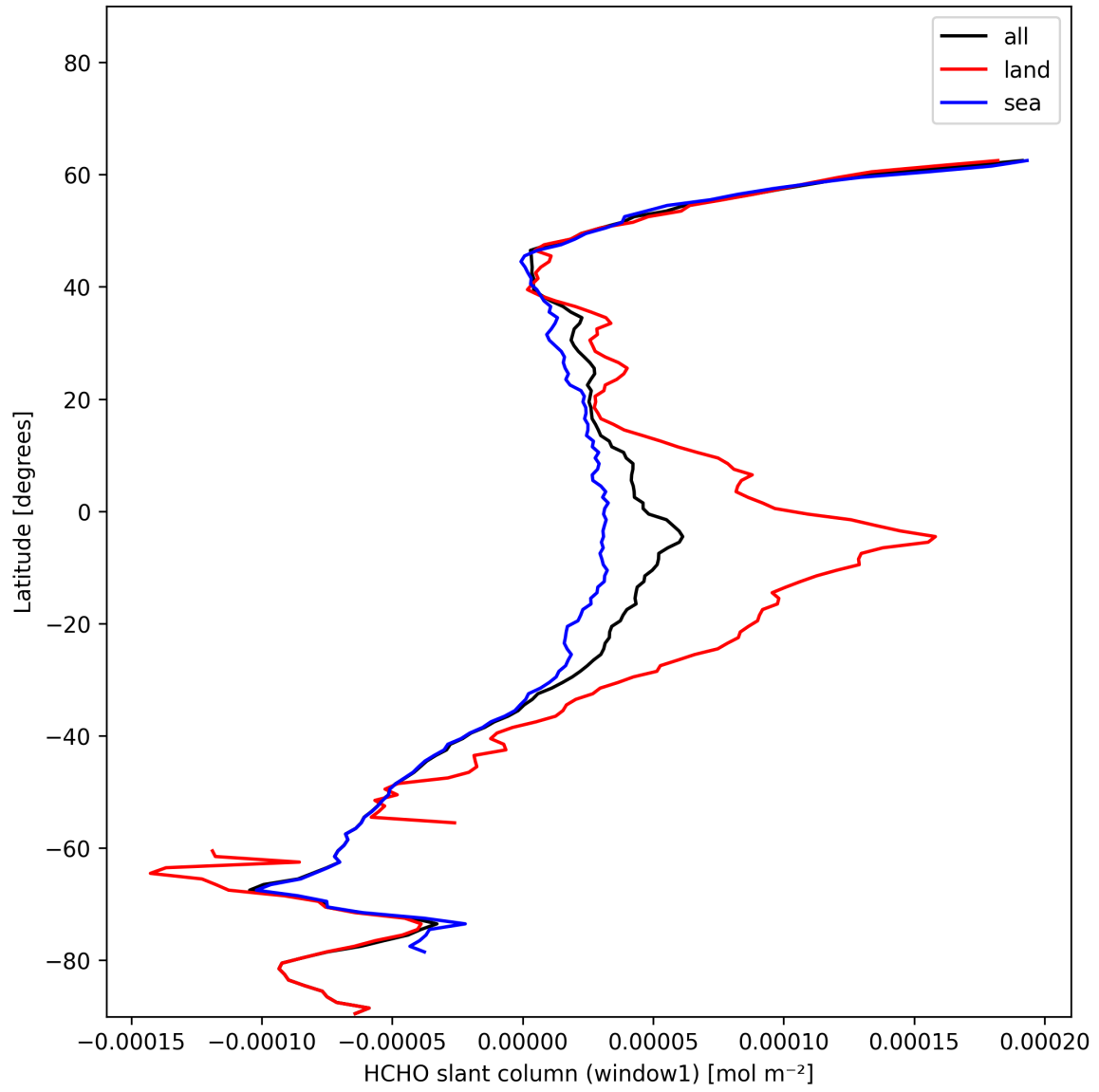
Figure 22: Zonal average of “HCHO slant column (window1)” for 2024-12-02 to 2024-12-03.
