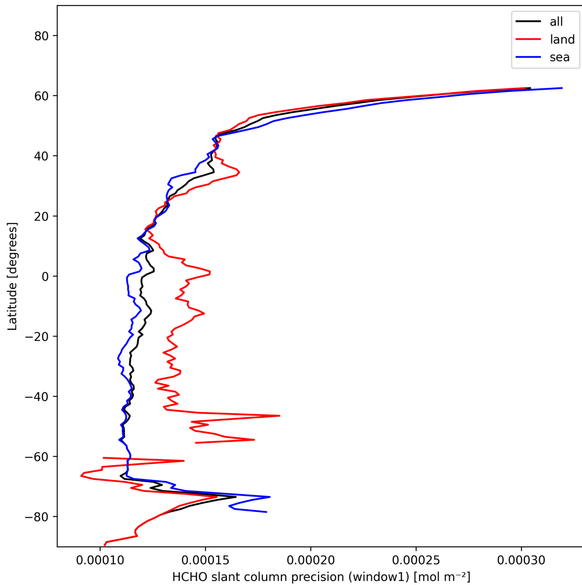
Figure 23: Zonal average of “HCHO slant column precision (window1)” for 2024-12-02 to 2024-12-03.
