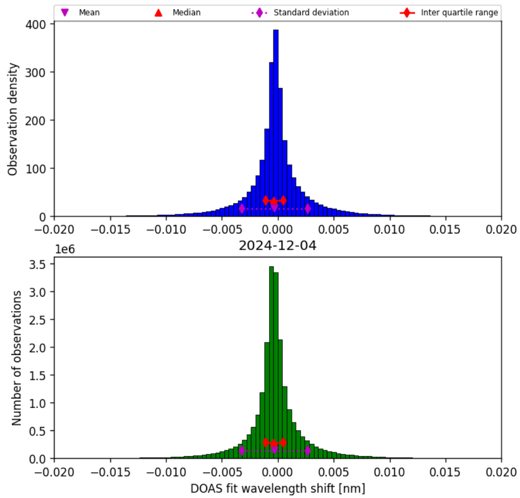
Figure 42: Histogram of “DOAS fit wavelength shift” for 2024-12-04 to 2024-12-04
