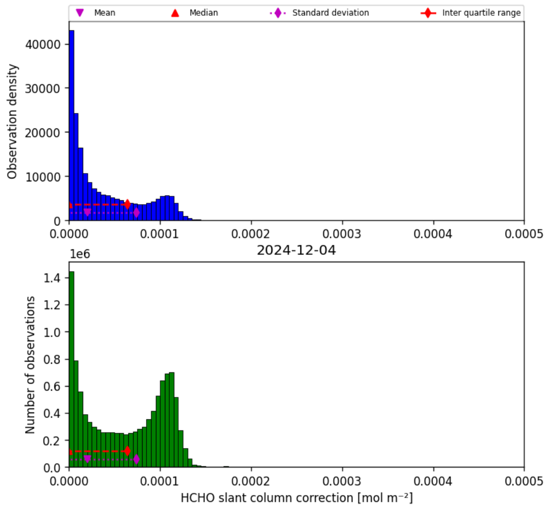
Figure 45: Histogram of “HCHO slant column correction” for 2024-12-04 to 2024-12-04
