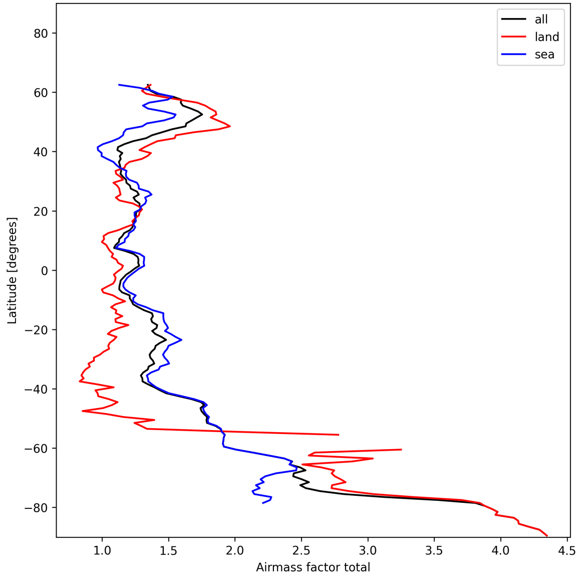
Figure 24: Zonal average of “Airmass factor total” for 2024-12-04 to 2024-12-04.
