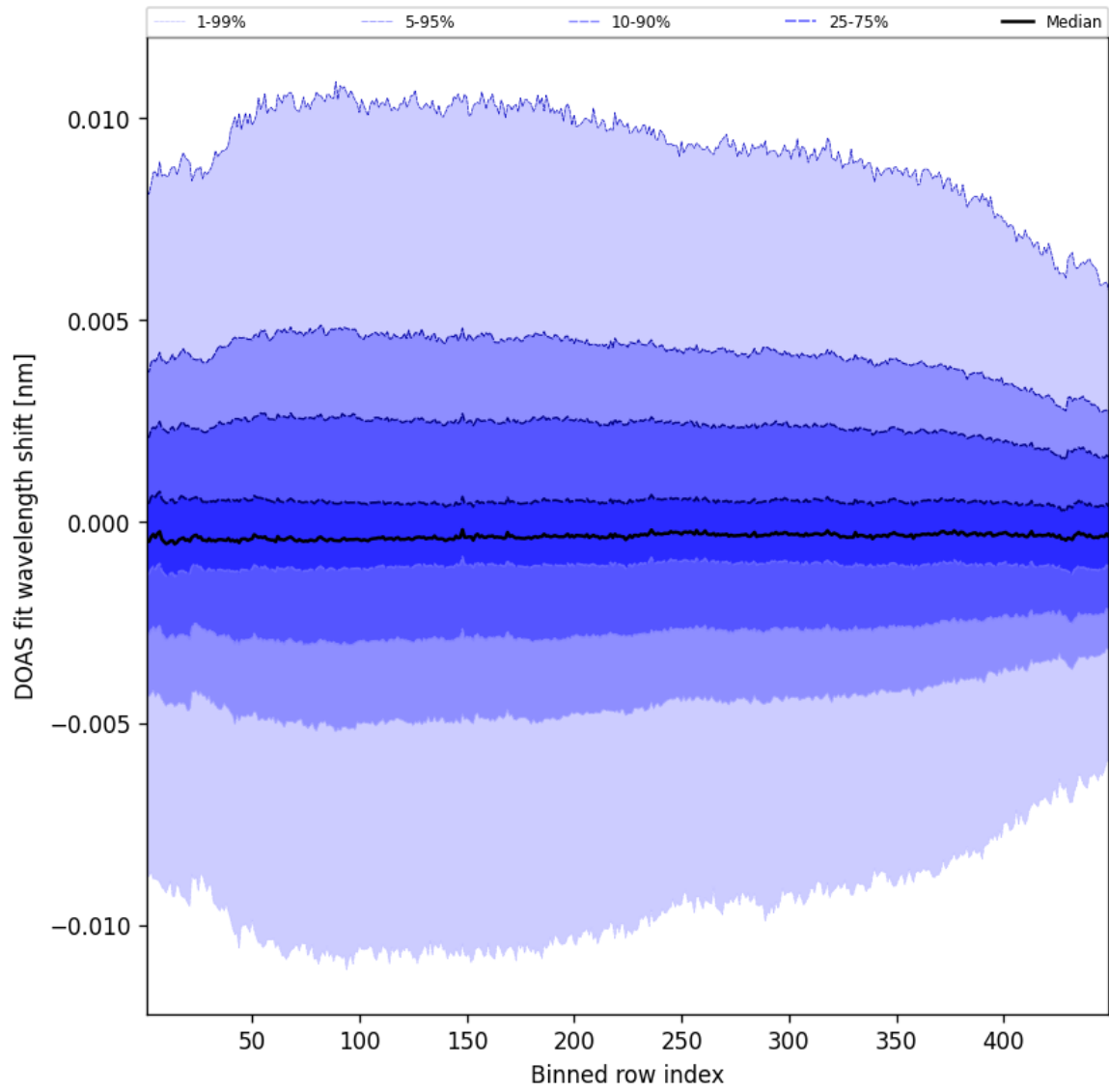
Figure 56: Along track statistics of “DOAS fit wavelength shift” for 2024-12-04 to 2024-12-04
