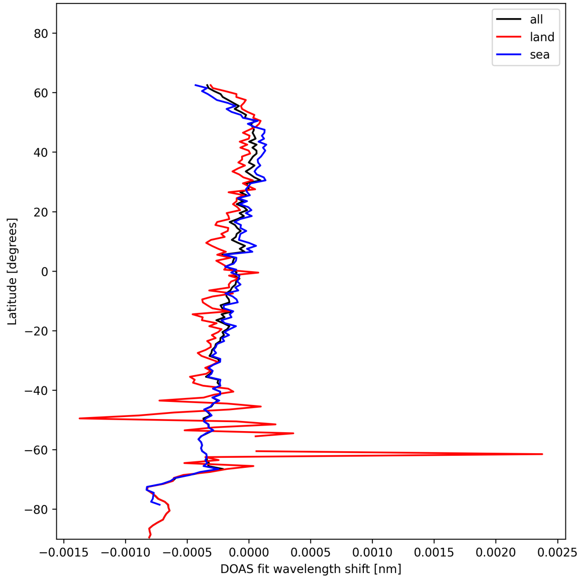
Figure 28: Zonal average of "DOAS fit wavelength shift" for 2024-12-04 to 2024-12-04.
