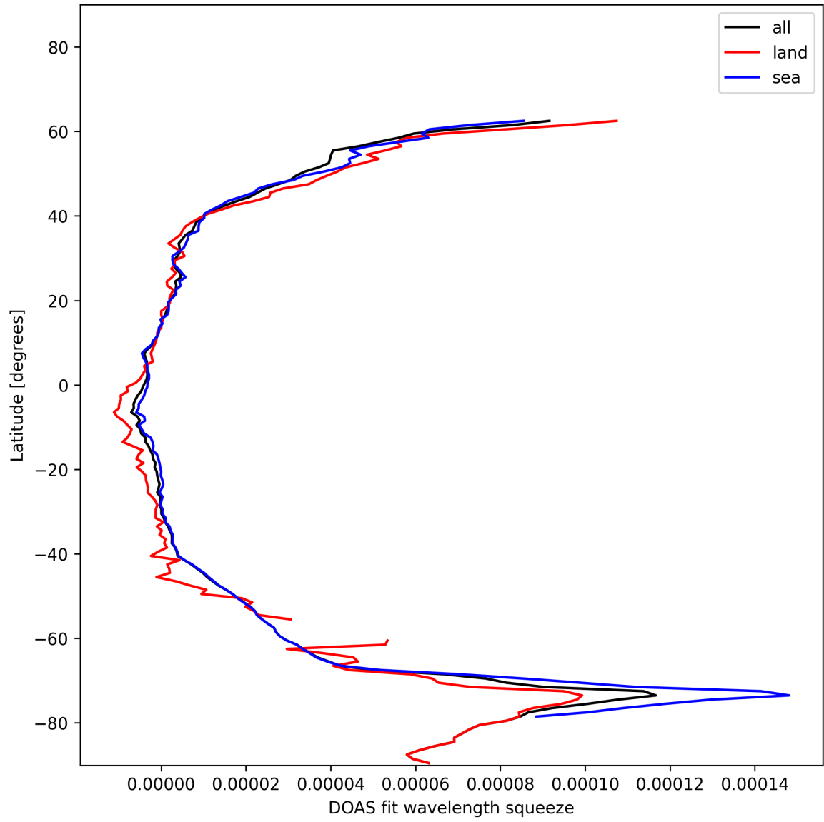
Figure 29: Zonal average of “DOAS fit wavelength squeeze” for 2024-12-04 to 2024-12-04.
