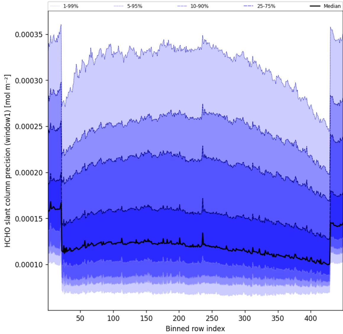
Figure 51: Along track statistics of “HCHO slant column precision (window1)” for 2024-12-04 to 2024-12-04
