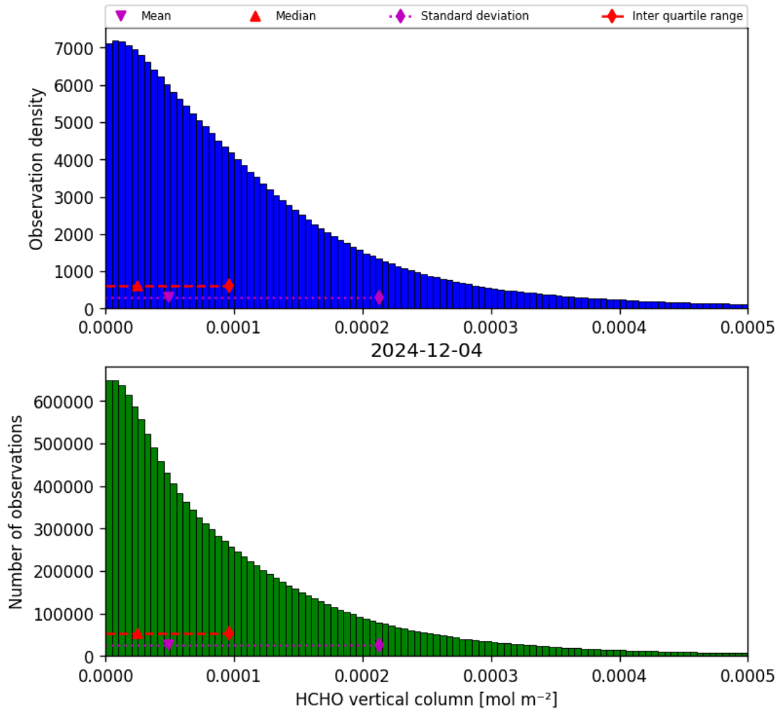
Figure 33: Histogram of “HCHO vertical column” for 2024-12-04 to 2024-12-04
