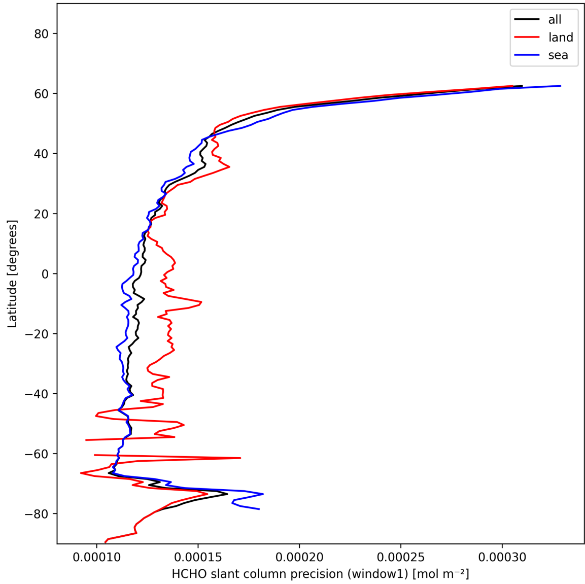
Figure 23: Zonal average of “HCHO slant column precision (window1)” for 2024-12-04 to 2024-12-04.
