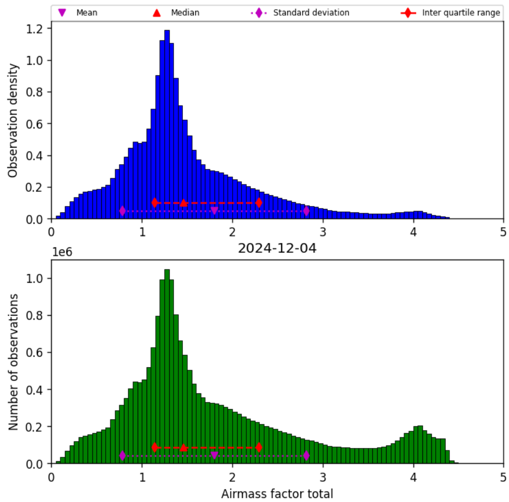
Figure 38: Histogram of “Airmass factor total” for 2024-12-04 to 2024-12-04
