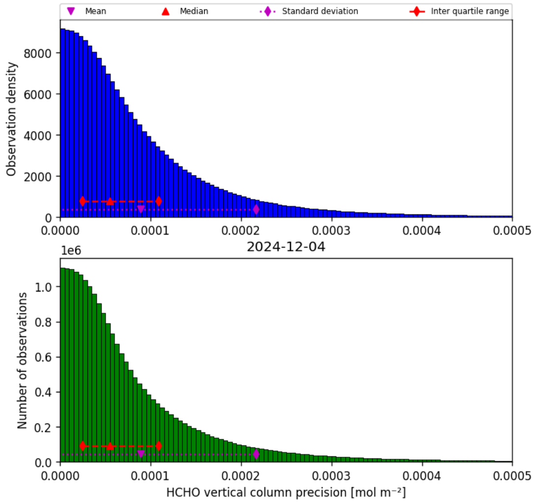
Figure 34: Histogram of “HCHO vertical column precision” for 2024-12-04 to 2024-12-04
