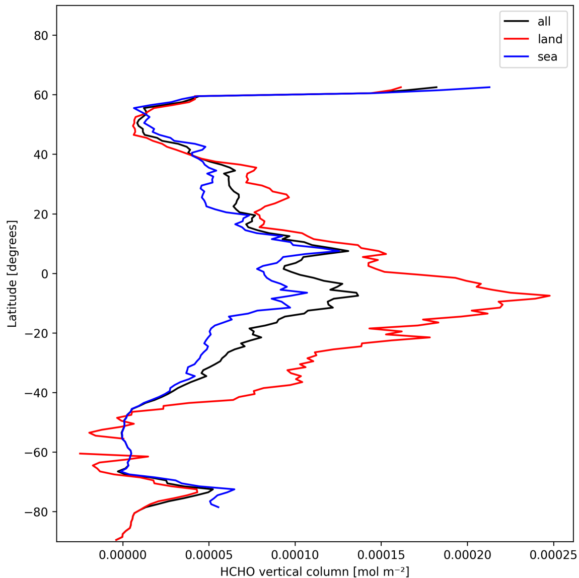
Figure 19: Zonal average of “HCHO vertical column” for 2024-12-04 to 2024-12-04.
