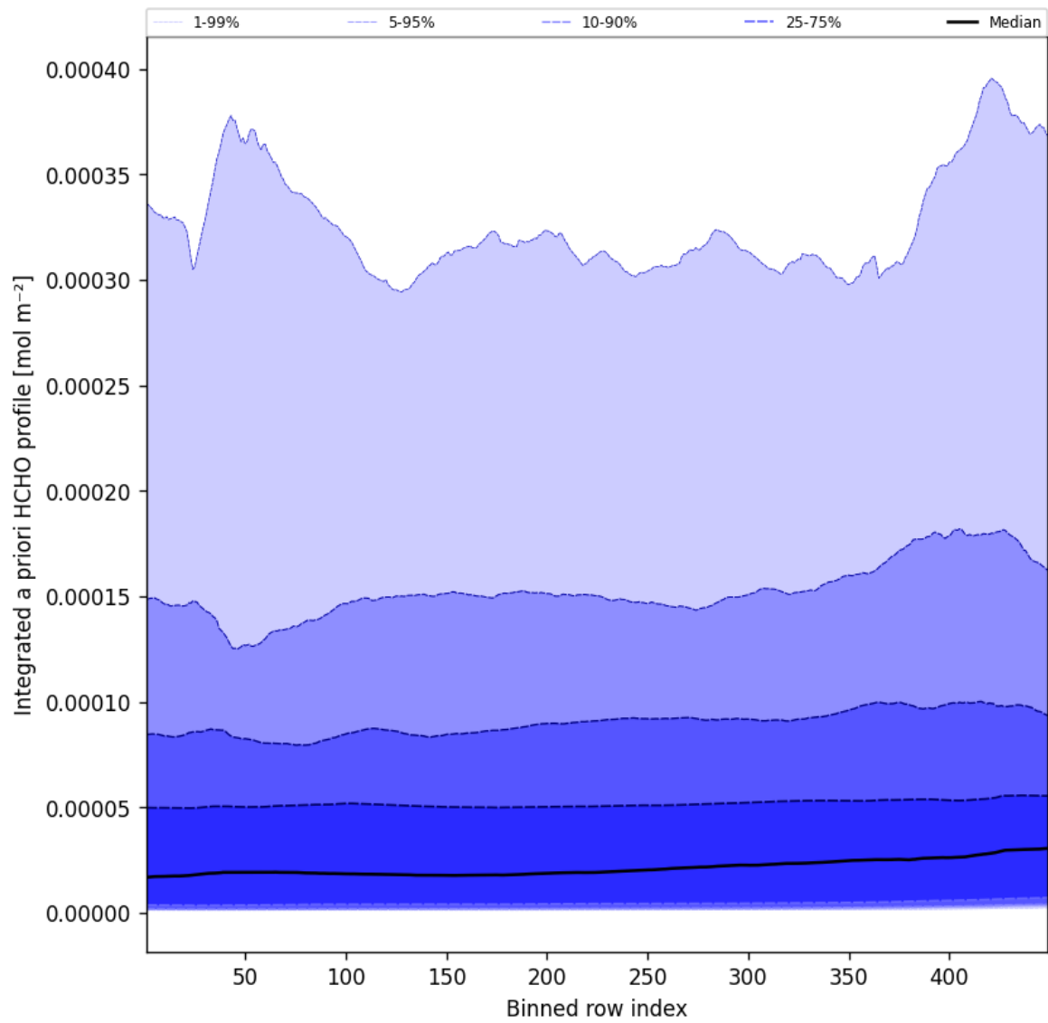
Figure 55: Along track statistics of "Integrated a priori HCHO profile" for 2024-12-04 to 2024-12-04
