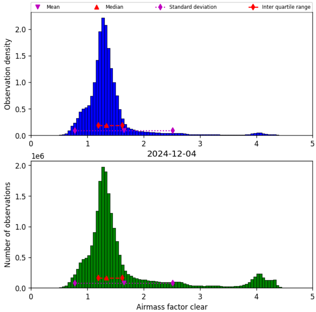
Figure 40: Histogram of “Airmass factor clear” for 2024-12-04 to 2024-12-04
