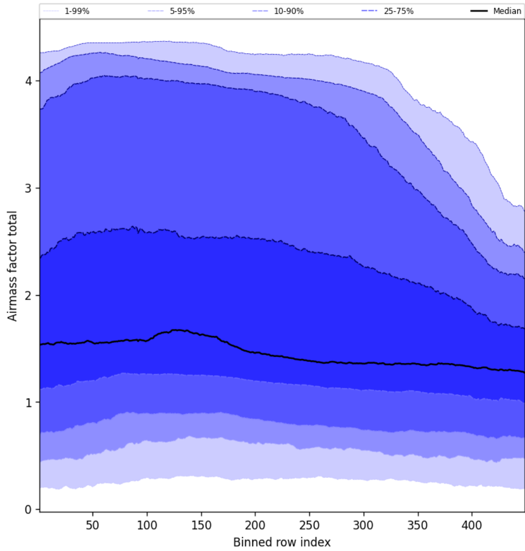
Figure 52: Along track statistics of “Airmass factor total” for 2024-12-04 to 2024-12-04
