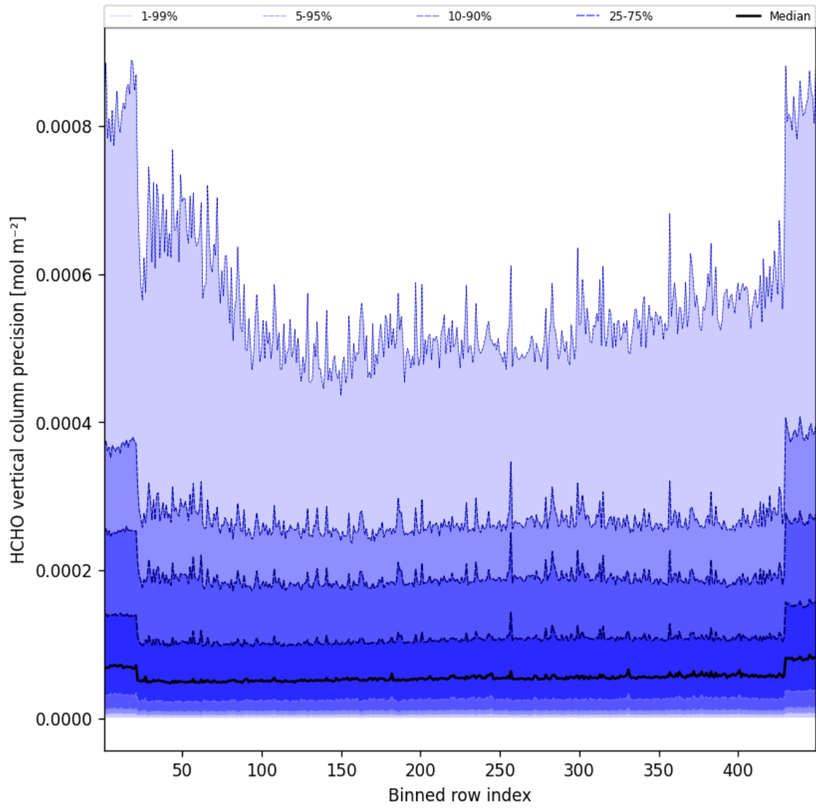
Figure 48: Along track statistics of "HCHO vertical column precision" for 2024-12-04 to 2024-12-04
