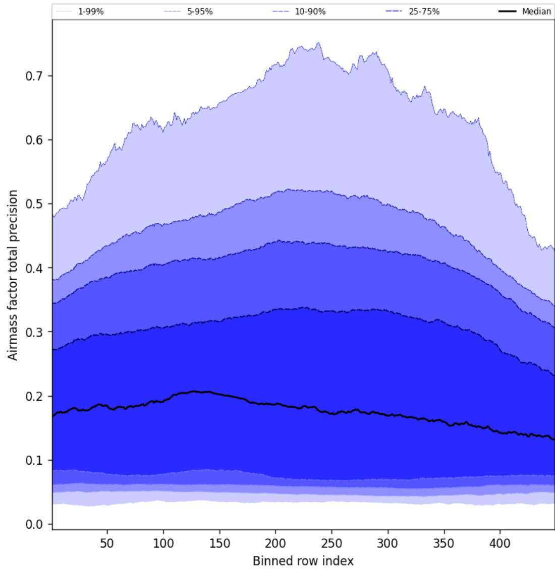
Figure 53: Along track statistics of “Airmass factor total precision” for 2024-12-04 to 2024-12-04
