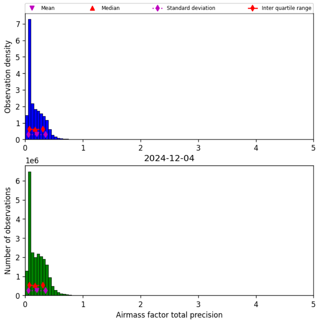
Figure 39: Histogram of “Airmass factor total precision” for 2024-12-04 to 2024-12-04
