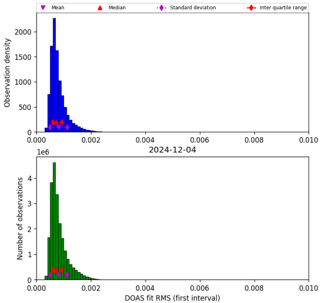
Figure 44: Histogram of “DOAS fit RMS (first interval)” for 2024-12-04 to 2024-12-04
