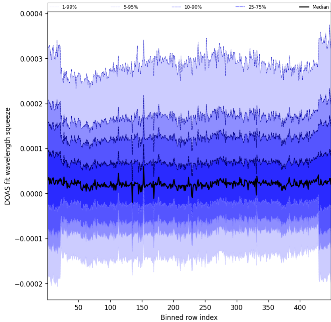
Figure 57: Along track statistics of “DOAS fit wavelength squeeze” for 2024-12-04 to 2024-12-04
