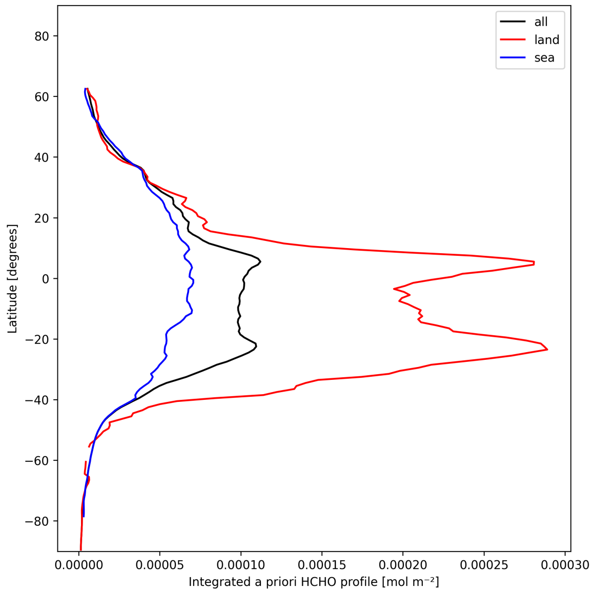
Figure 27: Zonal average of “Integrated a priori HCHO profile” for 2024-12-04 to 2024-12-04.
