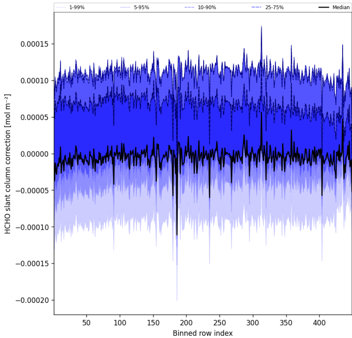
Figure 59: Along track statistics of “HCHO slant column correction” for 2024-12-04 to 2024-12-04
