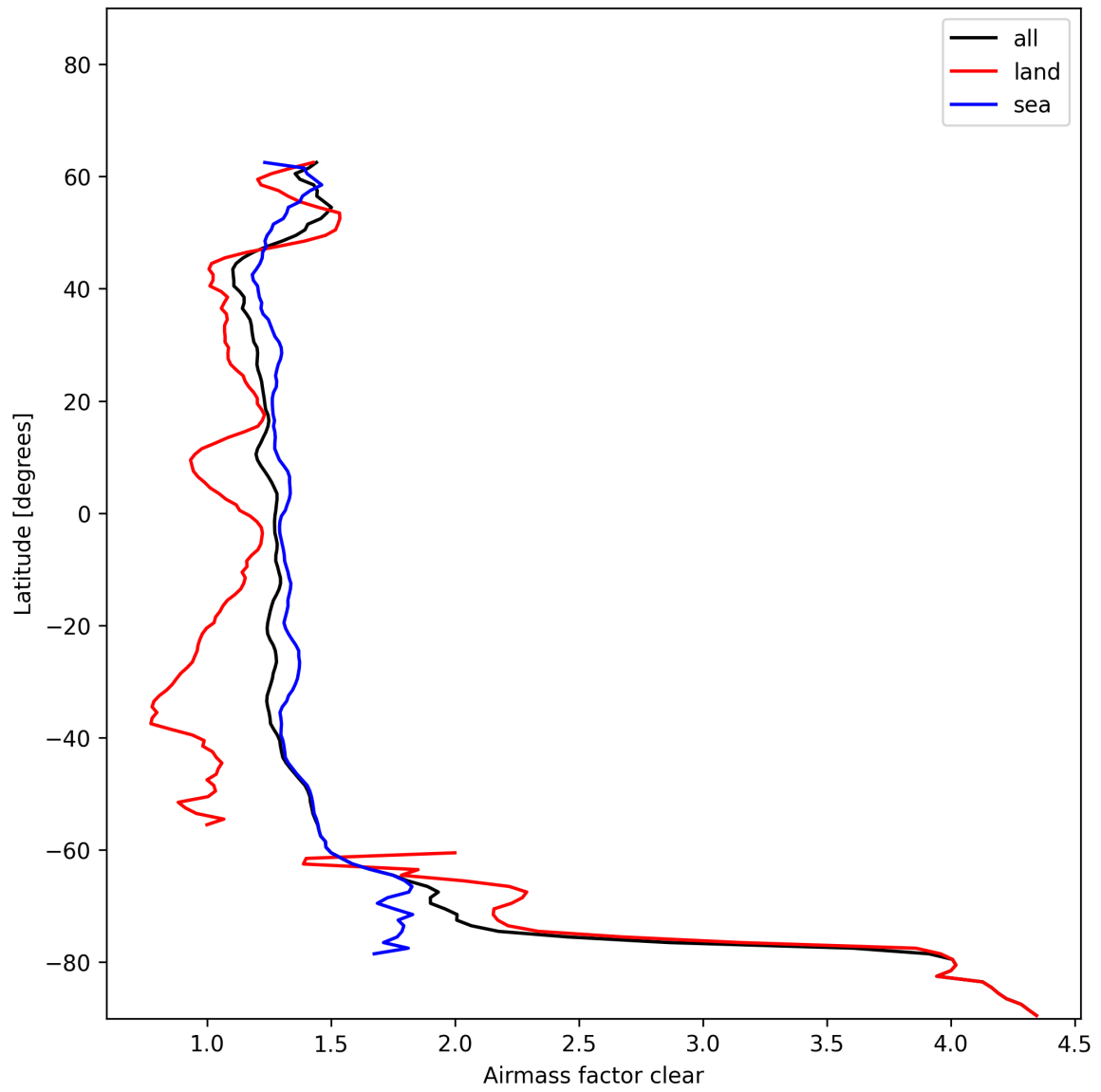
Figure 26: Zonal average of “Airmass factor clear” for 2024-12-04 to 2024-12-04.
