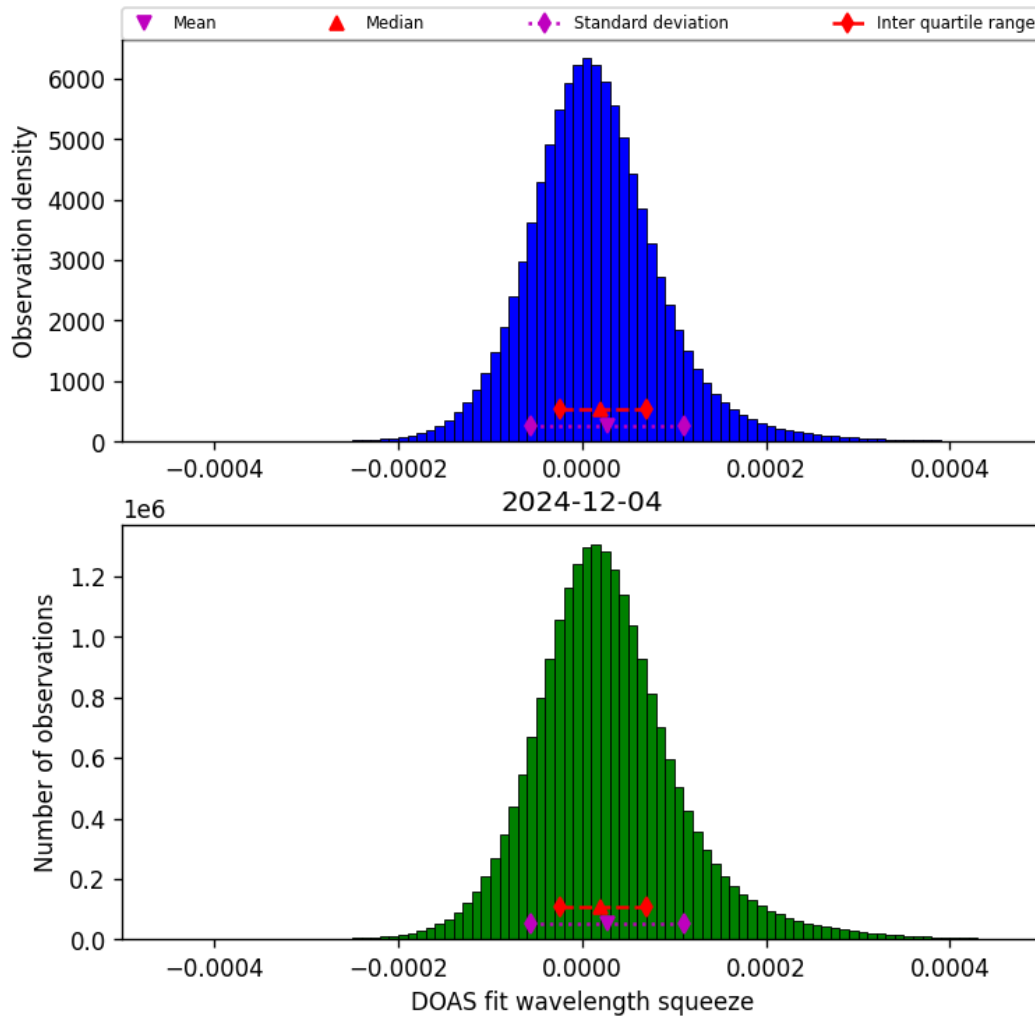
Figure 43: Histogram of “DOAS fit wavelength squeeze” for 2024-12-04 to 2024-12-04
