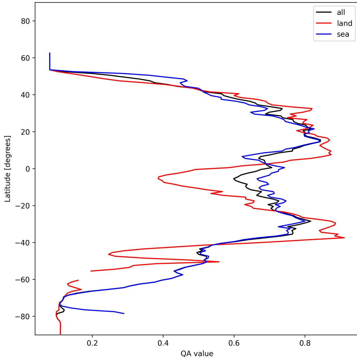
Figure 18: Zonal average of “QA value” for 2024-12-04 to 2024-12-04.
