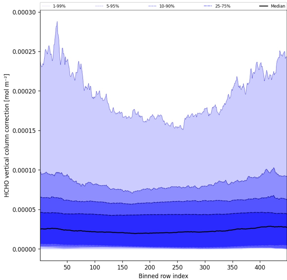
Figure 49: Along track statistics of “HCHO vertical column correction” for 2024-12-04 to 2024-12-04
