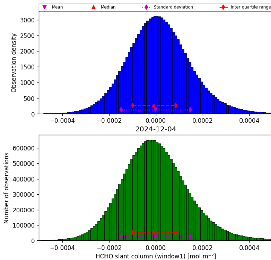
Figure 36: Histogram of “HCHO slant column (window1)” for 2024-12-04 to 2024-12-04
