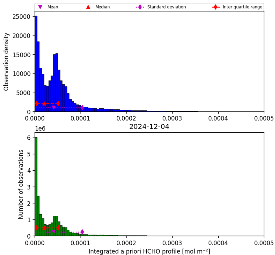
Figure 41: Histogram of “Integrated a priori HCHO profile” for 2024-12-04 to 2024-12-04
