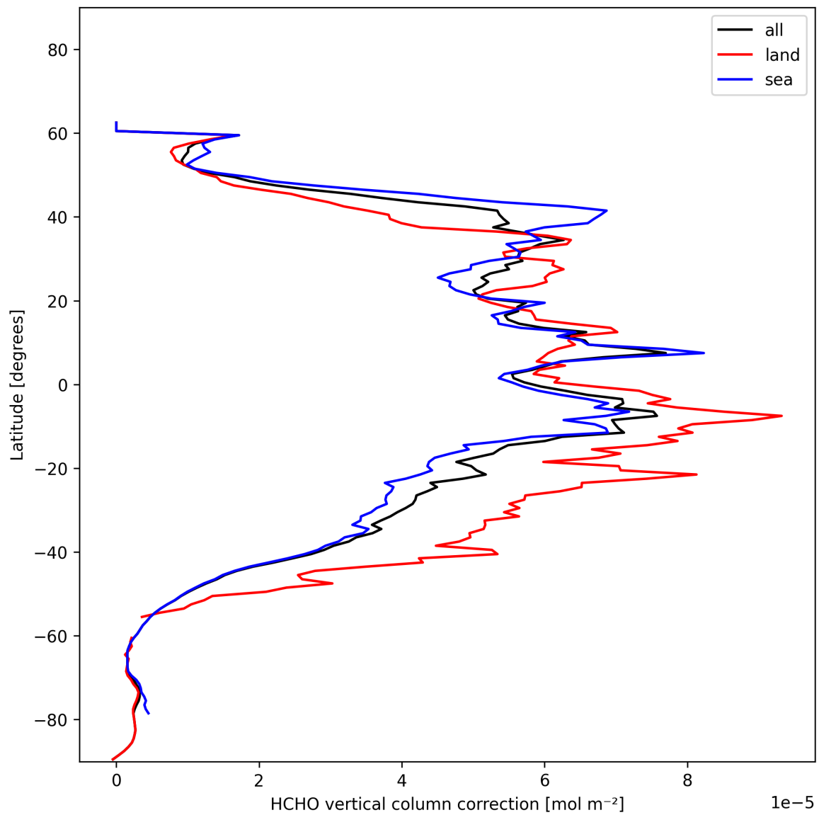
Figure 21: Zonal average of “HCHO vertical column correction” for 2024-12-04 to 2024-12-04.
