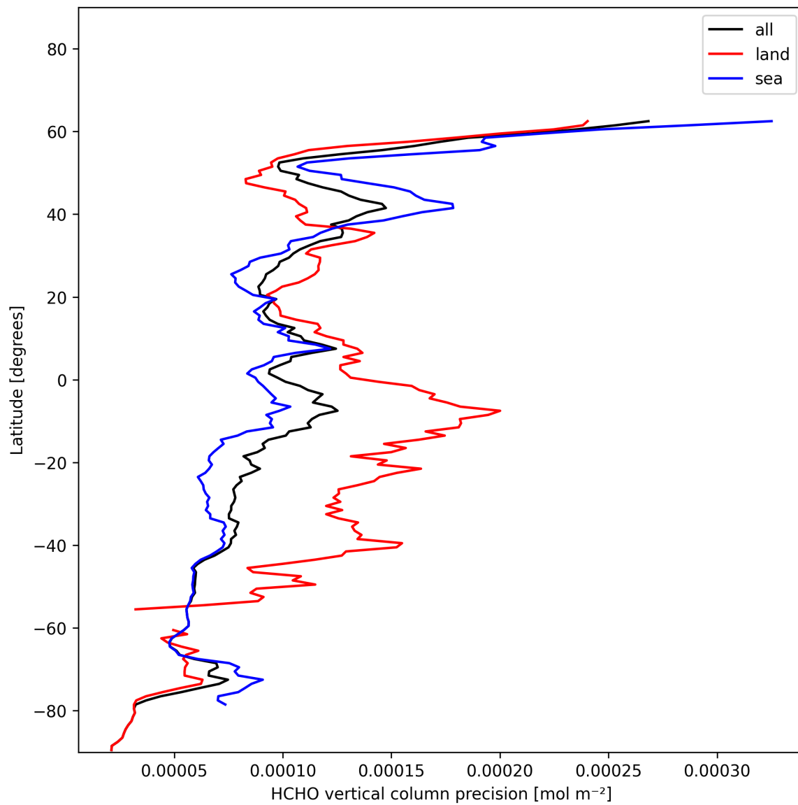
Figure 20: Zonal average of “HCHO vertical column precision” for 2024-12-04 to 2024-12-04.
