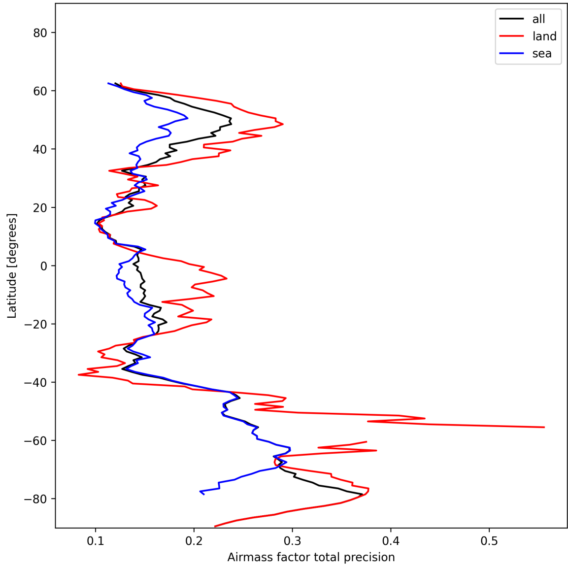
Figure 25: Zonal average of “Airmass factor total precision” for 2024-12-04 to 2024-12-04.
