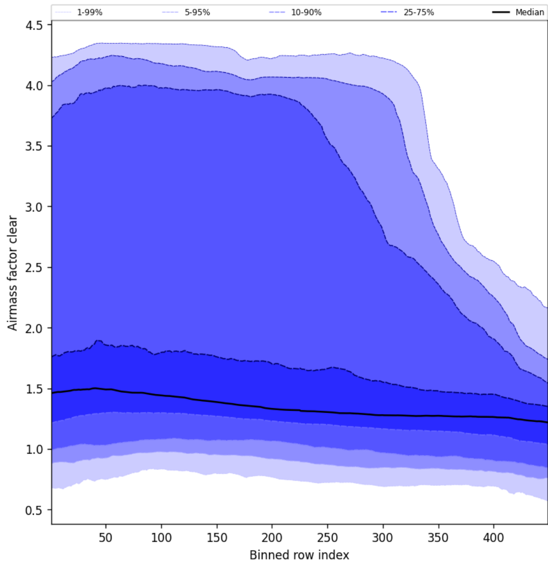
Figure 54: Along track statistics of “Airmass factor clear” for 2024-12-04 to 2024-12-04
