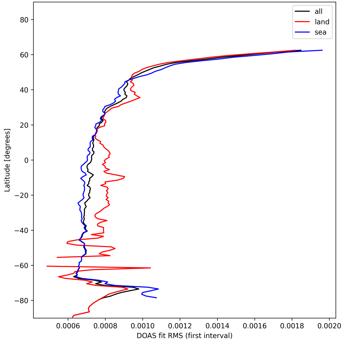
Figure 30: Zonal average of "DOAS fit RMS (first interval)" for 2024-12-04 to 2024-12-04.
