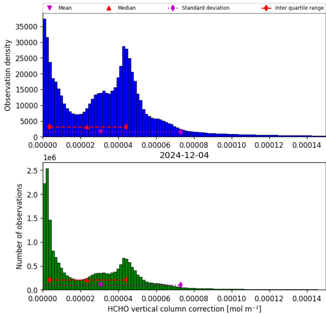
Figure 35: Histogram of “HCHO vertical column correction” for 2024-12-04 to 2024-12-04
