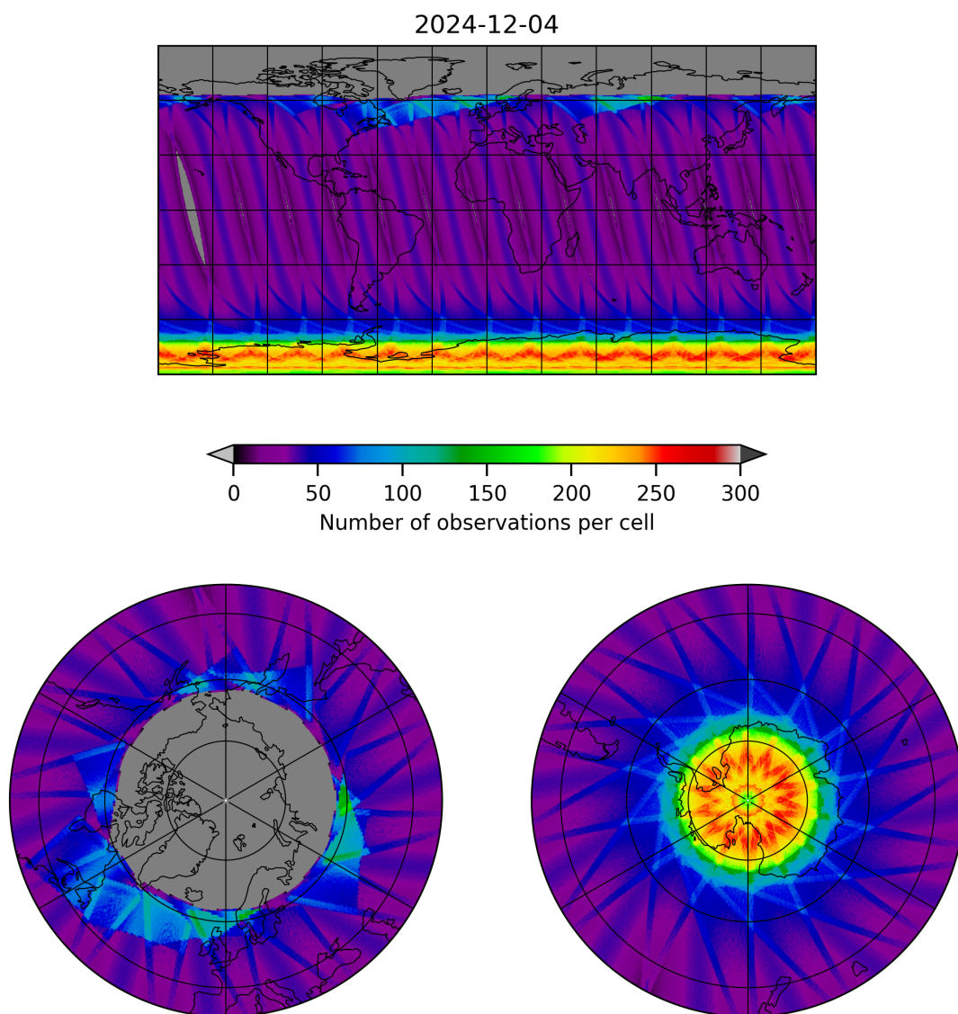
Figure 17: Map of the number of observations for 2024-12-04 to 2024-12-04
