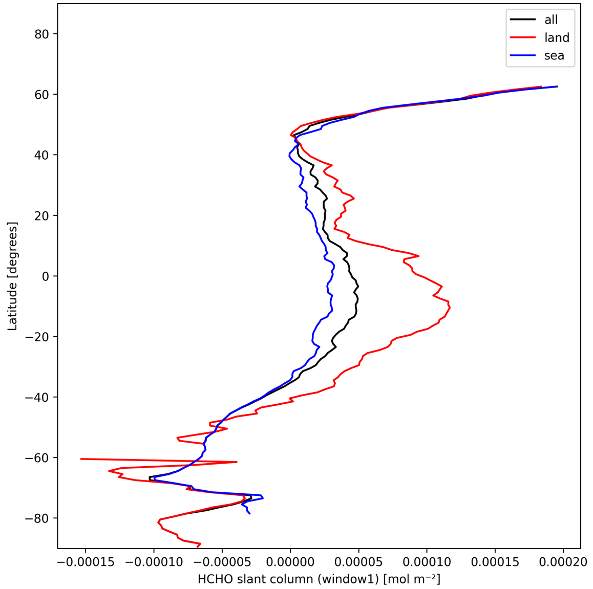
Figure 22: Zonal average of “HCHO slant column (window1)” for 2024-12-04 to 2024-12-04.
