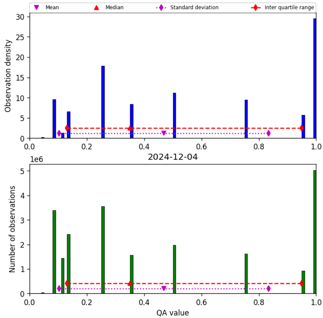
Figure 32: Histogram of “QA value” for 2024-12-04 to 2024-12-04
