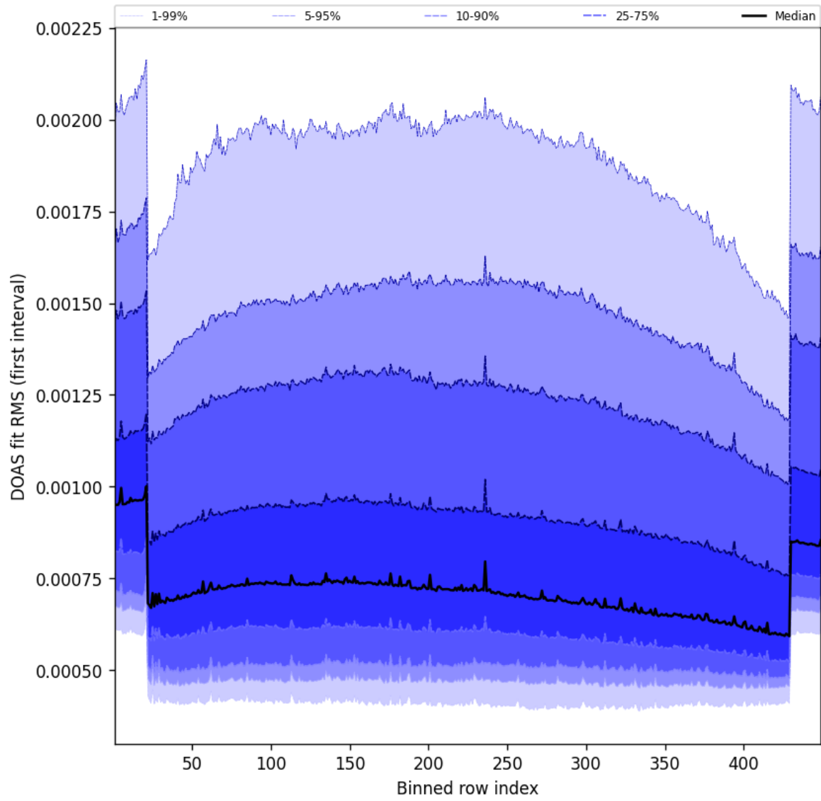
Figure 58: Along track statistics of “DOAS fit RMS (first interval)” for 2024-12-04 to 2024-12-04
