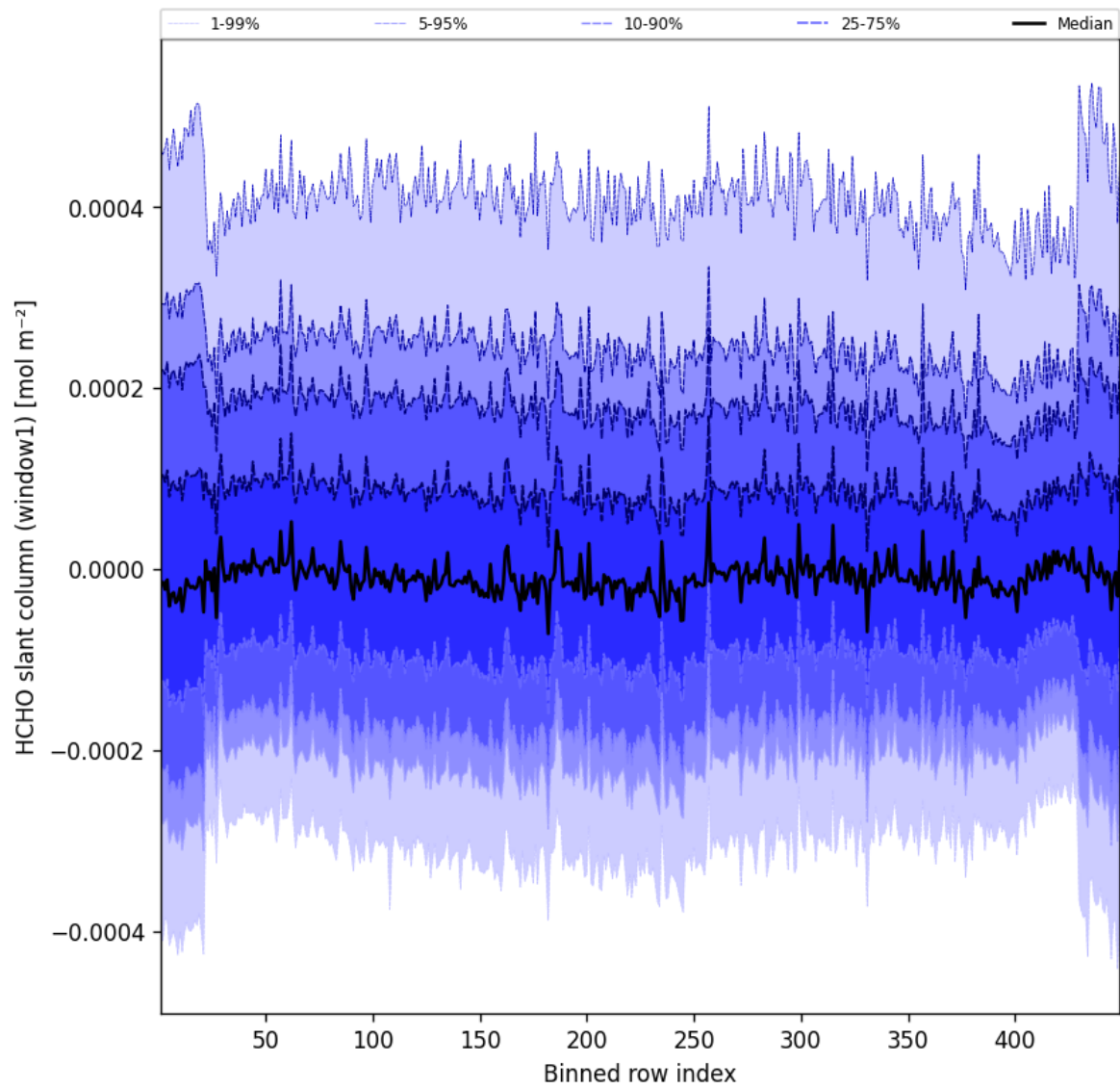
Figure 50: Along track statistics of “HCHO slant column (window1)” for 2024-12-04 to 2024-12-04
