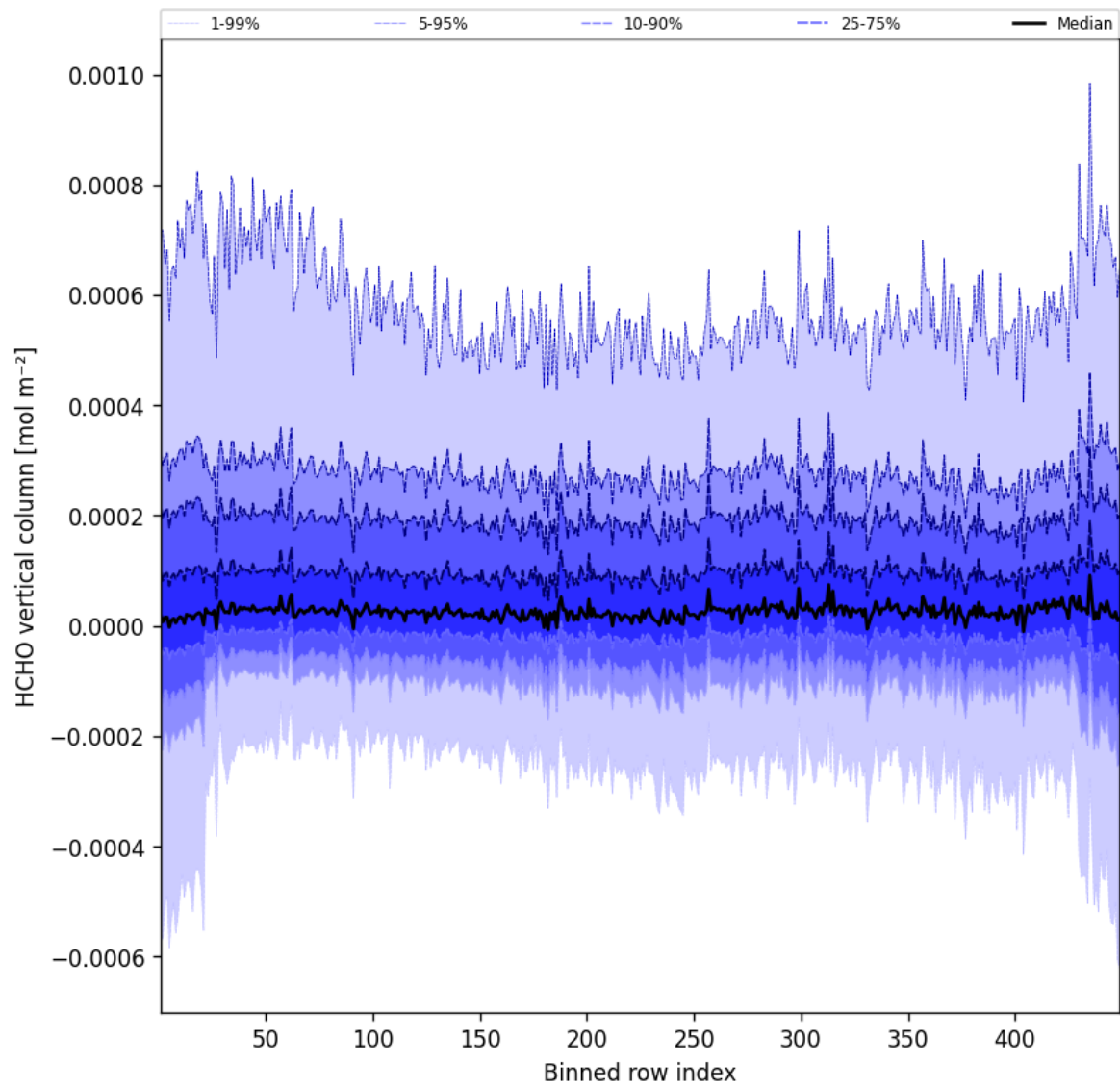
Figure 47: Along track statistics of “HCHO vertical column” for 2024-12-04 to 2024-12-04
