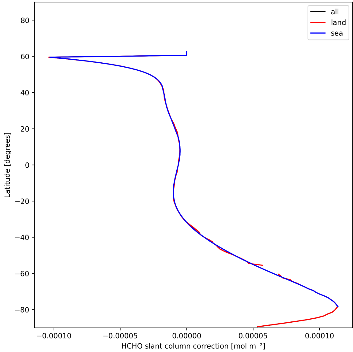
Figure 31: Zonal average of “HCHO slant column correction” for 2024-12-04 to 2024-12-04.
