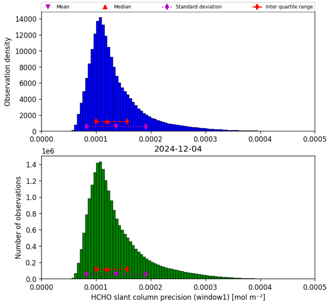
Figure 37: Histogram of “HCHO slant column precision (window1)” for 2024-12-04 to 2024-12-04
