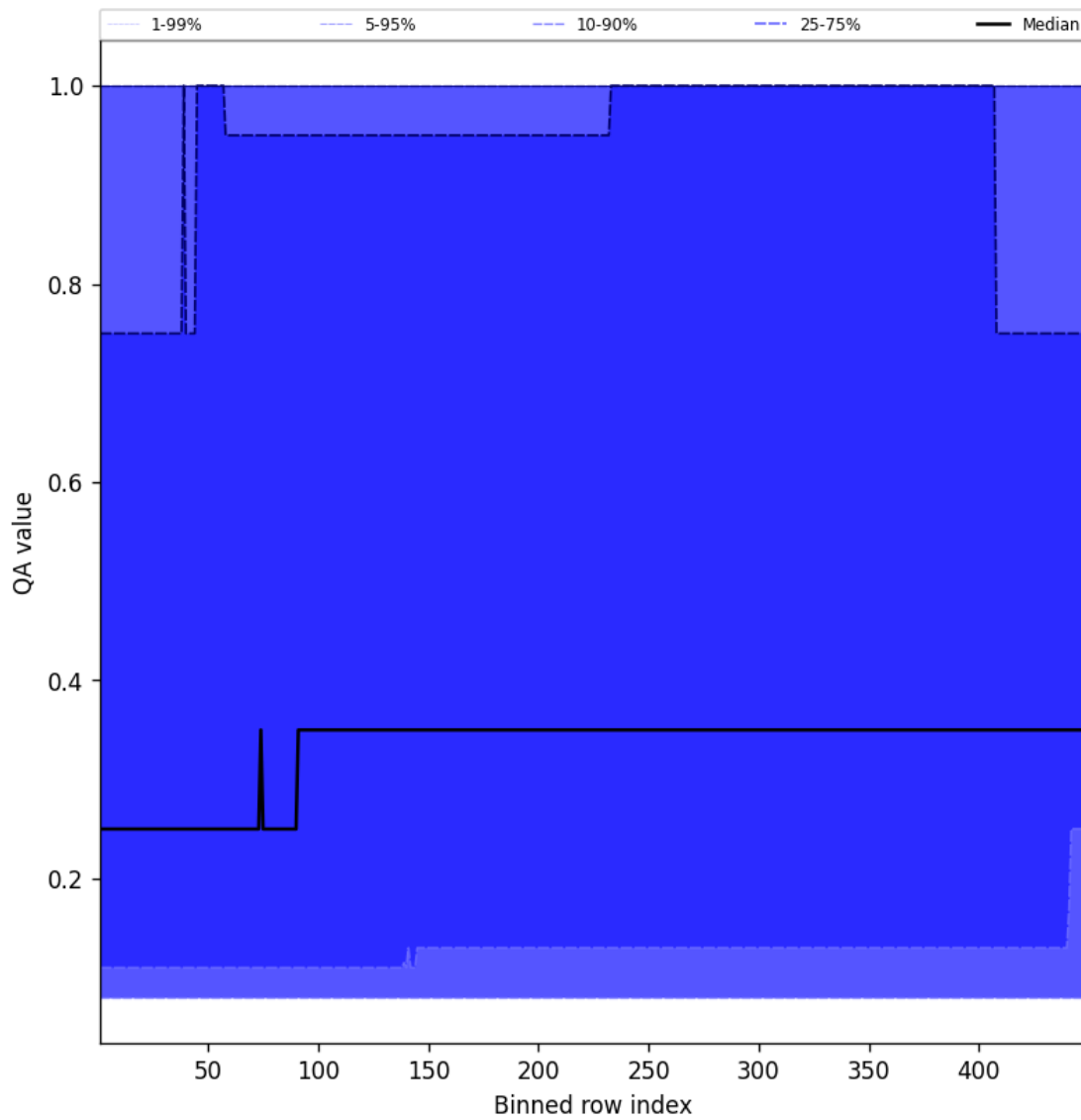
Figure 46: Along track statistics of “QA value” for 2024-12-04 to 2024-12-04
