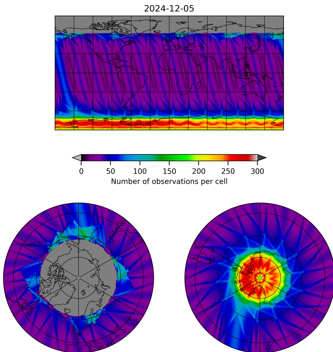
Figure 17: Map of the number of observations for 2024-12-05 to 2024-12-06
