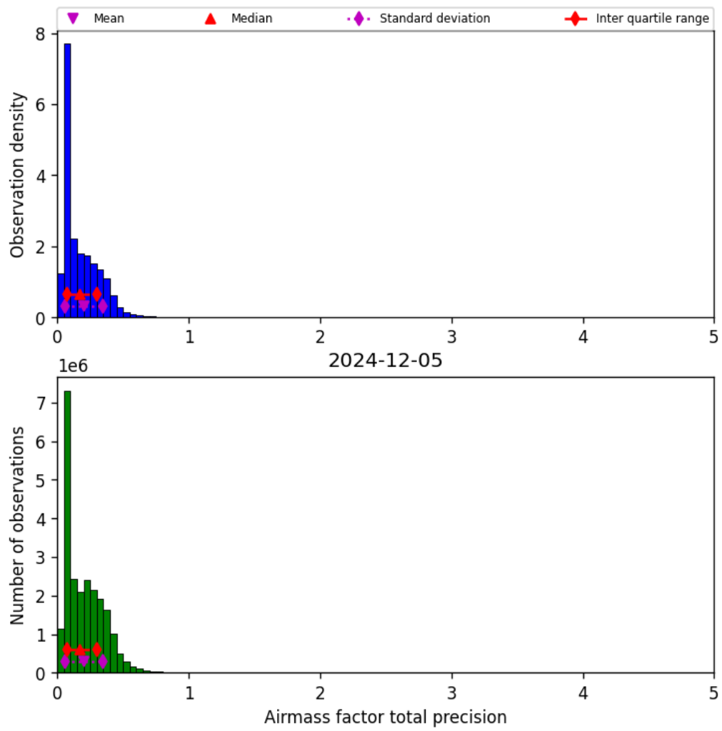
Figure 39: Histogram of “Airmass factor total precision” for 2024-12-05 to 2024-12-06
