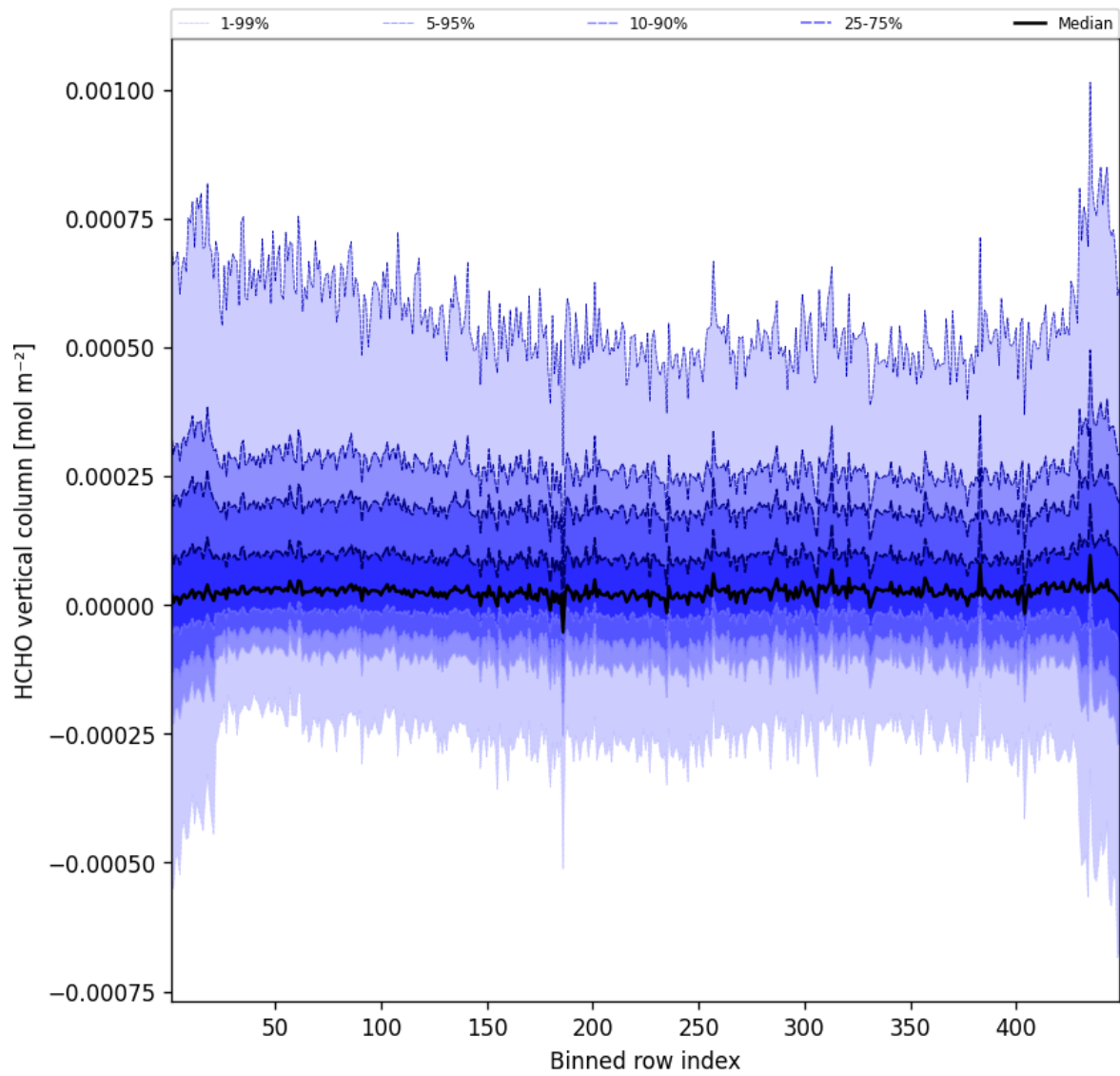
Figure 47: Along track statistics of “HCHO vertical column” for 2024-12-05 to 2024-12-06
