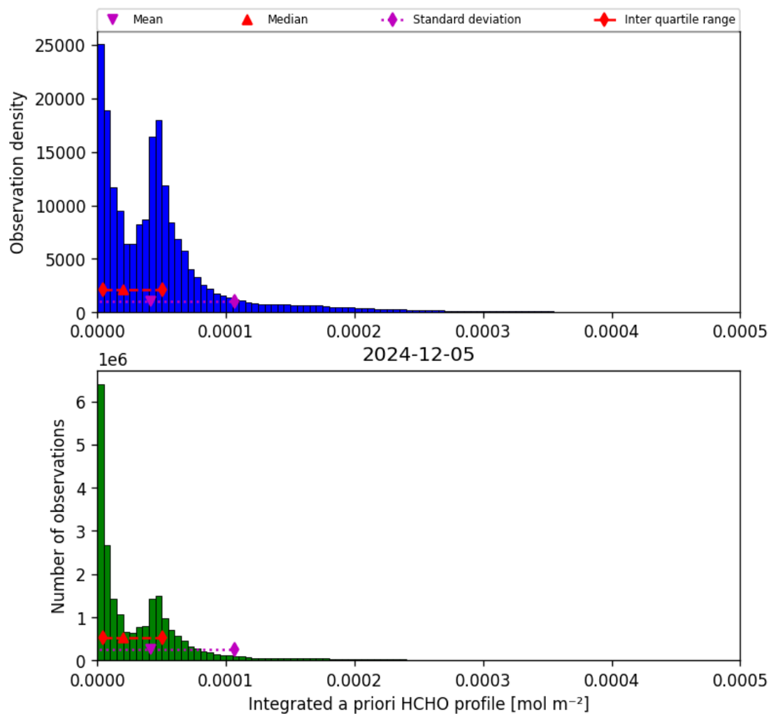
Figure 41: Histogram of “Integrated a priori HCHO profile” for 2024-12-05 to 2024-12-06
