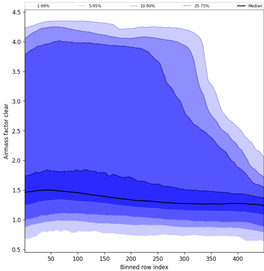
Figure 54: Along track statistics of “Airmass factor clear” for 2024-12-05 to 2024-12-06
