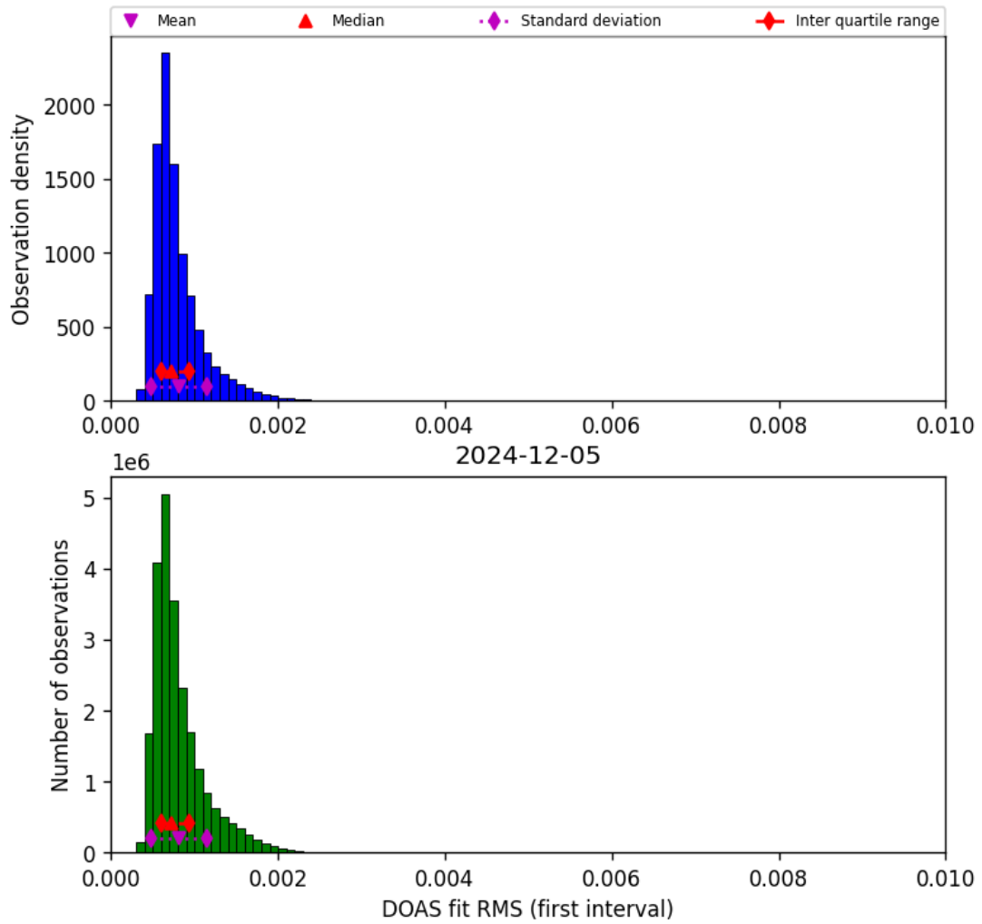
Figure 44: Histogram of “DOAS fit RMS (first interval)” for 2024-12-05 to 2024-12-06
