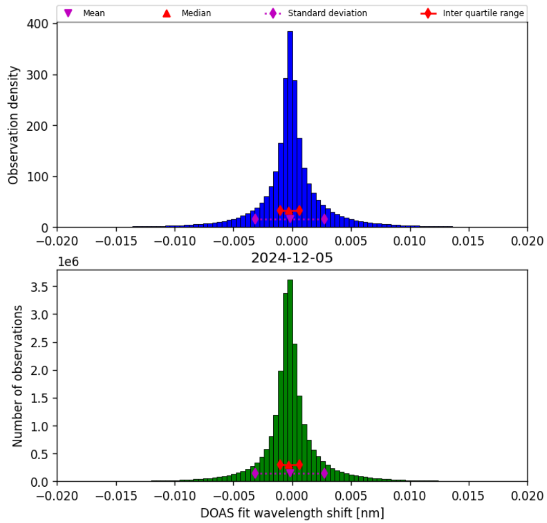
Figure 42: Histogram of “DOAS fit wavelength shift” for 2024-12-05 to 2024-12-06
