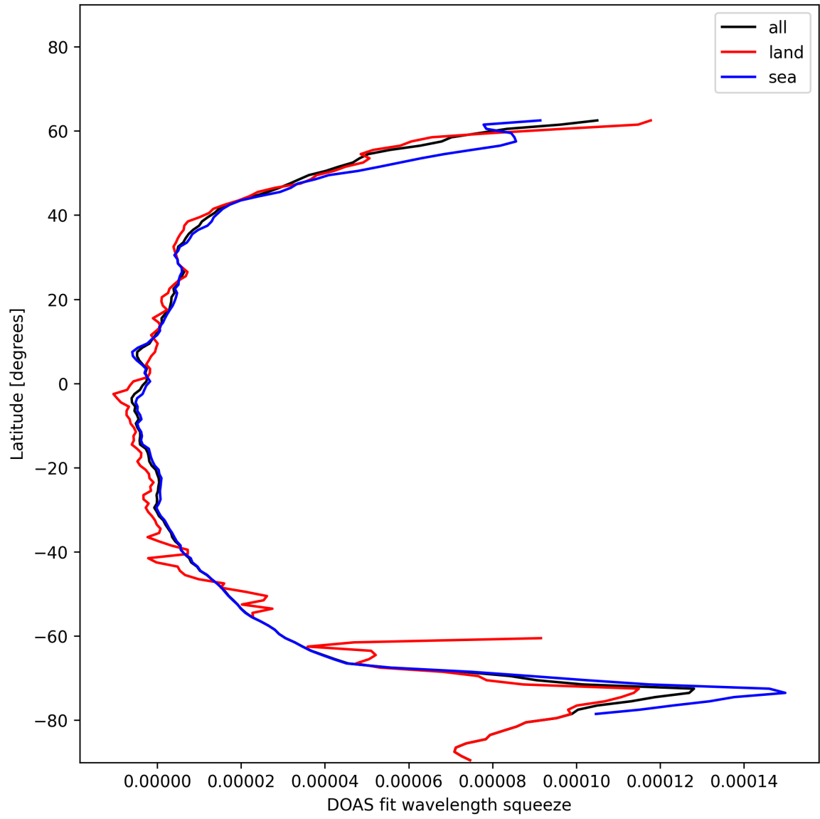
Figure 29: Zonal average of “DOAS fit wavelength squeeze” for 2024-12-05 to 2024-12-06.
