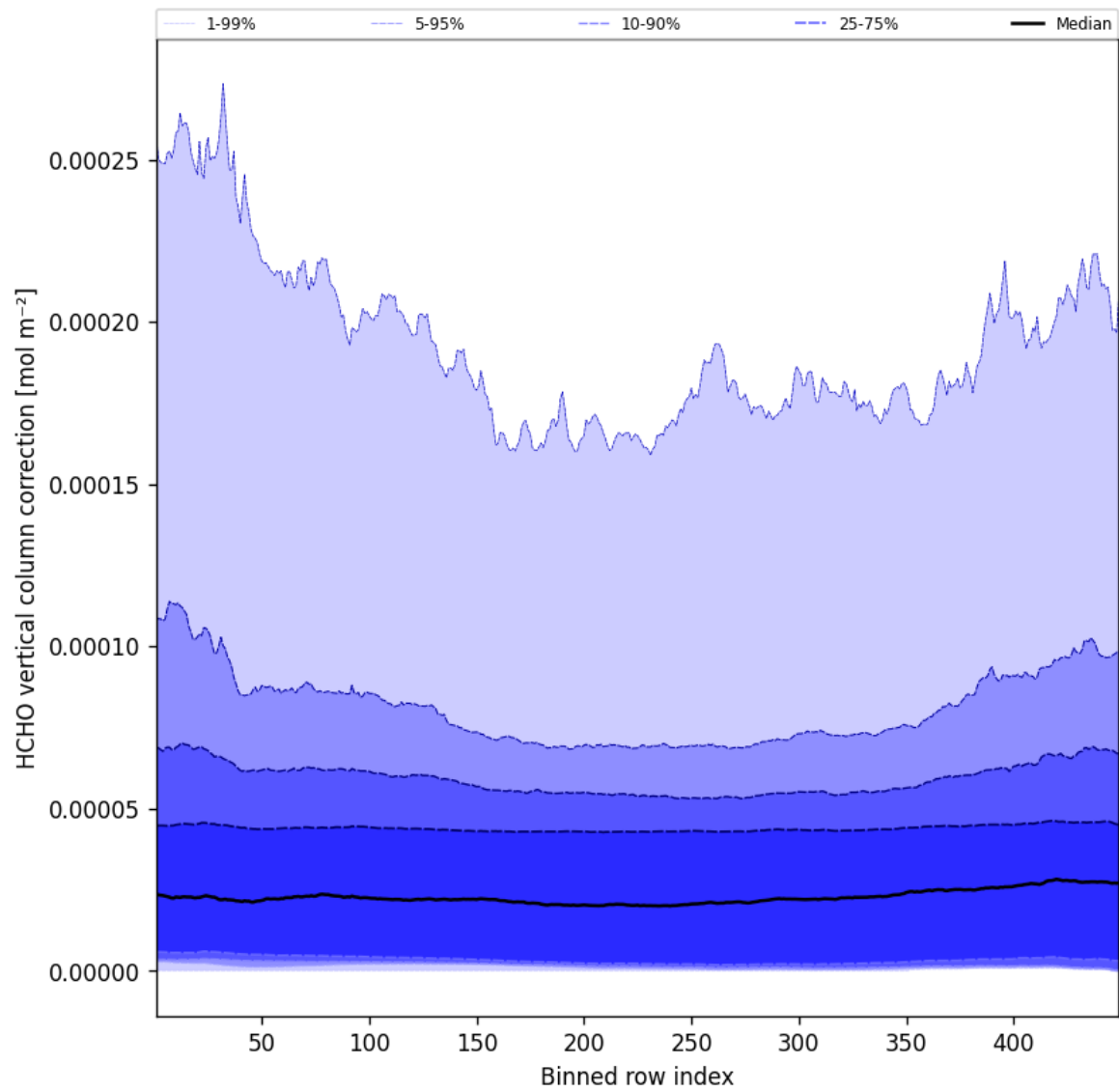
Figure 49: Along track statistics of “HCHO vertical column correction” for 2024-12-05 to 2024-12-06
