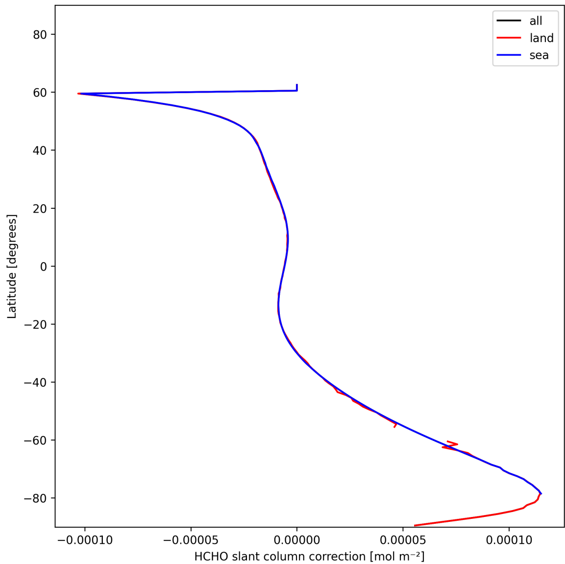
Figure 31: Zonal average of “HCHO slant column correction” for 2024-12-05 to 2024-12-06.
