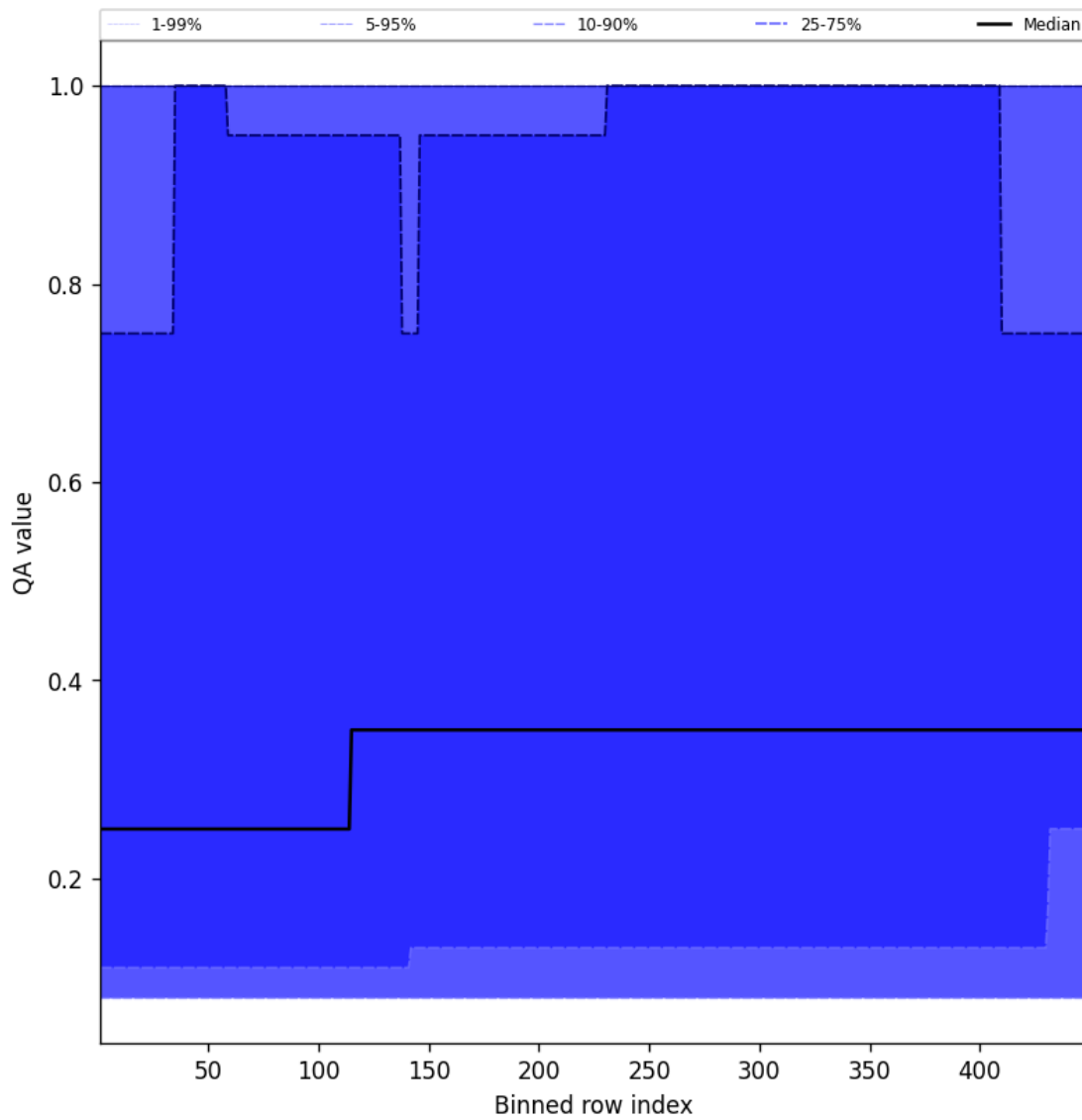
Figure 46: Along track statistics of “QA value” for 2024-12-05 to 2024-12-06
