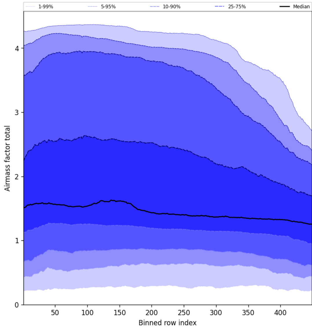
Figure 52: Along track statistics of “Airmass factor total” for 2024-12-05 to 2024-12-06
