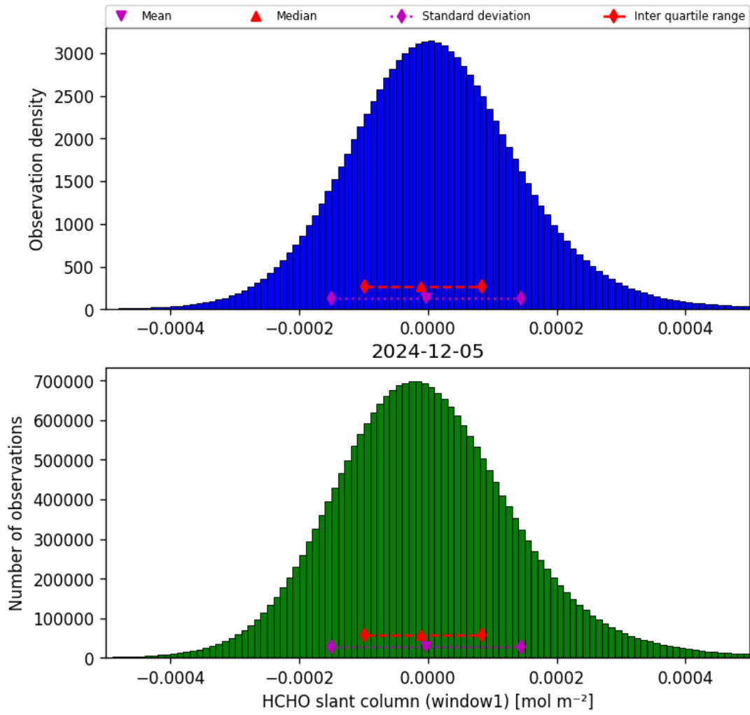
Figure 36: Histogram of “HCHO slant column (window1)” for 2024-12-05 to 2024-12-06
