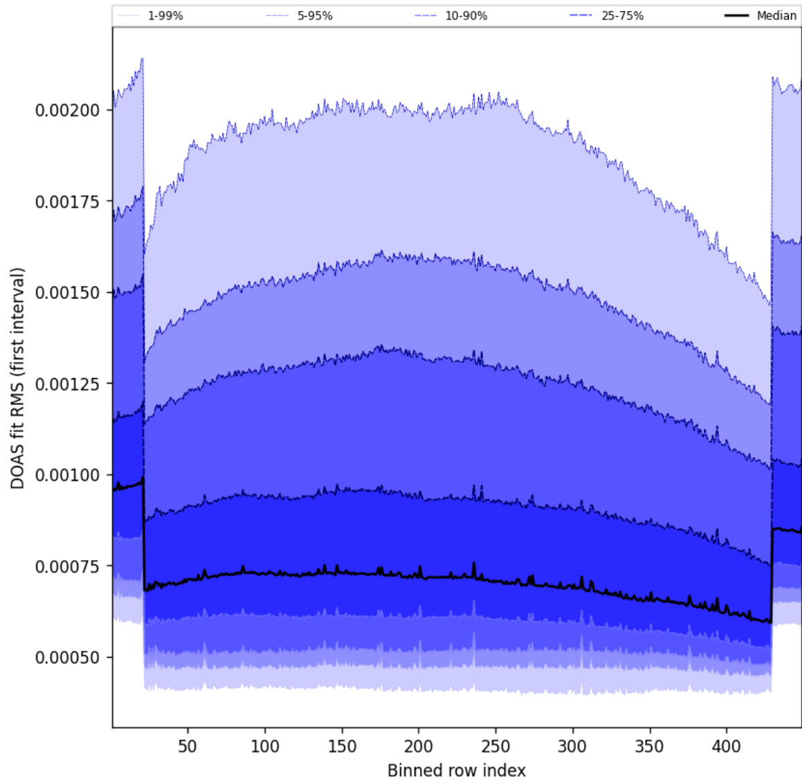
Figure 58: Along track statistics of “DOAS fit RMS (first interval)” for 2024-12-05 to 2024-12-06
