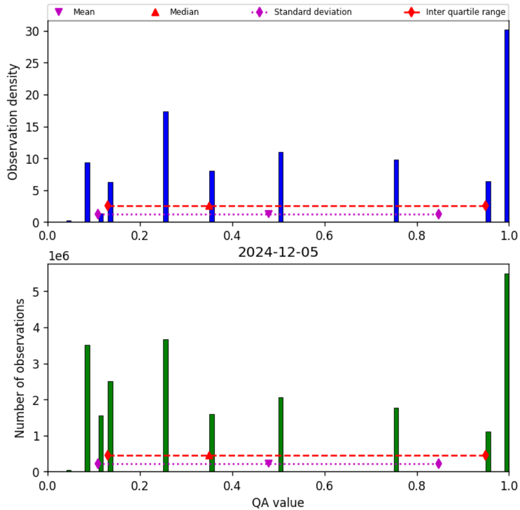
Figure 32: Histogram of “QA value” for 2024-12-05 to 2024-12-06
