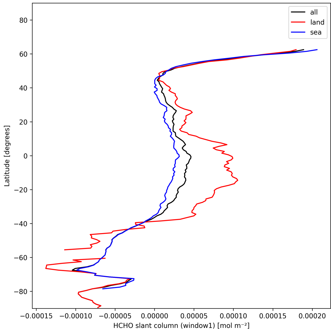
Figure 22: Zonal average of “HCHO slant column (window1)” for 2024-12-05 to 2024-12-06.
