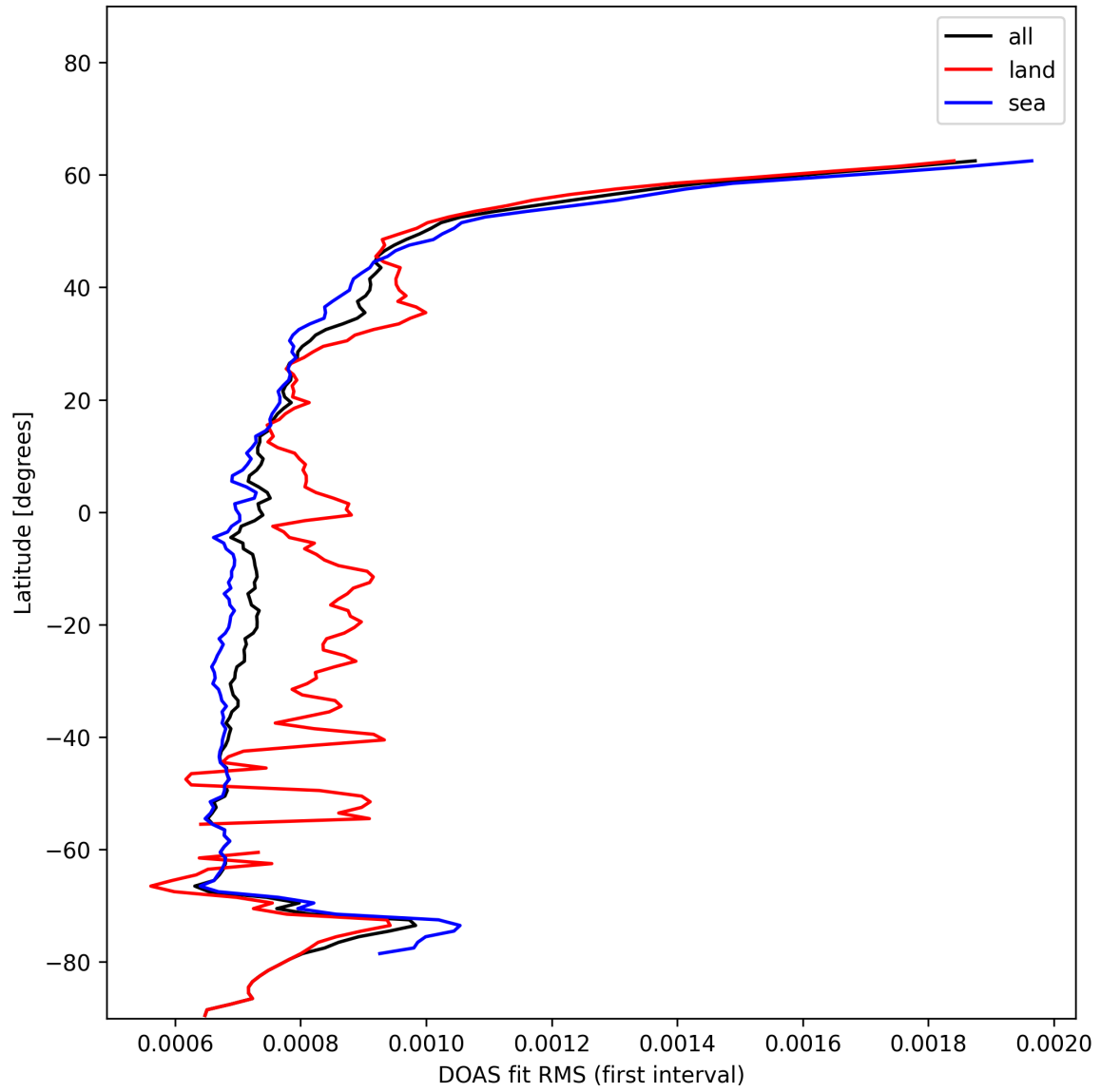
Figure 30: Zonal average of "DOAS fit RMS (first interval)" for 2024-12-05 to 2024-12-06.
