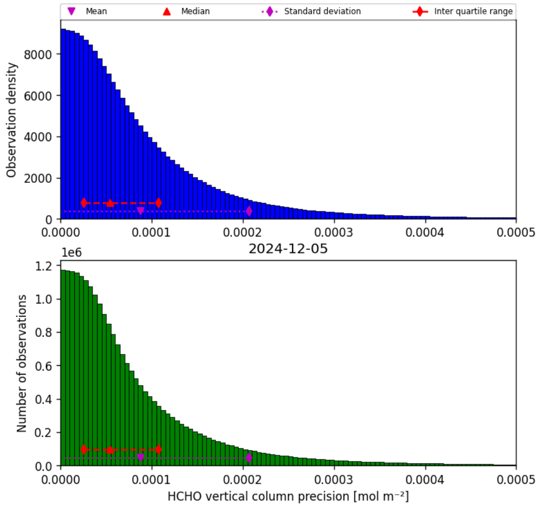
Figure 34: Histogram of “HCHO vertical column precision” for 2024-12-05 to 2024-12-06
