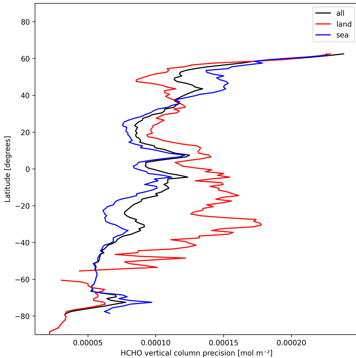
Figure 20: Zonal average of “HCHO vertical column precision” for 2024-12-05 to 2024-12-06.
