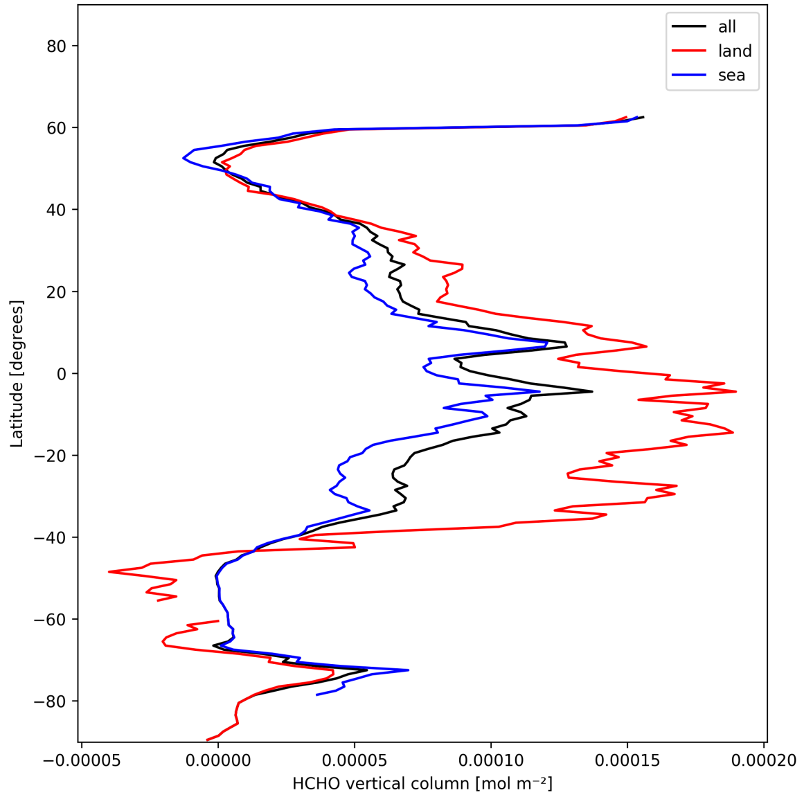
Figure 19: Zonal average of “HCHO vertical column” for 2024-12-05 to 2024-12-06.
