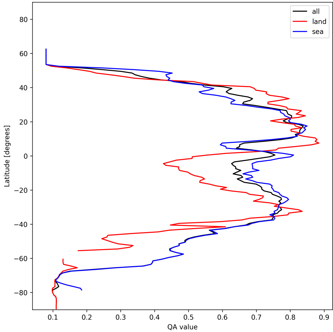
Figure 18: Zonal average of “QA value” for 2024-12-05 to 2024-12-06.
