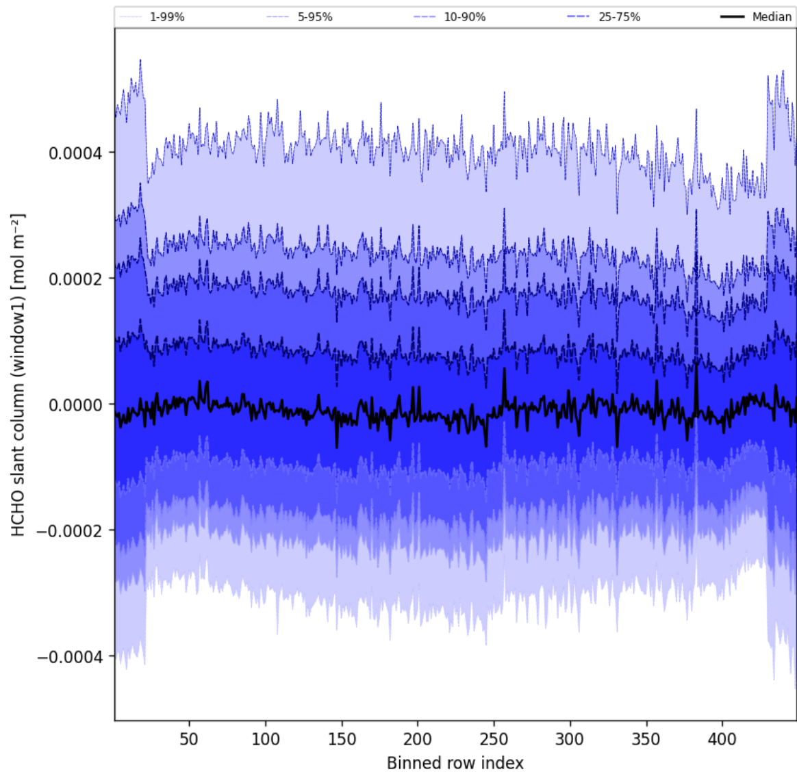
Figure 50: Along track statistics of “HCHO slant column (window1)” for 2024-12-05 to 2024-12-06
