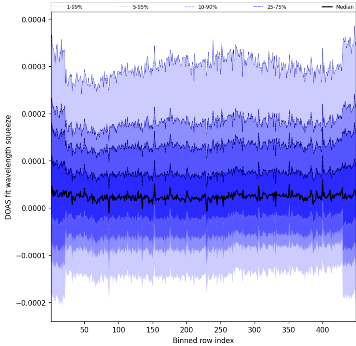
Figure 57: Along track statistics of “DOAS fit wavelength squeeze” for 2024-12-05 to 2024-12-06
