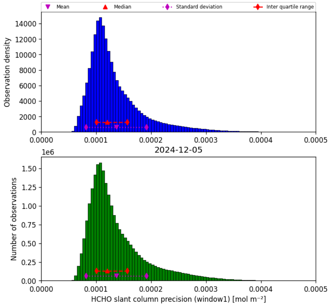
Figure 37: Histogram of “HCHO slant column precision (window1)” for 2024-12-05 to 2024-12-06
