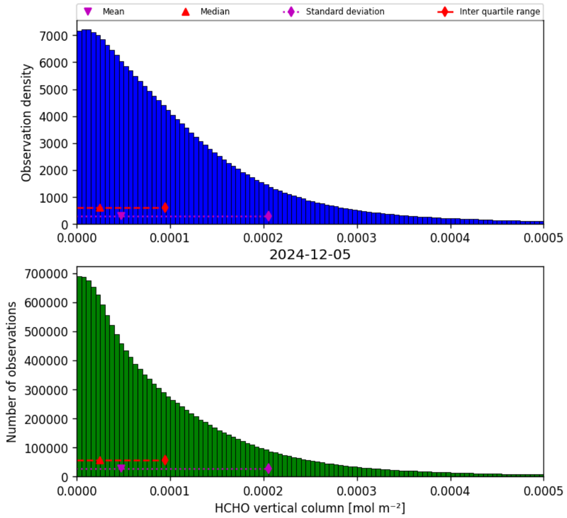
Figure 33: Histogram of “HCHO vertical column” for 2024-12-05 to 2024-12-06
