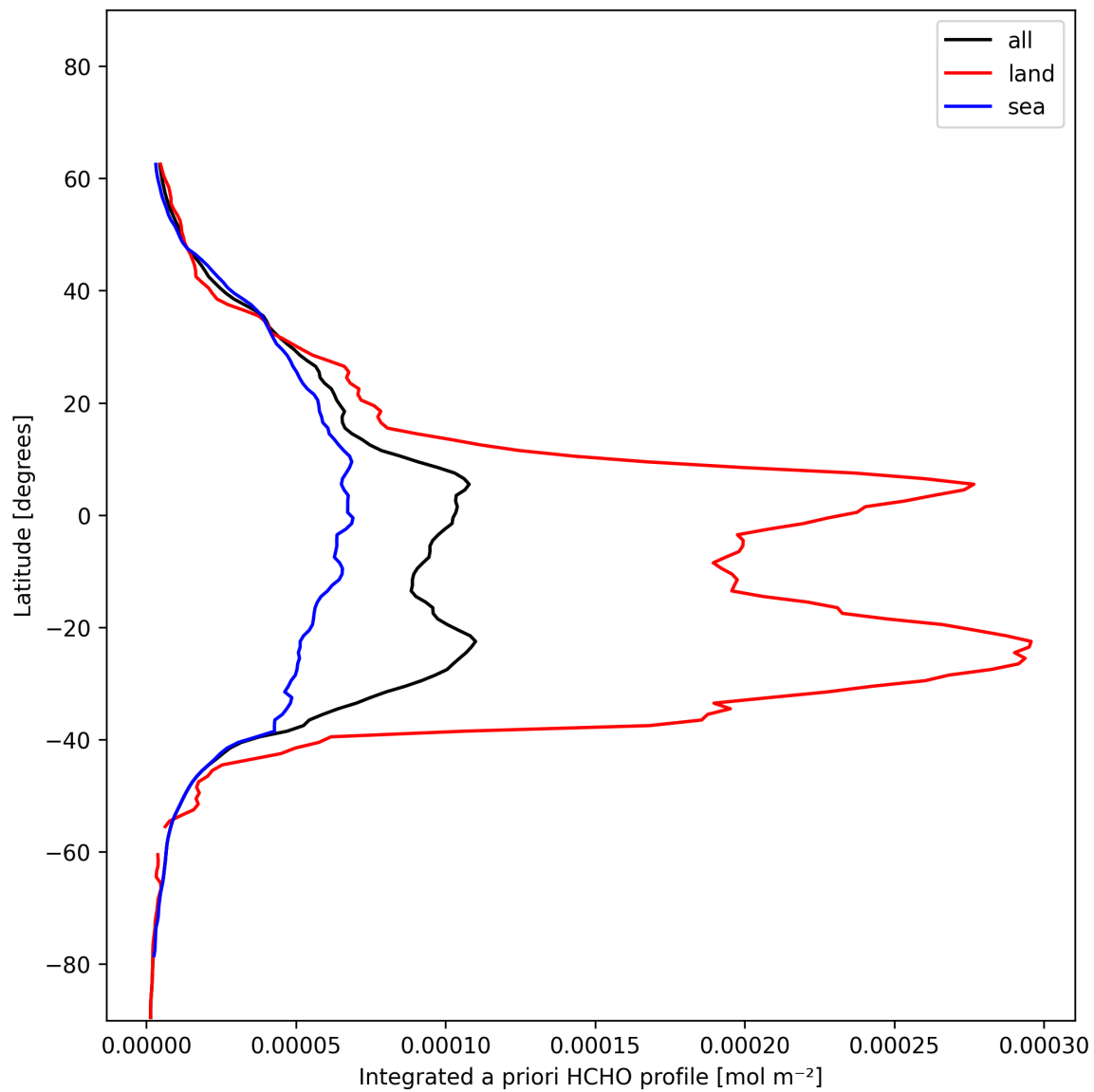
Figure 27: Zonal average of “Integrated a priori HCHO profile” for 2024-12-05 to 2024-12-06.
