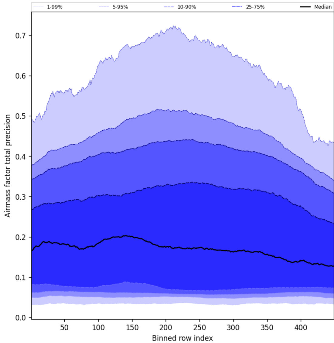
Figure 53: Along track statistics of “Airmass factor total precision” for 2024-12-05 to 2024-12-06
