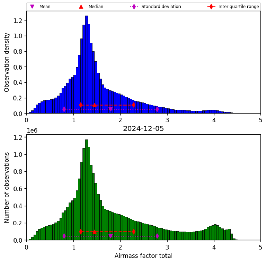
Figure 38: Histogram of “Airmass factor total” for 2024-12-05 to 2024-12-06
