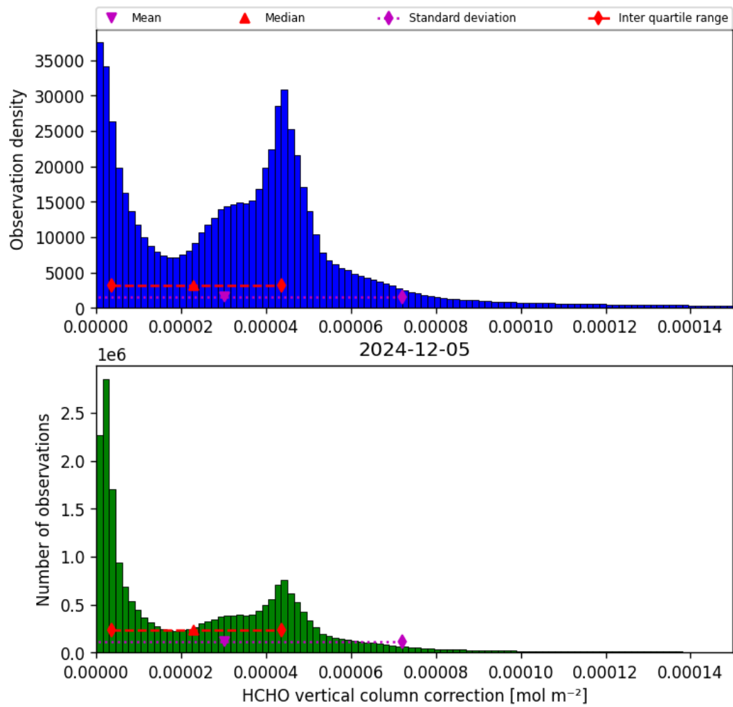
Figure 35: Histogram of “HCHO vertical column correction” for 2024-12-05 to 2024-12-06
