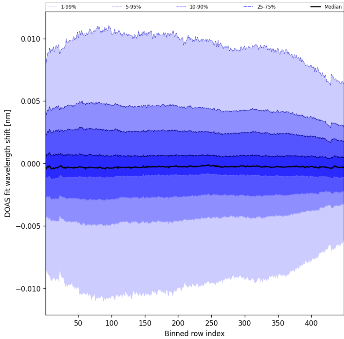
Figure 56: Along track statistics of “DOAS fit wavelength shift” for 2024-12-05 to 2024-12-06
