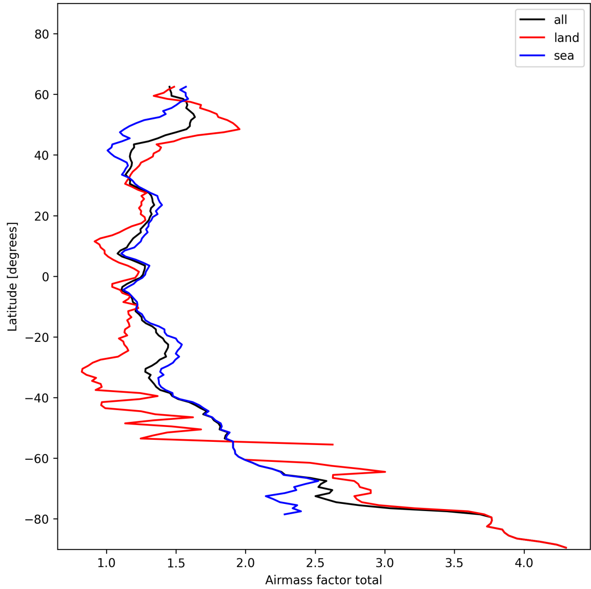
Figure 24: Zonal average of “Airmass factor total” for 2024-12-05 to 2024-12-06.
