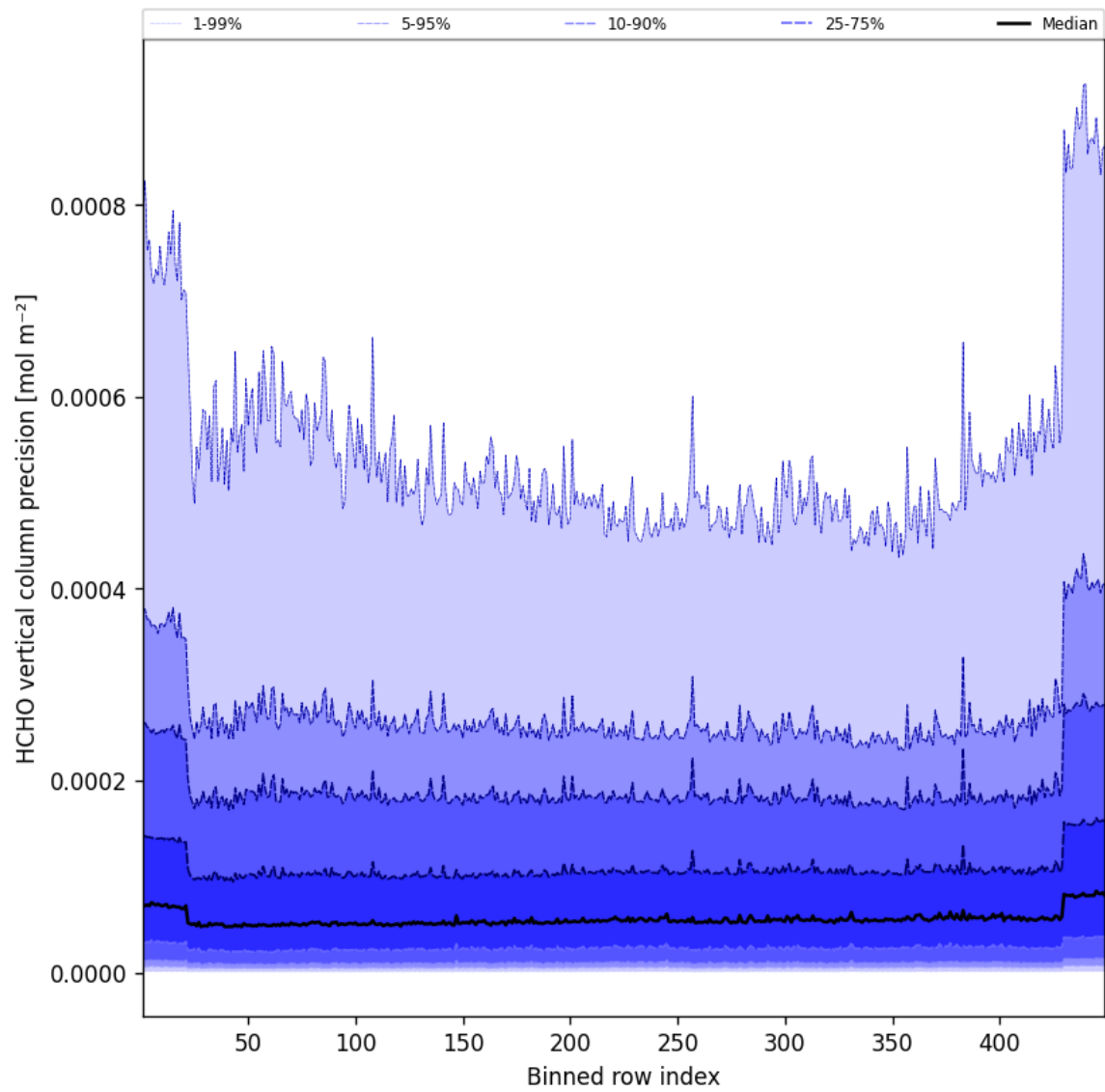
Figure 48: Along track statistics of “HCHO vertical column precision” for 2024-12-05 to 2024-12-06
