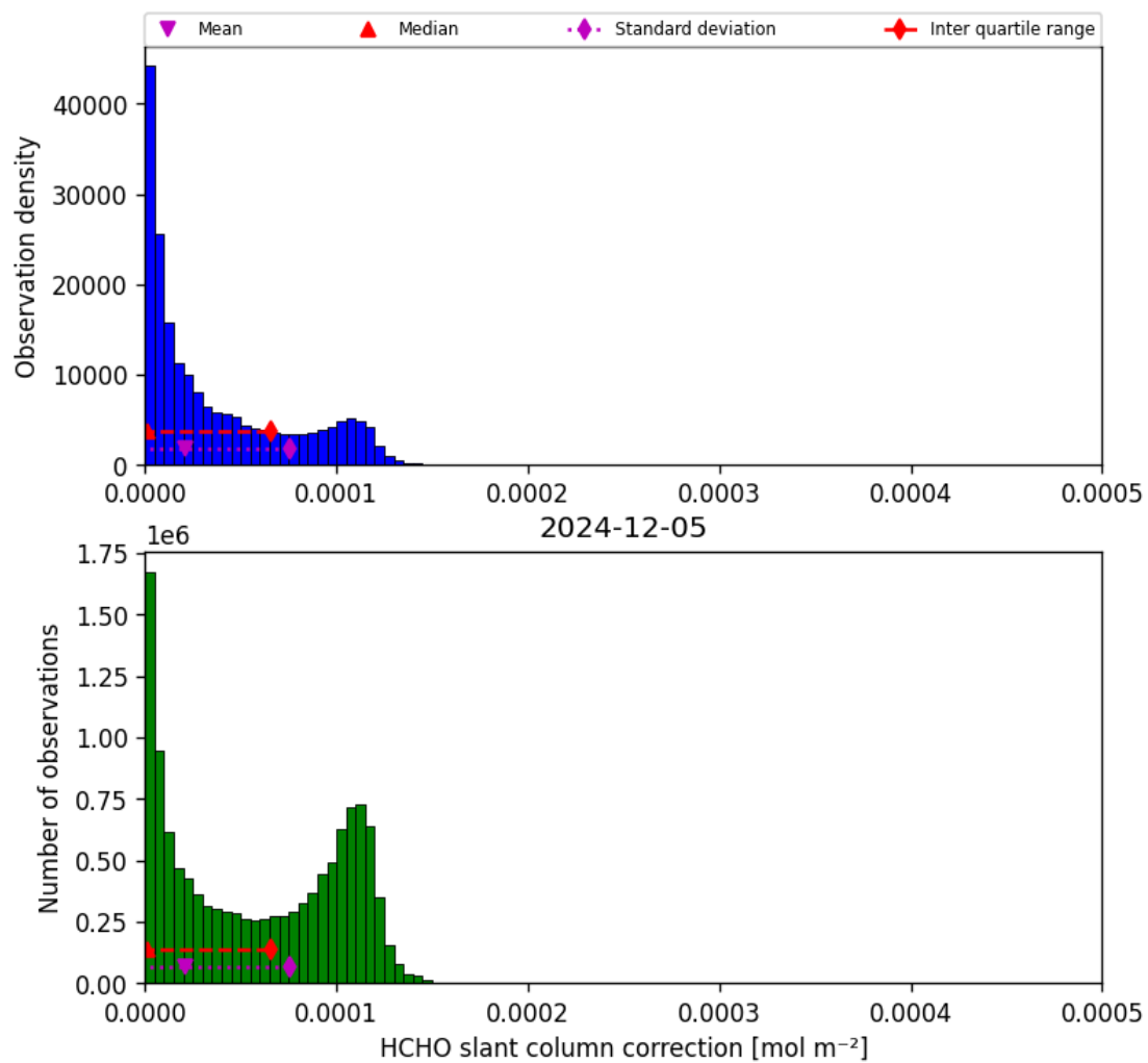
Figure 45: Histogram of “HCHO slant column correction” for 2024-12-05 to 2024-12-06
