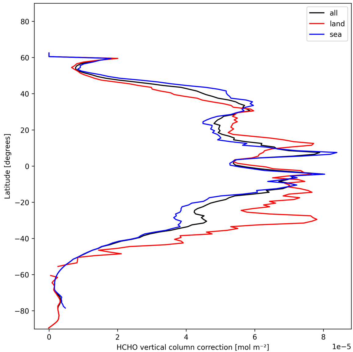
Figure 21: Zonal average of “HCHO vertical column correction” for 2024-12-05 to 2024-12-06.
