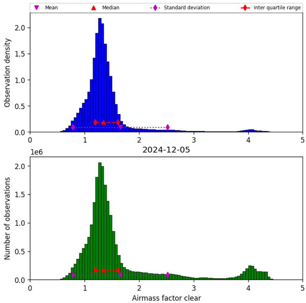
Figure 40: Histogram of “Airmass factor clear” for 2024-12-05 to 2024-12-06
