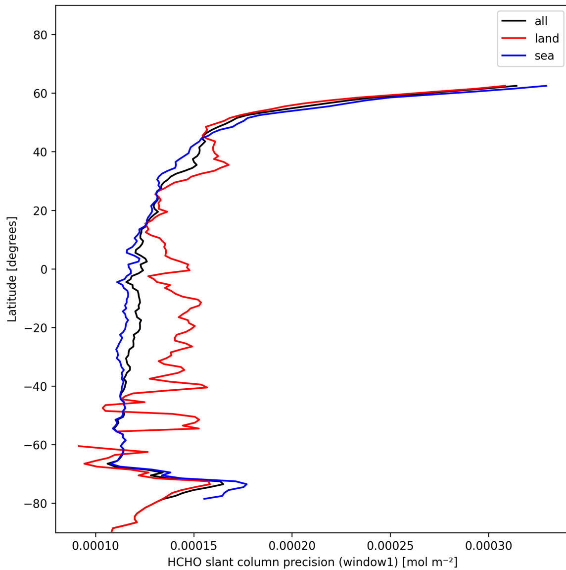
Figure 23: Zonal average of “HCHO slant column precision (window1)” for 2024-12-05 to 2024-12-06.
