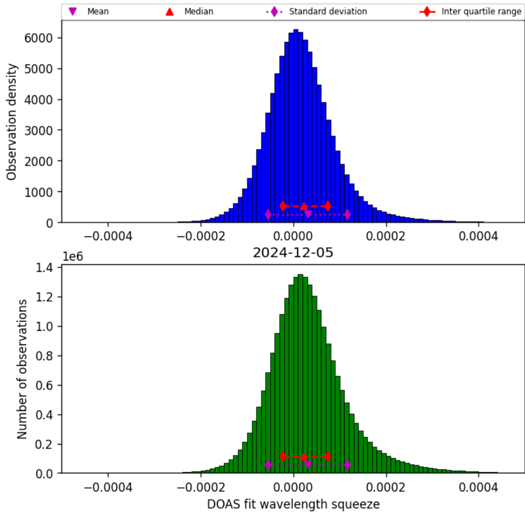
Figure 43: Histogram of “DOAS fit wavelength squeeze” for 2024-12-05 to 2024-12-06
