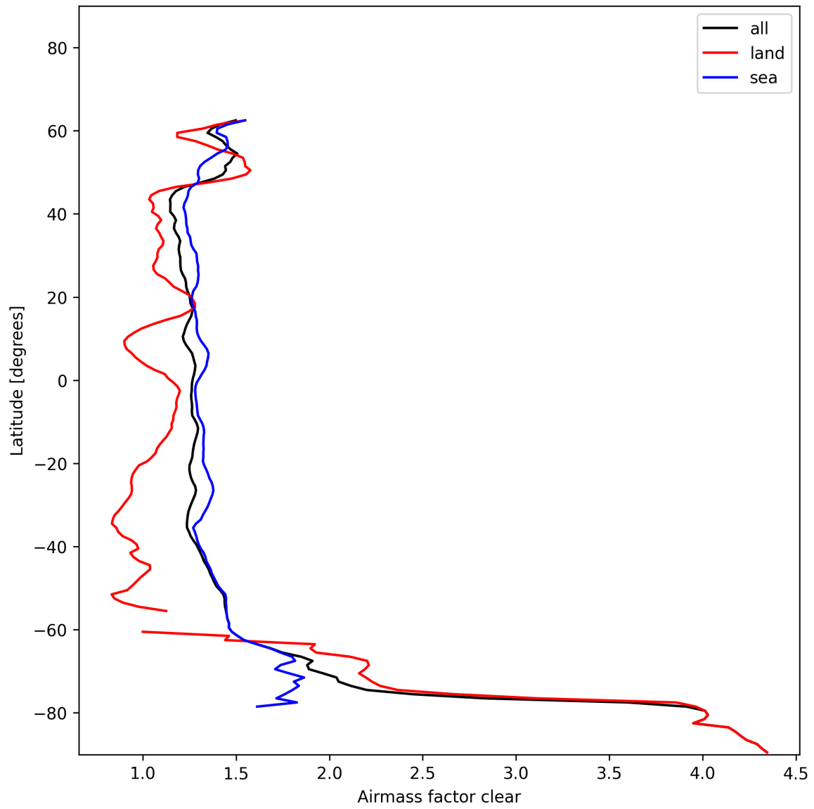
Figure 26: Zonal average of “Airmass factor clear” for 2024-12-05 to 2024-12-06.
