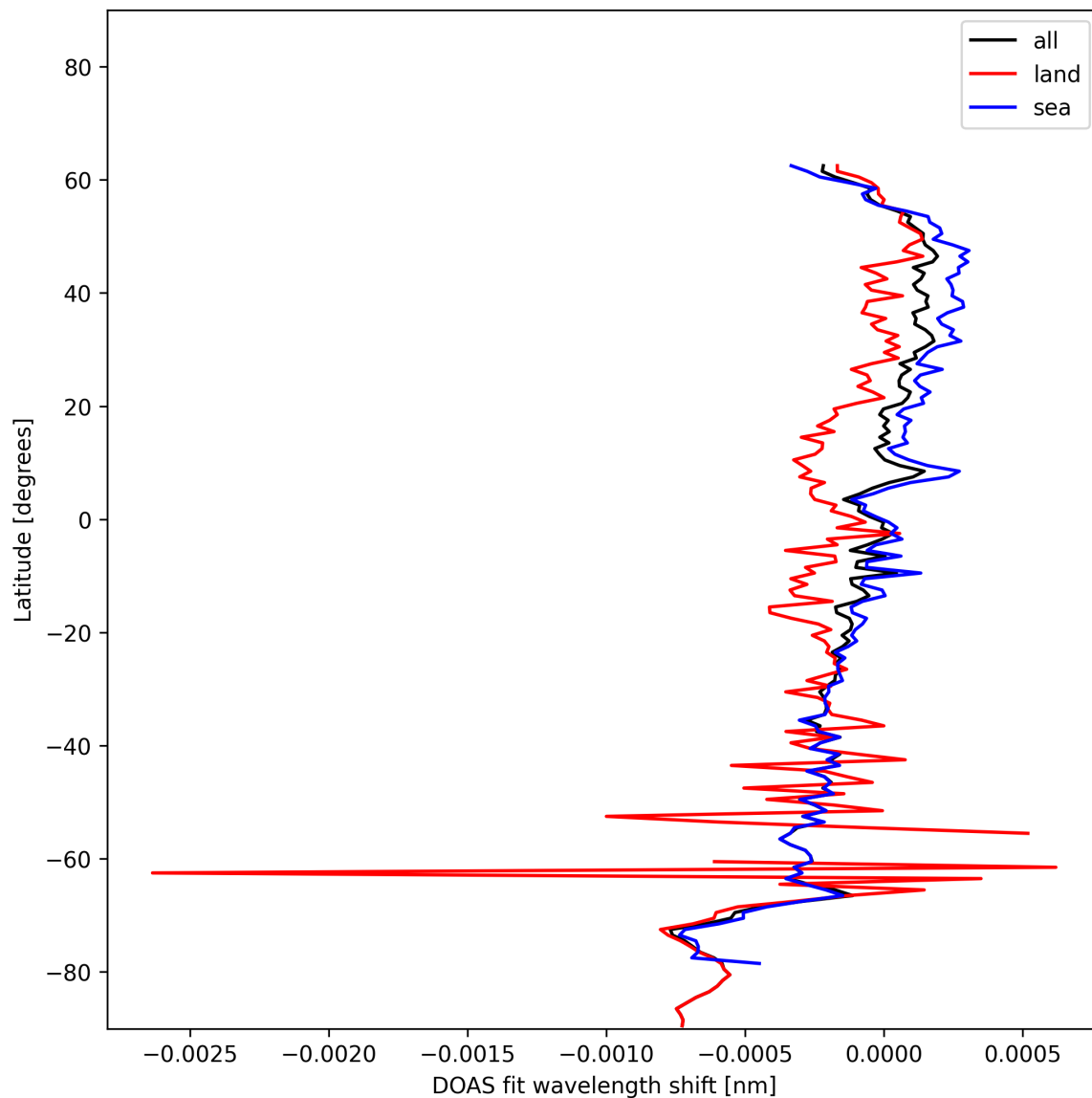
Figure 28: Zonal average of “DOAS fit wavelength shift” for 2024-12-05 to 2024-12-06.
