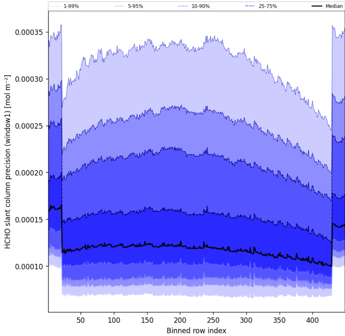
Figure 51: Along track statistics of “HCHO slant column precision (window1)” for 2024-12-05 to 2024-12-06
