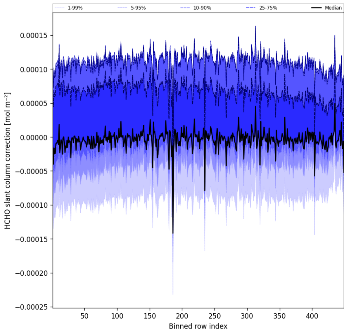
Figure 59: Along track statistics of “HCHO slant column correction” for 2024-12-05 to 2024-12-06
