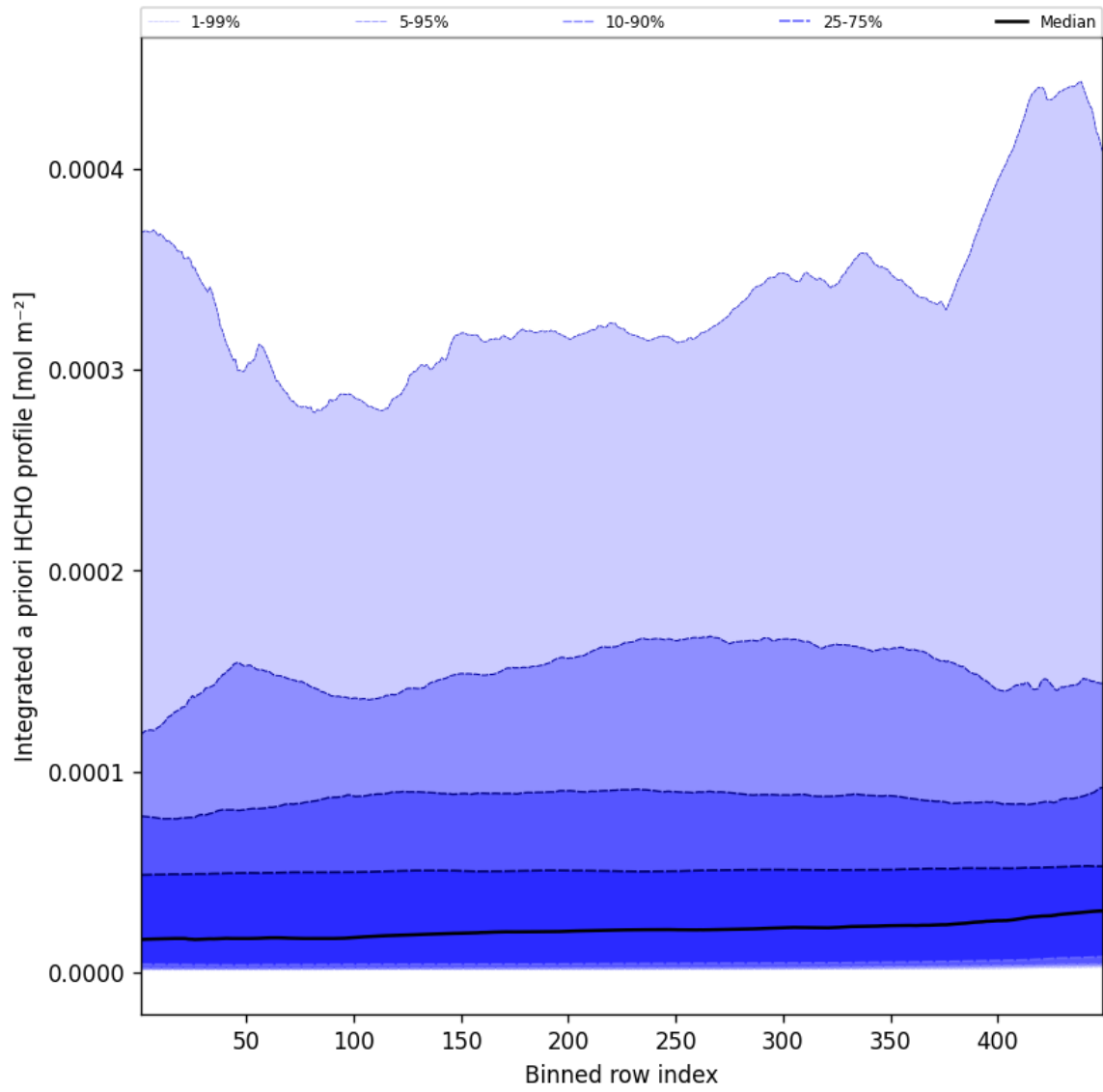
Figure 55: Along track statistics of “Integrated a priori HCHO profile” for 2024-12-05 to 2024-12-06
