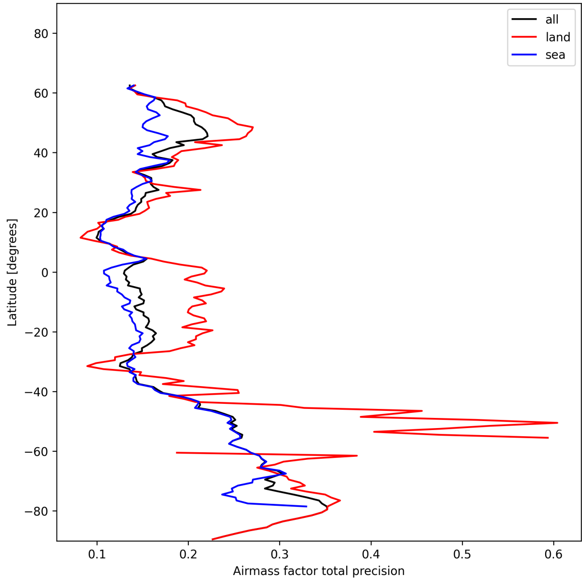
Figure 25: Zonal average of “Airmass factor total precision” for 2024-12-05 to 2024-12-06.
