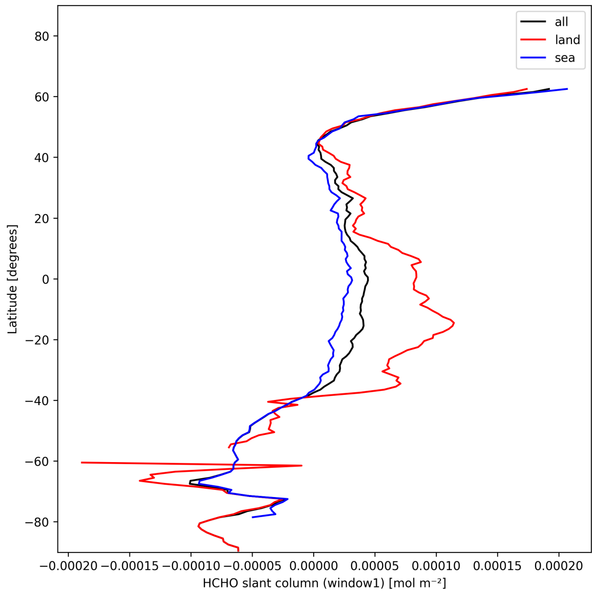
Figure 22: Zonal average of “HCHO slant column (window1)” for 2024-12-06 to 2024-12-07.
