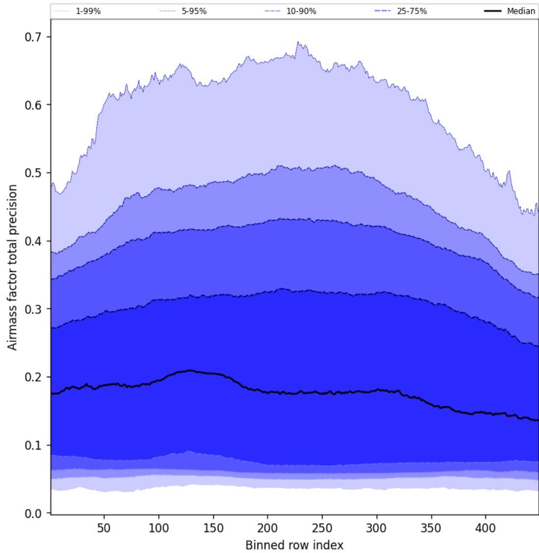
Figure 53: Along track statistics of “Airmass factor total precision” for 2024-12-06 to 2024-12-07
