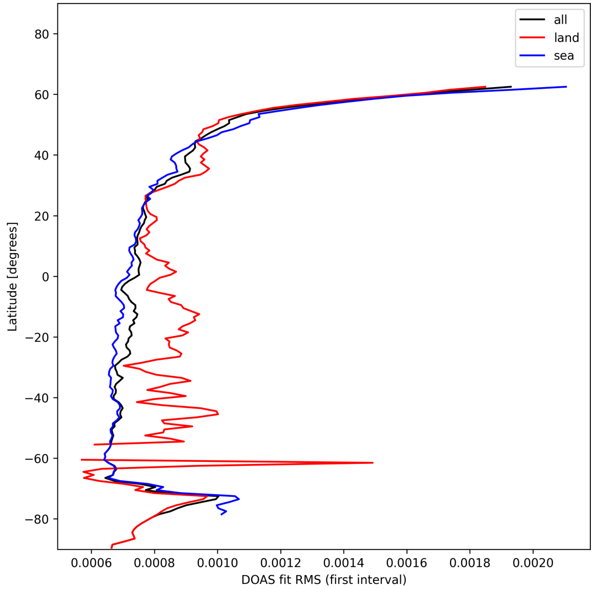
Figure 30: Zonal average of “DOAS fit RMS (first interval)” for 2024-12-06 to 2024-12-07.
