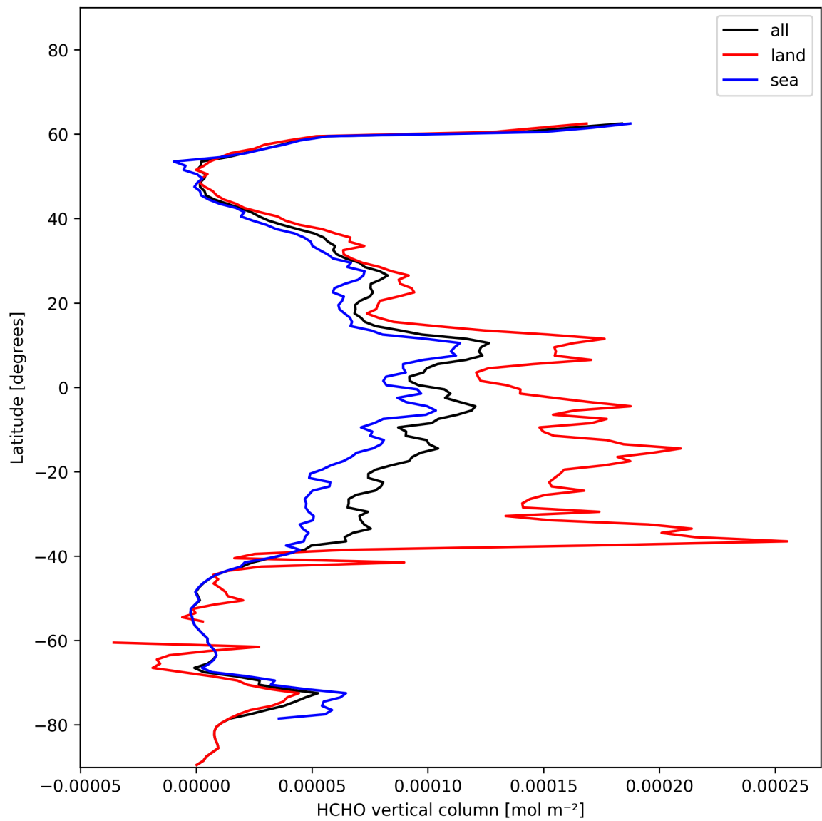
Figure 19: Zonal average of “HCHO vertical column” for 2024-12-06 to 2024-12-07.
