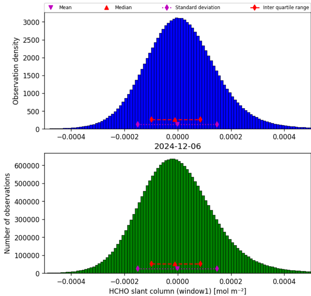
Figure 36: Histogram of “HCHO slant column (window1)” for 2024-12-06 to 2024-12-07
