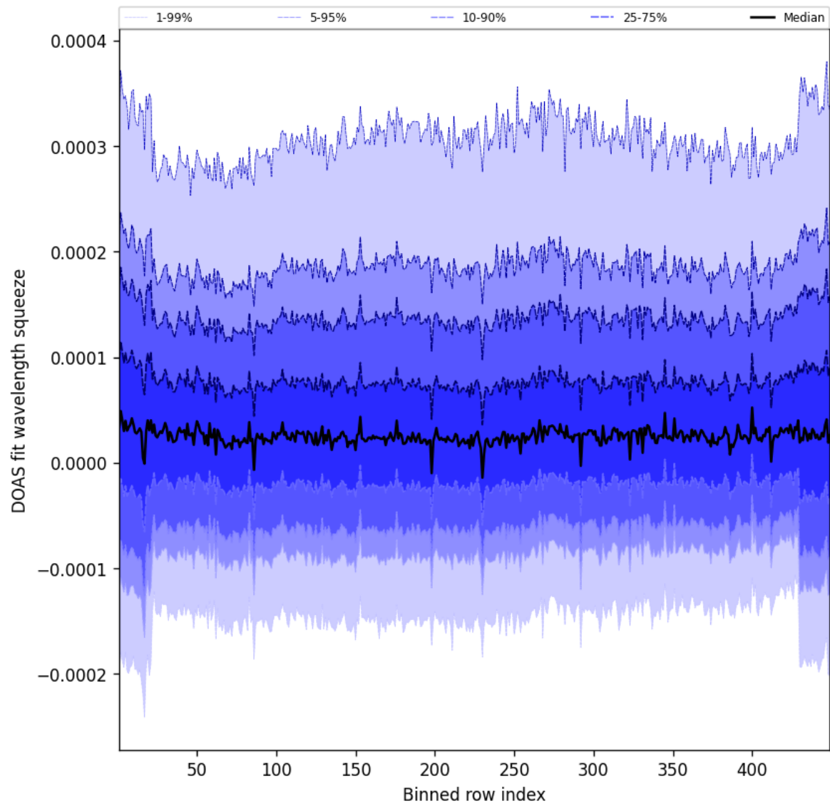
Figure 57: Along track statistics of “DOAS fit wavelength squeeze” for 2024-12-06 to 2024-12-07
