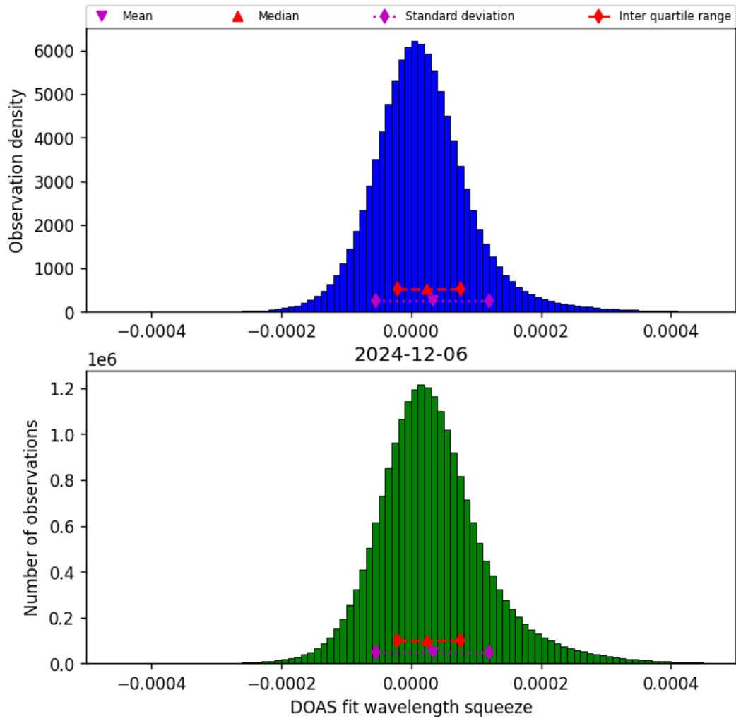
Figure 43: Histogram of “DOAS fit wavelength squeeze” for 2024-12-06 to 2024-12-07
