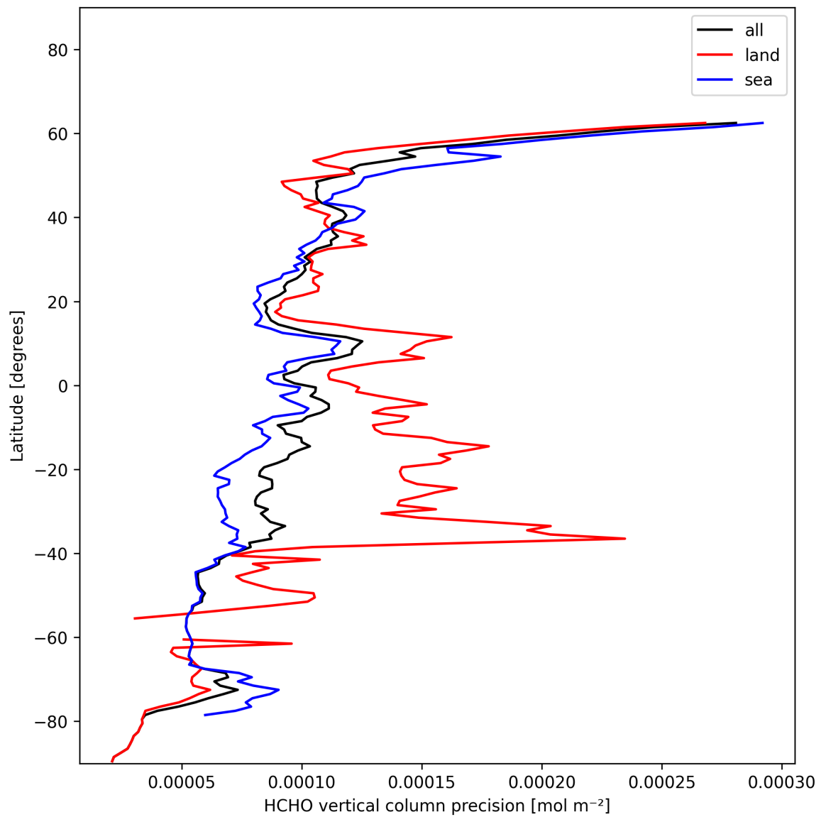
Figure 20: Zonal average of “HCHO vertical column precision” for 2024-12-06 to 2024-12-07.
