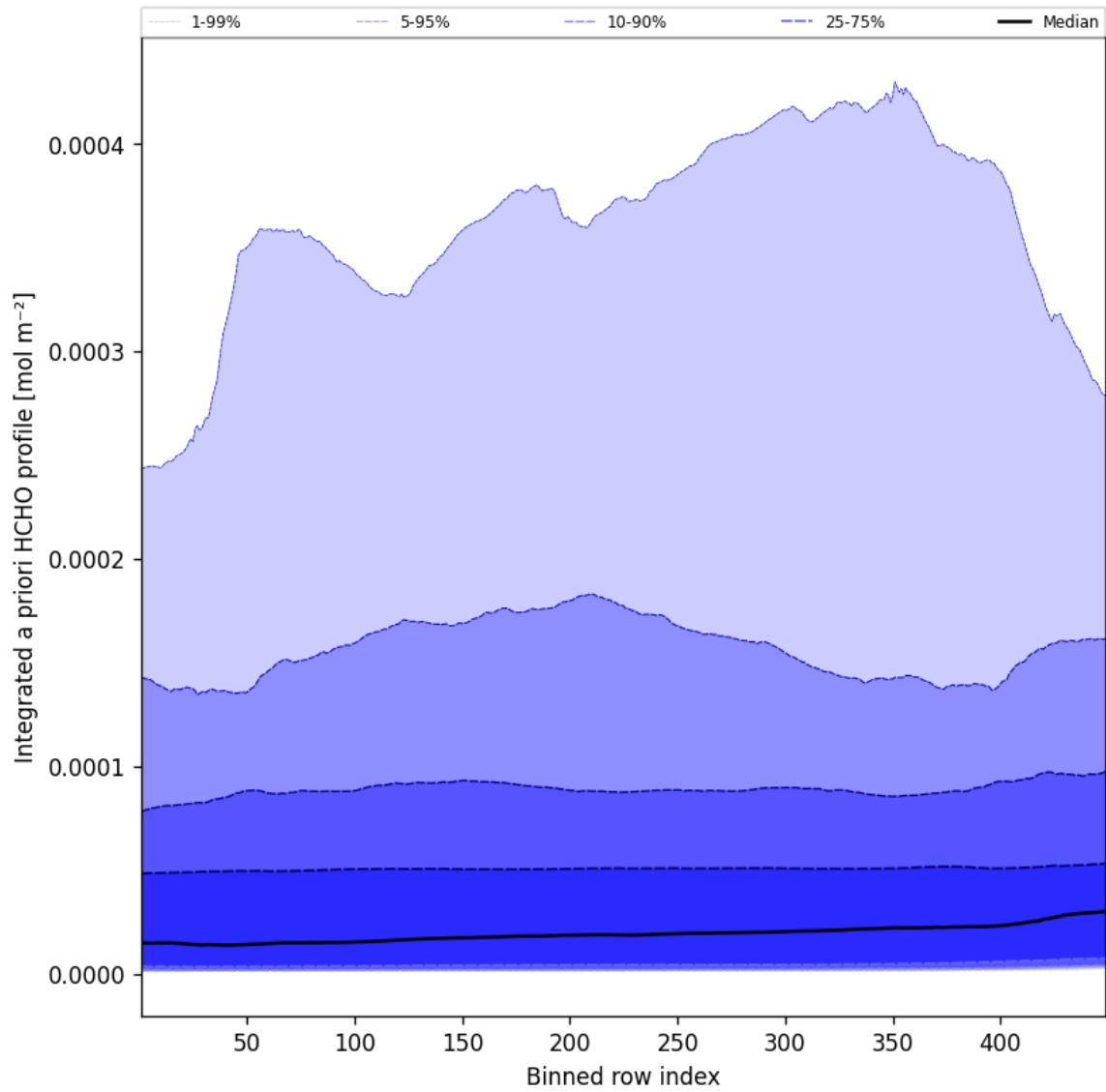
Figure 55: Along track statistics of “Integrated a priori HCHO profile” for 2024-12-06 to 2024-12-07
