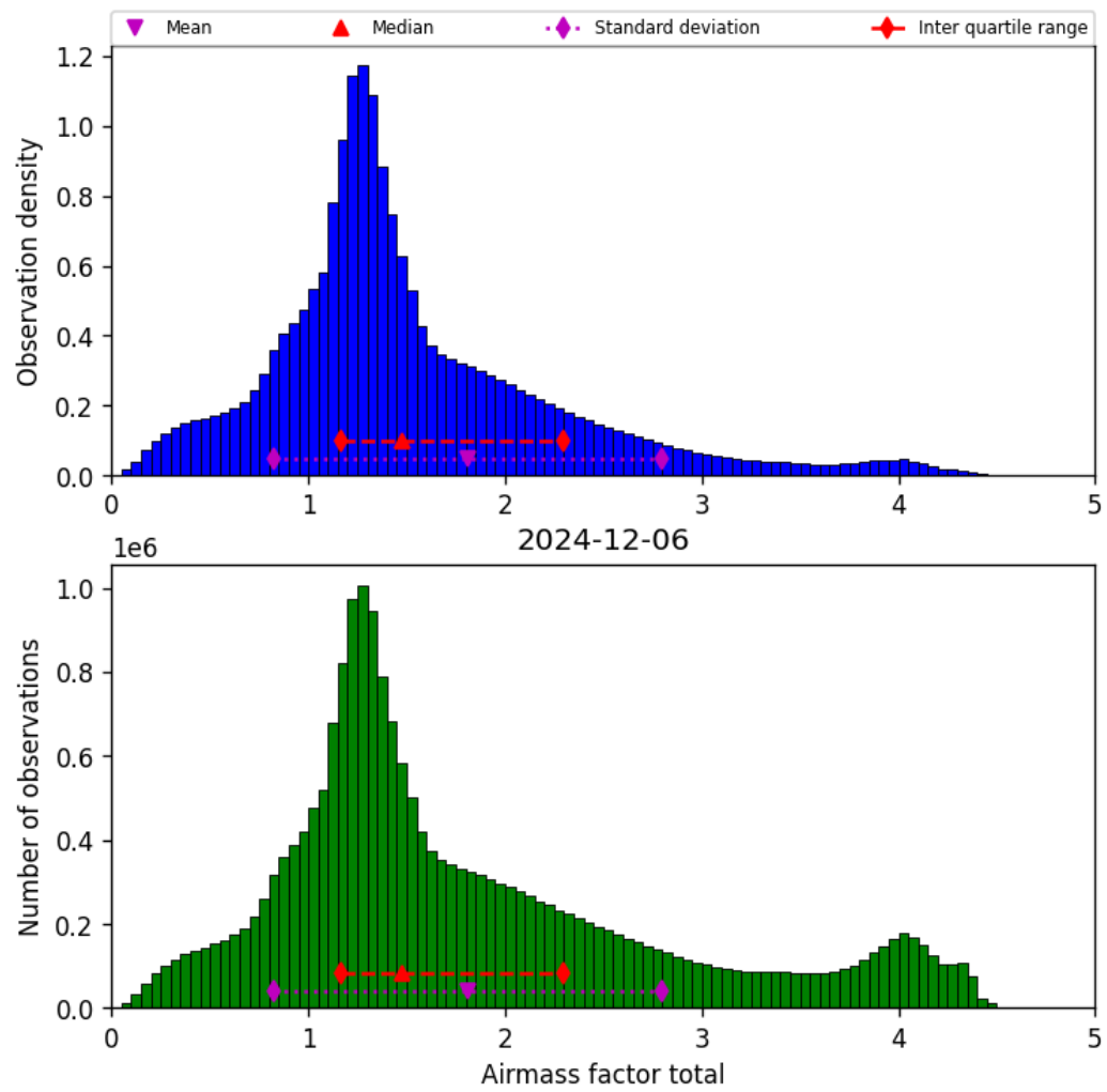
Figure 38: Histogram of “Airmass factor total” for 2024-12-06 to 2024-12-07
