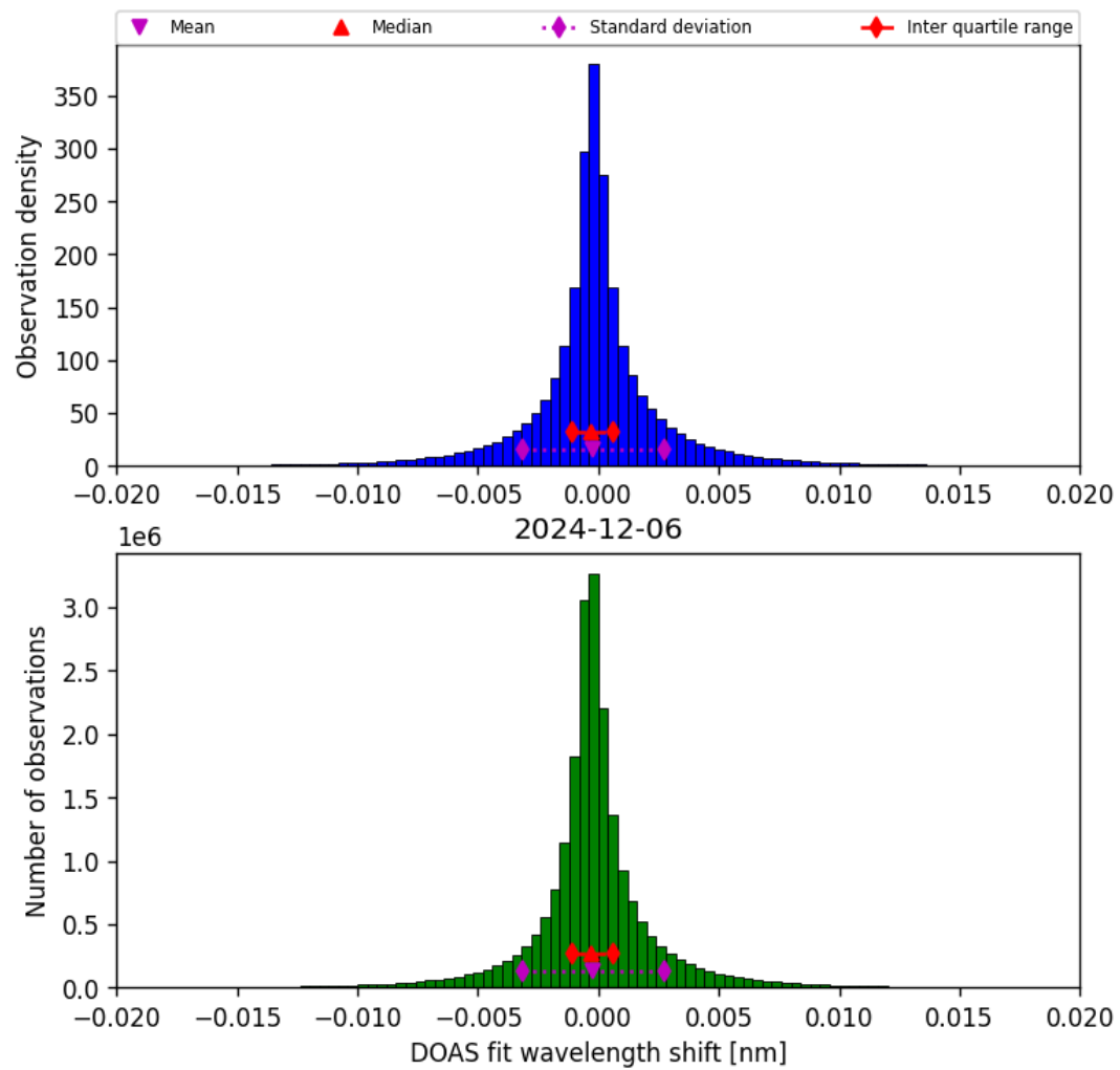
Figure 42: Histogram of “DOAS fit wavelength shift” for 2024-12-06 to 2024-12-07
