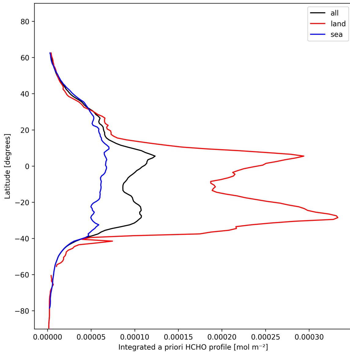
Figure 27: Zonal average of “Integrated a priori HCHO profile” for 2024-12-06 to 2024-12-07.
