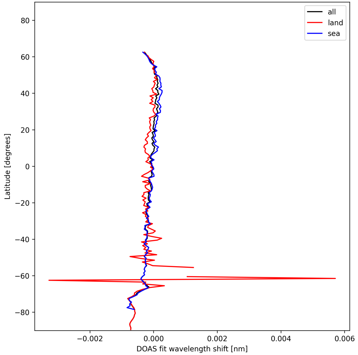
Figure 28: Zonal average of "DOAS fit wavelength shift" for 2024-12-06 to 2024-12-07.
