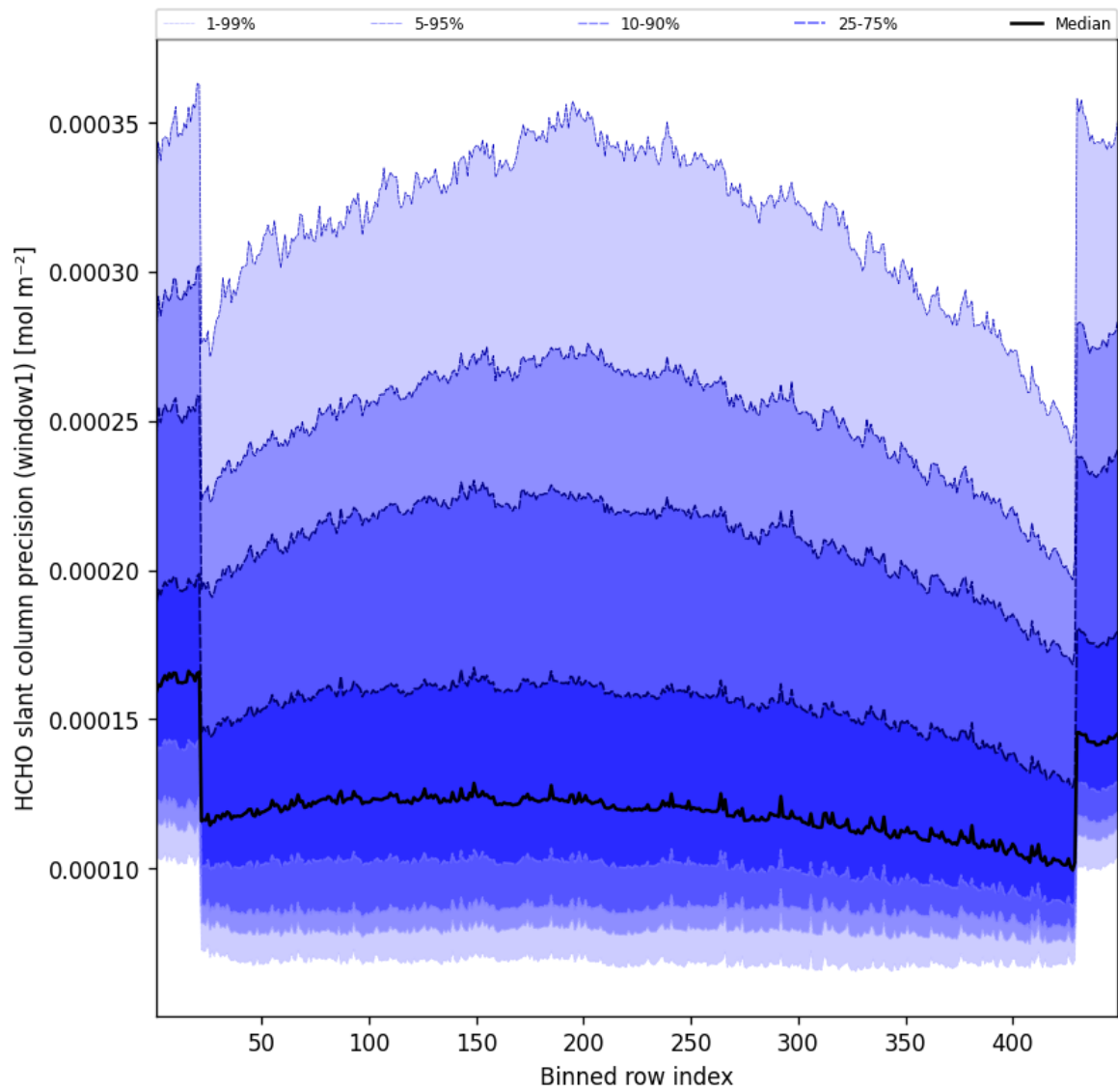
Figure 51: Along track statistics of “HCHO slant column precision (window1)” for 2024-12-06 to 2024-12-07
