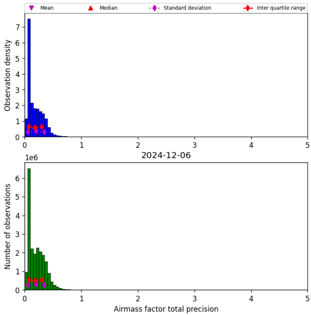
Figure 39: Histogram of “Airmass factor total precision” for 2024-12-06 to 2024-12-07
