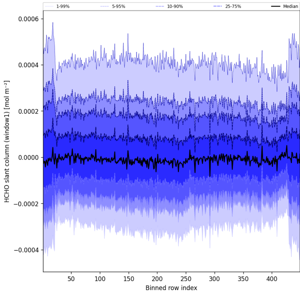
Figure 50: Along track statistics of “HCHO slant column (window1)” for 2024-12-06 to 2024-12-07
