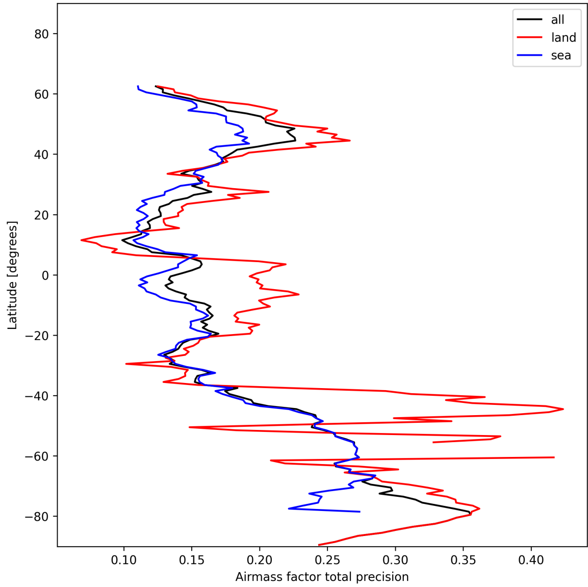
Figure 25: Zonal average of “Airmass factor total precision” for 2024-12-06 to 2024-12-07.
