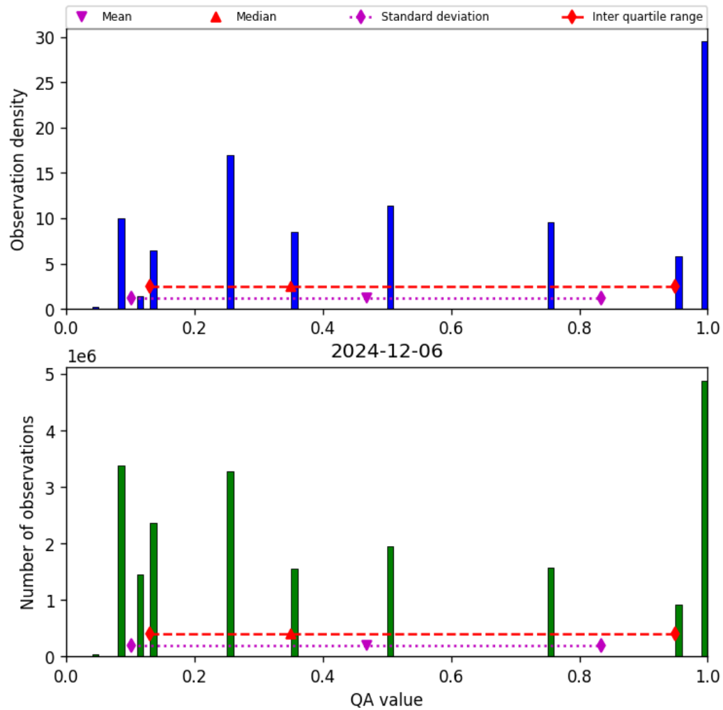
Figure 32: Histogram of “QA value” for 2024-12-06 to 2024-12-07
