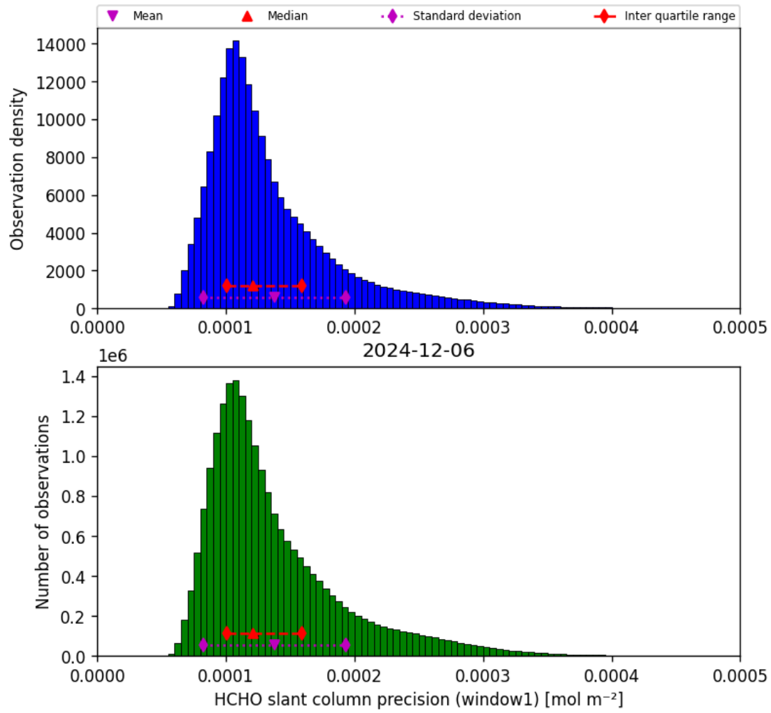
Figure 37: Histogram of “HCHO slant column precision (window1)” for 2024-12-06 to 2024-12-07
