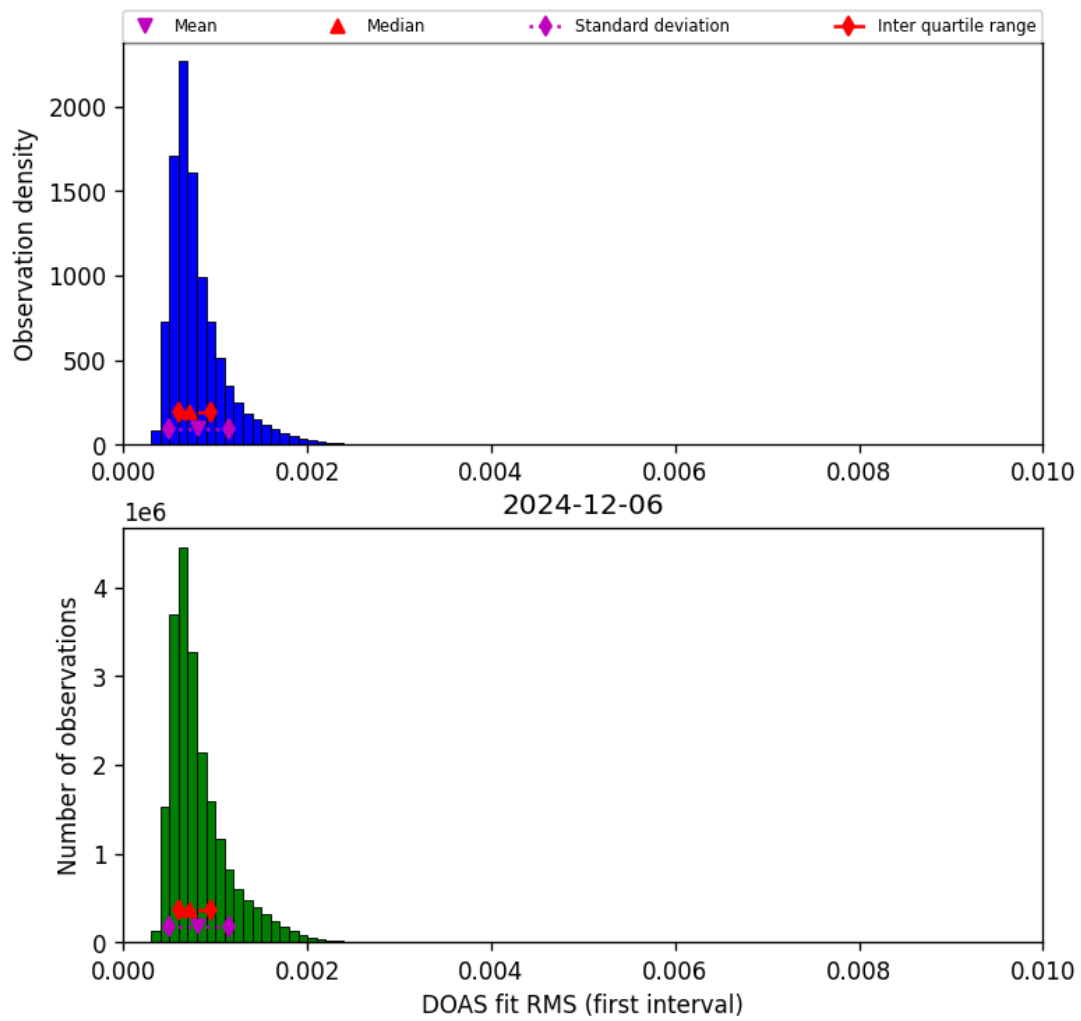
Figure 44: Histogram of “DOAS fit RMS (first interval)” for 2024-12-06 to 2024-12-07
