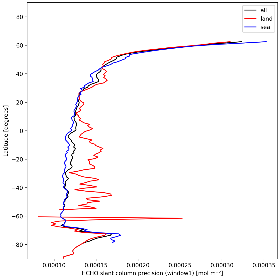
Figure 23: Zonal average of “HCHO slant column precision (window1)” for 2024-12-06 to 2024-12-07.
