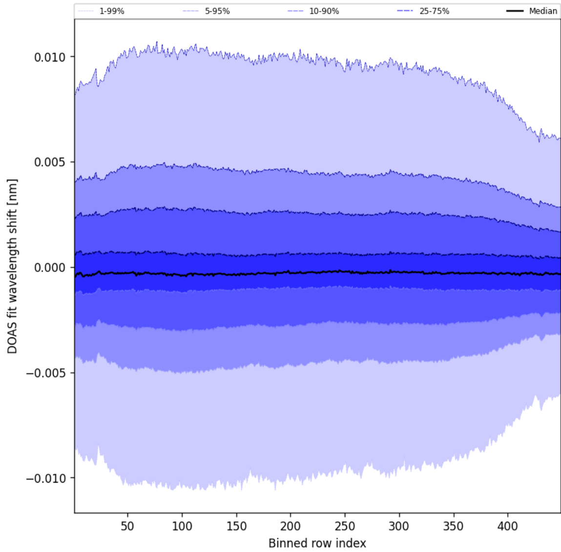
Figure 56: Along track statistics of “DOAS fit wavelength shift” for 2024-12-06 to 2024-12-07
