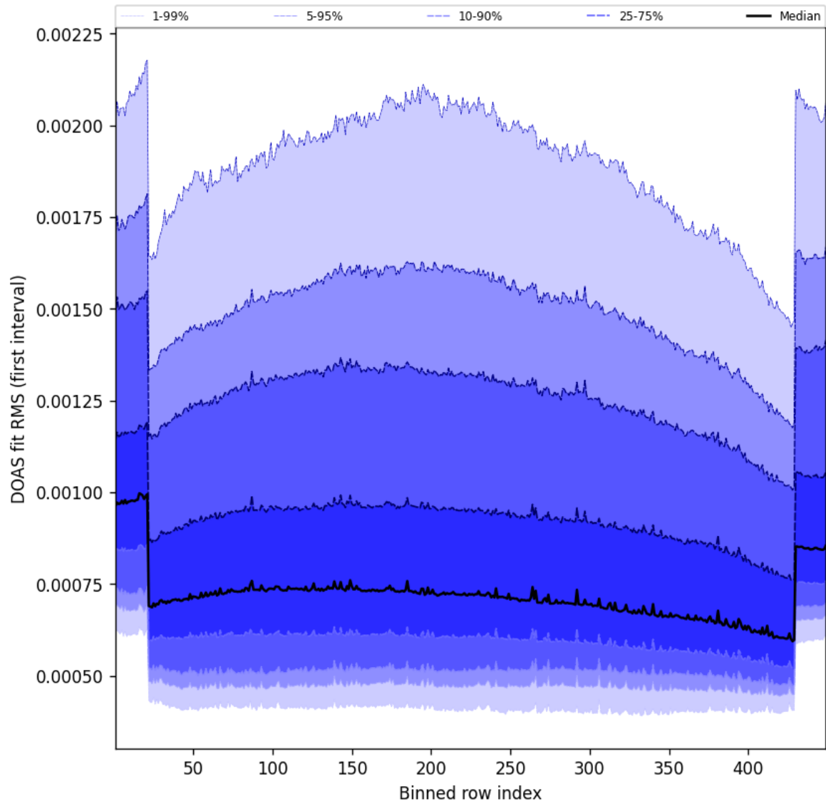
Figure 58: Along track statistics of “DOAS fit RMS (first interval)” for 2024-12-06 to 2024-12-07
