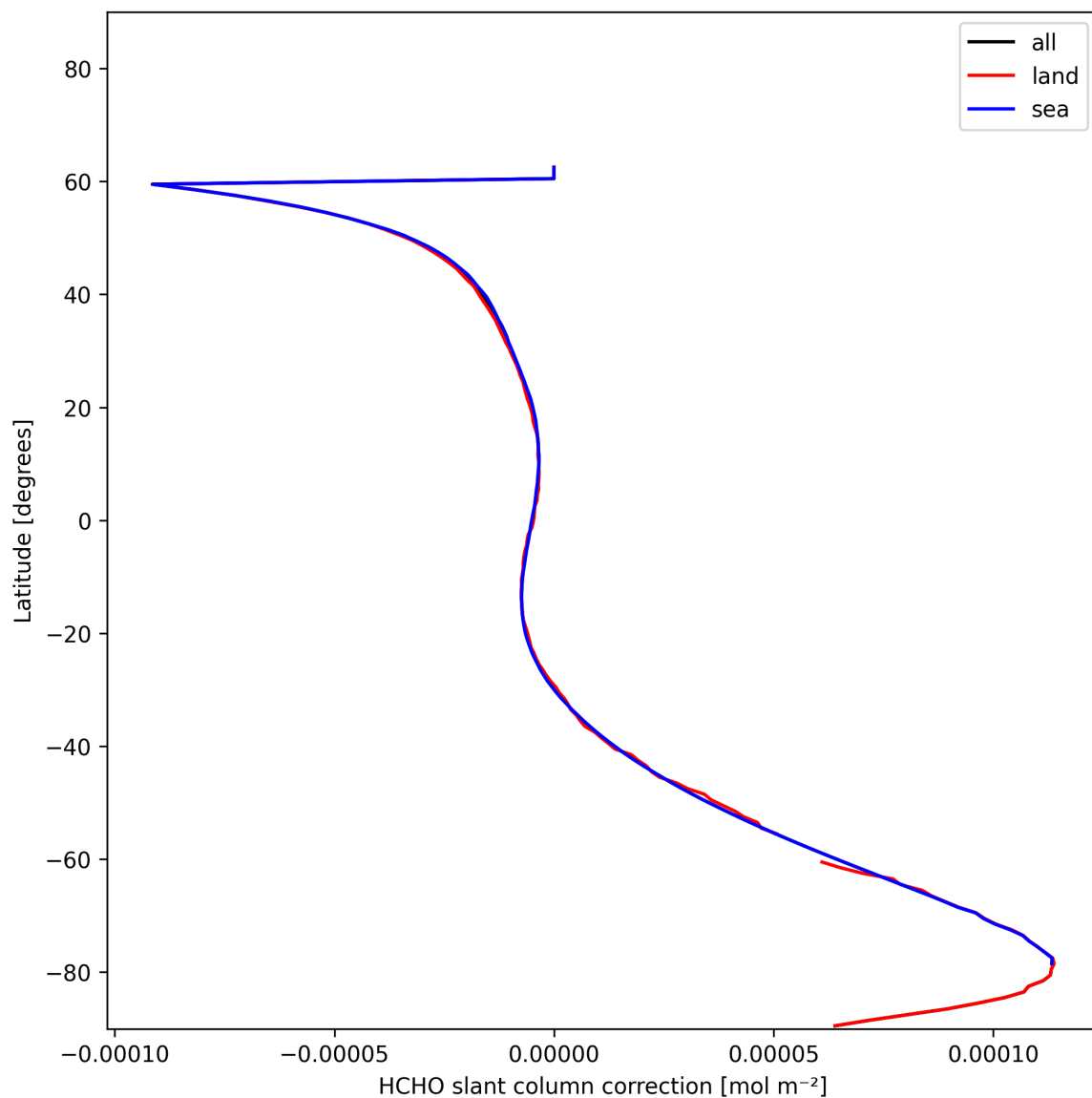
Figure 31: Zonal average of “HCHO slant column correction” for 2024-12-06 to 2024-12-07.
