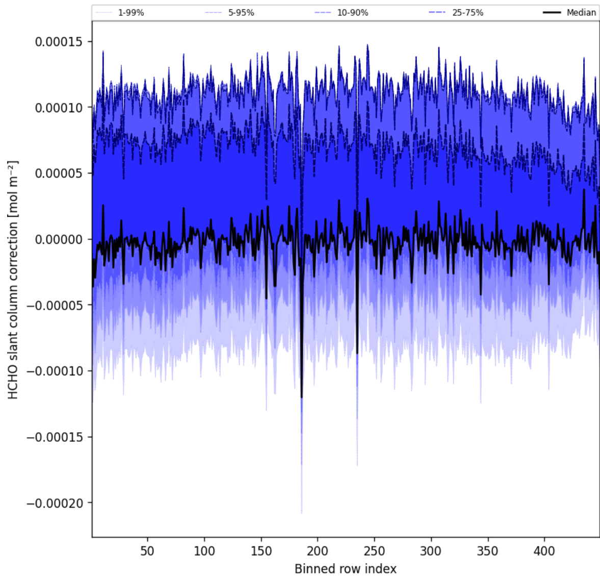
Figure 59: Along track statistics of “HCHO slant column correction” for 2024-12-06 to 2024-12-07
