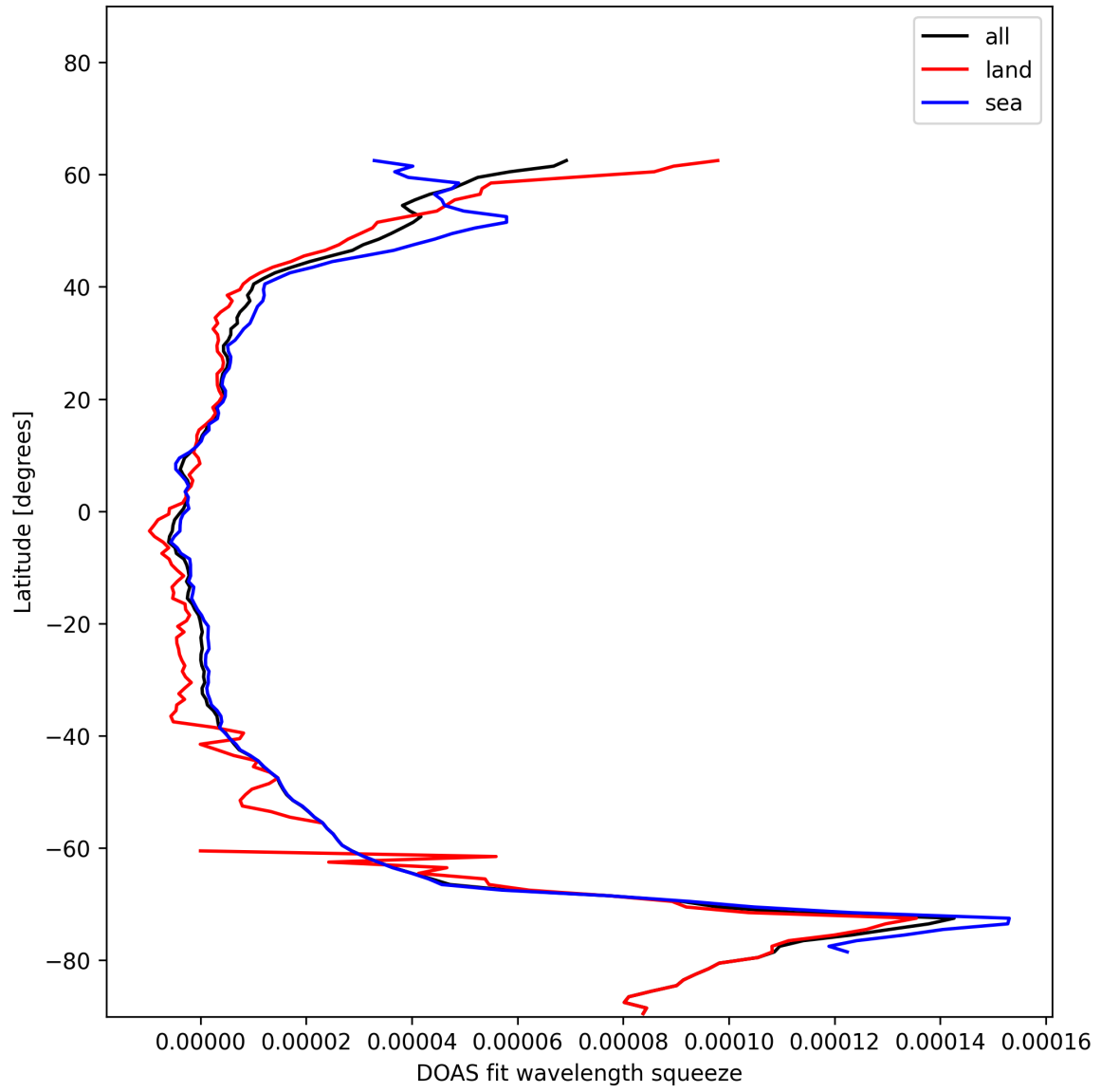
Figure 29: Zonal average of “DOAS fit wavelength squeeze” for 2024-12-06 to 2024-12-07.
