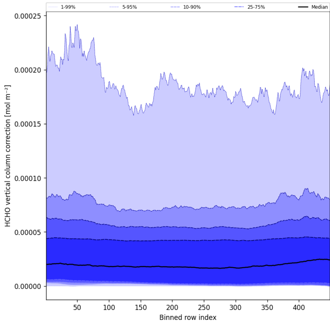
Figure 49: Along track statistics of “HCHO vertical column correction” for 2024-12-06 to 2024-12-07
