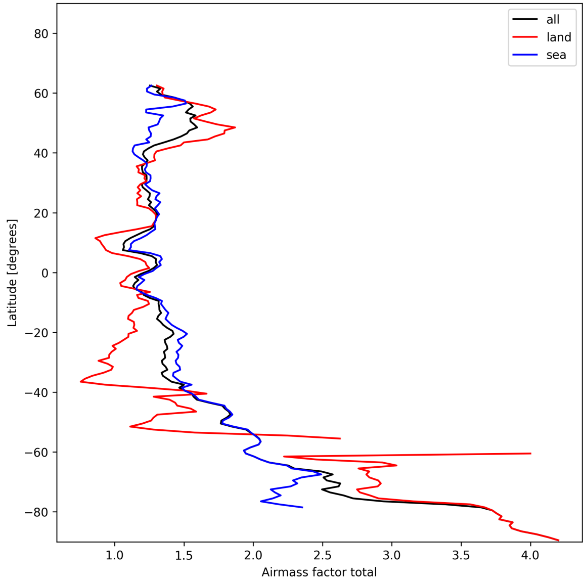
Figure 24: Zonal average of “Airmass factor total” for 2024-12-06 to 2024-12-07.
