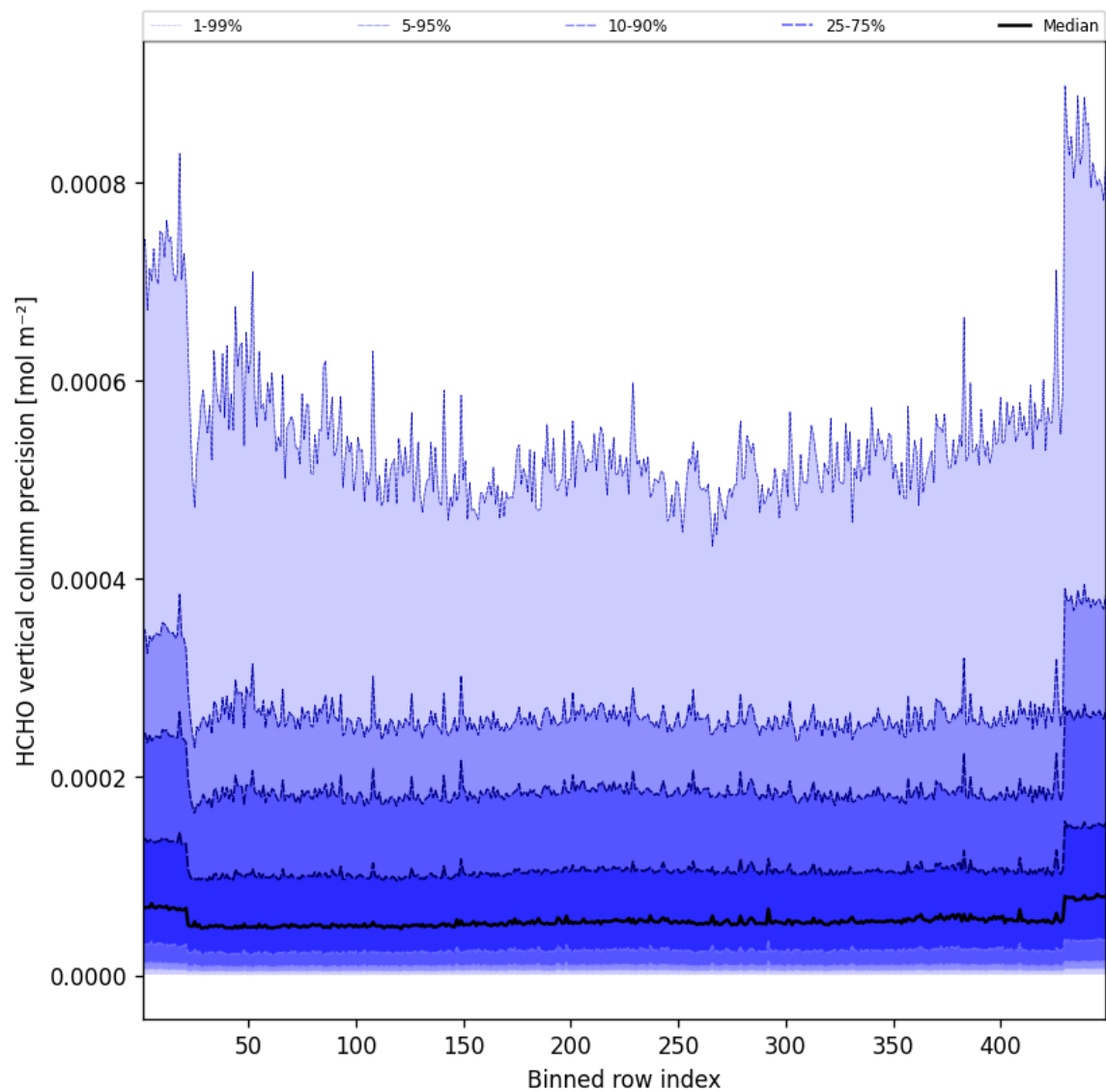
Figure 48: Along track statistics of “HCHO vertical column precision” for 2024-12-06 to 2024-12-07
