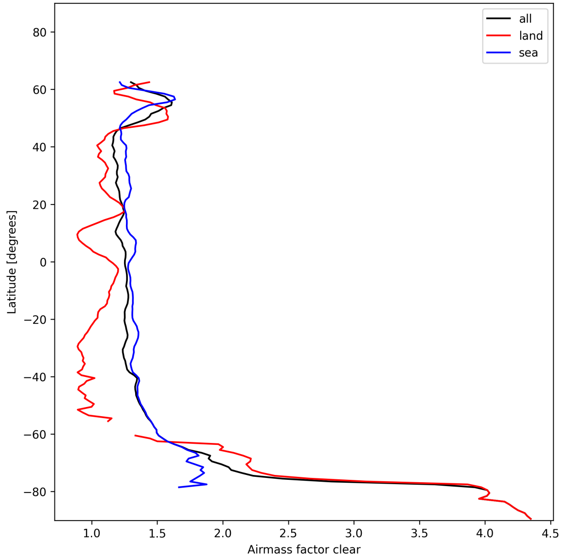
Figure 26: Zonal average of “Airmass factor clear” for 2024-12-06 to 2024-12-07.
