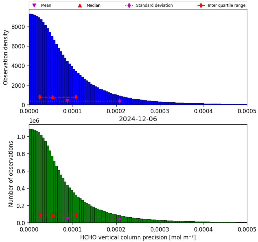
Figure 34: Histogram of “HCHO vertical column precision” for 2024-12-06 to 2024-12-07
