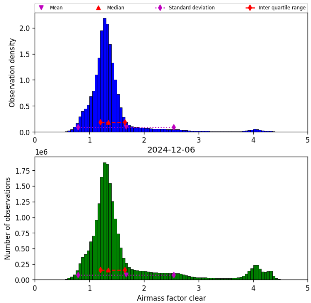
Figure 40: Histogram of “Airmass factor clear” for 2024-12-06 to 2024-12-07
