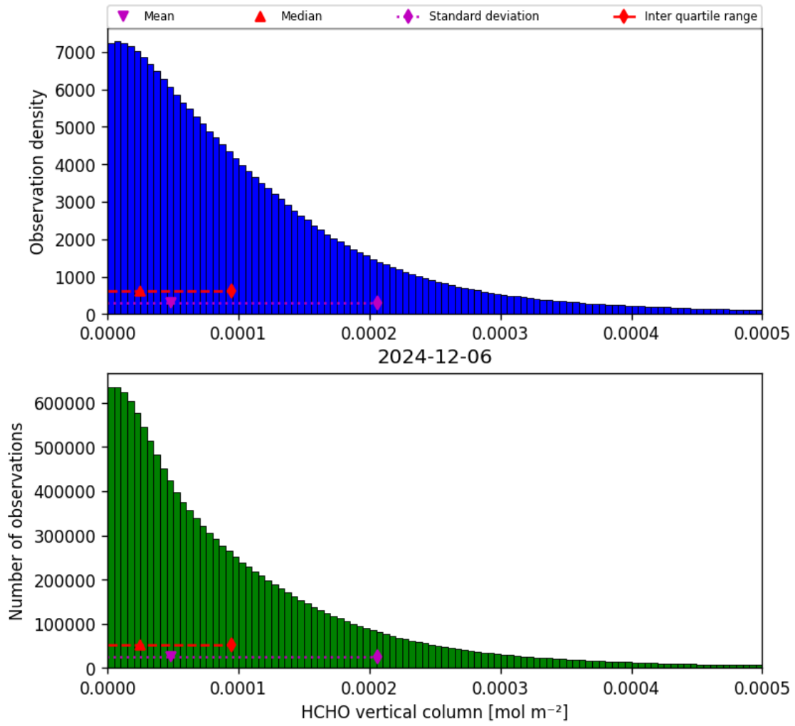
Figure 33: Histogram of “HCHO vertical column” for 2024-12-06 to 2024-12-07
