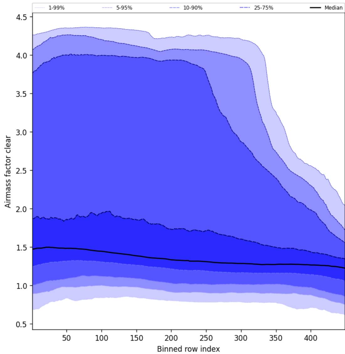
Figure 54: Along track statistics of “Airmass factor clear” for 2024-12-06 to 2024-12-07
