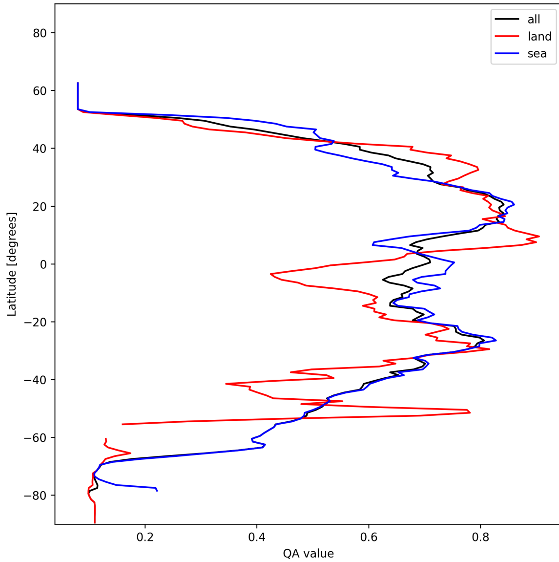
Figure 18: Zonal average of “QA value” for 2024-12-06 to 2024-12-07.
