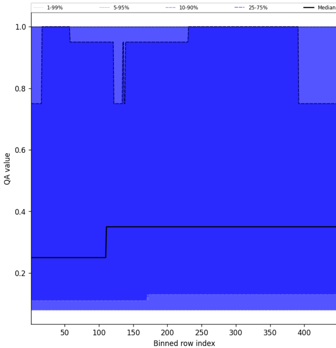
Figure 46: Along track statistics of “QA value” for 2024-12-06 to 2024-12-07
