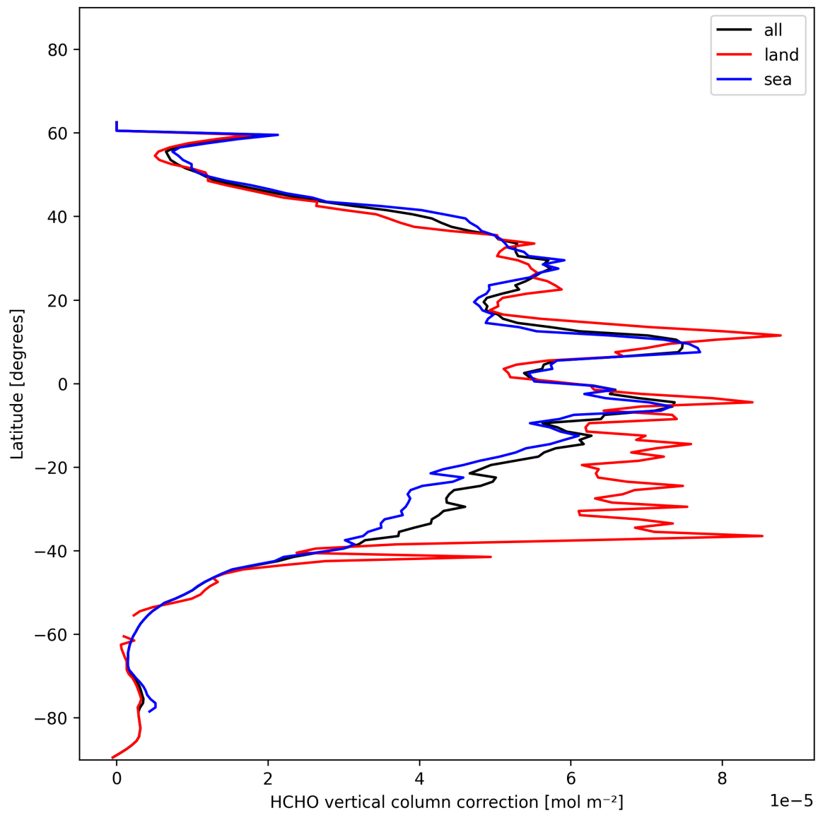
Figure 21: Zonal average of “HCHO vertical column correction” for 2024-12-06 to 2024-12-07.
