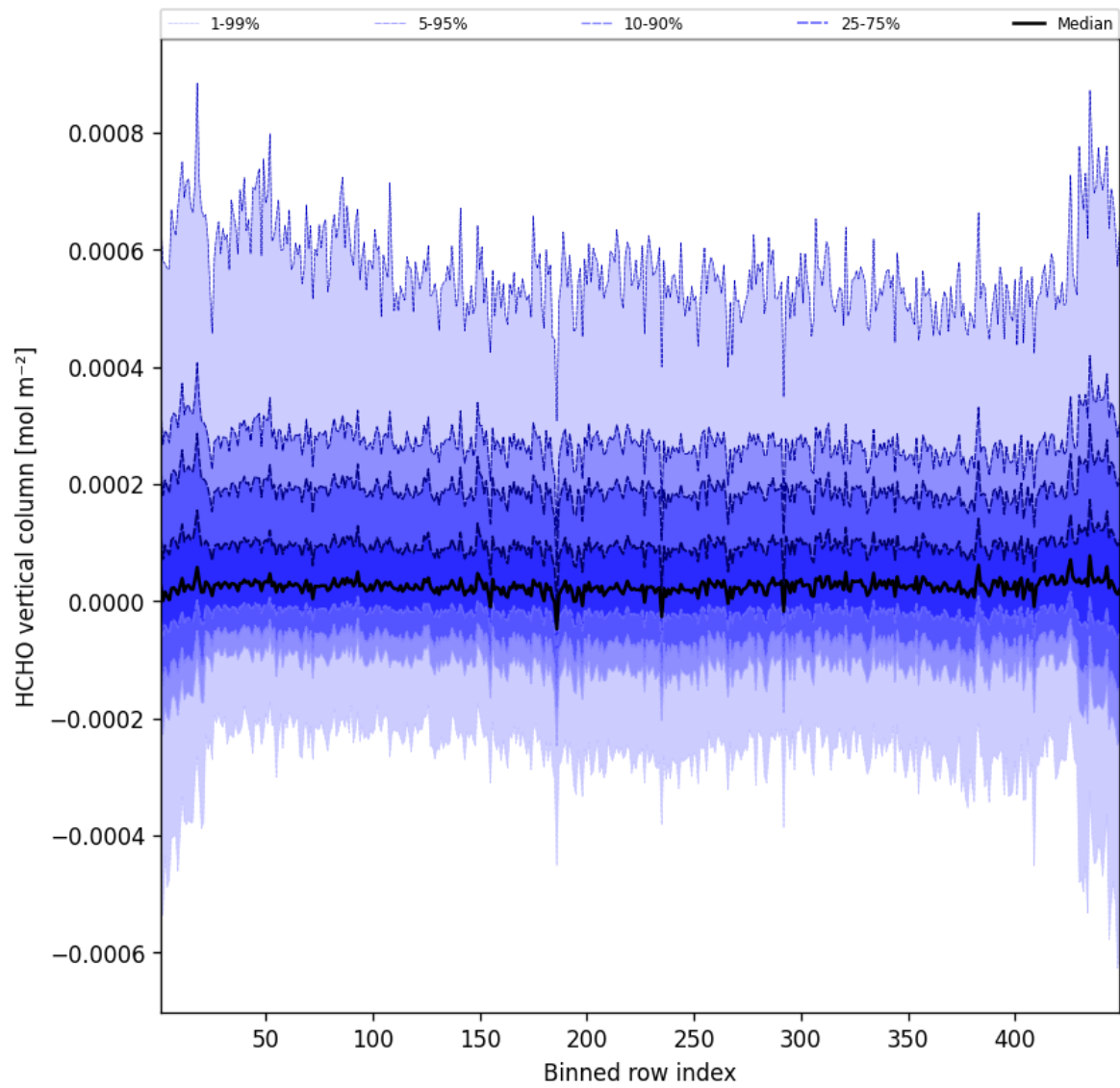
Figure 47: Along track statistics of “HCHO vertical column” for 2024-12-06 to 2024-12-07
