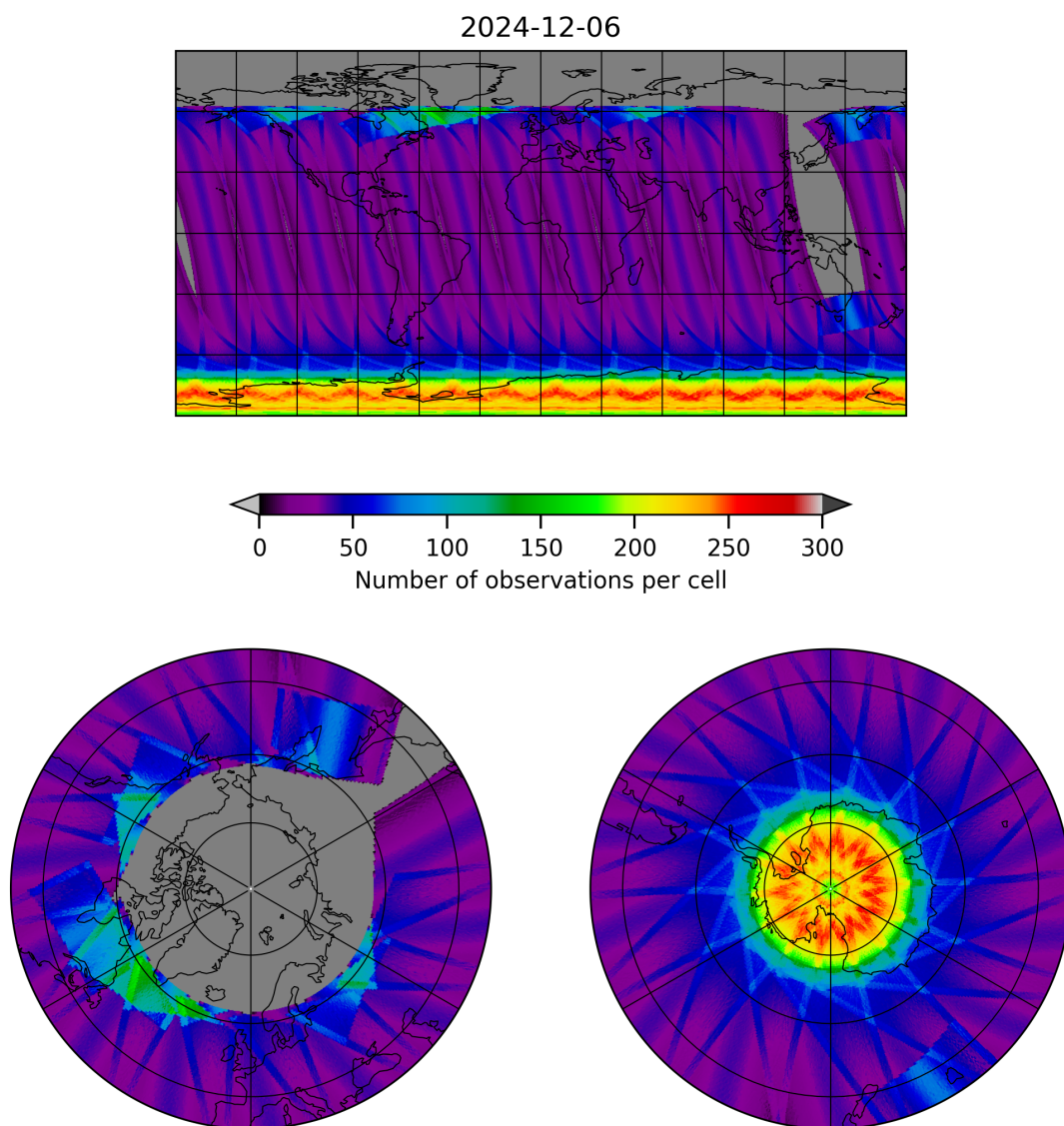
Figure 17: Map of the number of observations for 2024-12-06 to 2024-12-07
