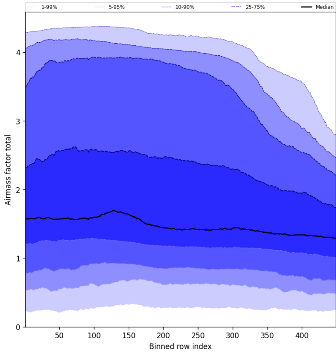
Figure 52: Along track statistics of “Airmass factor total” for 2024-12-06 to 2024-12-07
