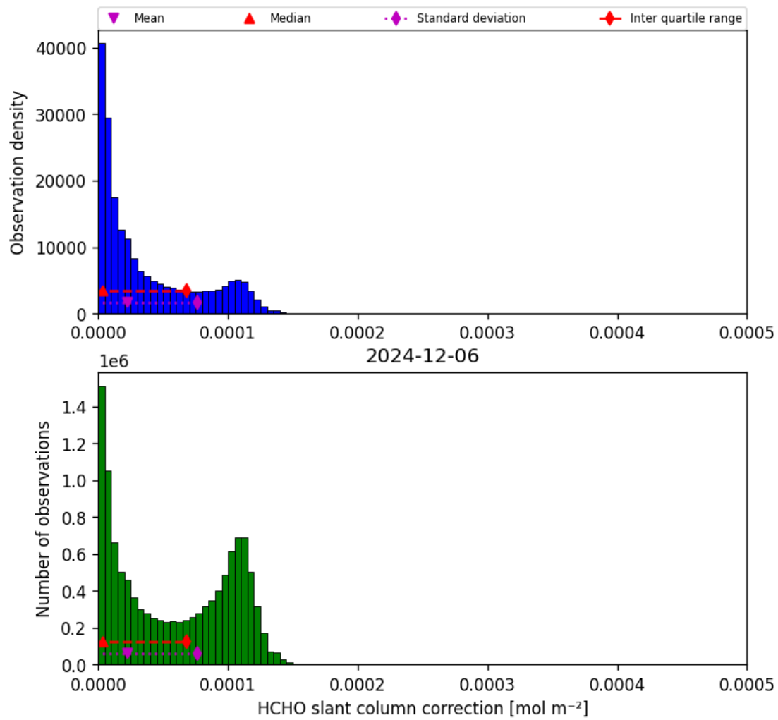
Figure 45: Histogram of “HCHO slant column correction” for 2024-12-06 to 2024-12-07
