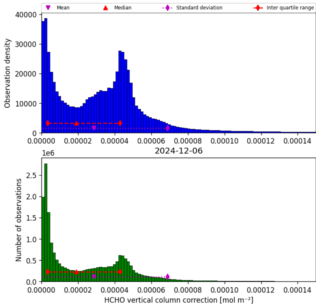
Figure 35: Histogram of “HCHO vertical column correction” for 2024-12-06 to 2024-12-07
