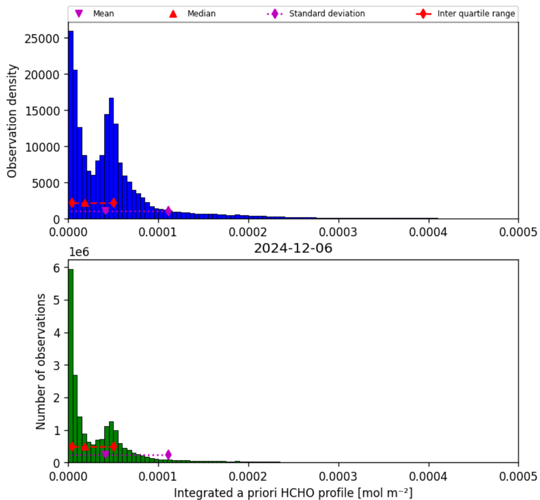
Figure 41: Histogram of “Integrated a priori HCHO profile” for 2024-12-06 to 2024-12-07
