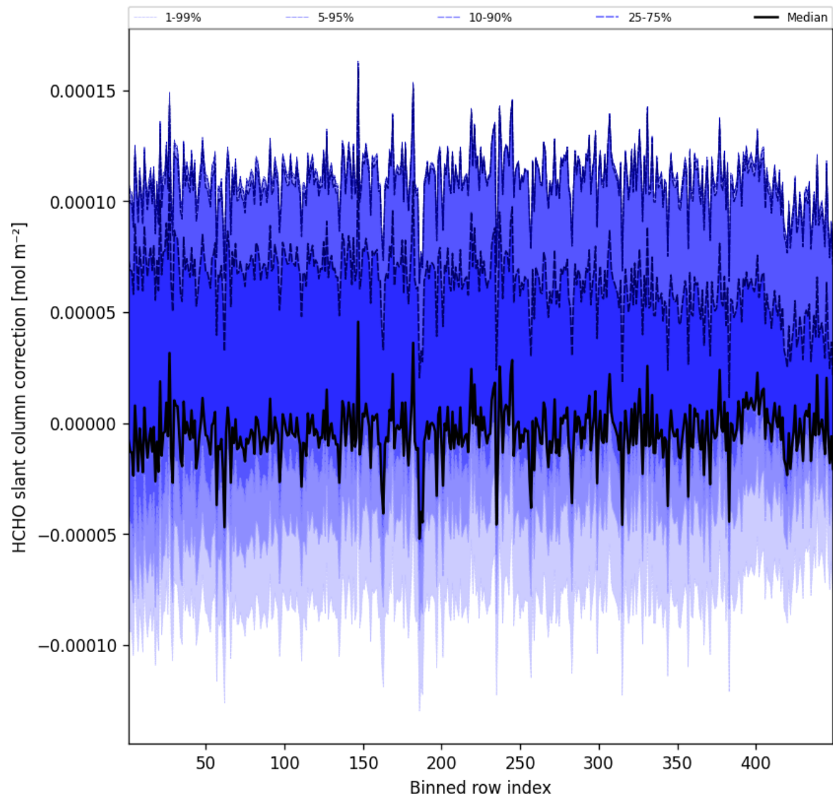
Figure 59: Along track statistics of “HCHO slant column correction” for 2024-12-08 to 2024-12-09
