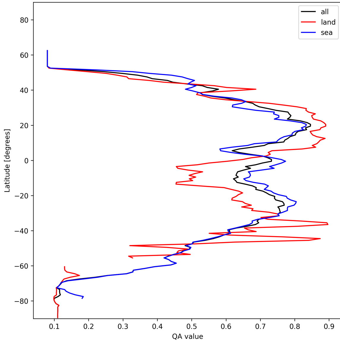
Figure 18: Zonal average of “QA value” for 2024-12-08 to 2024-12-09.
