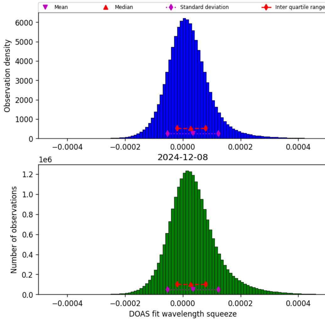
Figure 43: Histogram of “DOAS fit wavelength squeeze” for 2024-12-08 to 2024-12-09
