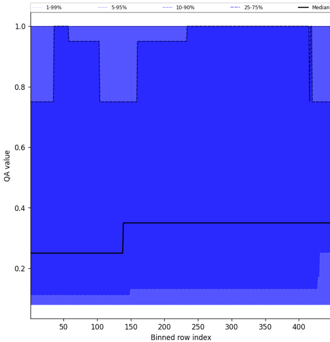
Figure 46: Along track statistics of “QA value” for 2024-12-08 to 2024-12-09
