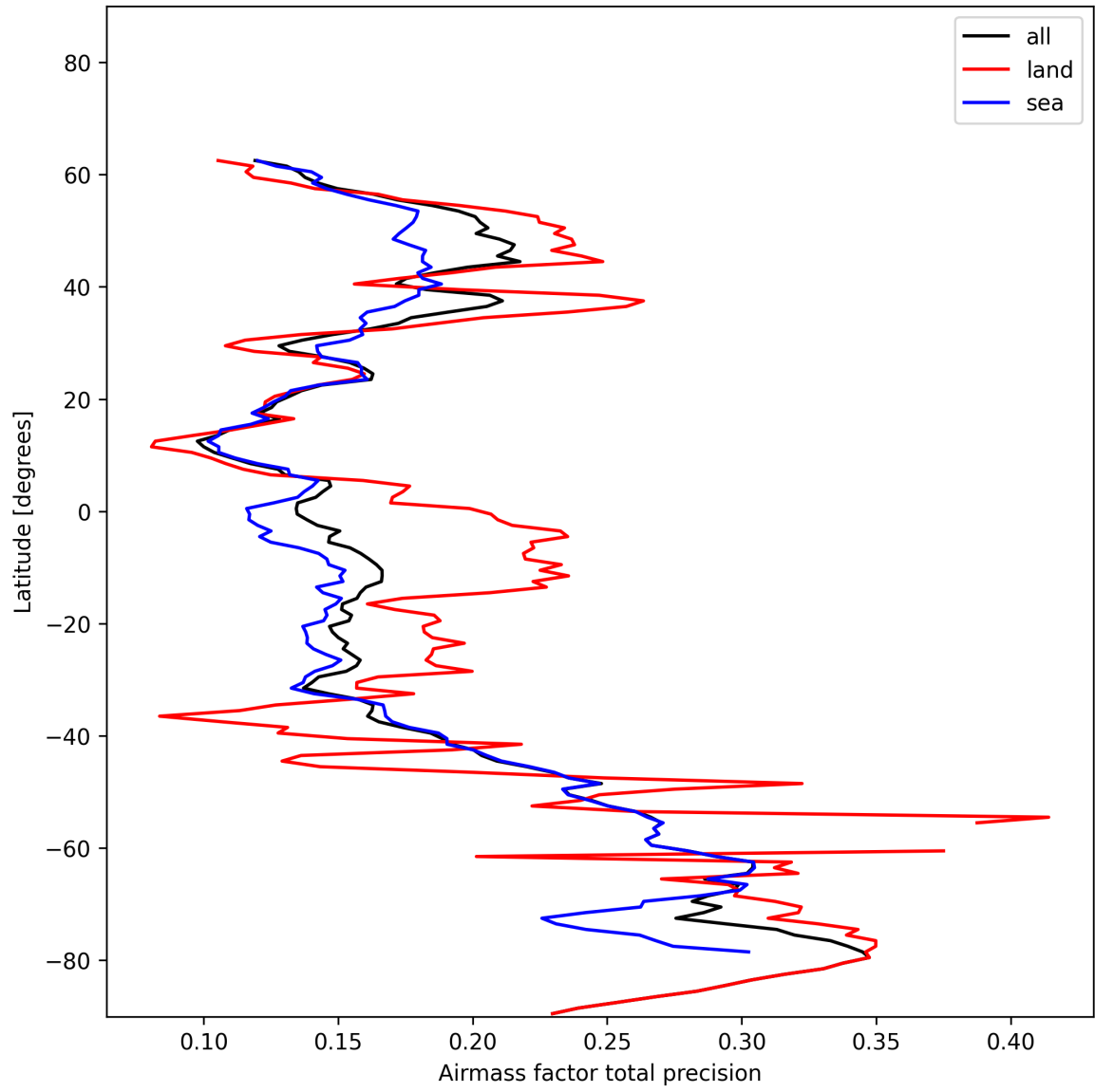
Figure 25: Zonal average of “Airmass factor total precision” for 2024-12-08 to 2024-12-09.
