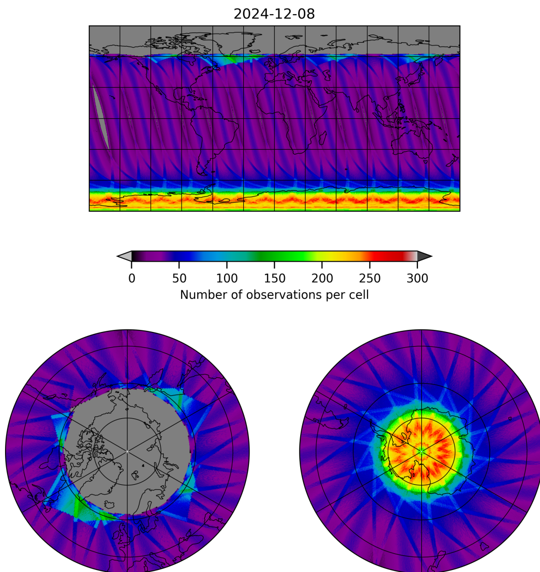
Figure 17: Map of the number of observations for 2024-12-08 to 2024-12-09
