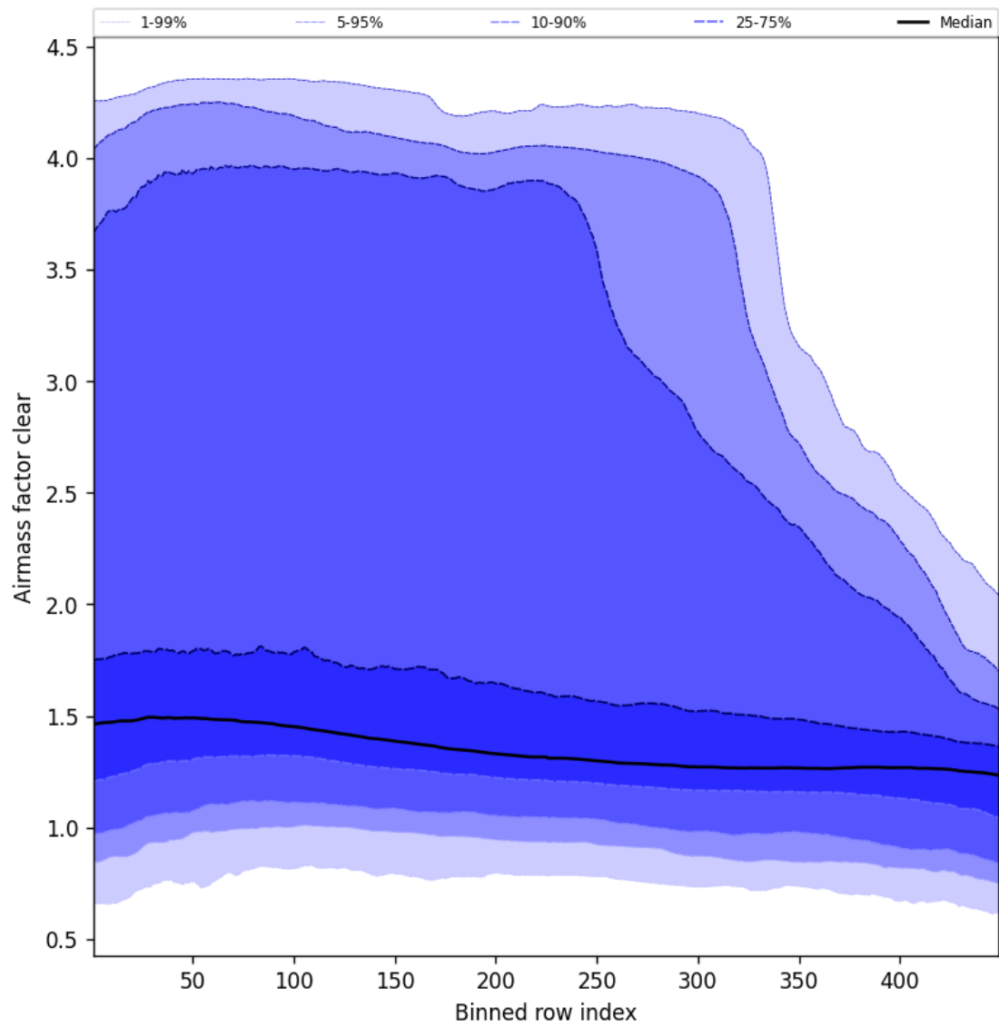
Figure 54: Along track statistics of “Air mass factor clear” for 2024-12-08 to 2024-12-09
