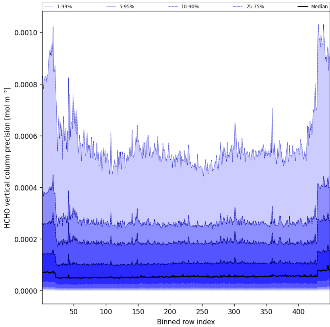
Figure 48: Along track statistics of “HCHO vertical column precision” for 2024-12-08 to 2024-12-09
