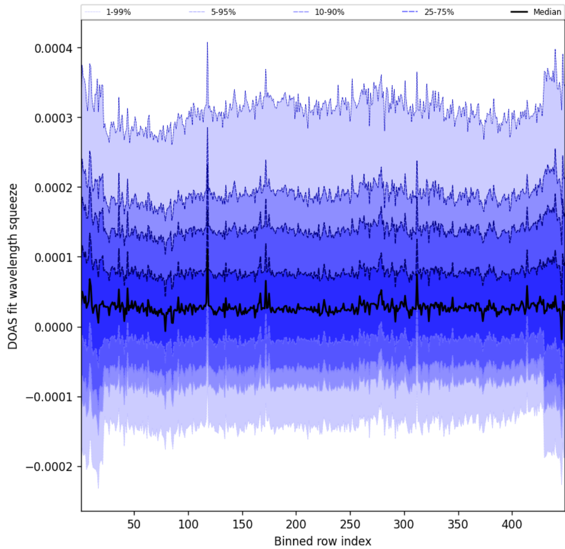
Figure 57: Along track statistics of “DOAS fit wavelength squeeze” for 2024-12-08 to 2024-12-09
