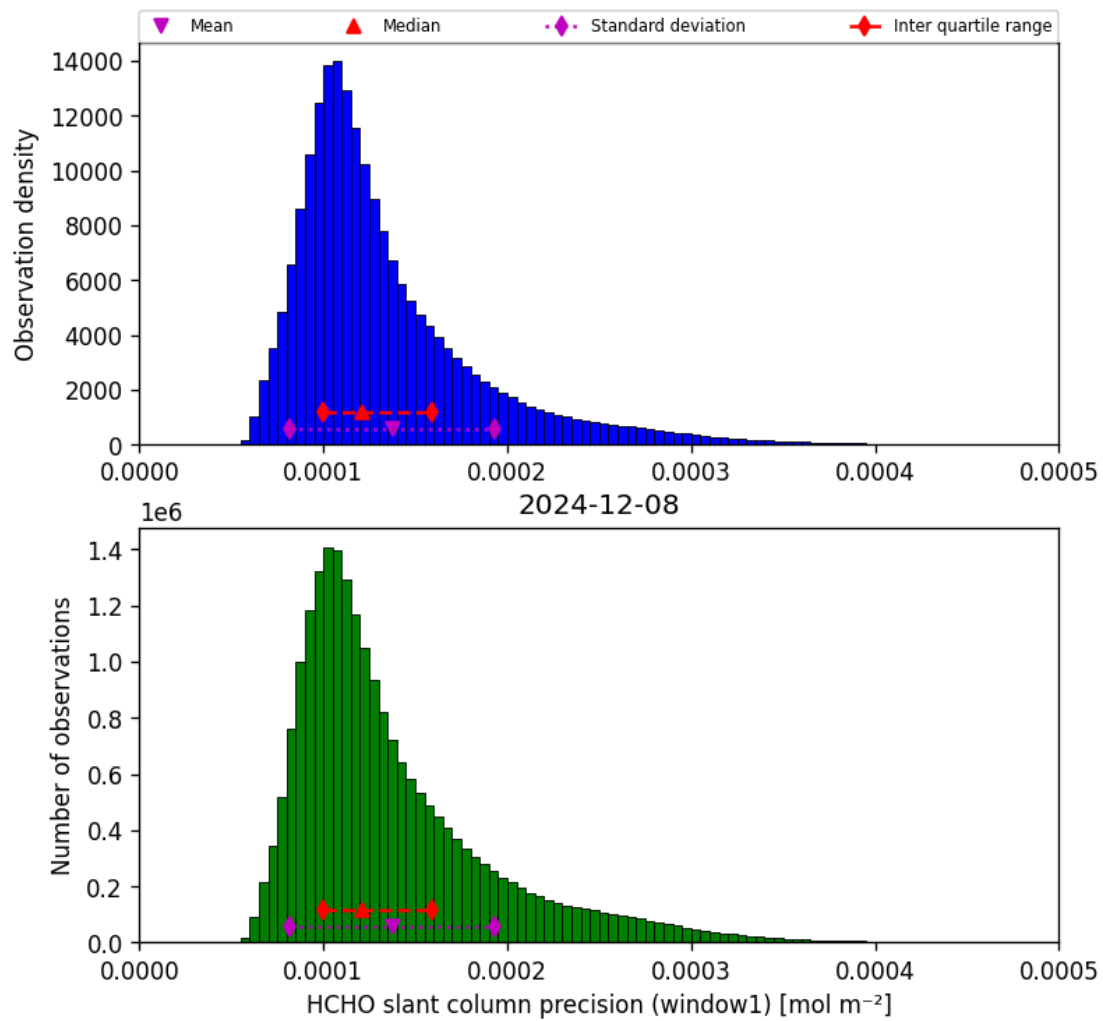
Figure 37: Histogram of “HCHO slant column precision (window1)” for 2024-12-08 to 2024-12-09
