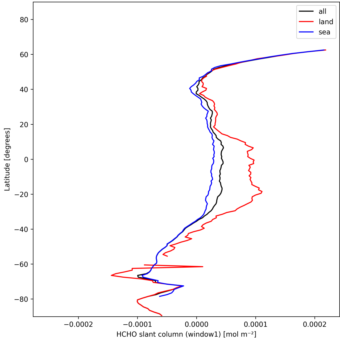
Figure 22: Zonal average of “HCHO slant column (window1)” for 2024-12-08 to 2024-12-09.
