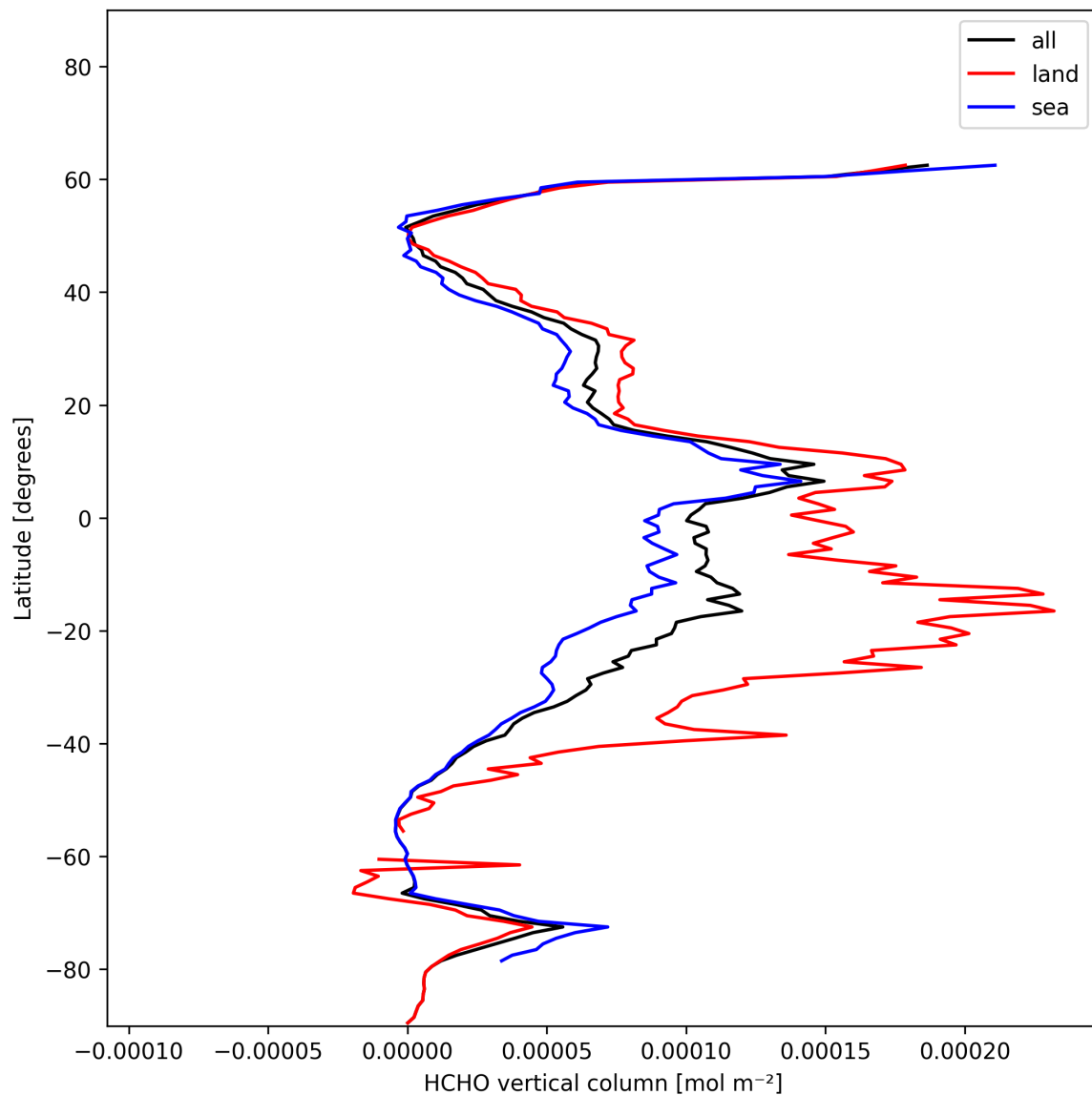
Figure 19: Zonal average of “HCHO vertical column” for 2024-12-08 to 2024-12-09.
