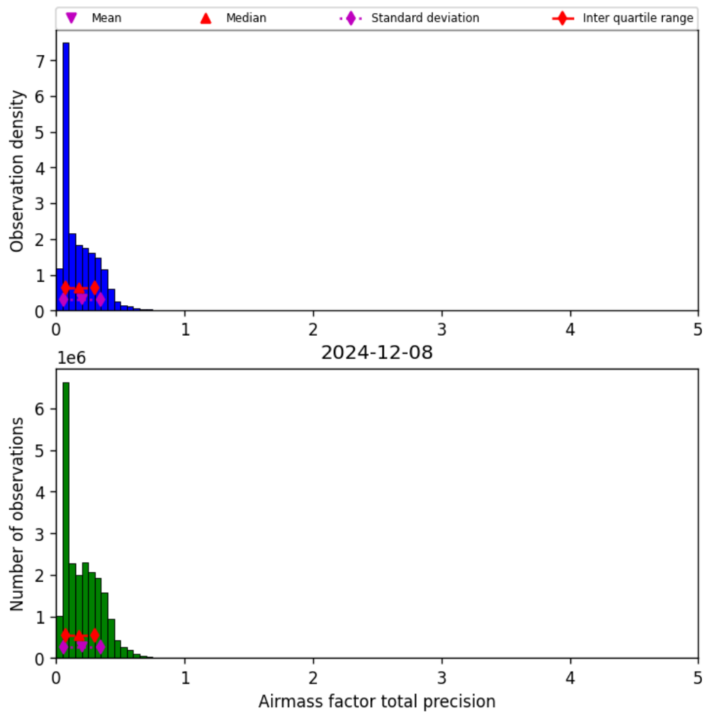
Figure 39: Histogram of “Airmass factor total precision” for 2024-12-08 to 2024-12-09
