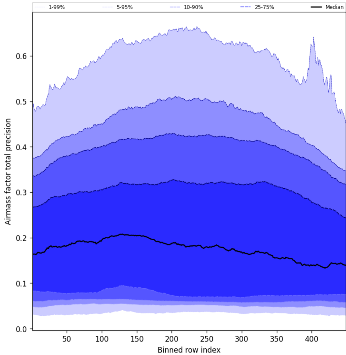
Figure 53: Along track statistics of “Airmass factor total precision” for 2024-12-08 to 2024-12-09
