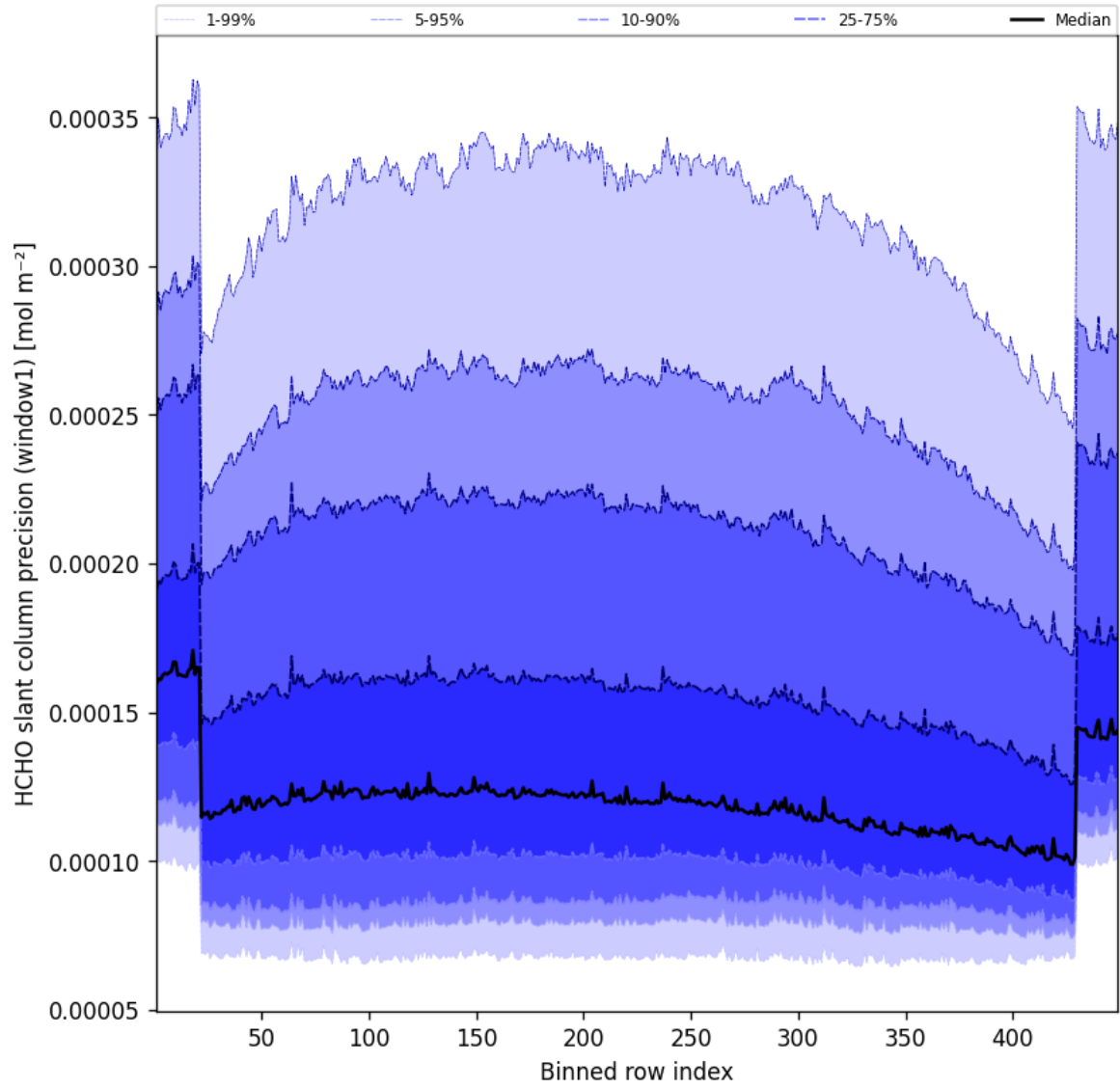
Figure 51: Along track statistics of “HCHO slant column precision (window1)” for 2024-12-08 to 2024-12-09
