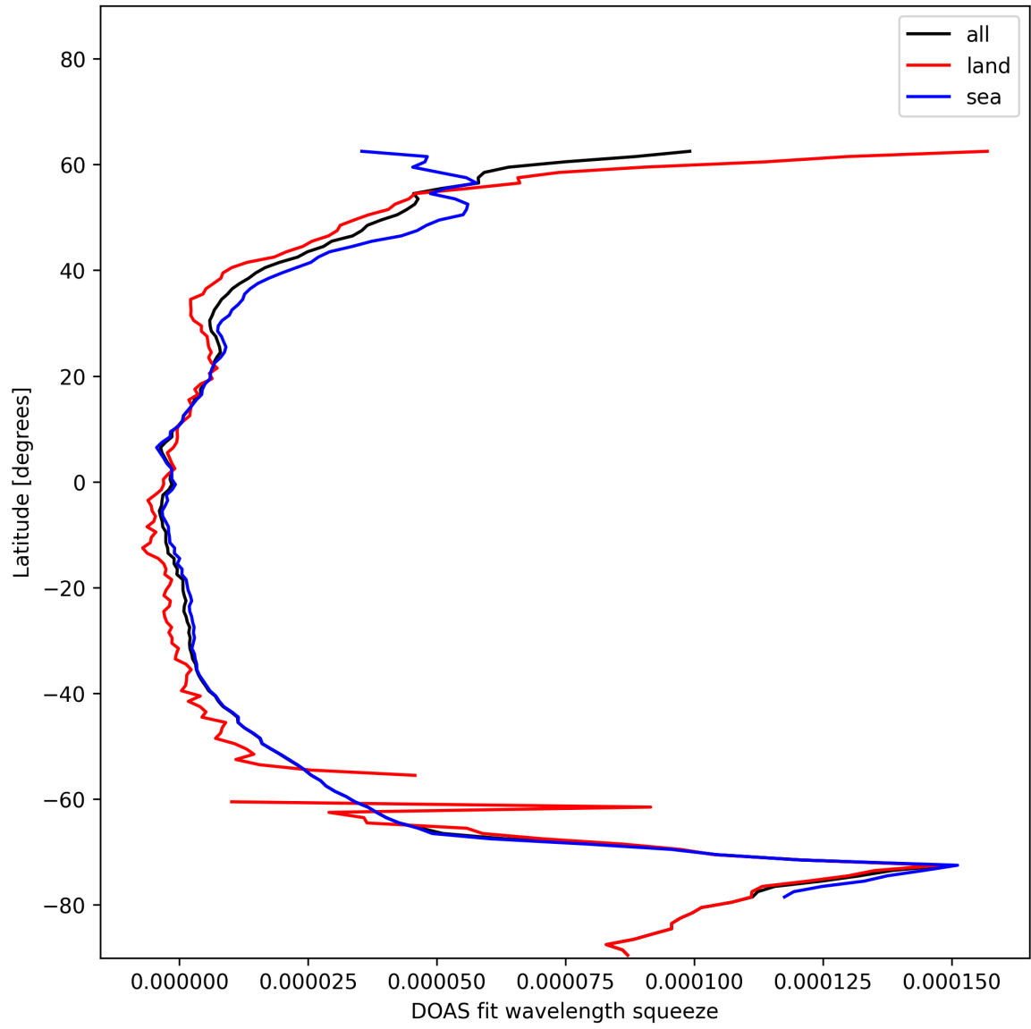
Figure 29: Zonal average of “DOAS fit wavelength squeeze” for 2024-12-08 to 2024-12-09.
