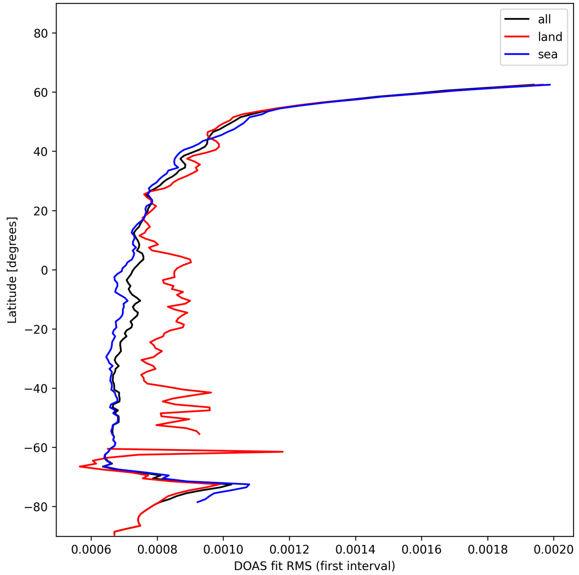
Figure 30: Zonal average of “DOAS fit RMS (first interval)” for 2024-12-08 to 2024-12-09.
