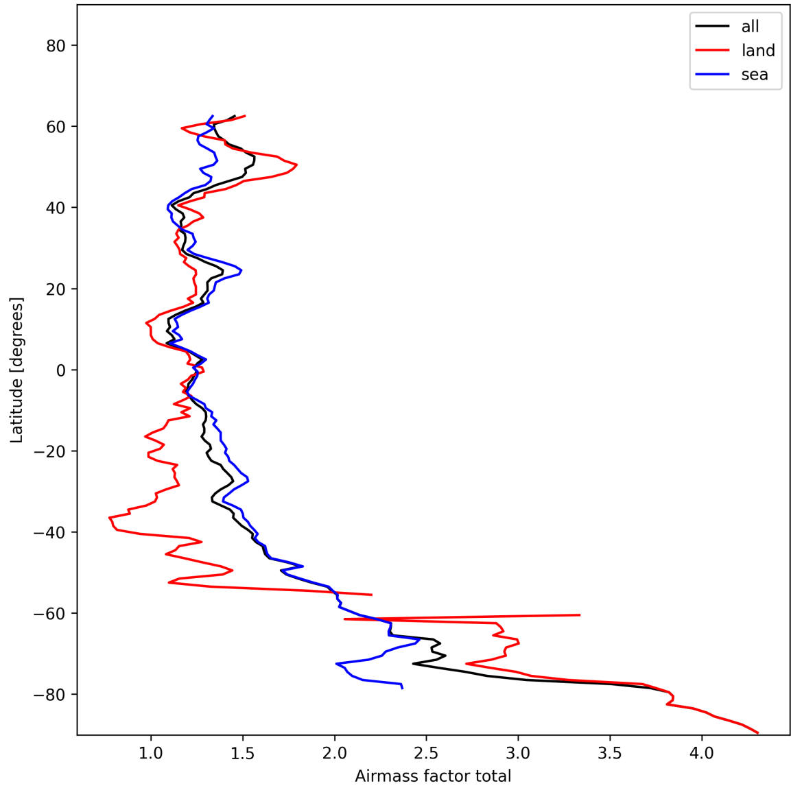
Figure 24: Zonal average of “Airmass factor total” for 2024-12-08 to 2024-12-09.
