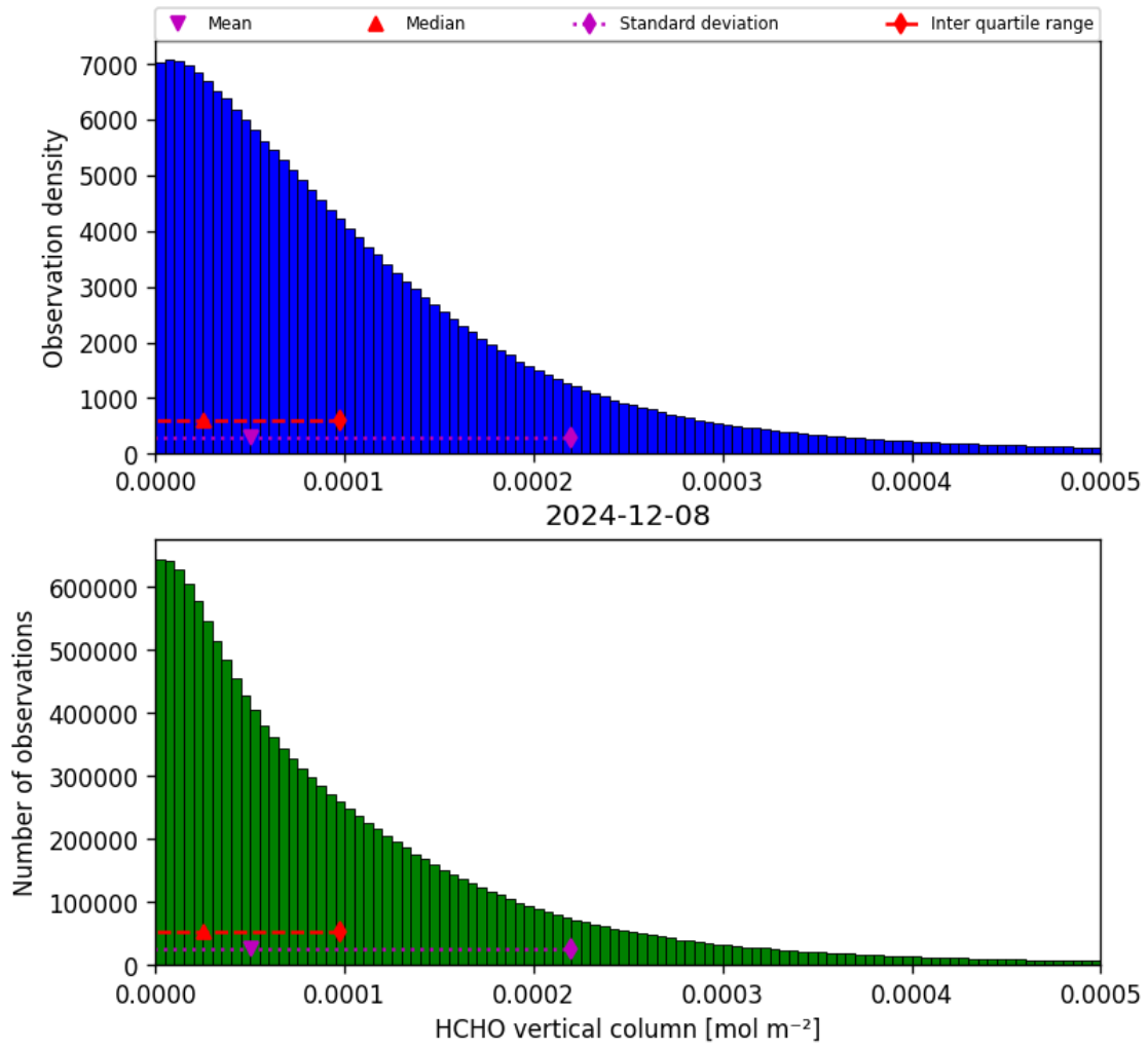
Figure 33: Histogram of “HCHO vertical column” for 2024-12-08 to 2024-12-09
