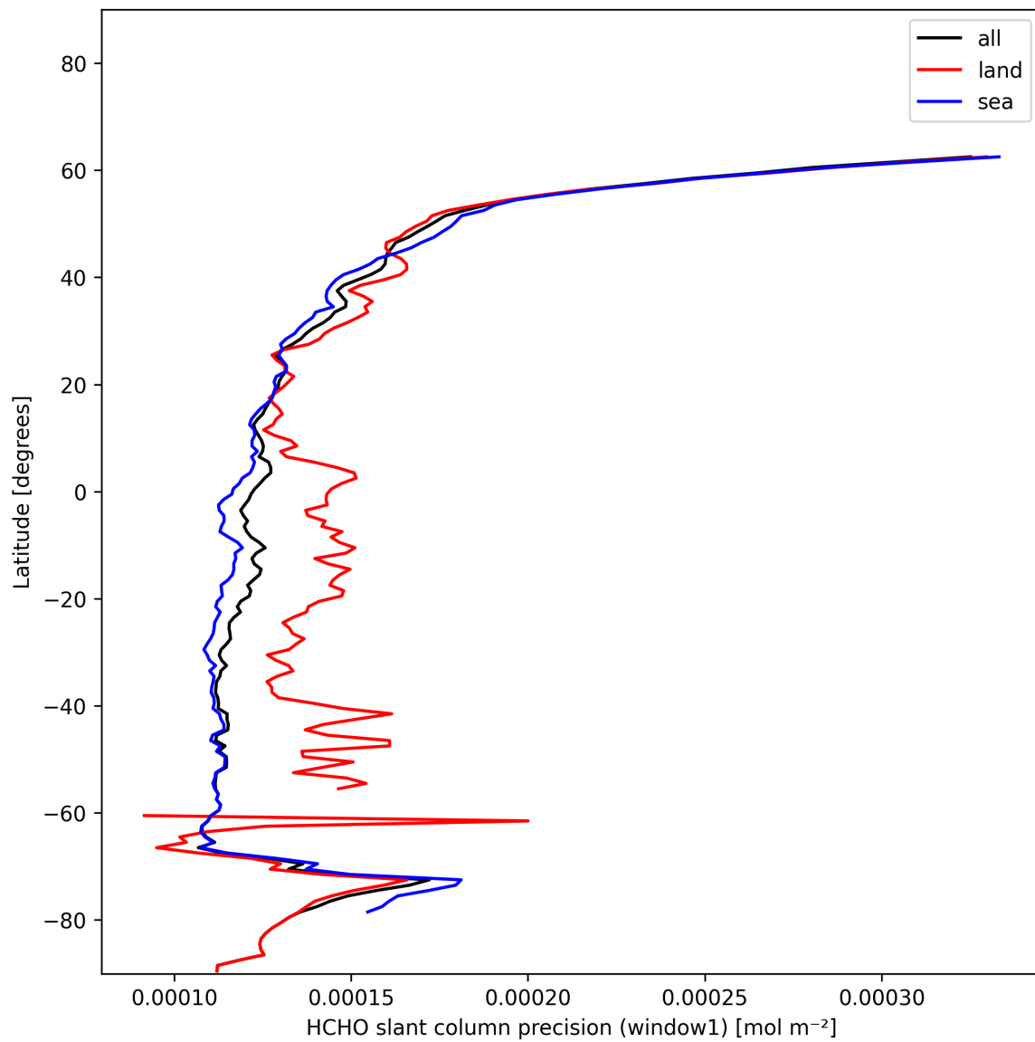
Figure 23: Zonal average of “HCHO slant column precision (window1)” for 2024-12-08 to 2024-12-09.
