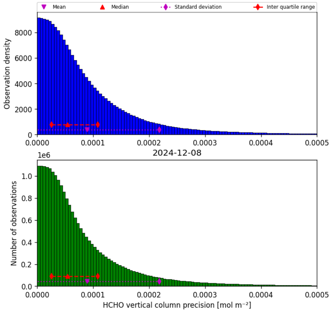
Figure 34: Histogram of “HCHO vertical column precision” for 2024-12-08 to 2024-12-09
