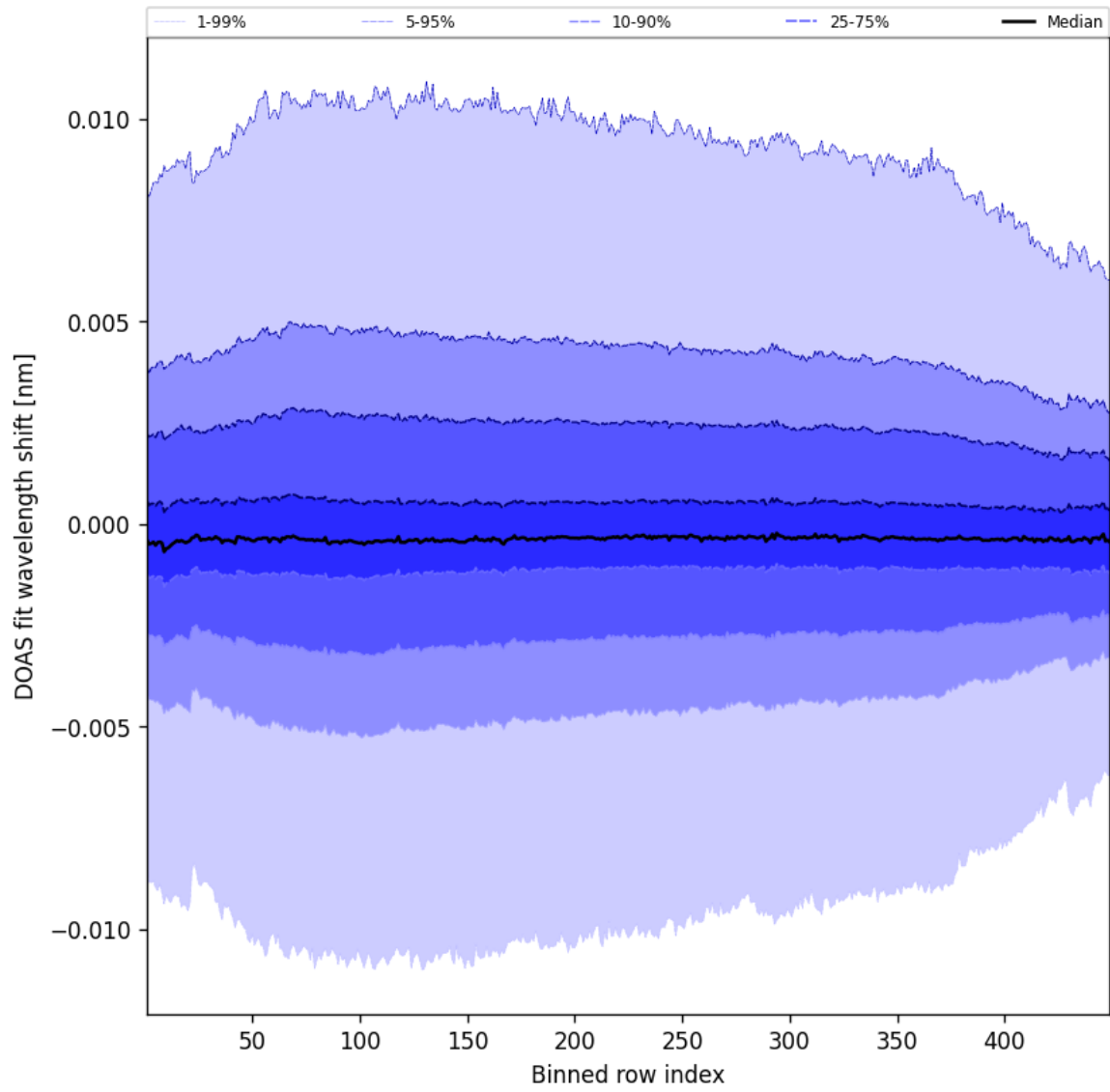
Figure 56: Along track statistics of “DOAS fit wavelength shift” for 2024-12-08 to 2024-12-09
