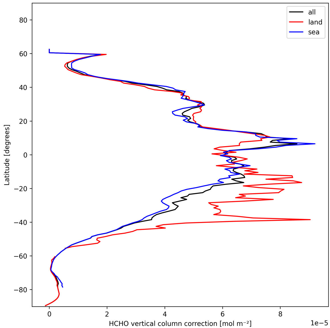
Figure 21: Zonal average of “HCHO vertical column correction” for 2024-12-08 to 2024-12-09.
