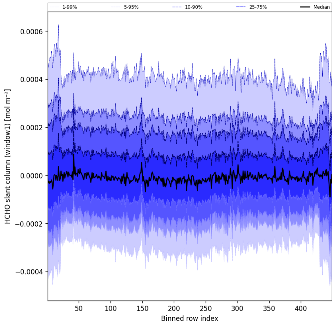
Figure 50: Along track statistics of “HCHO slant column (window1)” for 2024-12-08 to 2024-12-09
