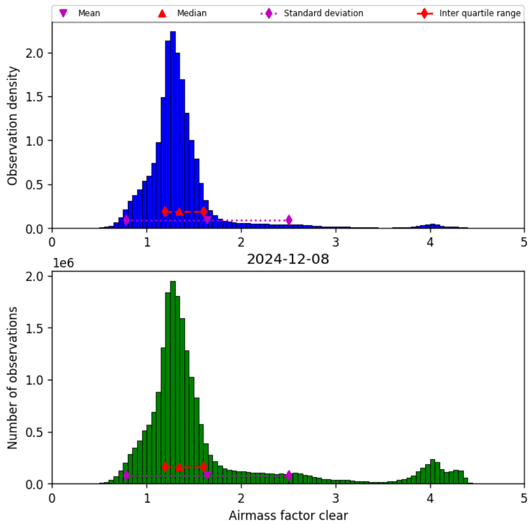
Figure 40: Histogram of “Airmass factor clear” for 2024-12-08 to 2024-12-09
