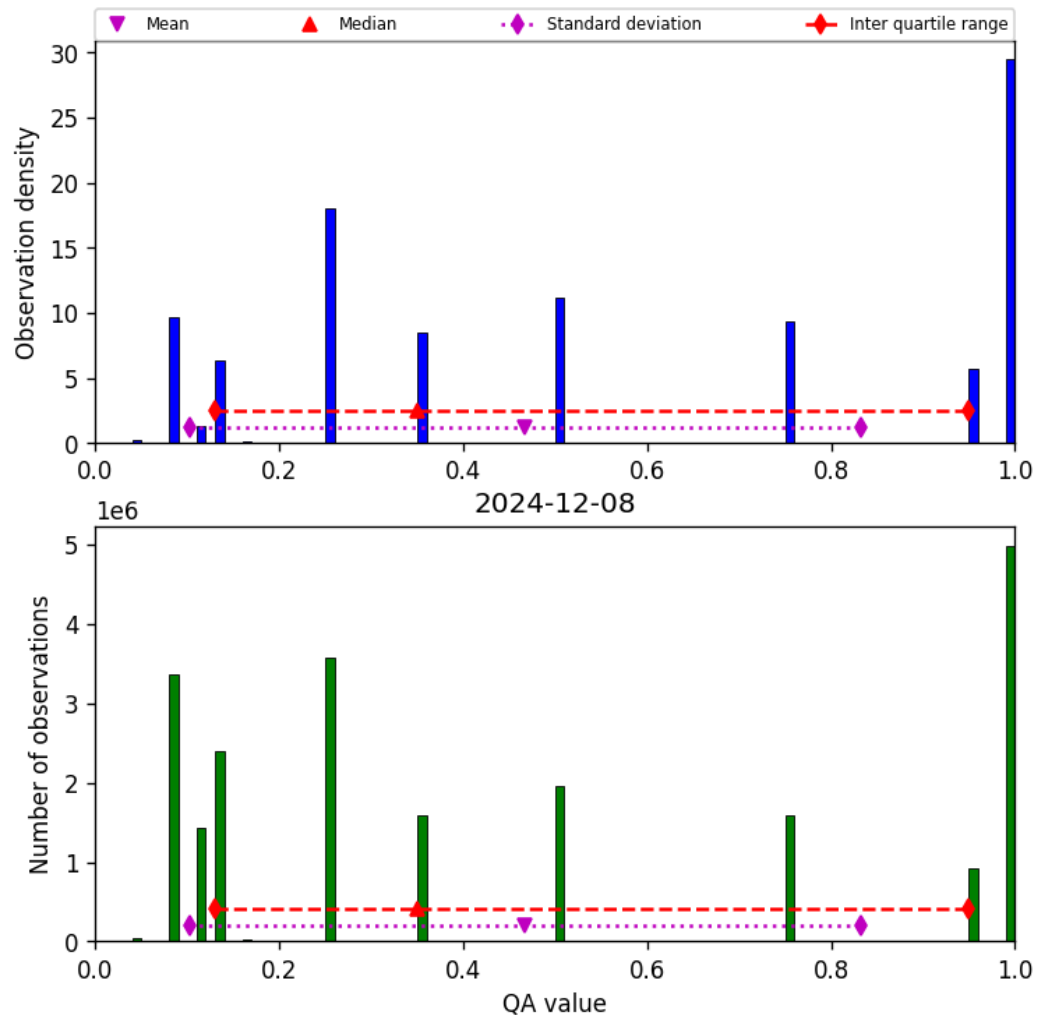
Figure 32: Histogram of “QA value” for 2024-12-08 to 2024-12-09
