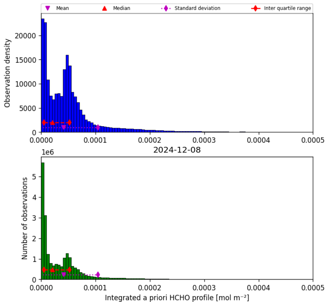
Figure 41: Histogram of “Integrated a priori HCHO profile” for 2024-12-08 to 2024-12-09
