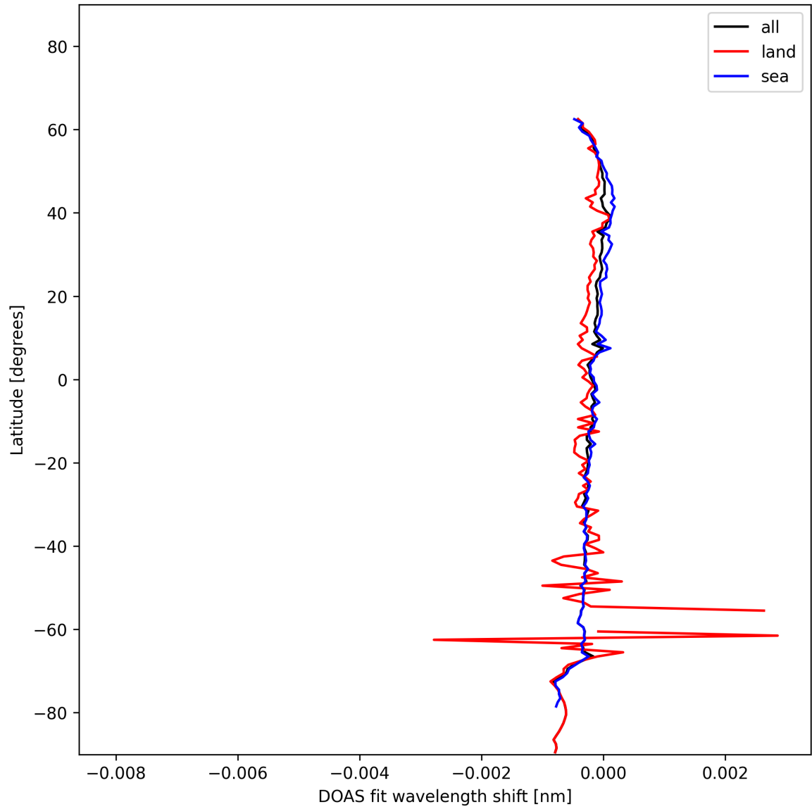
Figure 28: Zonal average of “DOAS fit wavelength shift” for 2024-12-08 to 2024-12-09.
