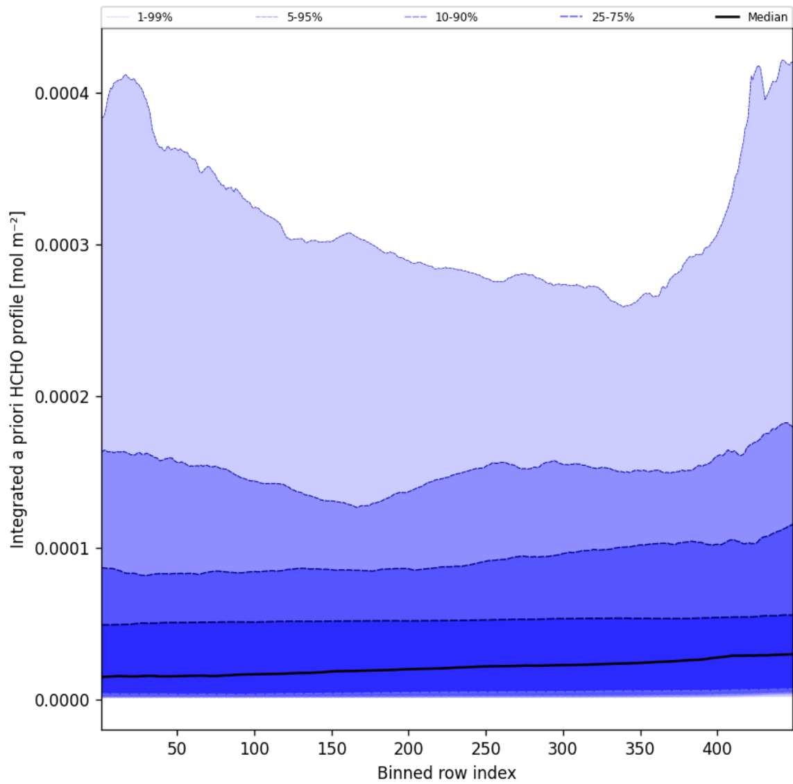
Figure 55: Along track statistics of "Integrated a priori HCHO profile" for 2024-12-08 to 2024-12-09
