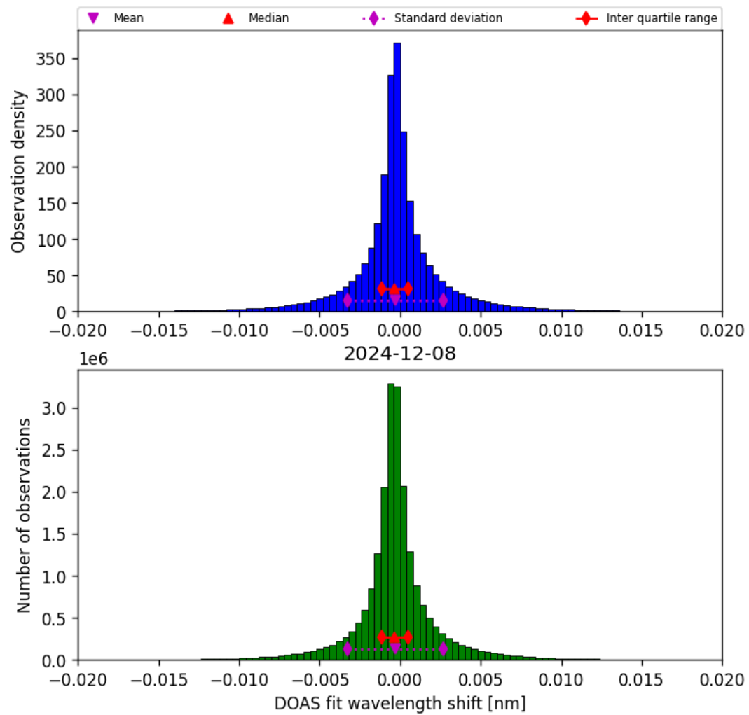
Figure 42: Histogram of “DOAS fit wavelength shift” for 2024-12-08 to 2024-12-09
