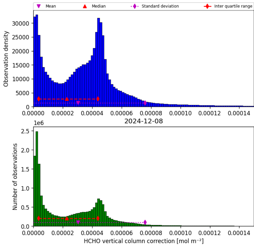
Figure 35: Histogram of “HCHO vertical column correction” for 2024-12-08 to 2024-12-09
