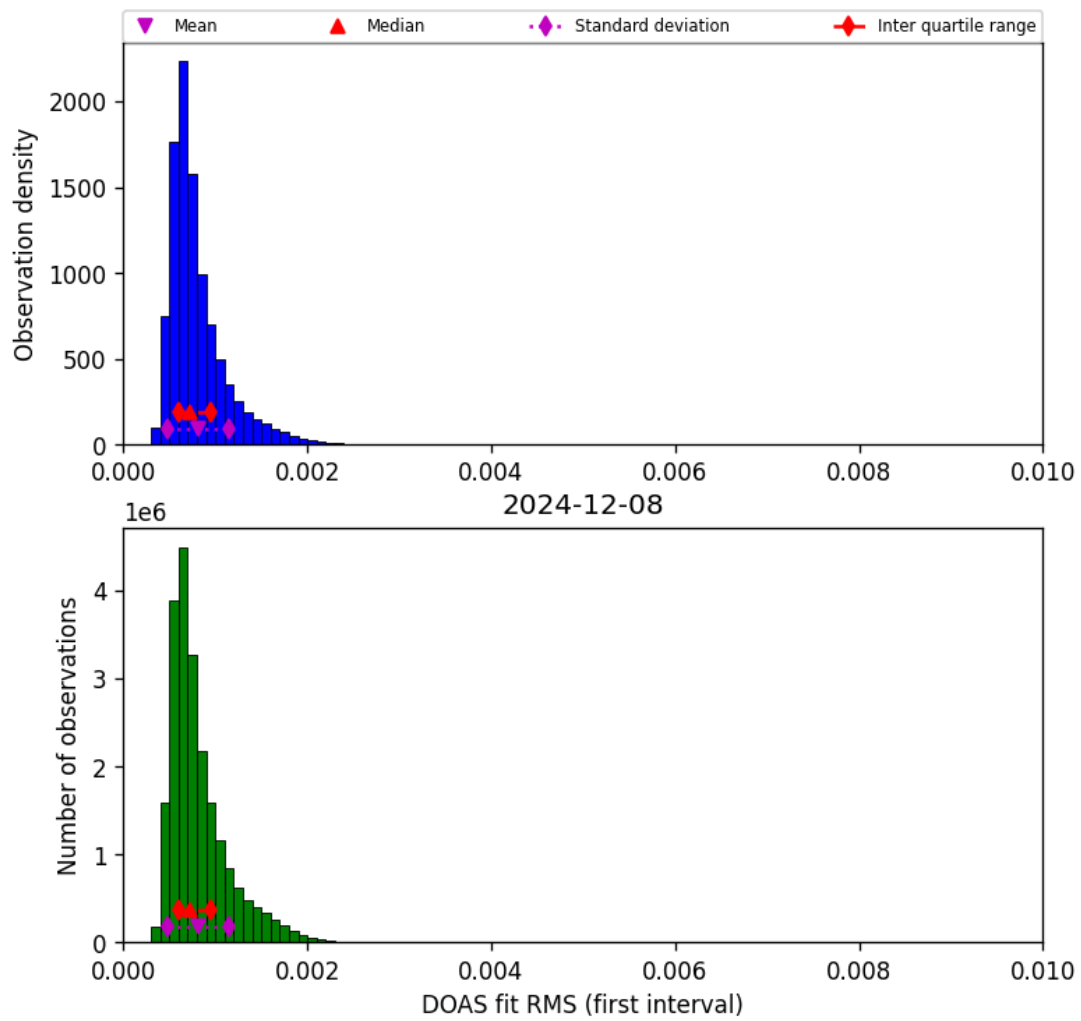
Figure 44: Histogram of “DOAS fit RMS (first interval)” for 2024-12-08 to 2024-12-09
