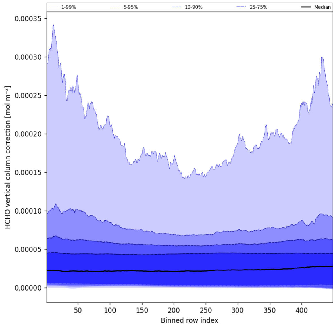
Figure 49: Along track statistics of “HCHO vertical column correction” for 2024-12-08 to 2024-12-09
