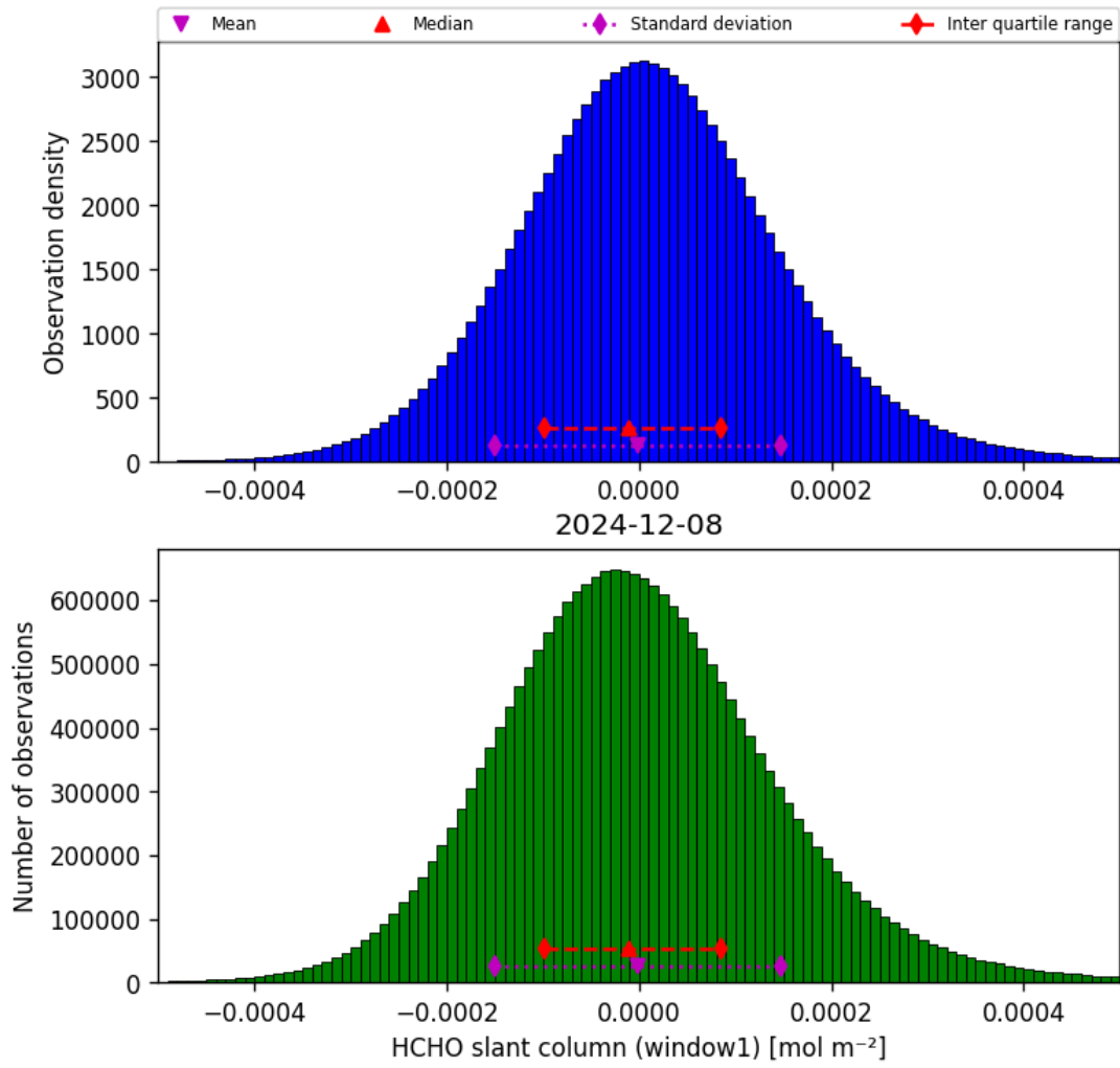
Figure 36: Histogram of “HCHO slant column (window1)” for 2024-12-08 to 2024-12-09
