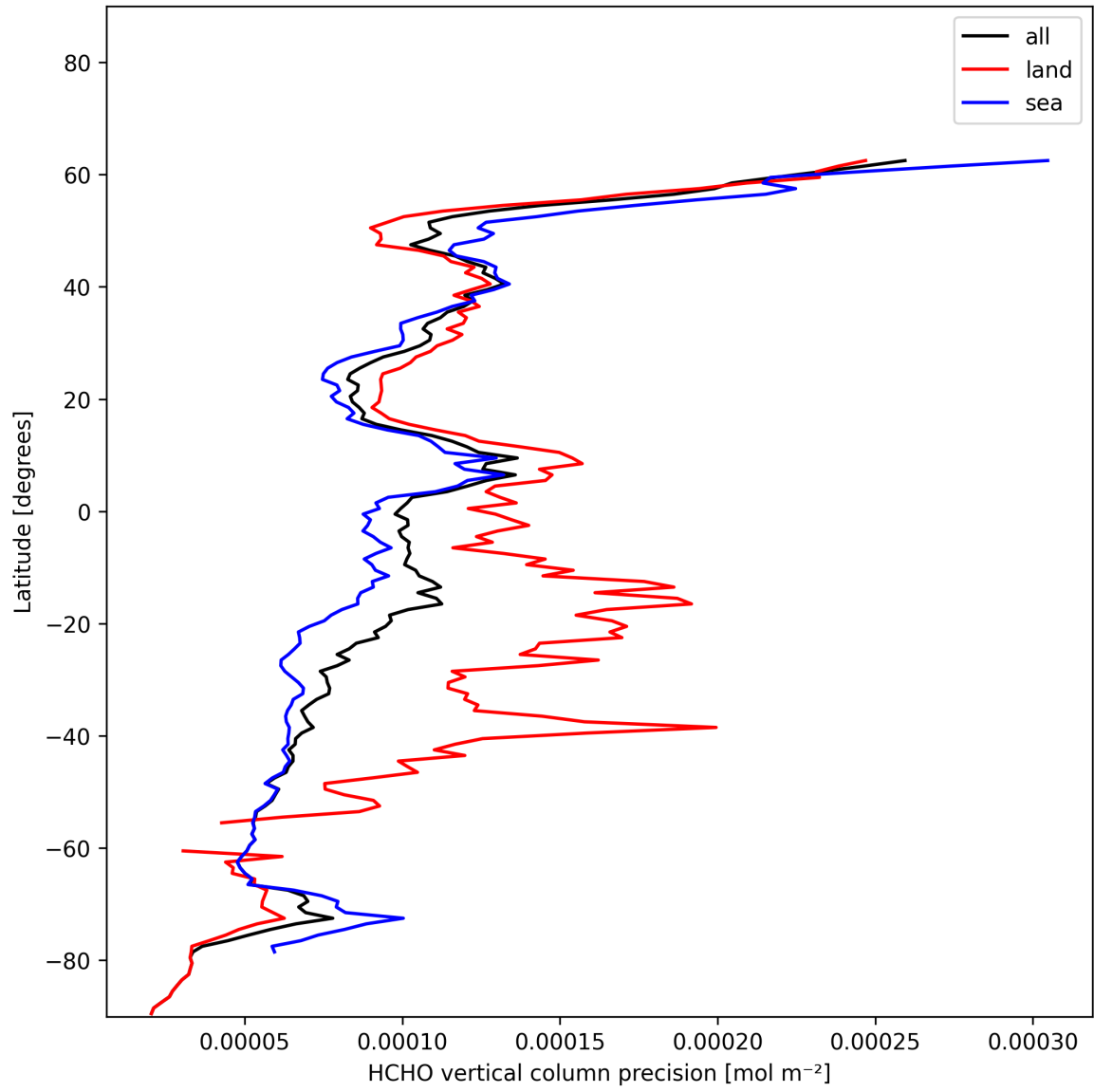
Figure 20: Zonal average of "HCHO vertical column precision" for 2024-12-08 to 2024-12-09.
