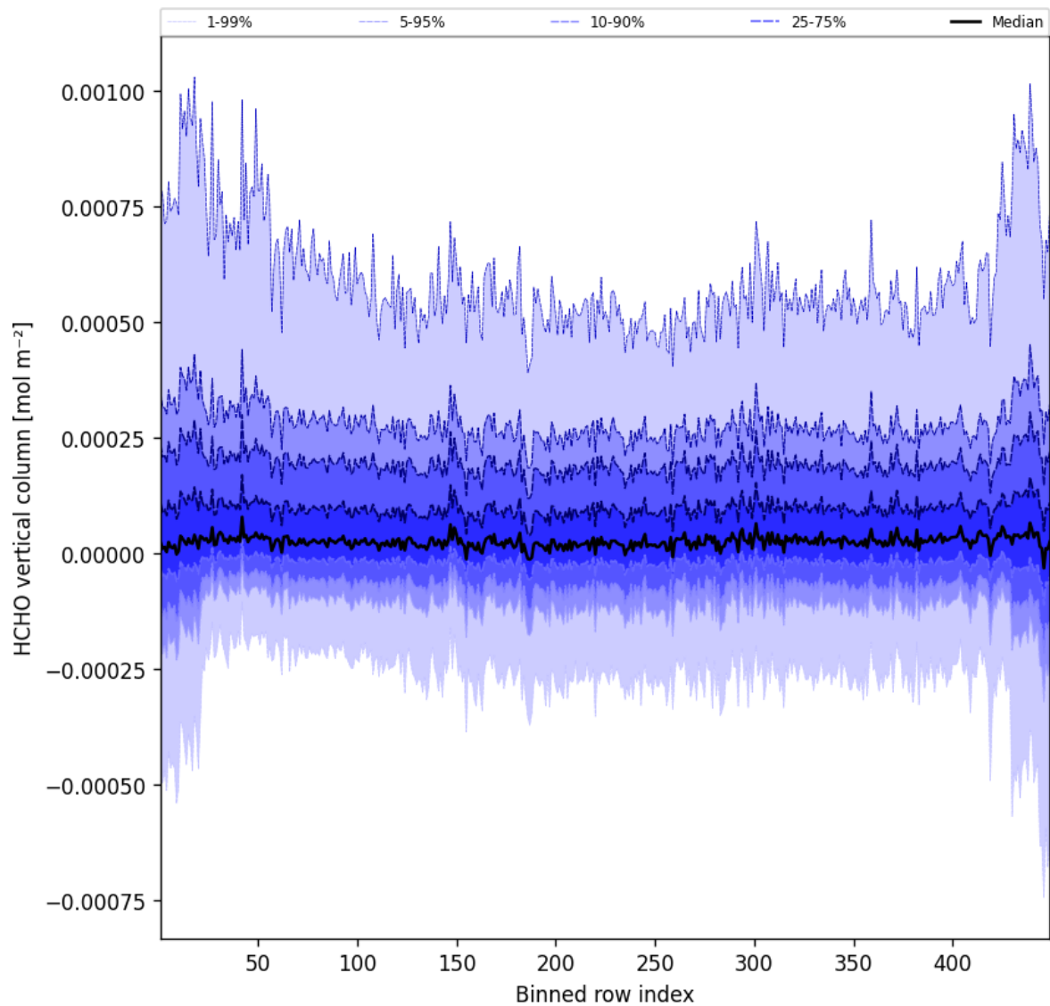
Figure 47: Along track statistics of “HCHO vertical column” for 2024-12-08 to 2024-12-09
