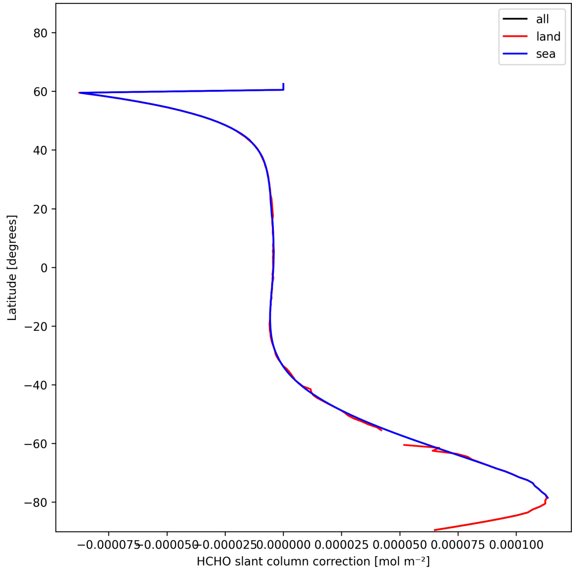
Figure 31: Zonal average of “HCHO slant column correction” for 2024-12-08 to 2024-12-09.
