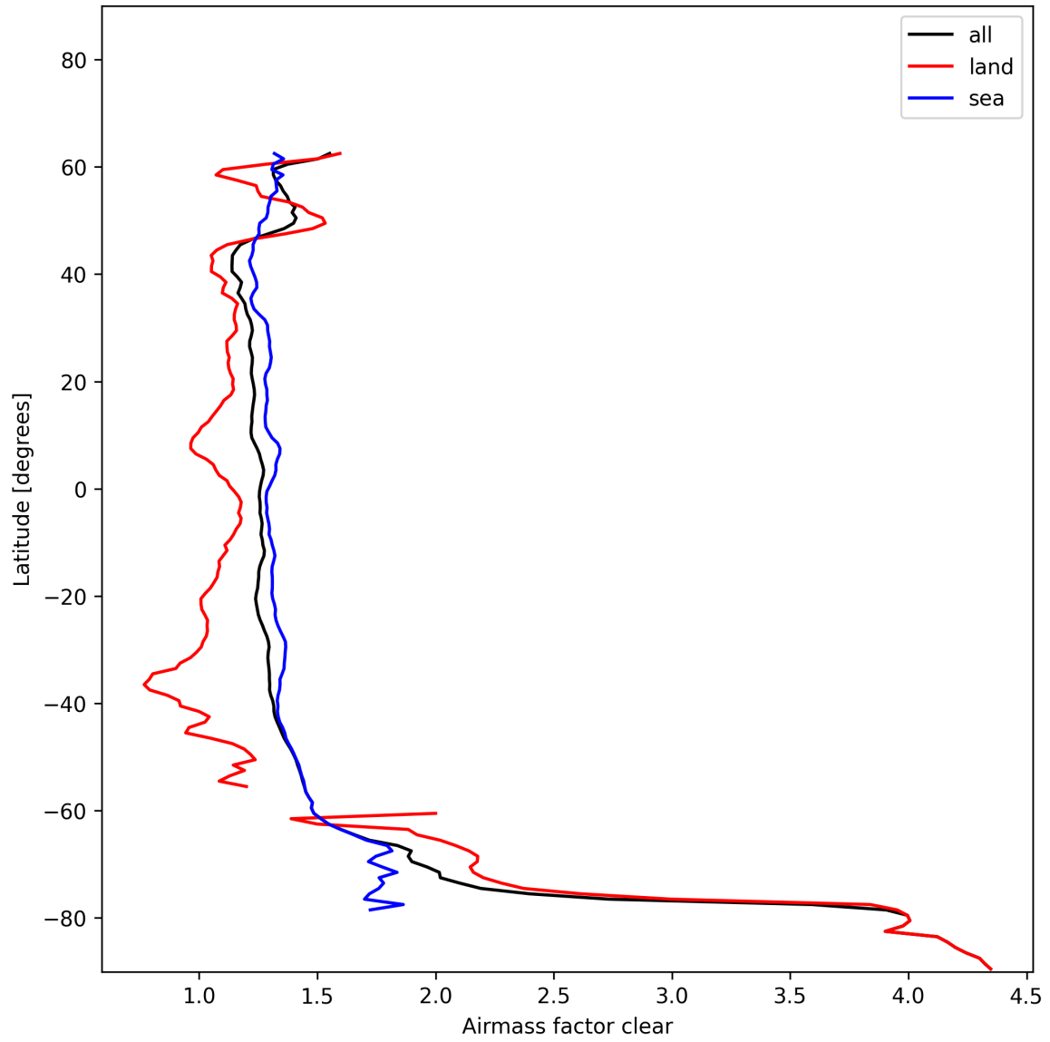
Figure 26: Zonal average of “Airmass factor clear” for 2024-12-08 to 2024-12-09.
