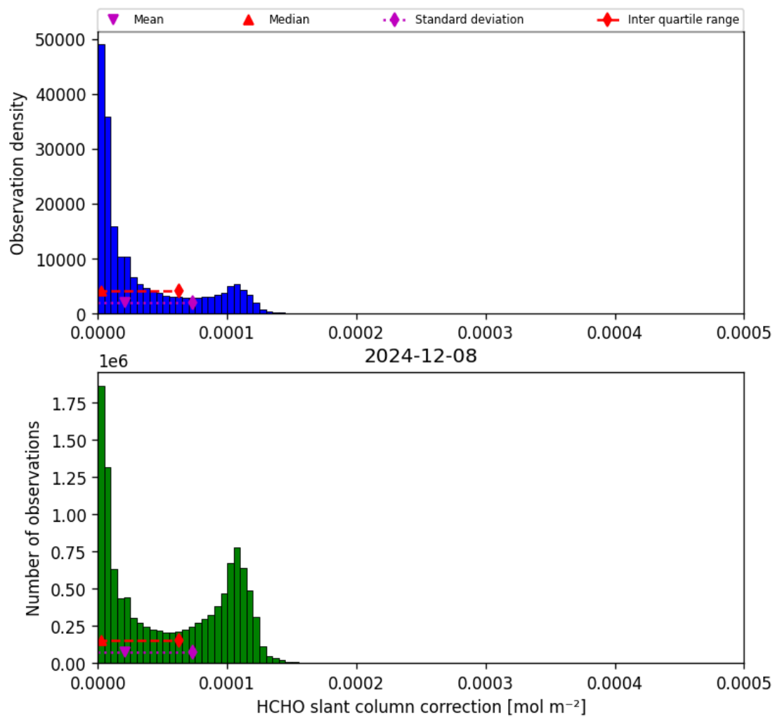
Figure 45: Histogram of "HCHO slant column correction" for 2024-12-08 to 2024-12-09
