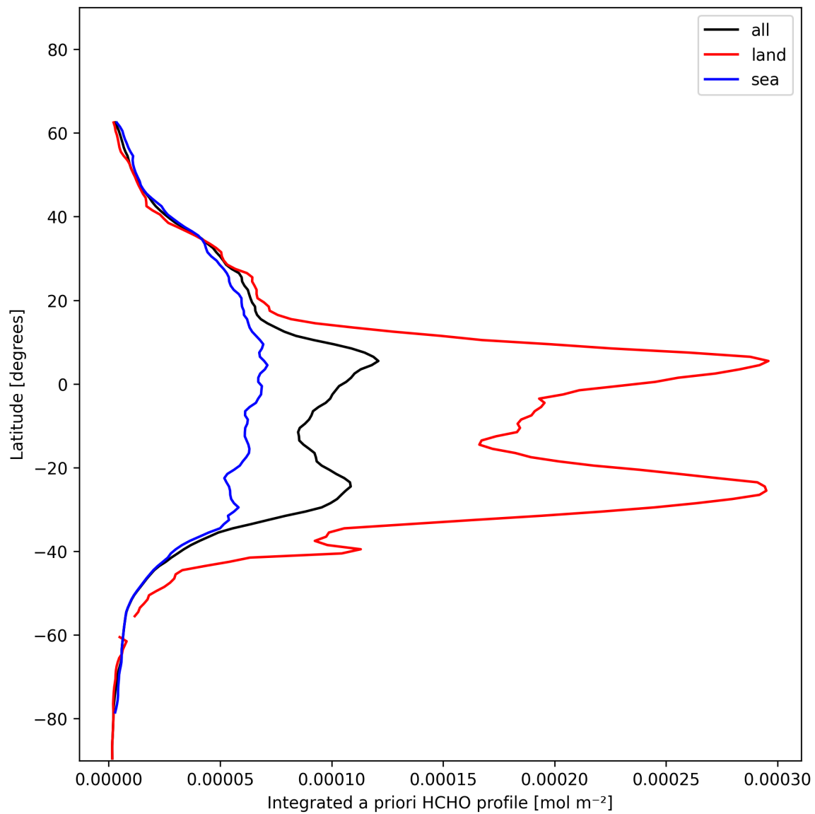
Figure 27: Zonal average of “Integrated a priori HCHO profile” for 2024-12-08 to 2024-12-09.
