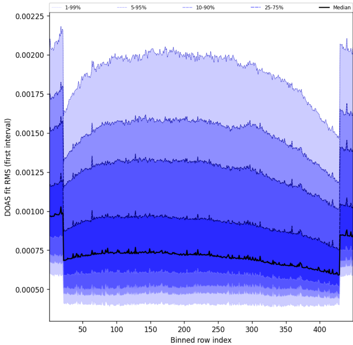
Figure 58: Along track statistics of “DOAS fit RMS (first interval)” for 2024-12-08 to 2024-12-09
