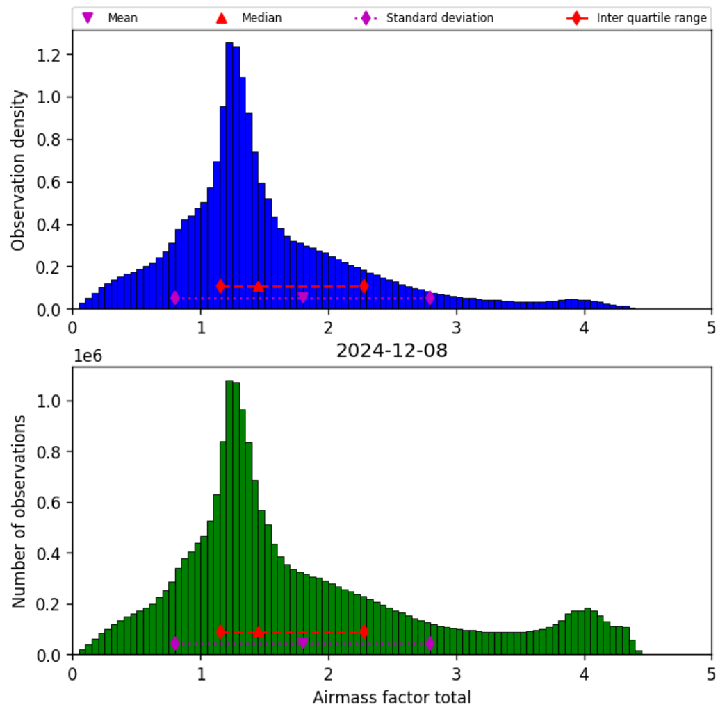
Figure 38: Histogram of “Airmass factor total” for 2024-12-08 to 2024-12-09
