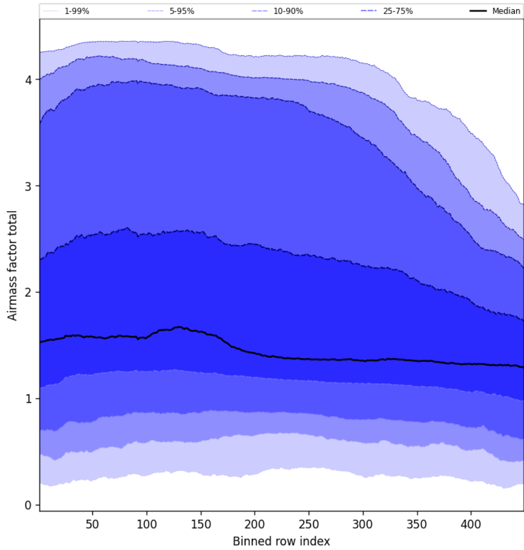
Figure 52: Along track statistics of “Airmass factor total” for 2024-12-08 to 2024-12-09
