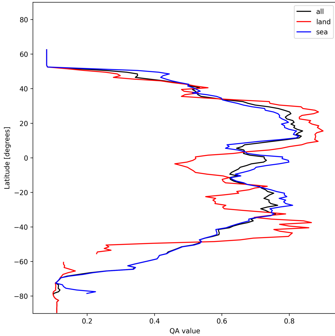
Figure 18: Zonal average of “QA value” for 2024-12-09 to 2024-12-09.
