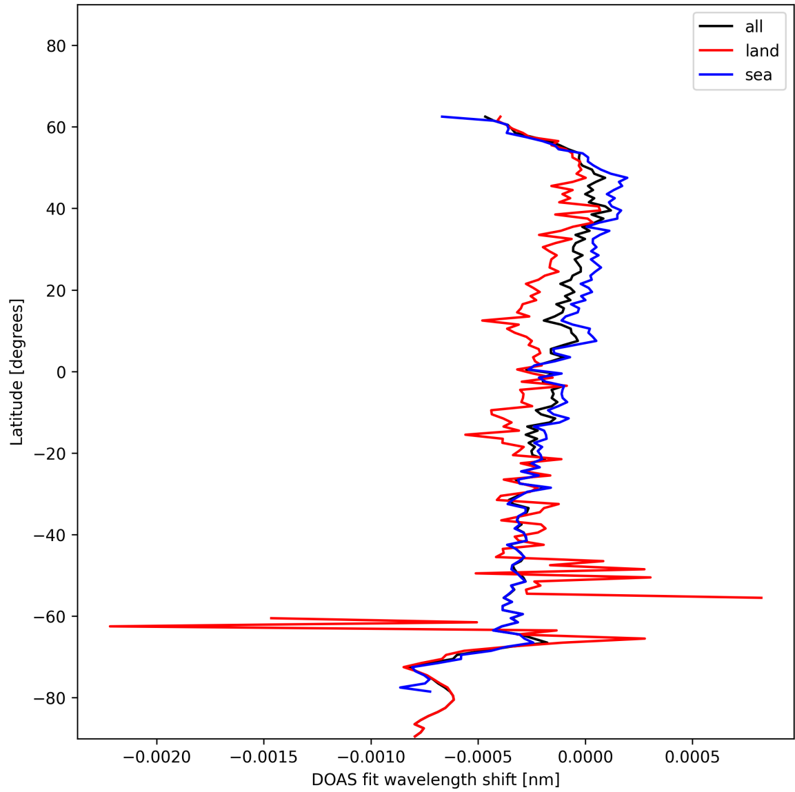
Figure 28: Zonal average of “DOAS fit wavelength shift” for 2024-12-09 to 2024-12-09.
