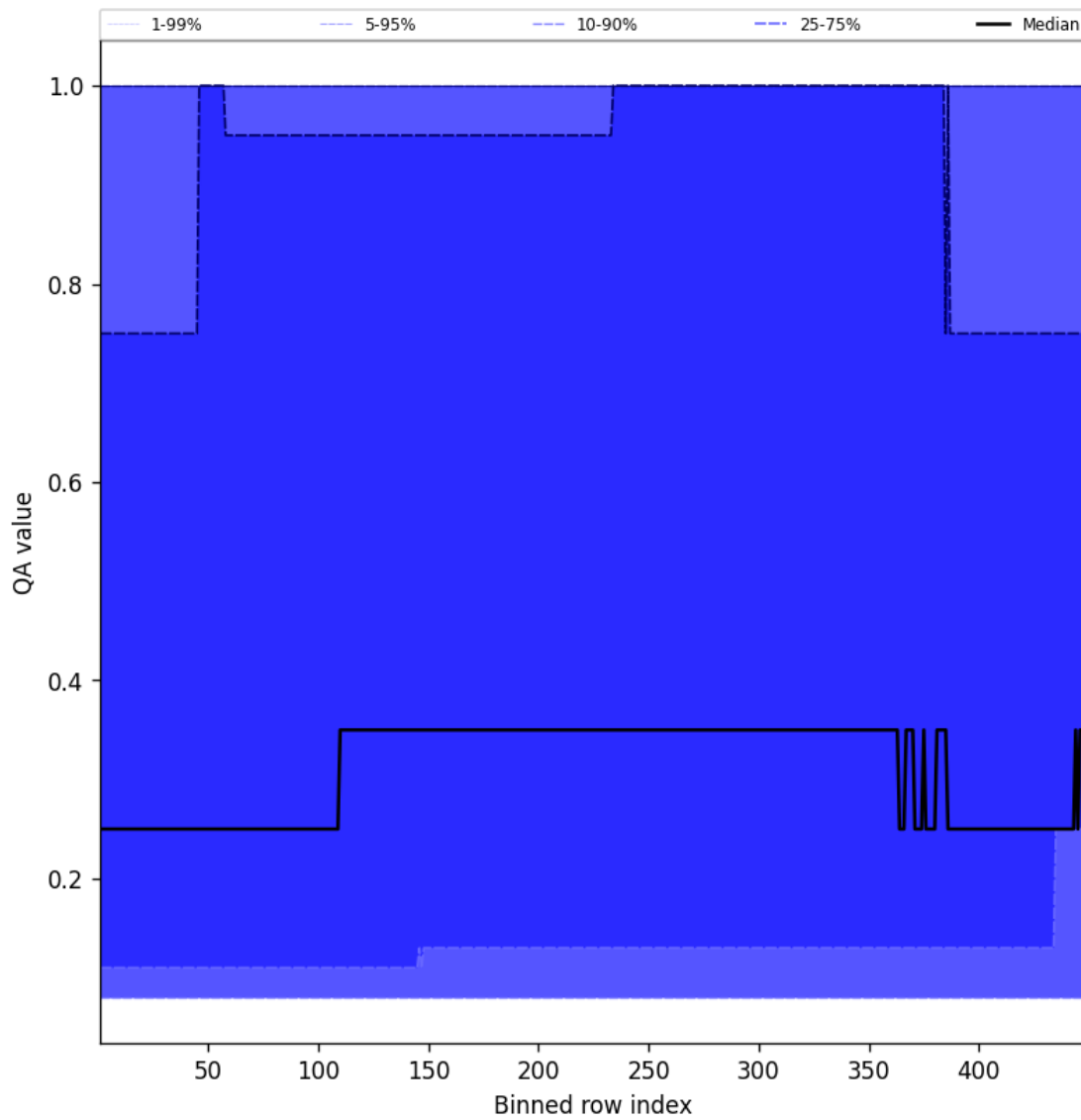
Figure 46: Along track statistics of “QA value” for 2024-12-09 to 2024-12-09
