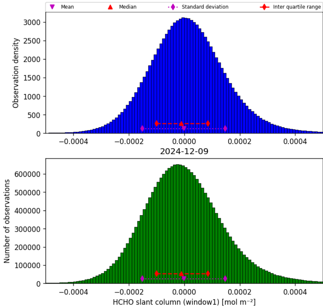
Figure 36: Histogram of “HCHO slant column (window1)” for 2024-12-09 to 2024-12-09
