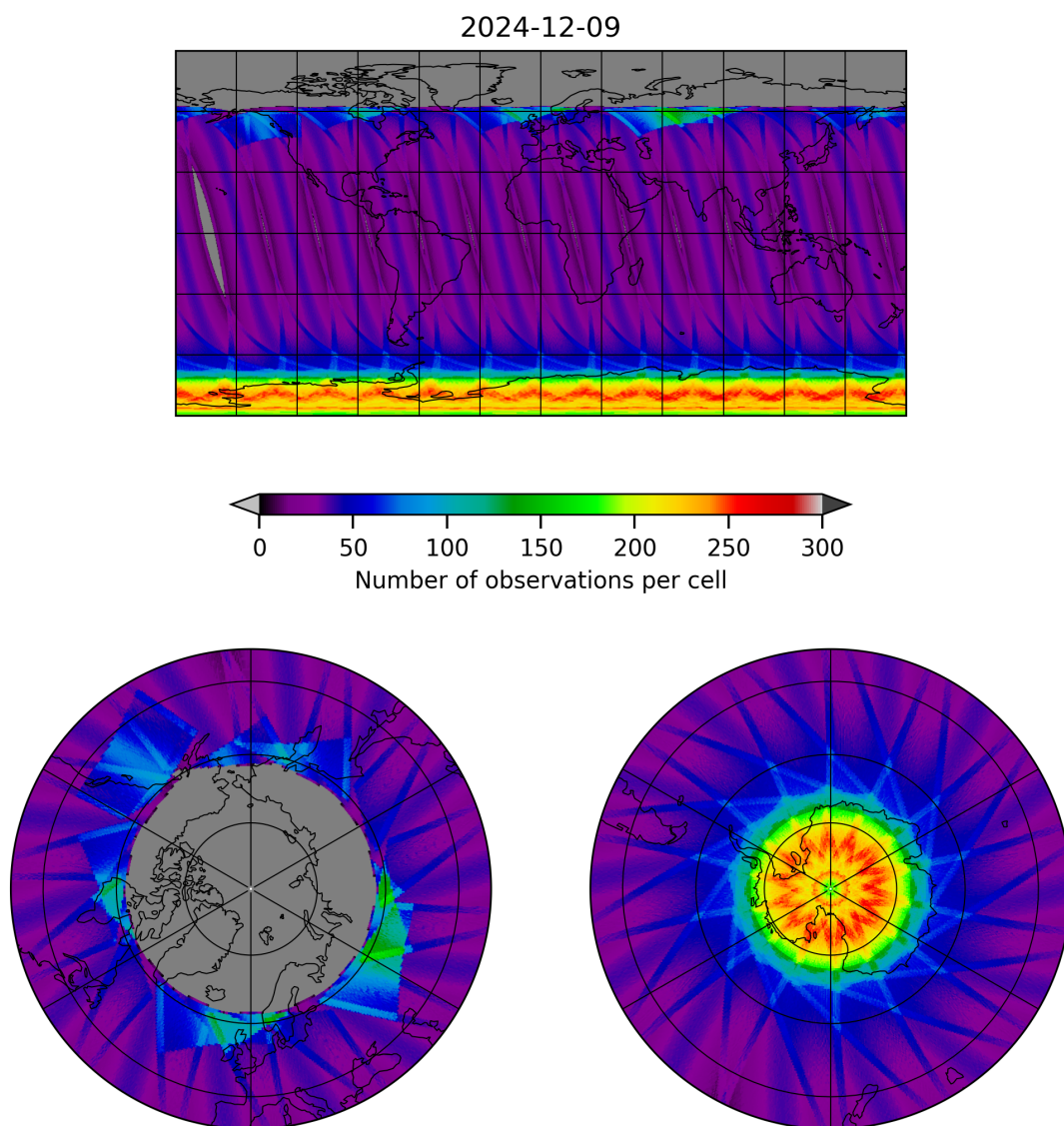
Figure 17: Map of the number of observations for 2024-12-09 to 2024-12-09
