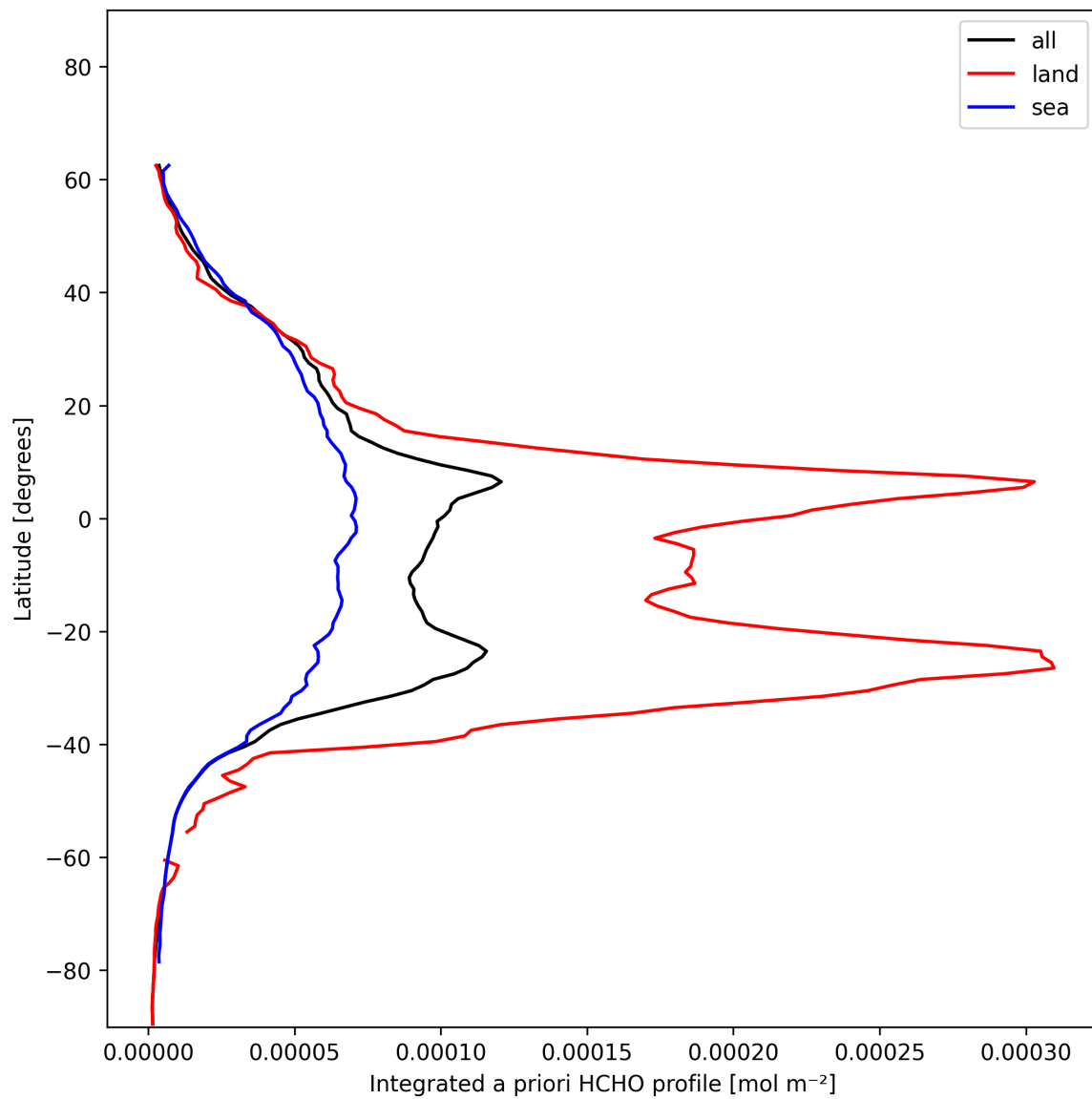
Figure 27: Zonal average of “Integrated a priori HCHO profile” for 2024-12-09 to 2024-12-09.
