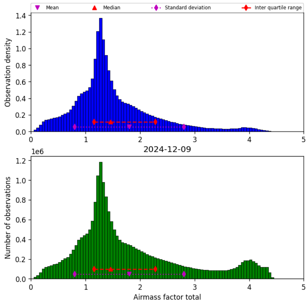
Figure 38: Histogram of “Airmass factor total” for 2024-12-09 to 2024-12-09
