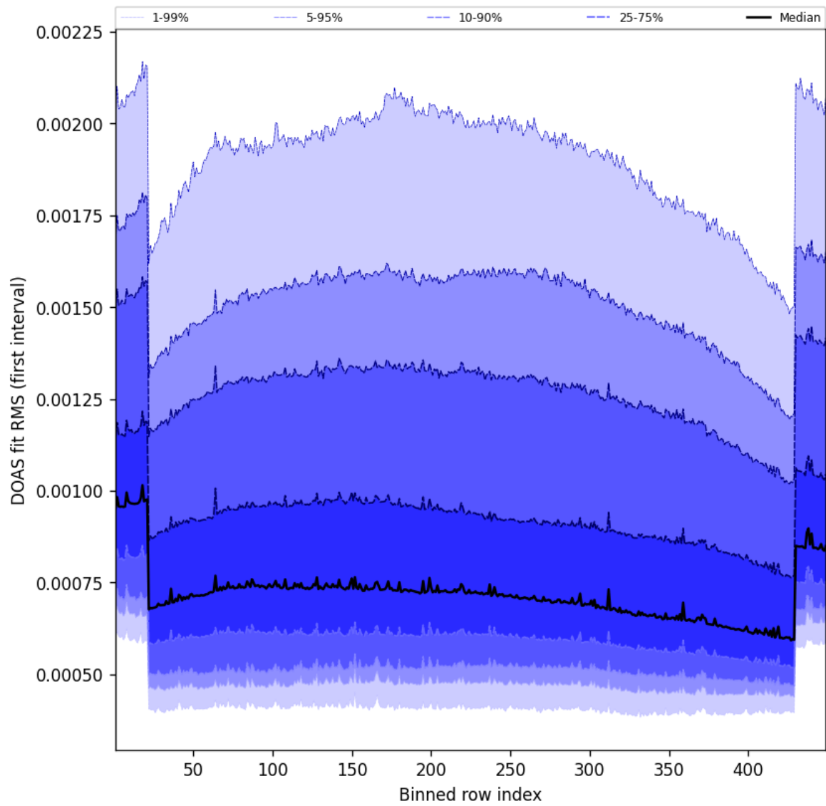
Figure 58: Along track statistics of “DOAS fit RMS (first interval)” for 2024-12-09 to 2024-12-09
