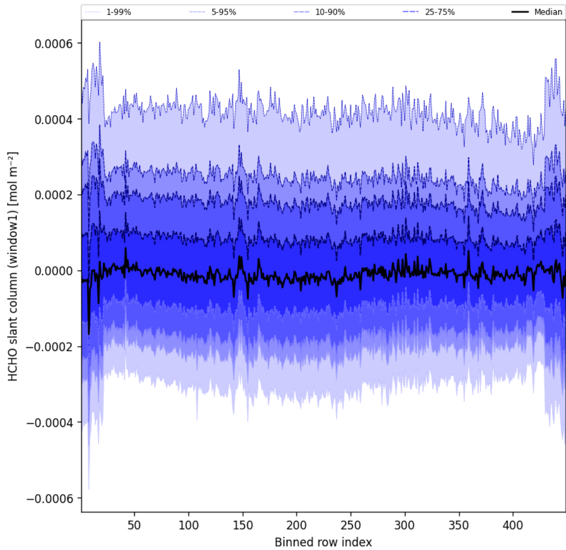
Figure 50: Along track statistics of “HCHO slant column (window1)” for 2024-12-09 to 2024-12-09
