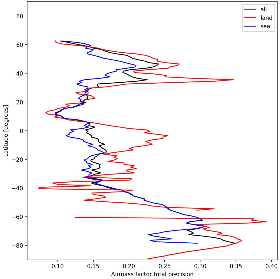
Figure 25: Zonal average of “Airmass factor total precision” for 2024-12-09 to 2024-12-09.
