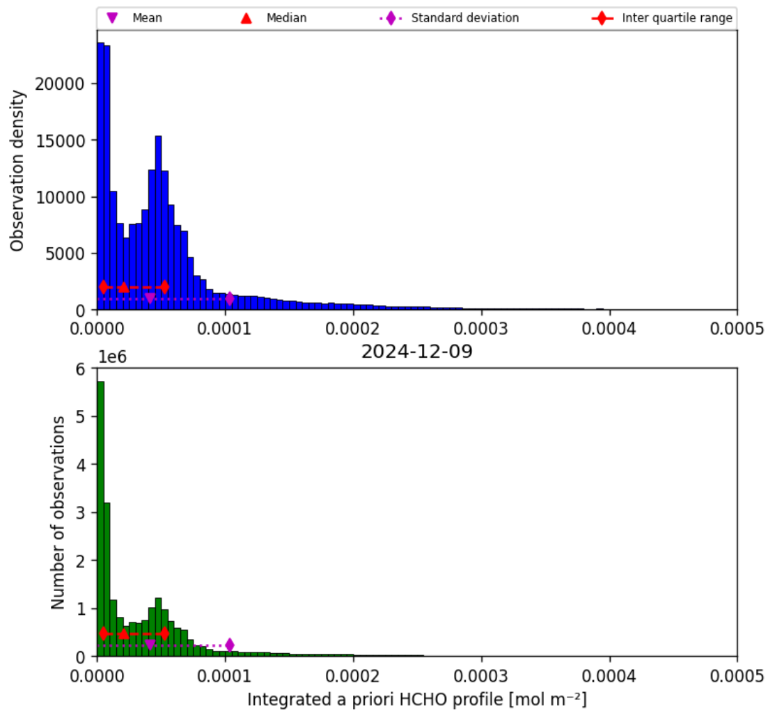
Figure 41: Histogram of “Integrated a priori HCHO profile” for 2024-12-09 to 2024-12-09
