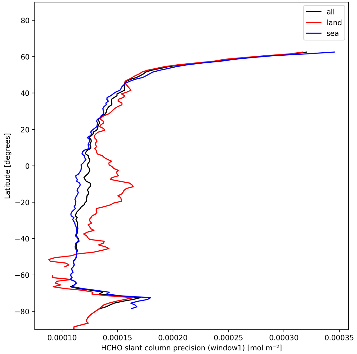
Figure 23: Zonal average of “HCHO slant column precision (window1)” for 2024-12-09 to 2024-12-09.
