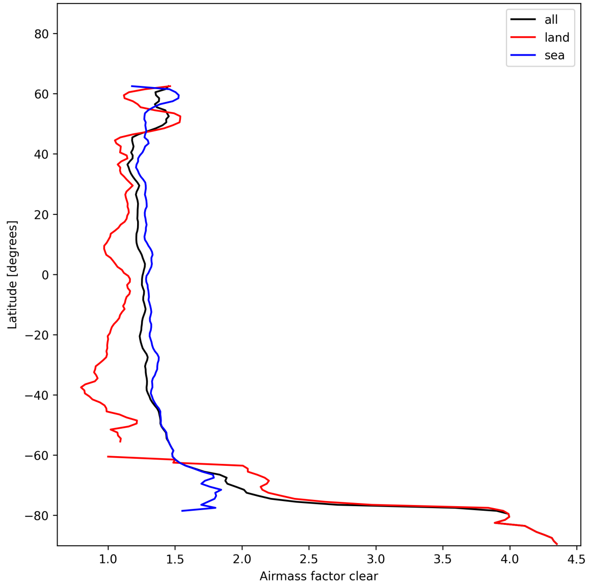
Figure 26: Zonal average of “Airmass factor clear” for 2024-12-09 to 2024-12-09.
