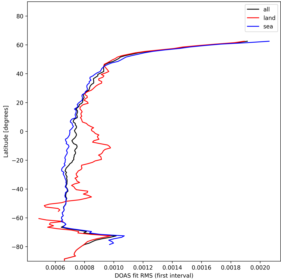
Figure 30: Zonal average of “DOAS fit RMS (first interval)” for 2024-12-09 to 2024-12-09.
