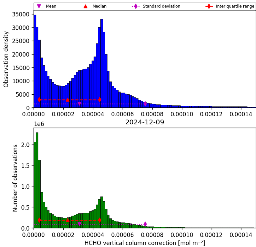
Figure 35: Histogram of “HCHO vertical column correction” for 2024-12-09 to 2024-12-09
