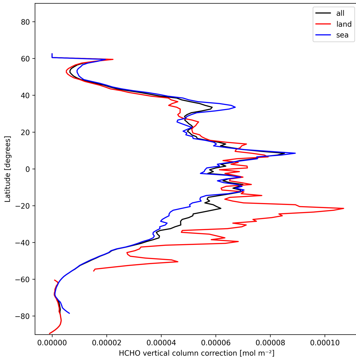
Figure 21: Zonal average of “HCHO vertical column correction” for 2024-12-09 to 2024-12-09.
