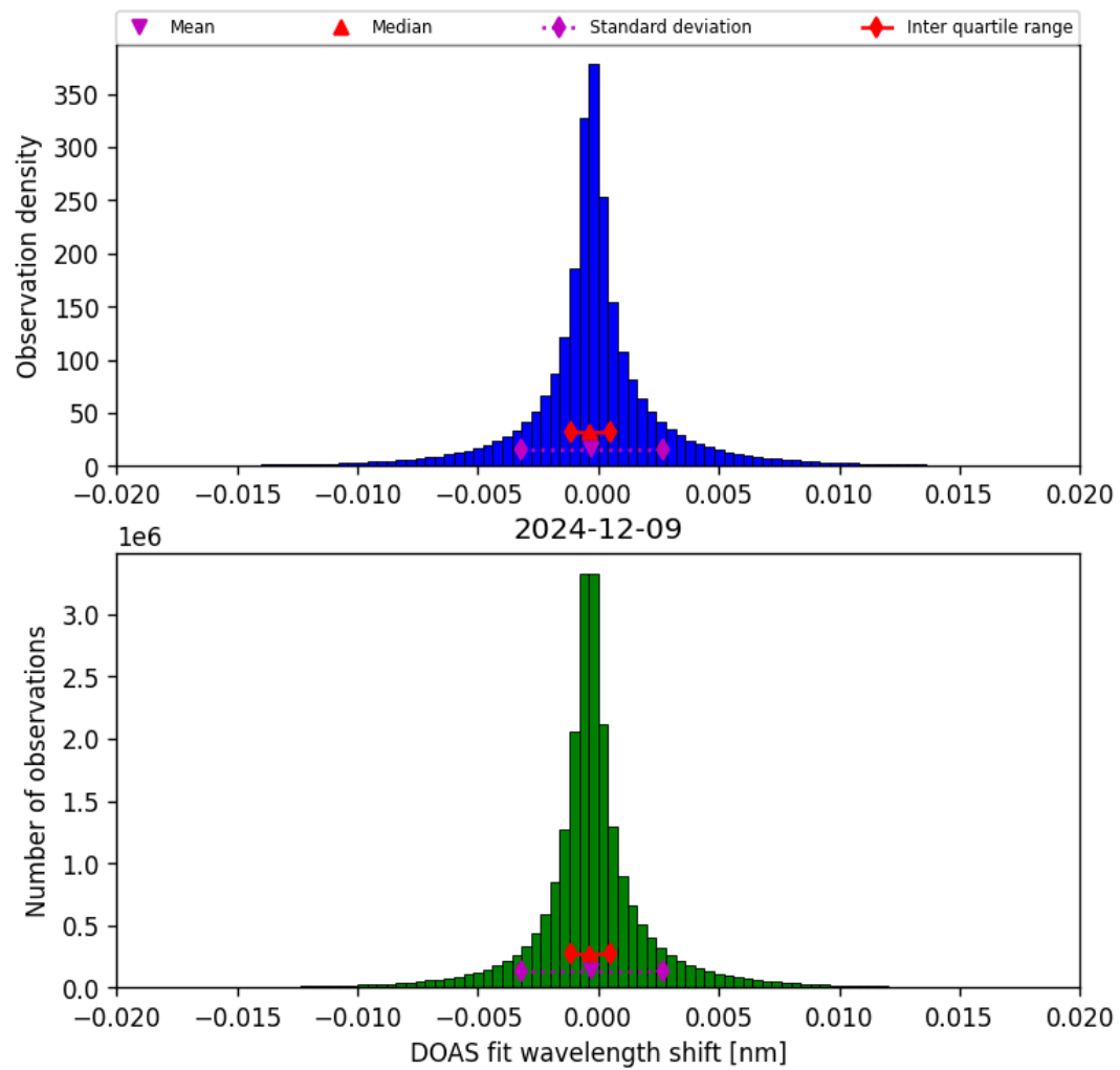
Figure 42: Histogram of “DOAS fit wavelength shift” for 2024-12-09 to 2024-12-09
