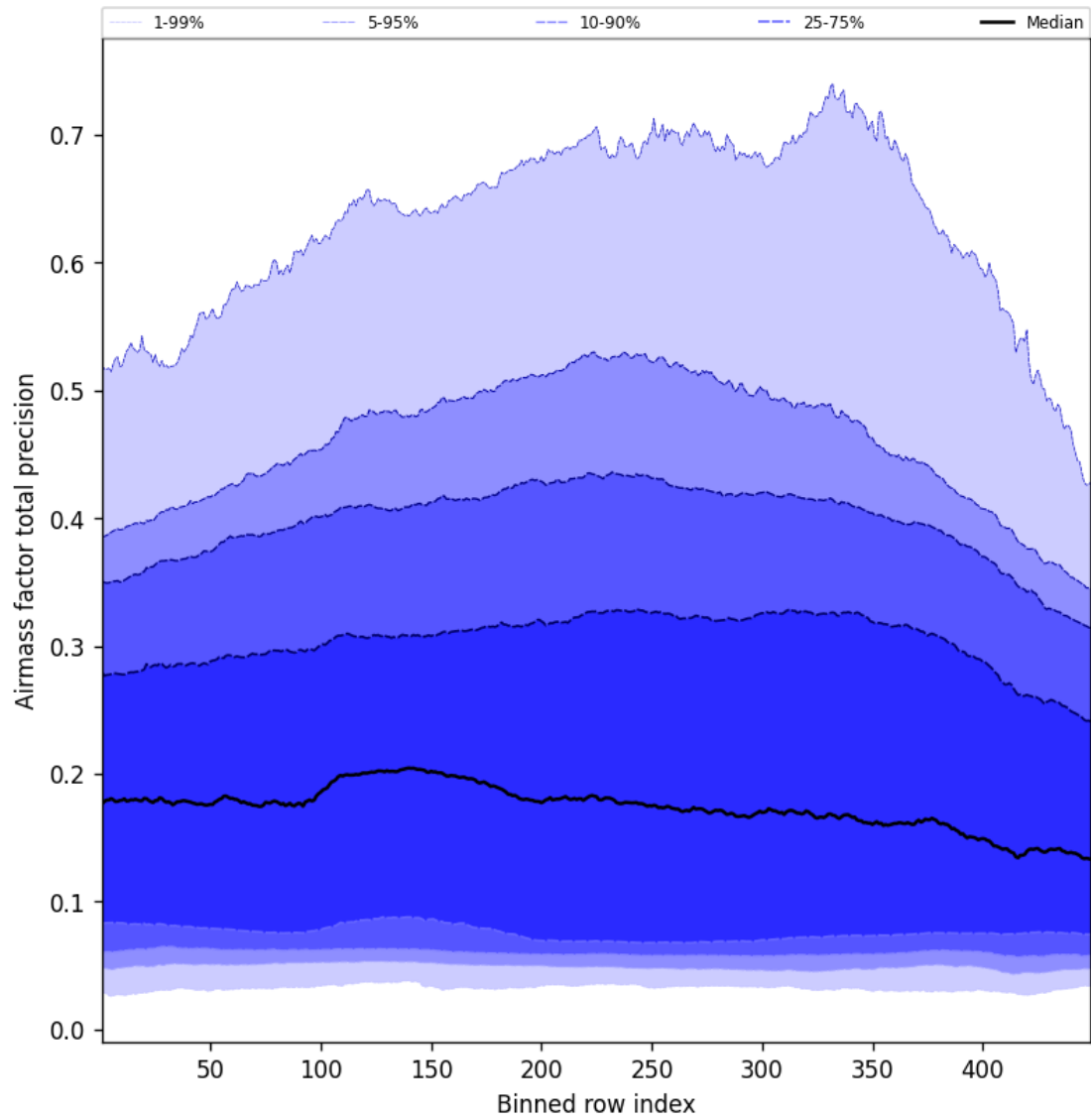
Figure 53: Along track statistics of “Airmass factor total precision” for 2024-12-09 to 2024-12-09
