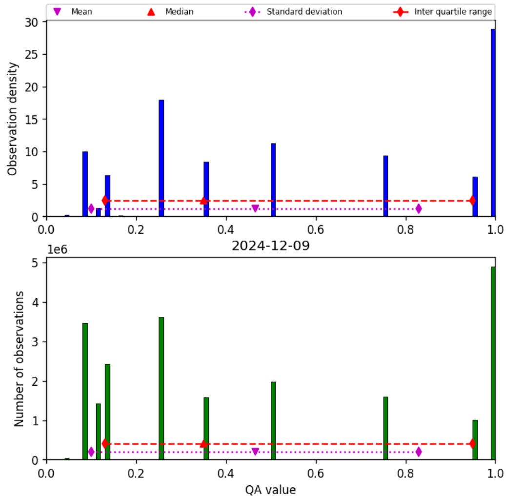
Figure 32: Histogram of “QA value” for 2024-12-09 to 2024-12-09
