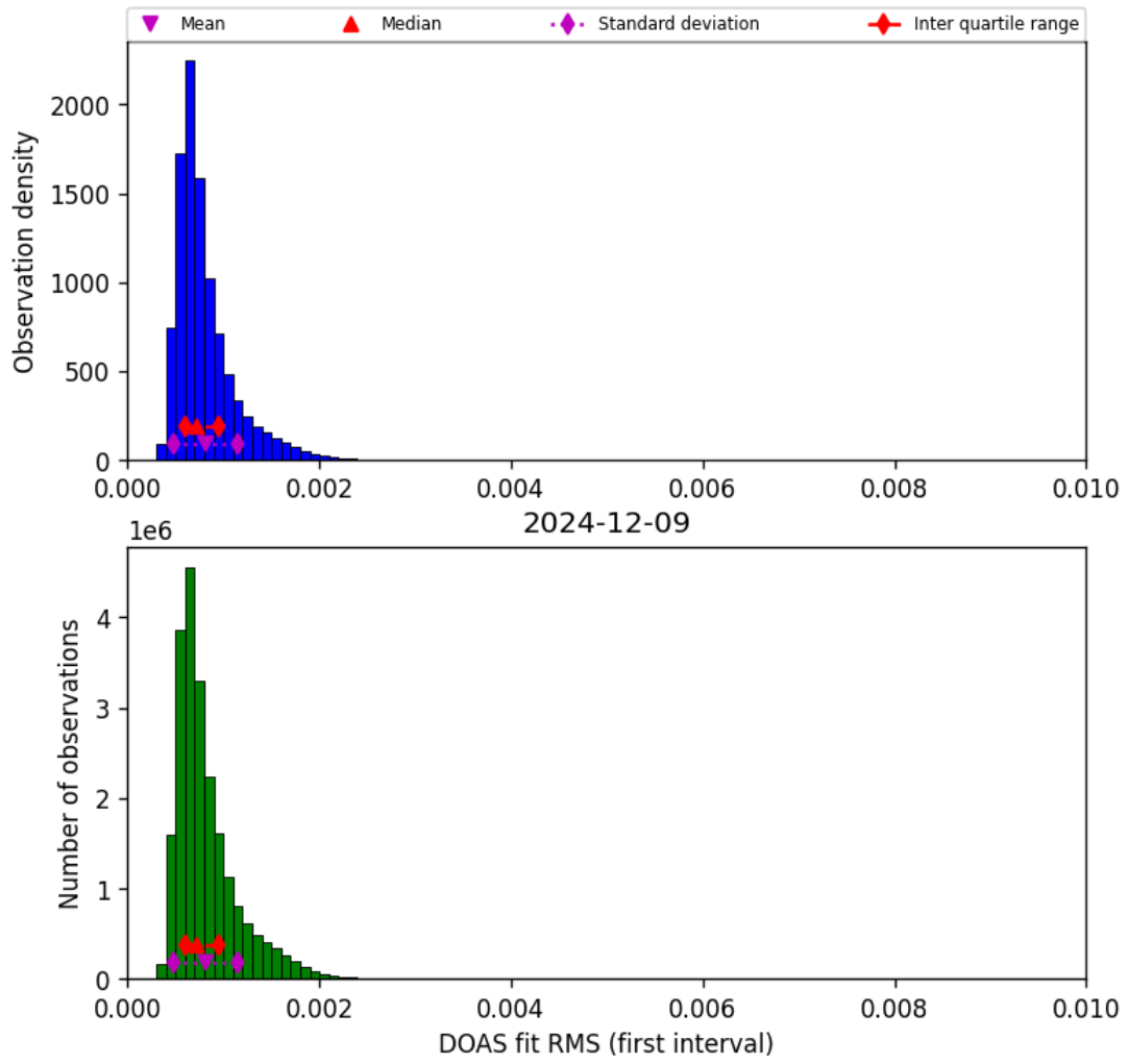
Figure 44: Histogram of “DOAS fit RMS (first interval)” for 2024-12-09 to 2024-12-09
