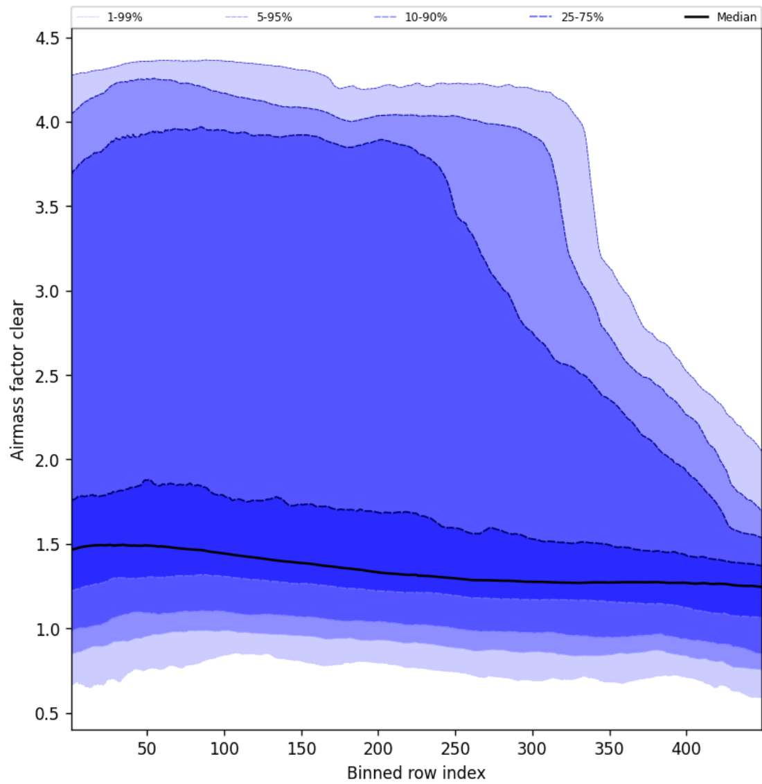
Figure 54: Along track statistics of “Airmass factor clear” for 2024-12-09 to 2024-12-09
