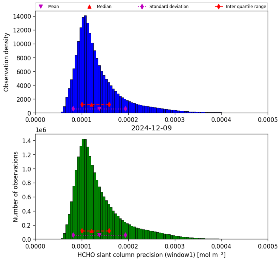
Figure 37: Histogram of “HCHO slant column precision (window1)” for 2024-12-09 to 2024-12-09
