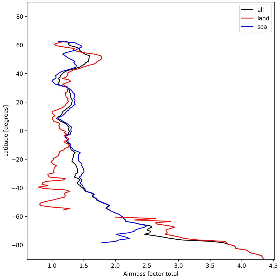
Figure 24: Zonal average of “Airmass factor total” for 2024-12-09 to 2024-12-09.
