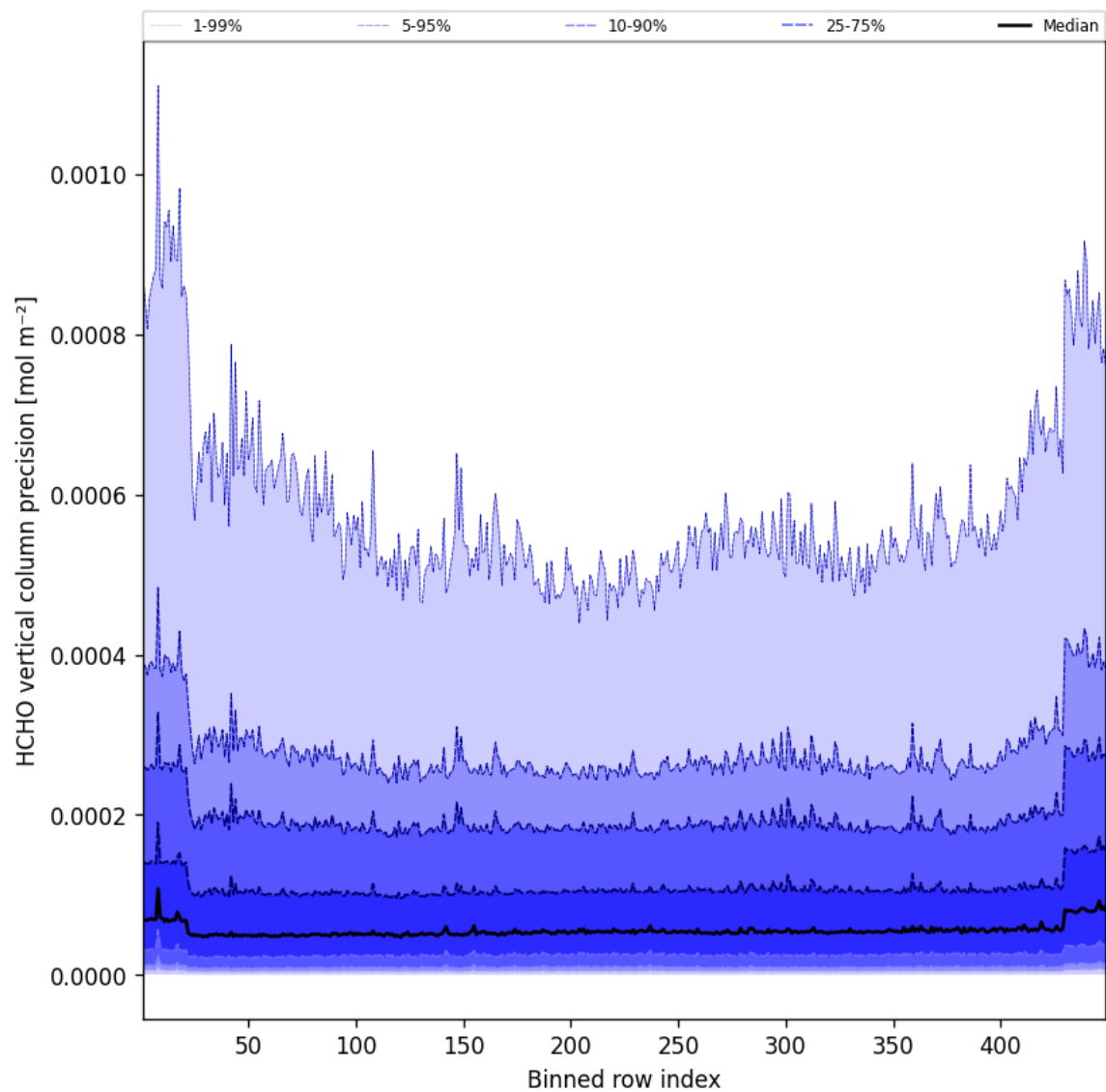
Figure 48: Along track statistics of “HCHO vertical column precision” for 2024-12-09 to 2024-12-09
