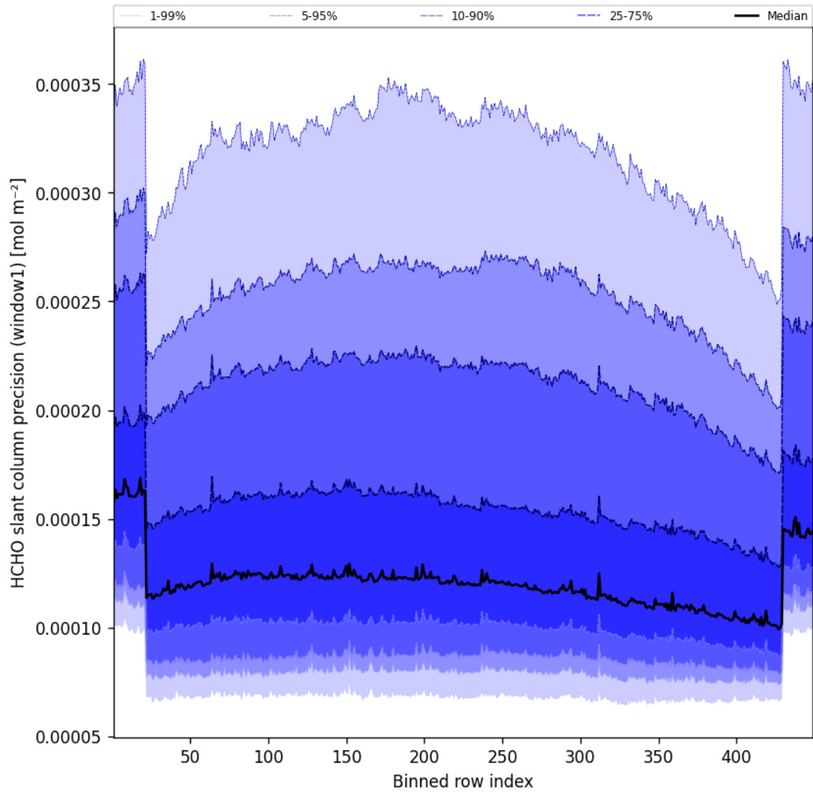
Figure 51: Along track statistics of “HCHO slant column precision (window1)” for 2024-12-09 to 2024-12-09
