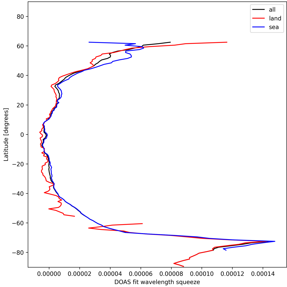
Figure 29: Zonal average of “DOAS fit wavelength squeeze” for 2024-12-09 to 2024-12-09.
