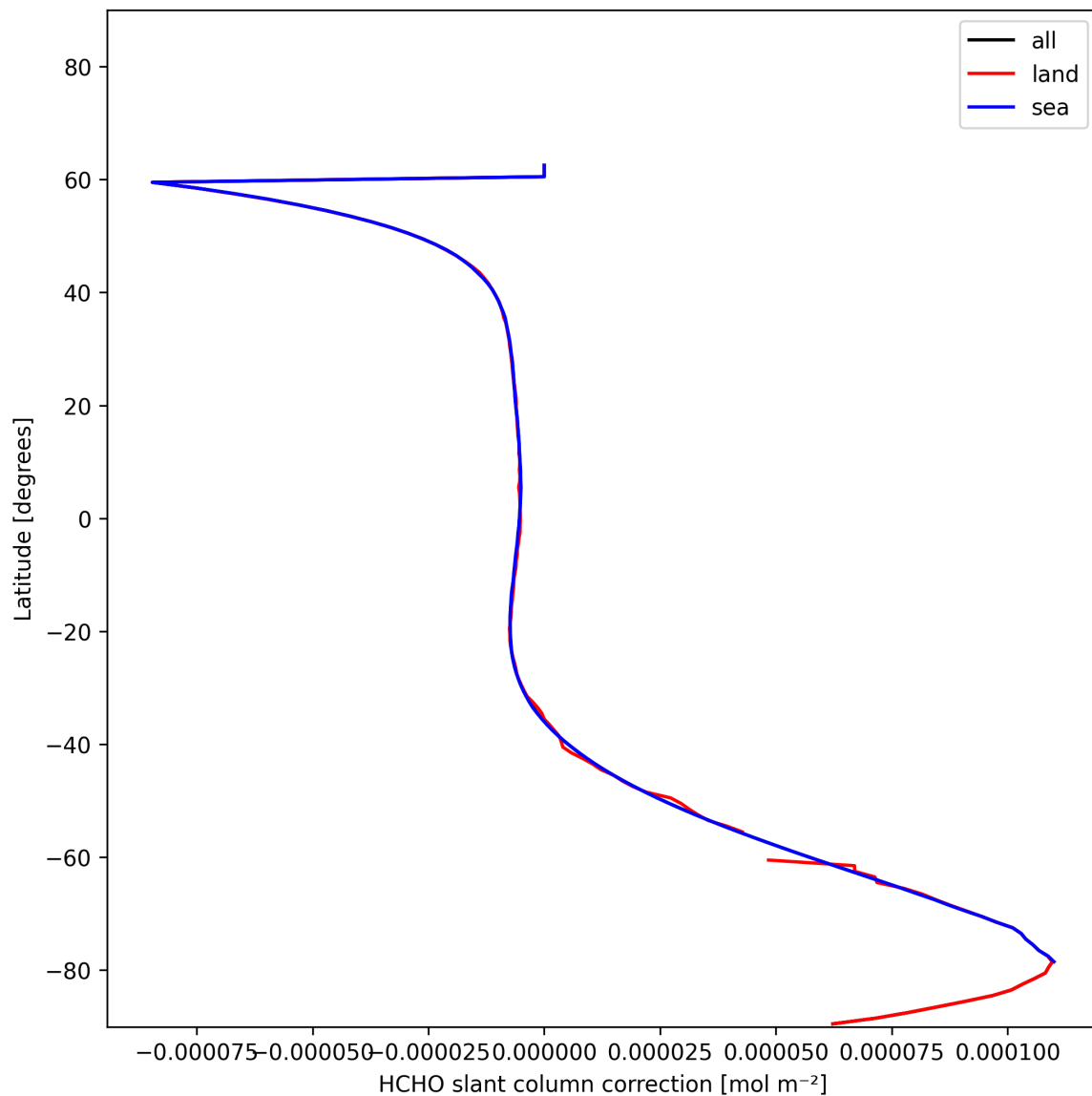
Figure 31: Zonal average of “HCHO slant column correction” for 2024-12-09 to 2024-12-09.
