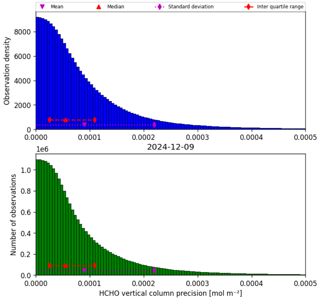
Figure 34: Histogram of “HCHO vertical column precision” for 2024-12-09 to 2024-12-09
