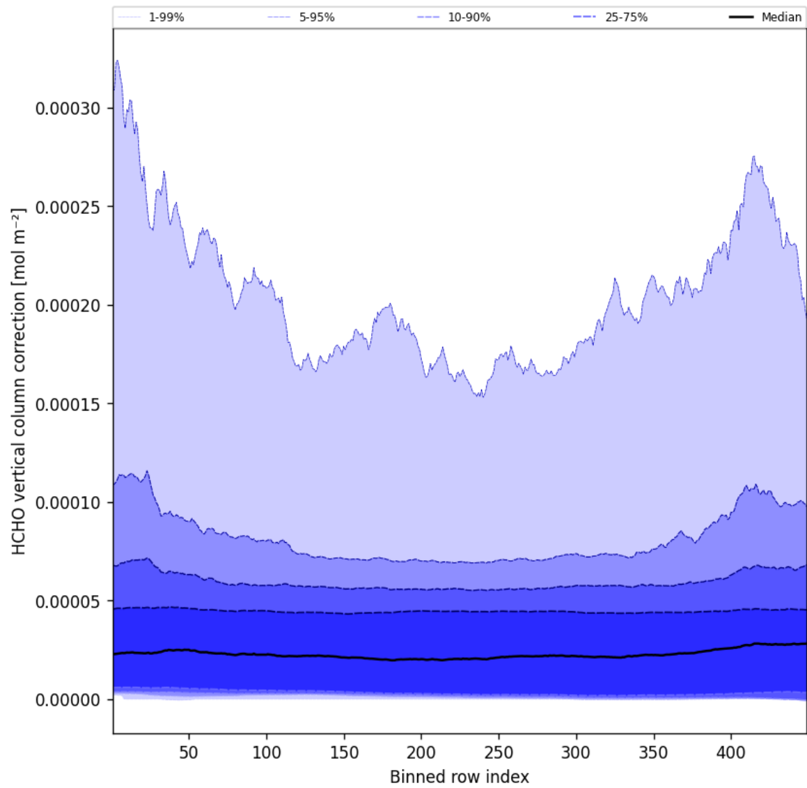
Figure 49: Along track statistics of “HCHO vertical column correction” for 2024-12-09 to 2024-12-09
