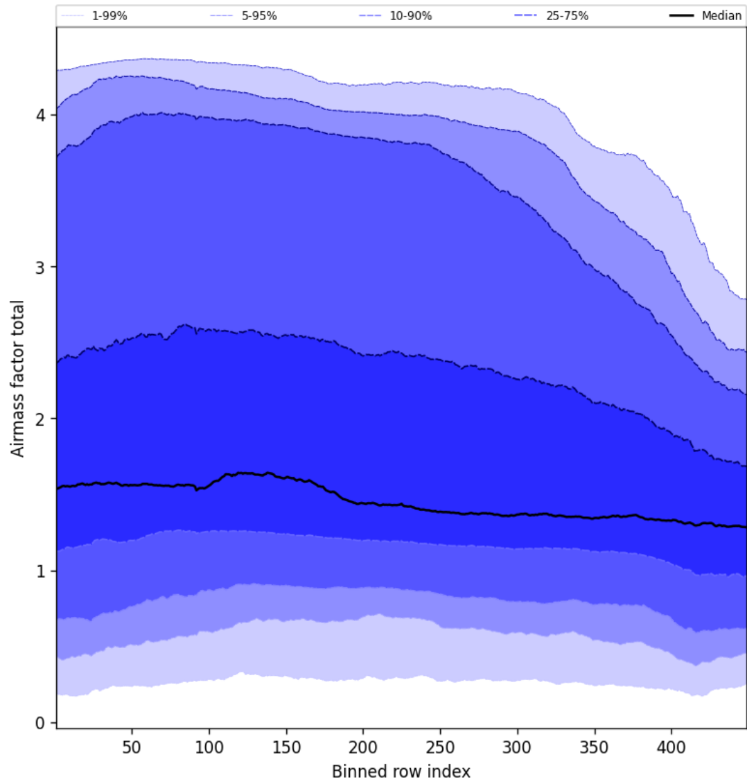
Figure 52: Along track statistics of “Airmass factor total” for 2024-12-09 to 2024-12-09
