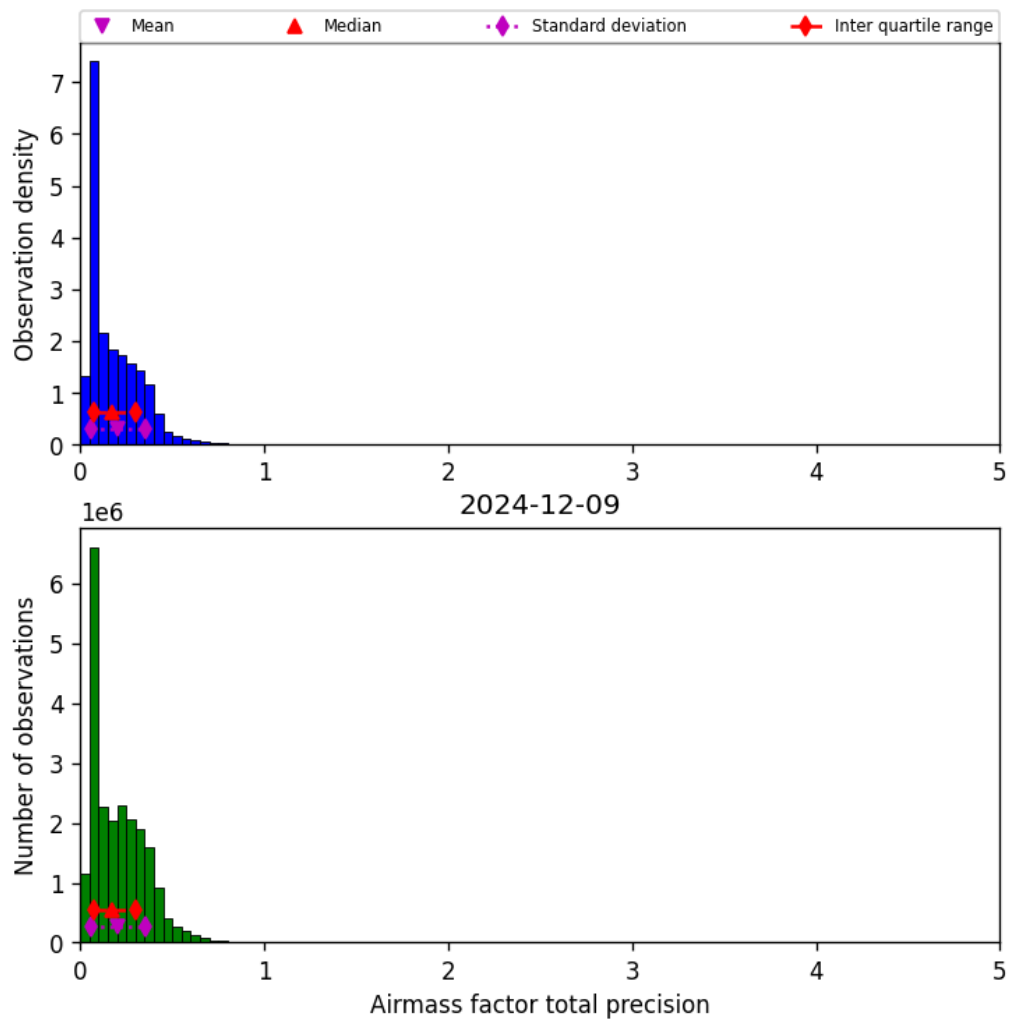
Figure 39: Histogram of “Airmass factor total precision” for 2024-12-09 to 2024-12-09
