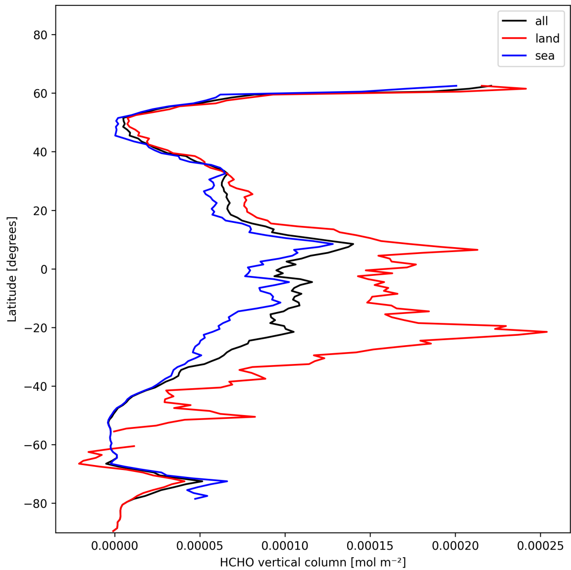
Figure 19: Zonal average of “HCHO vertical column” for 2024-12-09 to 2024-12-09.
