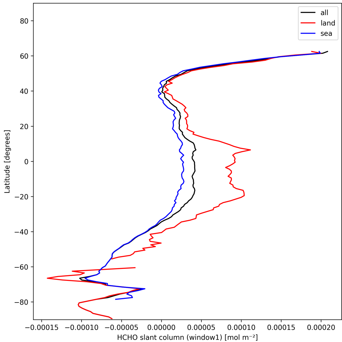
Figure 22: Zonal average of “HCHO slant column (window1)” for 2024-12-09 to 2024-12-09.
