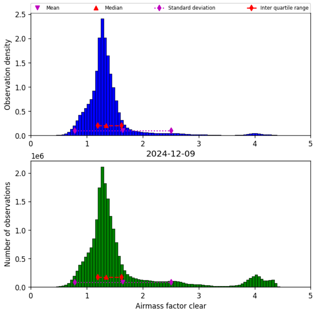
Figure 40: Histogram of “Airmass factor clear” for 2024-12-09 to 2024-12-09
