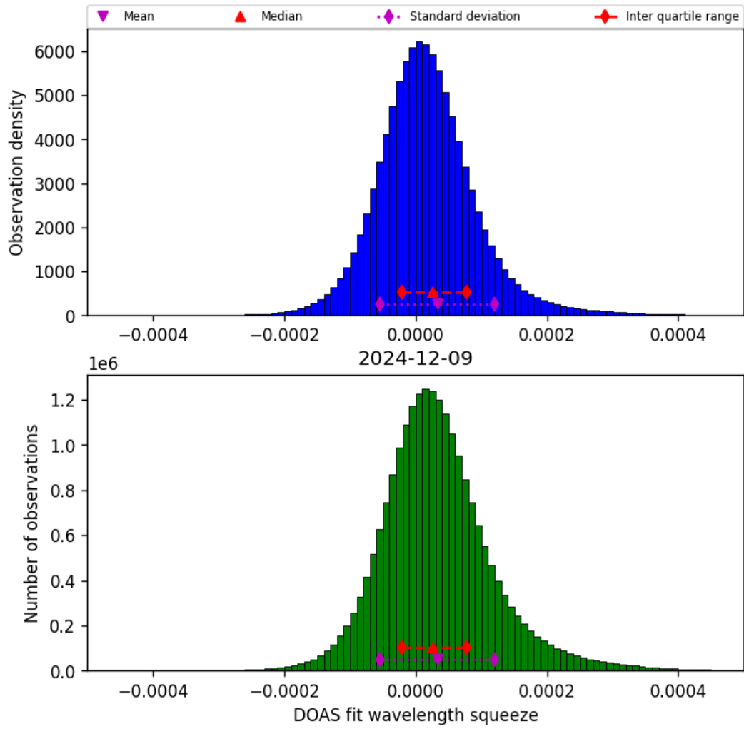
Figure 43: Histogram of “DOAS fit wavelength squeeze” for 2024-12-09 to 2024-12-09
