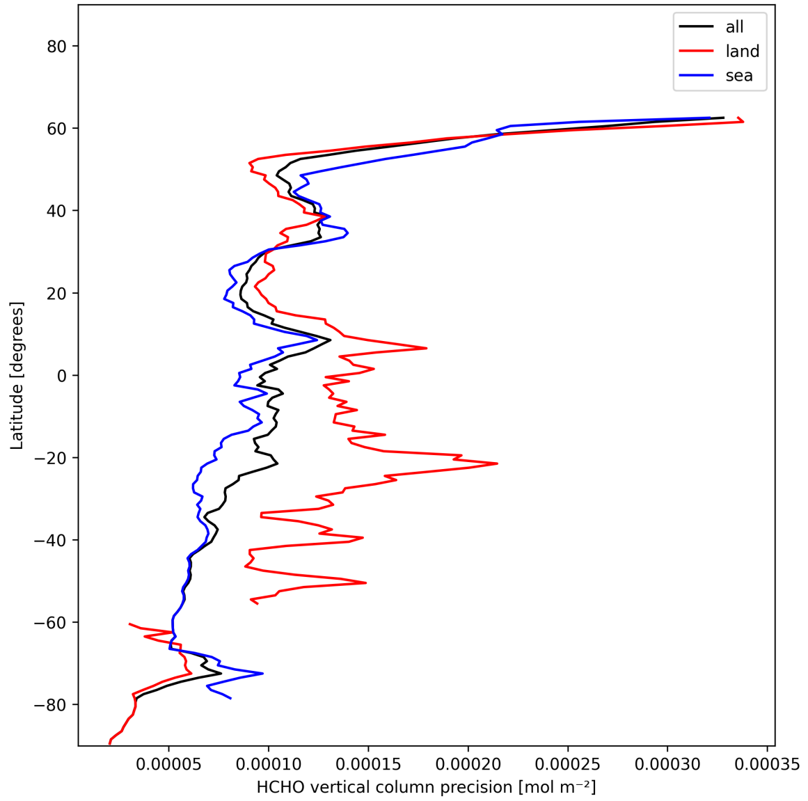
Figure 20: Zonal average of “HCHO vertical column precision” for 2024-12-09 to 2024-12-09.
