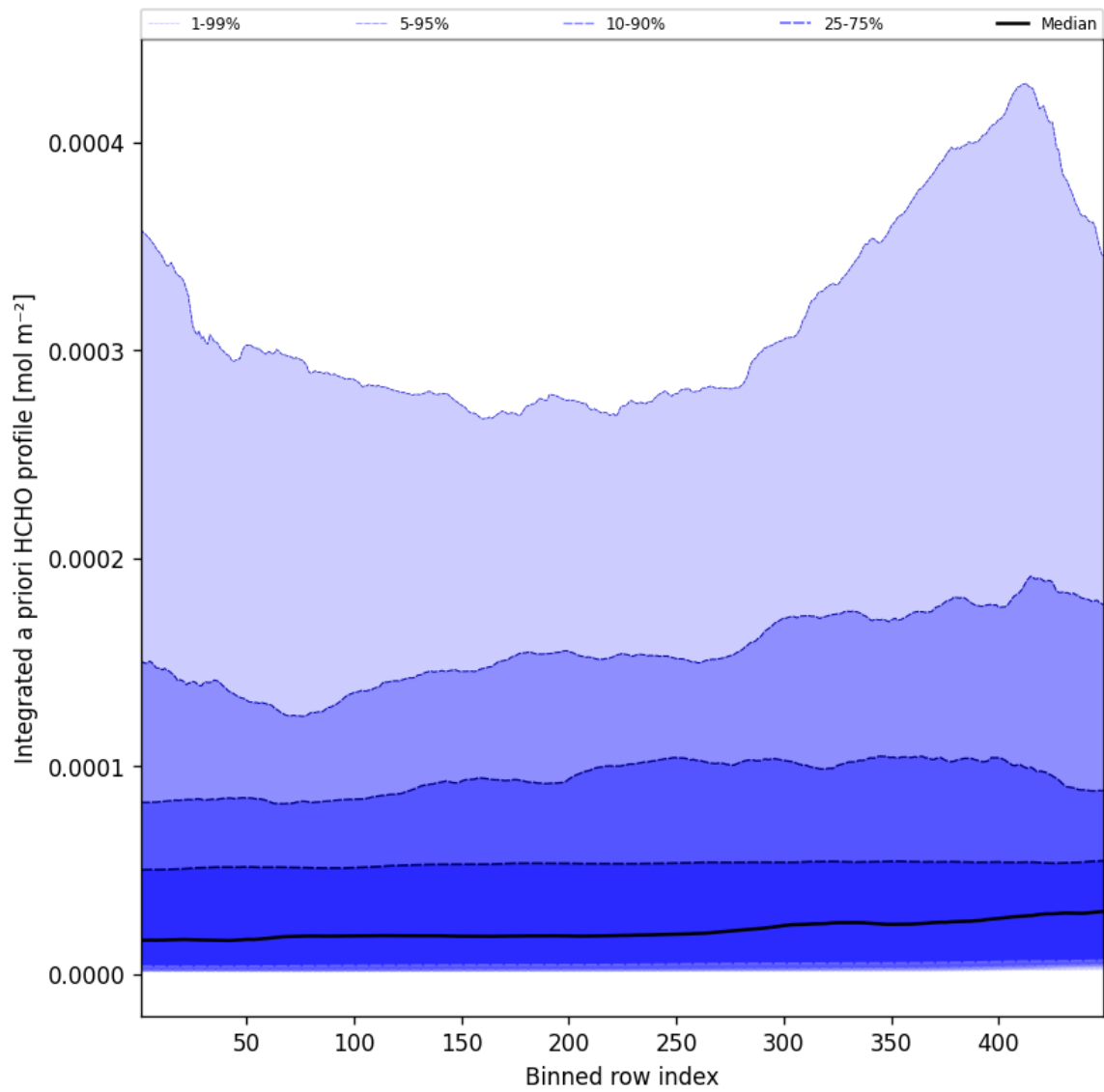
Figure 55: Along track statistics of “Integrated a priori HCHO profile” for 2024-12-09 to 2024-12-09
