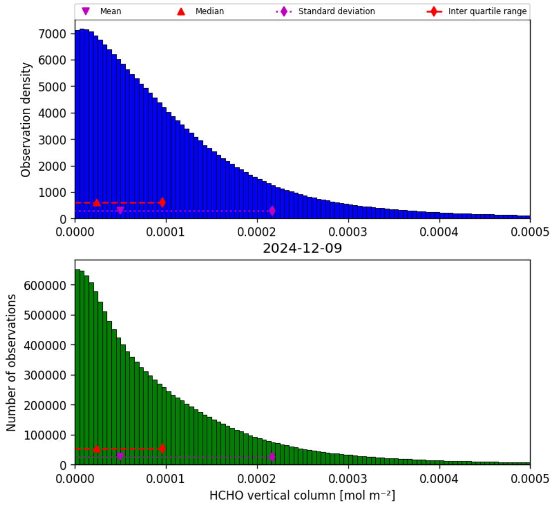
Figure 33: Histogram of “HCHO vertical column” for 2024-12-09 to 2024-12-09
