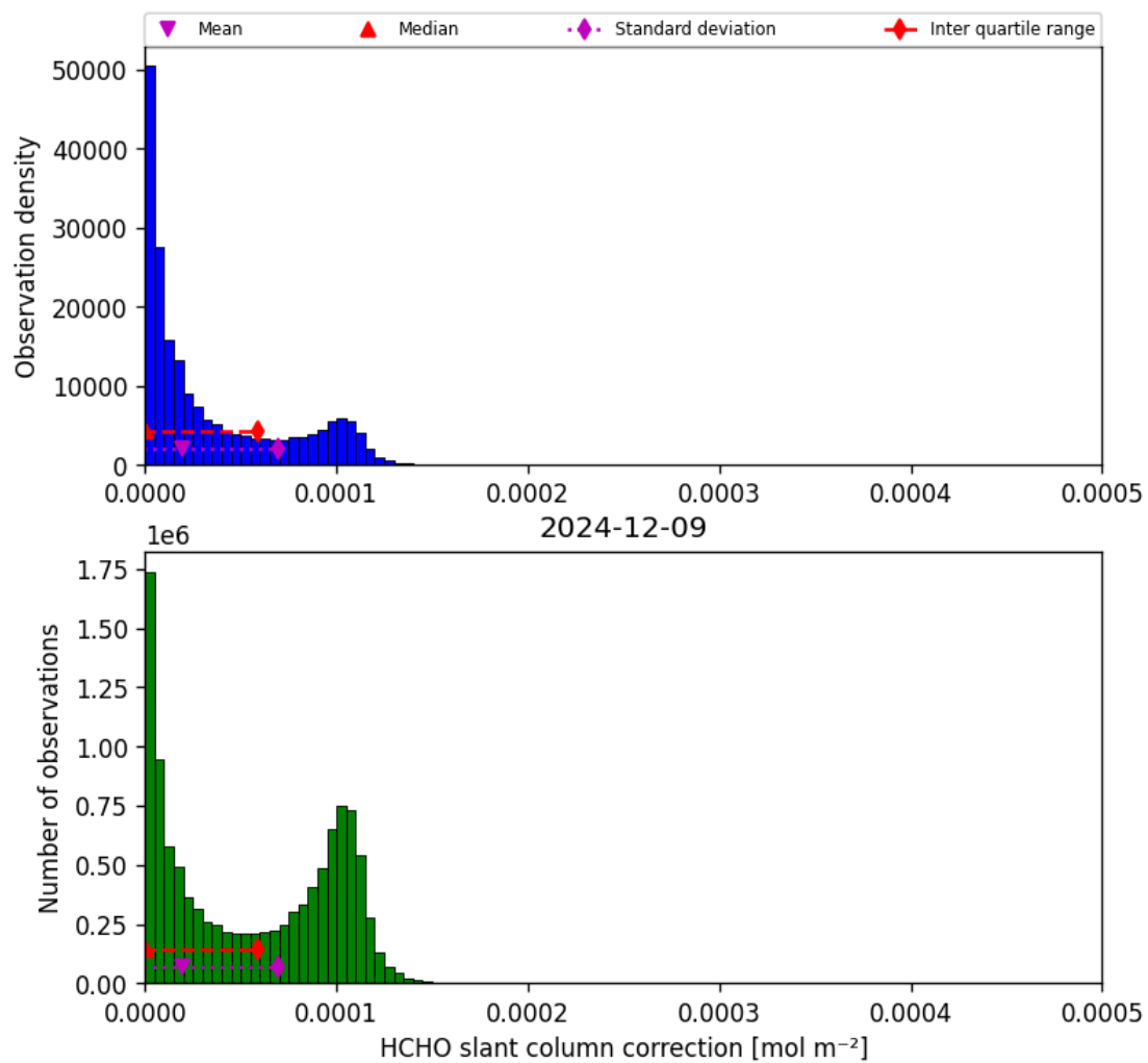
Figure 45: Histogram of “HCHO slant column correction” for 2024-12-09 to 2024-12-09
