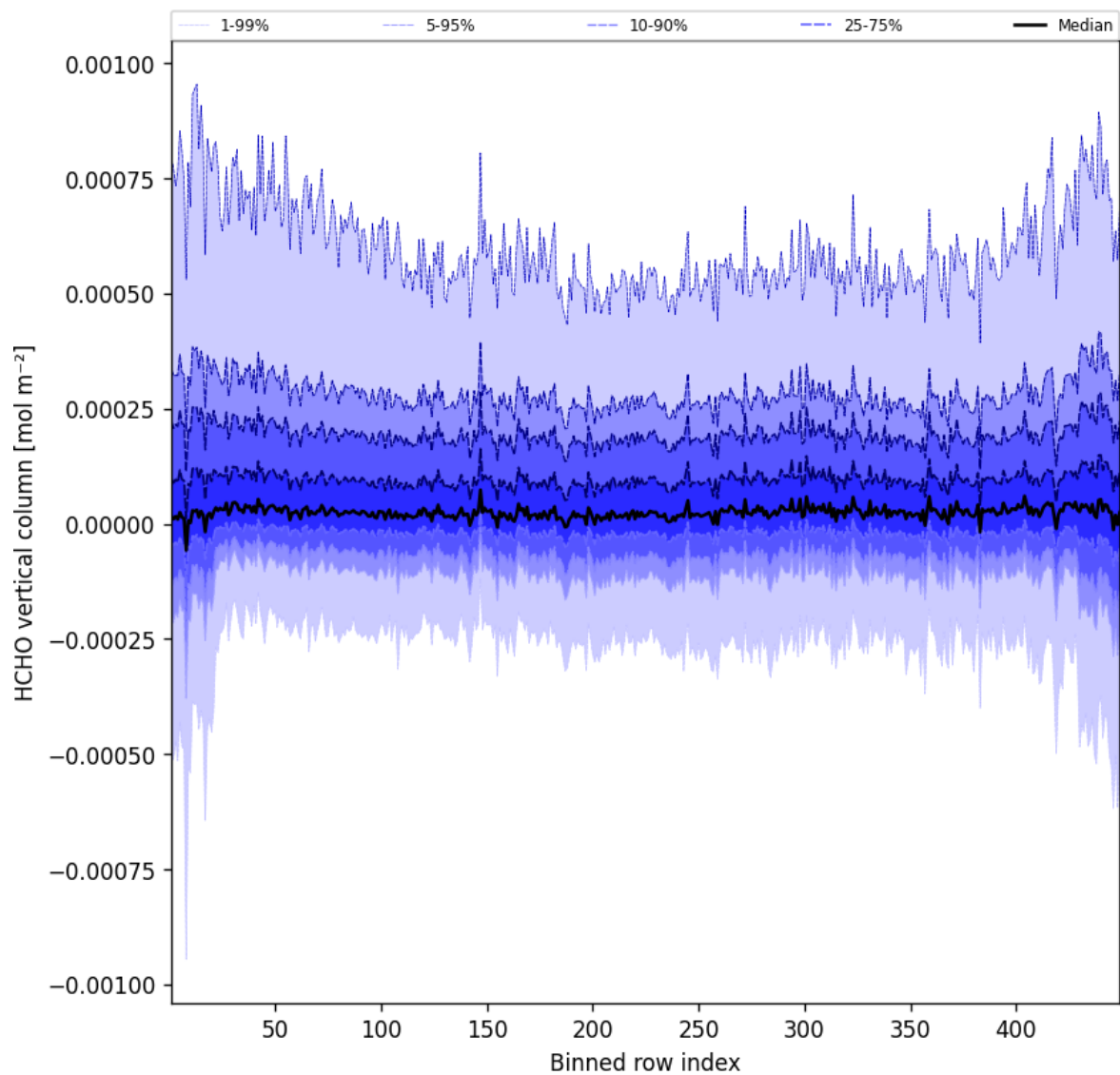
Figure 47: Along track statistics of “HCHO vertical column” for 2024-12-09 to 2024-12-09
