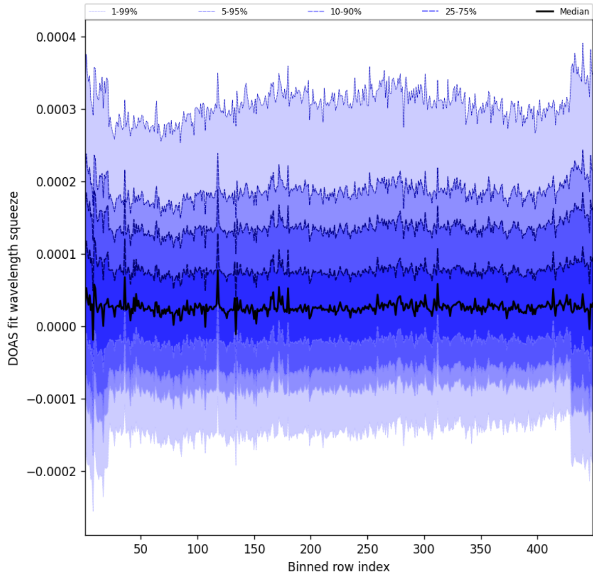
Figure 57: Along track statistics of “DOAS fit wavelength squeeze” for 2024-12-09 to 2024-12-09
