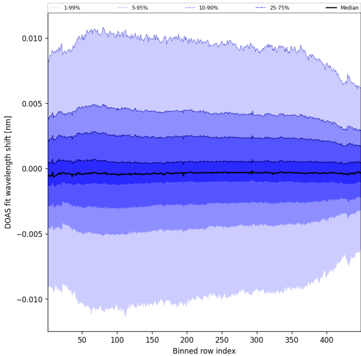
Figure 56: Along track statistics of “DOAS fit wavelength shift” for 2024-12-09 to 2024-12-09
