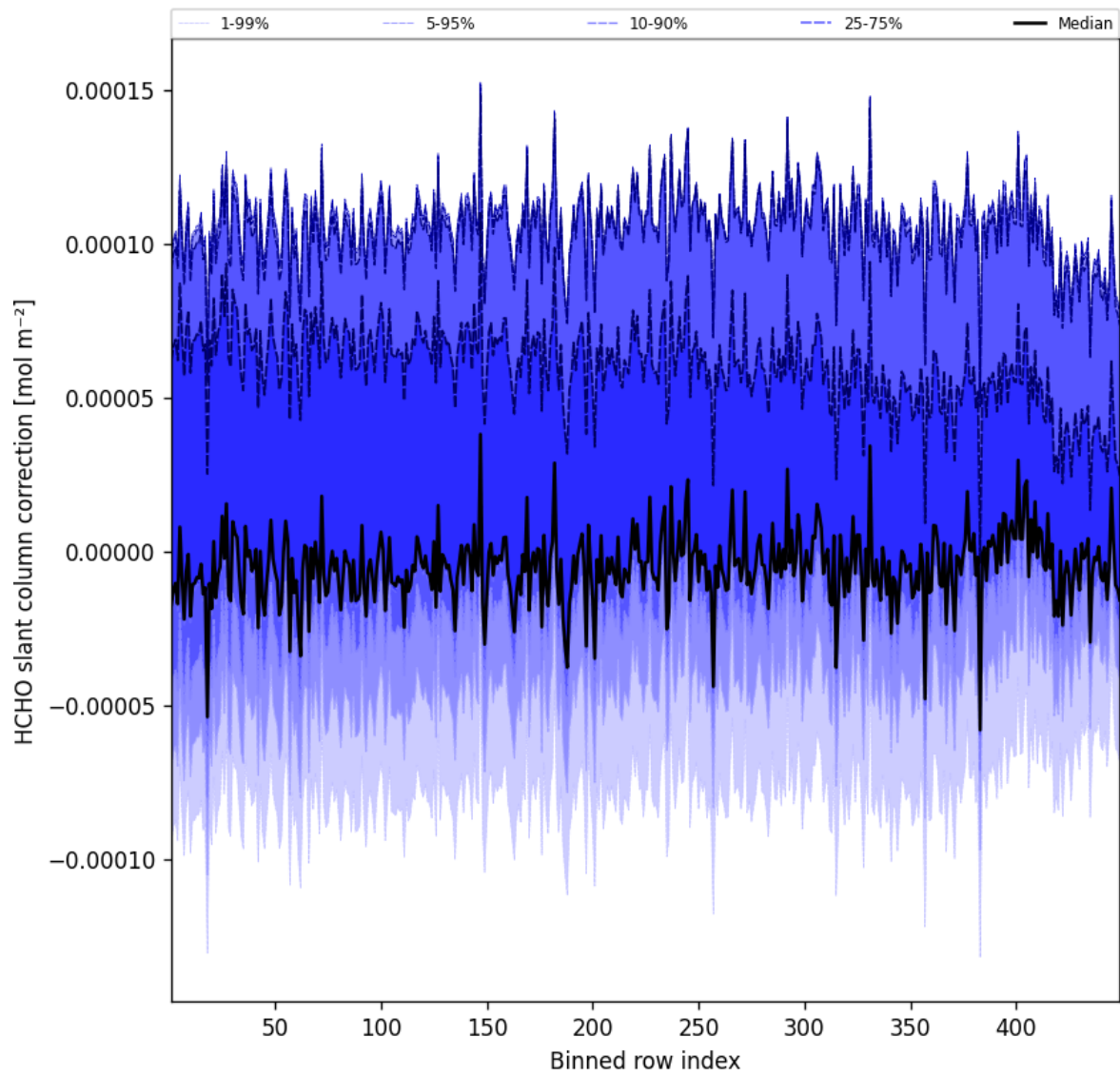
Figure 59: Along track statistics of “HCHO slant column correction” for 2024-12-09 to 2024-12-09
