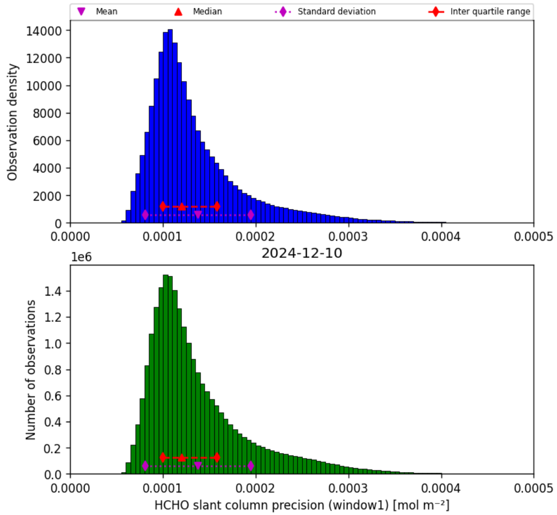
Figure 37: Histogram of “HCHO slant column precision (window1)” for 2024-12-10 to 2024-12-11
