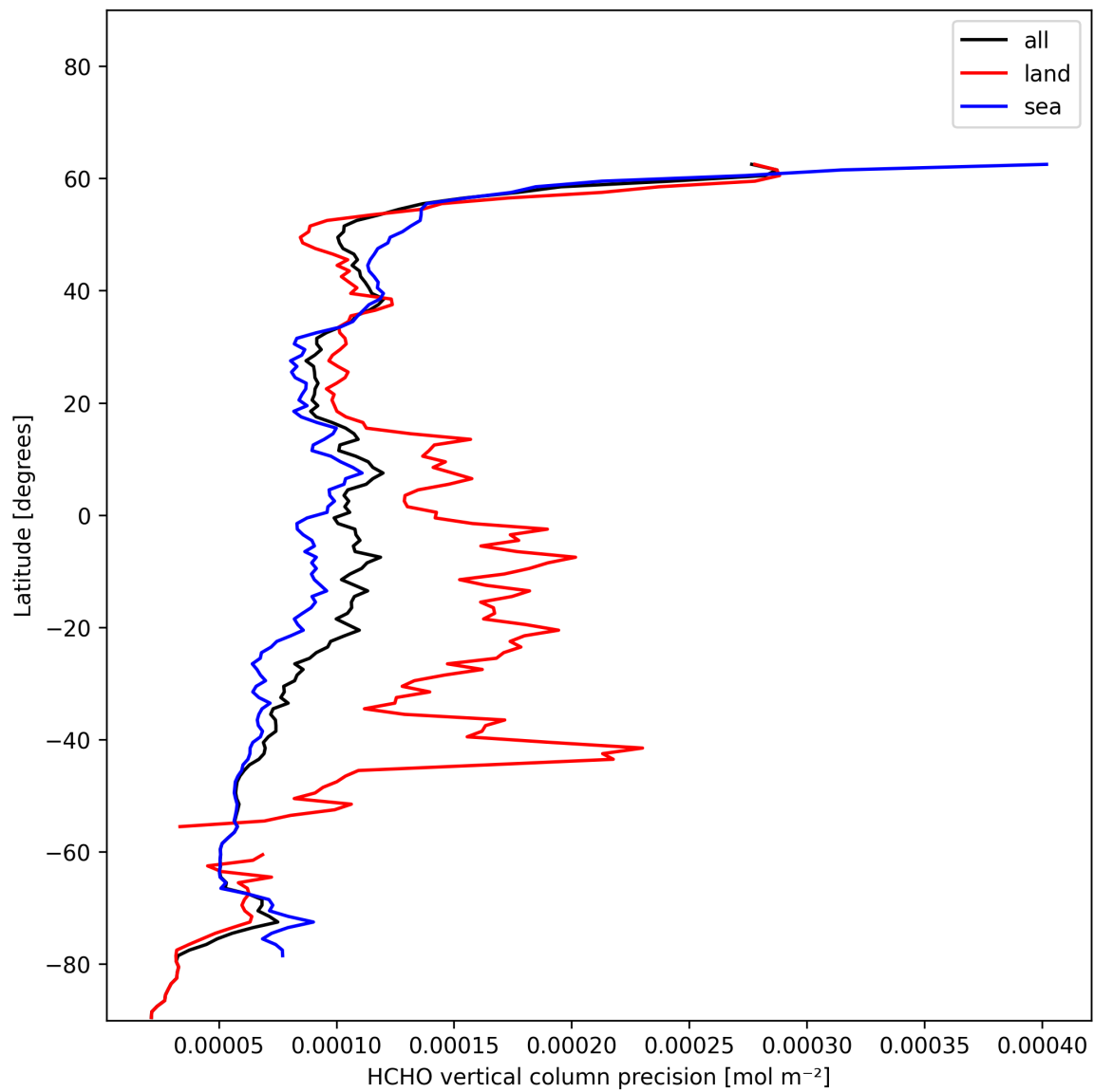
Figure 20: Zonal average of “HCHO vertical column precision” for 2024-12-10 to 2024-12-11.
