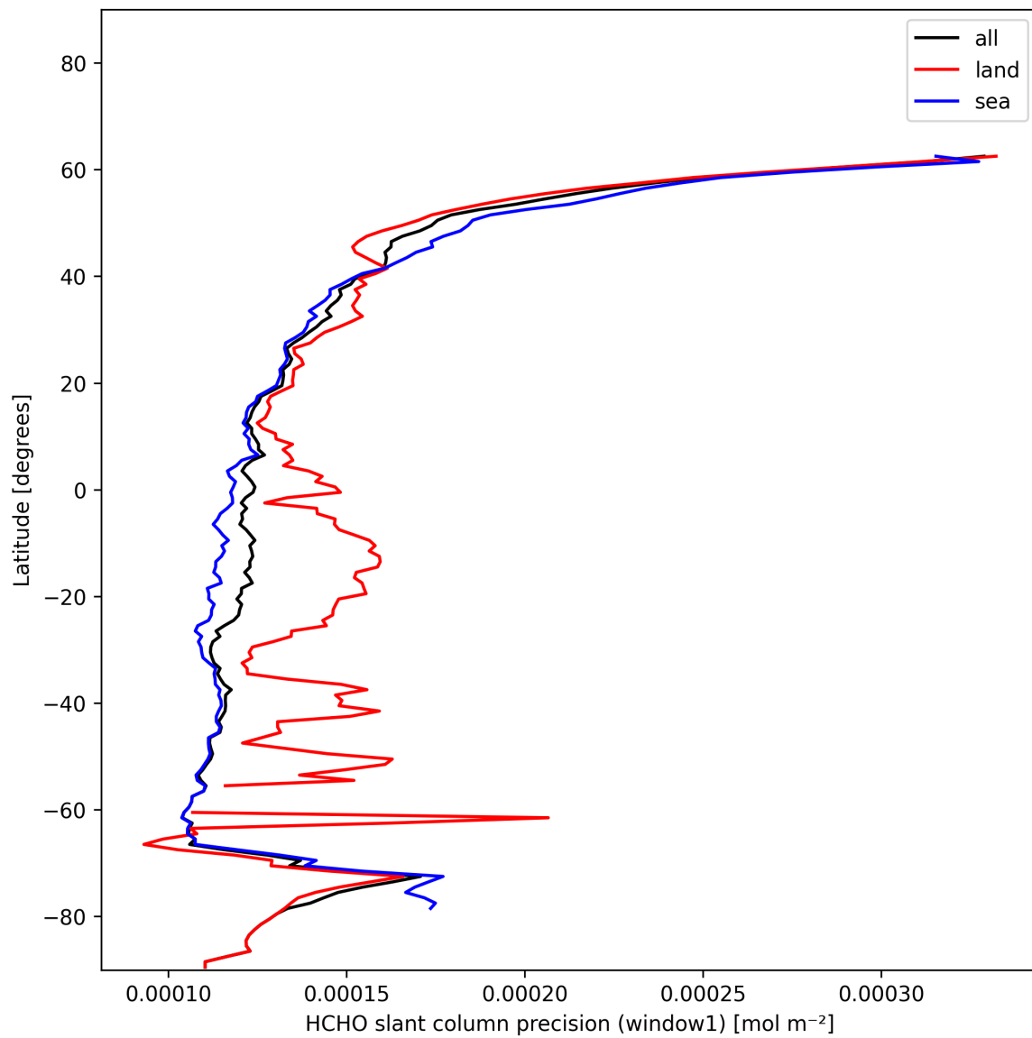
Figure 23: Zonal average of “HCHO slant column precision (window1)” for 2024-12-10 to 2024-12-11.
