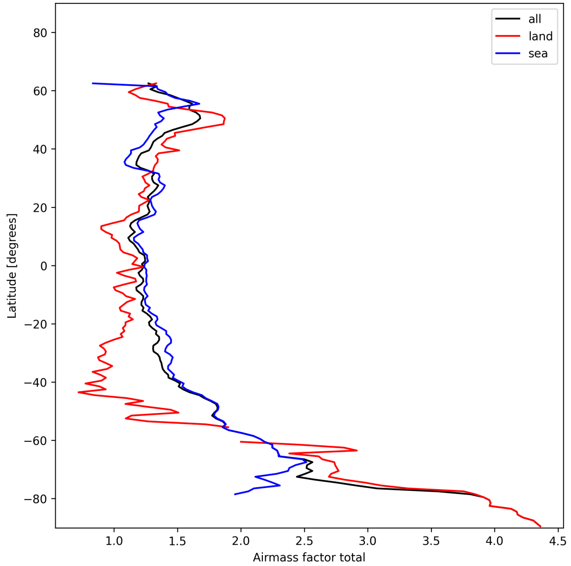
Figure 24: Zonal average of “Airmass factor total” for 2024-12-10 to 2024-12-11.
