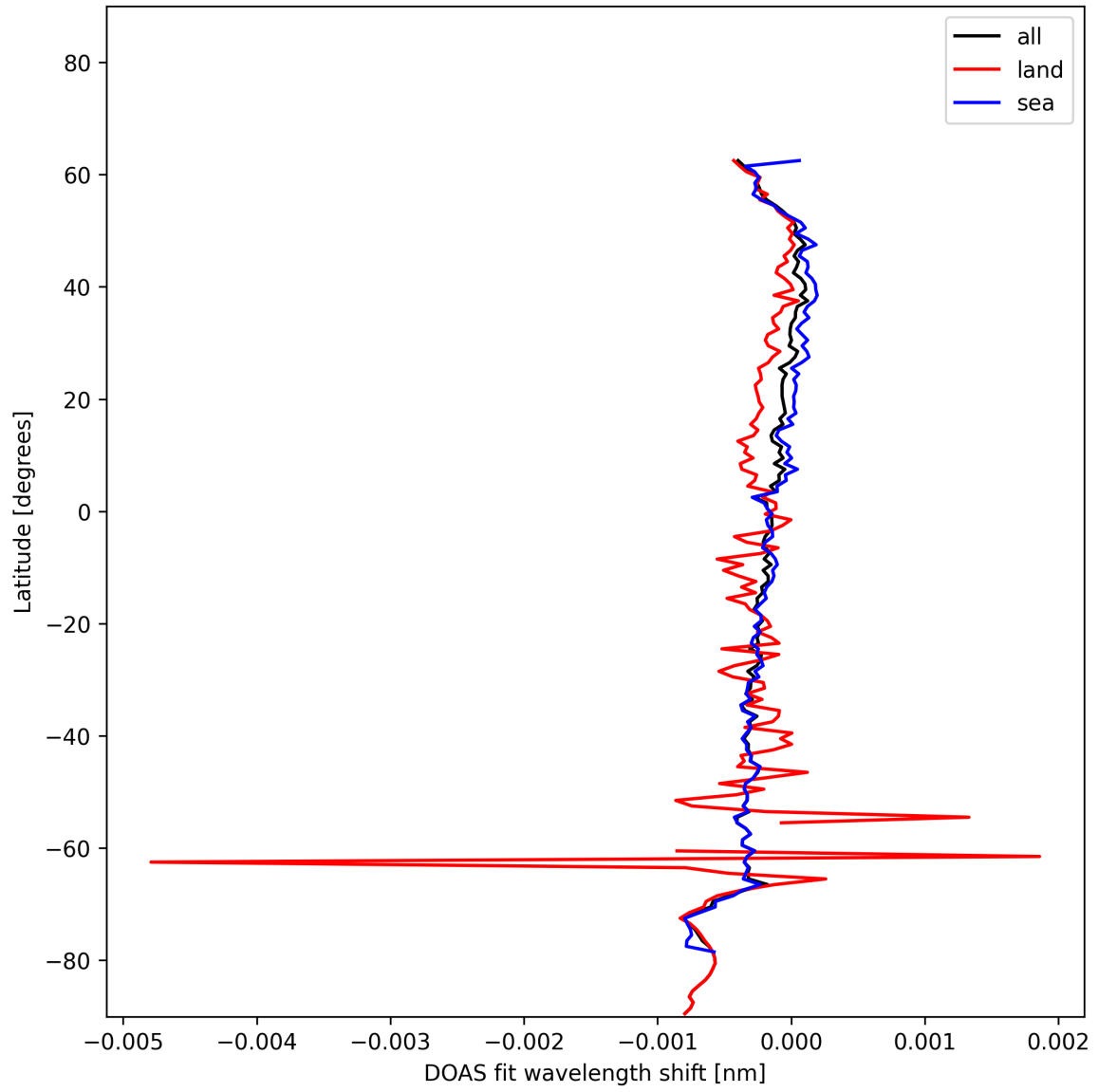
Figure 28: Zonal average of “DOAS fit wavelength shift” for 2024-12-10 to 2024-12-11.
