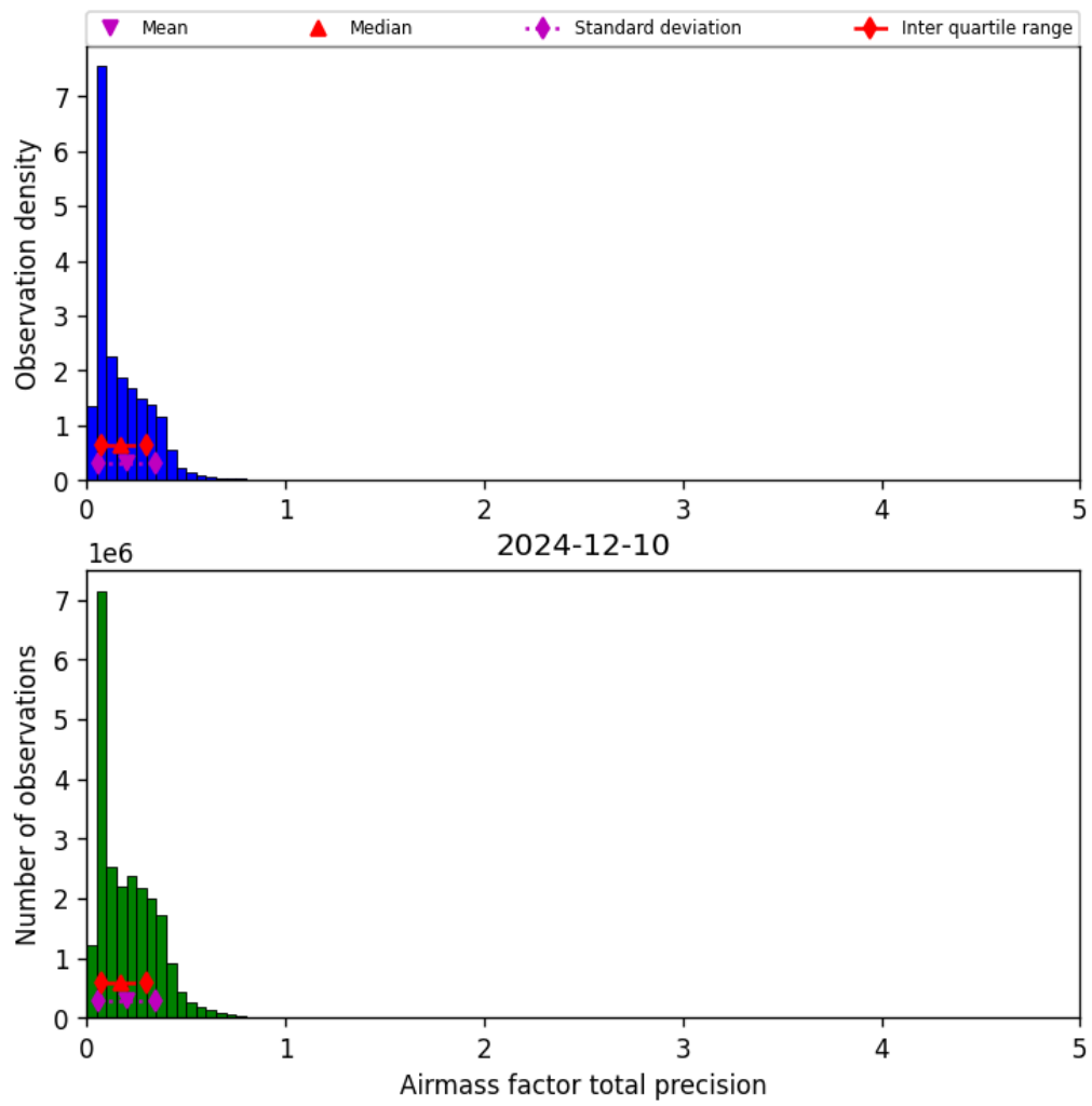
Figure 39: Histogram of “Airmass factor total precision” for 2024-12-10 to 2024-12-11
