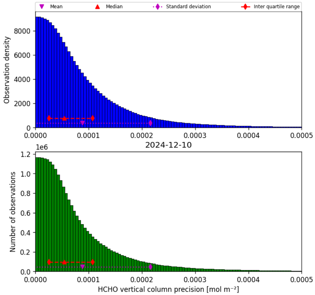
Figure 34: Histogram of “HCHO vertical column precision” for 2024-12-10 to 2024-12-11
