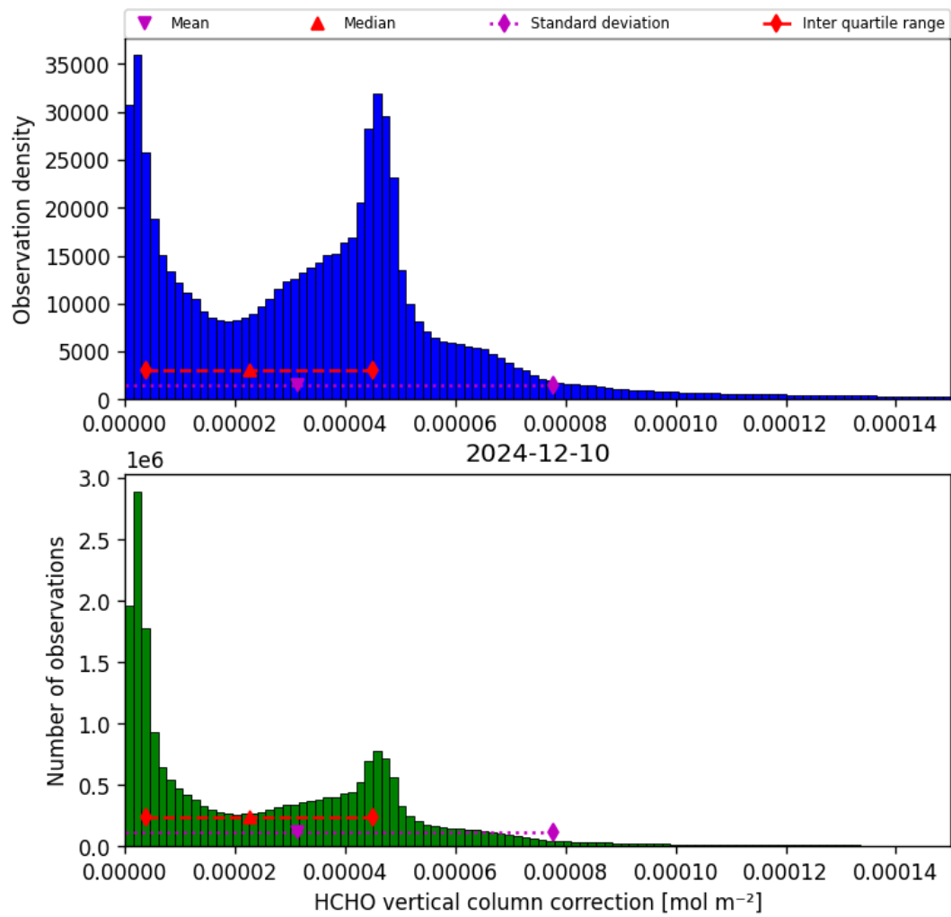
Figure 35: Histogram of “HCHO vertical column correction” for 2024-12-10 to 2024-12-11
