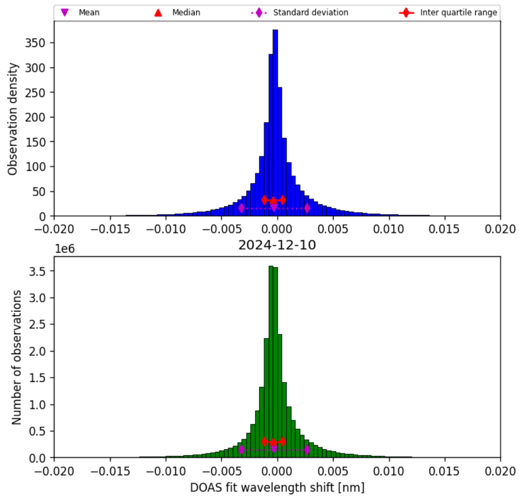
Figure 42: Histogram of “DOAS fit wavelength shift” for 2024-12-10 to 2024-12-11
