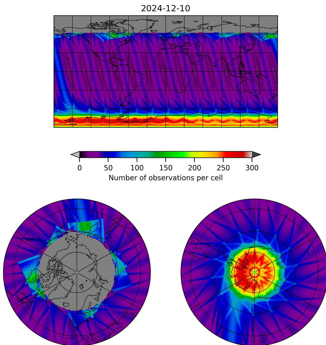
Figure 17: Map of the number of observations for 2024-12-10 to 2024-12-11
