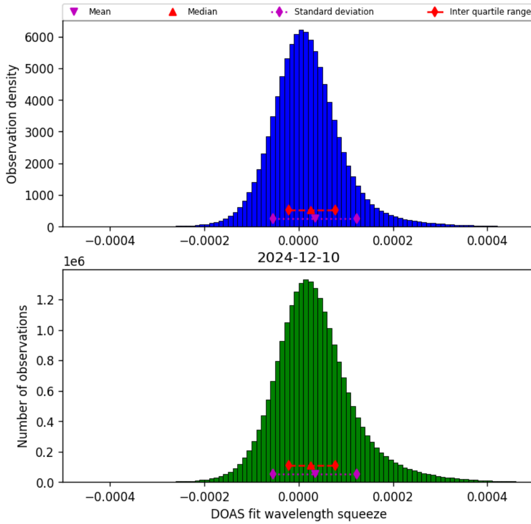
Figure 43: Histogram of “DOAS fit wavelength squeeze” for 2024-12-10 to 2024-12-11
