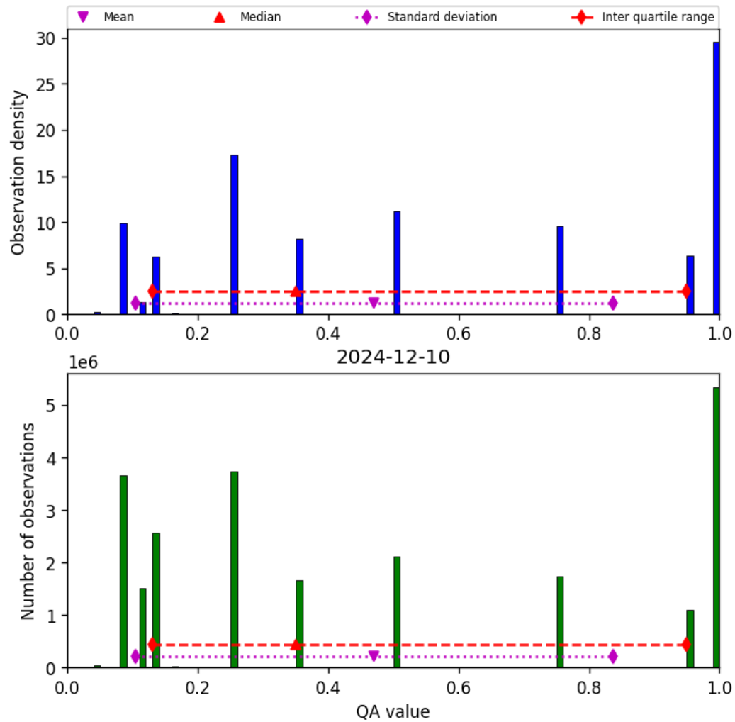
Figure 32: Histogram of “QA value” for 2024-12-10 to 2024-12-11
