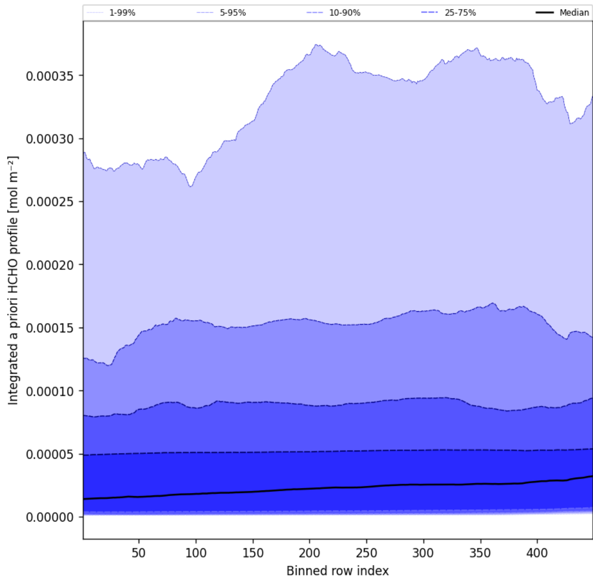
Figure 55: Along track statistics of “Integrated a priori HCHO profile” for 2024-12-10 to 2024-12-11
