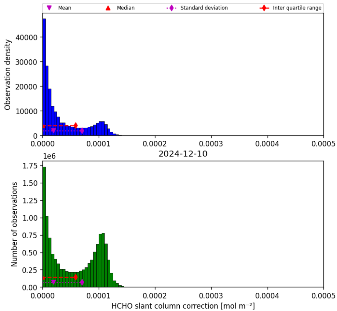
Figure 45: Histogram of “HCHO slant column correction” for 2024-12-10 to 2024-12-11
