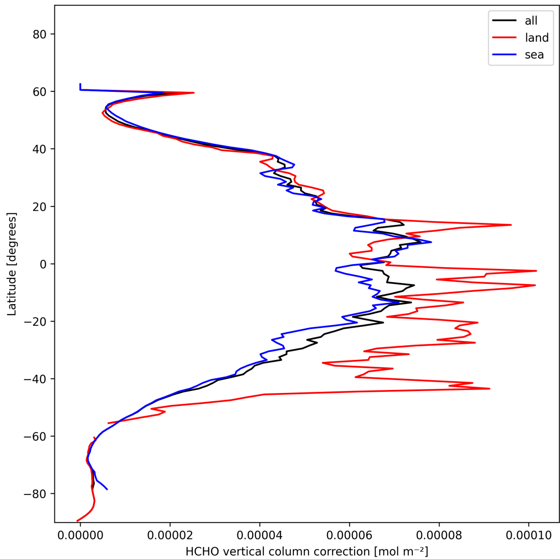
Figure 21: Zonal average of “HCHO vertical column correction” for 2024-12-10 to 2024-12-11.
