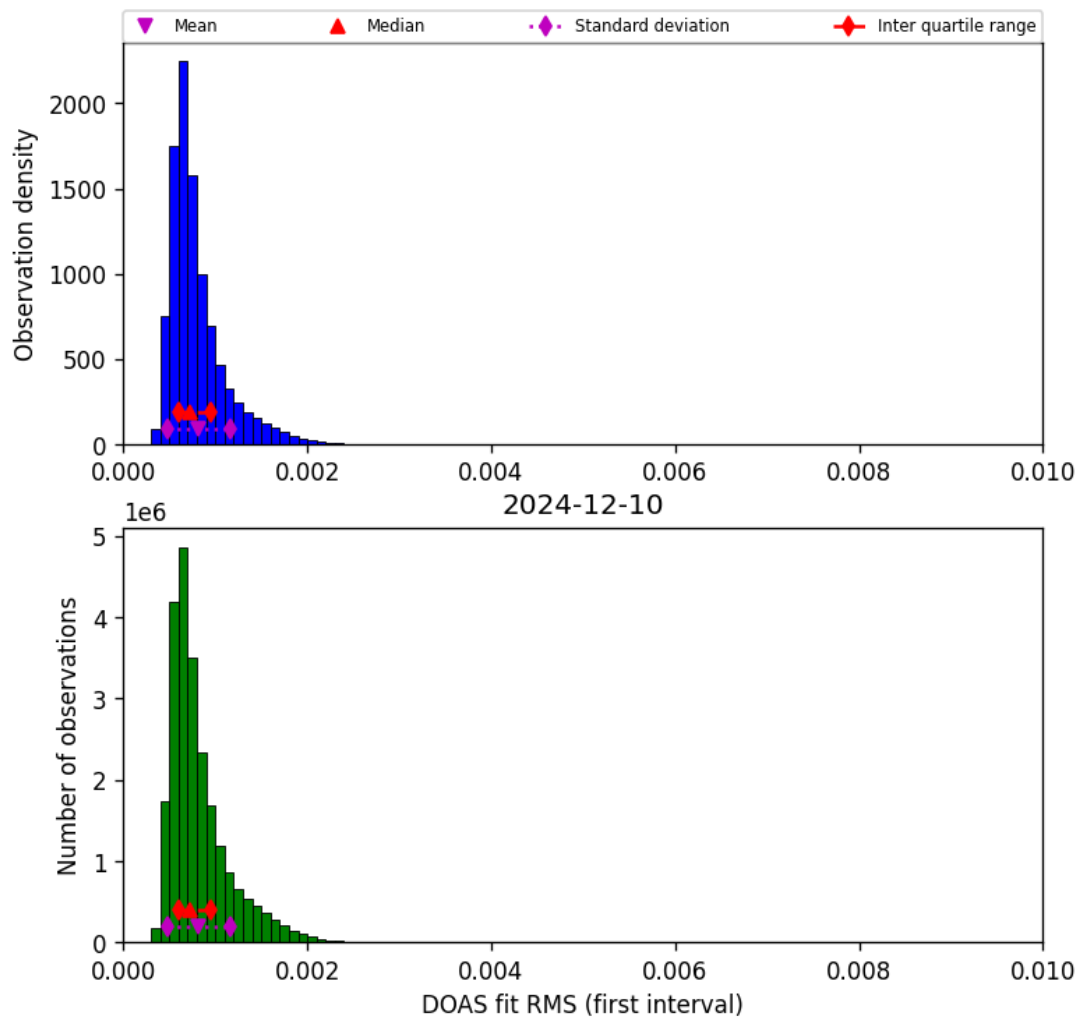
Figure 44: Histogram of “DOAS fit RMS (first interval)” for 2024-12-10 to 2024-12-11
