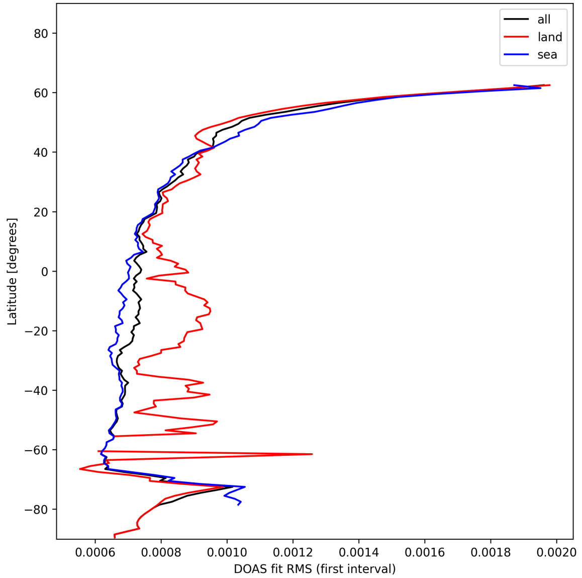
Figure 30: Zonal average of "DOAS fit RMS (first interval)" for 2024-12-10 to 2024-12-11.
