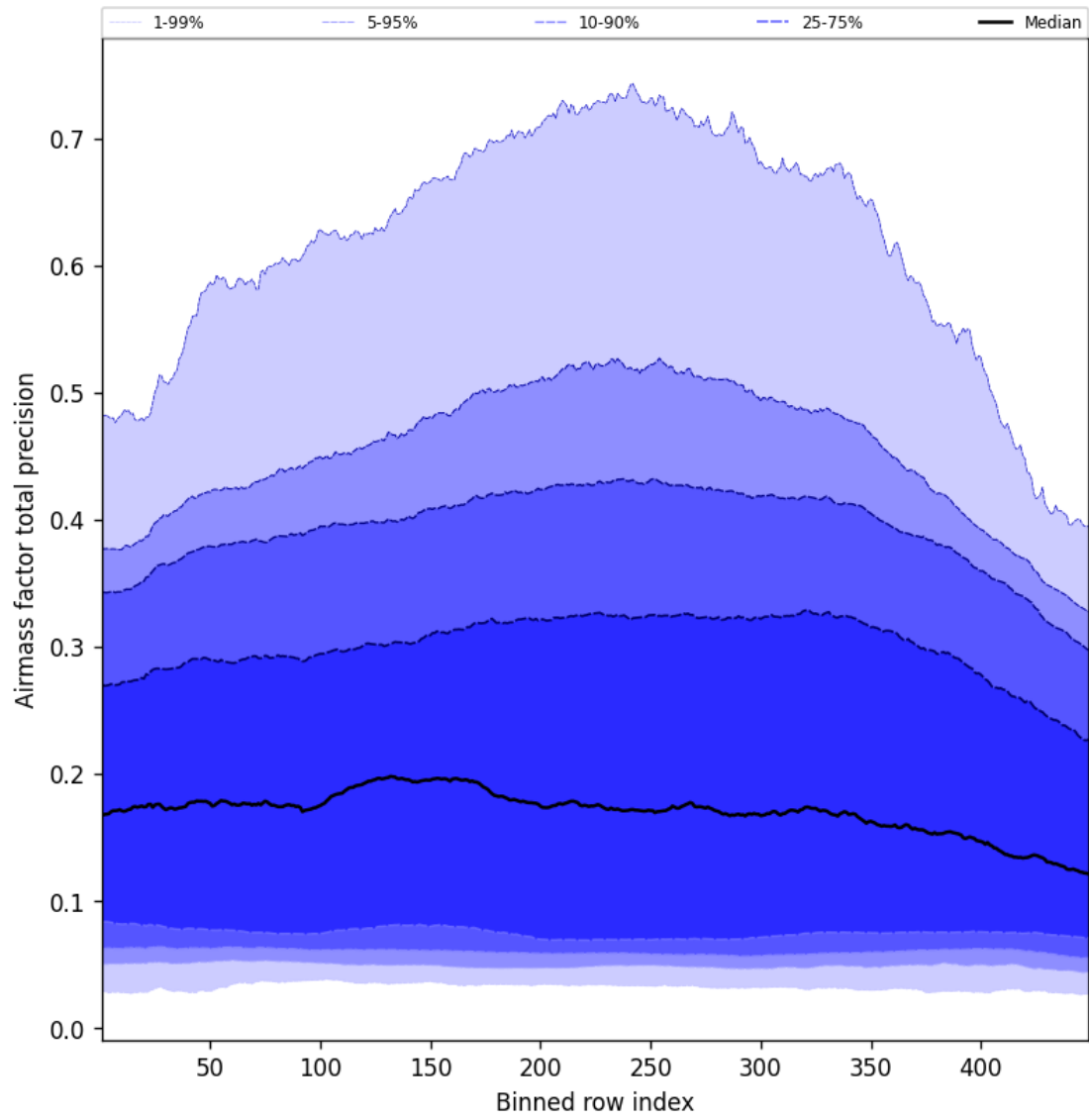
Figure 53: Along track statistics of “Airmass factor total precision” for 2024-12-10 to 2024-12-11
