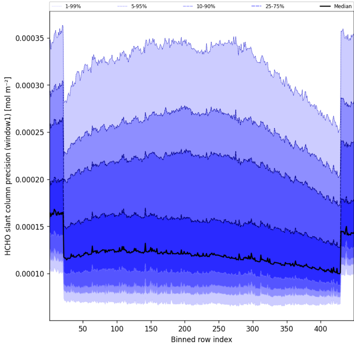
Figure 51: Along track statistics of “HCHO slant column precision (window1)” for 2024-12-10 to 2024-12-11
