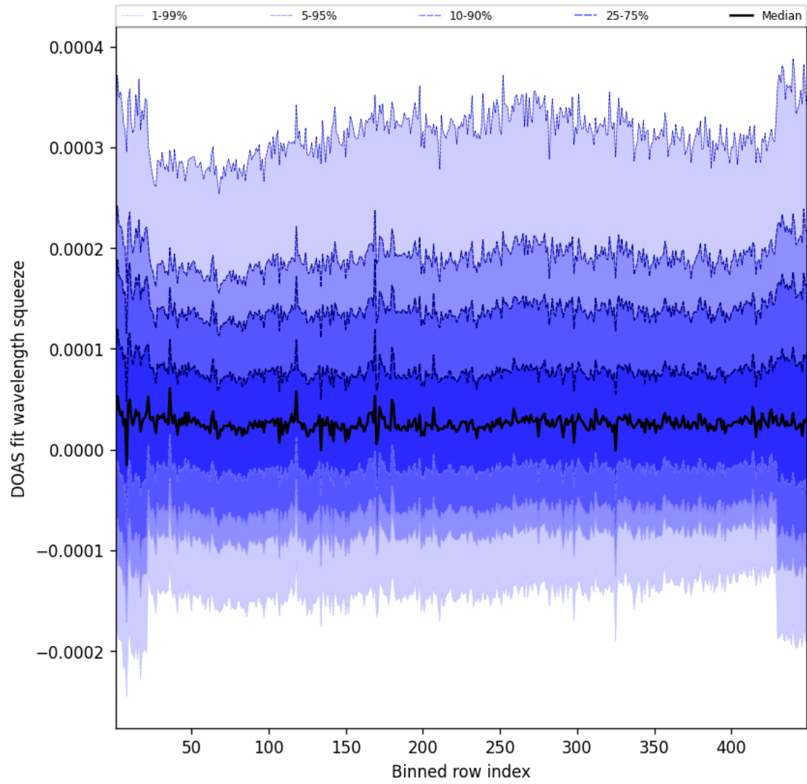
Figure 57: Along track statistics of “DOAS fit wavelength squeeze” for 2024-12-10 to 2024-12-11
