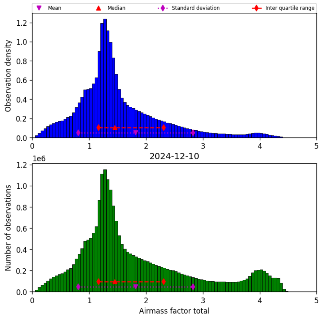
Figure 38: Histogram of “Airmass factor total” for 2024-12-10 to 2024-12-11
