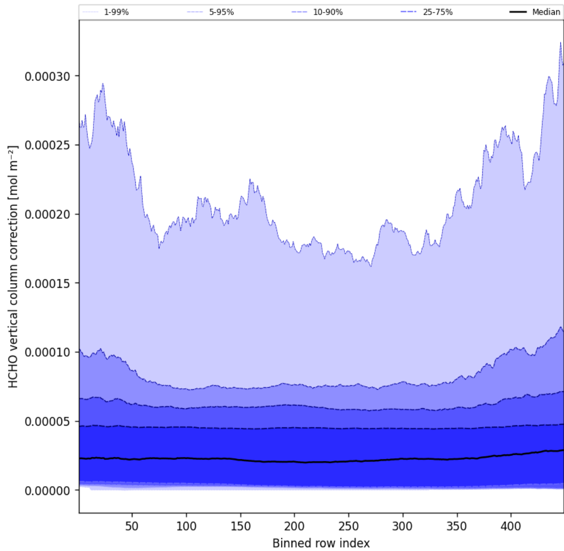
Figure 49: Along track statistics of “HCHO vertical column correction” for 2024-12-10 to 2024-12-11
