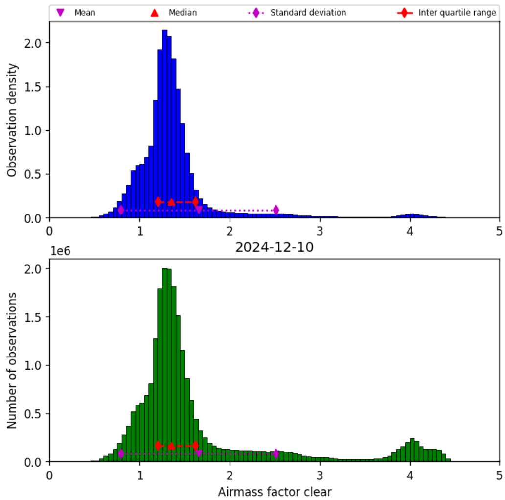
Figure 40: Histogram of “Airmass factor clear” for 2024-12-10 to 2024-12-11
