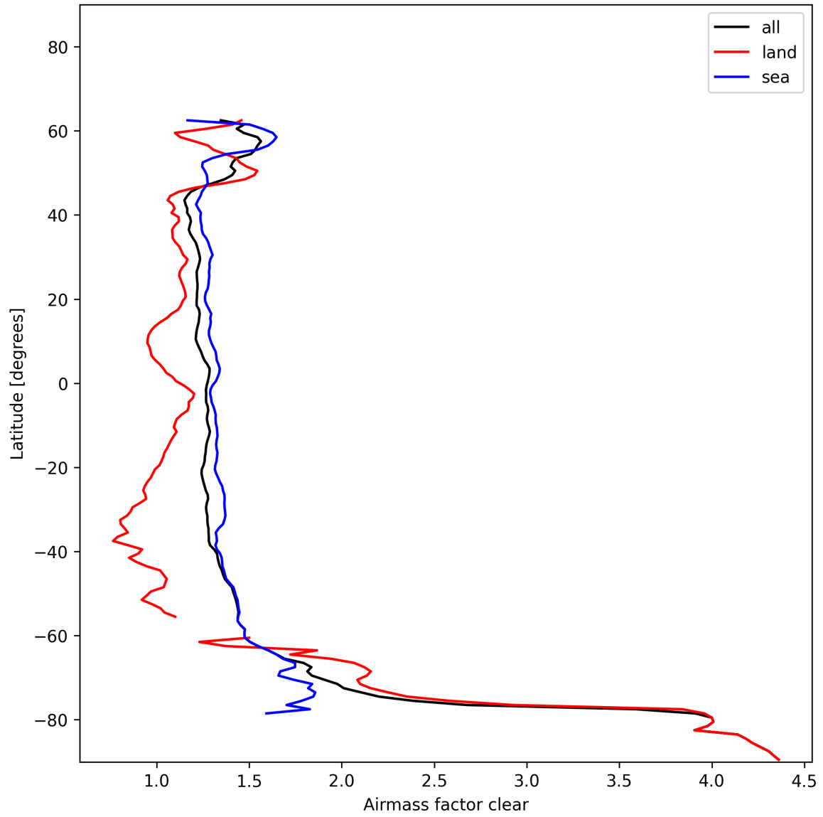
Figure 26: Zonal average of “Airmass factor clear” for 2024-12-10 to 2024-12-11.
