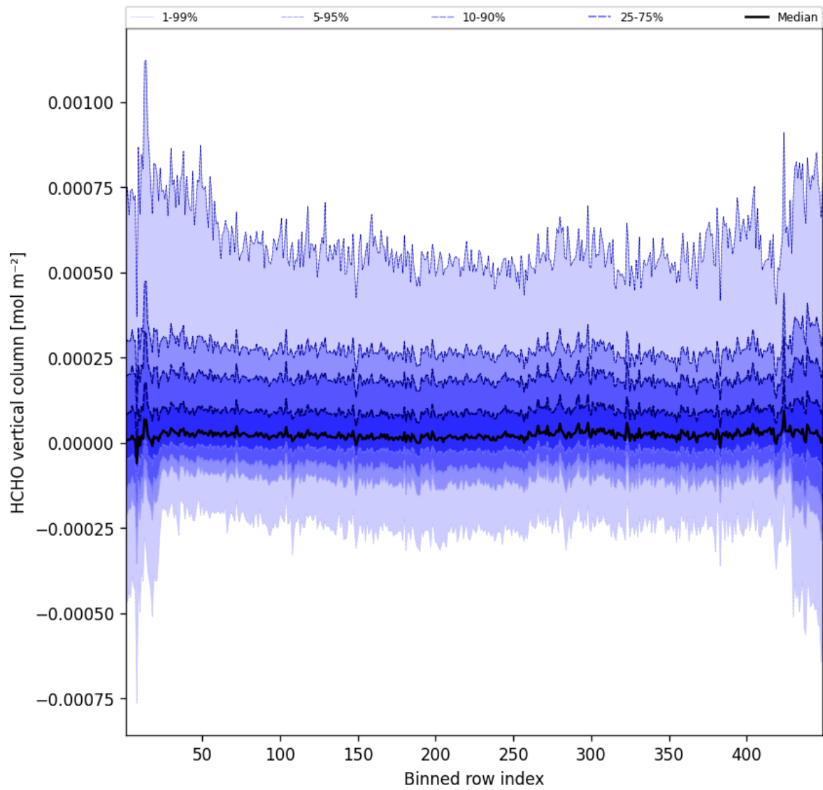
Figure 47: Along track statistics of “HCHO vertical column” for 2024-12-10 to 2024-12-11
