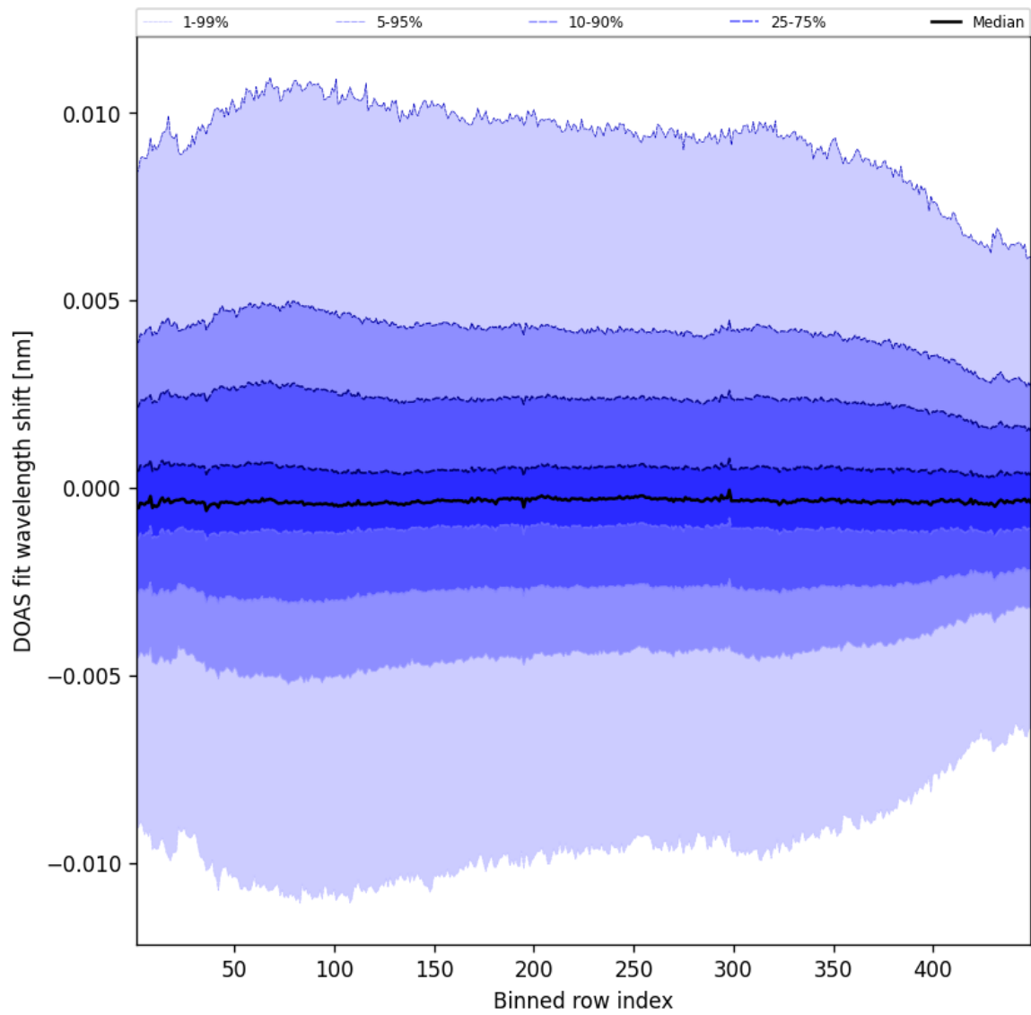
Figure 56: Along track statistics of “DOAS fit wavelength shift” for 2024-12-10 to 2024-12-11
