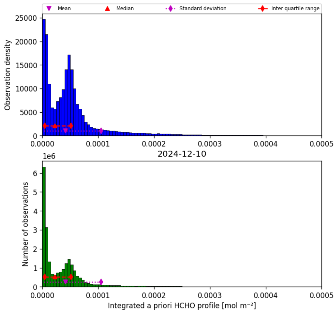
Figure 41: Histogram of “Integrated a priori HCHO profile” for 2024-12-10 to 2024-12-11
