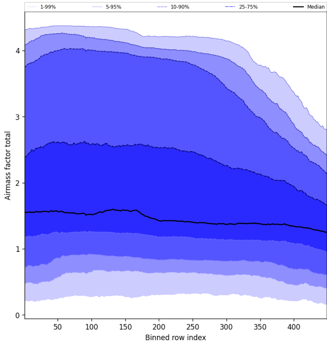
Figure 52: Along track statistics of “Airmass factor total” for 2024-12-10 to 2024-12-11
