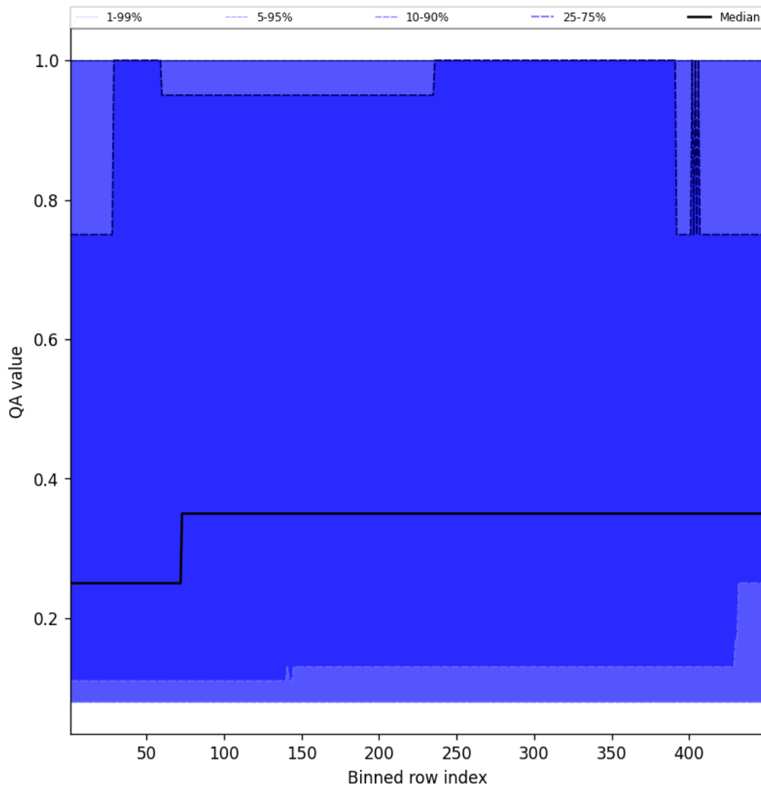
Figure 46: Along track statistics of “QA value” for 2024-12-10 to 2024-12-11
