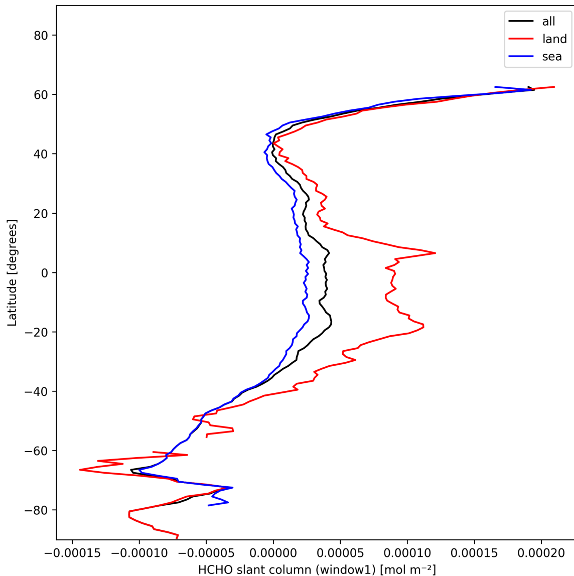
Figure 22: Zonal average of “HCHO slant column (window1)” for 2024-12-10 to 2024-12-11.
