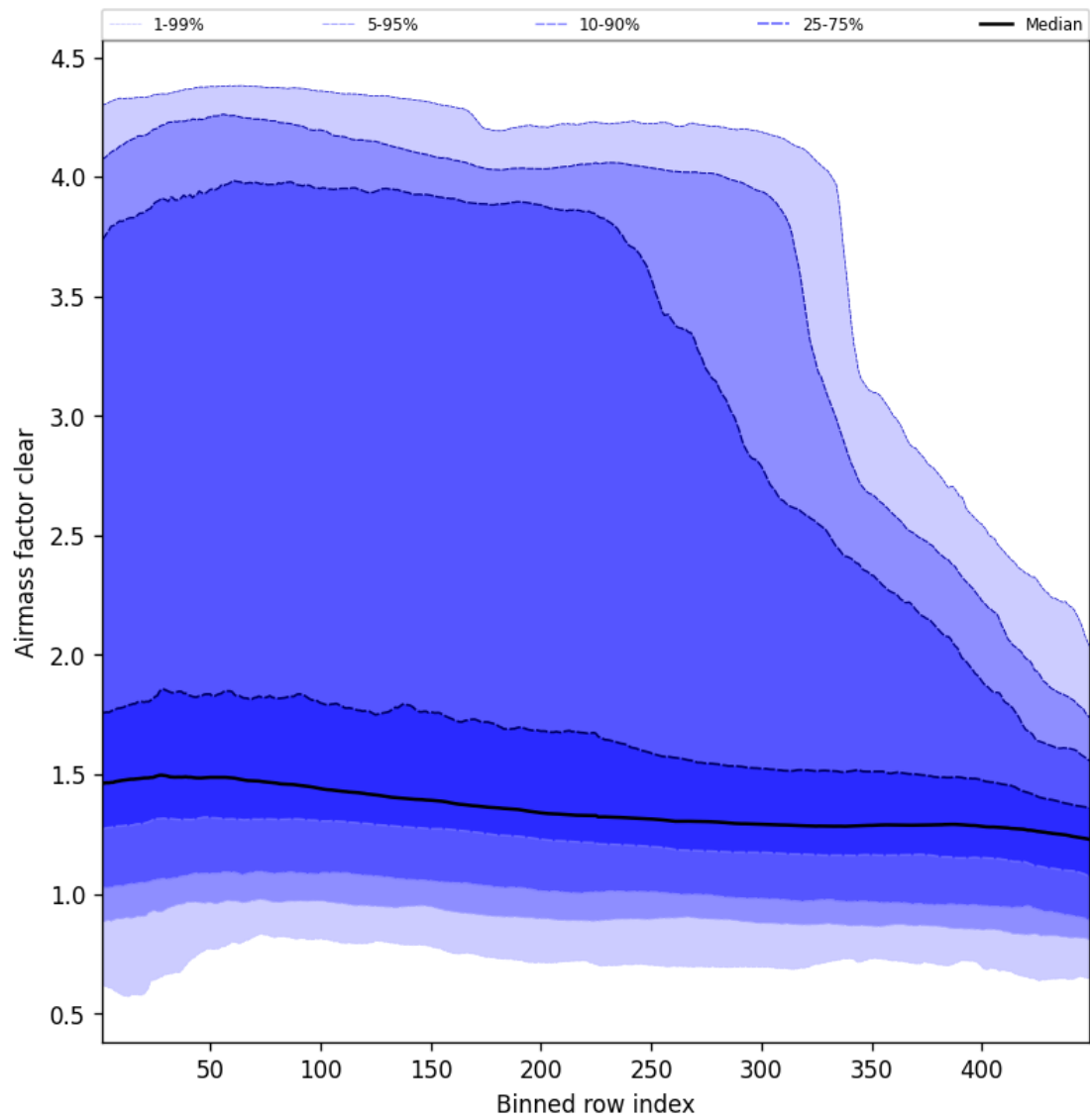
Figure 54: Along track statistics of “Airmass factor clear” for 2024-12-10 to 2024-12-11
