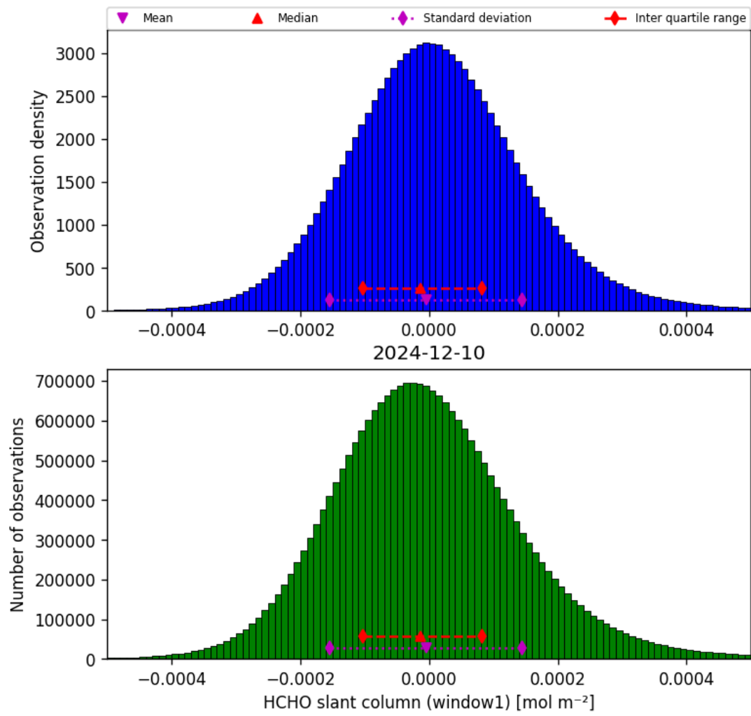
Figure 36: Histogram of “HCHO slant column (window1)” for 2024-12-10 to 2024-12-11
