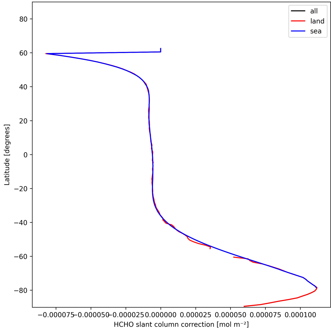
Figure 31: Zonal average of "HCHO slant column correction" for 2024-12-10 to 2024-12-11.
