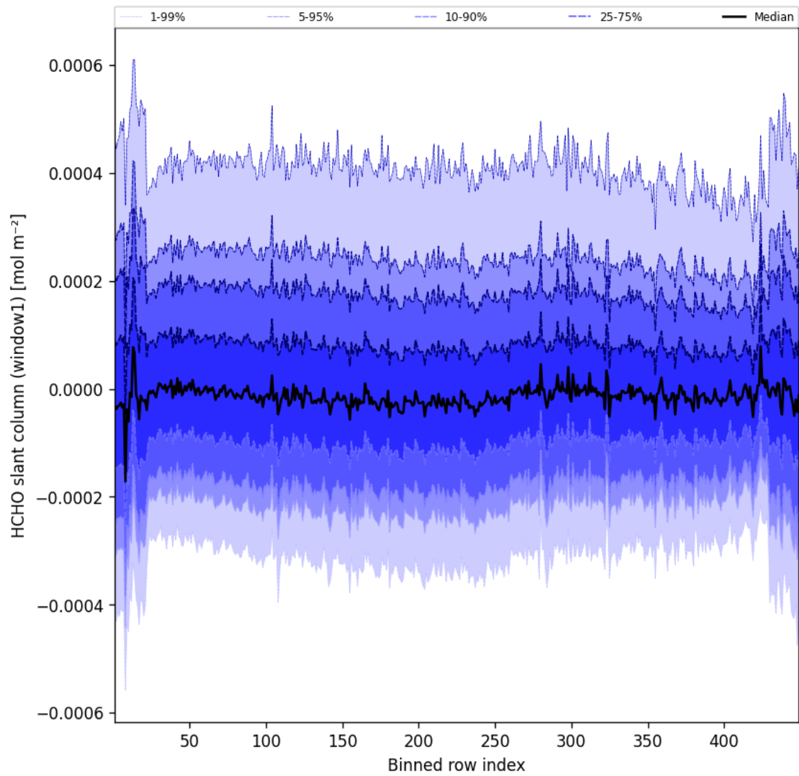
Figure 50: Along track statistics of “HCHO slant column (window1)” for 2024-12-10 to 2024-12-11
