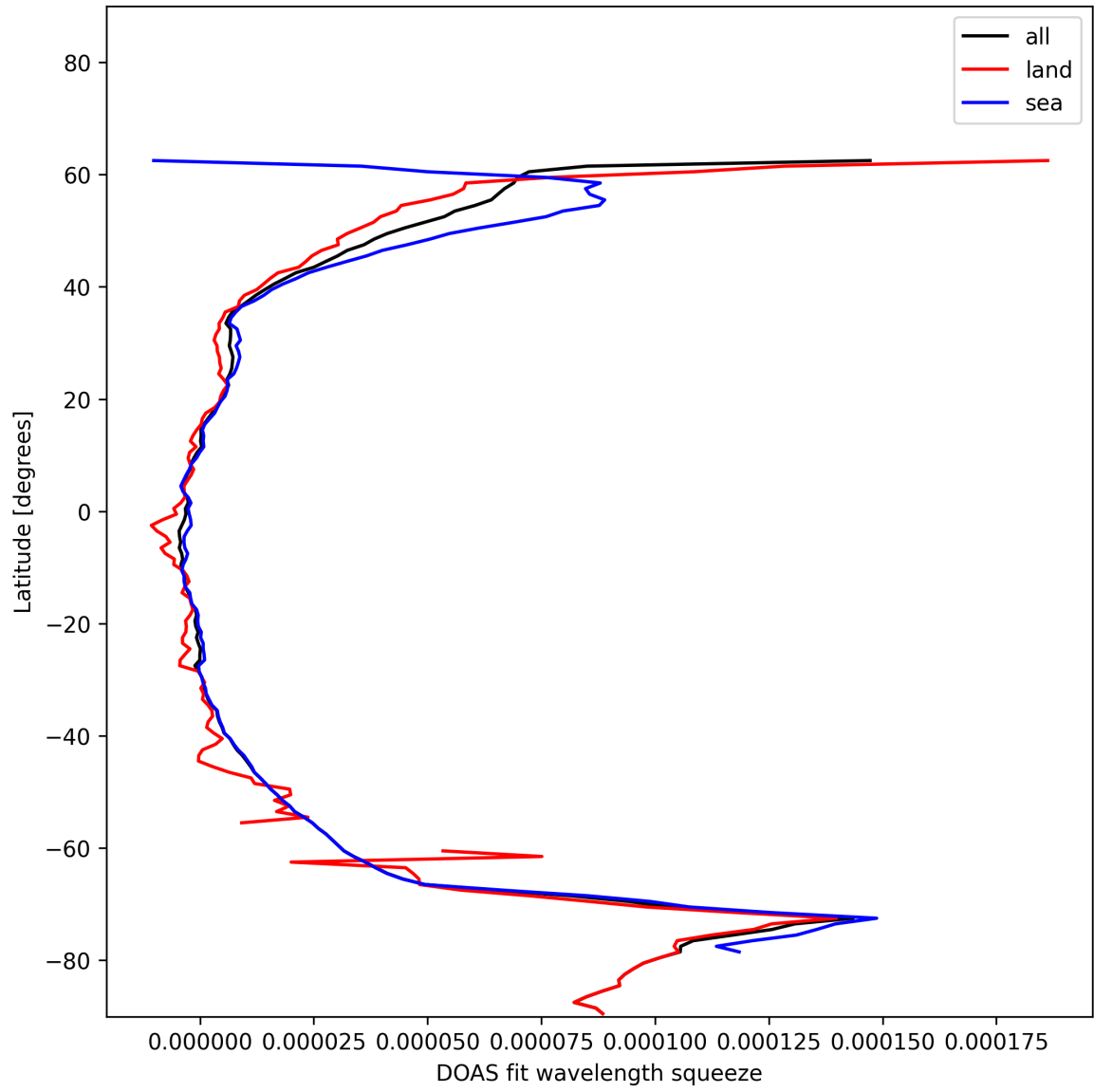
Figure 29: Zonal average of “DOAS fit wavelength squeeze” for 2024-12-10 to 2024-12-11.
