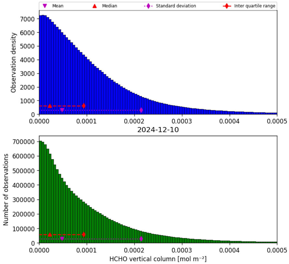
Figure 33: Histogram of “HCHO vertical column” for 2024-12-10 to 2024-12-11
