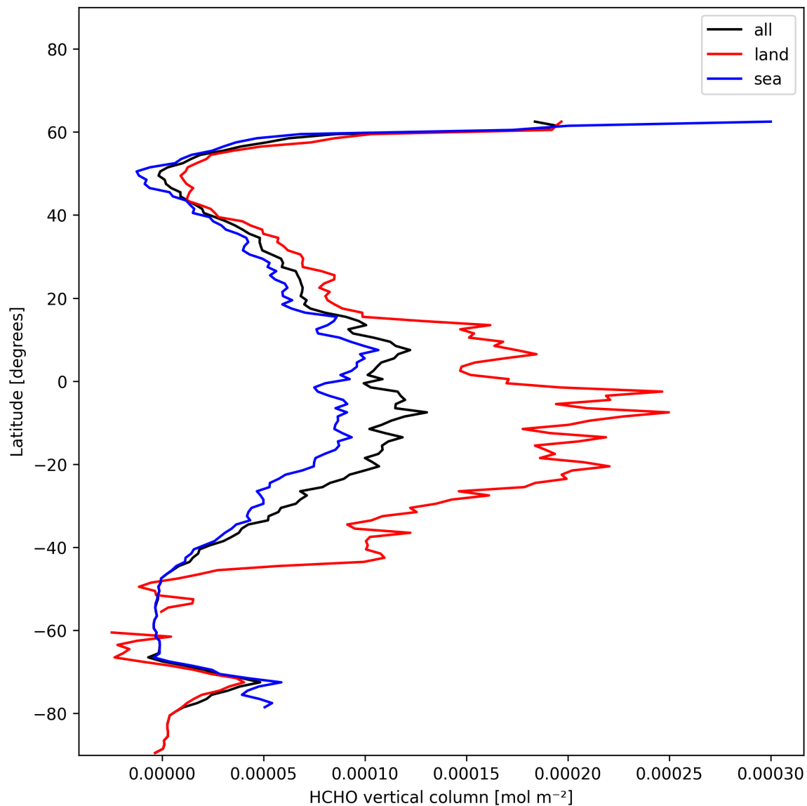
Figure 19: Zonal average of “HCHO vertical column” for 2024-12-10 to 2024-12-11.
