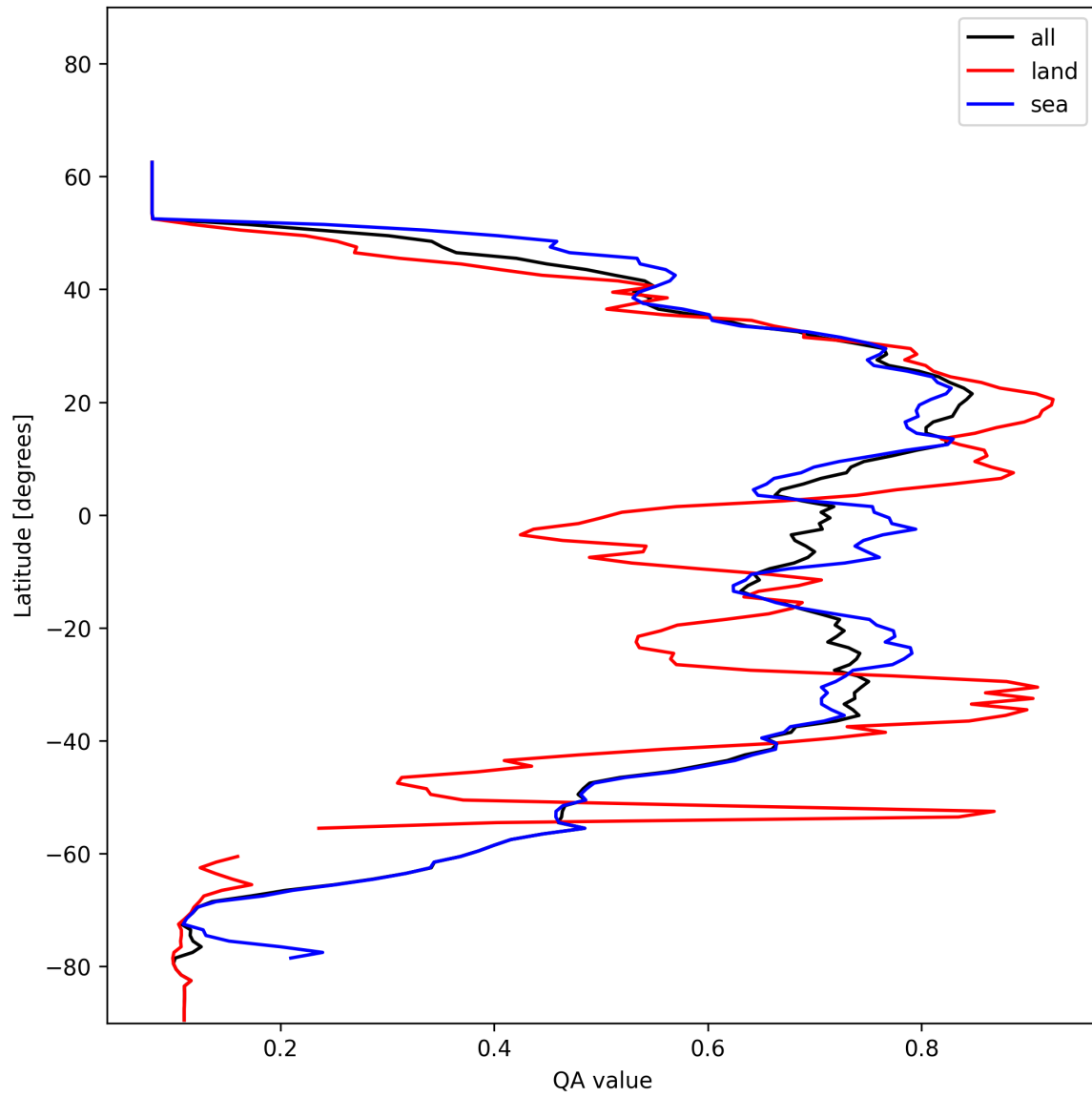
Figure 18: Zonal average of “QA value” for 2024-12-10 to 2024-12-11.
