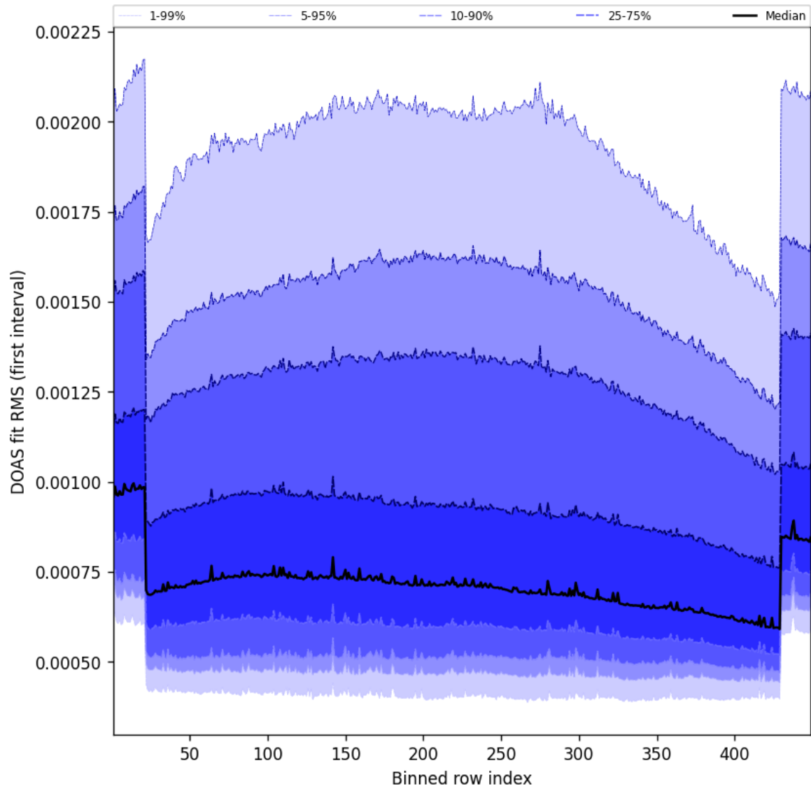
Figure 58: Along track statistics of “DOAS fit RMS (first interval)” for 2024-12-10 to 2024-12-11
