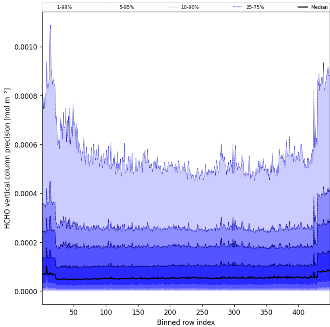
Figure 48: Along track statistics of “HCHO vertical column precision” for 2024-12-10 to 2024-12-11
