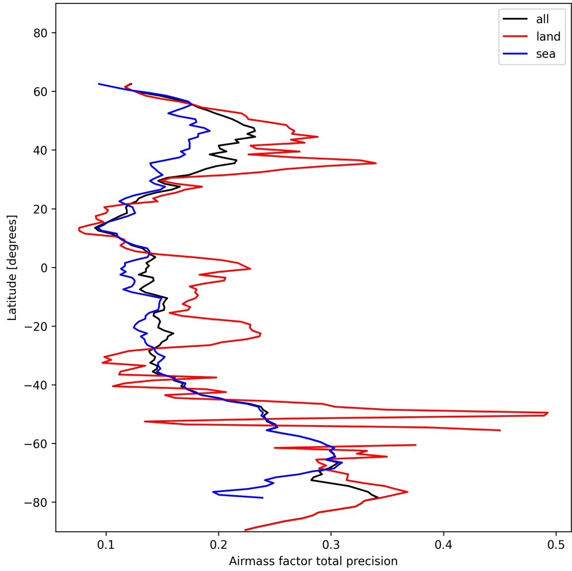
Figure 25: Zonal average of “Airmass factor total precision” for 2024-12-10 to 2024-12-11.
