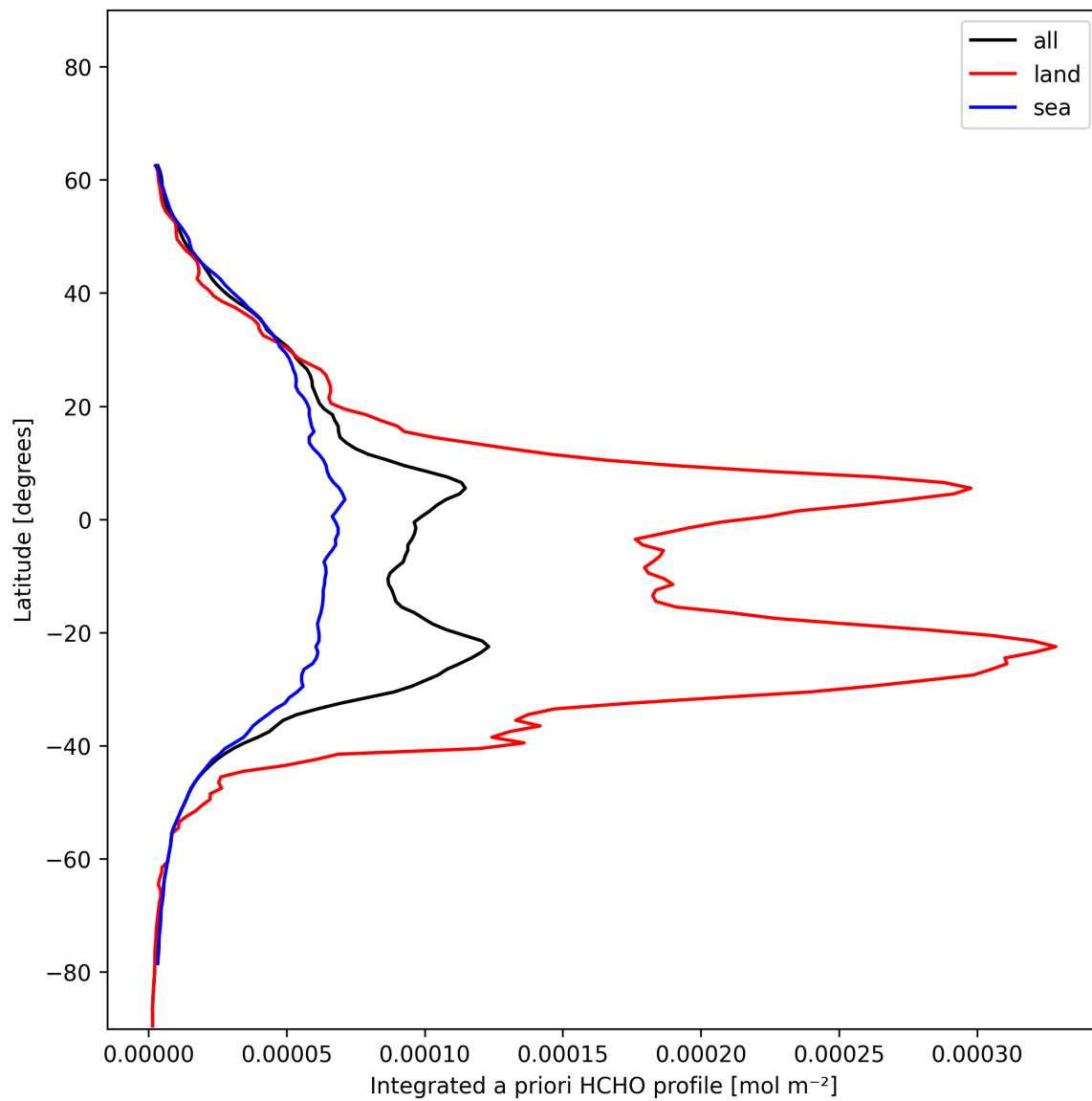
Figure 27: Zonal average of “Integrated a priori HCHO profile” for 2024-12-10 to 2024-12-11.
