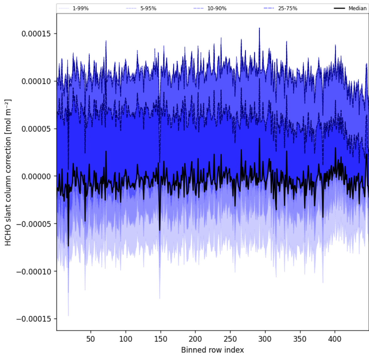
Figure 59: Along track statistics of “HCHO slant column correction” for 2024-12-10 to 2024-12-11
