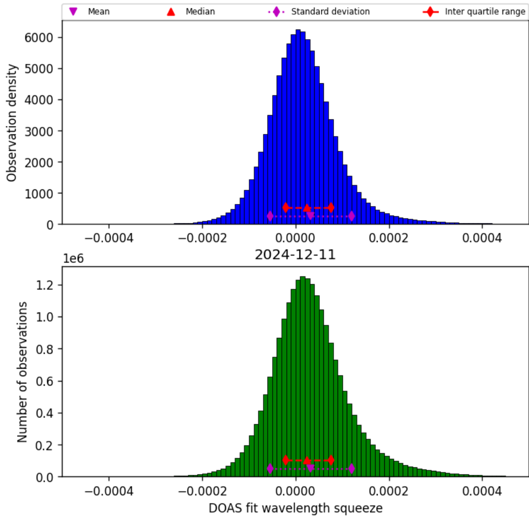
Figure 43: Histogram of “DOAS fit wavelength squeeze” for 2024-12-11 to 2024-12-12
