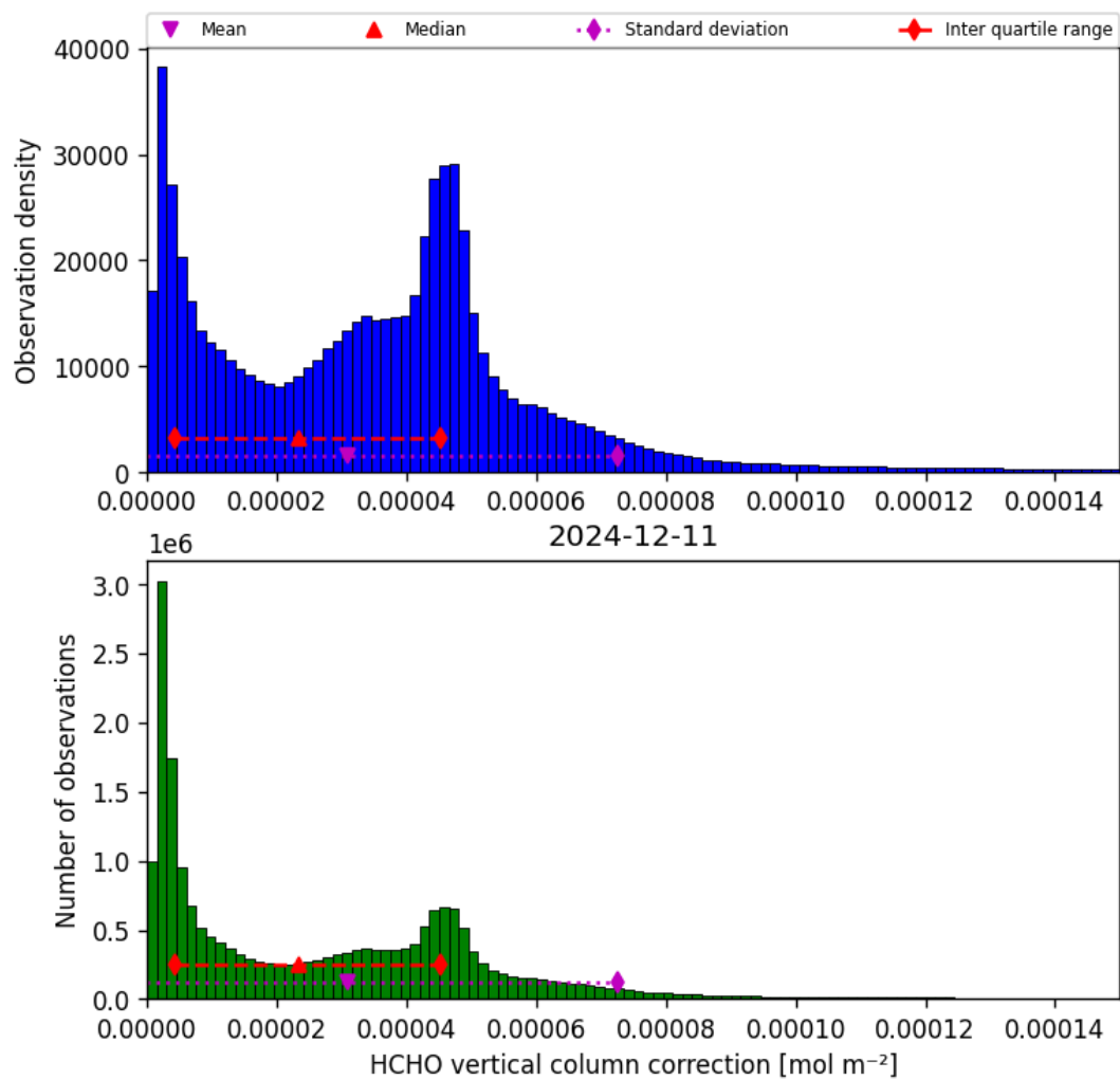
Figure 35: Histogram of “HCHO vertical column correction” for 2024-12-11 to 2024-12-12
