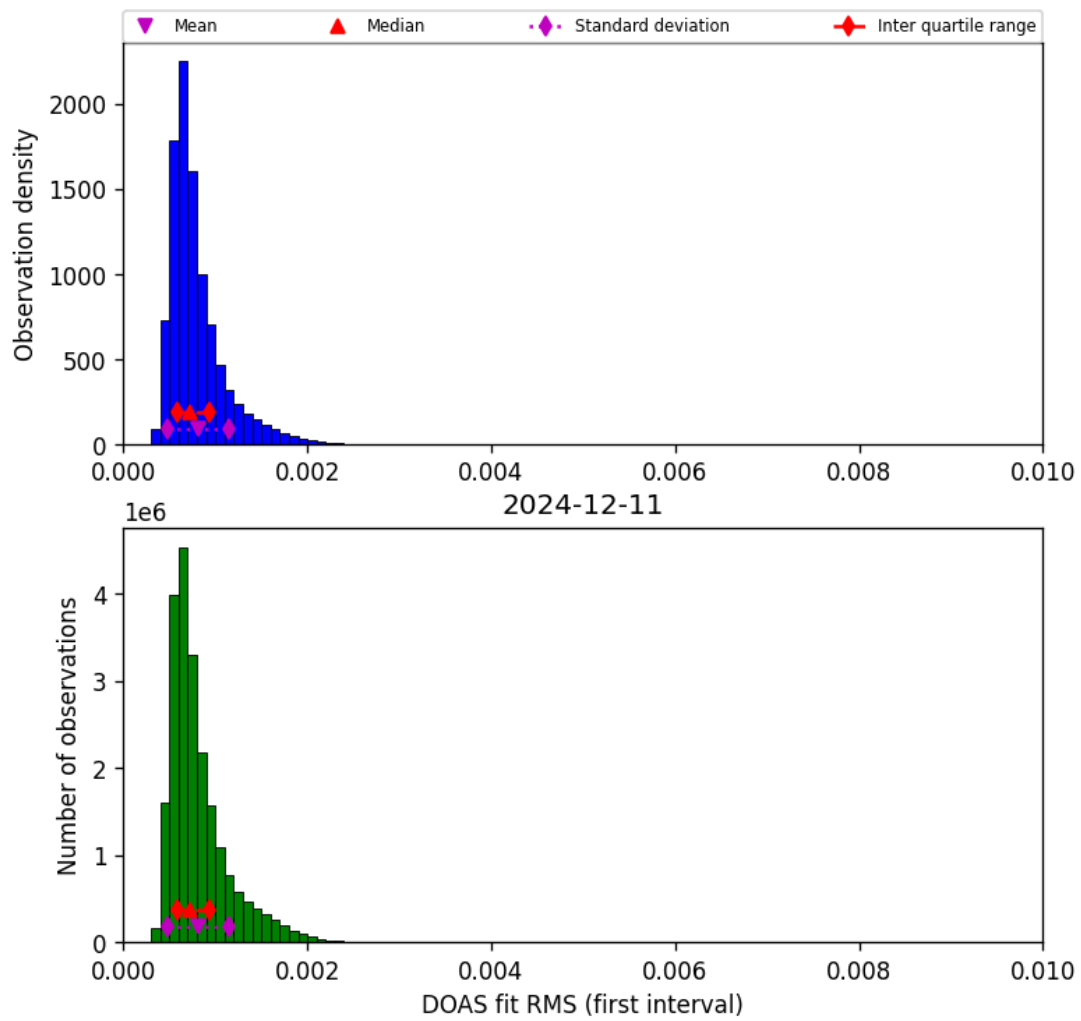
Figure 44: Histogram of “DOAS fit RMS (first interval)” for 2024-12-11 to 2024-12-12
