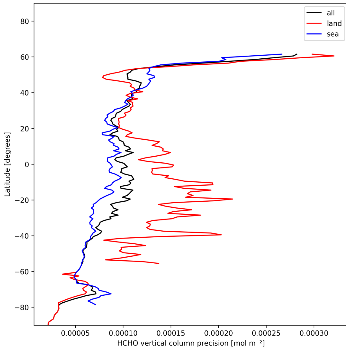
Figure 20: Zonal average of “HCHO vertical column precision” for 2024-12-11 to 2024-12-12.
