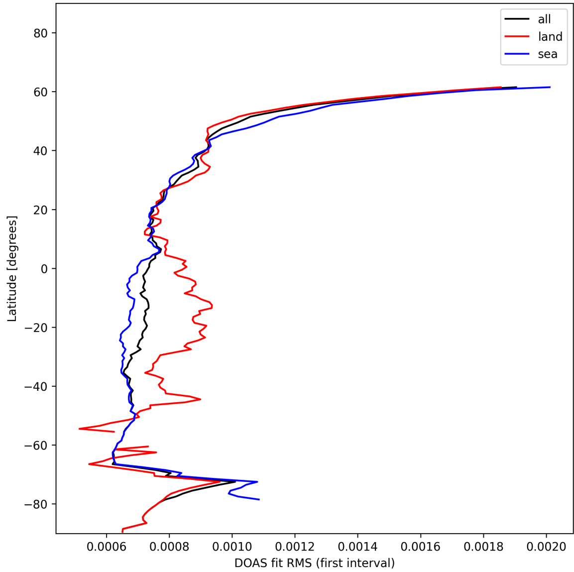
Figure 30: Zonal average of “DOAS fit RMS (first interval)” for 2024-12-11 to 2024-12-12.
