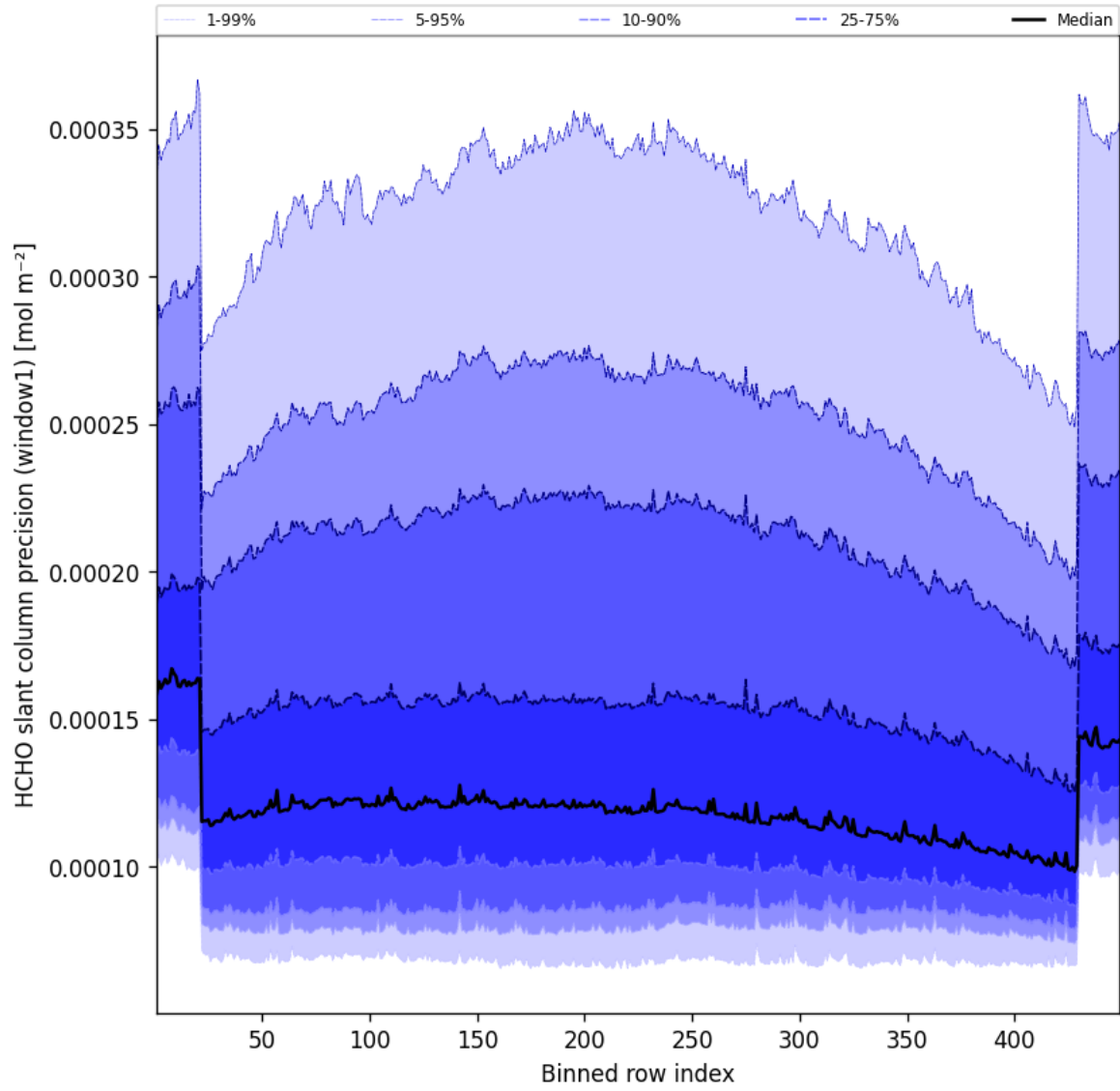
Figure 51: Along track statistics of “HCHO slant column precision (window1)” for 2024-12-11 to 2024-12-12
