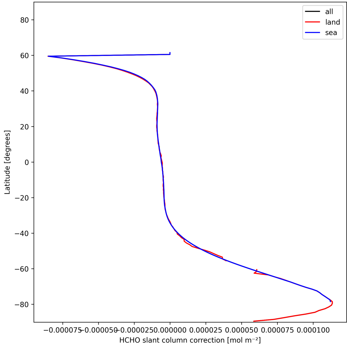
Figure 31: Zonal average of “HCHO slant column correction” for 2024-12-11 to 2024-12-12.
