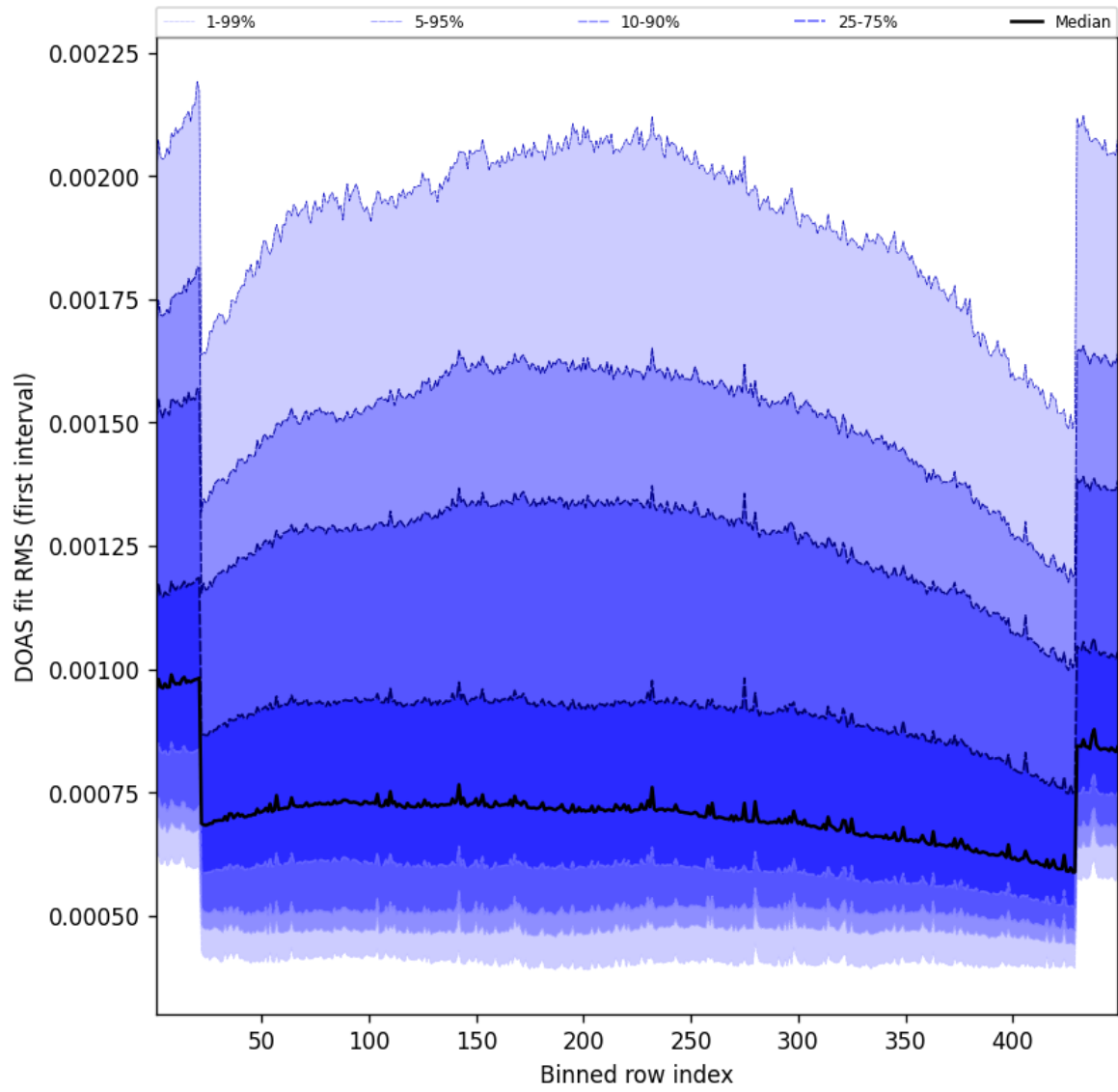
Figure 58: Along track statistics of “DOAS fit RMS (first interval)” for 2024-12-11 to 2024-12-12
