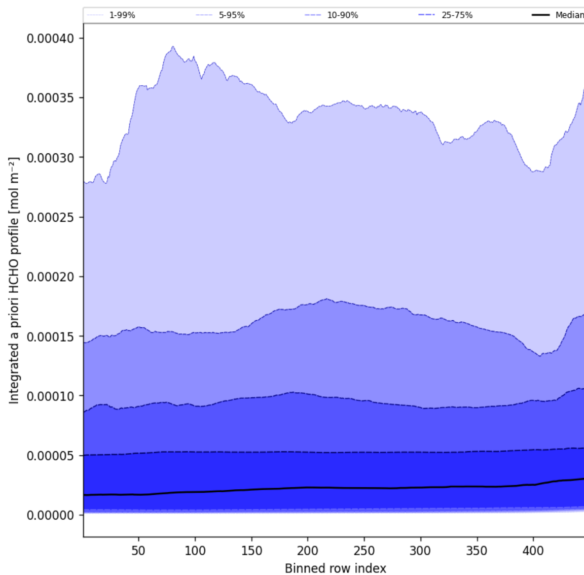
Figure 55: Along track statistics of "Integrated a priori HCHO profile" for 2024-12-11 to 2024-12-12
