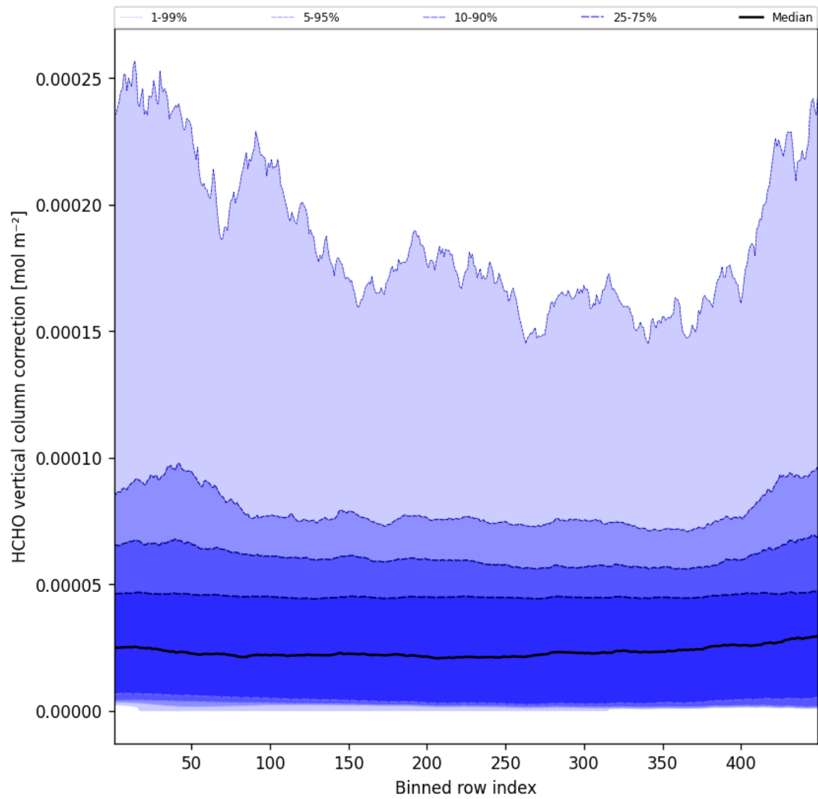
Figure 49: Along track statistics of “HCHO vertical column correction” for 2024-12-11 to 2024-12-12
