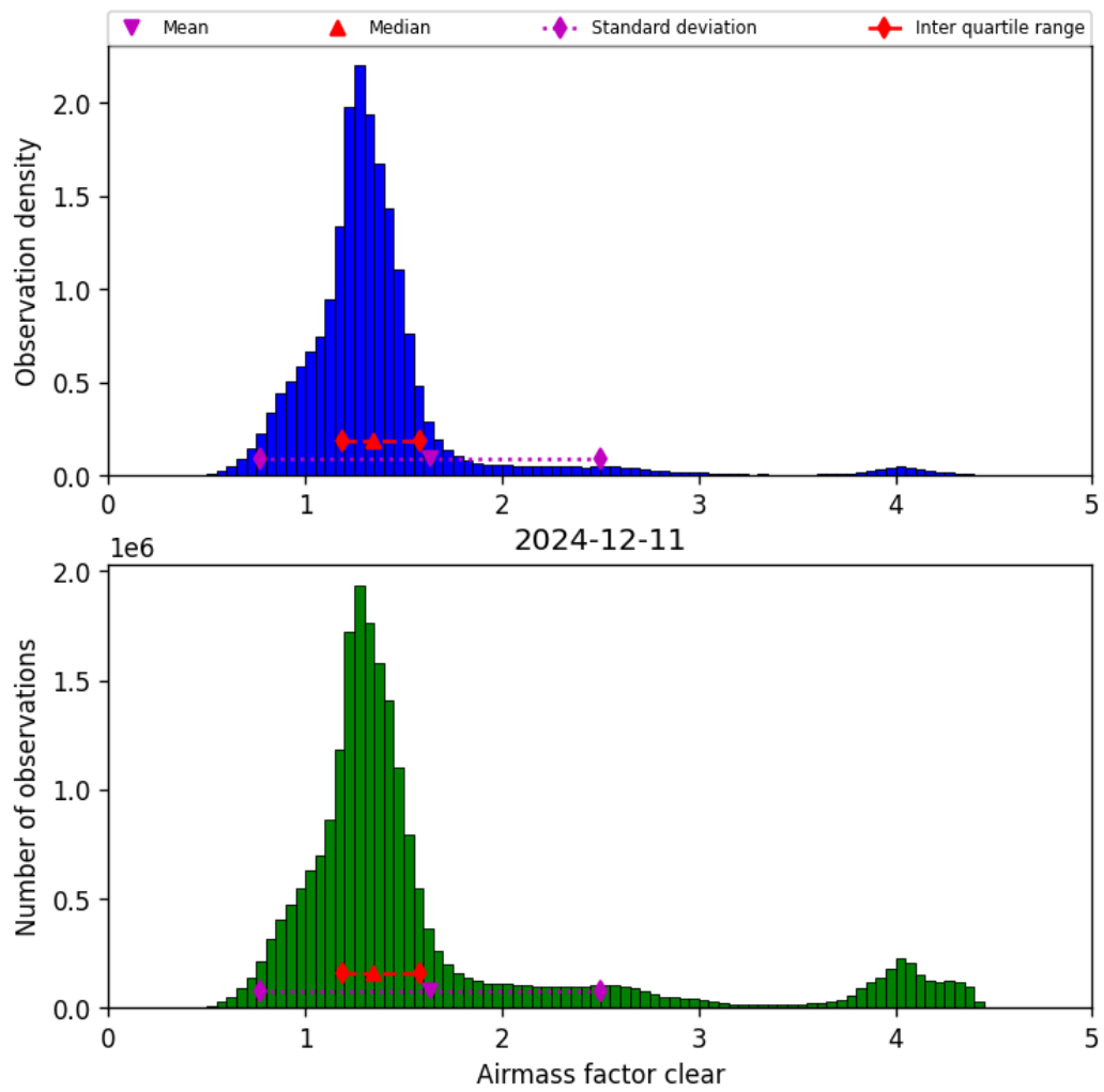
Figure 40: Histogram of “Airmass factor clear” for 2024-12-11 to 2024-12-12
