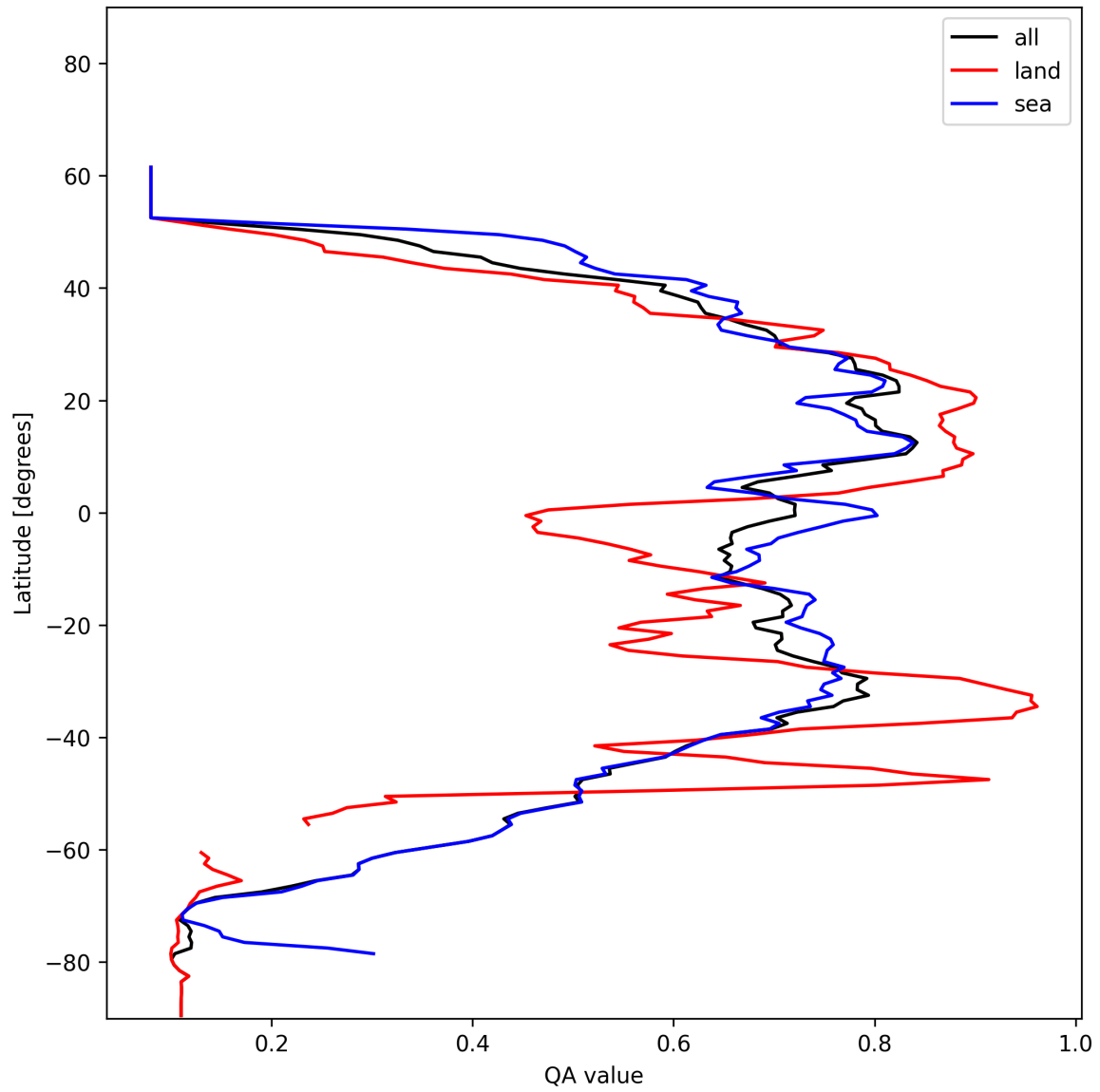
Figure 18: Zonal average of “QA value” for 2024-12-11 to 2024-12-12.
