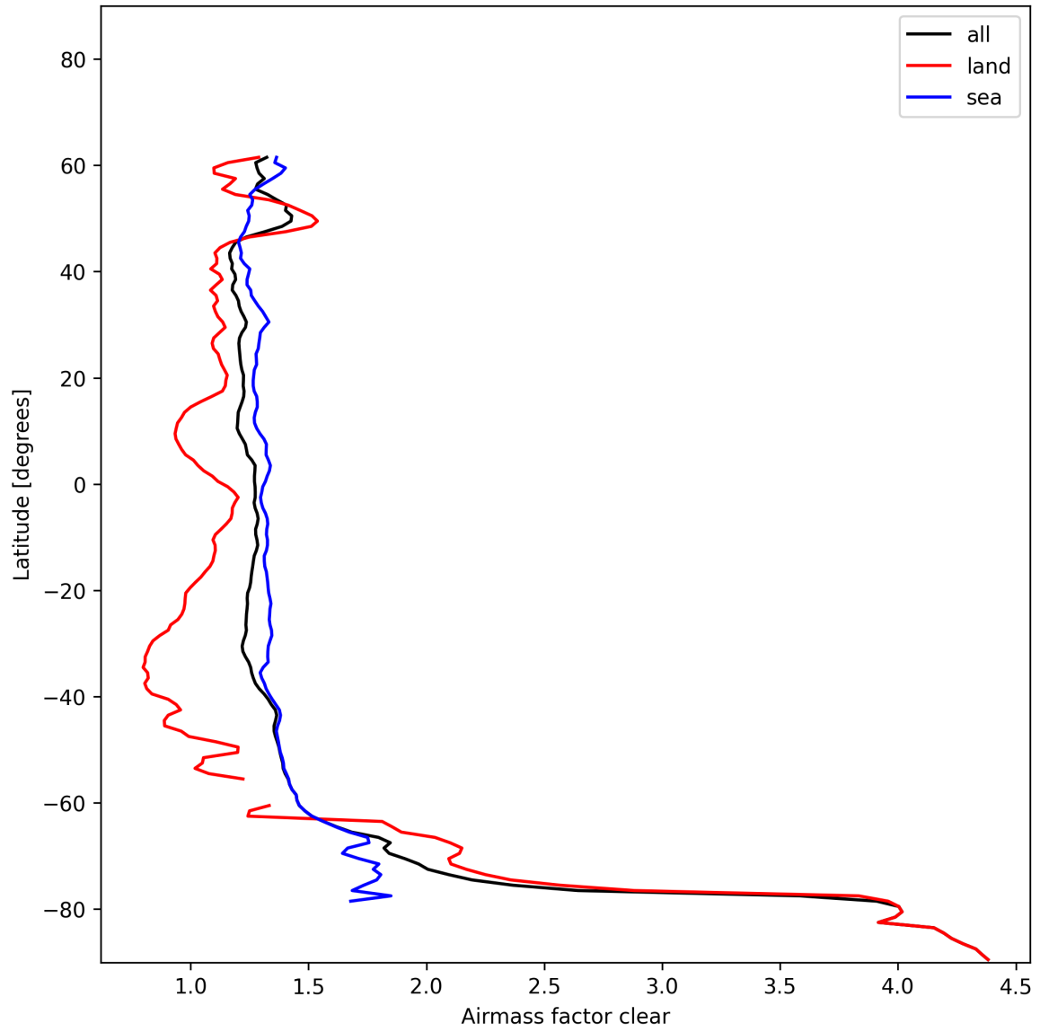
Figure 26: Zonal average of “Airmass factor clear” for 2024-12-11 to 2024-12-12.
