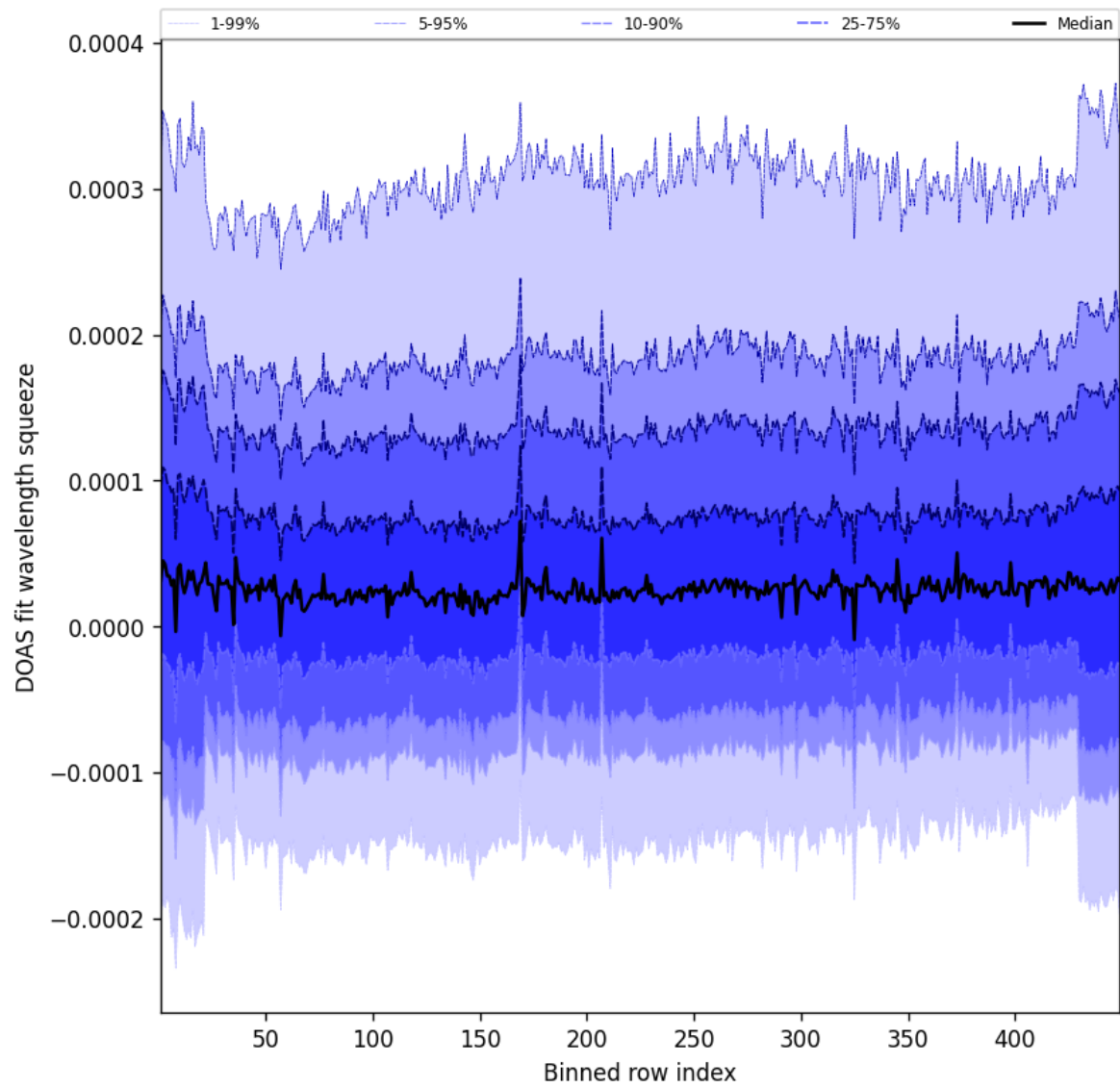
Figure 57: Along track statistics of “DOAS fit wavelength squeeze” for 2024-12-11 to 2024-12-12
