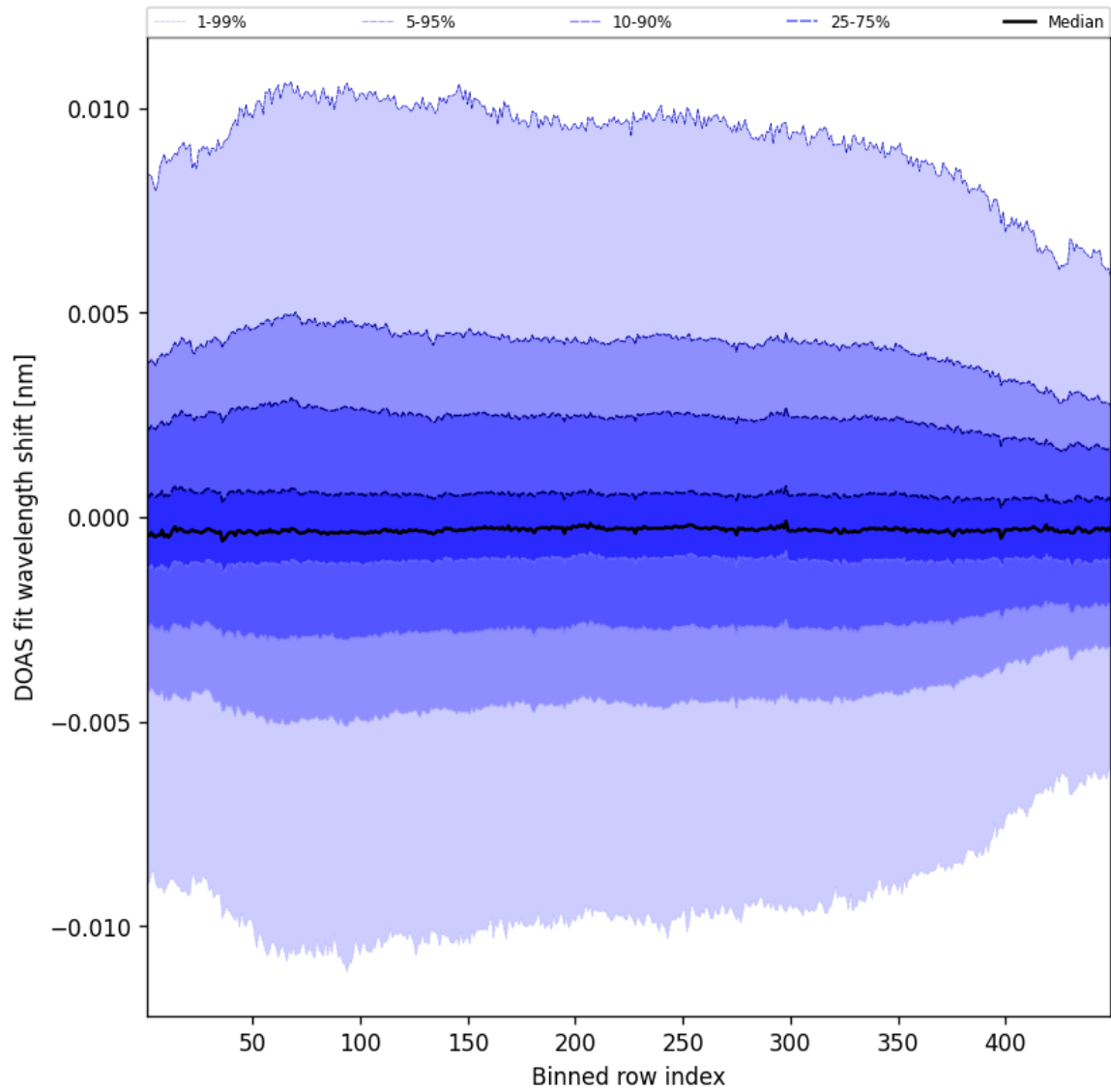
Figure 56: Along track statistics of “DOAS fit wavelength shift” for 2024-12-11 to 2024-12-12
