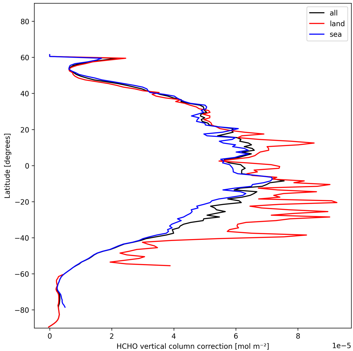
Figure 21: Zonal average of “HCHO vertical column correction” for 2024-12-11 to 2024-12-12.
