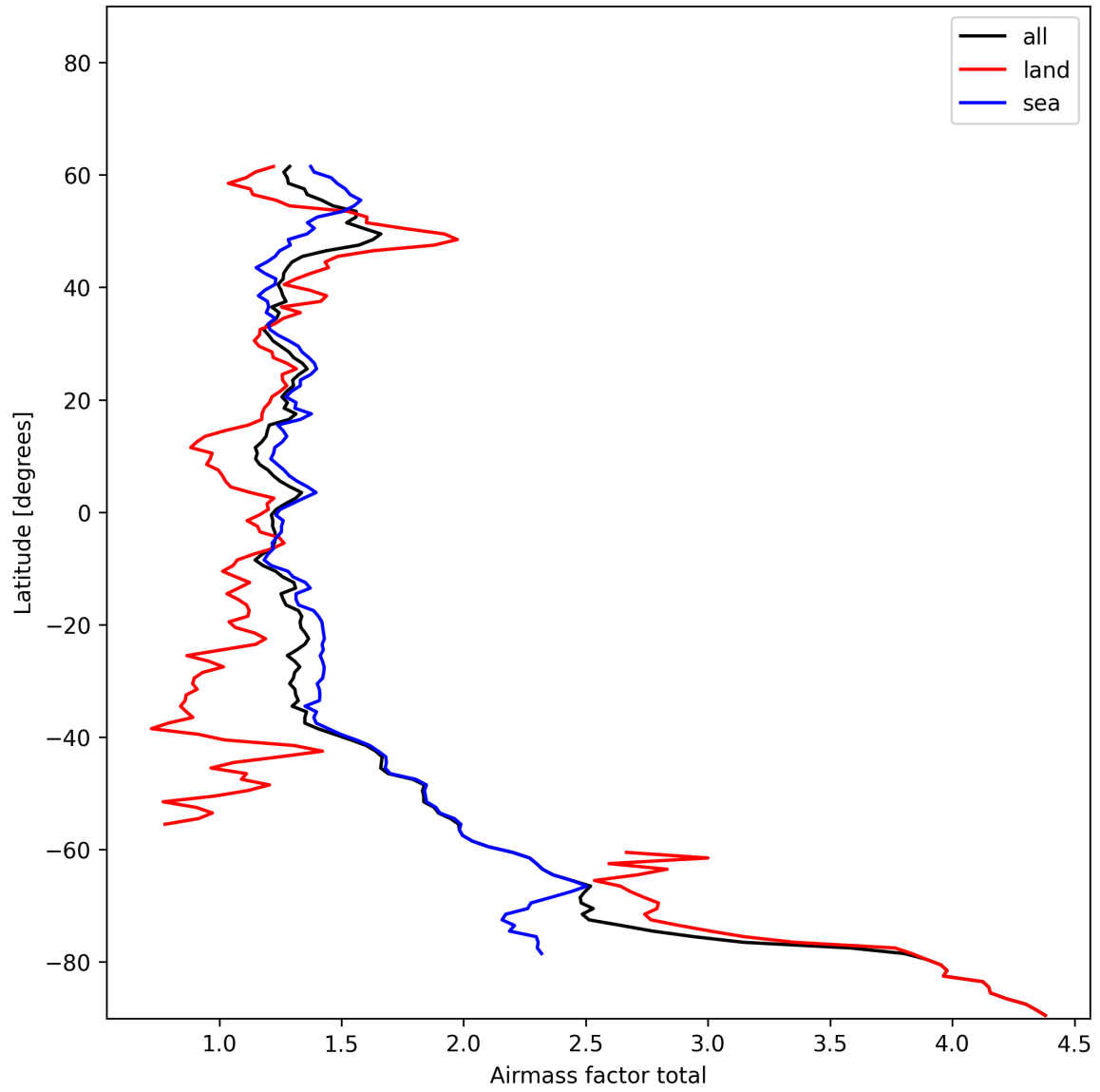
Figure 24: Zonal average of “Airmass factor total” for 2024-12-11 to 2024-12-12.
