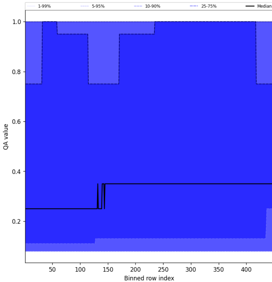
Figure 46: Along track statistics of “QA value” for 2024-12-11 to 2024-12-12
