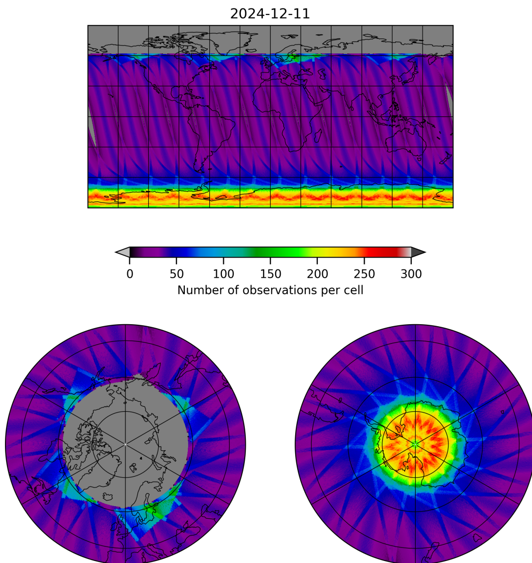
Figure 17: Map of the number of observations for 2024-12-11 to 2024-12-12
