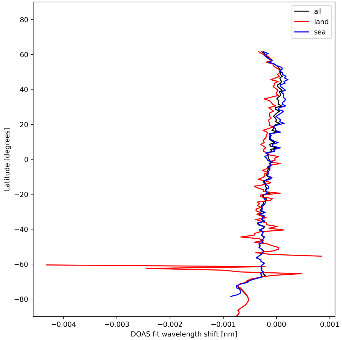
Figure 28: Zonal average of “DOAS fit wavelength shift” for 2024-12-11 to 2024-12-12.
