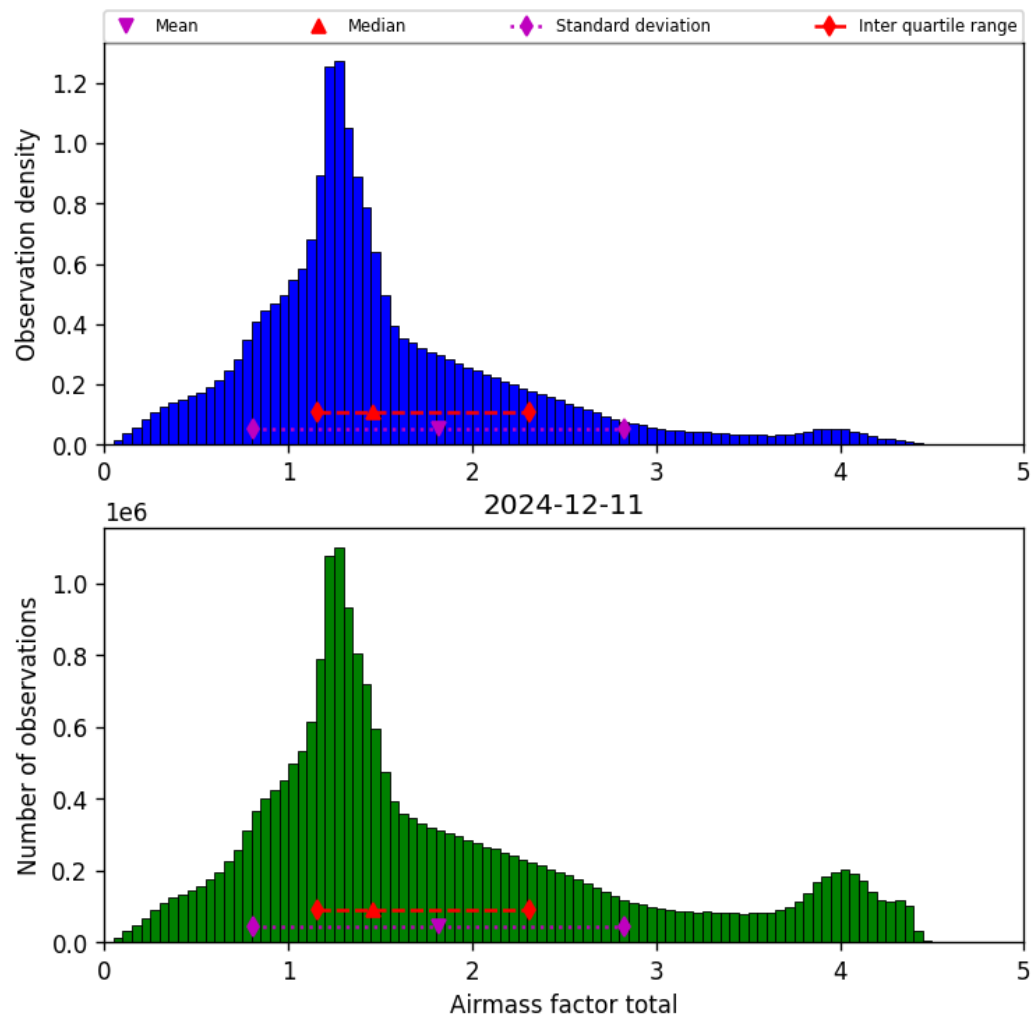
Figure 38: Histogram of “Airmass factor total” for 2024-12-11 to 2024-12-12
