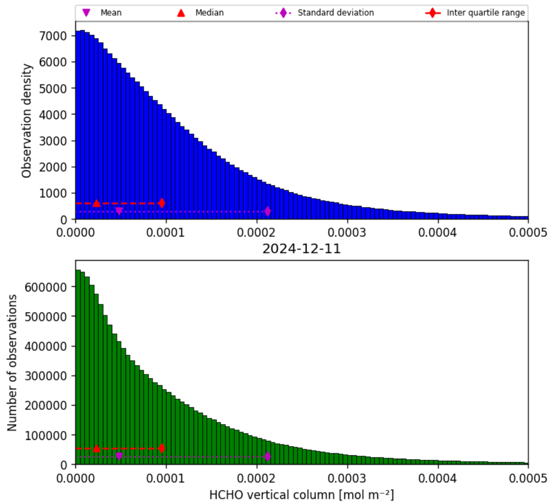
Figure 33: Histogram of “HCHO vertical column” for 2024-12-11 to 2024-12-12
