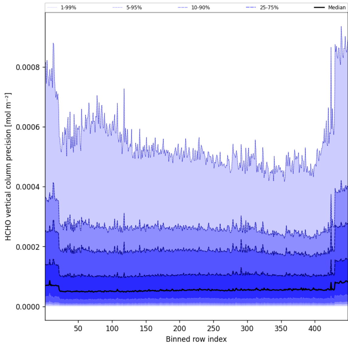
Figure 48: Along track statistics of “HCHO vertical column precision” for 2024-12-11 to 2024-12-12
