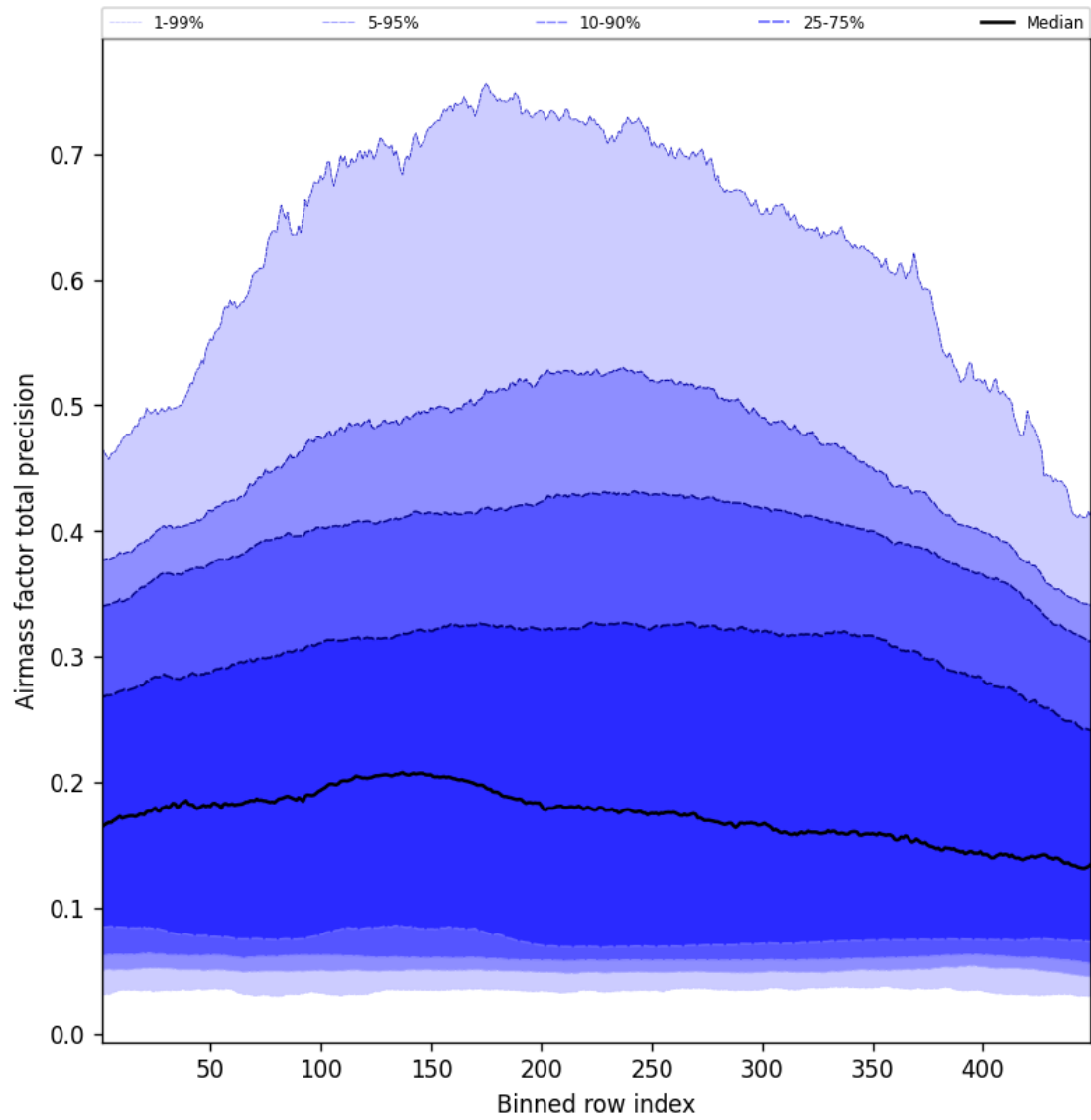
Figure 53: Along track statistics of “Airmass factor total precision” for 2024-12-11 to 2024-12-12
