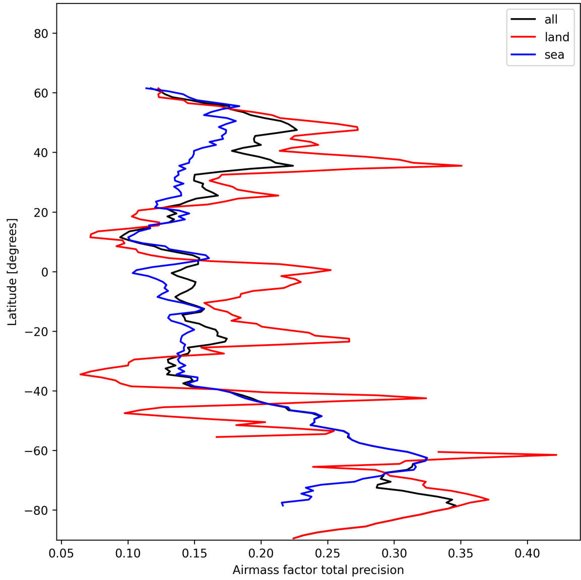
Figure 25: Zonal average of “Airmass factor total precision” for 2024-12-11 to 2024-12-12.
