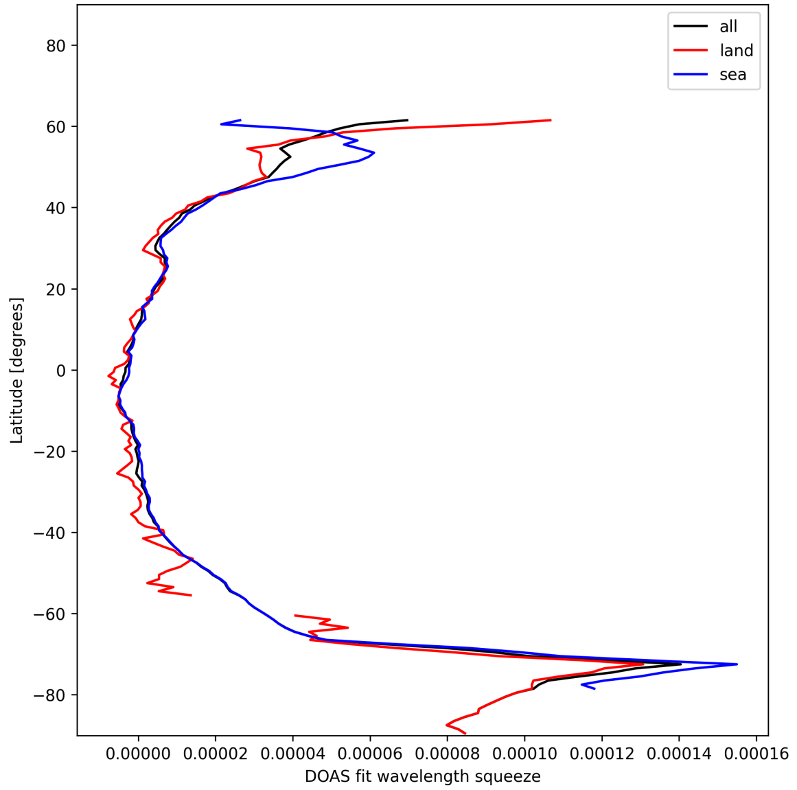
Figure 29: Zonal average of “DOAS fit wavelength squeeze” for 2024-12-11 to 2024-12-12.
