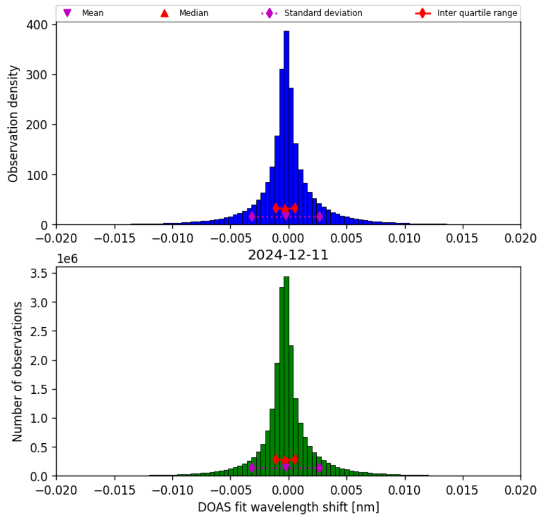
Figure 42: Histogram of “DOAS fit wavelength shift” for 2024-12-11 to 2024-12-12
