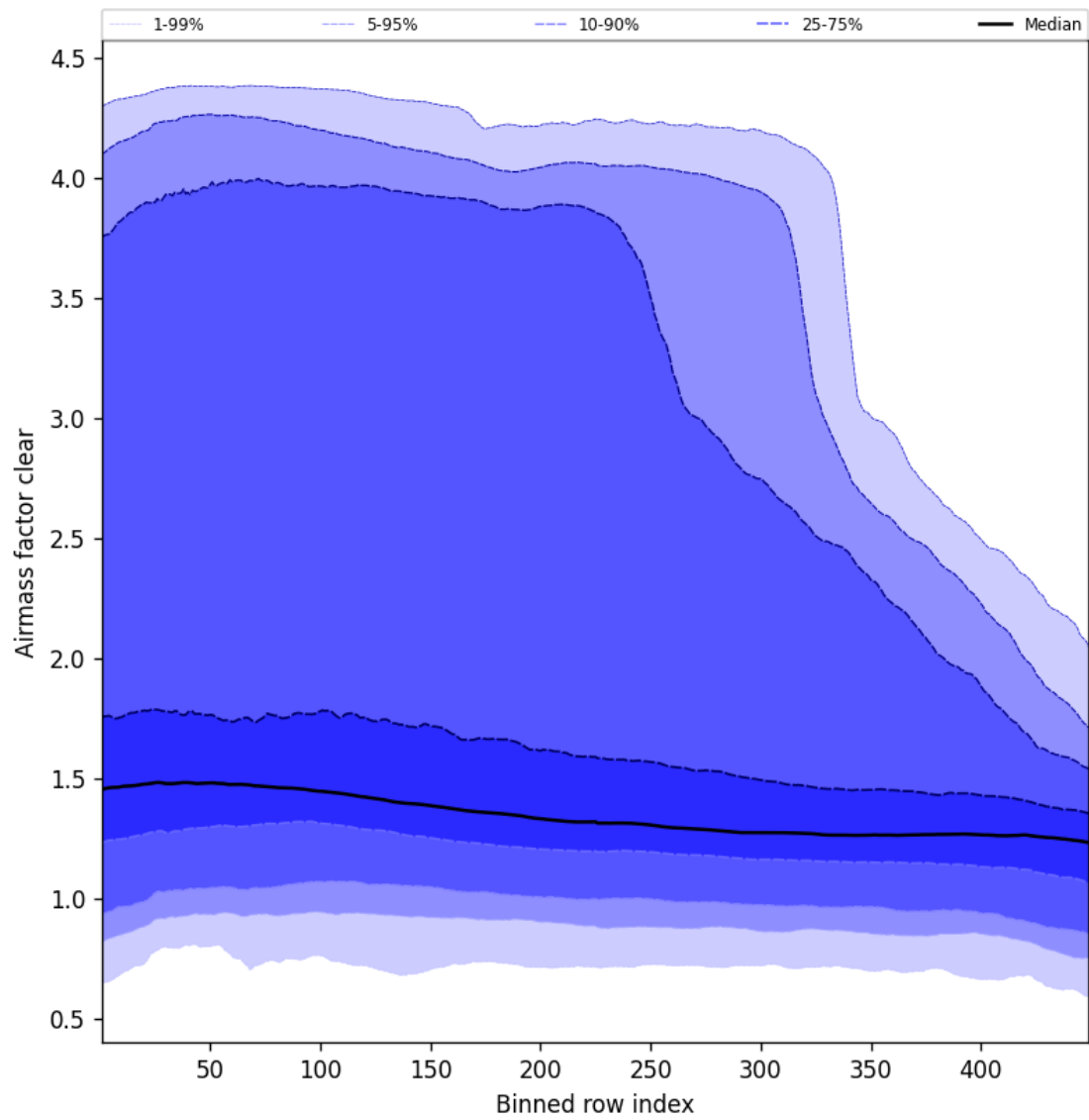
Figure 54: Along track statistics of “Air mass factor clear” for 2024-12-11 to 2024-12-12
