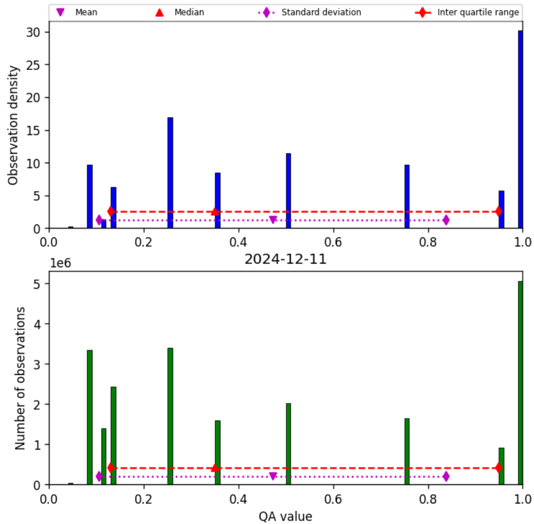
Figure 32: Histogram of “QA value” for 2024-12-11 to 2024-12-12
