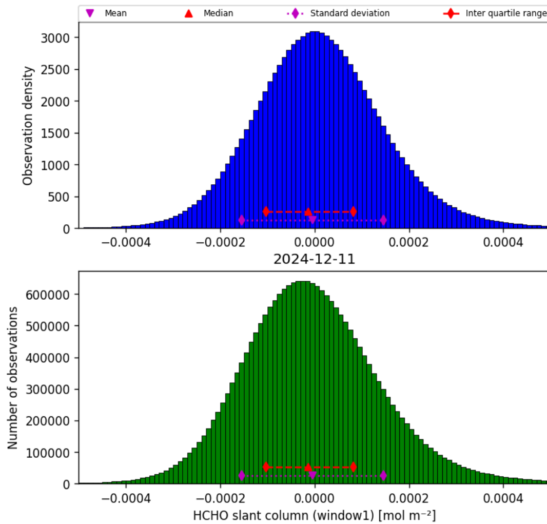
Figure 36: Histogram of “HCHO slant column (window1)” for 2024-12-11 to 2024-12-12
