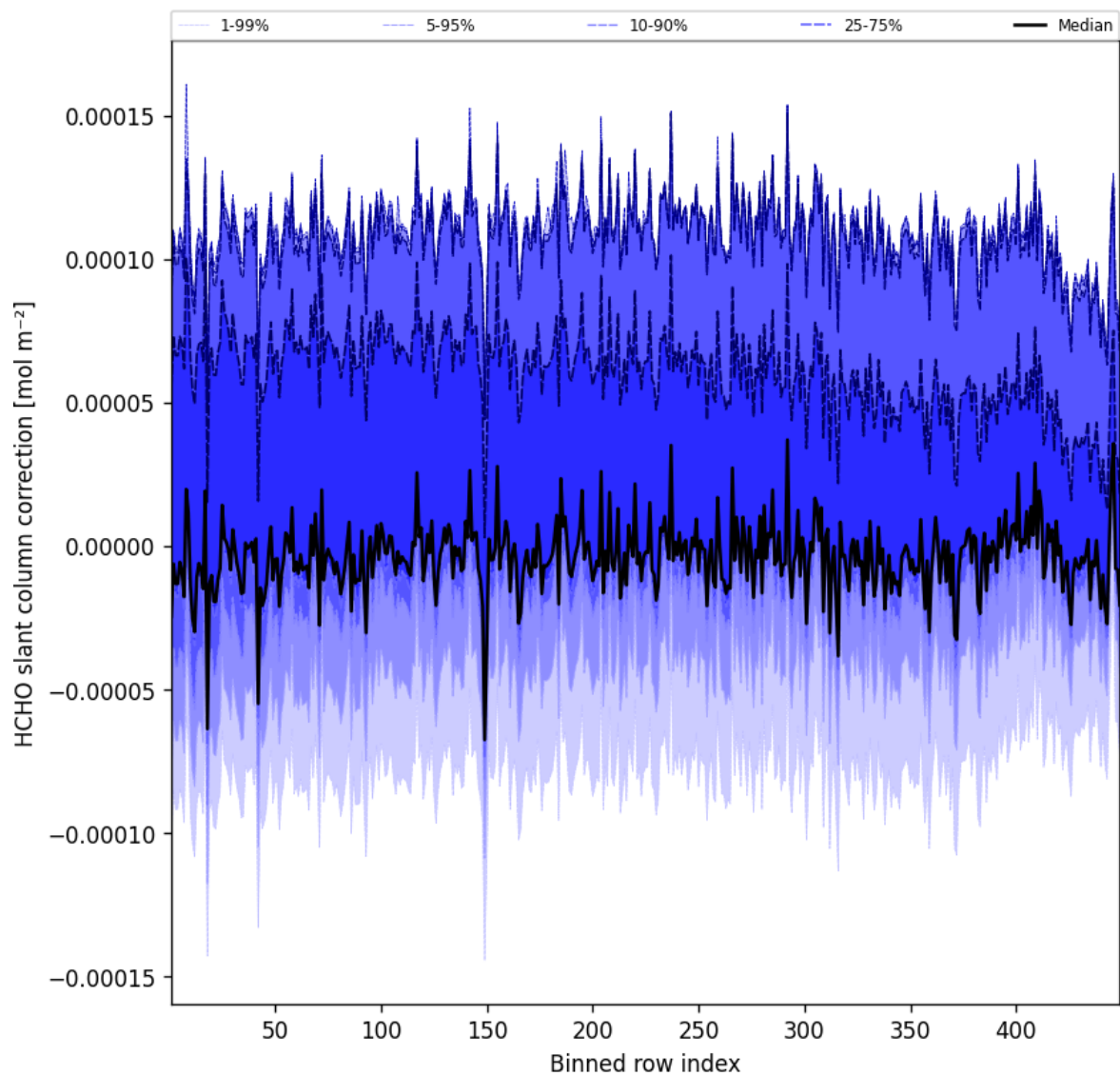
Figure 59: Along track statistics of “HCHO slant column correction” for 2024-12-11 to 2024-12-12
