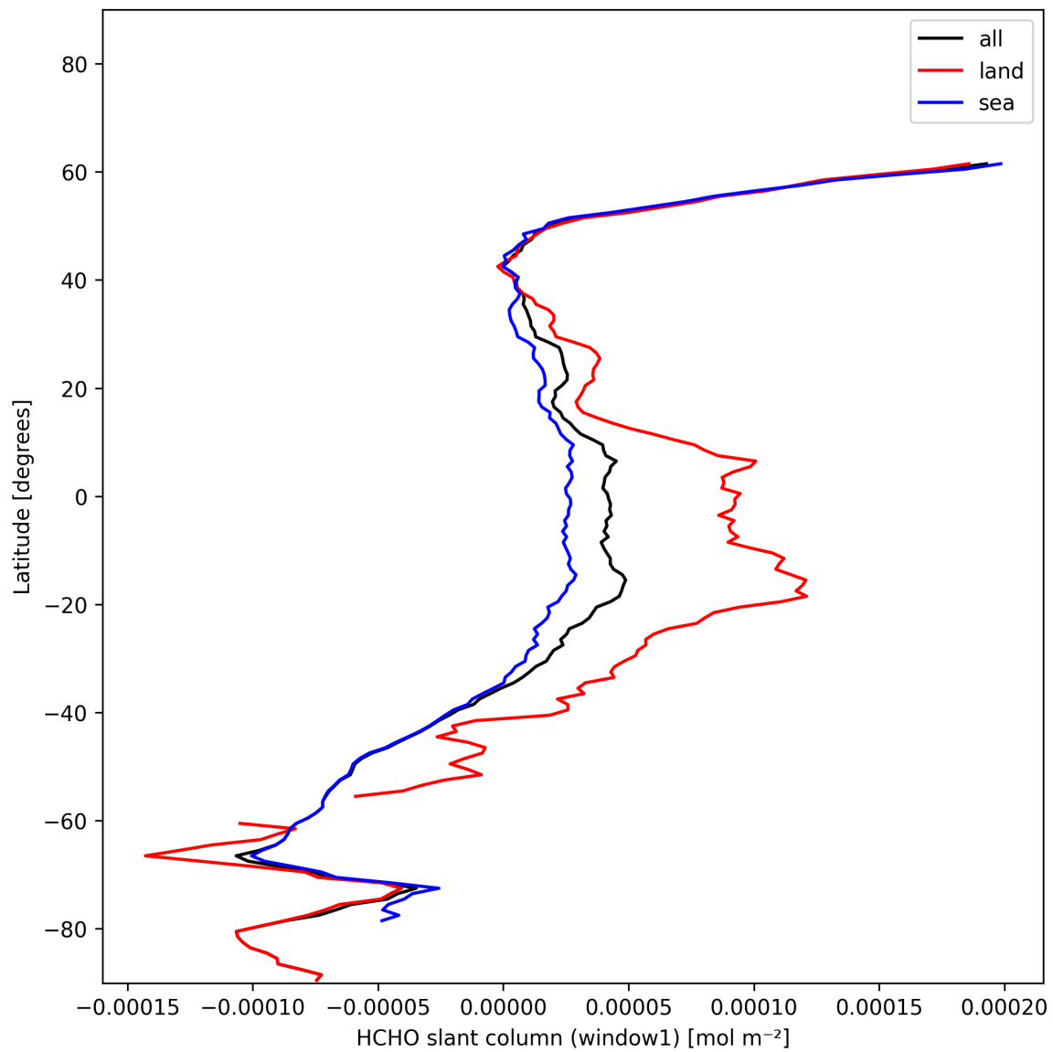
Figure 22: Zonal average of “HCHO slant column (window1)” for 2024-12-11 to 2024-12-12.
