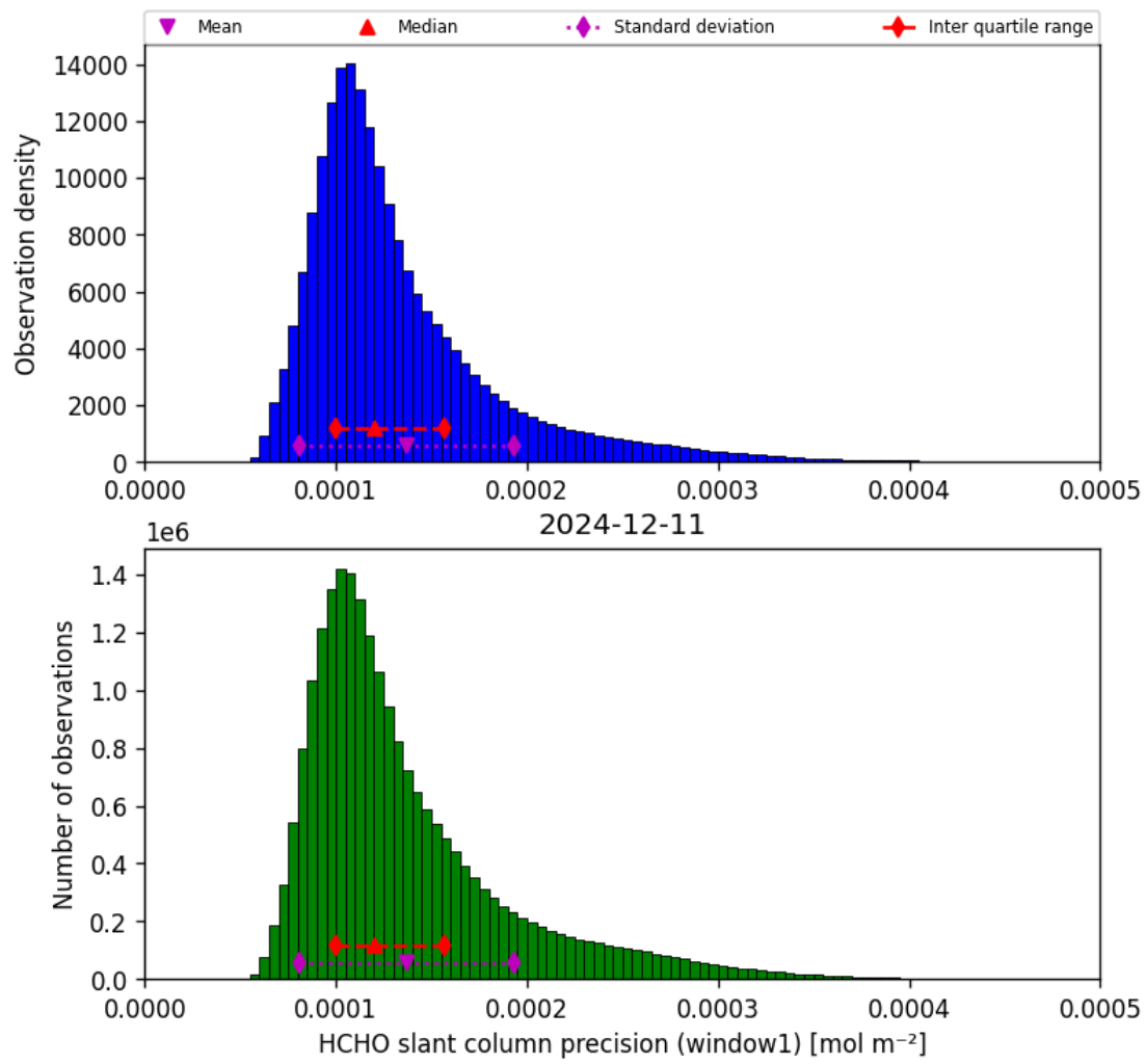
Figure 37: Histogram of “HCHO slant column precision (window1)” for 2024-12-11 to 2024-12-12
