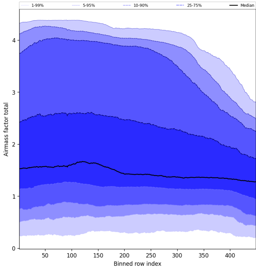
Figure 52: Along track statistics of “Airmass factor total” for 2024-12-11 to 2024-12-12
