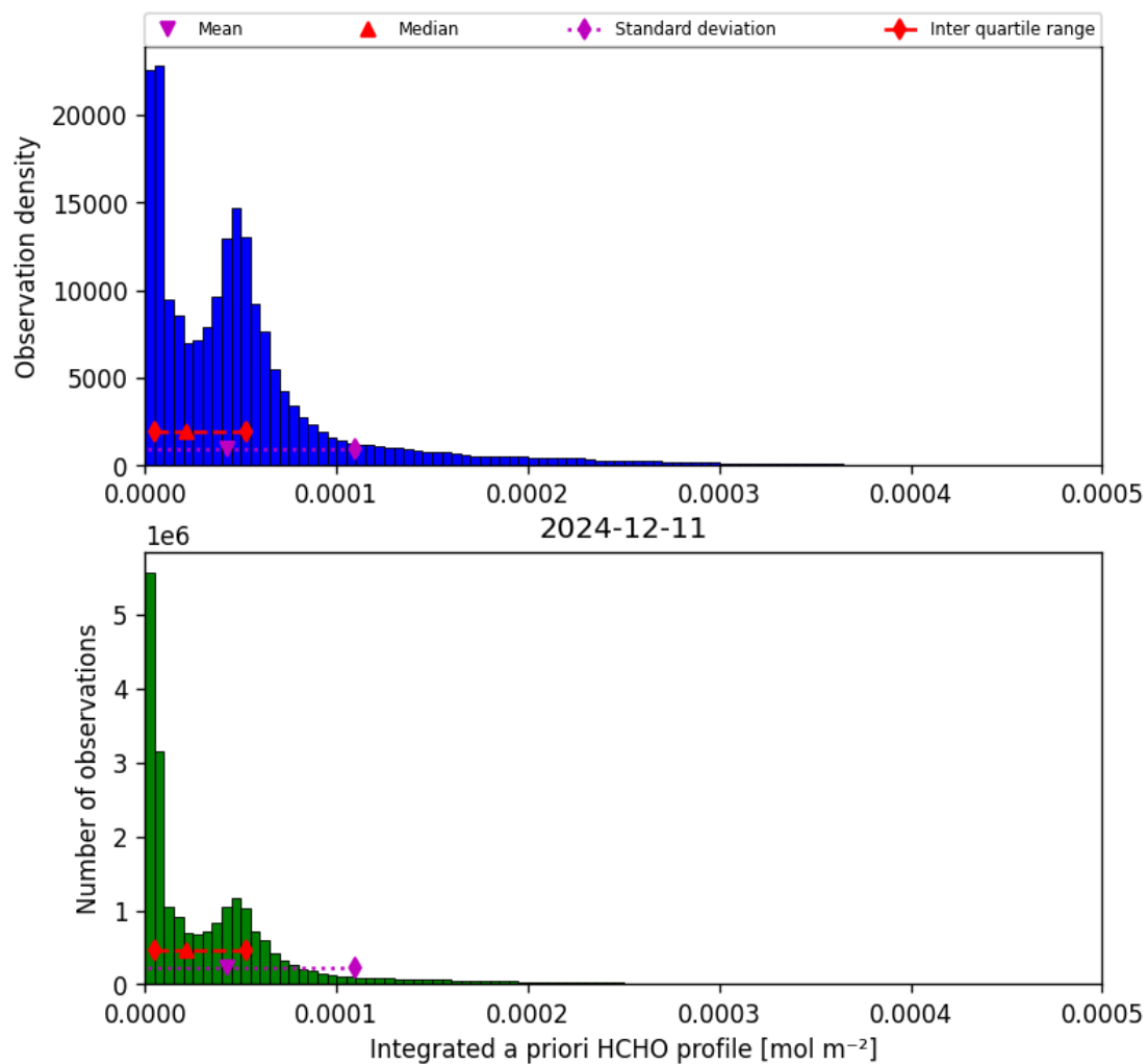
Figure 41: Histogram of “Integrated a priori HCHO profile” for 2024-12-11 to 2024-12-12
