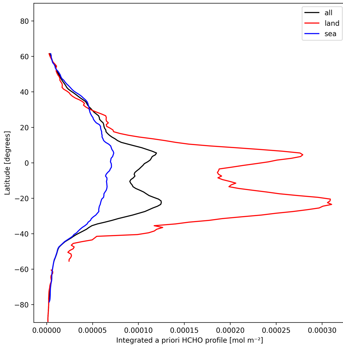
Figure 27: Zonal average of “Integrated a priori HCHO profile” for 2024-12-11 to 2024-12-12.
