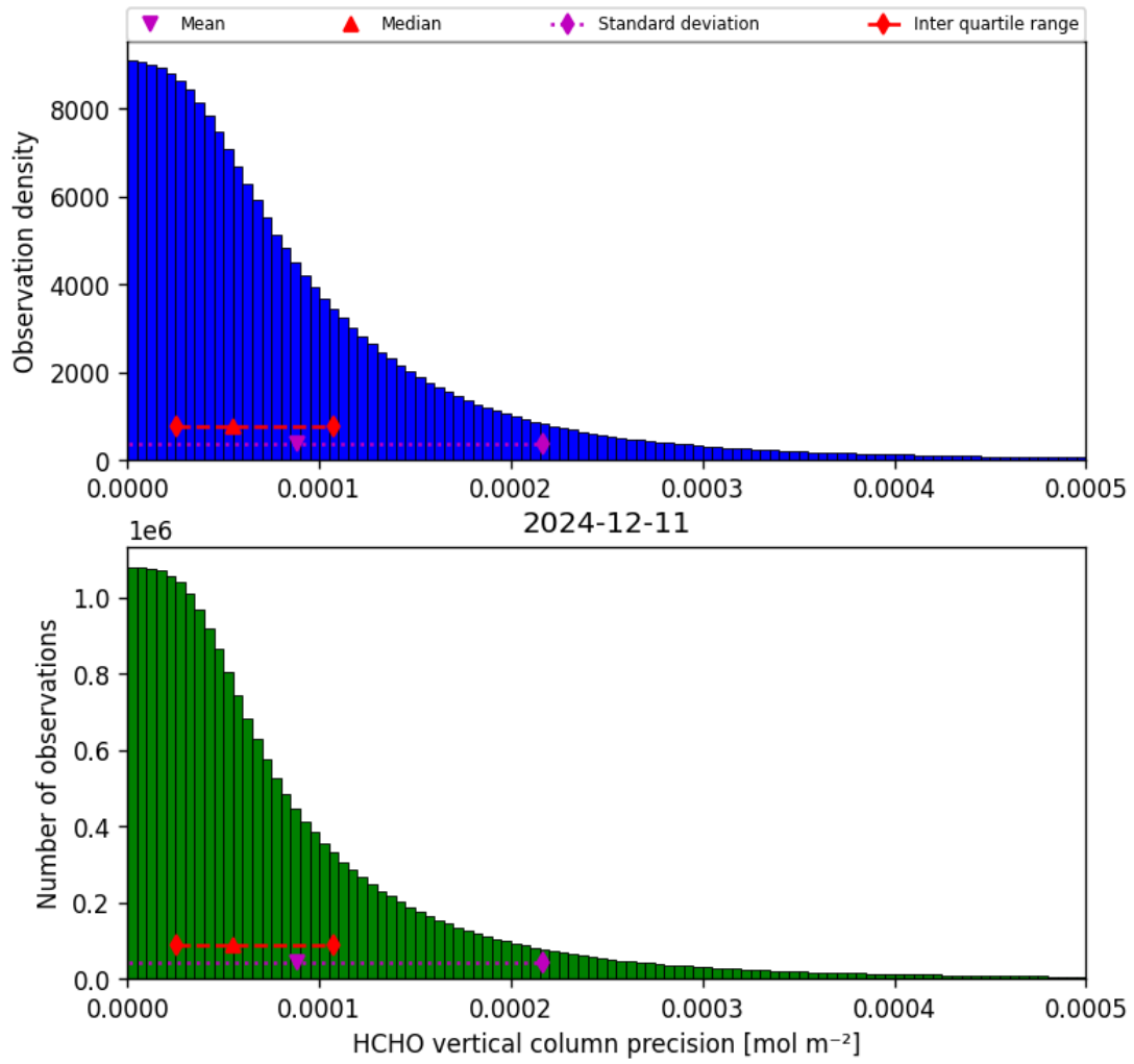
Figure 34: Histogram of “HCHO vertical column precision” for 2024-12-11 to 2024-12-12
