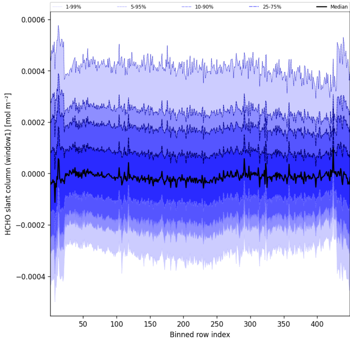
Figure 50: Along track statistics of “HCHO slant column (window1)” for 2024-12-11 to 2024-12-12
