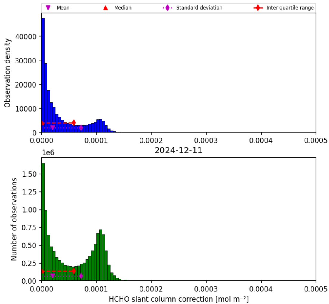
Figure 45: Histogram of “HCHO slant column correction” for 2024-12-11 to 2024-12-12
