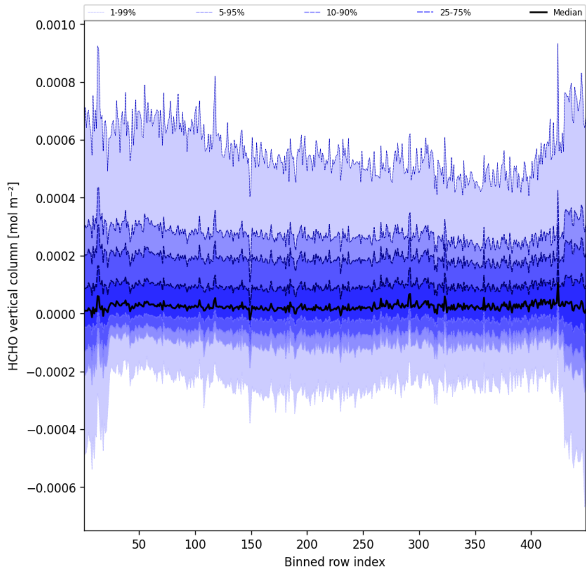
Figure 47: Along track statistics of “HCHO vertical column” for 2024-12-11 to 2024-12-12
