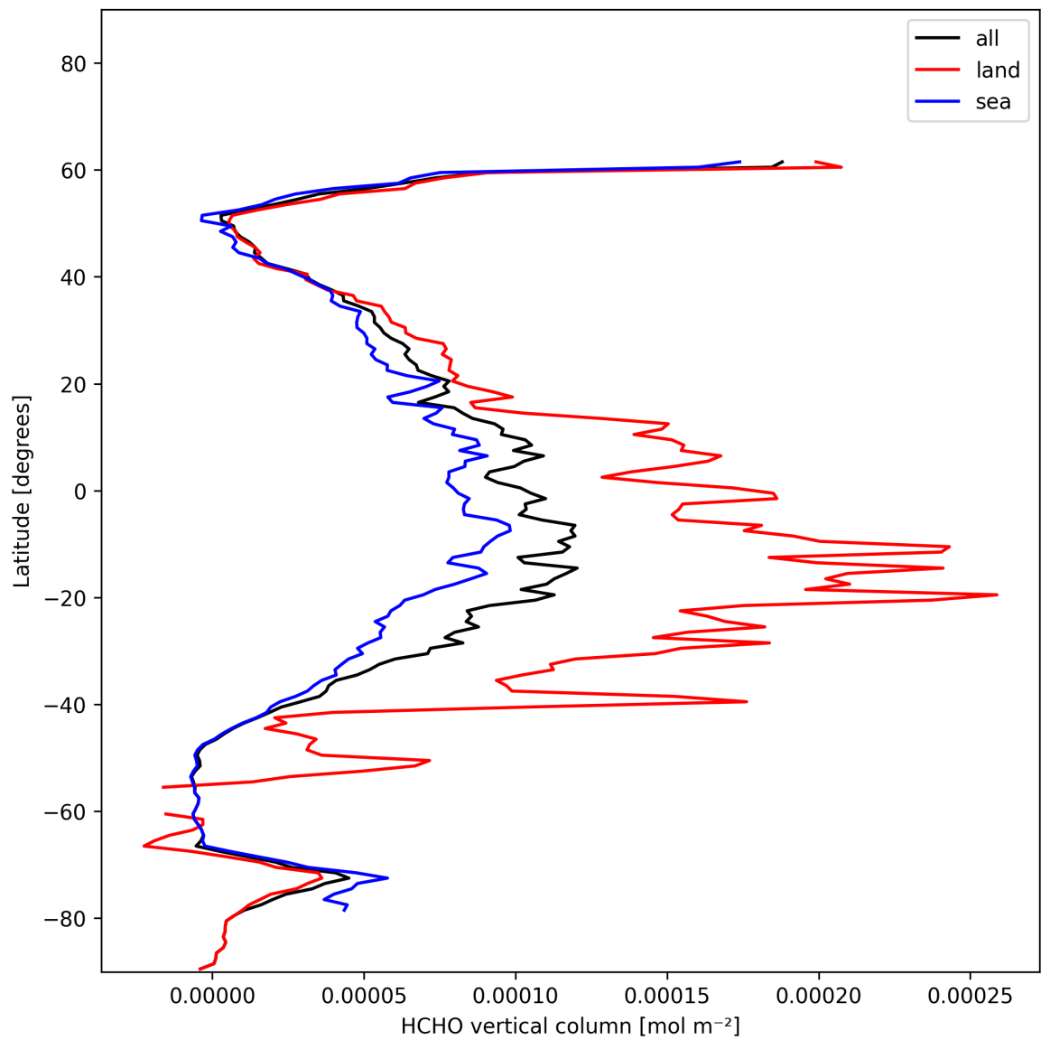
Figure 19: Zonal average of “HCHO vertical column” for 2024-12-11 to 2024-12-12.
