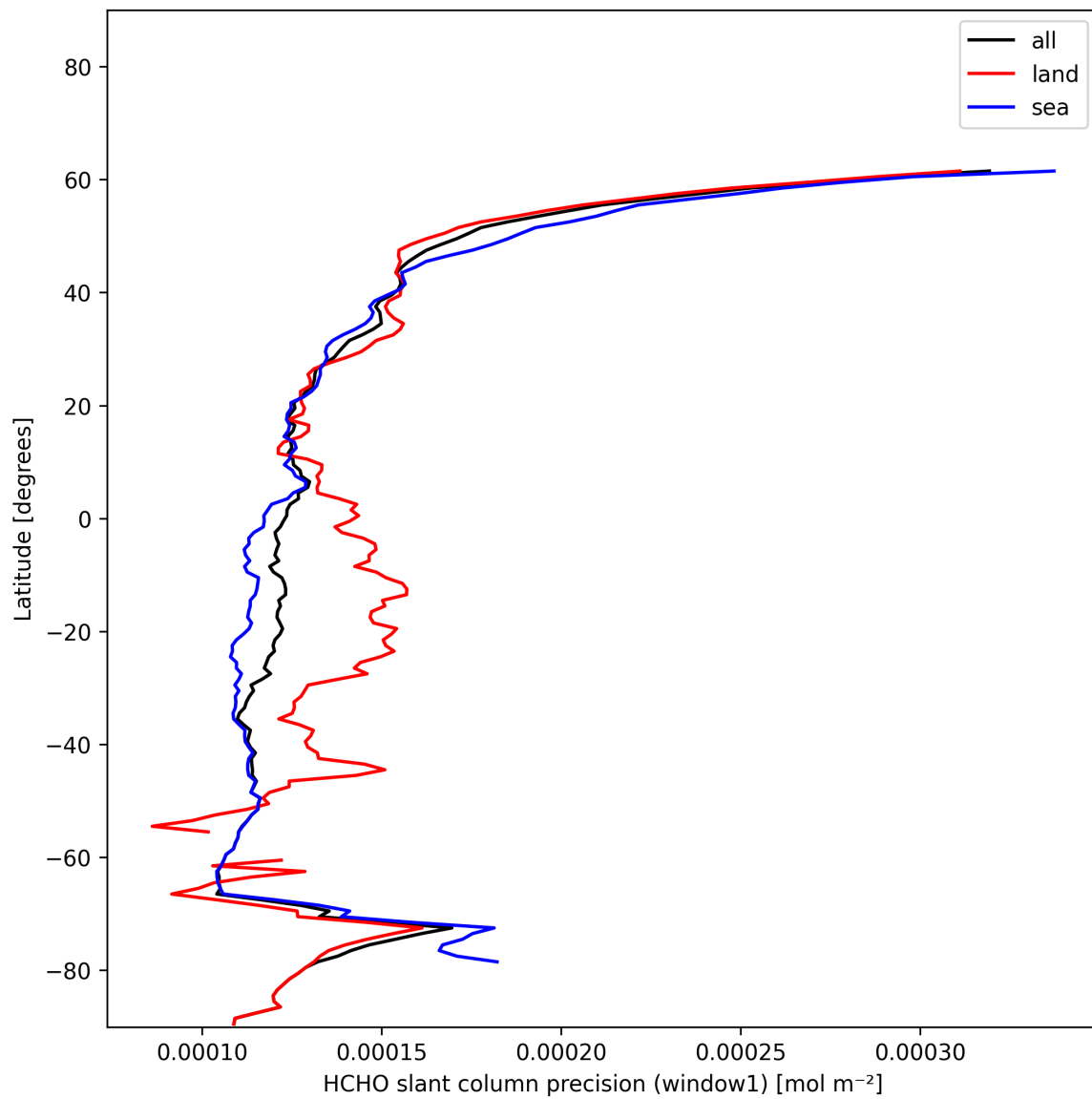
Figure 23: Zonal average of “HCHO slant column precision (window1)” for 2024-12-11 to 2024-12-12.
