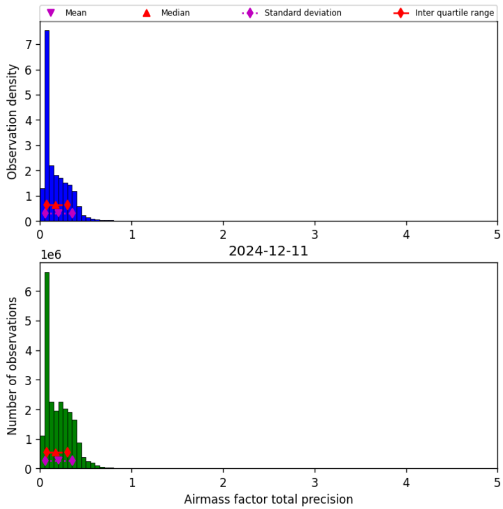
Figure 39: Histogram of “Airmass factor total precision” for 2024-12-11 to 2024-12-12
