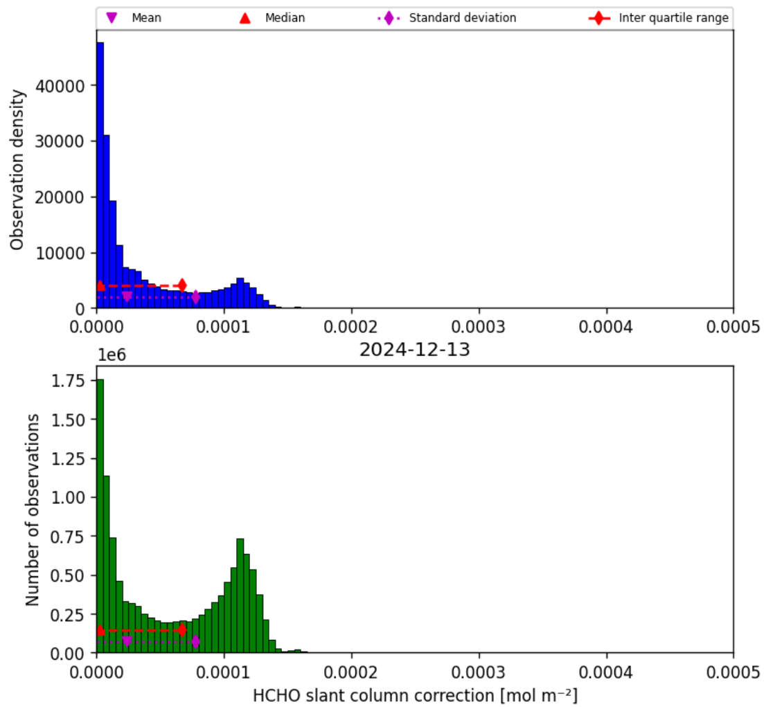
Figure 45: Histogram of “HCHO slant column correction” for 2024-12-13 to 2024-12-14
