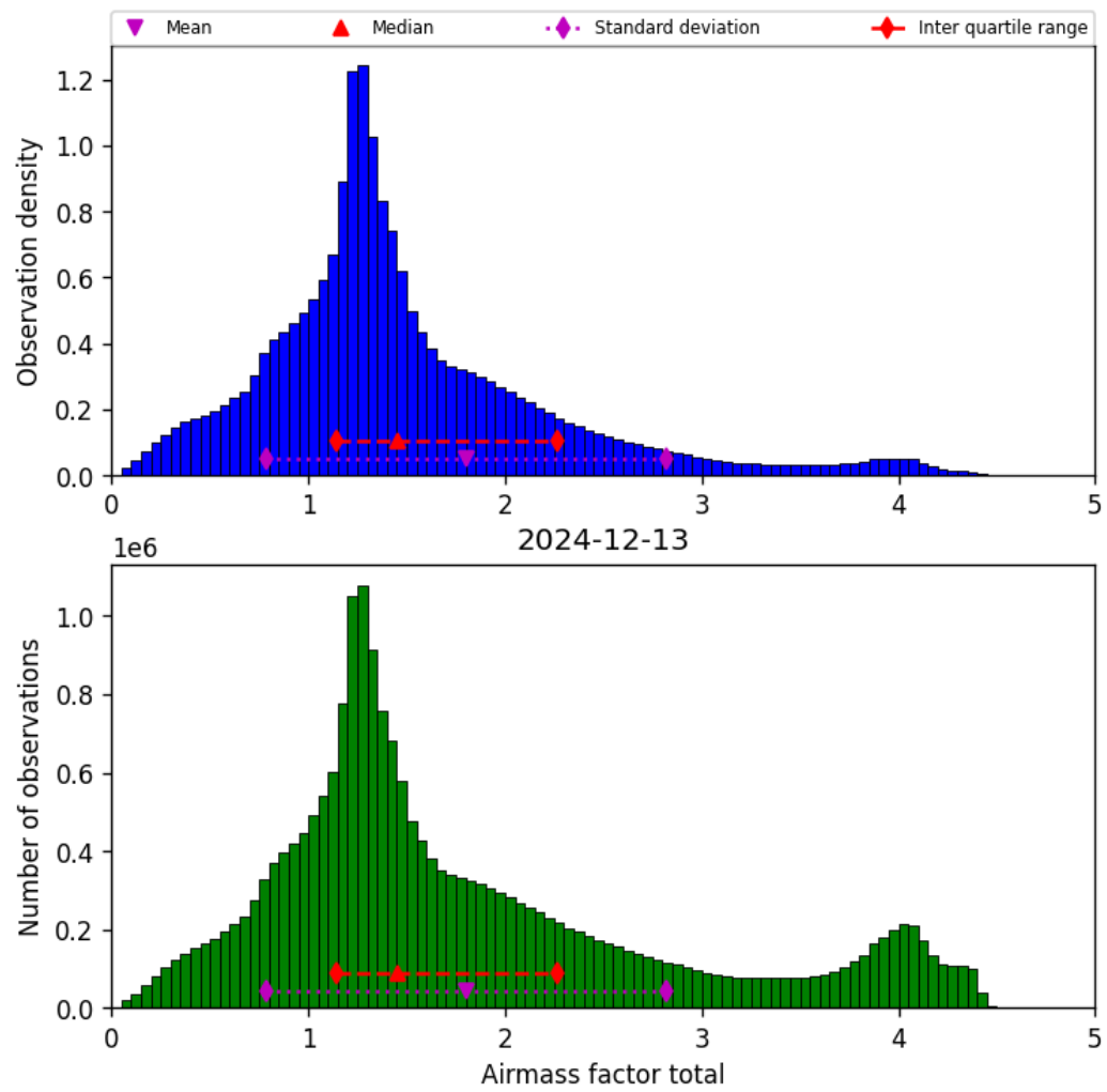
Figure 38: Histogram of “Airmass factor total” for 2024-12-13 to 2024-12-14
