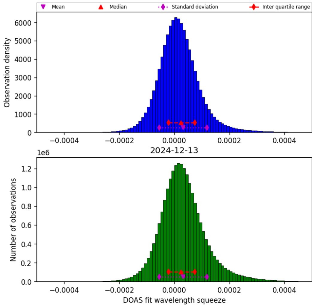
Figure 43: Histogram of “DOAS fit wavelength squeeze” for 2024-12-13 to 2024-12-14
