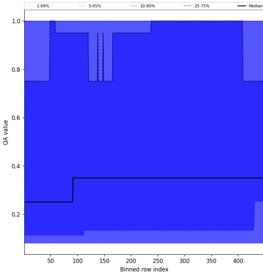
Figure 46: Along track statistics of “QA value” for 2024-12-13 to 2024-12-14
