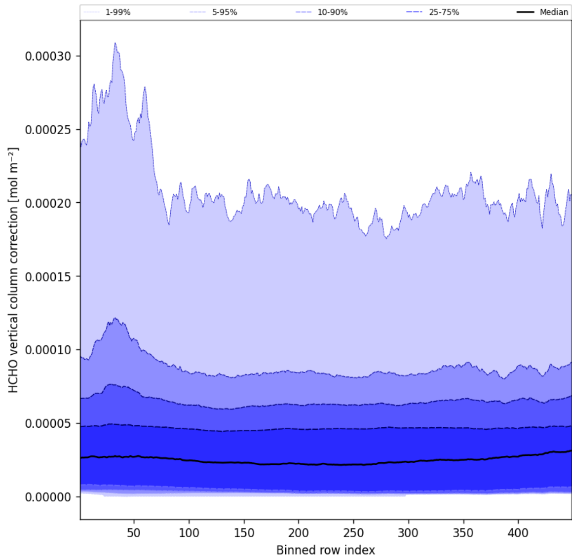
Figure 49: Along track statistics of “HCHO vertical column correction” for 2024-12-13 to 2024-12-14
