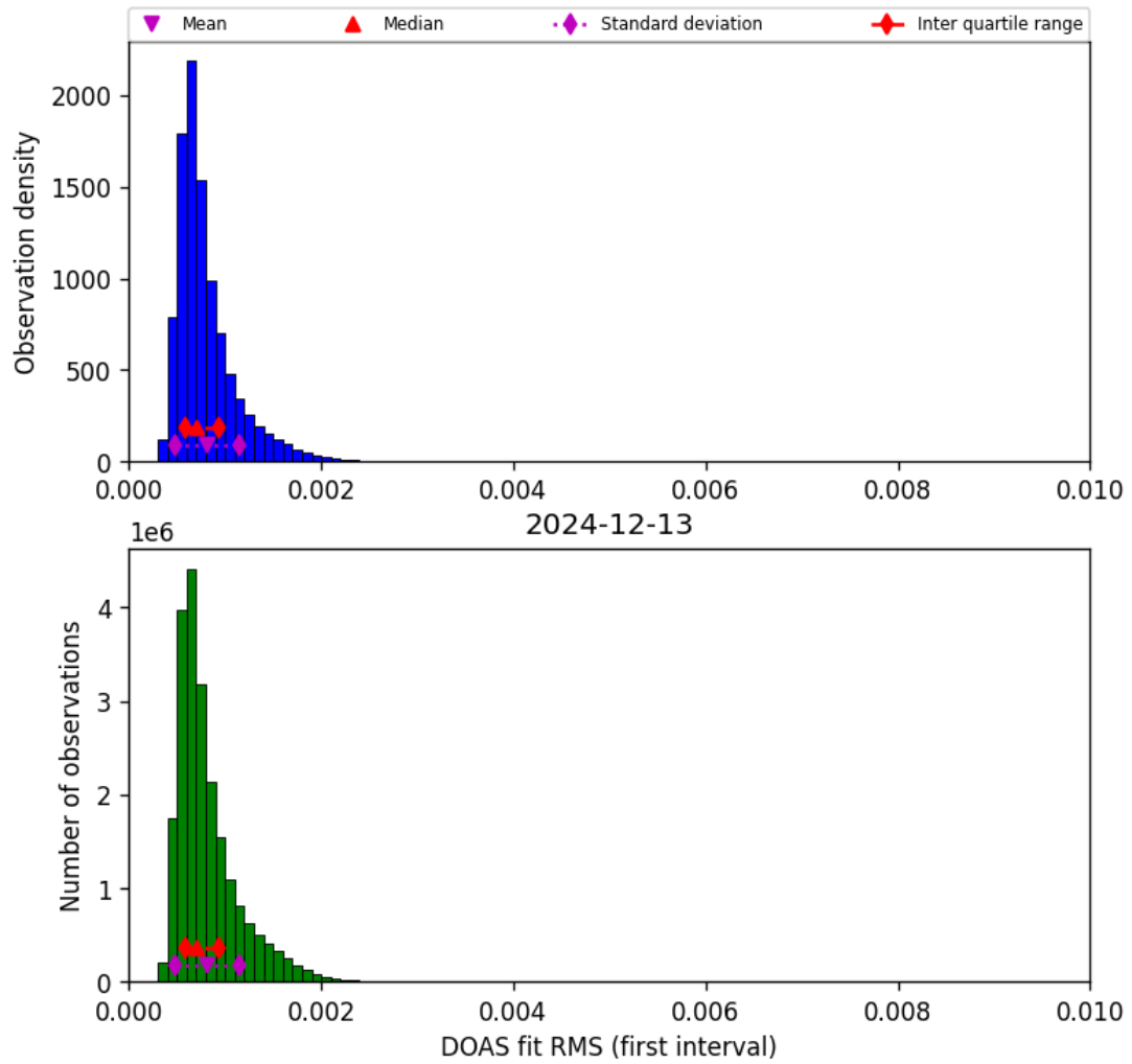
Figure 44: Histogram of “DOAS fit RMS (first interval)” for 2024-12-13 to 2024-12-14
