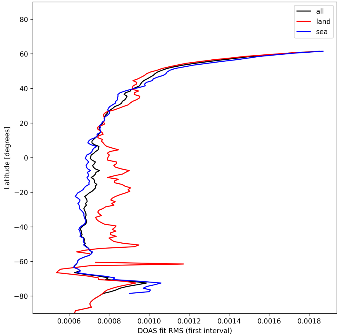
Figure 30: Zonal average of “DOAS fit RMS (first interval)” for 2024-12-13 to 2024-12-14.
