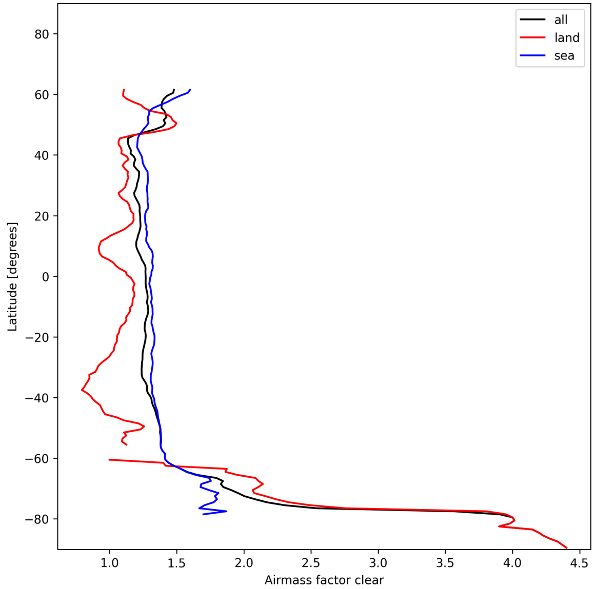
Figure 26: Zonal average of “Airmass factor clear” for 2024-12-13 to 2024-12-14.
