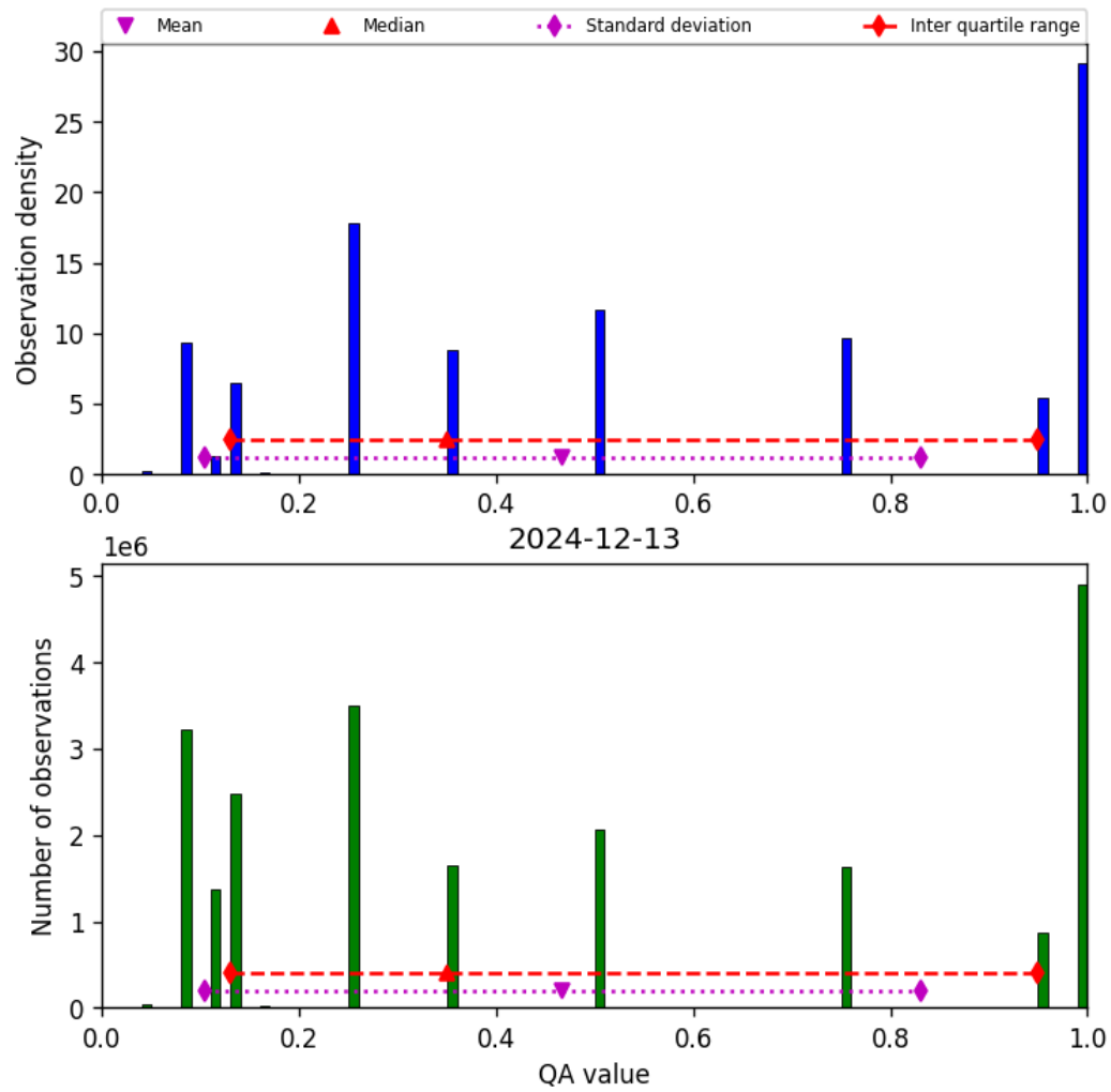
Figure 32: Histogram of “QA value” for 2024-12-13 to 2024-12-14
