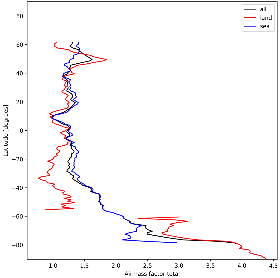
Figure 24: Zonal average of “Airmass factor total” for 2024-12-13 to 2024-12-14.
