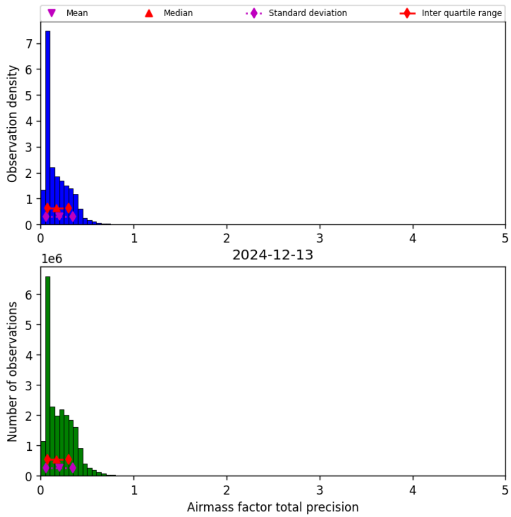
Figure 39: Histogram of “Airmass factor total precision” for 2024-12-13 to 2024-12-14
