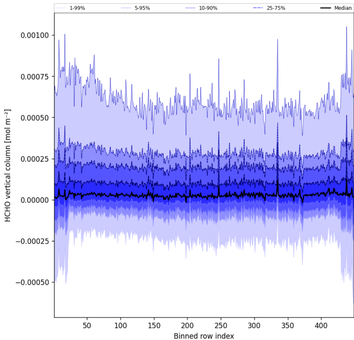
Figure 47: Along track statistics of “HCHO vertical column” for 2024-12-13 to 2024-12-14
