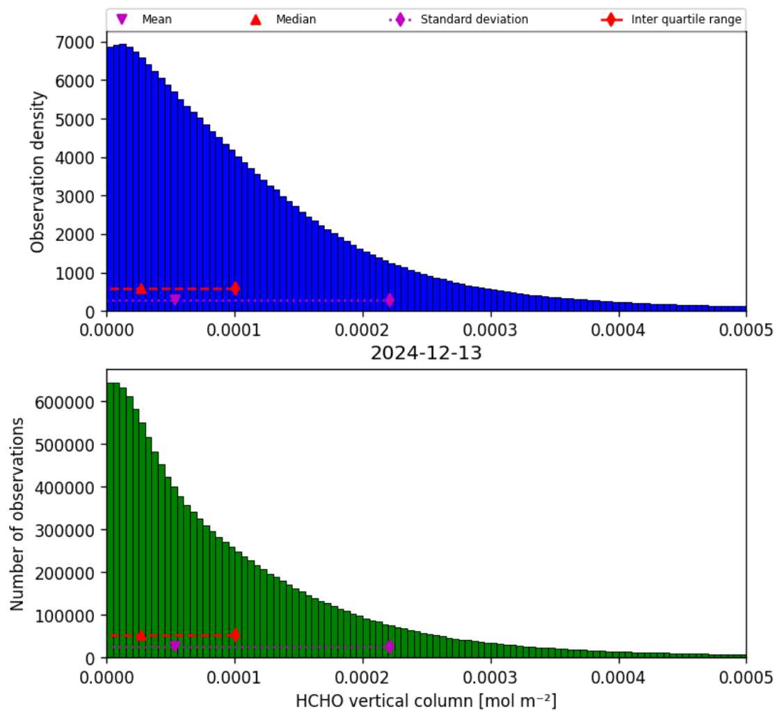
Figure 33: Histogram of “HCHO vertical column” for 2024-12-13 to 2024-12-14
