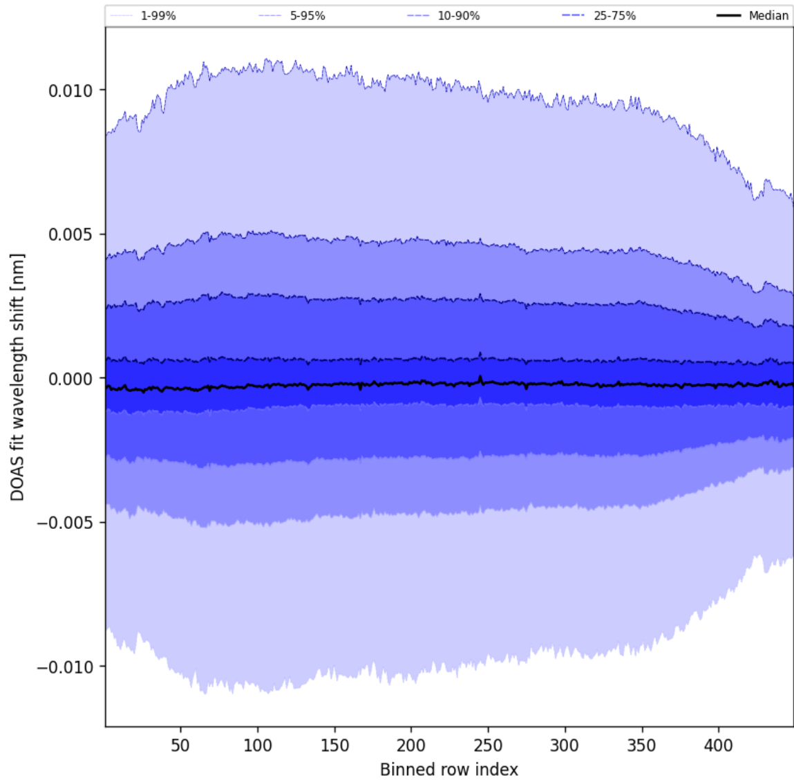
Figure 56: Along track statistics of “DOAS fit wavelength shift” for 2024-12-13 to 2024-12-14
