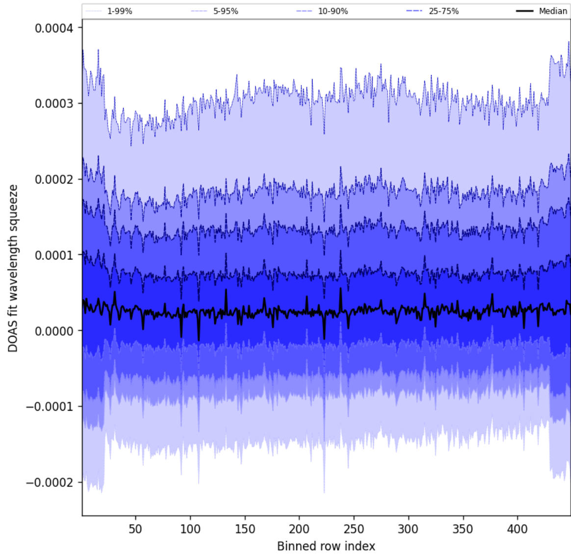
Figure 57: Along track statistics of “DOAS fit wavelength squeeze” for 2024-12-13 to 2024-12-14
