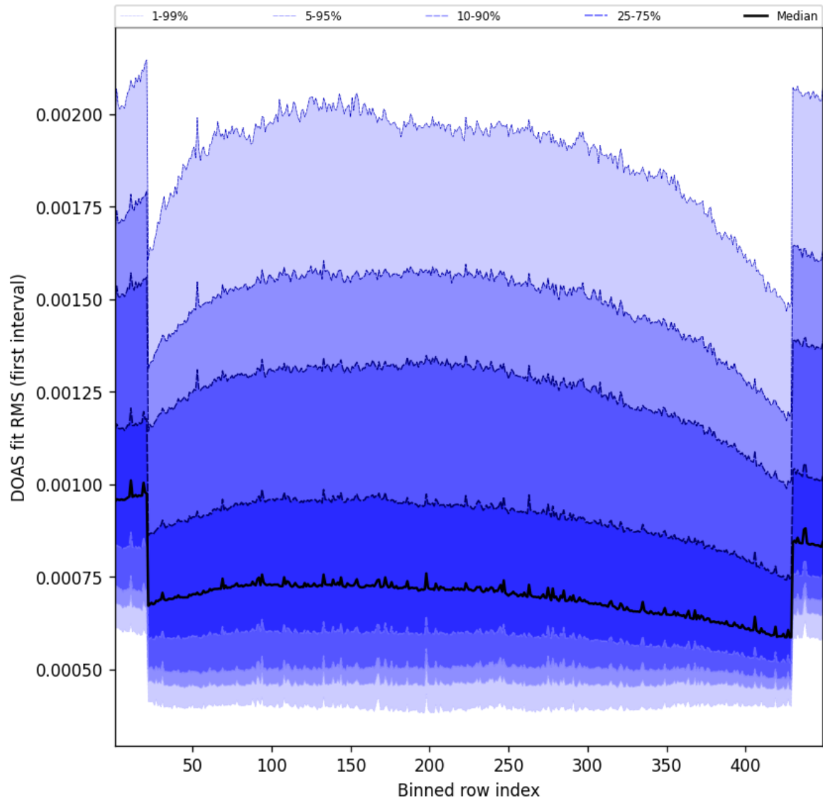
Figure 58: Along track statistics of “DOAS fit RMS (first interval)” for 2024-12-13 to 2024-12-14
