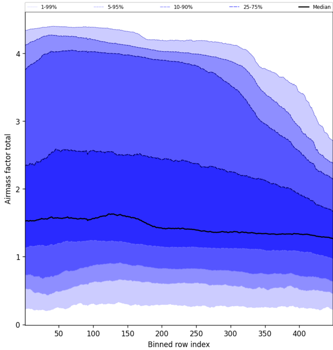
Figure 52: Along track statistics of “Airmass factor total” for 2024-12-13 to 2024-12-14
