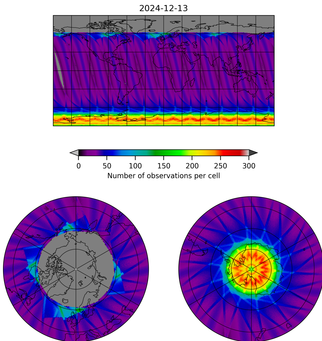
Figure 17: Map of the number of observations for 2024-12-13 to 2024-12-14
