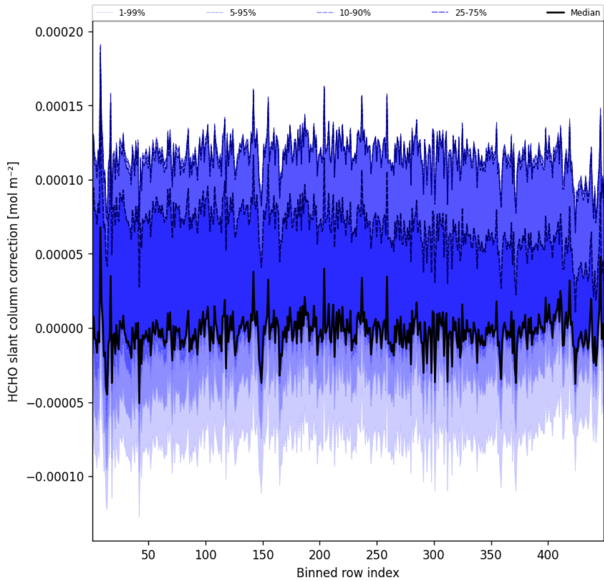
Figure 59: Along track statistics of “HCHO slant column correction” for 2024-12-13 to 2024-12-14
