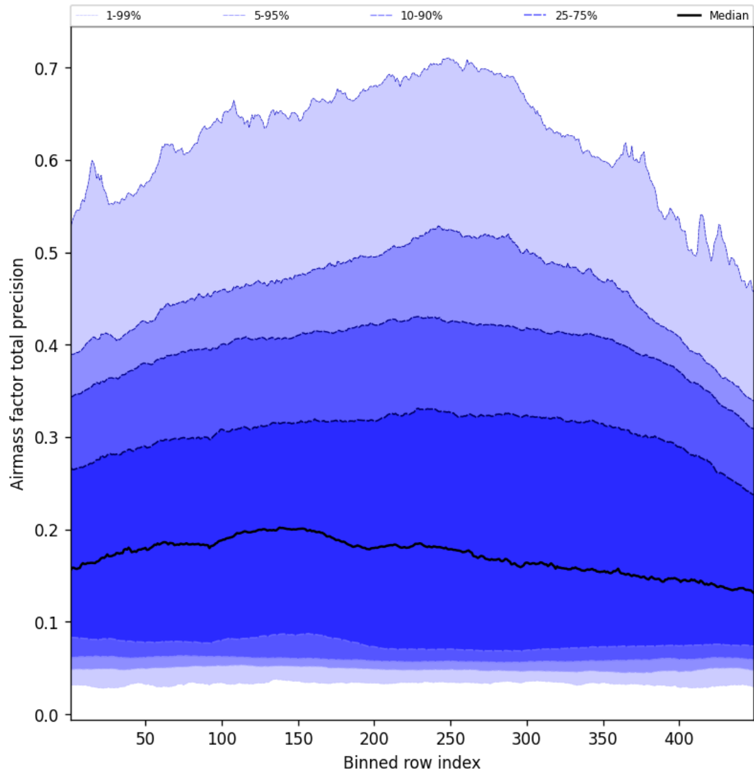
Figure 53: Along track statistics of “Airmass factor total precision” for 2024-12-13 to 2024-12-14
