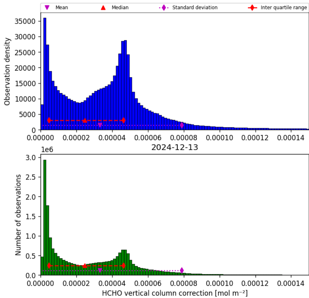
Figure 35: Histogram of “HCHO vertical column correction” for 2024-12-13 to 2024-12-14
