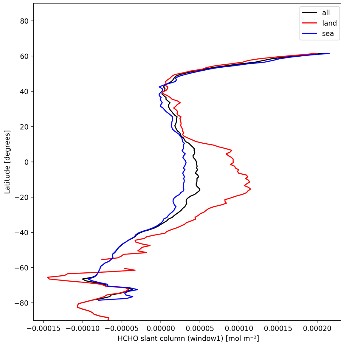
Figure 22: Zonal average of “HCHO slant column (window1)” for 2024-12-13 to 2024-12-14.
