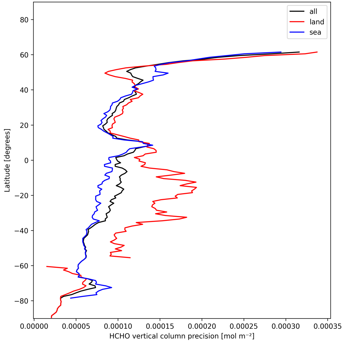
Figure 20: Zonal average of “HCHO vertical column precision” for 2024-12-13 to 2024-12-14.
