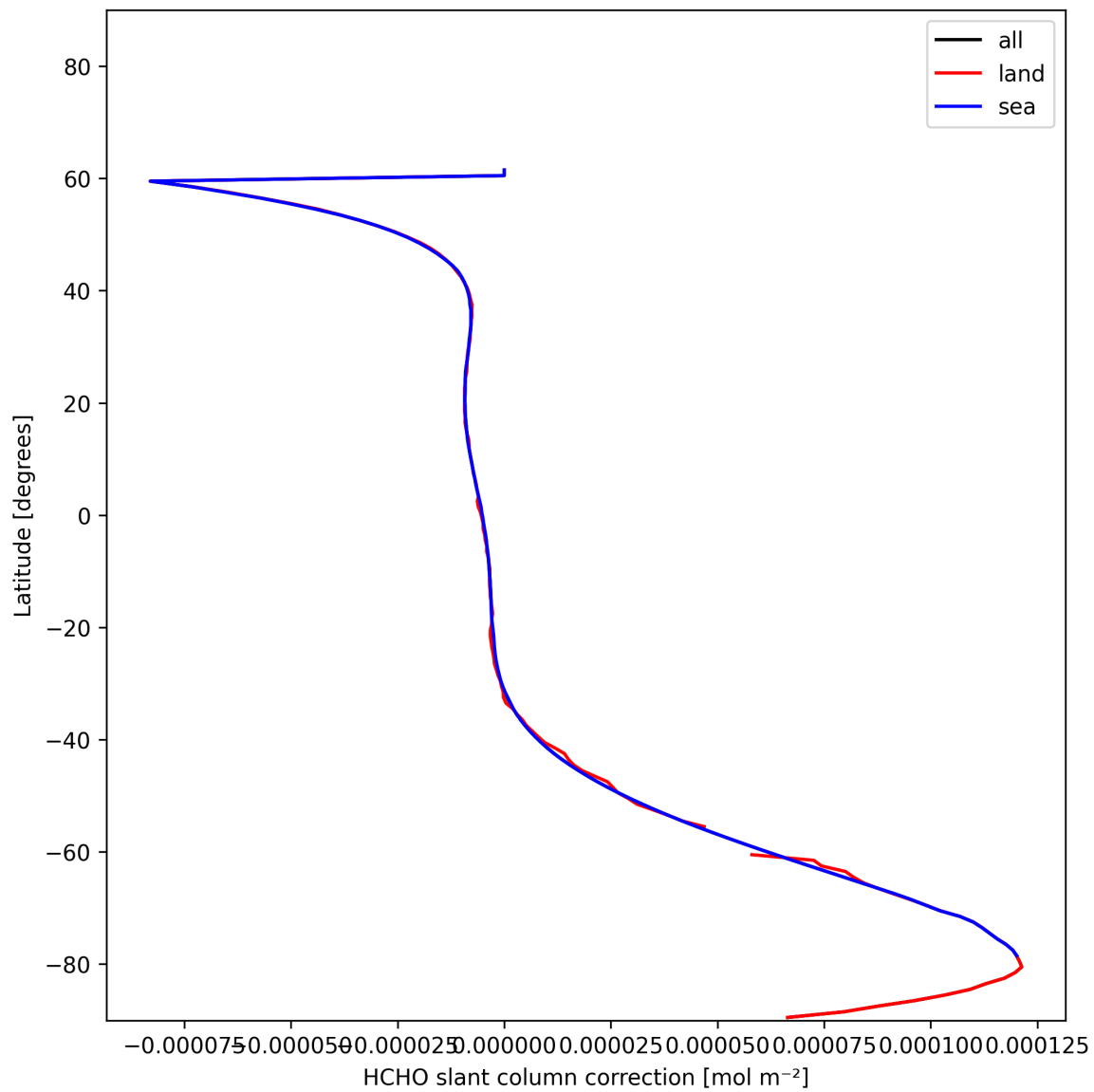
Figure 31: Zonal average of “HCHO slant column correction” for 2024-12-13 to 2024-12-14.
