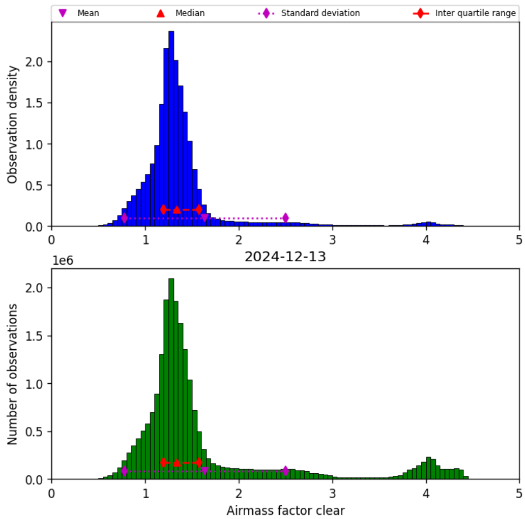
Figure 40: Histogram of “Airmass factor clear” for 2024-12-13 to 2024-12-14
