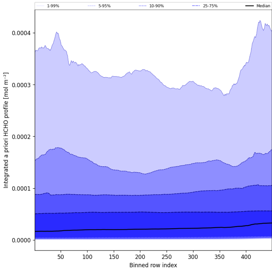
Figure 55: Along track statistics of “Integrated a priori HCHO profile” for 2024-12-13 to 2024-12-14
