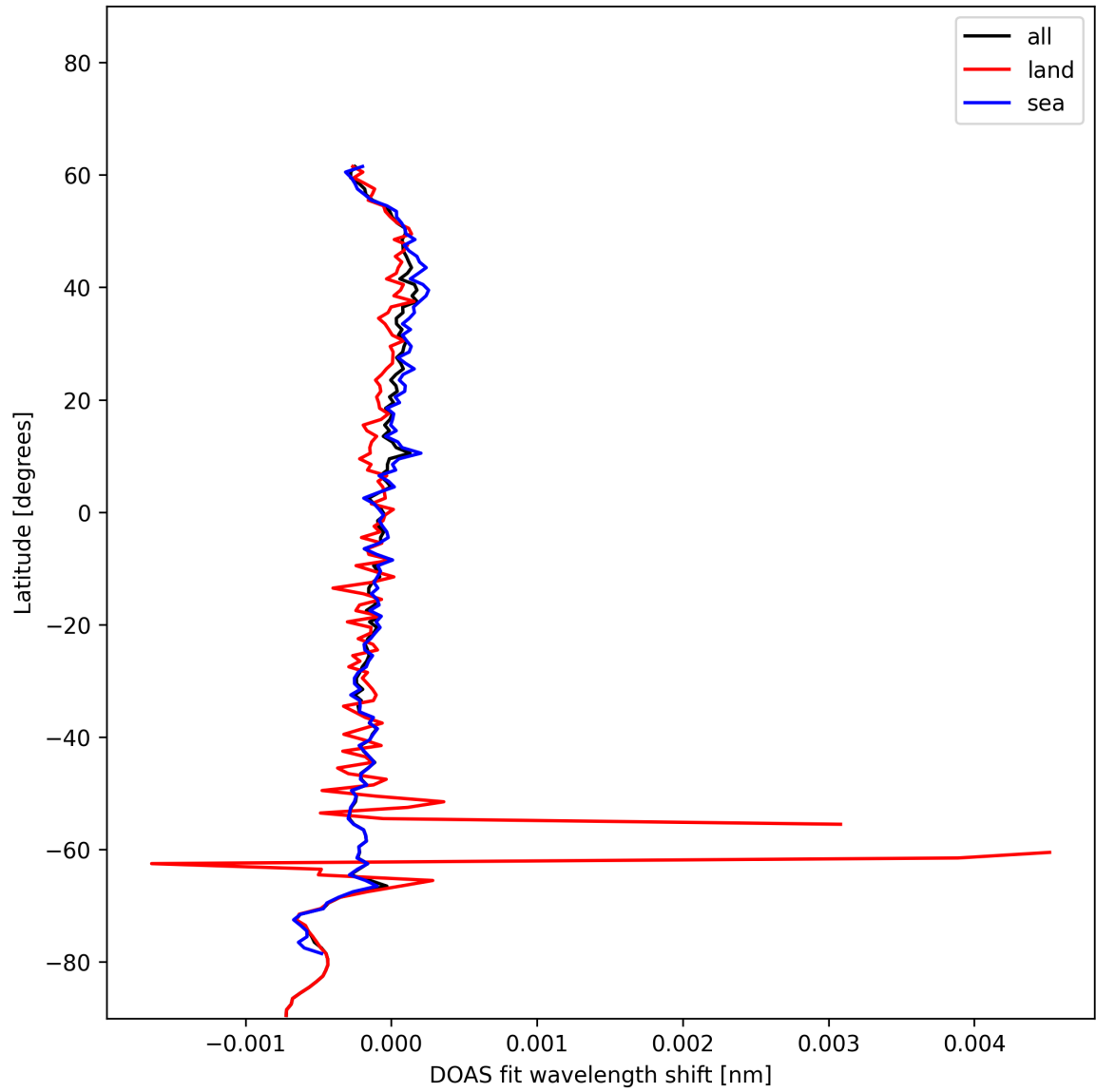
Figure 28: Zonal average of “DOAS fit wavelength shift” for 2024-12-13 to 2024-12-14.
