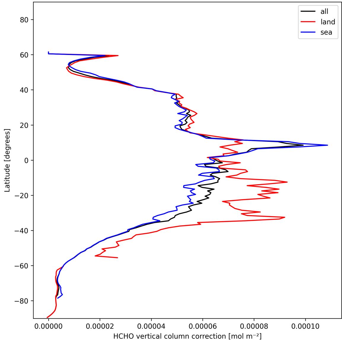
Figure 21: Zonal average of “HCHO vertical column correction” for 2024-12-13 to 2024-12-14.
