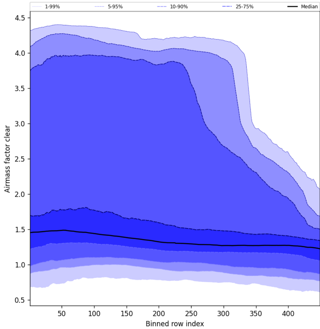
Figure 54: Along track statistics of “Air mass factor clear” for 2024-12-13 to 2024-12-14
