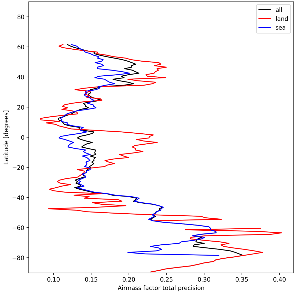
Figure 25: Zonal average of “Airmass factor total precision” for 2024-12-13 to 2024-12-14.
