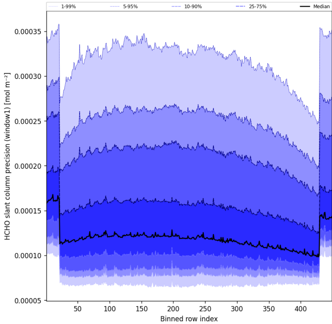
Figure 51: Along track statistics of “HCHO slant column precision (window1)” for 2024-12-13 to 2024-12-14
