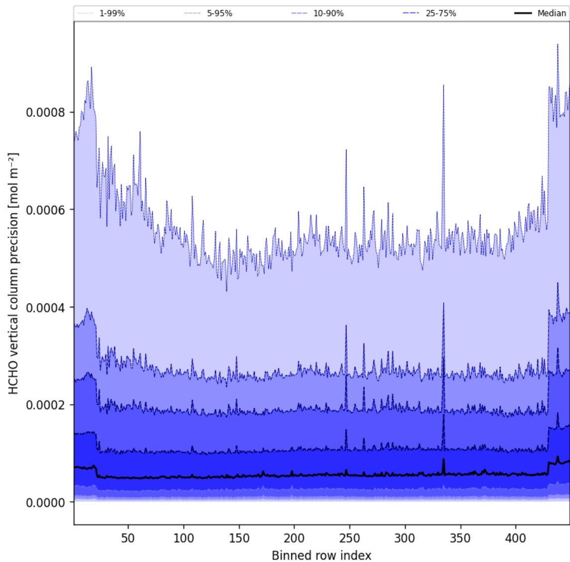
Figure 48: Along track statistics of “HCHO vertical column precision” for 2024-12-13 to 2024-12-14
