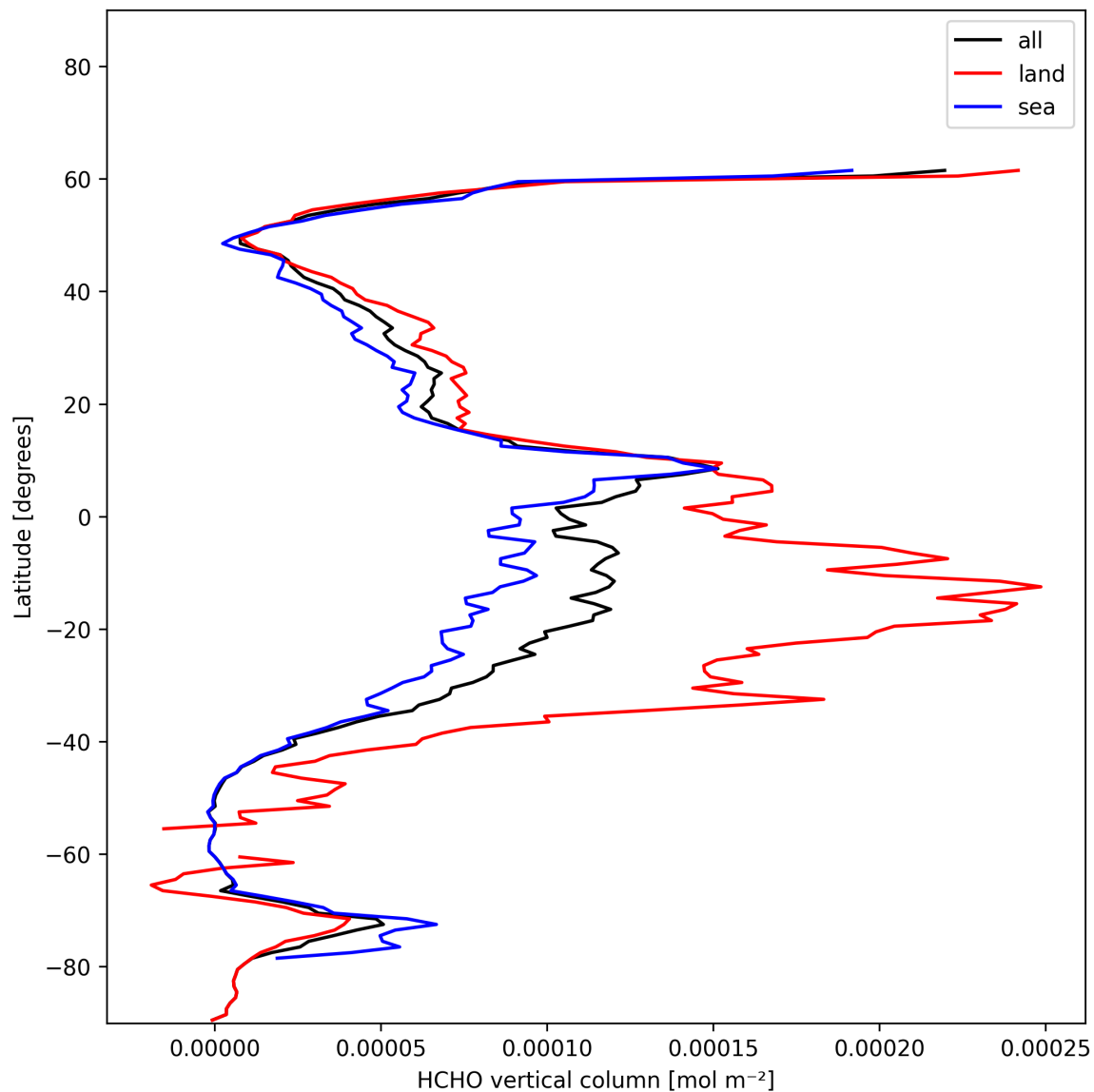
Figure 19: Zonal average of “HCHO vertical column” for 2024-12-13 to 2024-12-14.
