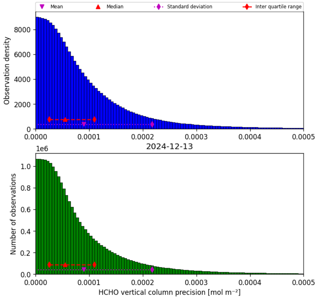
Figure 34: Histogram of “HCHO vertical column precision” for 2024-12-13 to 2024-12-14
