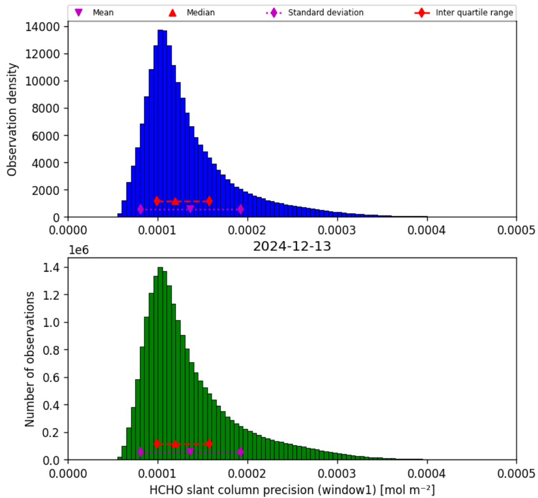
Figure 37: Histogram of “HCHO slant column precision (window1)” for 2024-12-13 to 2024-12-14
