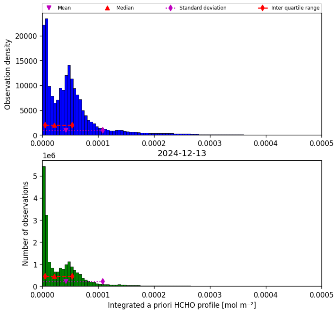
Figure 41: Histogram of “Integrated a priori HCHO profile” for 2024-12-13 to 2024-12-14
