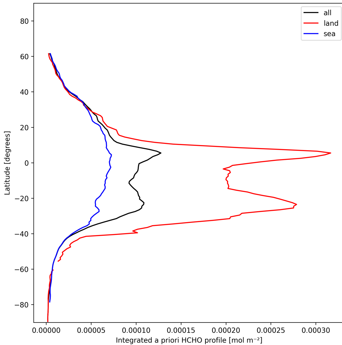
Figure 27: Zonal average of “Integrated a priori HCHO profile” for 2024-12-13 to 2024-12-14.
