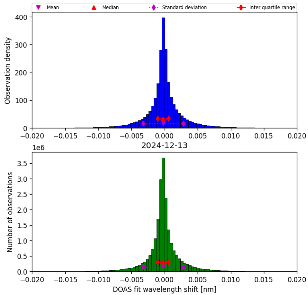
Figure 42: Histogram of “DOAS fit wavelength shift” for 2024-12-13 to 2024-12-14
