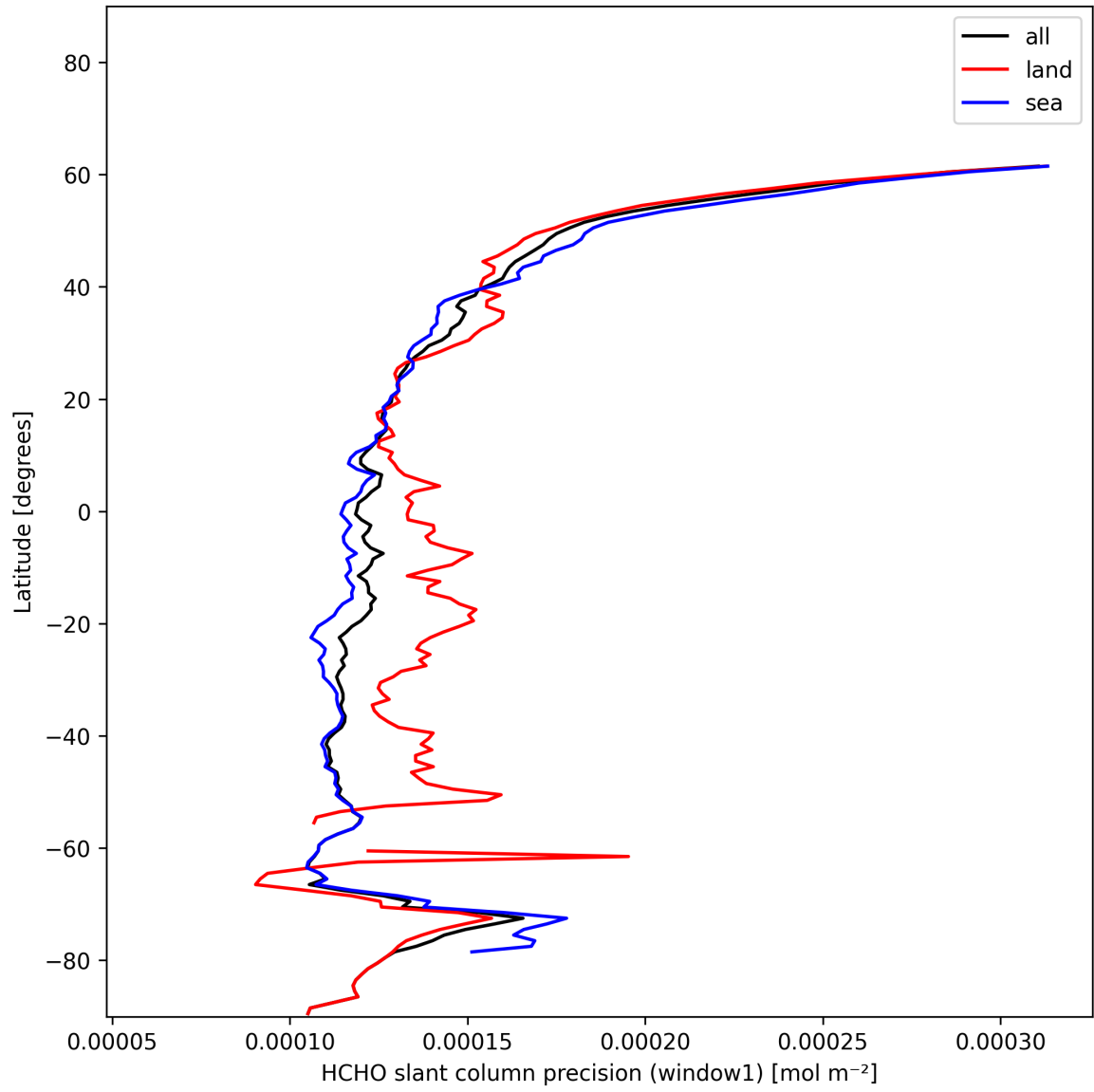
Figure 23: Zonal average of “HCHO slant column precision (window1)” for 2024-12-13 to 2024-12-14.
