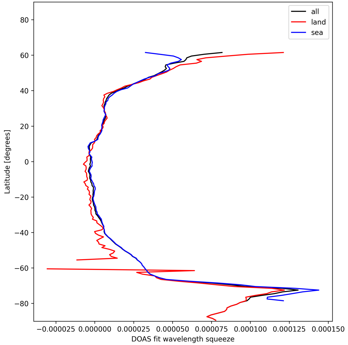
Figure 29: Zonal average of “DOAS fit wavelength squeeze” for 2024-12-13 to 2024-12-14.
