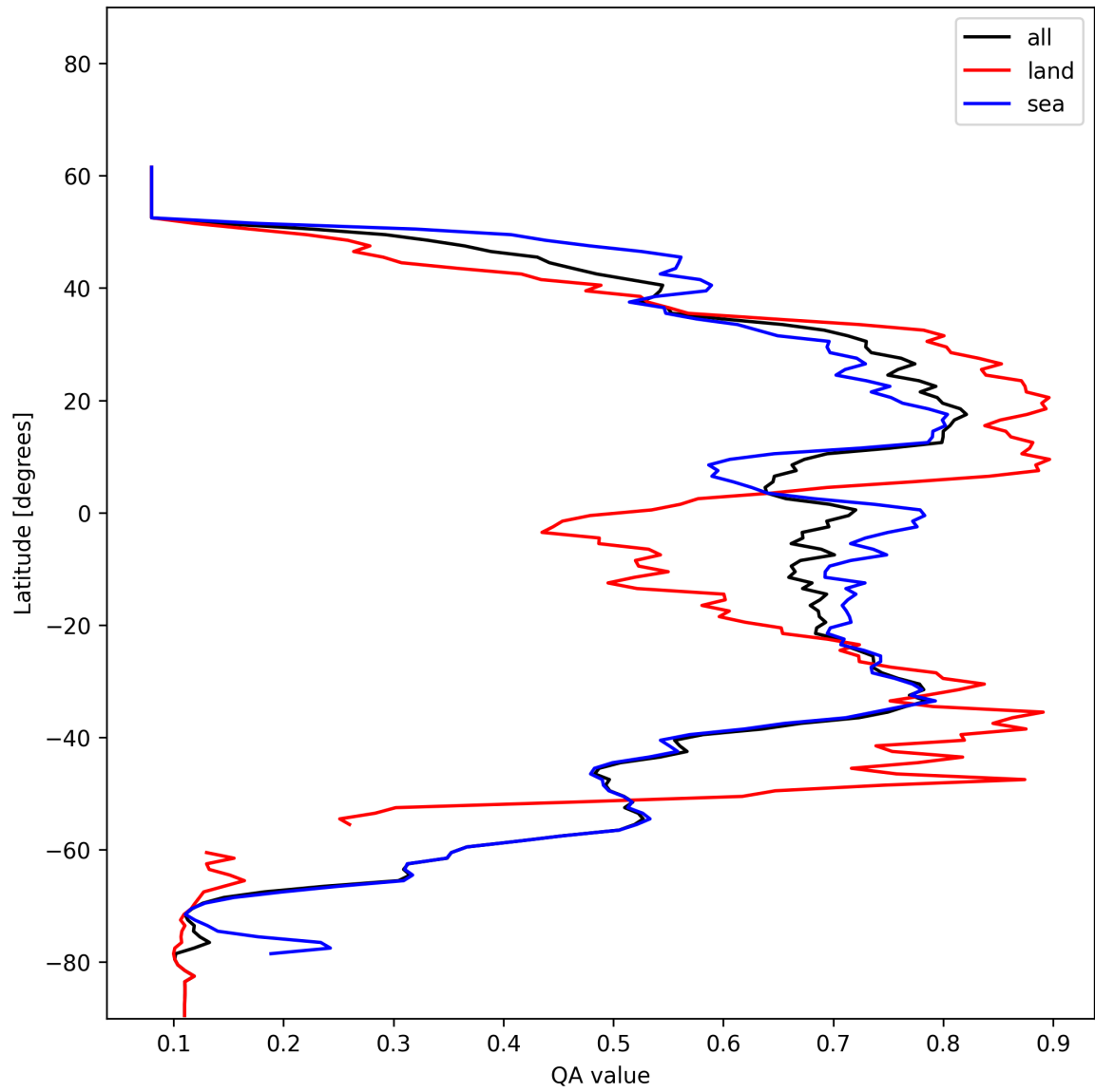
Figure 18: Zonal average of “QA value” for 2024-12-13 to 2024-12-14.
