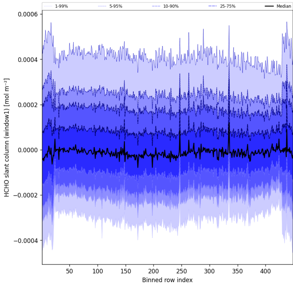
Figure 50: Along track statistics of “HCHO slant column (window1)” for 2024-12-13 to 2024-12-14
