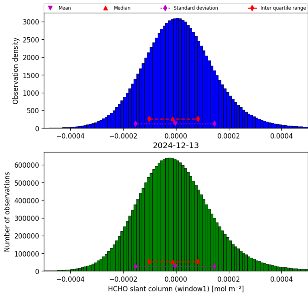
Figure 36: Histogram of “HCHO slant column (window1)” for 2024-12-13 to 2024-12-14
