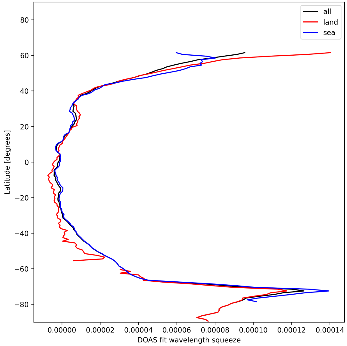
Figure 29: Zonal average of “DOAS fit wavelength squeeze” for 2024-12-14 to 2024-12-14.
