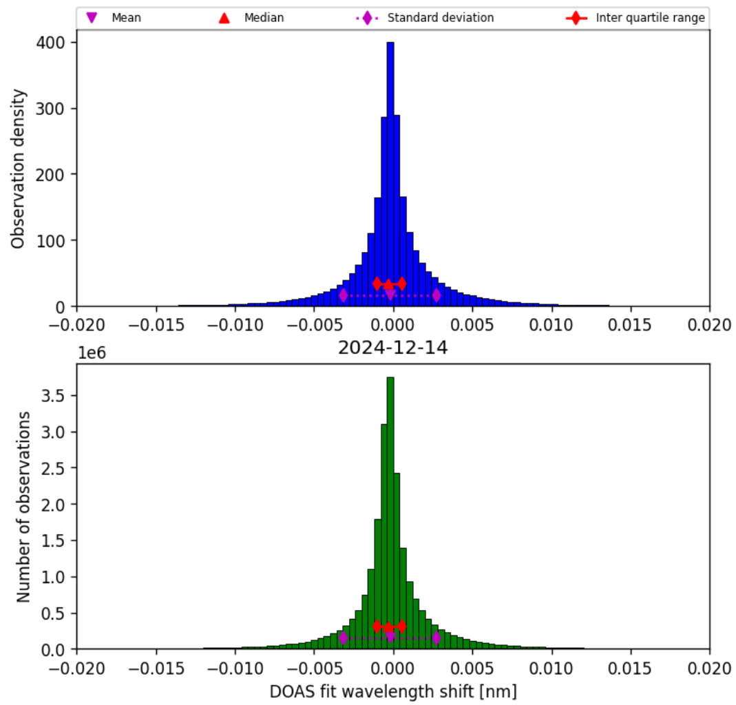
Figure 42: Histogram of “DOAS fit wavelength shift” for 2024-12-14 to 2024-12-14
