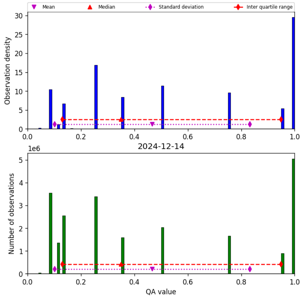
Figure 32: Histogram of “QA value” for 2024-12-14 to 2024-12-14
