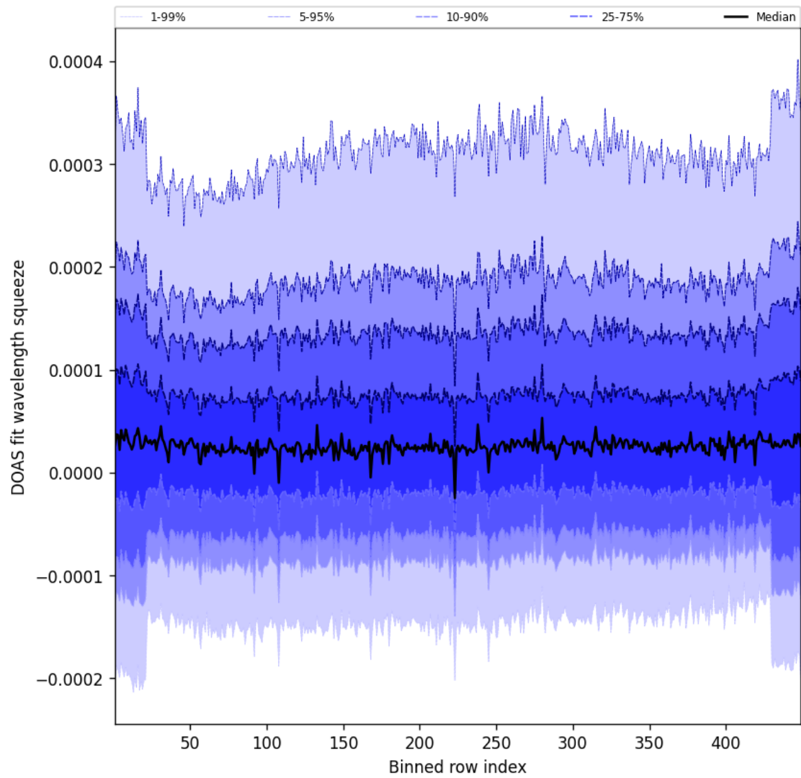
Figure 57: Along track statistics of “DOAS fit wavelength squeeze” for 2024-12-14 to 2024-12-14
