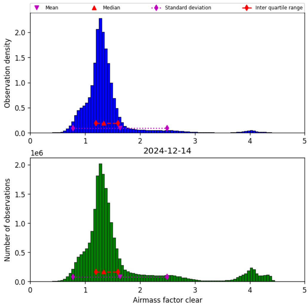
Figure 40: Histogram of “Airmass factor clear” for 2024-12-14 to 2024-12-14
