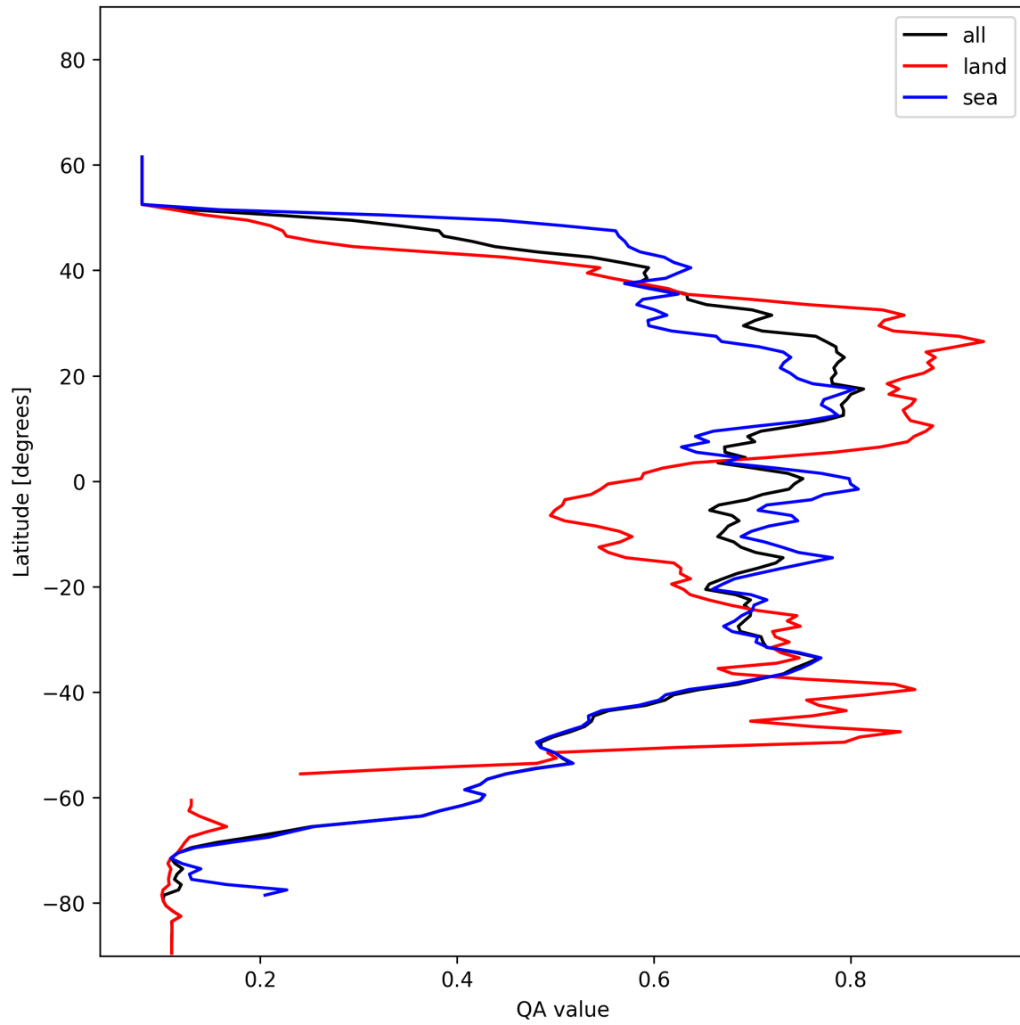
Figure 18: Zonal average of “QA value” for 2024-12-14 to 2024-12-14.
