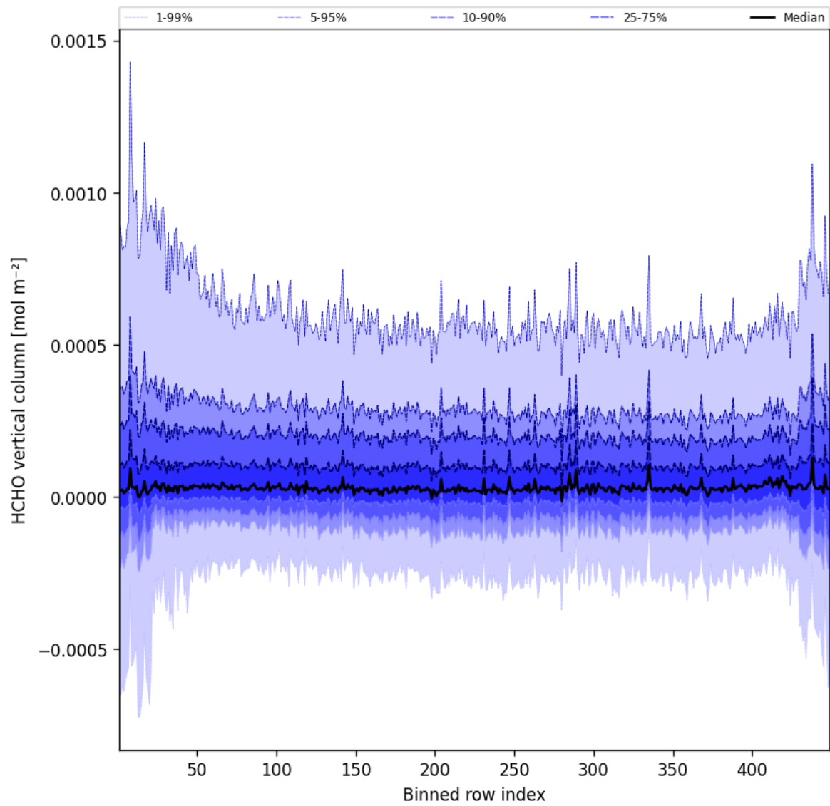
Figure 47: Along track statistics of “HCHO vertical column” for 2024-12-14 to 2024-12-14
