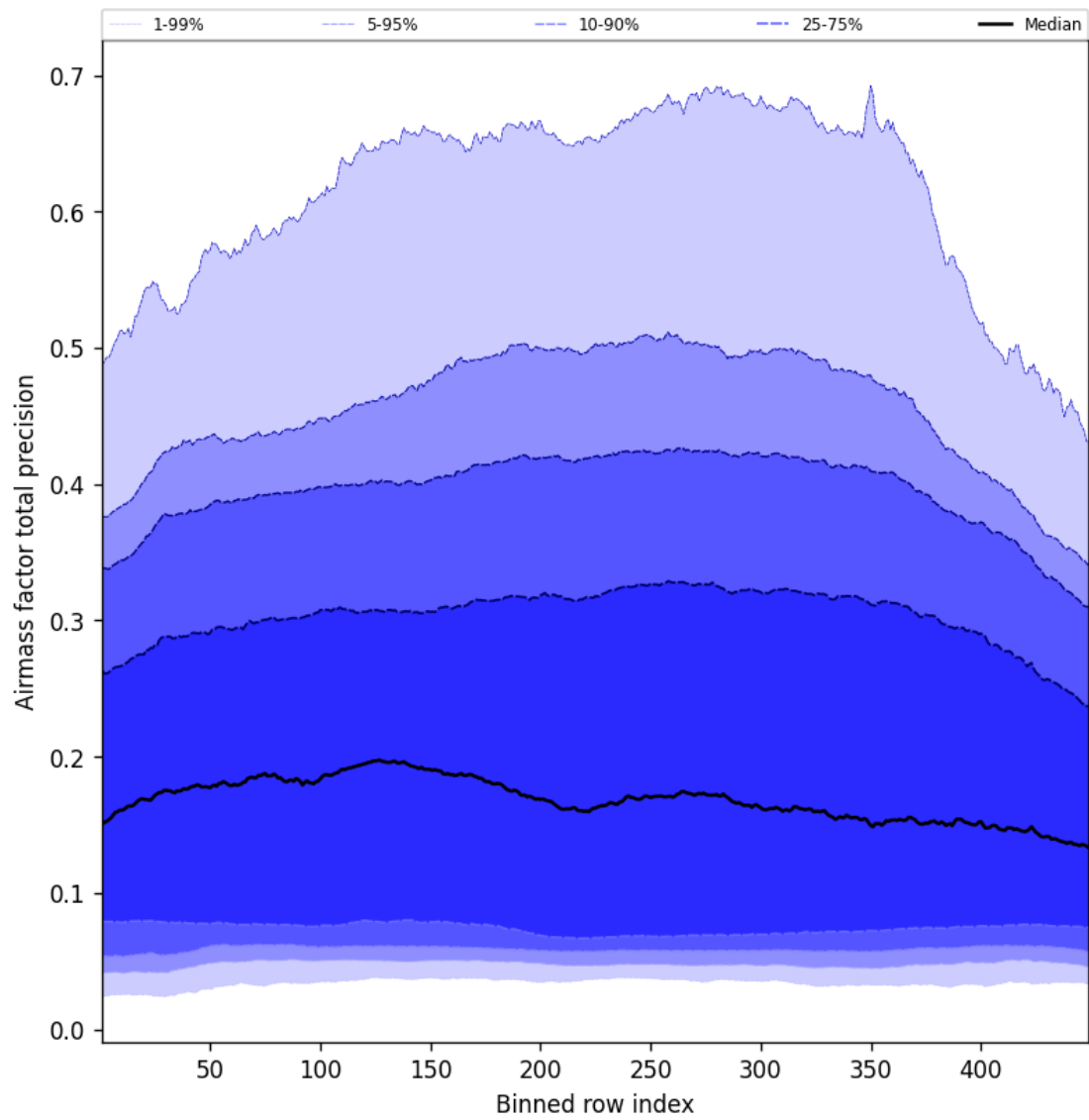
Figure 53: Along track statistics of “Airmass factor total precision” for 2024-12-14 to 2024-12-14
