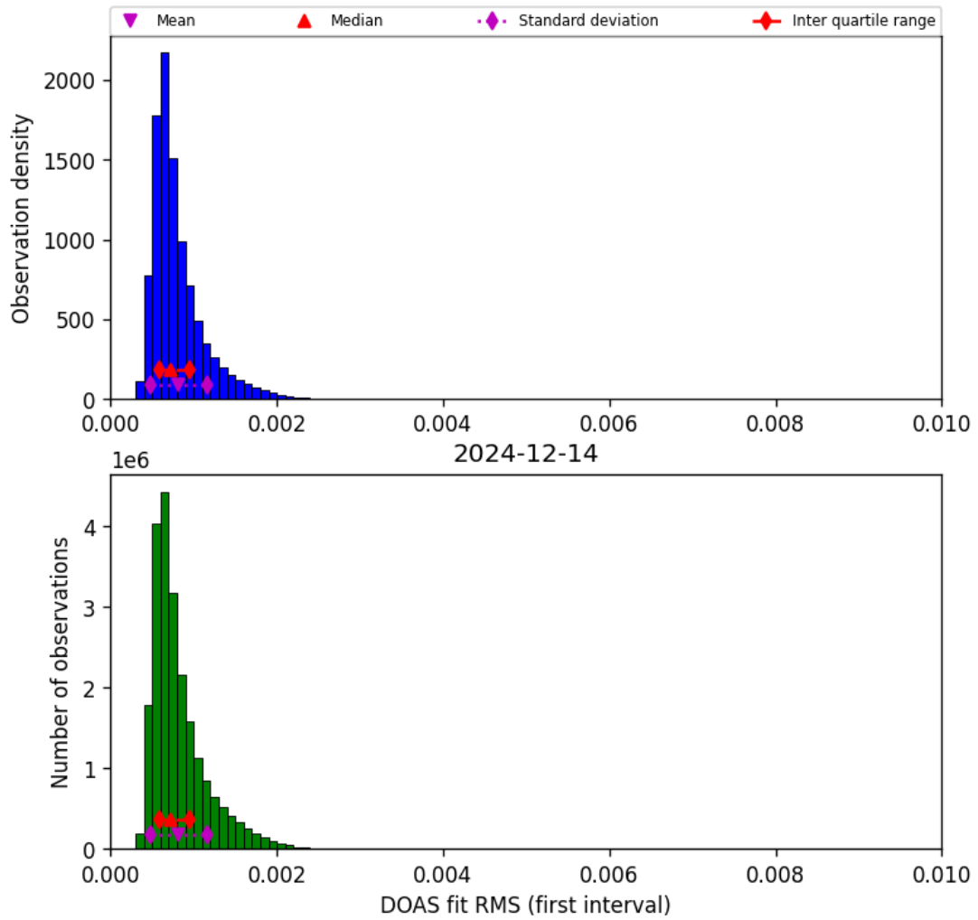
Figure 44: Histogram of “DOAS fit RMS (first interval)” for 2024-12-14 to 2024-12-14
