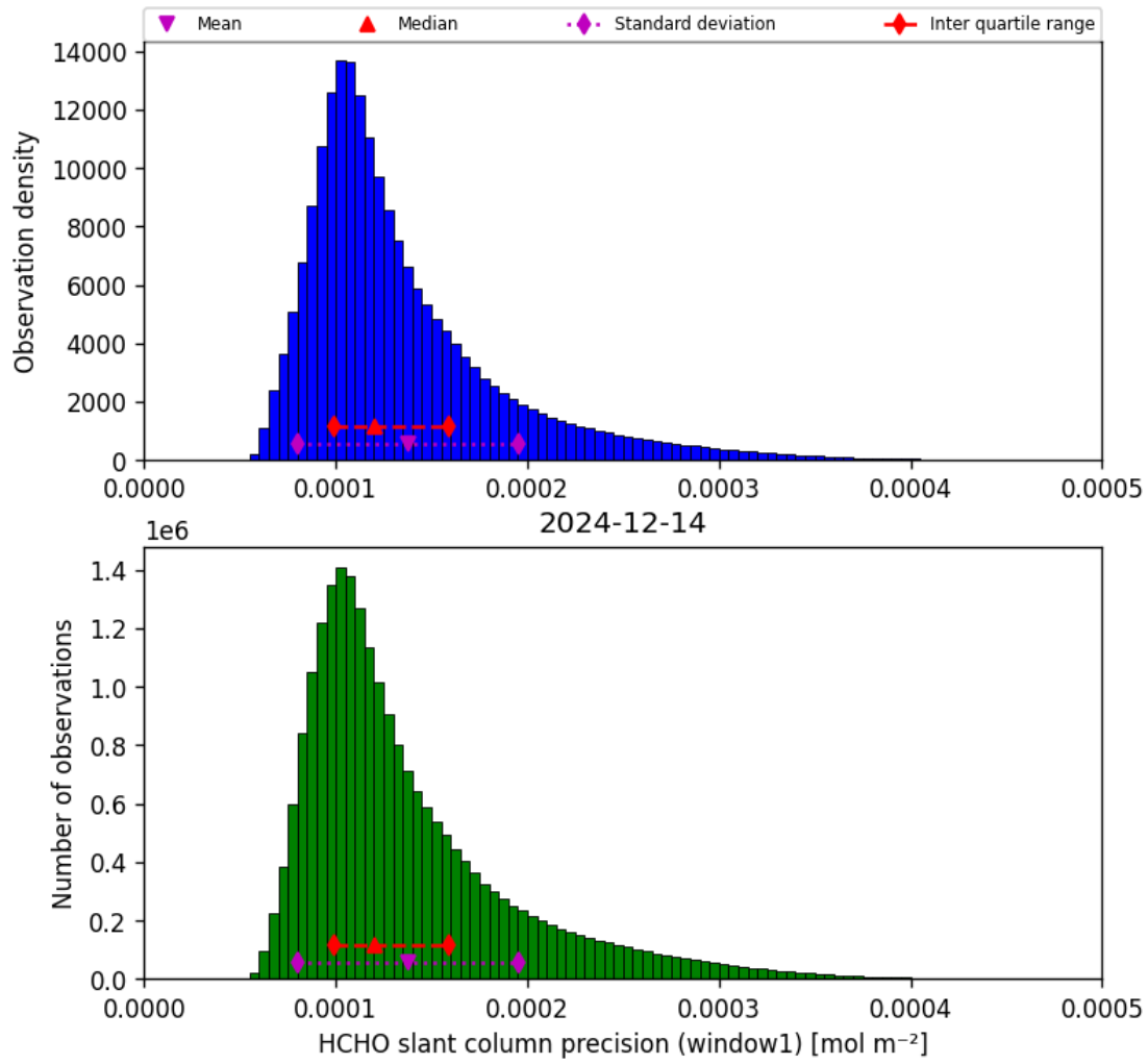
Figure 37: Histogram of “HCHO slant column precision (window1)” for 2024-12-14 to 2024-12-14
