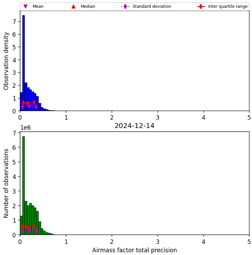
Figure 39: Histogram of “Airmass factor total precision” for 2024-12-14 to 2024-12-14
