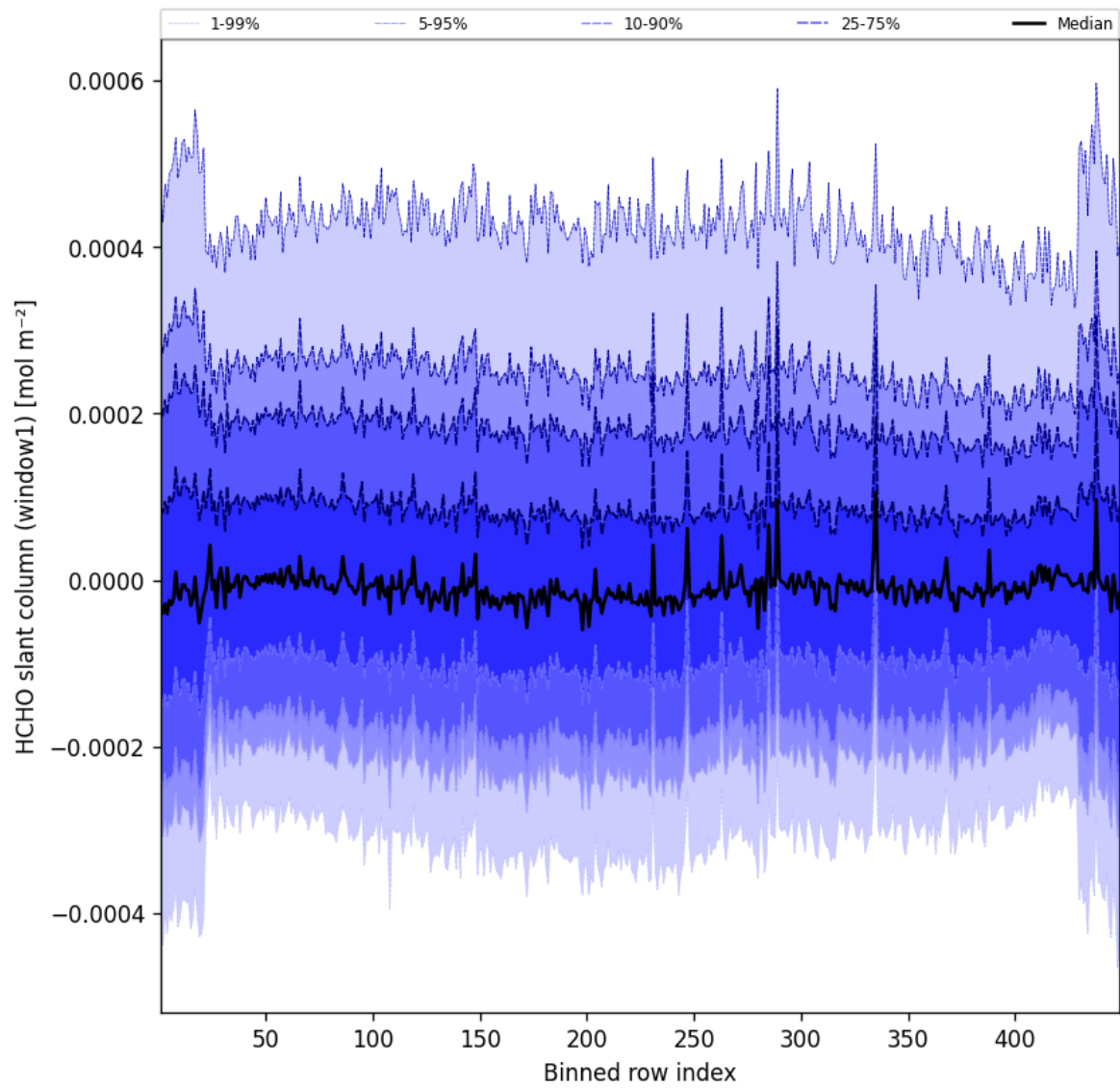
Figure 50: Along track statistics of “HCHO slant column (window1)” for 2024-12-14 to 2024-12-14
