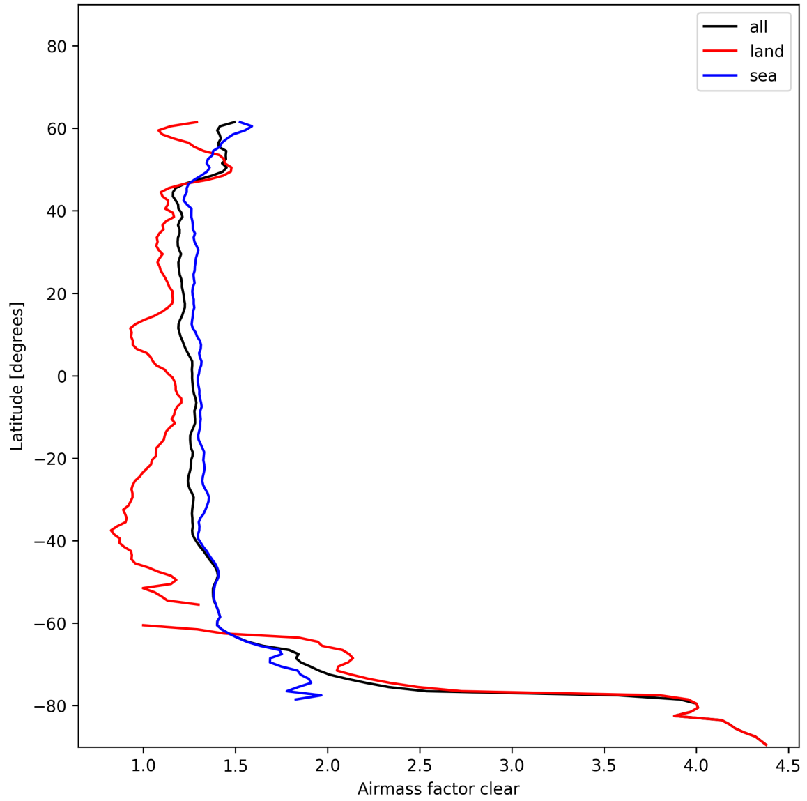
Figure 26: Zonal average of “Airmass factor clear” for 2024-12-14 to 2024-12-14.
