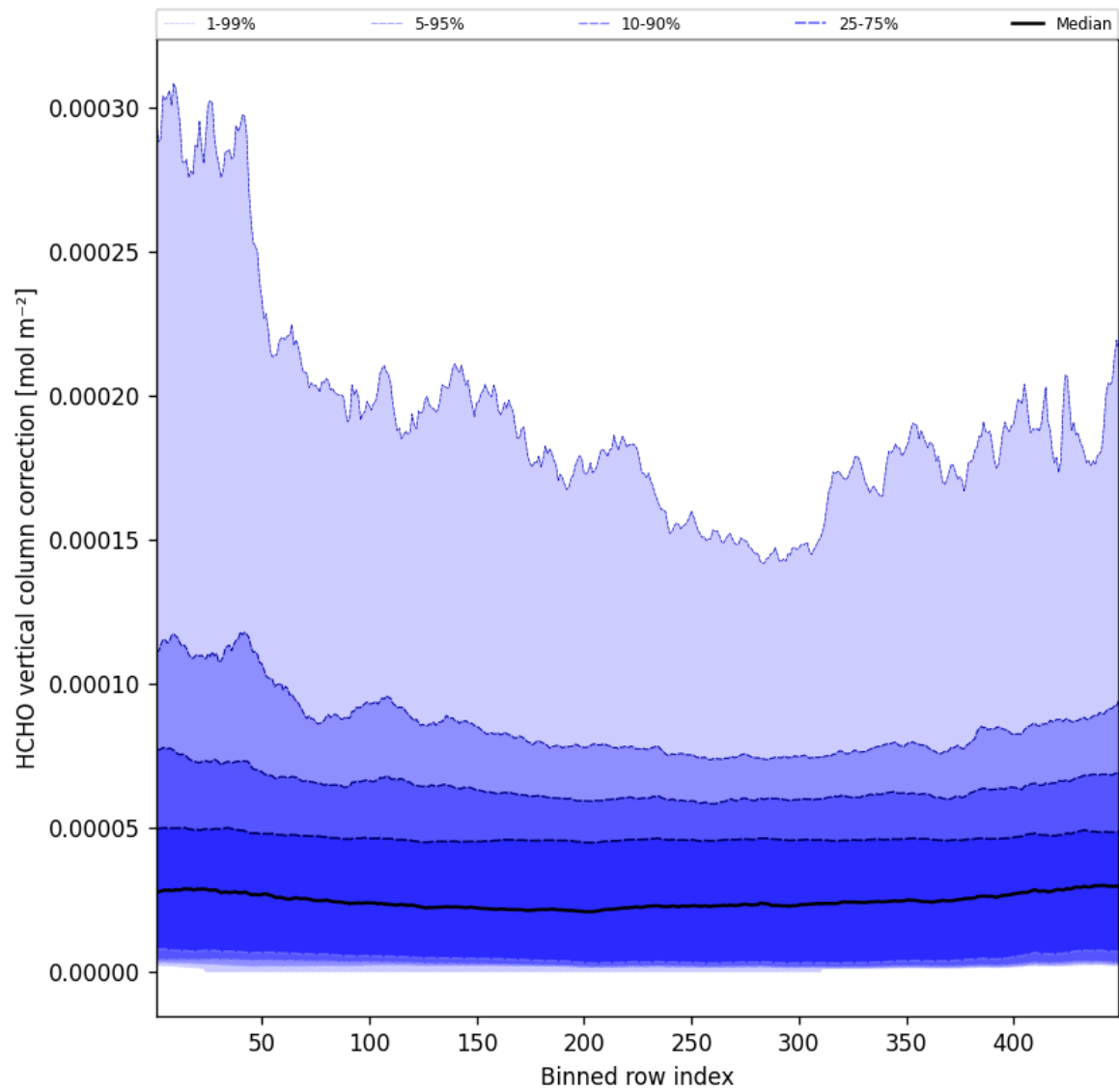
Figure 49: Along track statistics of “HCHO vertical column correction” for 2024-12-14 to 2024-12-14
