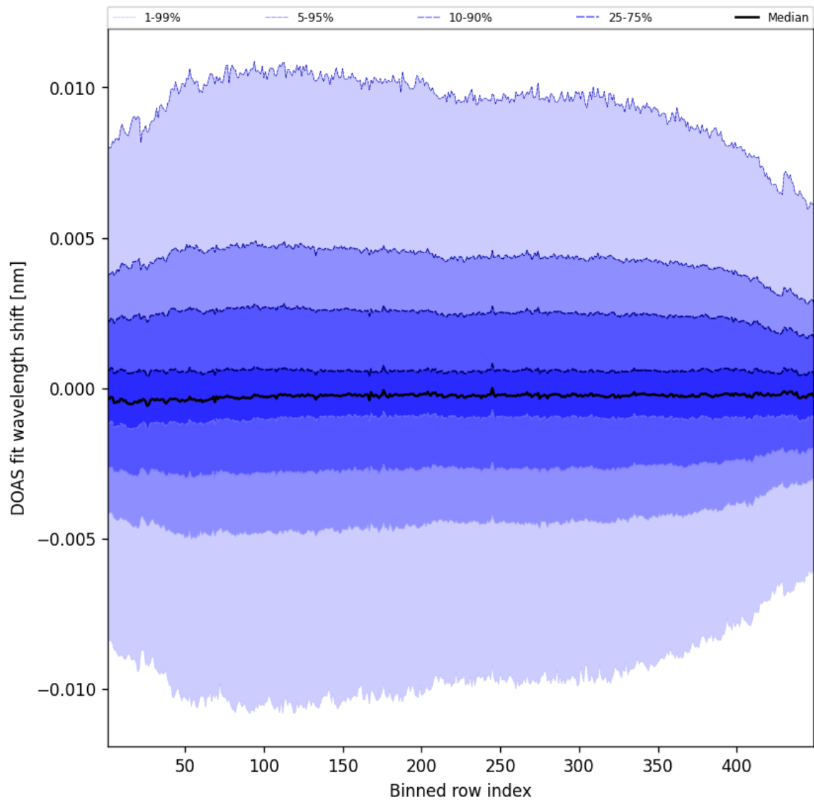
Figure 56: Along track statistics of “DOAS fit wavelength shift” for 2024-12-14 to 2024-12-14
