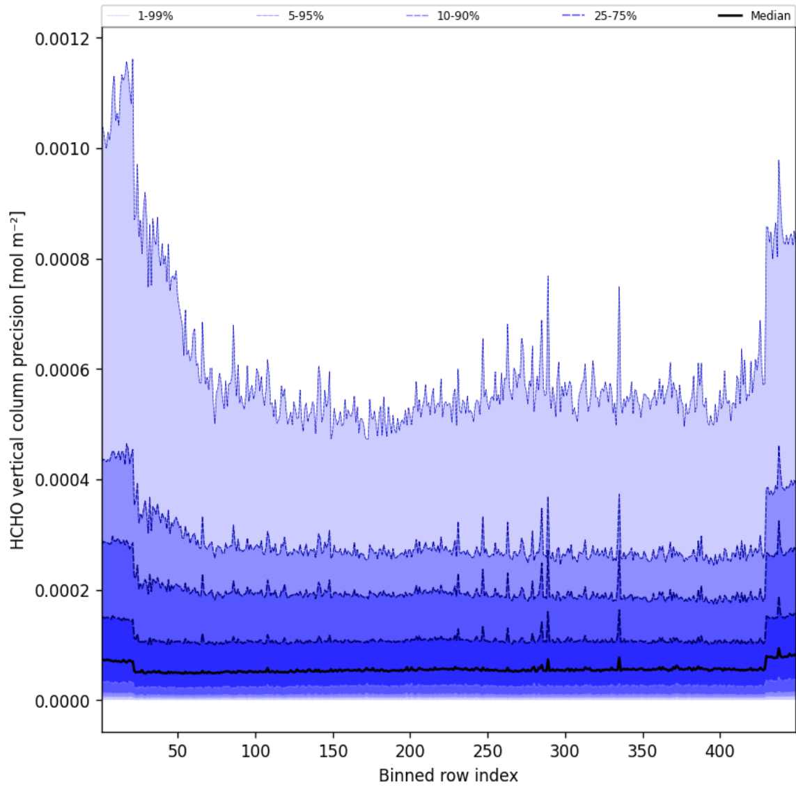
Figure 48: Along track statistics of “HCHO vertical column precision” for 2024-12-14 to 2024-12-14
