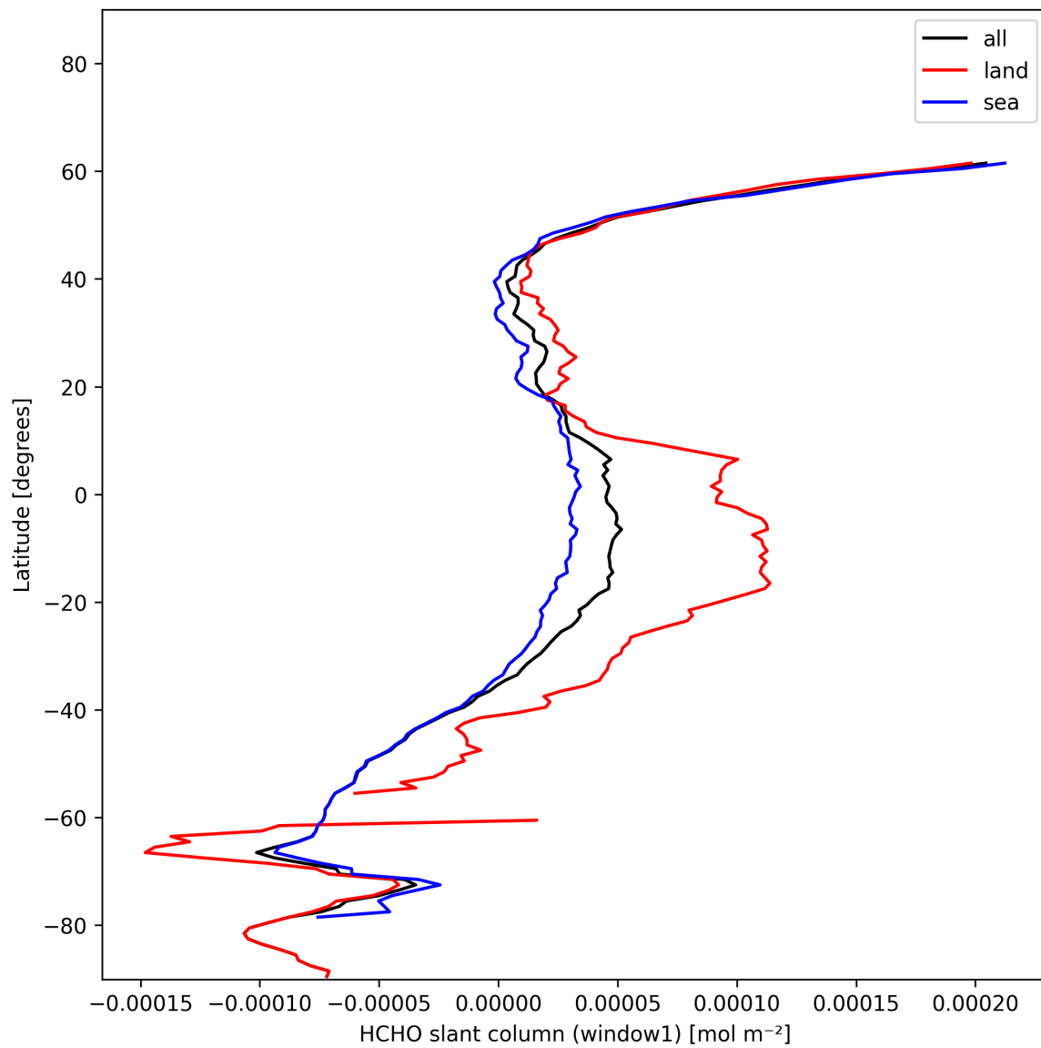
Figure 22: Zonal average of “HCHO slant column (window1)” for 2024-12-14 to 2024-12-14.
