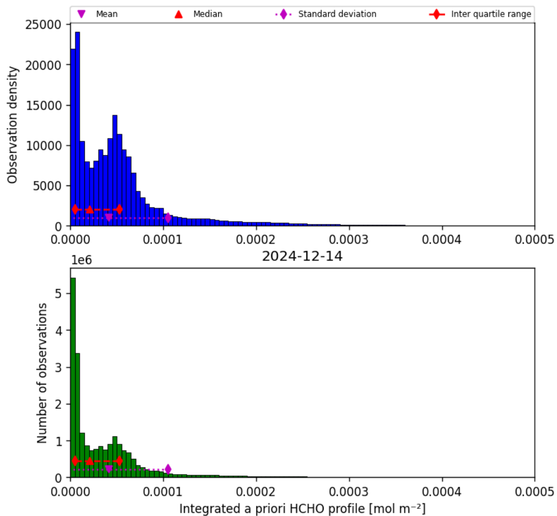
Figure 41: Histogram of “Integrated a priori HCHO profile” for 2024-12-14 to 2024-12-14
