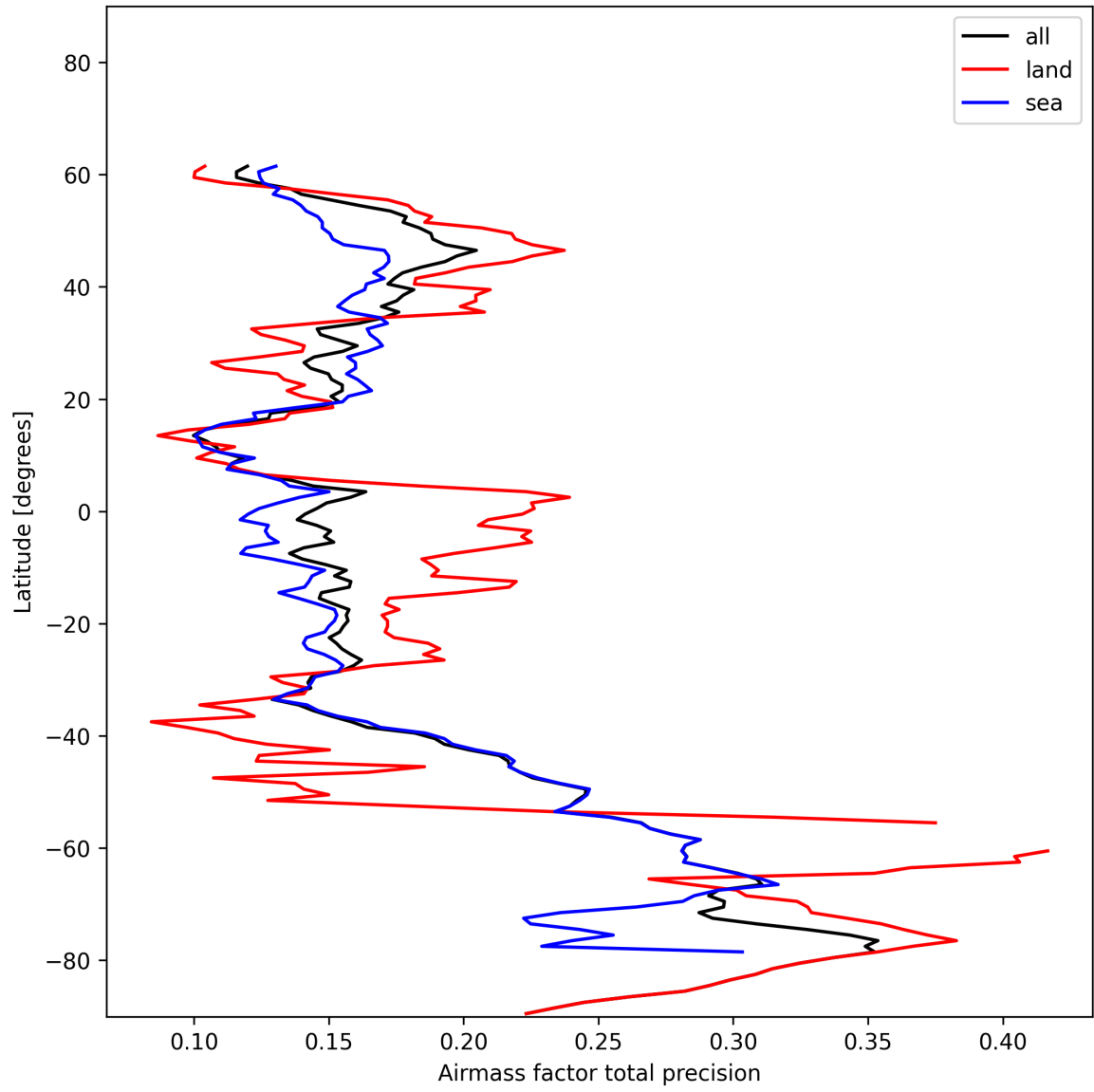
Figure 25: Zonal average of “Airmass factor total precision” for 2024-12-14 to 2024-12-14.
