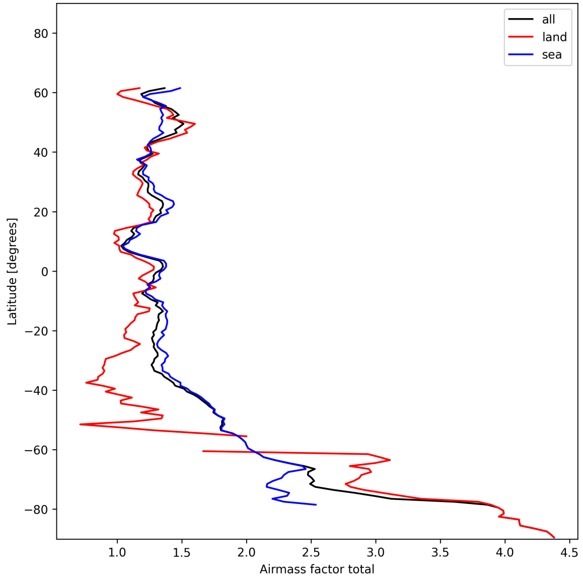
Figure 24: Zonal average of “Airmass factor total” for 2024-12-14 to 2024-12-14.
