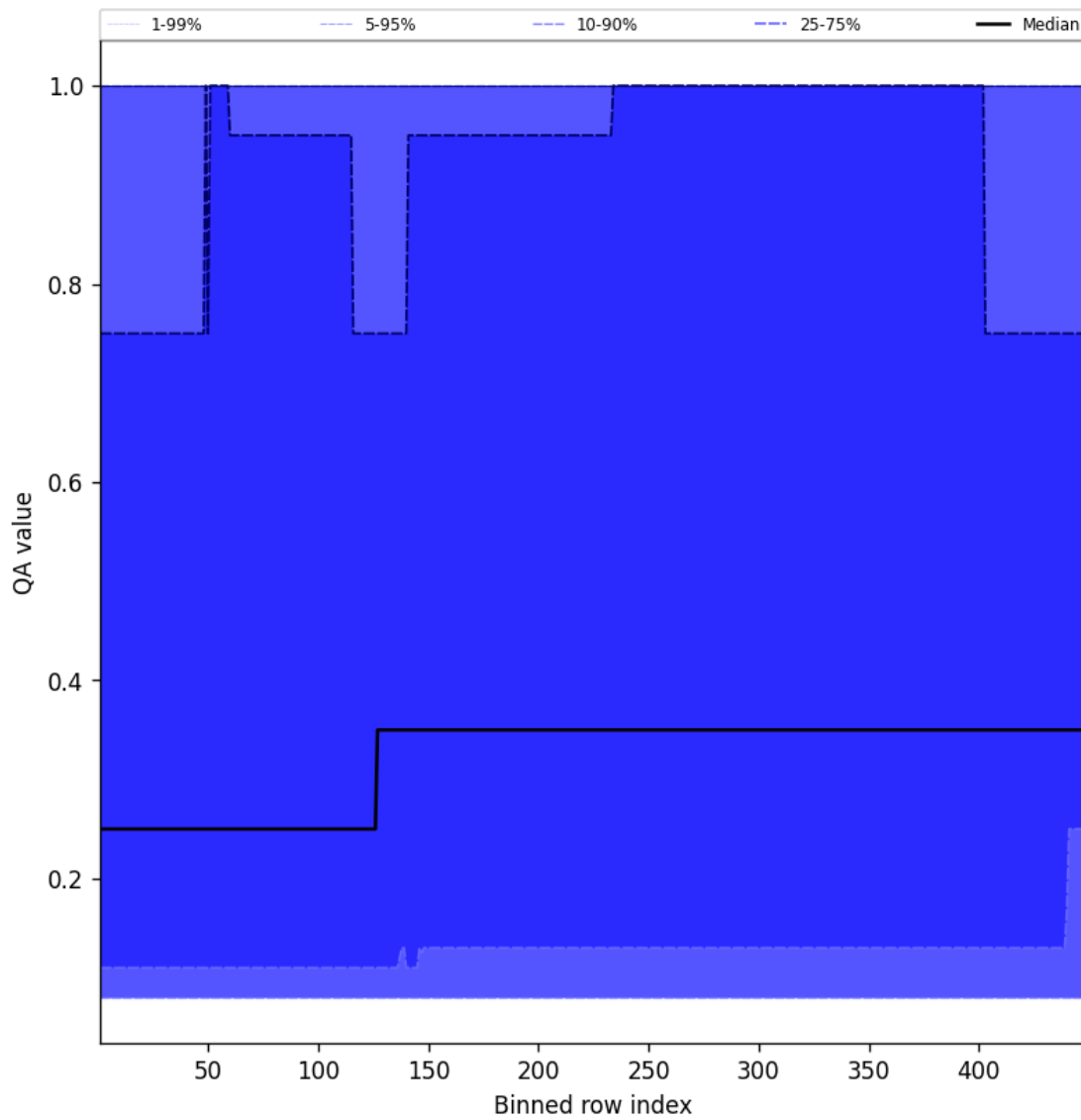
Figure 46: Along track statistics of “QA value” for 2024-12-14 to 2024-12-14
