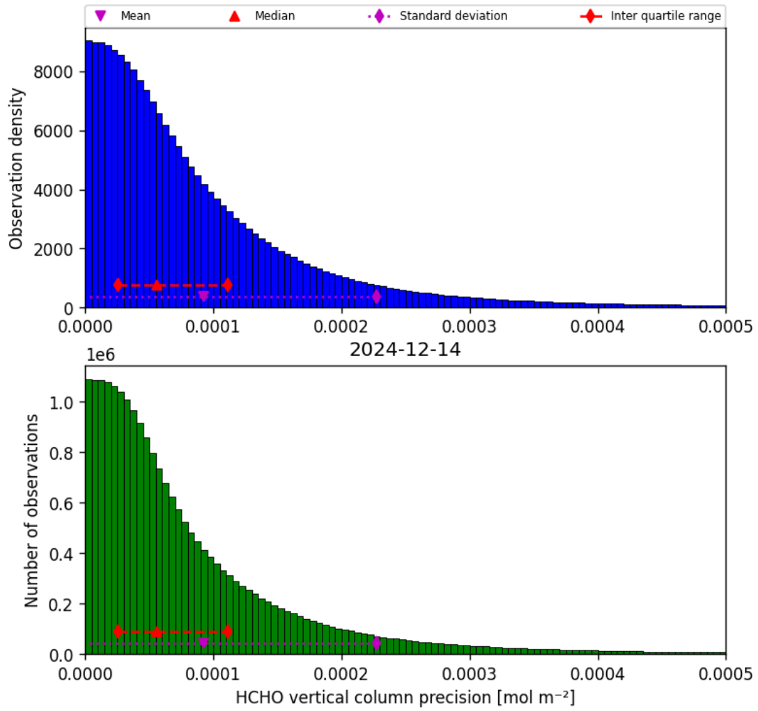
Figure 34: Histogram of “HCHO vertical column precision” for 2024-12-14 to 2024-12-14
