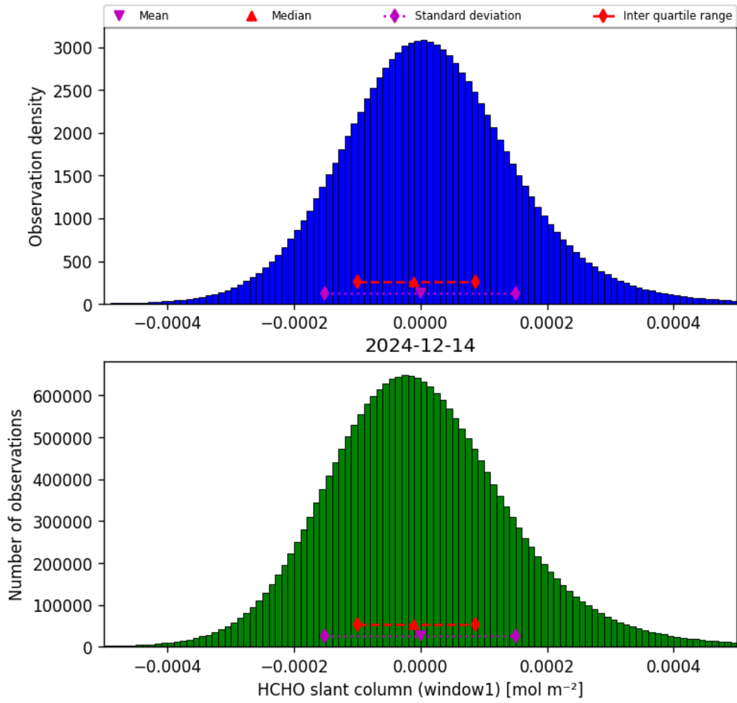
Figure 36: Histogram of “HCHO slant column (window1)” for 2024-12-14 to 2024-12-14
