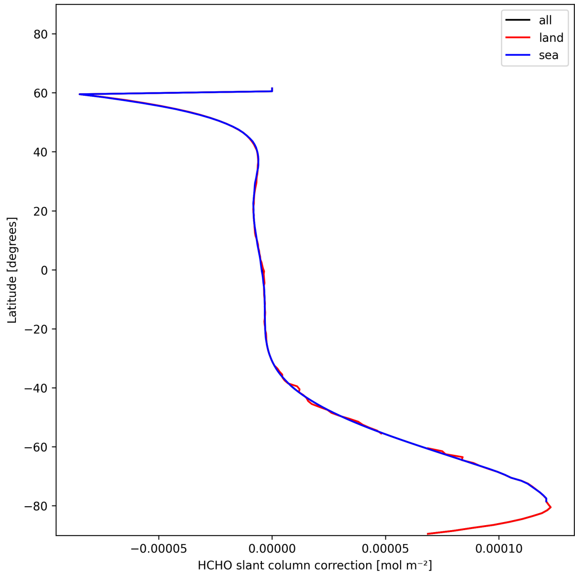
Figure 31: Zonal average of “HCHO slant column correction” for 2024-12-14 to 2024-12-14.
