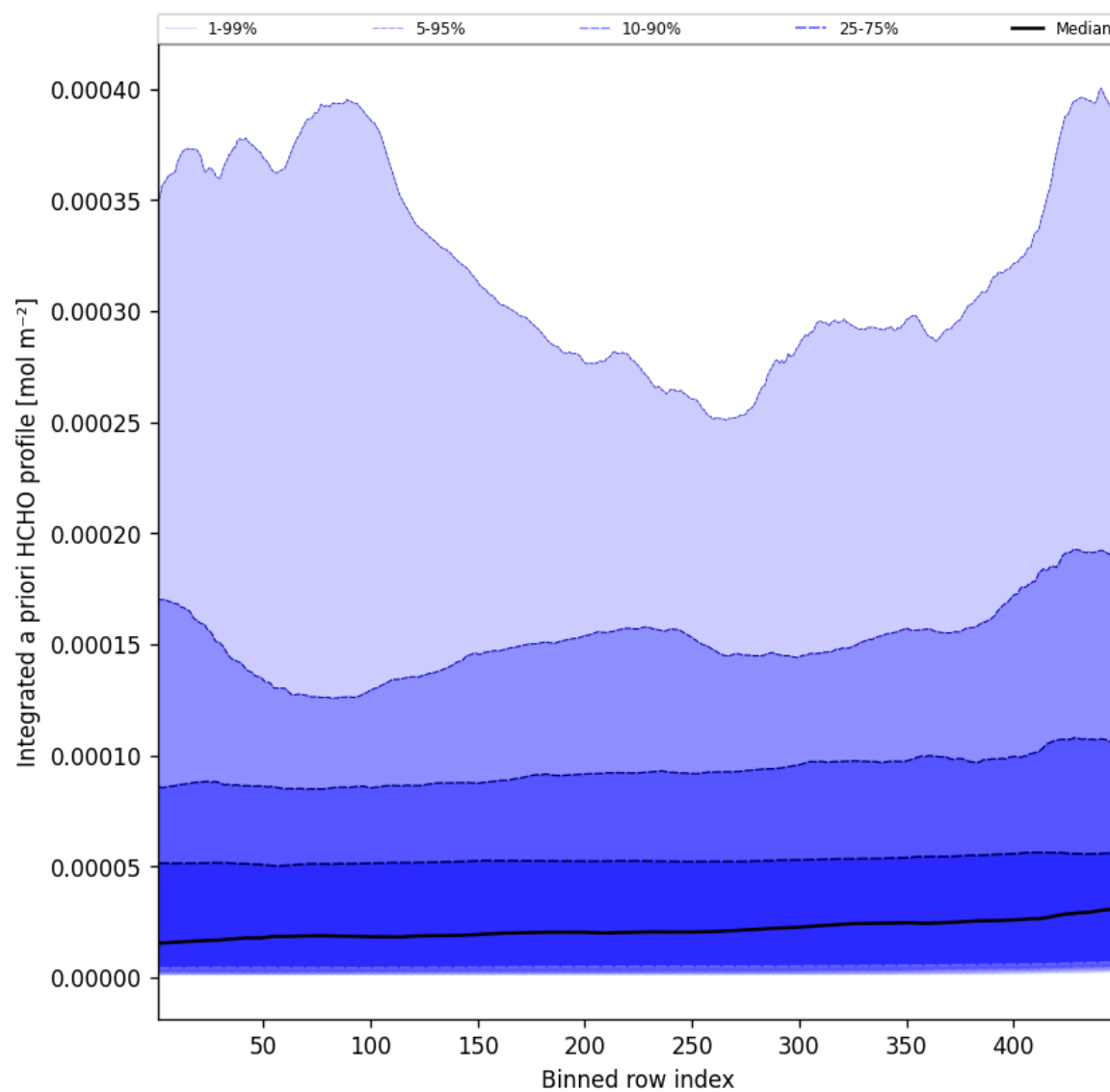
Figure 55: Along track statistics of “Integrated a priori HCHO profile” for 2024-12-14 to 2024-12-14
