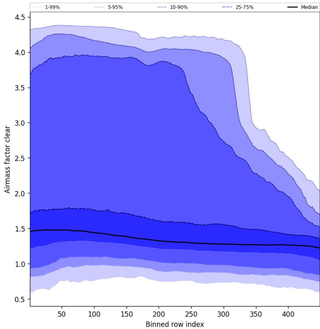
Figure 54: Along track statistics of “Air mass factor clear” for 2024-12-14 to 2024-12-14
