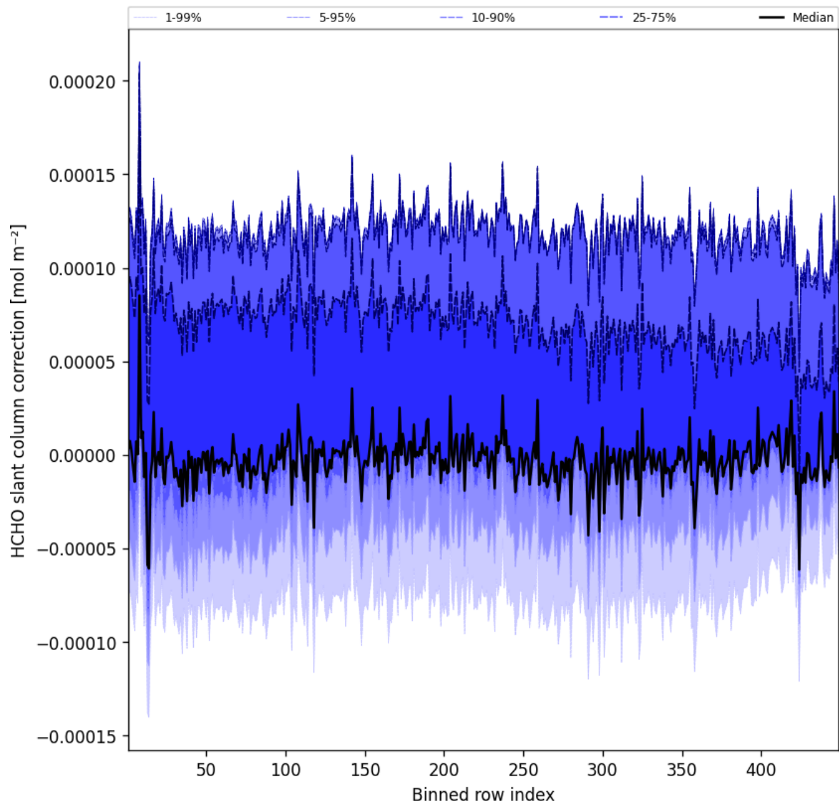
Figure 59: Along track statistics of “HCHO slant column correction” for 2024-12-14 to 2024-12-14
