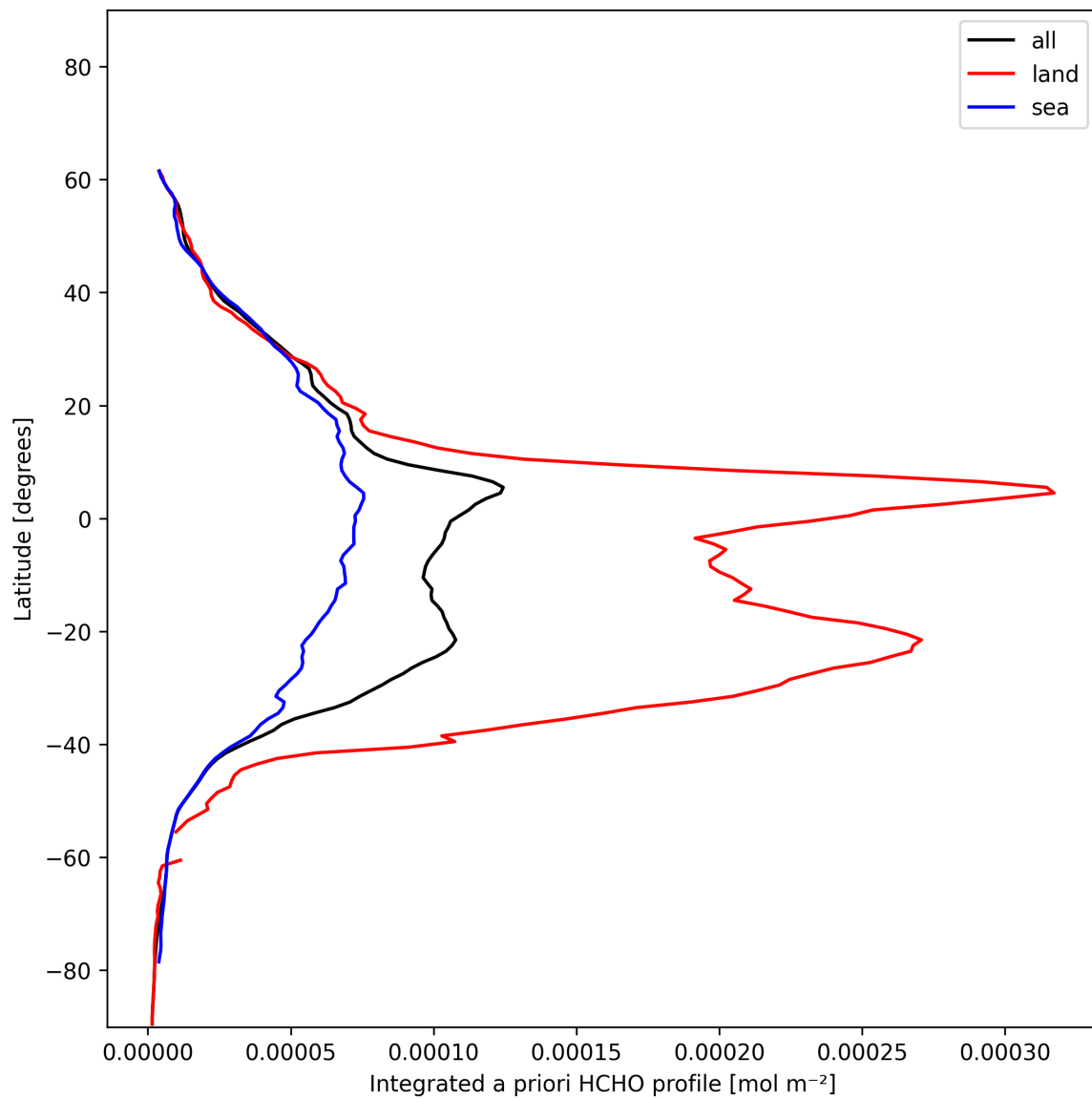
Figure 27: Zonal average of “Integrated a priori HCHO profile” for 2024-12-14 to 2024-12-14.
