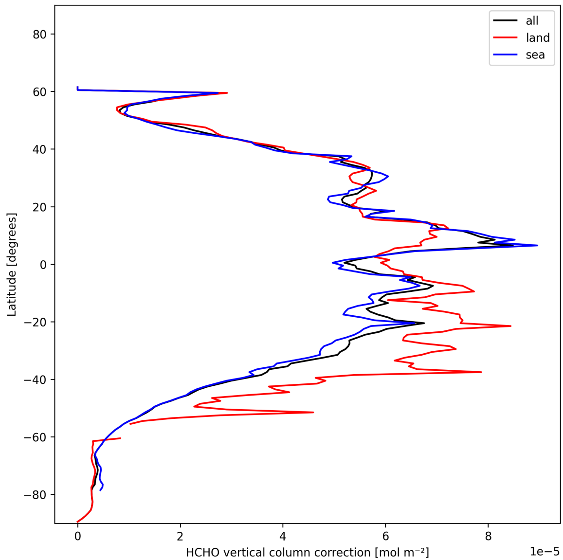
Figure 21: Zonal average of “HCHO vertical column correction” for 2024-12-14 to 2024-12-14.
