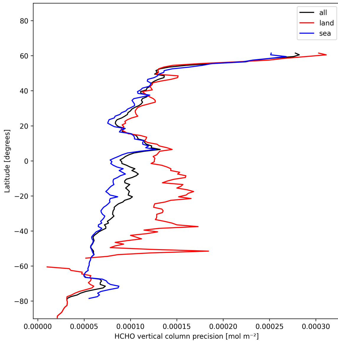
Figure 20: Zonal average of “HCHO vertical column precision” for 2024-12-14 to 2024-12-14.
