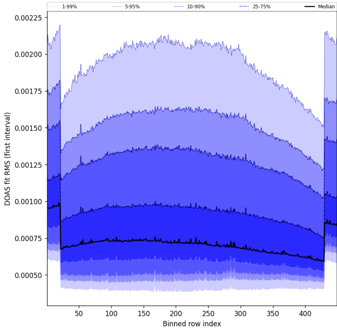
Figure 58: Along track statistics of “DOAS fit RMS (first interval)” for 2024-12-14 to 2024-12-14
