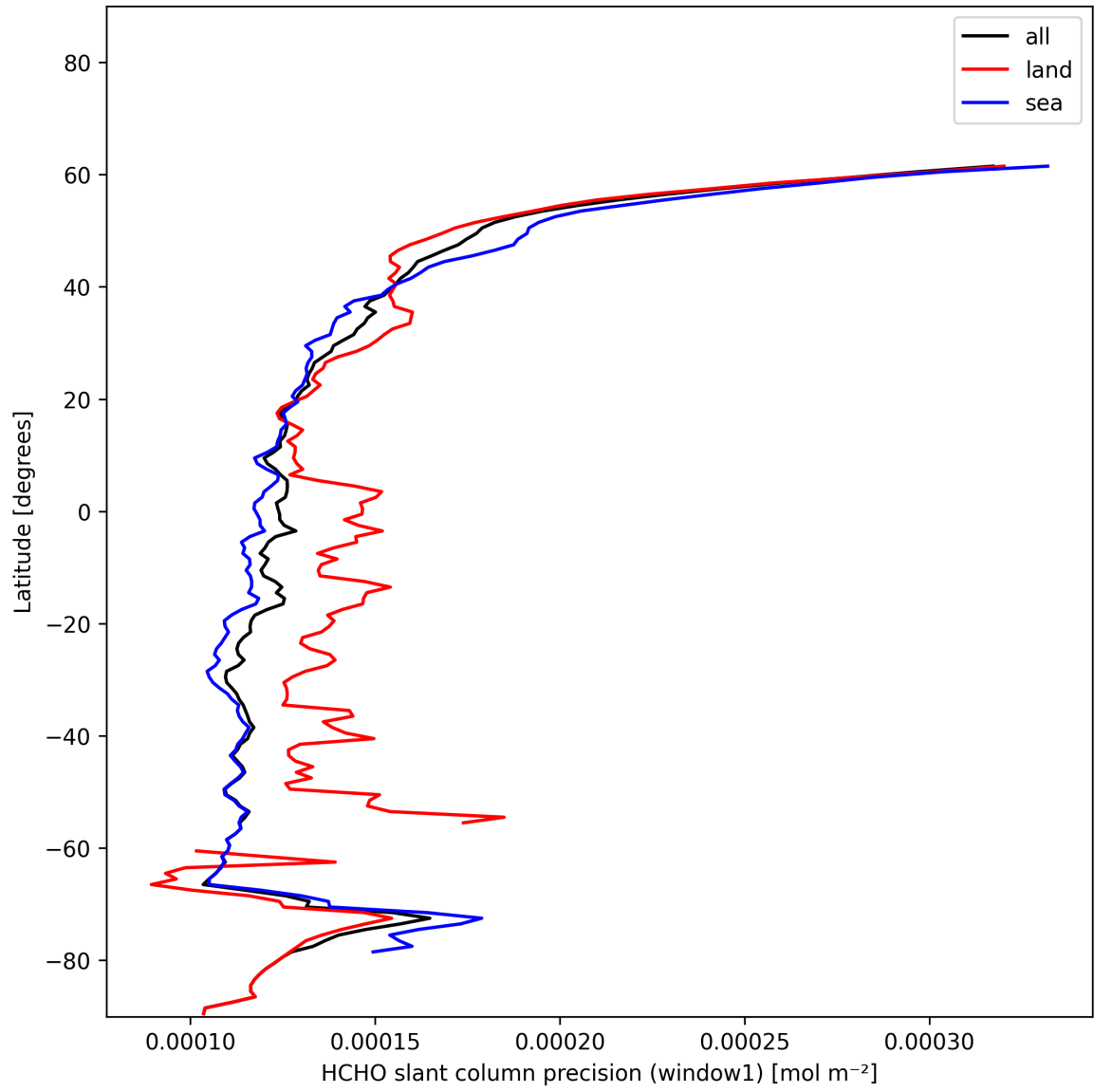
Figure 23: Zonal average of “HCHO slant column precision (window1)” for 2024-12-14 to 2024-12-14.
