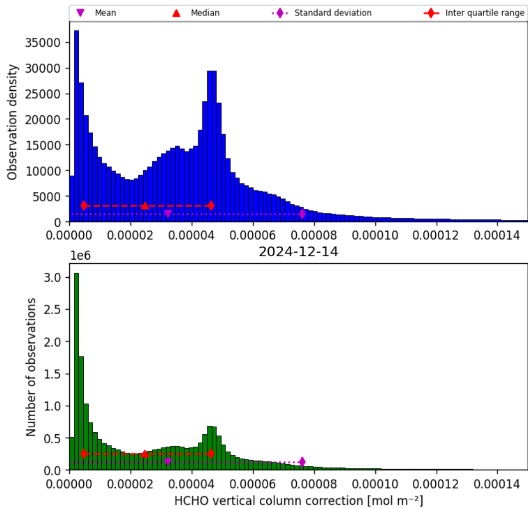
Figure 35: Histogram of “HCHO vertical column correction” for 2024-12-14 to 2024-12-14
