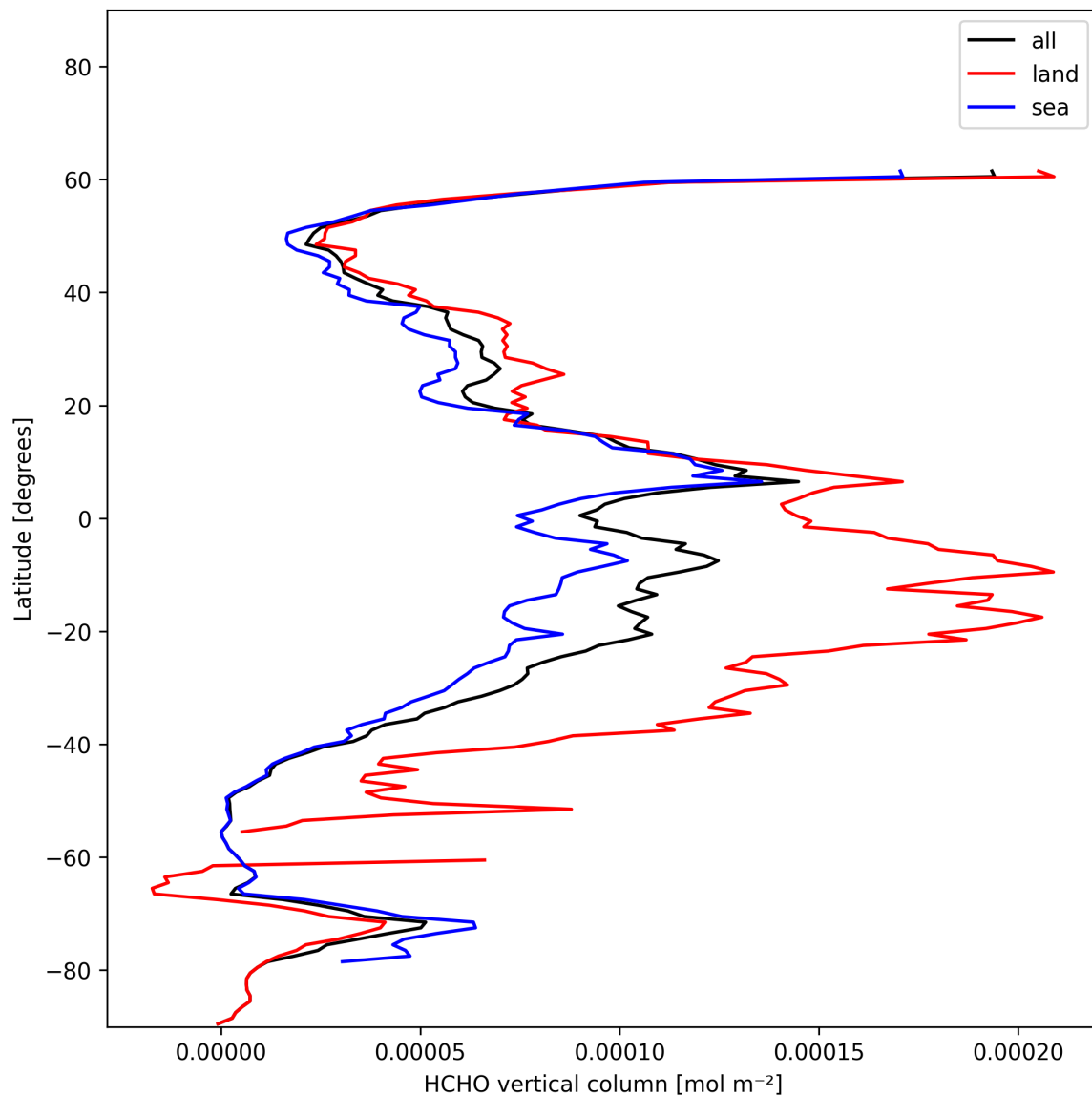
Figure 19: Zonal average of “HCHO vertical column” for 2024-12-14 to 2024-12-14.
