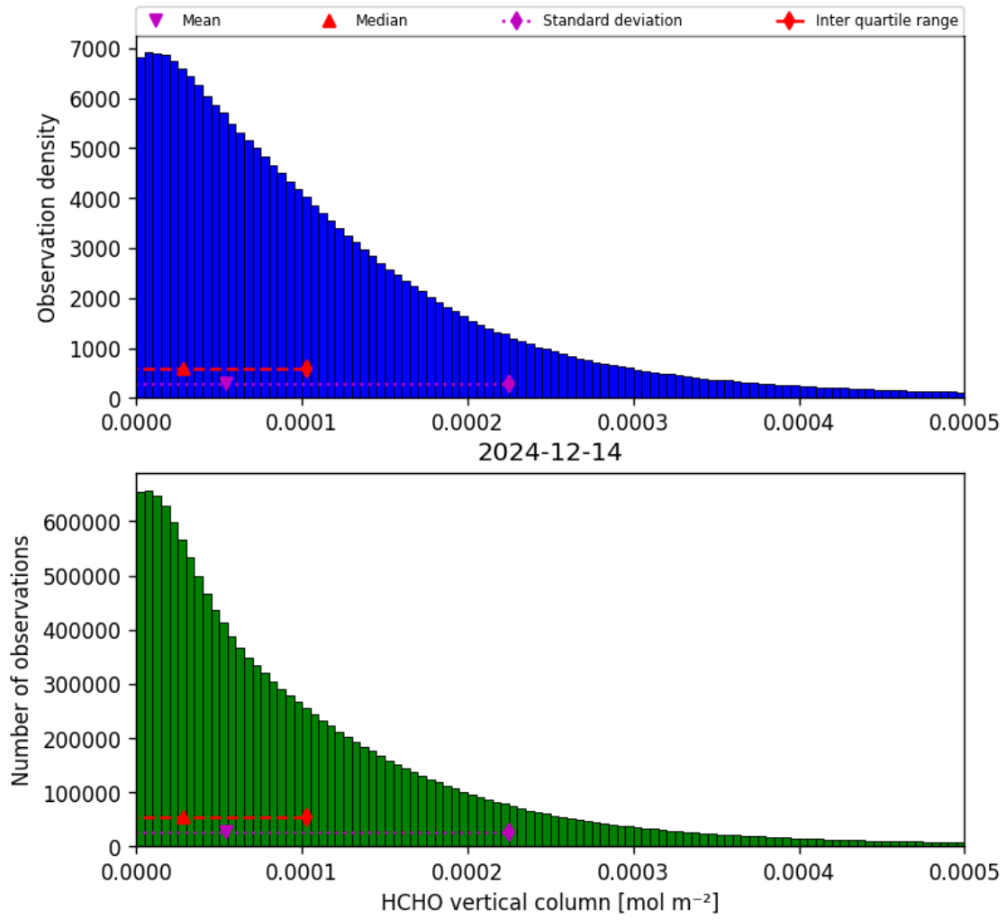
Figure 33: Histogram of “HCHO vertical column” for 2024-12-14 to 2024-12-14
