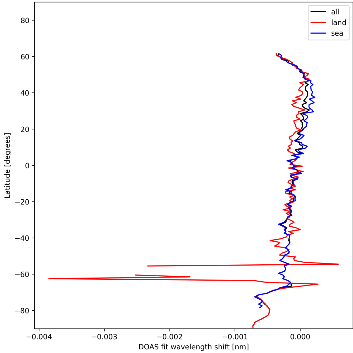
Figure 28: Zonal average of “DOAS fit wavelength shift” for 2024-12-14 to 2024-12-14.
