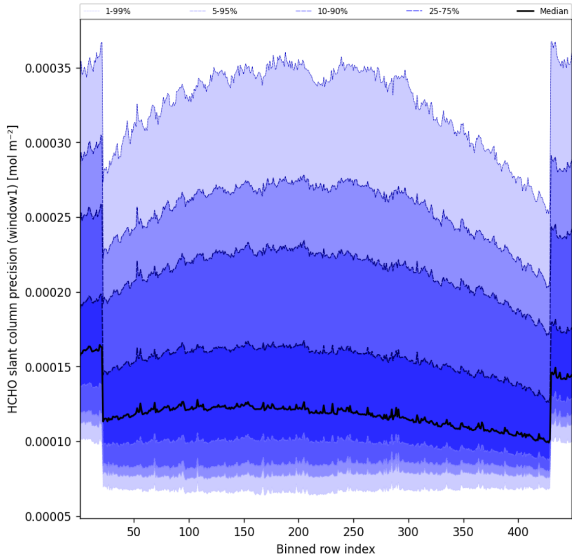
Figure 51: Along track statistics of “HCHO slant column precision (window1)” for 2024-12-14 to 2024-12-14
