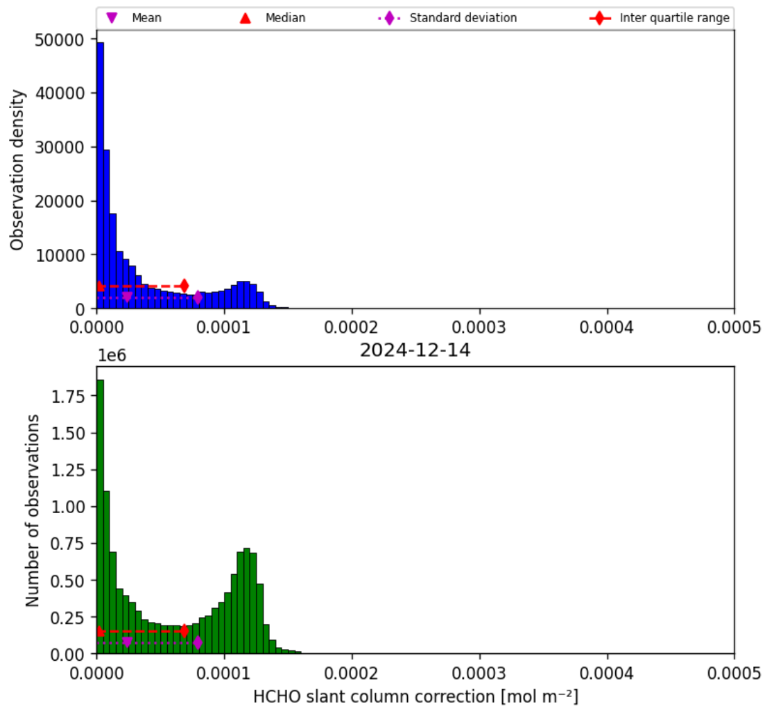
Figure 45: Histogram of “HCHO slant column correction” for 2024-12-14 to 2024-12-14
