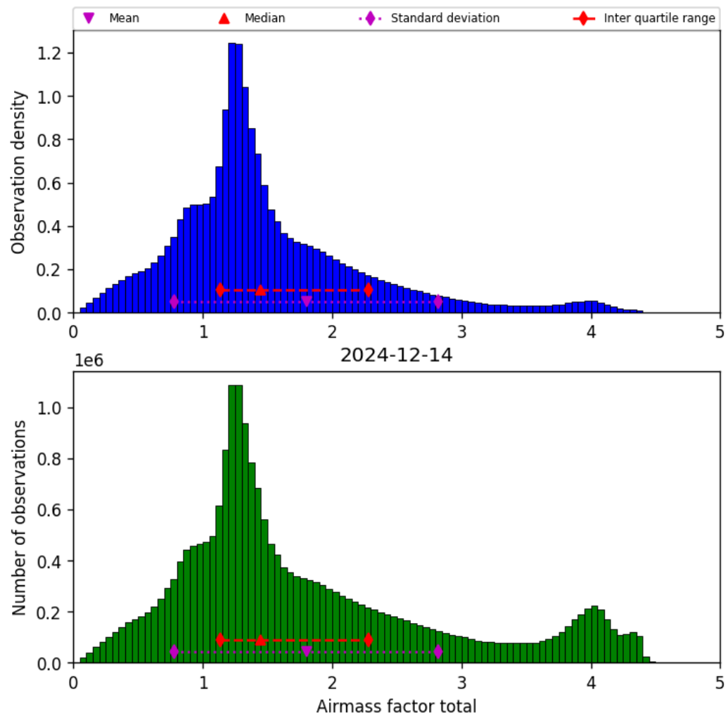
Figure 38: Histogram of “Airmass factor total” for 2024-12-14 to 2024-12-14
