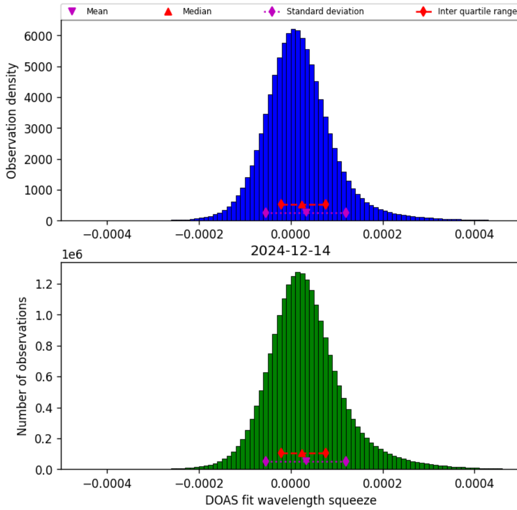
Figure 43: Histogram of “DOAS fit wavelength squeeze” for 2024-12-14 to 2024-12-14
