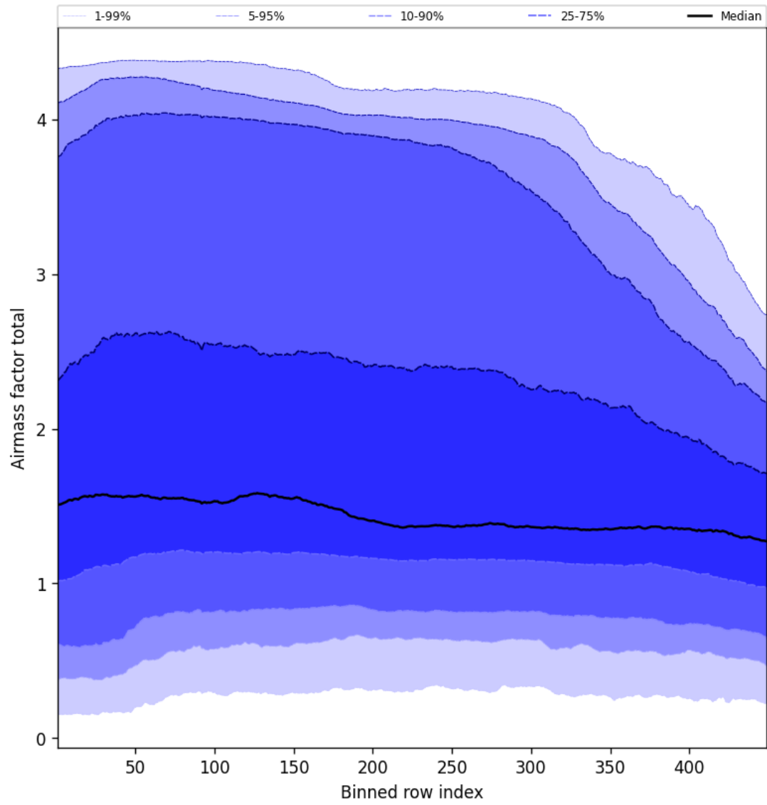
Figure 52: Along track statistics of “Airmass factor total” for 2024-12-14 to 2024-12-14
