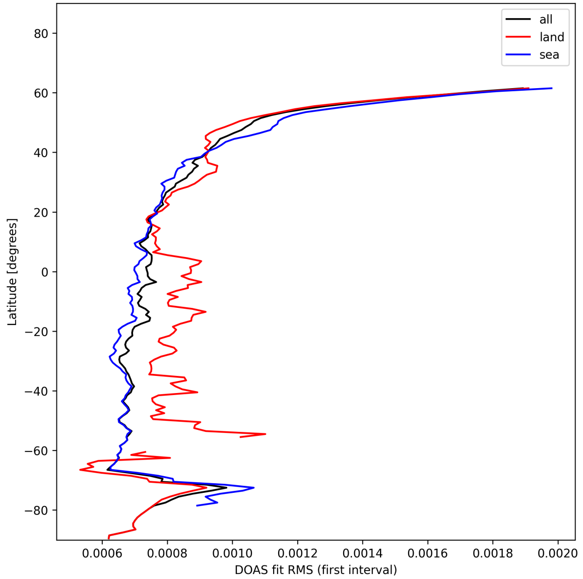
Figure 30: Zonal average of “DOAS fit RMS (first interval)” for 2024-12-14 to 2024-12-14.
