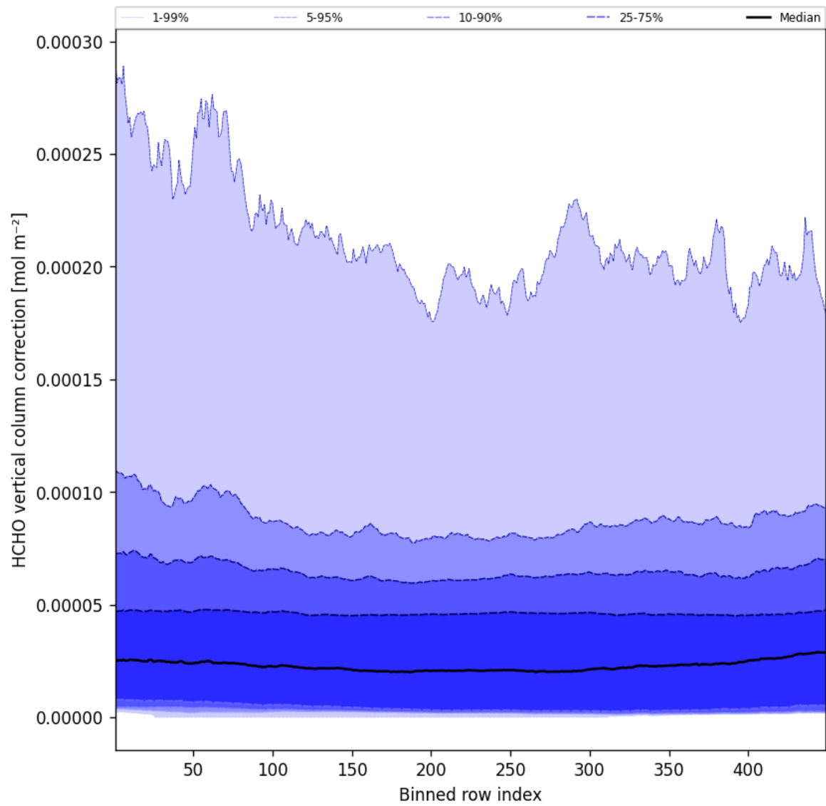
Figure 49: Along track statistics of “HCHO vertical column correction” for 2024-12-16 to 2024-12-17
