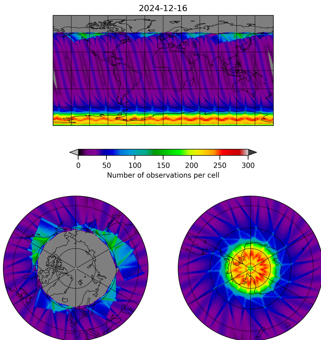
Figure 17: Map of the number of observations for 2024-12-16 to 2024-12-17
