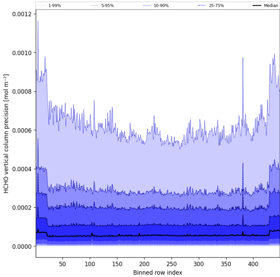
Figure 48: Along track statistics of “HCHO vertical column precision” for 2024-12-16 to 2024-12-17
