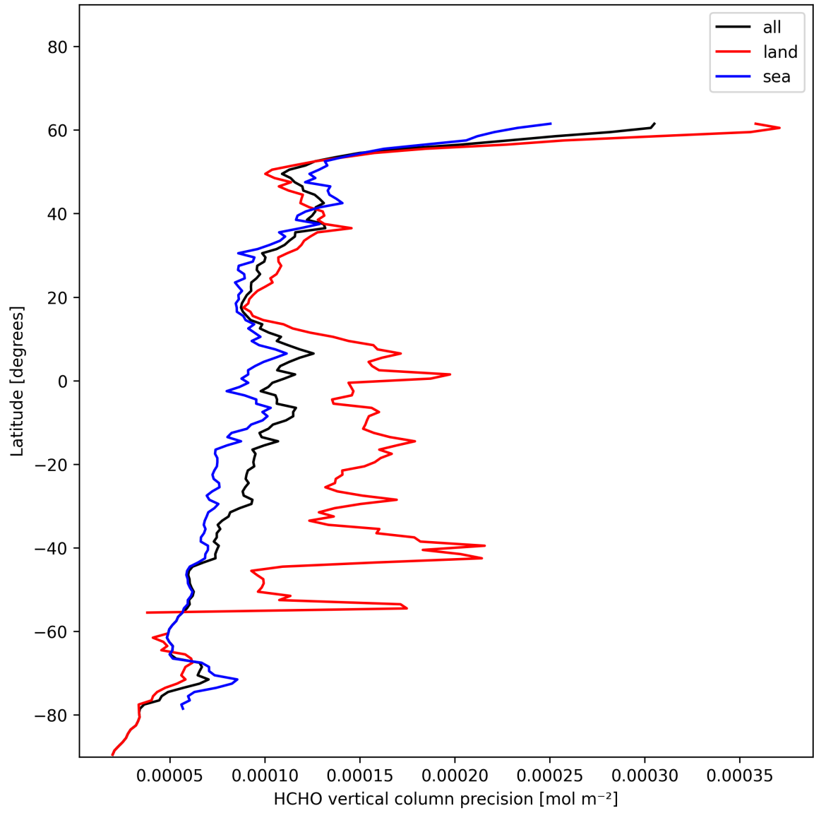
Figure 20: Zonal average of “HCHO vertical column precision” for 2024-12-16 to 2024-12-17.
