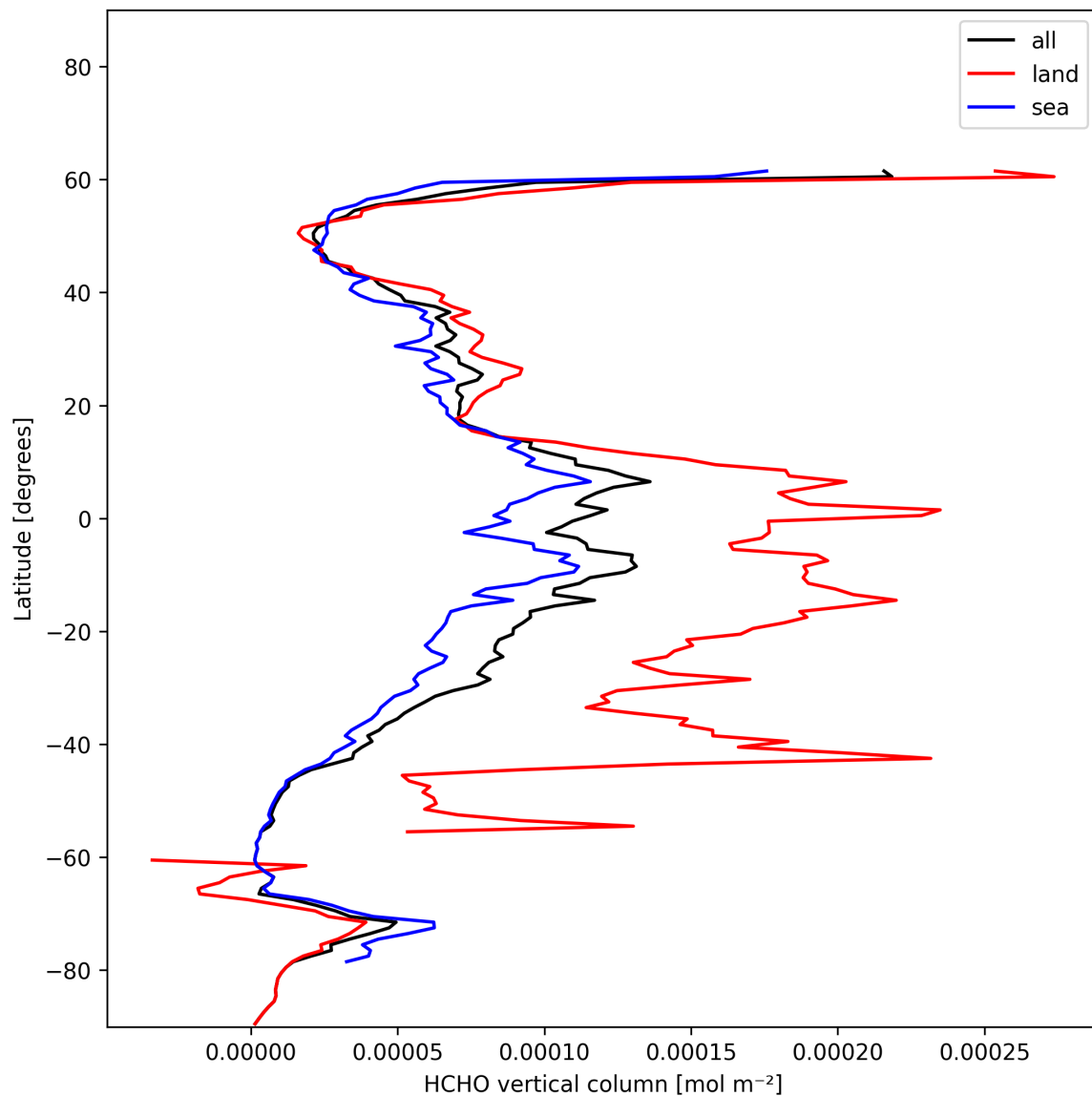
Figure 19: Zonal average of “HCHO vertical column” for 2024-12-16 to 2024-12-17.
