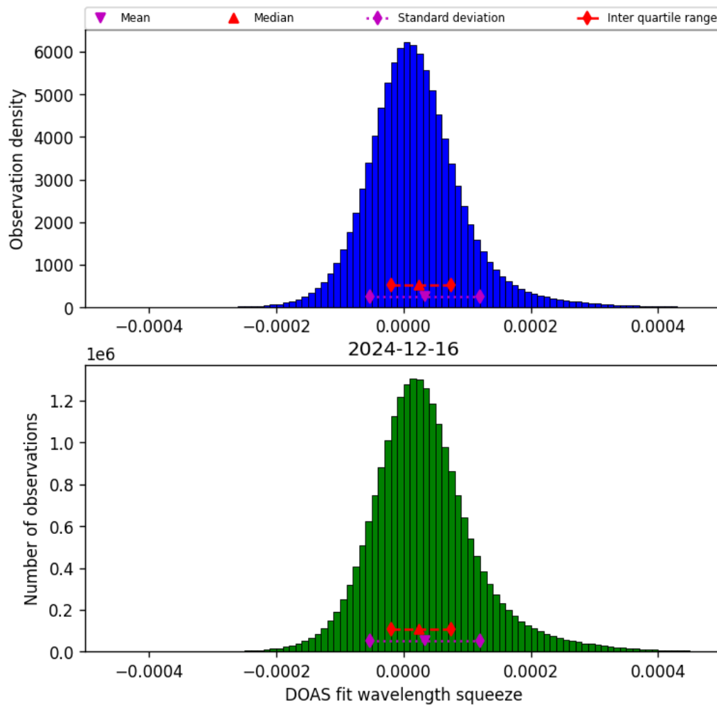
Figure 43: Histogram of “DOAS fit wavelength squeeze” for 2024-12-16 to 2024-12-17
