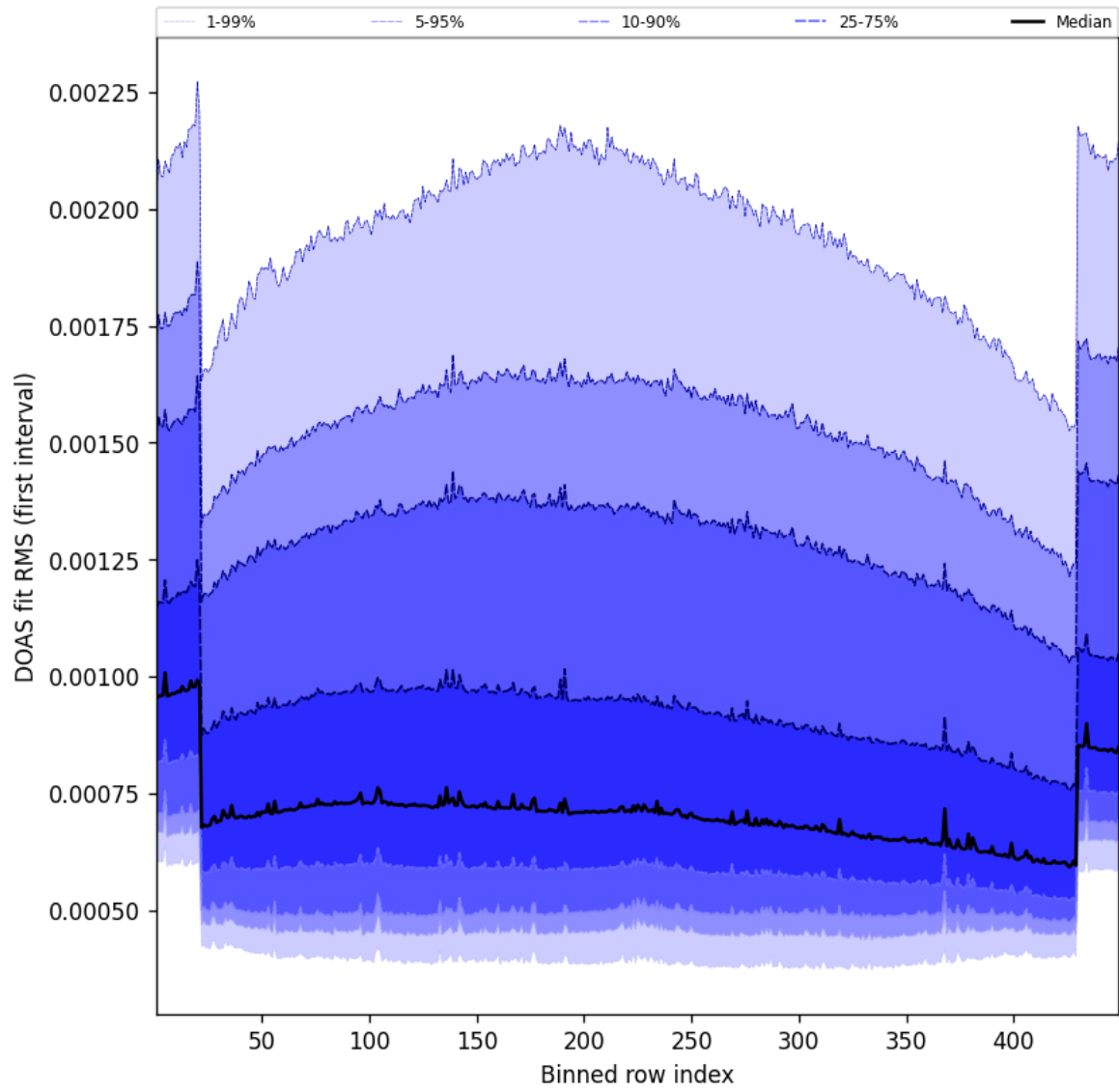
Figure 58: Along track statistics of “DOAS fit RMS (first interval)” for 2024-12-16 to 2024-12-17
