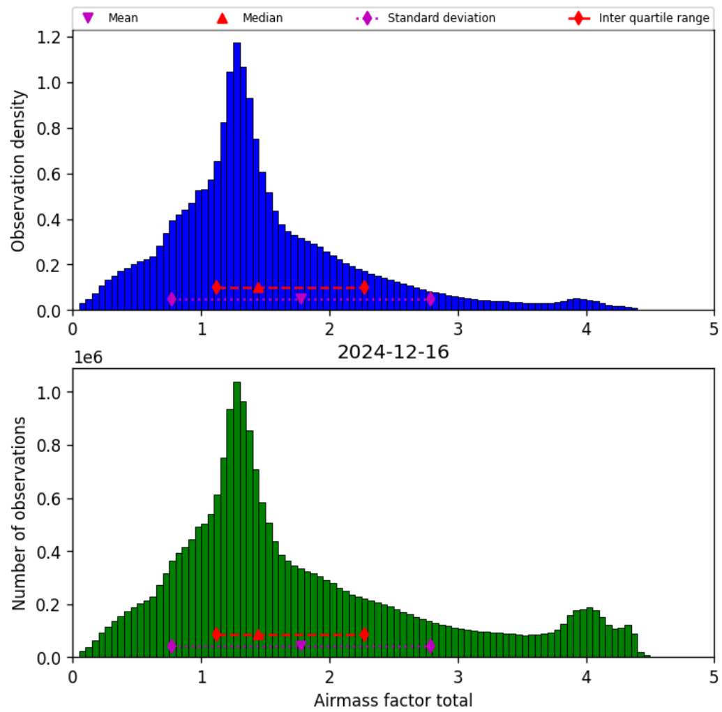
Figure 38: Histogram of “Airmass factor total” for 2024-12-16 to 2024-12-17
