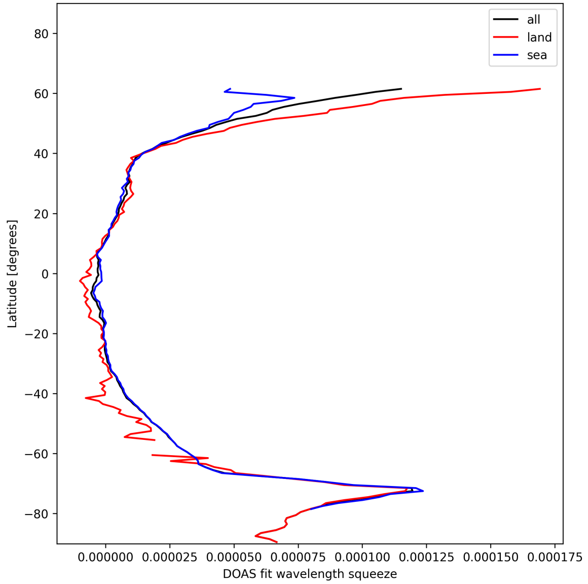
Figure 29: Zonal average of “DOAS fit wavelength squeeze” for 2024-12-16 to 2024-12-17.
