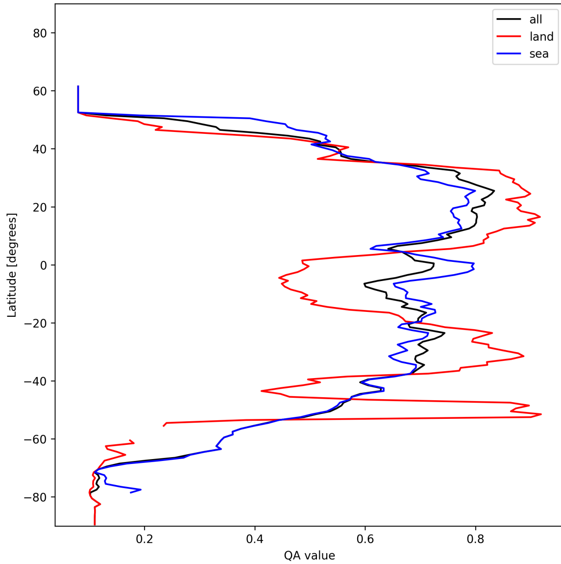
Figure 18: Zonal average of “QA value” for 2024-12-16 to 2024-12-17.
