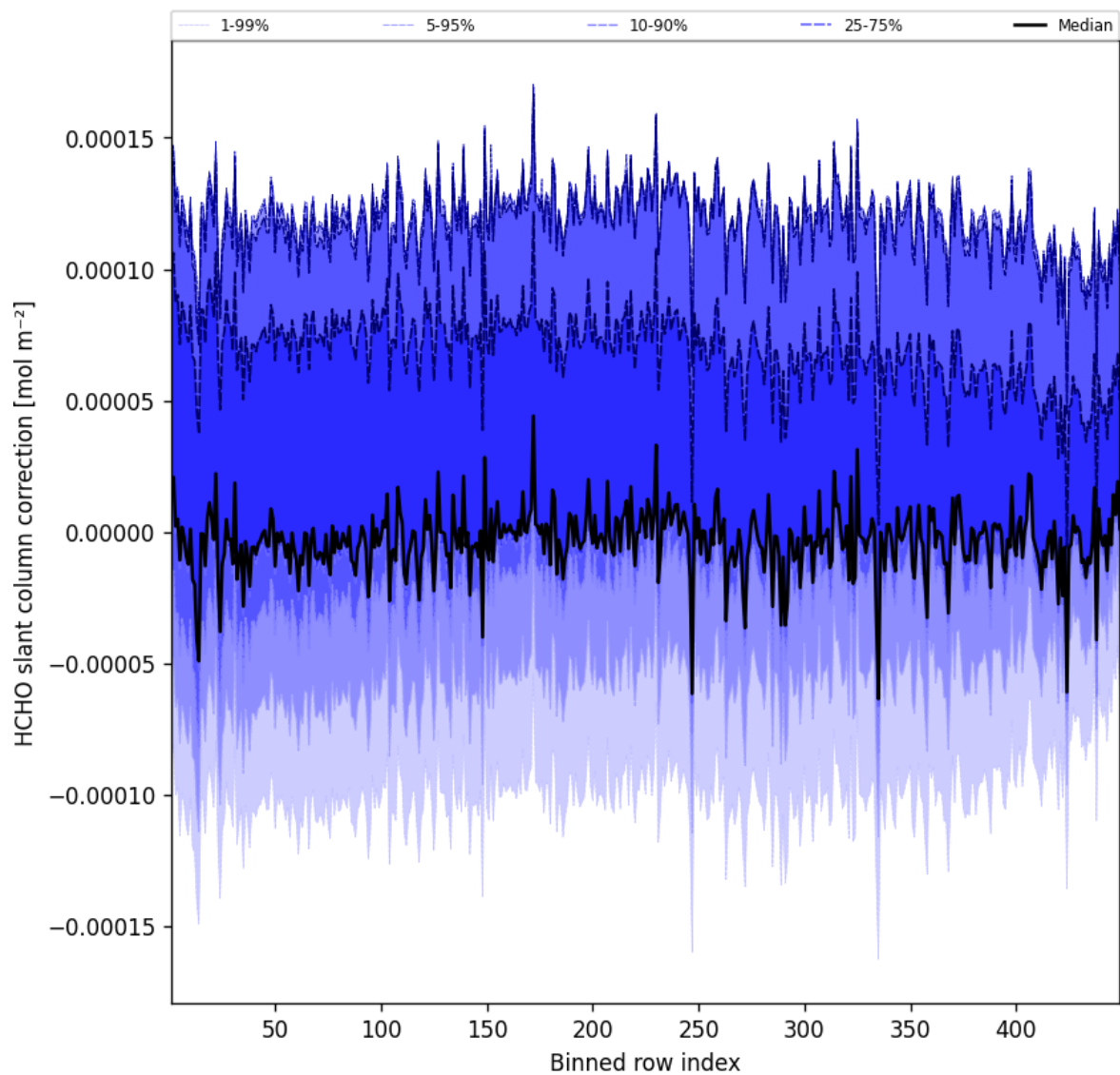
Figure 59: Along track statistics of “HCHO slant column correction” for 2024-12-16 to 2024-12-17
