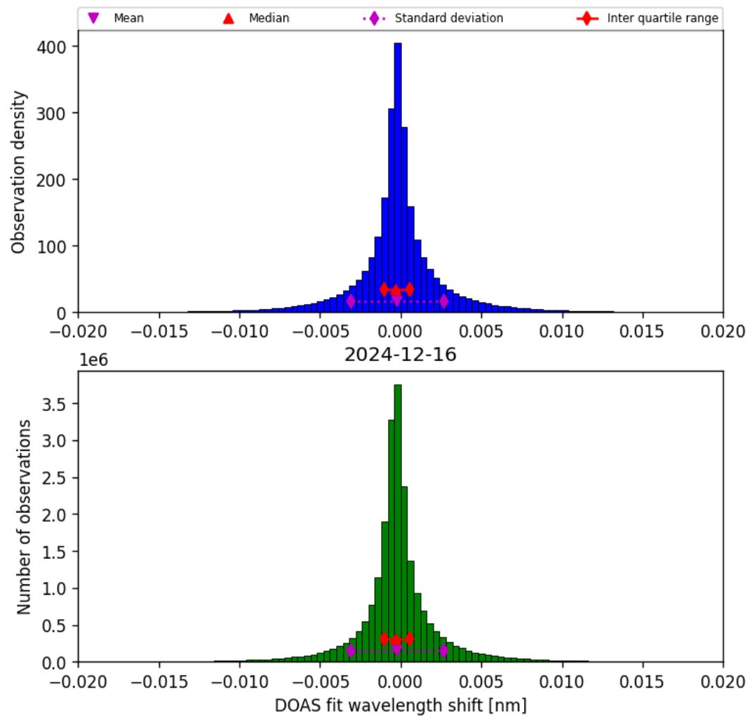
Figure 42: Histogram of “DOAS fit wavelength shift” for 2024-12-16 to 2024-12-17
