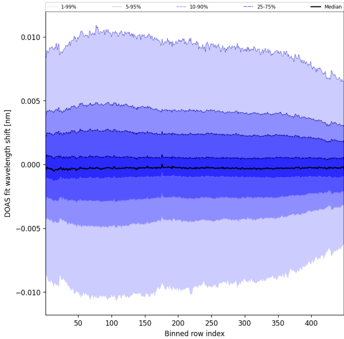
Figure 56: Along track statistics of “DOAS fit wavelength shift” for 2024-12-16 to 2024-12-17
