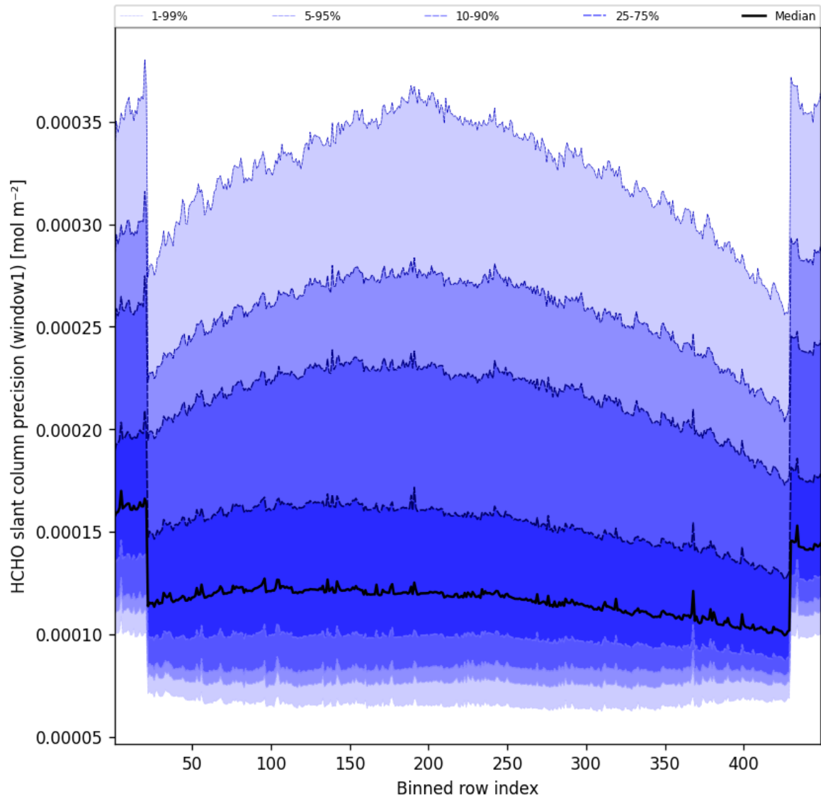
Figure 51: Along track statistics of “HCHO slant column precision (window1)” for 2024-12-16 to 2024-12-17
