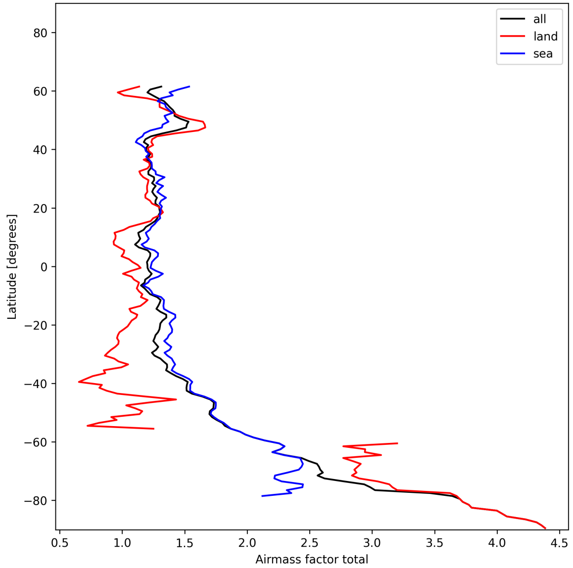
Figure 24: Zonal average of “Airmass factor total” for 2024-12-16 to 2024-12-17.
