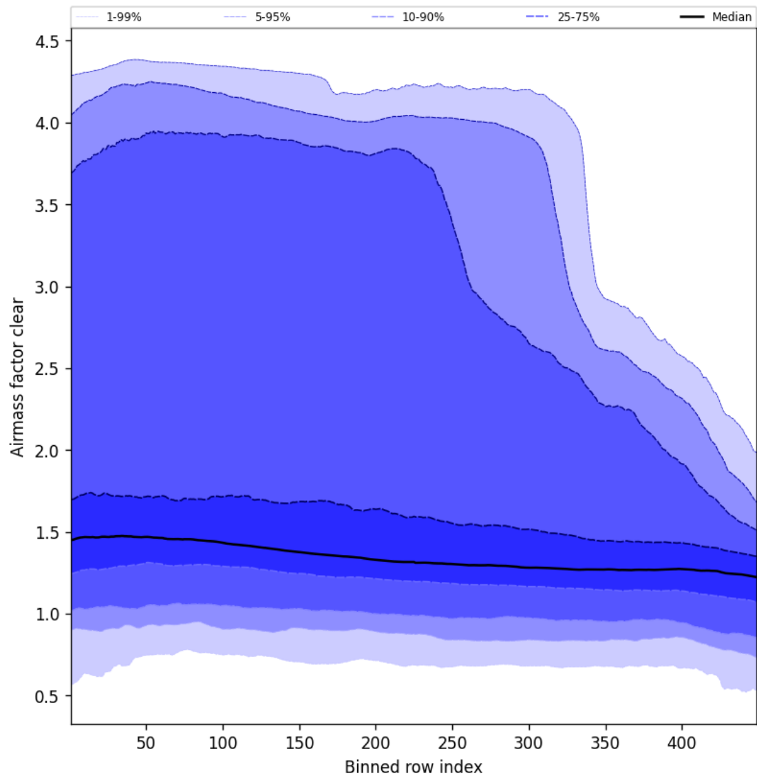
Figure 54: Along track statistics of “Airmass factor clear” for 2024-12-16 to 2024-12-17
