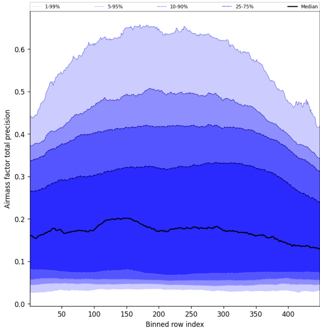
Figure 53: Along track statistics of “Airmass factor total precision” for 2024-12-16 to 2024-12-17
