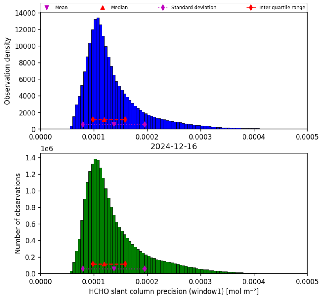
Figure 37: Histogram of “HCHO slant column precision (window1)” for 2024-12-16 to 2024-12-17
