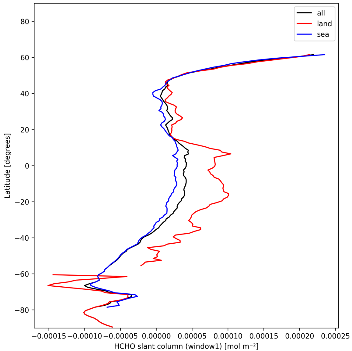
Figure 22: Zonal average of “HCHO slant column (window1)” for 2024-12-16 to 2024-12-17.
