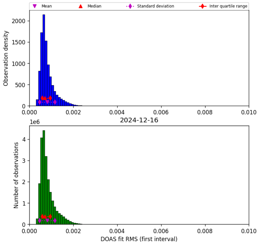
Figure 44: Histogram of “DOAS fit RMS (first interval)” for 2024-12-16 to 2024-12-17
