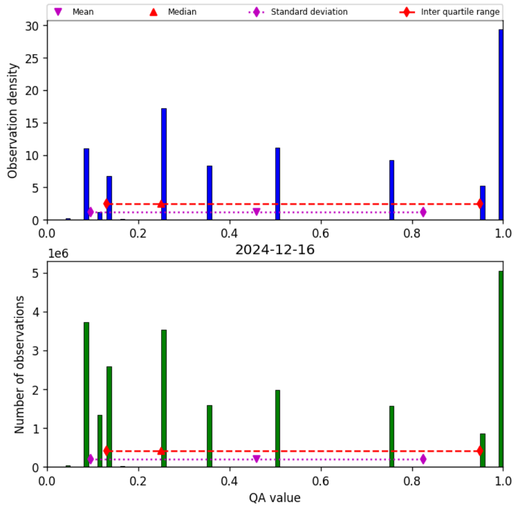
Figure 32: Histogram of “QA value” for 2024-12-16 to 2024-12-17
