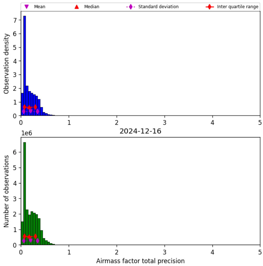
Figure 39: Histogram of “Airmass factor total precision” for 2024-12-16 to 2024-12-17
