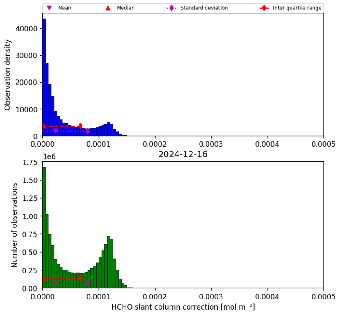
Figure 45: Histogram of “HCHO slant column correction” for 2024-12-16 to 2024-12-17
