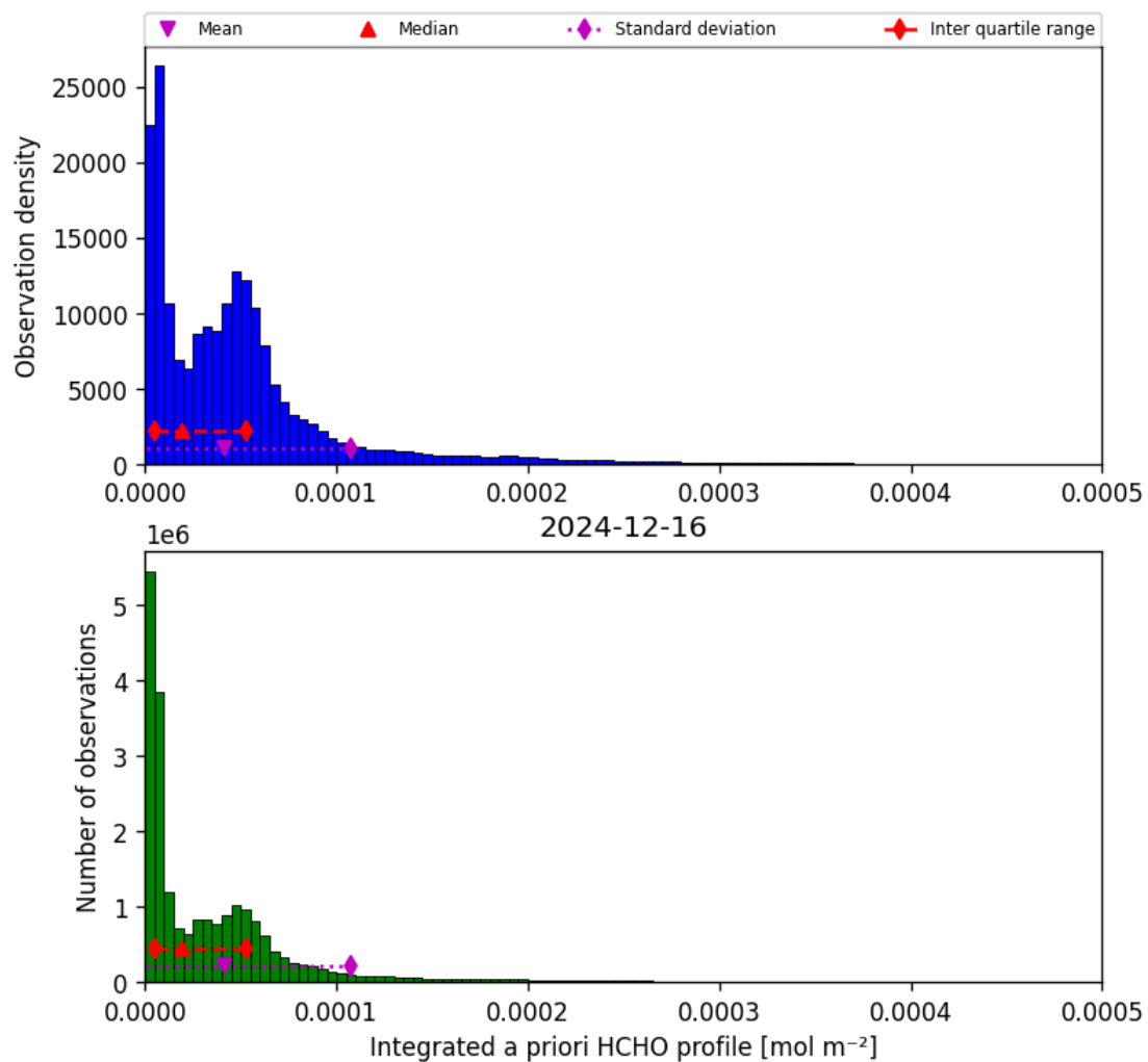
Figure 41: Histogram of “Integrated a priori HCHO profile” for 2024-12-16 to 2024-12-17
