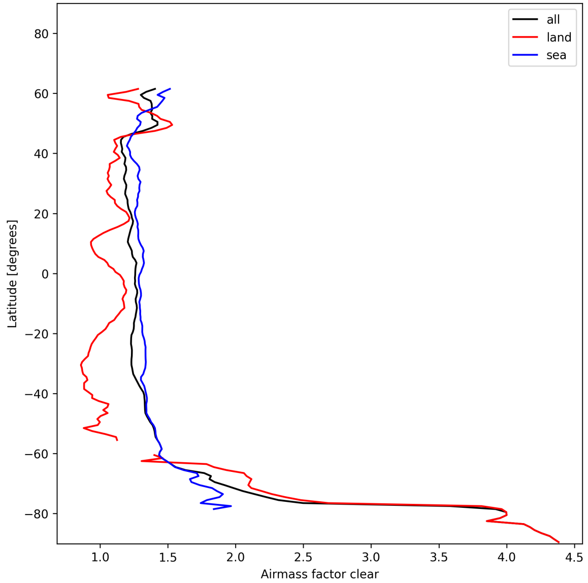
Figure 26: Zonal average of “Airmass factor clear” for 2024-12-16 to 2024-12-17.
