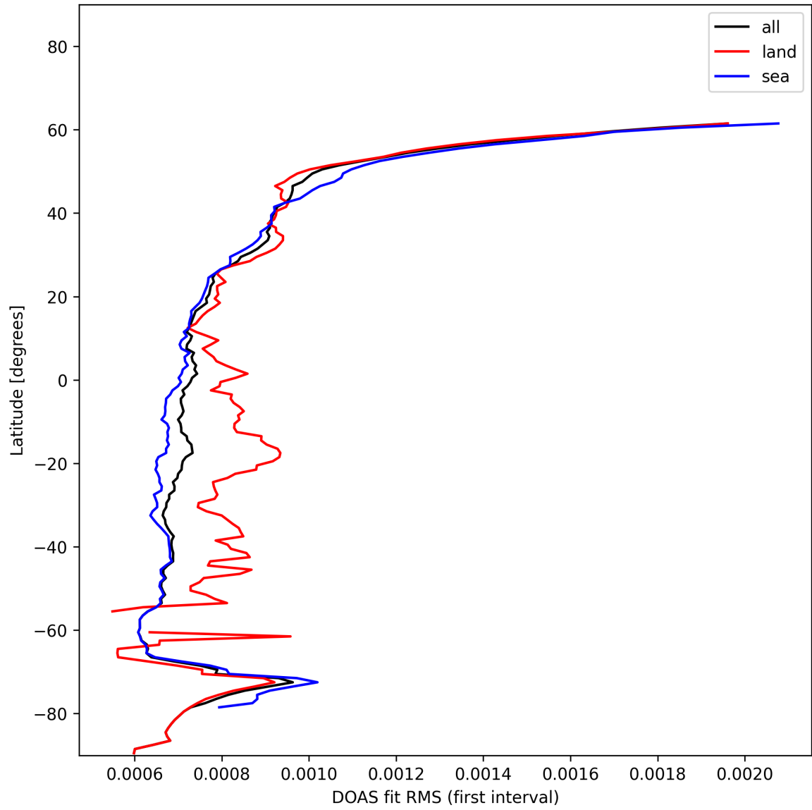
Figure 30: Zonal average of “DOAS fit RMS (first interval)” for 2024-12-16 to 2024-12-17.
