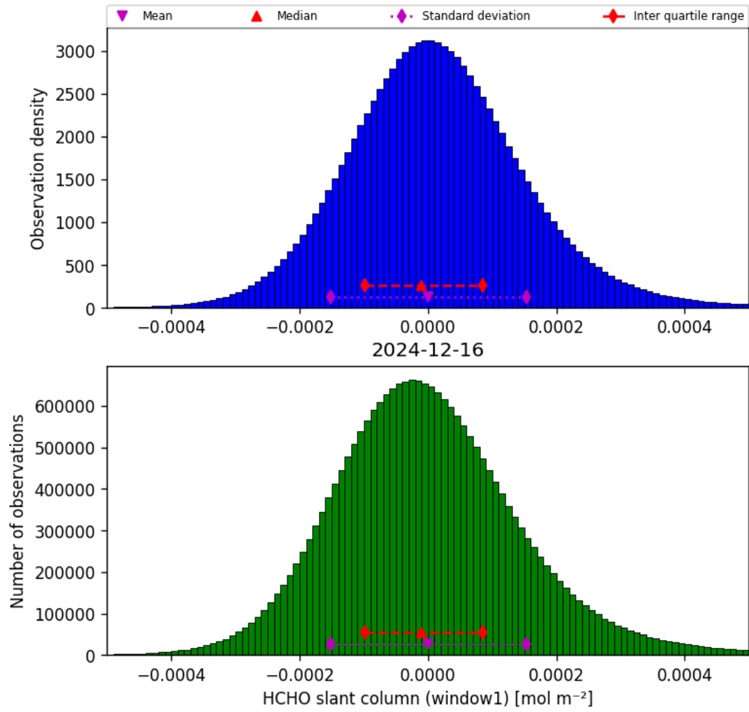
Figure 36: Histogram of “HCHO slant column (window1)” for 2024-12-16 to 2024-12-17
