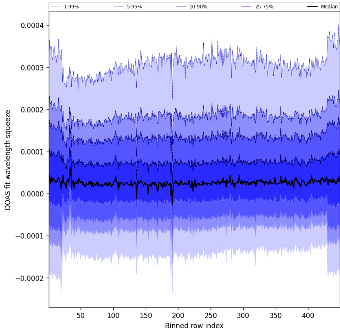
Figure 57: Along track statistics of “DOAS fit wavelength squeeze” for 2024-12-16 to 2024-12-17
