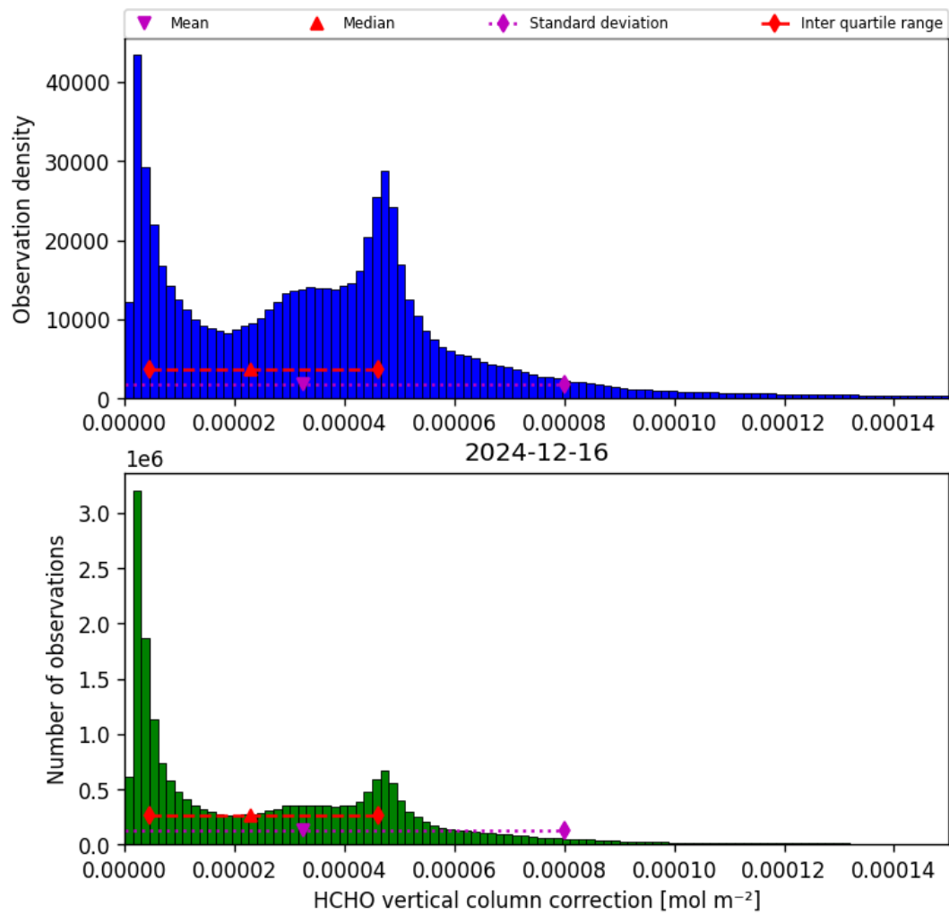
Figure 35: Histogram of “HCHO vertical column correction” for 2024-12-16 to 2024-12-17
