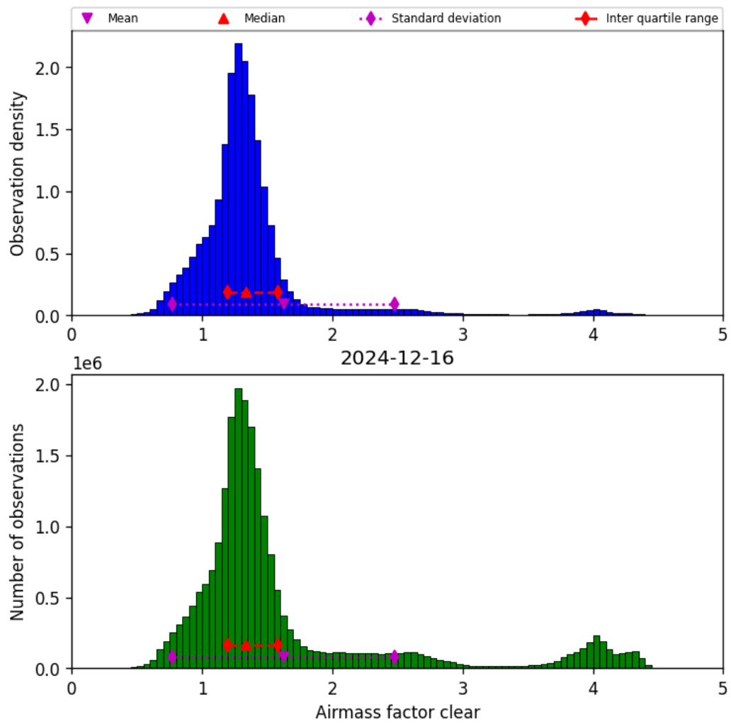
Figure 40: Histogram of “Airmass factor clear” for 2024-12-16 to 2024-12-17
