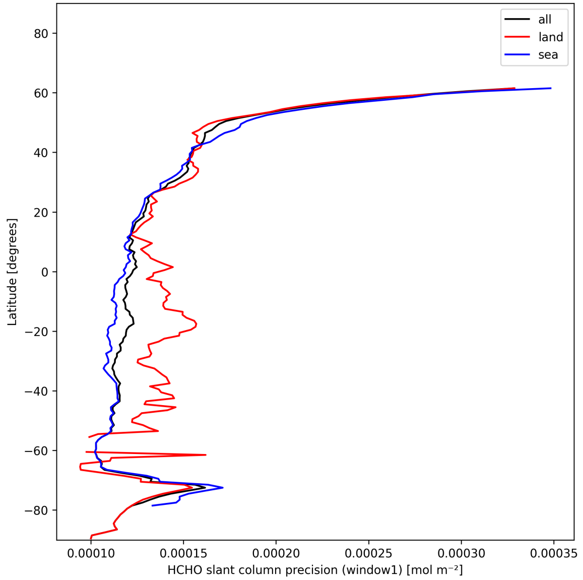
Figure 23: Zonal average of “HCHO slant column precision (window1)” for 2024-12-16 to 2024-12-17.
