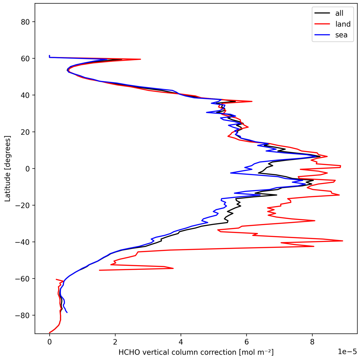
Figure 21: Zonal average of “HCHO vertical column correction” for 2024-12-16 to 2024-12-17.
