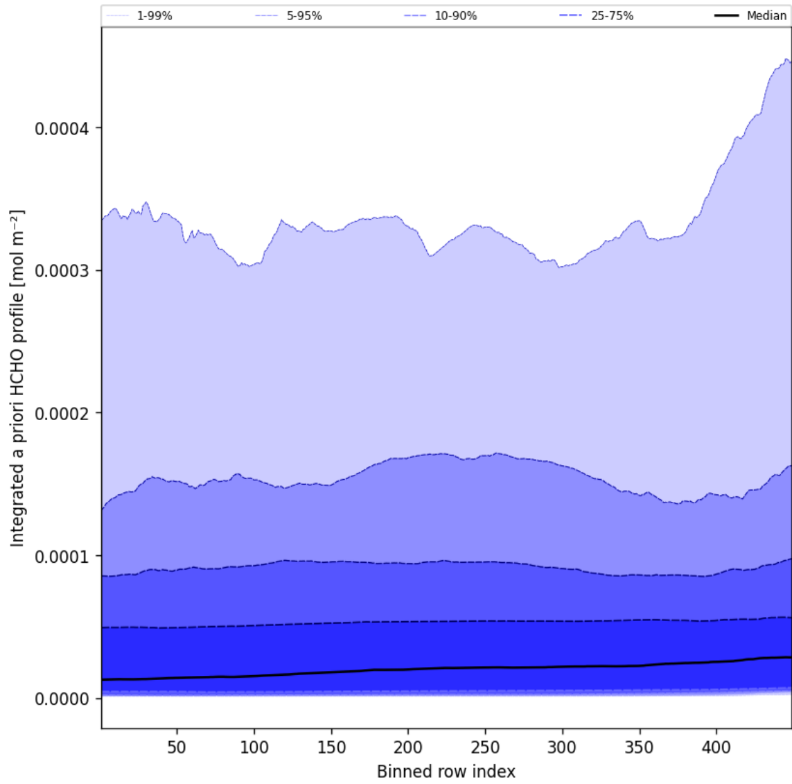
Figure 55: Along track statistics of “Integrated a priori HCHO profile” for 2024-12-16 to 2024-12-17
