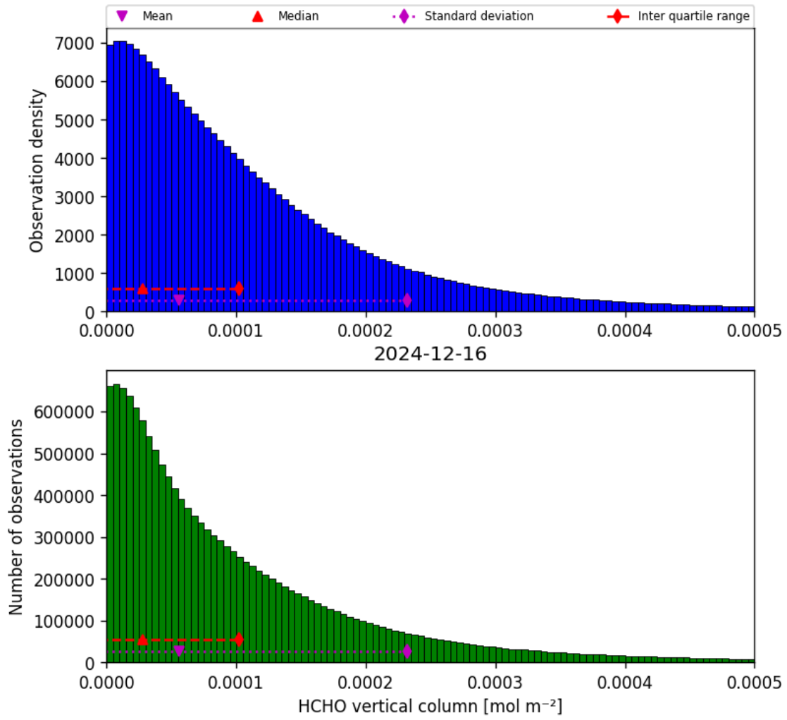
Figure 33: Histogram of “HCHO vertical column” for 2024-12-16 to 2024-12-17
