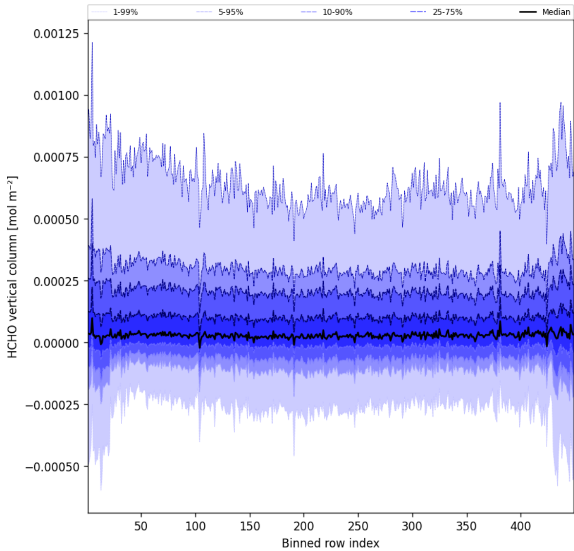
Figure 47: Along track statistics of “HCHO vertical column” for 2024-12-16 to 2024-12-17
