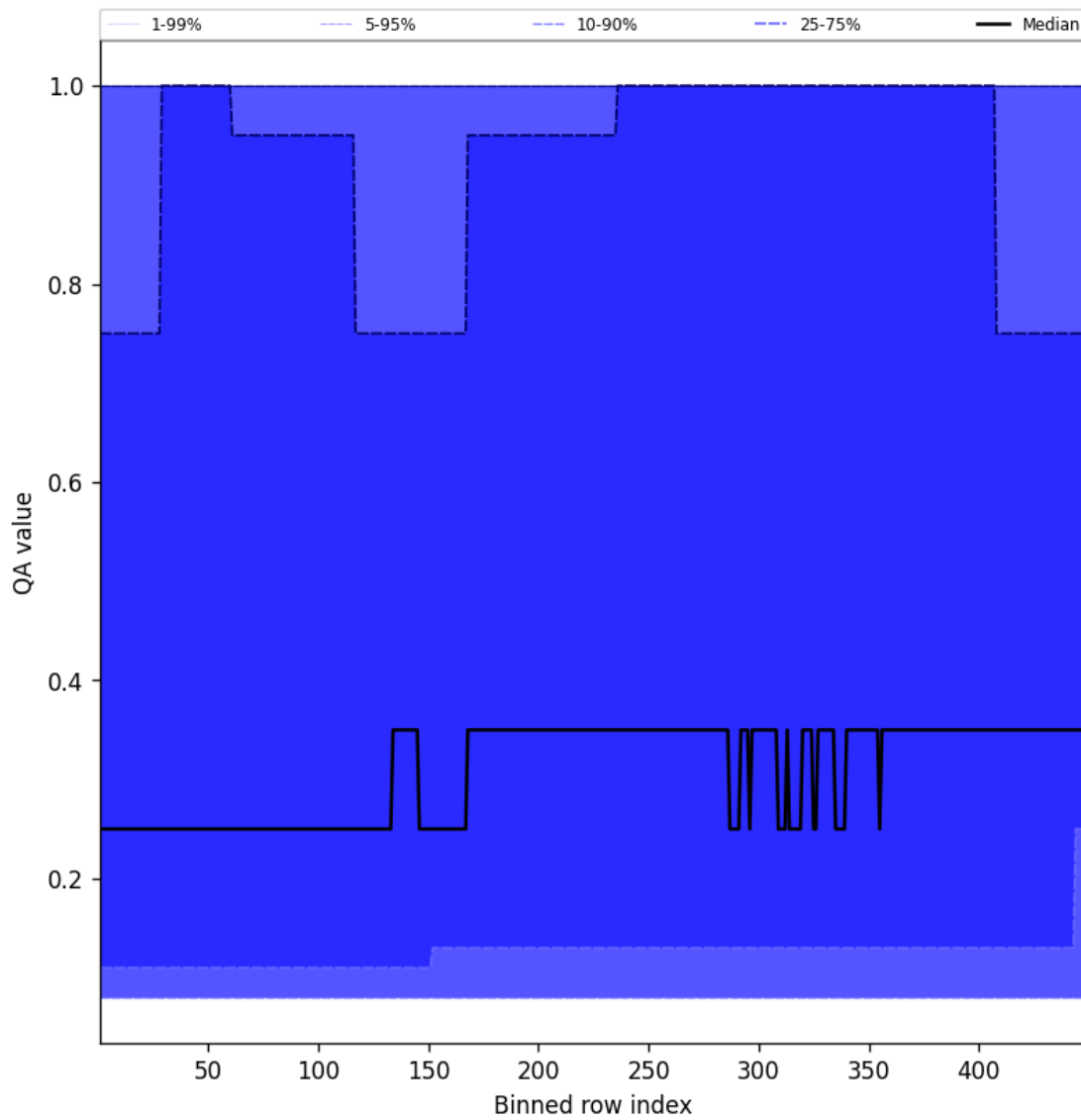
Figure 46: Along track statistics of “QA value” for 2024-12-16 to 2024-12-17
