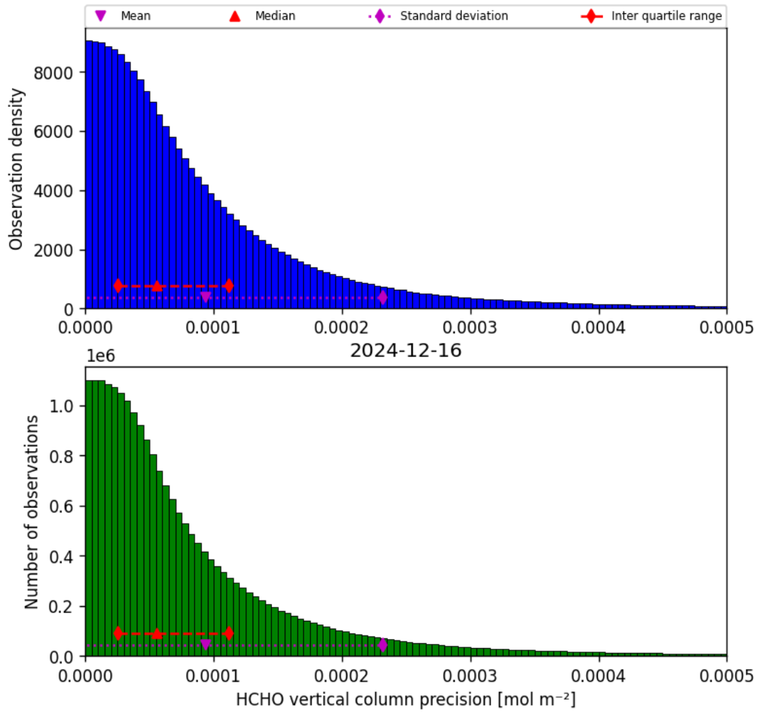
Figure 34: Histogram of “HCHO vertical column precision” for 2024-12-16 to 2024-12-17
