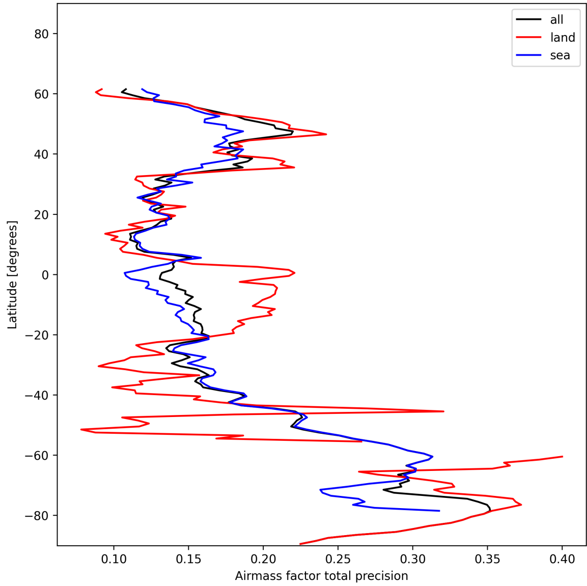
Figure 25: Zonal average of “Airmass factor total precision” for 2024-12-16 to 2024-12-17.
