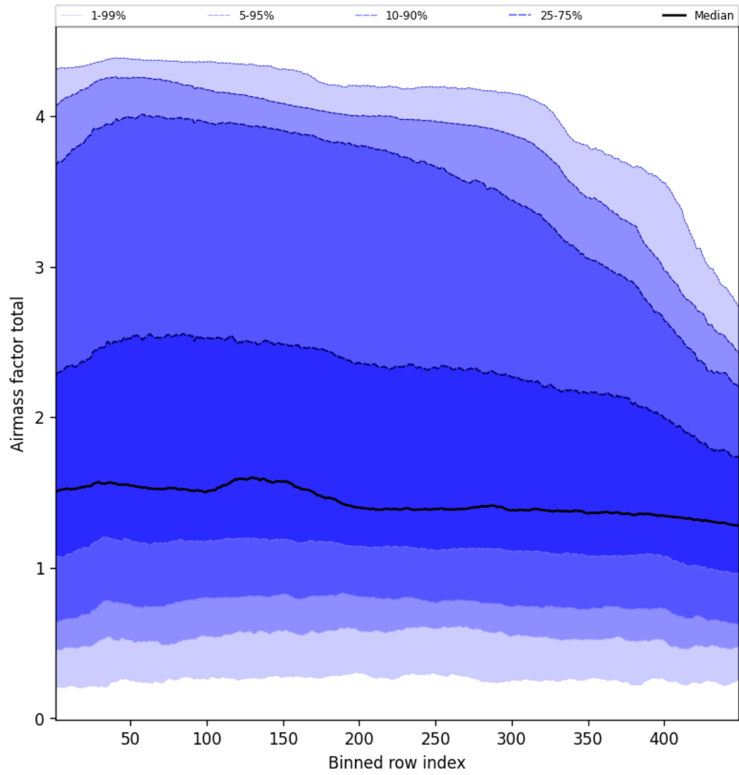
Figure 52: Along track statistics of “Airmass factor total” for 2024-12-16 to 2024-12-17
