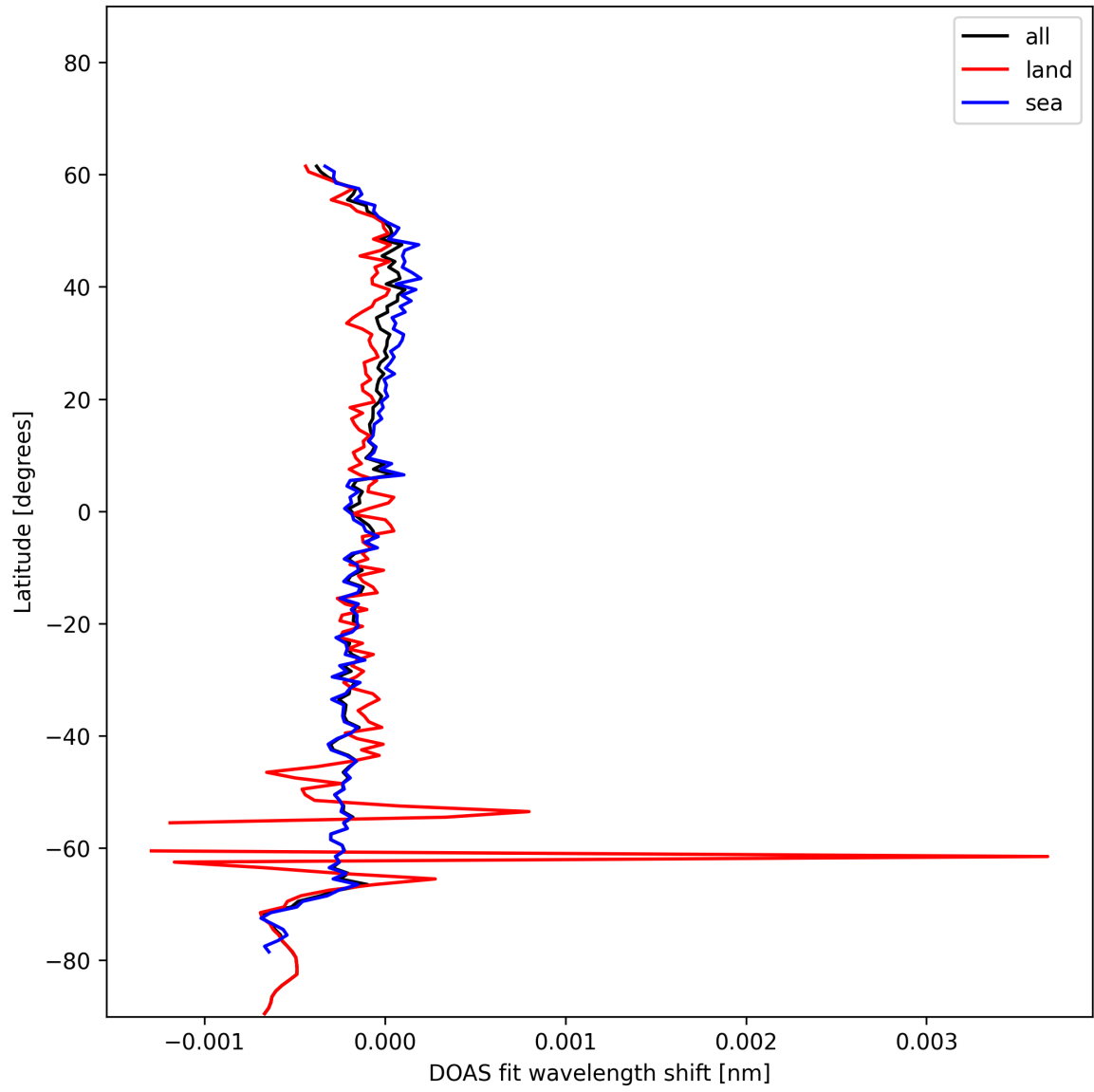
Figure 28: Zonal average of “DOAS fit wavelength shift” for 2024-12-16 to 2024-12-17.
