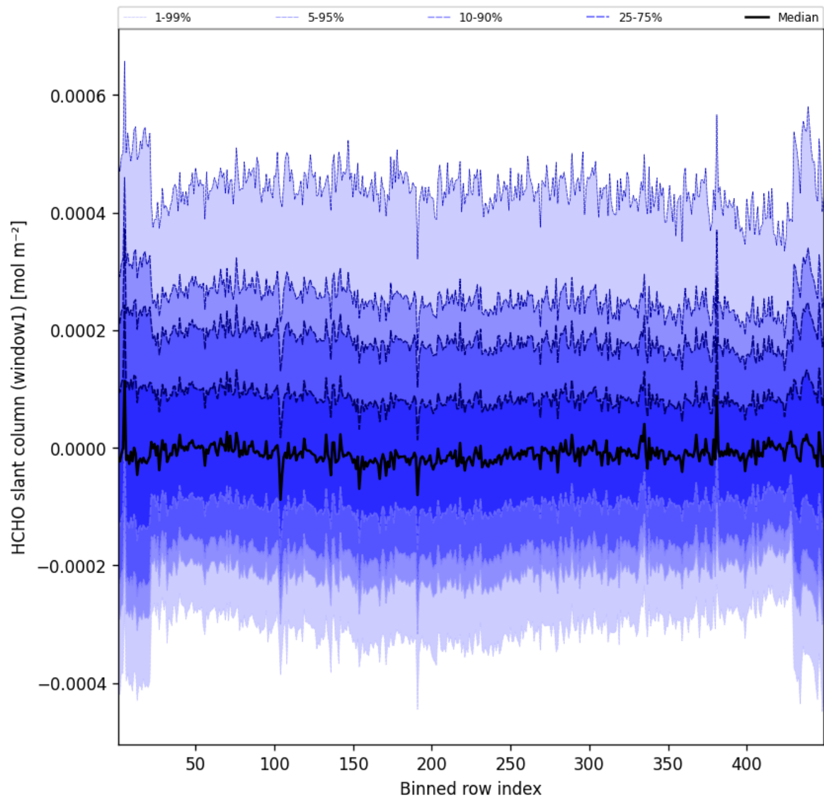
Figure 50: Along track statistics of “HCHO slant column (window1)” for 2024-12-16 to 2024-12-17
