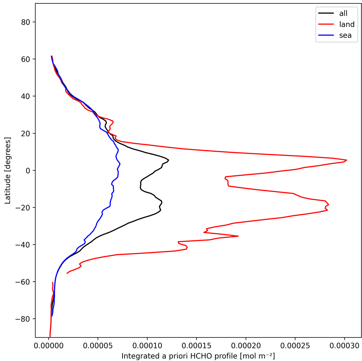
Figure 27: Zonal average of “Integrated a priori HCHO profile” for 2024-12-16 to 2024-12-17.
