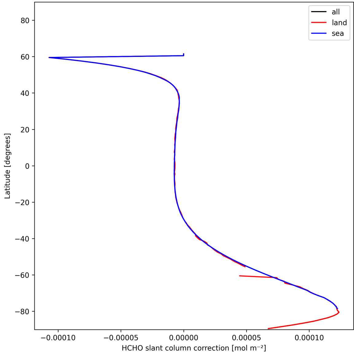
Figure 31: Zonal average of “HCHO slant column correction” for 2024-12-16 to 2024-12-17.
