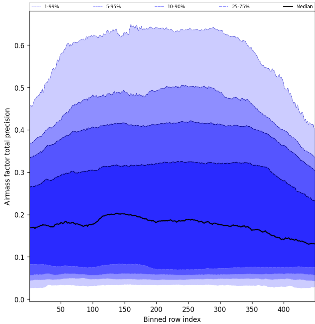
Figure 53: Along track statistics of “Airmass factor total precision” for 2024-12-17 to 2024-12-18
