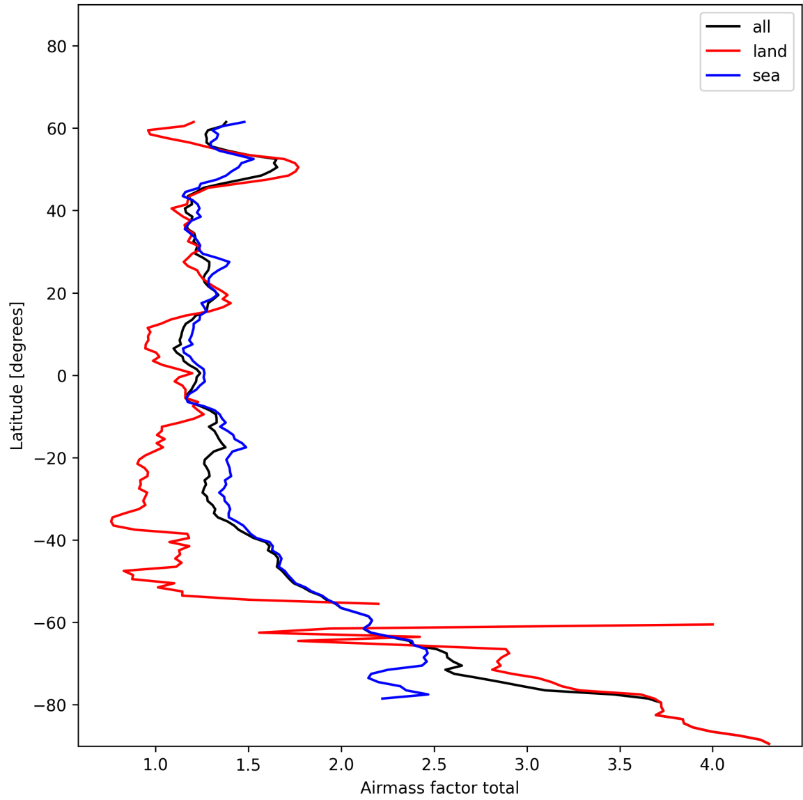
Figure 24: Zonal average of “Airmass factor total” for 2024-12-17 to 2024-12-18.
