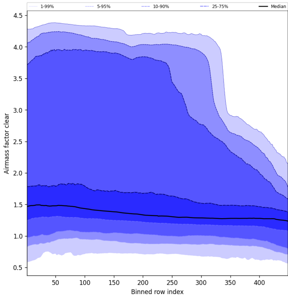
Figure 54: Along track statistics of “Airmass factor clear” for 2024-12-17 to 2024-12-18
