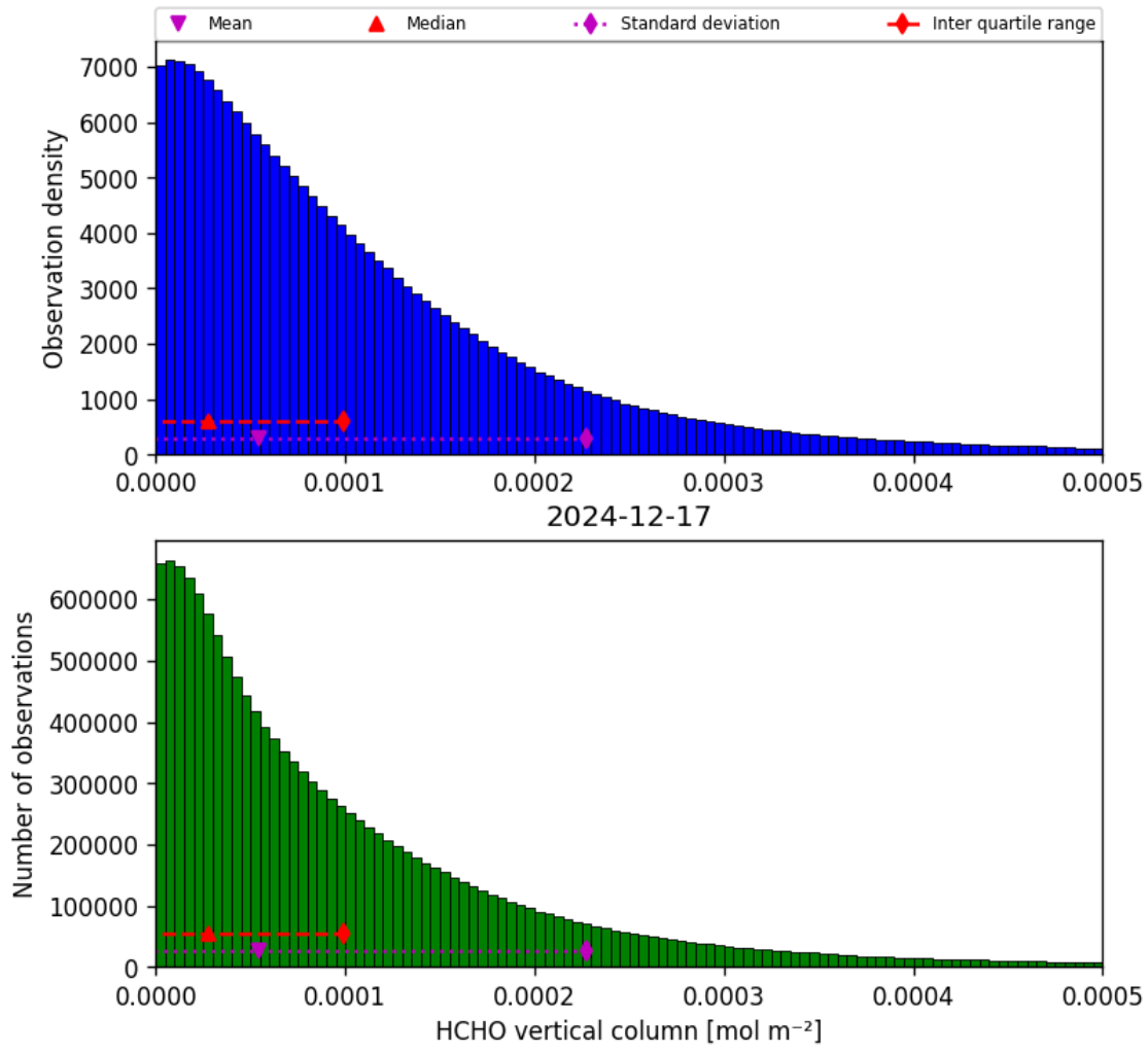
Figure 33: Histogram of “HCHO vertical column” for 2024-12-17 to 2024-12-18
