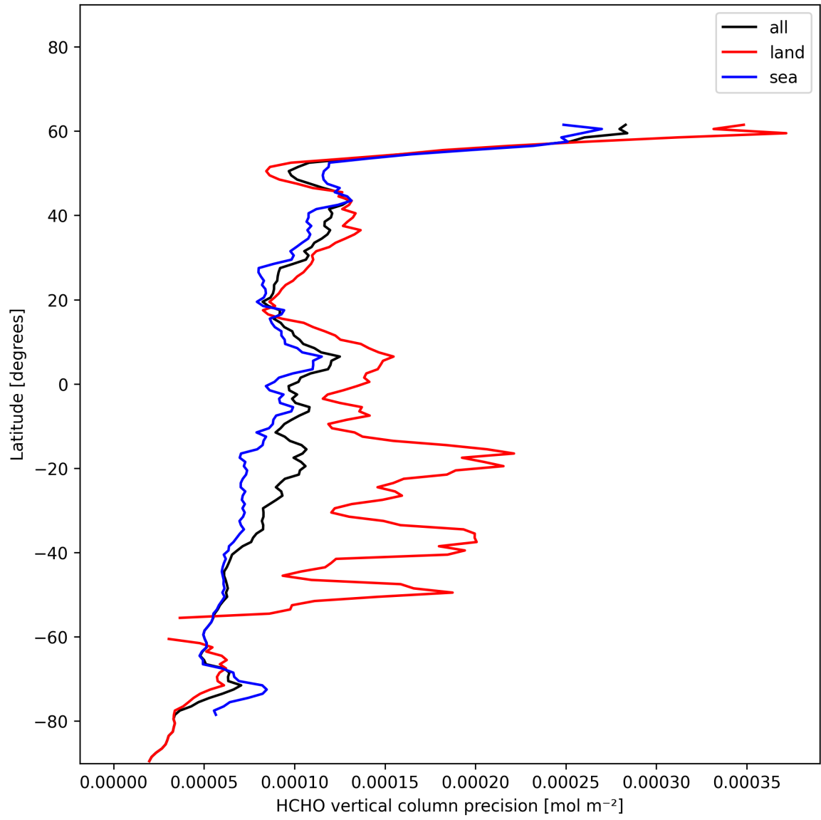
Figure 20: Zonal average of “HCHO vertical column precision” for 2024-12-17 to 2024-12-18.
