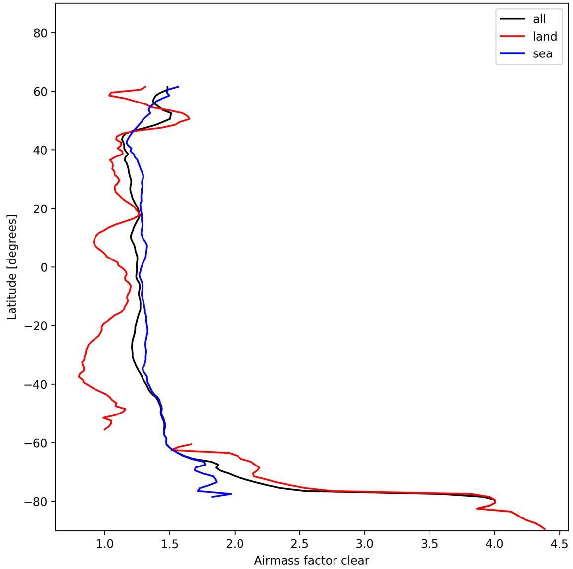
Figure 26: Zonal average of “Airmass factor clear” for 2024-12-17 to 2024-12-18.
