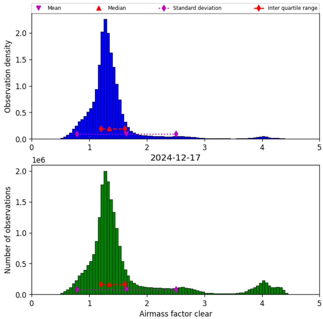
Figure 40: Histogram of “Airmass factor clear” for 2024-12-17 to 2024-12-18
