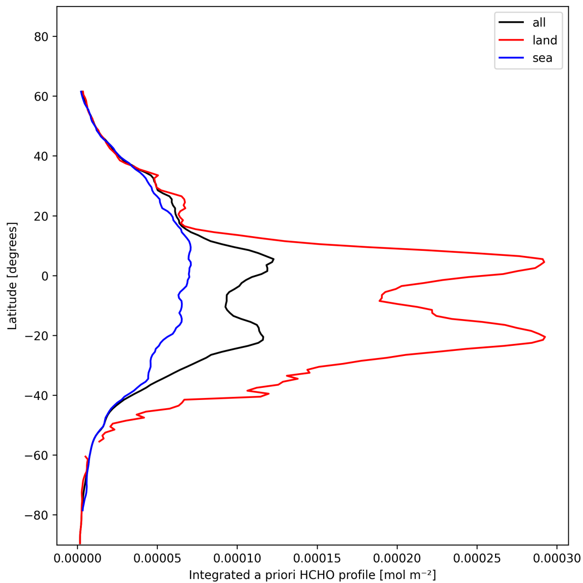
Figure 27: Zonal average of “Integrated a priori HCHO profile” for 2024-12-17 to 2024-12-18.
