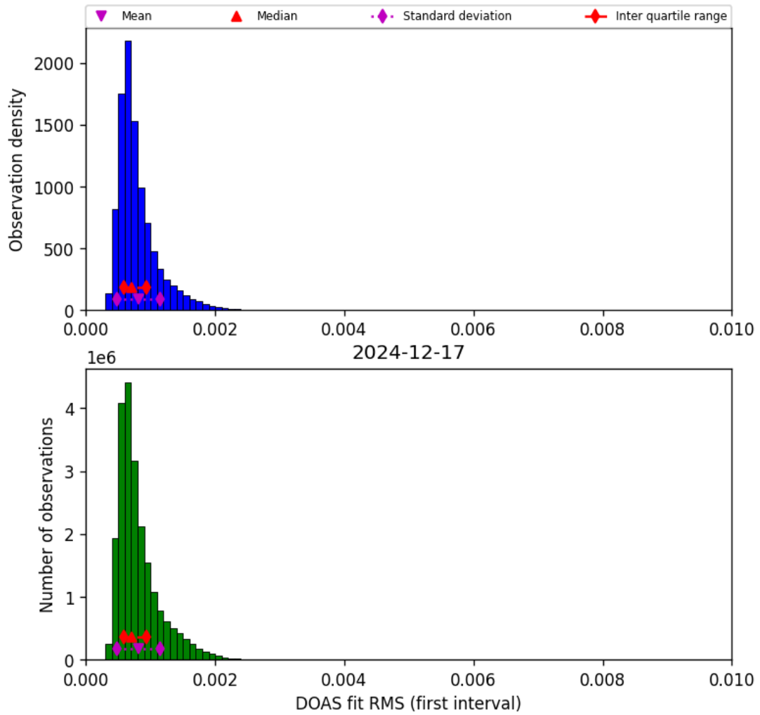
Figure 44: Histogram of “DOAS fit RMS (first interval)” for 2024-12-17 to 2024-12-18
