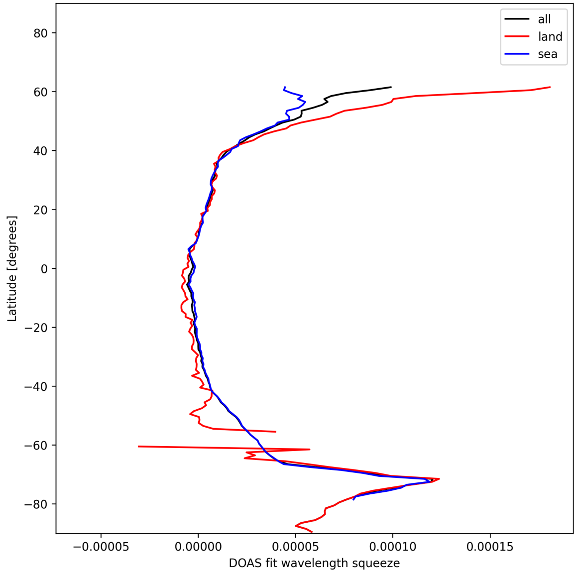
Figure 29: Zonal average of “DOAS fit wavelength squeeze” for 2024-12-17 to 2024-12-18.
