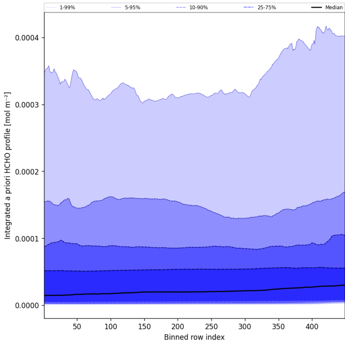
Figure 55: Along track statistics of “Integrated a priori HCHO profile” for 2024-12-17 to 2024-12-18
