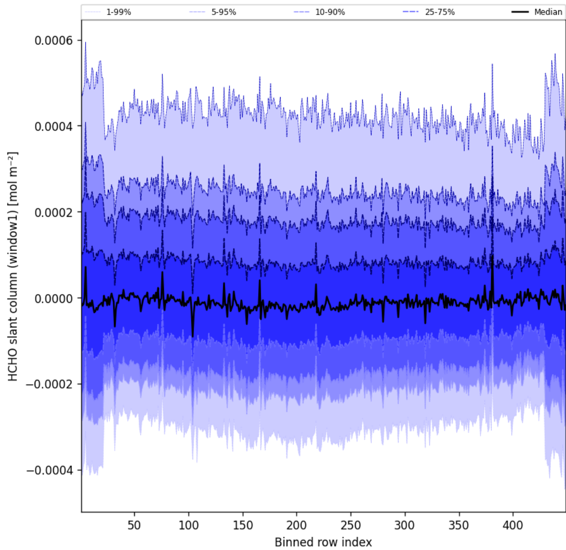
Figure 50: Along track statistics of “HCHO slant column (window1)” for 2024-12-17 to 2024-12-18
