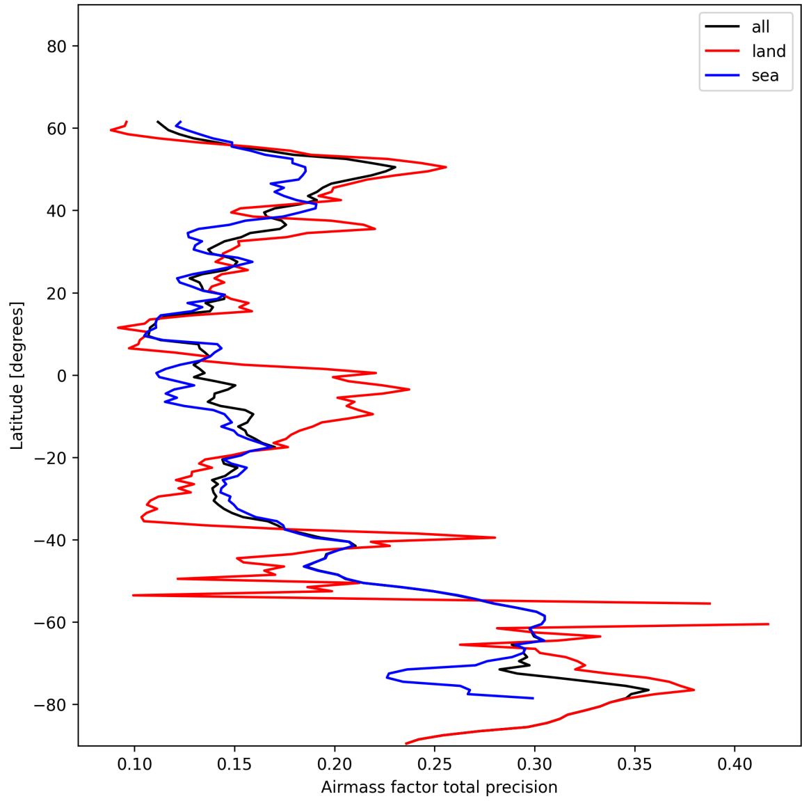
Figure 25: Zonal average of “Airmass factor total precision” for 2024-12-17 to 2024-12-18.
