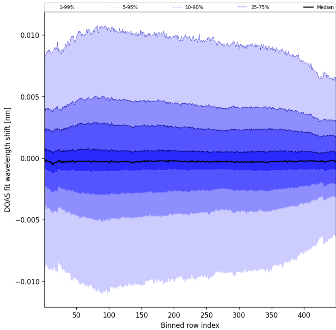
Figure 56: Along track statistics of “DOAS fit wavelength shift” for 2024-12-17 to 2024-12-18
