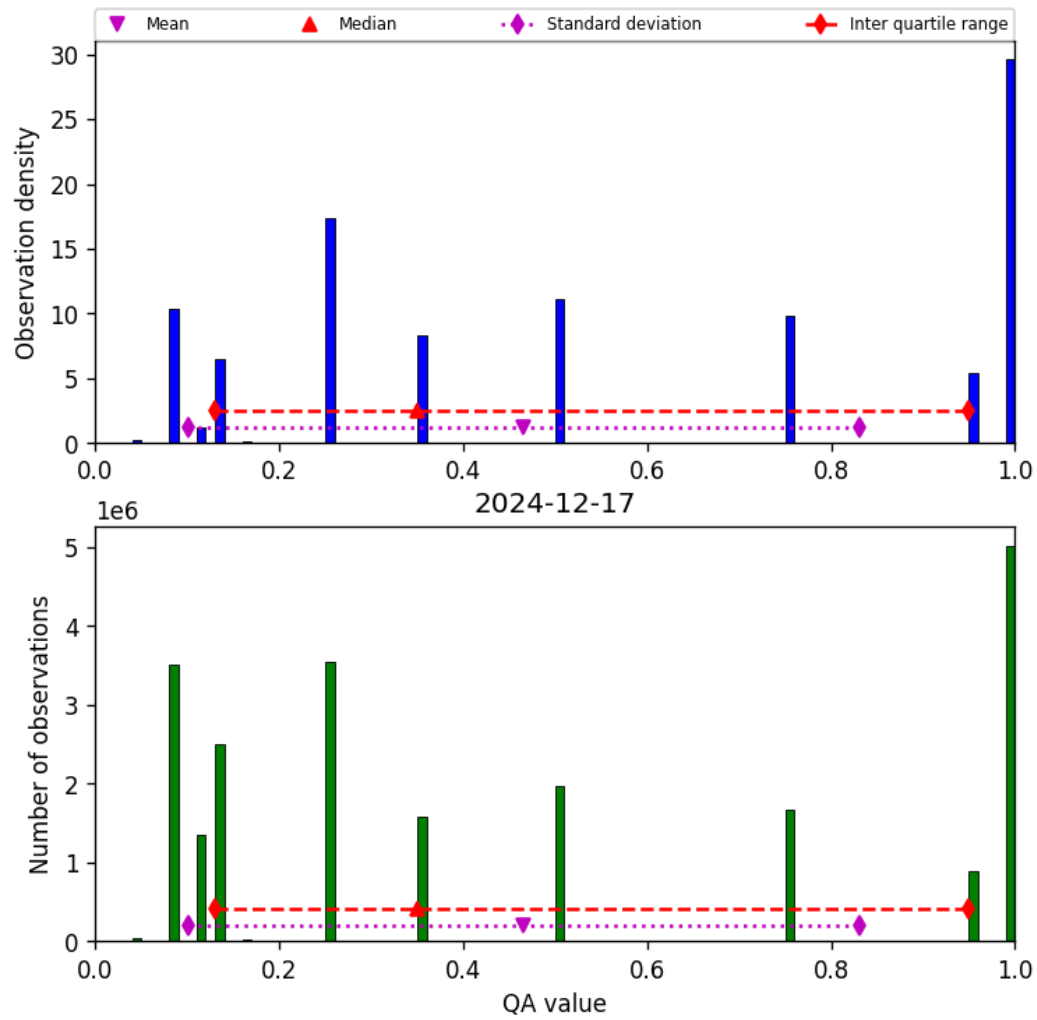
Figure 32: Histogram of “QA value” for 2024-12-17 to 2024-12-18
