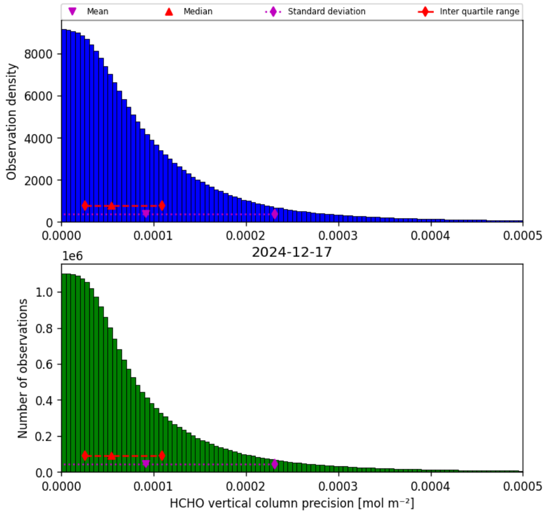
Figure 34: Histogram of “HCHO vertical column precision” for 2024-12-17 to 2024-12-18
