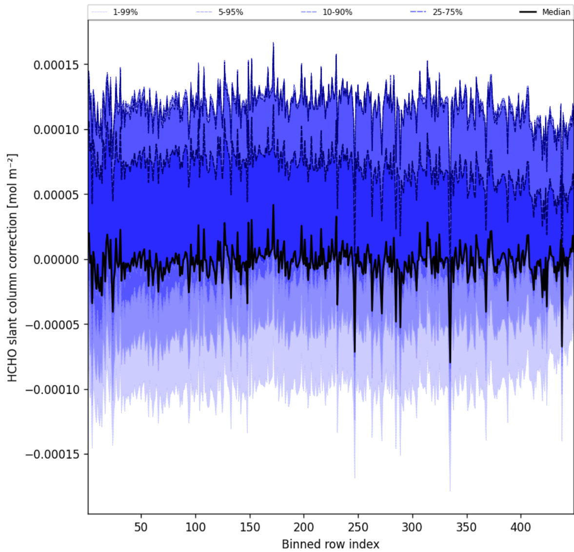
Figure 59: Along track statistics of “HCHO slant column correction” for 2024-12-17 to 2024-12-18
