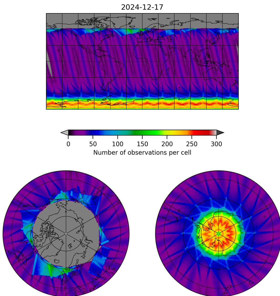
Figure 17: Map of the number of observations for 2024-12-17 to 2024-12-18
