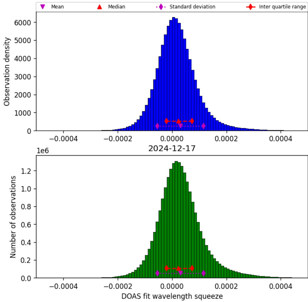
Figure 43: Histogram of “DOAS fit wavelength squeeze” for 2024-12-17 to 2024-12-18
