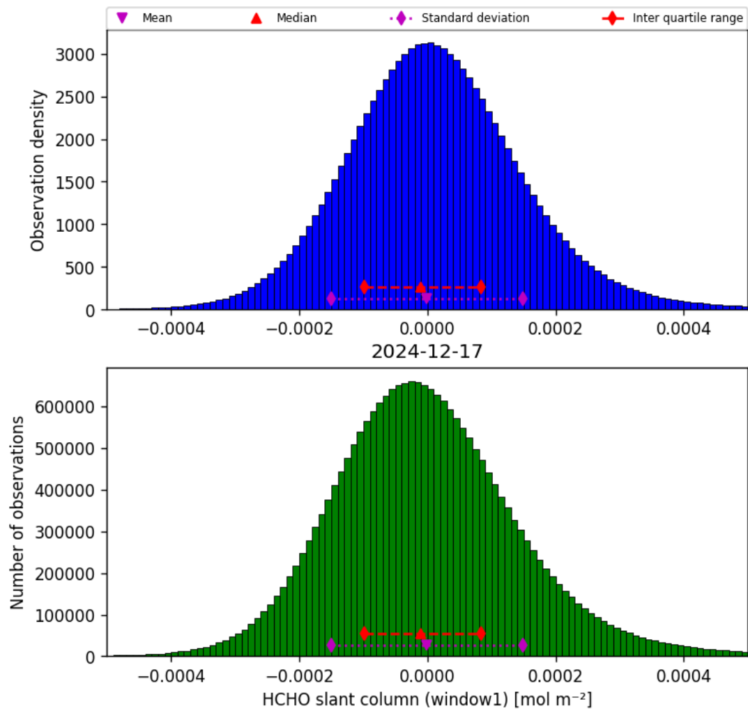
Figure 36: Histogram of “HCHO slant column (window1)” for 2024-12-17 to 2024-12-18
