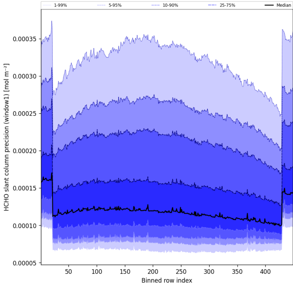
Figure 51: Along track statistics of “HCHO slant column precision (window1)” for 2024-12-17 to 2024-12-18
