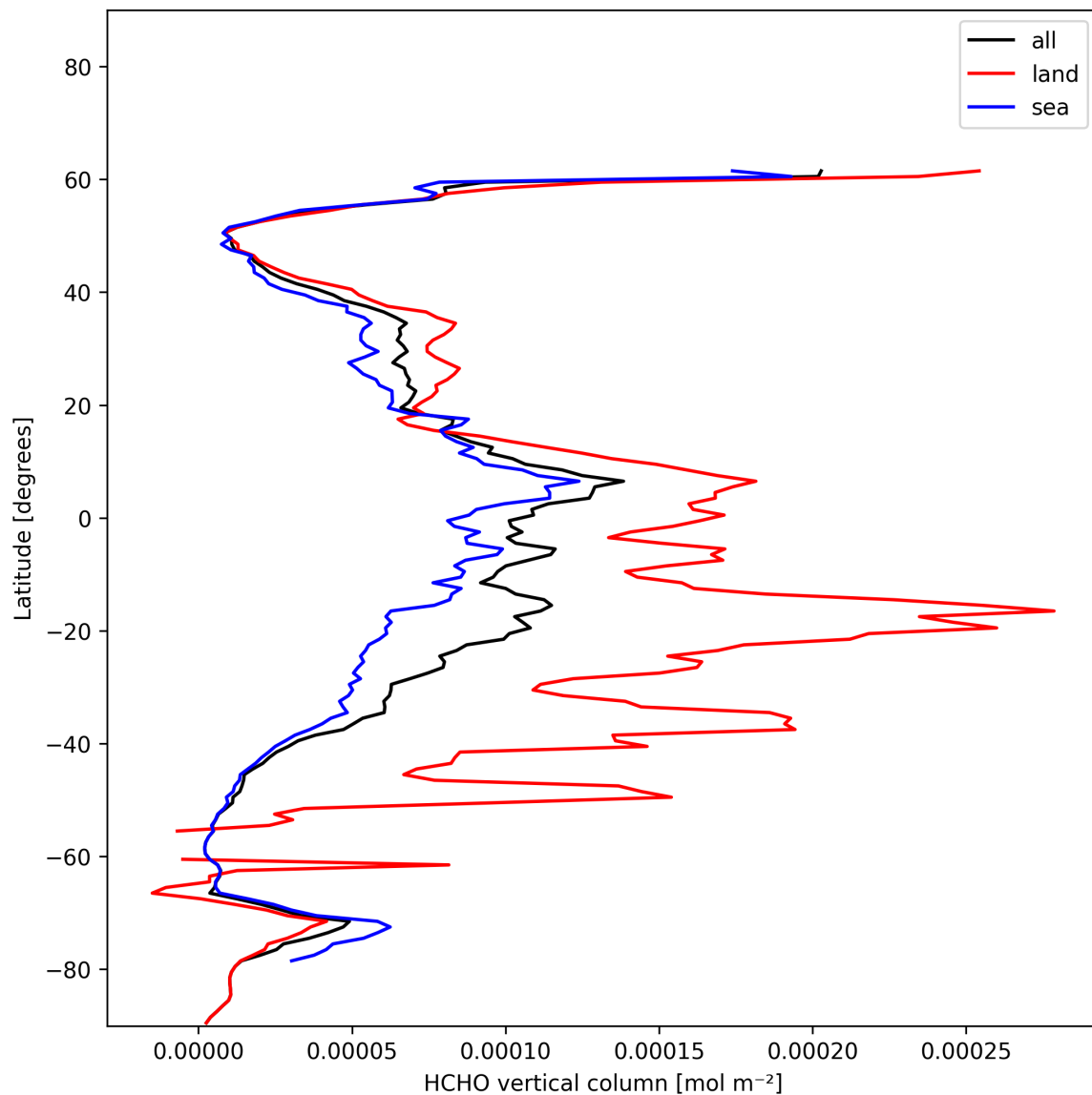
Figure 19: Zonal average of “HCHO vertical column” for 2024-12-17 to 2024-12-18.
