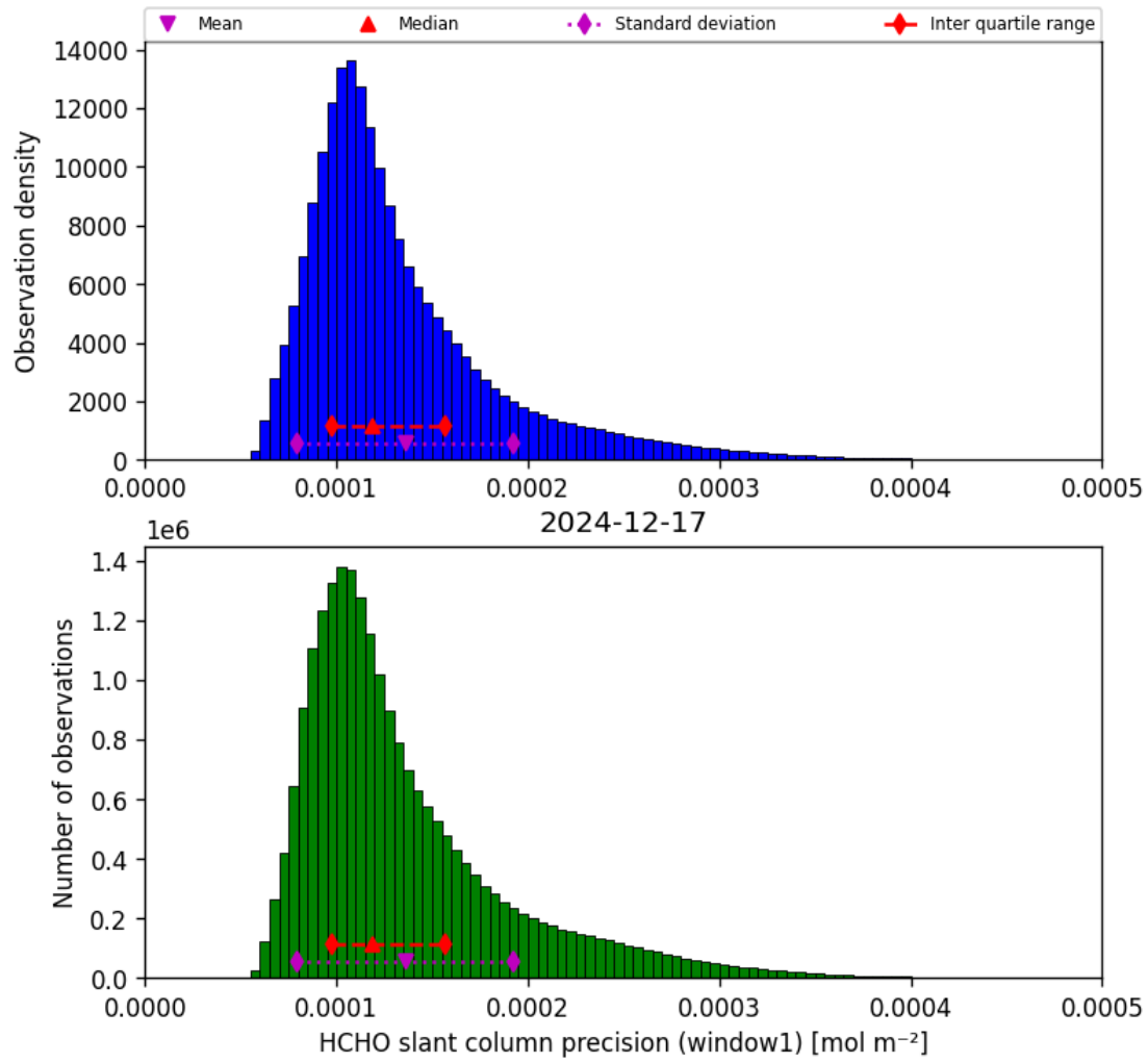
Figure 37: Histogram of “HCHO slant column precision (window1)” for 2024-12-17 to 2024-12-18
