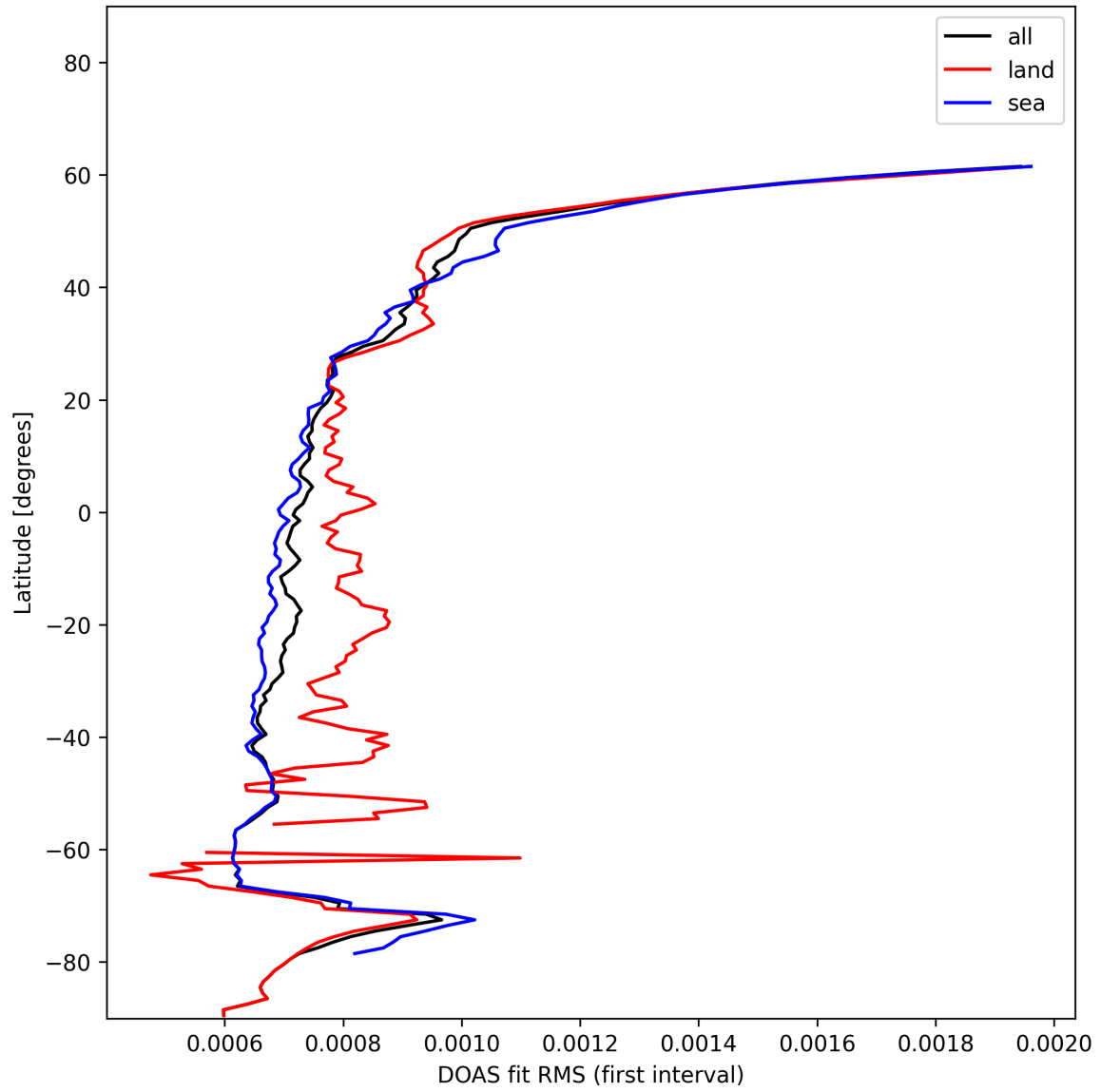
Figure 30: Zonal average of "DOAS fit RMS (first interval)" for 2024-12-17 to 2024-12-18.
