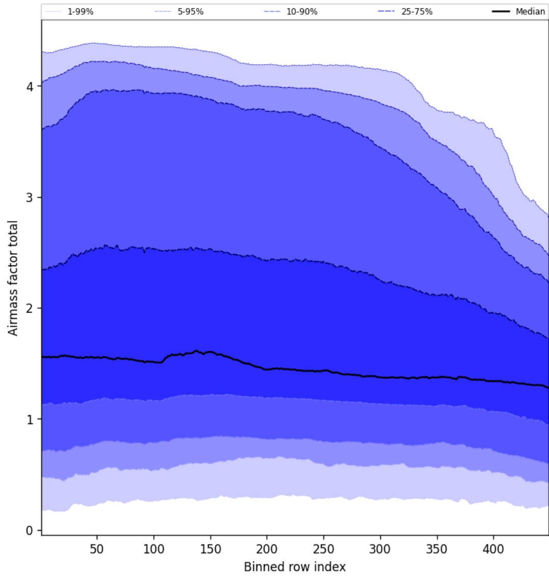
Figure 52: Along track statistics of “Airmass factor total” for 2024-12-17 to 2024-12-18
