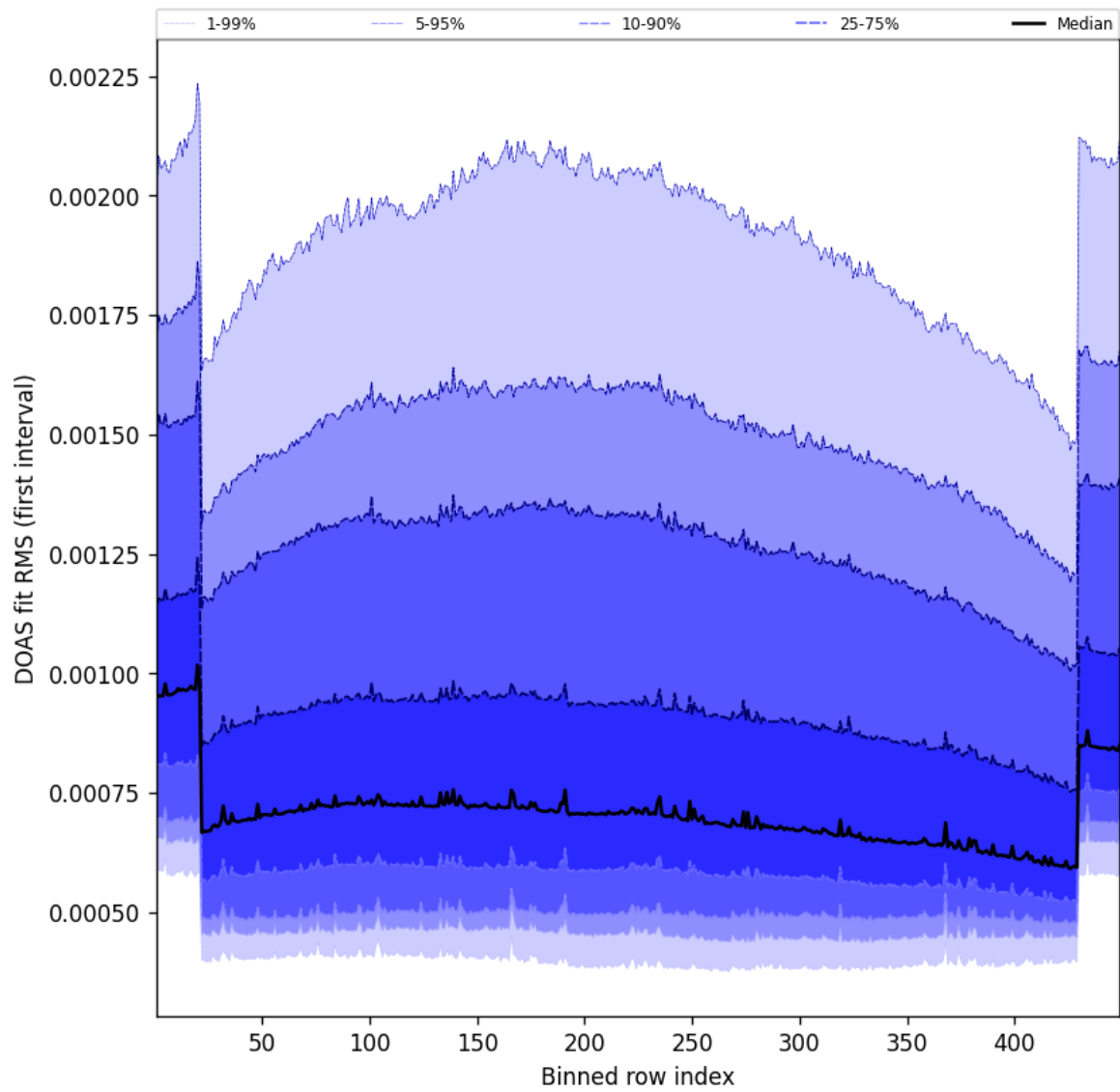
Figure 58: Along track statistics of “DOAS fit RMS (first interval)” for 2024-12-17 to 2024-12-18
