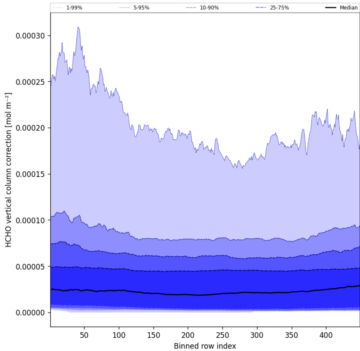
Figure 49: Along track statistics of “HCHO vertical column correction” for 2024-12-17 to 2024-12-18
