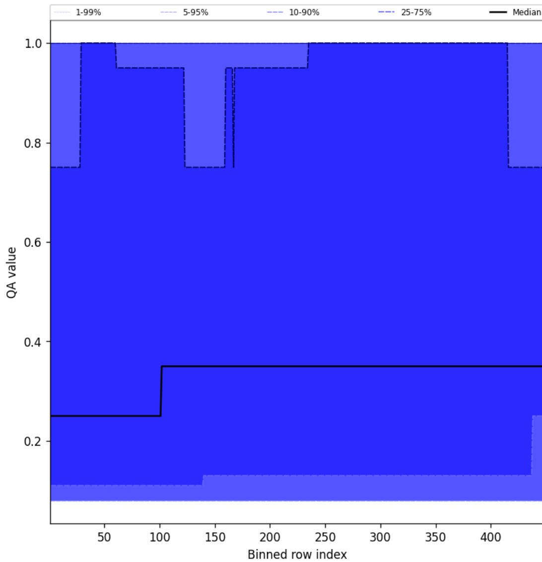
Figure 46: Along track statistics of “QA value” for 2024-12-17 to 2024-12-18
