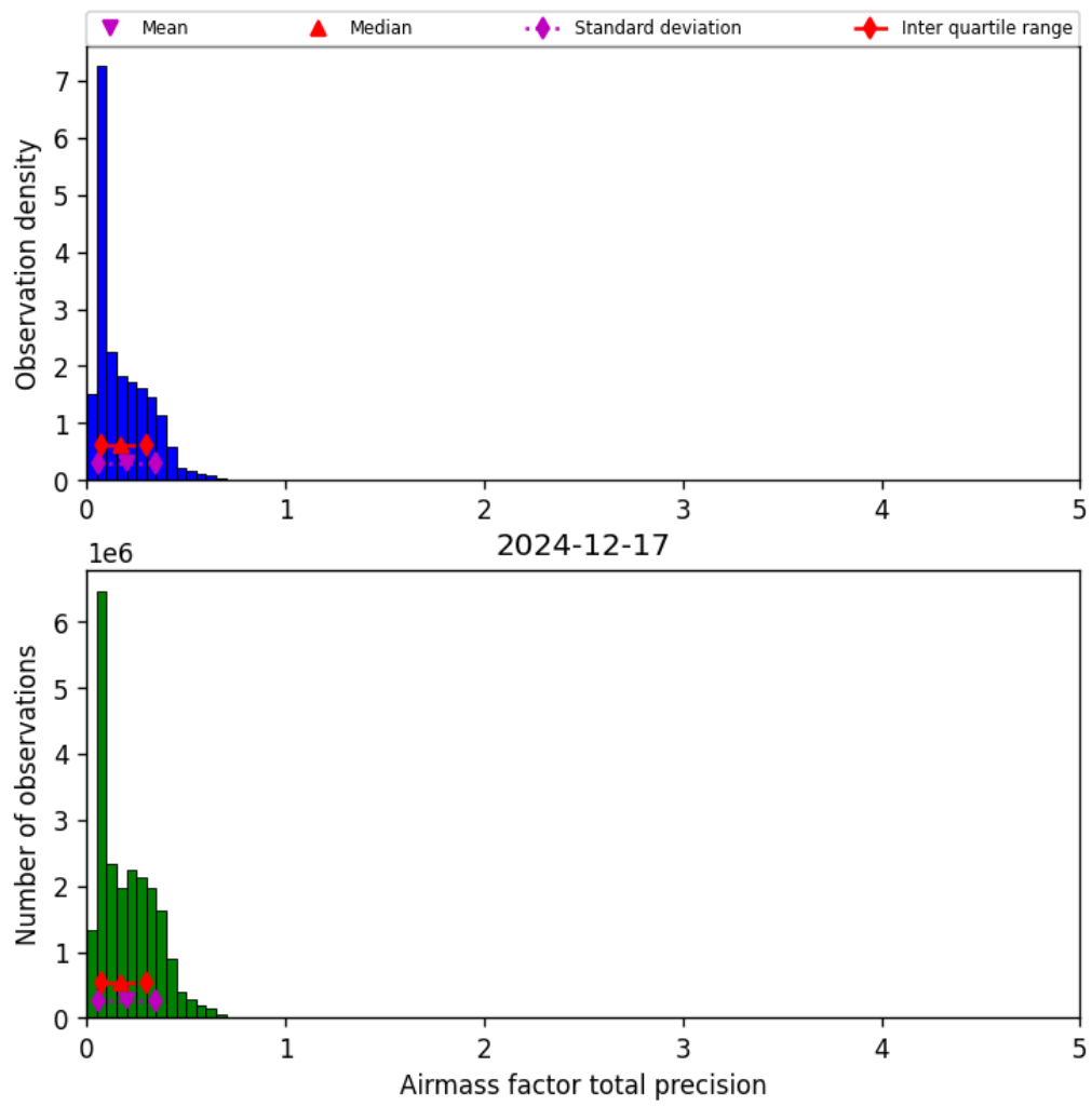
Figure 39: Histogram of “Airmass factor total precision” for 2024-12-17 to 2024-12-18
