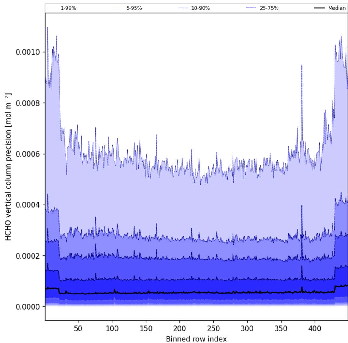
Figure 48: Along track statistics of “HCHO vertical column precision” for 2024-12-17 to 2024-12-18
