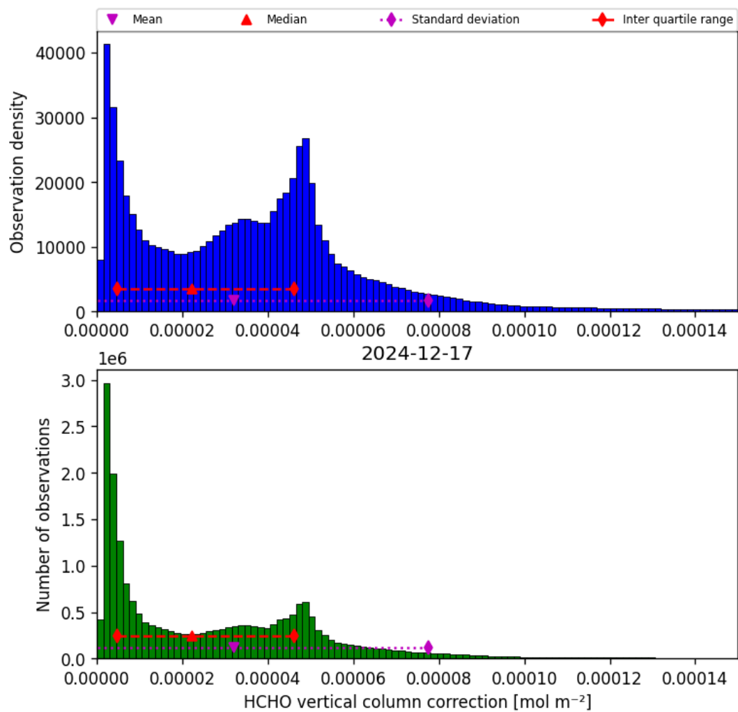
Figure 35: Histogram of “HCHO vertical column correction” for 2024-12-17 to 2024-12-18
