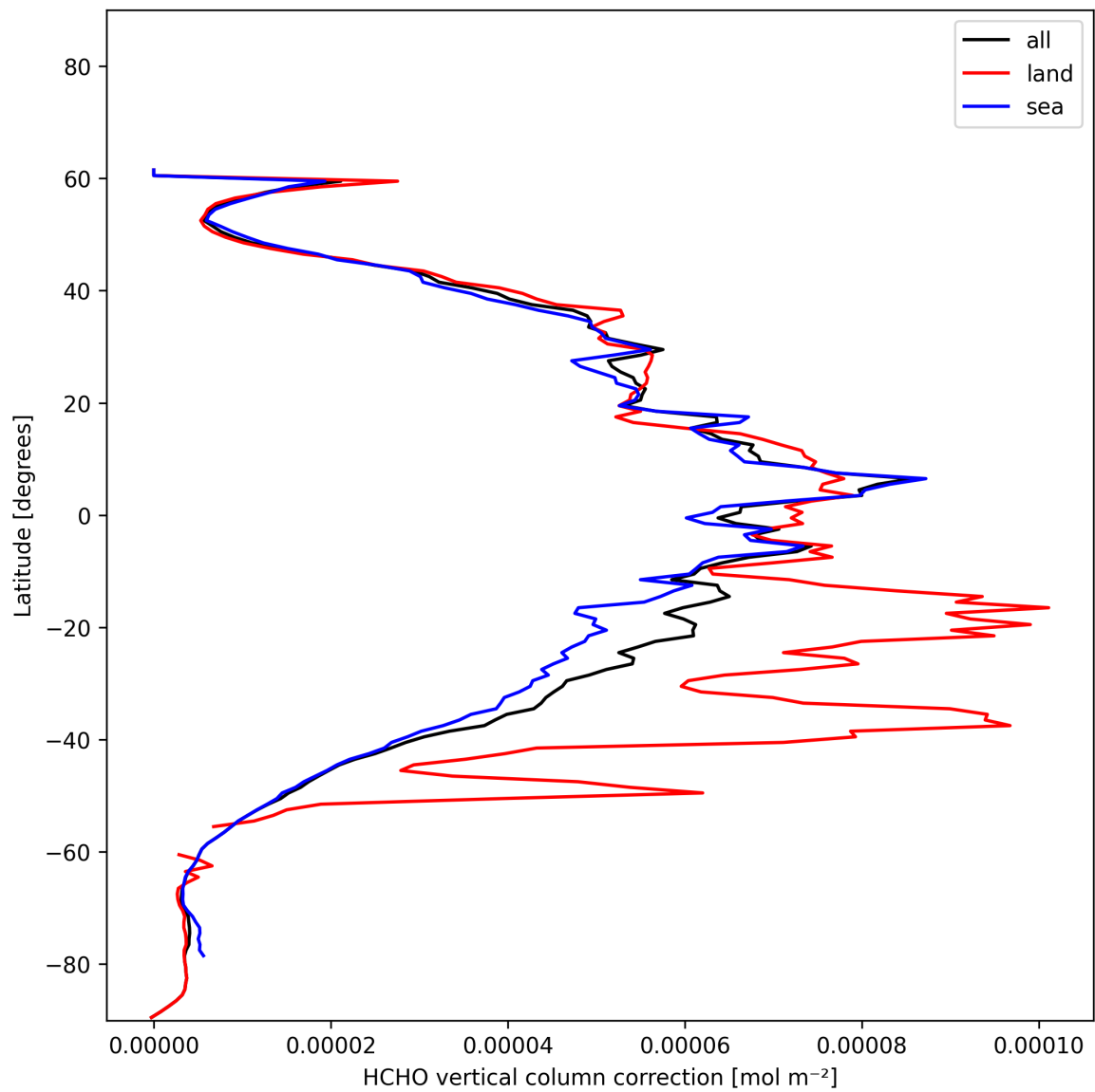
Figure 21: Zonal average of “HCHO vertical column correction” for 2024-12-17 to 2024-12-18.
