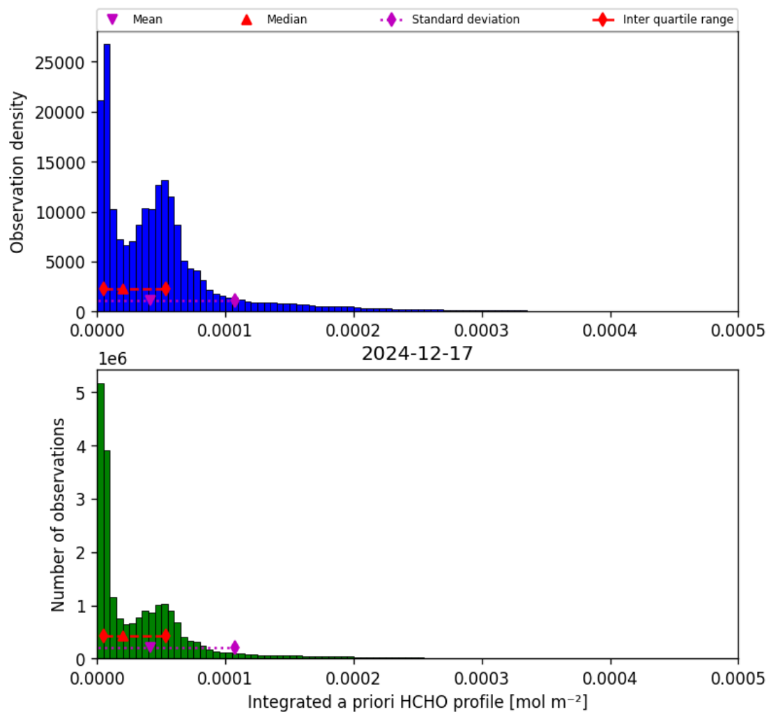
Figure 41: Histogram of “Integrated a priori HCHO profile” for 2024-12-17 to 2024-12-18
