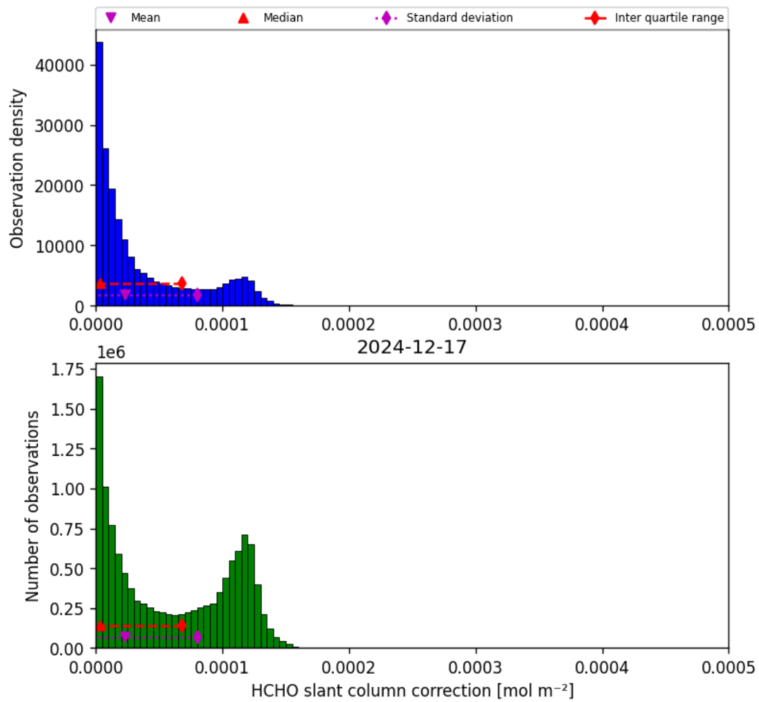
Figure 45: Histogram of “HCHO slant column correction” for 2024-12-17 to 2024-12-18
