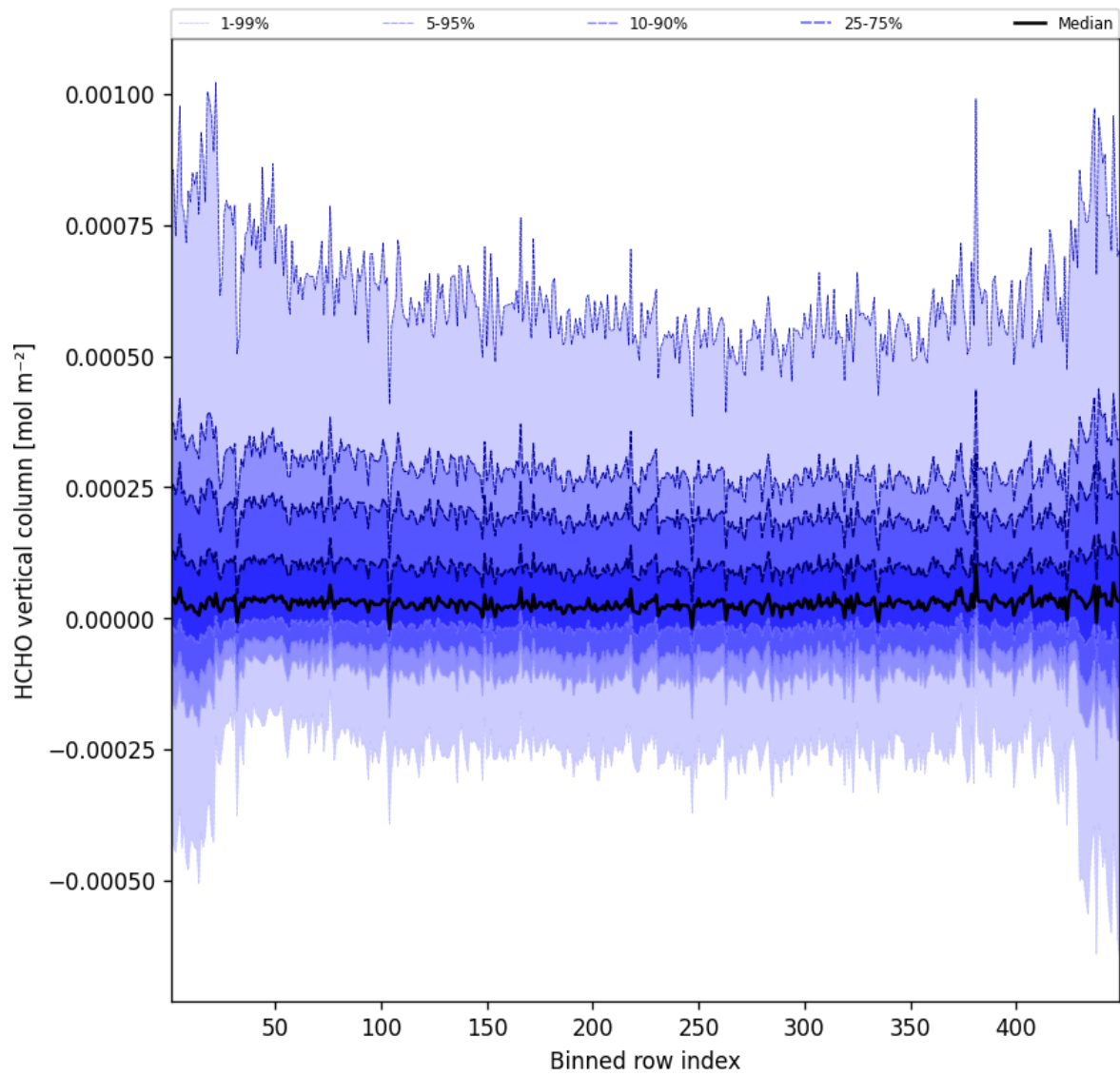
Figure 47: Along track statistics of “HCHO vertical column” for 2024-12-17 to 2024-12-18
