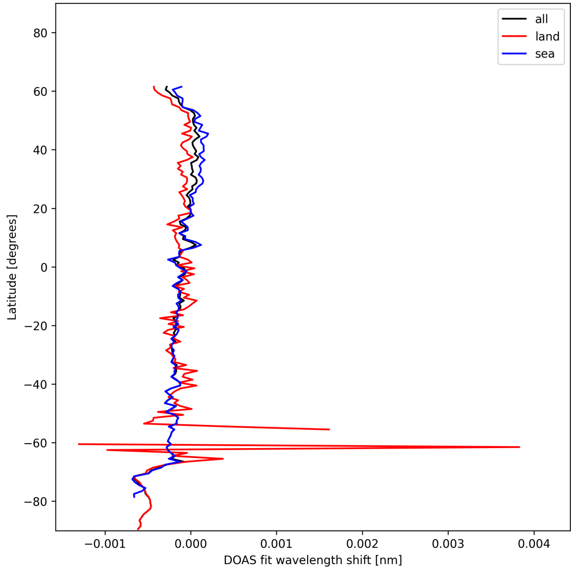
Figure 28: Zonal average of “DOAS fit wavelength shift” for 2024-12-17 to 2024-12-18.
