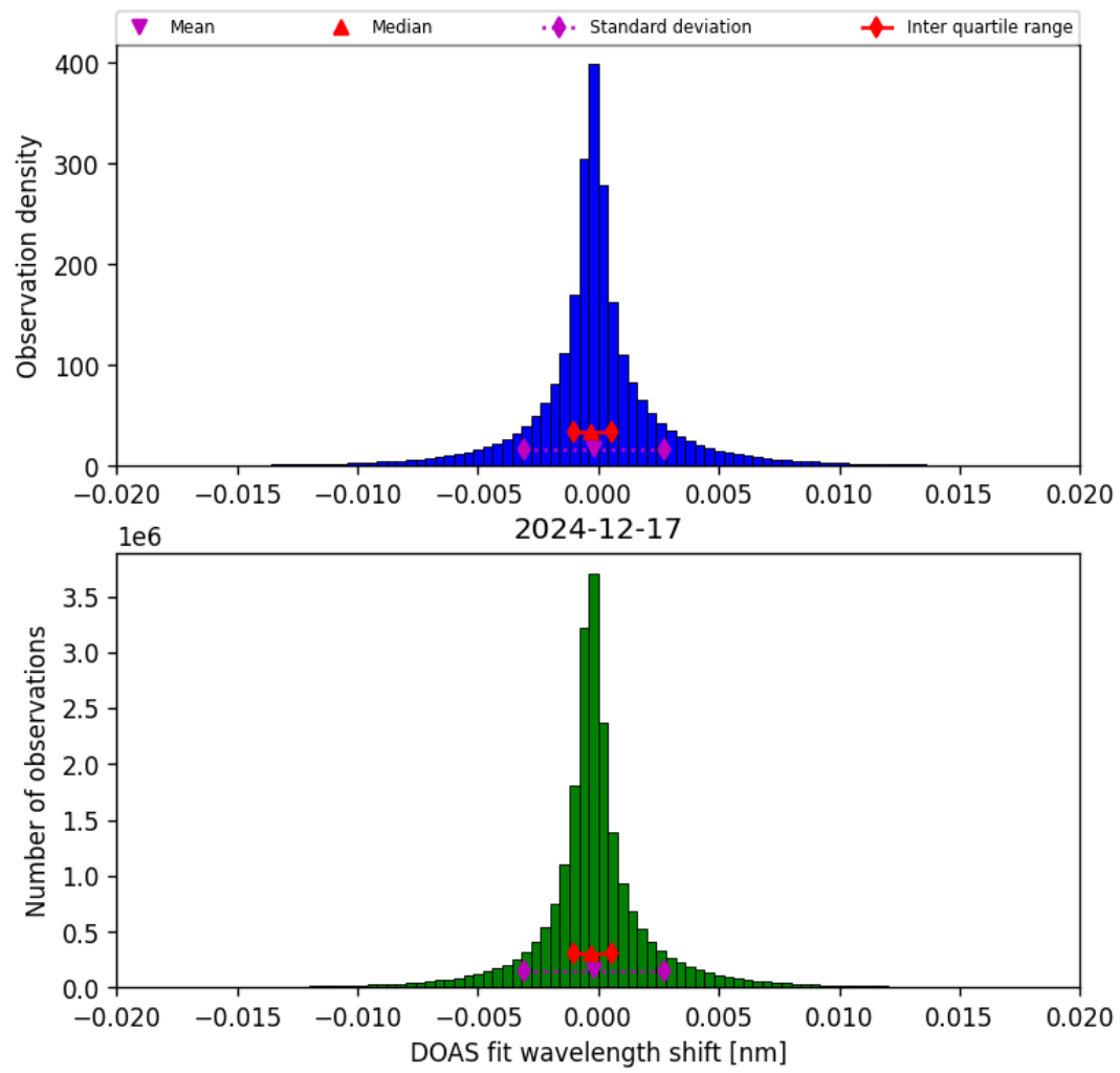
Figure 42: Histogram of “DOAS fit wavelength shift” for 2024-12-17 to 2024-12-18
