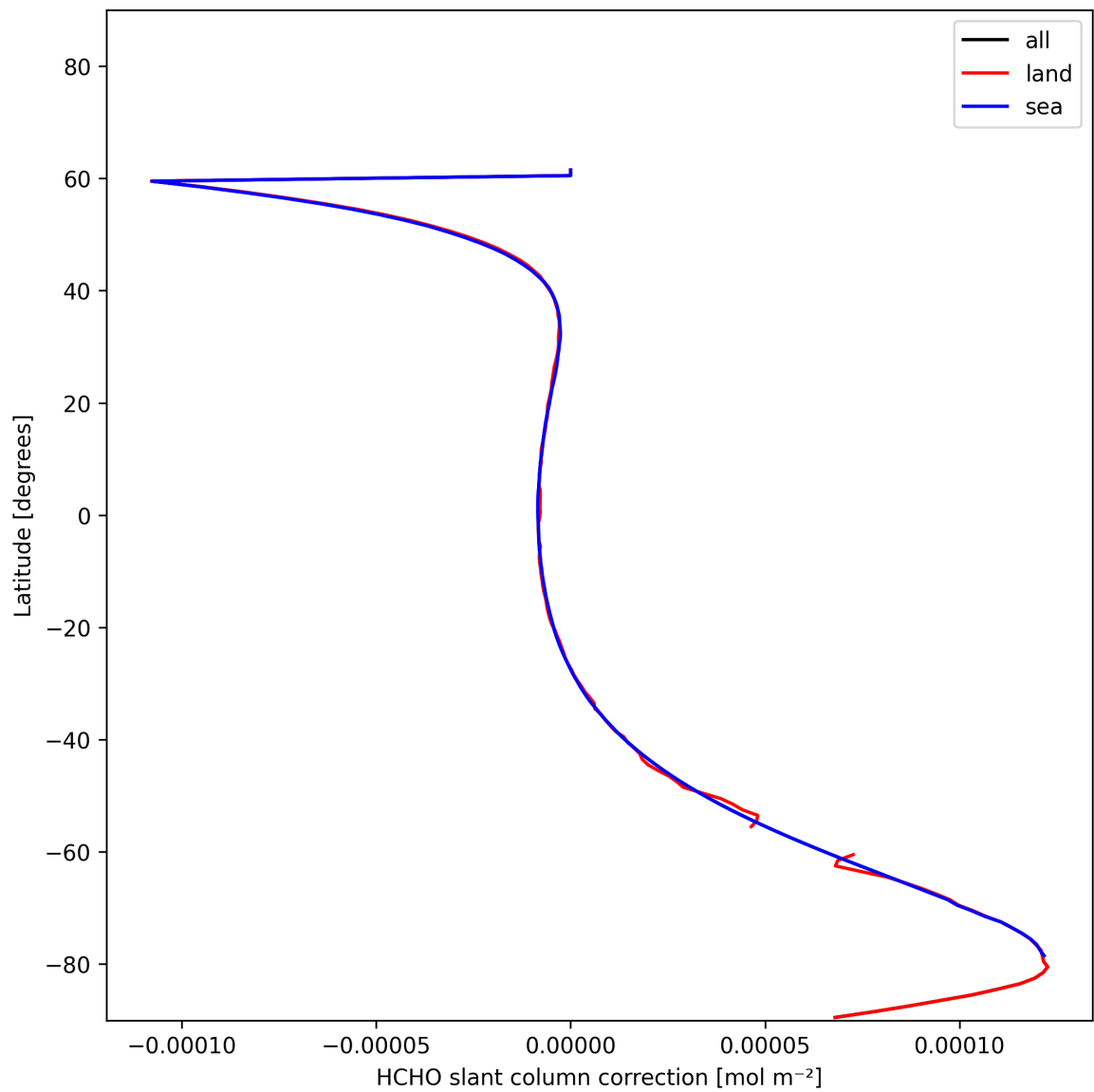
Figure 31: Zonal average of “HCHO slant column correction” for 2024-12-17 to 2024-12-18.
