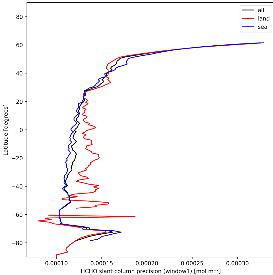
Figure 23: Zonal average of “HCHO slant column precision (window1)” for 2024-12-17 to 2024-12-18.
