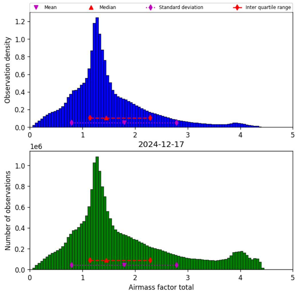
Figure 38: Histogram of “Airmass factor total” for 2024-12-17 to 2024-12-18
