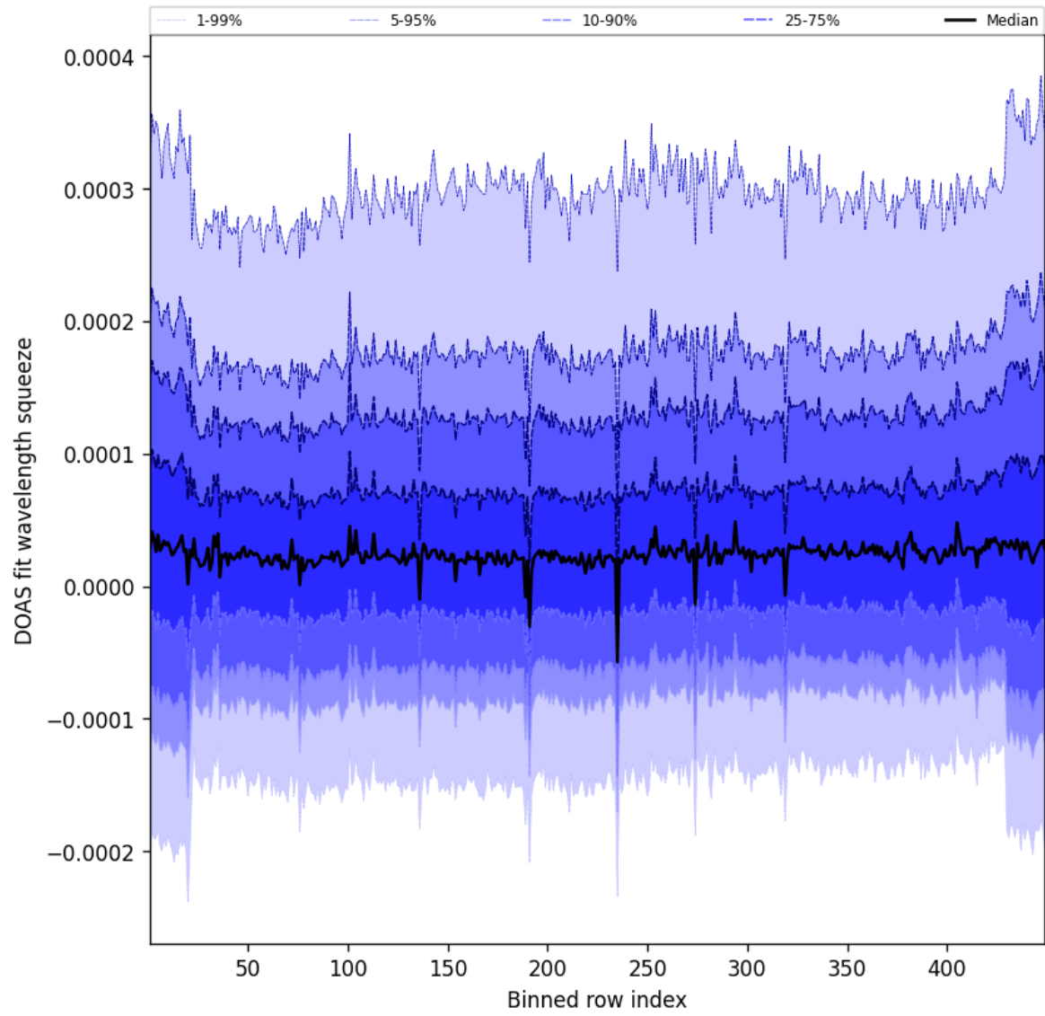
Figure 57: Along track statistics of “DOAS fit wavelength squeeze” for 2024-12-17 to 2024-12-18
