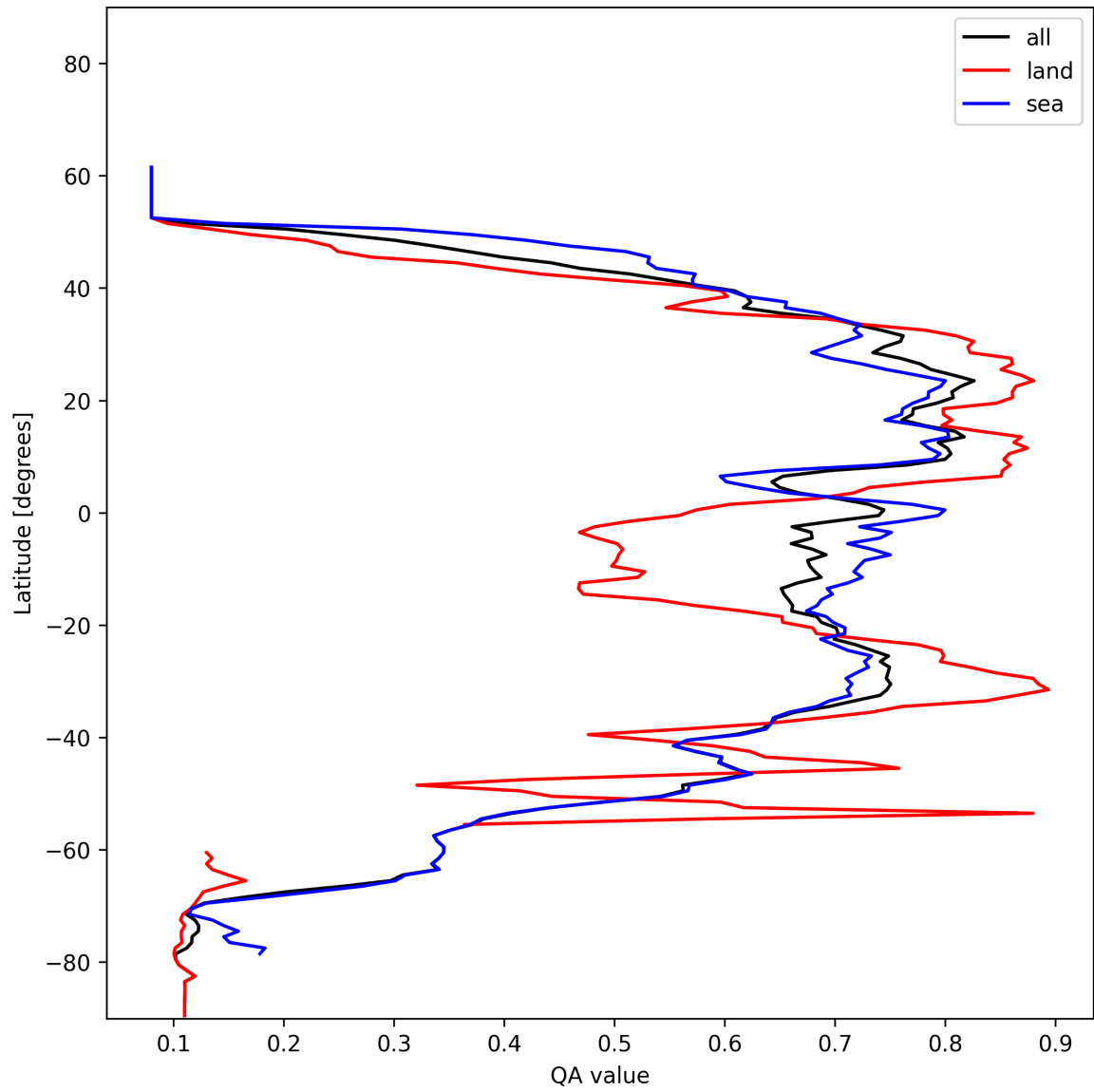
Figure 18: Zonal average of “QA value” for 2024-12-17 to 2024-12-18.
