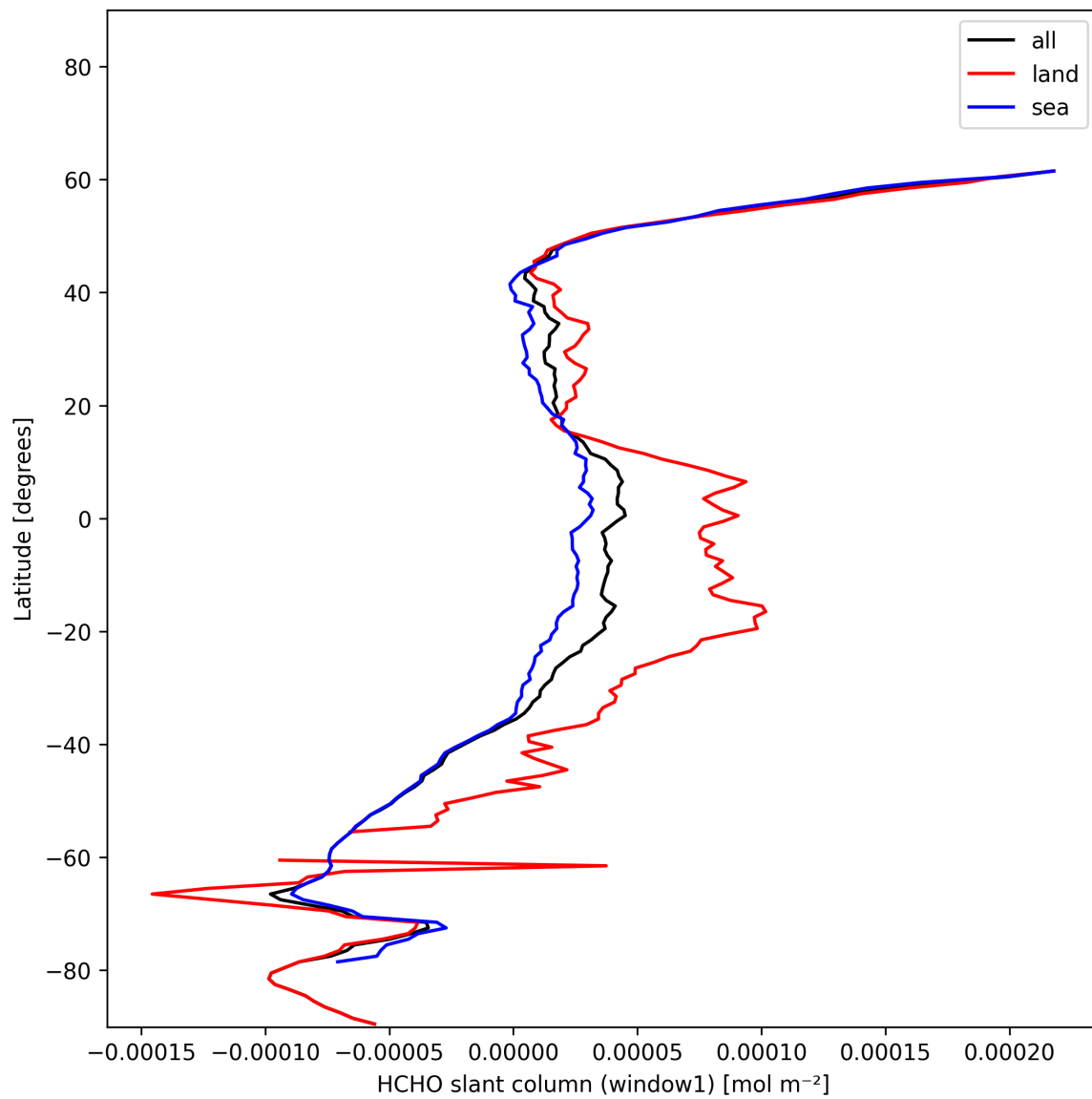
Figure 22: Zonal average of “HCHO slant column (window1)” for 2024-12-17 to 2024-12-18.
