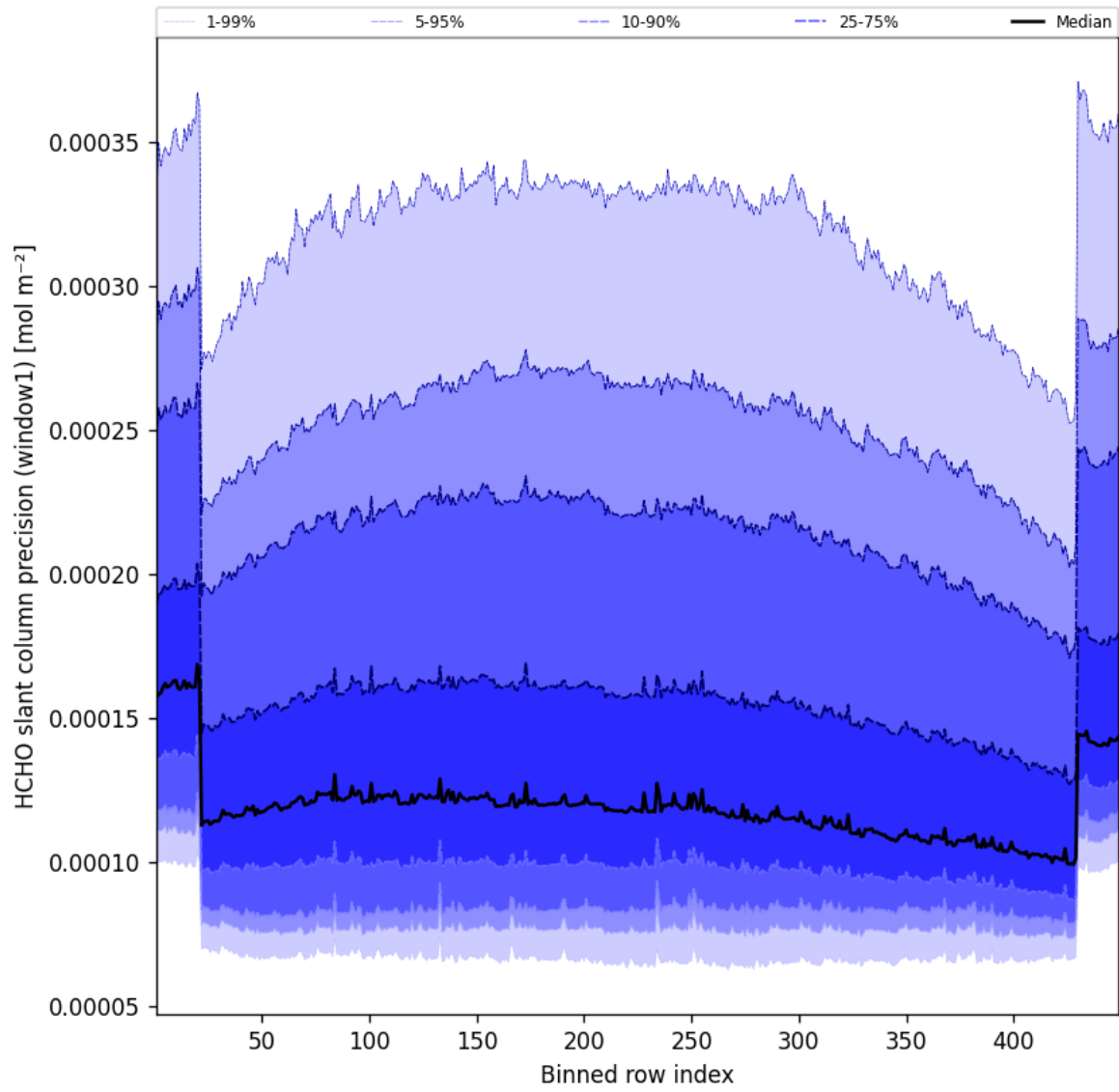
Figure 51: Along track statistics of “HCHO slant column precision (window1)” for 2024-12-18 to 2024-12-19
