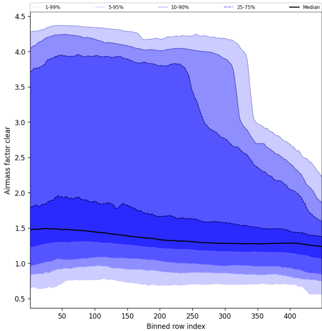
Figure 54: Along track statistics of “Airmass factor clear” for 2024-12-18 to 2024-12-19
