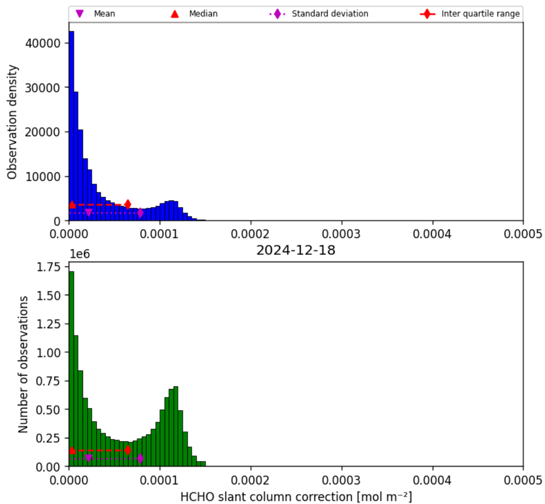
Figure 45: Histogram of “HCHO slant column correction” for 2024-12-18 to 2024-12-19
