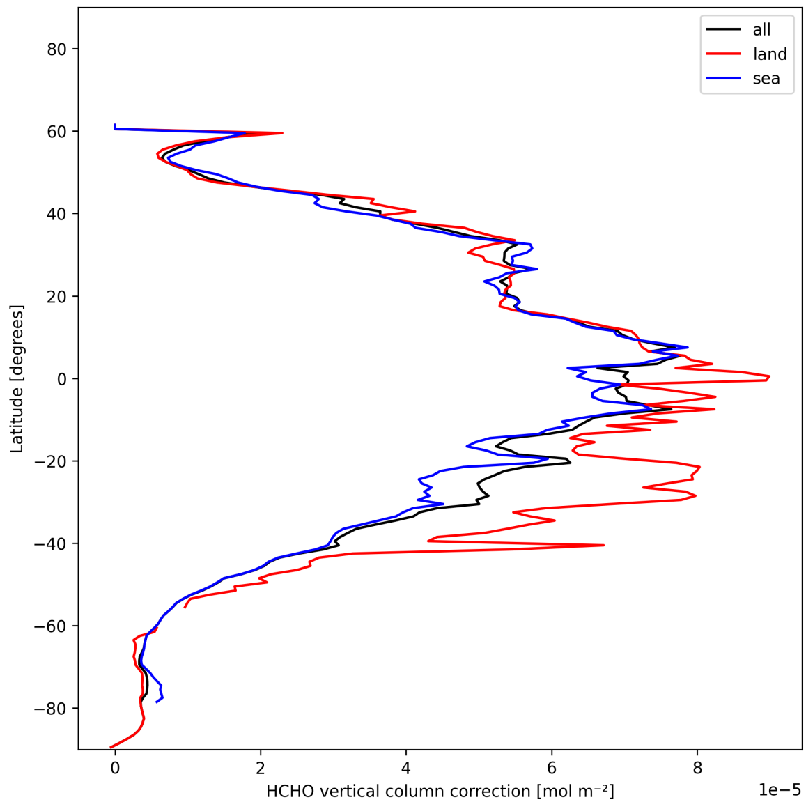
Figure 21: Zonal average of “HCHO vertical column correction” for 2024-12-18 to 2024-12-19.
