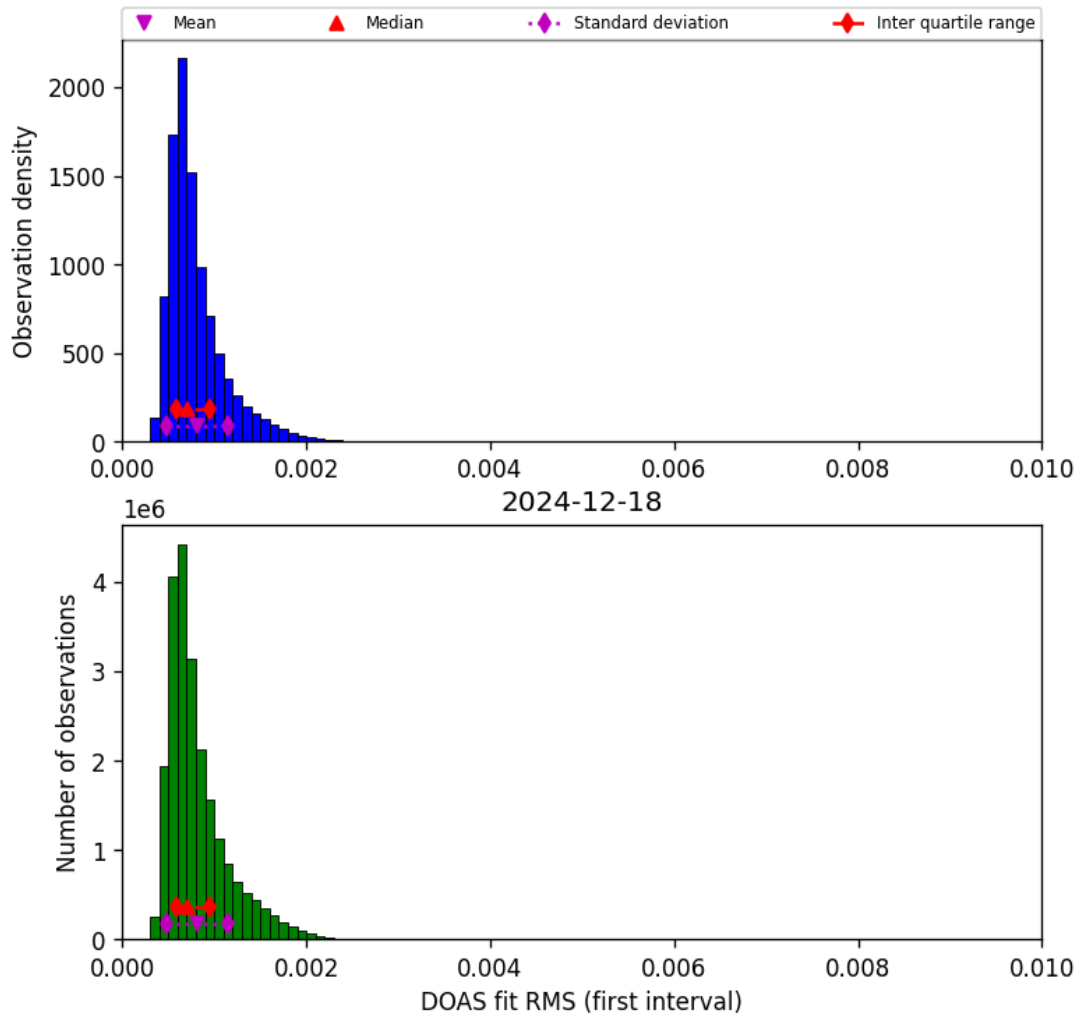
Figure 44: Histogram of “DOAS fit RMS (first interval)” for 2024-12-18 to 2024-12-19
