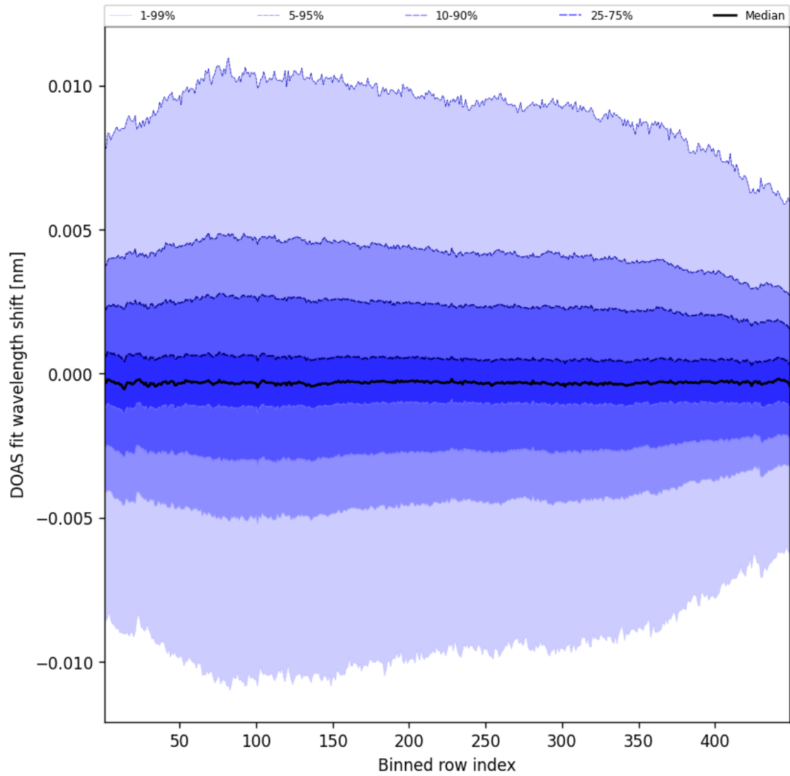
Figure 56: Along track statistics of “DOAS fit wavelength shift” for 2024-12-18 to 2024-12-19
