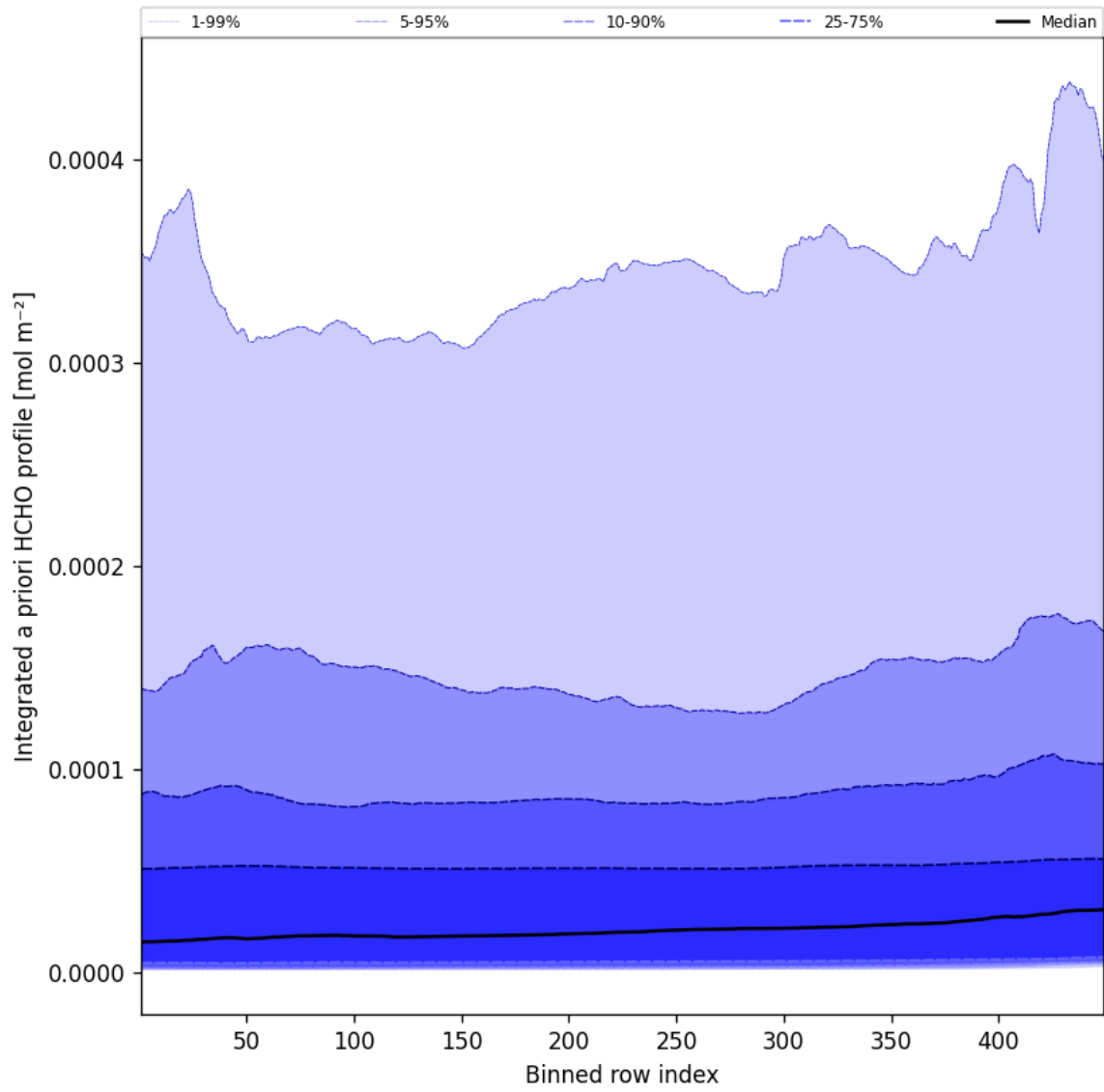
Figure 55: Along track statistics of “Integrated a priori HCHO profile” for 2024-12-18 to 2024-12-19
