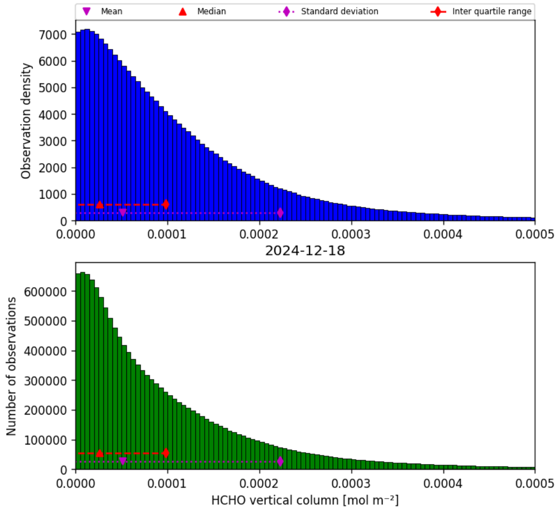
Figure 33: Histogram of “HCHO vertical column” for 2024-12-18 to 2024-12-19
