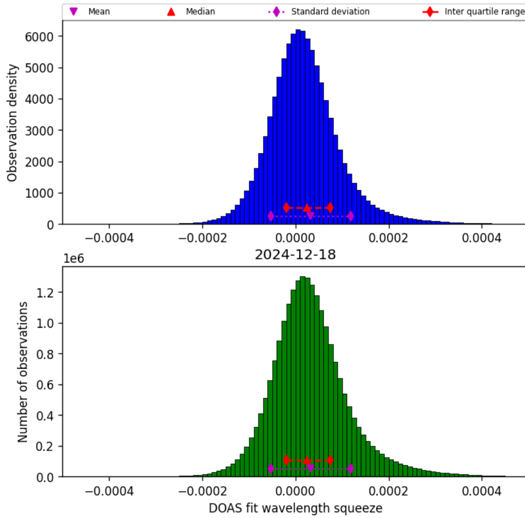
Figure 43: Histogram of “DOAS fit wavelength squeeze” for 2024-12-18 to 2024-12-19
