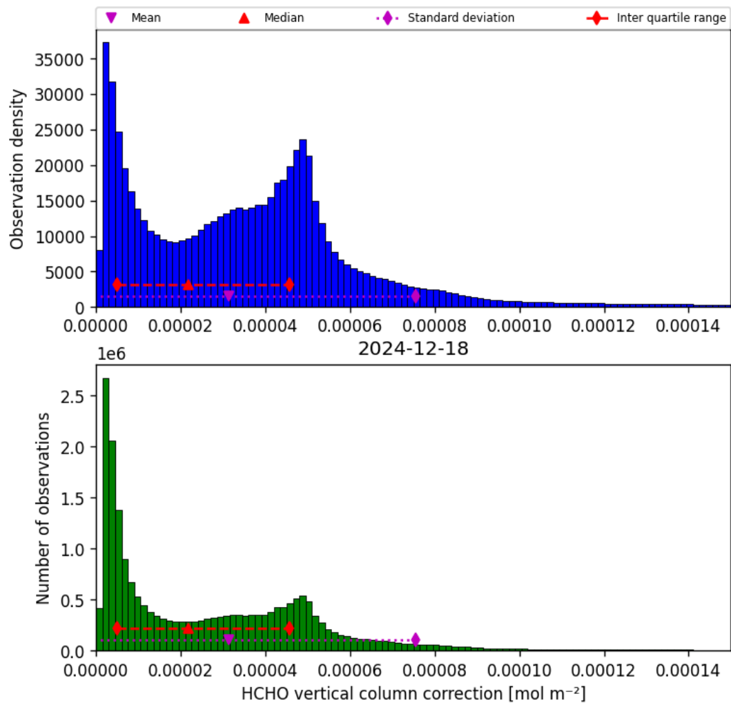
Figure 35: Histogram of “HCHO vertical column correction” for 2024-12-18 to 2024-12-19
