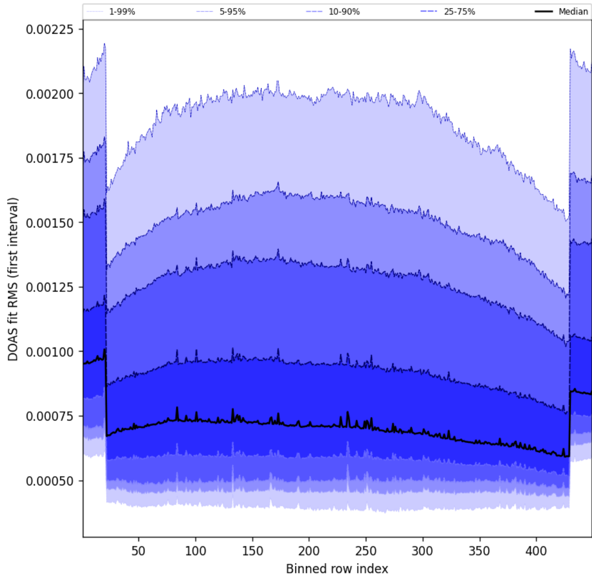
Figure 58: Along track statistics of “DOAS fit RMS (first interval)” for 2024-12-18 to 2024-12-19
