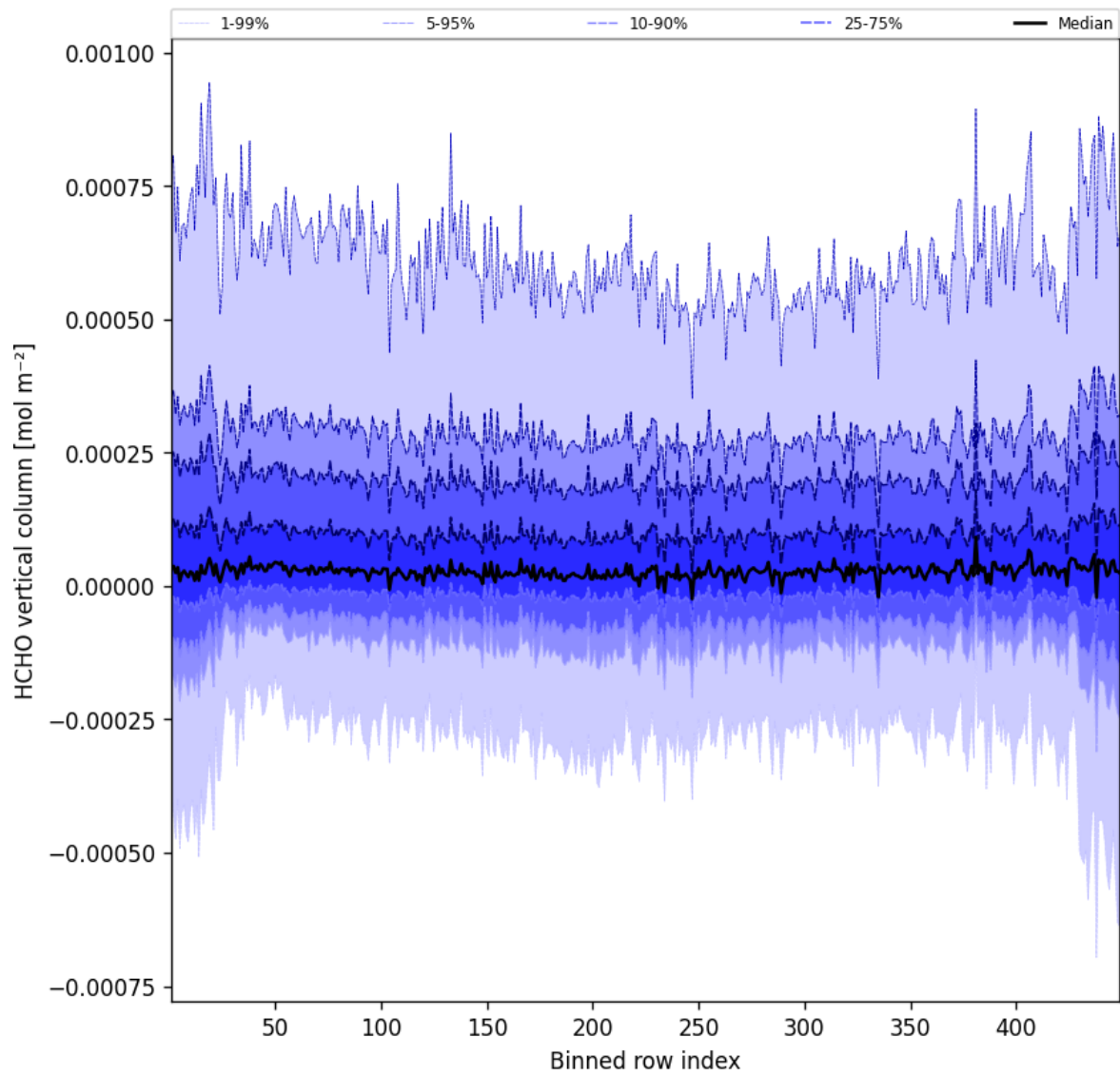
Figure 47: Along track statistics of “HCHO vertical column” for 2024-12-18 to 2024-12-19
