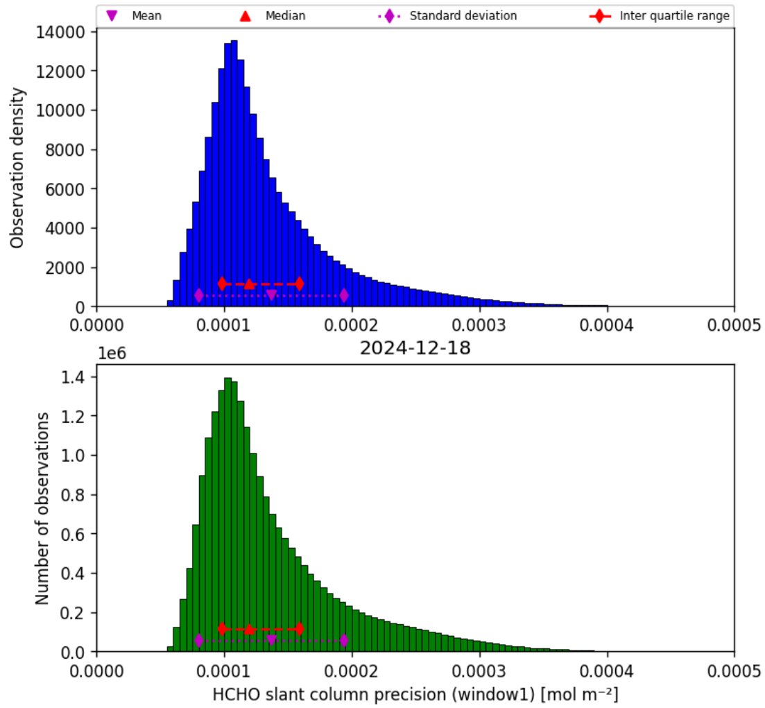
Figure 37: Histogram of “HCHO slant column precision (window1)” for 2024-12-18 to 2024-12-19
