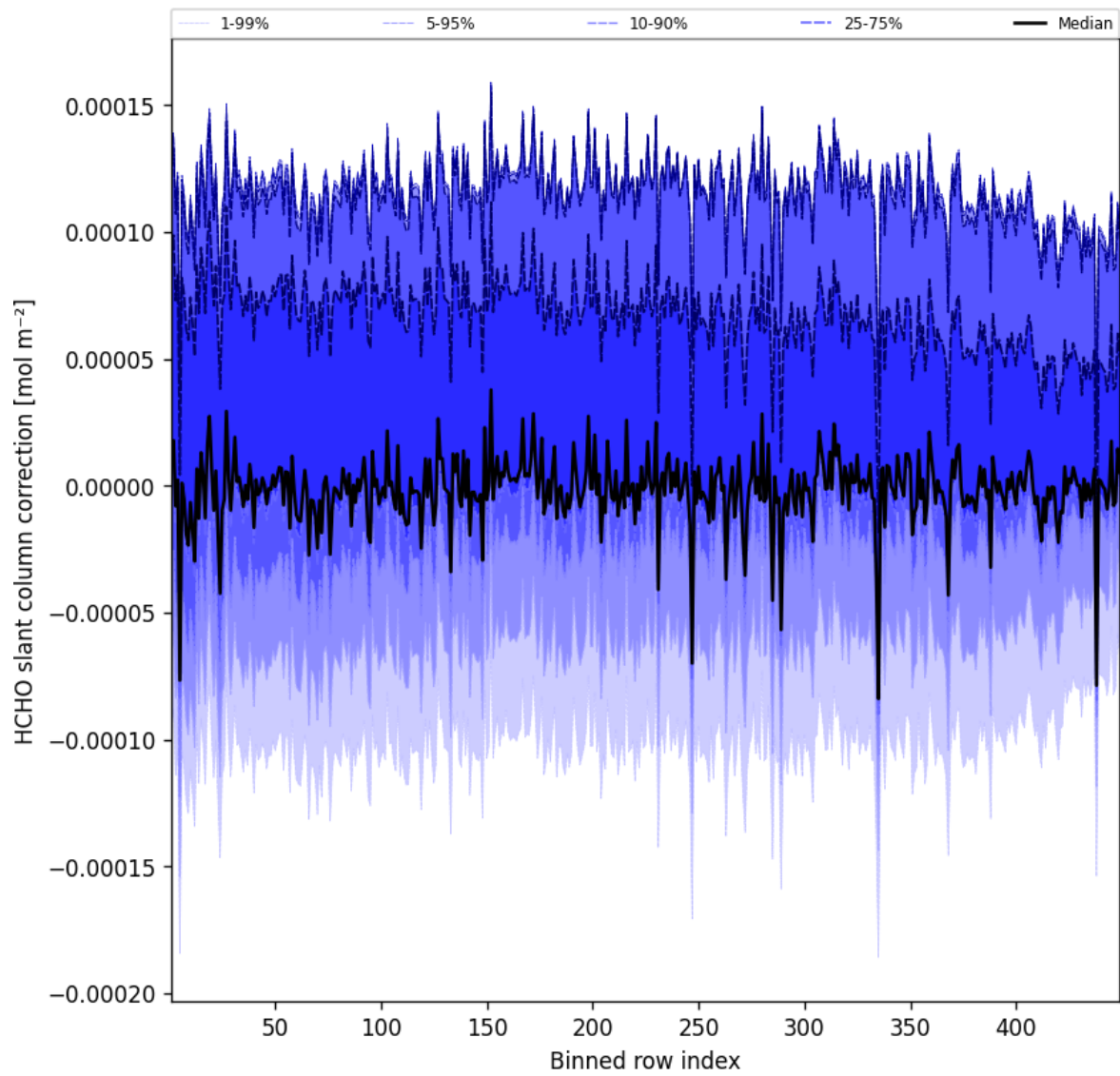
Figure 59: Along track statistics of “HCHO slant column correction” for 2024-12-18 to 2024-12-19
