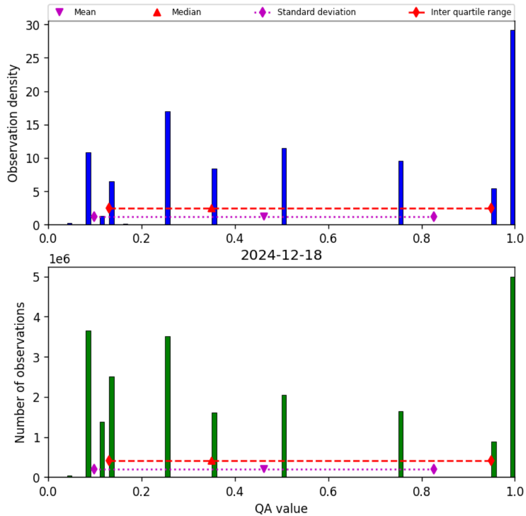
Figure 32: Histogram of “QA value” for 2024-12-18 to 2024-12-19
