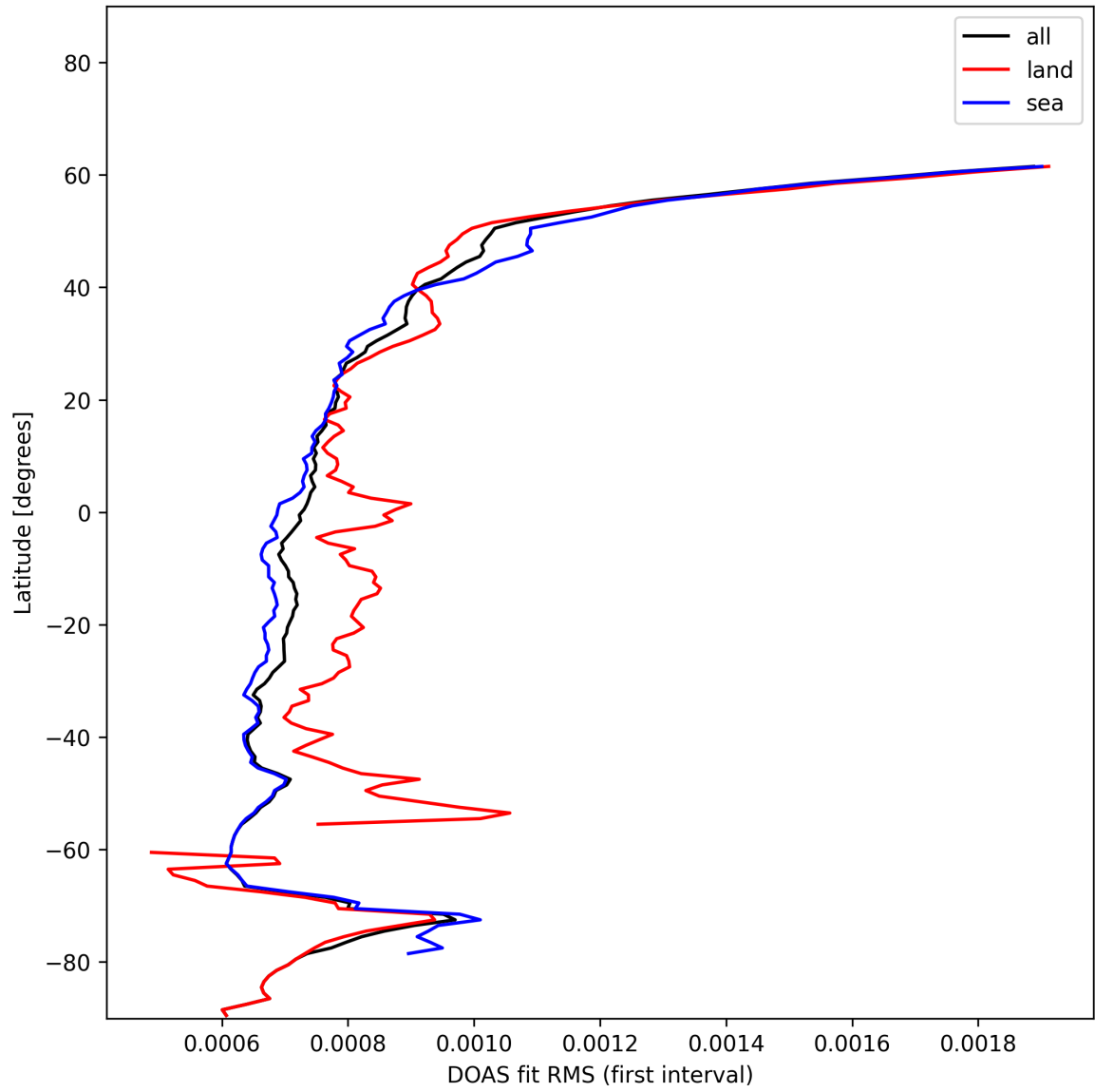
Figure 30: Zonal average of “DOAS fit RMS (first interval)” for 2024-12-18 to 2024-12-19.
