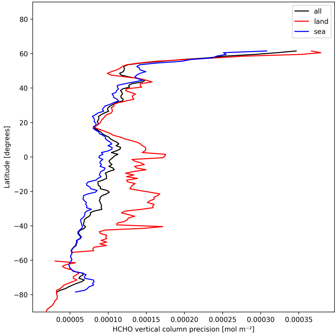
Figure 20: Zonal average of “HCHO vertical column precision” for 2024-12-18 to 2024-12-19.
