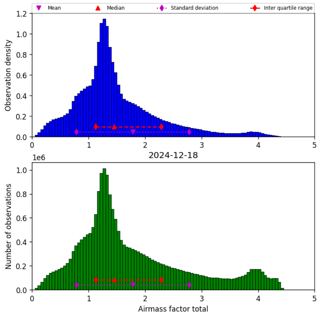
Figure 38: Histogram of “Airmass factor total” for 2024-12-18 to 2024-12-19
