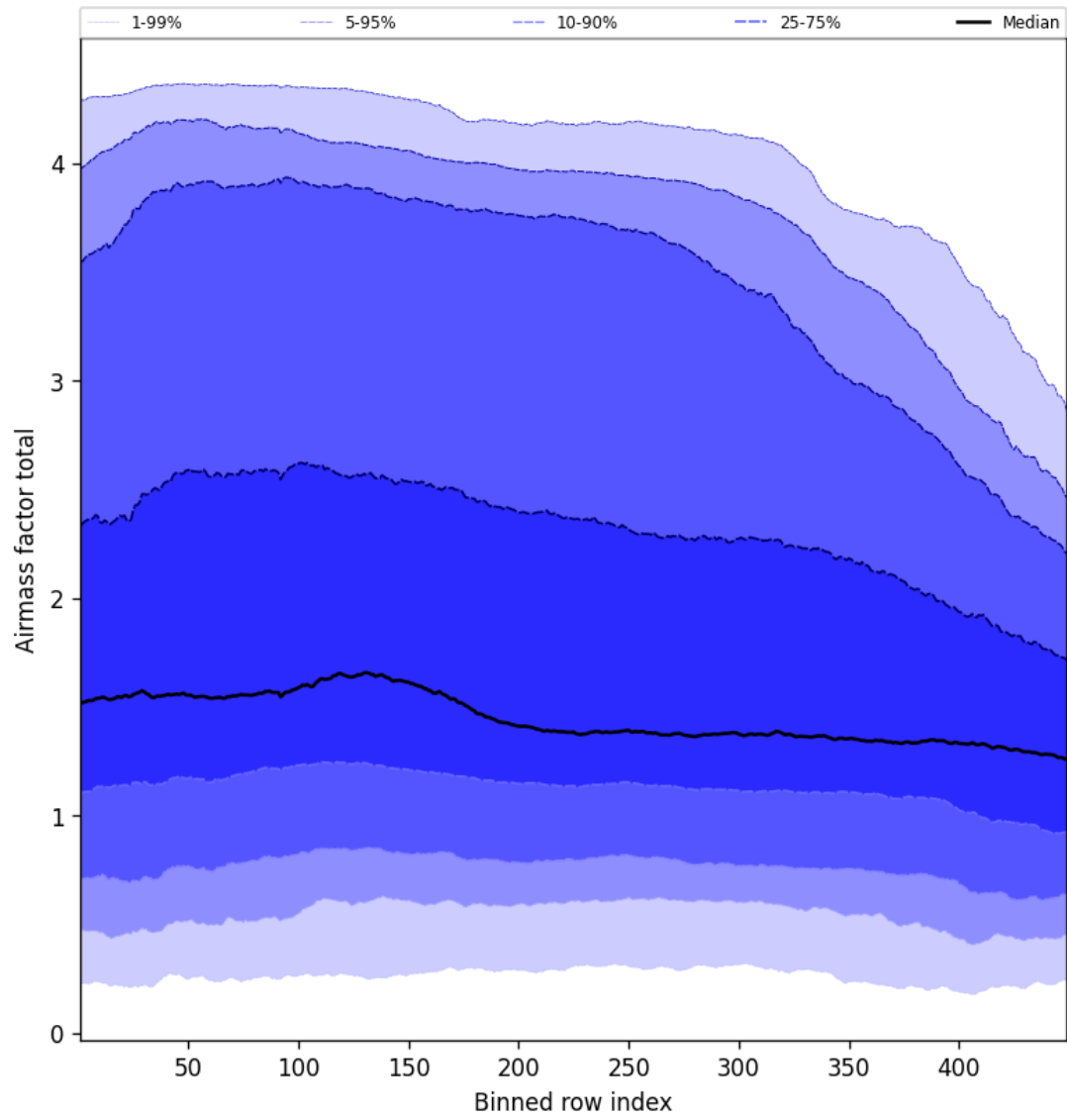
Figure 52: Along track statistics of “Airmass factor total” for 2024-12-18 to 2024-12-19
