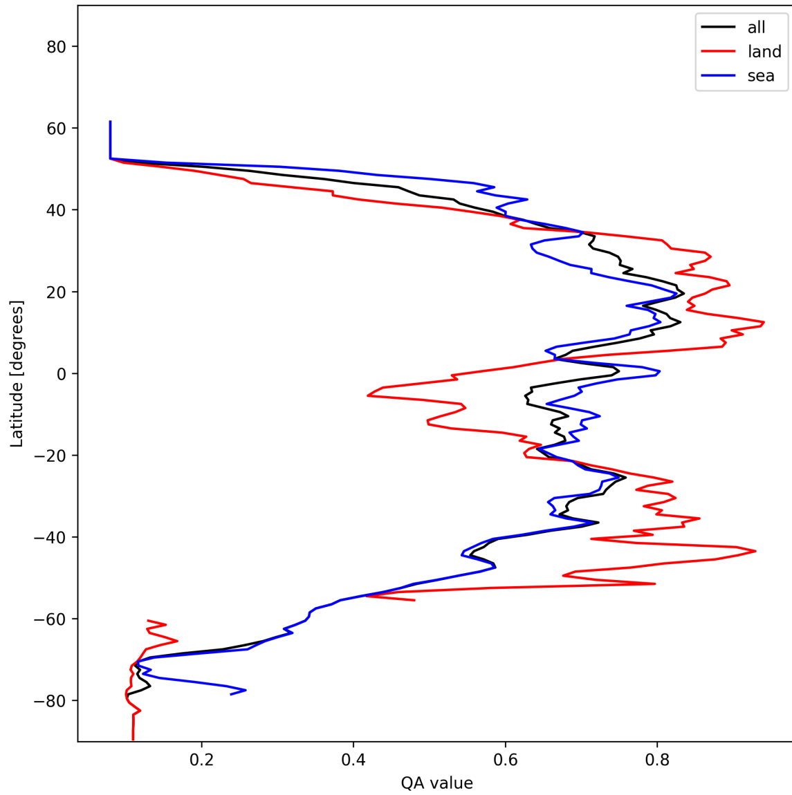
Figure 18: Zonal average of “QA value” for 2024-12-18 to 2024-12-19.
