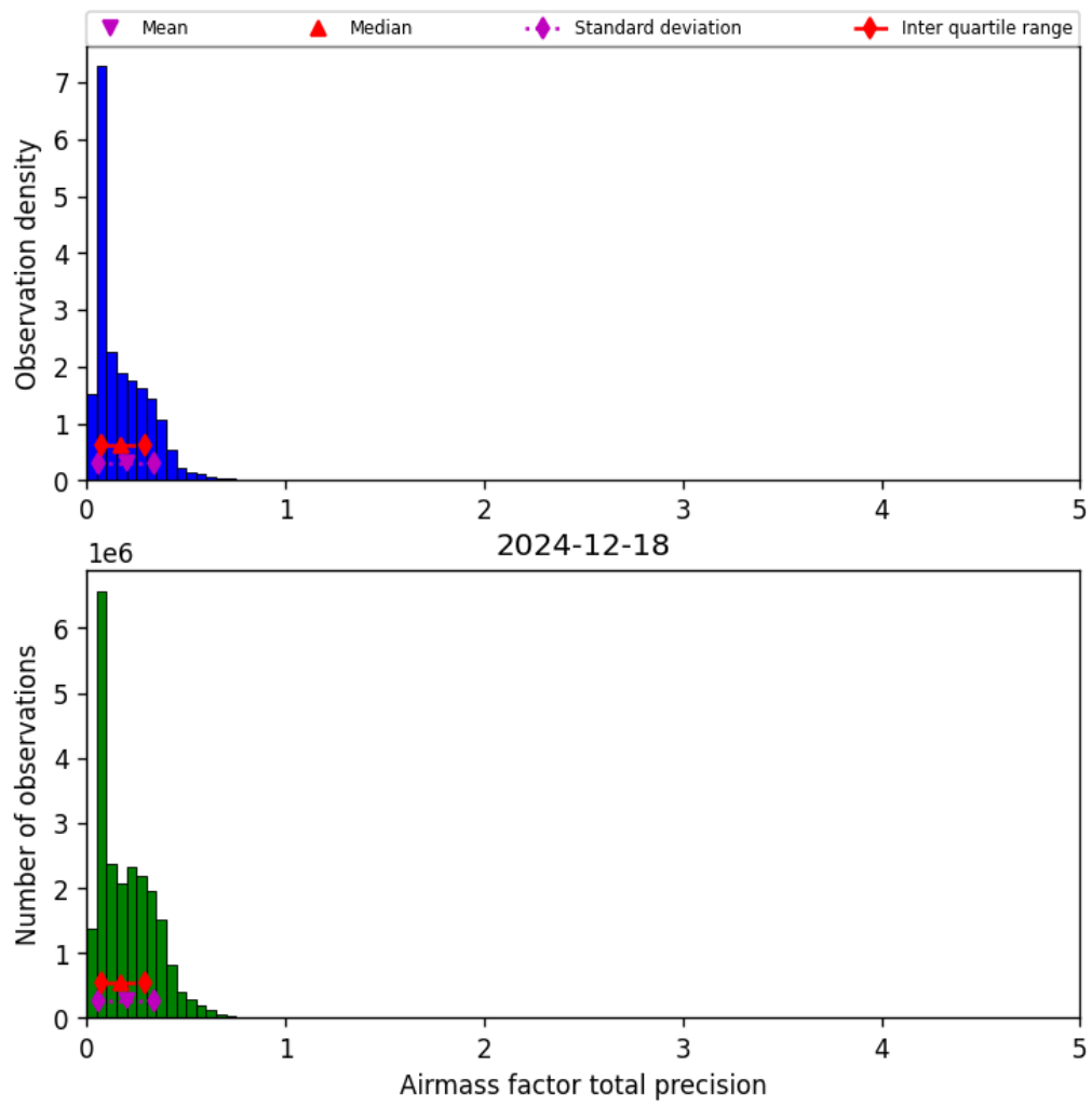
Figure 39: Histogram of “Airmass factor total precision” for 2024-12-18 to 2024-12-19
