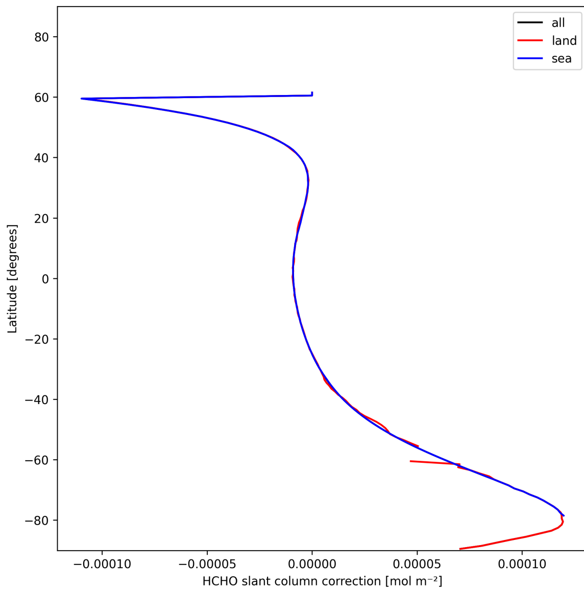
Figure 31: Zonal average of “HCHO slant column correction” for 2024-12-18 to 2024-12-19.
