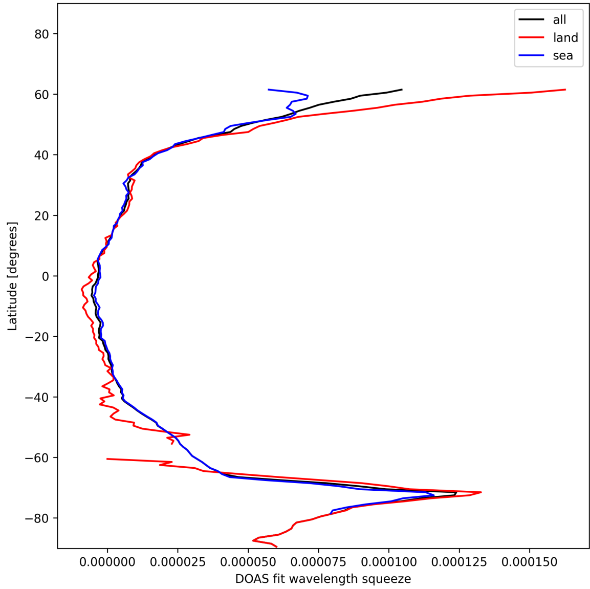
Figure 29: Zonal average of “DOAS fit wavelength squeeze” for 2024-12-18 to 2024-12-19.
