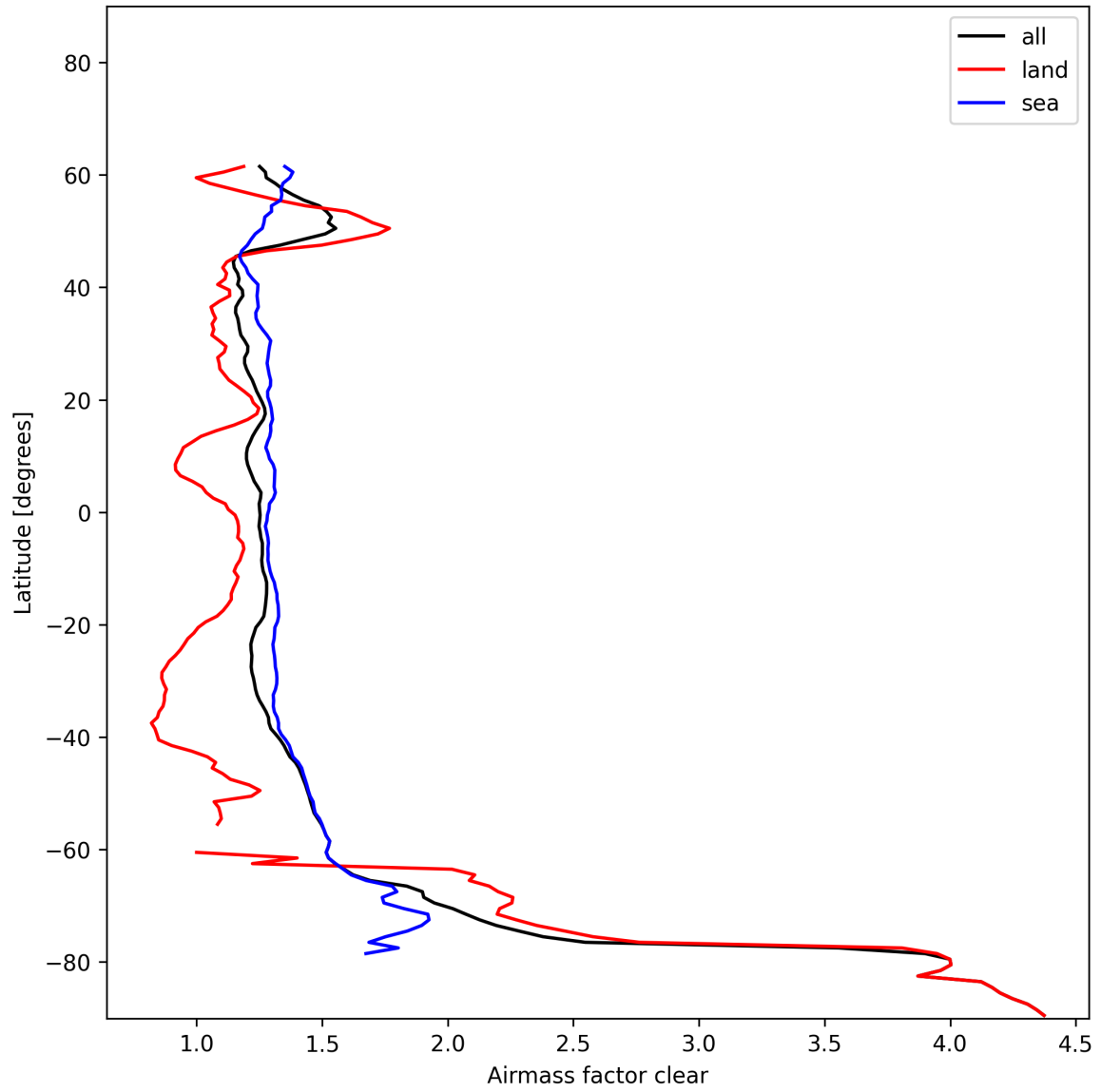
Figure 26: Zonal average of “Airmass factor clear” for 2024-12-18 to 2024-12-19.
