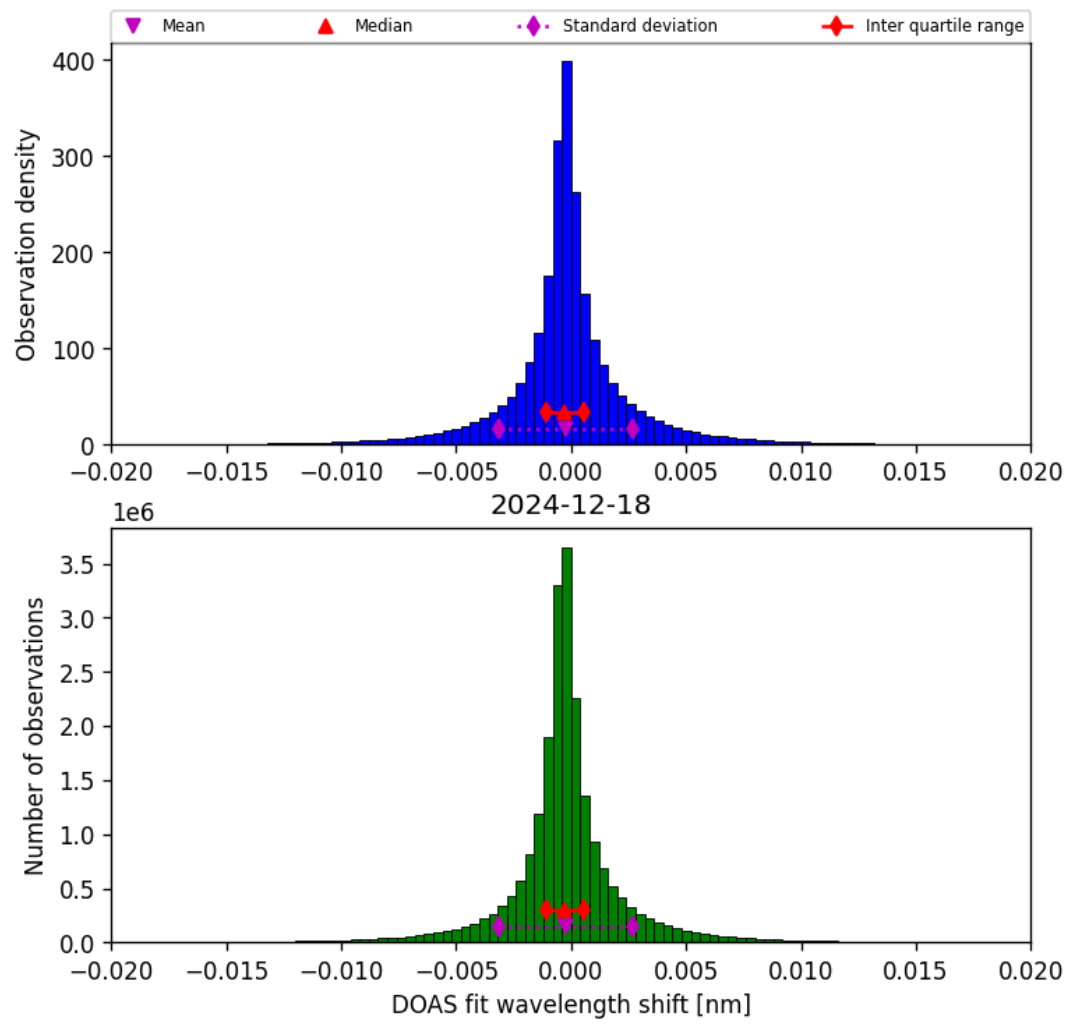
Figure 42: Histogram of “DOAS fit wavelength shift” for 2024-12-18 to 2024-12-19
