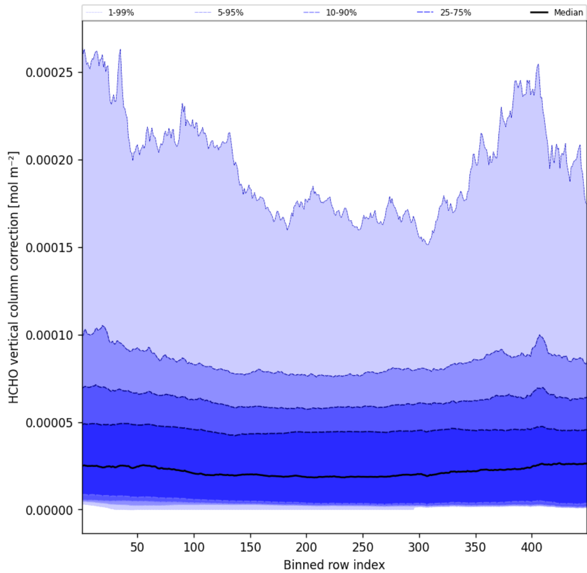
Figure 49: Along track statistics of “HCHO vertical column correction” for 2024-12-18 to 2024-12-19
