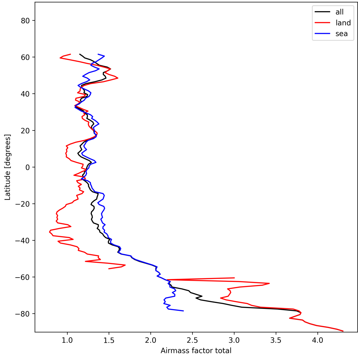
Figure 24: Zonal average of “Airmass factor total” for 2024-12-18 to 2024-12-19.
