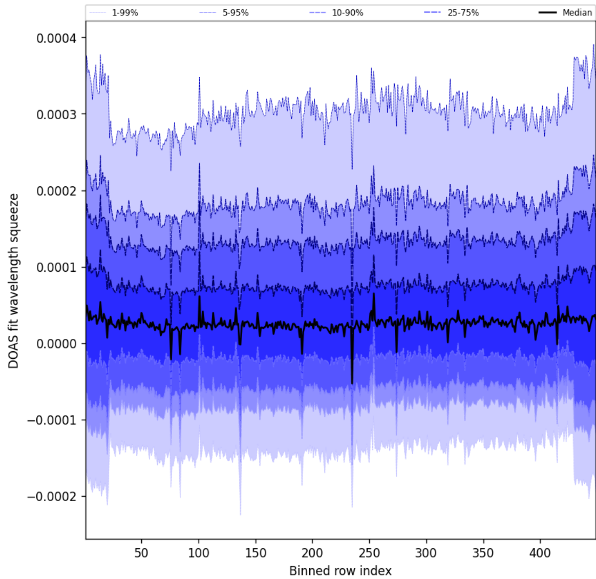
Figure 57: Along track statistics of “DOAS fit wavelength squeeze” for 2024-12-18 to 2024-12-19
