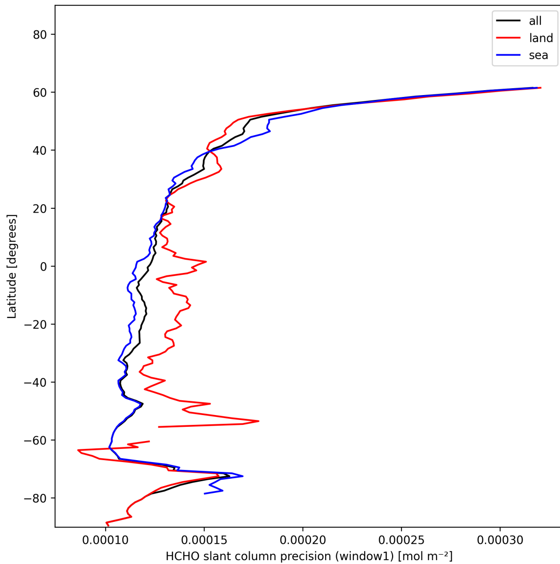
Figure 23: Zonal average of “HCHO slant column precision (window1)” for 2024-12-18 to 2024-12-19.
