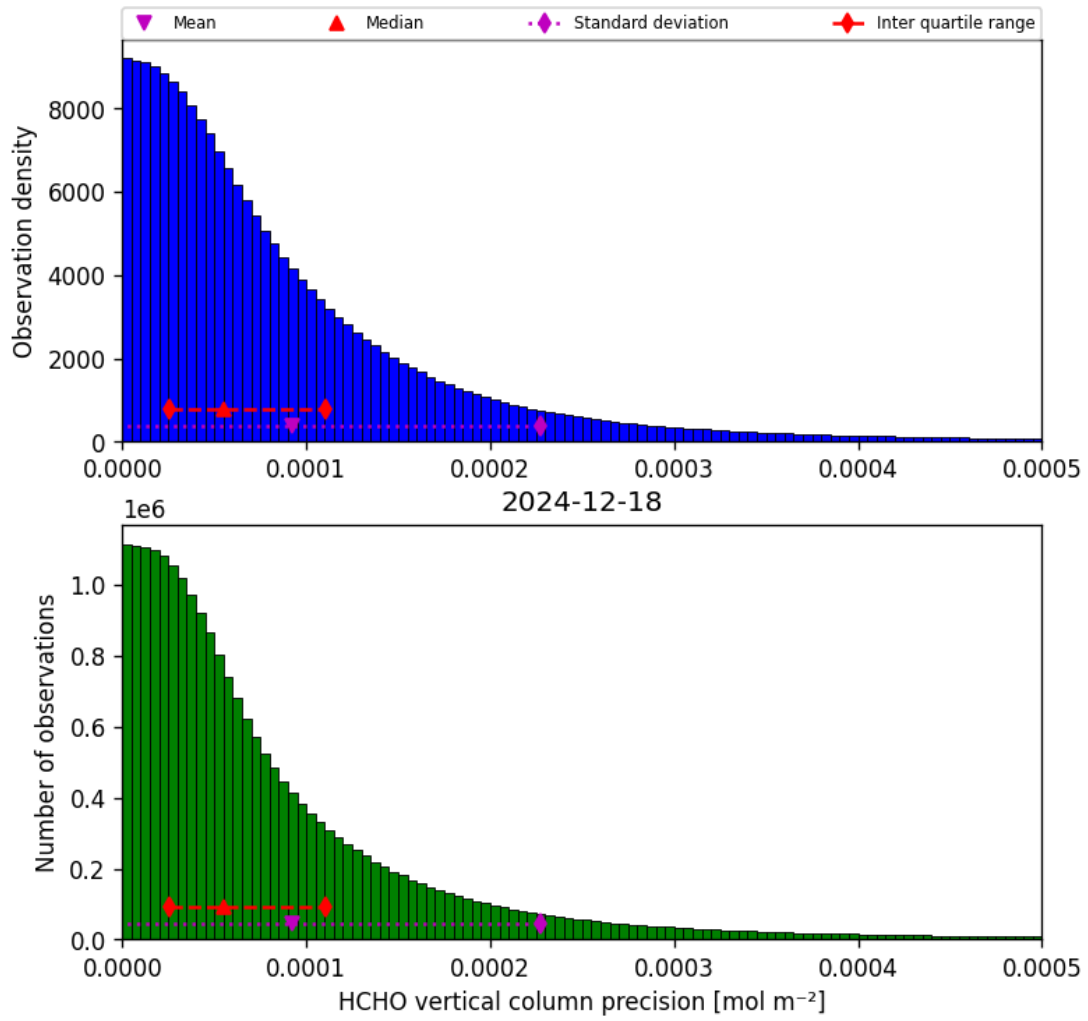
Figure 34: Histogram of “HCHO vertical column precision” for 2024-12-18 to 2024-12-19
