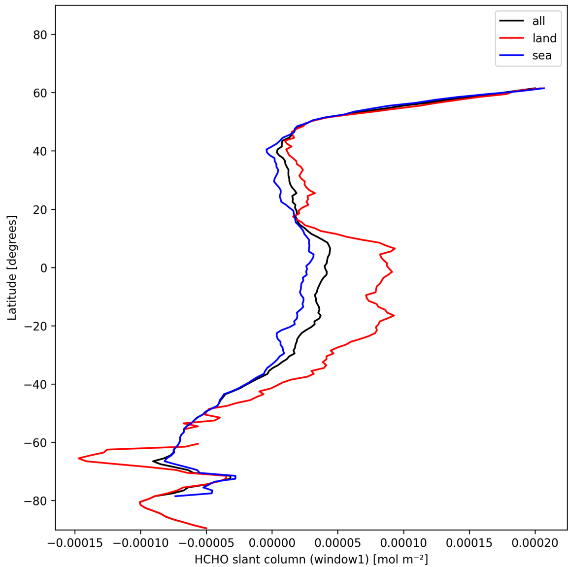
Figure 22: Zonal average of “HCHO slant column (window1)” for 2024-12-18 to 2024-12-19.
