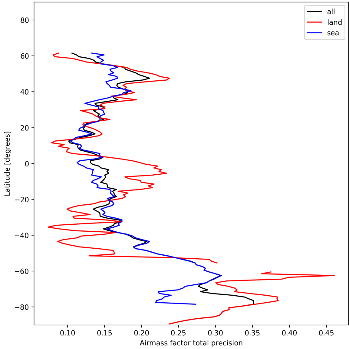
Figure 25: Zonal average of “Airmass factor total precision” for 2024-12-18 to 2024-12-19.
