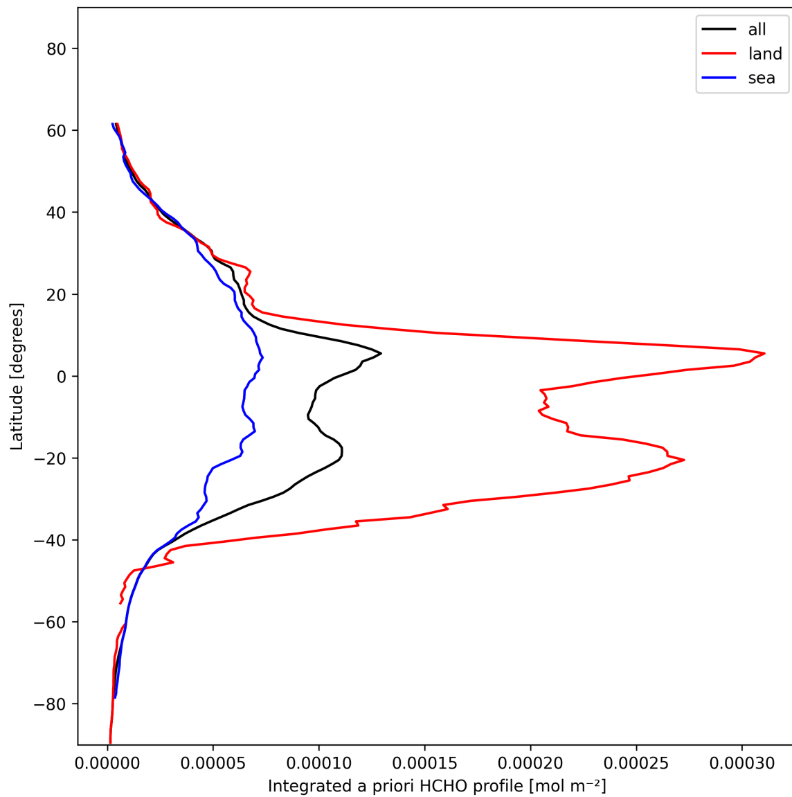
Figure 27: Zonal average of “Integrated a priori HCHO profile” for 2024-12-18 to 2024-12-19.
