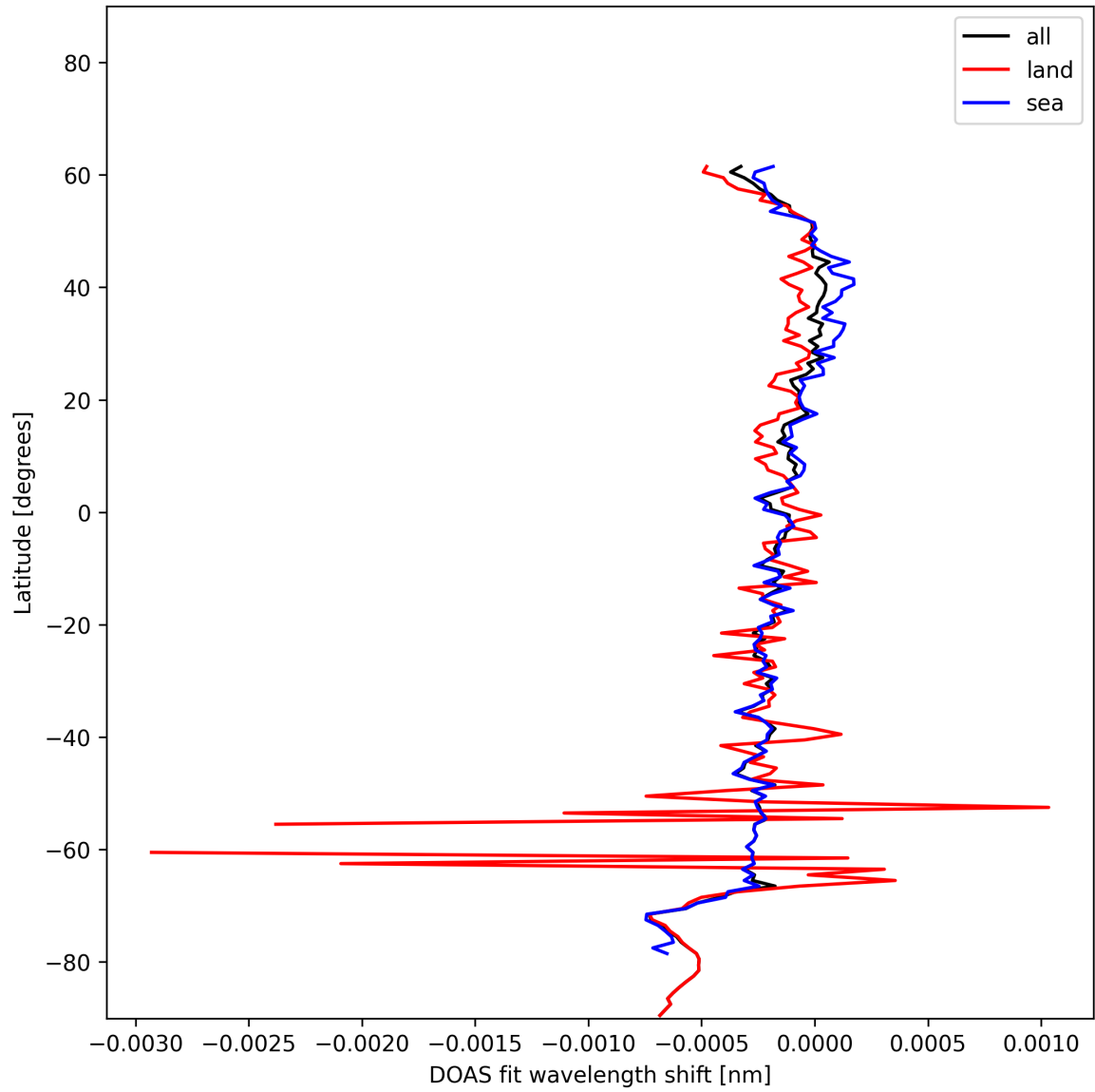
Figure 28: Zonal average of “DOAS fit wavelength shift” for 2024-12-18 to 2024-12-19.
