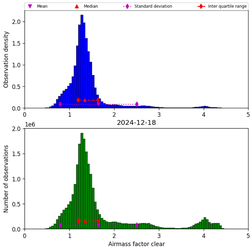
Figure 40: Histogram of “Airmass factor clear” for 2024-12-18 to 2024-12-19
