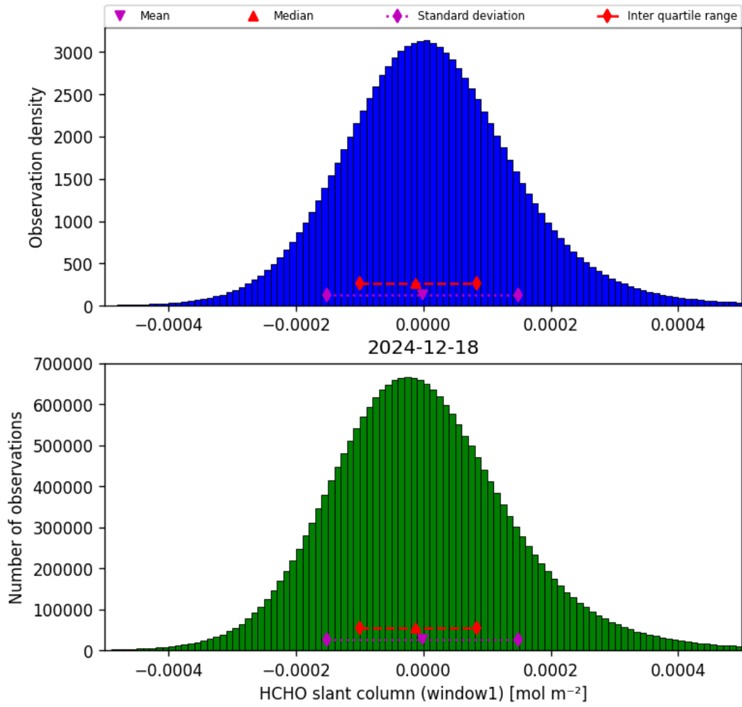
Figure 36: Histogram of “HCHO slant column (window1)” for 2024-12-18 to 2024-12-19
