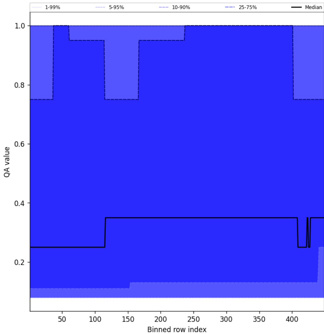
Figure 46: Along track statistics of “QA value” for 2024-12-18 to 2024-12-19
