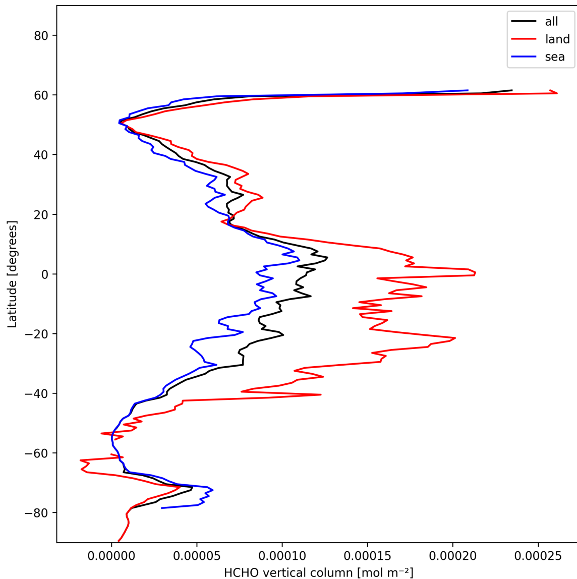
Figure 19: Zonal average of “HCHO vertical column” for 2024-12-18 to 2024-12-19.
