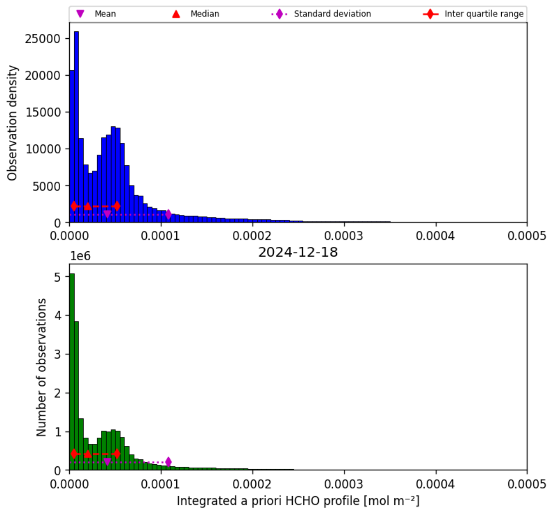
Figure 41: Histogram of “Integrated a priori HCHO profile” for 2024-12-18 to 2024-12-19
