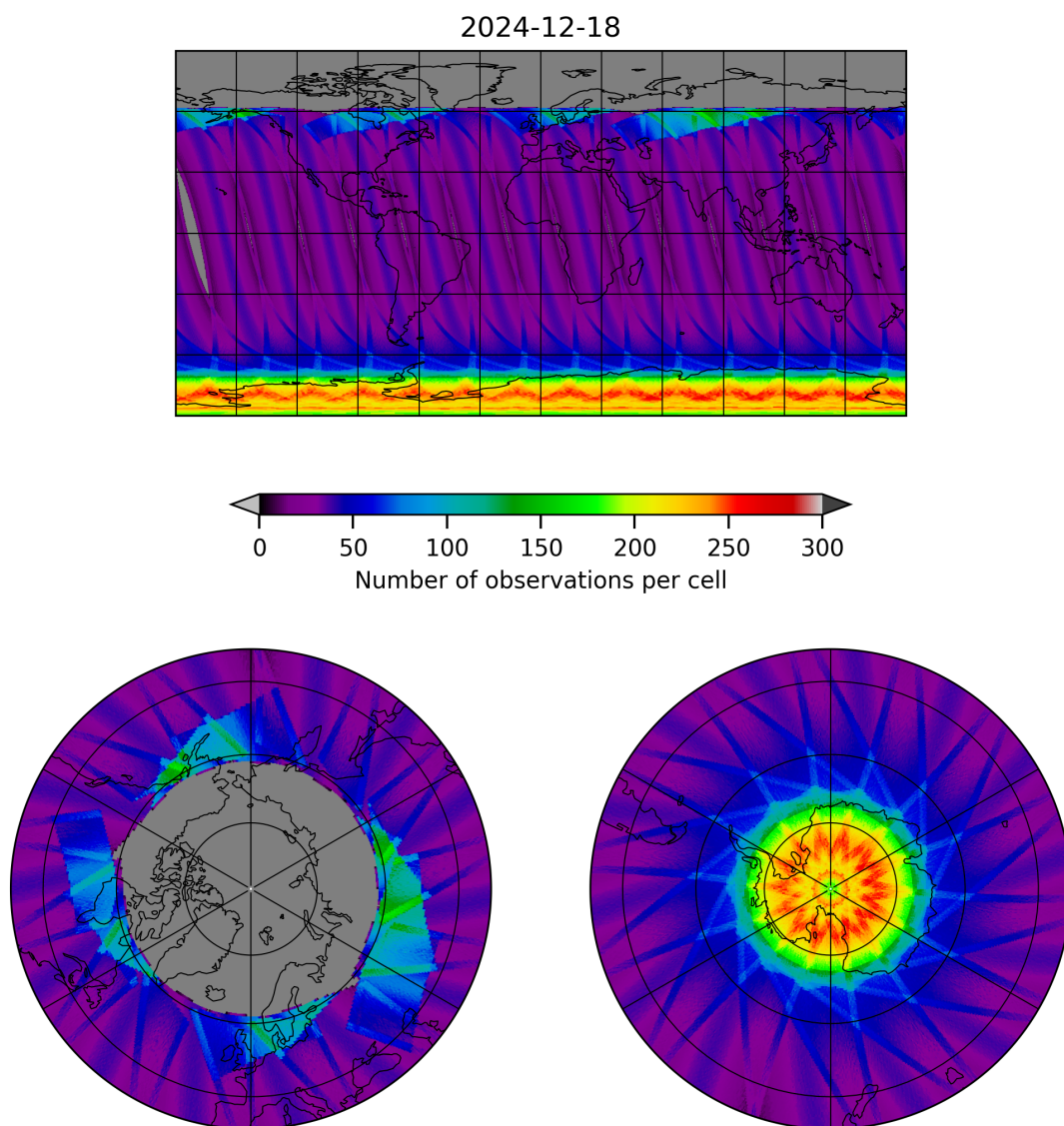
Figure 17: Map of the number of observations for 2024-12-18 to 2024-12-19
