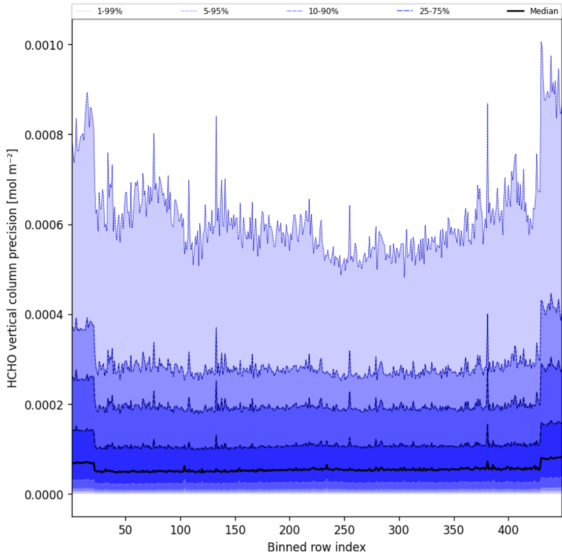
Figure 48: Along track statistics of “HCHO vertical column precision” for 2024-12-18 to 2024-12-19
