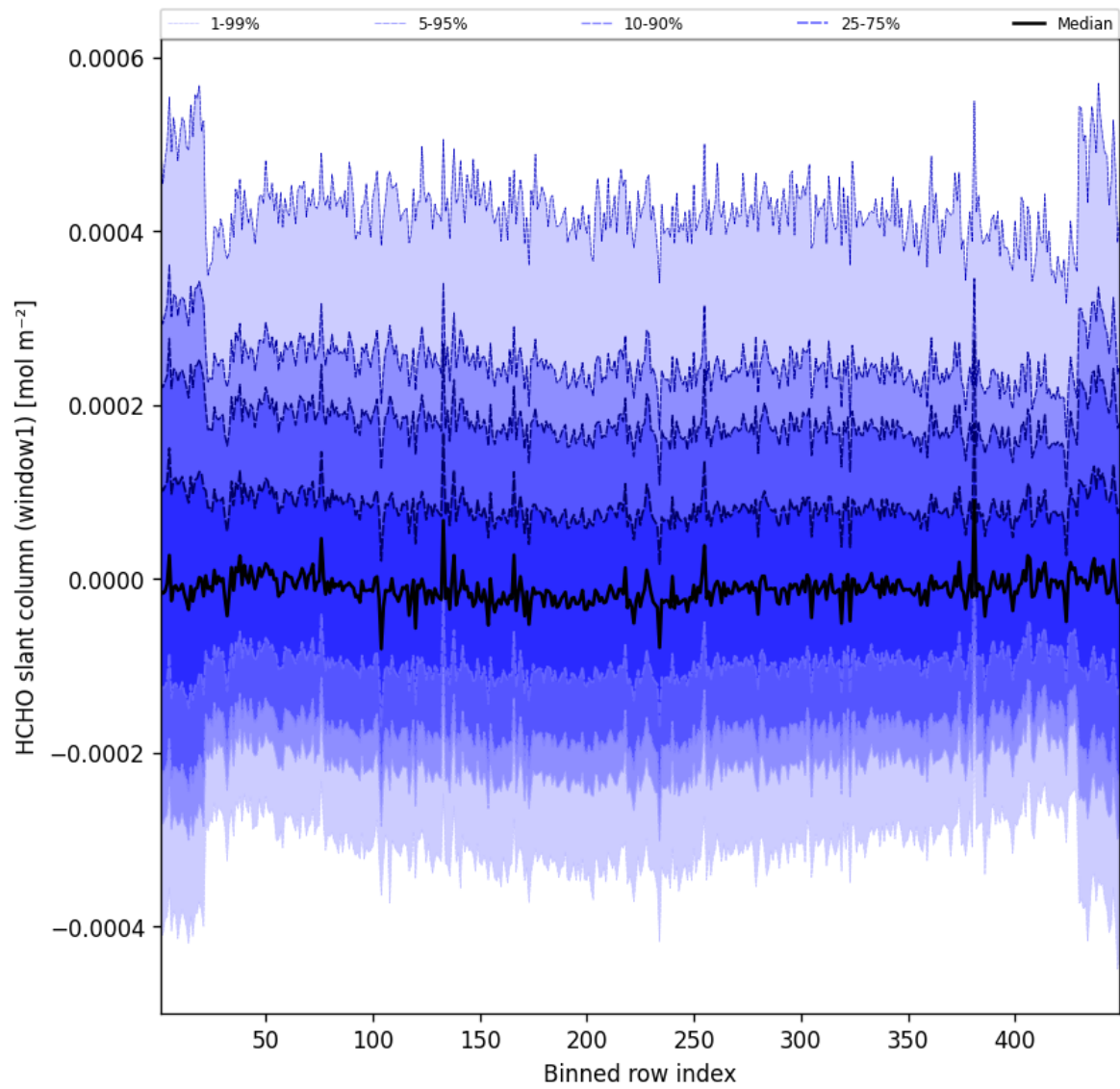
Figure 50: Along track statistics of “HCHO slant column (window1)” for 2024-12-18 to 2024-12-19
