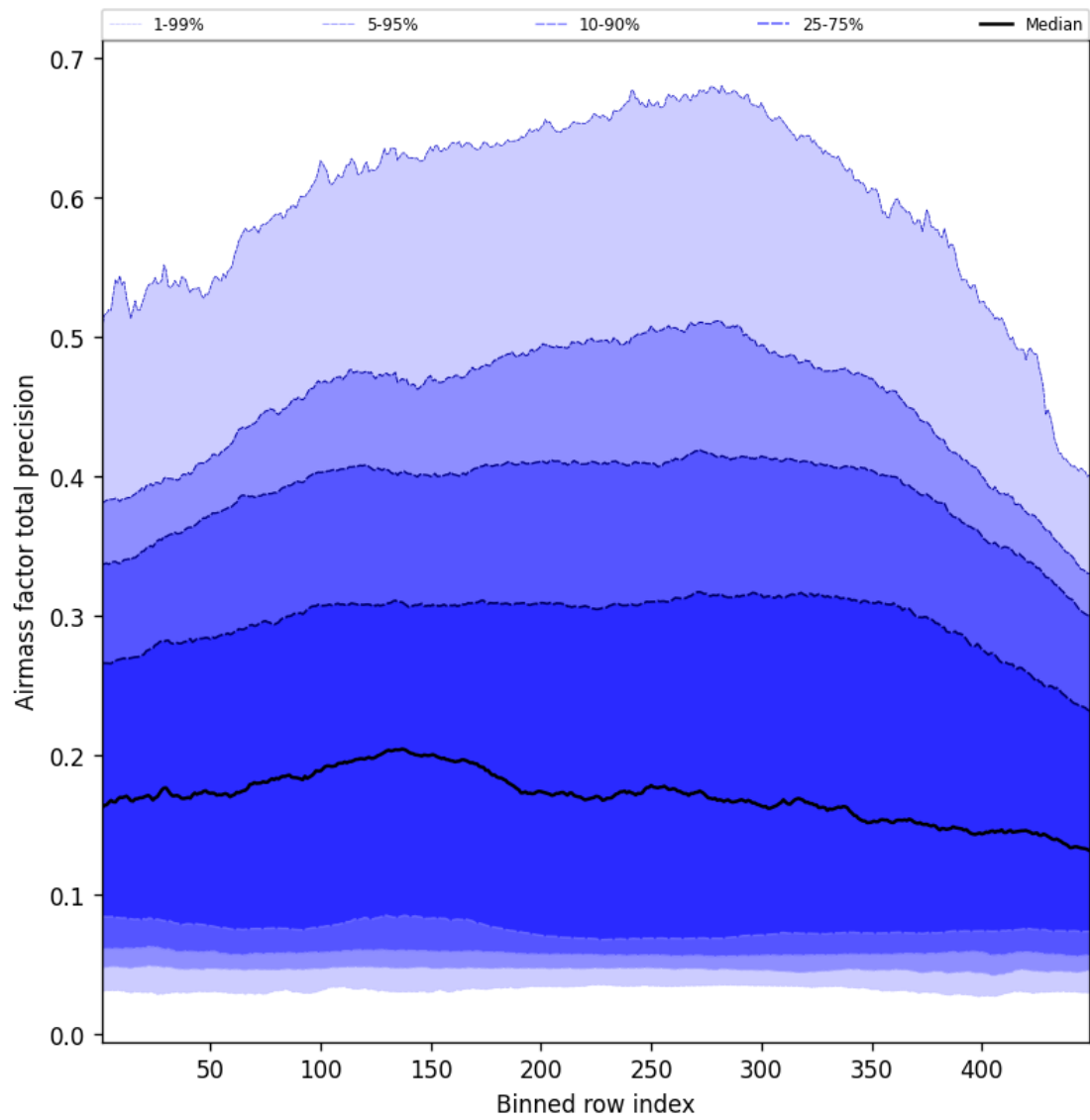
Figure 53: Along track statistics of “Airmass factor total precision” for 2024-12-18 to 2024-12-19
