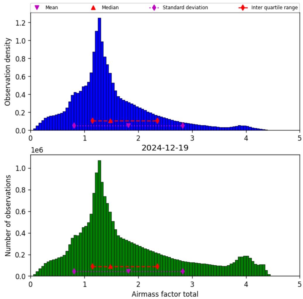
Figure 38: Histogram of “Airmass factor total” for 2024-12-19 to 2024-12-19
