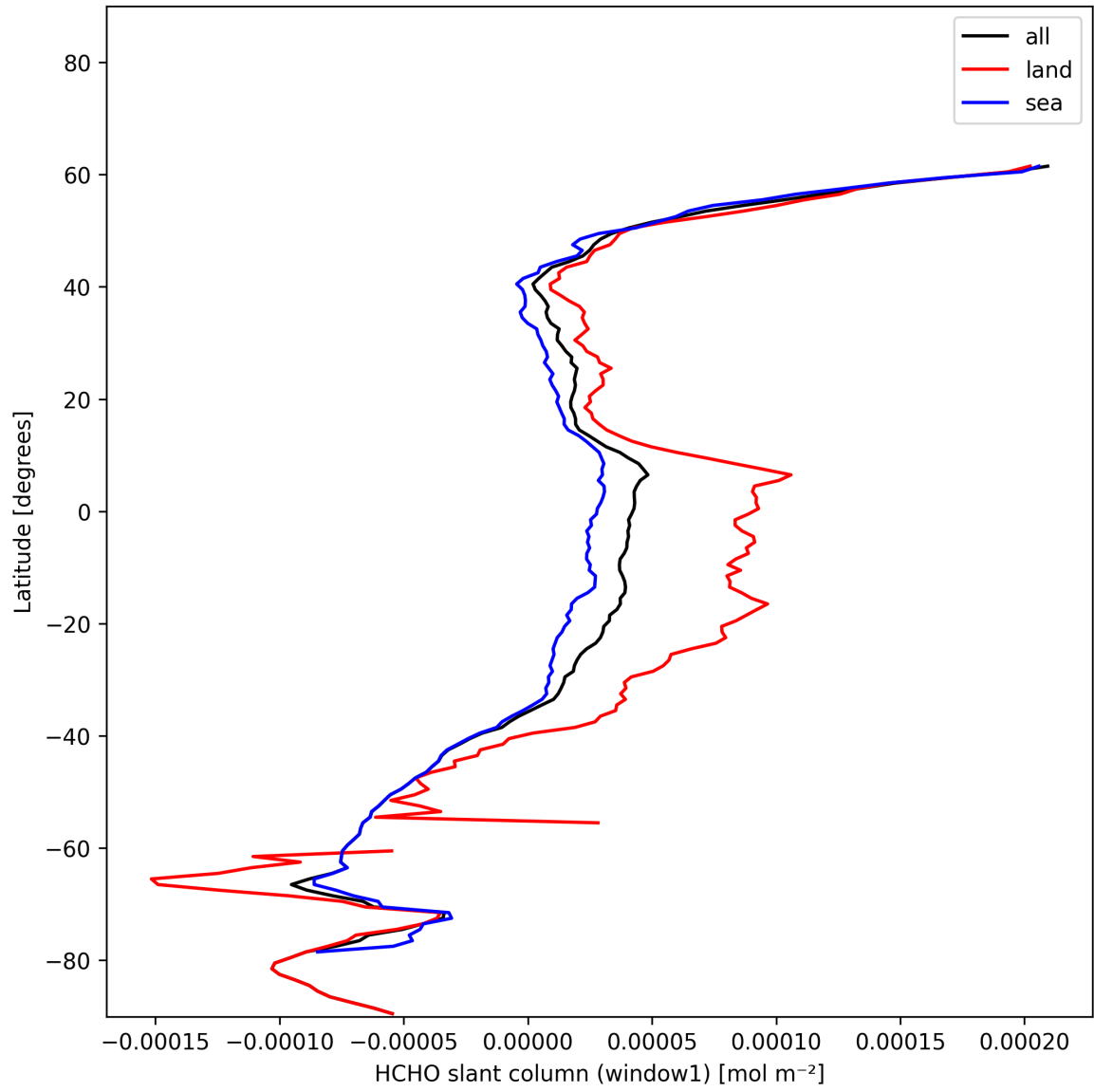
Figure 22: Zonal average of “HCHO slant column (window1)” for 2024-12-19 to 2024-12-19.
