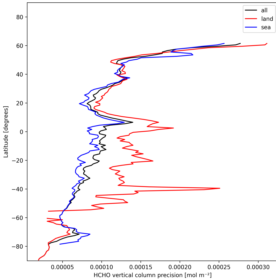
Figure 20: Zonal average of “HCHO vertical column precision” for 2024-12-19 to 2024-12-19.
