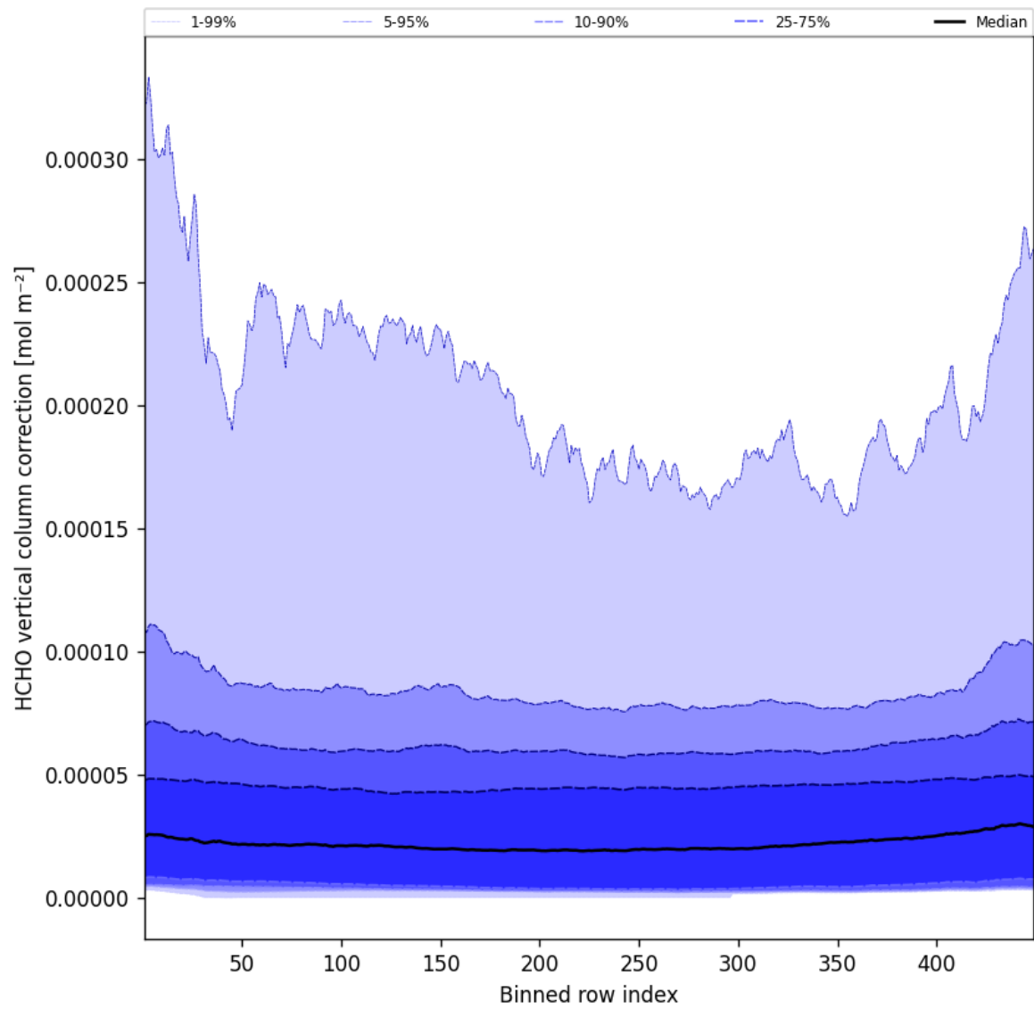
Figure 49: Along track statistics of “HCHO vertical column correction” for 2024-12-19 to 2024-12-19
