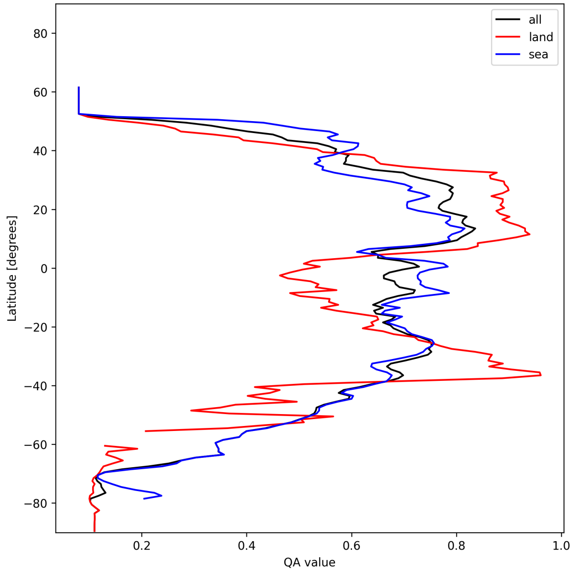
Figure 18: Zonal average of “QA value” for 2024-12-19 to 2024-12-19.
