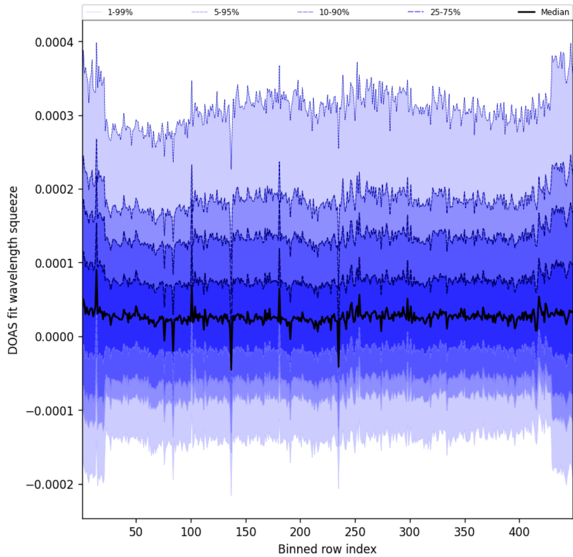
Figure 57: Along track statistics of “DOAS fit wavelength squeeze” for 2024-12-19 to 2024-12-19
