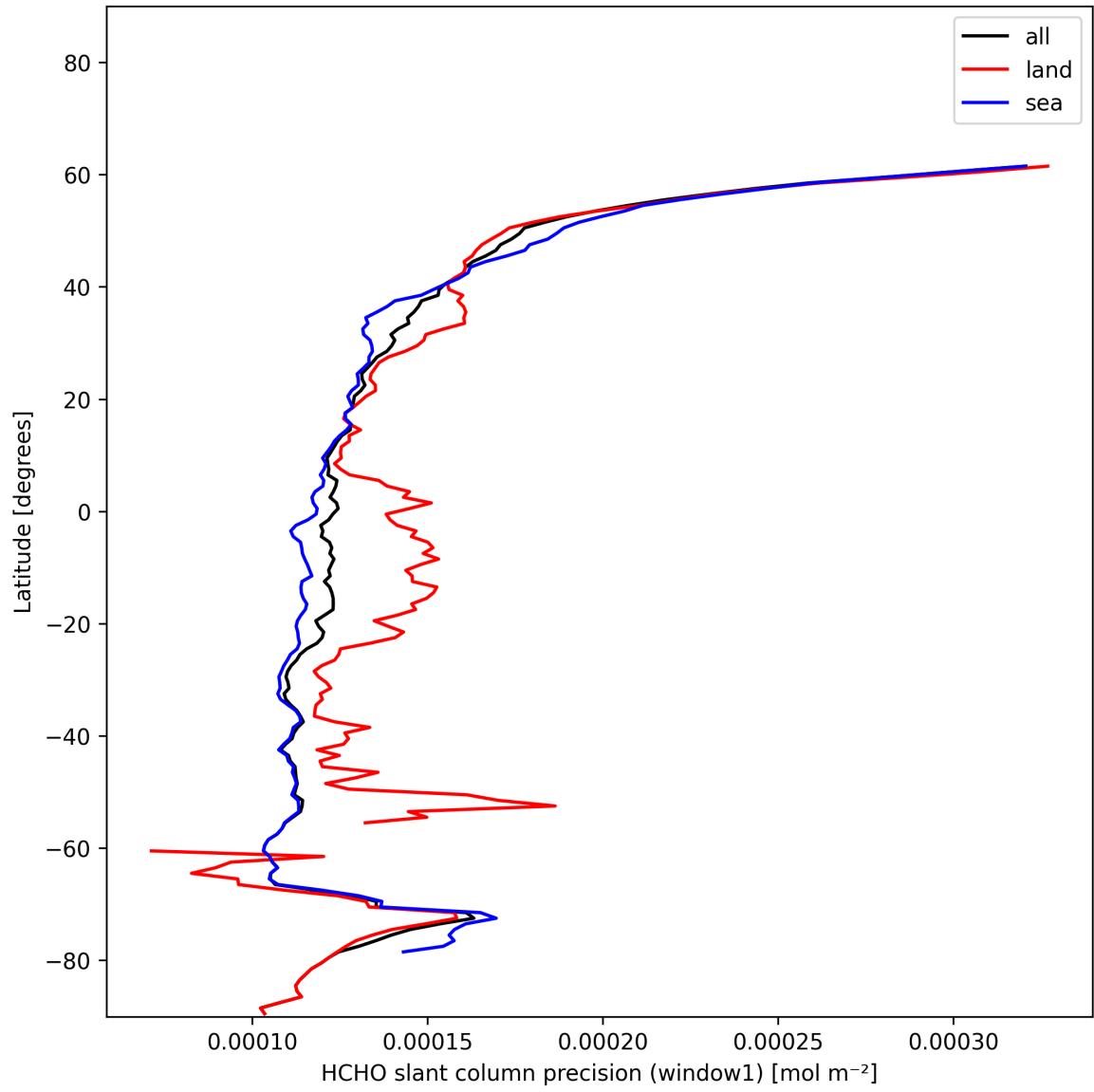
Figure 23: Zonal average of “HCHO slant column precision (window1)” for 2024-12-19 to 2024-12-19.
