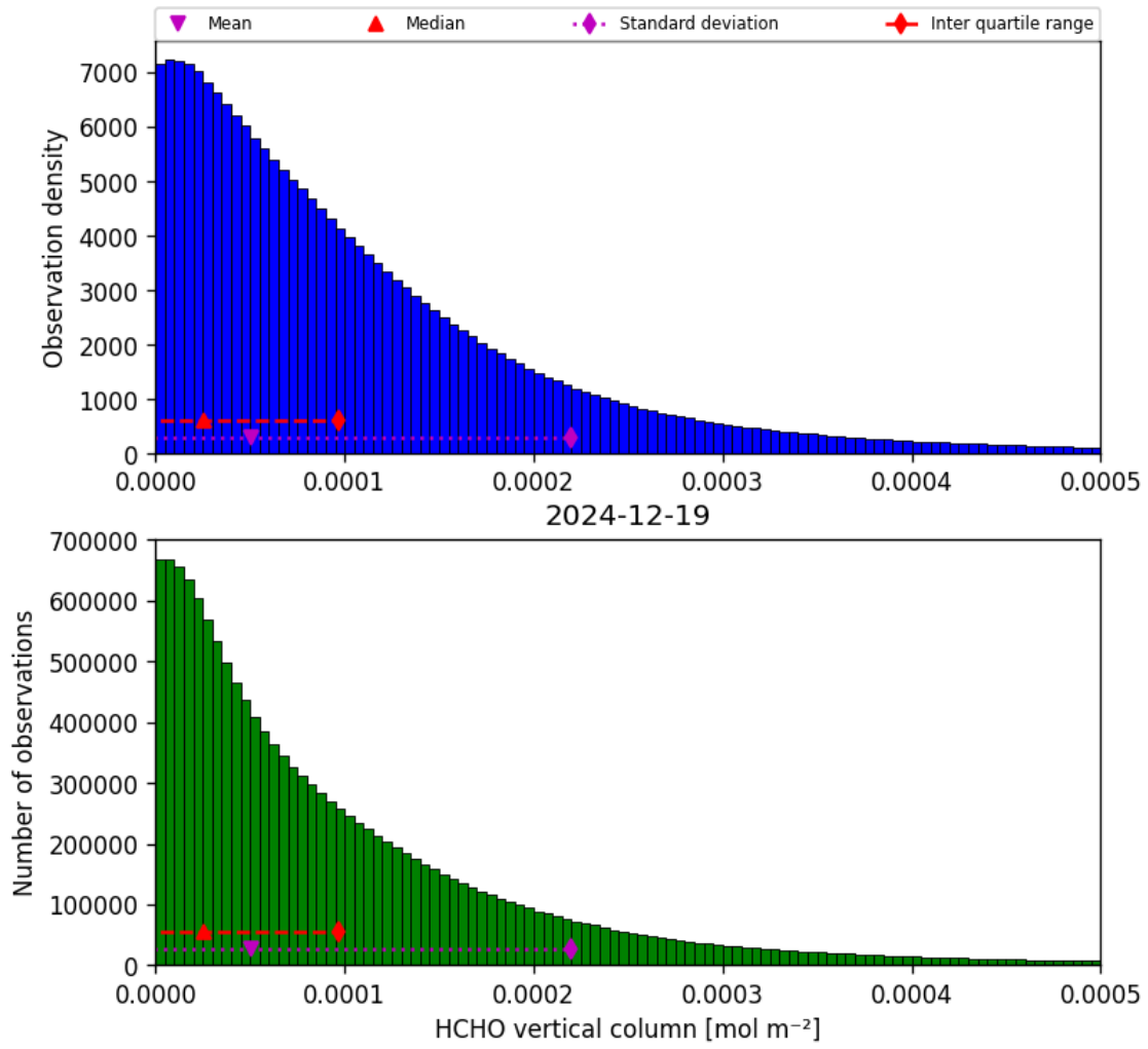
Figure 33: Histogram of “HCHO vertical column” for 2024-12-19 to 2024-12-19
