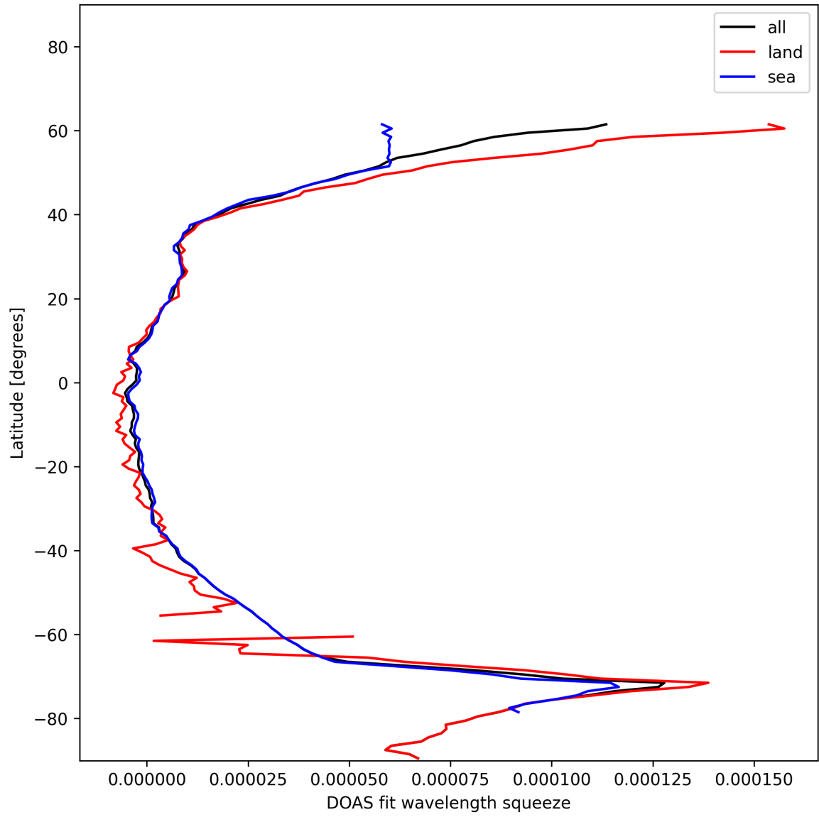
Figure 29: Zonal average of “DOAS fit wavelength squeeze” for 2024-12-19 to 2024-12-19.
