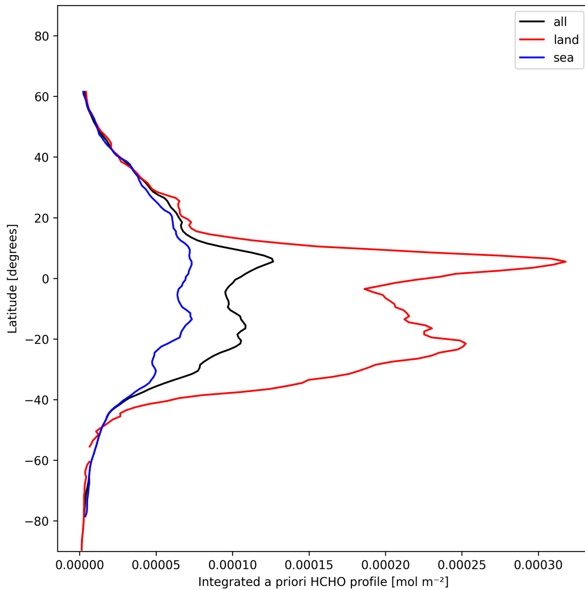
Figure 27: Zonal average of “Integrated a priori HCHO profile” for 2024-12-19 to 2024-12-19.
