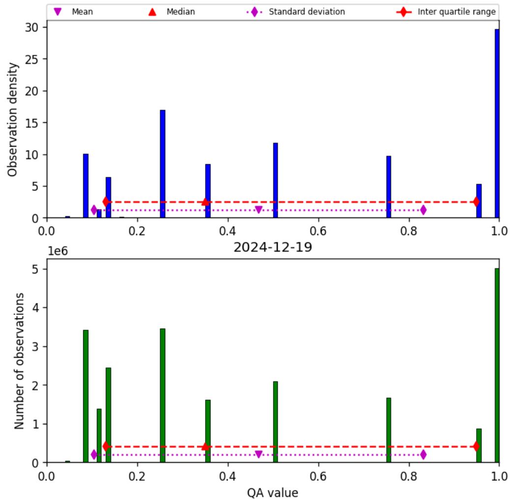
Figure 32: Histogram of “QA value” for 2024-12-19 to 2024-12-19
