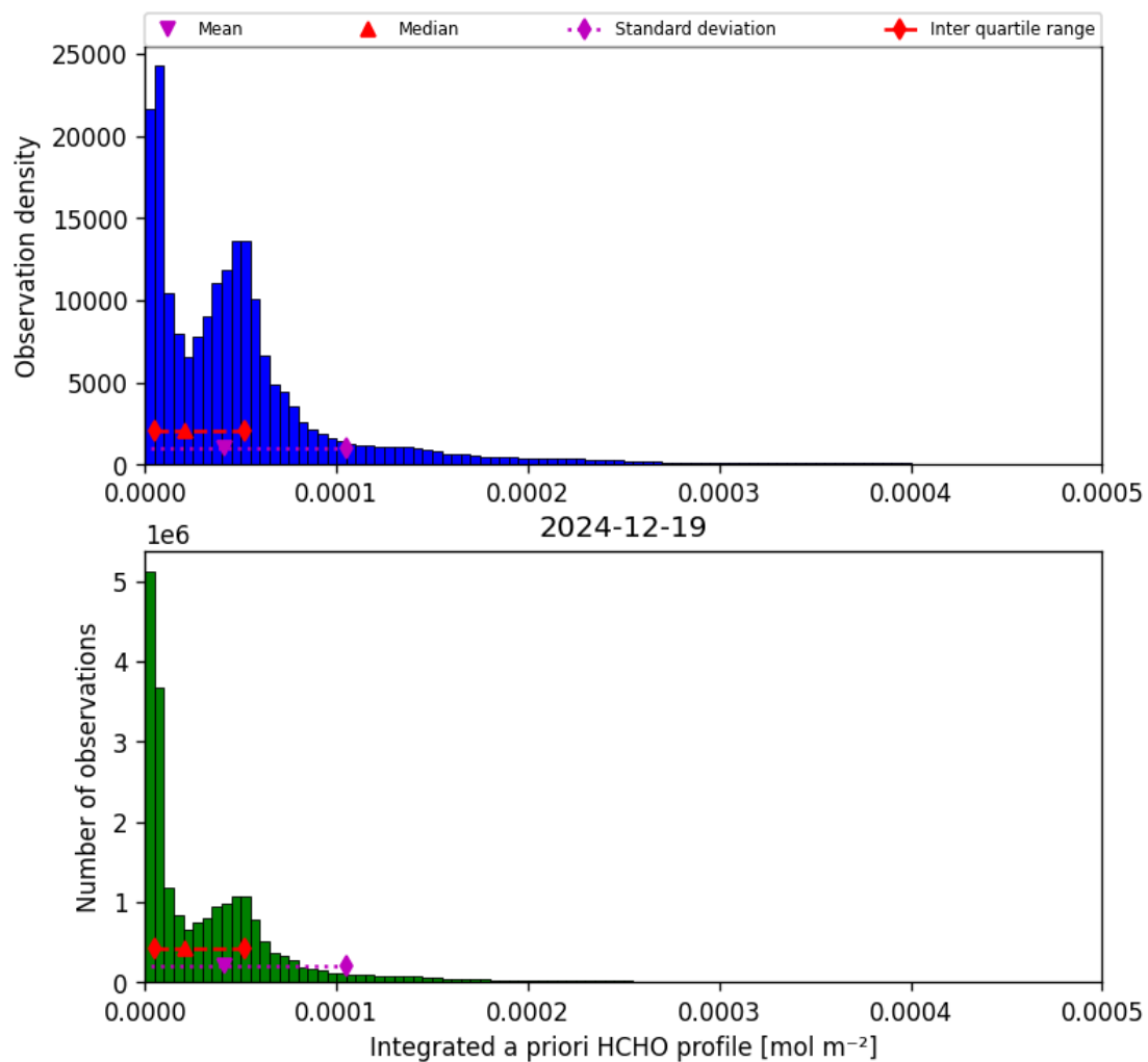
Figure 41: Histogram of “Integrated a priori HCHO profile” for 2024-12-19 to 2024-12-19
