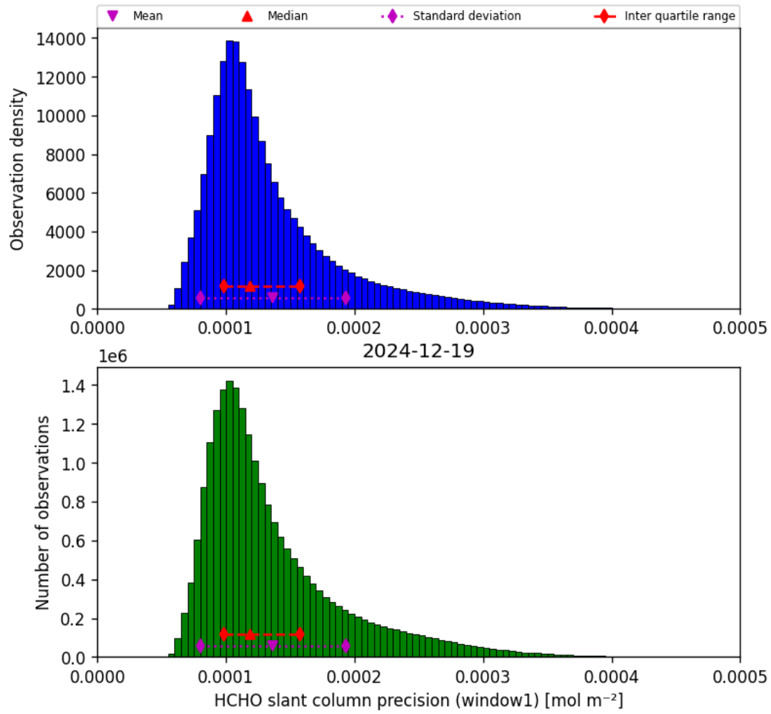
Figure 37: Histogram of “HCHO slant column precision (window1)” for 2024-12-19 to 2024-12-19
