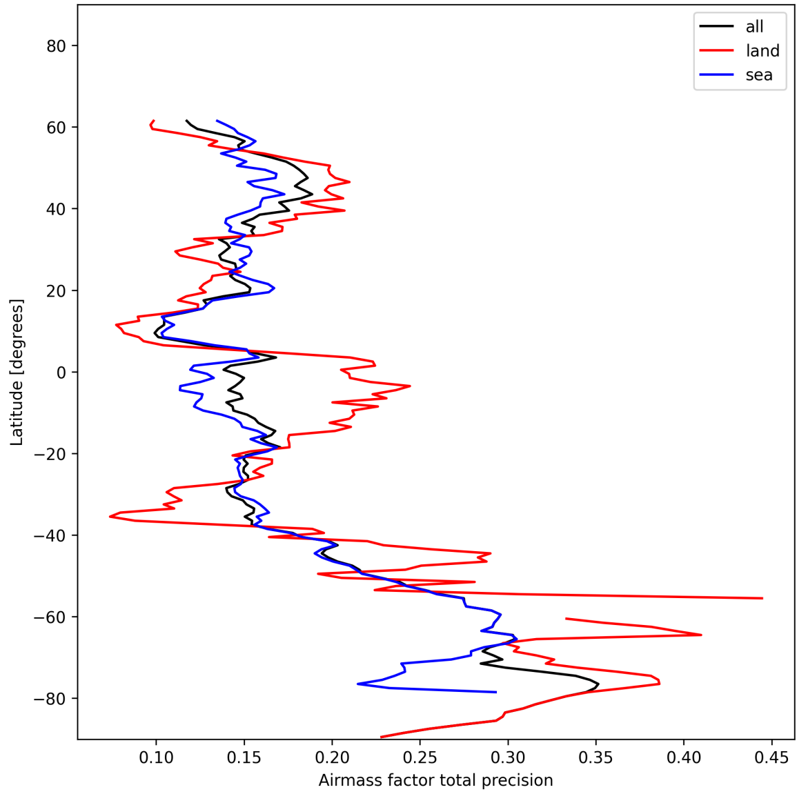
Figure 25: Zonal average of “Airmass factor total precision” for 2024-12-19 to 2024-12-19.
