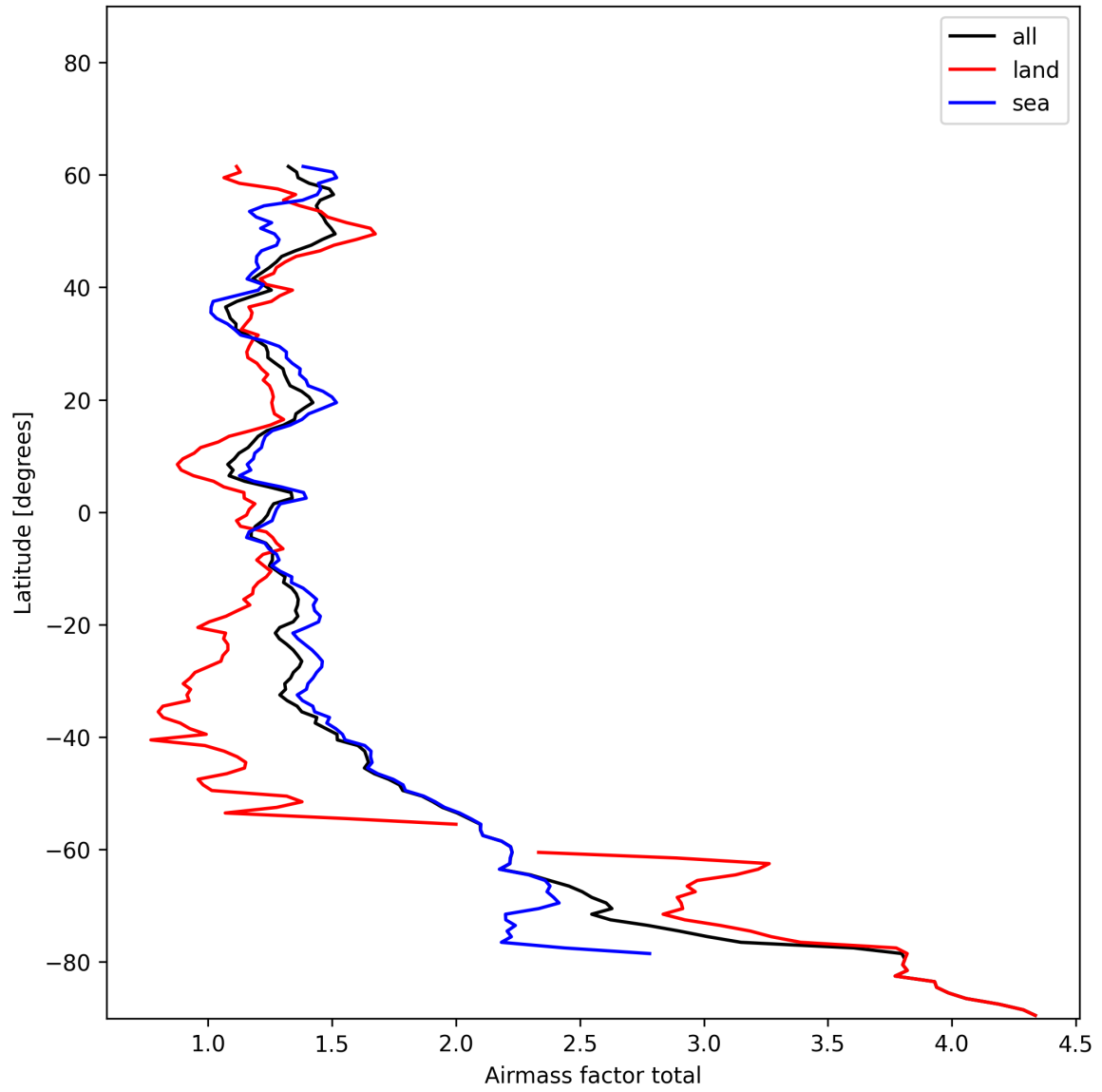
Figure 24: Zonal average of “Airmass factor total” for 2024-12-19 to 2024-12-19.
