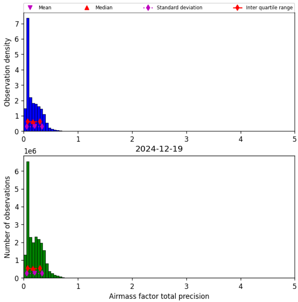
Figure 39: Histogram of “Airmass factor total precision” for 2024-12-19 to 2024-12-19
