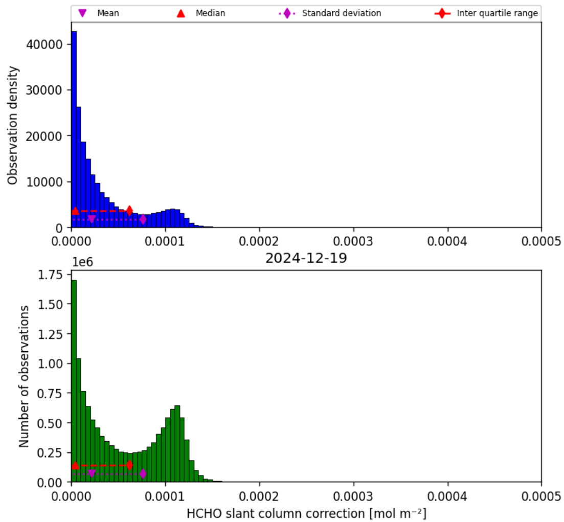
Figure 45: Histogram of “HCHO slant column correction” for 2024-12-19 to 2024-12-19
