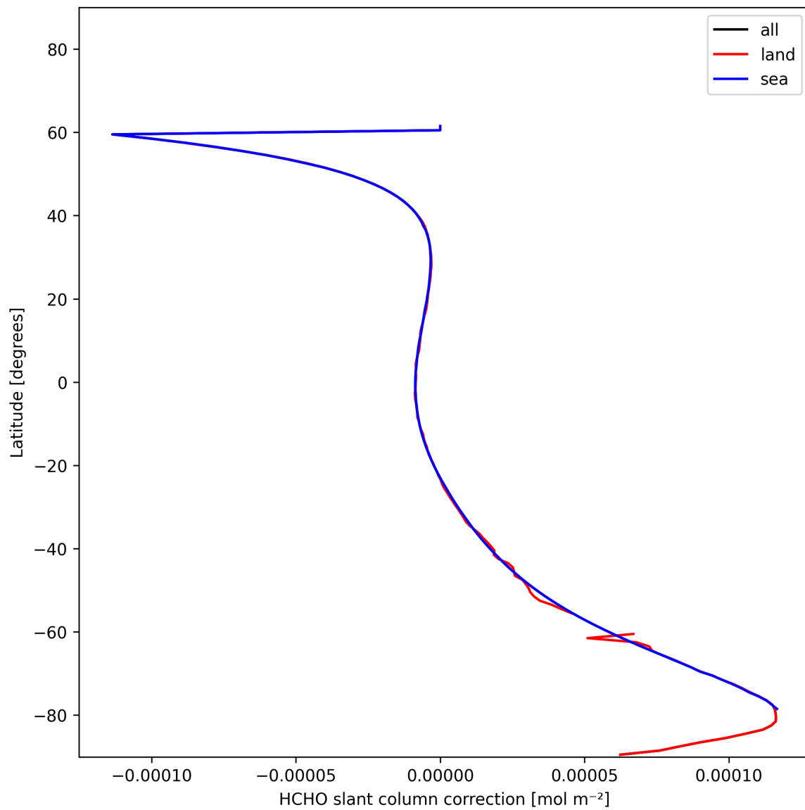
Figure 31: Zonal average of “HCHO slant column correction” for 2024-12-19 to 2024-12-19.
