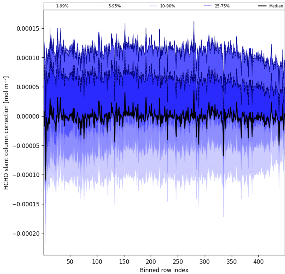
Figure 59: Along track statistics of “HCHO slant column correction” for 2024-12-19 to 2024-12-19
