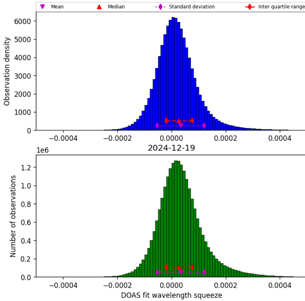
Figure 43: Histogram of “DOAS fit wavelength squeeze” for 2024-12-19 to 2024-12-19
