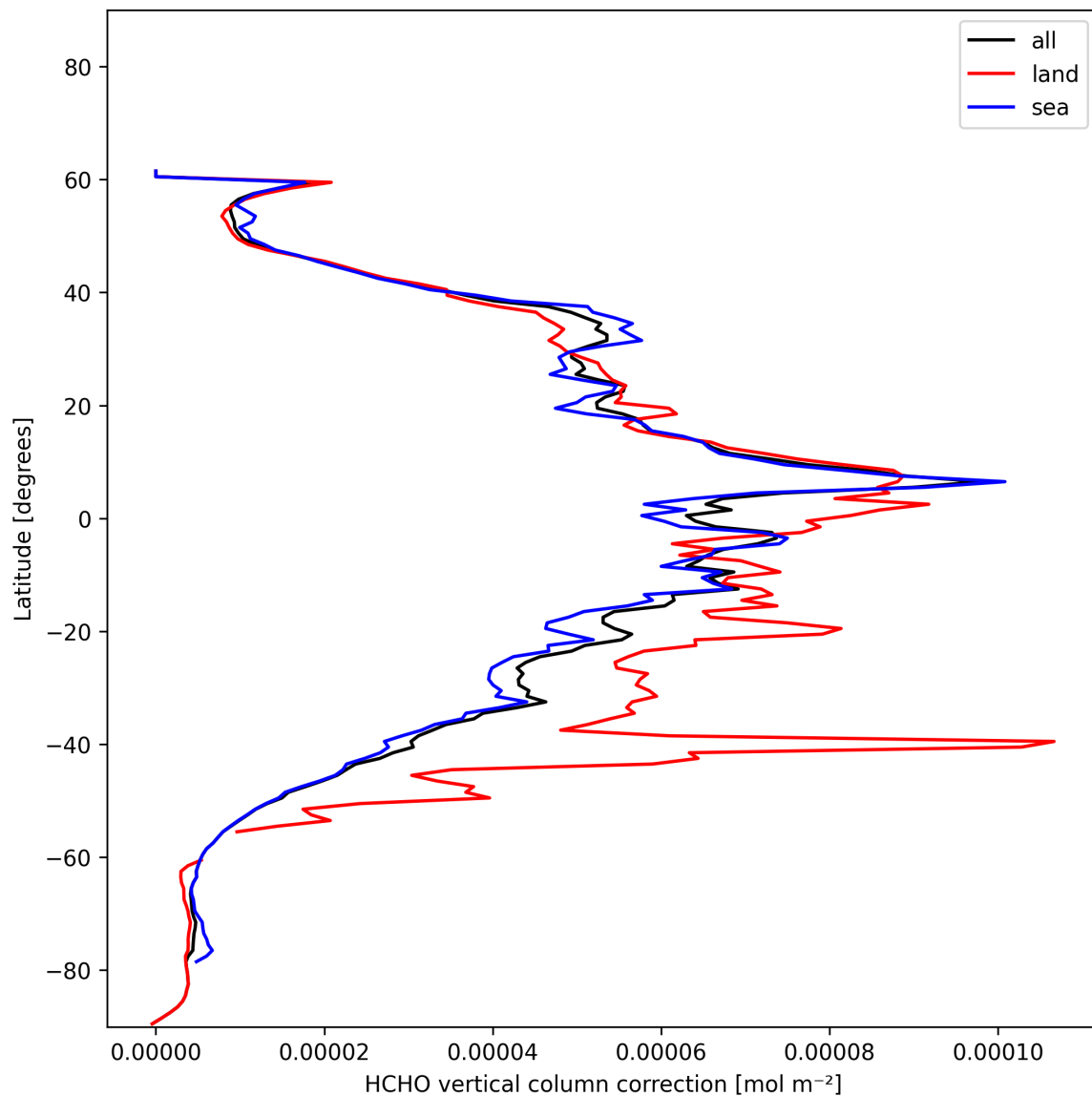
Figure 21: Zonal average of “HCHO vertical column correction” for 2024-12-19 to 2024-12-19.
