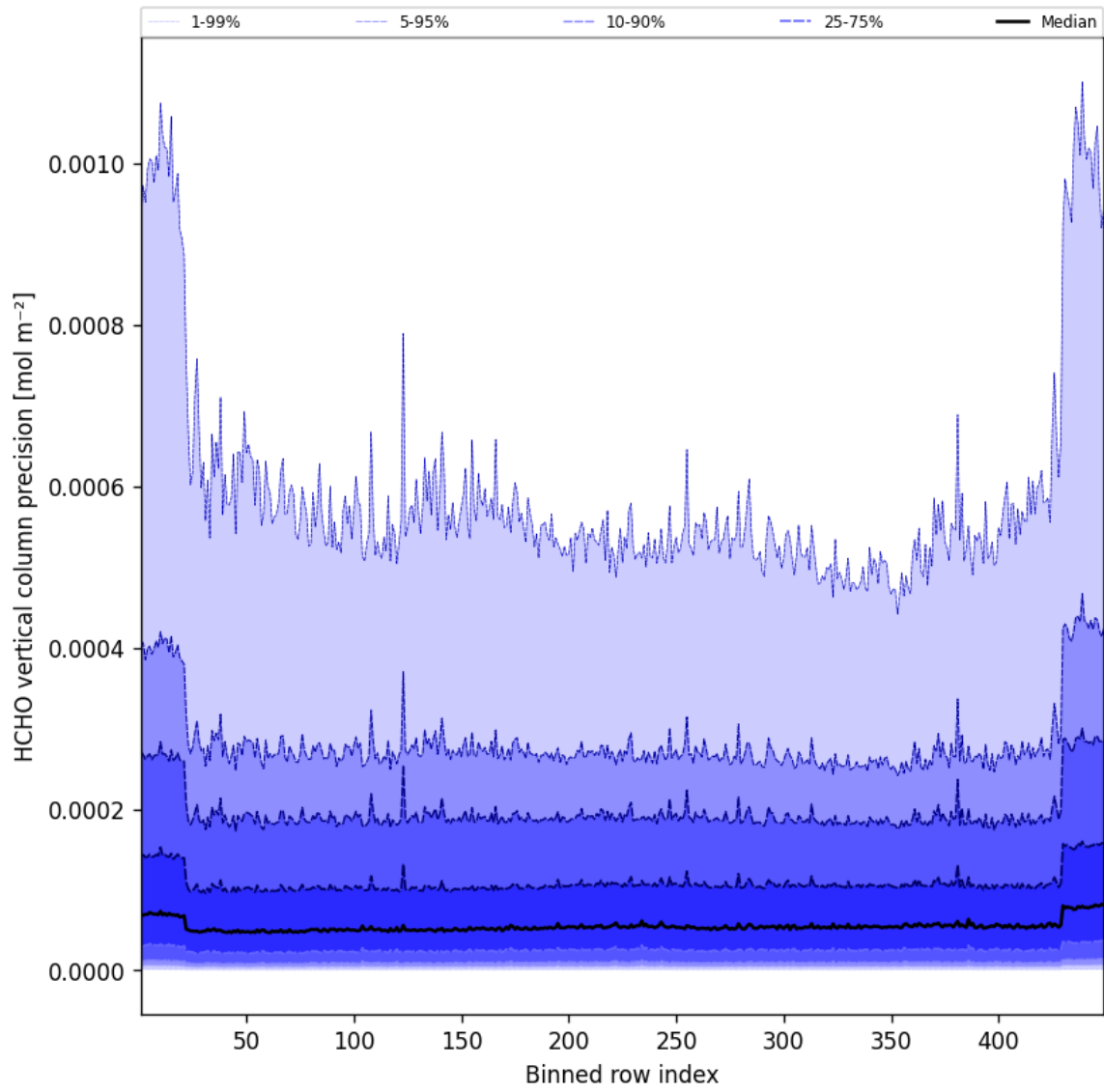
Figure 48: Along track statistics of “HCHO vertical column precision” for 2024-12-19 to 2024-12-19
