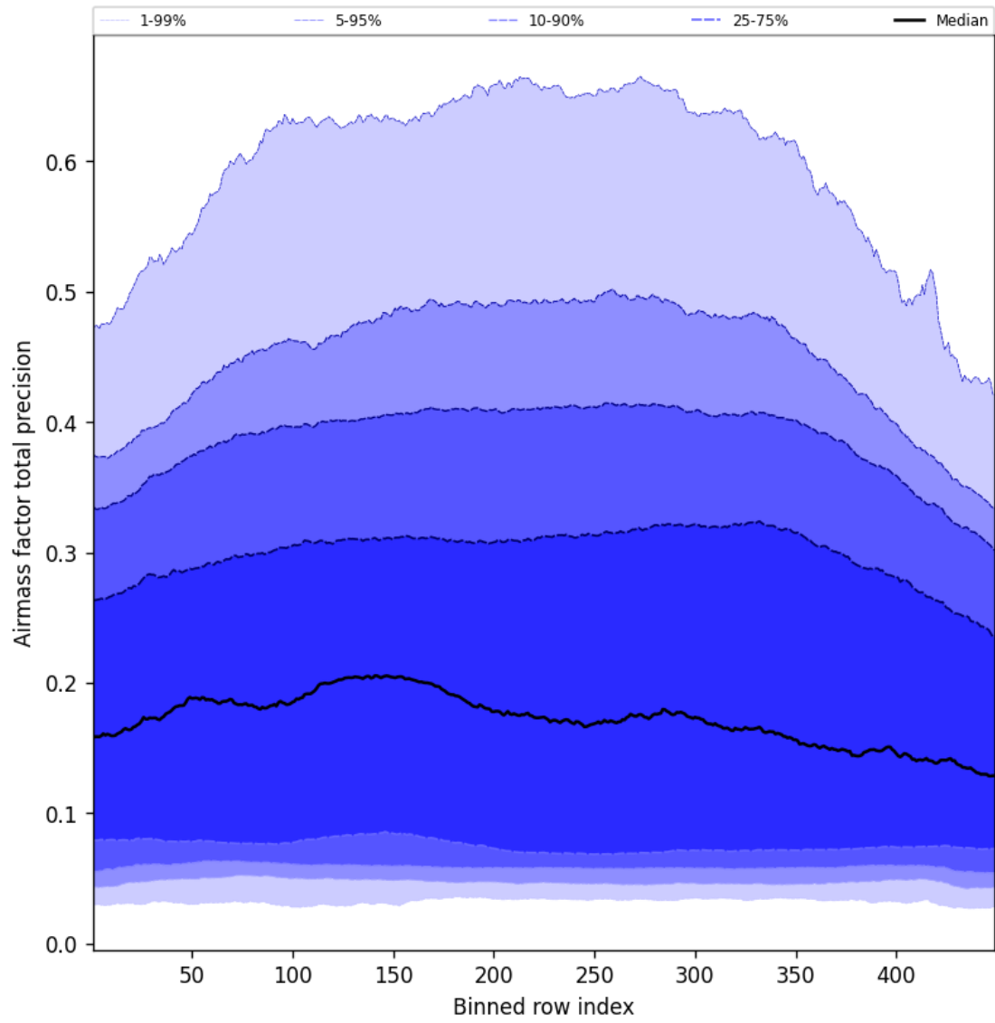
Figure 53: Along track statistics of “Airmass factor total precision” for 2024-12-19 to 2024-12-19
