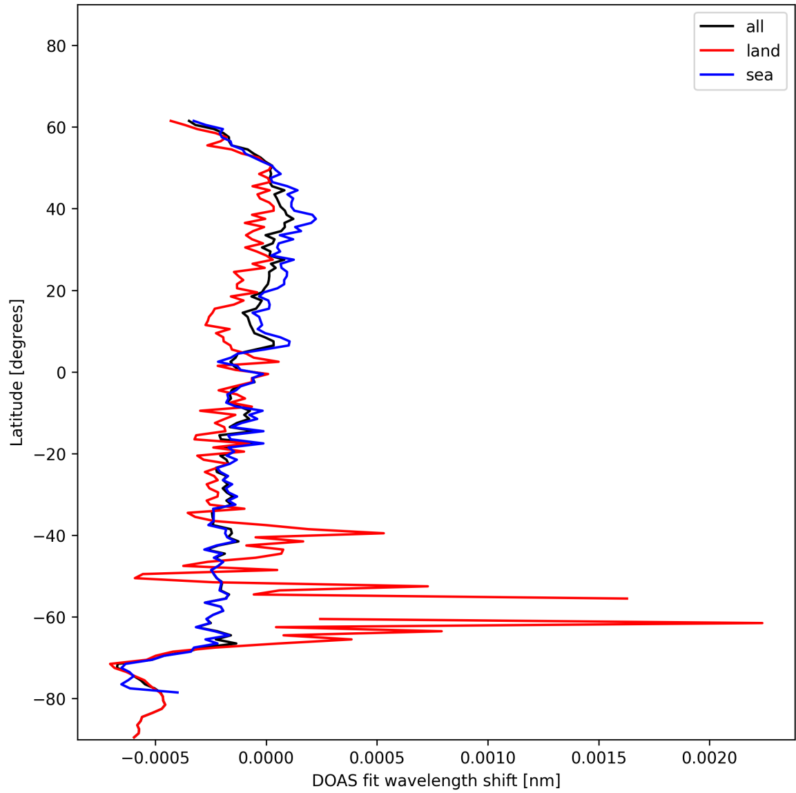
Figure 28: Zonal average of “DOAS fit wavelength shift” for 2024-12-19 to 2024-12-19.
