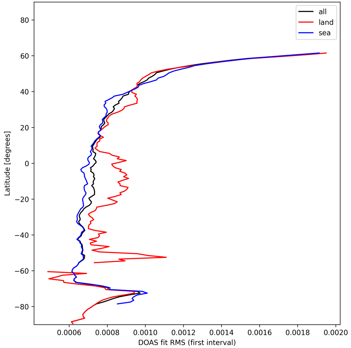
Figure 30: Zonal average of “DOAS fit RMS (first interval)” for 2024-12-19 to 2024-12-19.
