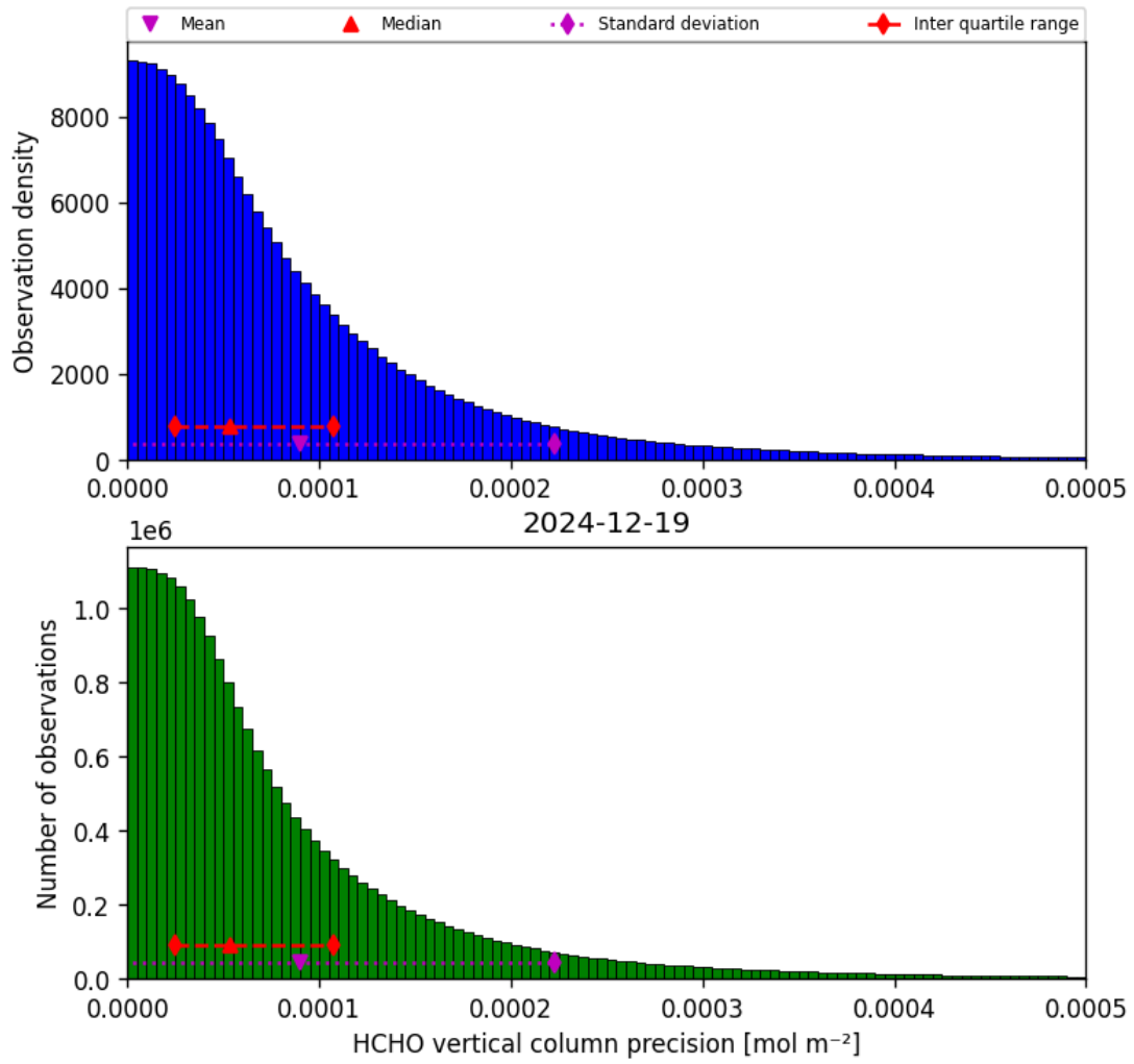
Figure 34: Histogram of “HCHO vertical column precision” for 2024-12-19 to 2024-12-19
