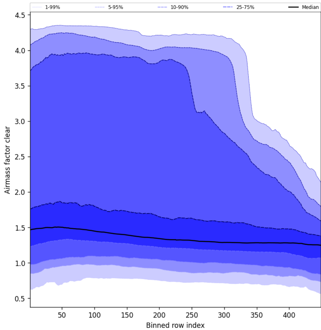
Figure 54: Along track statistics of “Air mass factor clear” for 2024-12-19 to 2024-12-19
