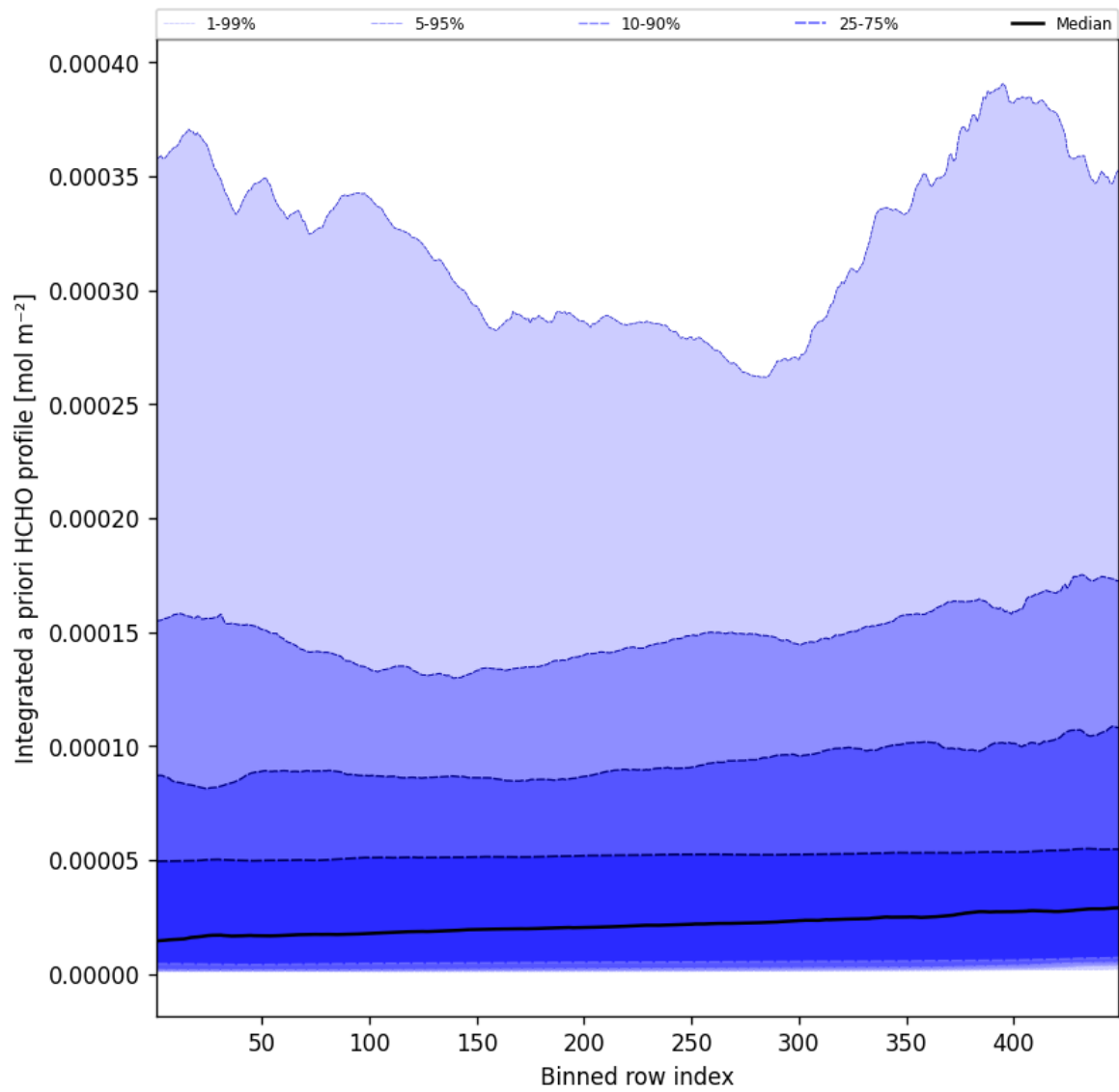
Figure 55: Along track statistics of “Integrated a priori HCHO profile” for 2024-12-19 to 2024-12-19
