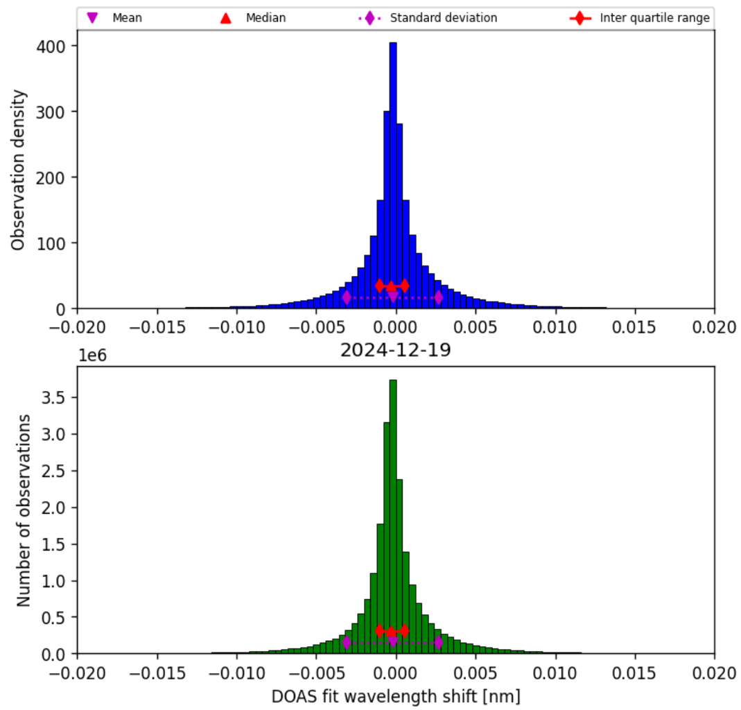
Figure 42: Histogram of “DOAS fit wavelength shift” for 2024-12-19 to 2024-12-19
