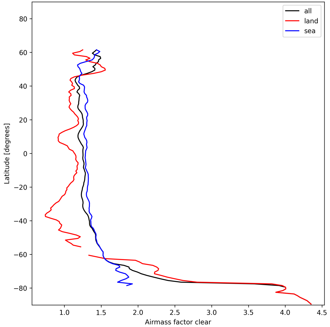
Figure 26: Zonal average of “Airmass factor clear” for 2024-12-19 to 2024-12-19.
