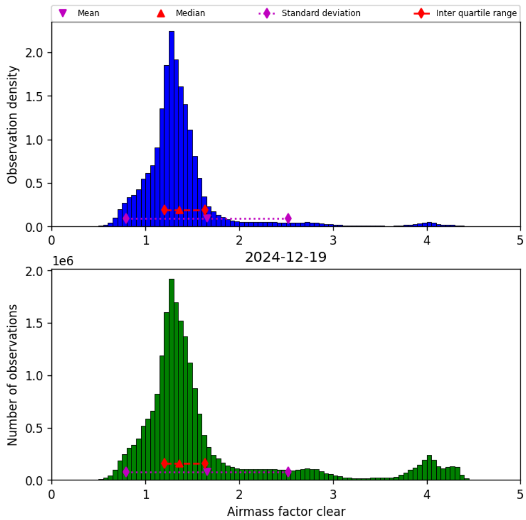
Figure 40: Histogram of “Airmass factor clear” for 2024-12-19 to 2024-12-19
