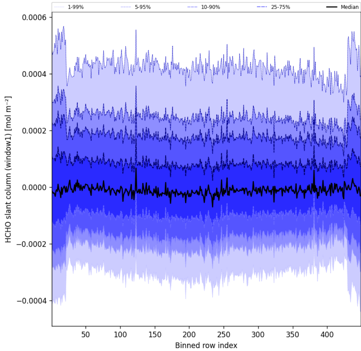
Figure 50: Along track statistics of “HCHO slant column (window1)” for 2024-12-19 to 2024-12-19
