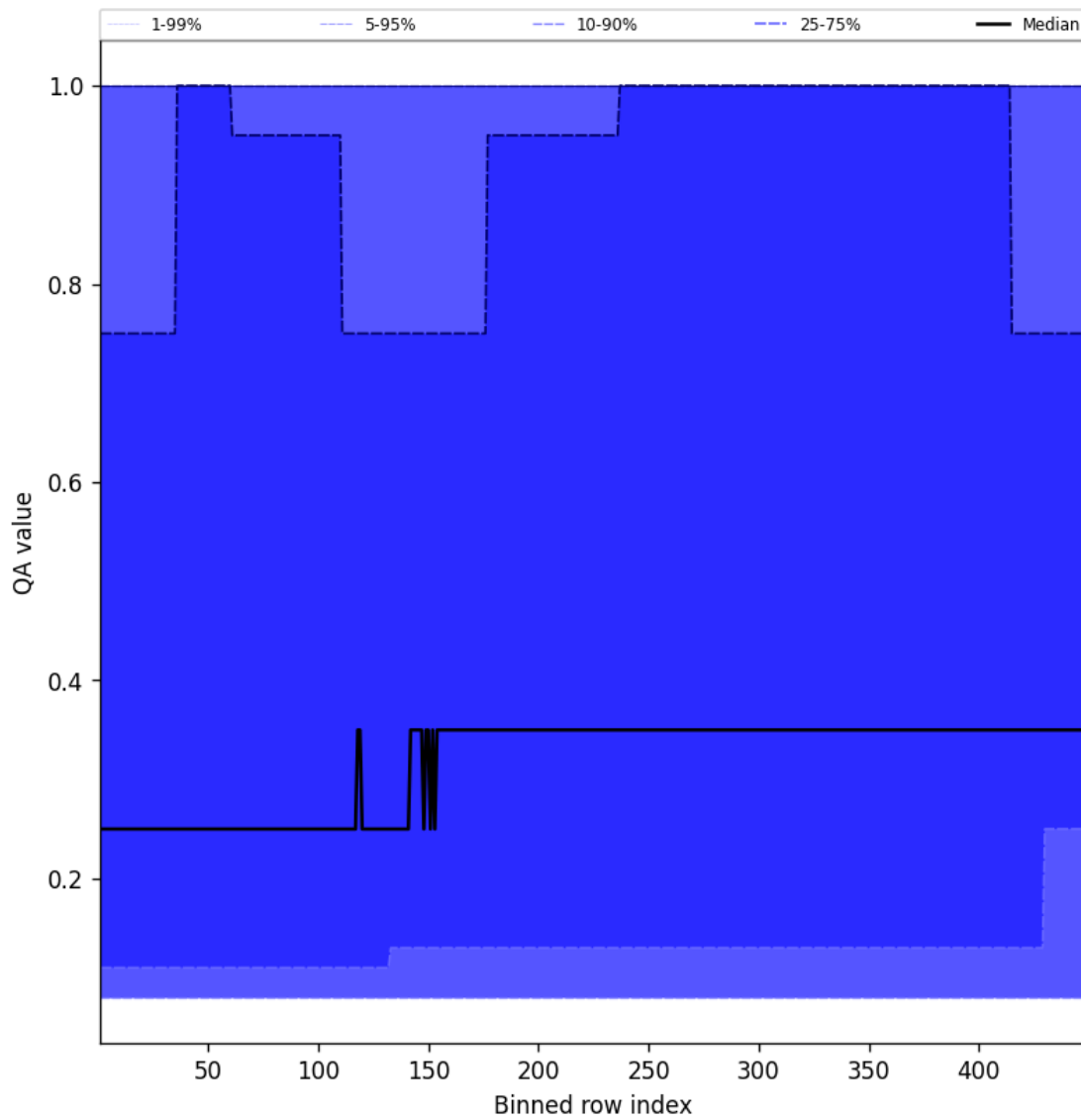
Figure 46: Along track statistics of “QA value” for 2024-12-19 to 2024-12-19
