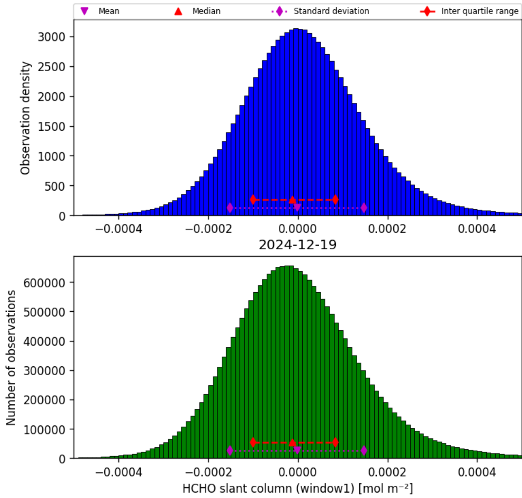
Figure 36: Histogram of “HCHO slant column (window1)” for 2024-12-19 to 2024-12-19
