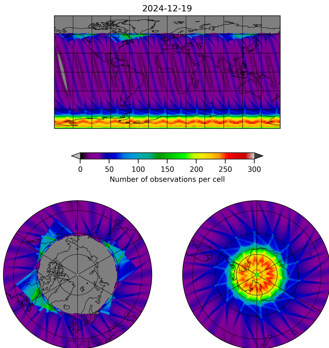
Figure 17: Map of the number of observations for 2024-12-19 to 2024-12-19
