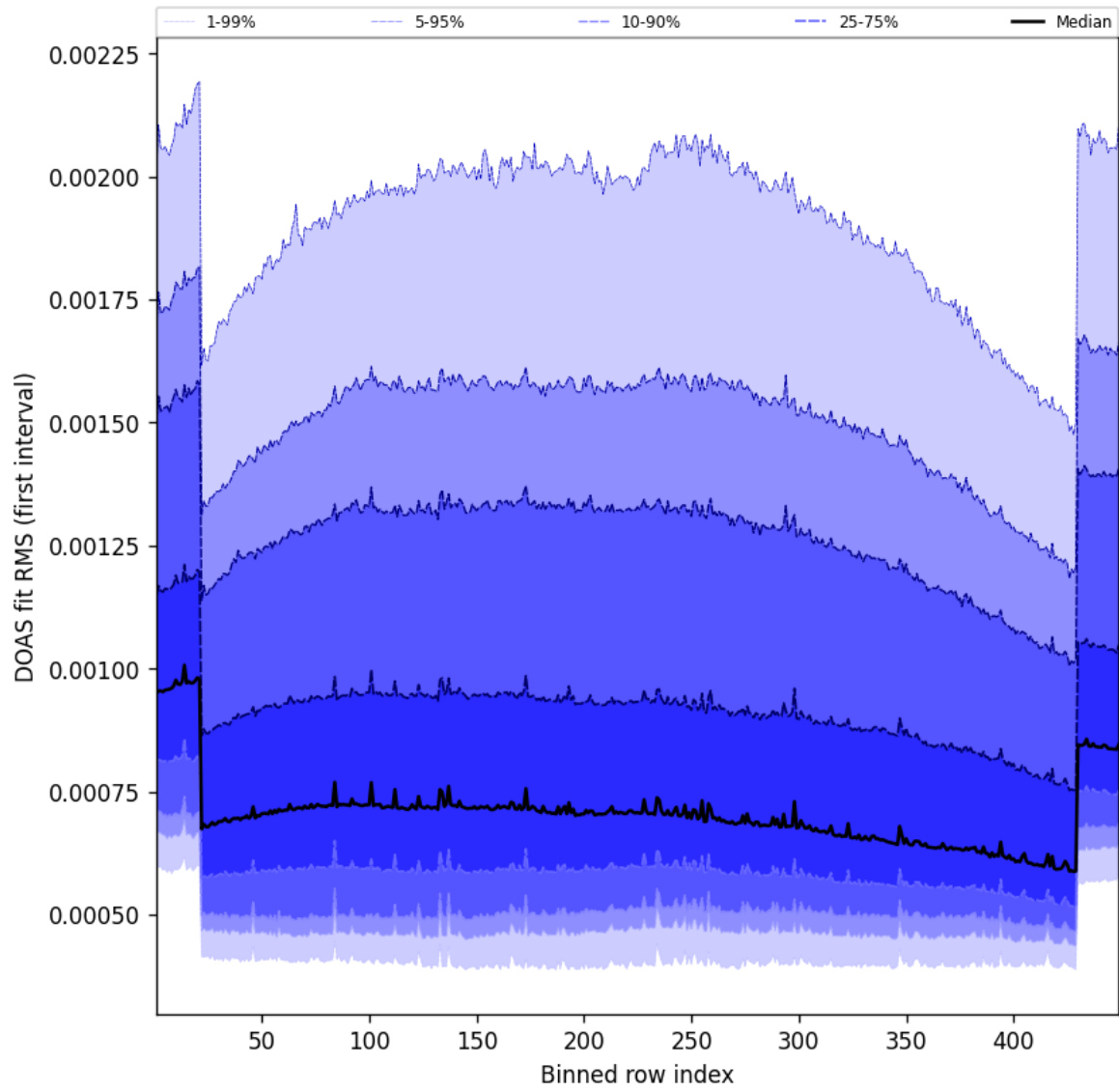
Figure 58: Along track statistics of “DOAS fit RMS (first interval)” for 2024-12-19 to 2024-12-19
