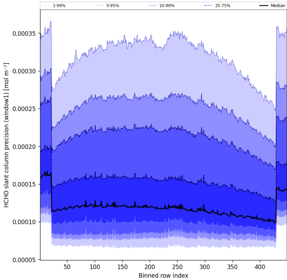
Figure 51: Along track statistics of “HCHO slant column precision (window1)” for 2024-12-19 to 2024-12-19
