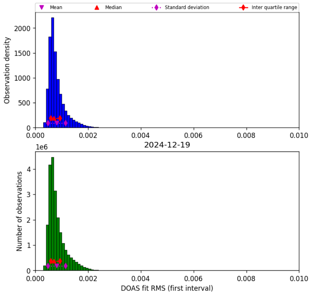
Figure 44: Histogram of “DOAS fit RMS (first interval)” for 2024-12-19 to 2024-12-19
