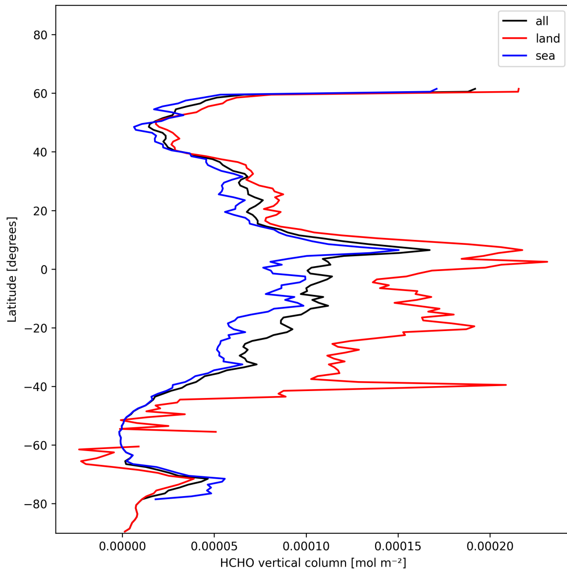
Figure 19: Zonal average of “HCHO vertical column” for 2024-12-19 to 2024-12-19.
