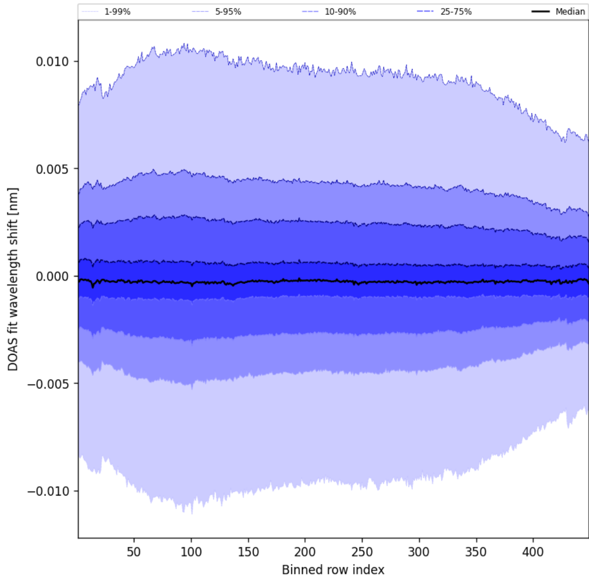
Figure 56: Along track statistics of “DOAS fit wavelength shift” for 2024-12-19 to 2024-12-19
