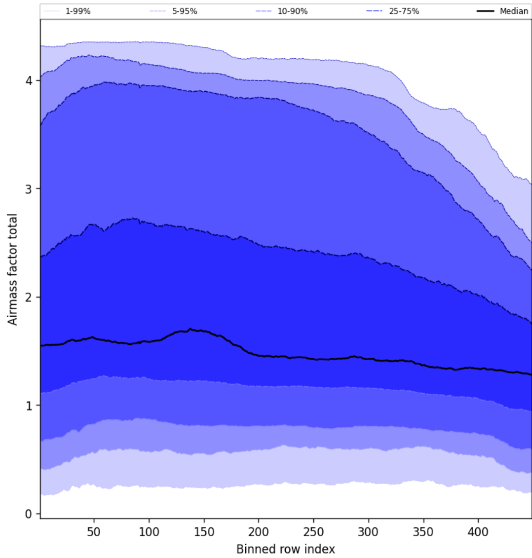
Figure 52: Along track statistics of “Airmass factor total” for 2024-12-19 to 2024-12-19
