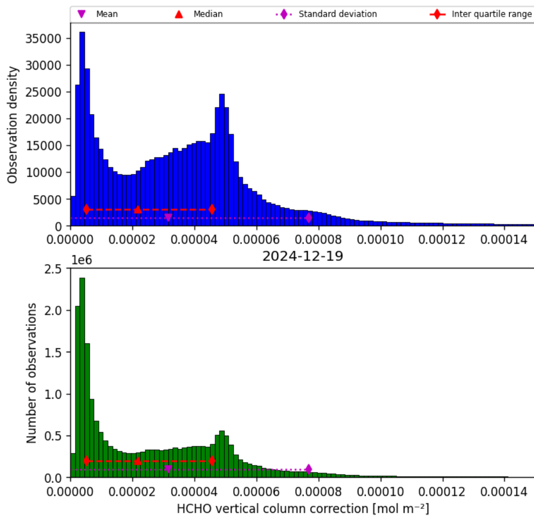
Figure 35: Histogram of “HCHO vertical column correction” for 2024-12-19 to 2024-12-19
