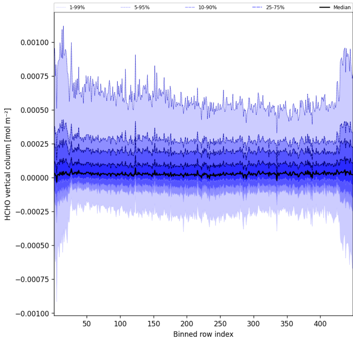
Figure 47: Along track statistics of “HCHO vertical column” for 2024-12-19 to 2024-12-19
