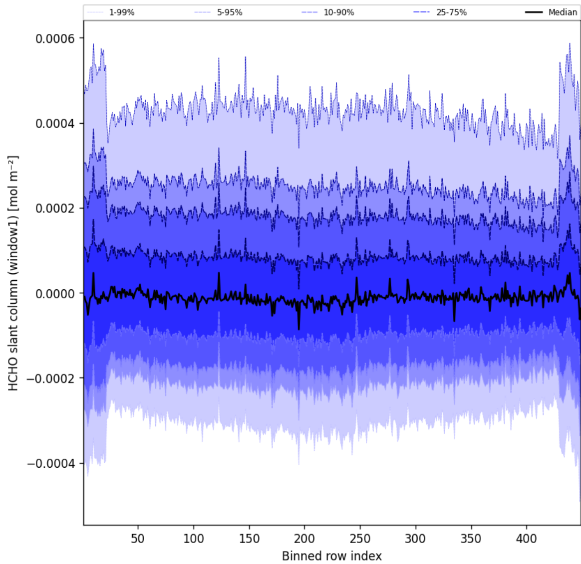
Figure 50: Along track statistics of “HCHO slant column (window1)” for 2024-12-20 to 2024-12-20
