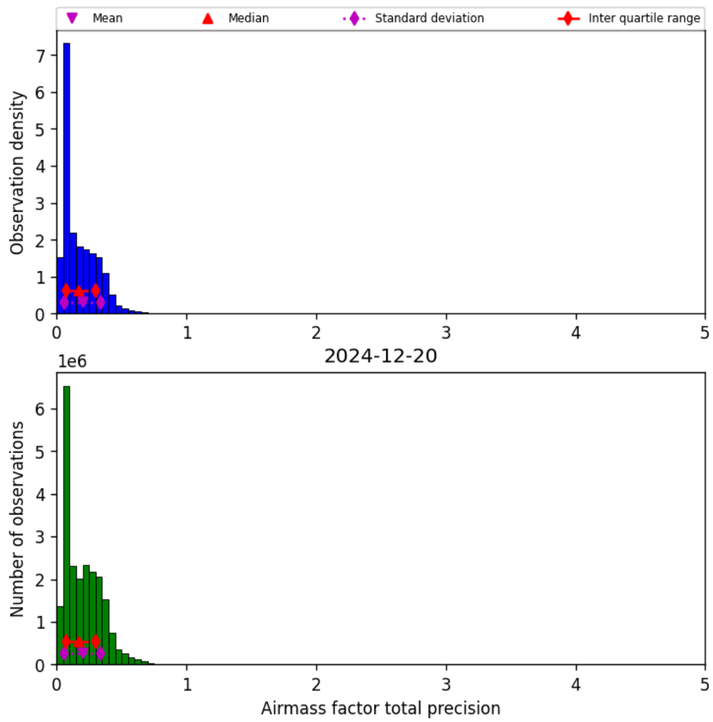
Figure 39: Histogram of “Airmass factor total precision” for 2024-12-20 to 2024-12-20
