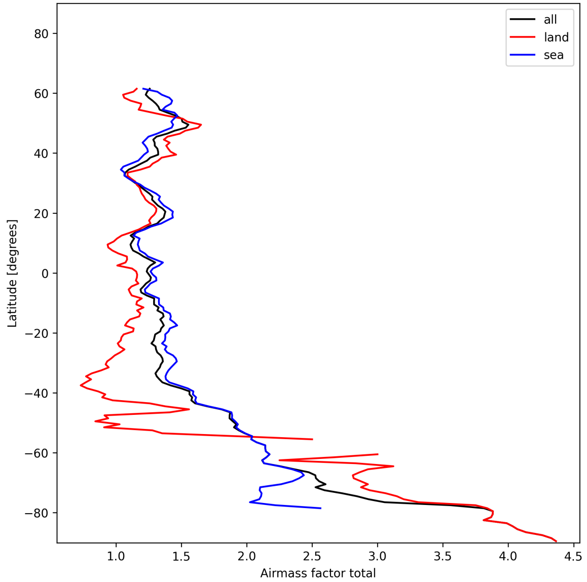
Figure 24: Zonal average of “Airmass factor total” for 2024-12-20 to 2024-12-20.
