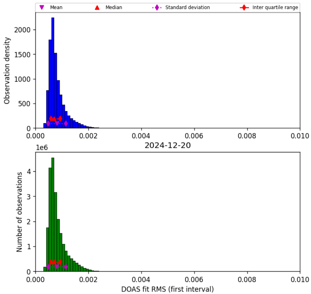
Figure 44: Histogram of “DOAS fit RMS (first interval)” for 2024-12-20 to 2024-12-20
