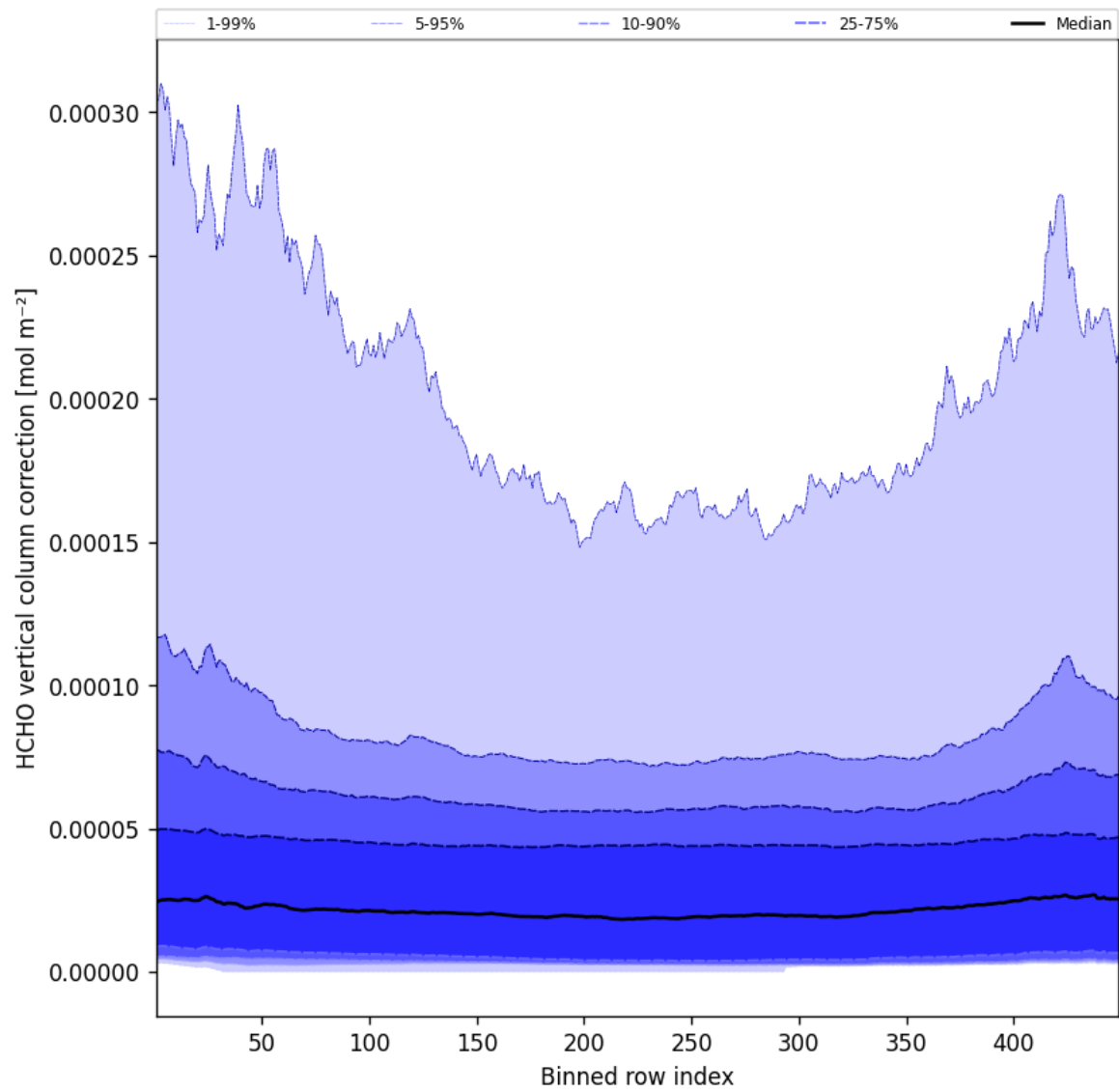
Figure 49: Along track statistics of “HCHO vertical column correction” for 2024-12-20 to 2024-12-20
