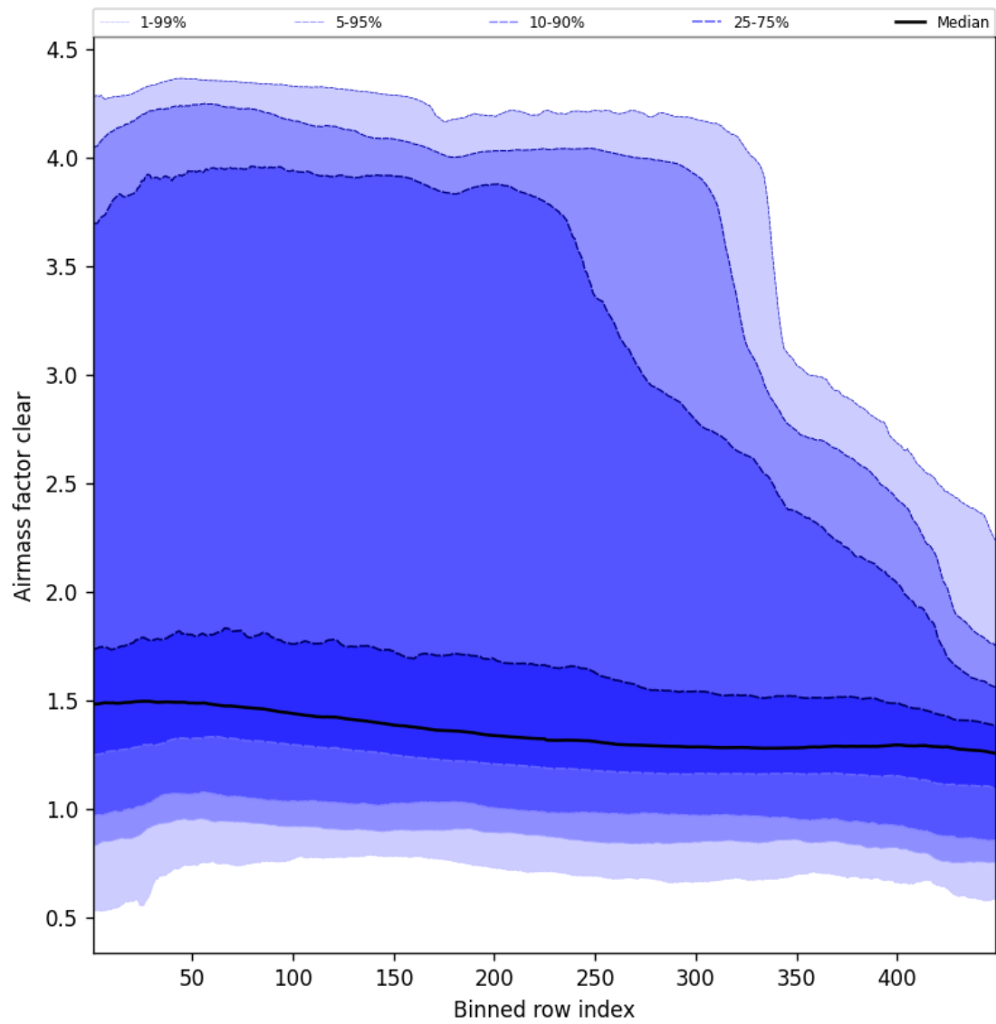
Figure 54: Along track statistics of “Airmass factor clear” for 2024-12-20 to 2024-12-20
