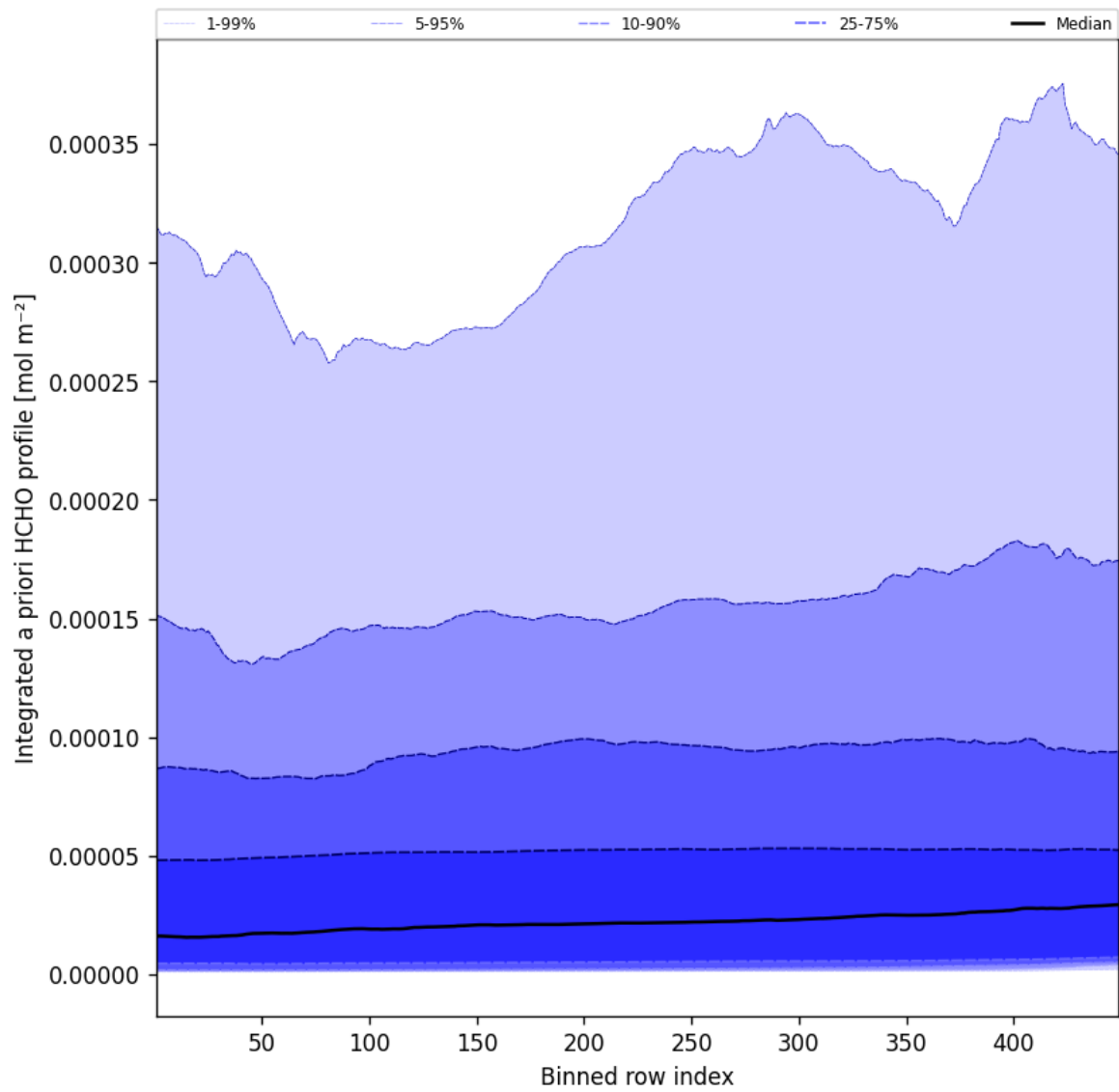
Figure 55: Along track statistics of “Integrated a priori HCHO profile” for 2024-12-20 to 2024-12-20
