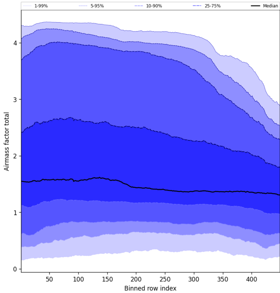
Figure 52: Along track statistics of “Airmass factor total” for 2024-12-20 to 2024-12-20
