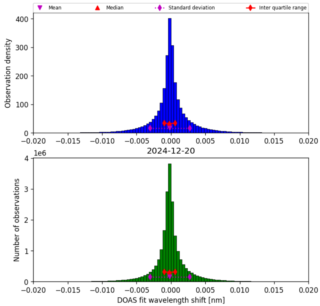
Figure 42: Histogram of “DOAS fit wavelength shift” for 2024-12-20 to 2024-12-20
