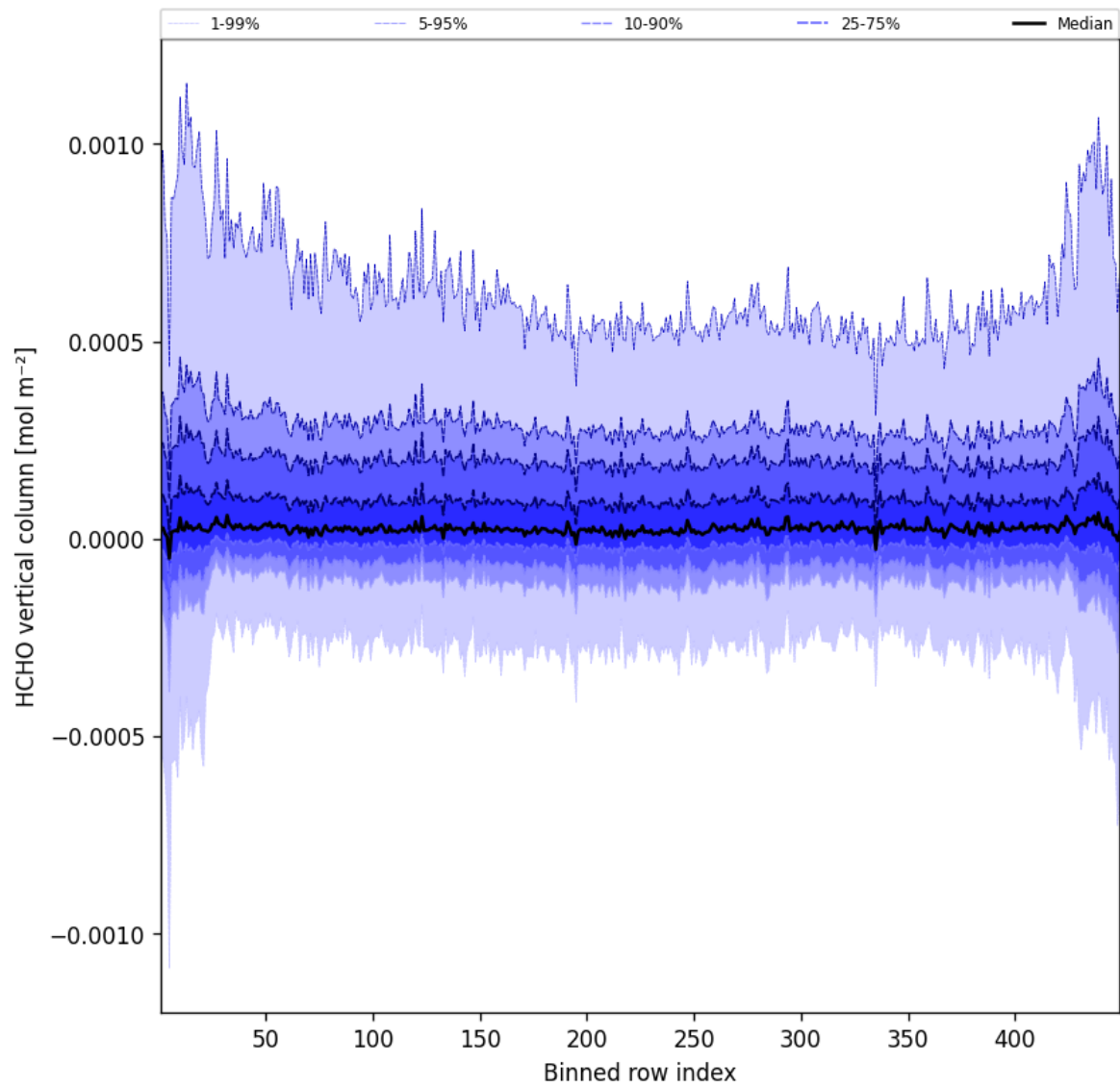
Figure 47: Along track statistics of “HCHO vertical column” for 2024-12-20 to 2024-12-20
