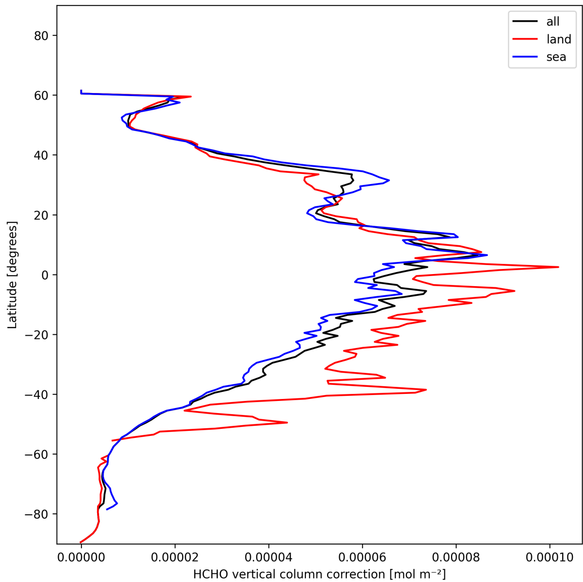
Figure 21: Zonal average of “HCHO vertical column correction” for 2024-12-20 to 2024-12-20.
