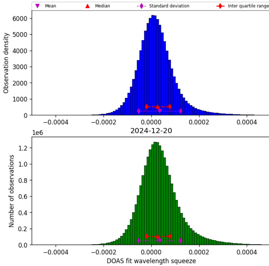
Figure 43: Histogram of “DOAS fit wavelength squeeze” for 2024-12-20 to 2024-12-20
