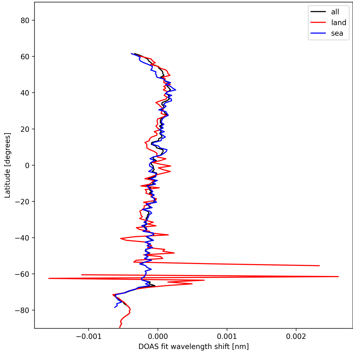
Figure 28: Zonal average of “DOAS fit wavelength shift” for 2024-12-20 to 2024-12-20.
