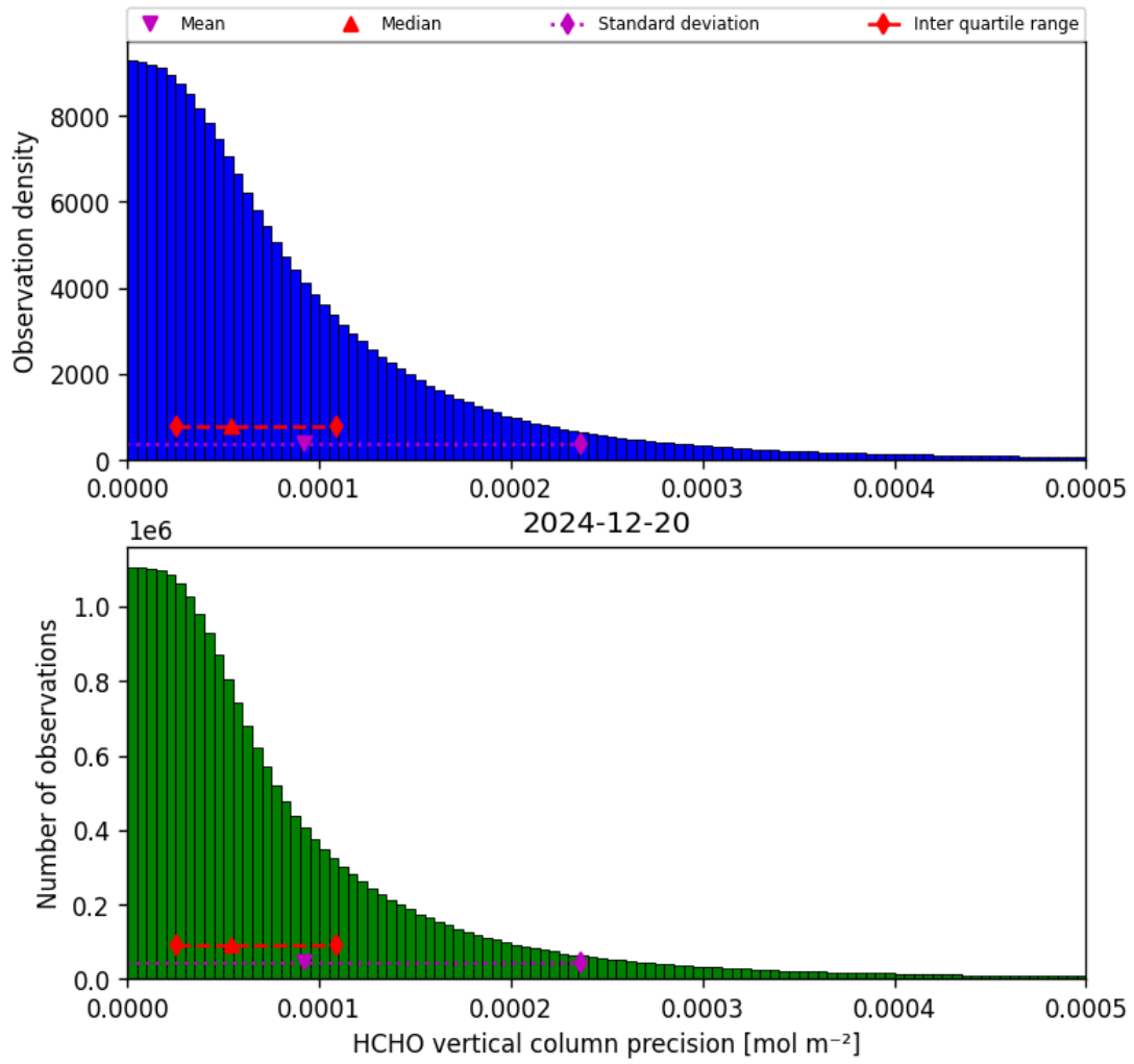
Figure 34: Histogram of “HCHO vertical column precision” for 2024-12-20 to 2024-12-20
