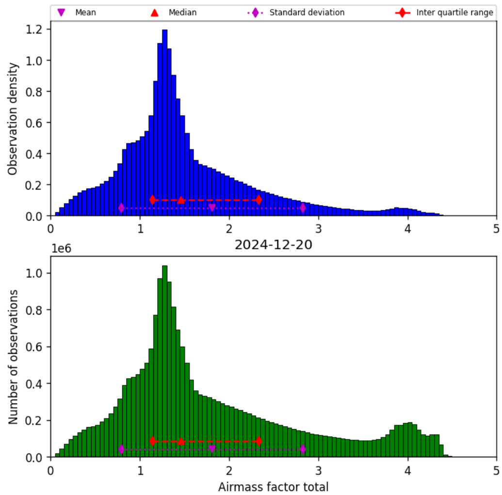
Figure 38: Histogram of “Airmass factor total” for 2024-12-20 to 2024-12-20
