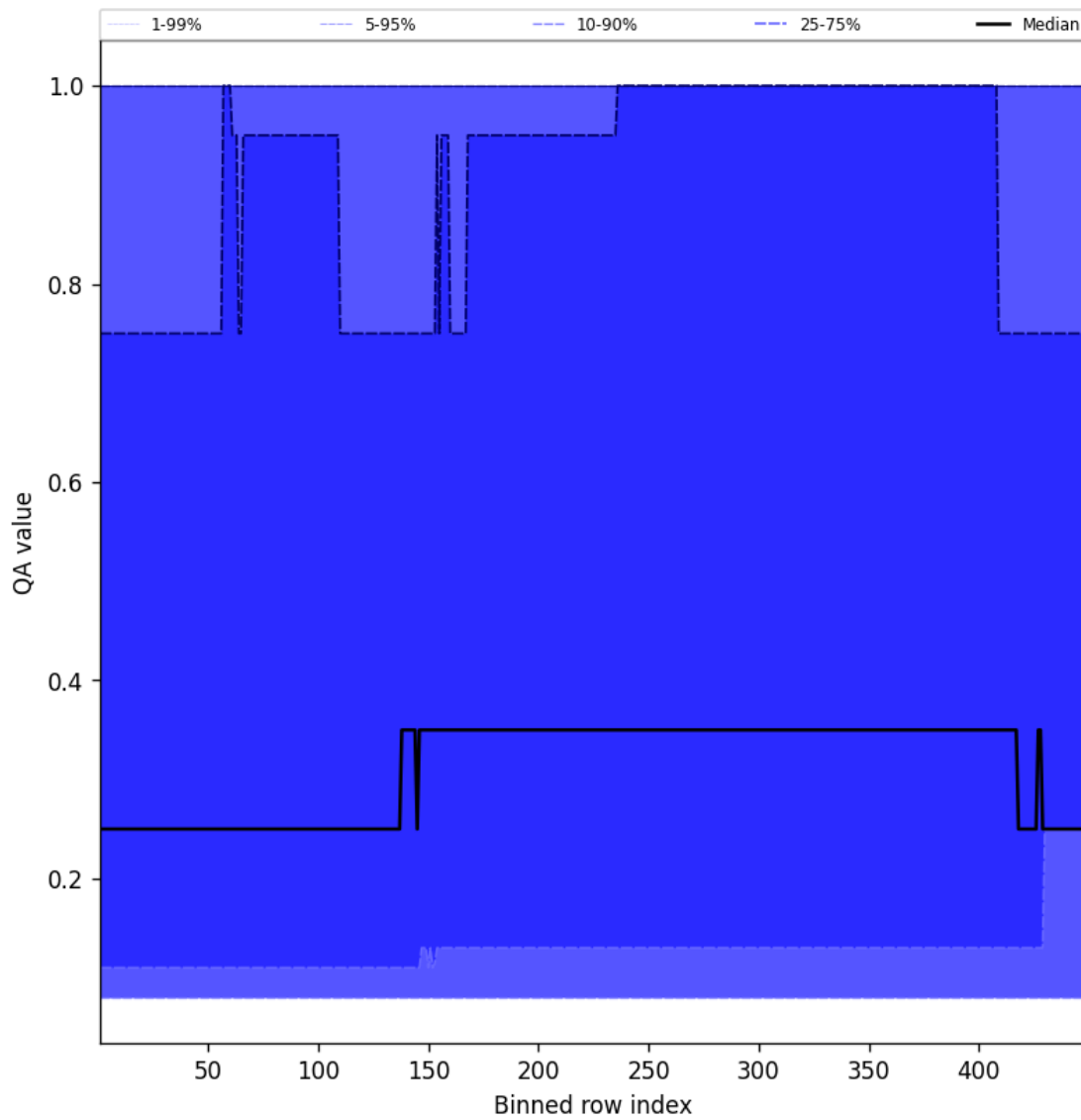
Figure 46: Along track statistics of “QA value” for 2024-12-20 to 2024-12-20
