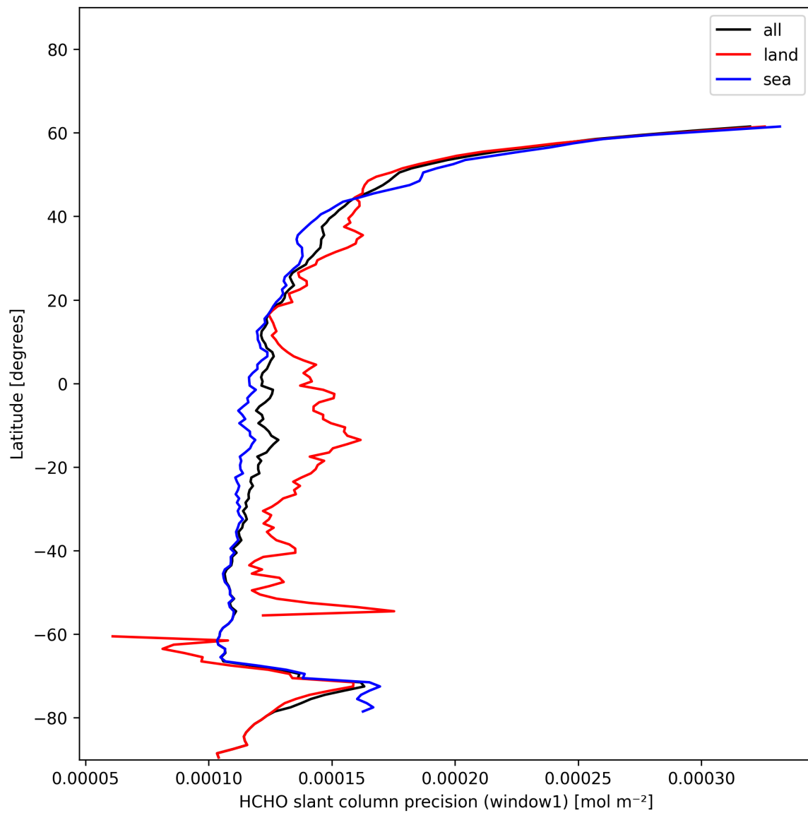
Figure 23: Zonal average of "HCHO slant column precision (window1)" for 2024-12-20 to 2024-12-20.
