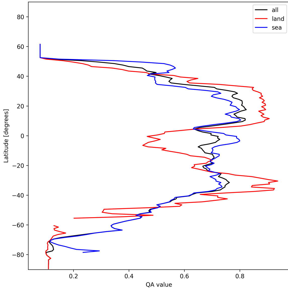
Figure 18: Zonal average of “QA value” for 2024-12-20 to 2024-12-20.
