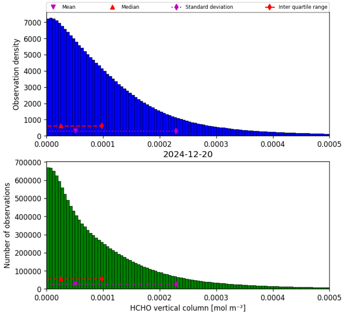
Figure 33: Histogram of “HCHO vertical column” for 2024-12-20 to 2024-12-20
