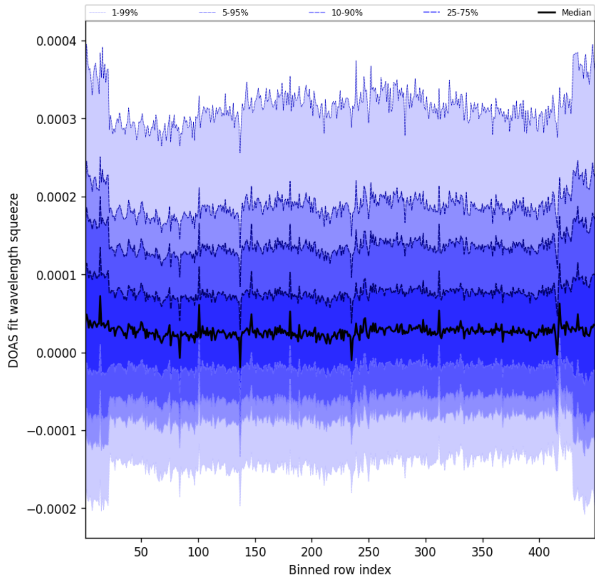
Figure 57: Along track statistics of “DOAS fit wavelength squeeze” for 2024-12-20 to 2024-12-20
