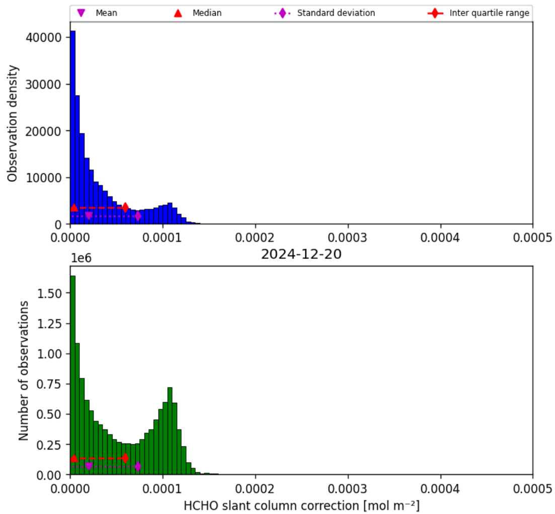
Figure 45: Histogram of “HCHO slant column correction” for 2024-12-20 to 2024-12-20
