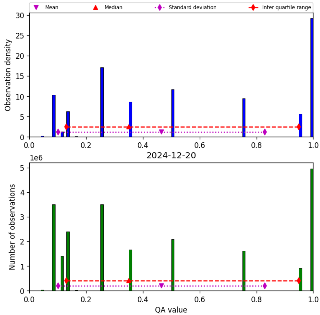
Figure 32: Histogram of “QA value” for 2024-12-20 to 2024-12-20
