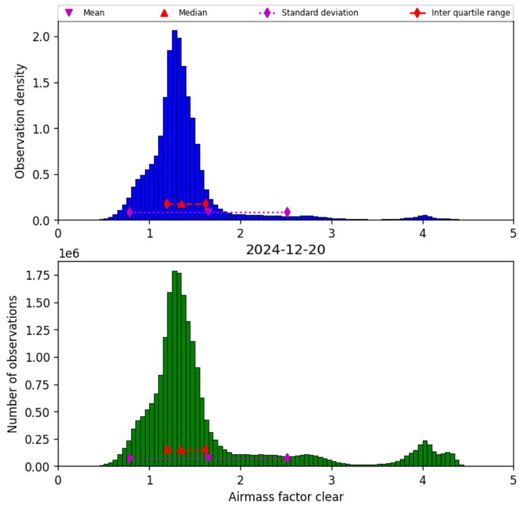
Figure 40: Histogram of “Airmass factor clear” for 2024-12-20 to 2024-12-20
