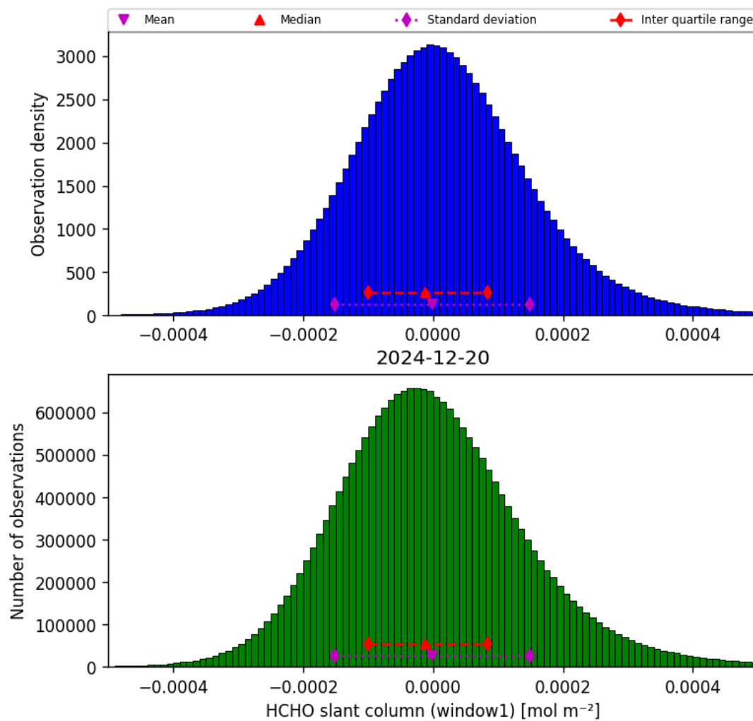
Figure 36: Histogram of “HCHO slant column (window1)” for 2024-12-20 to 2024-12-20
