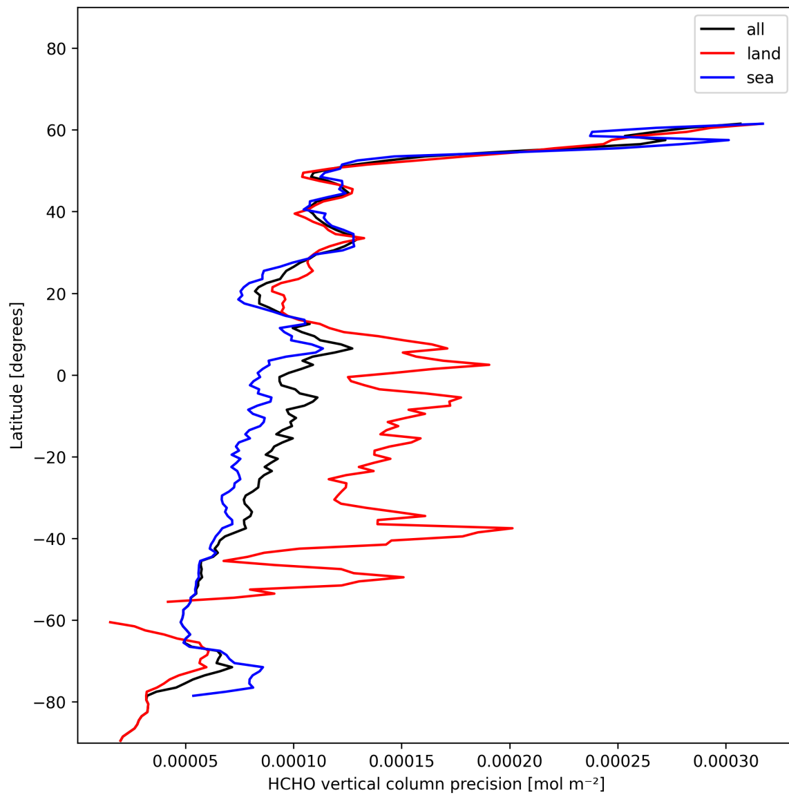
Figure 20: Zonal average of “HCHO vertical column precision” for 2024-12-20 to 2024-12-20.
