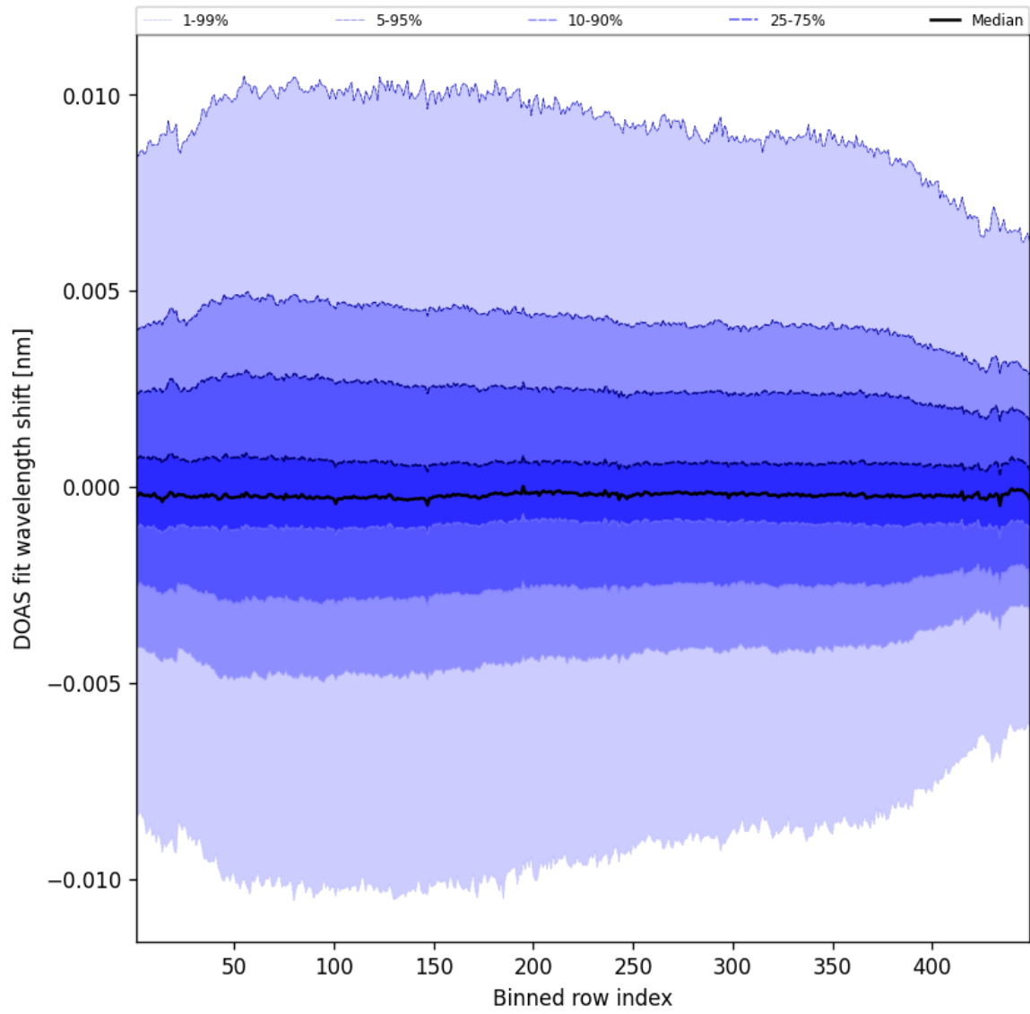
Figure 56: Along track statistics of “DOAS fit wavelength shift” for 2024-12-20 to 2024-12-20
