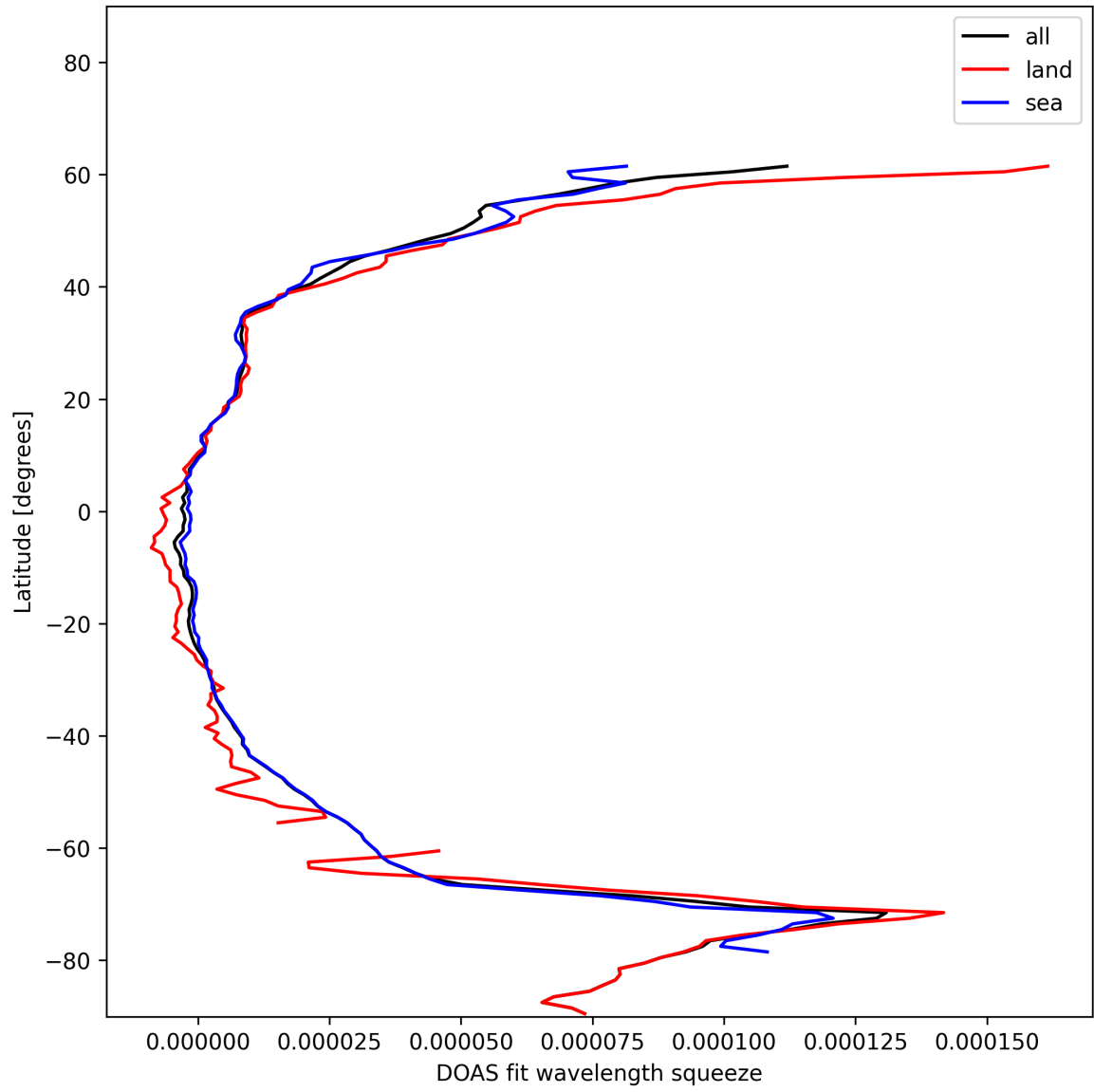
Figure 29: Zonal average of “DOAS fit wavelength squeeze” for 2024-12-20 to 2024-12-20.
