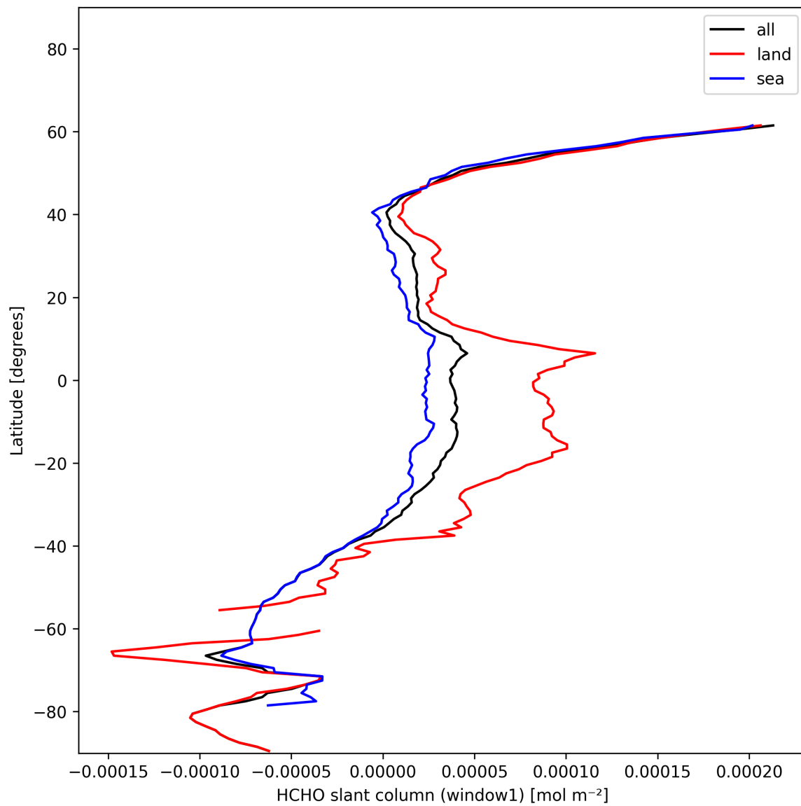
Figure 22: Zonal average of “HCHO slant column (window1)” for 2024-12-20 to 2024-12-20.
