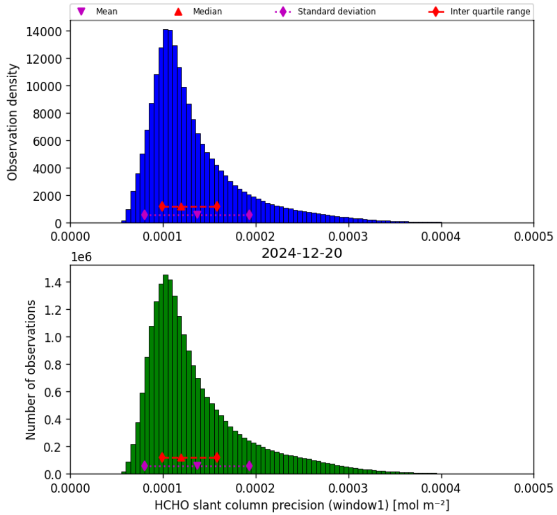
Figure 37: Histogram of “HCHO slant column precision (window1)” for 2024-12-20 to 2024-12-20
