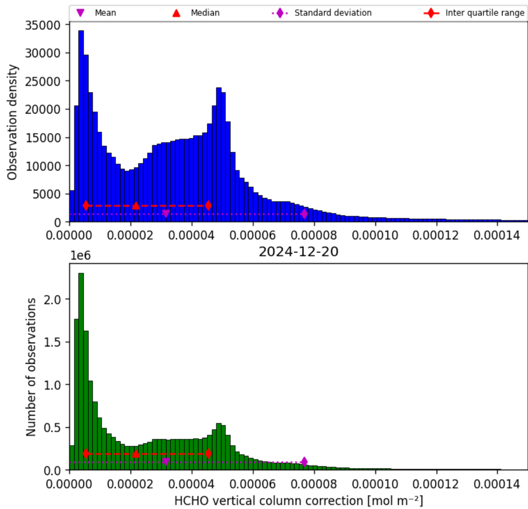
Figure 35: Histogram of “HCHO vertical column correction” for 2024-12-20 to 2024-12-20
