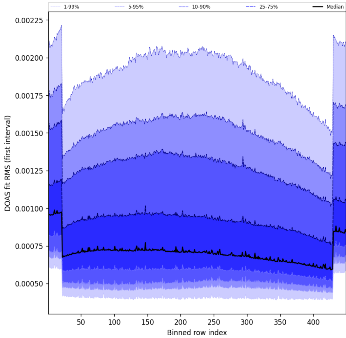
Figure 58: Along track statistics of “DOAS fit RMS (first interval)” for 2024-12-20 to 2024-12-20
