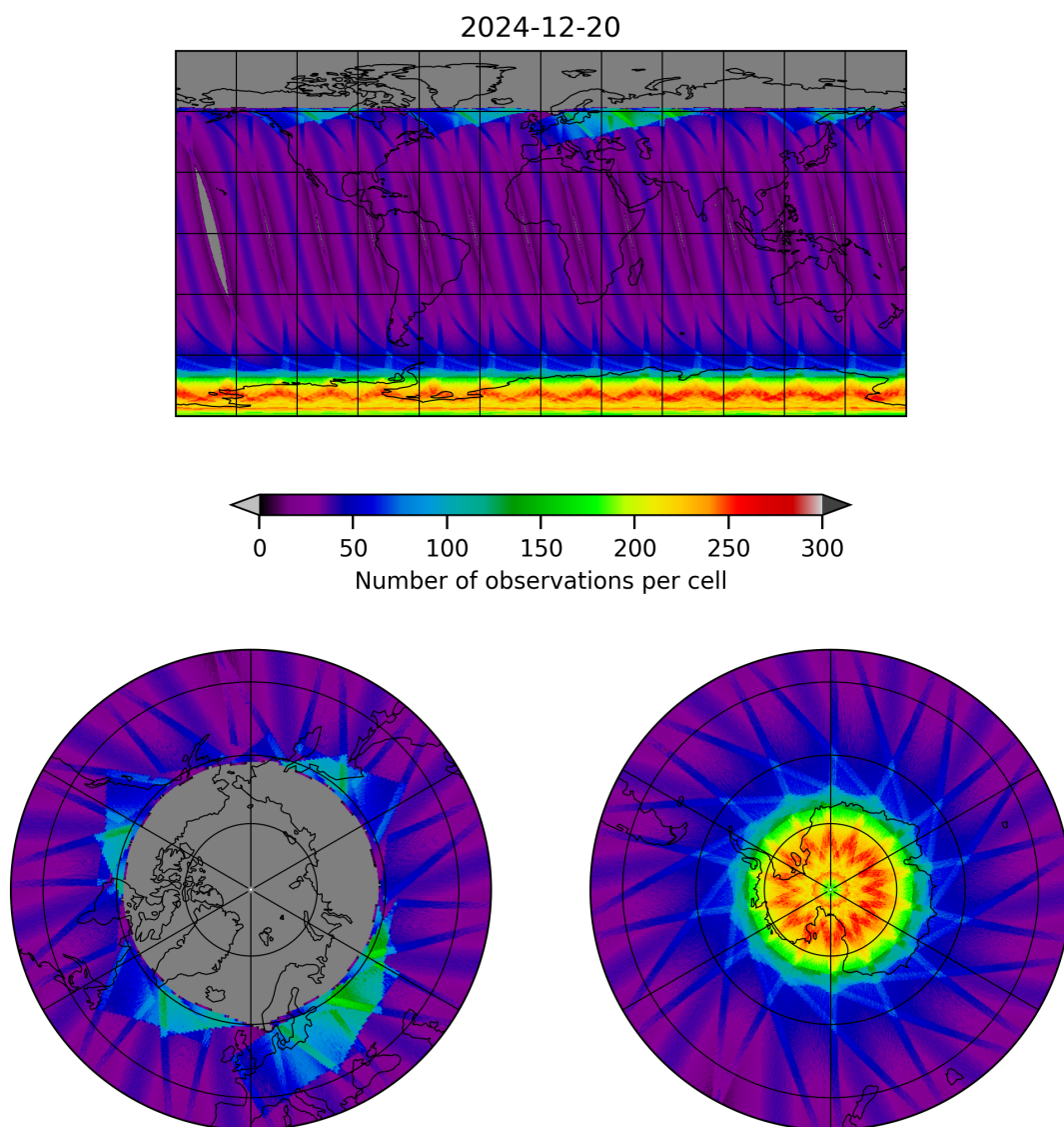
Figure 17: Map of the number of observations for 2024-12-20 to 2024-12-20
