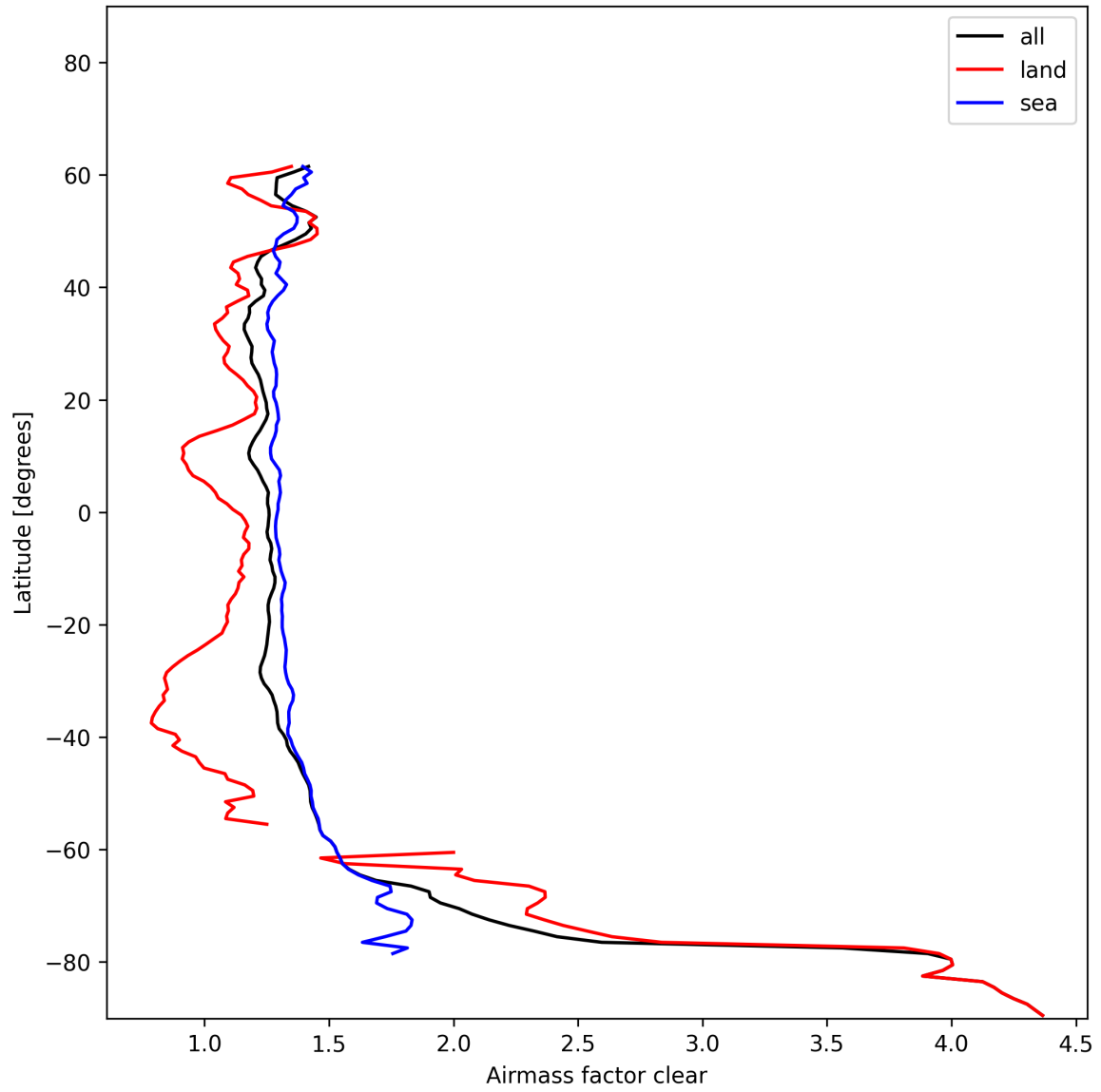
Figure 26: Zonal average of “Airmass factor clear” for 2024-12-20 to 2024-12-20.
