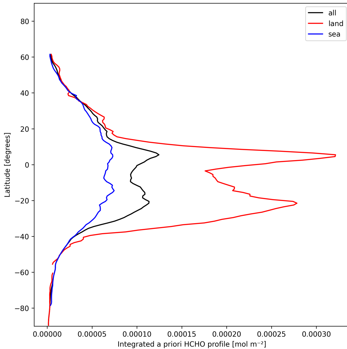
Figure 27: Zonal average of “Integrated a priori HCHO profile” for 2024-12-20 to 2024-12-20.
