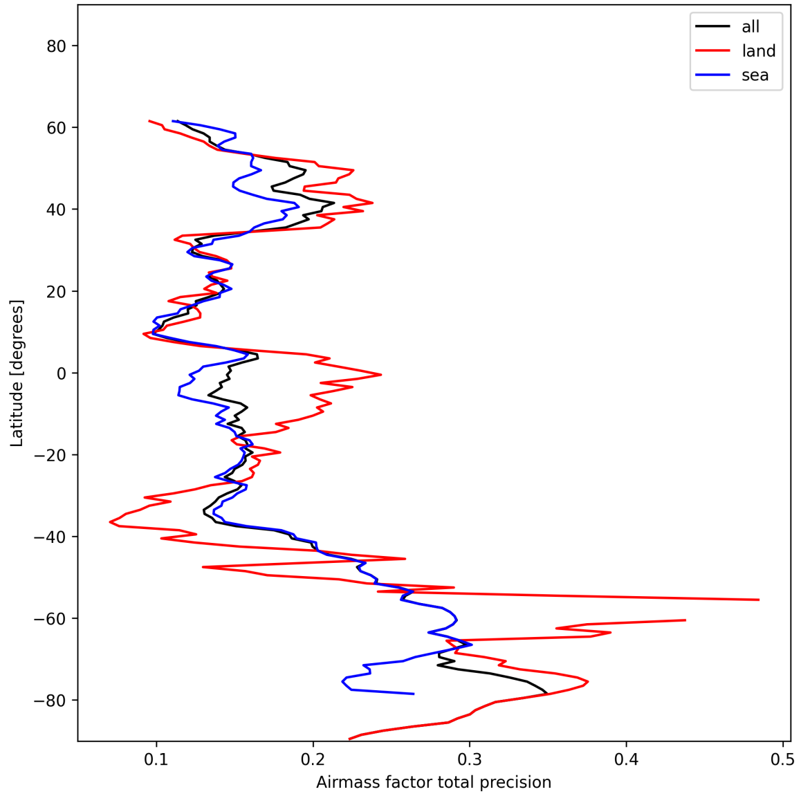
Figure 25: Zonal average of “Airmass factor total precision” for 2024-12-20 to 2024-12-20.
