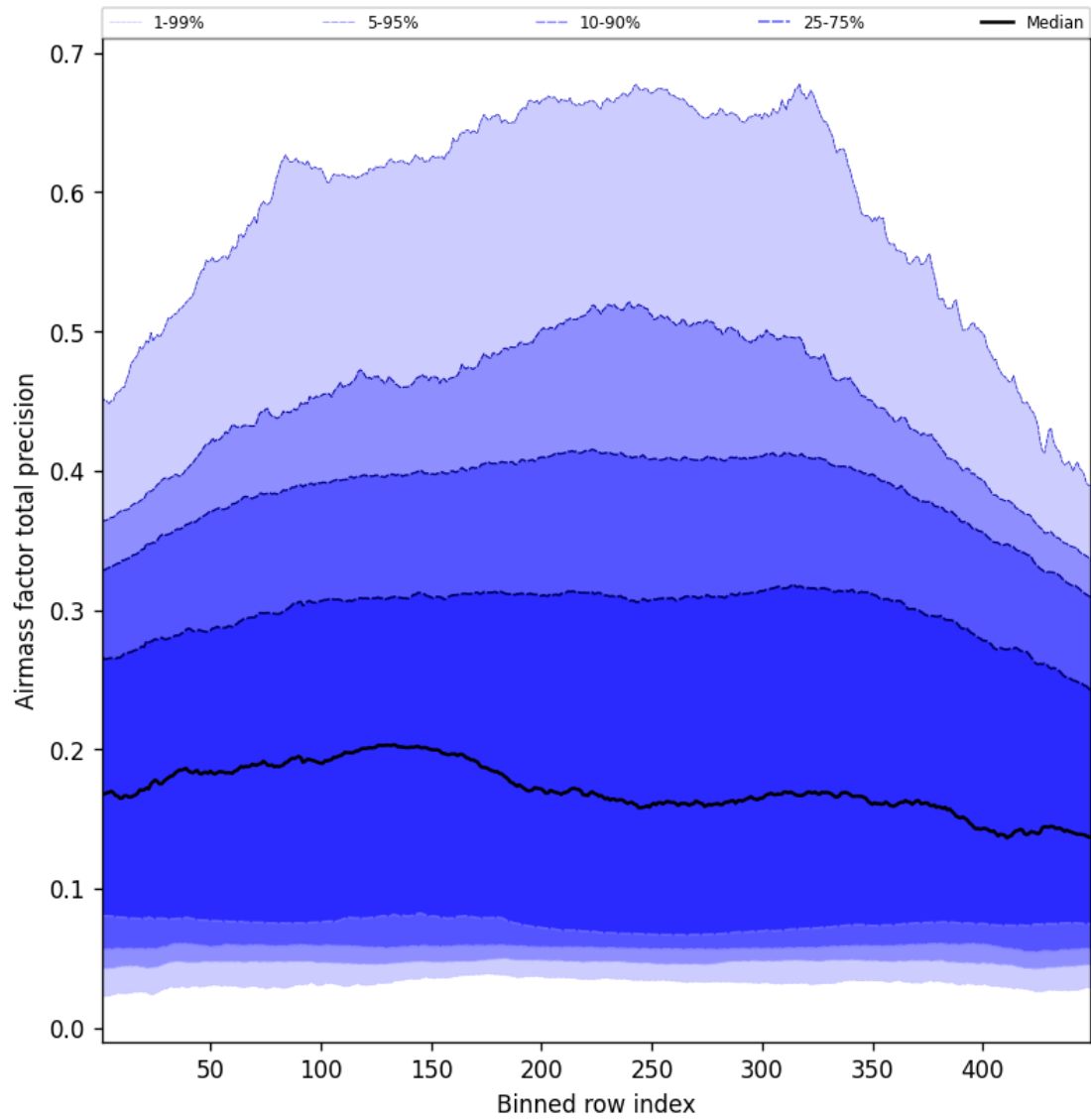
Figure 53: Along track statistics of “Airmass factor total precision” for 2024-12-20 to 2024-12-20
