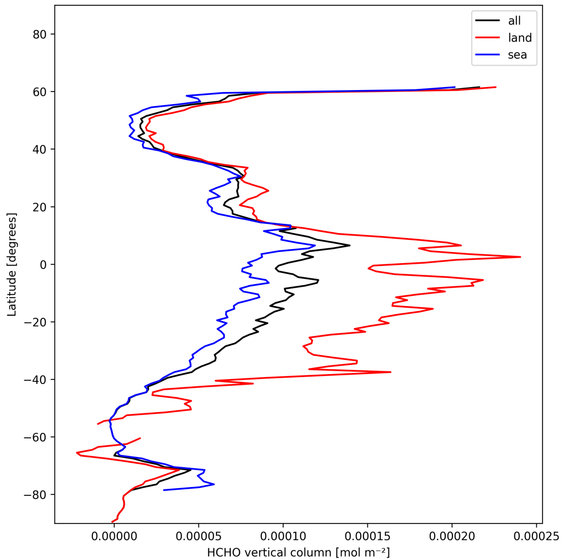
Figure 19: Zonal average of “HCHO vertical column” for 2024-12-20 to 2024-12-20.
