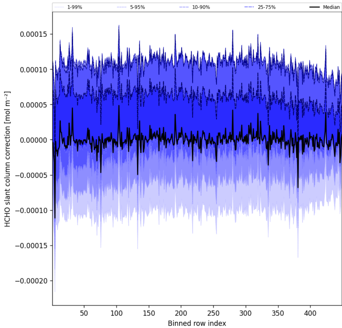
Figure 59: Along track statistics of “HCHO slant column correction” for 2024-12-20 to 2024-12-20
