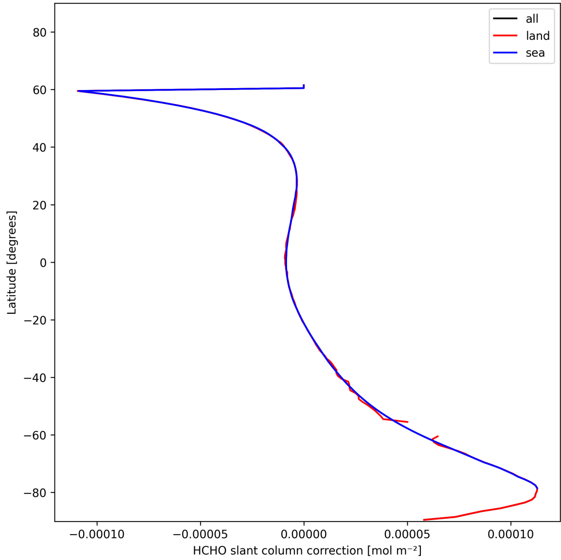
Figure 31: Zonal average of “HCHO slant column correction” for 2024-12-20 to 2024-12-20.
