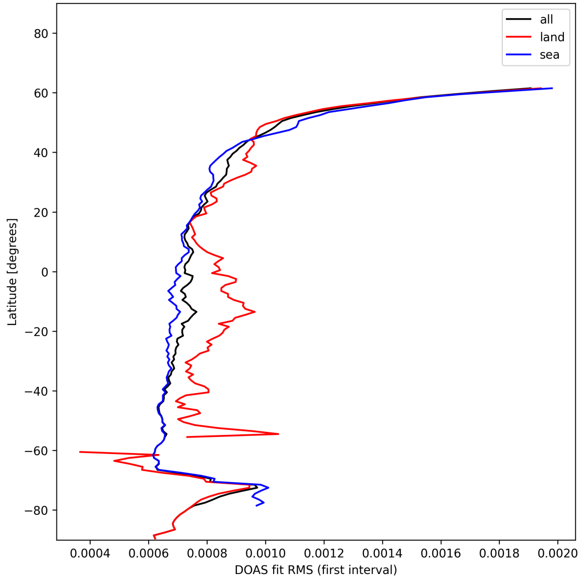
Figure 30: Zonal average of “DOAS fit RMS (first interval)” for 2024-12-20 to 2024-12-20.
