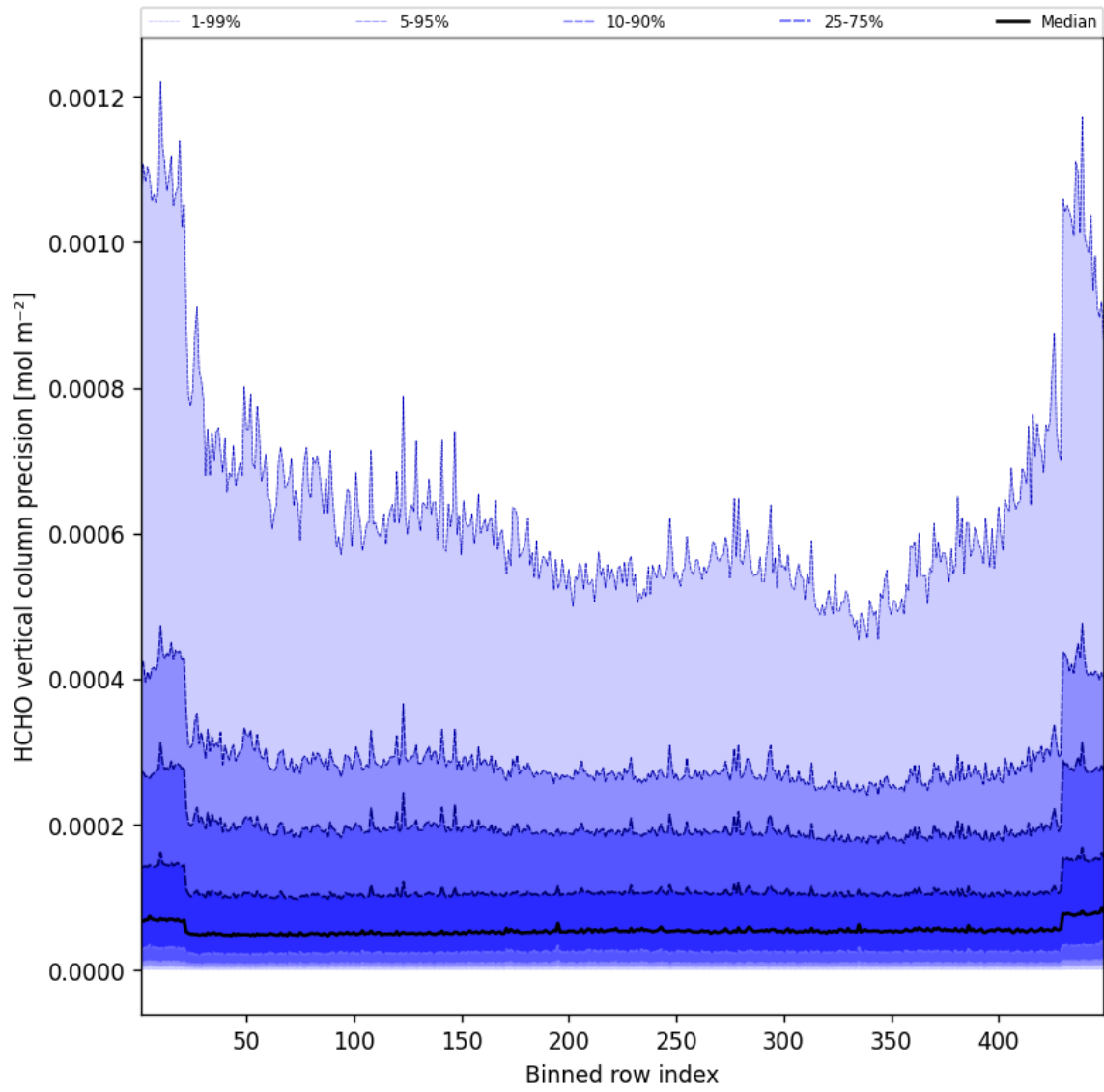
Figure 48: Along track statistics of “HCHO vertical column precision” for 2024-12-20 to 2024-12-20
