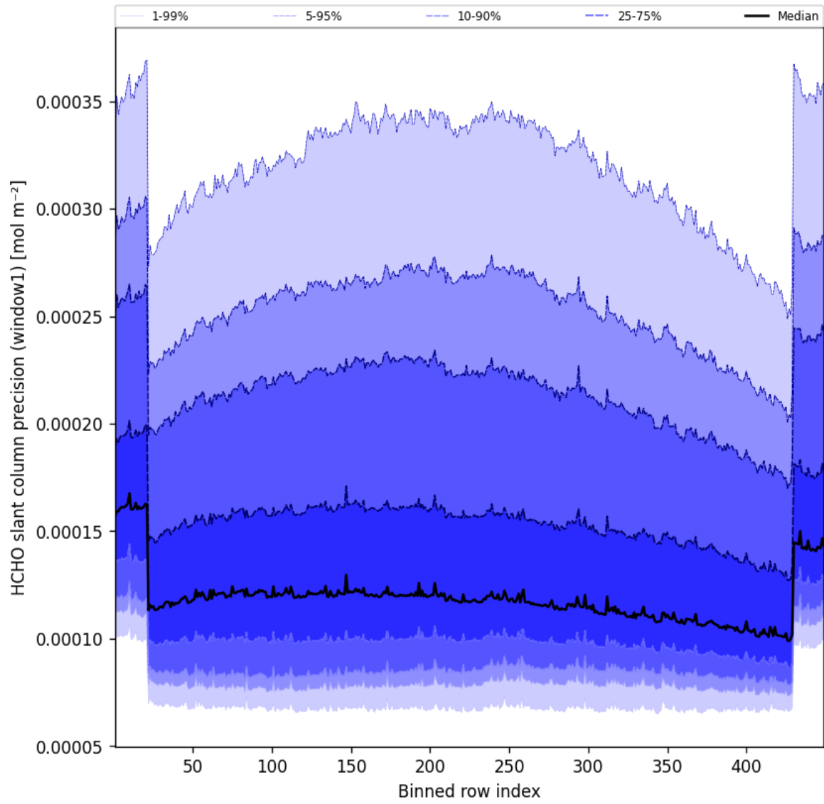
Figure 51: Along track statistics of “HCHO slant column precision (window1)” for 2024-12-20 to 2024-12-20
