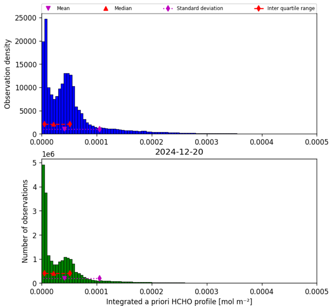
Figure 41: Histogram of “Integrated a priori HCHO profile” for 2024-12-20 to 2024-12-20
