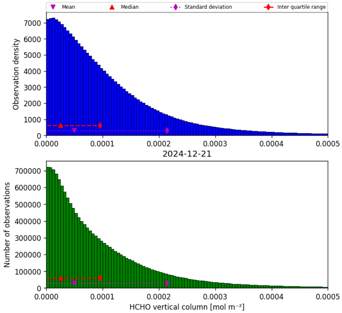
Figure 33: Histogram of “HCHO vertical column” for 2024-12-21 to 2024-12-22
