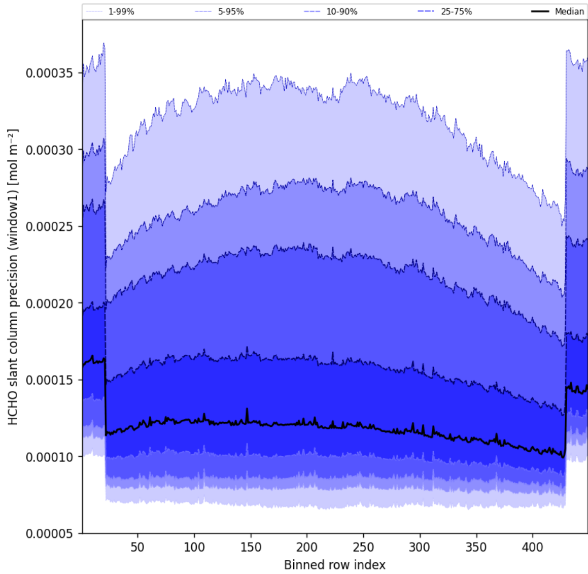
Figure 51: Along track statistics of “HCHO slant column precision (window1)” for 2024-12-21 to 2024-12-22
