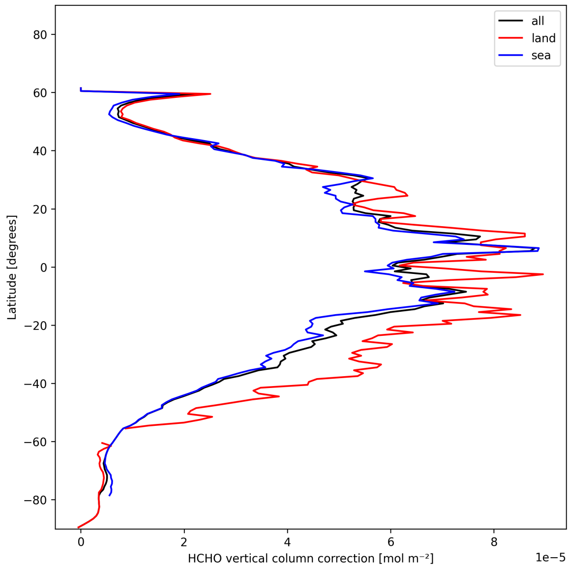
Figure 21: Zonal average of “HCHO vertical column correction” for 2024-12-21 to 2024-12-22.
