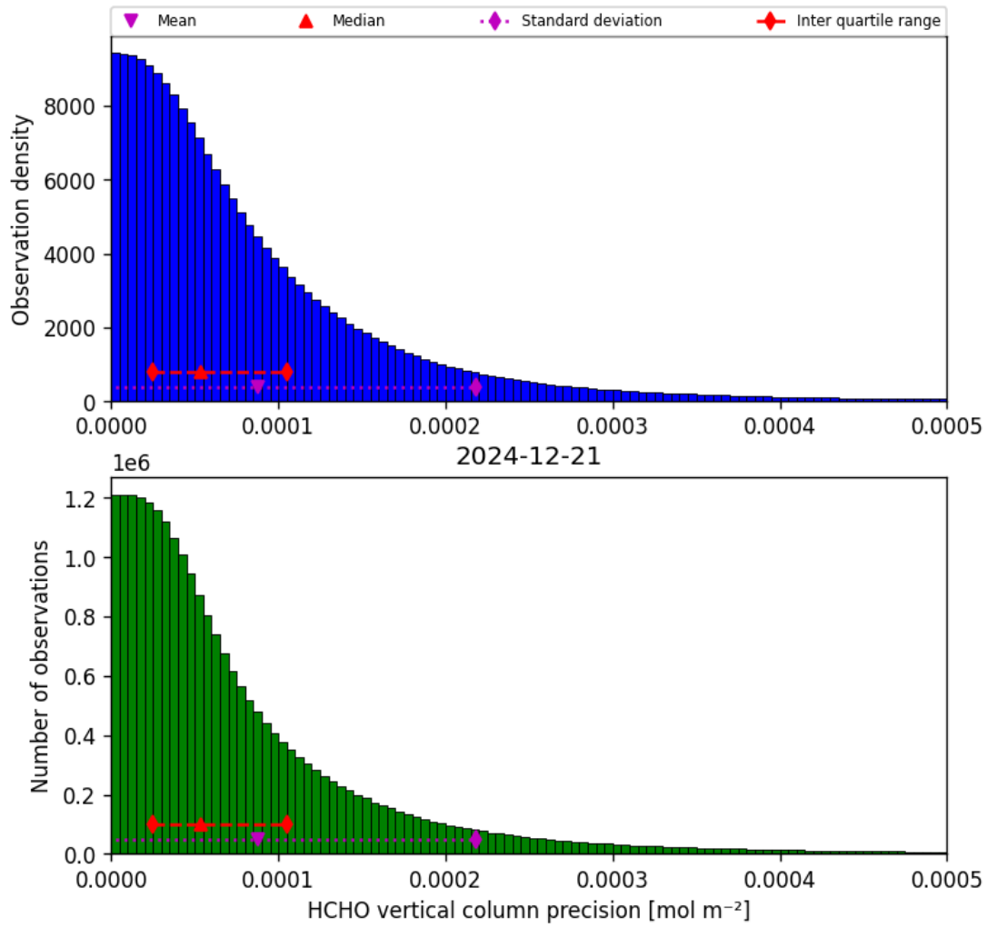
Figure 34: Histogram of “HCHO vertical column precision” for 2024-12-21 to 2024-12-22
