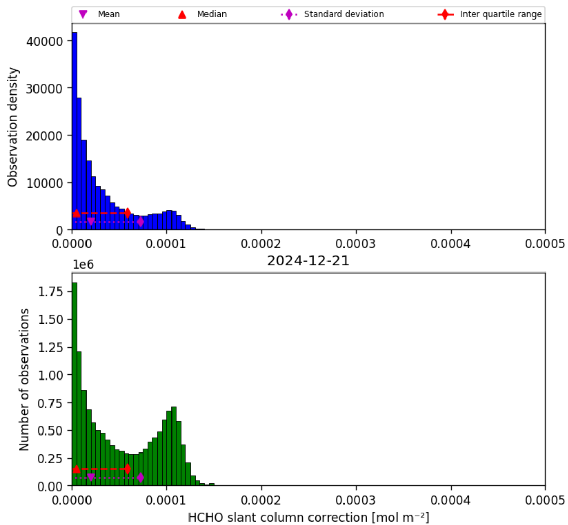
Figure 45: Histogram of “HCHO slant column correction” for 2024-12-21 to 2024-12-22
