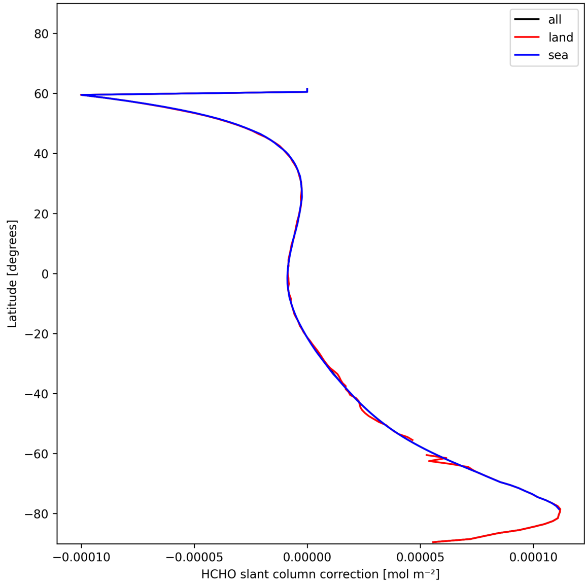
Figure 31: Zonal average of “HCHO slant column correction” for 2024-12-21 to 2024-12-22.
