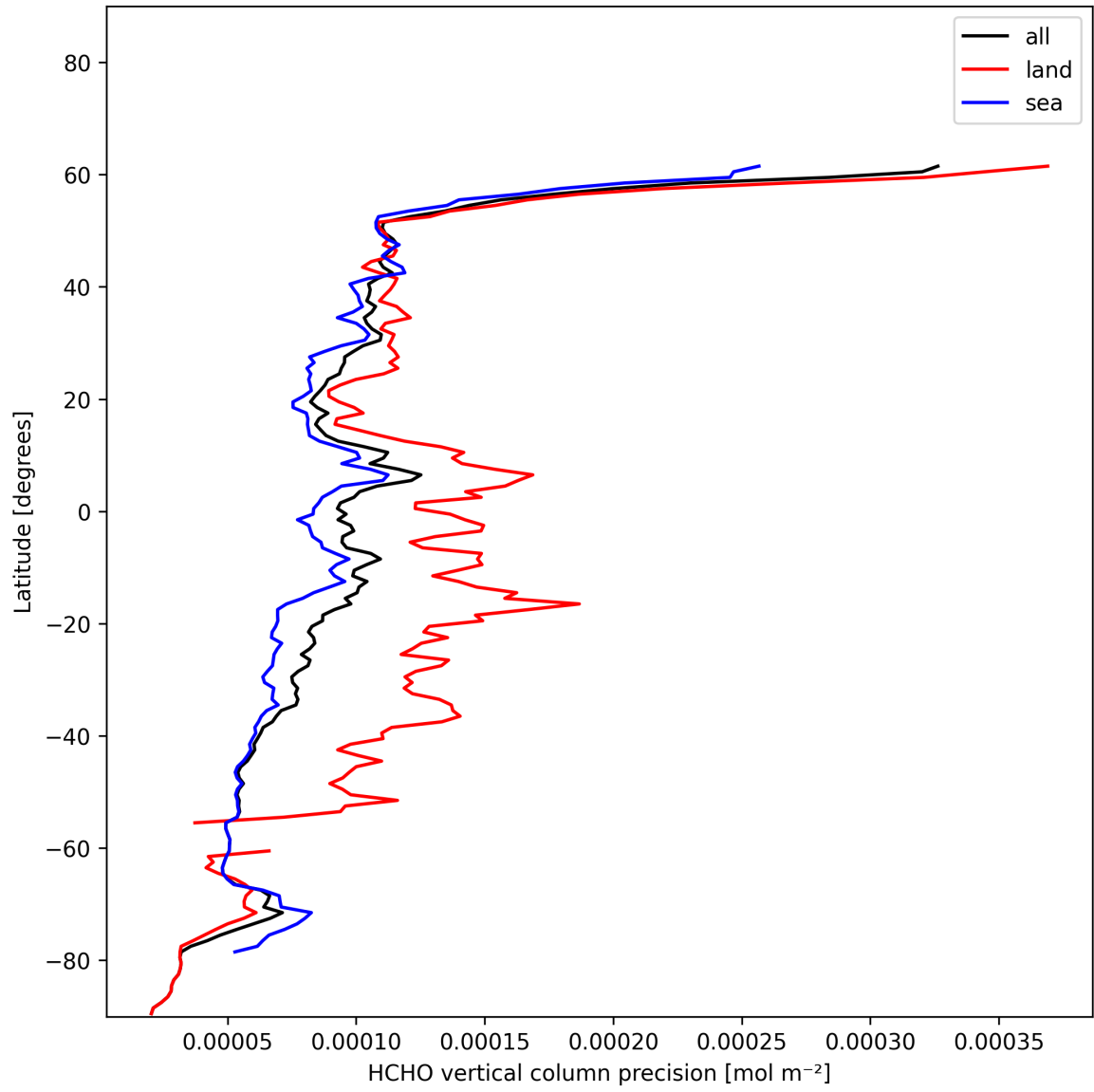
Figure 20: Zonal average of “HCHO vertical column precision” for 2024-12-21 to 2024-12-22.
