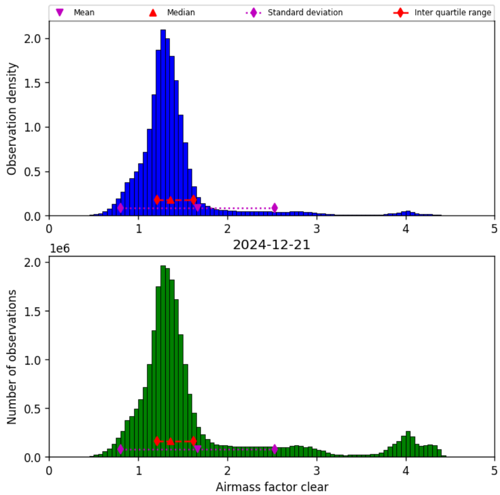
Figure 40: Histogram of “Airmass factor clear” for 2024-12-21 to 2024-12-22
