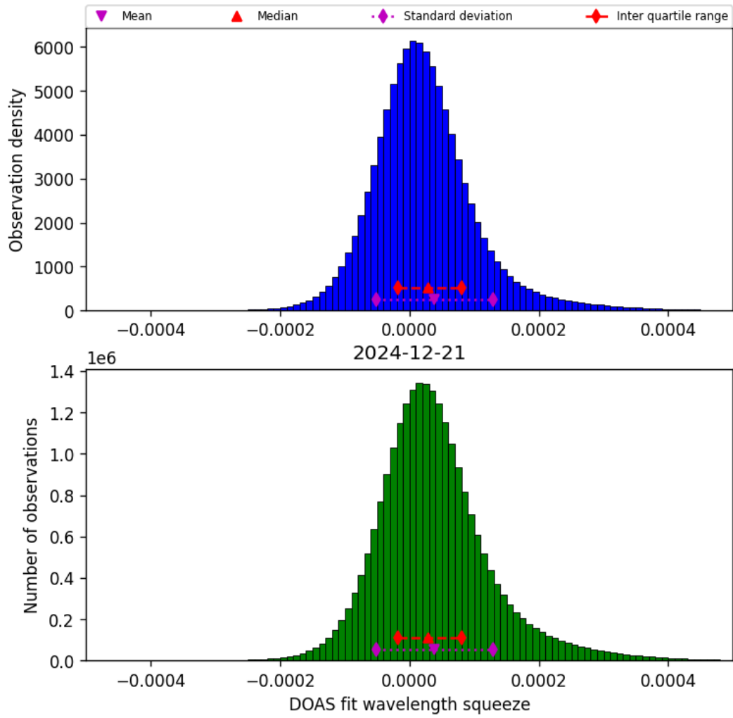
Figure 43: Histogram of “DOAS fit wavelength squeeze” for 2024-12-21 to 2024-12-22
