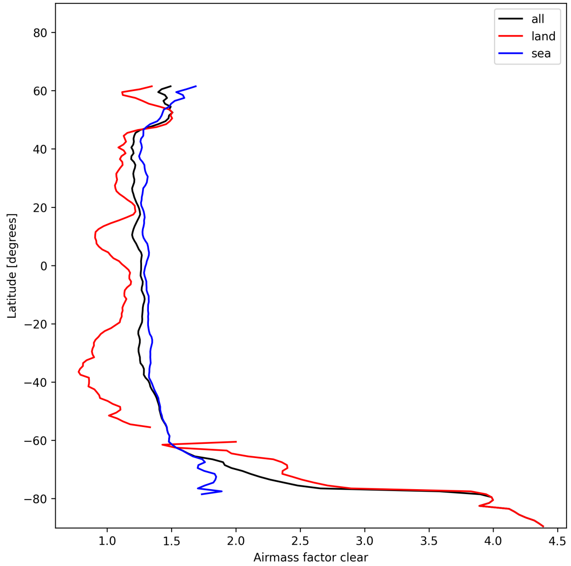
Figure 26: Zonal average of “Airmass factor clear” for 2024-12-21 to 2024-12-22.
