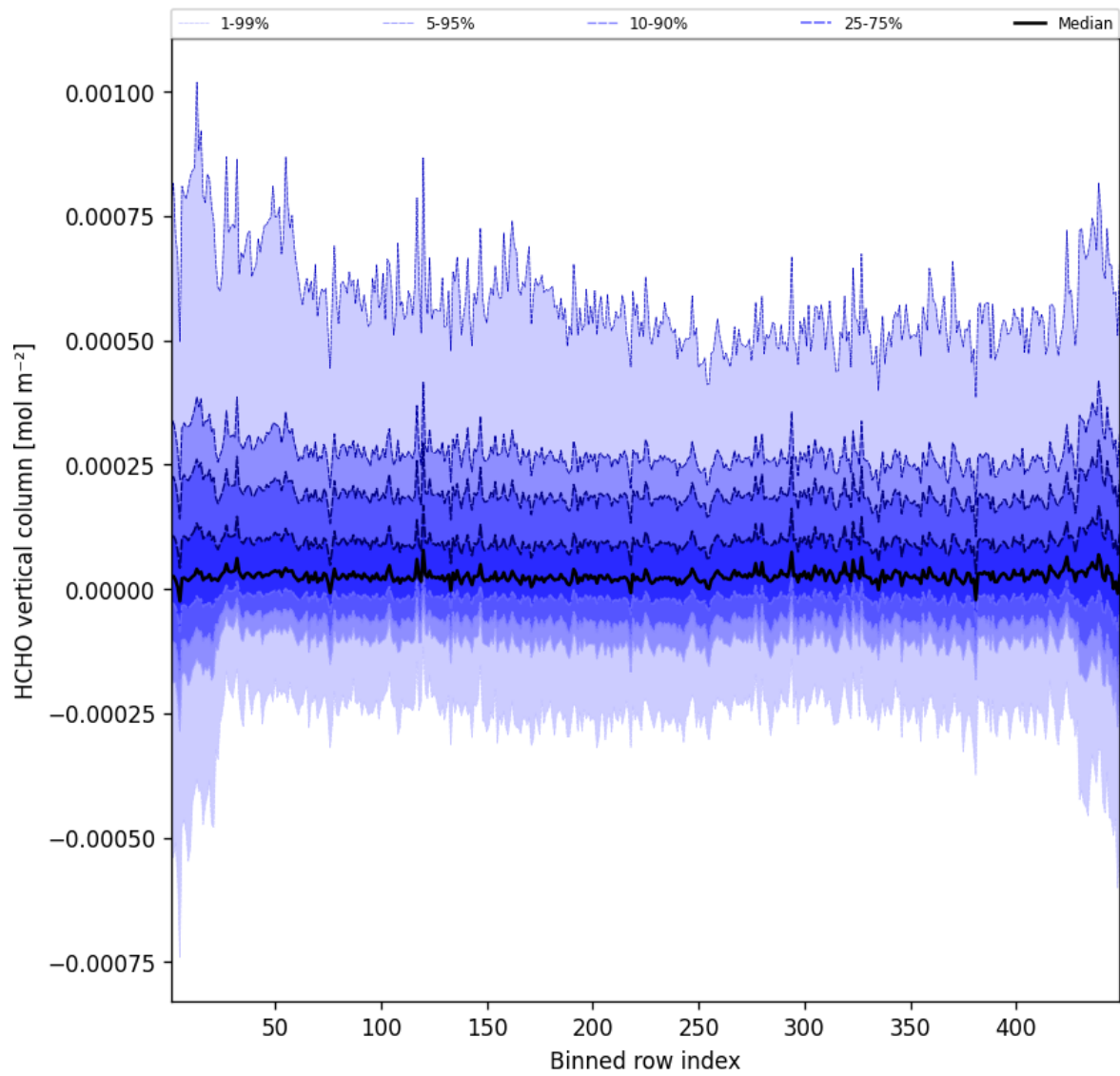
Figure 47: Along track statistics of “HCHO vertical column” for 2024-12-21 to 2024-12-22
