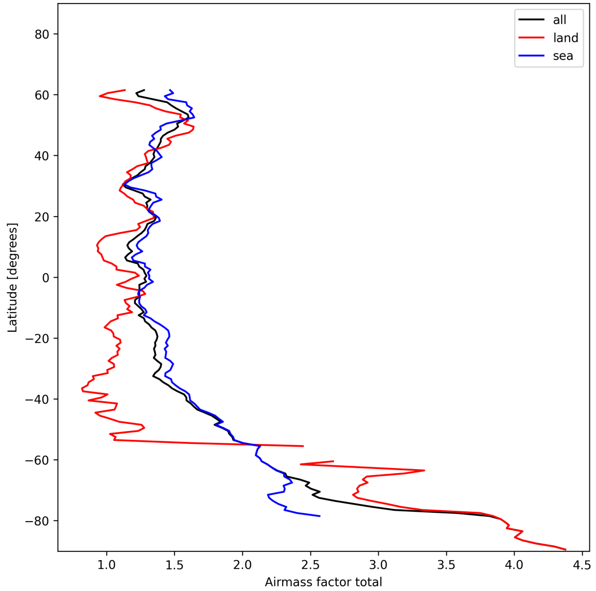
Figure 24: Zonal average of “Airmass factor total” for 2024-12-21 to 2024-12-22.
