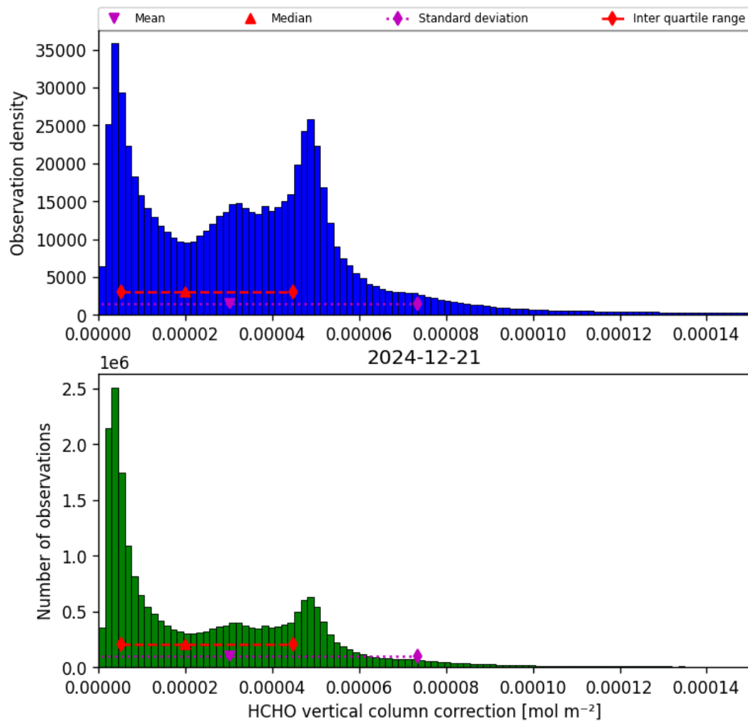
Figure 35: Histogram of “HCHO vertical column correction” for 2024-12-21 to 2024-12-22
