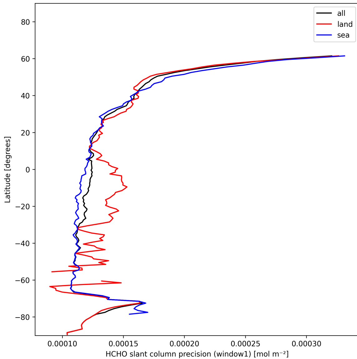
Figure 23: Zonal average of “HCHO slant column precision (window1)” for 2024-12-21 to 2024-12-22.
