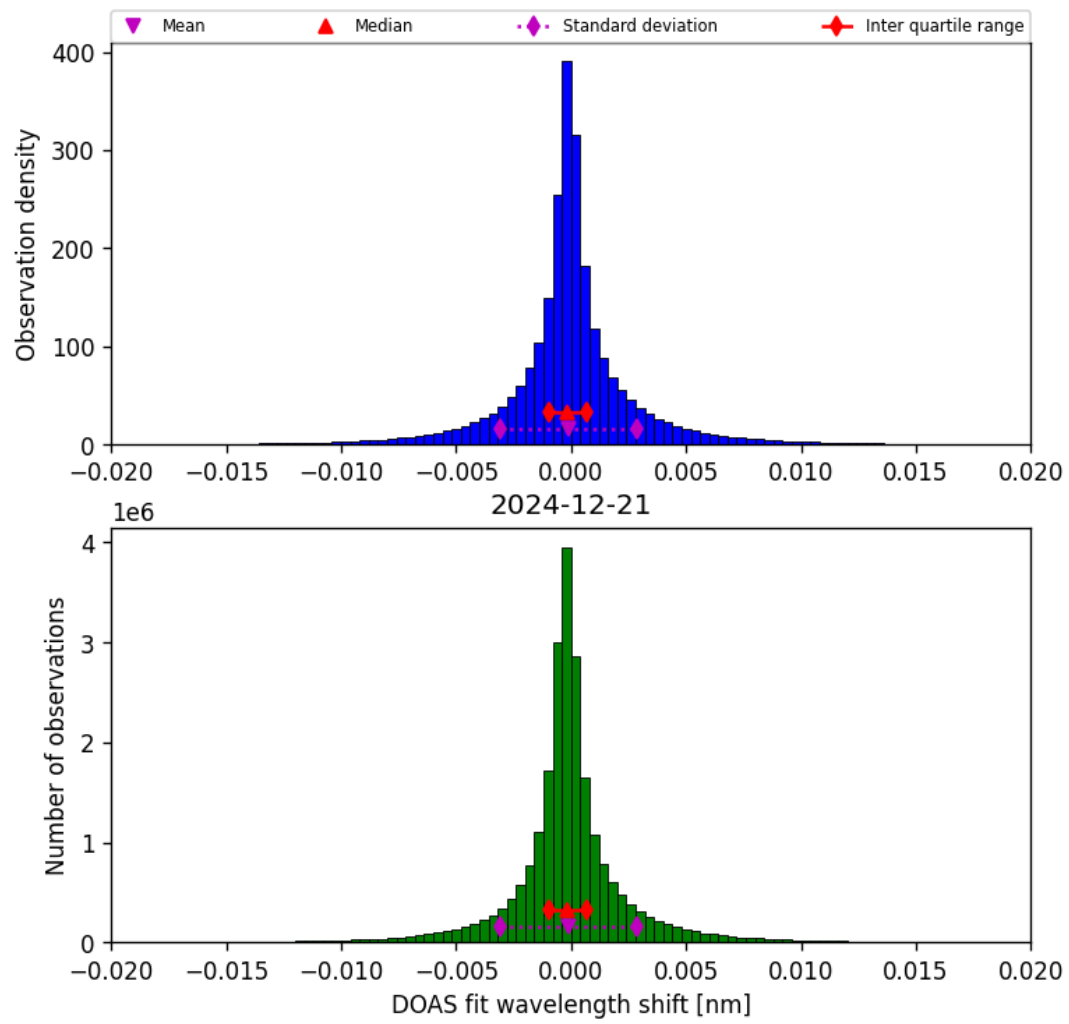
Figure 42: Histogram of “DOAS fit wavelength shift” for 2024-12-21 to 2024-12-22
