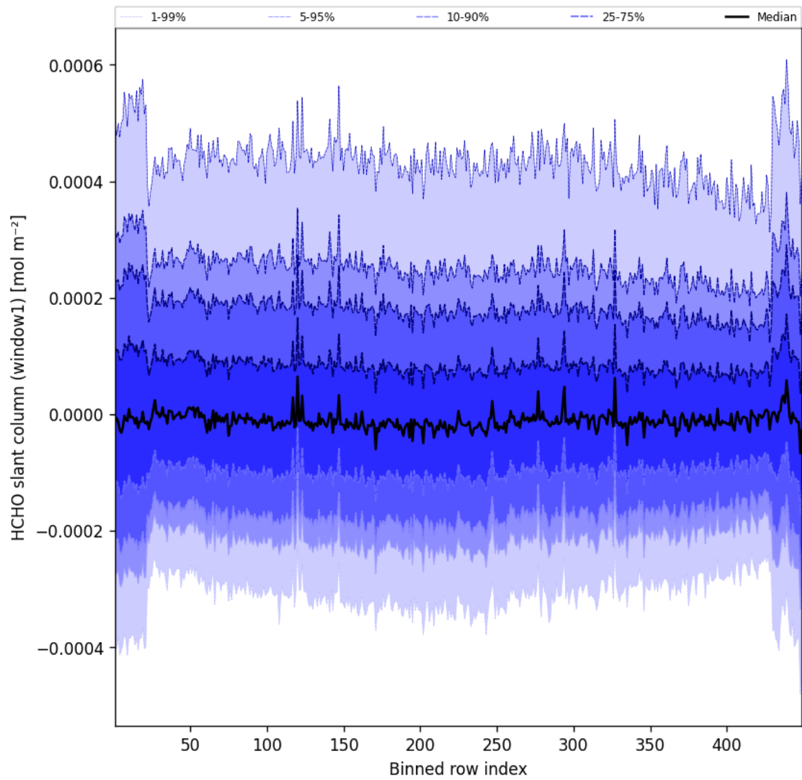
Figure 50: Along track statistics of “HCHO slant column (window1)” for 2024-12-21 to 2024-12-22
