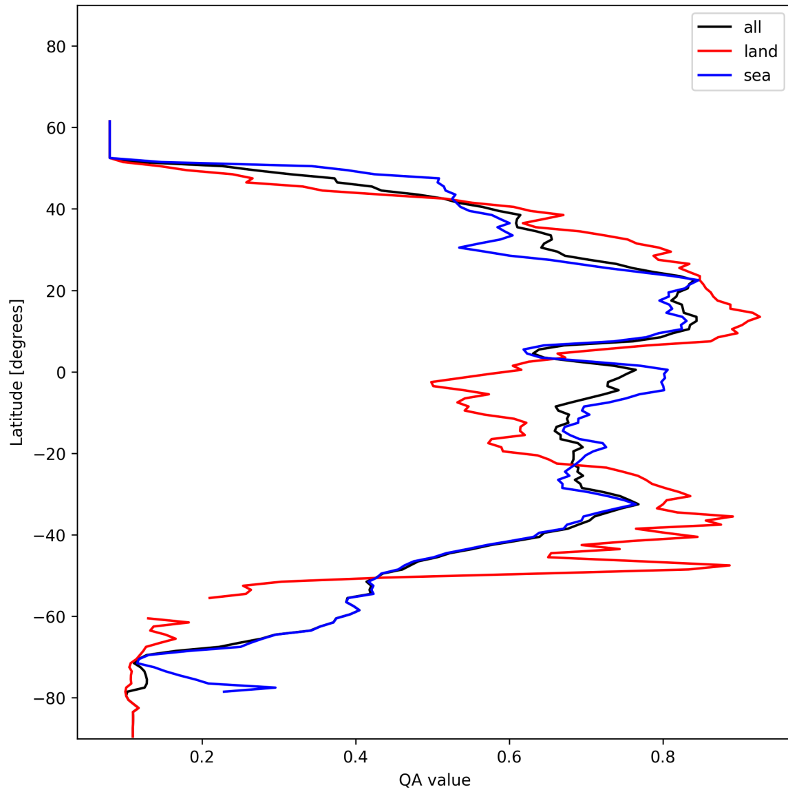
Figure 18: Zonal average of “QA value” for 2024-12-21 to 2024-12-22.
