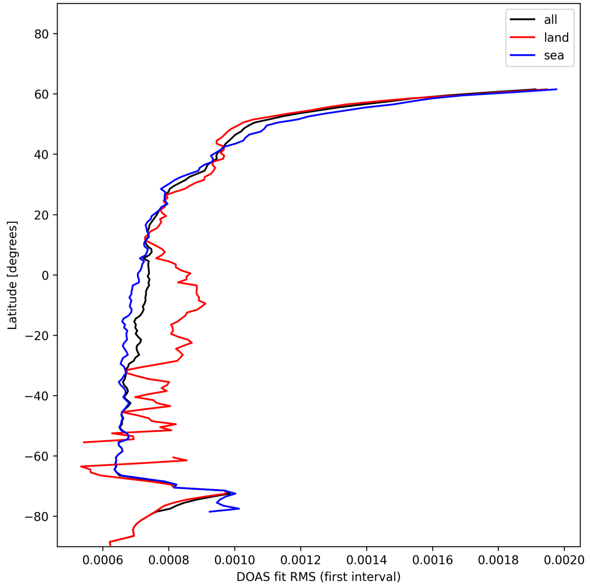
Figure 30: Zonal average of “DOAS fit RMS (first interval)” for 2024-12-21 to 2024-12-22.
