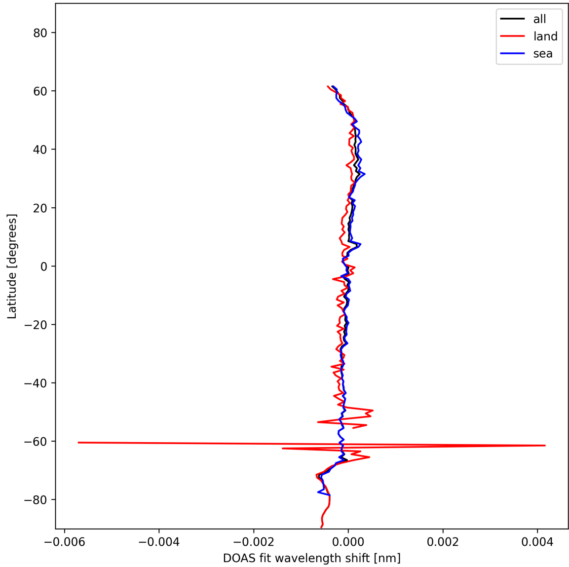
Figure 28: Zonal average of “DOAS fit wavelength shift” for 2024-12-21 to 2024-12-22.
