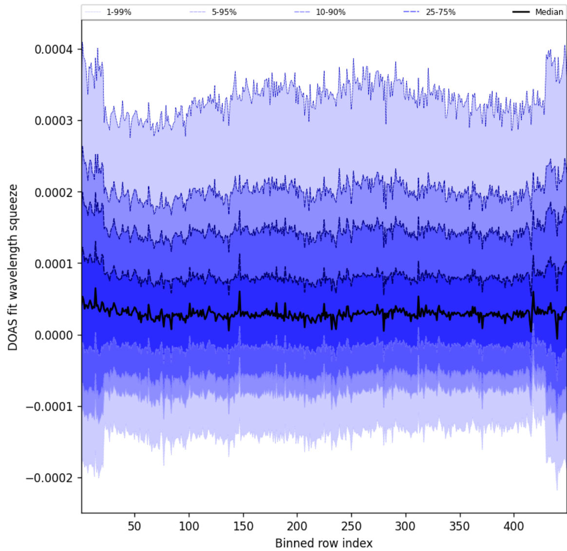
Figure 57: Along track statistics of “DOAS fit wavelength squeeze” for 2024-12-21 to 2024-12-22
