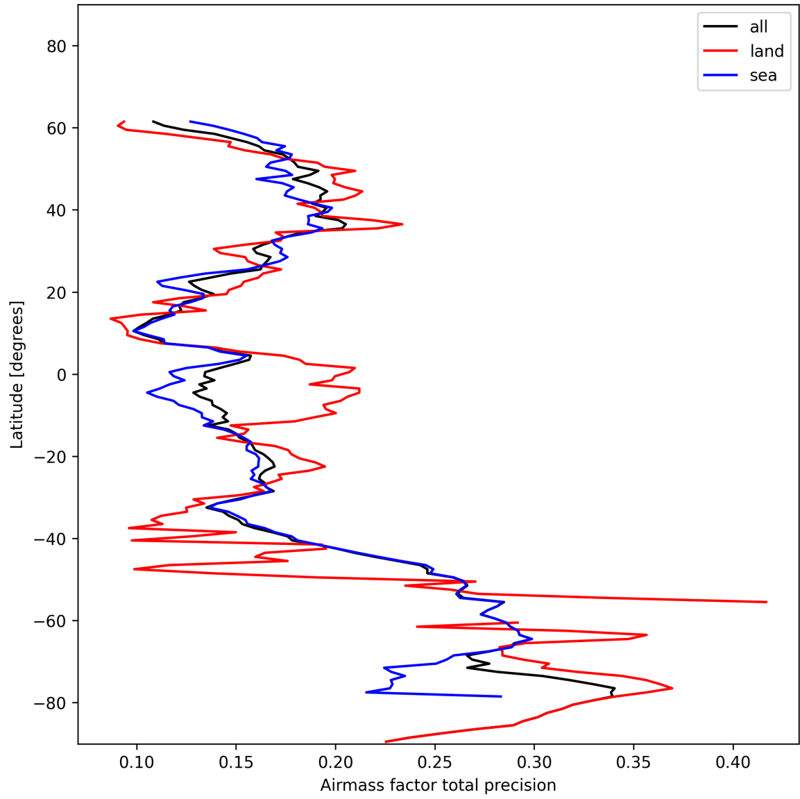
Figure 25: Zonal average of “Airmass factor total precision” for 2024-12-21 to 2024-12-22.
