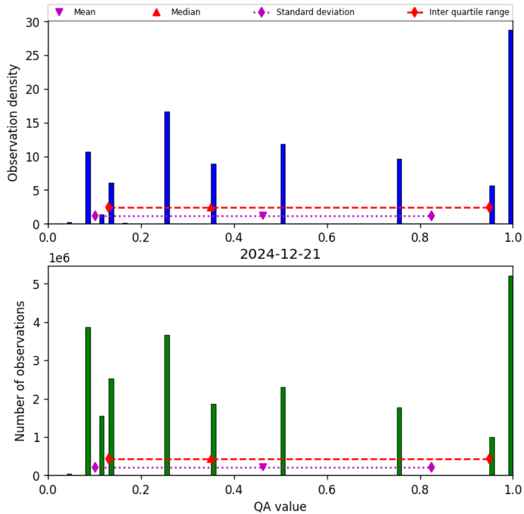
Figure 32: Histogram of “QA value” for 2024-12-21 to 2024-12-22
