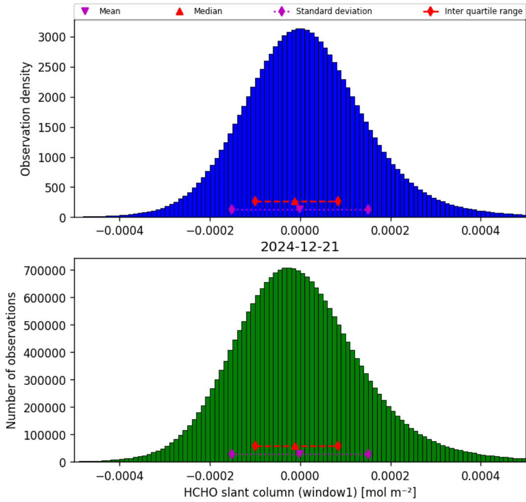
Figure 36: Histogram of “HCHO slant column (window1)” for 2024-12-21 to 2024-12-22
