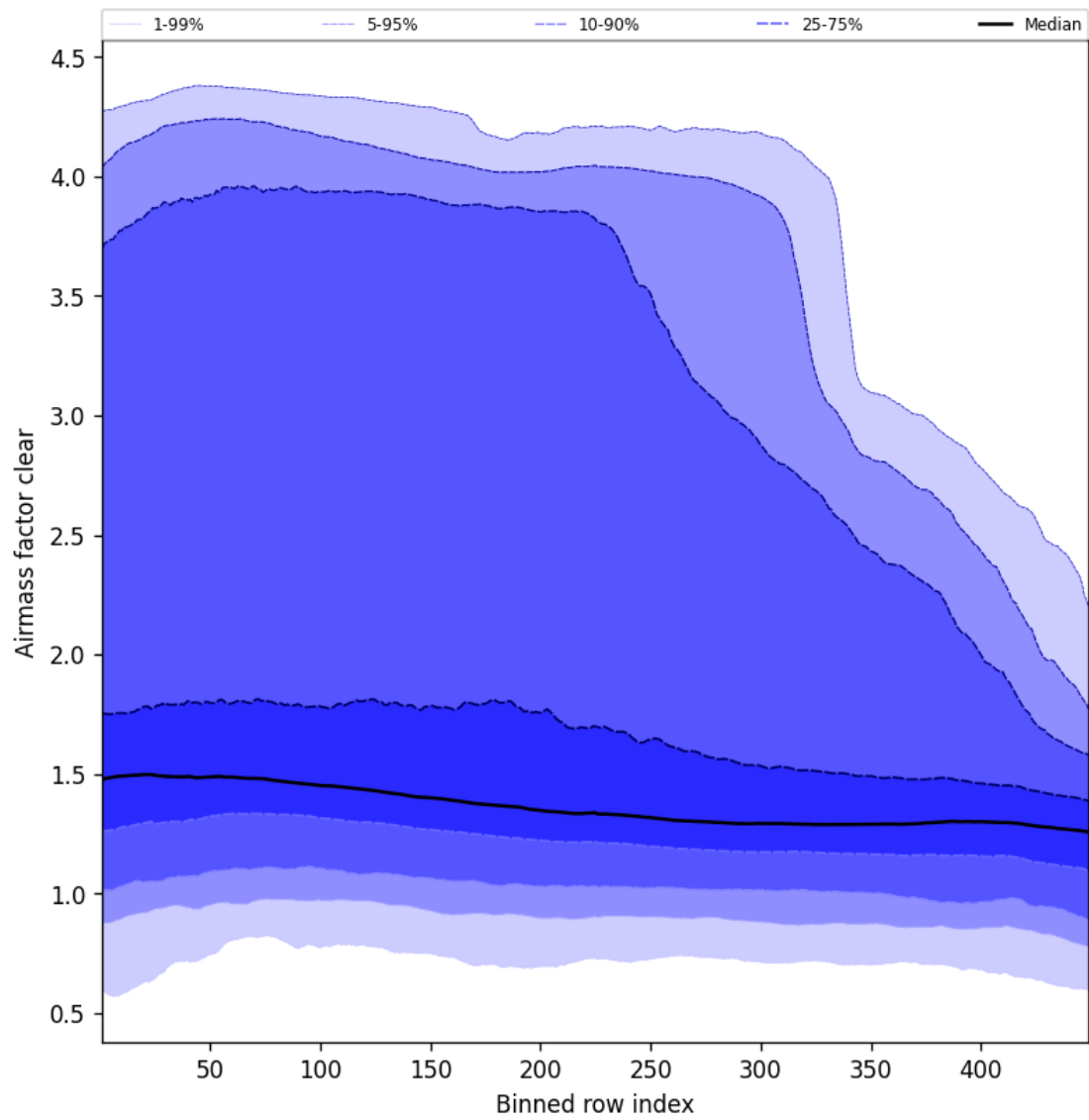
Figure 54: Along track statistics of “Air mass factor clear” for 2024-12-21 to 2024-12-22
