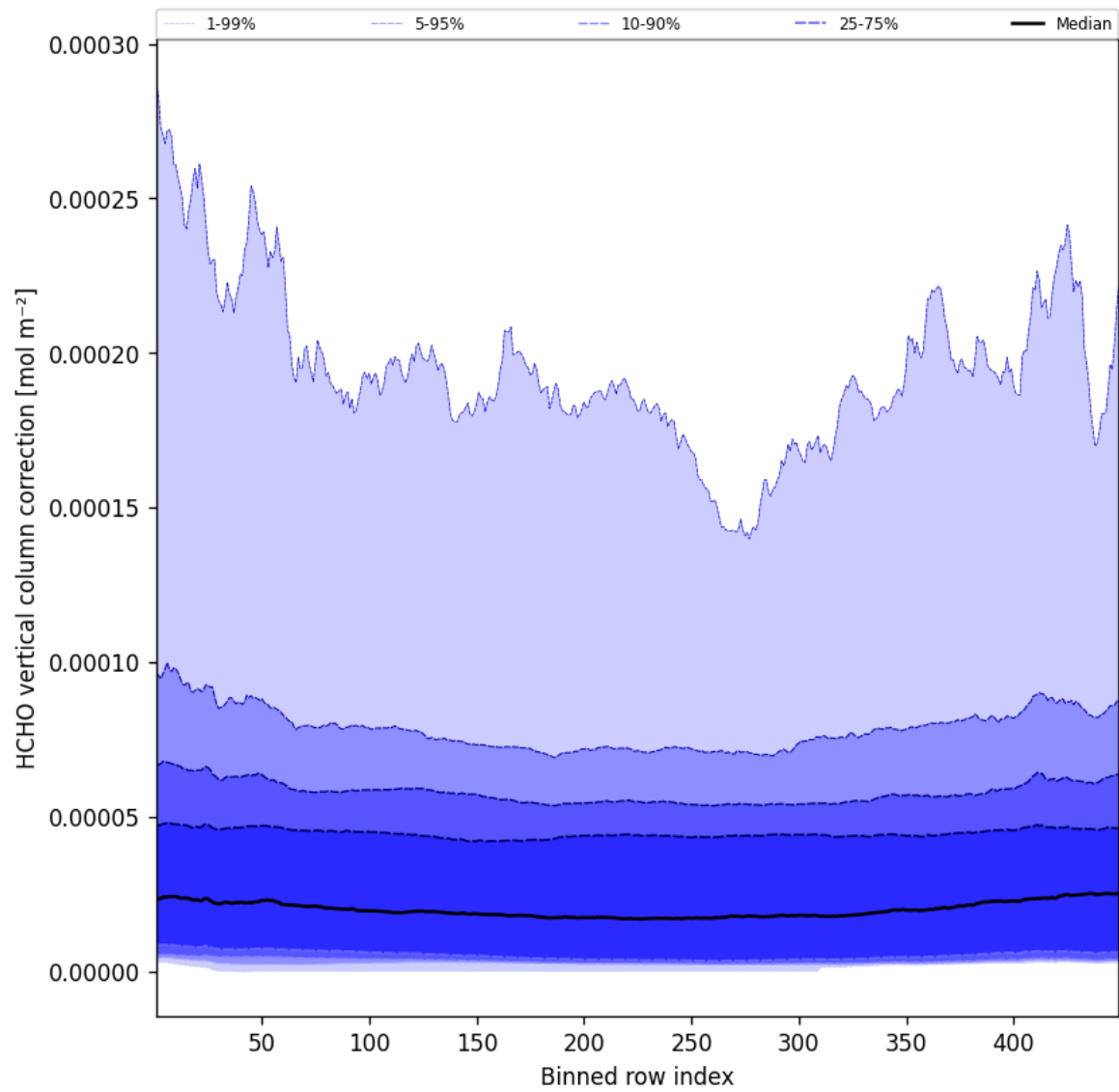
Figure 49: Along track statistics of “HCHO vertical column correction” for 2024-12-21 to 2024-12-22
