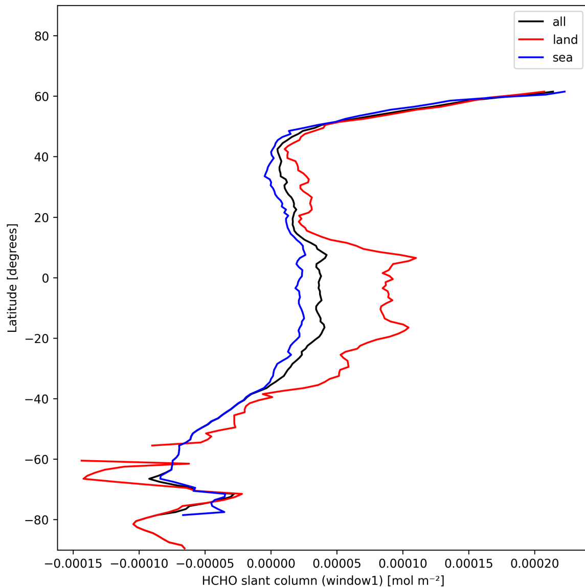
Figure 22: Zonal average of “HCHO slant column (window1)” for 2024-12-21 to 2024-12-22.
