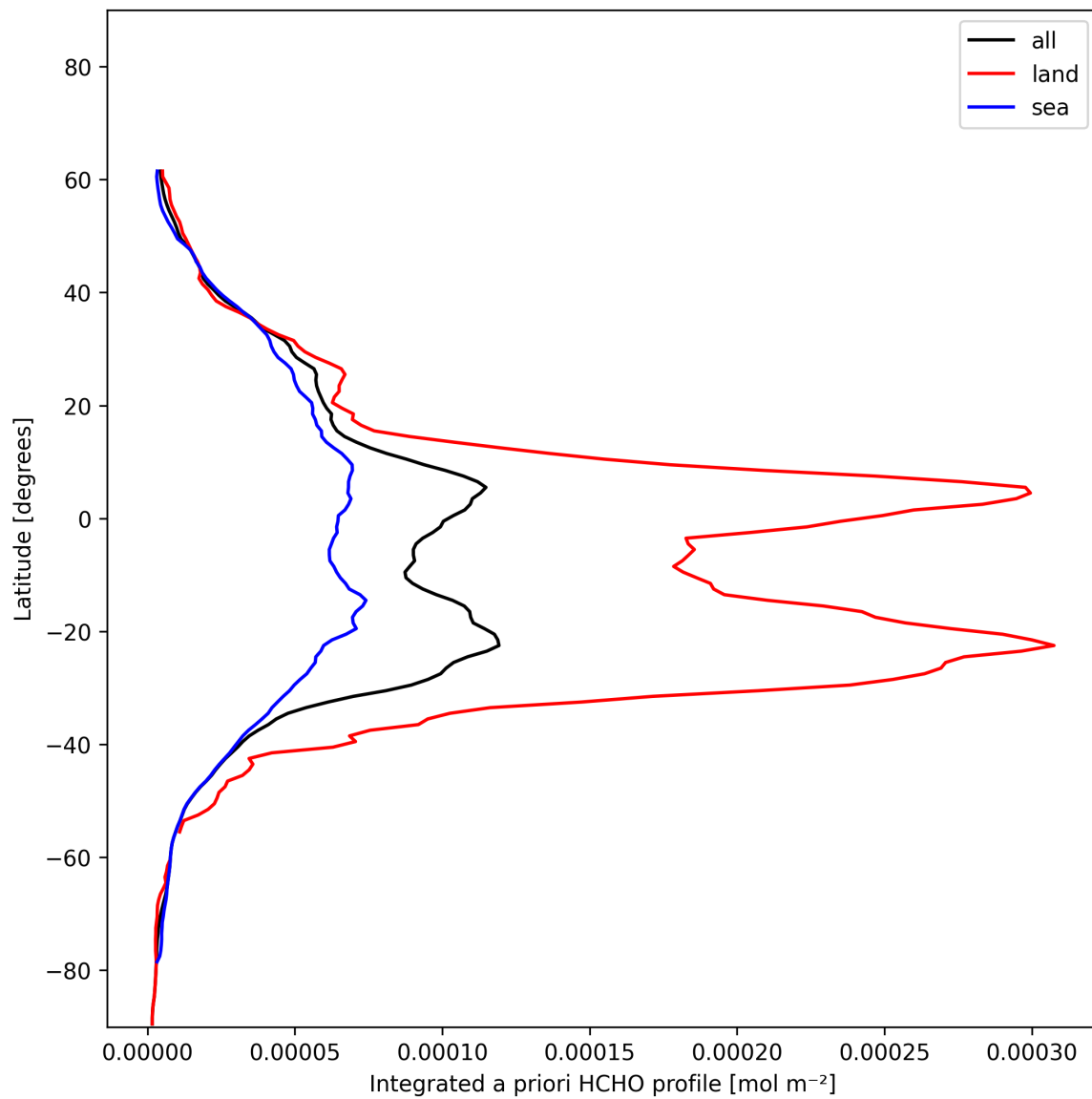
Figure 27: Zonal average of “Integrated a priori HCHO profile” for 2024-12-21 to 2024-12-22.
