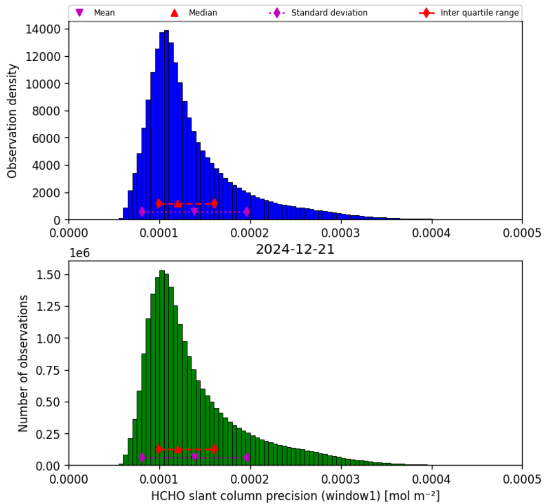
Figure 37: Histogram of “HCHO slant column precision (window1)” for 2024-12-21 to 2024-12-22
