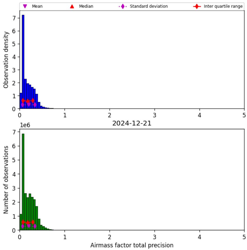
Figure 39: Histogram of “Airmass factor total precision” for 2024-12-21 to 2024-12-22
