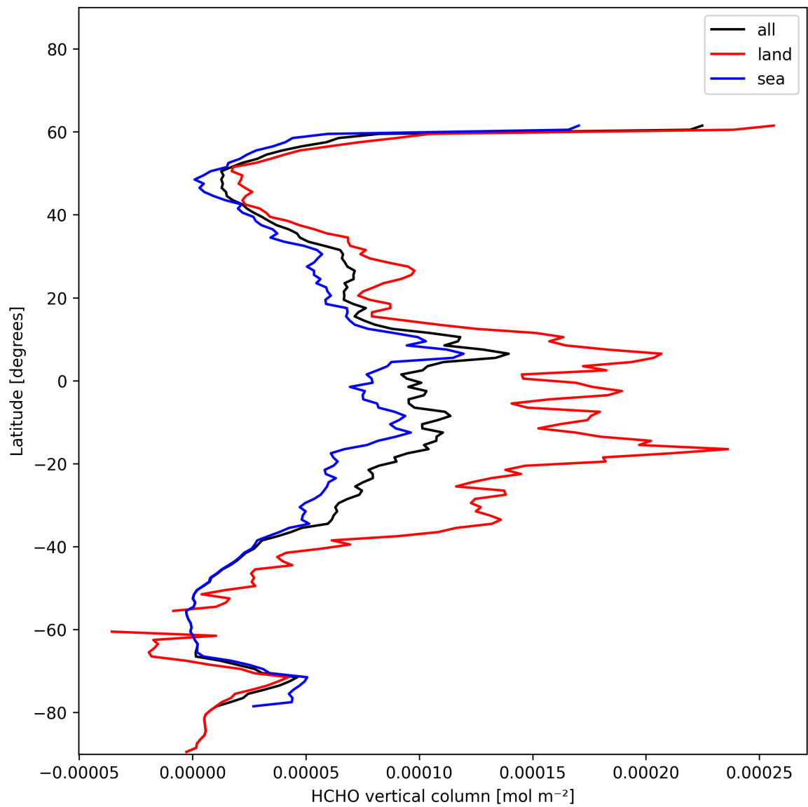
Figure 19: Zonal average of “HCHO vertical column” for 2024-12-21 to 2024-12-22.
