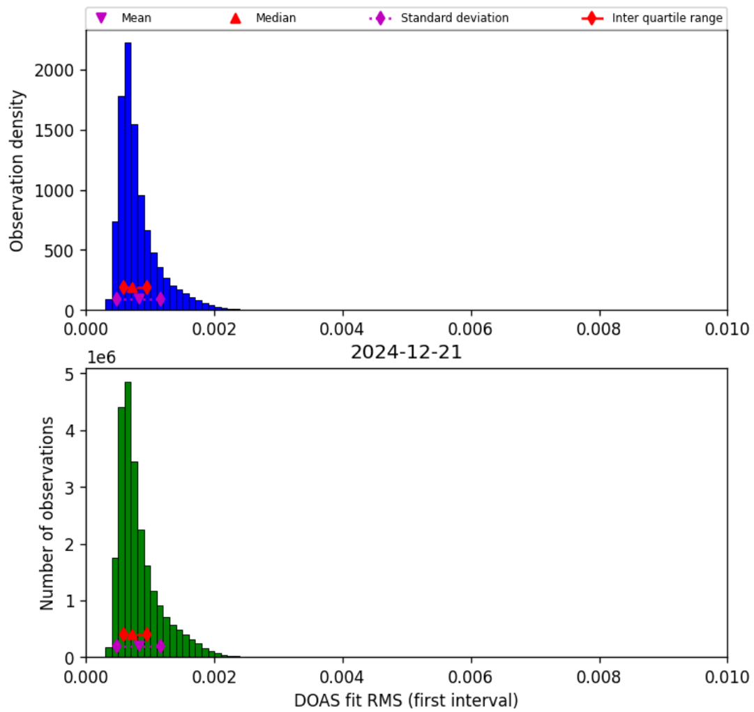
Figure 44: Histogram of “DOAS fit RMS (first interval)” for 2024-12-21 to 2024-12-22
