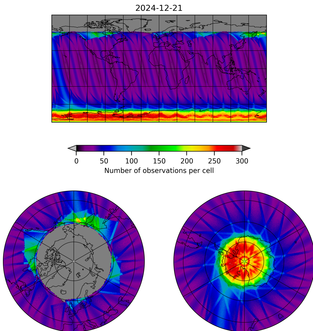
Figure 17: Map of the number of observations for 2024-12-21 to 2024-12-22
