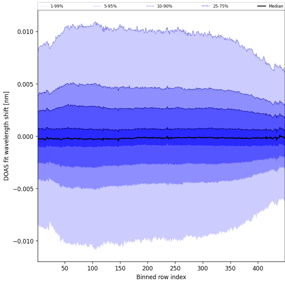
Figure 56: Along track statistics of “DOAS fit wavelength shift” for 2024-12-21 to 2024-12-22
