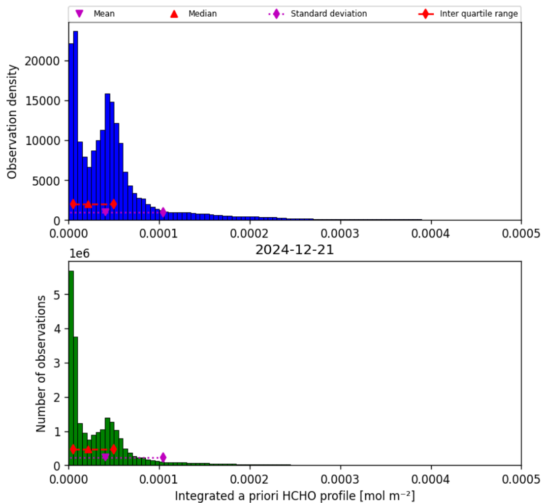
Figure 41: Histogram of “Integrated a priori HCHO profile” for 2024-12-21 to 2024-12-22
