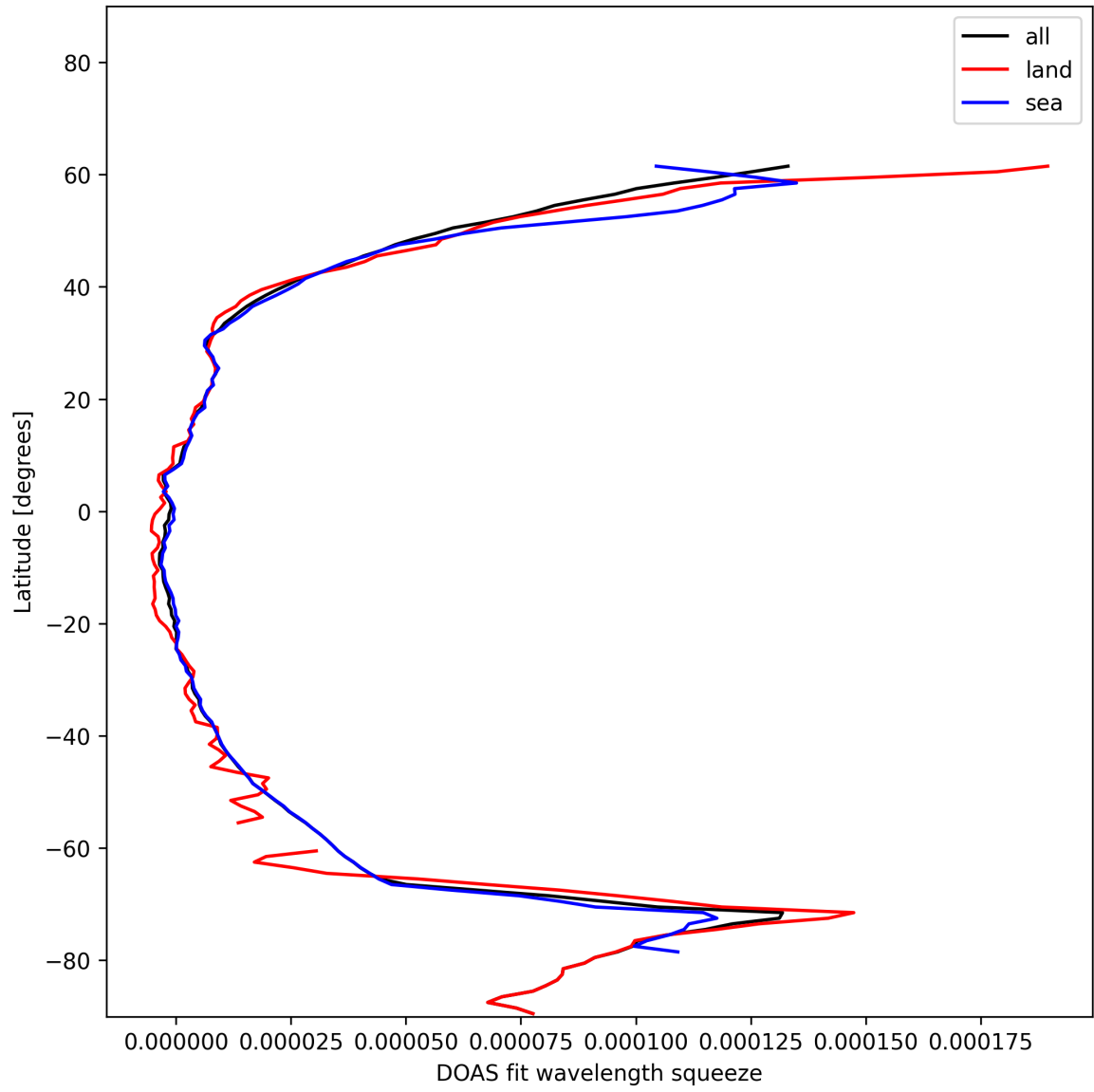
Figure 29: Zonal average of “DOAS fit wavelength squeeze” for 2024-12-21 to 2024-12-22.
