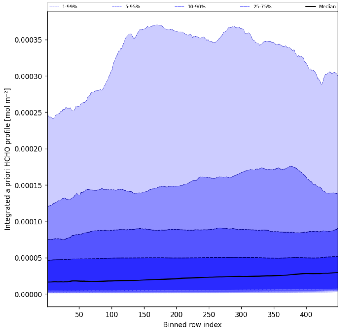
Figure 55: Along track statistics of "Integrated a priori HCHO profile" for 2024-12-21 to 2024-12-22
