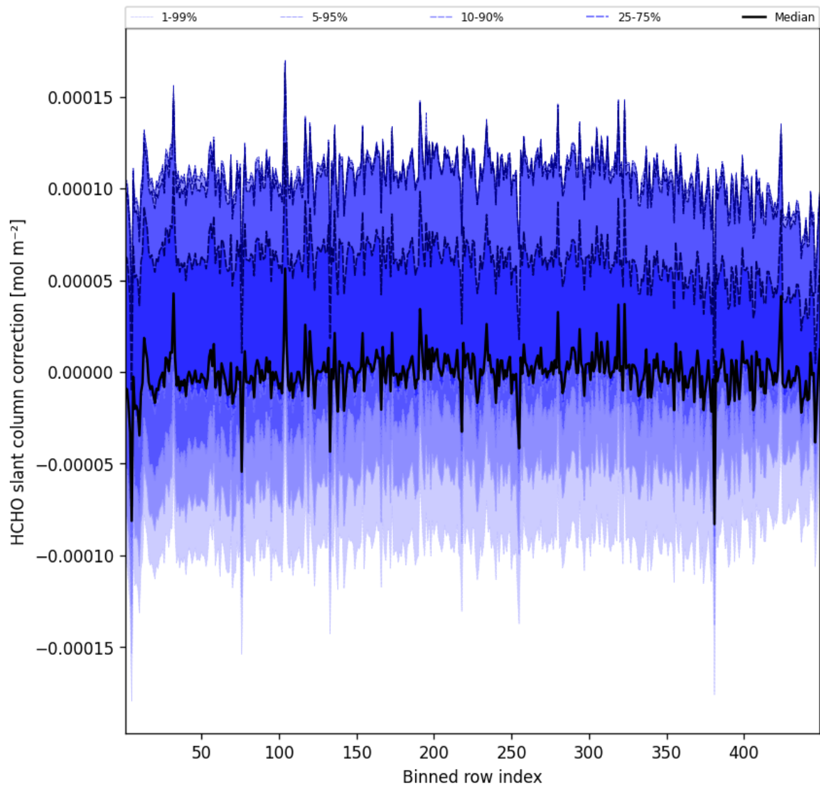
Figure 59: Along track statistics of “HCHO slant column correction” for 2024-12-21 to 2024-12-22
