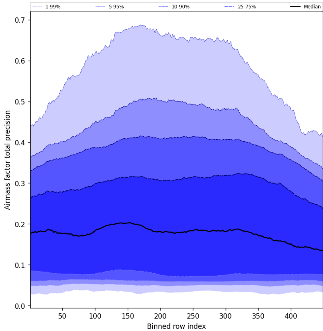
Figure 53: Along track statistics of “Airmass factor total precision” for 2024-12-21 to 2024-12-22
