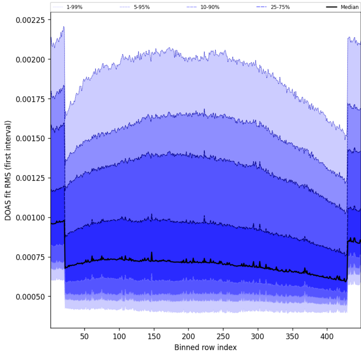
Figure 58: Along track statistics of “DOAS fit RMS (first interval)” for 2024-12-21 to 2024-12-22
