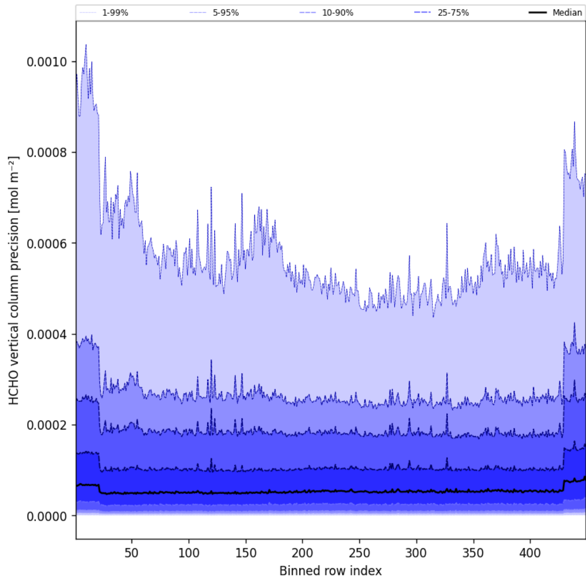
Figure 48: Along track statistics of “HCHO vertical column precision” for 2024-12-21 to 2024-12-22
