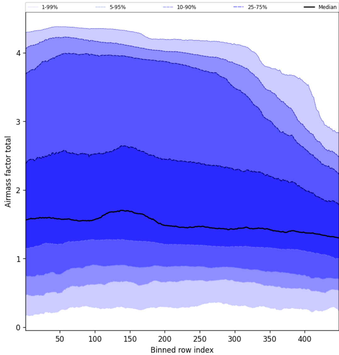
Figure 52: Along track statistics of “Airmass factor total” for 2024-12-21 to 2024-12-22
