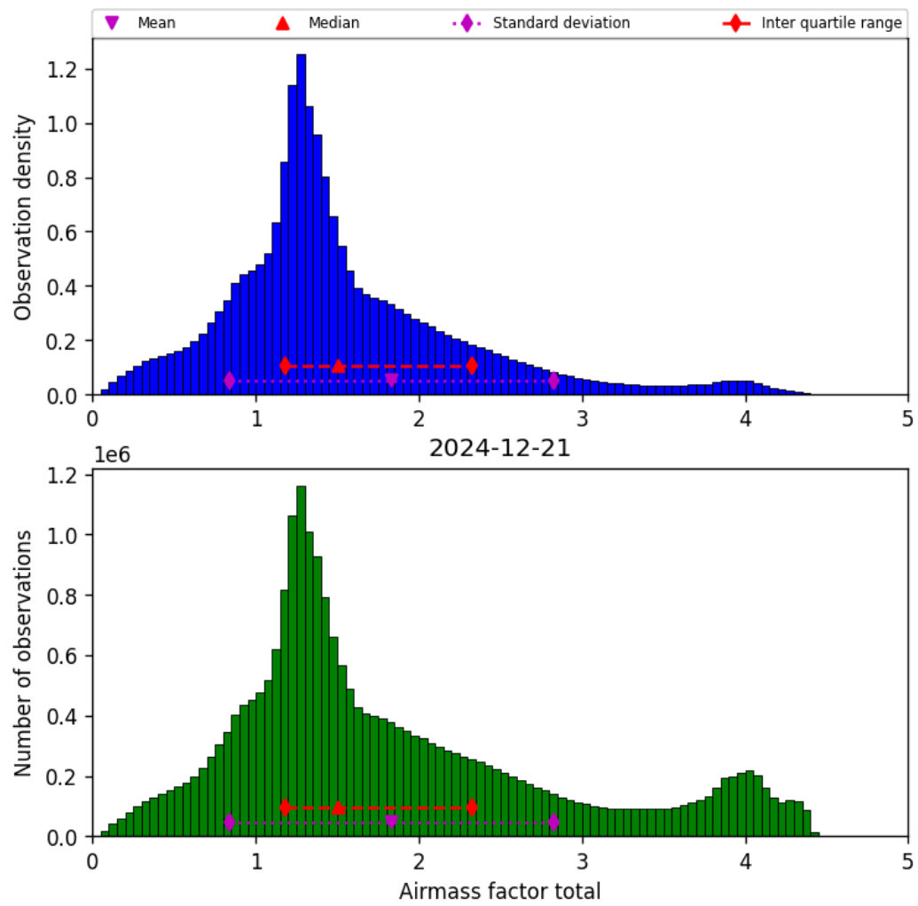
Figure 38: Histogram of “Airmass factor total” for 2024-12-21 to 2024-12-22
