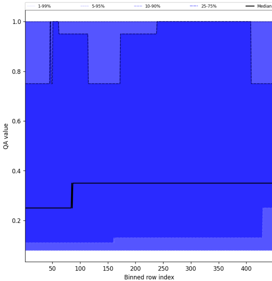
Figure 46: Along track statistics of “QA value” for 2024-12-21 to 2024-12-22
