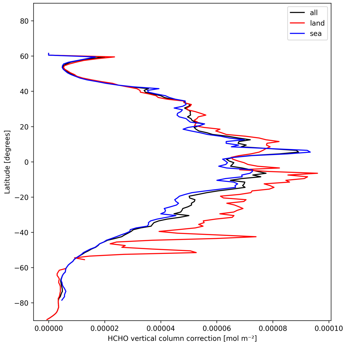
Figure 21: Zonal average of “HCHO vertical column correction” for 2024-12-22 to 2024-12-23.
