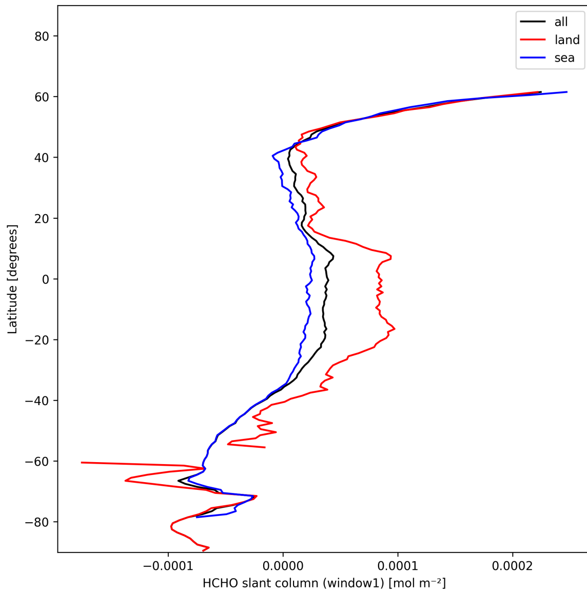
Figure 22: Zonal average of “HCHO slant column (window1)” for 2024-12-22 to 2024-12-23.
