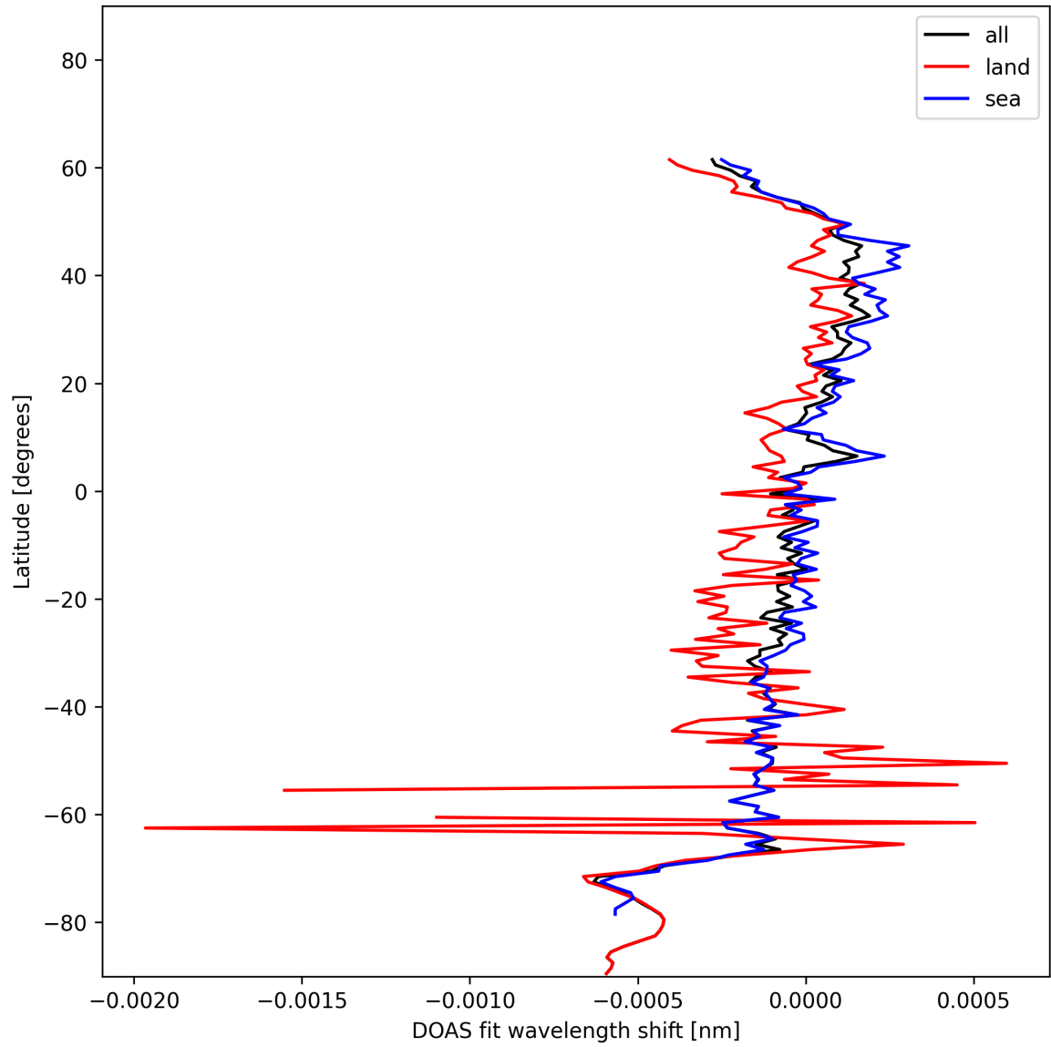
Figure 28: Zonal average of "DOAS fit wavelength shift" for 2024-12-22 to 2024-12-23.
