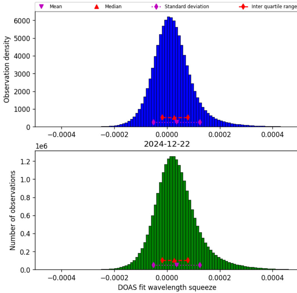
Figure 43: Histogram of “DOAS fit wavelength squeeze” for 2024-12-22 to 2024-12-23
