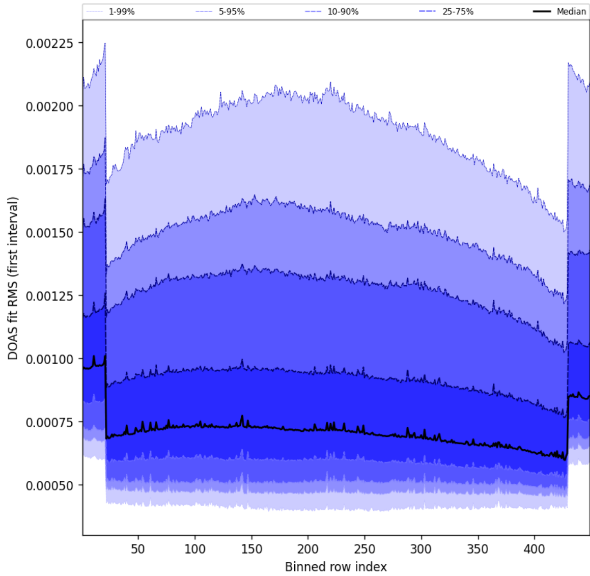
Figure 58: Along track statistics of “DOAS fit RMS (first interval)” for 2024-12-22 to 2024-12-23
