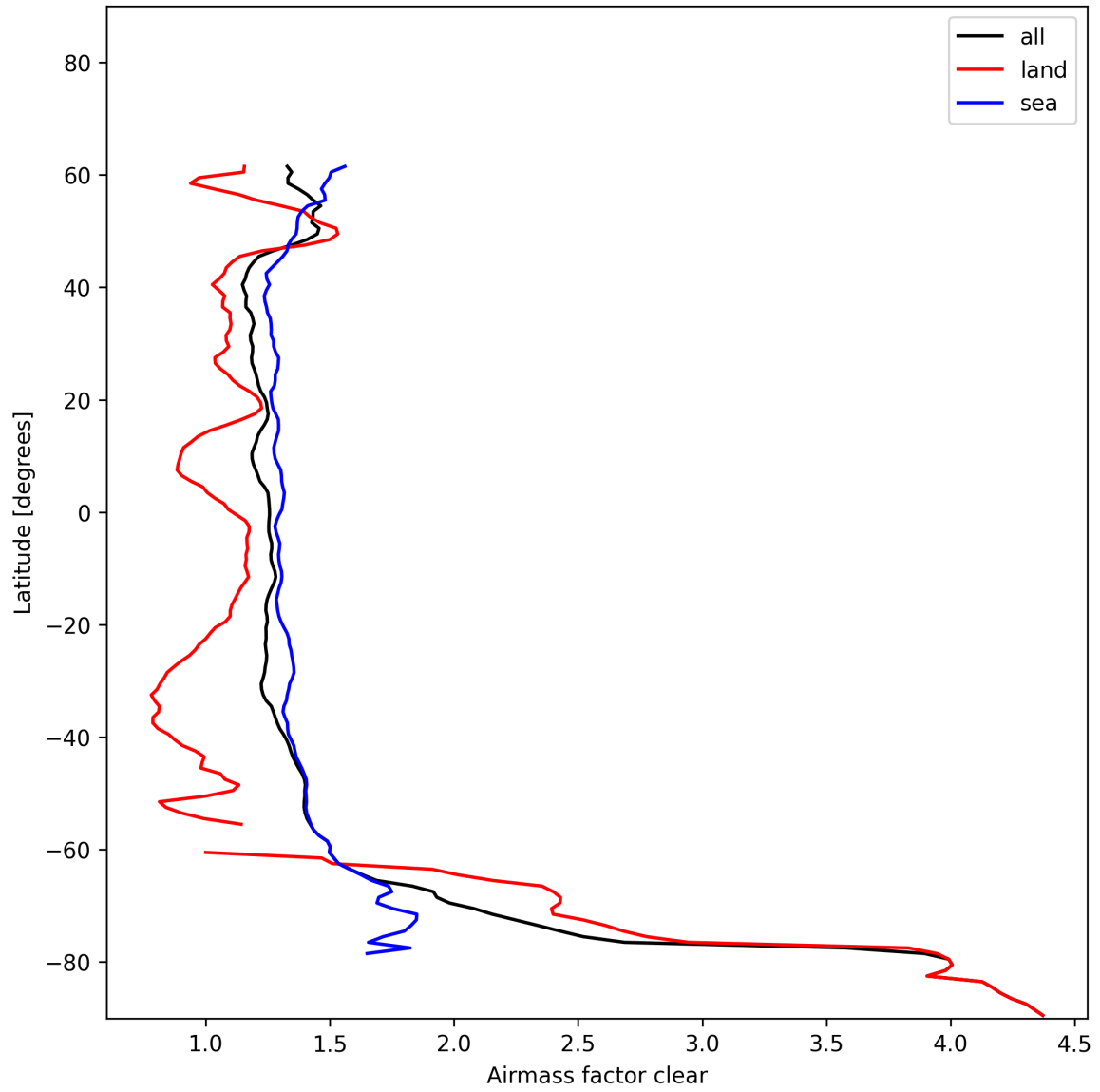
Figure 26: Zonal average of “Airmass factor clear” for 2024-12-22 to 2024-12-23.
