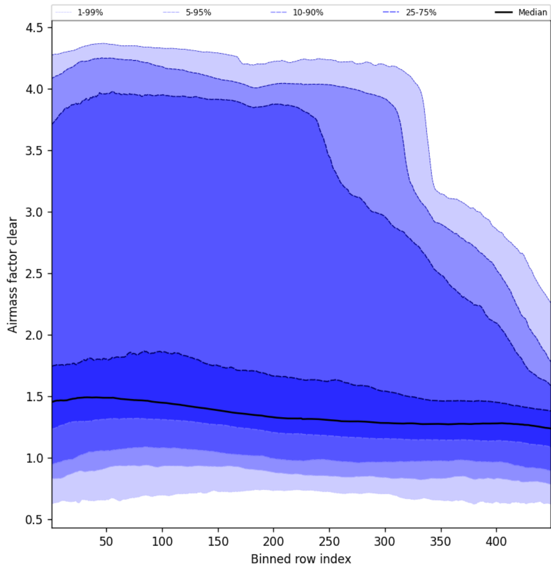
Figure 54: Along track statistics of “Air mass factor clear” for 2024-12-22 to 2024-12-23
