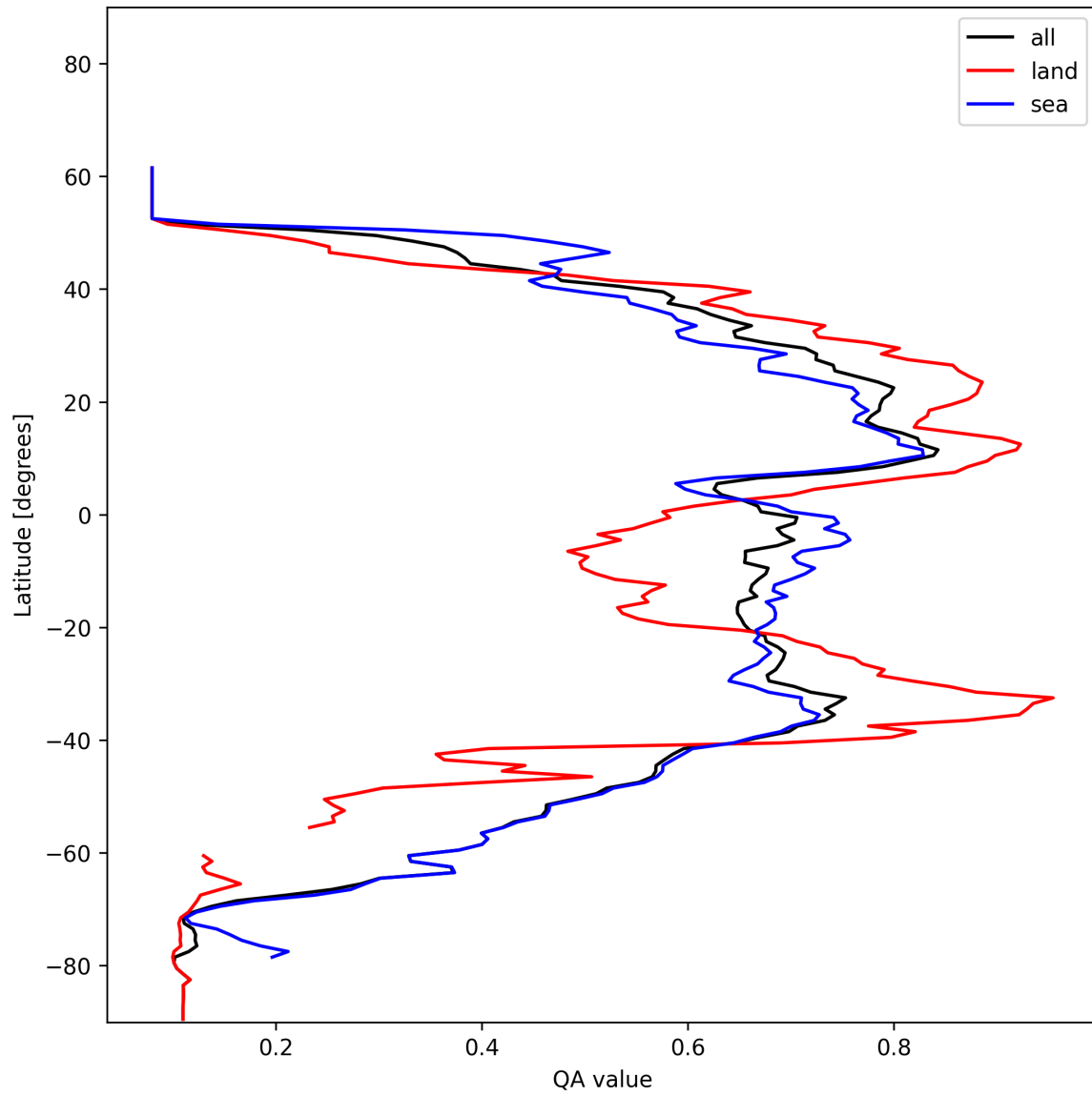
Figure 18: Zonal average of “QA value” for 2024-12-22 to 2024-12-23.
