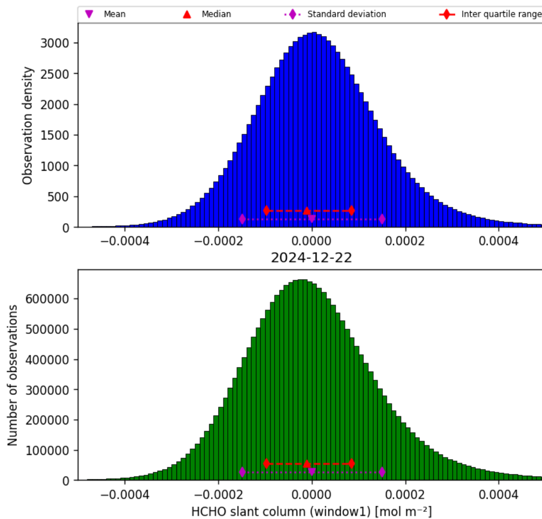
Figure 36: Histogram of “HCHO slant column (window1)” for 2024-12-22 to 2024-12-23
