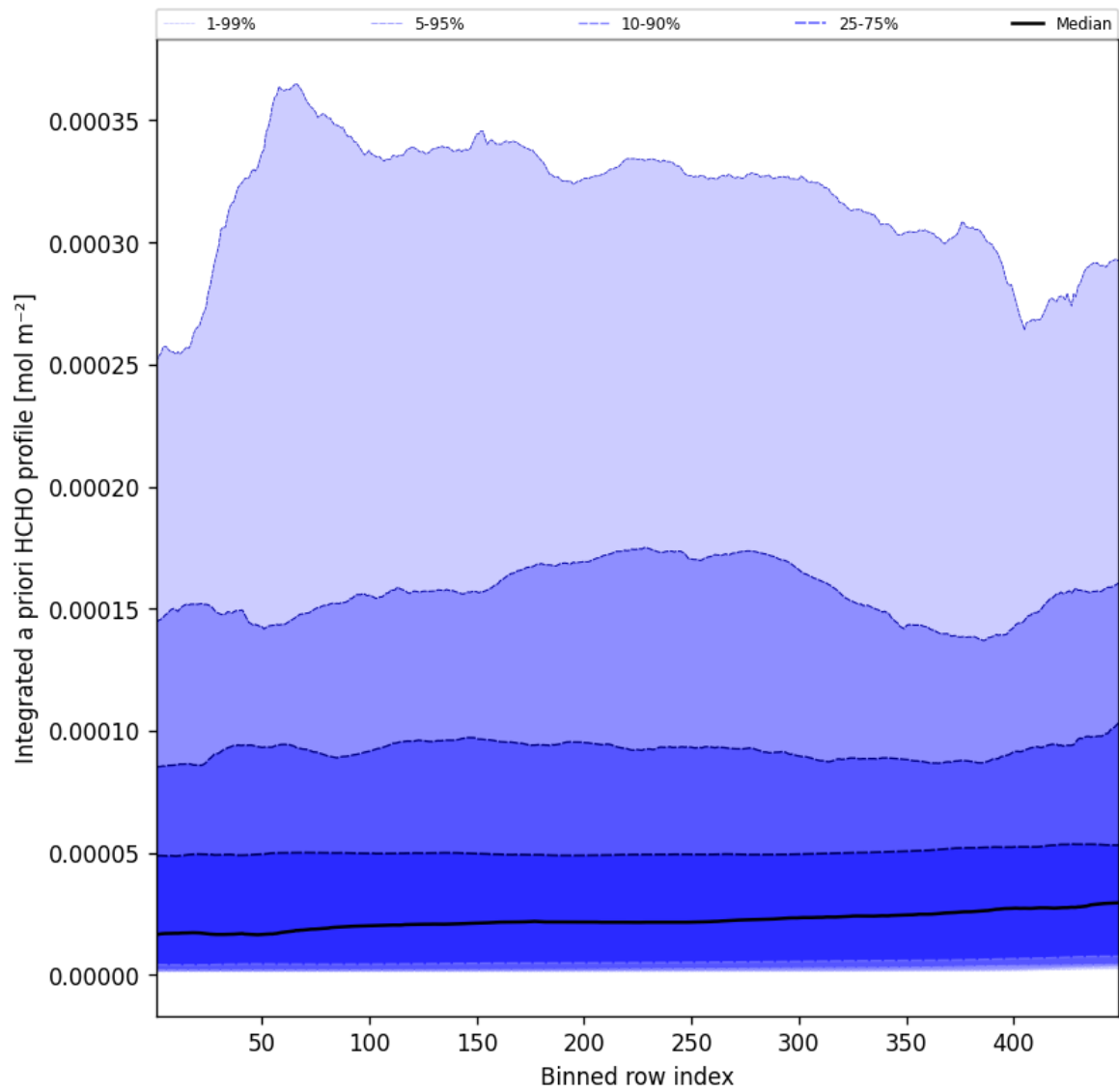
Figure 55: Along track statistics of “Integrated a priori HCHO profile” for 2024-12-22 to 2024-12-23
