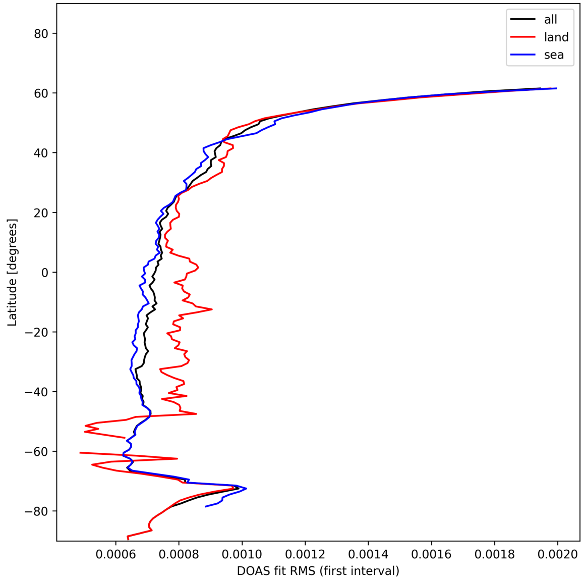
Figure 30: Zonal average of “DOAS fit RMS (first interval)” for 2024-12-22 to 2024-12-23.
