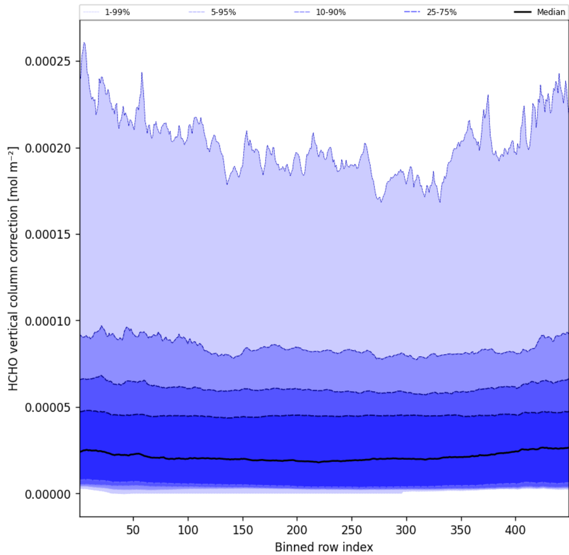
Figure 49: Along track statistics of “HCHO vertical column correction” for 2024-12-22 to 2024-12-23
