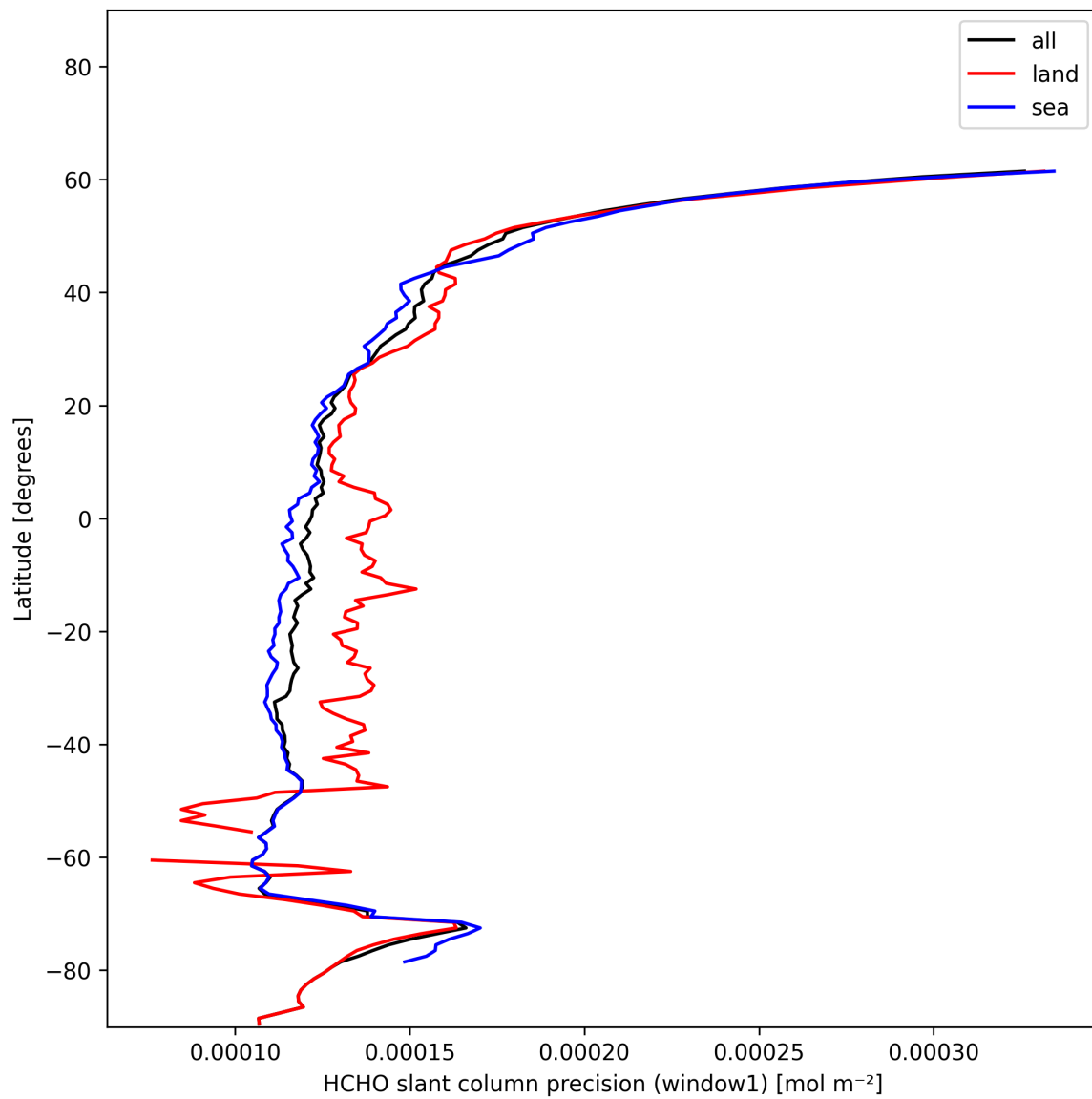
Figure 23: Zonal average of “HCHO slant column precision (window1)” for 2024-12-22 to 2024-12-23.
