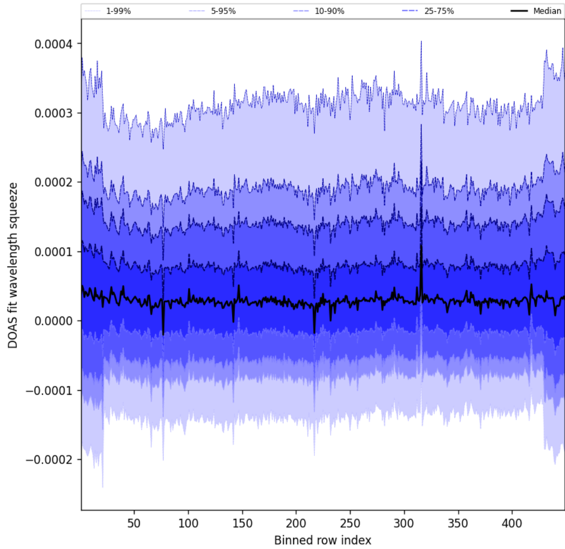
Figure 57: Along track statistics of “DOAS fit wavelength squeeze” for 2024-12-22 to 2024-12-23
