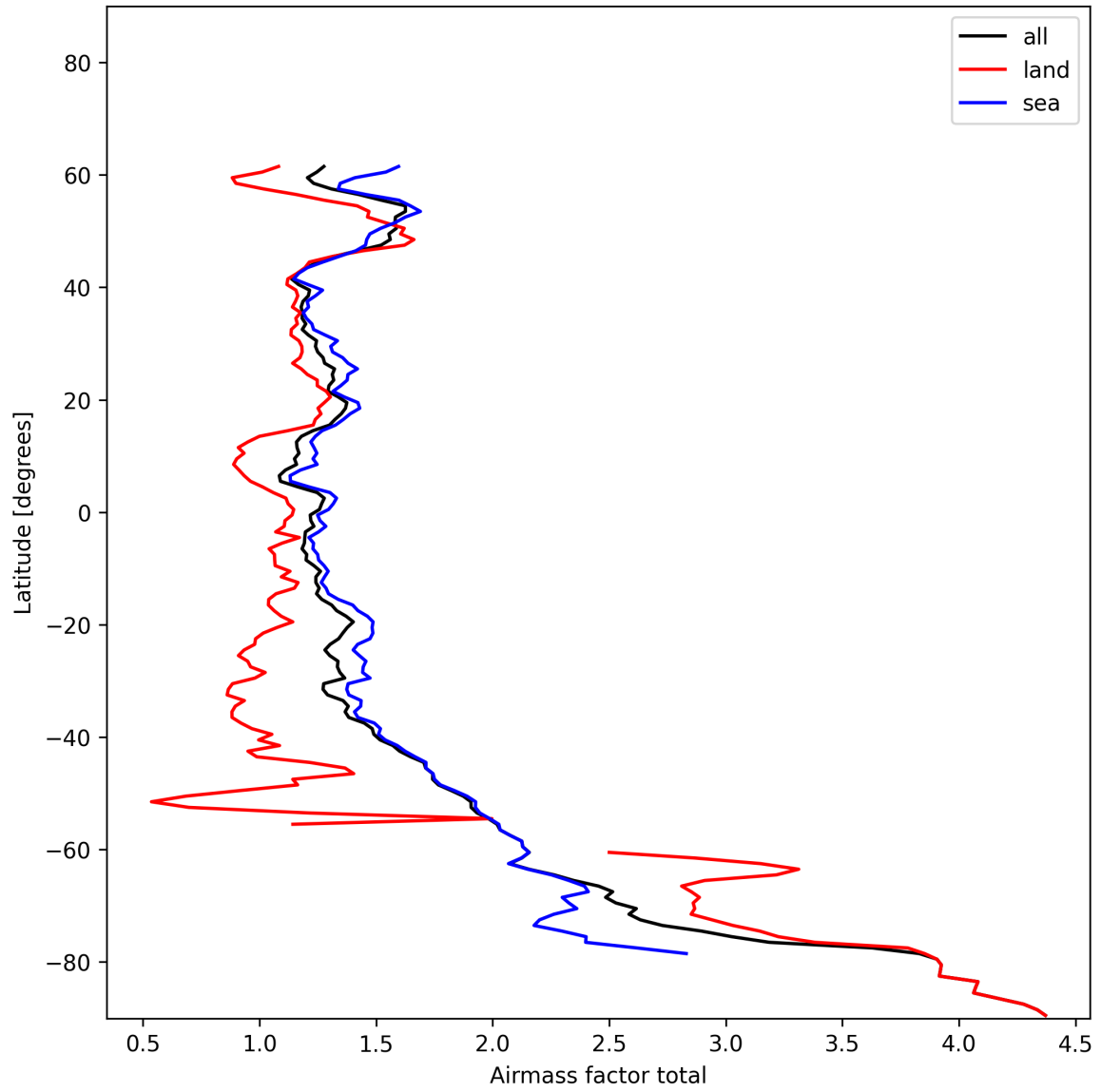
Figure 24: Zonal average of “Airmass factor total” for 2024-12-22 to 2024-12-23.
