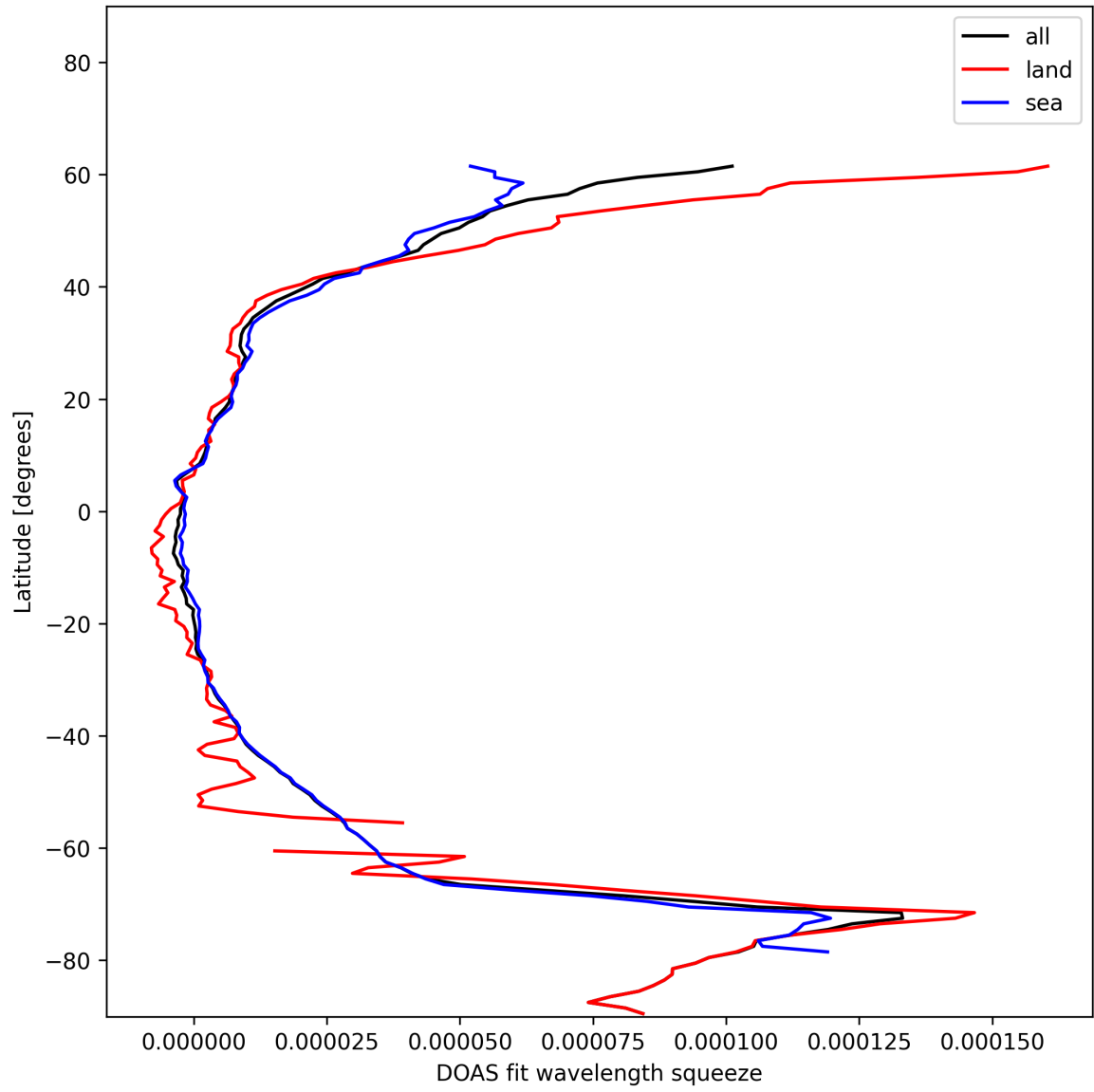
Figure 29: Zonal average of “DOAS fit wavelength squeeze” for 2024-12-22 to 2024-12-23.
