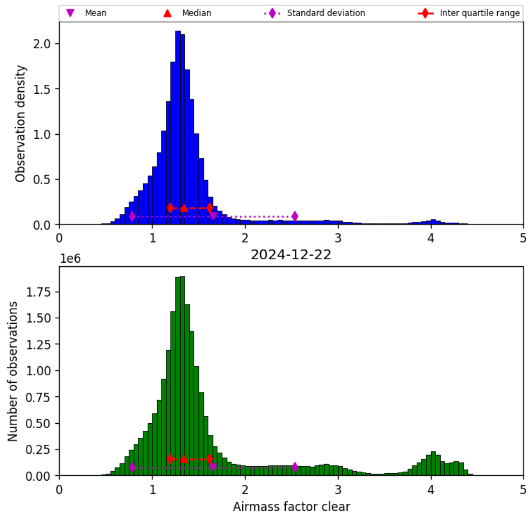
Figure 40: Histogram of “Airmass factor clear” for 2024-12-22 to 2024-12-23
