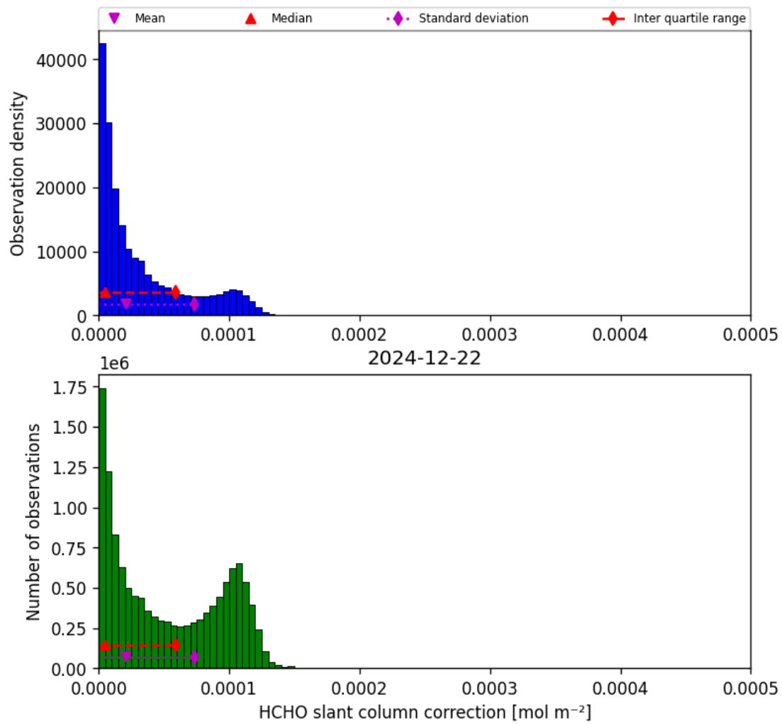
Figure 45: Histogram of “HCHO slant column correction” for 2024-12-22 to 2024-12-23
