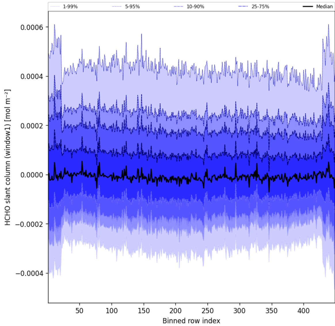
Figure 50: Along track statistics of “HCHO slant column (window1)” for 2024-12-22 to 2024-12-23
