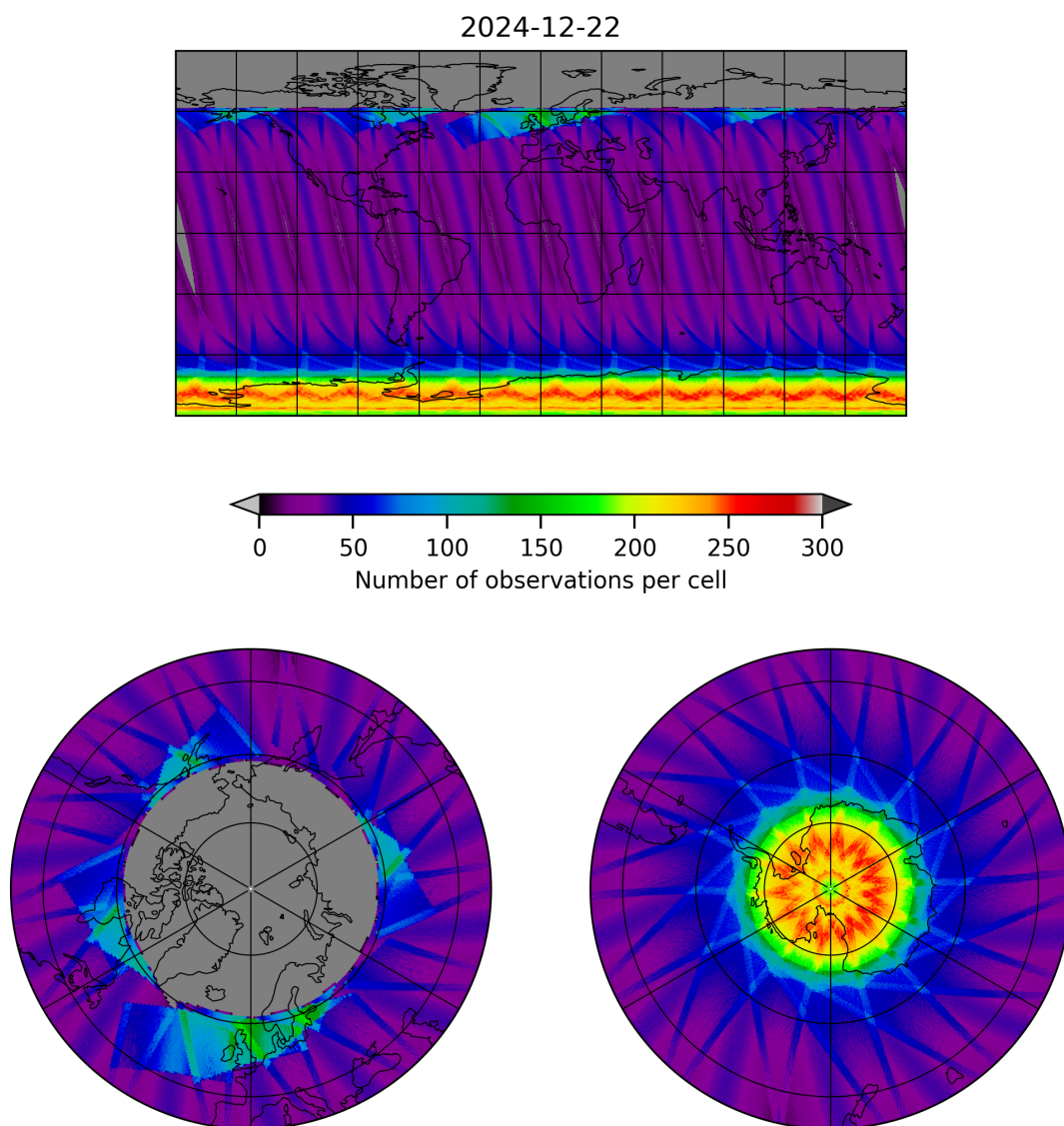
Figure 17: Map of the number of observations for 2024-12-22 to 2024-12-23
