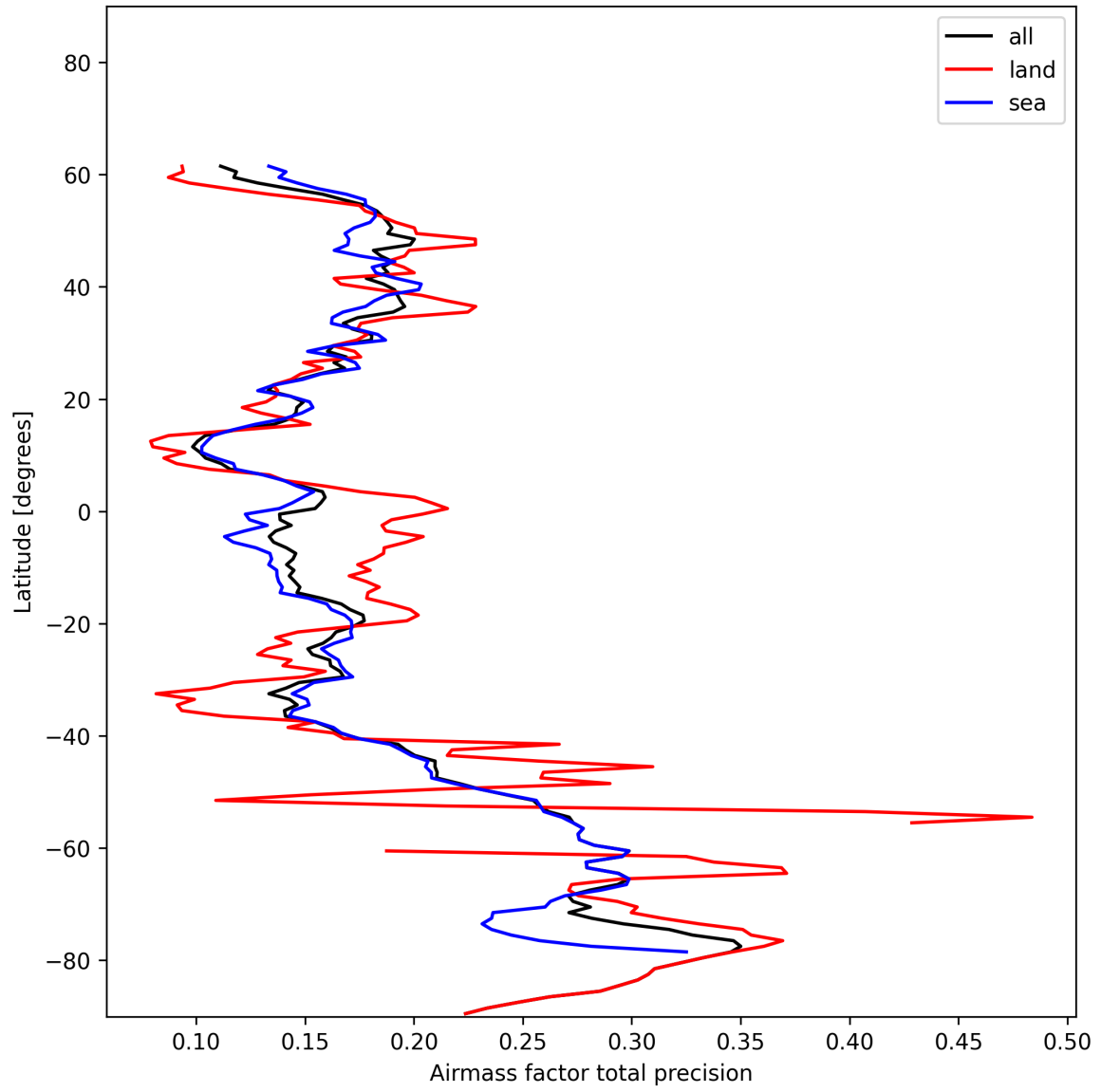
Figure 25: Zonal average of “Airmass factor total precision” for 2024-12-22 to 2024-12-23.
