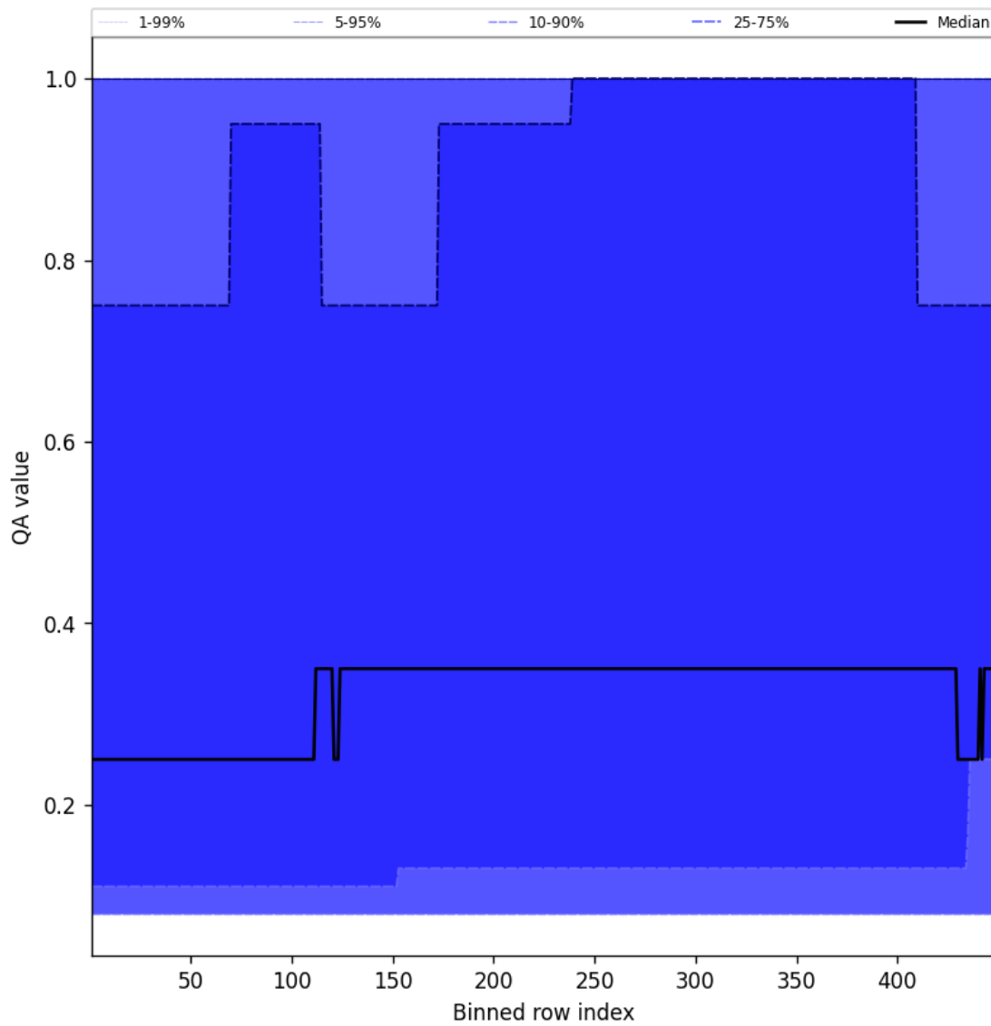
Figure 46: Along track statistics of “QA value” for 2024-12-22 to 2024-12-23
