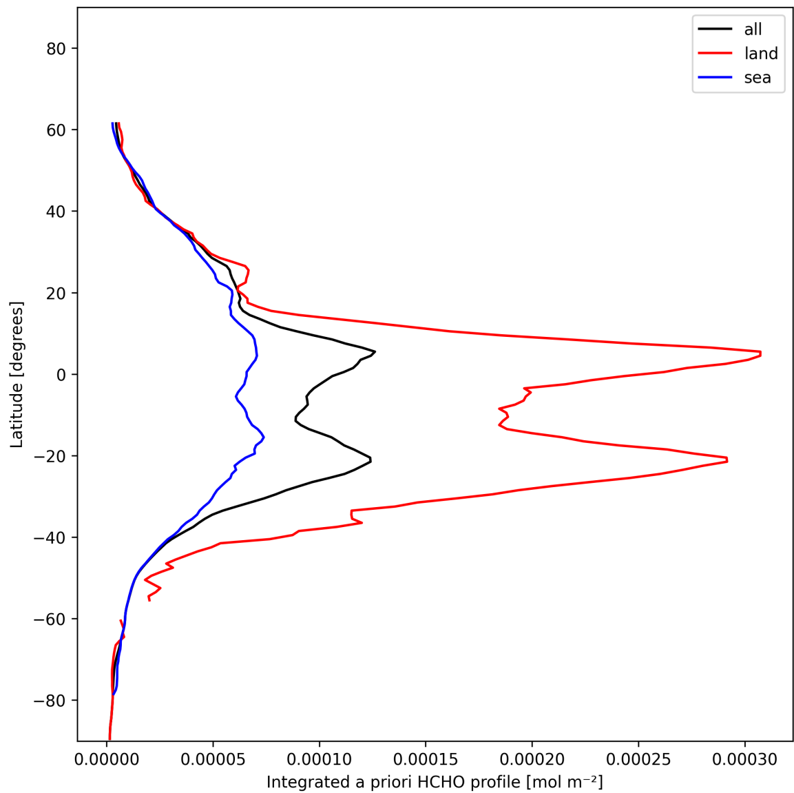
Figure 27: Zonal average of “Integrated a priori HCHO profile” for 2024-12-22 to 2024-12-23.
