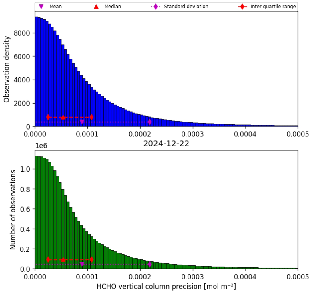
Figure 34: Histogram of “HCHO vertical column precision” for 2024-12-22 to 2024-12-23
