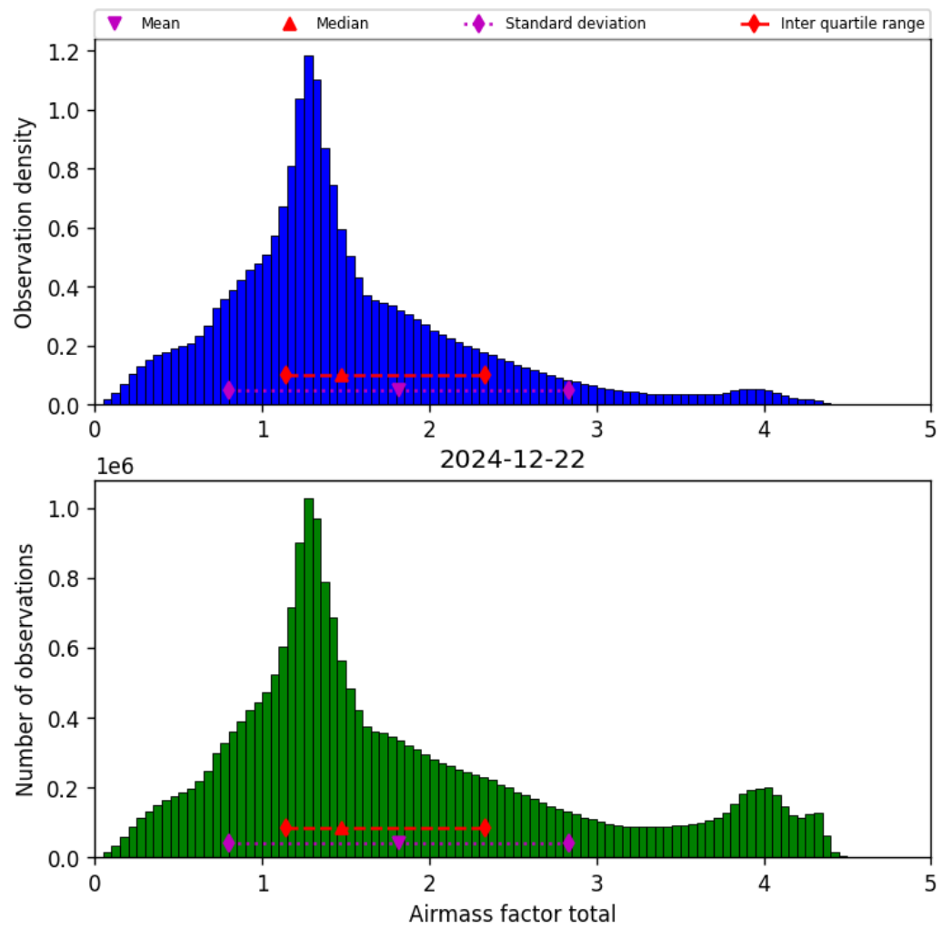
Figure 38: Histogram of “Airmass factor total” for 2024-12-22 to 2024-12-23
