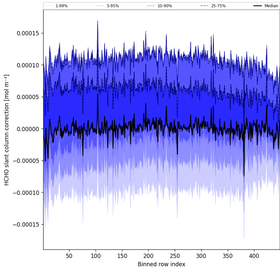
Figure 59: Along track statistics of “HCHO slant column correction” for 2024-12-22 to 2024-12-23
