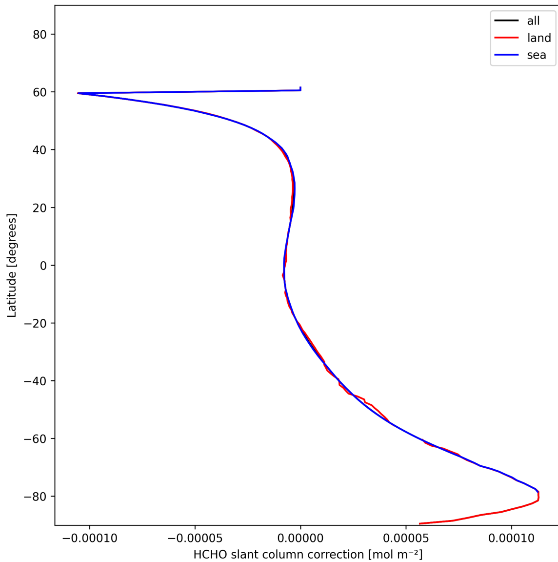
Figure 31: Zonal average of “HCHO slant column correction” for 2024-12-22 to 2024-12-23.
