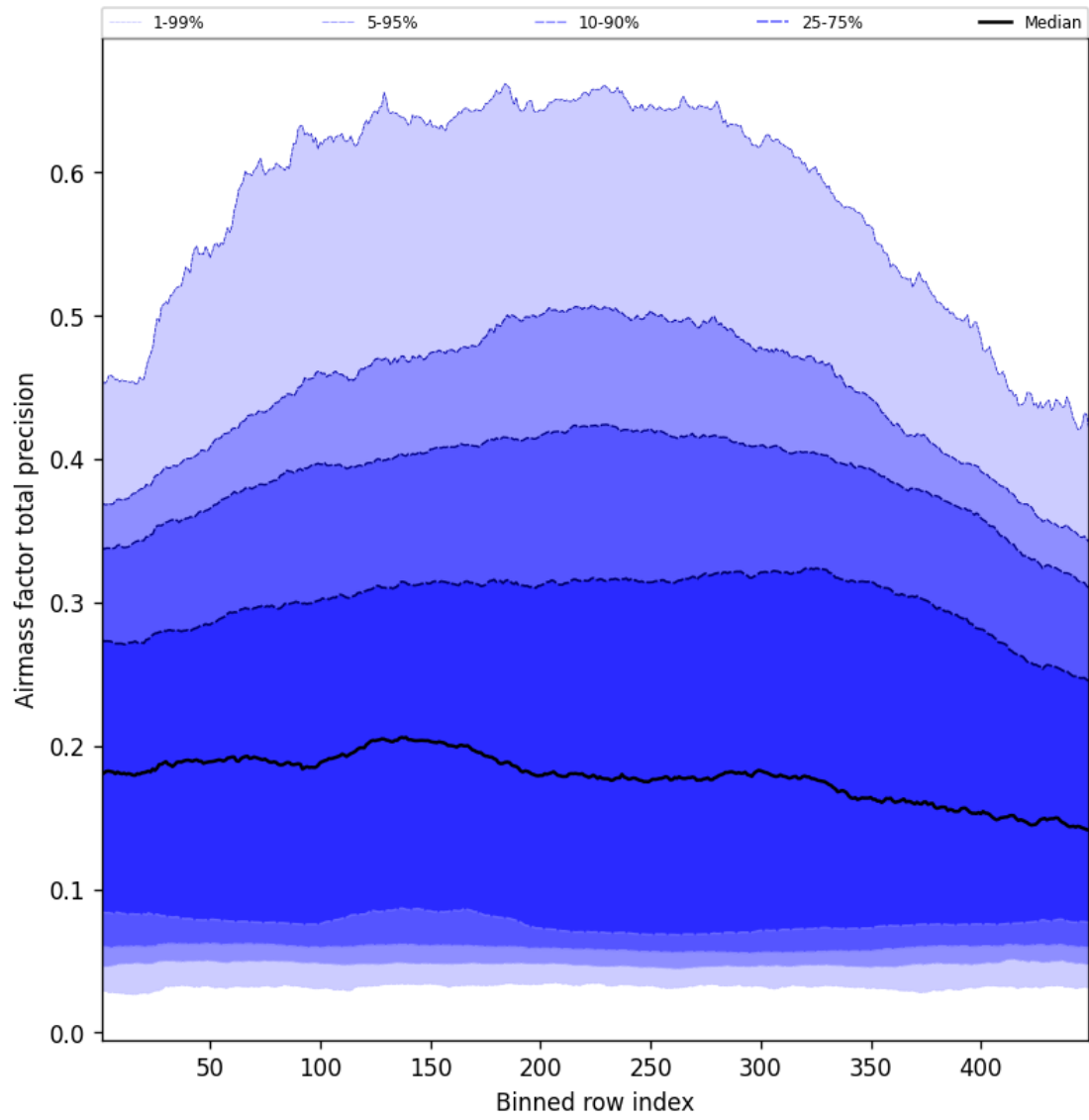
Figure 53: Along track statistics of “Airmass factor total precision” for 2024-12-22 to 2024-12-23
