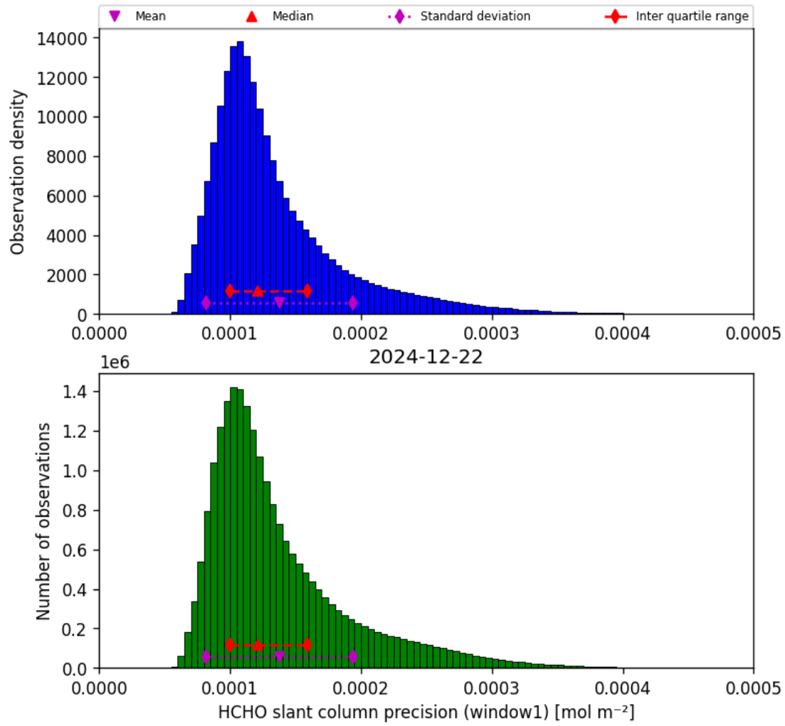
Figure 37: Histogram of “HCHO slant column precision (window1)” for 2024-12-22 to 2024-12-23
