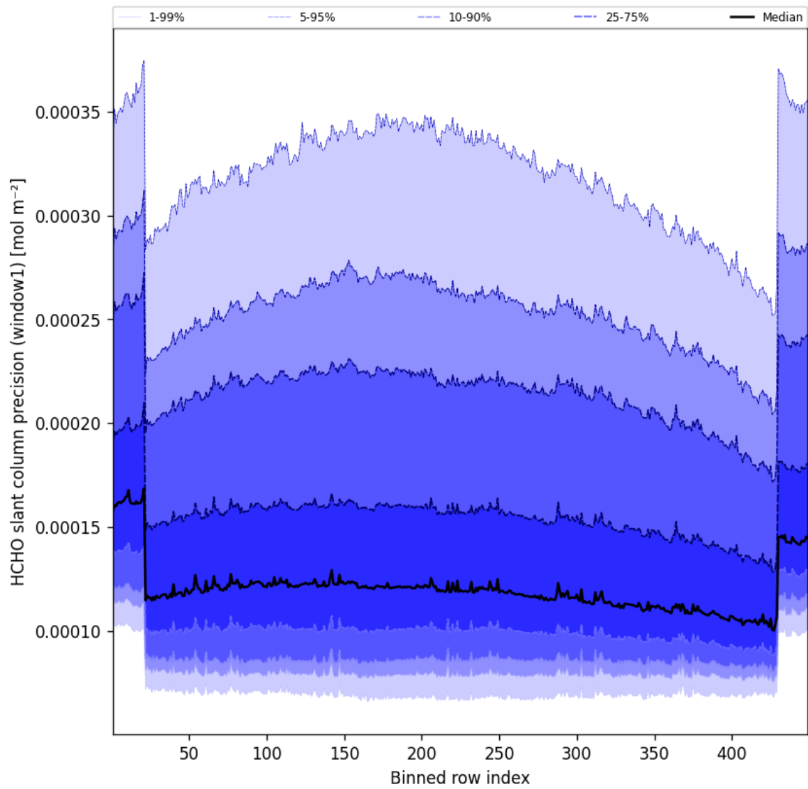
Figure 51: Along track statistics of "HCHO slant column precision (window1)" for 2024-12-22 to 2024-12-23
