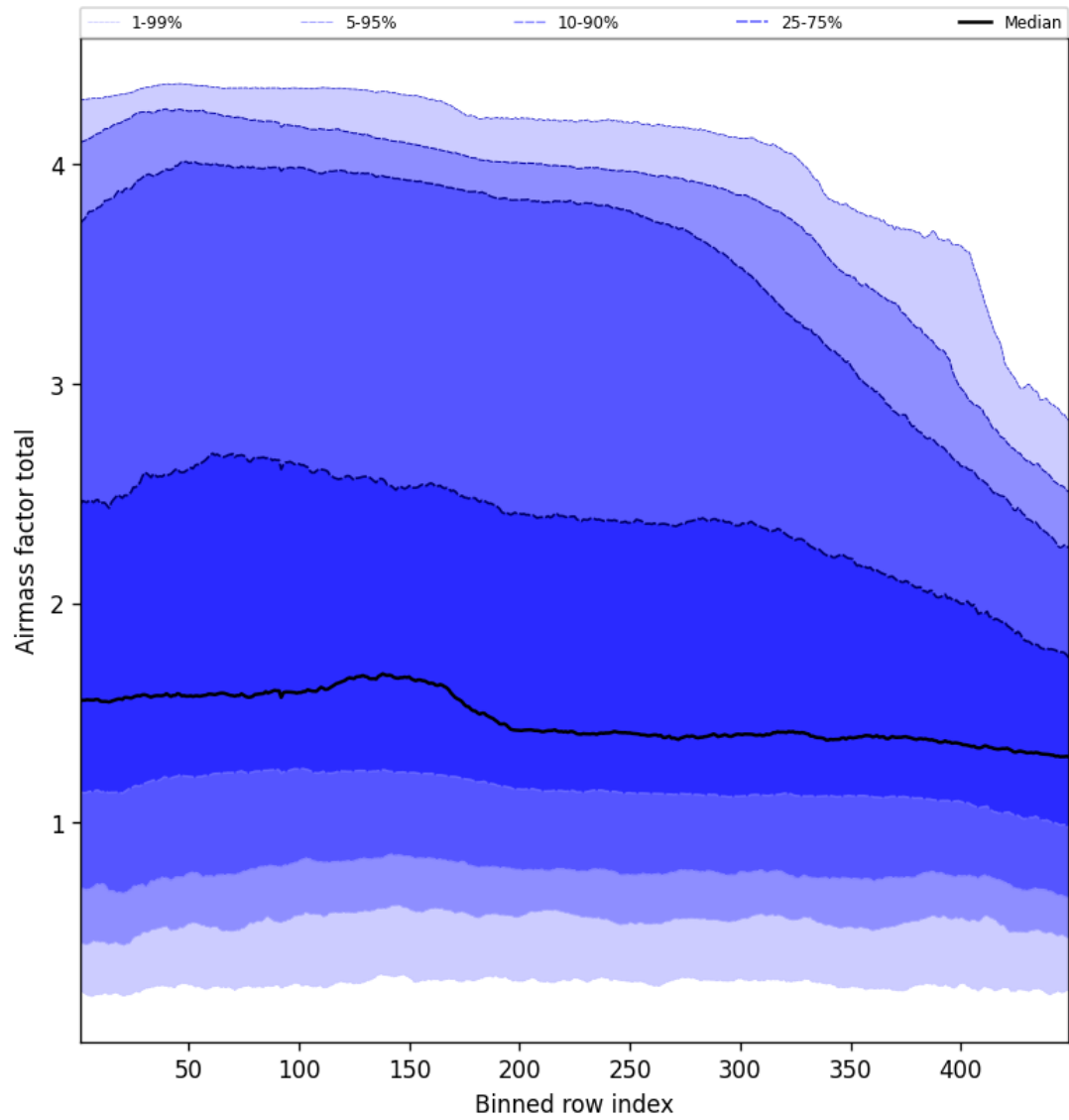
Figure 52: Along track statistics of “Airmass factor total” for 2024-12-22 to 2024-12-23
