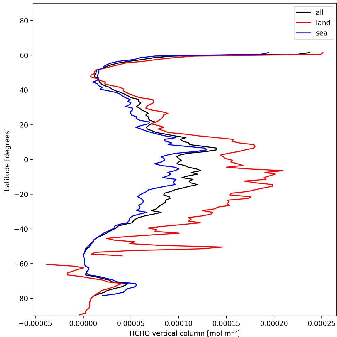
Figure 19: Zonal average of “HCHO vertical column” for 2024-12-22 to 2024-12-23.
