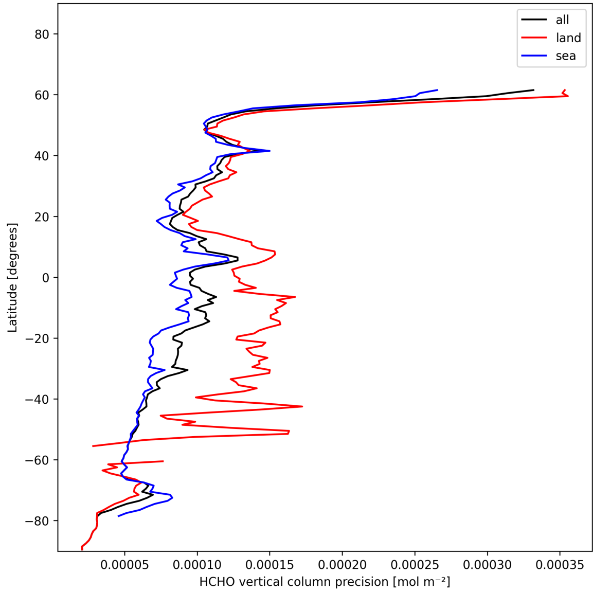
Figure 20: Zonal average of “HCHO vertical column precision” for 2024-12-22 to 2024-12-23.
