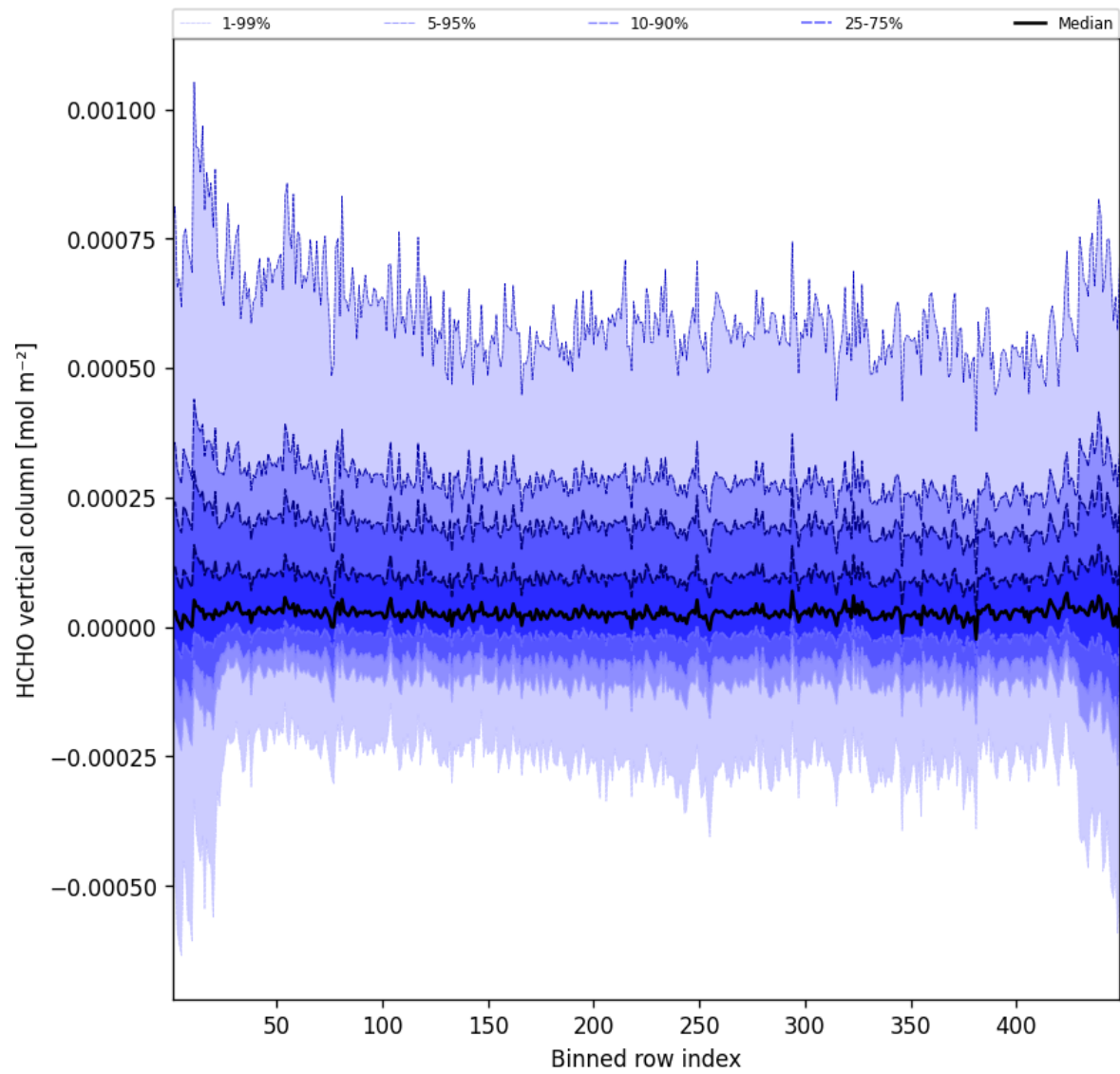
Figure 47: Along track statistics of “HCHO vertical column” for 2024-12-22 to 2024-12-23
