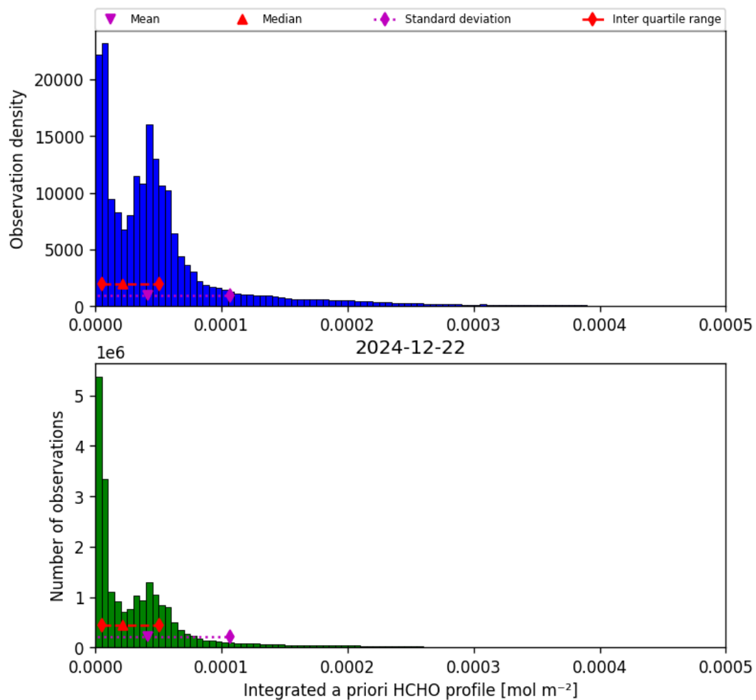
Figure 41: Histogram of “Integrated a priori HCHO profile” for 2024-12-22 to 2024-12-23
