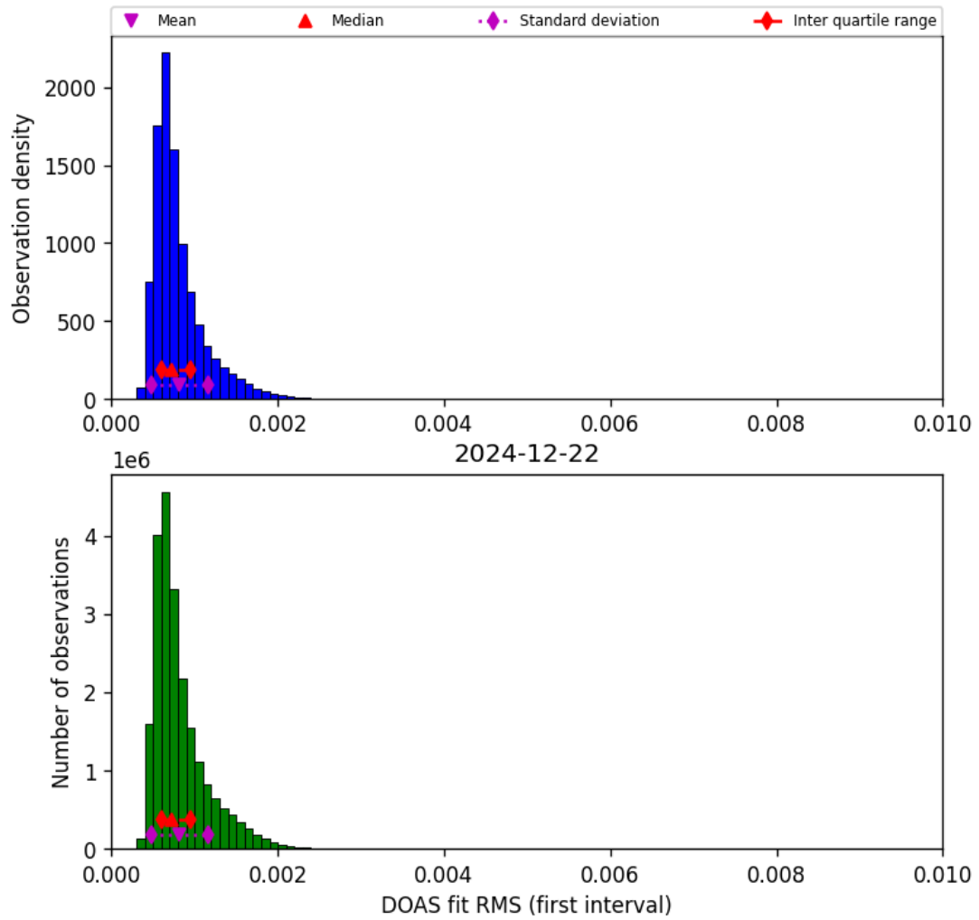
Figure 44: Histogram of “DOAS fit RMS (first interval)” for 2024-12-22 to 2024-12-23
