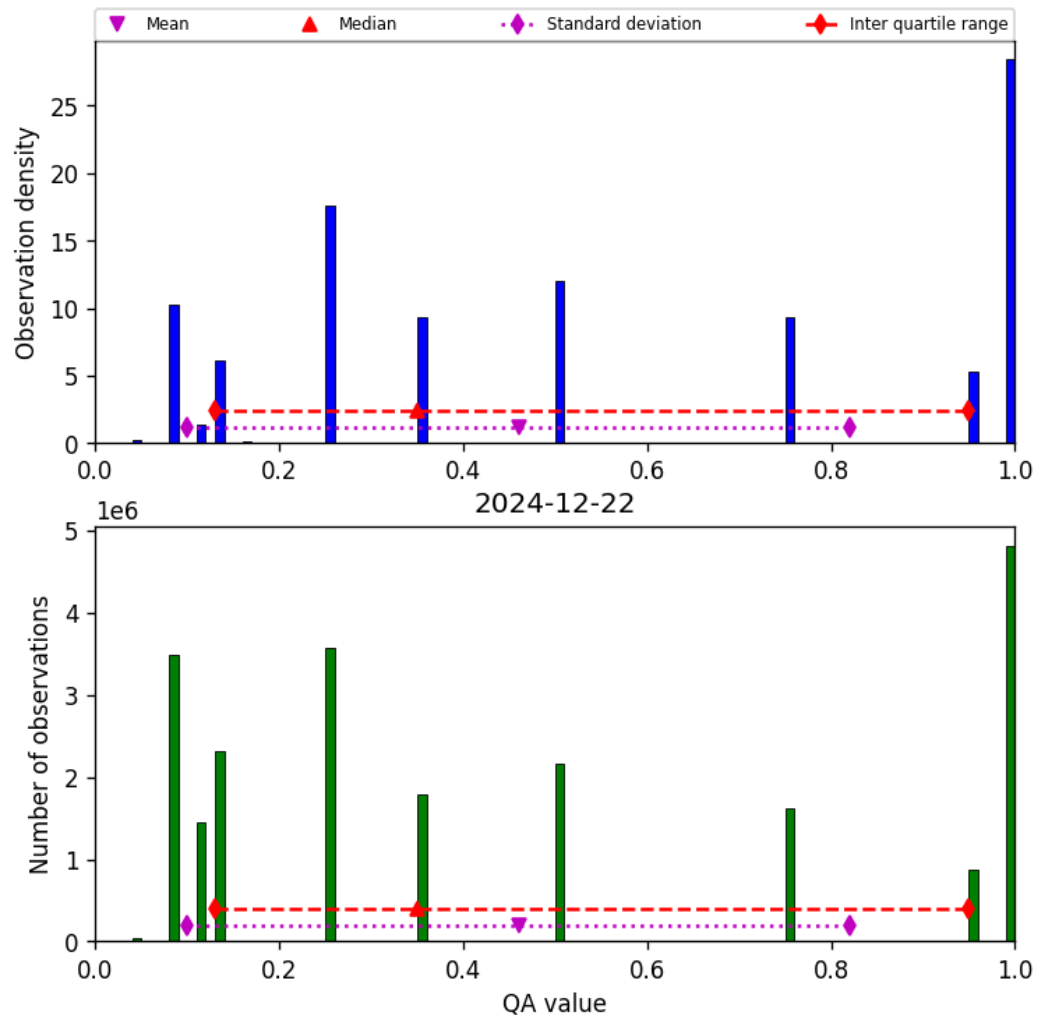
Figure 32: Histogram of “QA value” for 2024-12-22 to 2024-12-23
