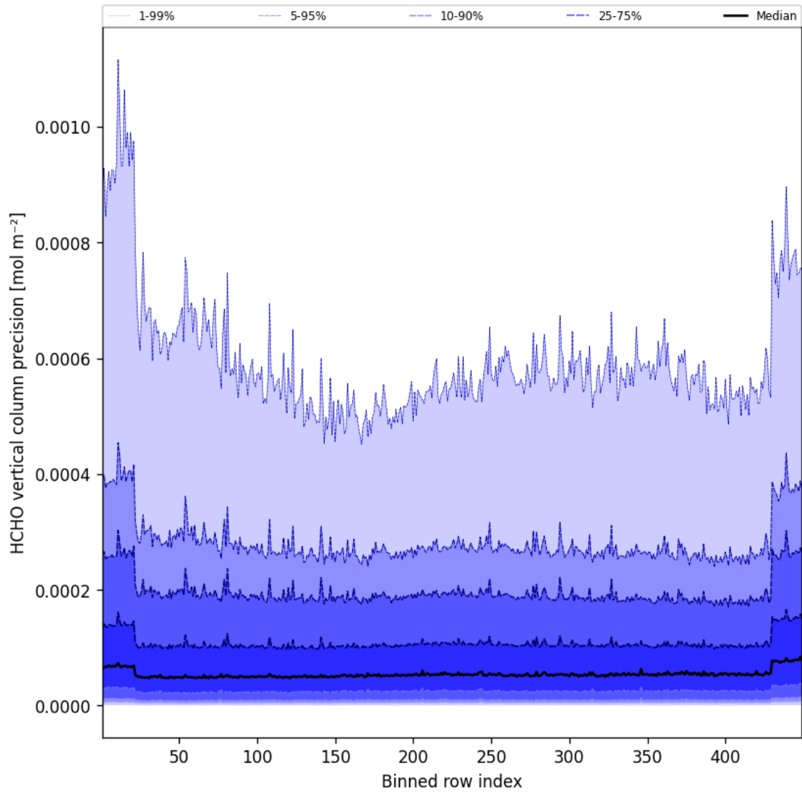
Figure 48: Along track statistics of “HCHO vertical column precision” for 2024-12-22 to 2024-12-23
