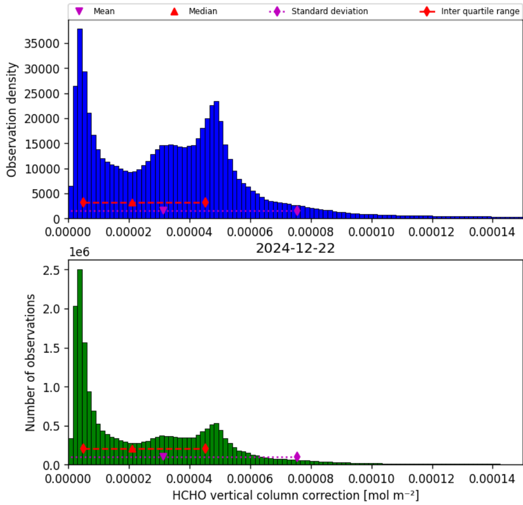
Figure 35: Histogram of “HCHO vertical column correction” for 2024-12-22 to 2024-12-23
