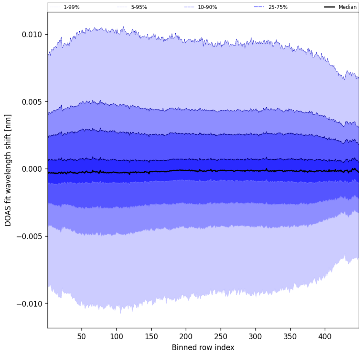
Figure 56: Along track statistics of “DOAS fit wavelength shift” for 2024-12-22 to 2024-12-23
