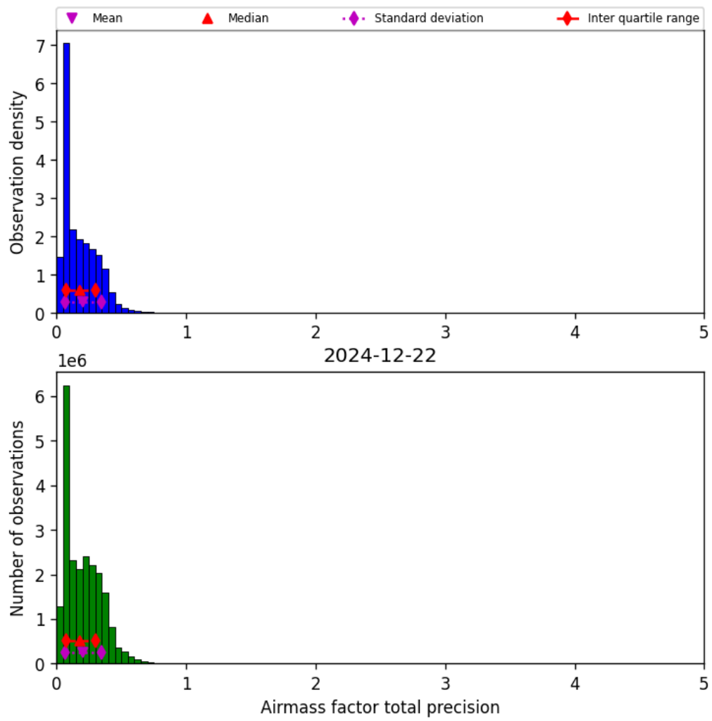
Figure 39: Histogram of “Airmass factor total precision” for 2024-12-22 to 2024-12-23
