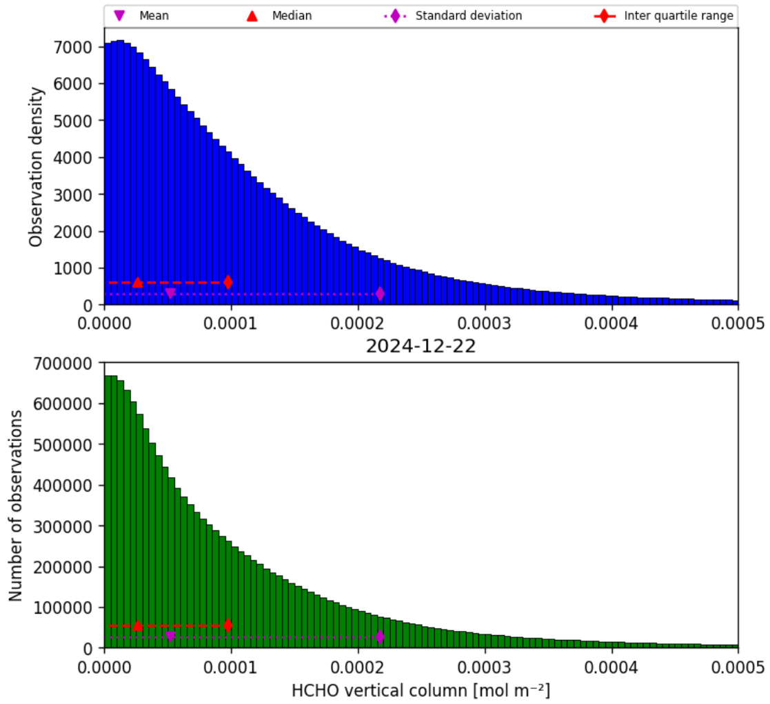
Figure 33: Histogram of “HCHO vertical column” for 2024-12-22 to 2024-12-23
