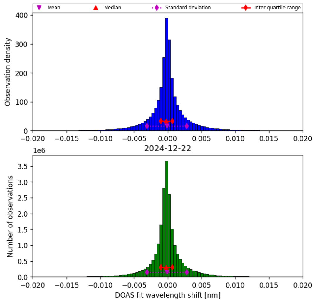
Figure 42: Histogram of “DOAS fit wavelength shift” for 2024-12-22 to 2024-12-23
