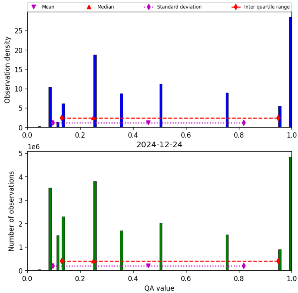
Figure 32: Histogram of “QA value” for 2024-12-24 to 2024-12-25
