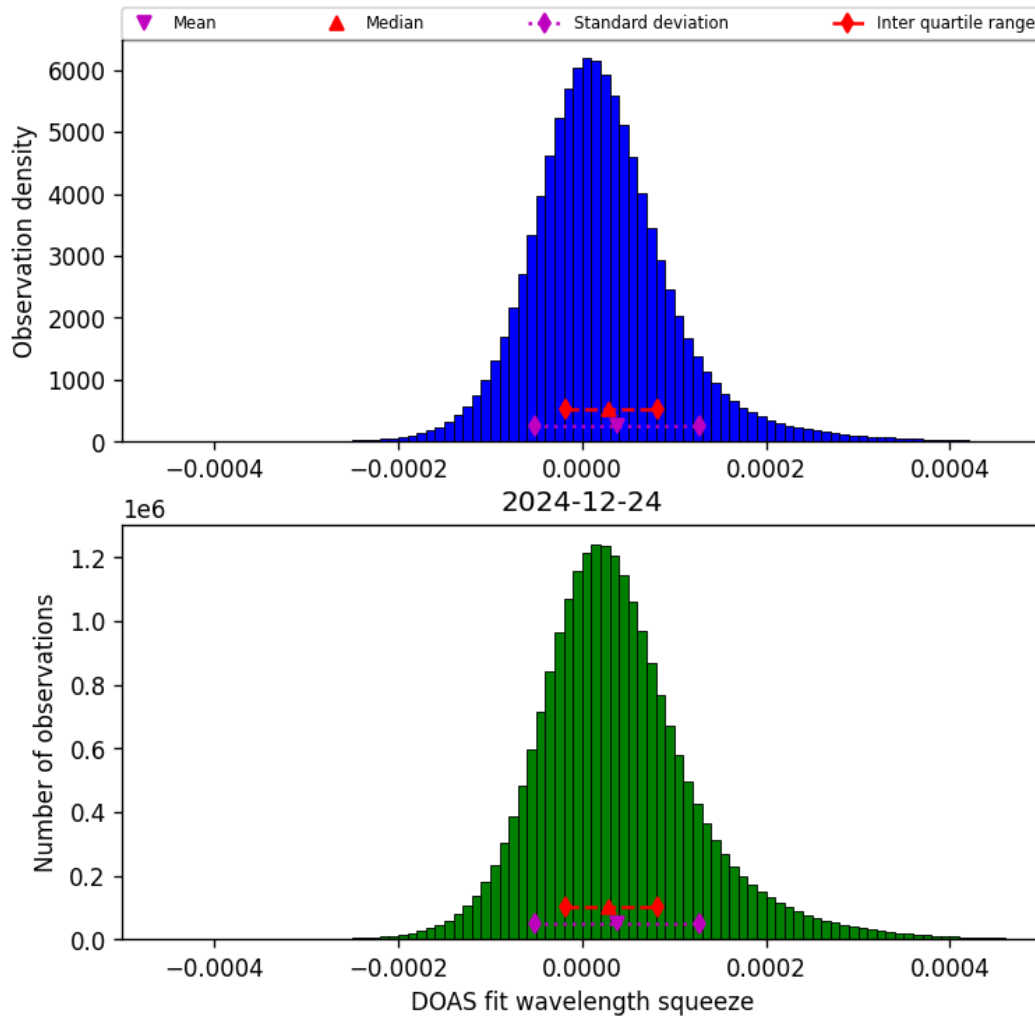
Figure 43: Histogram of “DOAS fit wavelength squeeze” for 2024-12-24 to 2024-12-25
