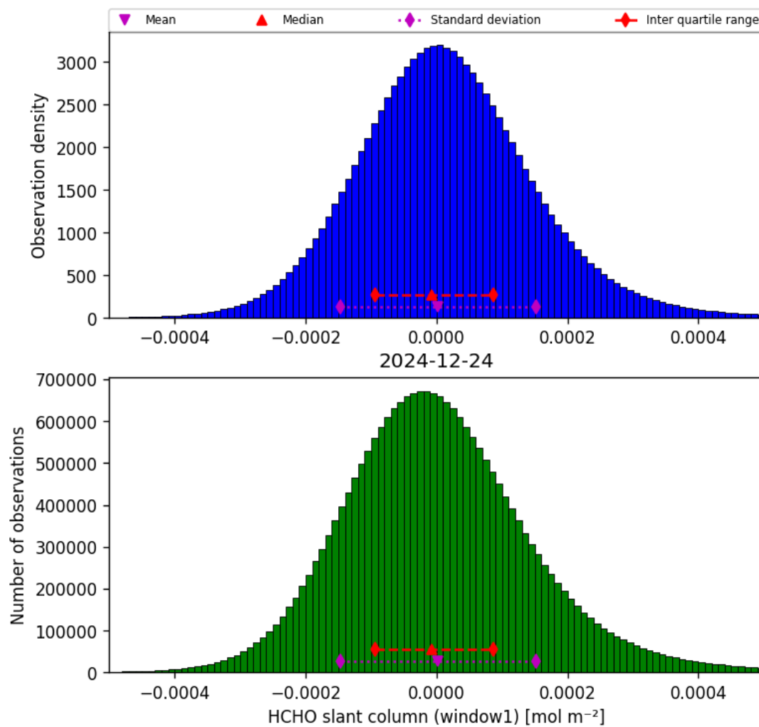
Figure 36: Histogram of “HCHO slant column (window1)” for 2024-12-24 to 2024-12-25
