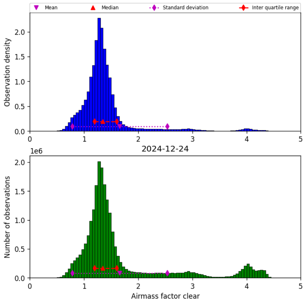
Figure 40: Histogram of “Airmass factor clear” for 2024-12-24 to 2024-12-25
