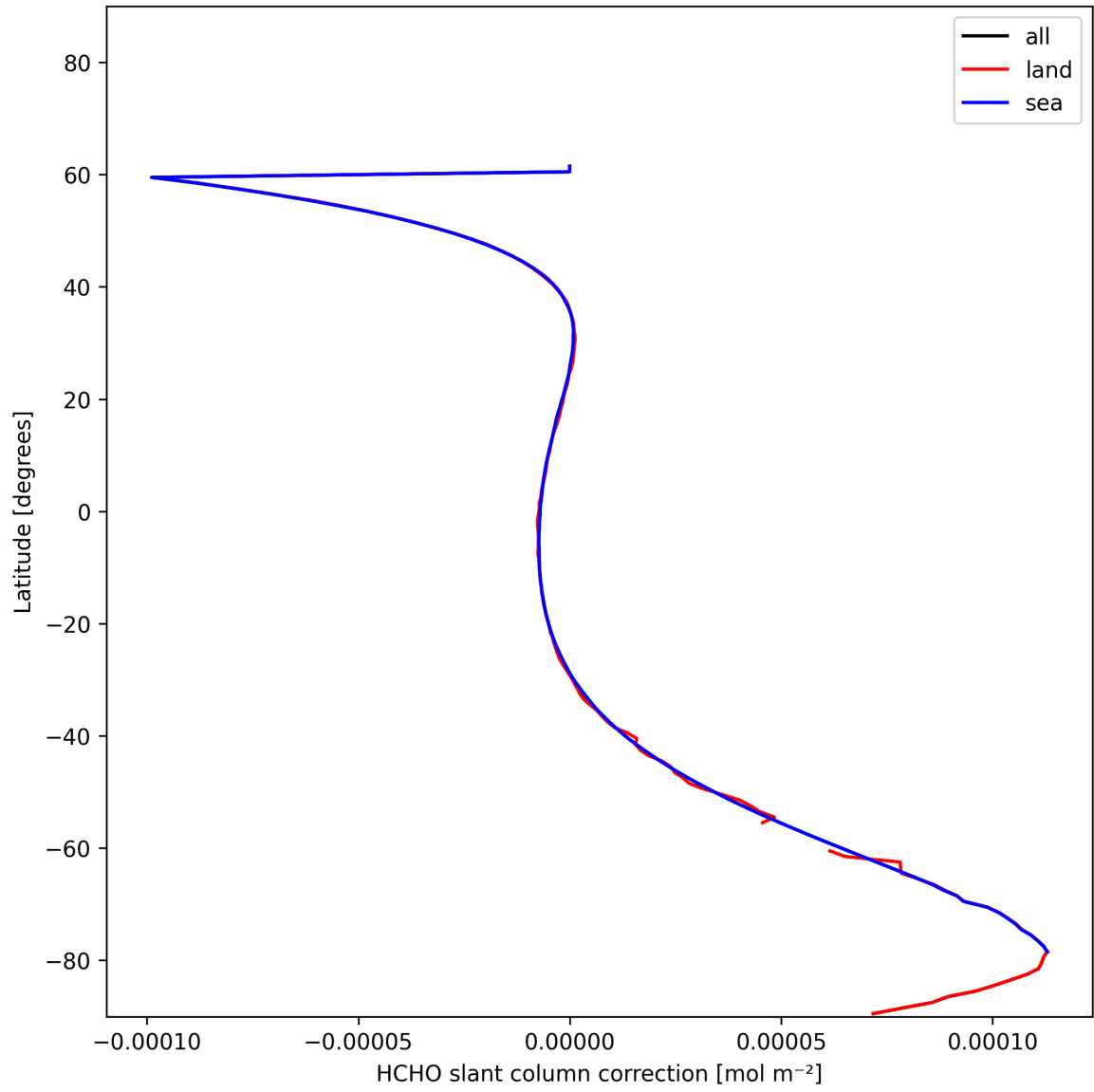
Figure 31: Zonal average of “HCHO slant column correction” for 2024-12-24 to 2024-12-25.
