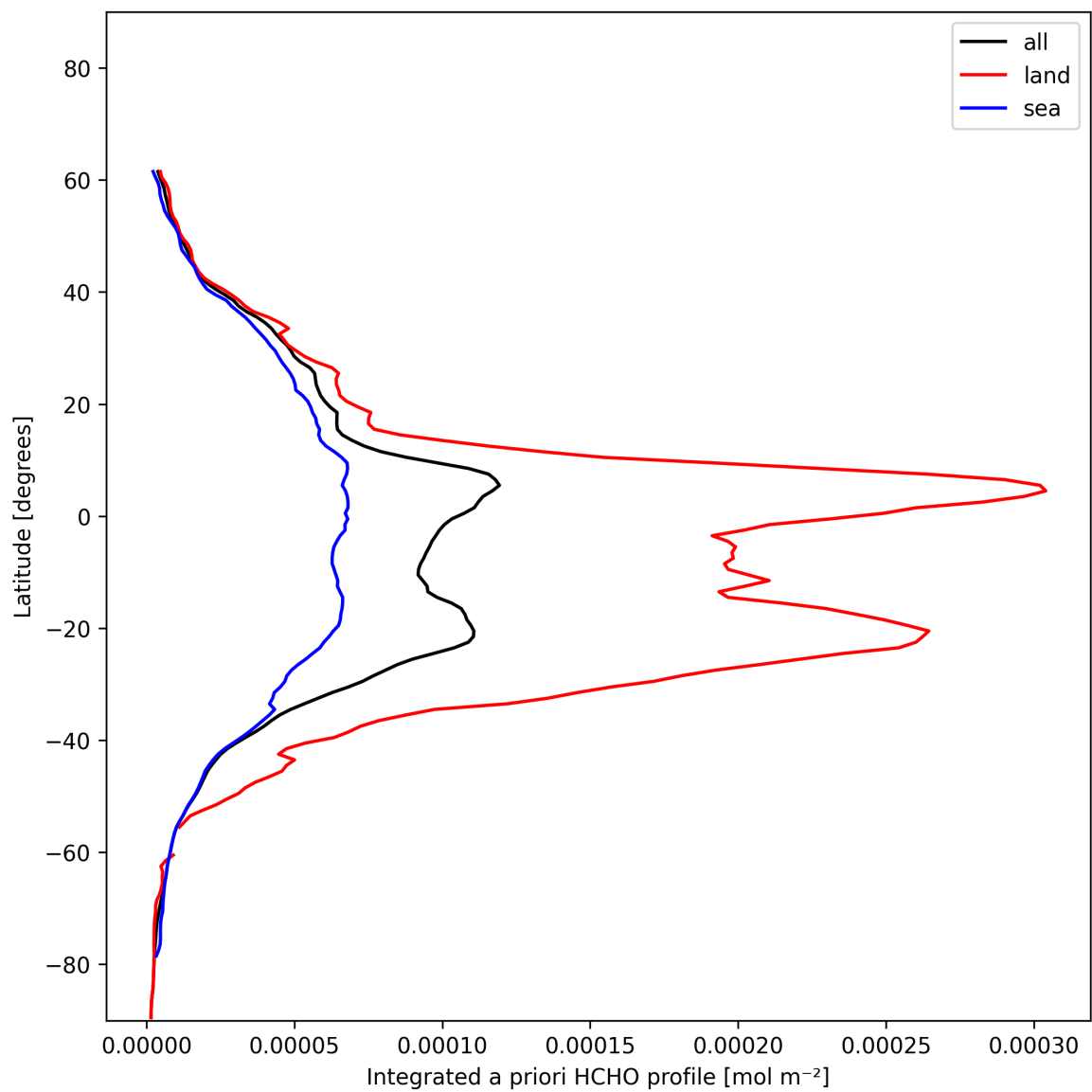
Figure 27: Zonal average of “Integrated a priori HCHO profile” for 2024-12-24 to 2024-12-25.
