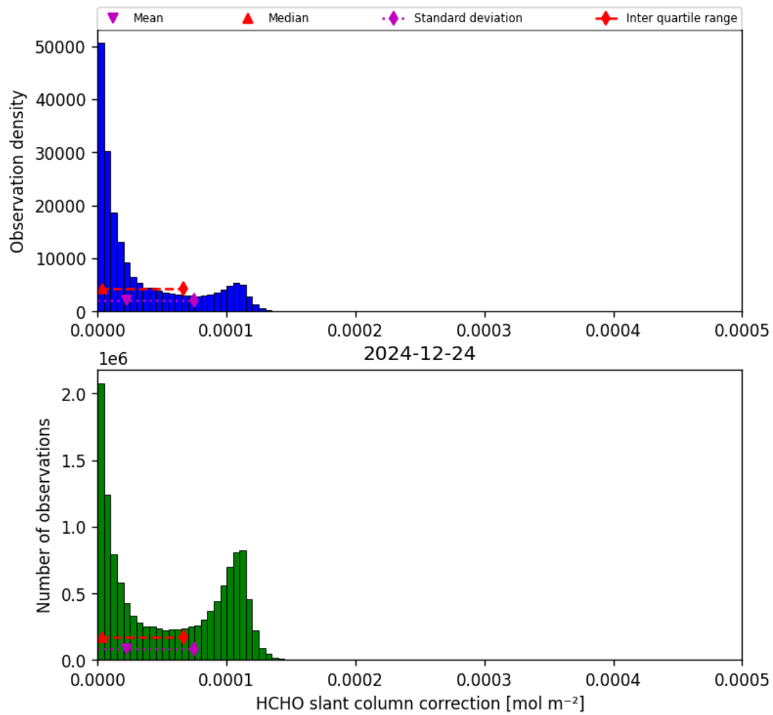
Figure 45: Histogram of “HCHO slant column correction” for 2024-12-24 to 2024-12-25
