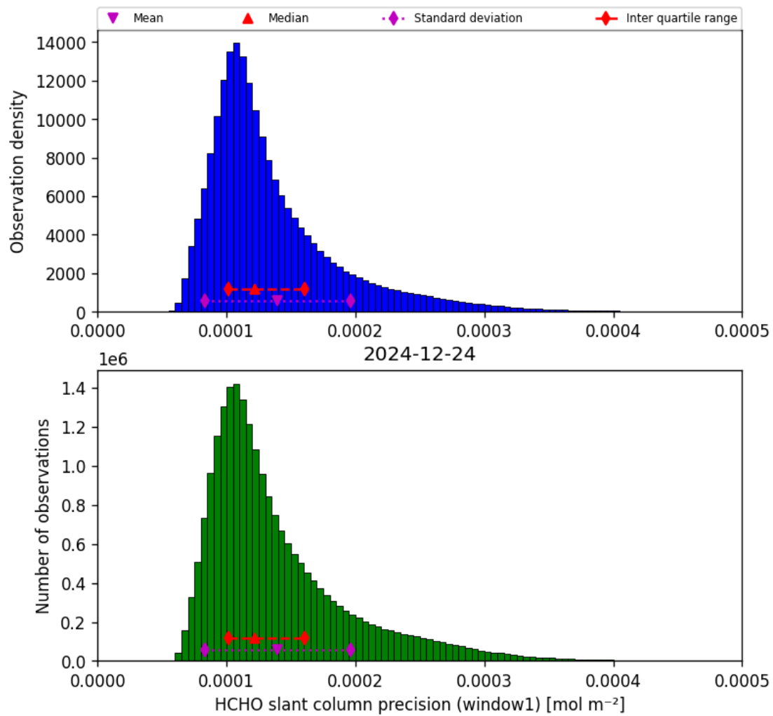
Figure 37: Histogram of “HCHO slant column precision (window1)” for 2024-12-24 to 2024-12-25
