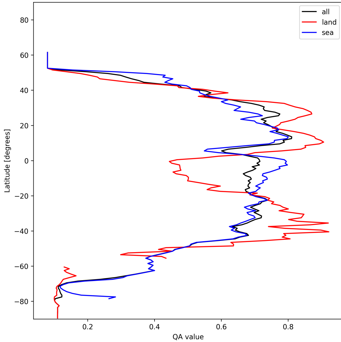
Figure 18: Zonal average of “QA value” for 2024-12-24 to 2024-12-25.
