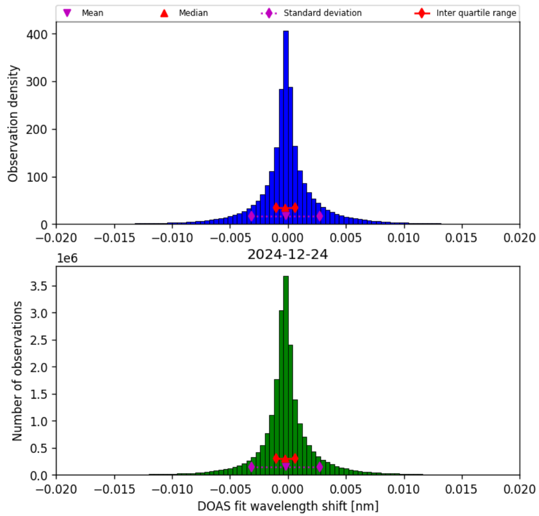
Figure 42: Histogram of “DOAS fit wavelength shift” for 2024-12-24 to 2024-12-25
