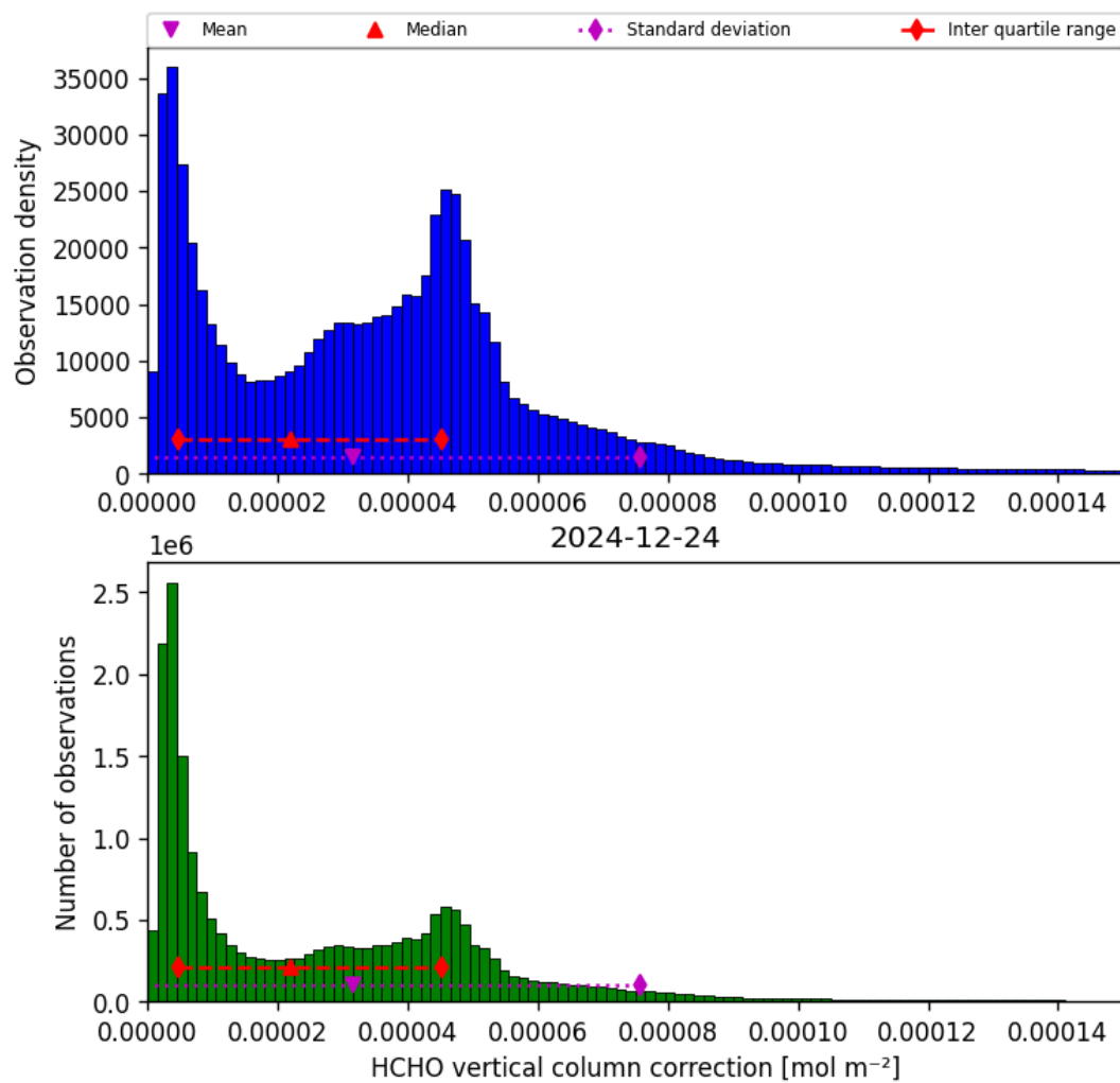
Figure 35: Histogram of “HCHO vertical column correction” for 2024-12-24 to 2024-12-25
