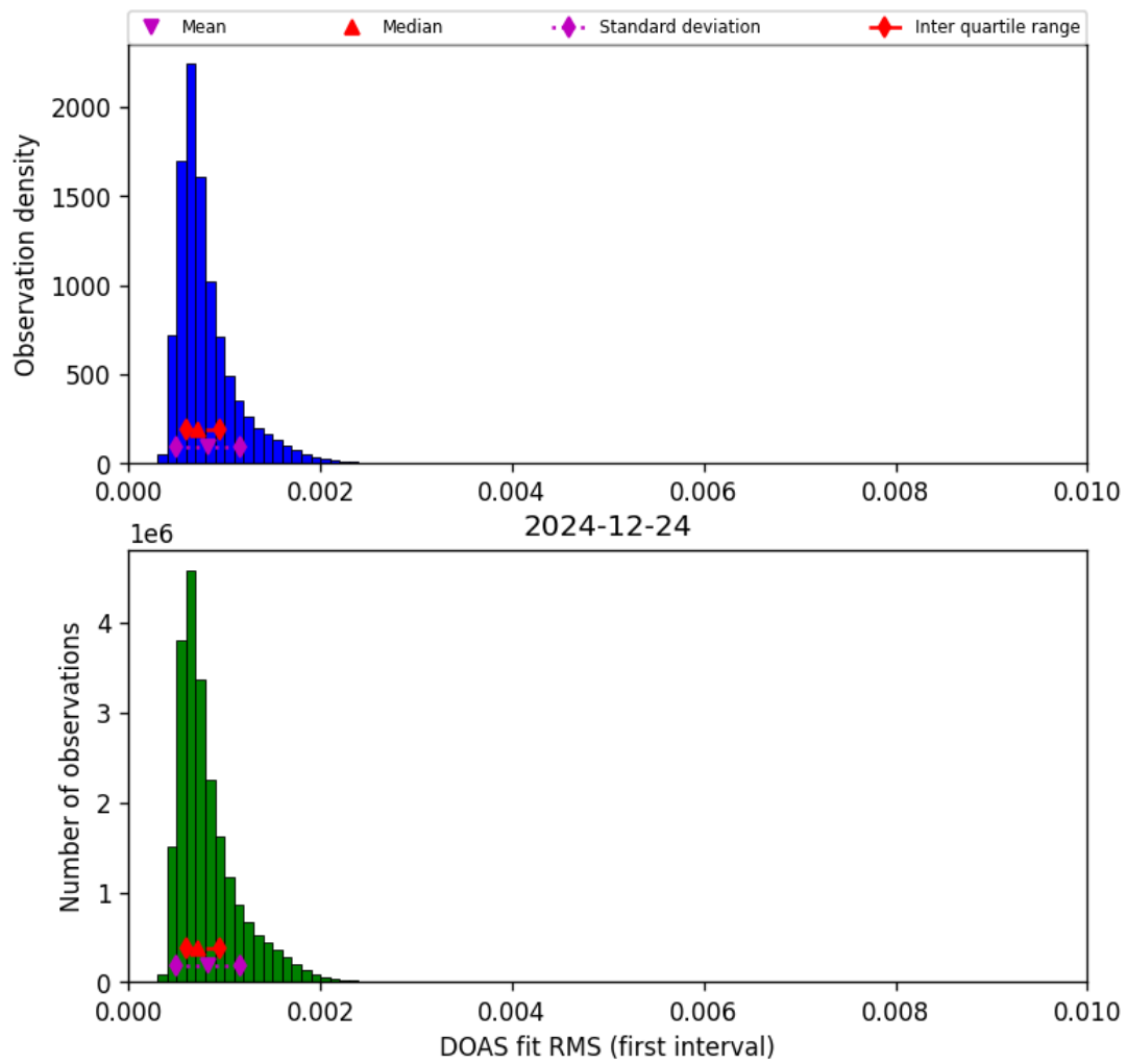
Figure 44: Histogram of “DOAS fit RMS (first interval)” for 2024-12-24 to 2024-12-25
