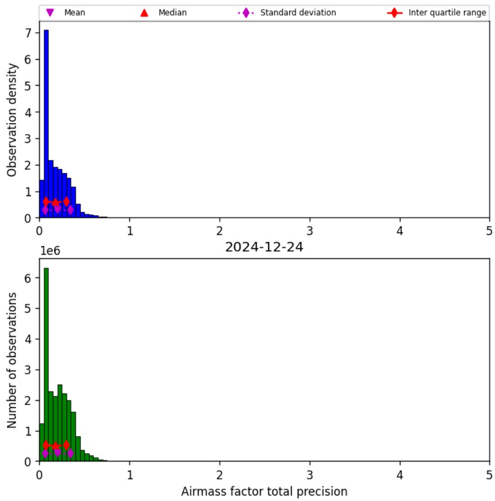
Figure 39: Histogram of “Airmass factor total precision” for 2024-12-24 to 2024-12-25
