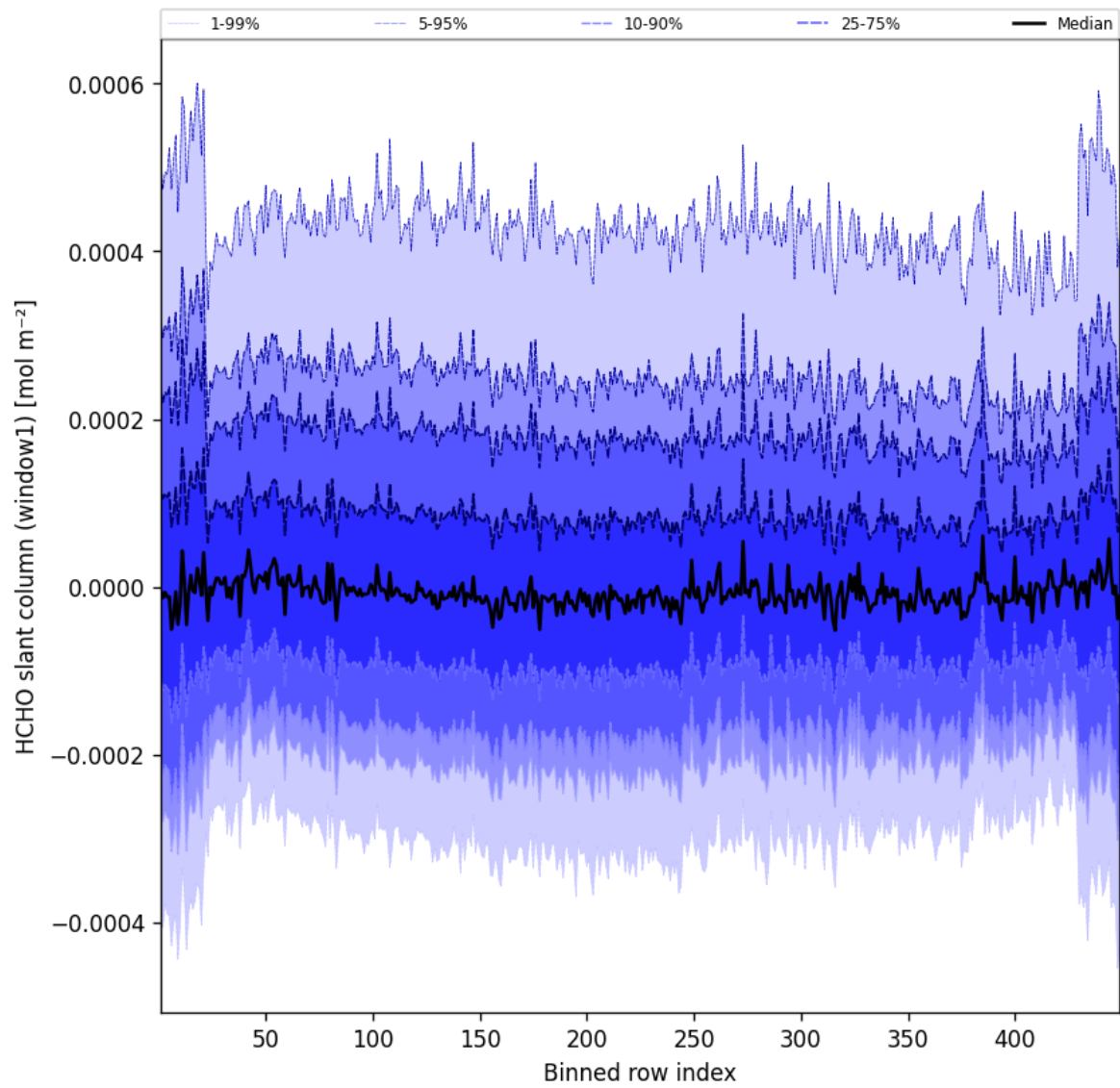
Figure 50: Along track statistics of “HCHO slant column (window1)” for 2024-12-24 to 2024-12-25
