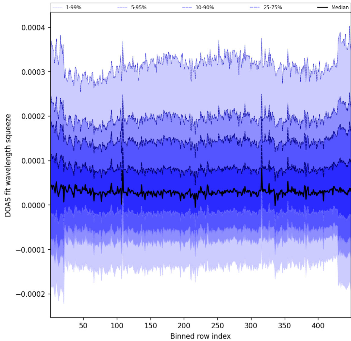
Figure 57: Along track statistics of “DOAS fit wavelength squeeze” for 2024-12-24 to 2024-12-25
