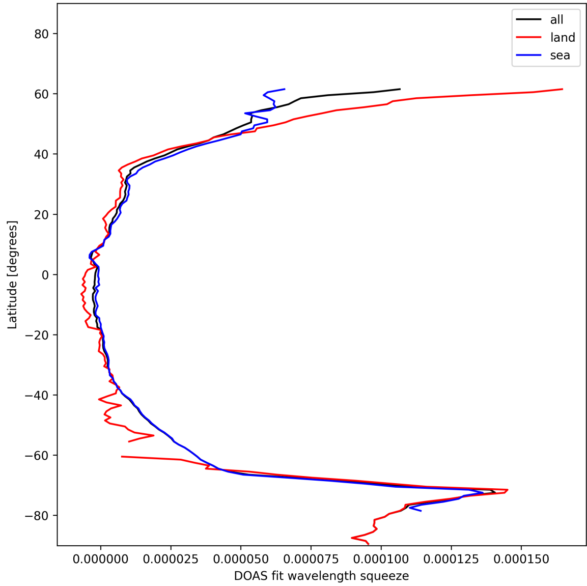
Figure 29: Zonal average of “DOAS fit wavelength squeeze” for 2024-12-24 to 2024-12-25.
