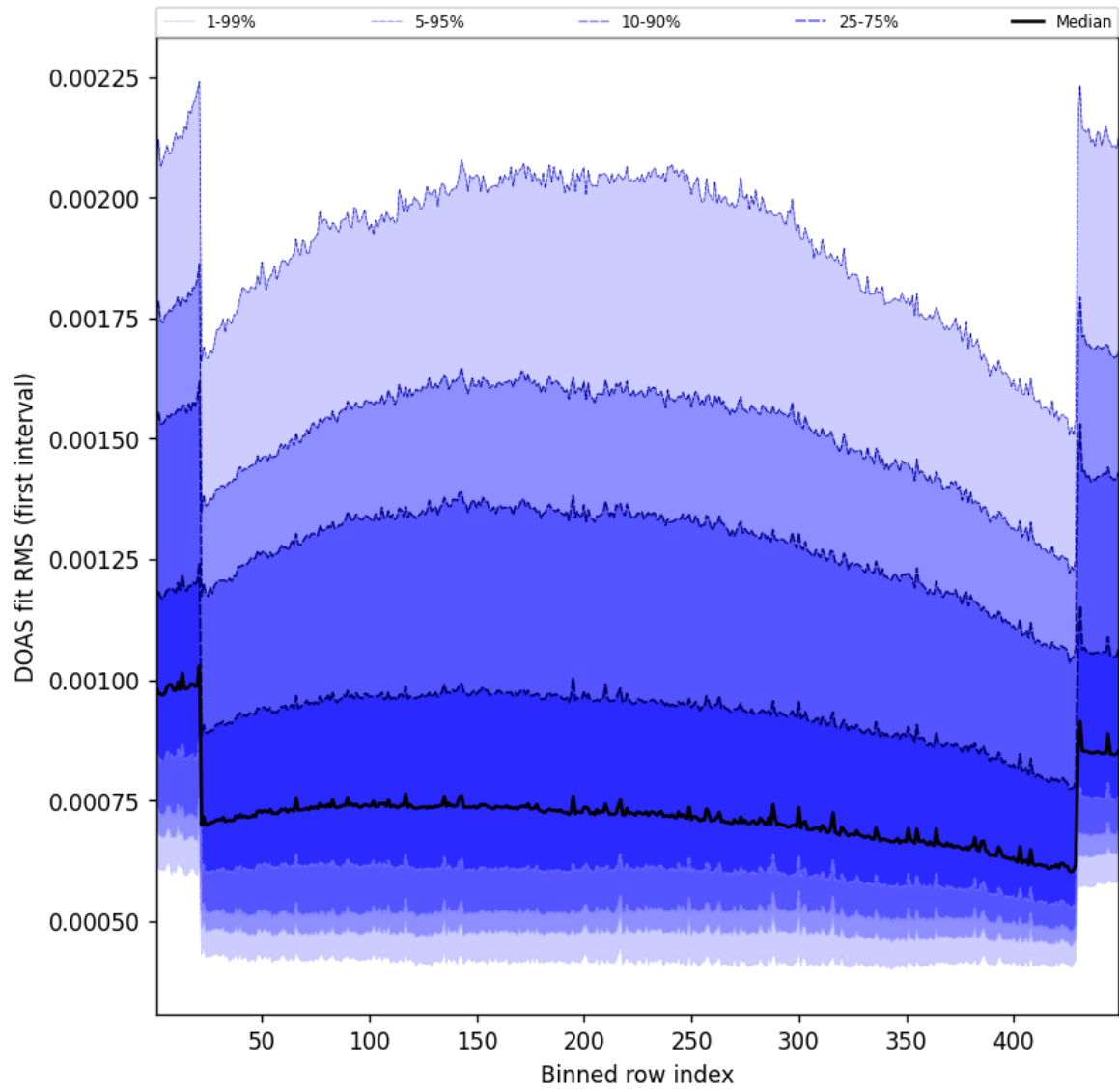
Figure 58: Along track statistics of “DOAS fit RMS (first interval)” for 2024-12-24 to 2024-12-25
