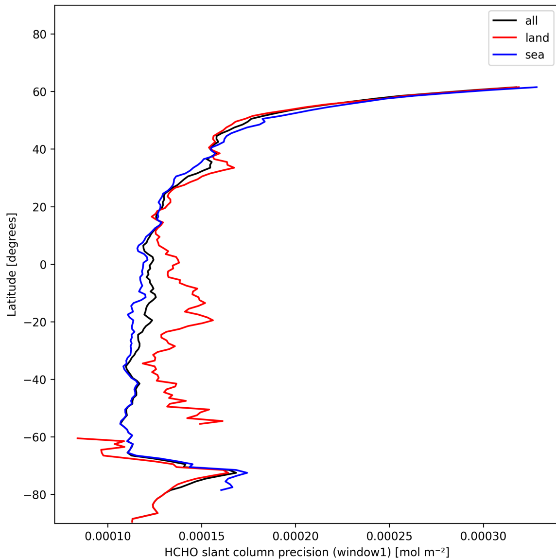
Figure 23: Zonal average of "HCHO slant column precision (window1)" for 2024-12-24 to 2024-12-25.
