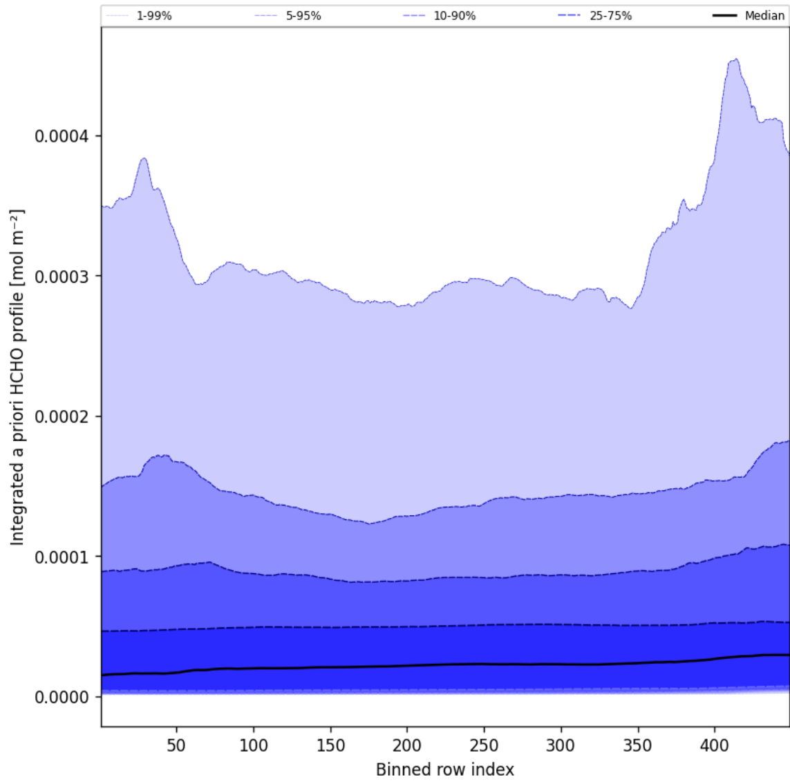
Figure 55: Along track statistics of "Integrated a priori HCHO profile" for 2024-12-24 to 2024-12-25
