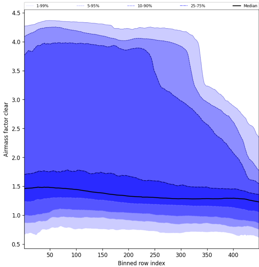
Figure 54: Along track statistics of “Air mass factor clear” for 2024-12-24 to 2024-12-25
