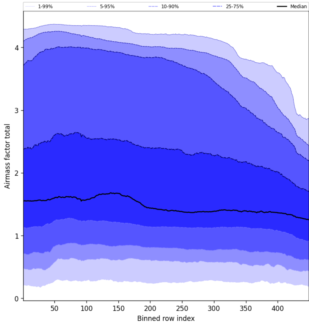
Figure 52: Along track statistics of “Airmass factor total” for 2024-12-24 to 2024-12-25
