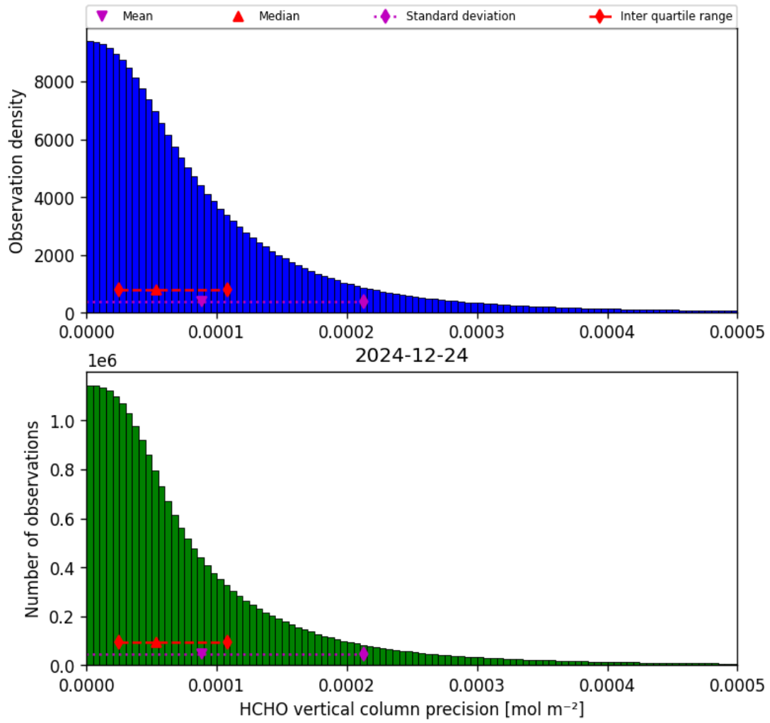
Figure 34: Histogram of “HCHO vertical column precision” for 2024-12-24 to 2024-12-25
