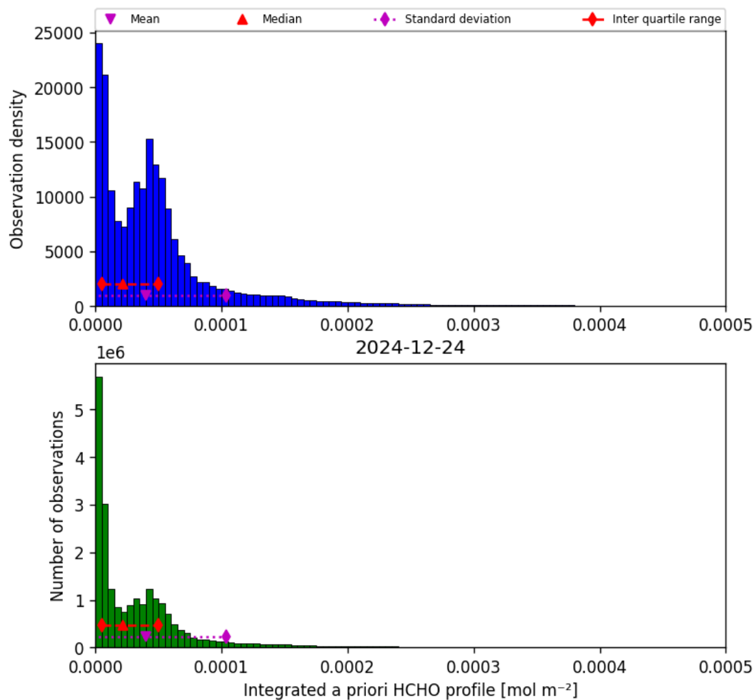
Figure 41: Histogram of “Integrated a priori HCHO profile” for 2024-12-24 to 2024-12-25
