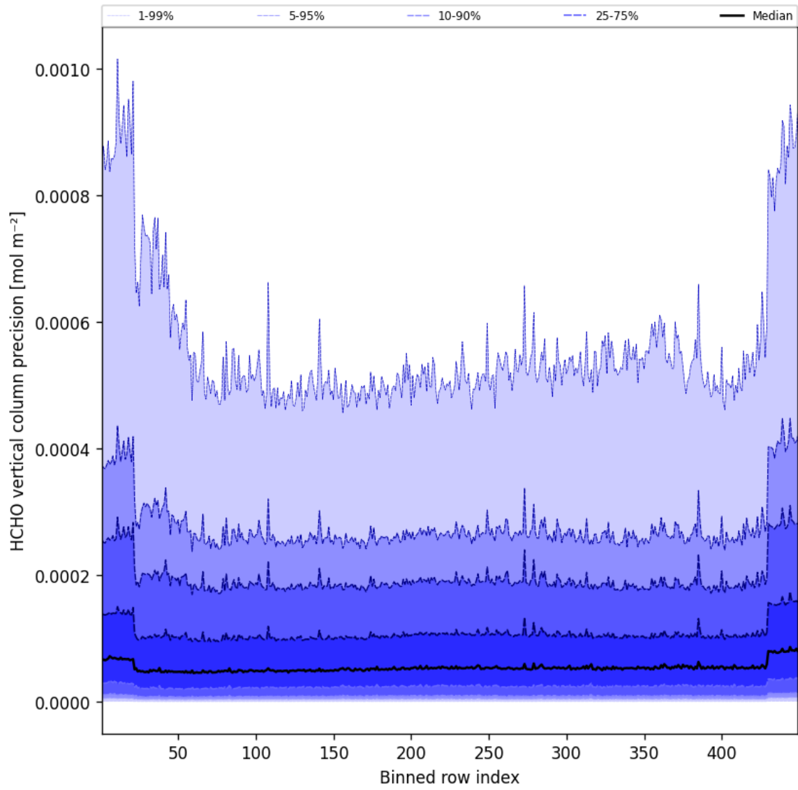
Figure 48: Along track statistics of “HCHO vertical column precision” for 2024-12-24 to 2024-12-25
