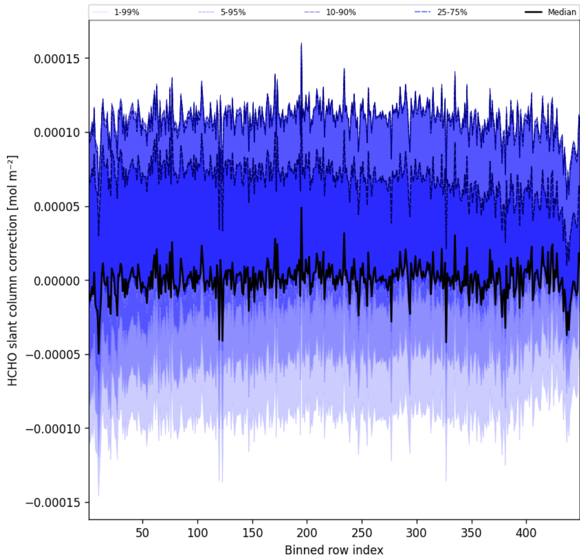
Figure 59: Along track statistics of “HCHO slant column correction” for 2024-12-24 to 2024-12-25
