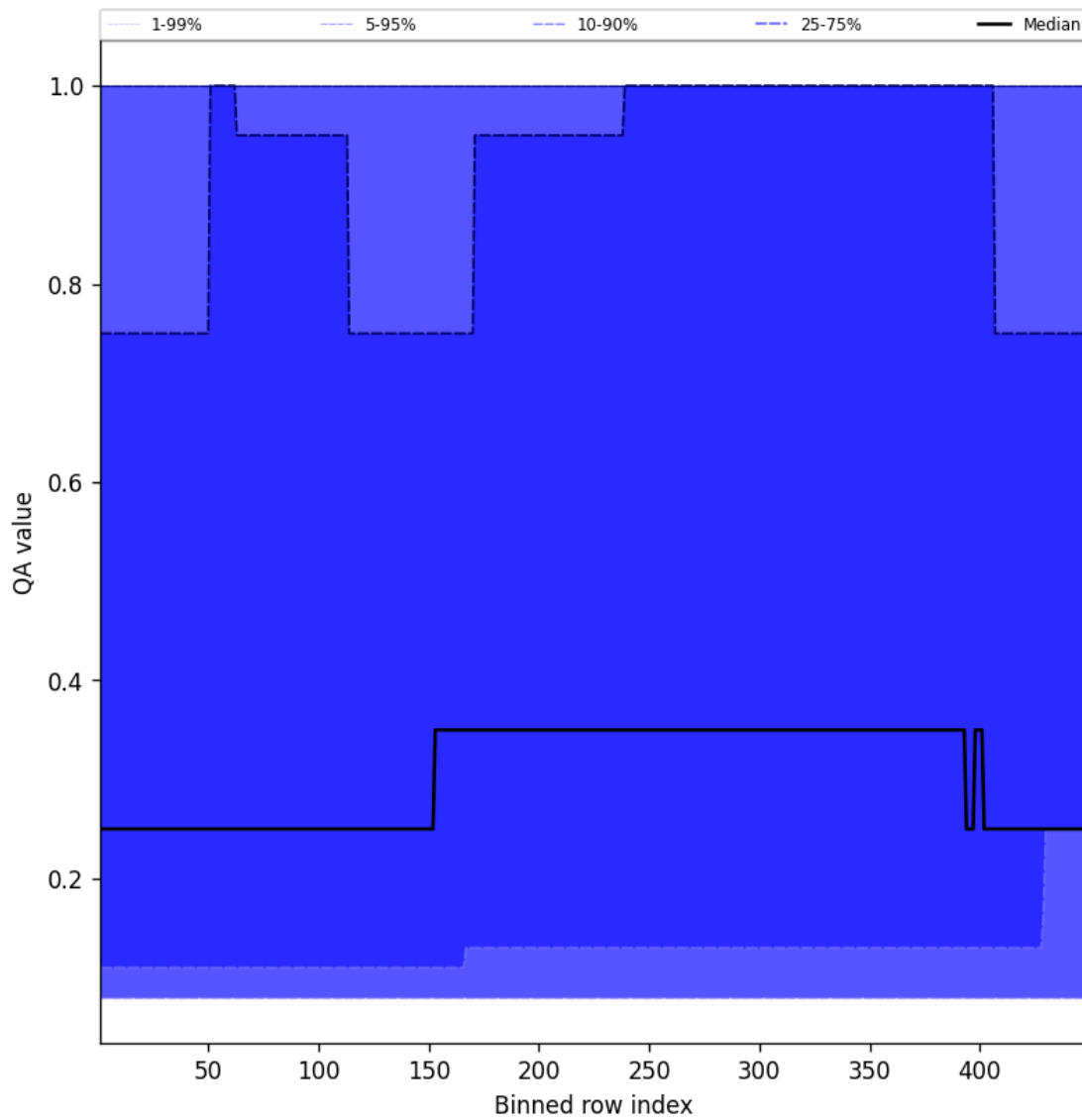
Figure 46: Along track statistics of “QA value” for 2024-12-24 to 2024-12-25
