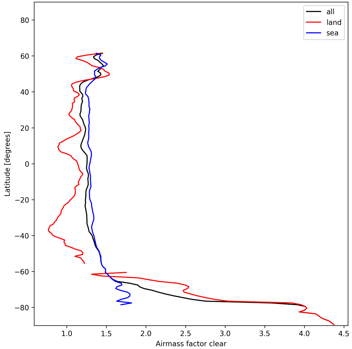
Figure 26: Zonal average of “Airmass factor clear” for 2024-12-24 to 2024-12-25.
