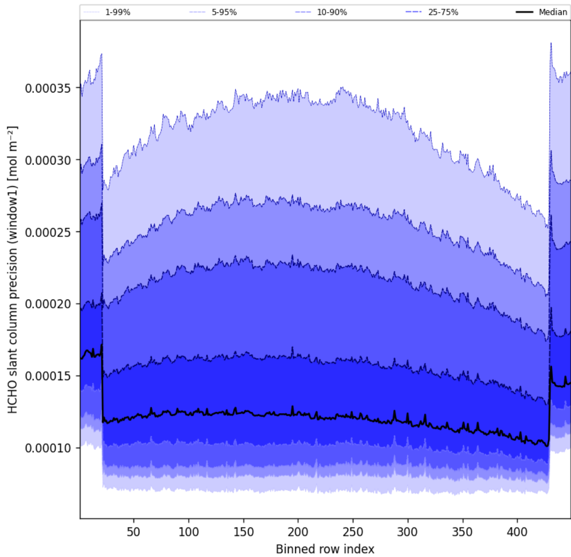
Figure 51: Along track statistics of “HCHO slant column precision (window1)” for 2024-12-24 to 2024-12-25
