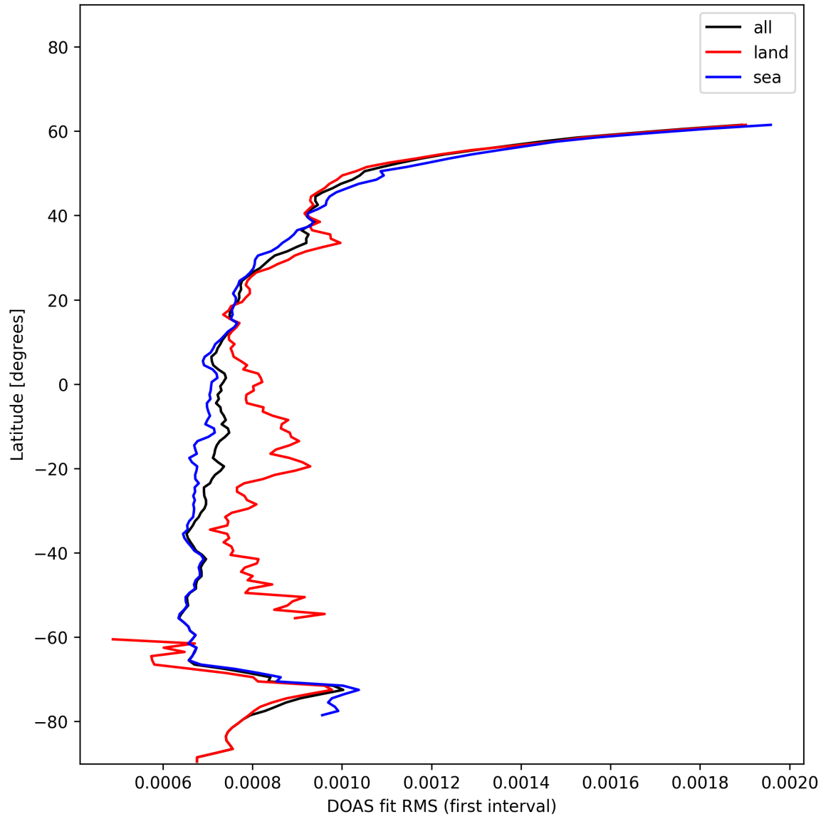
Figure 30: Zonal average of “DOAS fit RMS (first interval)” for 2024-12-24 to 2024-12-25.
