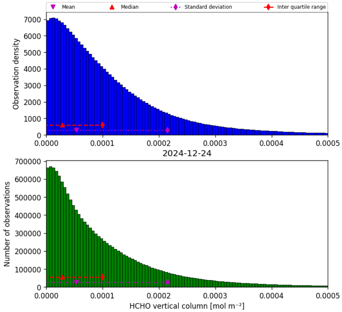
Figure 33: Histogram of “HCHO vertical column” for 2024-12-24 to 2024-12-25
