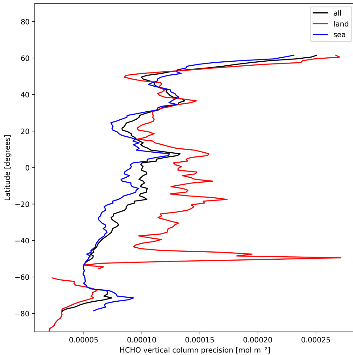
Figure 20: Zonal average of “HCHO vertical column precision” for 2024-12-24 to 2024-12-25.
