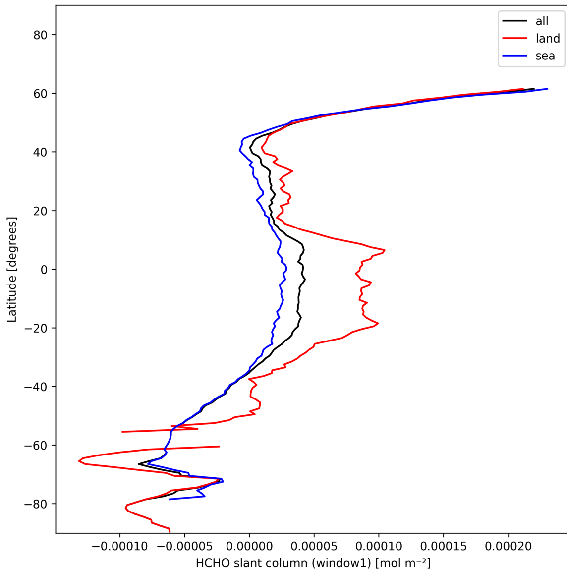
Figure 22: Zonal average of “HCHO slant column (window1)” for 2024-12-24 to 2024-12-25.
