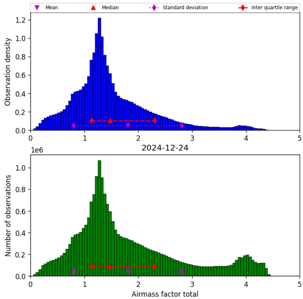
Figure 38: Histogram of “Airmass factor total” for 2024-12-24 to 2024-12-25
