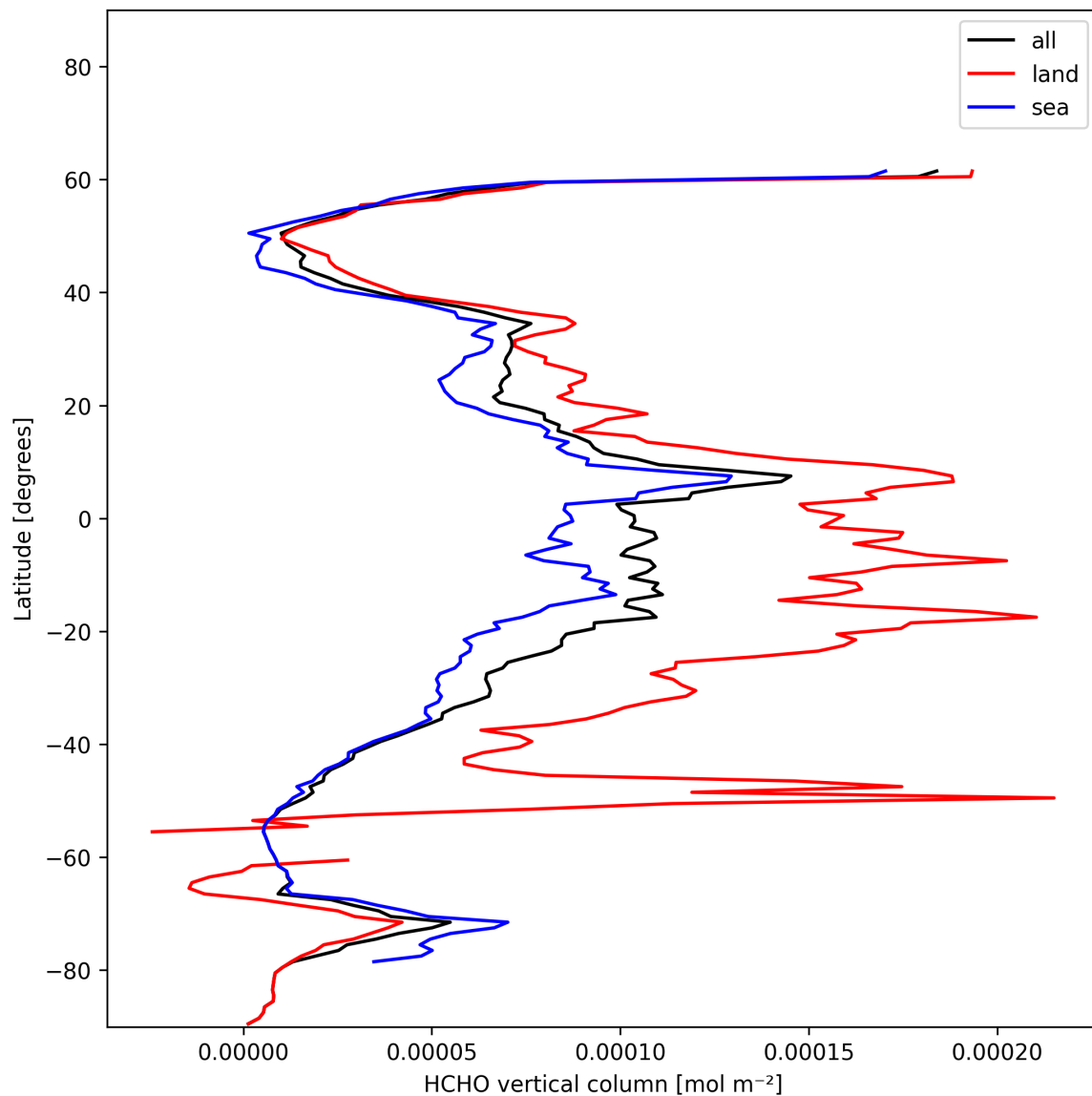
Figure 19: Zonal average of “HCHO vertical column” for 2024-12-24 to 2024-12-25.
