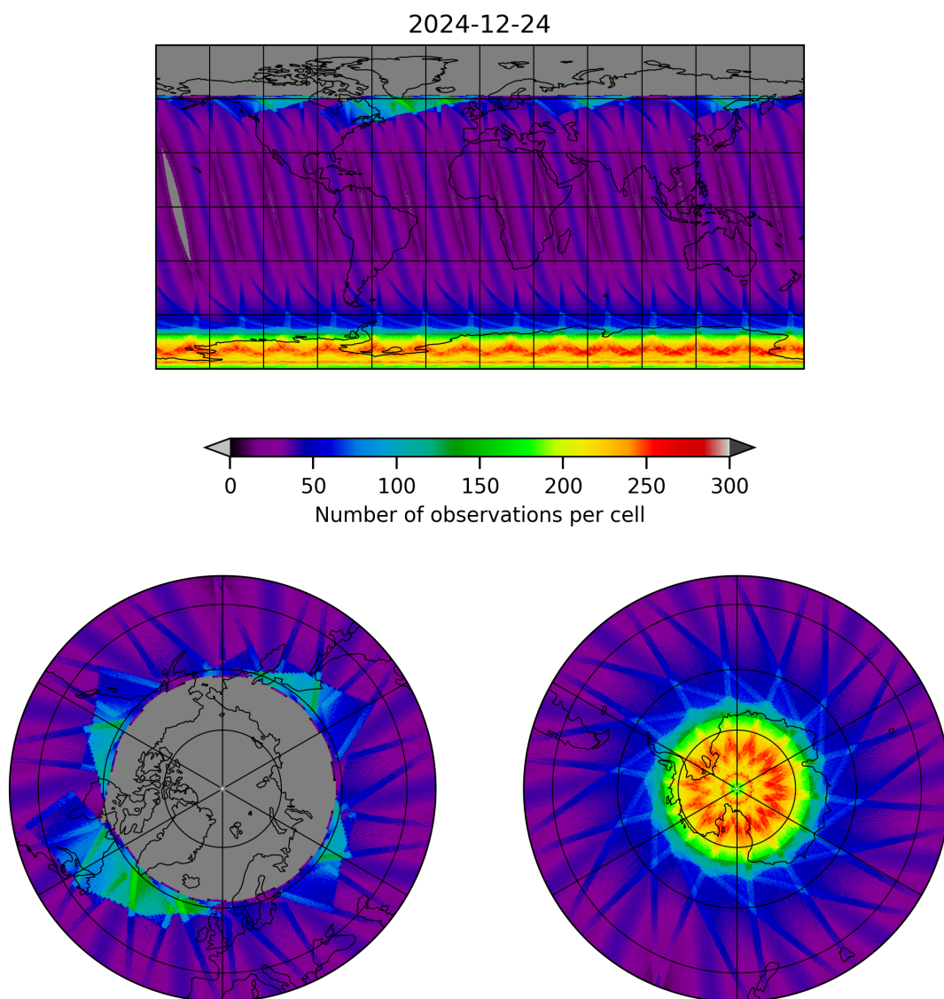
Figure 17: Map of the number of observations for 2024-12-24 to 2024-12-25
