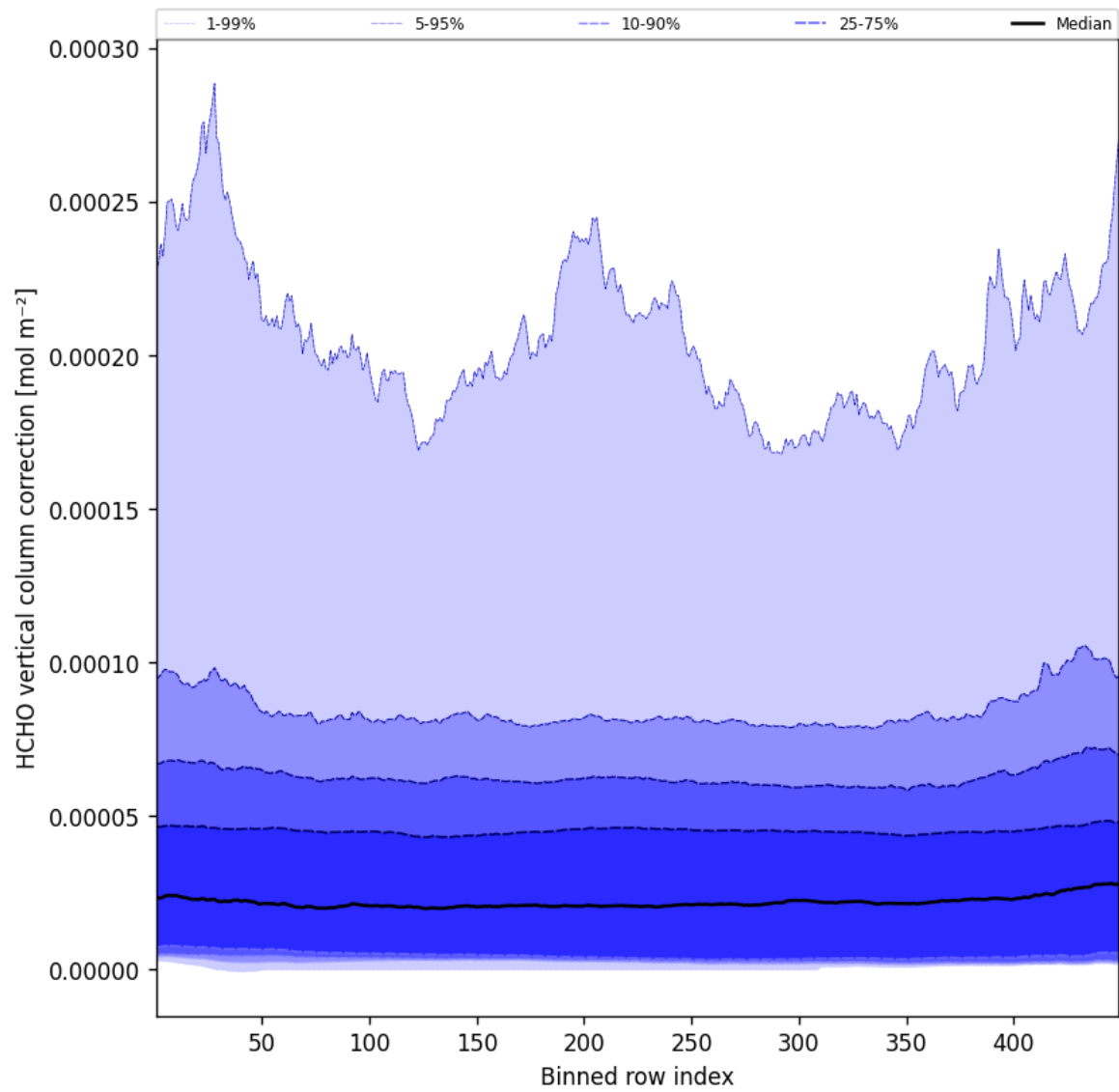
Figure 49: Along track statistics of “HCHO vertical column correction” for 2024-12-24 to 2024-12-25
