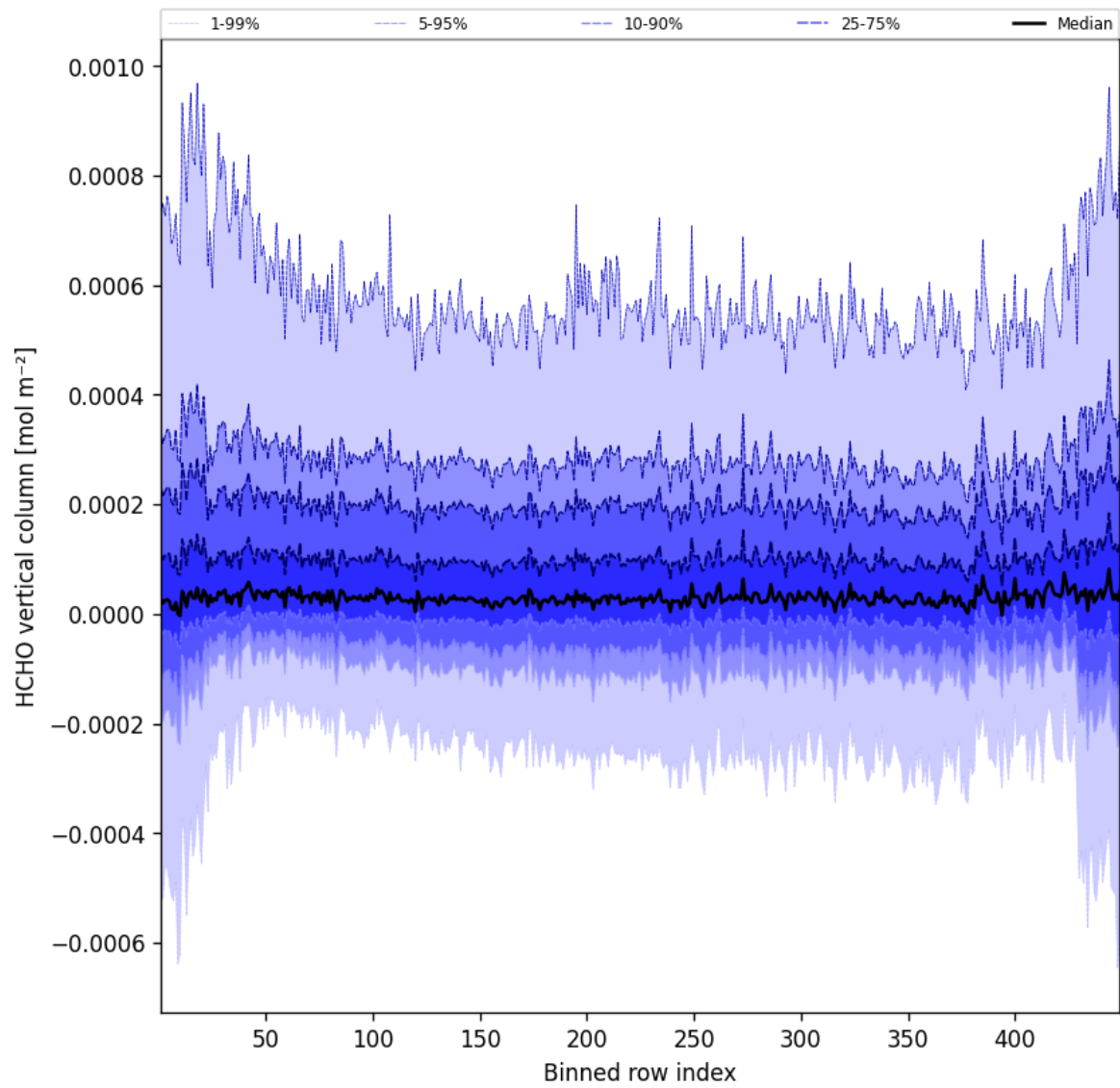
Figure 47: Along track statistics of “HCHO vertical column” for 2024-12-24 to 2024-12-25
