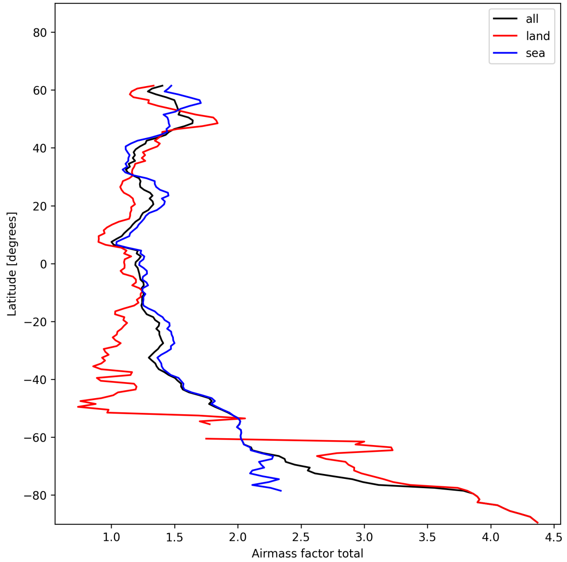
Figure 24: Zonal average of “Airmass factor total” for 2024-12-24 to 2024-12-25.
