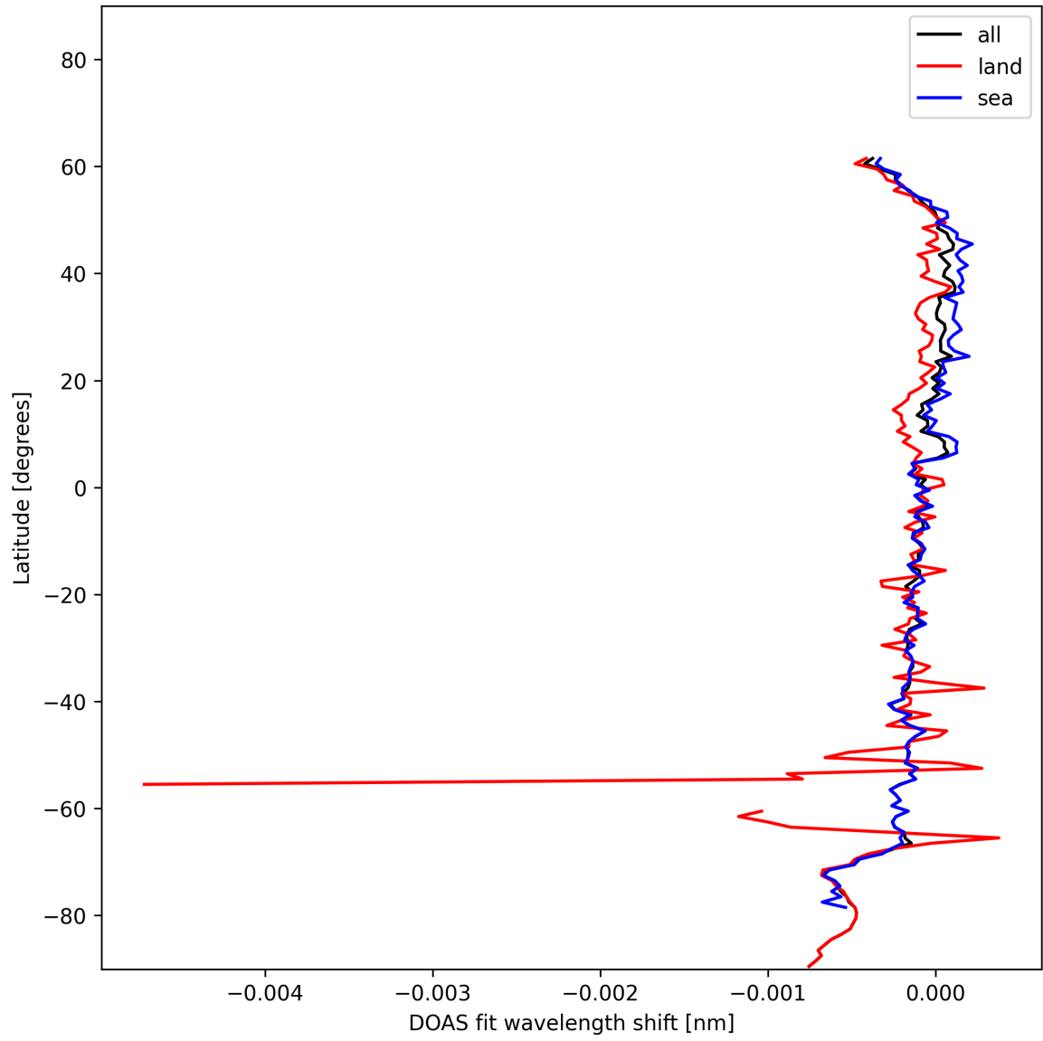
Figure 28: Zonal average of "DOAS fit wavelength shift" for 2024-12-24 to 2024-12-25.
