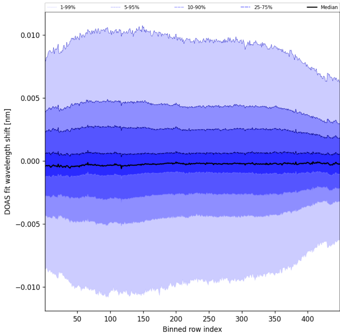
Figure 56: Along track statistics of “DOAS fit wavelength shift” for 2024-12-24 to 2024-12-25
