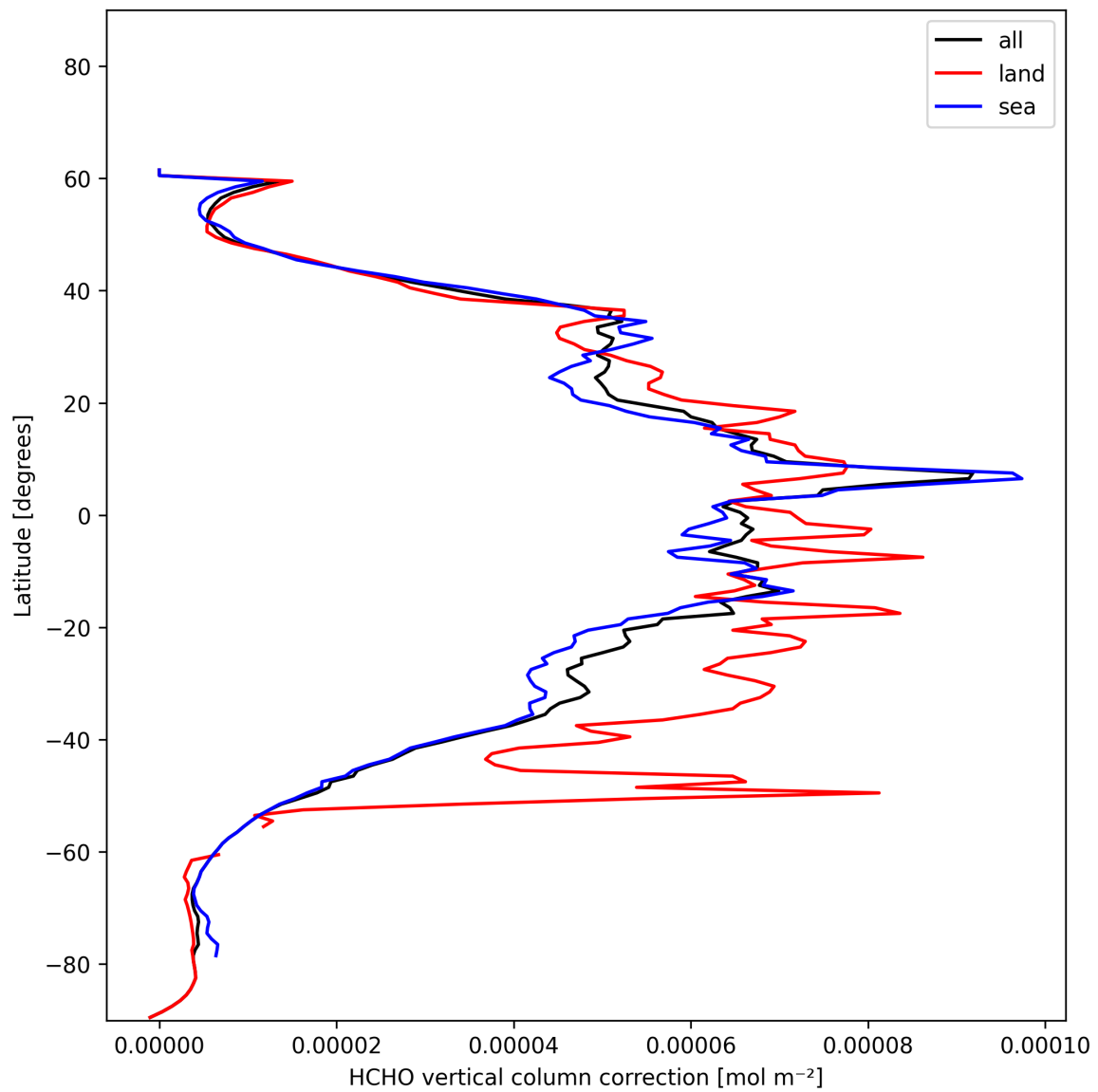
Figure 21: Zonal average of “HCHO vertical column correction” for 2024-12-24 to 2024-12-25.
