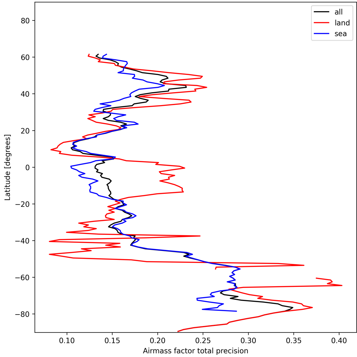
Figure 25: Zonal average of “Airmass factor total precision” for 2024-12-24 to 2024-12-25.
