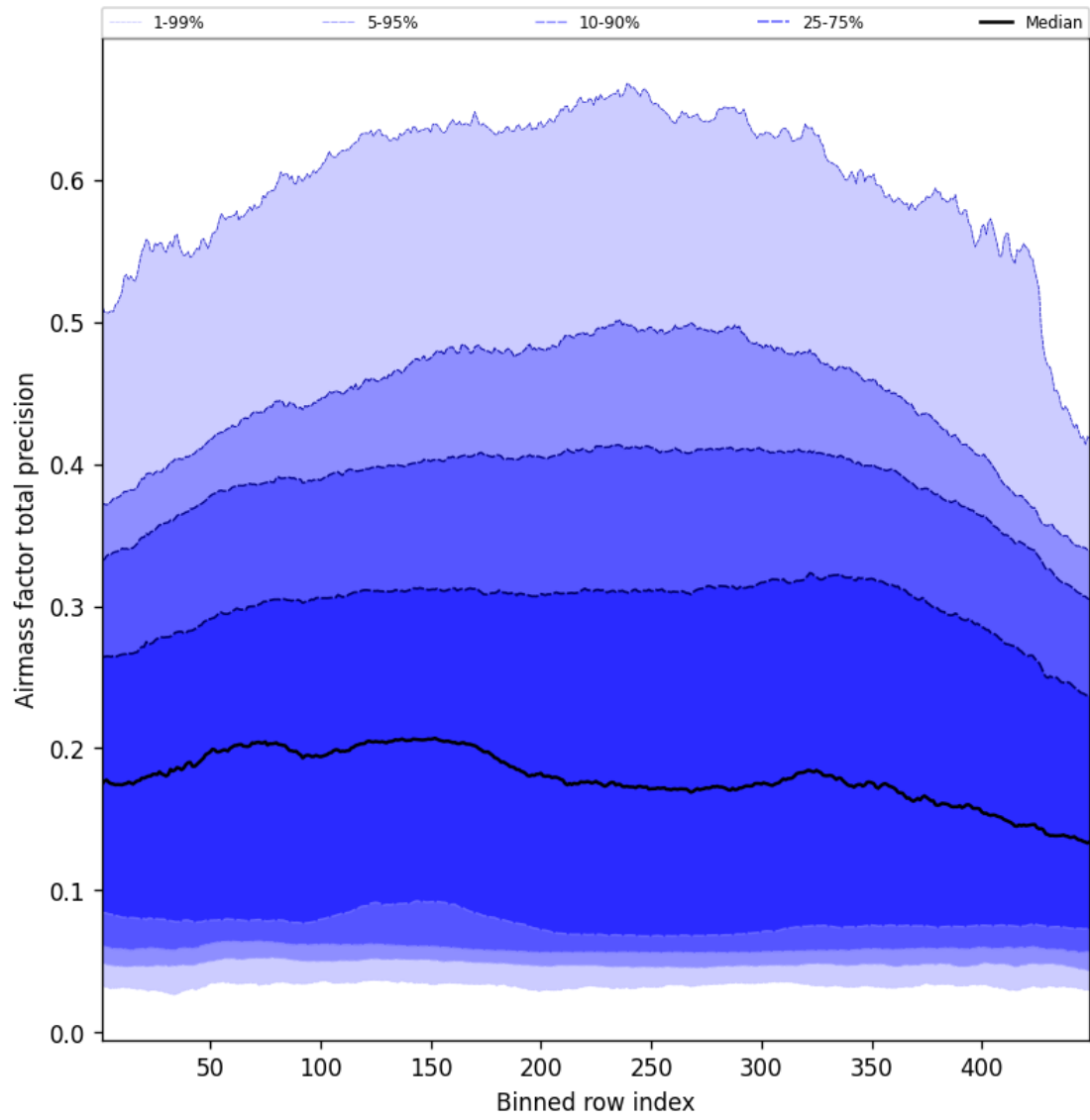
Figure 53: Along track statistics of “Airmass factor total precision” for 2024-12-24 to 2024-12-25
