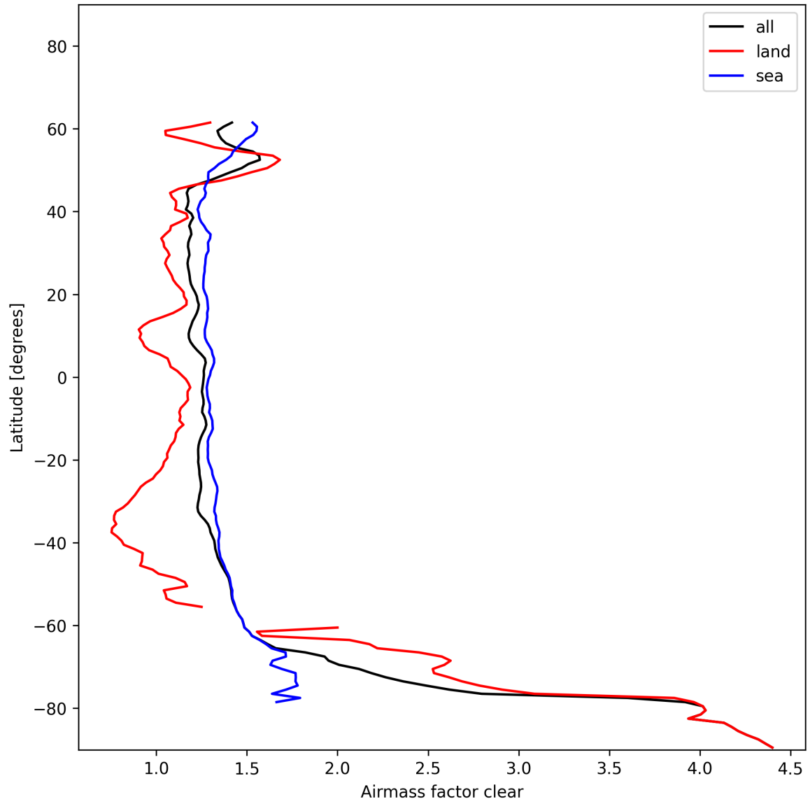
Figure 26: Zonal average of “Airmass factor clear” for 2024-12-25 to 2024-12-25.
