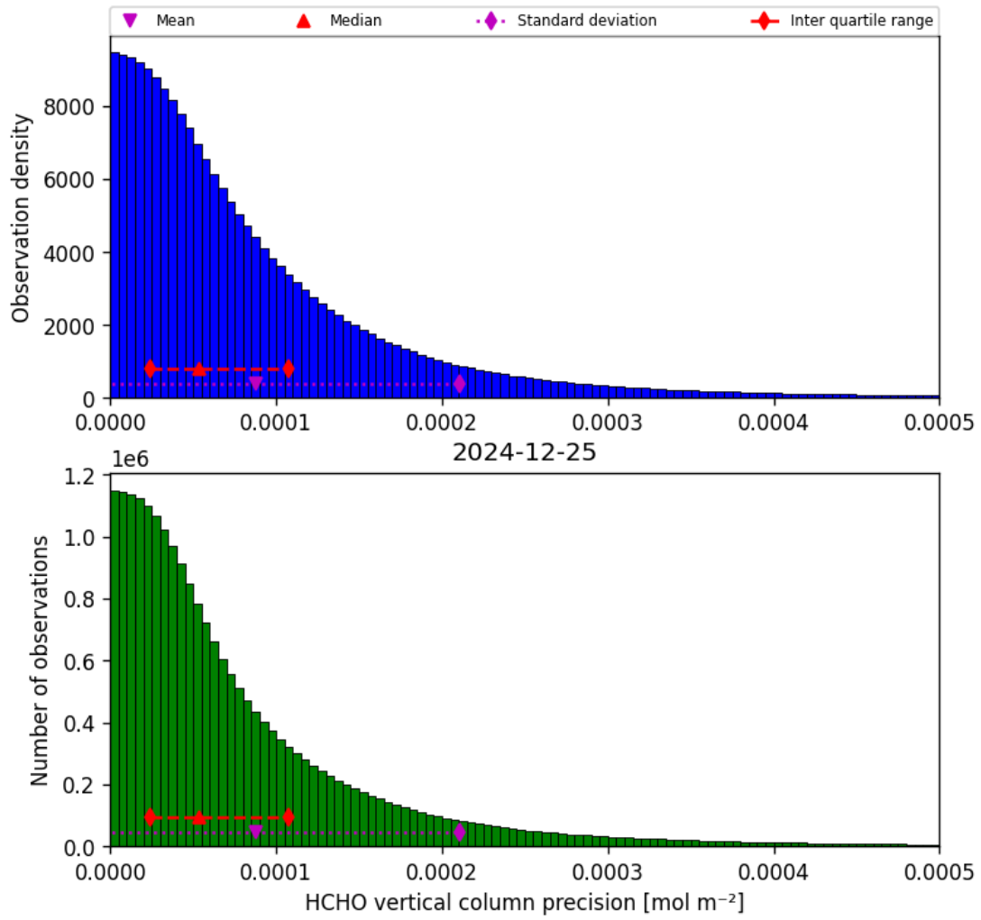
Figure 34: Histogram of “HCHO vertical column precision” for 2024-12-25 to 2024-12-25
