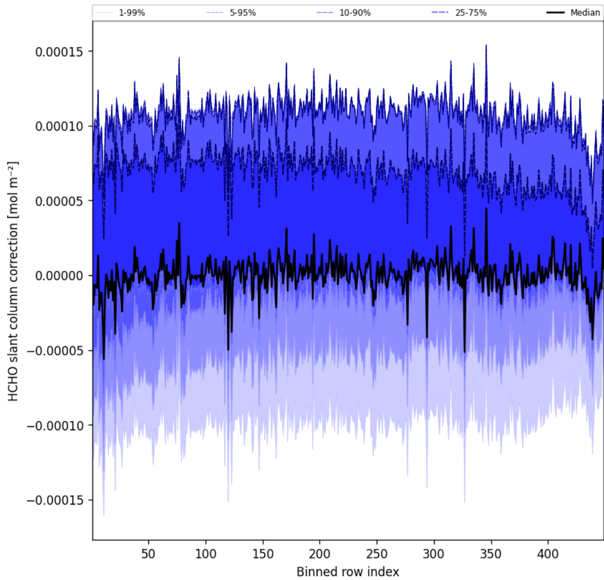
Figure 59: Along track statistics of “HCHO slant column correction” for 2024-12-25 to 2024-12-25
