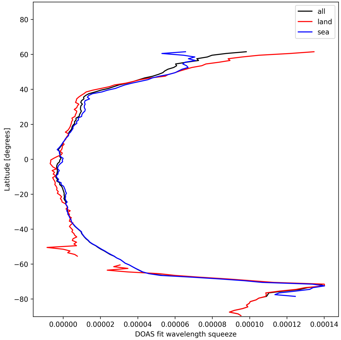
Figure 29: Zonal average of “DOAS fit wavelength squeeze” for 2024-12-25 to 2024-12-25.
