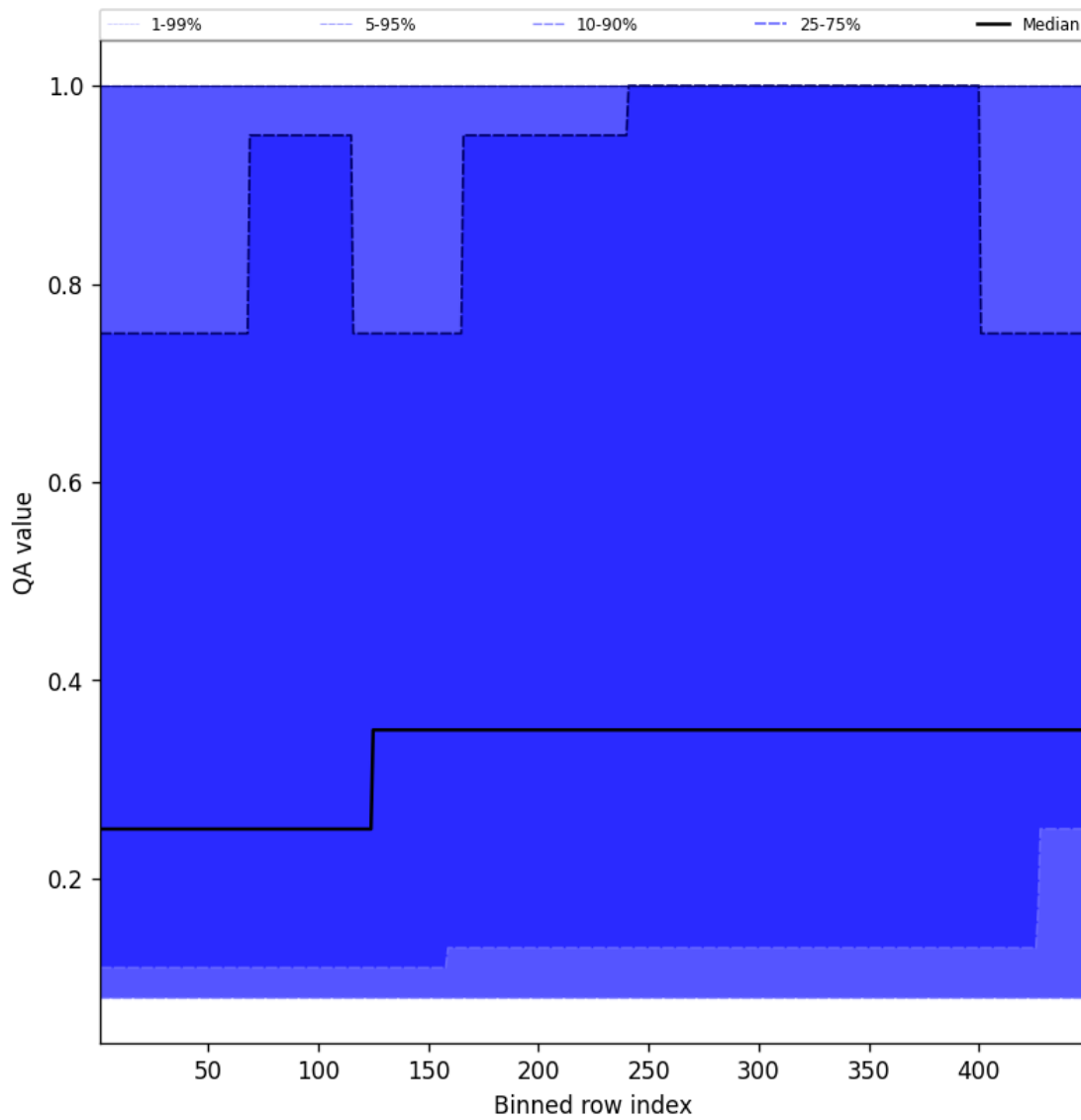
Figure 46: Along track statistics of “QA value” for 2024-12-25 to 2024-12-25
