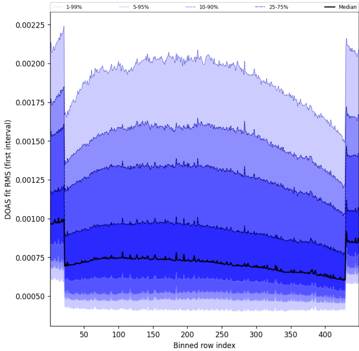
Figure 58: Along track statistics of “DOAS fit RMS (first interval)” for 2024-12-25 to 2024-12-25
