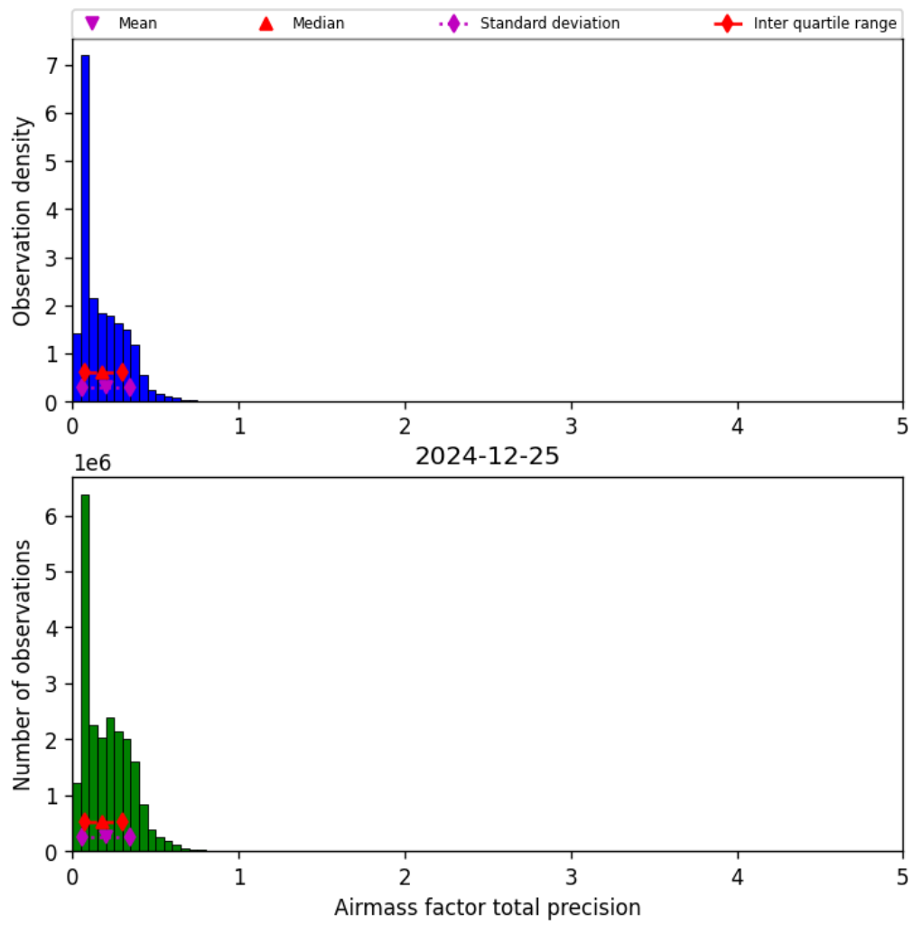
Figure 39: Histogram of “Airmass factor total precision” for 2024-12-25 to 2024-12-25
