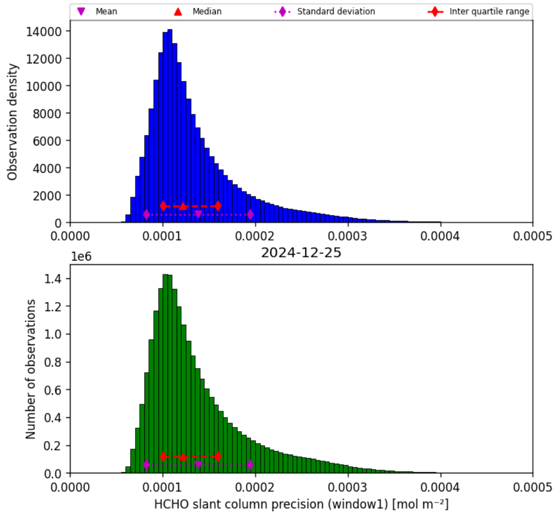
Figure 37: Histogram of “HCHO slant column precision (window1)” for 2024-12-25 to 2024-12-25
