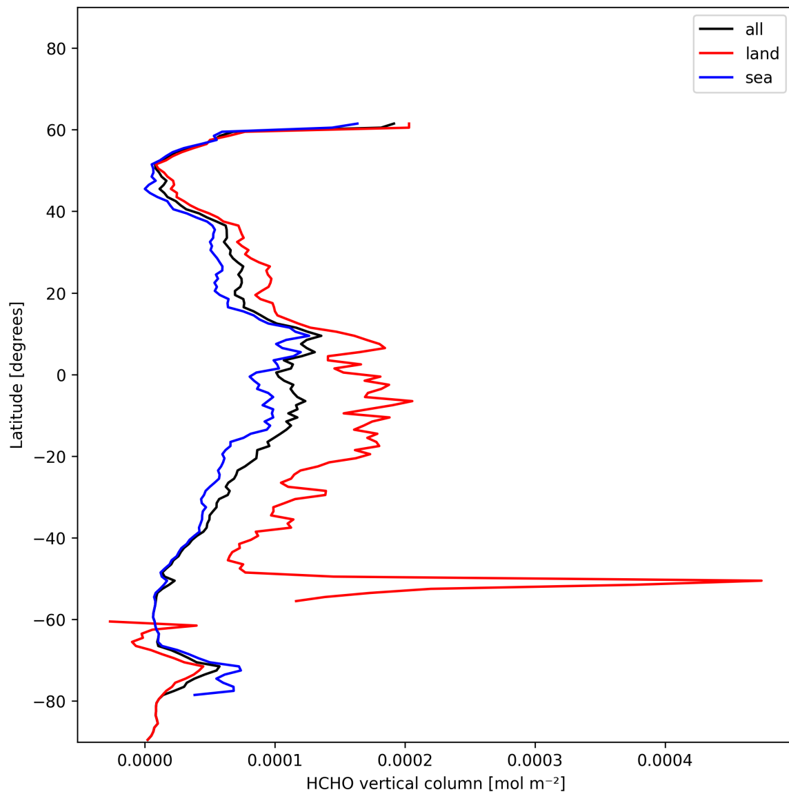
Figure 19: Zonal average of “HCHO vertical column” for 2024-12-25 to 2024-12-25.
