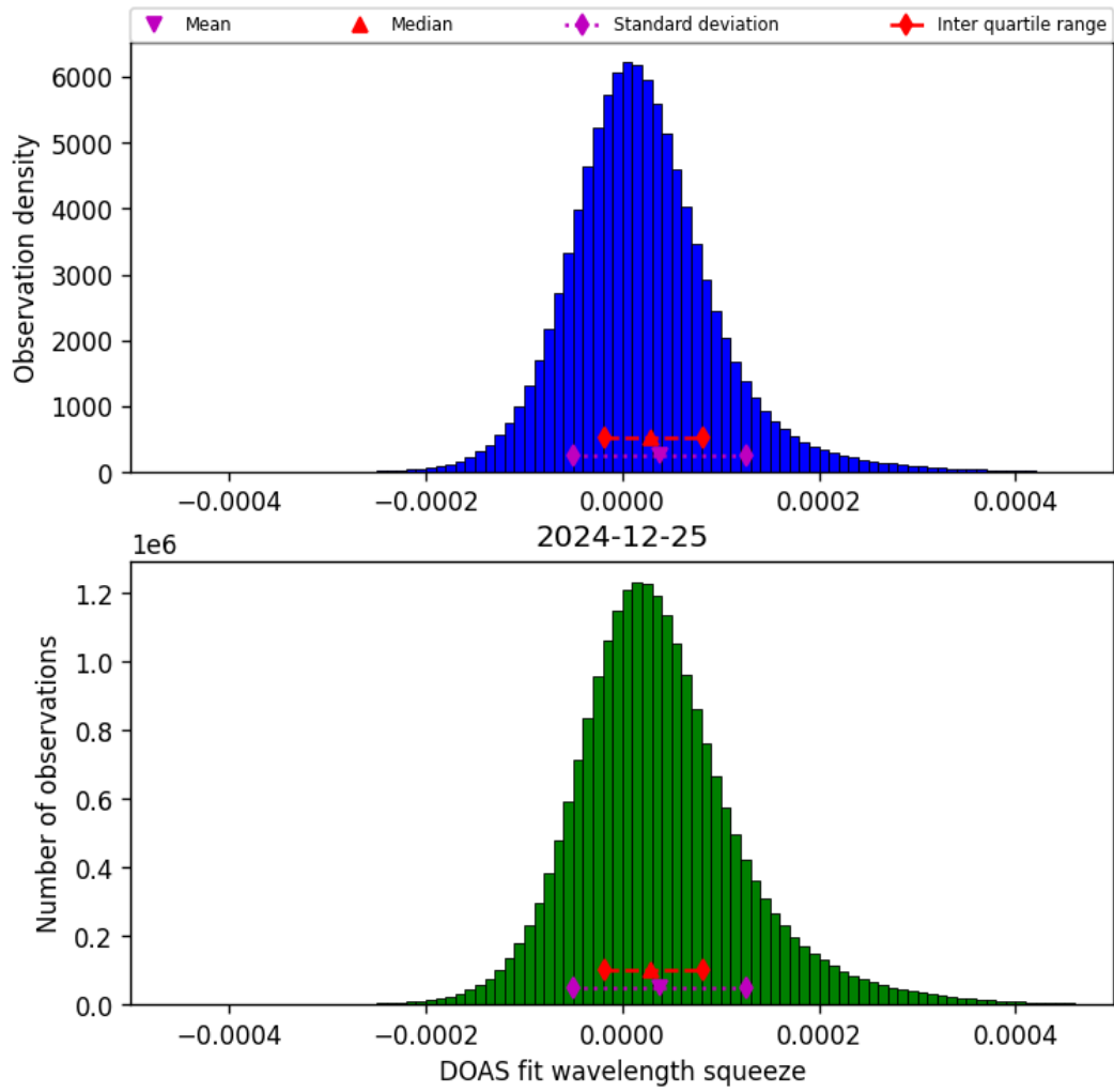
Figure 43: Histogram of “DOAS fit wavelength squeeze” for 2024-12-25 to 2024-12-25
