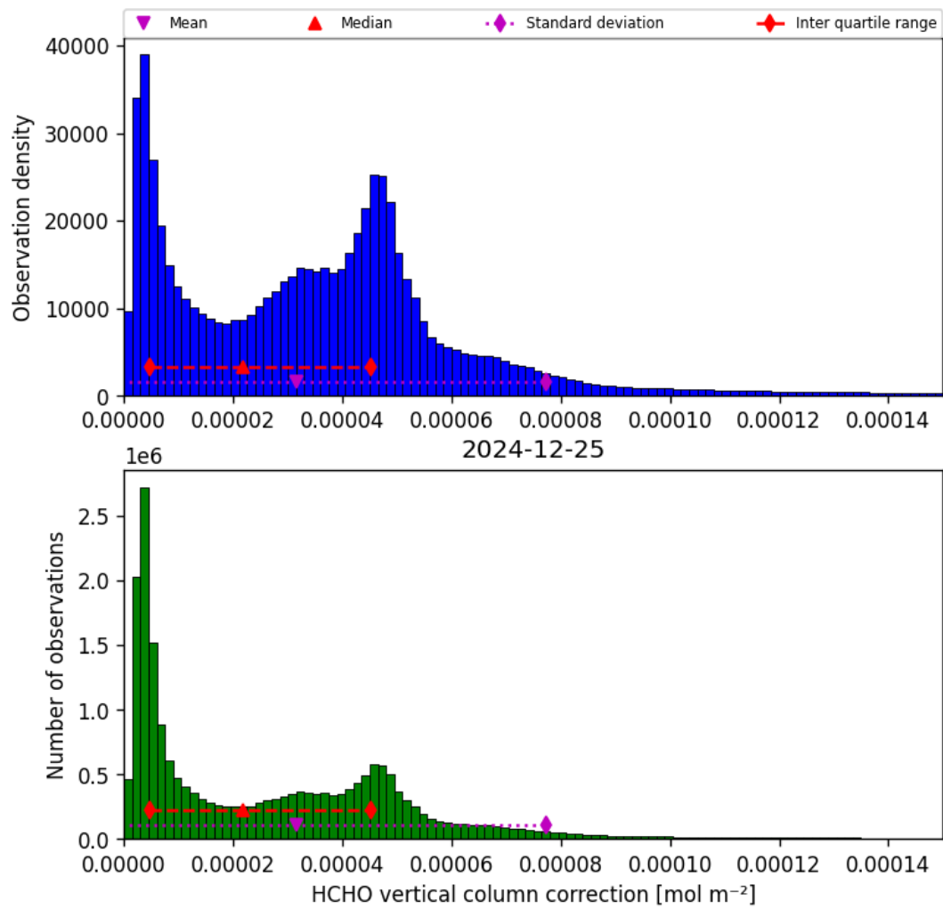
Figure 35: Histogram of “HCHO vertical column correction” for 2024-12-25 to 2024-12-25
