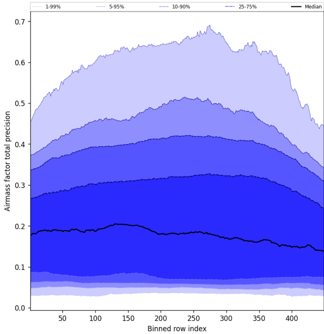
Figure 53: Along track statistics of “Airmass factor total precision” for 2024-12-25 to 2024-12-25
