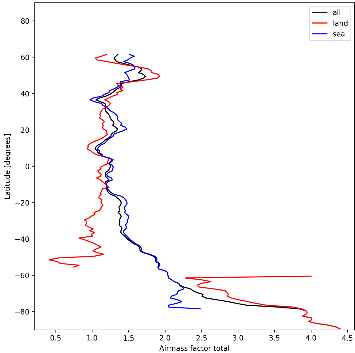
Figure 24: Zonal average of “Airmass factor total” for 2024-12-25 to 2024-12-25.
