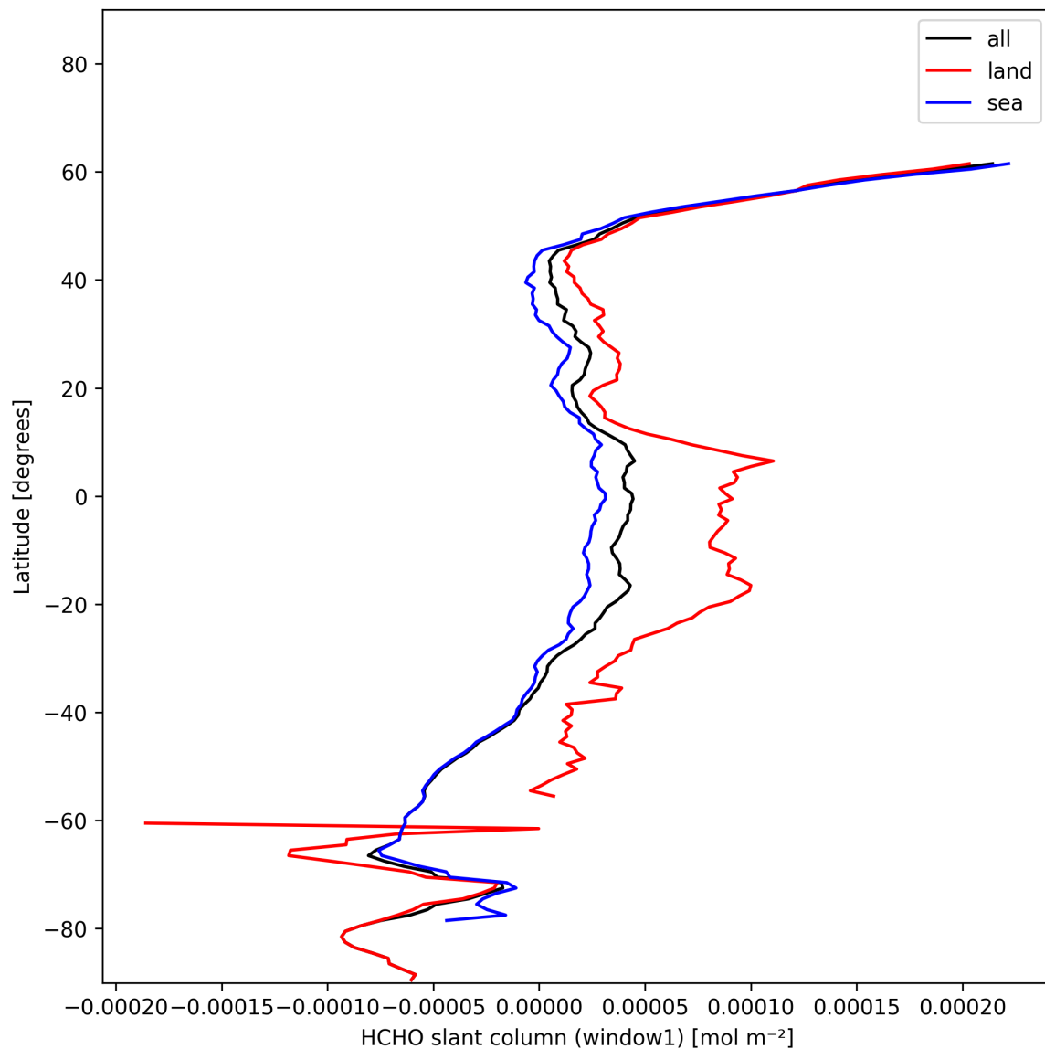
Figure 22: Zonal average of “HCHO slant column (window1)” for 2024-12-25 to 2024-12-25.
