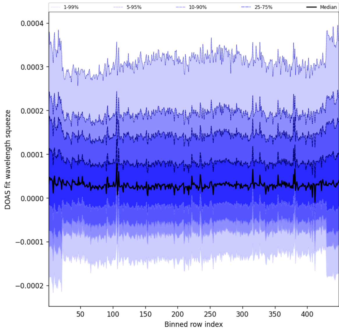
Figure 57: Along track statistics of “DOAS fit wavelength squeeze” for 2024-12-25 to 2024-12-25
