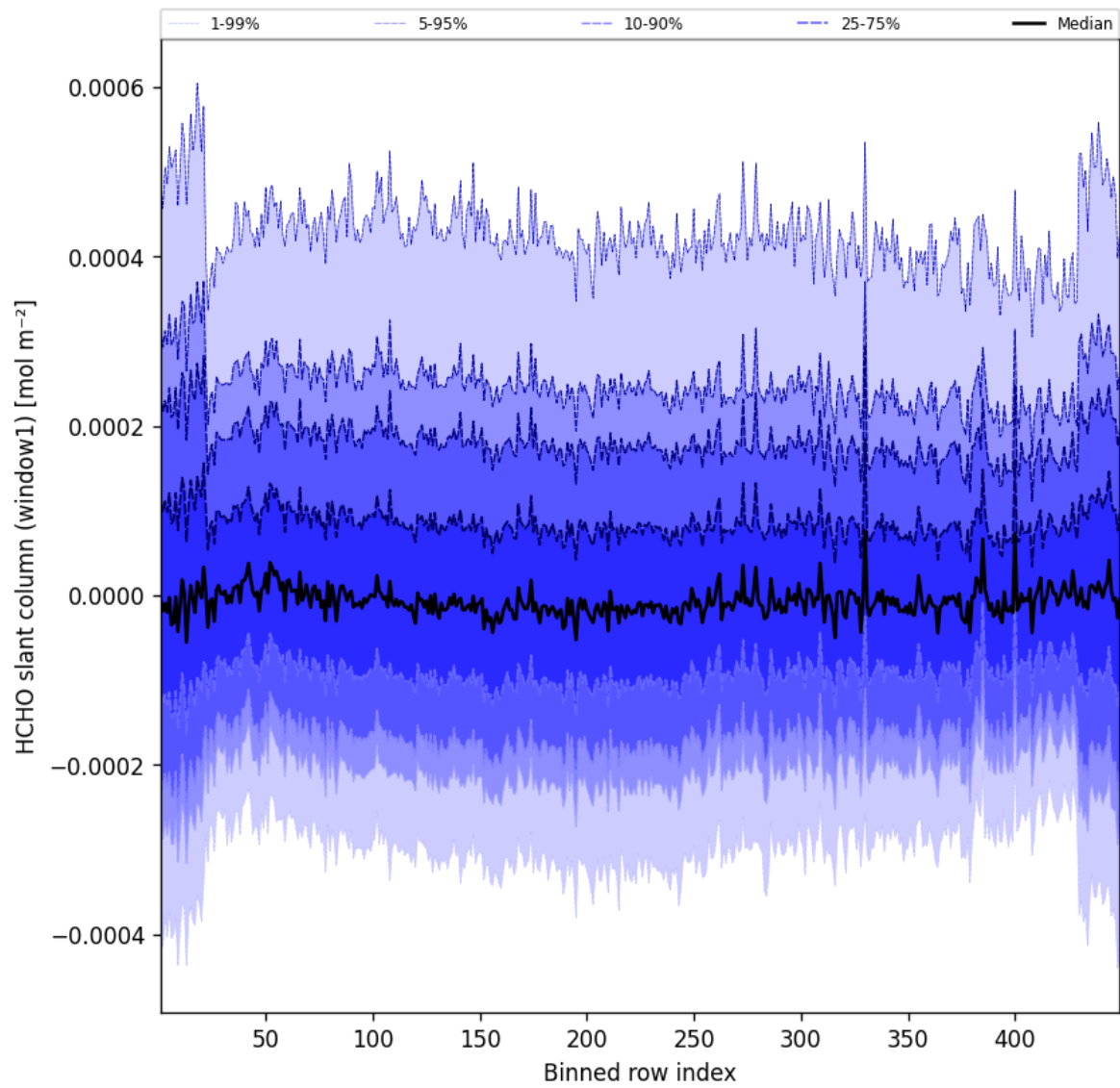
Figure 50: Along track statistics of "HCHO slant column (window1)" for 2024-12-25 to 2024-12-25
