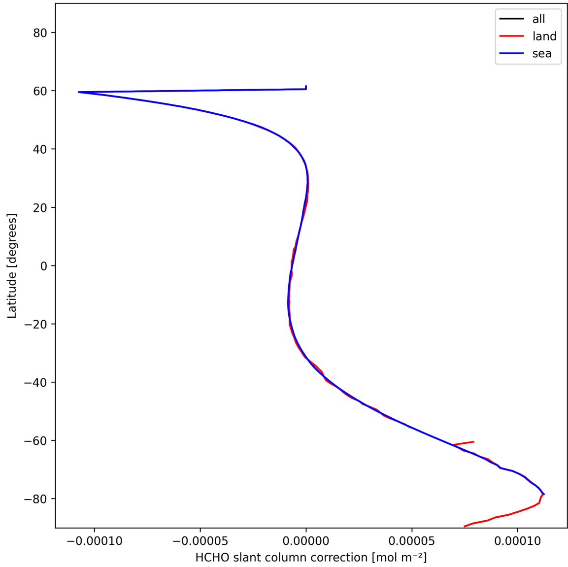
Figure 31: Zonal average of “HCHO slant column correction” for 2024-12-25 to 2024-12-25.
