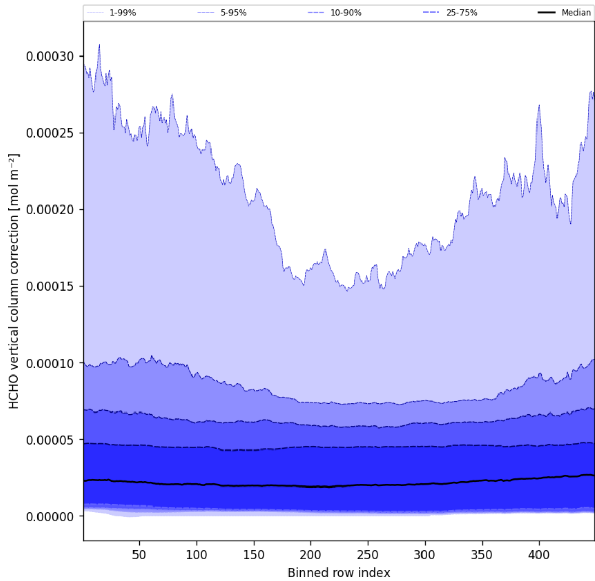
Figure 49: Along track statistics of “HCHO vertical column correction” for 2024-12-25 to 2024-12-25
