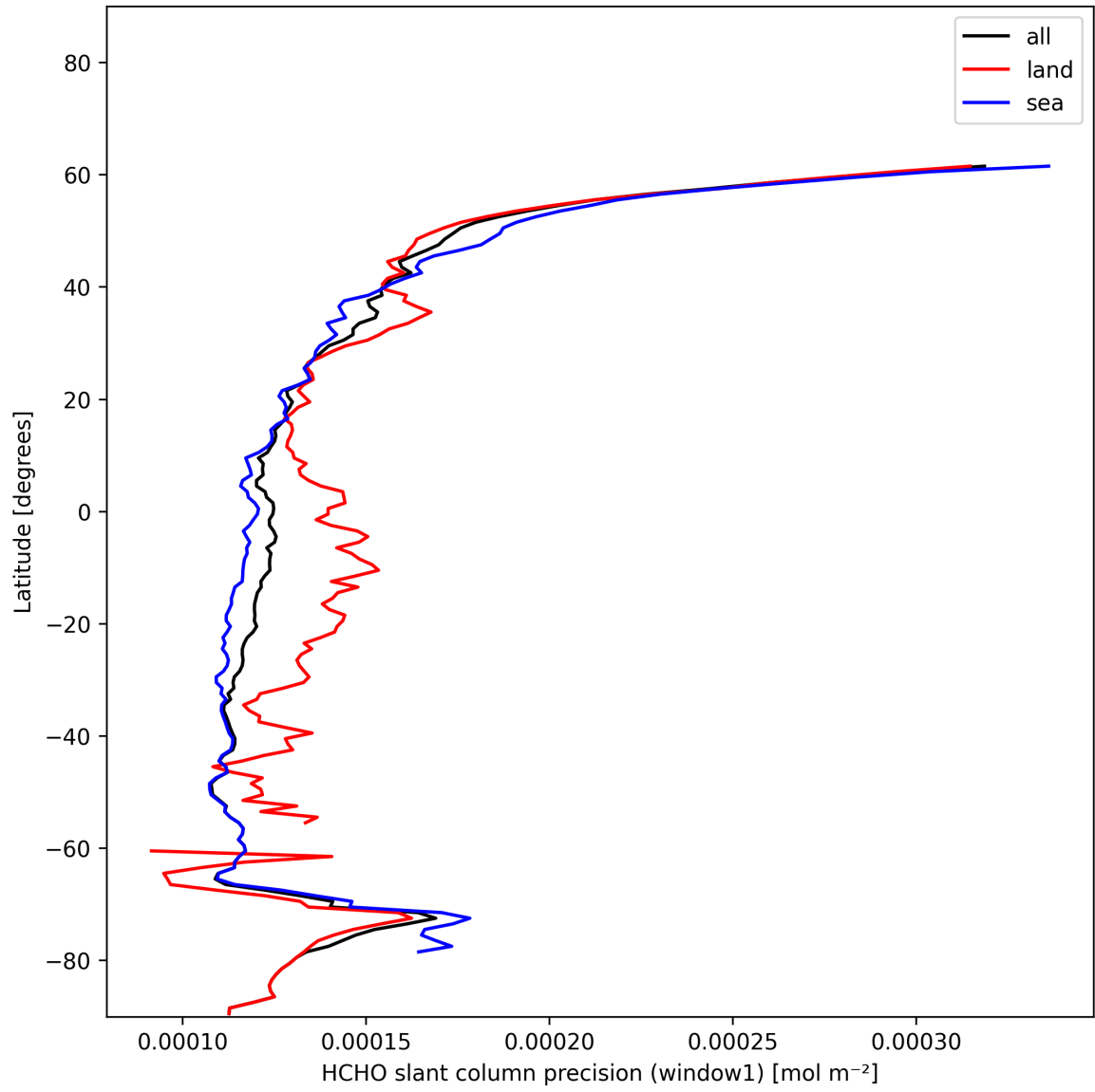
Figure 23: Zonal average of "HCHO slant column precision (window1)" for 2024-12-25 to 2024-12-25.
