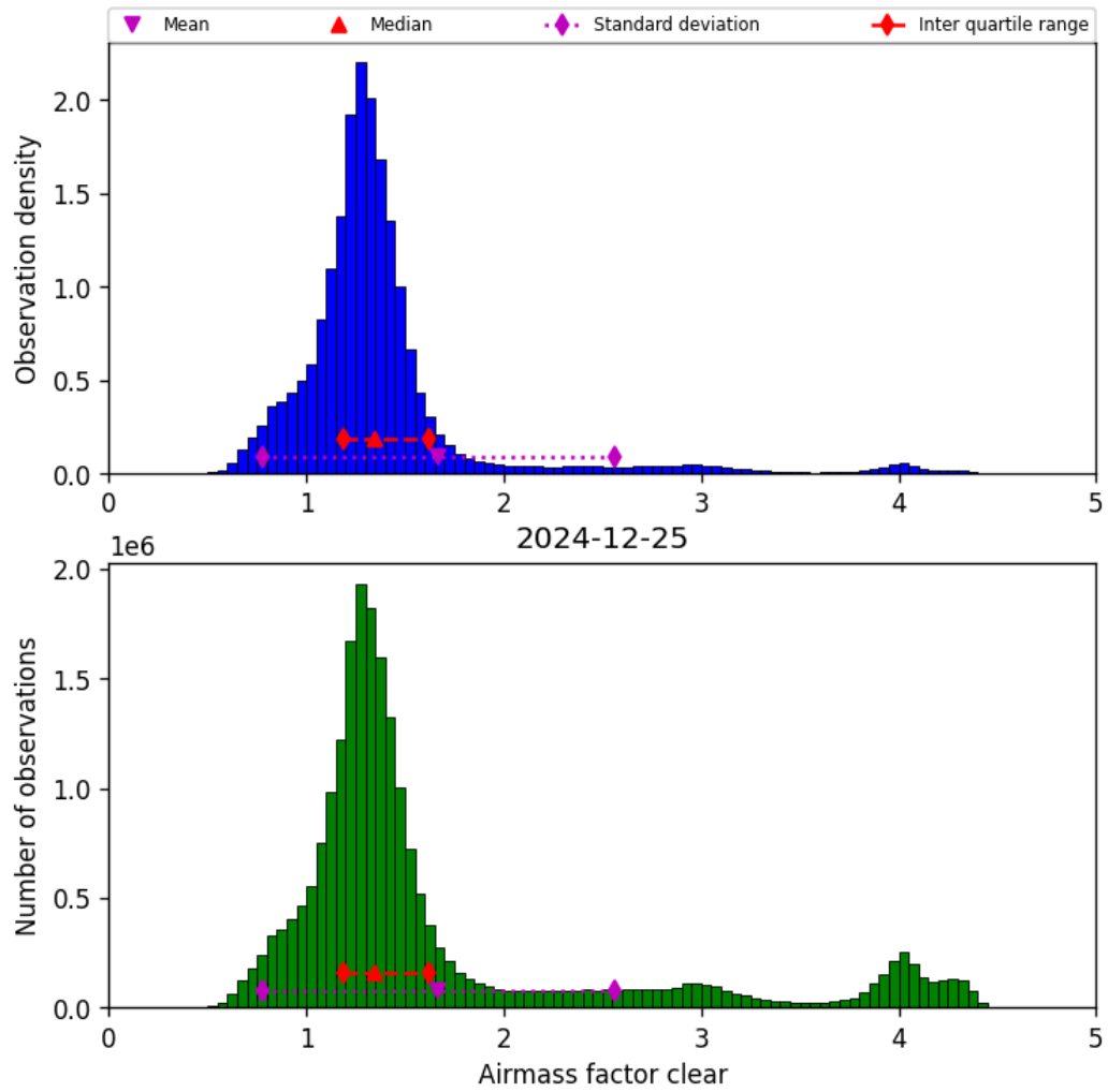
Figure 40: Histogram of “Airmass factor clear” for 2024-12-25 to 2024-12-25
