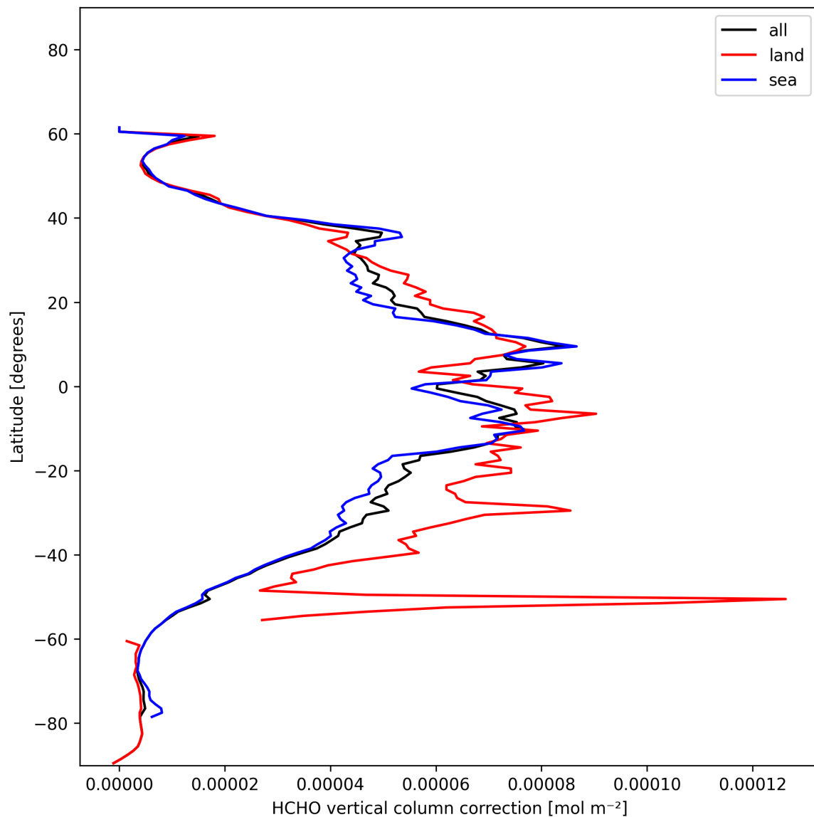
Figure 21: Zonal average of “HCHO vertical column correction” for 2024-12-25 to 2024-12-25.
