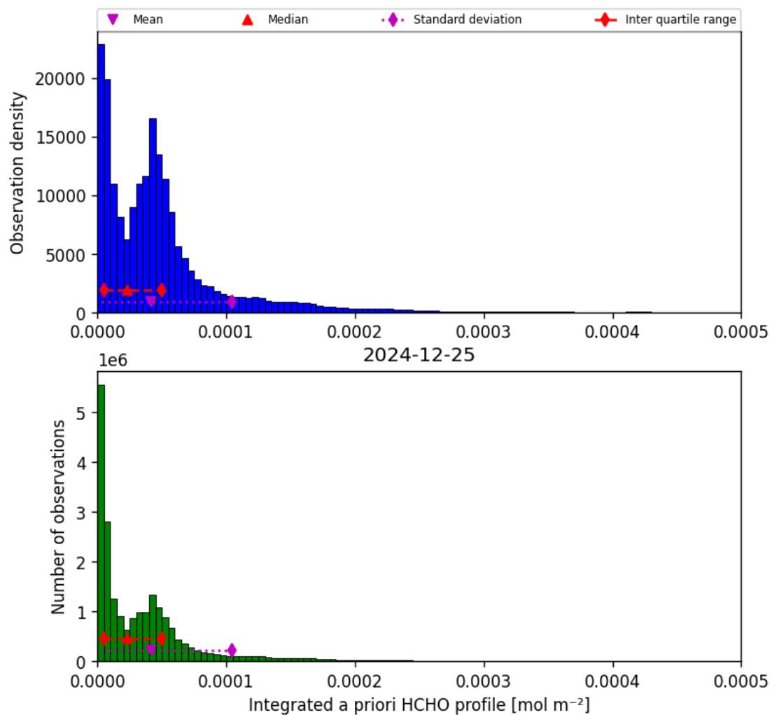
Figure 41: Histogram of “Integrated a priori HCHO profile” for 2024-12-25 to 2024-12-25
