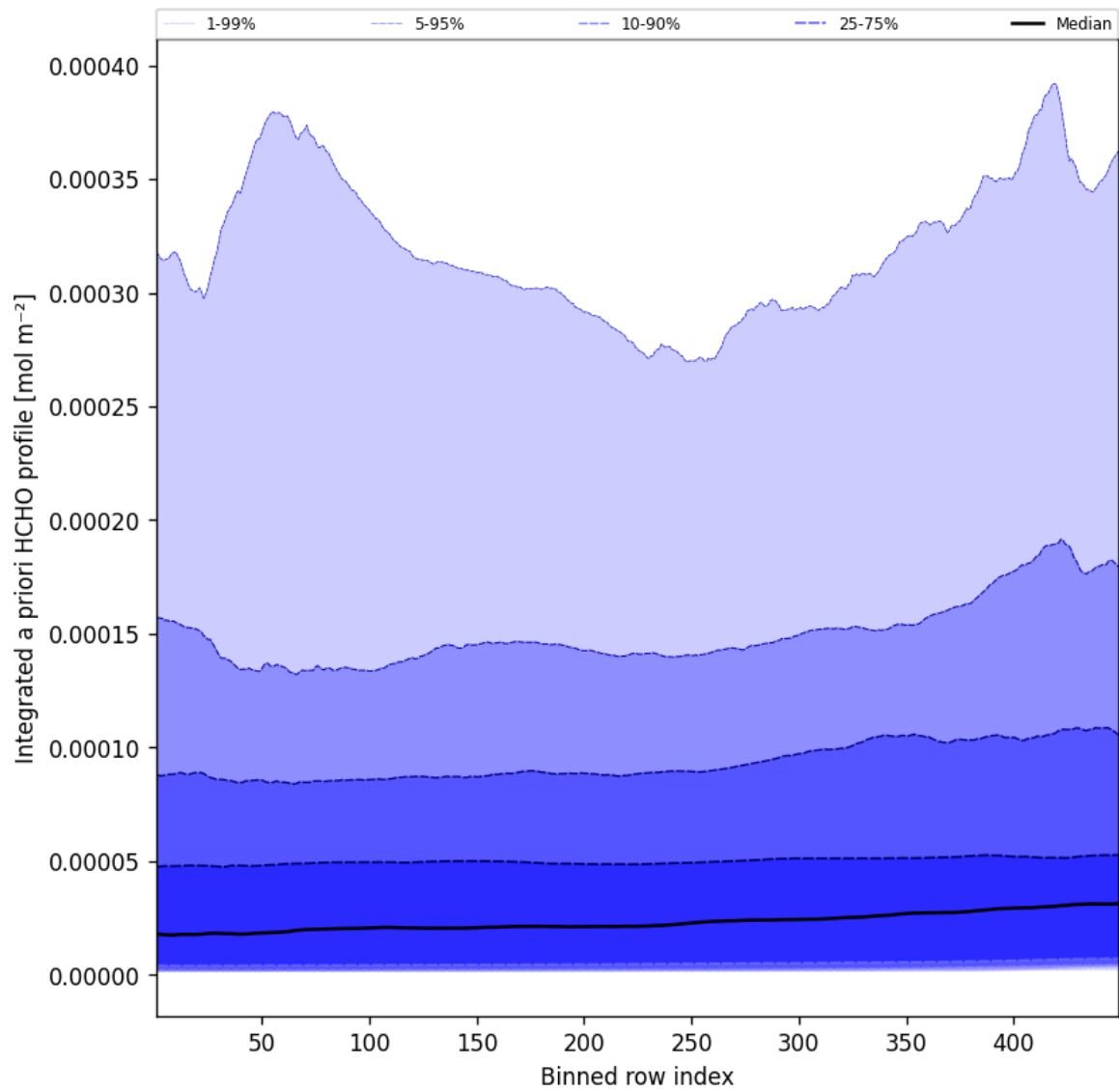
Figure 55: Along track statistics of "Integrated a priori HCHO profile" for 2024-12-25 to 2024-12-25
