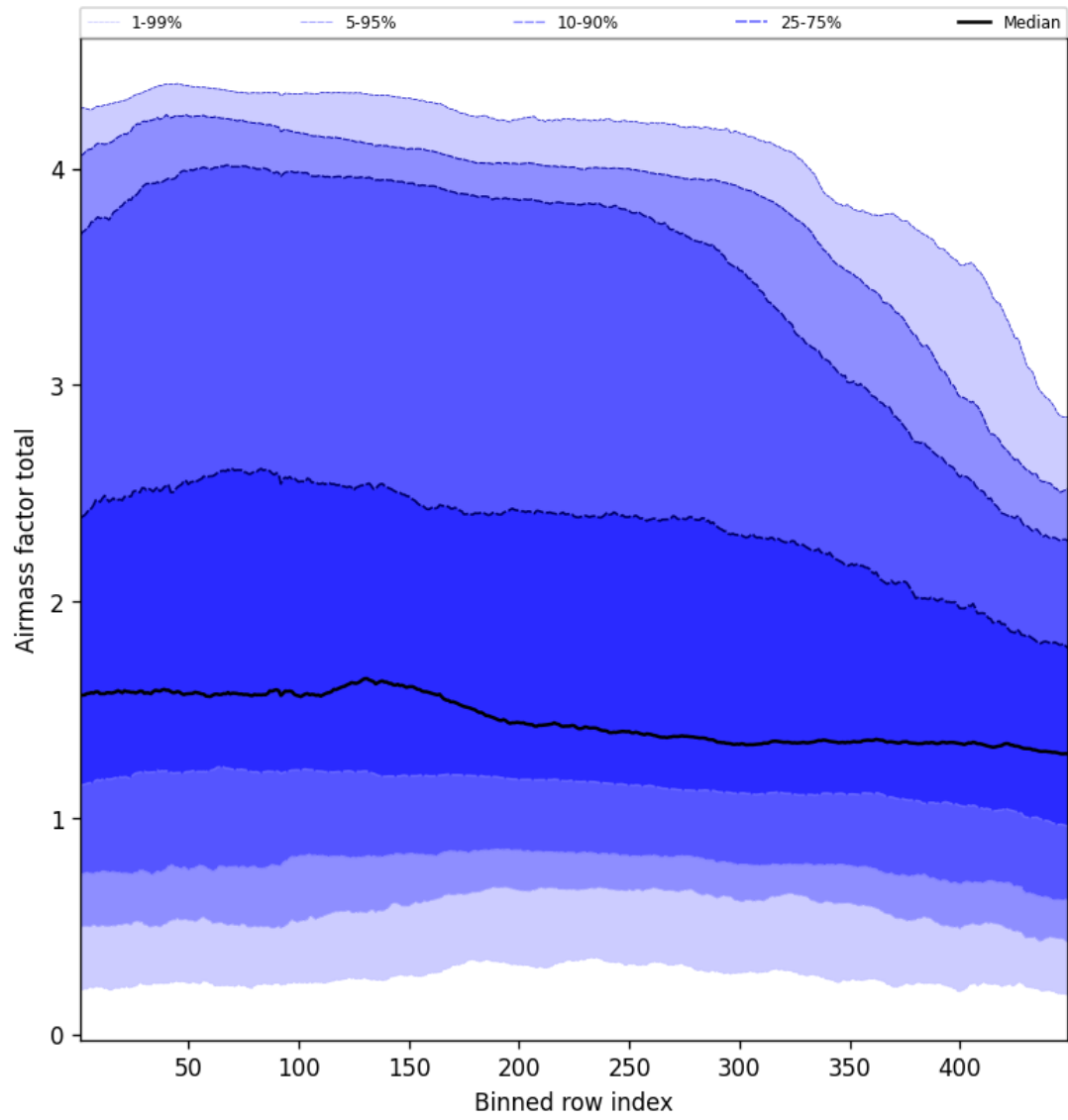
Figure 52: Along track statistics of “Airmass factor total” for 2024-12-25 to 2024-12-25
