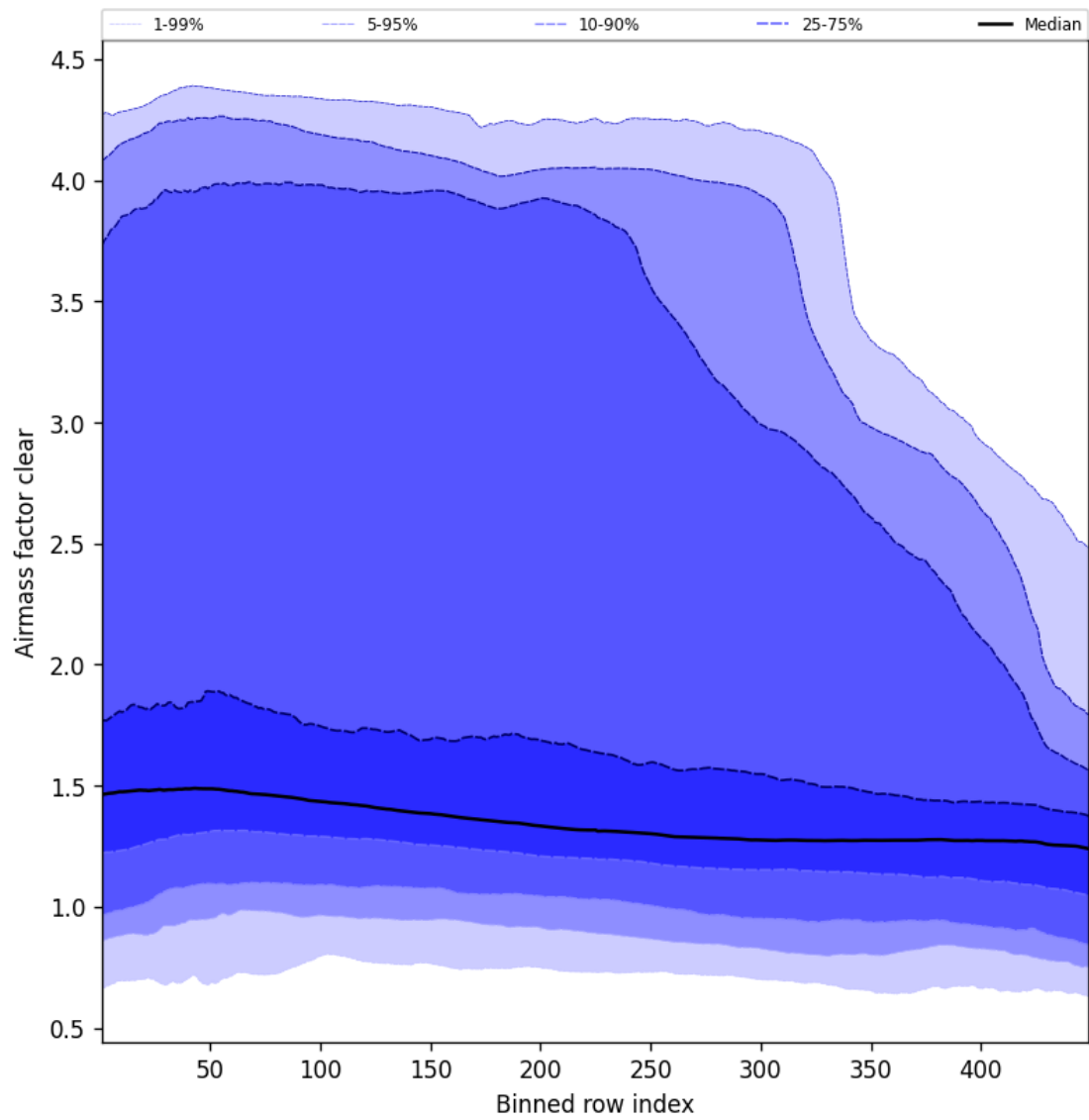
Figure 54: Along track statistics of “Air mass factor clear” for 2024-12-25 to 2024-12-25
