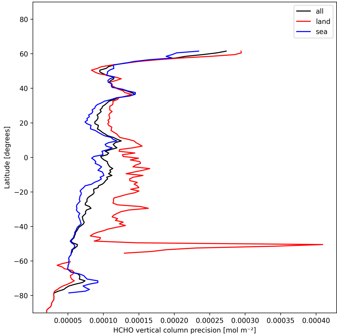
Figure 20: Zonal average of “HCHO vertical column precision” for 2024-12-25 to 2024-12-25.
