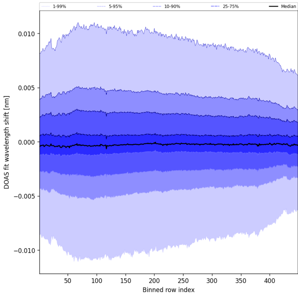
Figure 56: Along track statistics of “DOAS fit wavelength shift” for 2024-12-25 to 2024-12-25
