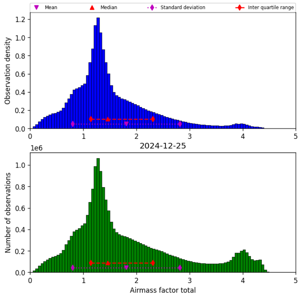
Figure 38: Histogram of “Airmass factor total” for 2024-12-25 to 2024-12-25
