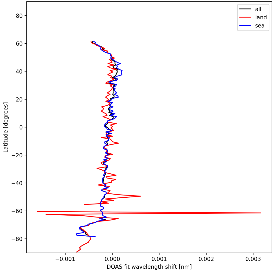
Figure 28: Zonal average of "DOAS fit wavelength shift" for 2024-12-25 to 2024-12-25.
