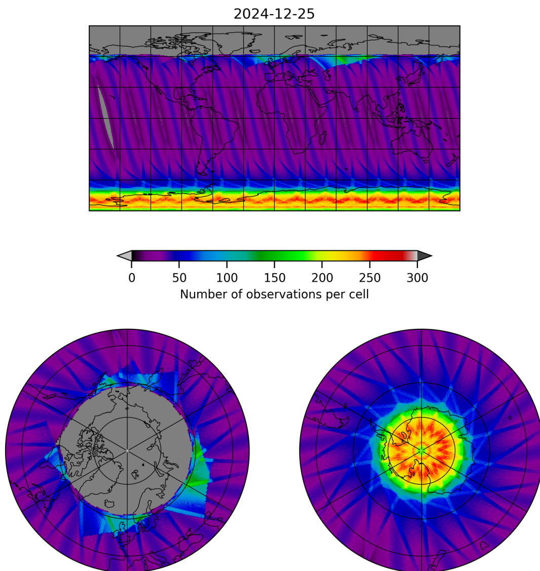
Figure 17: Map of the number of observations for 2024-12-25 to 2024-12-25
