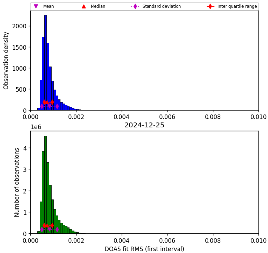
Figure 44: Histogram of “DOAS fit RMS (first interval)” for 2024-12-25 to 2024-12-25
