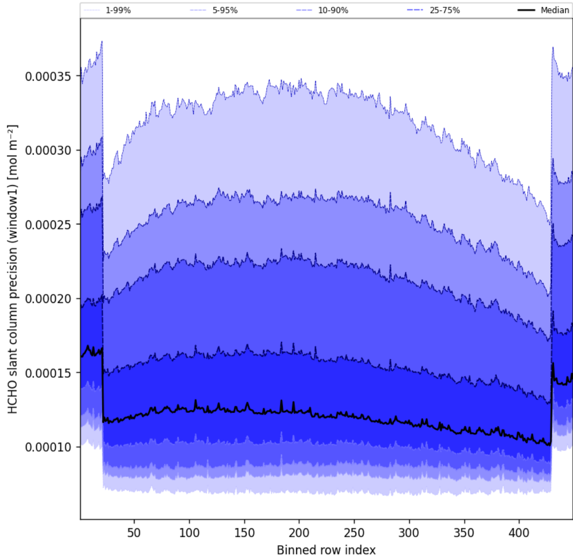
Figure 51: Along track statistics of “HCHO slant column precision (window1)” for 2024-12-25 to 2024-12-25
