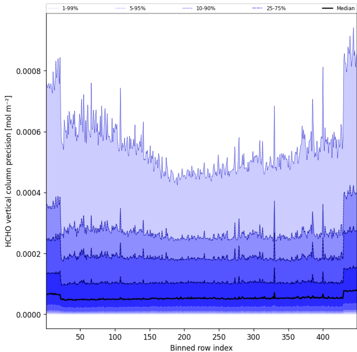
Figure 48: Along track statistics of "HCHO vertical column precision" for 2024-12-25 to 2024-12-25
