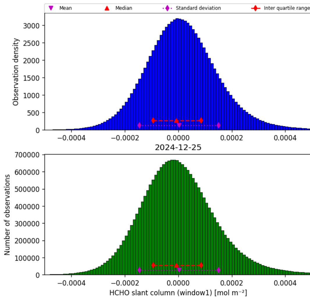
Figure 36: Histogram of “HCHO slant column (window1)” for 2024-12-25 to 2024-12-25
