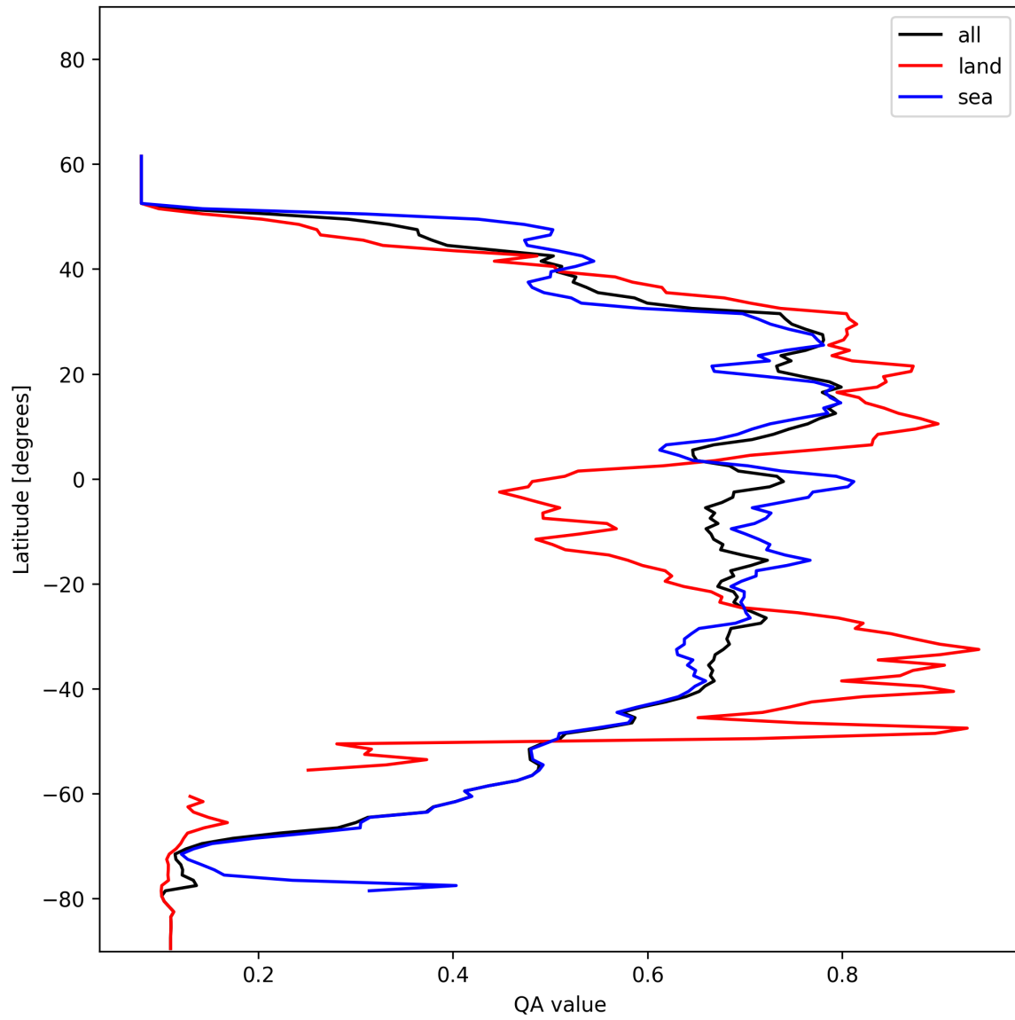
Figure 18: Zonal average of “QA value” for 2024-12-25 to 2024-12-25.
