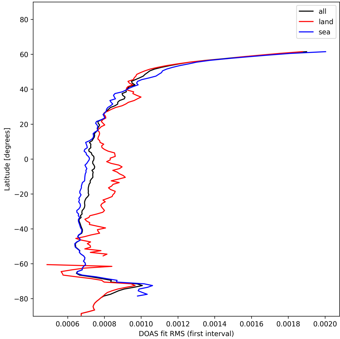
Figure 30: Zonal average of “DOAS fit RMS (first interval)” for 2024-12-25 to 2024-12-25.
