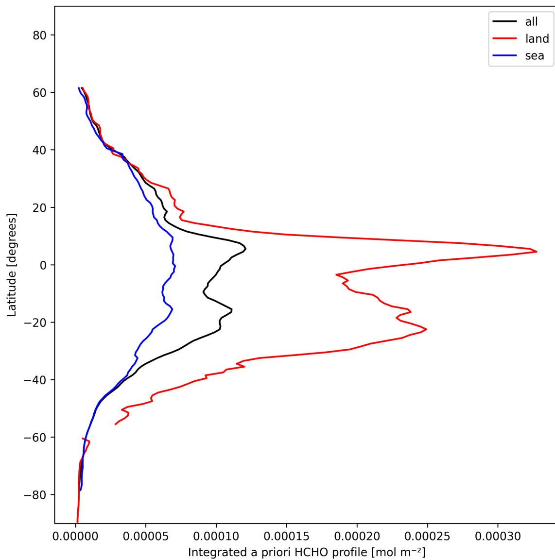
Figure 27: Zonal average of “Integrated a priori HCHO profile” for 2024-12-25 to 2024-12-25.
