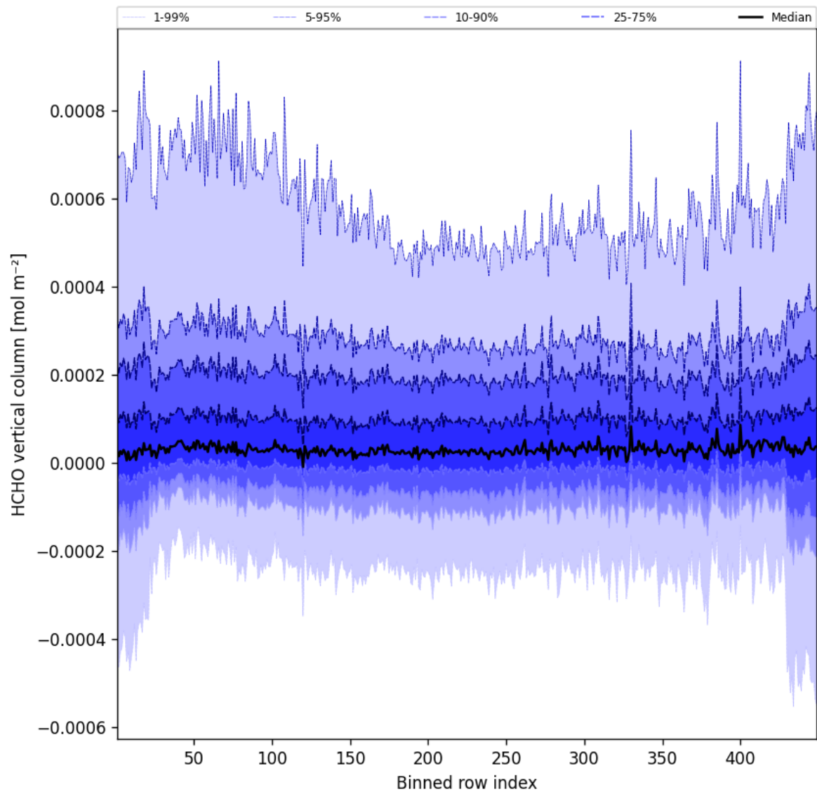
Figure 47: Along track statistics of “HCHO vertical column” for 2024-12-25 to 2024-12-25
