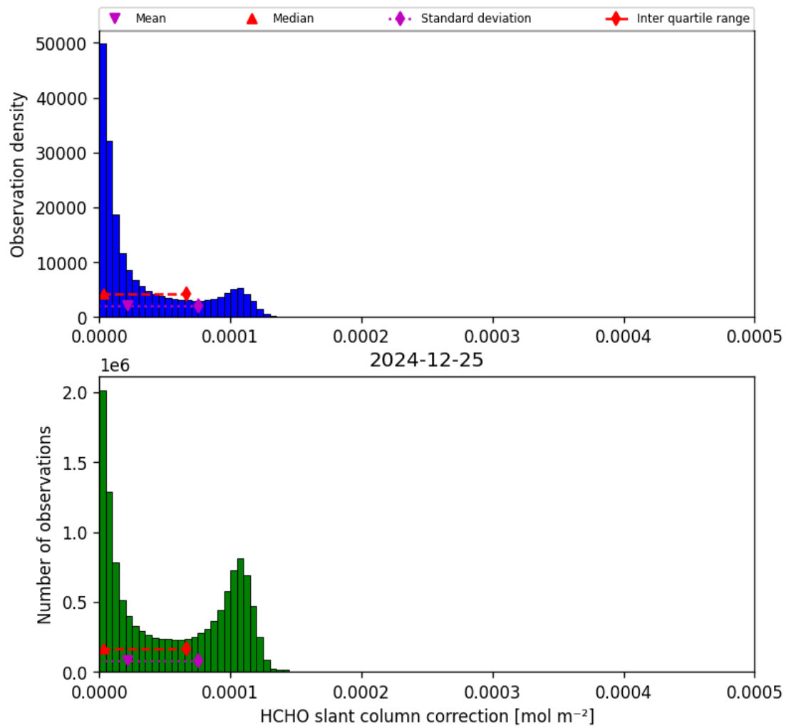
Figure 45: Histogram of “HCHO slant column correction” for 2024-12-25 to 2024-12-25
