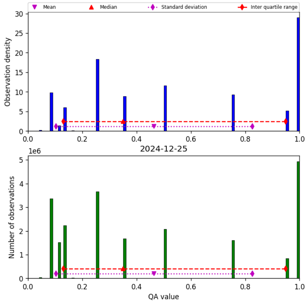
Figure 32: Histogram of “QA value” for 2024-12-25 to 2024-12-25
