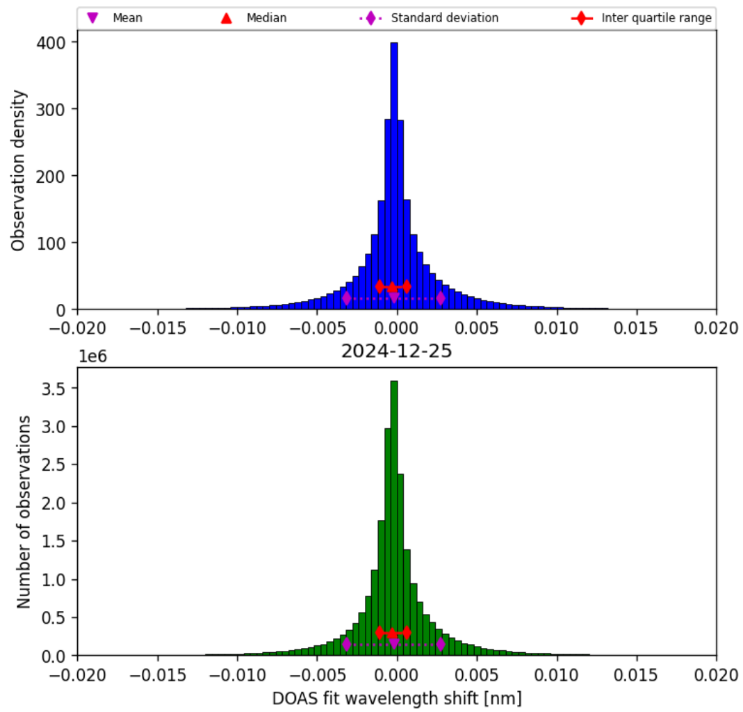
Figure 42: Histogram of “DOAS fit wavelength shift” for 2024-12-25 to 2024-12-25
