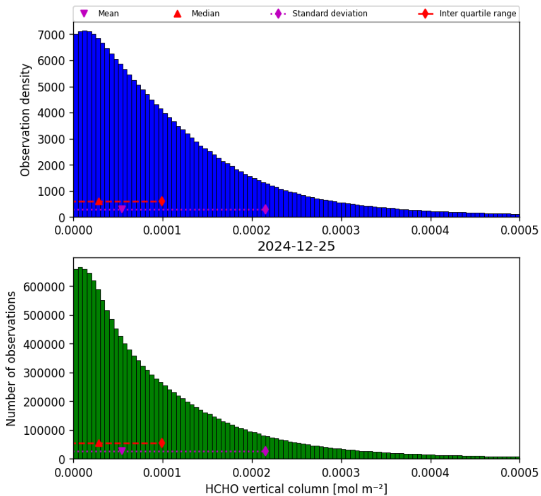
Figure 33: Histogram of “HCHO vertical column” for 2024-12-25 to 2024-12-25
