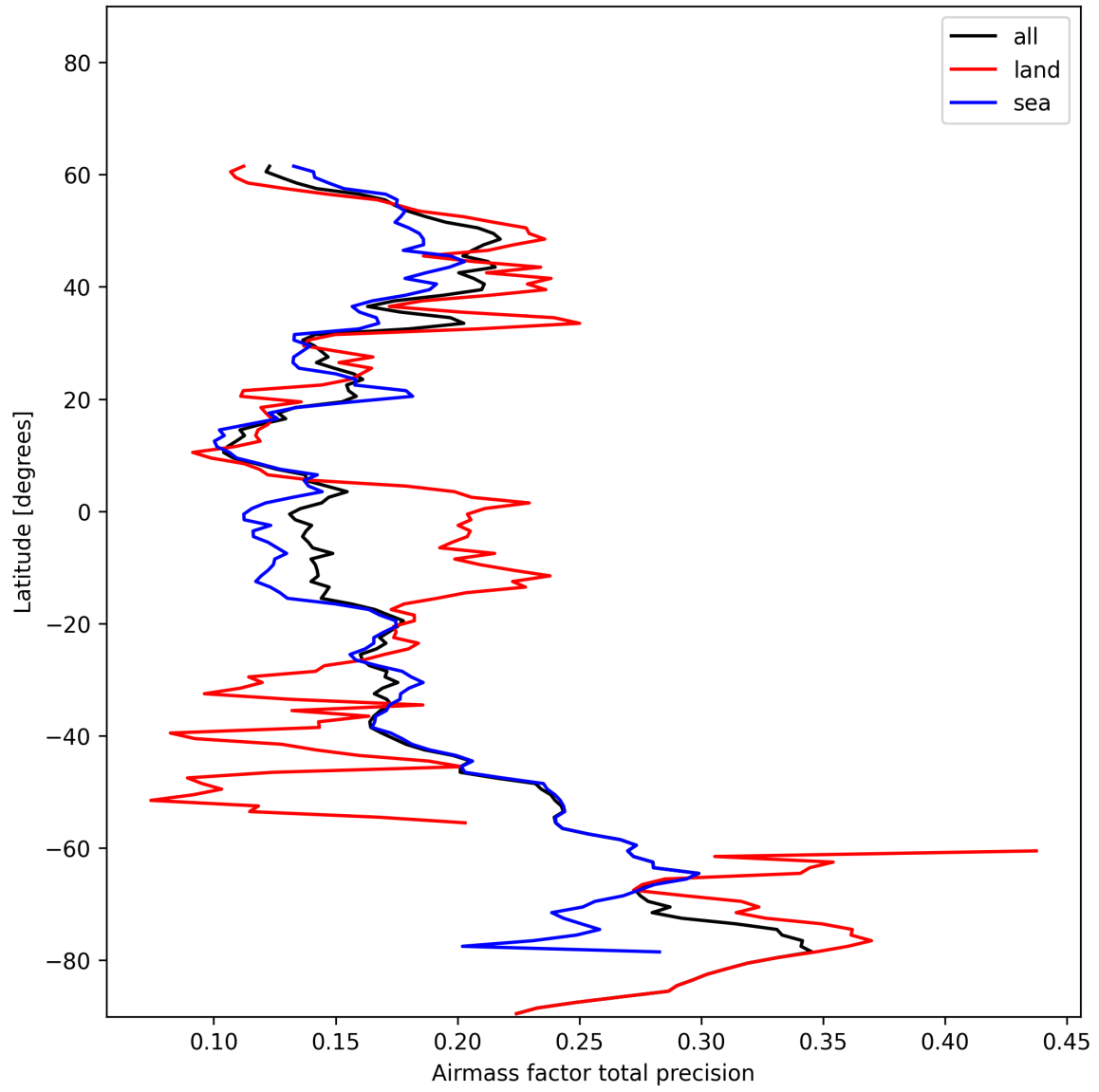
Figure 25: Zonal average of “Airmass factor total precision” for 2024-12-25 to 2024-12-25.
