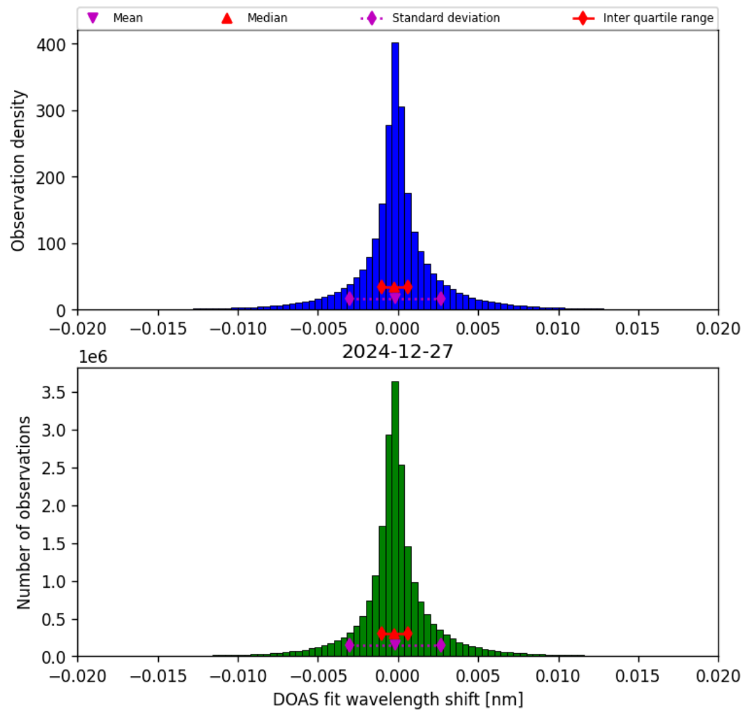
Figure 42: Histogram of “DOAS fit wavelength shift” for 2024-12-27 to 2024-12-28
