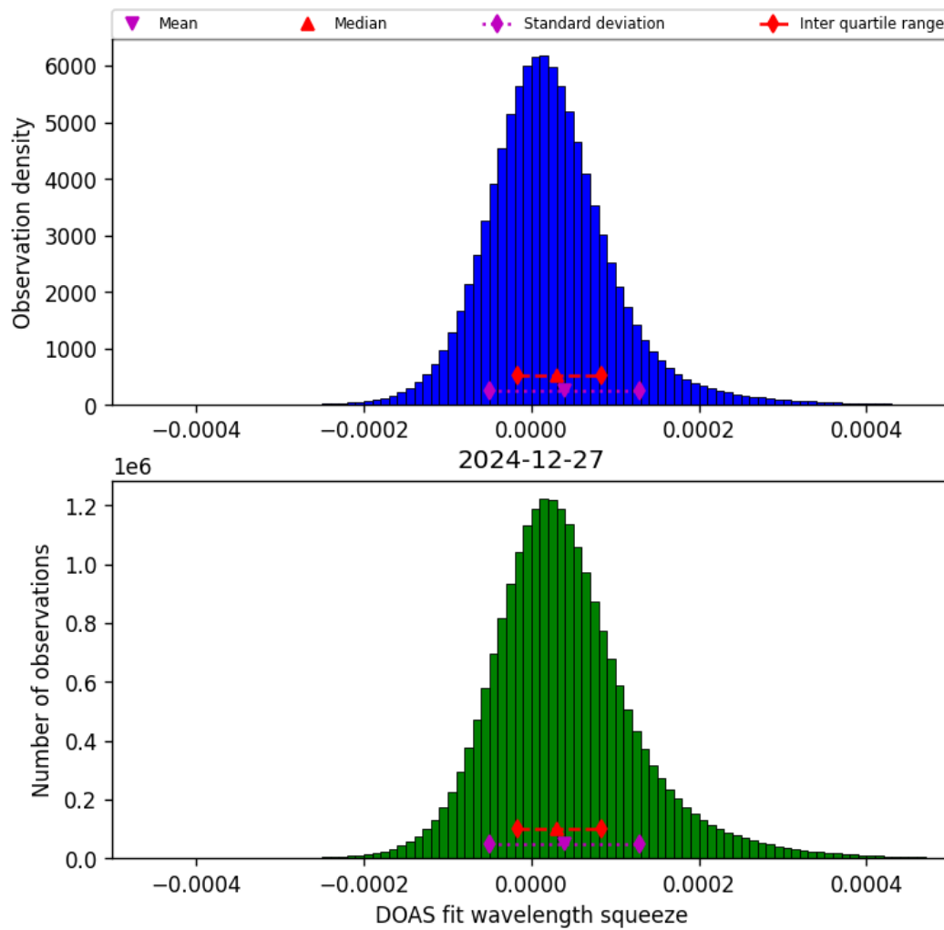
Figure 43: Histogram of “DOAS fit wavelength squeeze” for 2024-12-27 to 2024-12-28
