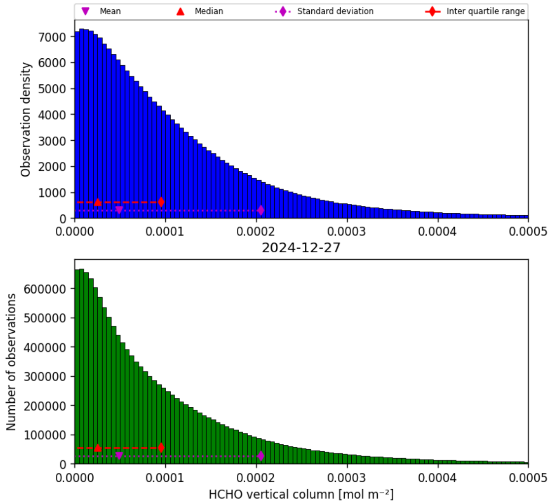
Figure 33: Histogram of “HCHO vertical column” for 2024-12-27 to 2024-12-28
