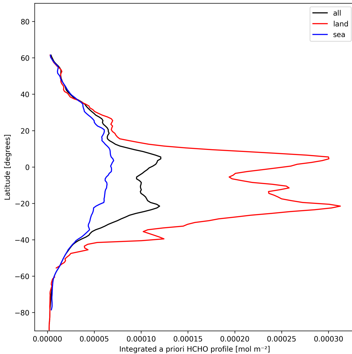
Figure 27: Zonal average of “Integrated a priori HCHO profile” for 2024-12-27 to 2024-12-28.
