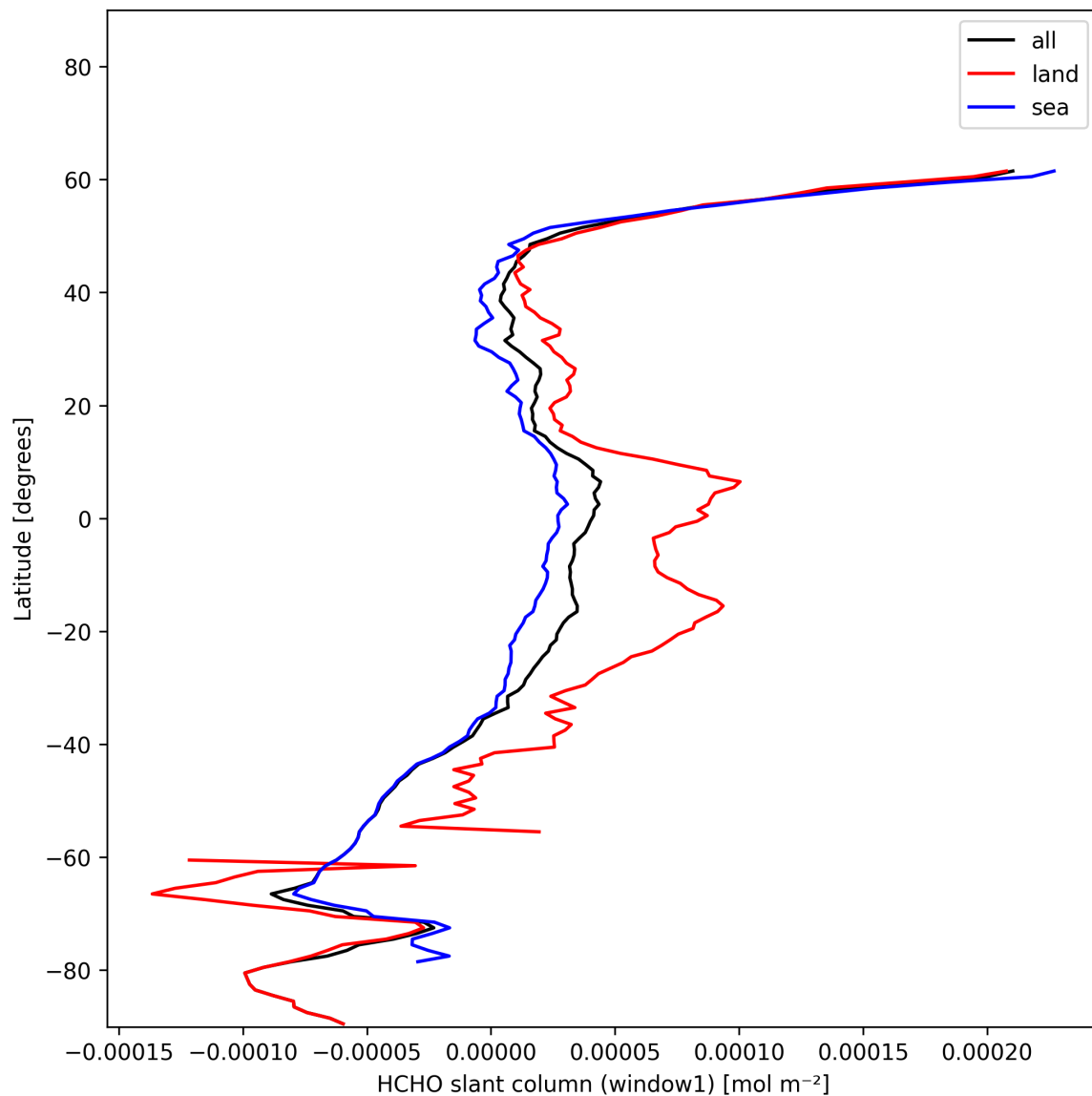
Figure 22: Zonal average of “HCHO slant column (window1)” for 2024-12-27 to 2024-12-28.
