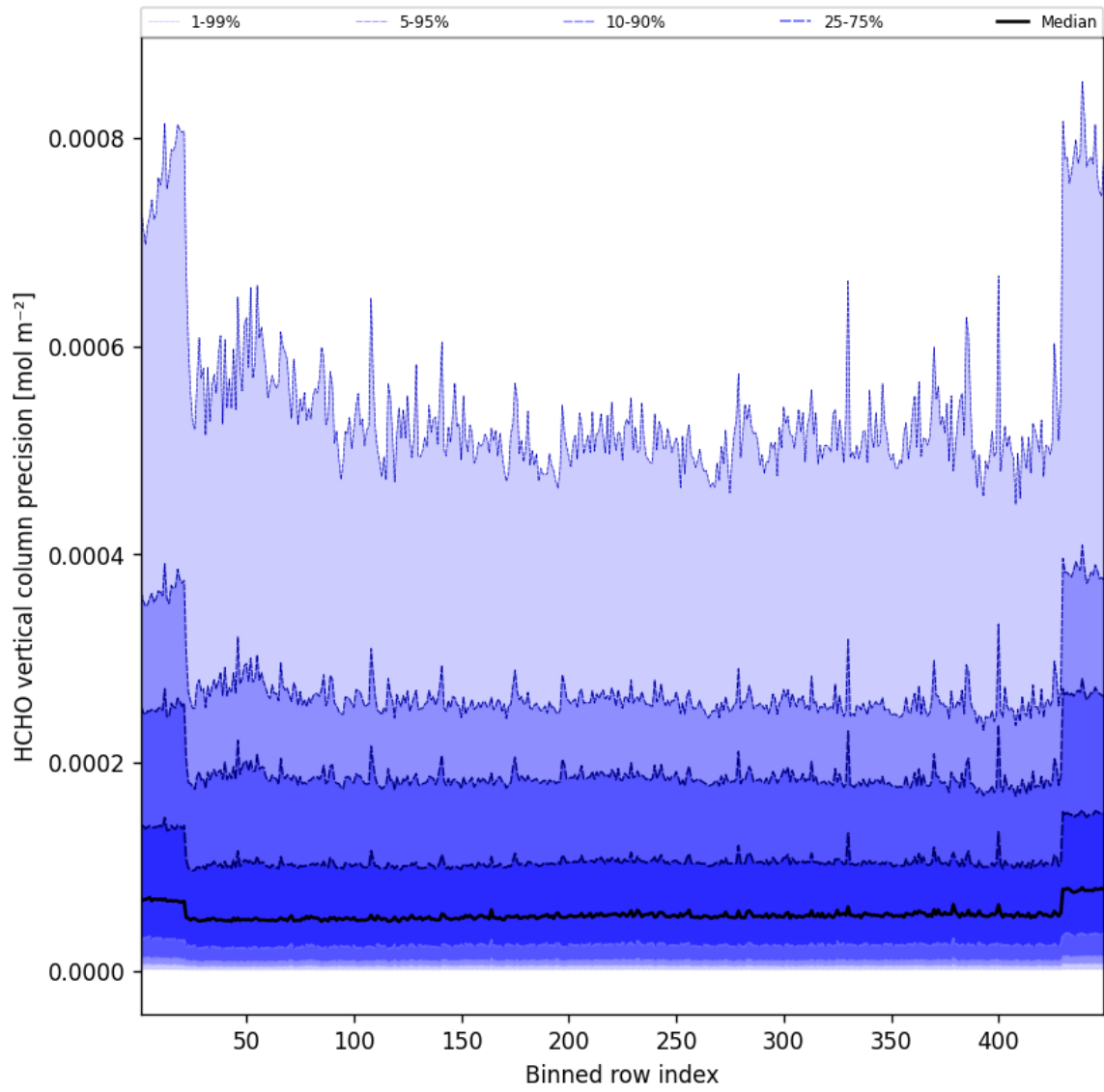
Figure 48: Along track statistics of “HCHO vertical column precision” for 2024-12-27 to 2024-12-28
