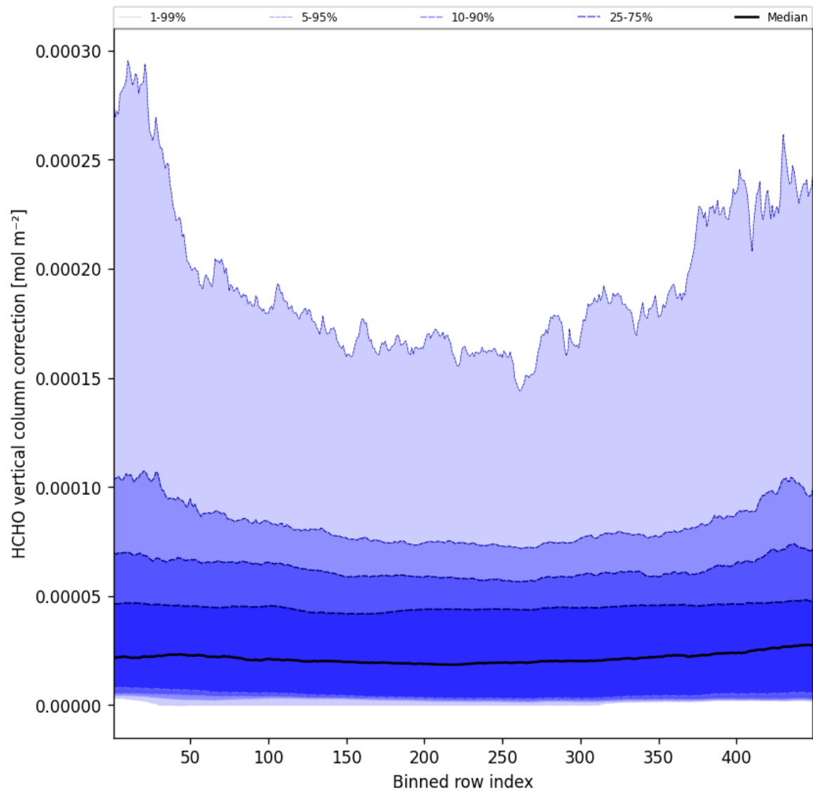
Figure 49: Along track statistics of “HCHO vertical column correction” for 2024-12-27 to 2024-12-28
