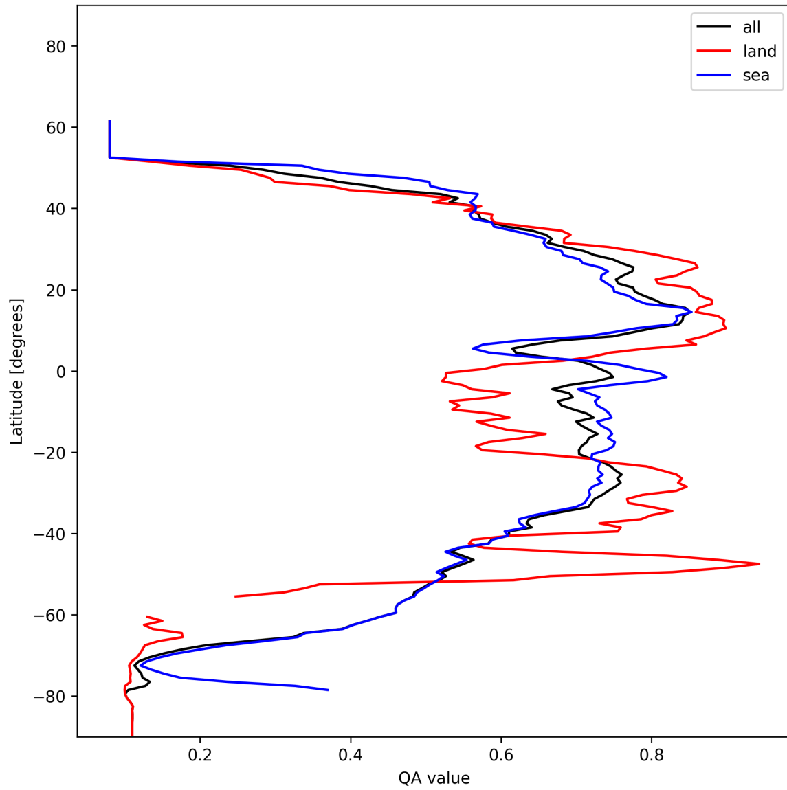
Figure 18: Zonal average of “QA value” for 2024-12-27 to 2024-12-28.
