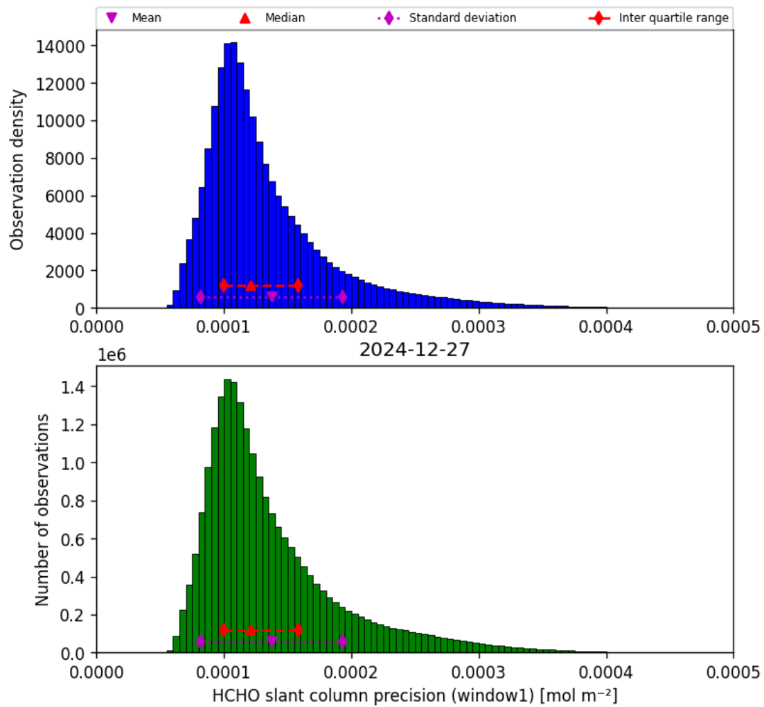
Figure 37: Histogram of “HCHO slant column precision (window1)” for 2024-12-27 to 2024-12-28
