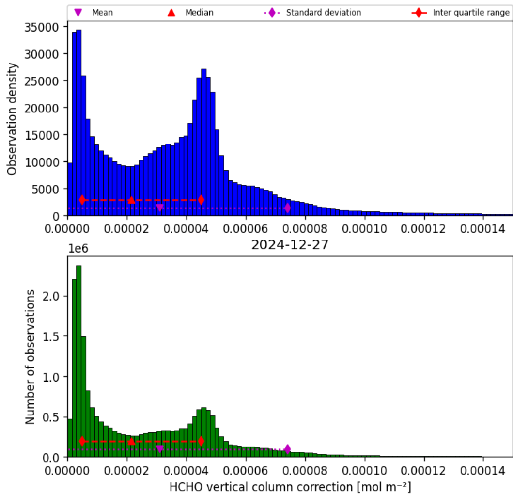
Figure 35: Histogram of “HCHO vertical column correction” for 2024-12-27 to 2024-12-28
