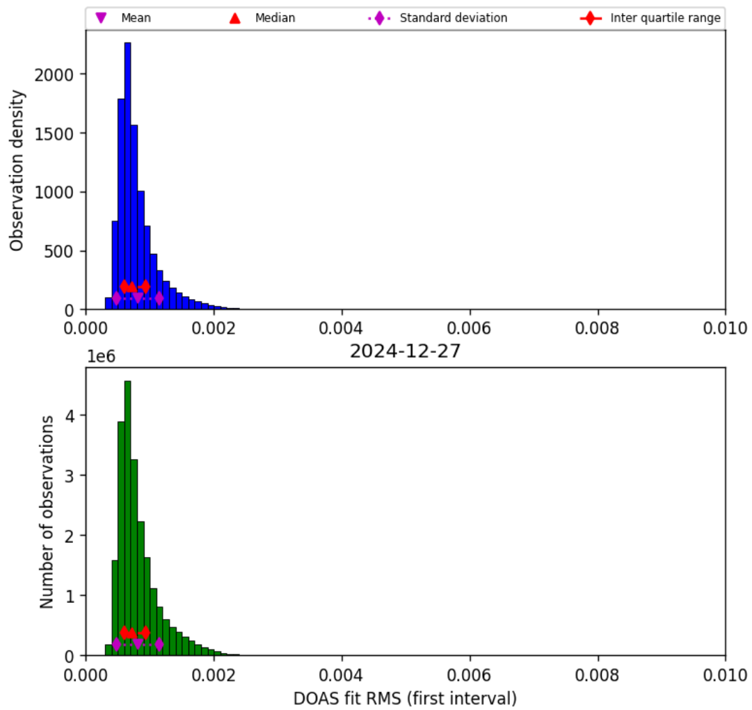
Figure 44: Histogram of “DOAS fit RMS (first interval)” for 2024-12-27 to 2024-12-28
