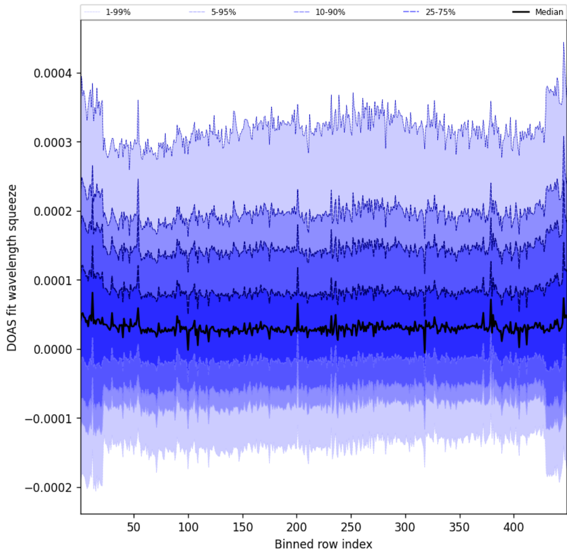
Figure 57: Along track statistics of “DOAS fit wavelength squeeze” for 2024-12-27 to 2024-12-28
