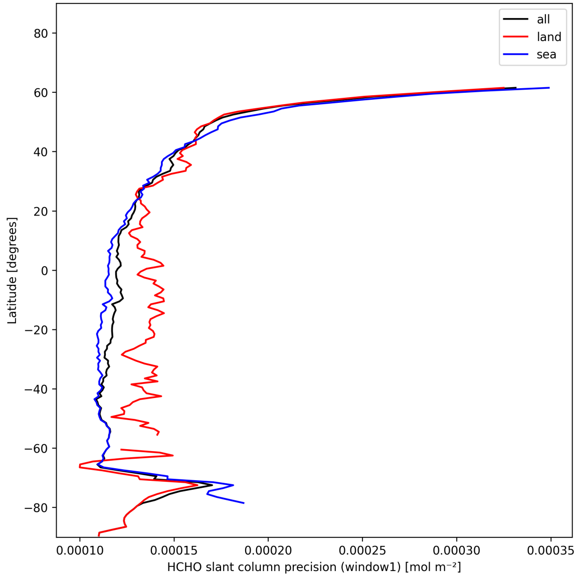
Figure 23: Zonal average of “HCHO slant column precision (window1)” for 2024-12-27 to 2024-12-28.
