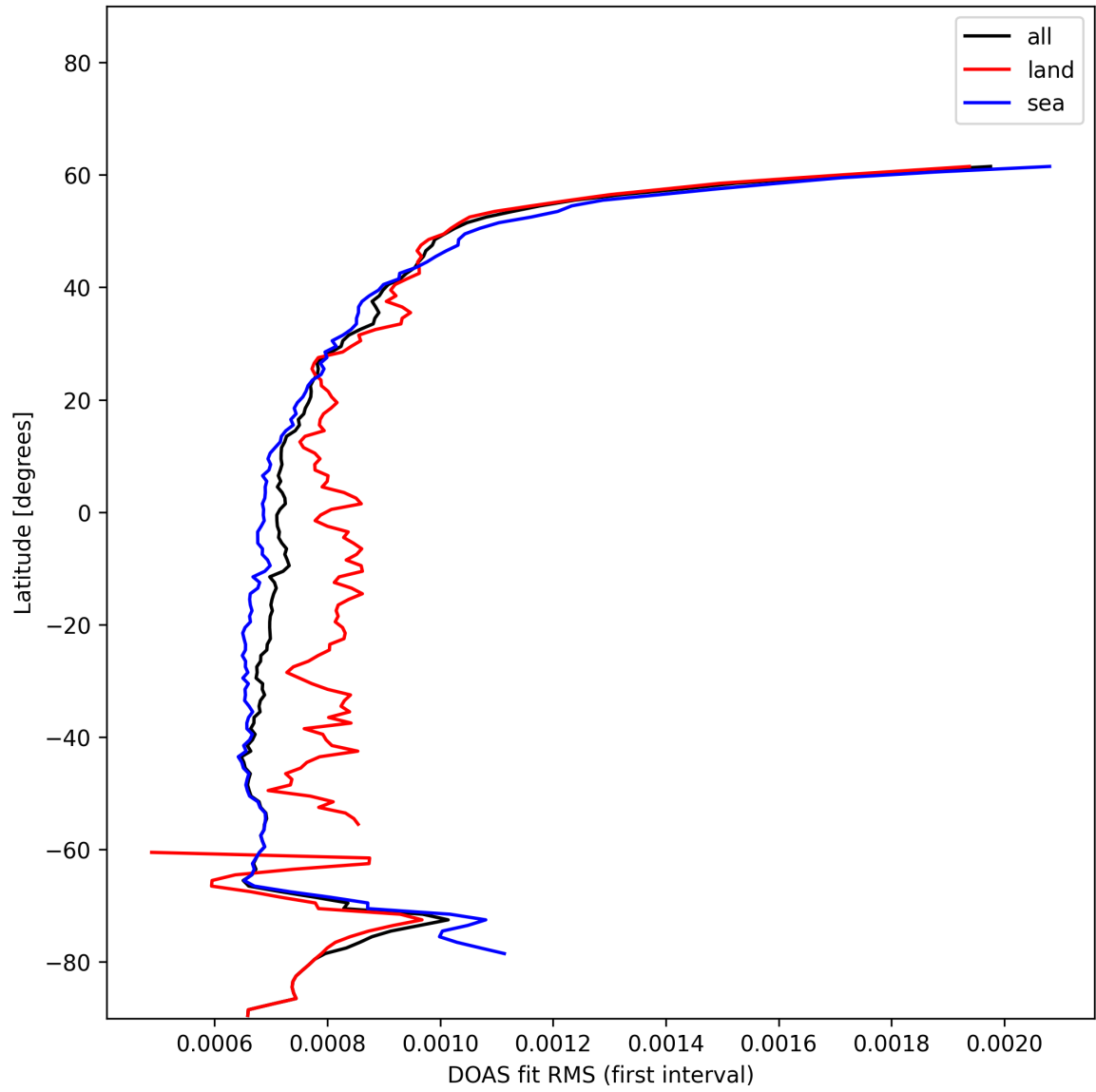
Figure 30: Zonal average of “DOAS fit RMS (first interval)” for 2024-12-27 to 2024-12-28.
