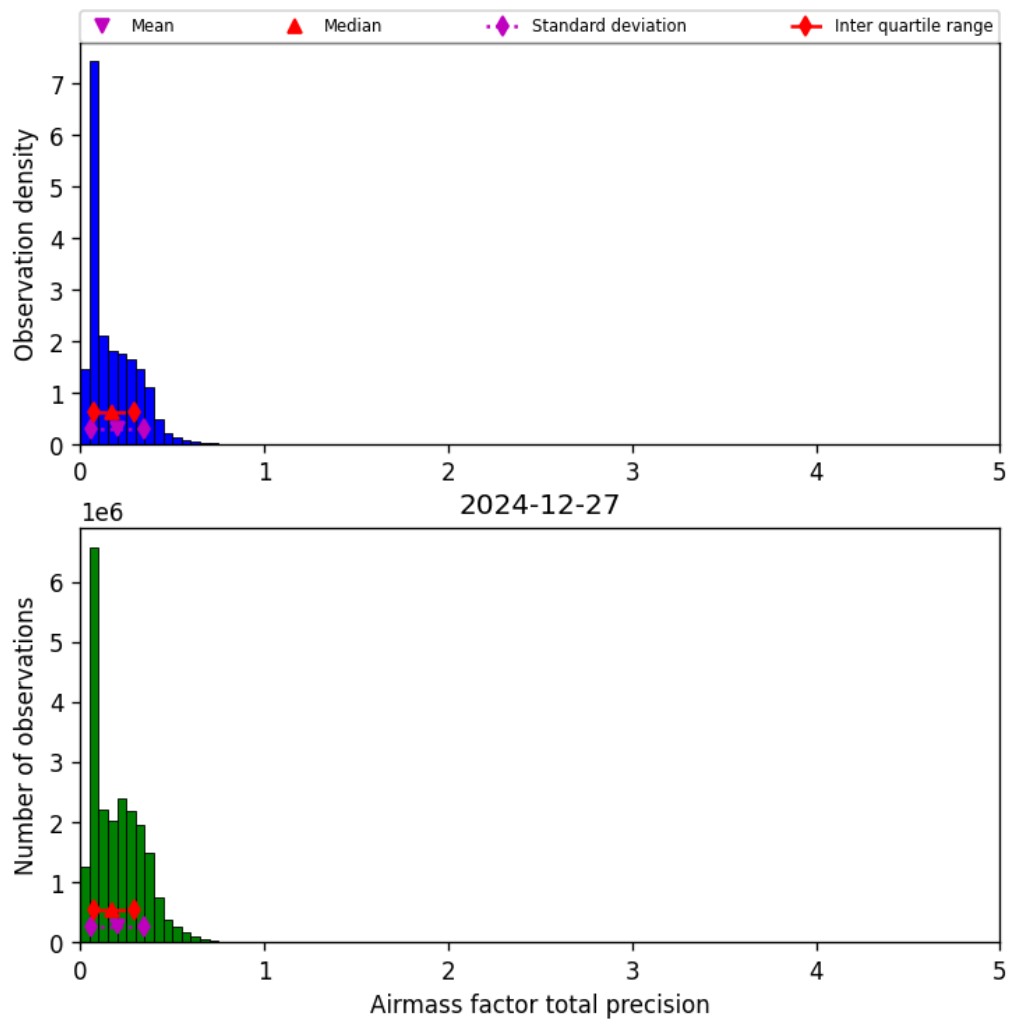
Figure 39: Histogram of “Airmass factor total precision” for 2024-12-27 to 2024-12-28
