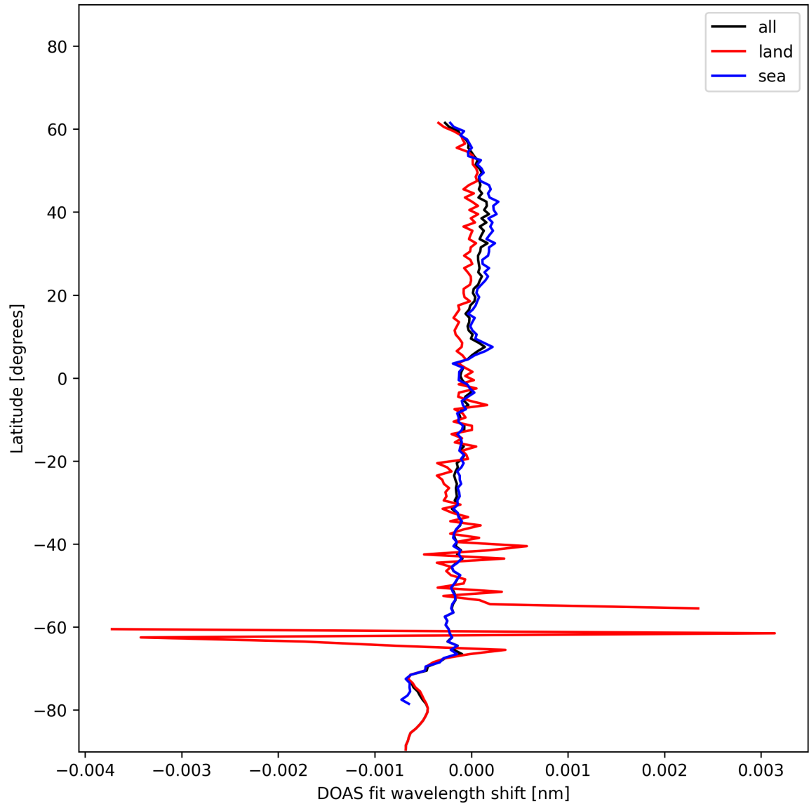
Figure 28: Zonal average of “DOAS fit wavelength shift” for 2024-12-27 to 2024-12-28.
