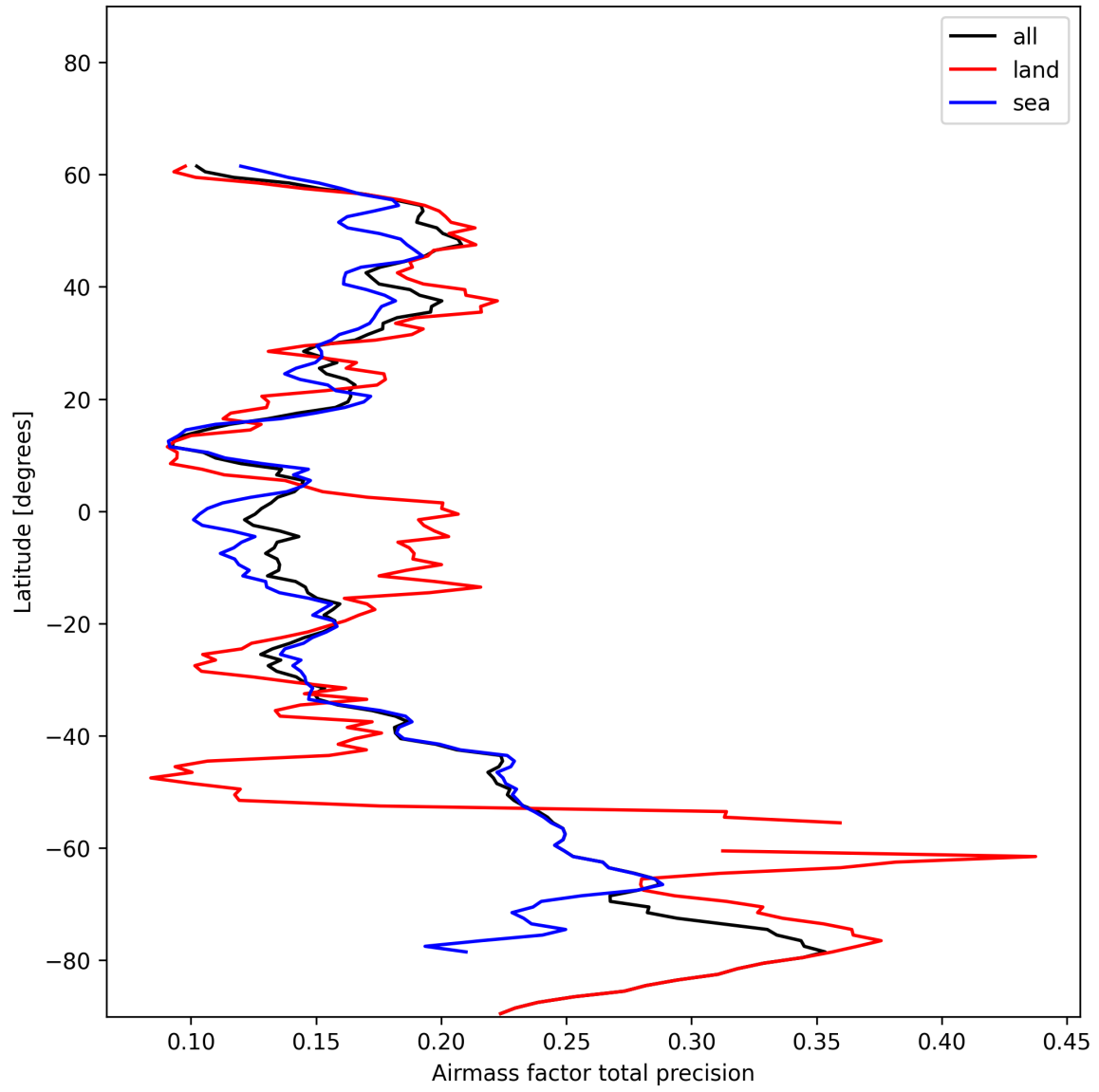
Figure 25: Zonal average of “Airmass factor total precision” for 2024-12-27 to 2024-12-28.
