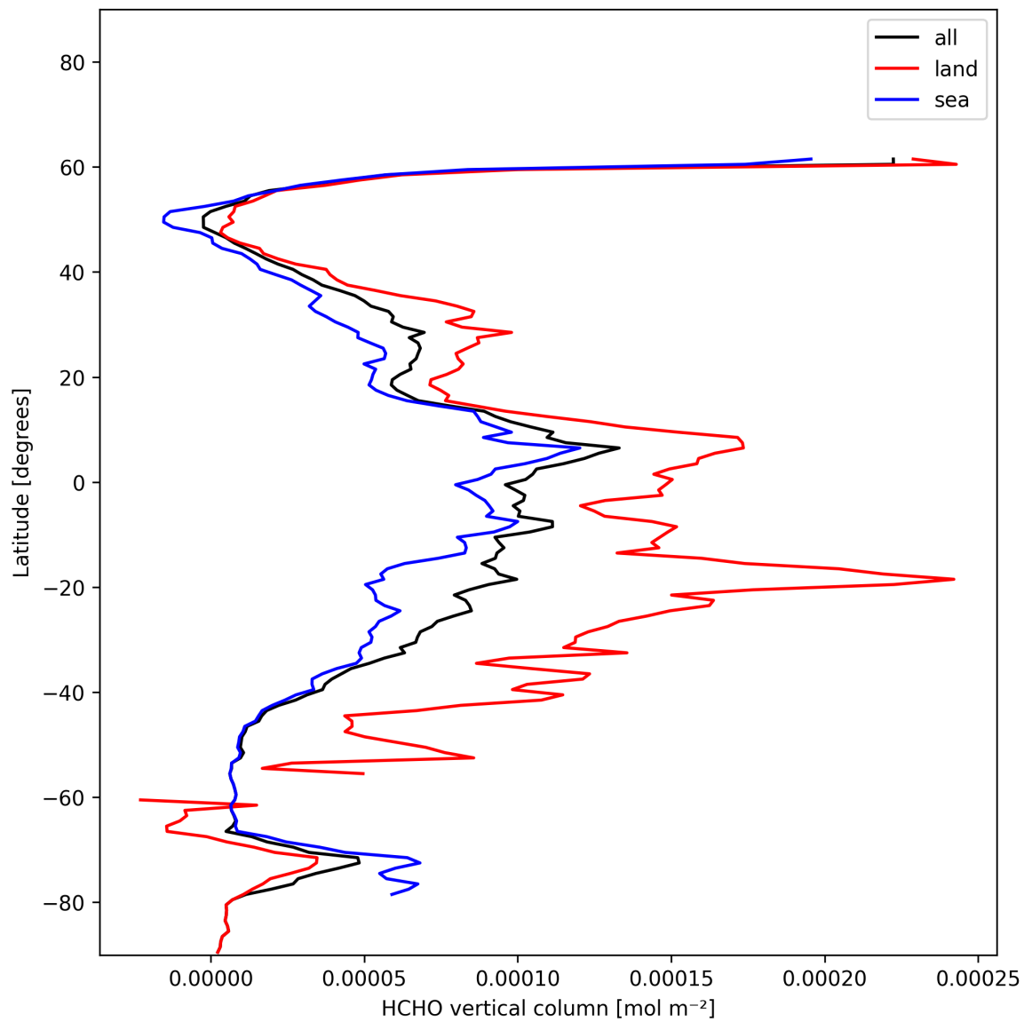
Figure 19: Zonal average of “HCHO vertical column” for 2024-12-27 to 2024-12-28.
