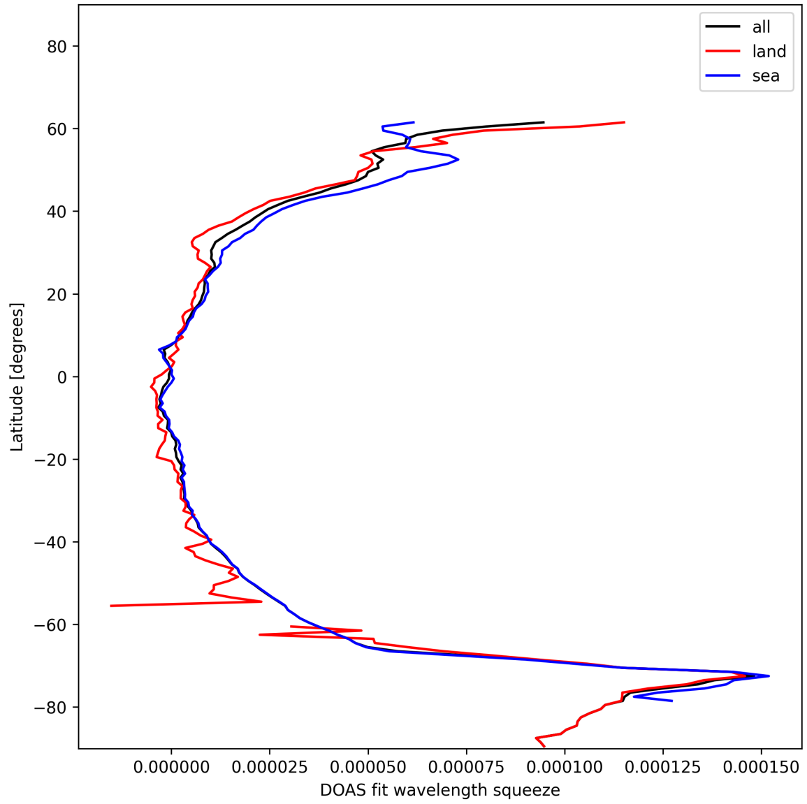
Figure 29: Zonal average of “DOAS fit wavelength squeeze” for 2024-12-27 to 2024-12-28.
