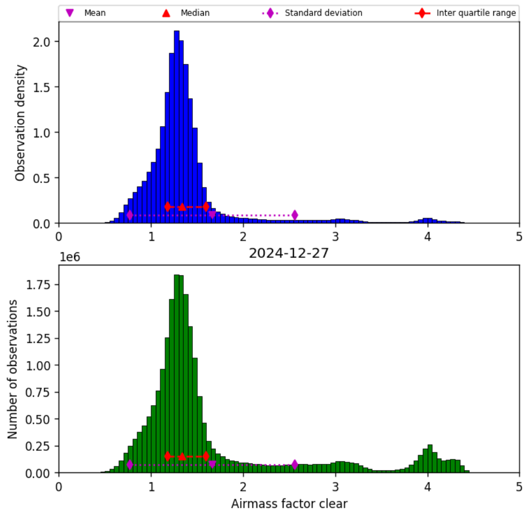
Figure 40: Histogram of “Airmass factor clear” for 2024-12-27 to 2024-12-28
