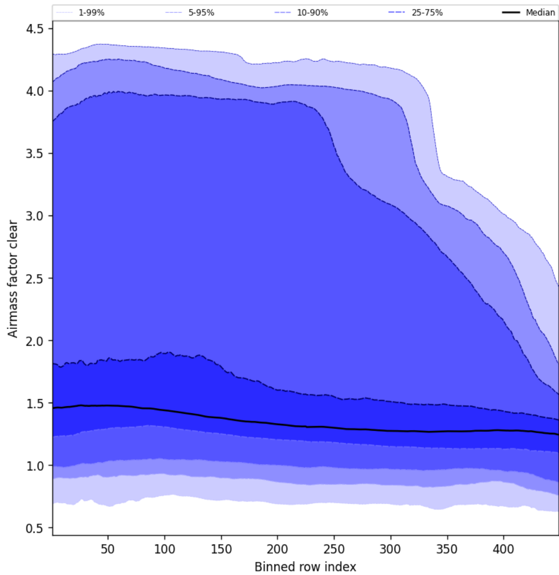
Figure 54: Along track statistics of “Airmass factor clear” for 2024-12-27 to 2024-12-28
