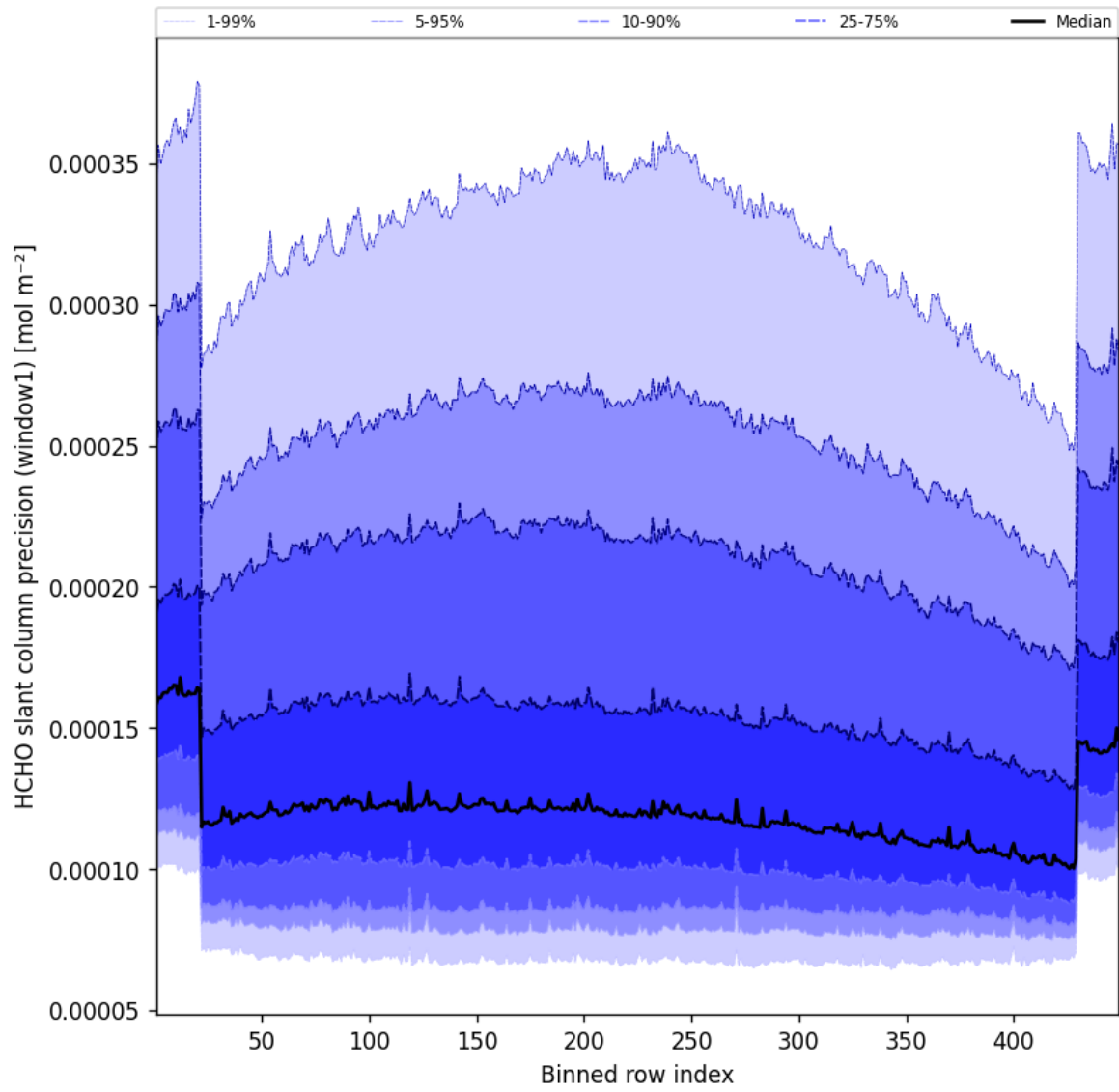
Figure 51: Along track statistics of “HCHO slant column precision (window1)” for 2024-12-27 to 2024-12-28
