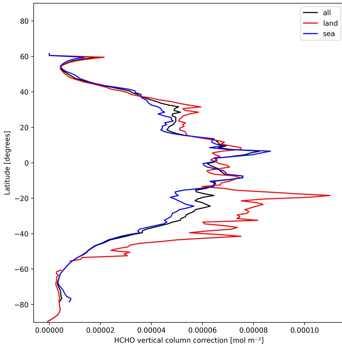
Figure 21: Zonal average of “HCHO vertical column correction” for 2024-12-27 to 2024-12-28.
