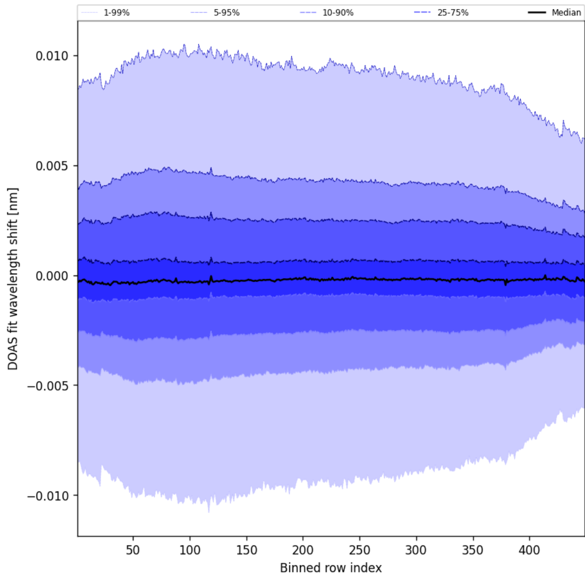
Figure 56: Along track statistics of “DOAS fit wavelength shift” for 2024-12-27 to 2024-12-28
