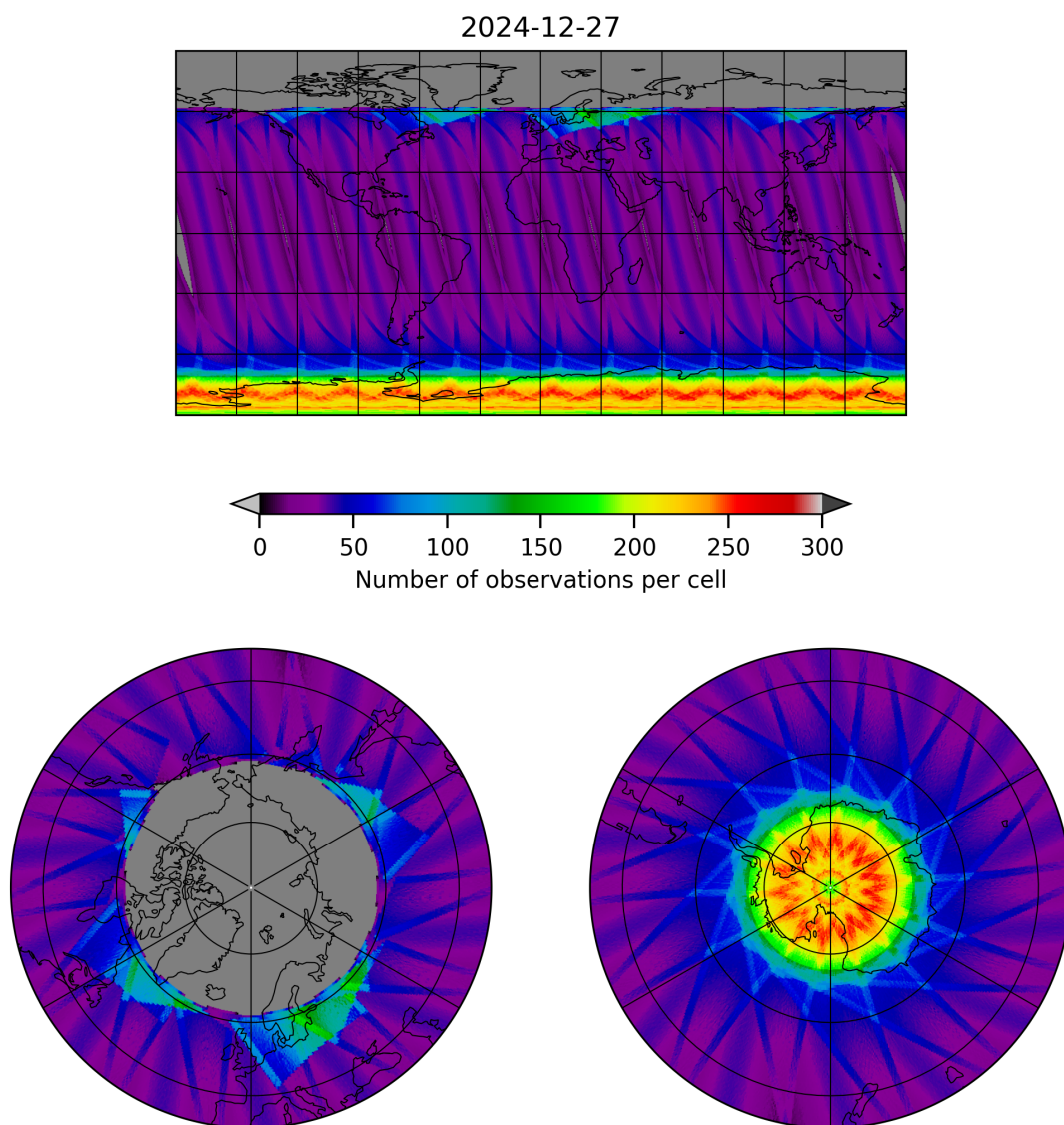
Figure 17: Map of the number of observations for 2024-12-27 to 2024-12-28
