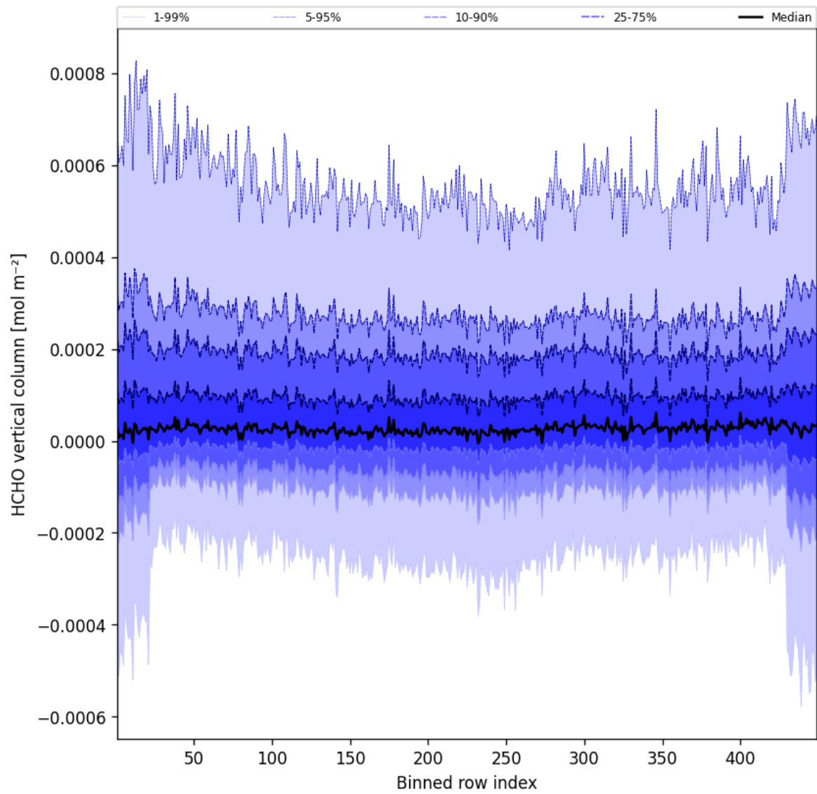
Figure 47: Along track statistics of “HCHO vertical column” for 2024-12-27 to 2024-12-28
