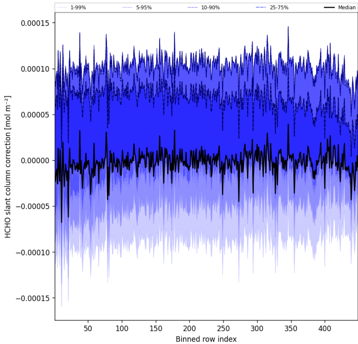
Figure 59: Along track statistics of “HCHO slant column correction” for 2024-12-27 to 2024-12-28
