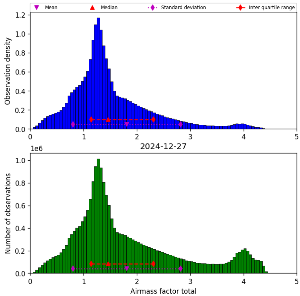
Figure 38: Histogram of “Airmass factor total” for 2024-12-27 to 2024-12-28
