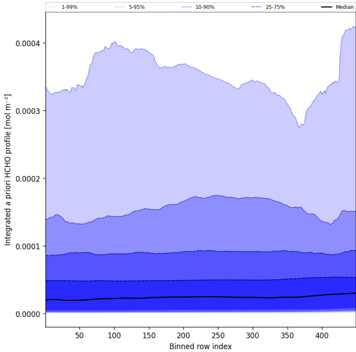
Figure 55: Along track statistics of “Integrated a priori HCHO profile” for 2024-12-27 to 2024-12-28
