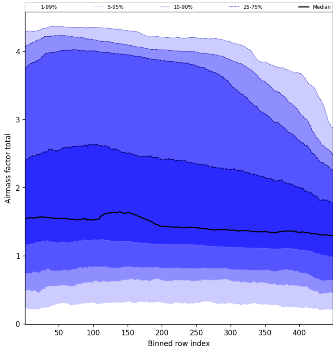
Figure 52: Along track statistics of “Airmass factor total” for 2024-12-27 to 2024-12-28
