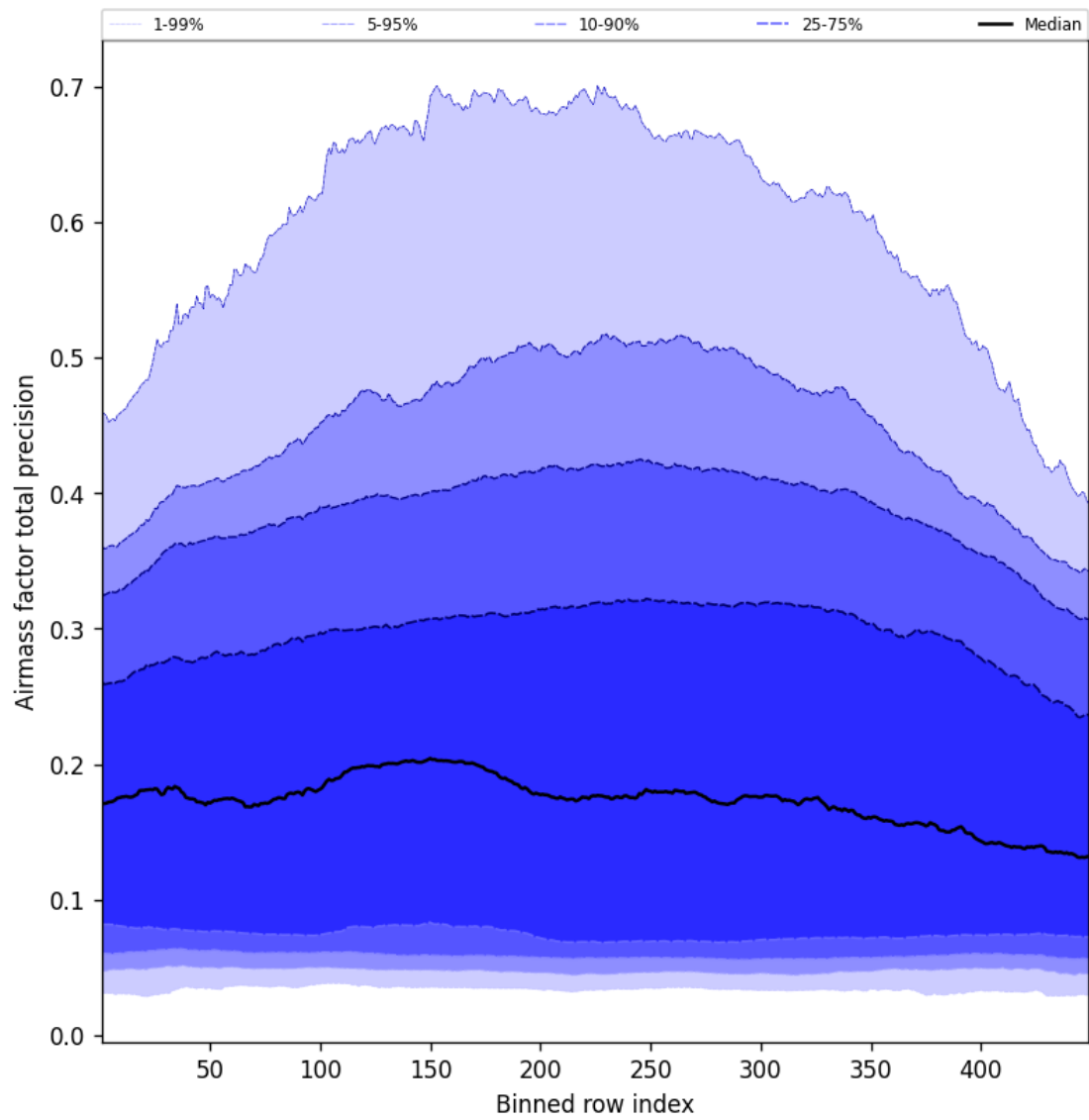
Figure 53: Along track statistics of “Airmass factor total precision” for 2024-12-27 to 2024-12-28
