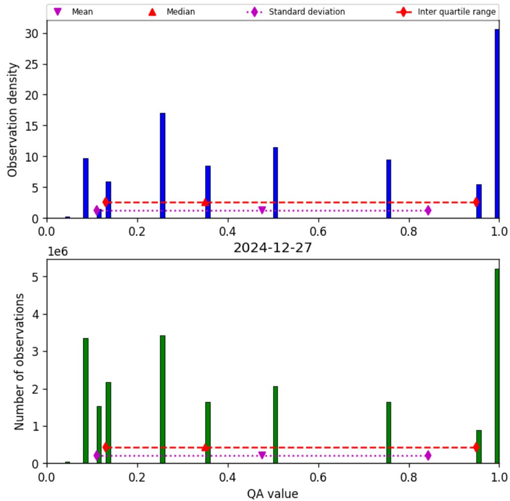
Figure 32: Histogram of “QA value” for 2024-12-27 to 2024-12-28
