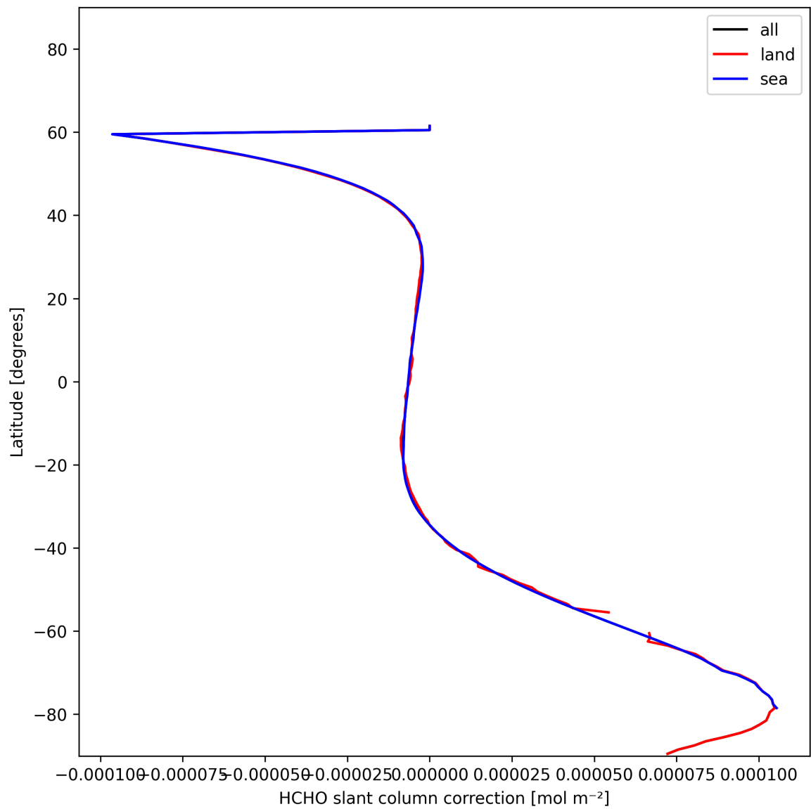
Figure 31: Zonal average of “HCHO slant column correction” for 2024-12-27 to 2024-12-28.
