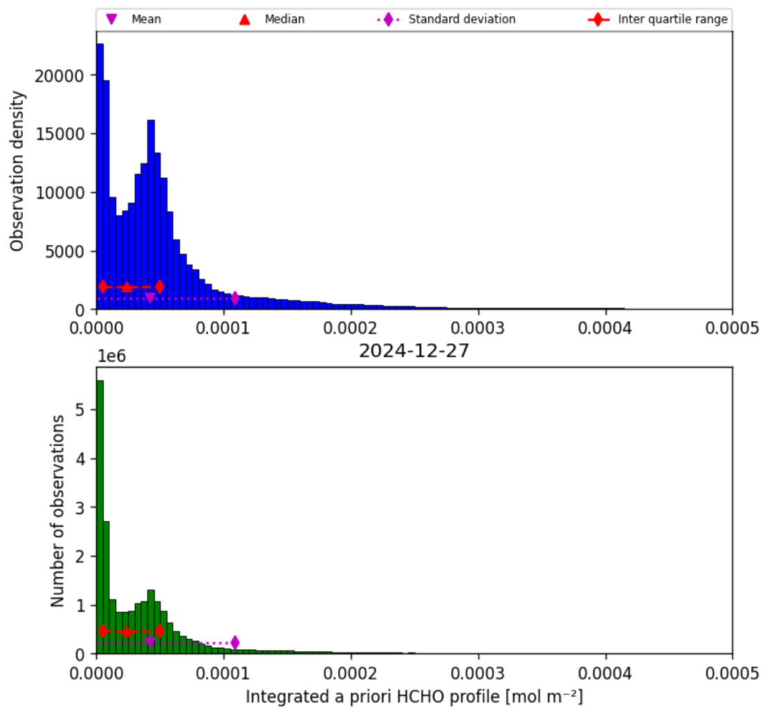
Figure 41: Histogram of “Integrated a priori HCHO profile” for 2024-12-27 to 2024-12-28
