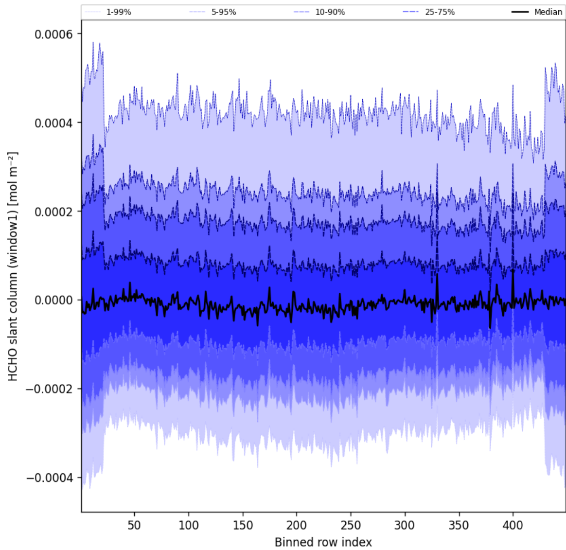
Figure 50: Along track statistics of “HCHO slant column (window1)” for 2024-12-27 to 2024-12-28
