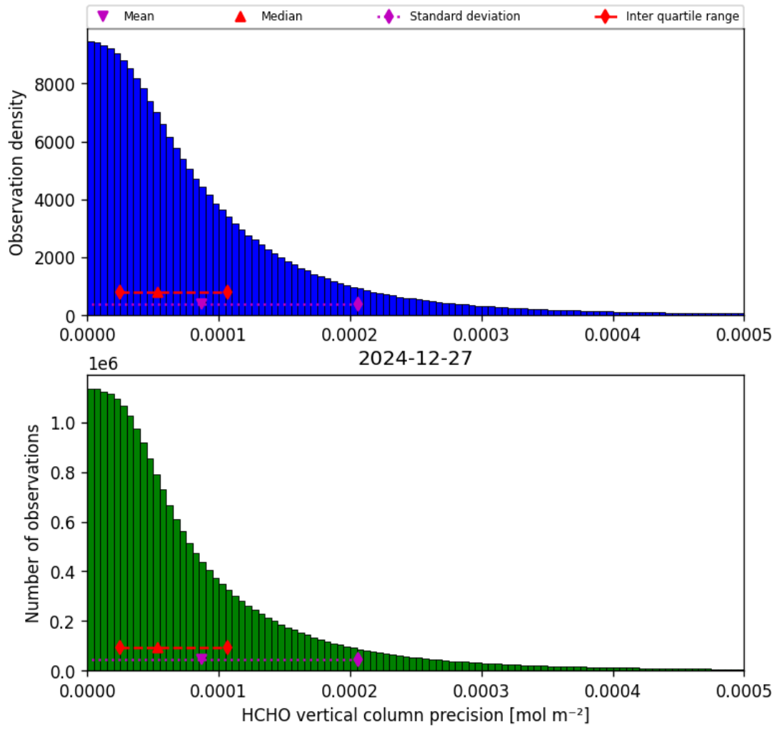
Figure 34: Histogram of “HCHO vertical column precision” for 2024-12-27 to 2024-12-28
