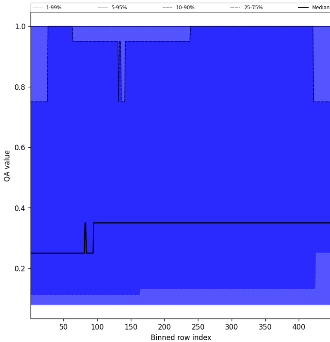
Figure 46: Along track statistics of “QA value” for 2024-12-27 to 2024-12-28
