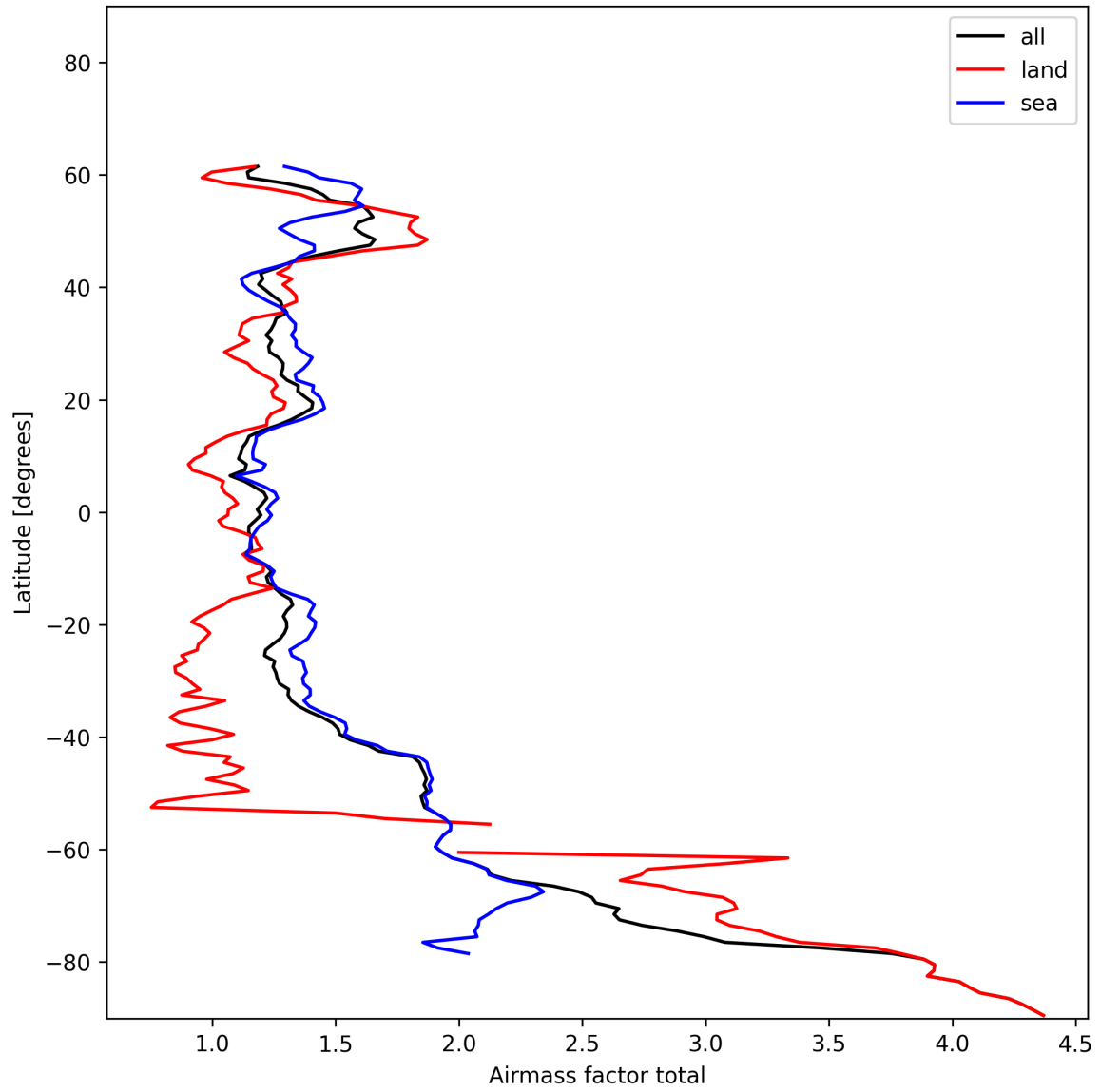
Figure 24: Zonal average of “Airmass factor total” for 2024-12-27 to 2024-12-28.
