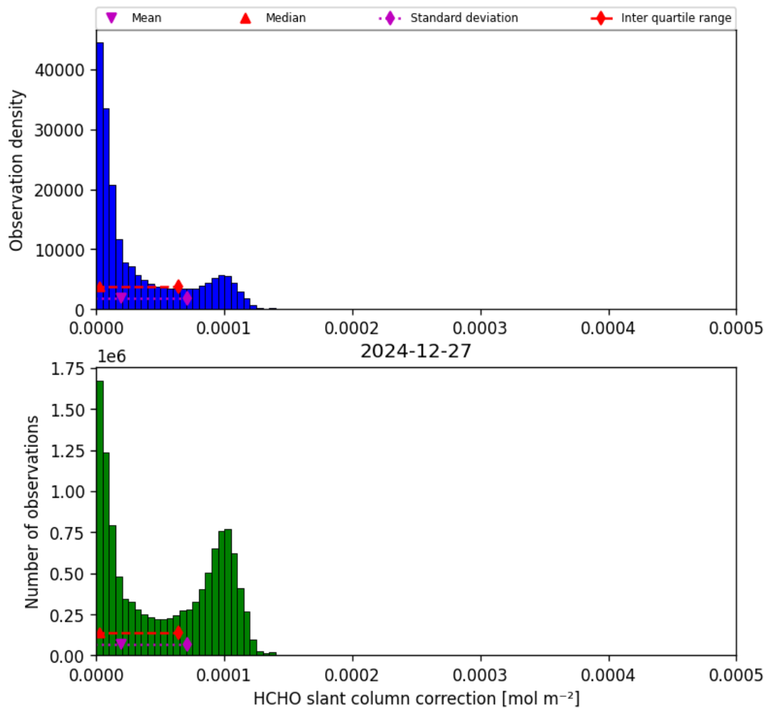
Figure 45: Histogram of “HCHO slant column correction” for 2024-12-27 to 2024-12-28
