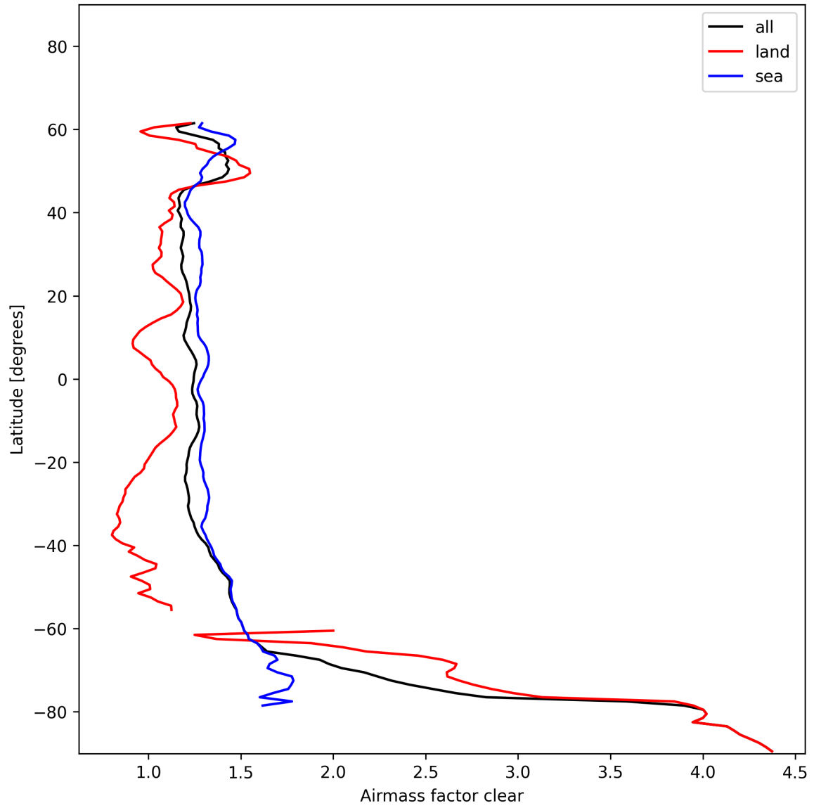
Figure 26: Zonal average of “Airmass factor clear” for 2024-12-27 to 2024-12-28.
