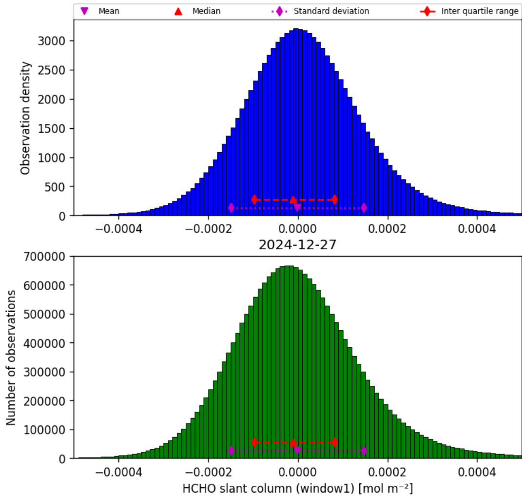
Figure 36: Histogram of “HCHO slant column (window1)” for 2024-12-27 to 2024-12-28
