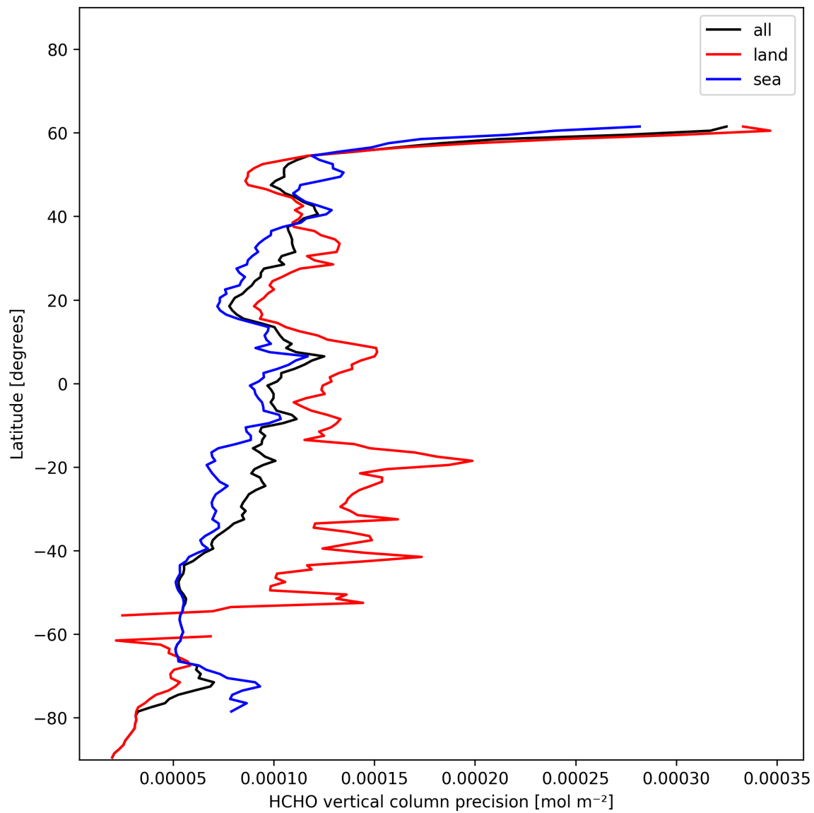
Figure 20: Zonal average of “HCHO vertical column precision” for 2024-12-27 to 2024-12-28.
