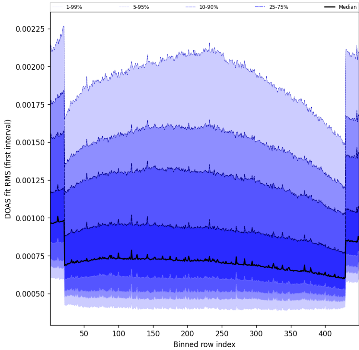
Figure 58: Along track statistics of “DOAS fit RMS (first interval)” for 2024-12-27 to 2024-12-28
