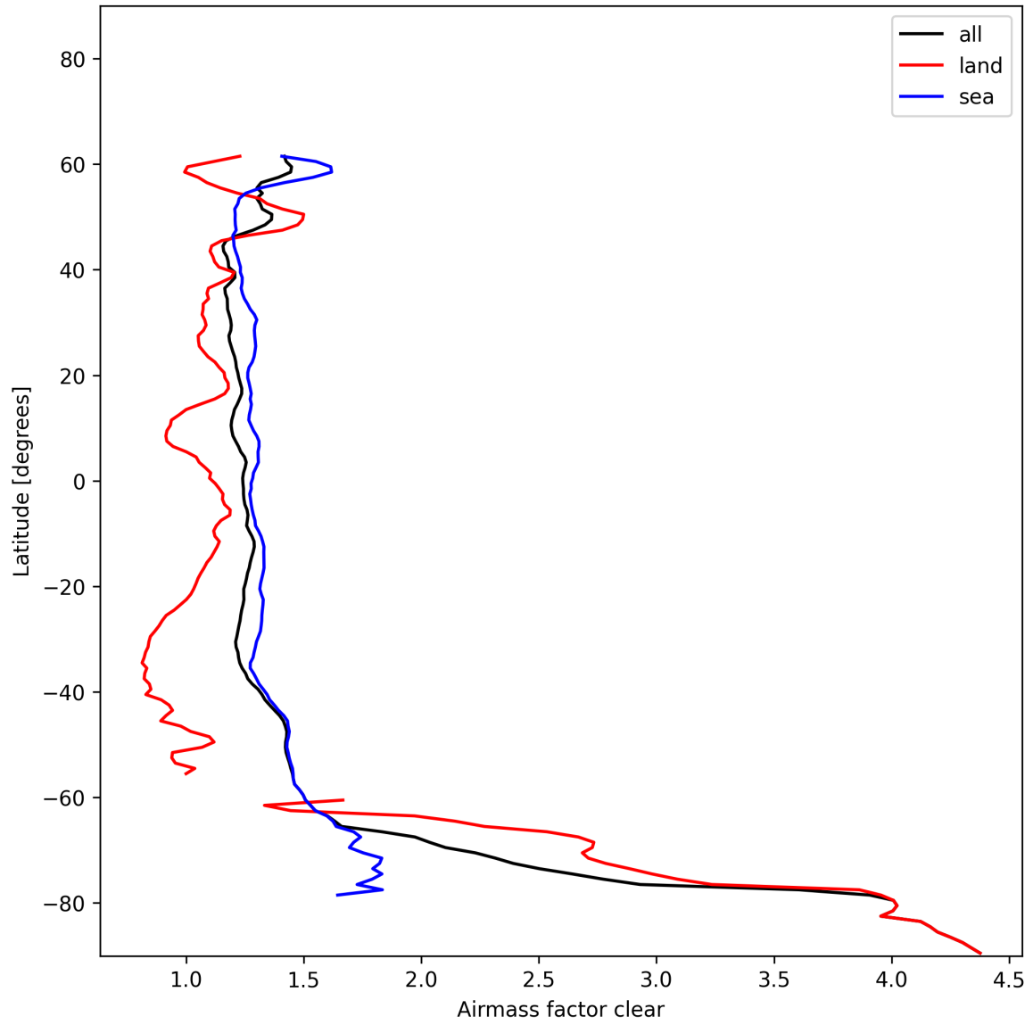
Figure 26: Zonal average of “Airmass factor clear” for 2024-12-29 to 2024-12-30.
