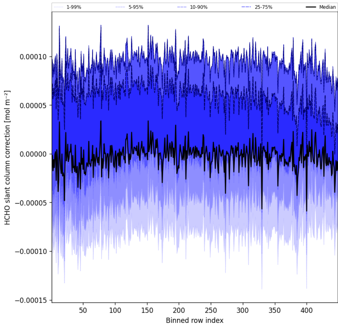
Figure 59: Along track statistics of “HCHO slant column correction” for 2024-12-29 to 2024-12-30
