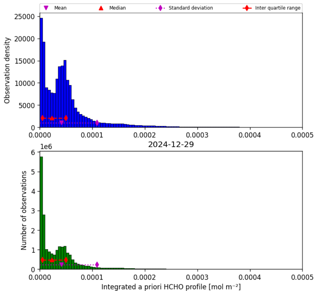
Figure 41: Histogram of “Integrated a priori HCHO profile” for 2024-12-29 to 2024-12-30
