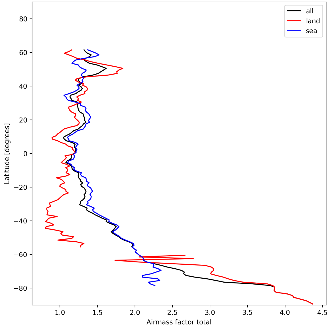
Figure 24: Zonal average of “Airmass factor total” for 2024-12-29 to 2024-12-30.
