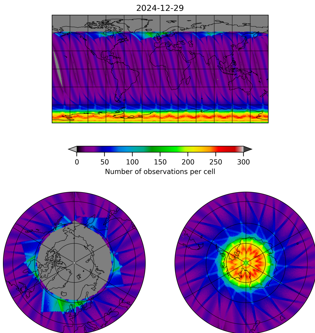
Figure 17: Map of the number of observations for 2024-12-29 to 2024-12-30
