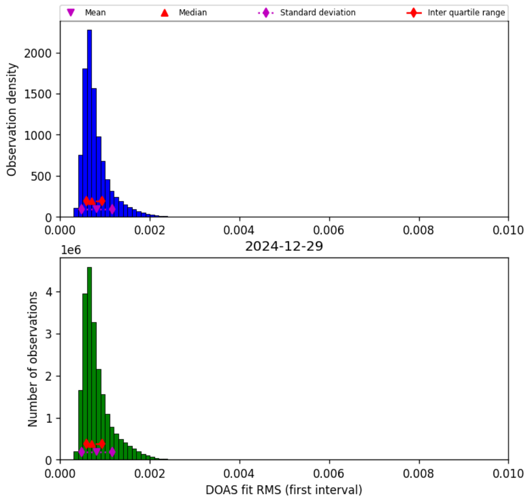
Figure 44: Histogram of “DOAS fit RMS (first interval)” for 2024-12-29 to 2024-12-30
