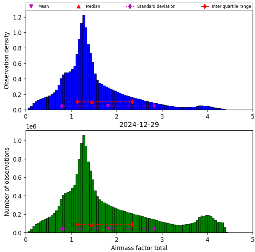
Figure 38: Histogram of “Airmass factor total” for 2024-12-29 to 2024-12-30
