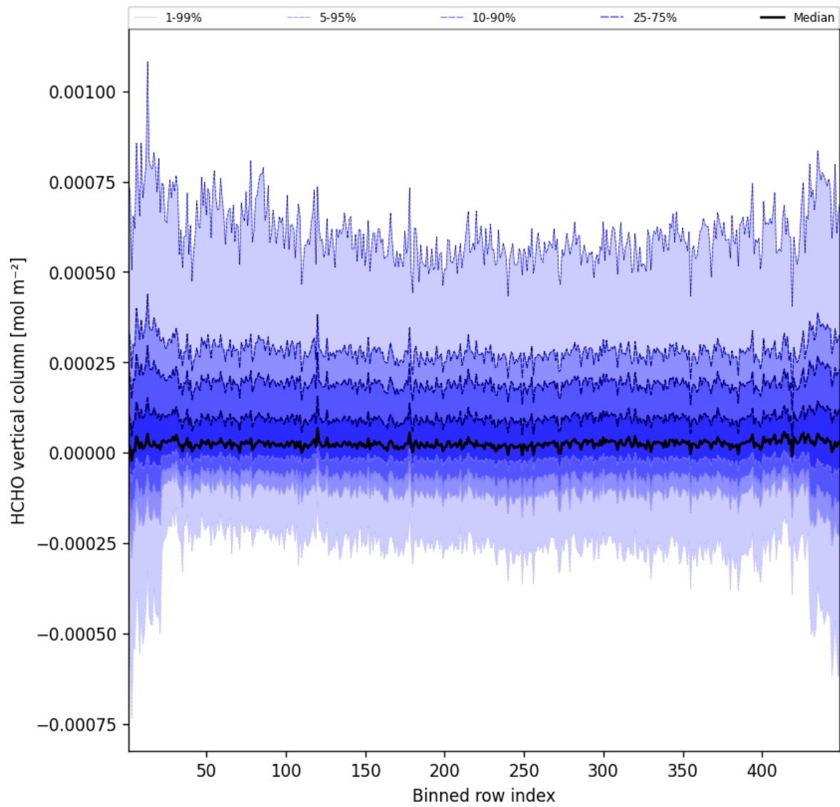
Figure 47: Along track statistics of “HCHO vertical column” for 2024-12-29 to 2024-12-30
