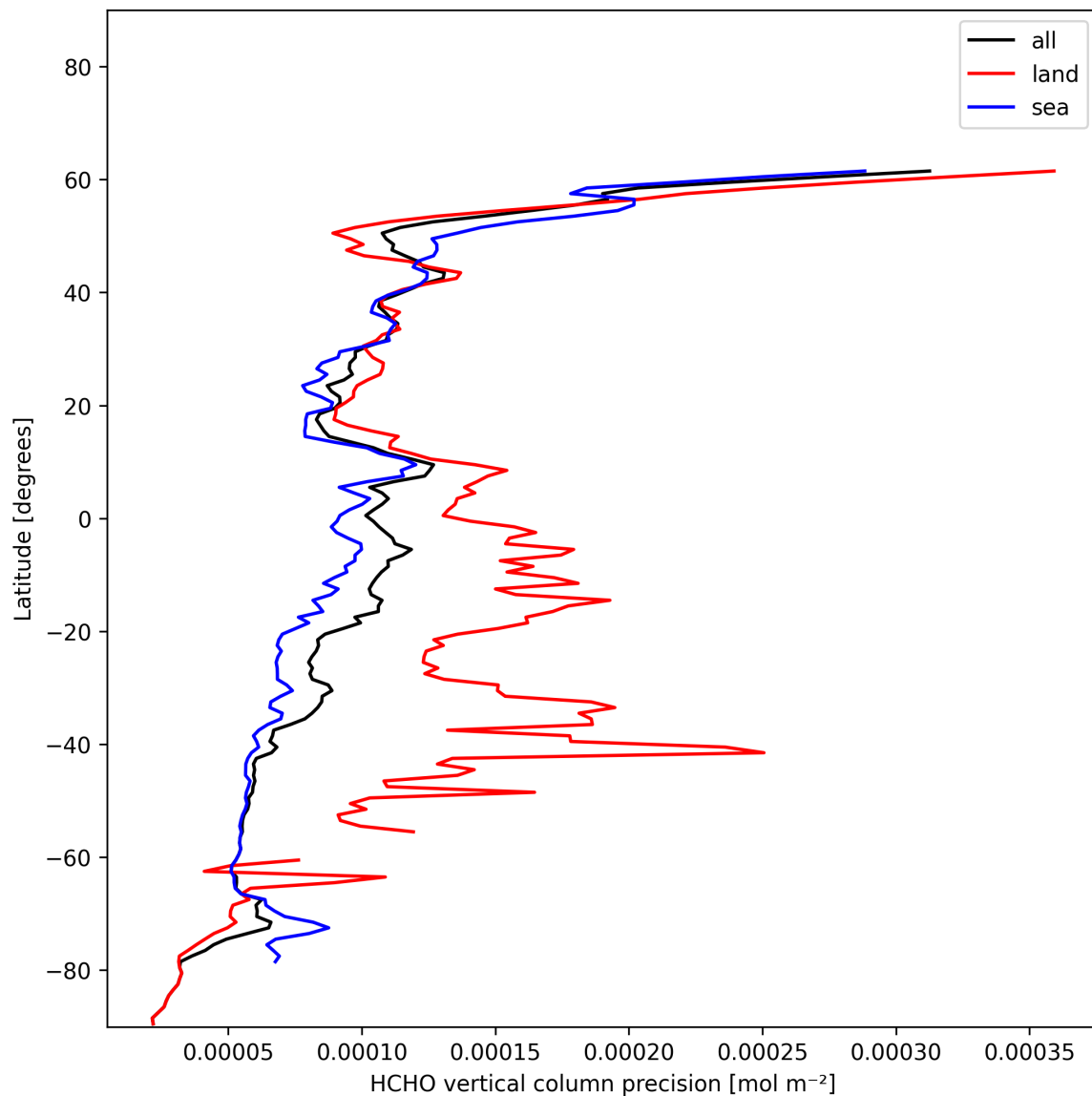
Figure 20: Zonal average of “HCHO vertical column precision” for 2024-12-29 to 2024-12-30.
