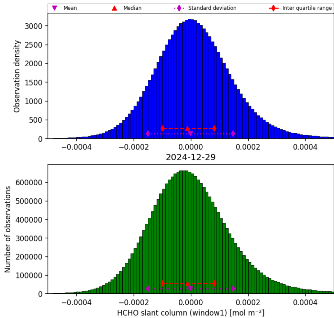
Figure 36: Histogram of “HCHO slant column (window1)” for 2024-12-29 to 2024-12-30
