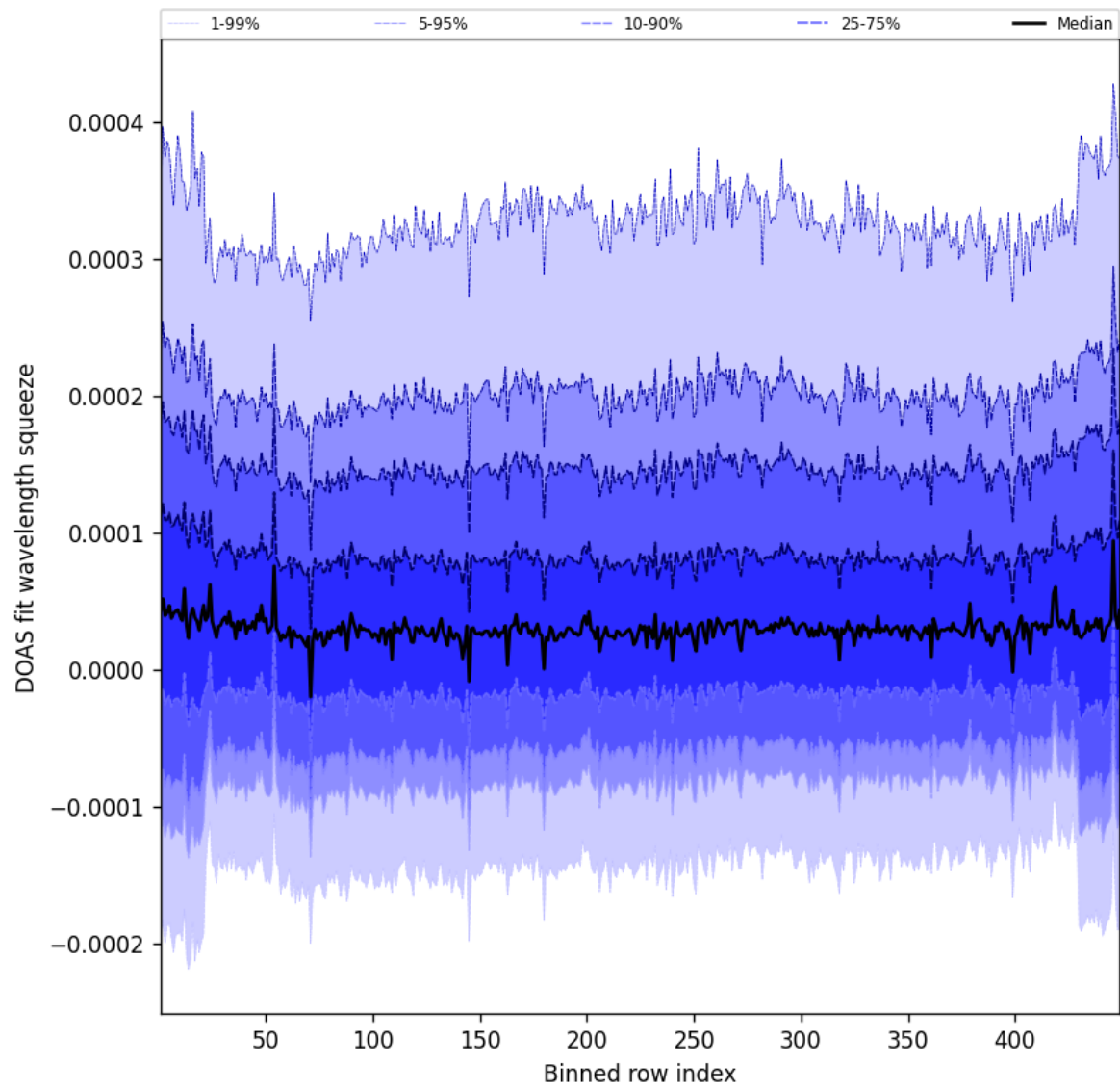
Figure 57: Along track statistics of “DOAS fit wavelength squeeze” for 2024-12-29 to 2024-12-30
