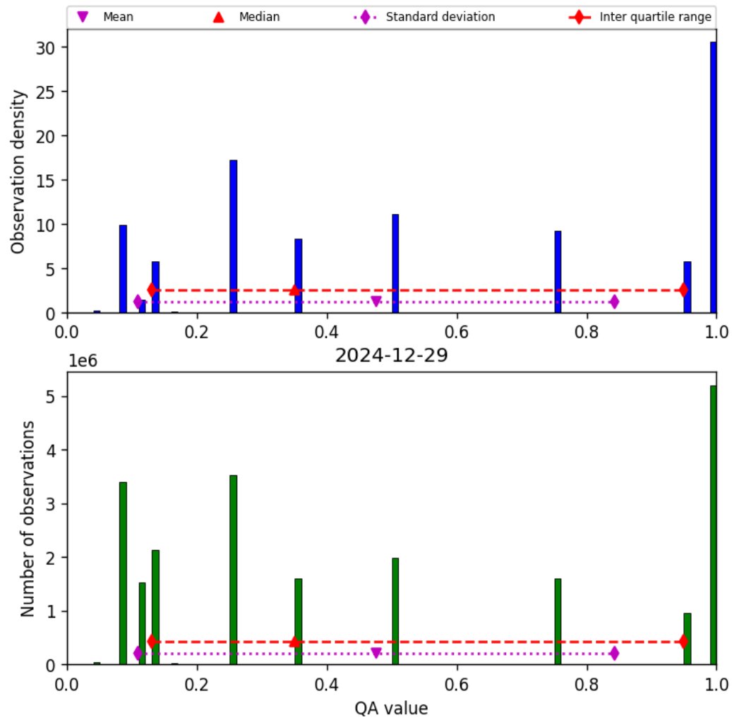
Figure 32: Histogram of “QA value” for 2024-12-29 to 2024-12-30
