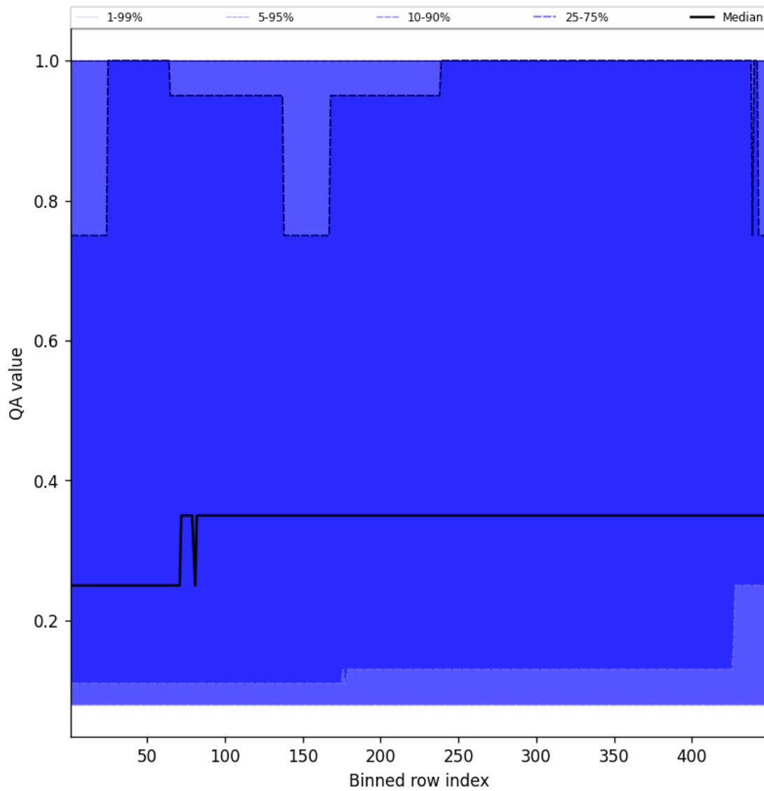
Figure 46: Along track statistics of “QA value” for 2024-12-29 to 2024-12-30
