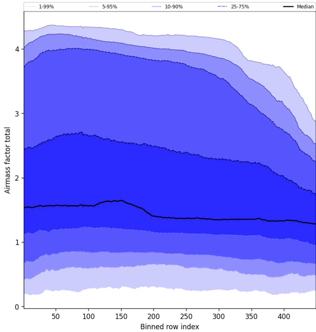
Figure 52: Along track statistics of “Airmass factor total” for 2024-12-29 to 2024-12-30
