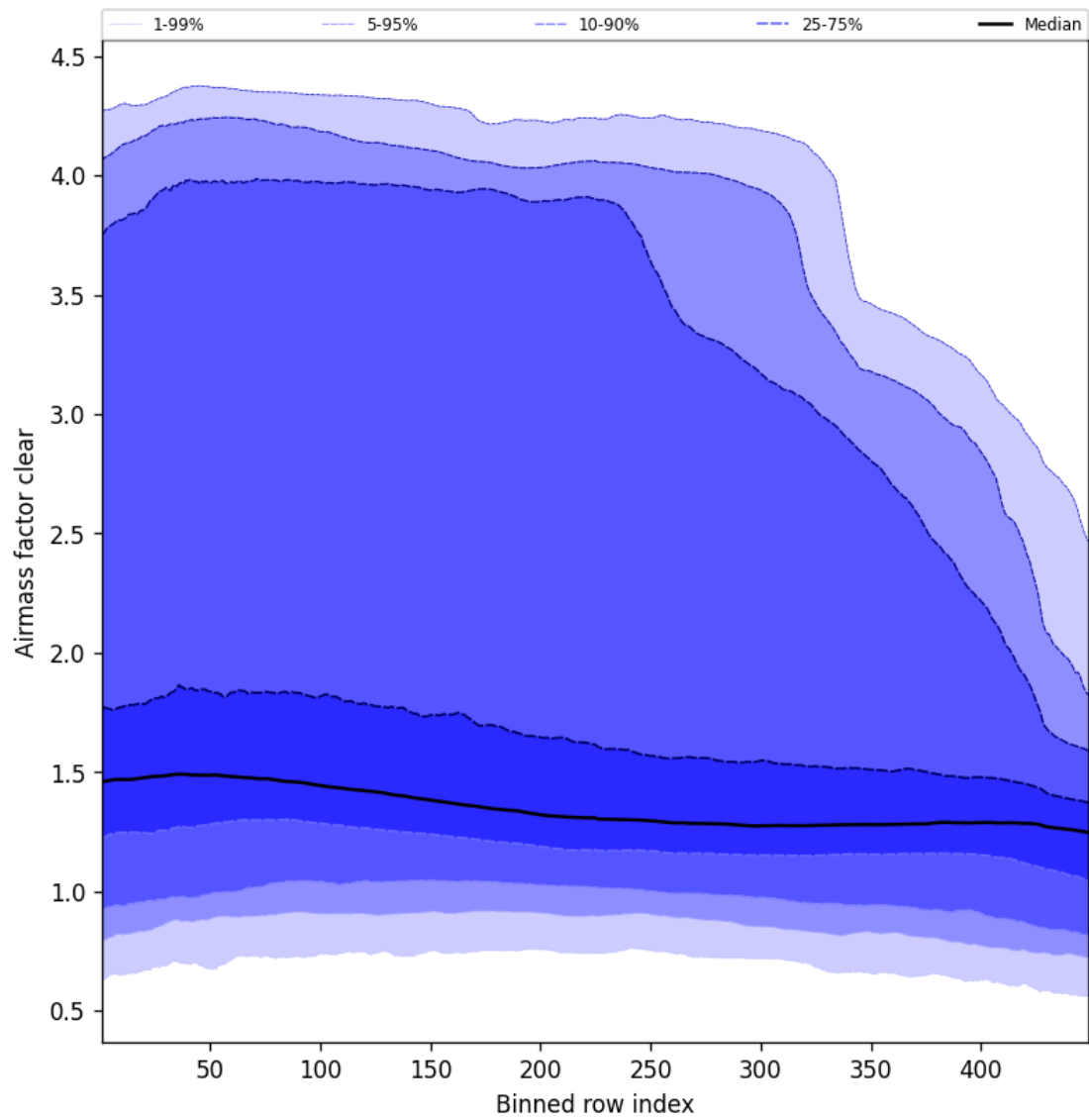
Figure 54: Along track statistics of “Air mass factor clear” for 2024-12-29 to 2024-12-30
