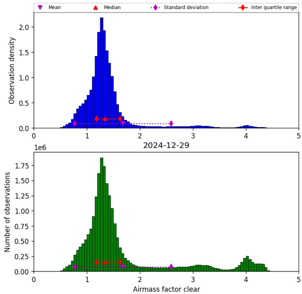
Figure 40: Histogram of “Airmass factor clear” for 2024-12-29 to 2024-12-30
