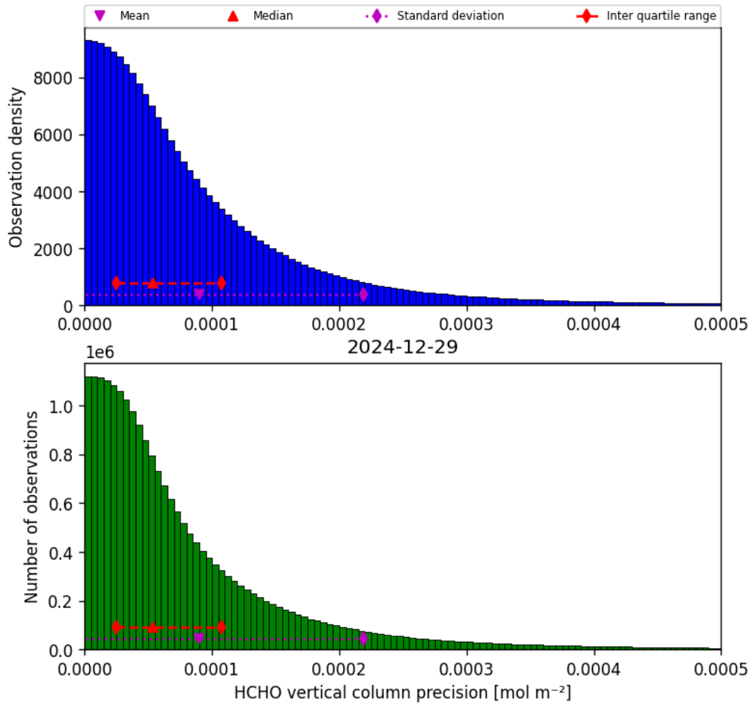
Figure 34: Histogram of “HCHO vertical column precision” for 2024-12-29 to 2024-12-30
