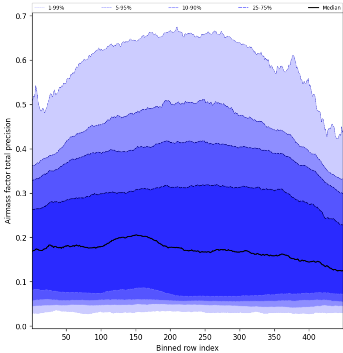
Figure 53: Along track statistics of “Airmass factor total precision” for 2024-12-29 to 2024-12-30
