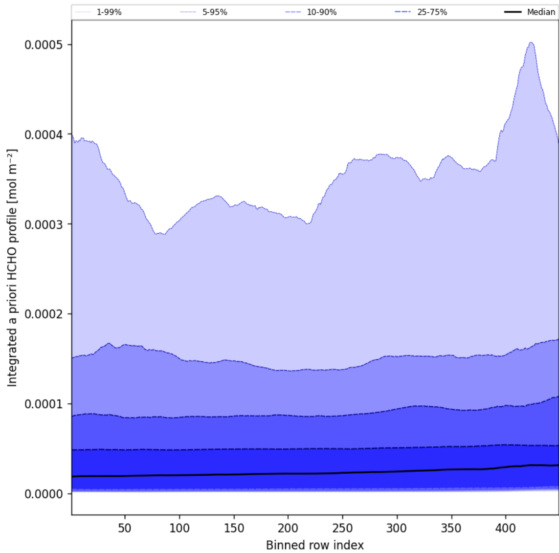
Figure 55: Along track statistics of “Integrated a priori HCHO profile” for 2024-12-29 to 2024-12-30
