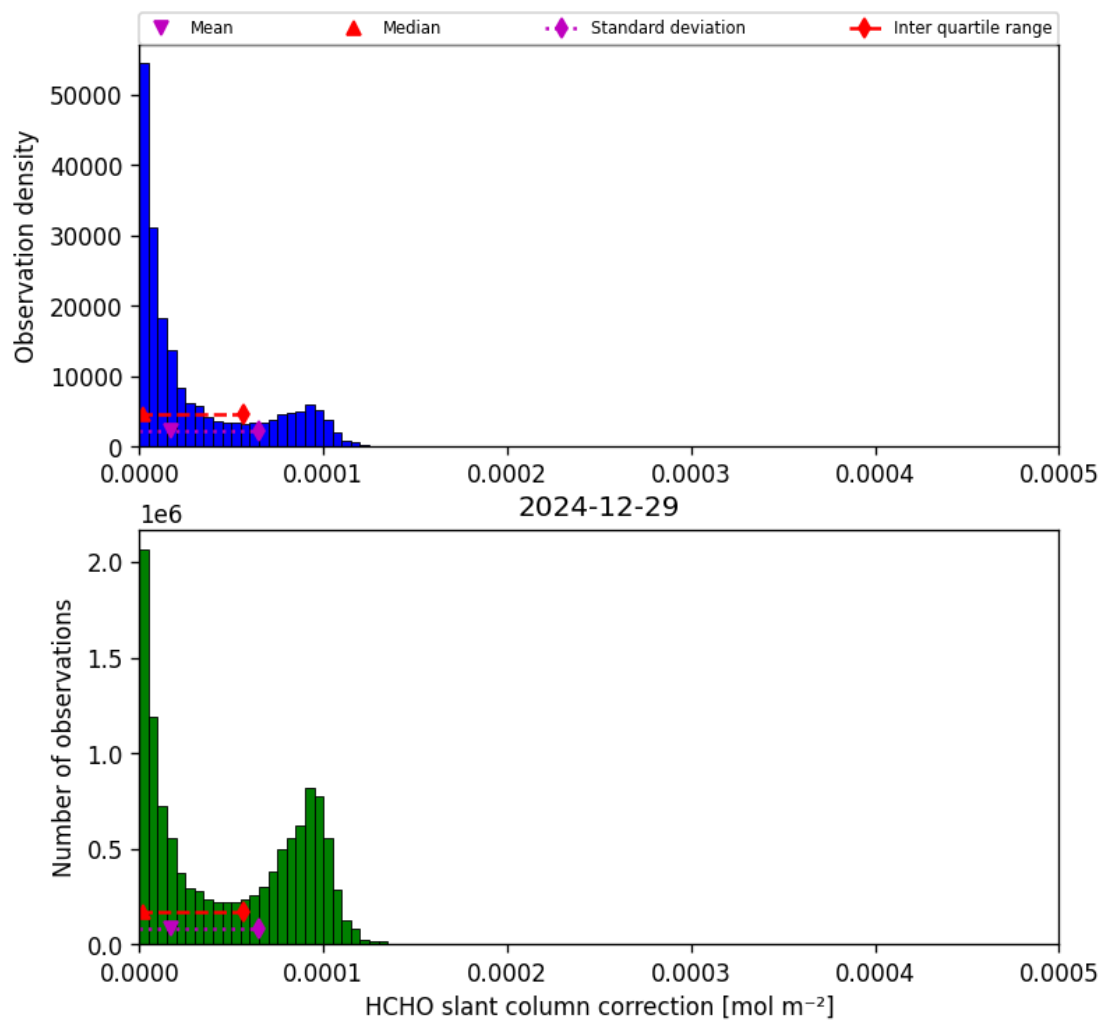
Figure 45: Histogram of “HCHO slant column correction” for 2024-12-29 to 2024-12-30
