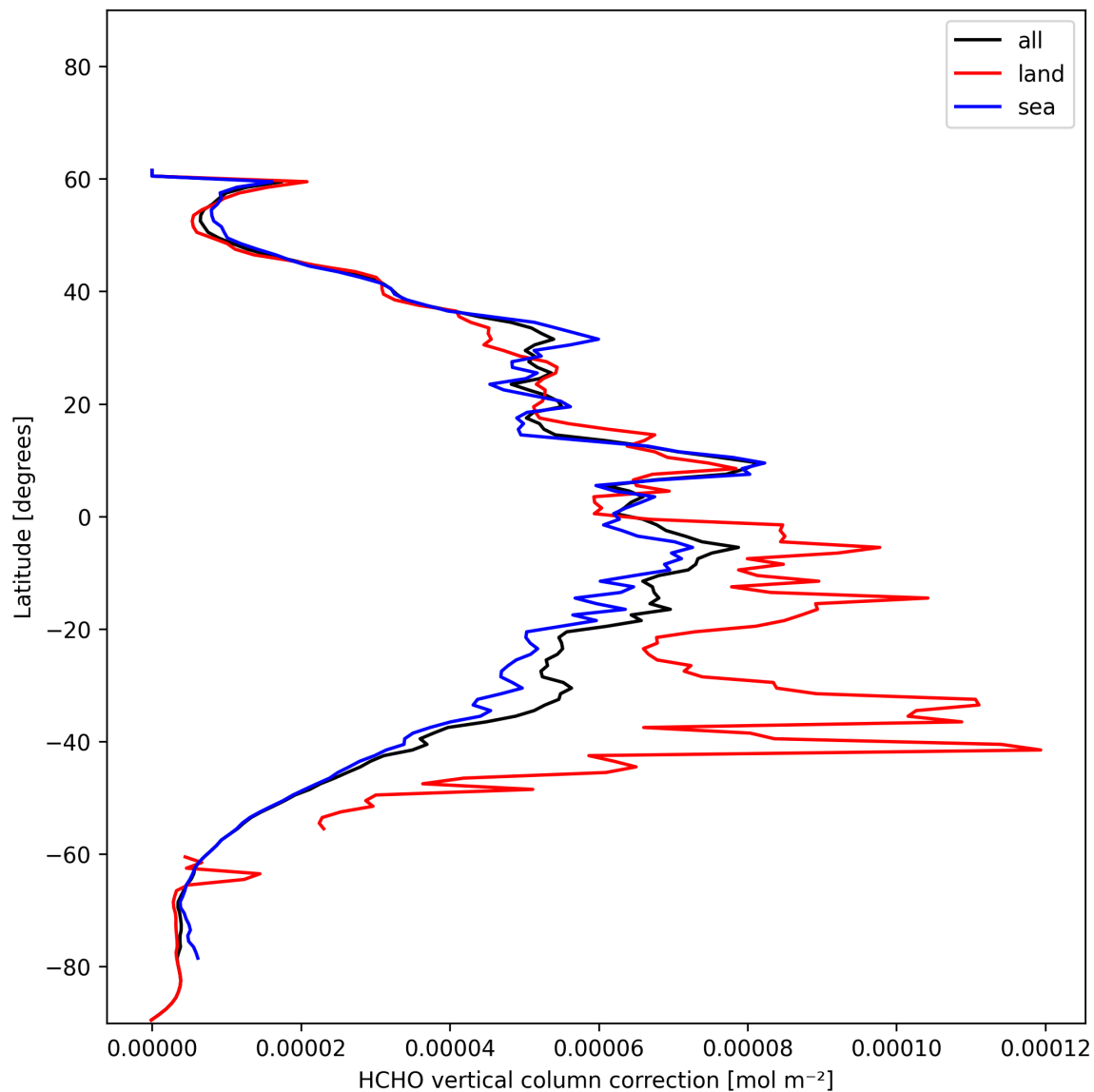
Figure 21: Zonal average of “HCHO vertical column correction” for 2024-12-29 to 2024-12-30.
