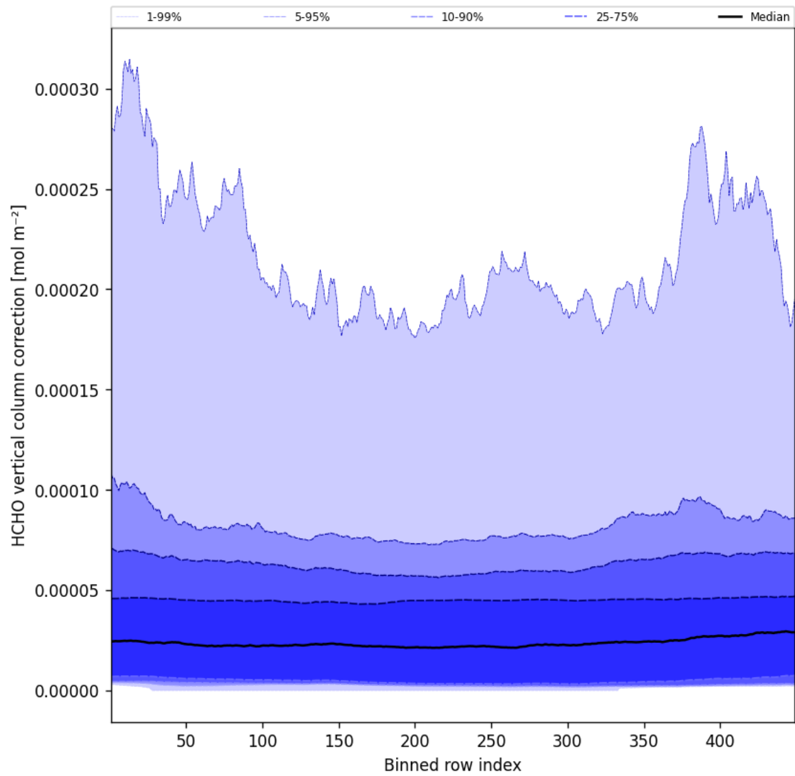
Figure 49: Along track statistics of “HCHO vertical column correction” for 2024-12-29 to 2024-12-30
