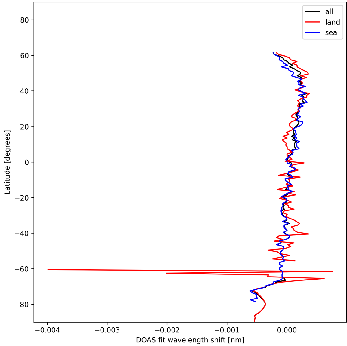
Figure 28: Zonal average of “DOAS fit wavelength shift” for 2024-12-29 to 2024-12-30.
