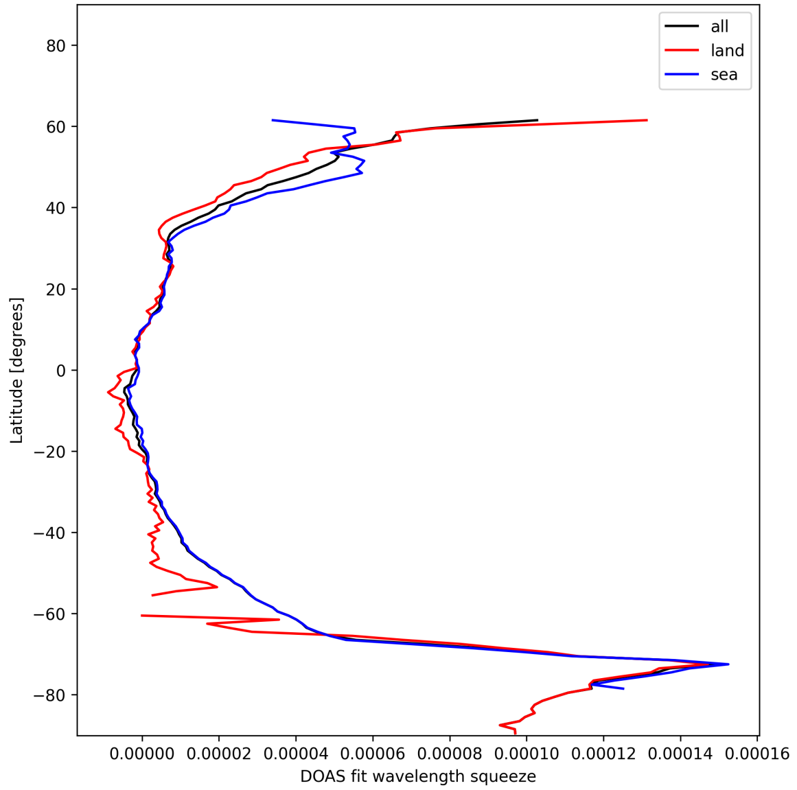
Figure 29: Zonal average of “DOAS fit wavelength squeeze” for 2024-12-29 to 2024-12-30.
