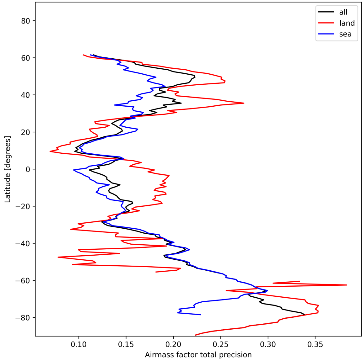
Figure 25: Zonal average of “Airmass factor total precision” for 2024-12-29 to 2024-12-30.
