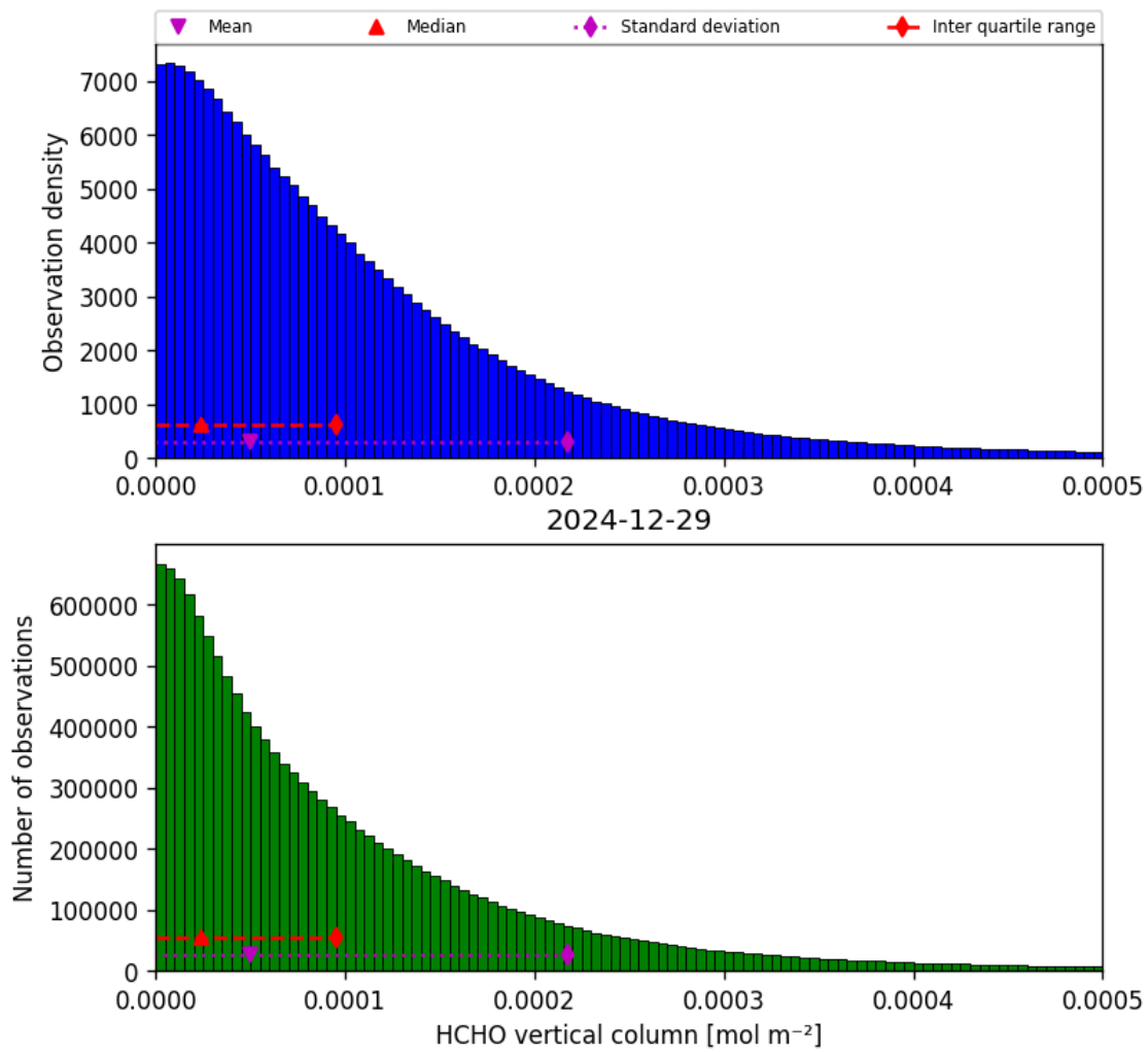
Figure 33: Histogram of “HCHO vertical column” for 2024-12-29 to 2024-12-30
