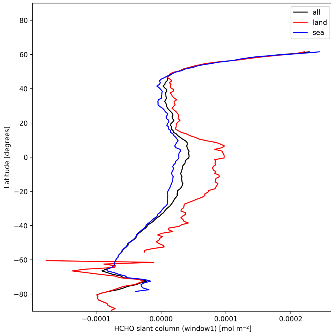
Figure 22: Zonal average of “HCHO slant column (window1)” for 2024-12-29 to 2024-12-30.
