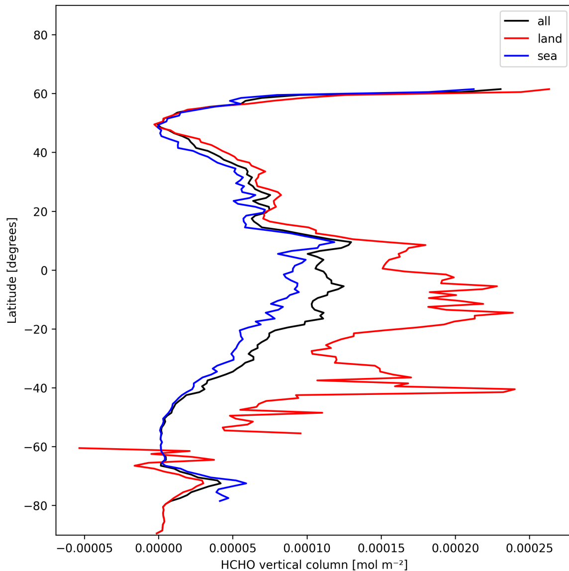
Figure 19: Zonal average of “HCHO vertical column” for 2024-12-29 to 2024-12-30.
