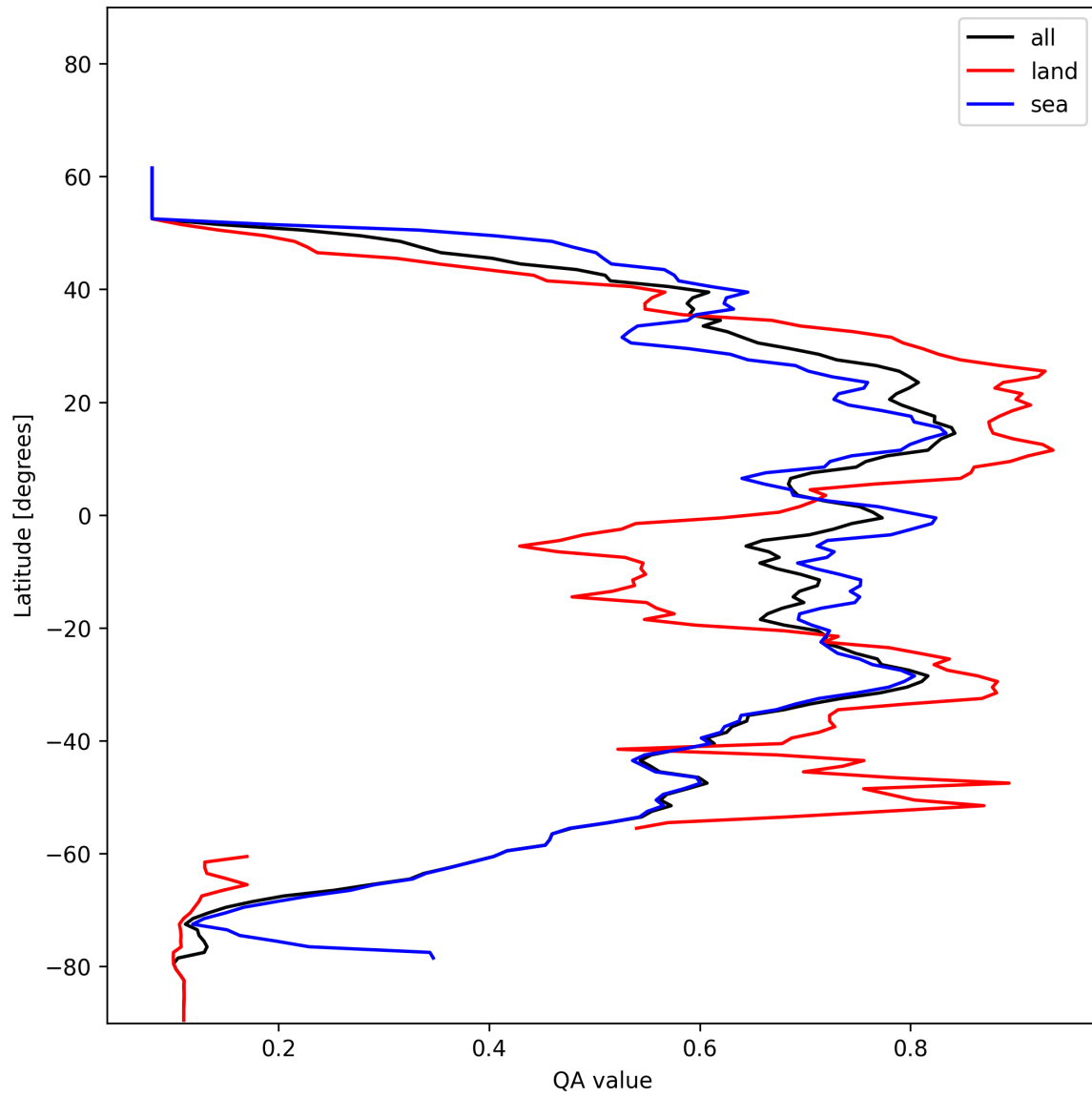
Figure 18: Zonal average of “QA value” for 2024-12-29 to 2024-12-30.
