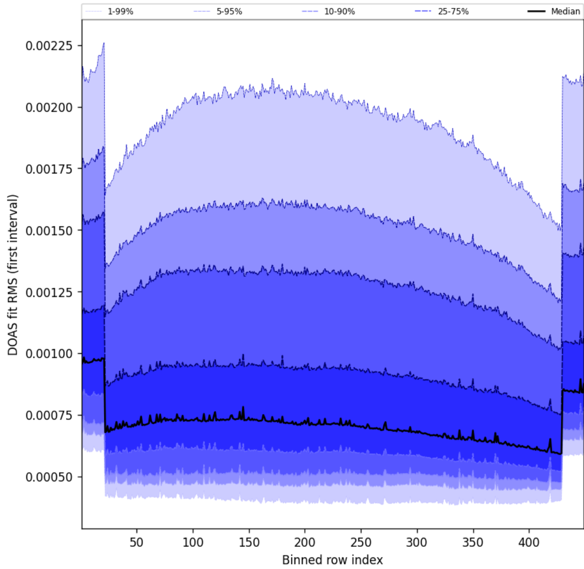
Figure 58: Along track statistics of “DOAS fit RMS (first interval)” for 2024-12-29 to 2024-12-30
