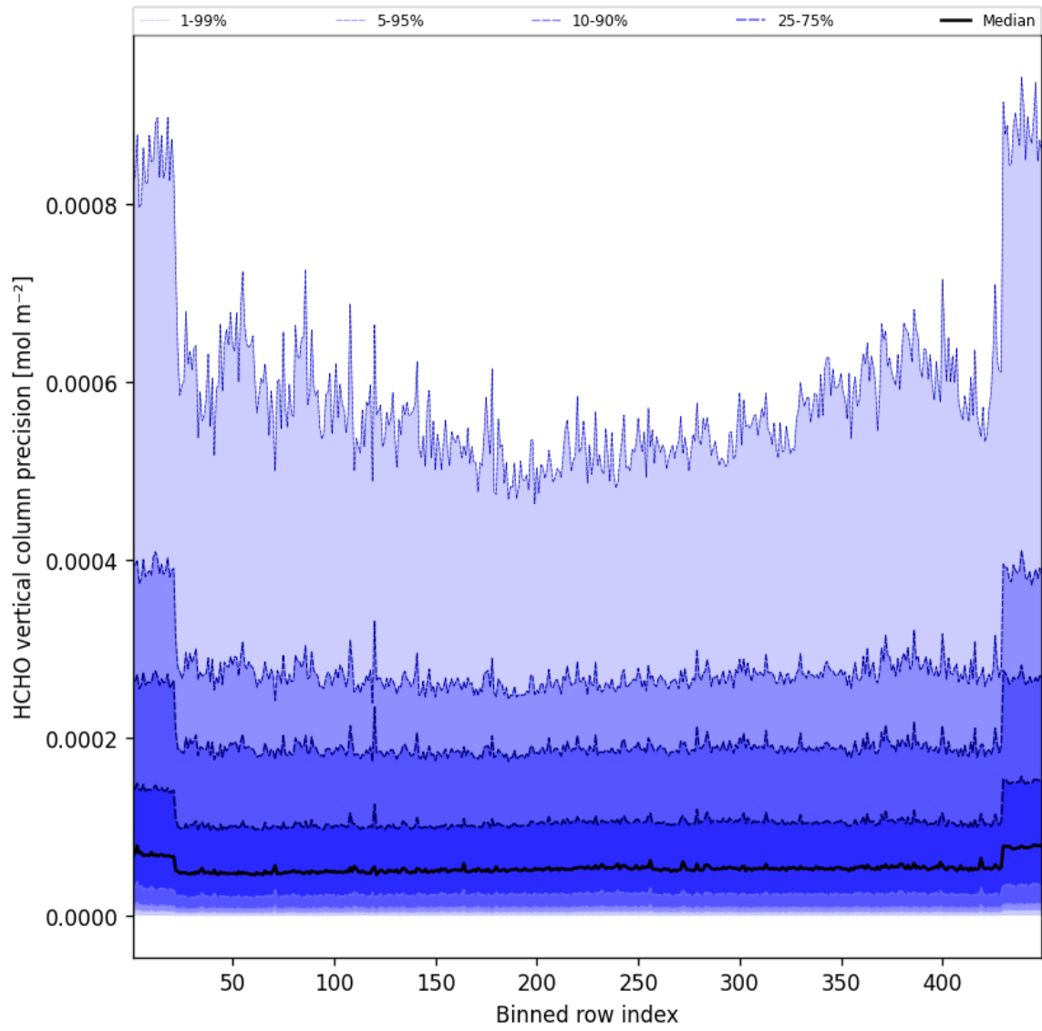
Figure 48: Along track statistics of “HCHO vertical column precision” for 2024-12-29 to 2024-12-30
