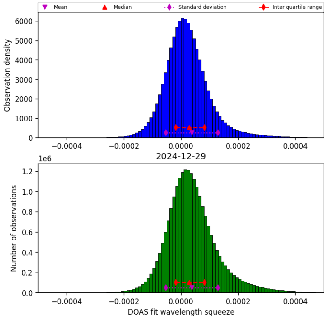
Figure 43: Histogram of “DOAS fit wavelength squeeze” for 2024-12-29 to 2024-12-30
