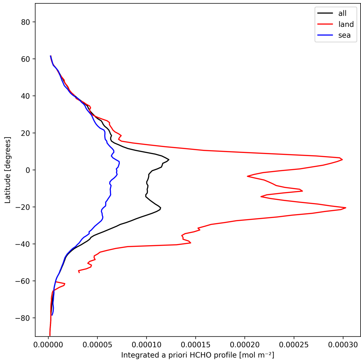
Figure 27: Zonal average of “Integrated a priori HCHO profile” for 2024-12-29 to 2024-12-30.
