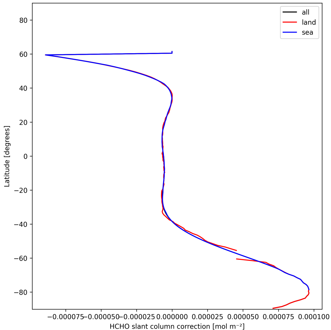
Figure 31: Zonal average of “HCHO slant column correction” for 2024-12-29 to 2024-12-30.
