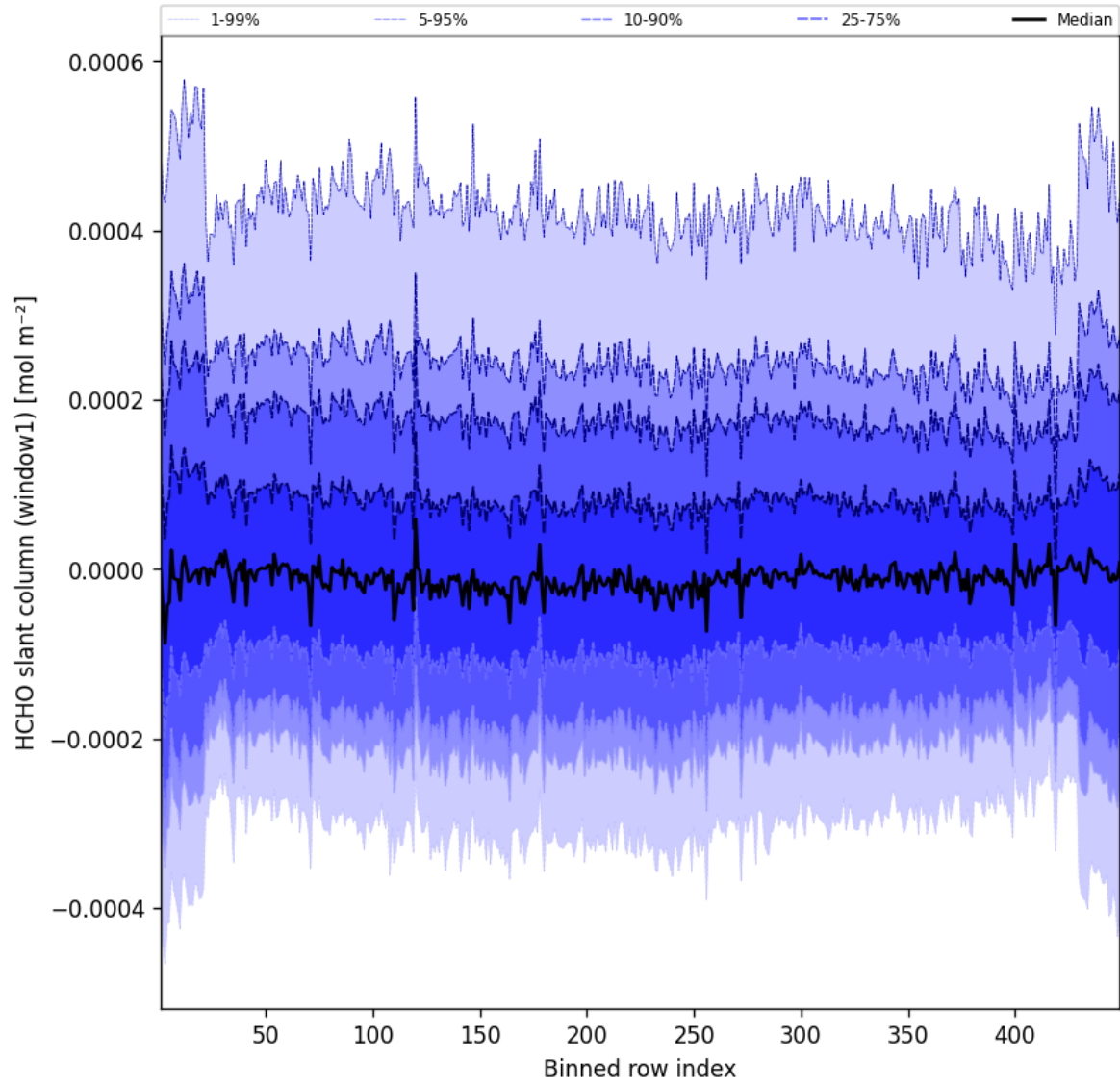
Figure 50: Along track statistics of “HCHO slant column (window1)” for 2024-12-29 to 2024-12-30
