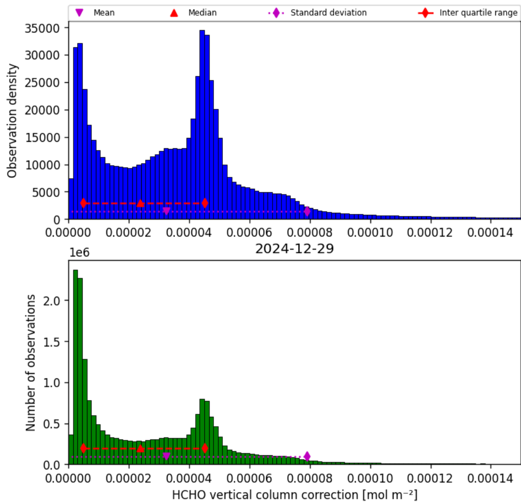
Figure 35: Histogram of “HCHO vertical column correction” for 2024-12-29 to 2024-12-30
