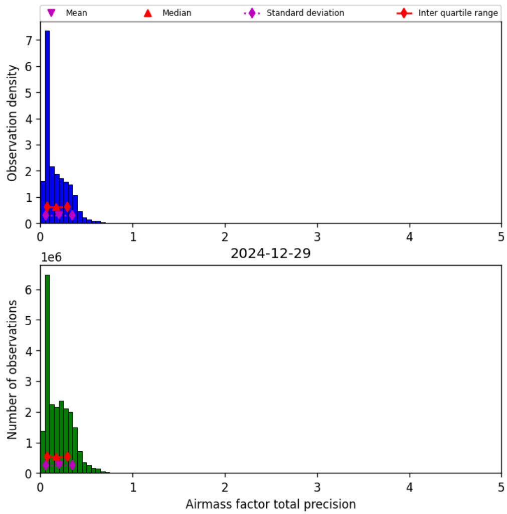
Figure 39: Histogram of “Airmass factor total precision” for 2024-12-29 to 2024-12-30
