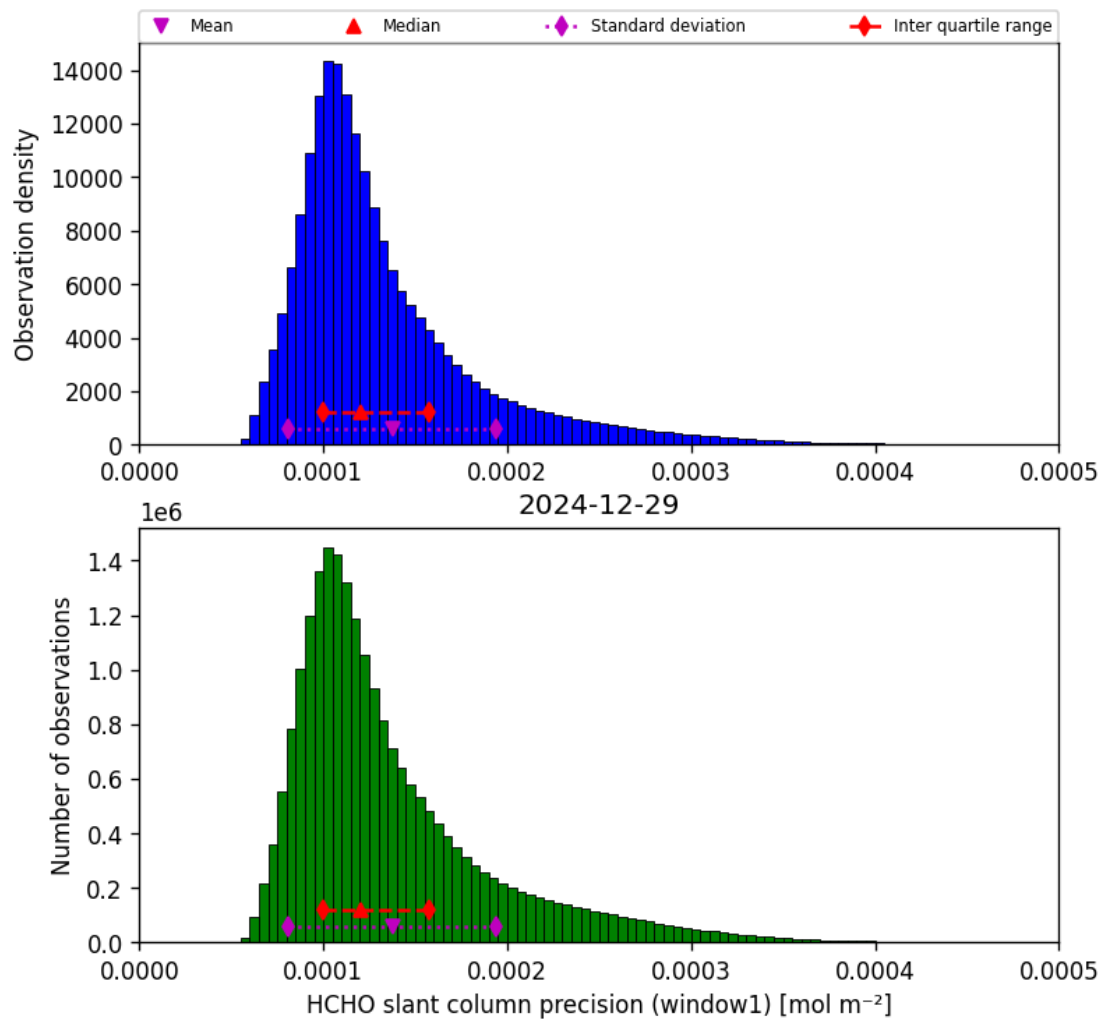
Figure 37: Histogram of “HCHO slant column precision (window1)” for 2024-12-29 to 2024-12-30
