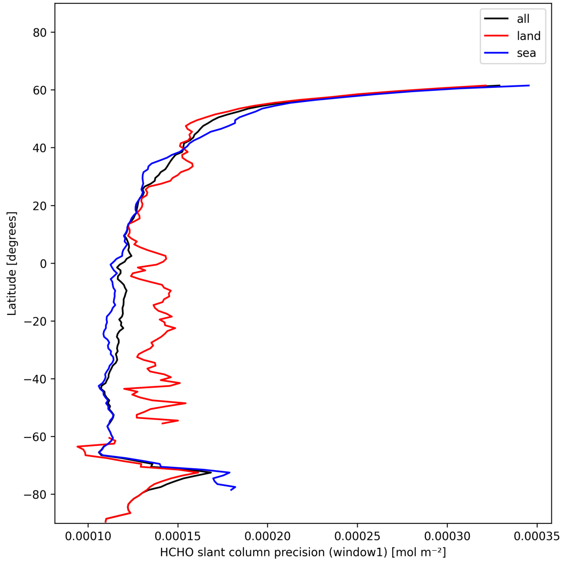
Figure 23: Zonal average of “HCHO slant column precision (window1)” for 2024-12-29 to 2024-12-30.
