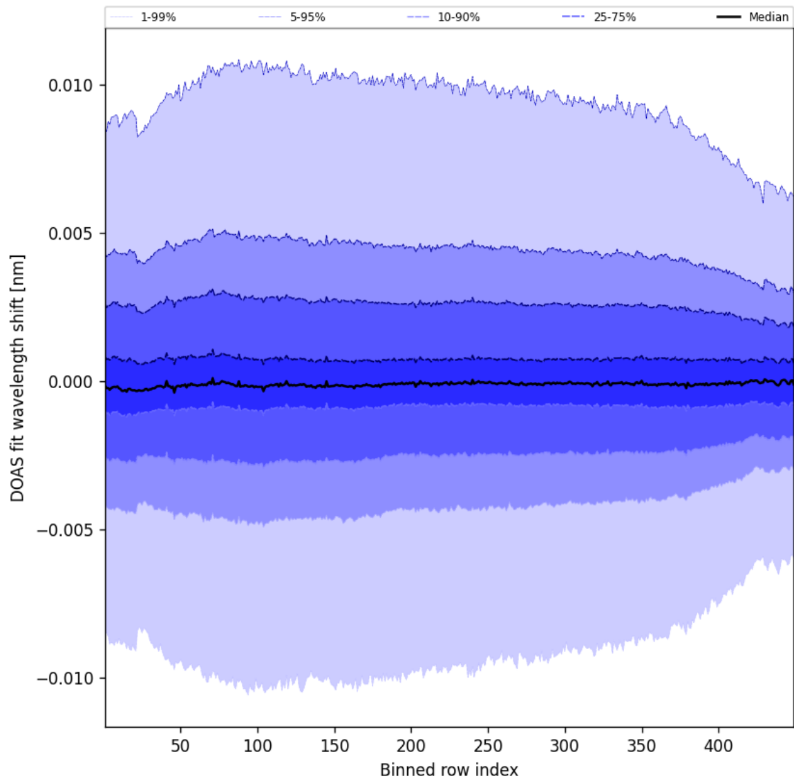
Figure 56: Along track statistics of “DOAS fit wavelength shift” for 2024-12-29 to 2024-12-30
