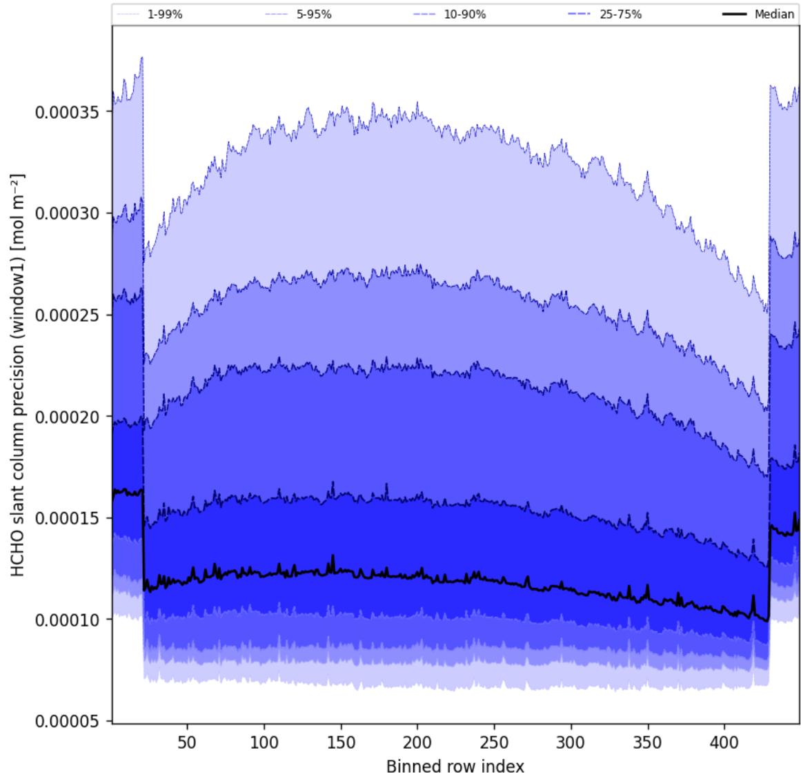
Figure 51: Along track statistics of “HCHO slant column precision (window1)” for 2024-12-29 to 2024-12-30
