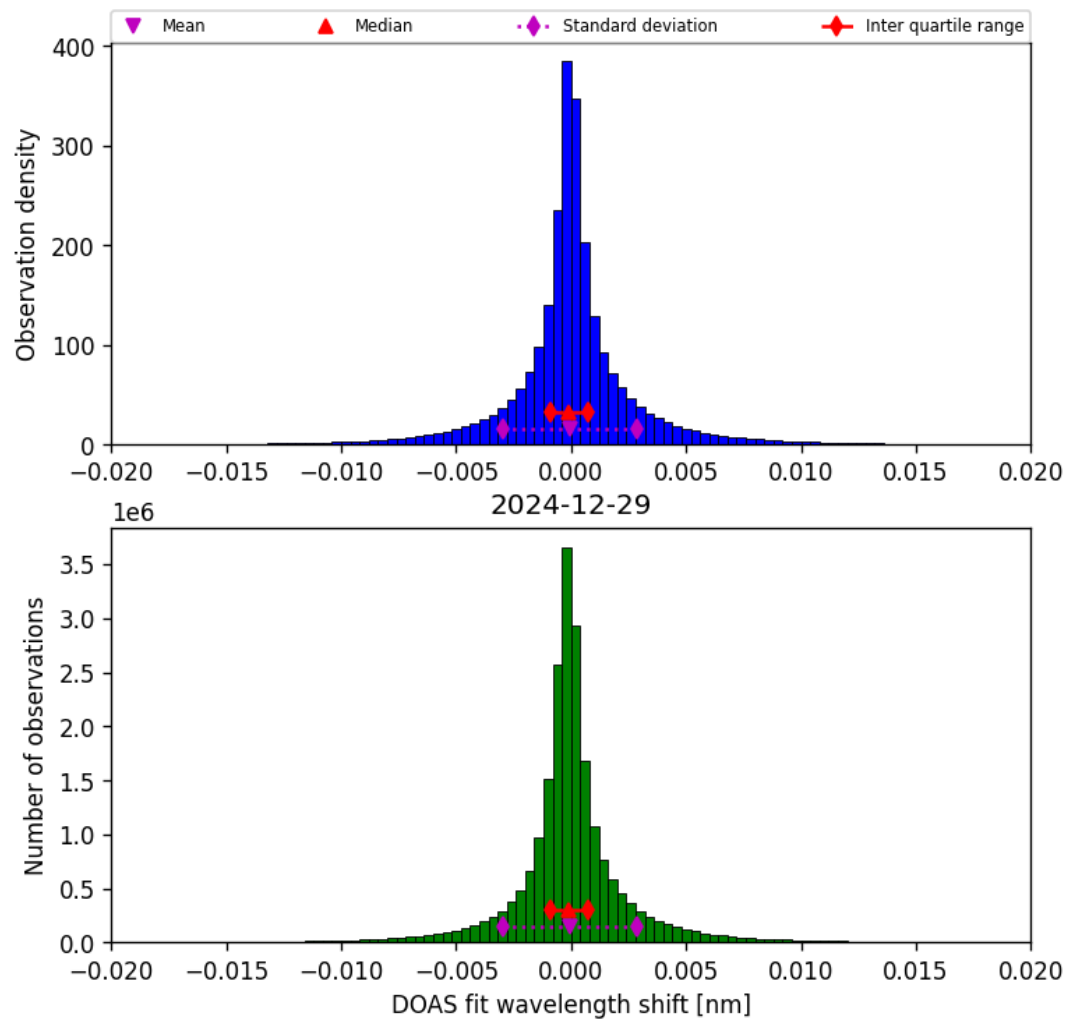
Figure 42: Histogram of “DOAS fit wavelength shift” for 2024-12-29 to 2024-12-30
