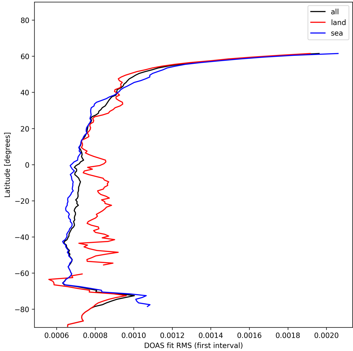
Figure 30: Zonal average of “DOAS fit RMS (first interval)” for 2024-12-29 to 2024-12-30.
