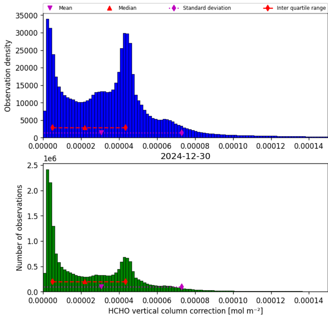
Figure 35: Histogram of “HCHO vertical column correction” for 2024-12-30 to 2024-12-30
