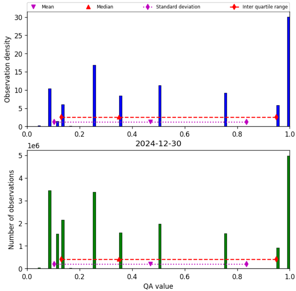
Figure 32: Histogram of “QA value” for 2024-12-30 to 2024-12-30
