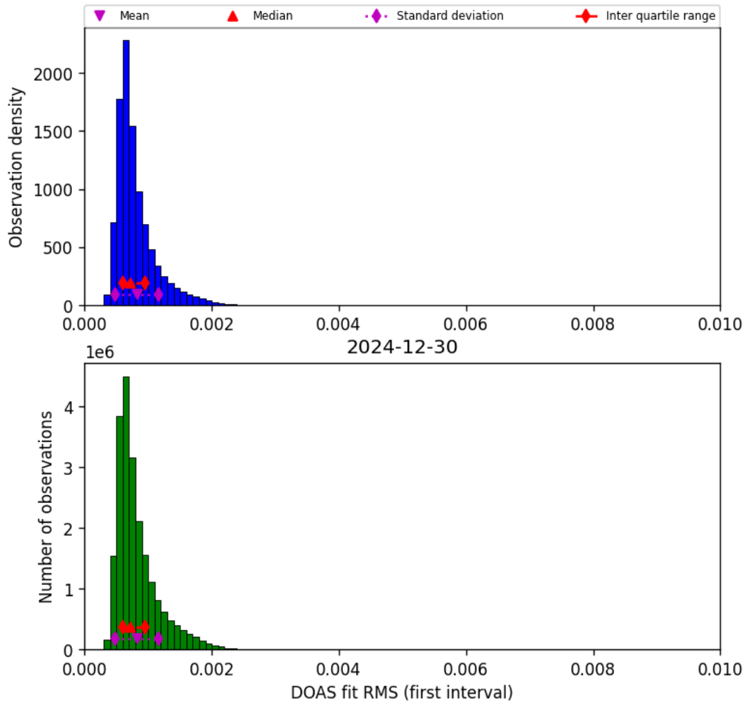
Figure 44: Histogram of “DOAS fit RMS (first interval)” for 2024-12-30 to 2024-12-30
