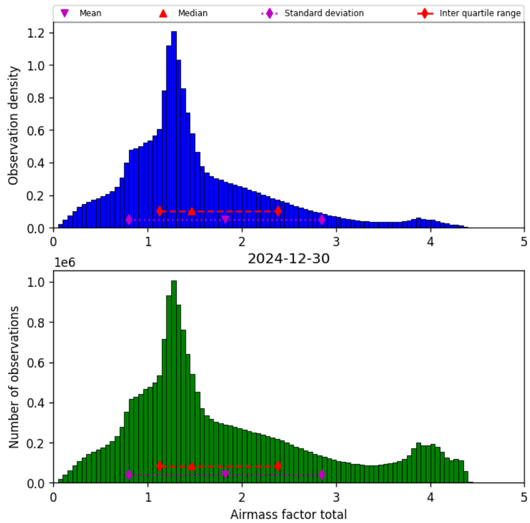
Figure 38: Histogram of “Airmass factor total” for 2024-12-30 to 2024-12-30
