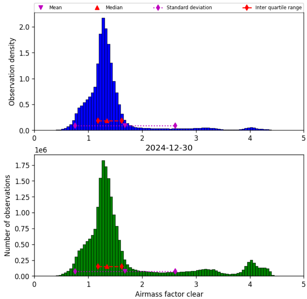
Figure 40: Histogram of “Airmass factor clear” for 2024-12-30 to 2024-12-30
