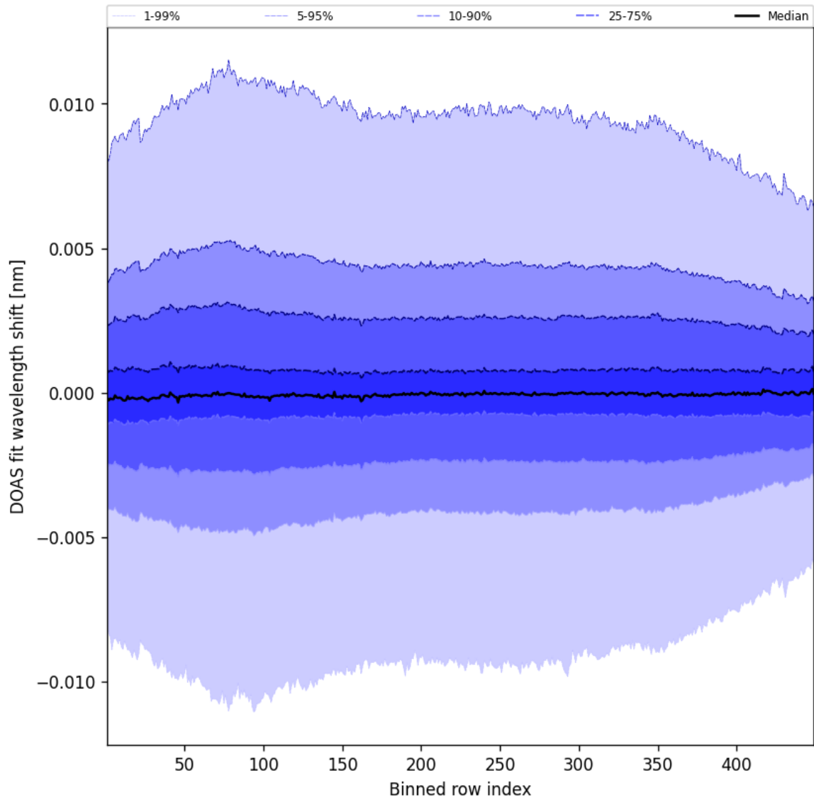
Figure 56: Along track statistics of “DOAS fit wavelength shift” for 2024-12-30 to 2024-12-30
