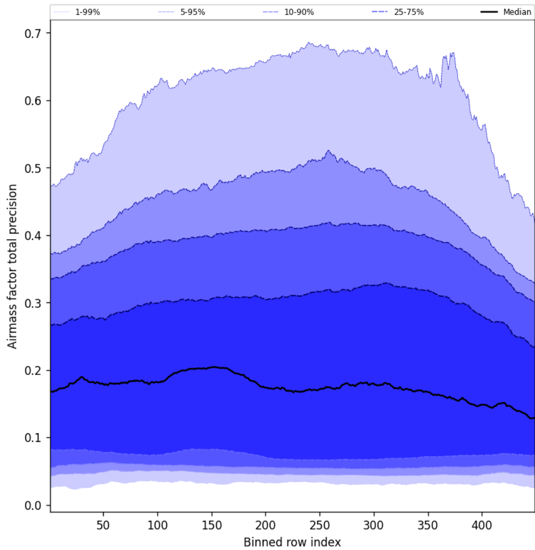
Figure 53: Along track statistics of “Airmass factor total precision” for 2024-12-30 to 2024-12-30
