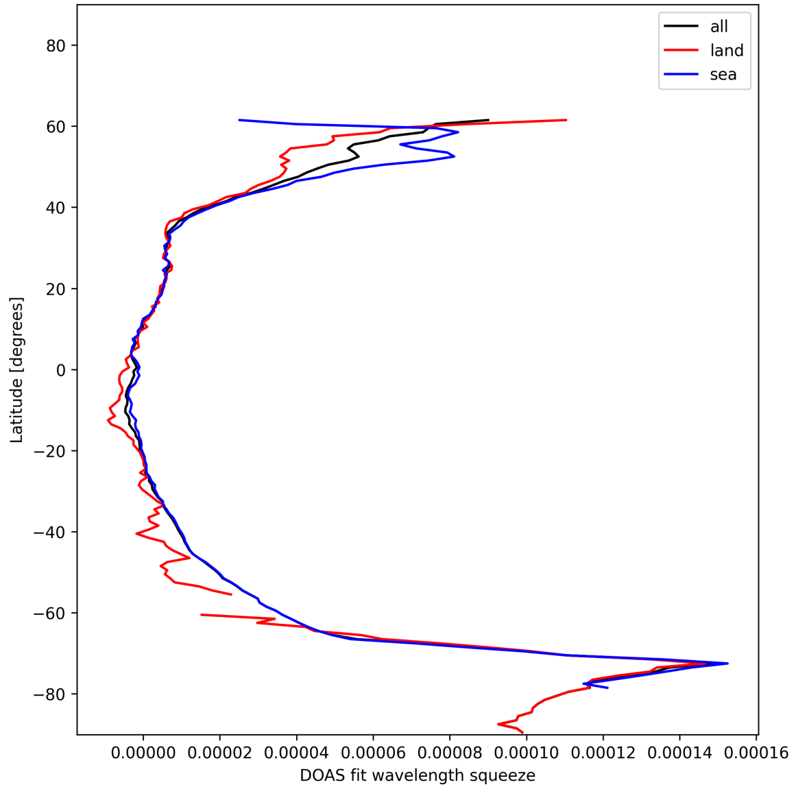
Figure 29: Zonal average of “DOAS fit wavelength squeeze” for 2024-12-30 to 2024-12-30.
