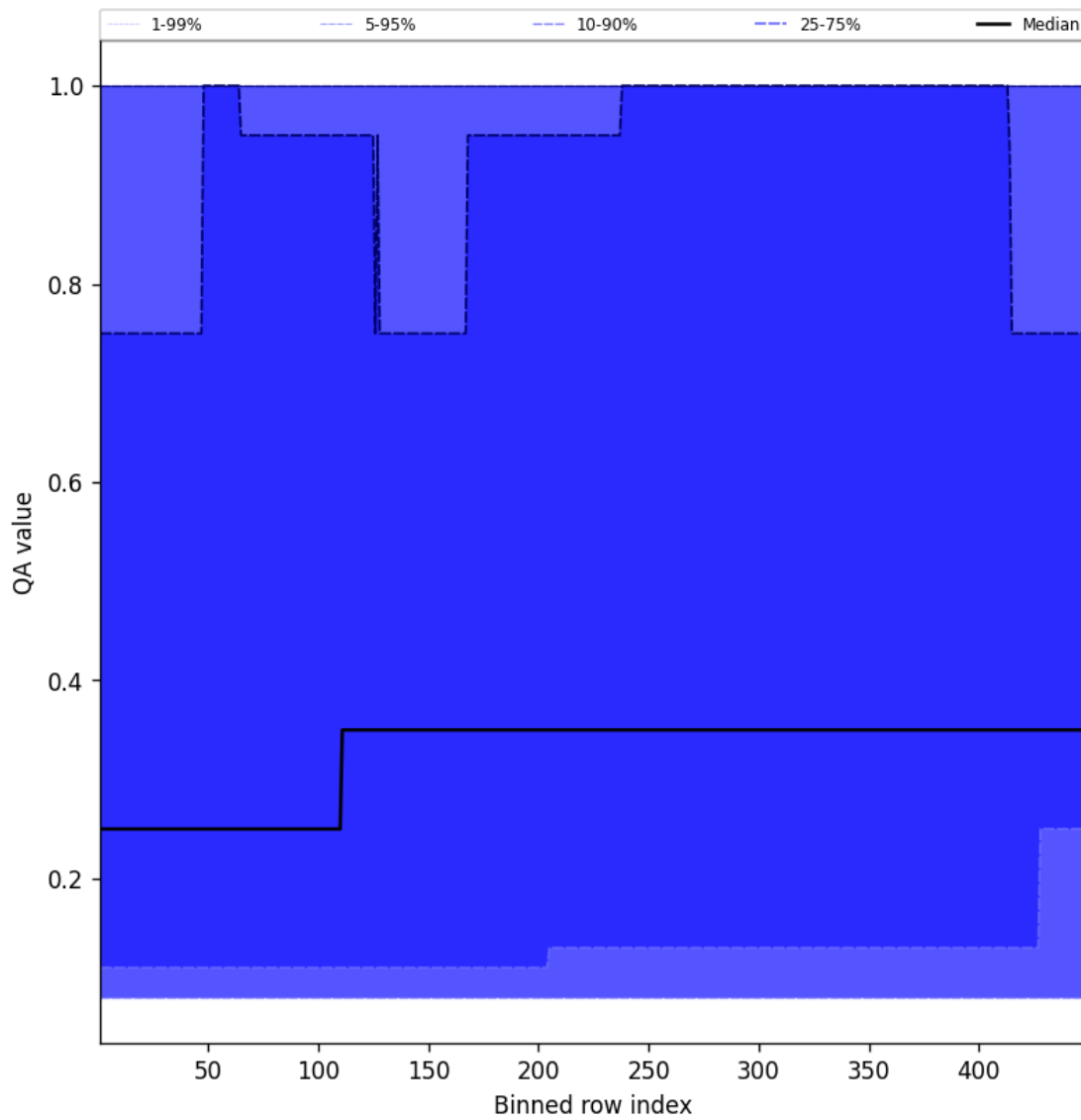
Figure 46: Along track statistics of “QA value” for 2024-12-30 to 2024-12-30
