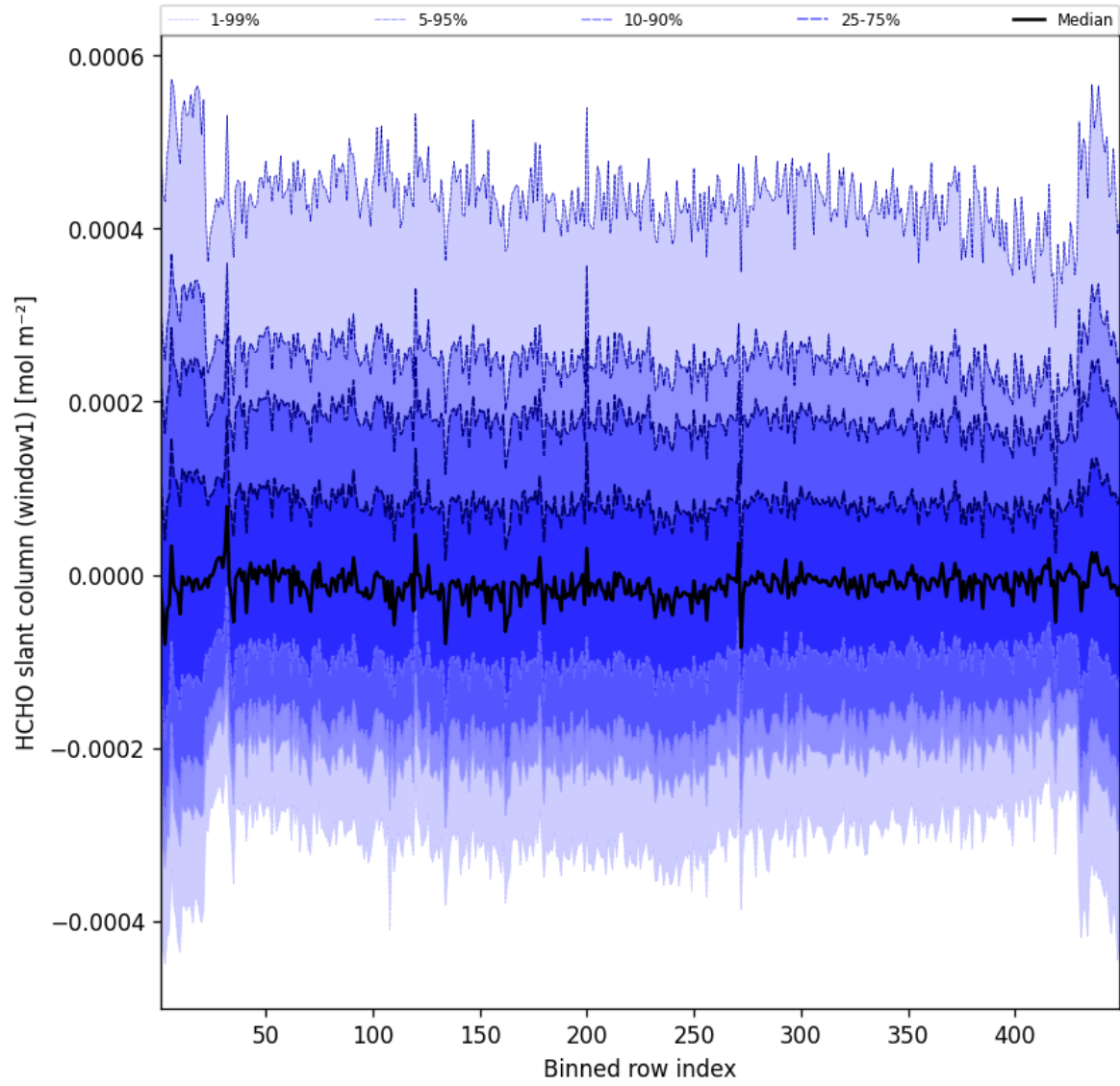
Figure 50: Along track statistics of “HCHO slant column (window1)” for 2024-12-30 to 2024-12-30
