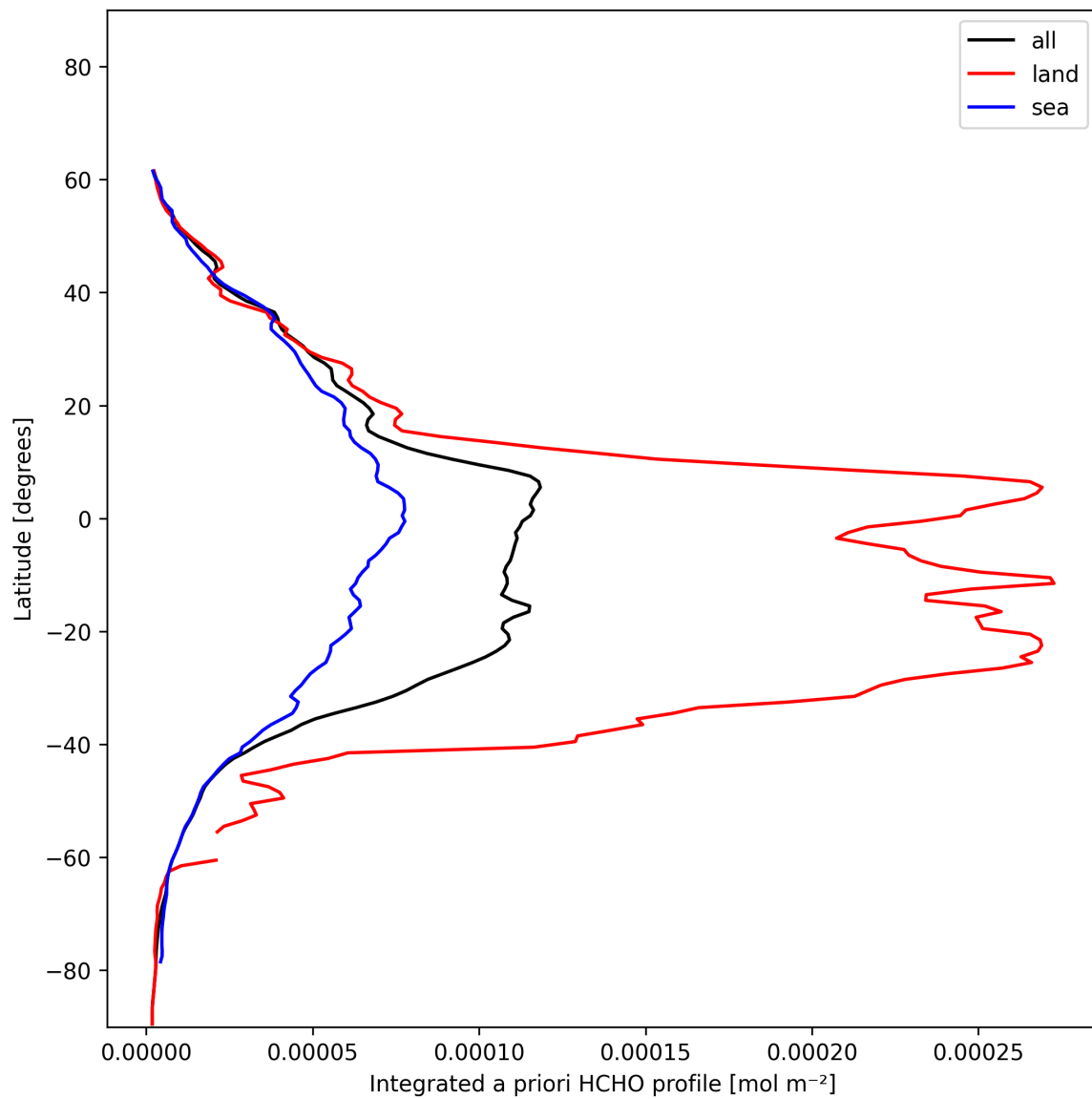
Figure 27: Zonal average of “Integrated a priori HCHO profile” for 2024-12-30 to 2024-12-30.
