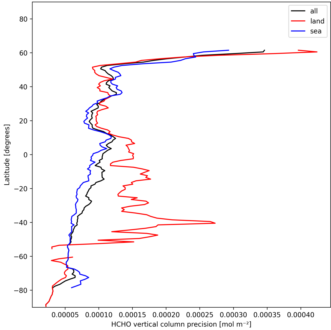
Figure 20: Zonal average of “HCHO vertical column precision” for 2024-12-30 to 2024-12-30.
