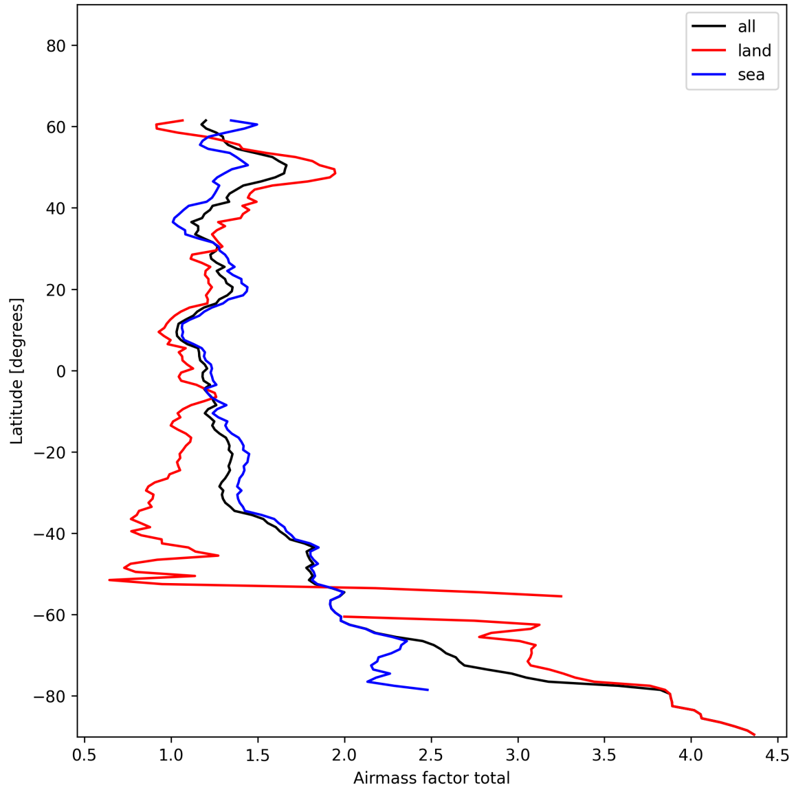
Figure 24: Zonal average of “Airmass factor total” for 2024-12-30 to 2024-12-30.
