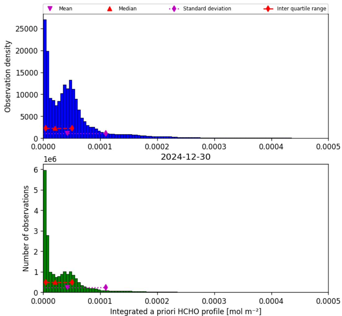
Figure 41: Histogram of “Integrated a priori HCHO profile” for 2024-12-30 to 2024-12-30
