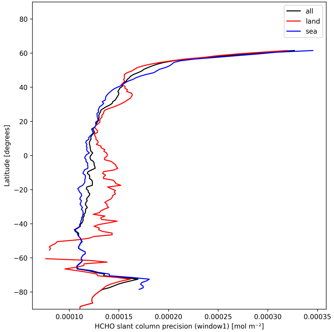
Figure 23: Zonal average of “HCHO slant column precision (window1)” for 2024-12-30 to 2024-12-30.
