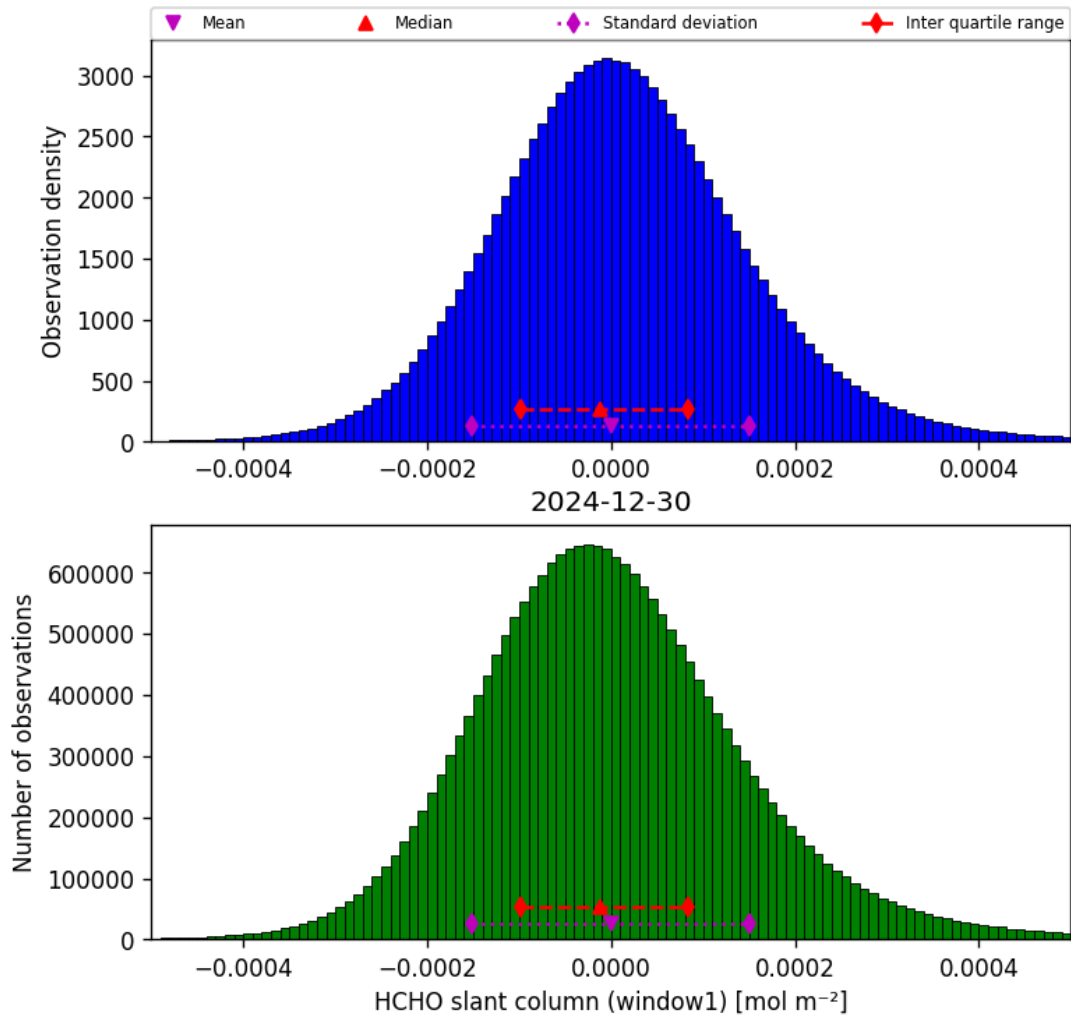
Figure 36: Histogram of “HCHO slant column (window1)” for 2024-12-30 to 2024-12-30
