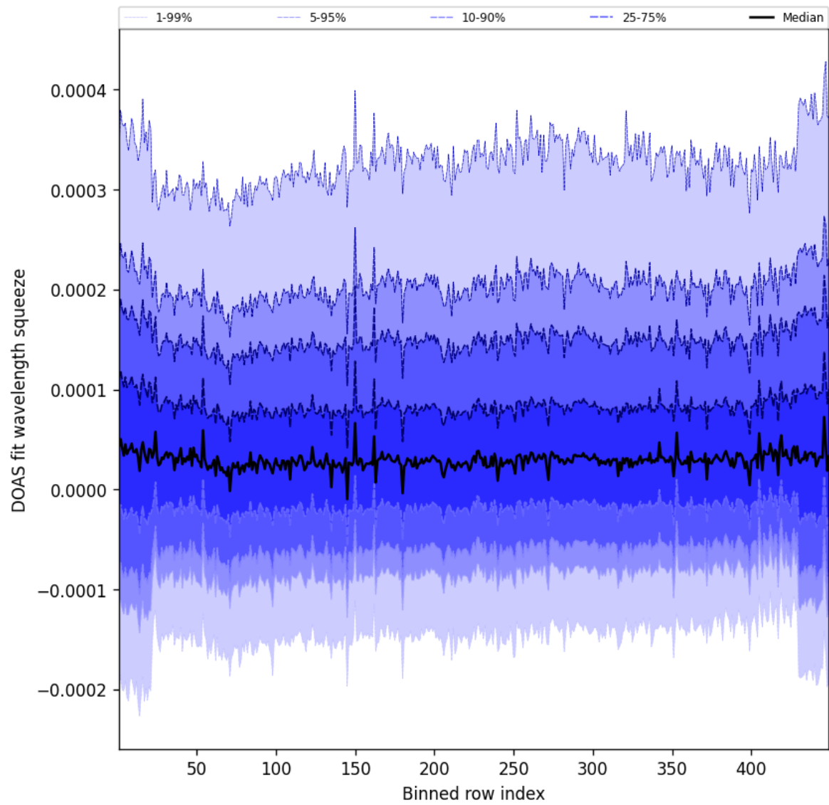
Figure 57: Along track statistics of “DOAS fit wavelength squeeze” for 2024-12-30 to 2024-12-30
