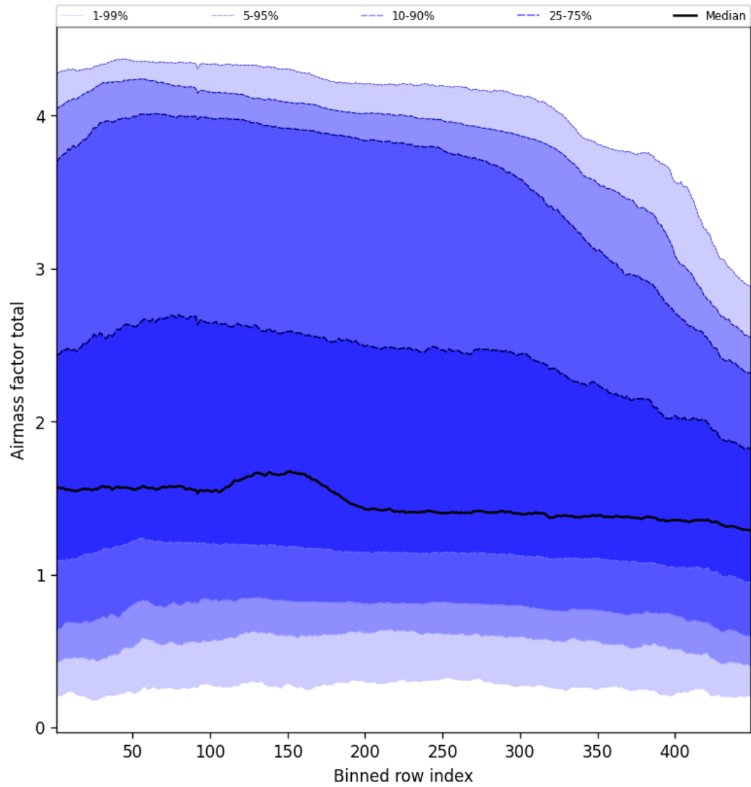
Figure 52: Along track statistics of “Airmass factor total” for 2024-12-30 to 2024-12-30
