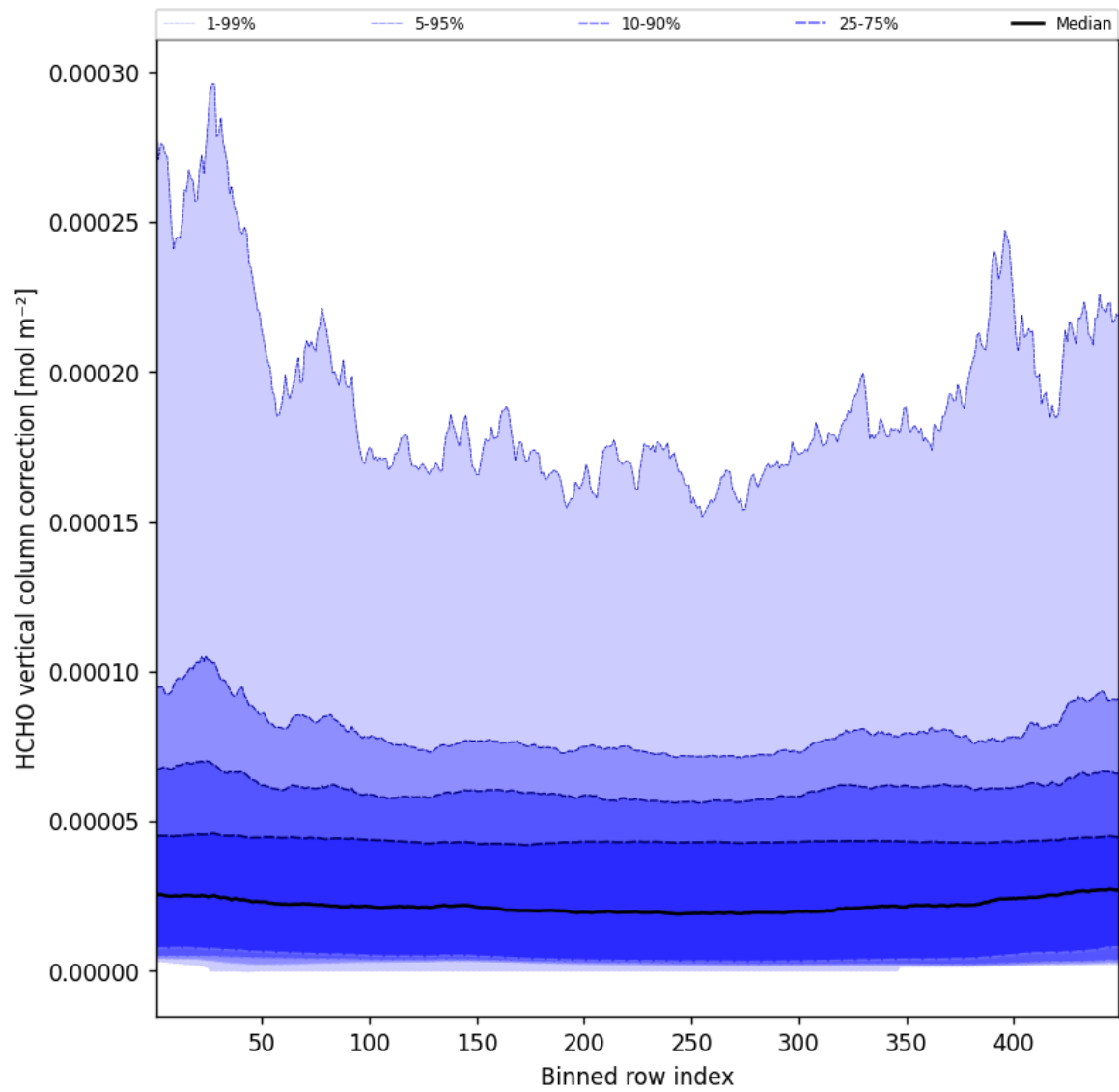
Figure 49: Along track statistics of “HCHO vertical column correction” for 2024-12-30 to 2024-12-30
