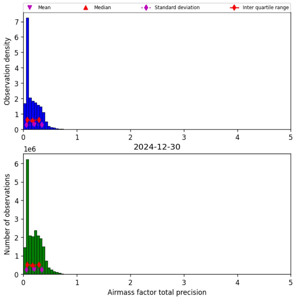
Figure 39: Histogram of “Airmass factor total precision” for 2024-12-30 to 2024-12-30
