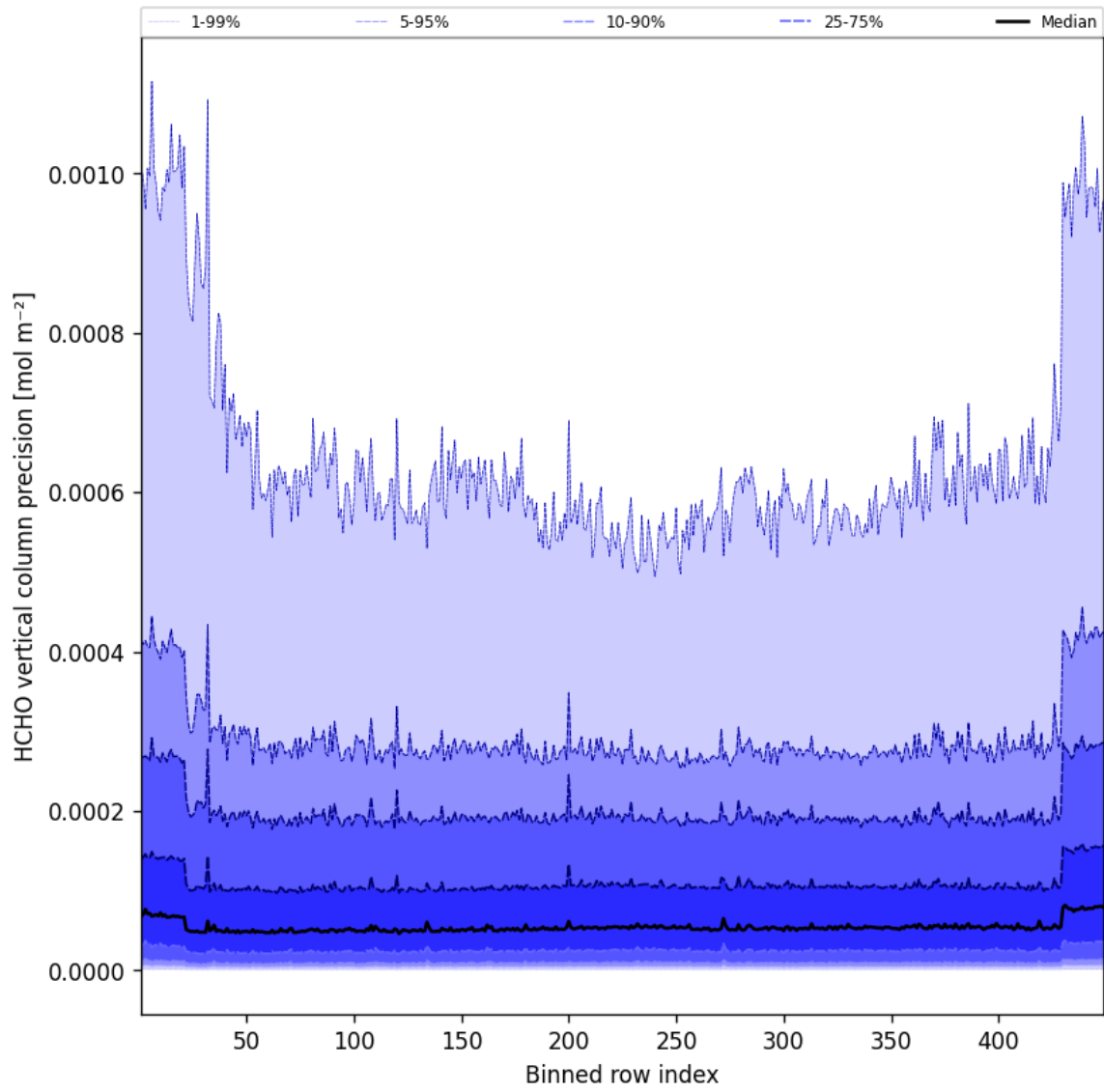
Figure 48: Along track statistics of “HCHO vertical column precision” for 2024-12-30 to 2024-12-30
