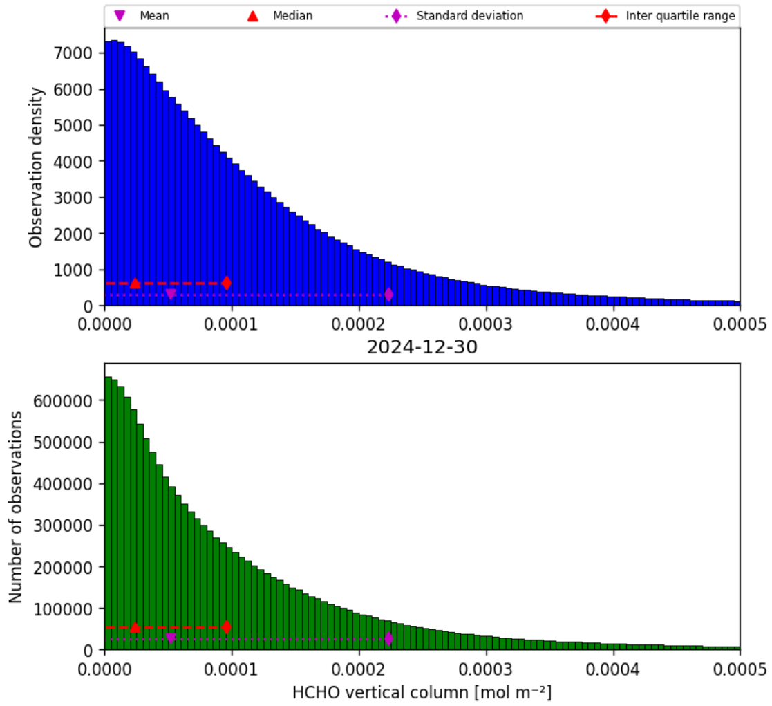
Figure 33: Histogram of “HCHO vertical column” for 2024-12-30 to 2024-12-30
