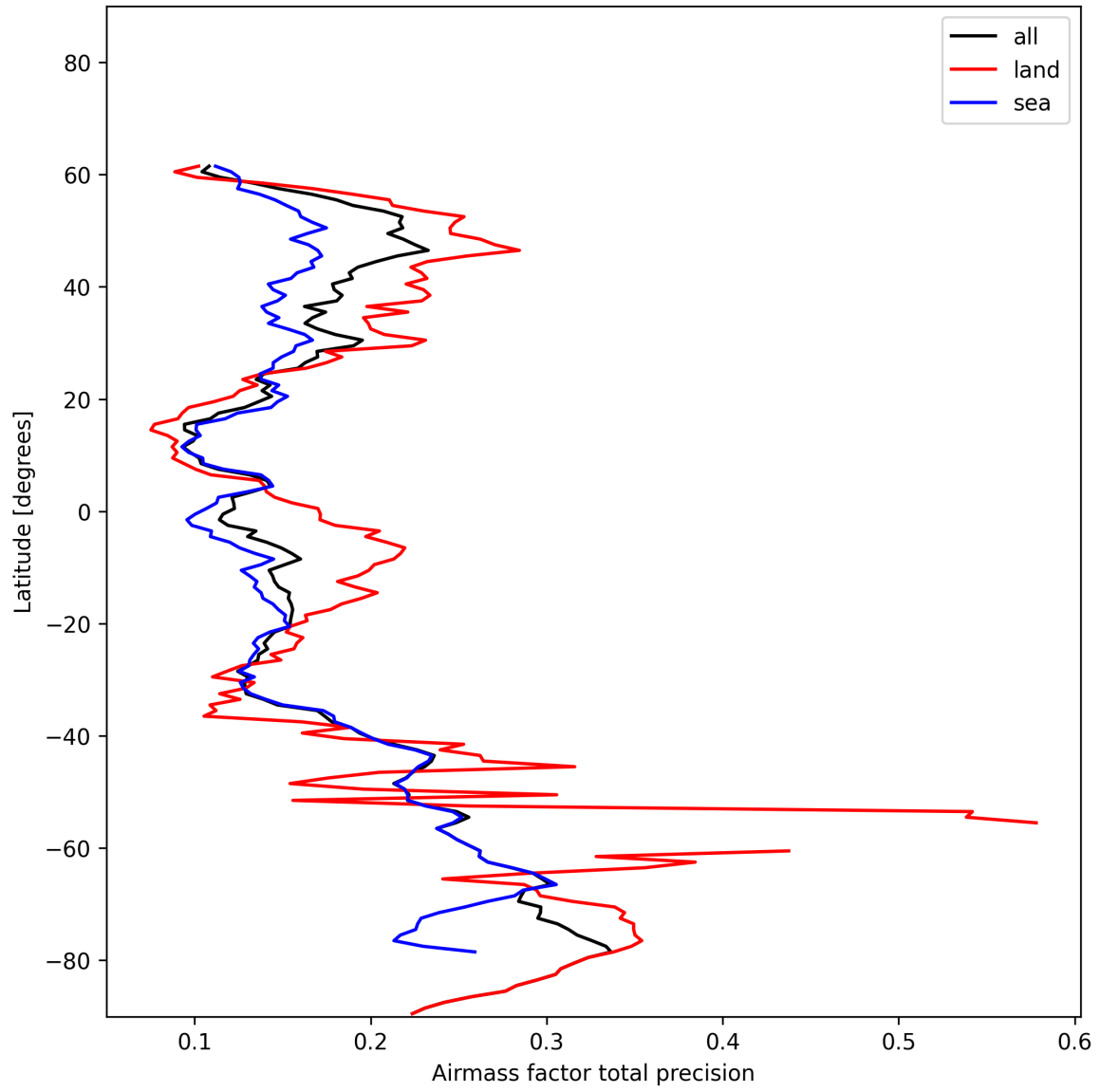
Figure 25: Zonal average of “Airmass factor total precision” for 2024-12-30 to 2024-12-30.
