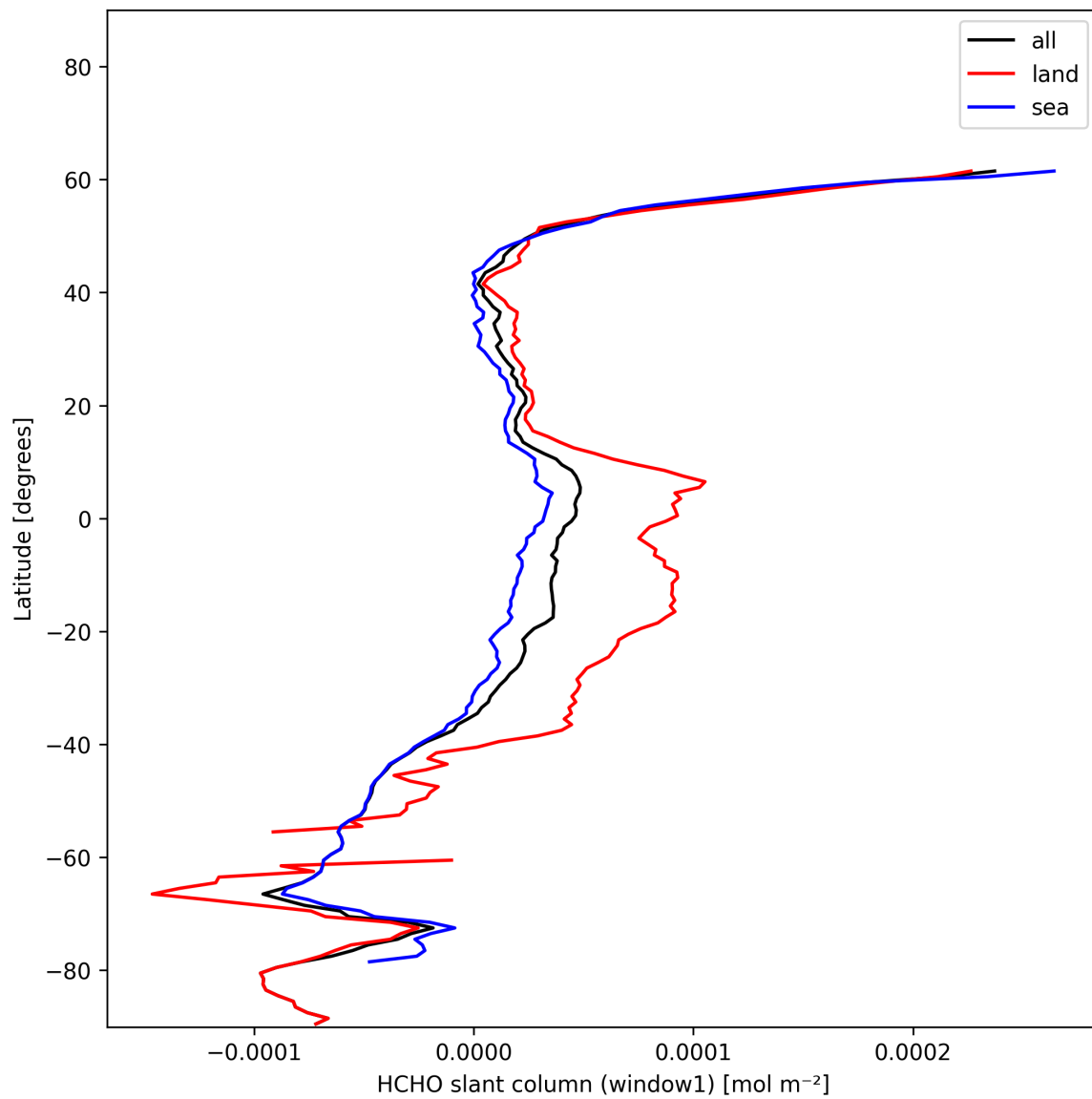
Figure 22: Zonal average of “HCHO slant column (window1)” for 2024-12-30 to 2024-12-30.
