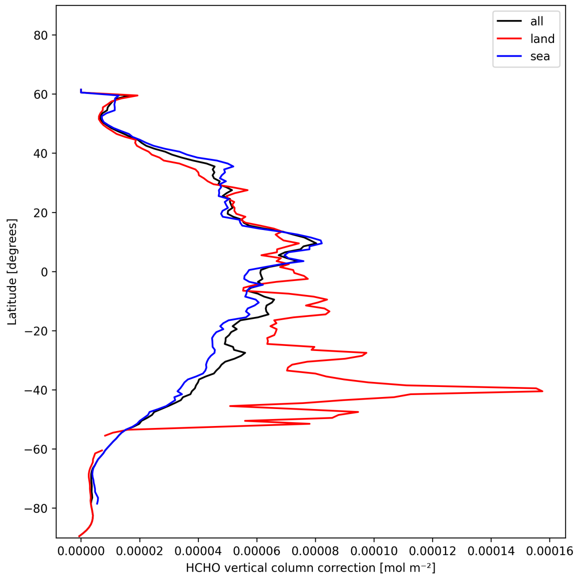
Figure 21: Zonal average of “HCHO vertical column correction” for 2024-12-30 to 2024-12-30.
