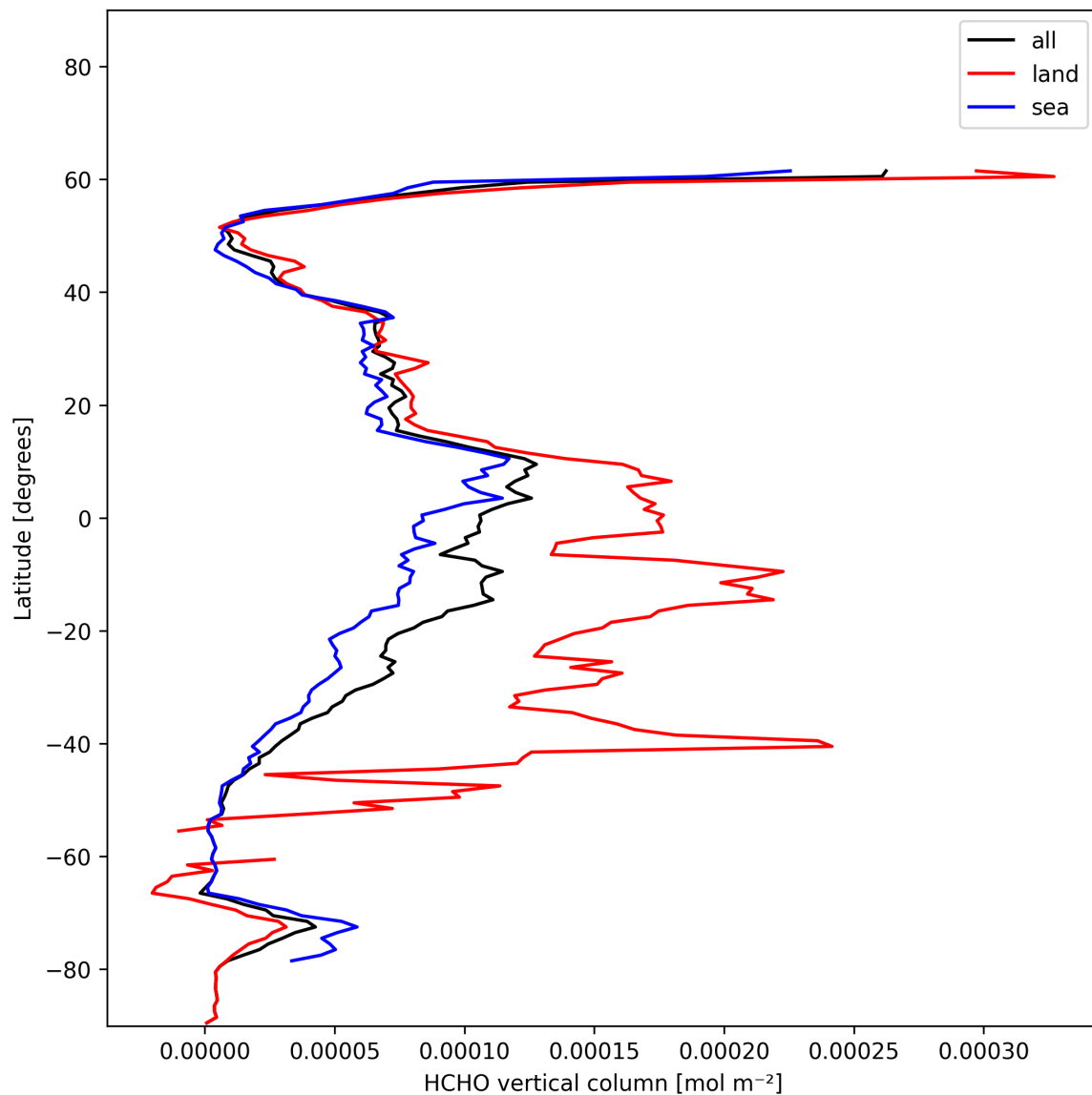
Figure 19: Zonal average of “HCHO vertical column” for 2024-12-30 to 2024-12-30.
