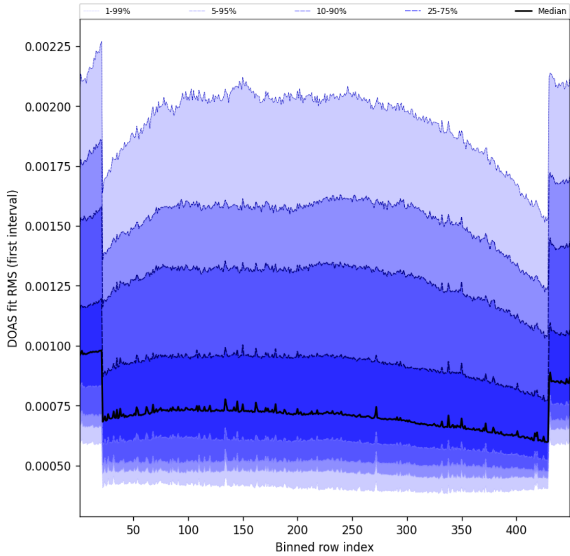
Figure 58: Along track statistics of “DOAS fit RMS (first interval)” for 2024-12-30 to 2024-12-30
