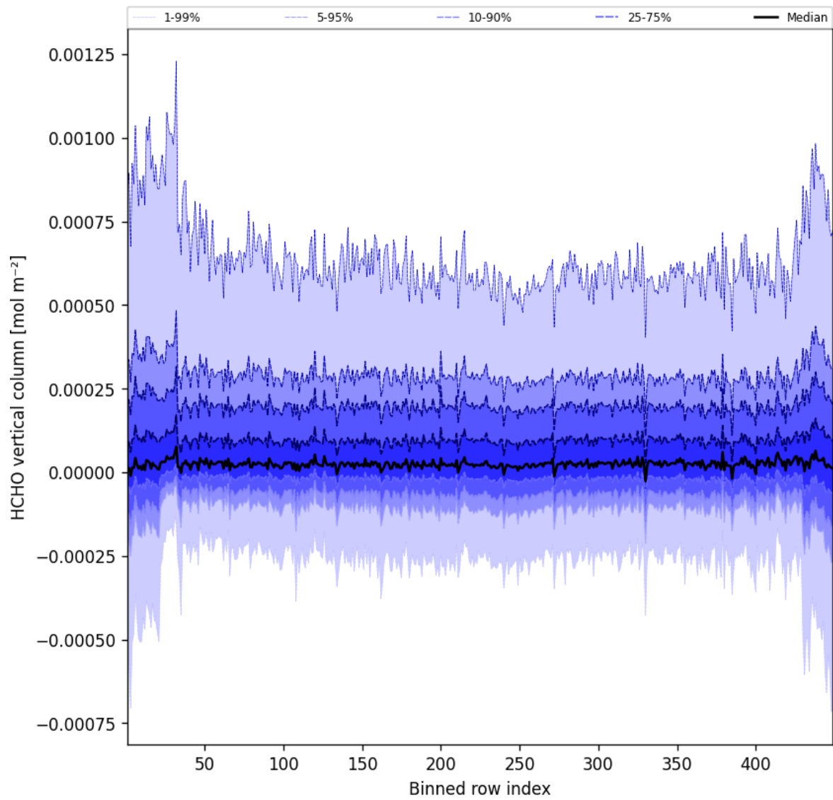
Figure 47: Along track statistics of “HCHO vertical column” for 2024-12-30 to 2024-12-30
