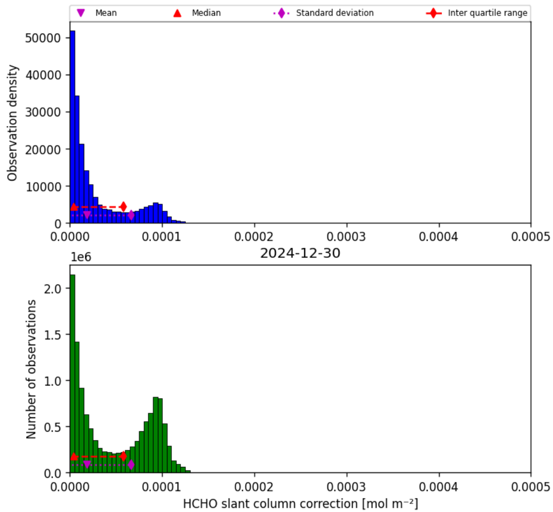
Figure 45: Histogram of “HCHO slant column correction” for 2024-12-30 to 2024-12-30
