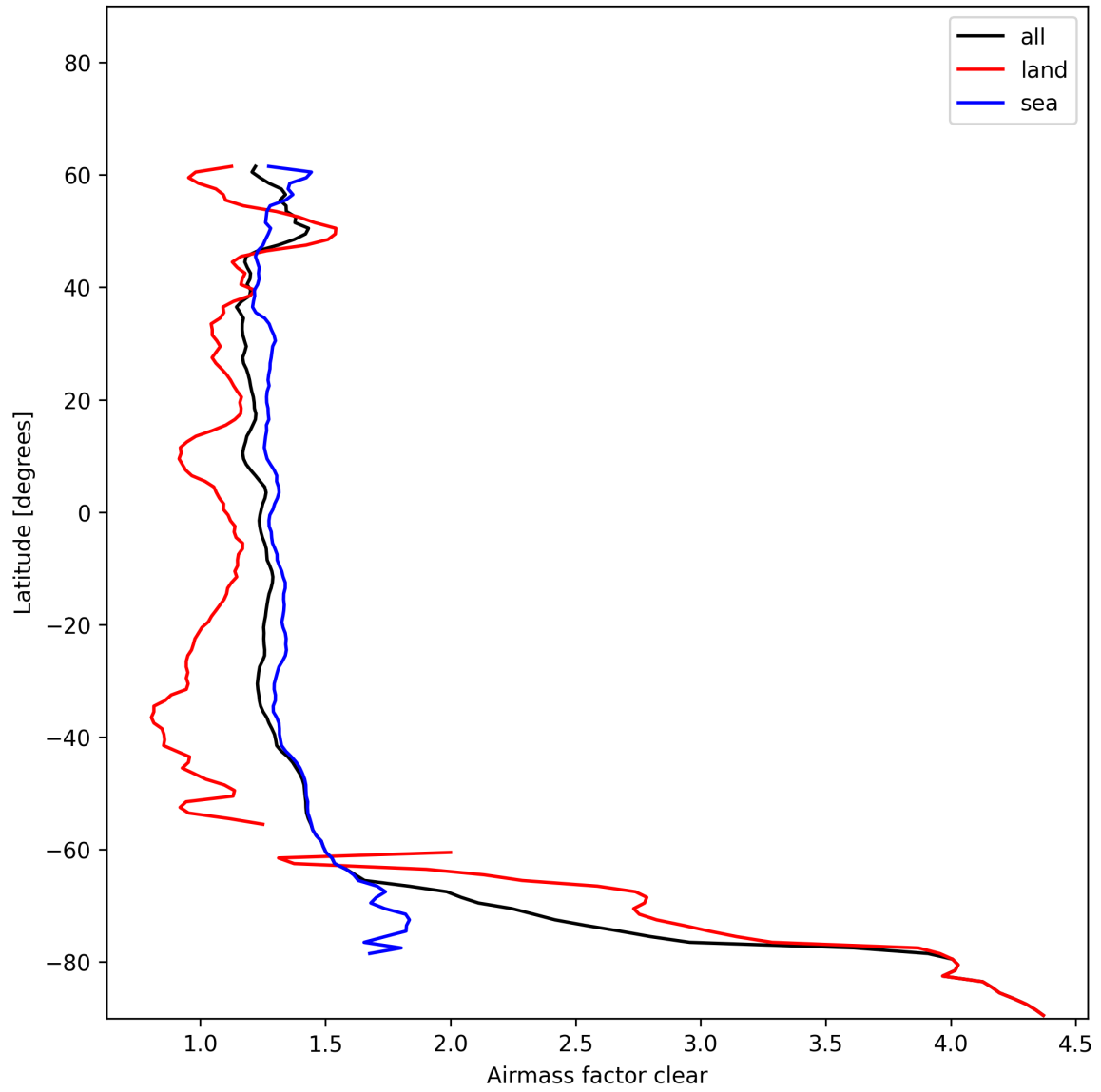
Figure 26: Zonal average of “Airmass factor clear” for 2024-12-30 to 2024-12-30.
