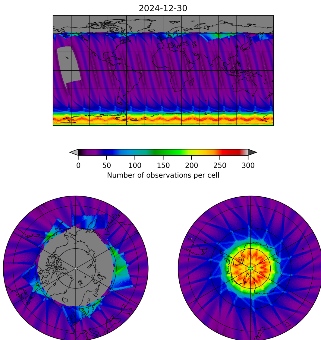
Figure 17: Map of the number of observations for 2024-12-30 to 2024-12-30
