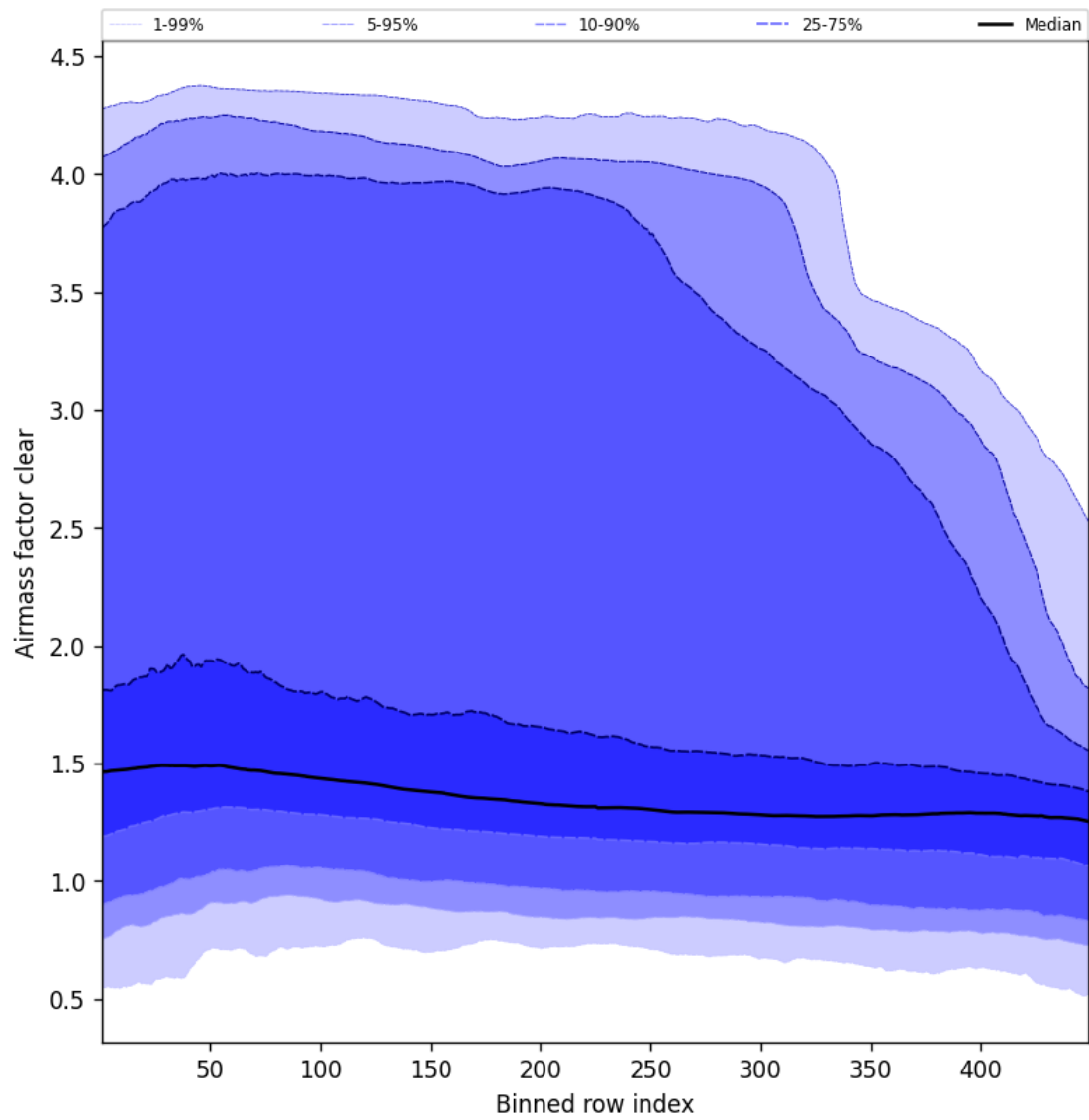
Figure 54: Along track statistics of "Airmass factor clear" for 2024-12-30 to 2024-12-30
