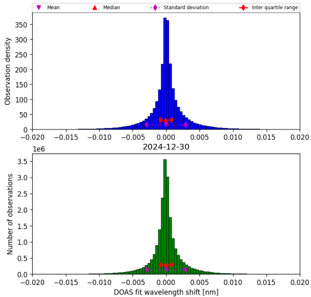
Figure 42: Histogram of “DOAS fit wavelength shift” for 2024-12-30 to 2024-12-30
