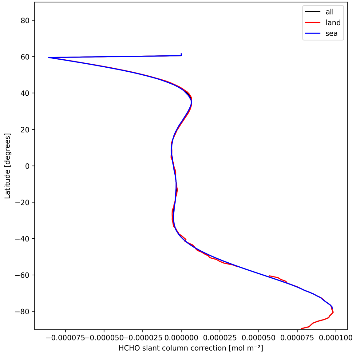
Figure 31: Zonal average of “HCHO slant column correction” for 2024-12-30 to 2024-12-30.
