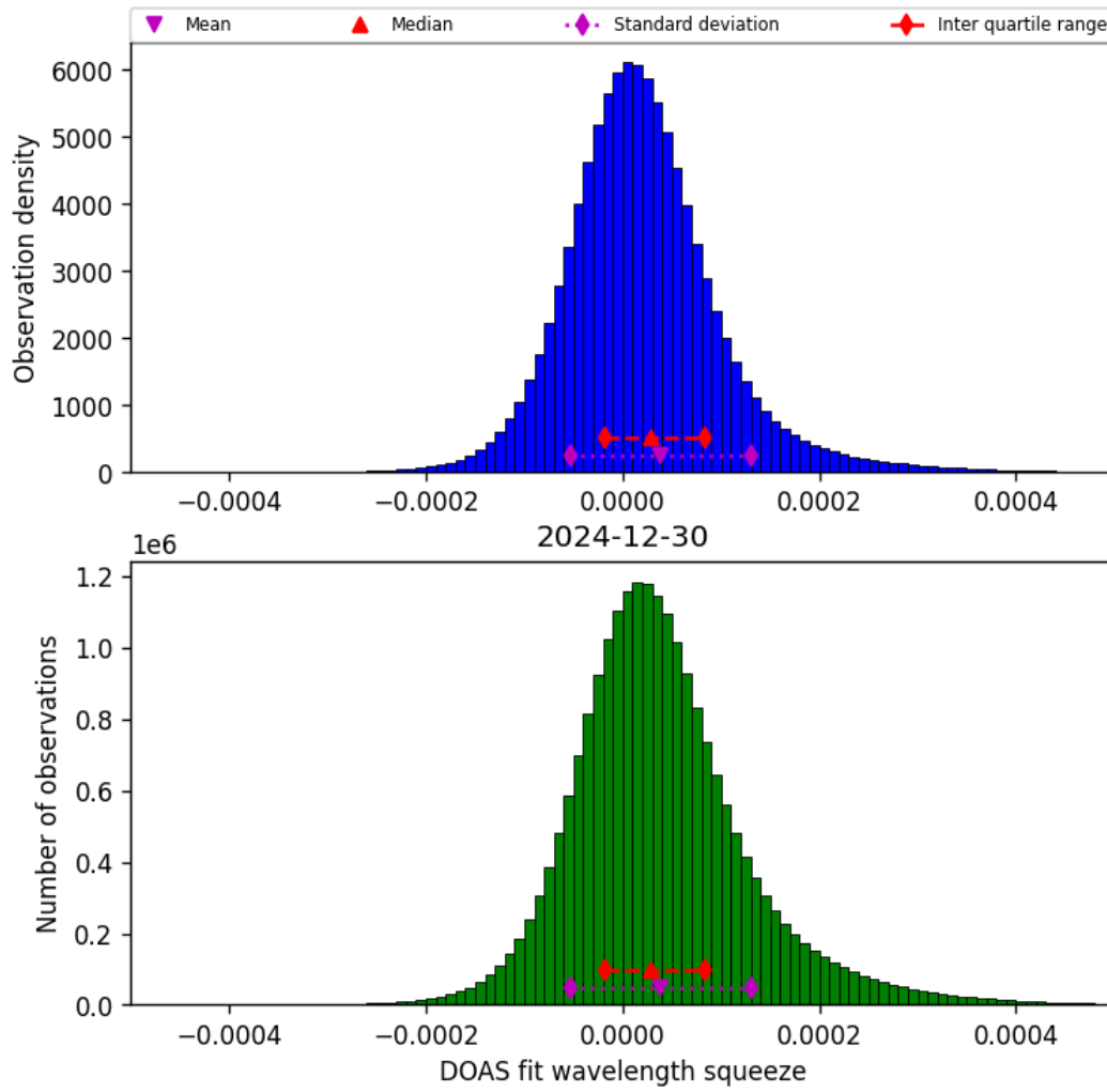
Figure 43: Histogram of “DOAS fit wavelength squeeze” for 2024-12-30 to 2024-12-30
