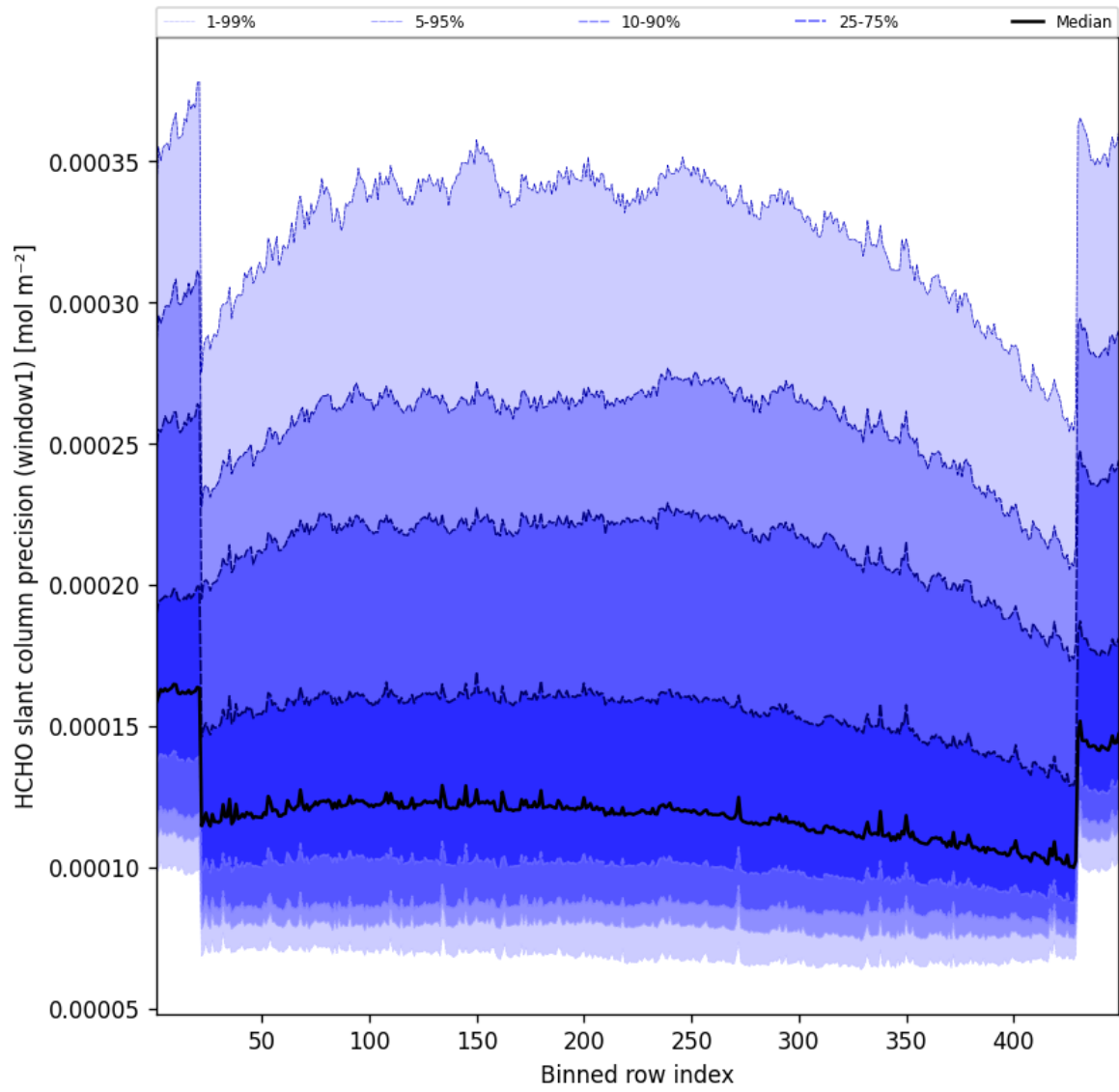
Figure 51: Along track statistics of “HCHO slant column precision (window1)” for 2024-12-30 to 2024-12-30
