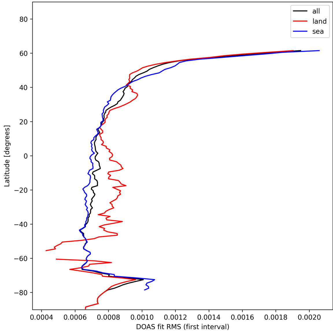
Figure 30: Zonal average of “DOAS fit RMS (first interval)” for 2024-12-30 to 2024-12-30.
