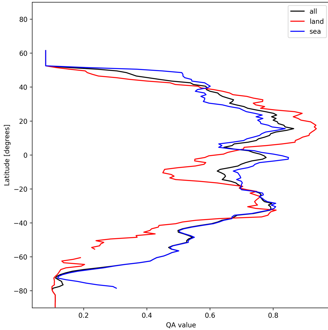
Figure 18: Zonal average of “QA value” for 2024-12-30 to 2024-12-30.
