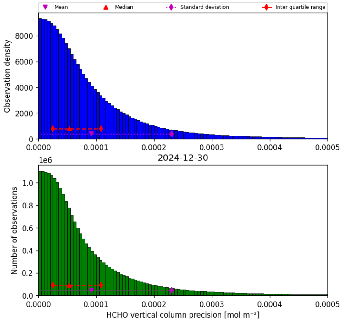
Figure 34: Histogram of “HCHO vertical column precision” for 2024-12-30 to 2024-12-30
