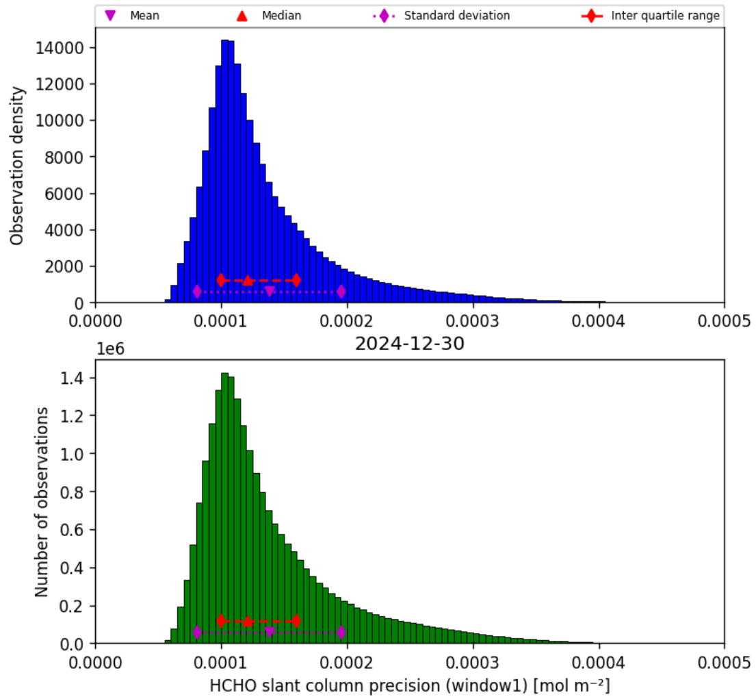
Figure 37: Histogram of “HCHO slant column precision (window1)” for 2024-12-30 to 2024-12-30
