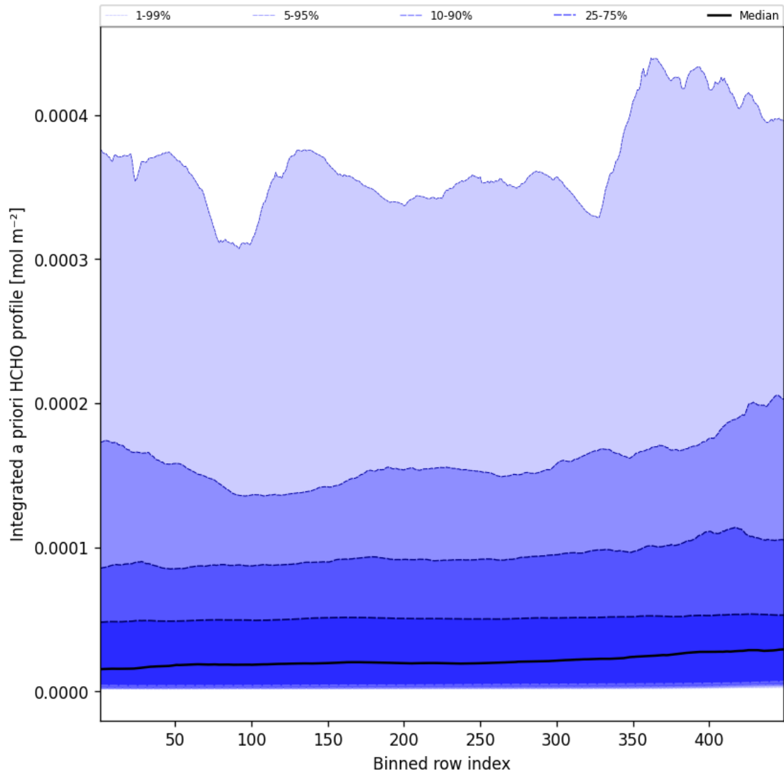
Figure 55: Along track statistics of “Integrated a priori HCHO profile” for 2024-12-30 to 2024-12-30
