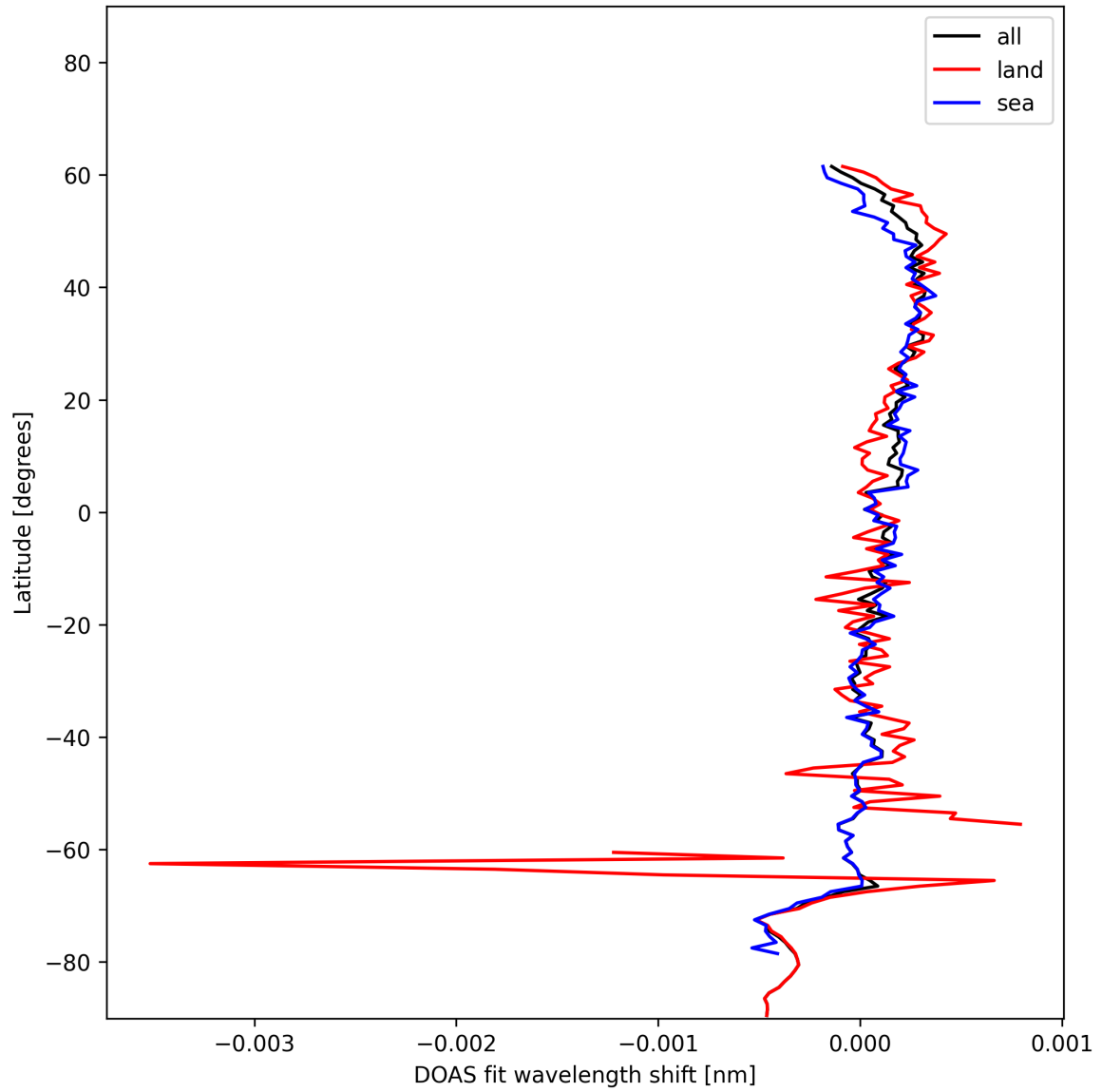
Figure 28: Zonal average of “DOAS fit wavelength shift” for 2024-12-30 to 2024-12-30.
