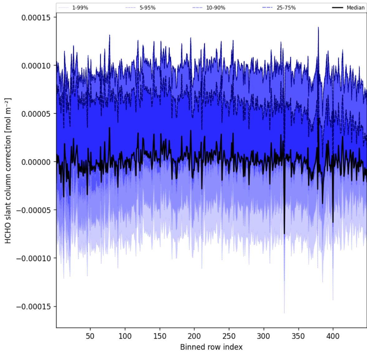
Figure 59: Along track statistics of “HCHO slant column correction” for 2024-12-30 to 2024-12-30
