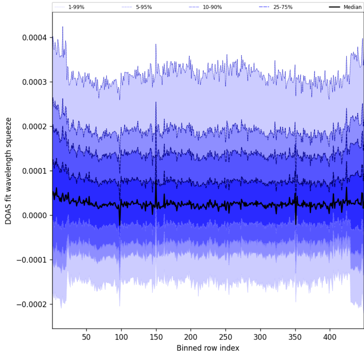
Figure 57: Along track statistics of “DOAS fit wavelength squeeze” for 2024-12-31 to 2024-12-31
