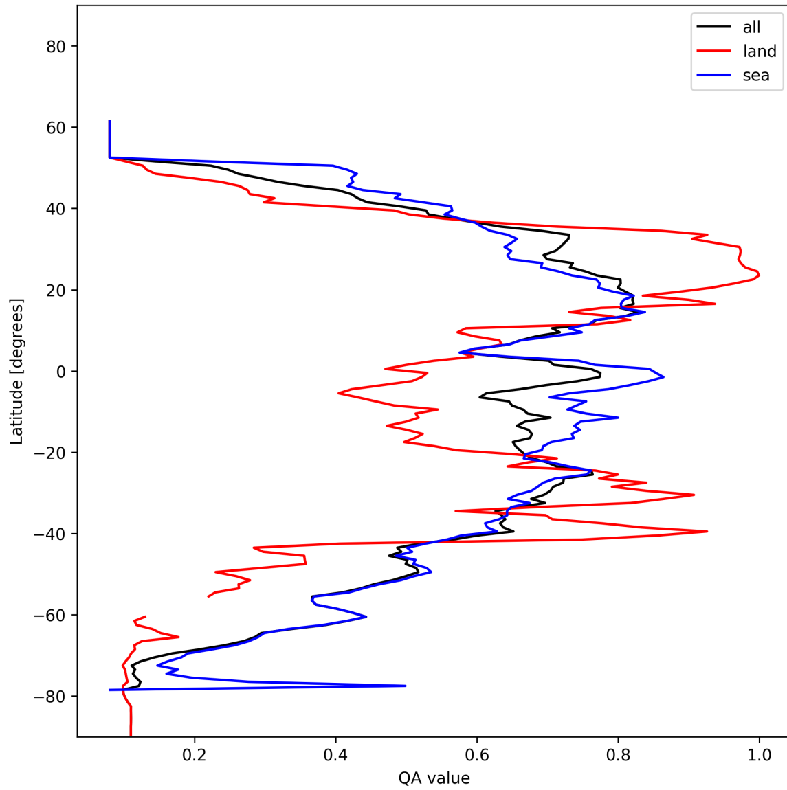
Figure 18: Zonal average of “QA value” for 2024-12-31 to 2024-12-31.
