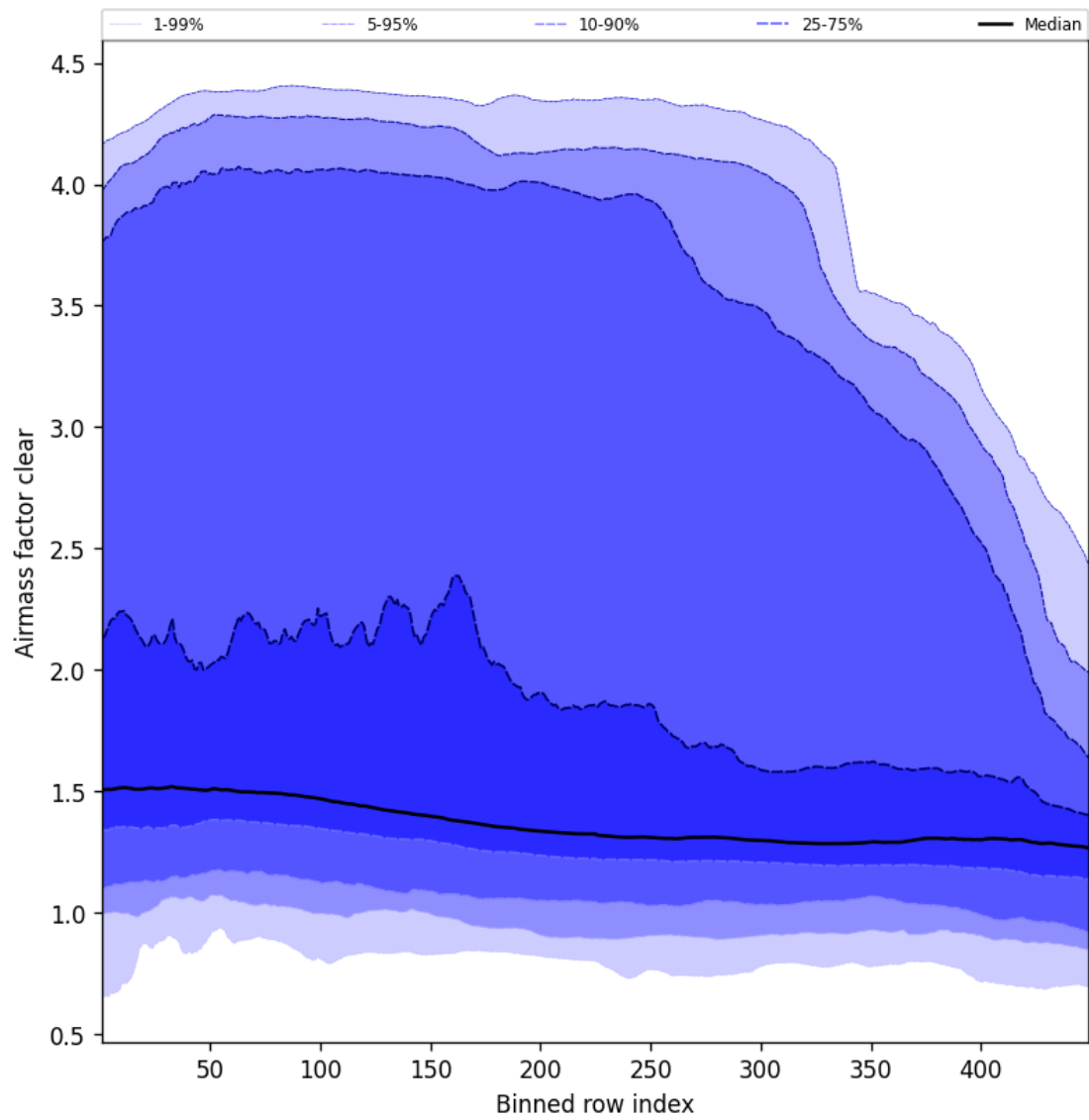
Figure 54: Along track statistics of “Airmass factor clear” for 2024-12-31 to 2024-12-31
