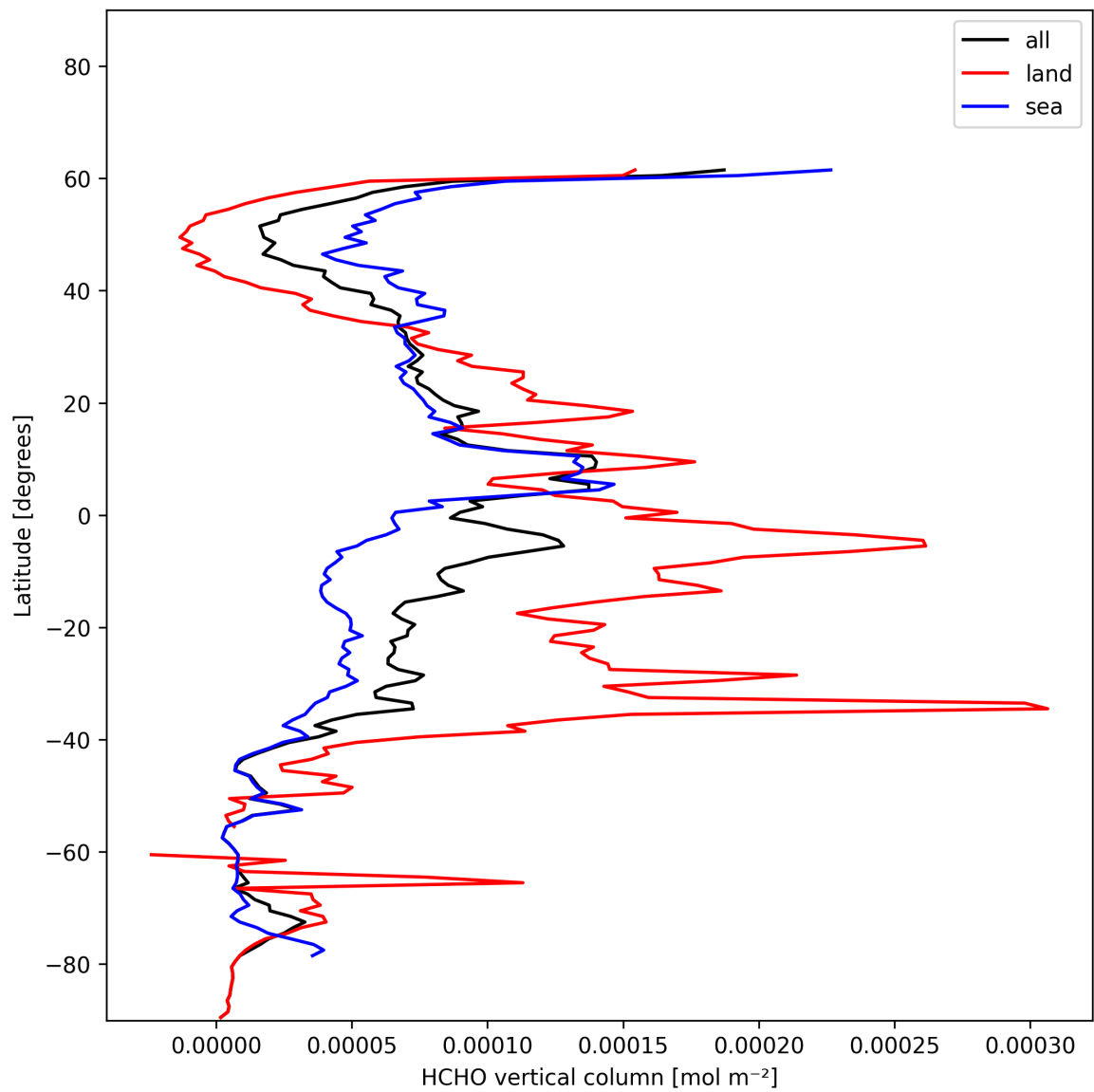
Figure 19: Zonal average of “HCHO vertical column” for 2024-12-31 to 2024-12-31.
