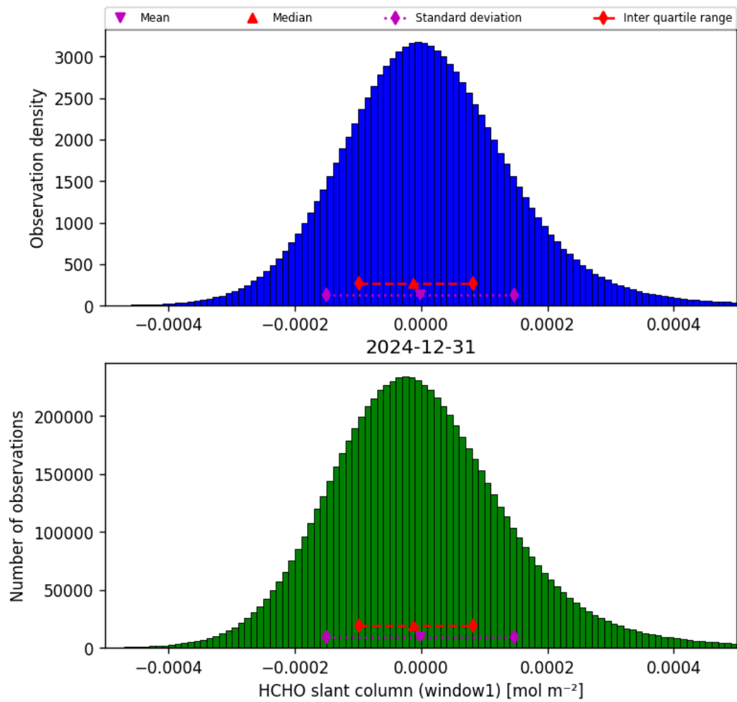
Figure 36: Histogram of “HCHO slant column (window1)” for 2024-12-31 to 2024-12-31
