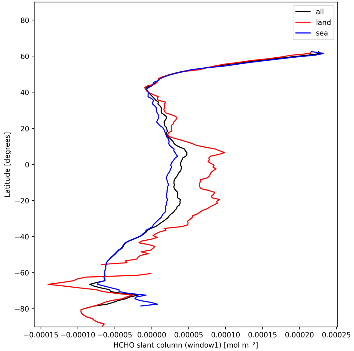
Figure 22: Zonal average of “HCHO slant column (window1)” for 2025-01-02 to 2025-01-03.
