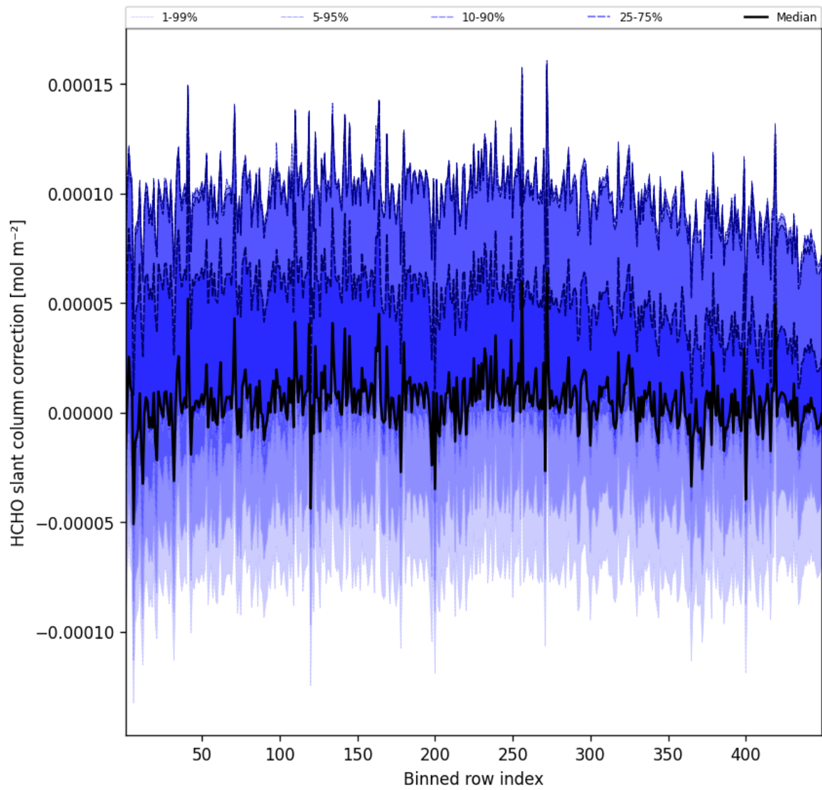
Figure 59: Along track statistics of “HCHO slant column correction” for 2025-01-02 to 2025-01-03
