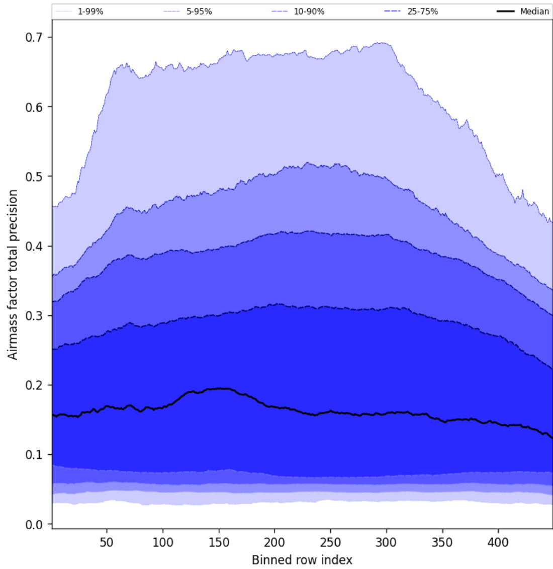
Figure 53: Along track statistics of “Airmass factor total precision” for 2025-01-02 to 2025-01-03
