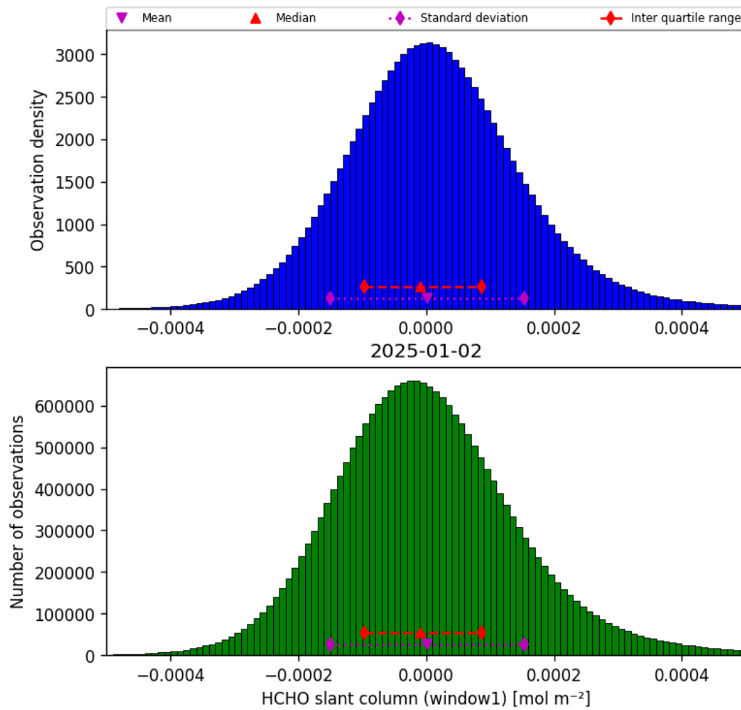
Figure 36: Histogram of “HCHO slant column (window1)” for 2025-01-02 to 2025-01-03
