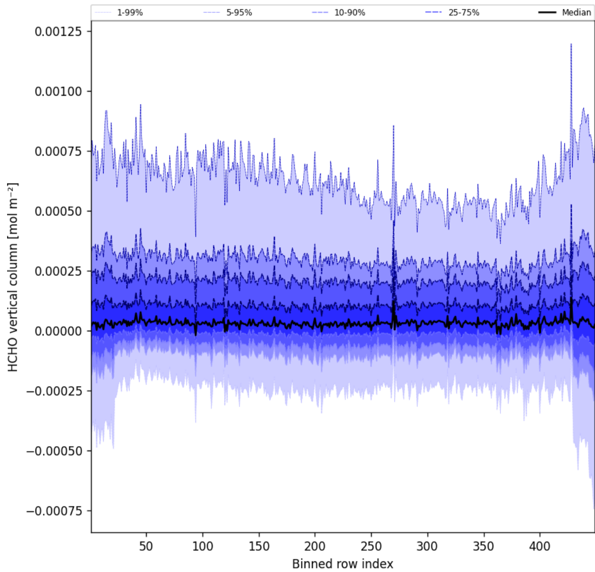
Figure 47: Along track statistics of “HCHO vertical column” for 2025-01-02 to 2025-01-03
