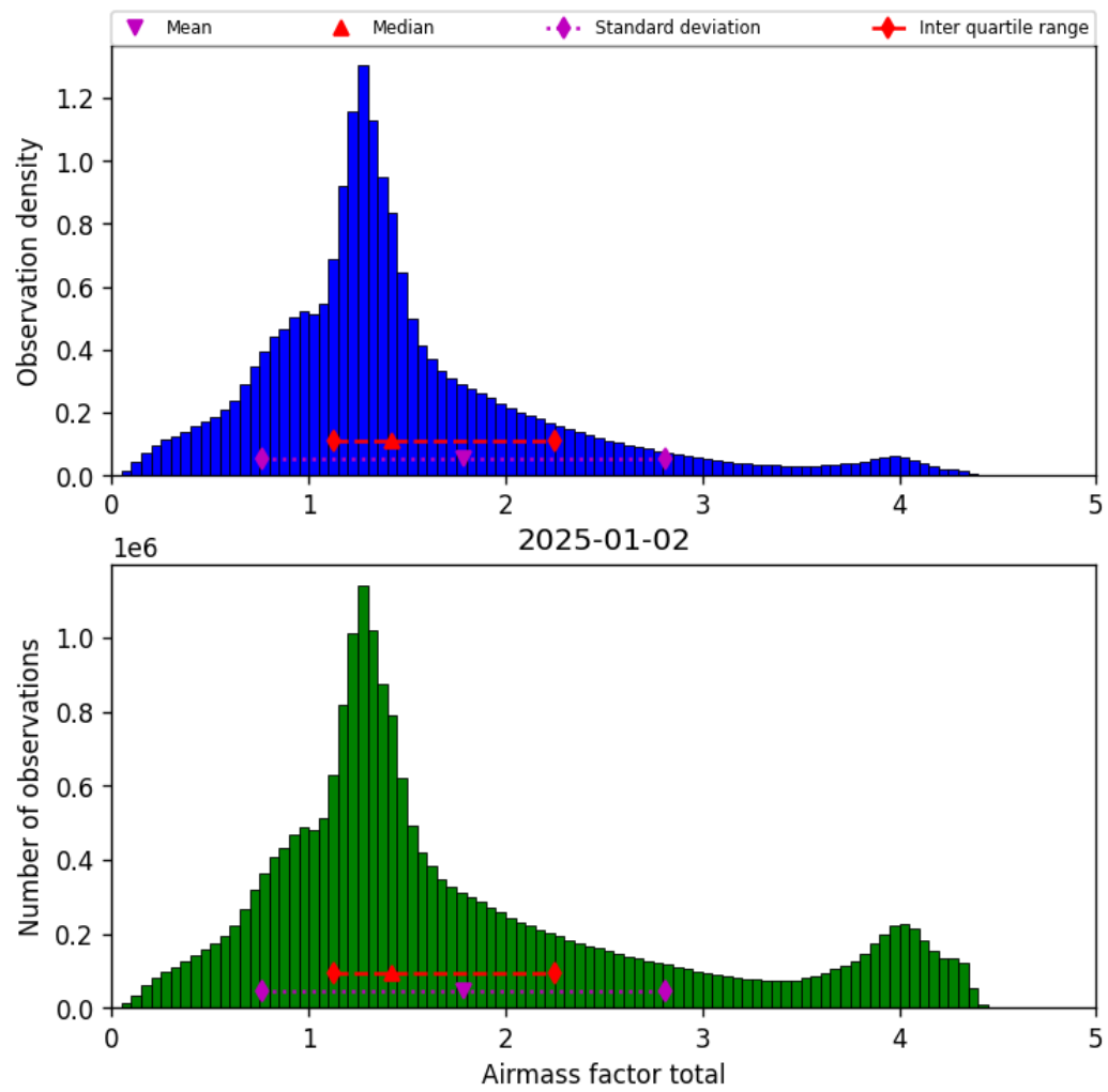
Figure 38: Histogram of “Airmass factor total” for 2025-01-02 to 2025-01-03
