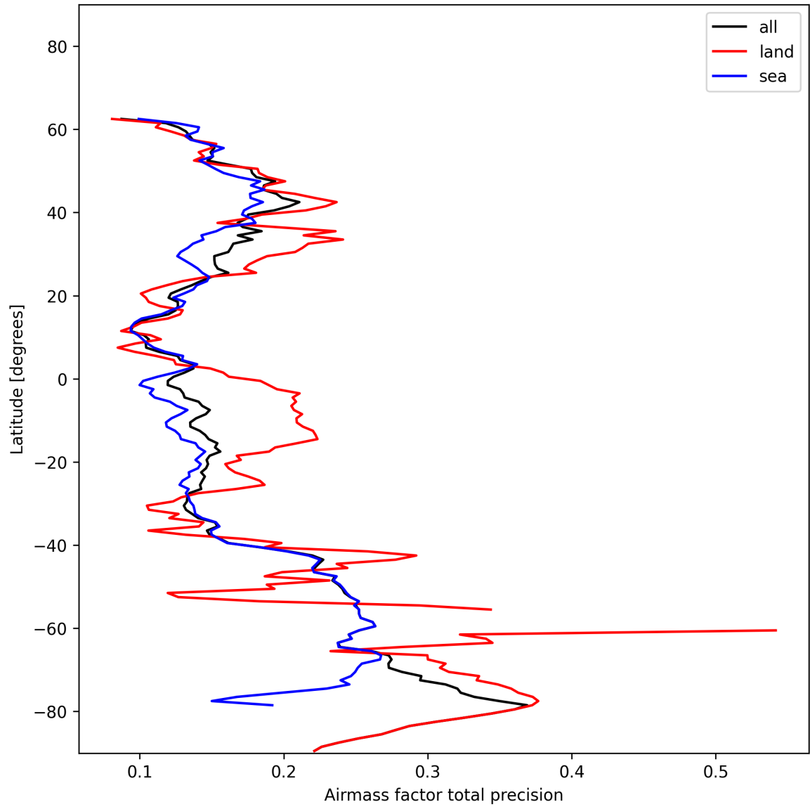
Figure 25: Zonal average of “Airmass factor total precision” for 2025-01-02 to 2025-01-03.
