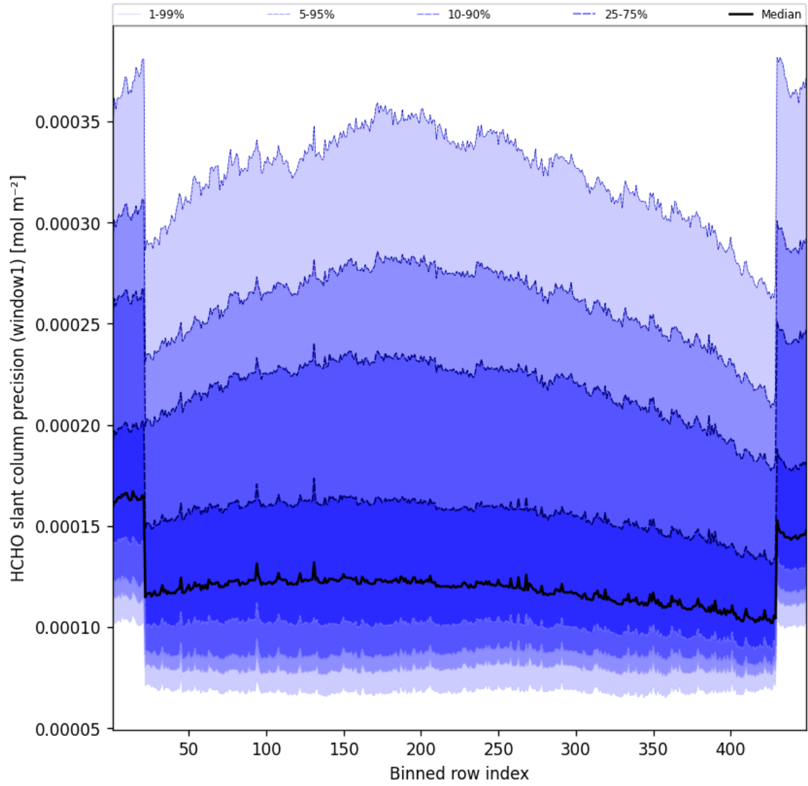
Figure 51: Along track statistics of “HCHO slant column precision (window1)” for 2025-01-02 to 2025-01-03
