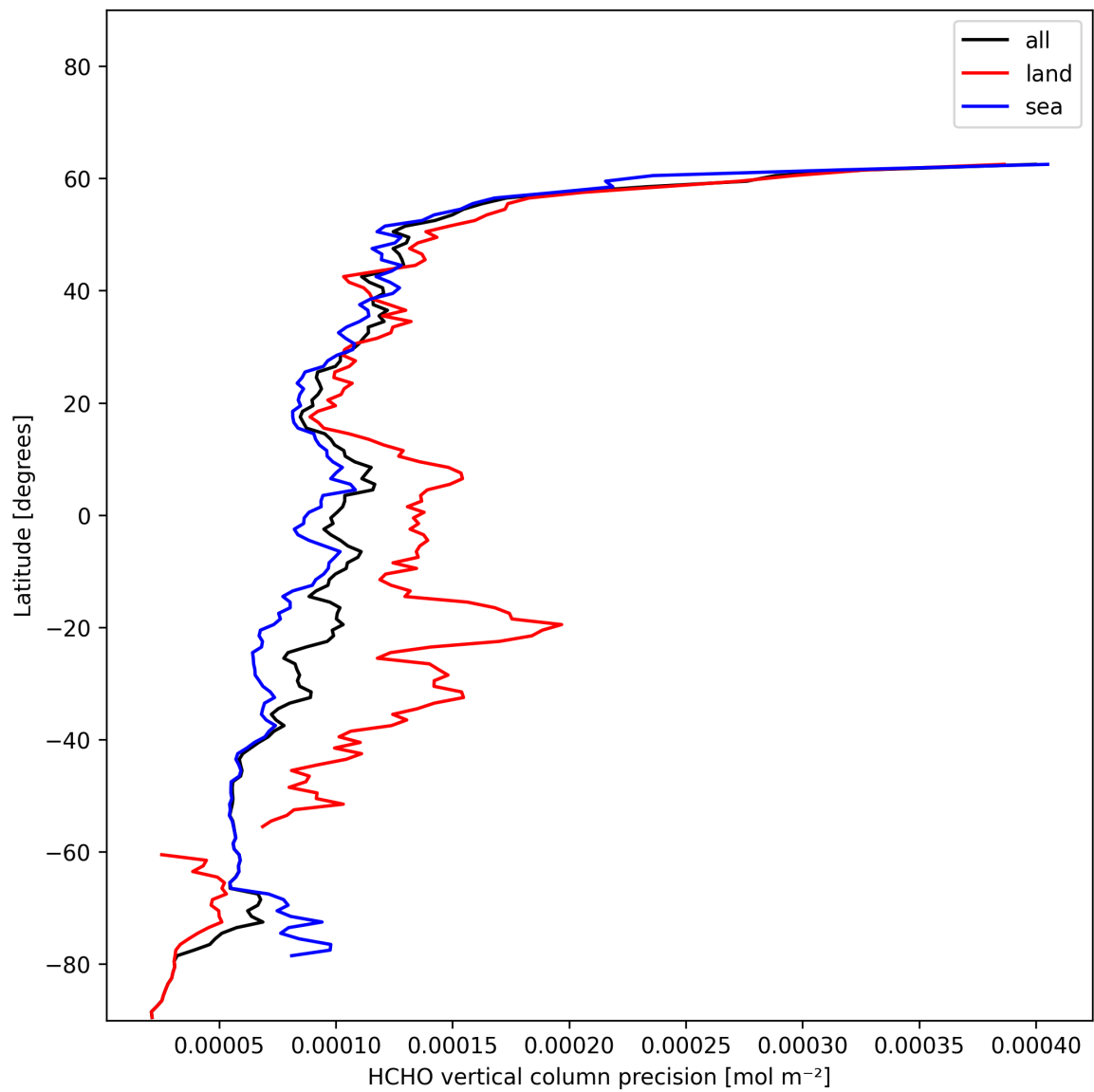
Figure 20: Zonal average of "HCHO vertical column precision" for 2025-01-02 to 2025-01-03.
