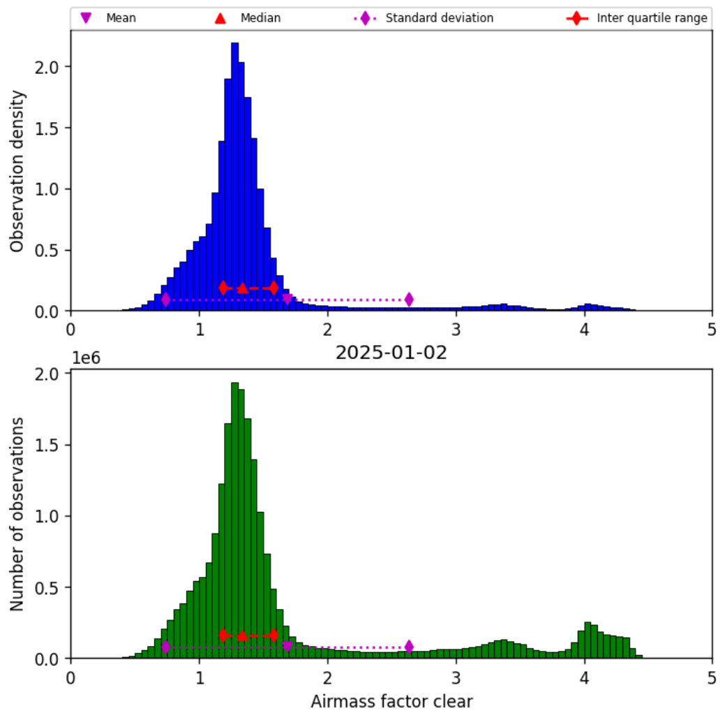
Figure 40: Histogram of “Airmass factor clear” for 2025-01-02 to 2025-01-03
