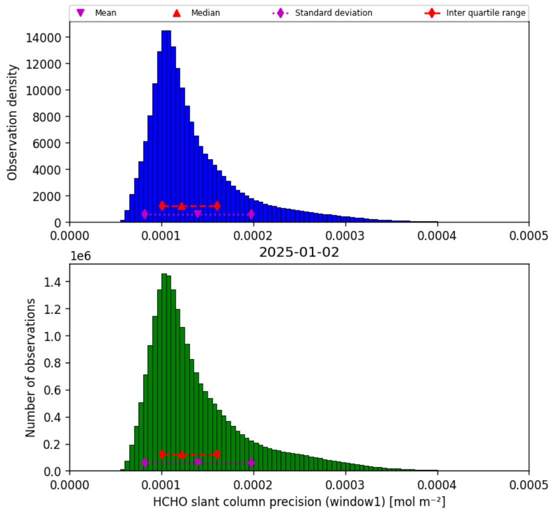
Figure 37: Histogram of “HCHO slant column precision (window1)” for 2025-01-02 to 2025-01-03
