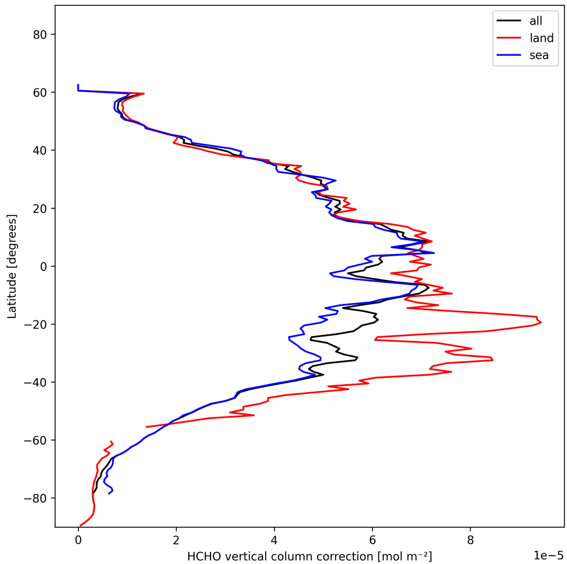
Figure 21: Zonal average of “HCHO vertical column correction” for 2025-01-02 to 2025-01-03.
