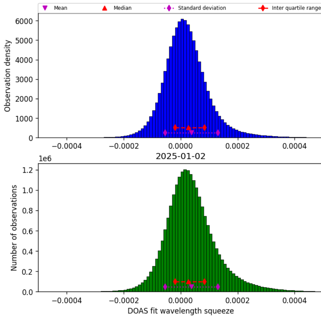
Figure 43: Histogram of “DOAS fit wavelength squeeze” for 2025-01-02 to 2025-01-03
