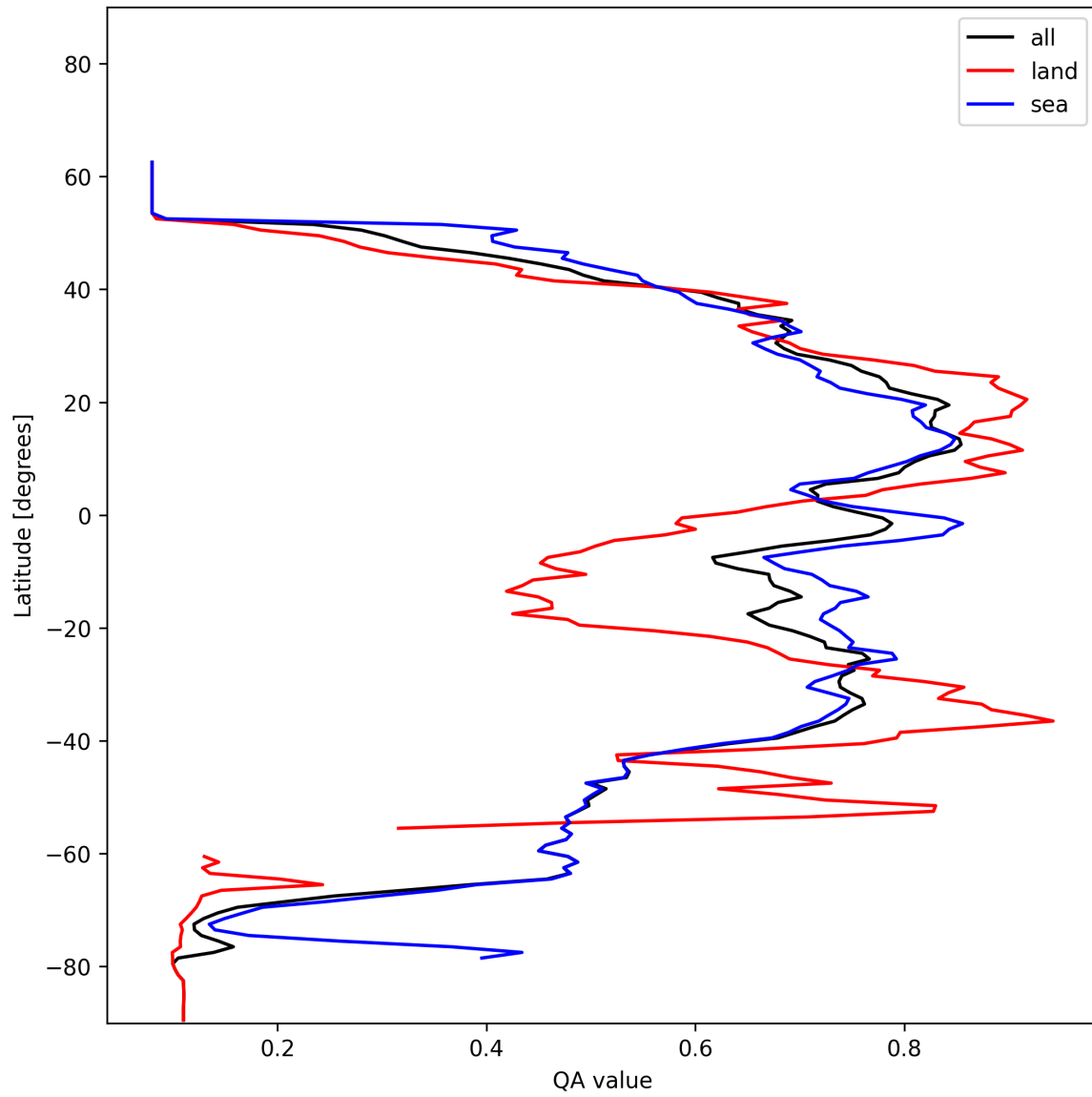
Figure 18: Zonal average of “QA value” for 2025-01-02 to 2025-01-03.
