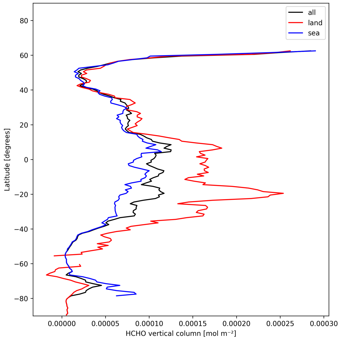
Figure 19: Zonal average of “HCHO vertical column” for 2025-01-02 to 2025-01-03.
