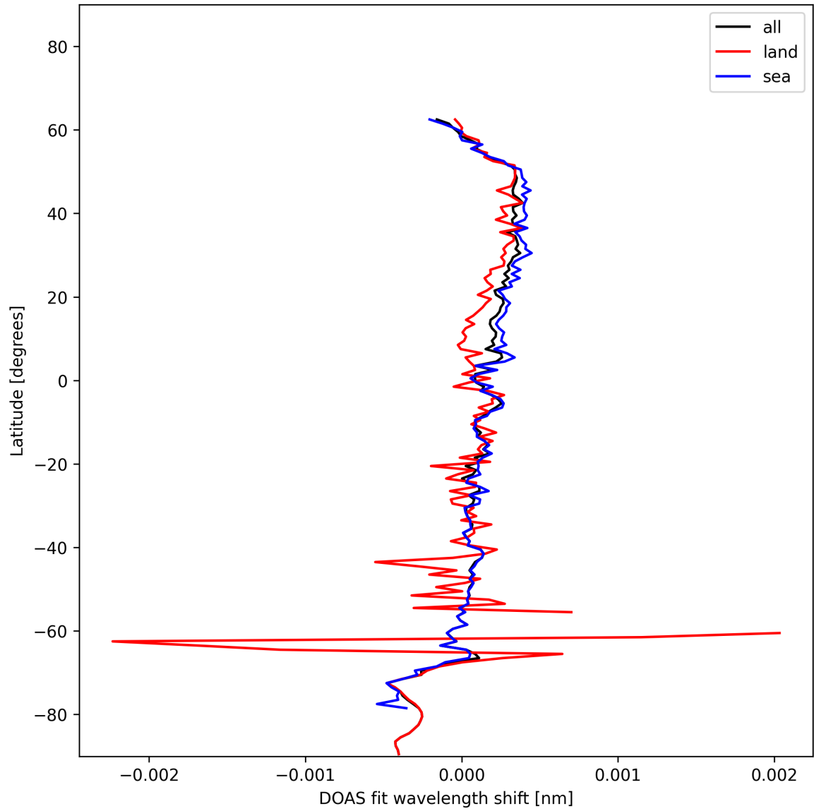
Figure 28: Zonal average of “DOAS fit wavelength shift” for 2025-01-02 to 2025-01-03.
