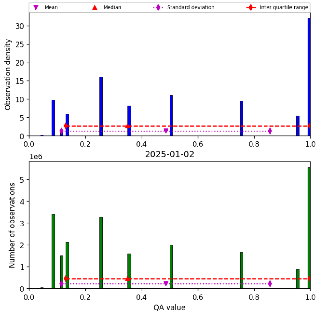
Figure 32: Histogram of “QA value” for 2025-01-02 to 2025-01-03
