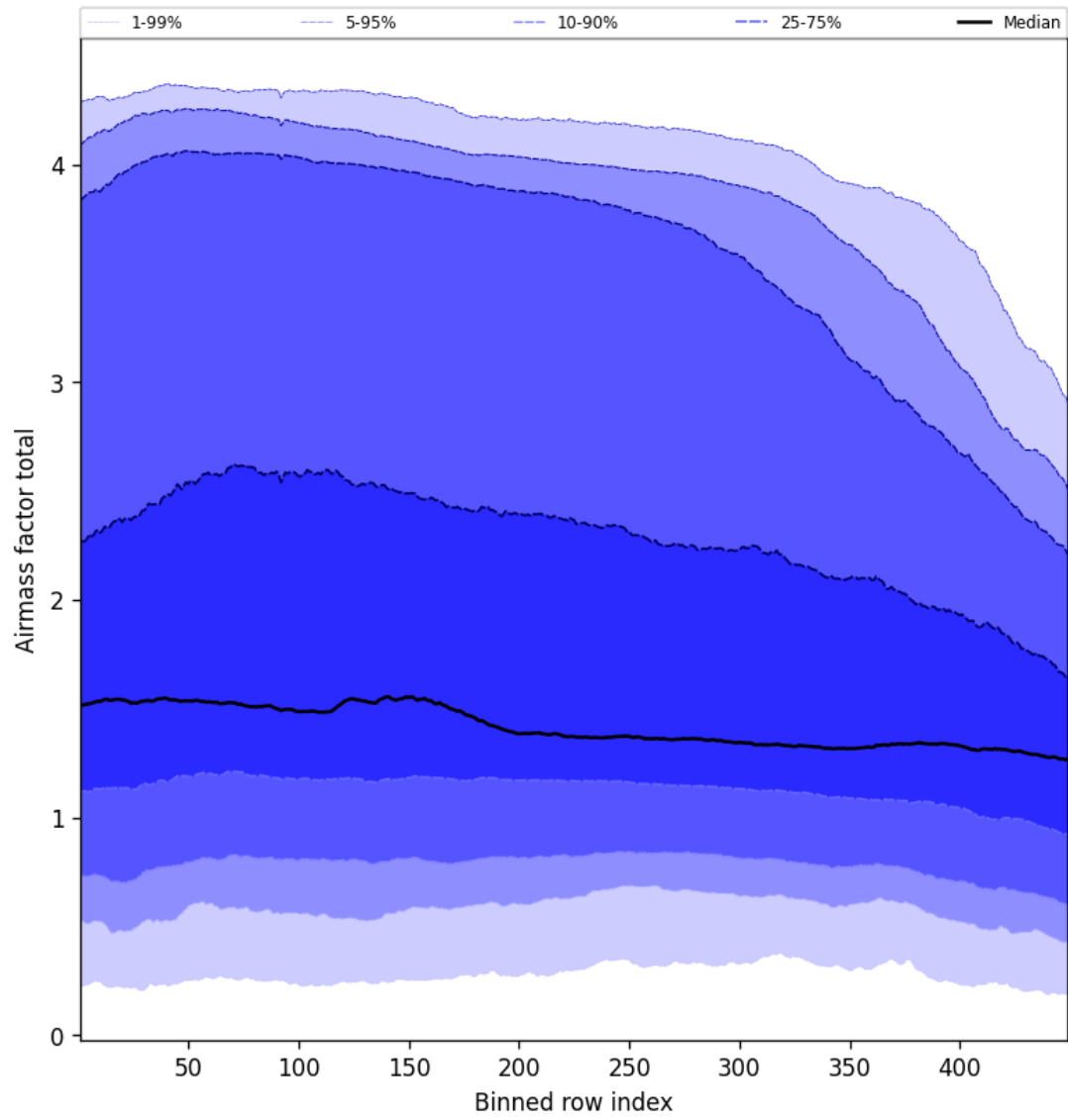
Figure 52: Along track statistics of “Airmass factor total” for 2025-01-02 to 2025-01-03
