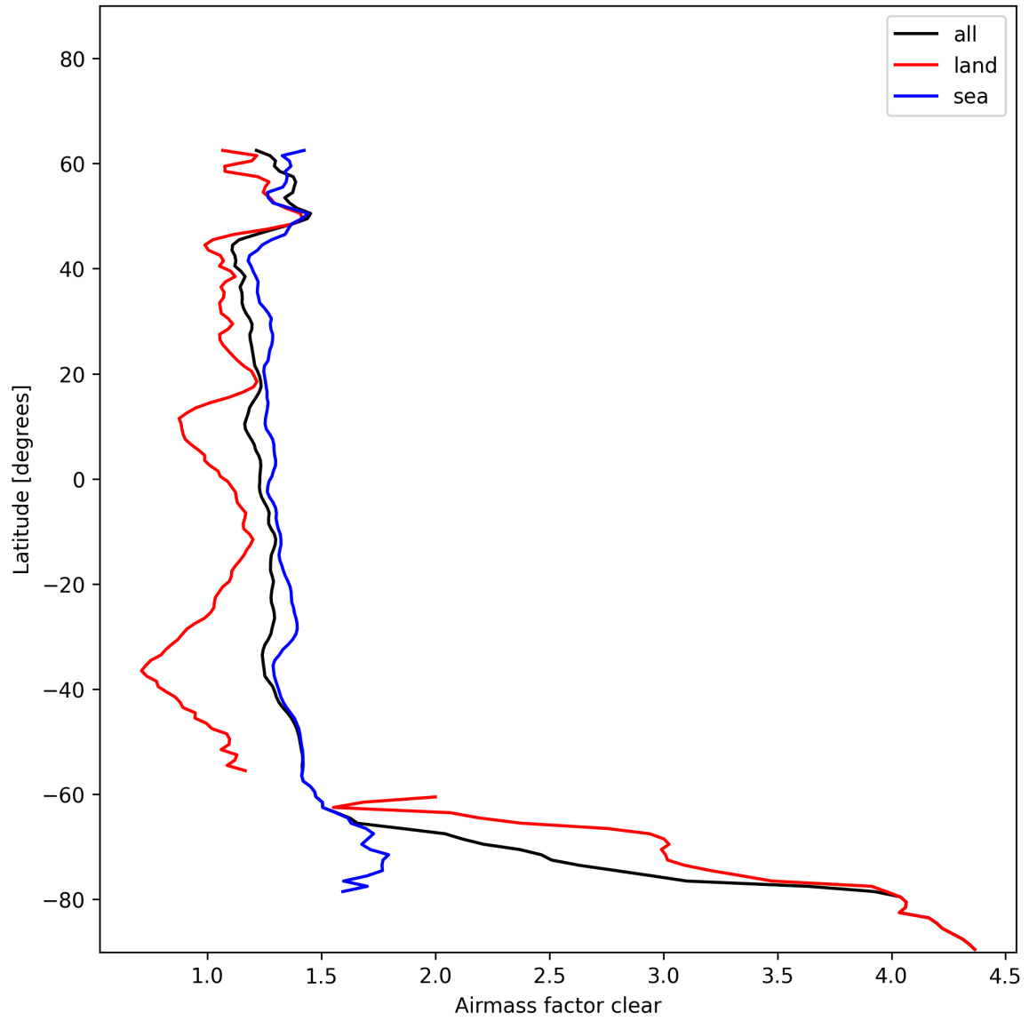
Figure 26: Zonal average of “Airmass factor clear” for 2025-01-02 to 2025-01-03.
