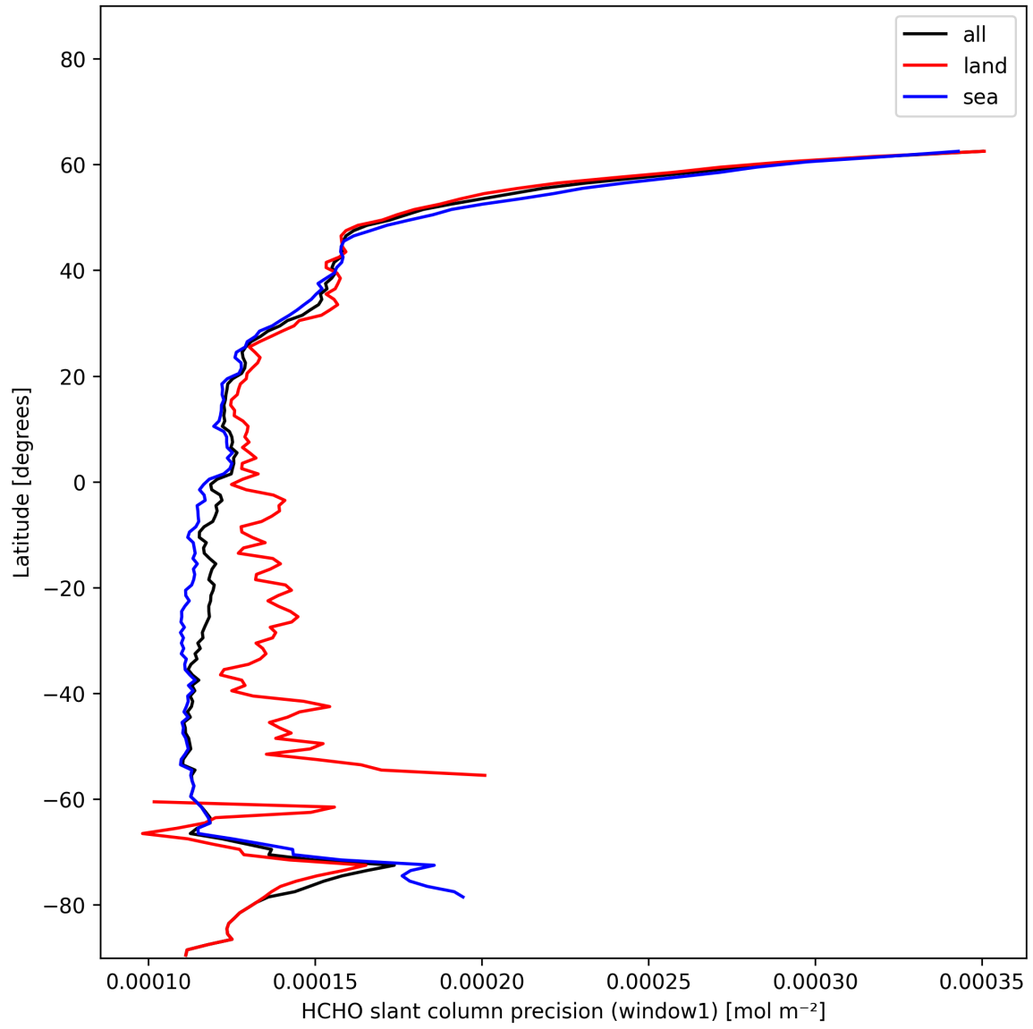
Figure 23: Zonal average of “HCHO slant column precision (window1)” for 2025-01-02 to 2025-01-03.
