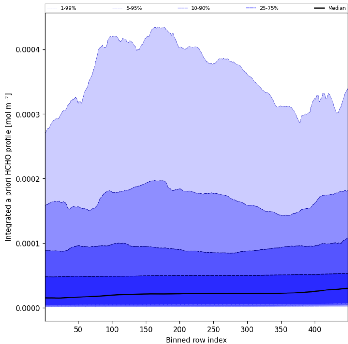
Figure 55: Along track statistics of “Integrated a priori HCHO profile” for 2025-01-02 to 2025-01-03
