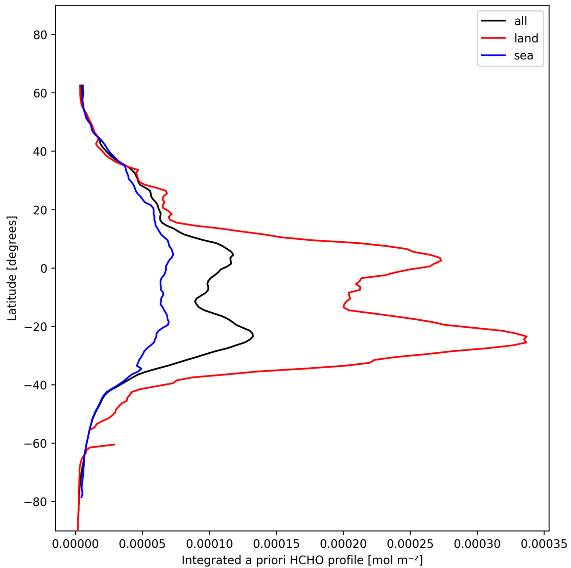
Figure 27: Zonal average of “Integrated a priori HCHO profile” for 2025-01-02 to 2025-01-03.
