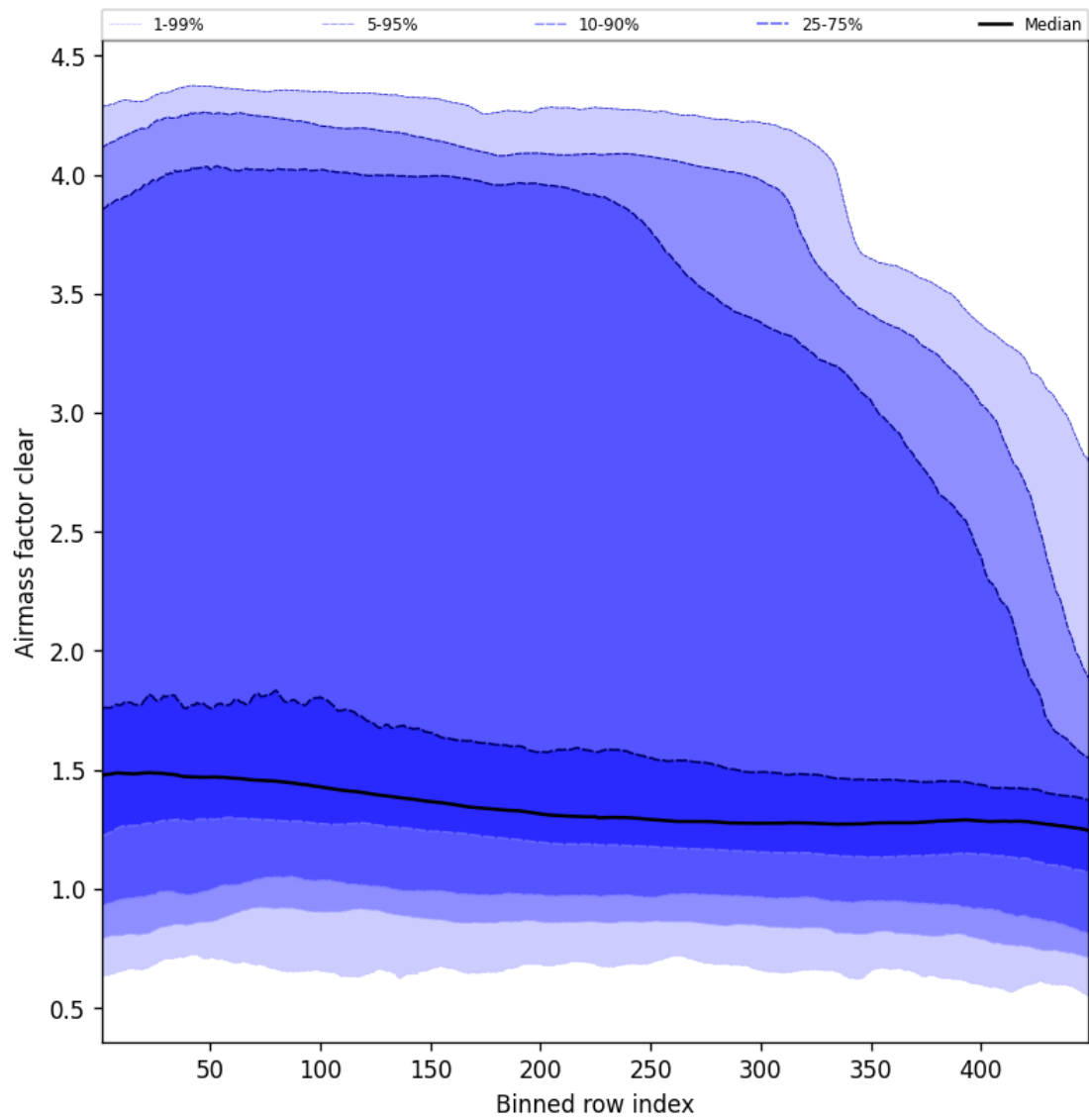
Figure 54: Along track statistics of “Airmass factor clear” for 2025-01-02 to 2025-01-03
