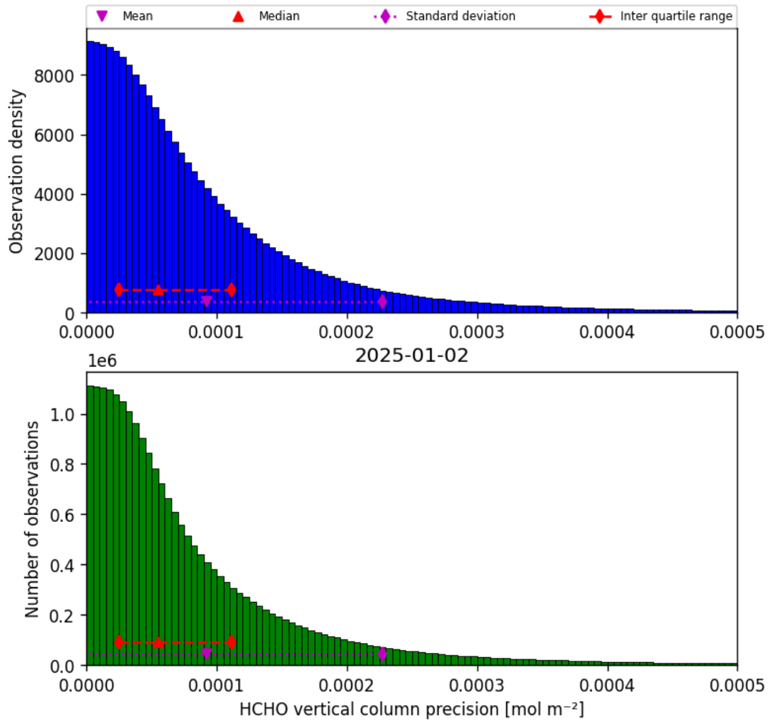
Figure 34: Histogram of “HCHO vertical column precision” for 2025-01-02 to 2025-01-03
