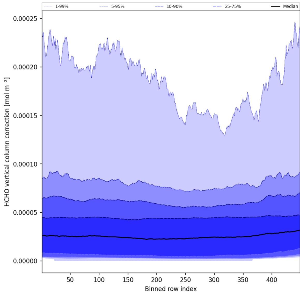
Figure 49: Along track statistics of "HCHO vertical column correction" for 2025-01-02 to 2025-01-03
