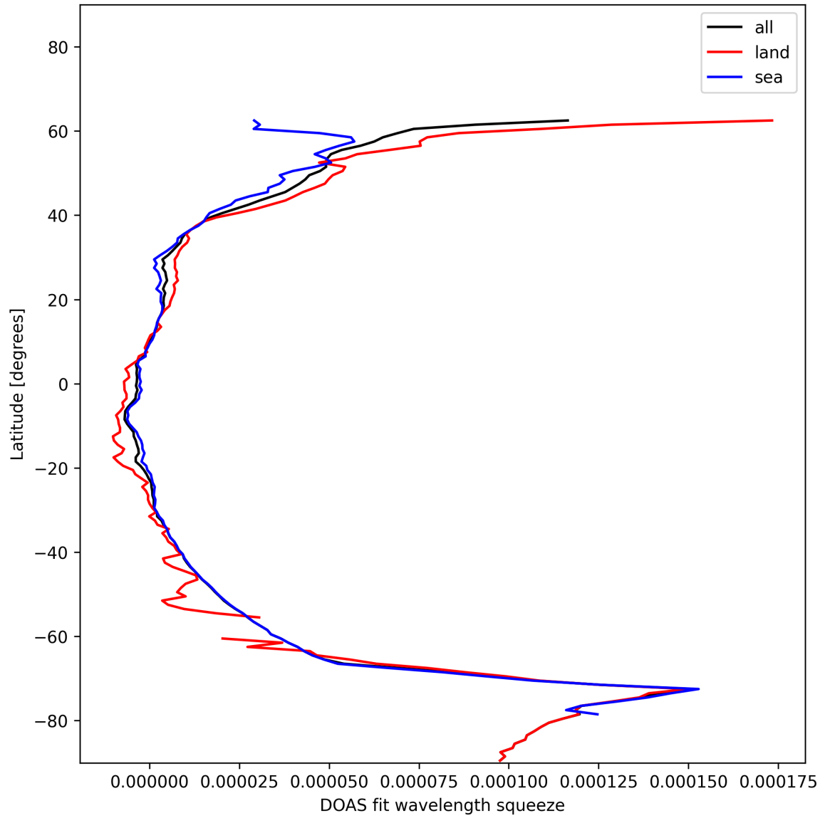
Figure 29: Zonal average of “DOAS fit wavelength squeeze” for 2025-01-02 to 2025-01-03.
