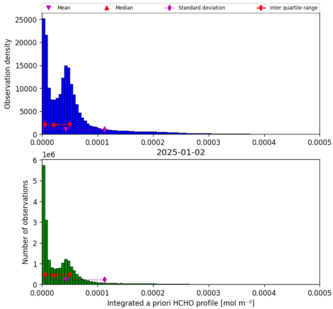
Figure 41: Histogram of “Integrated a priori HCHO profile” for 2025-01-02 to 2025-01-03
