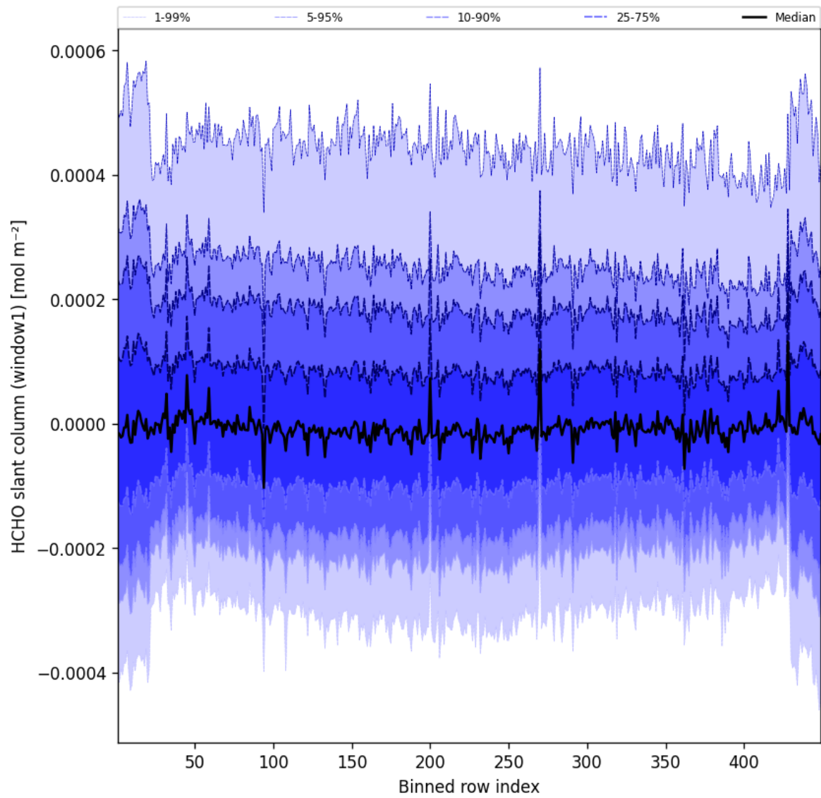
Figure 50: Along track statistics of “HCHO slant column (window1)” for 2025-01-02 to 2025-01-03
