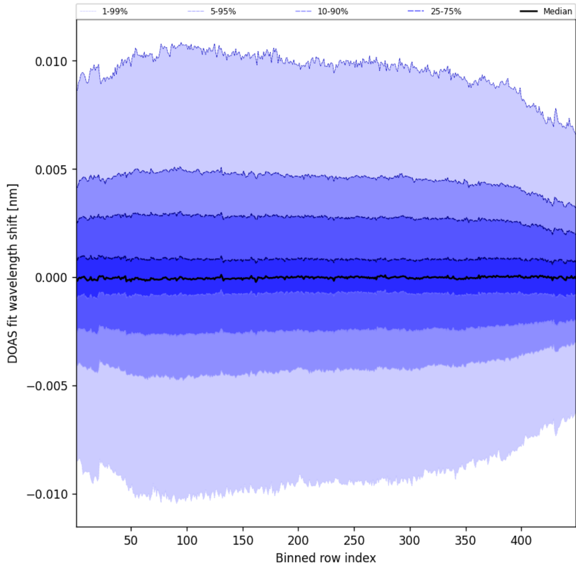
Figure 56: Along track statistics of “DOAS fit wavelength shift” for 2025-01-02 to 2025-01-03
