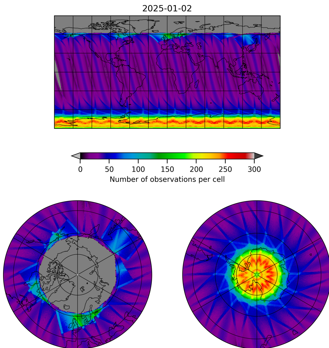
Figure 17: Map of the number of observations for 2025-01-02 to 2025-01-03
