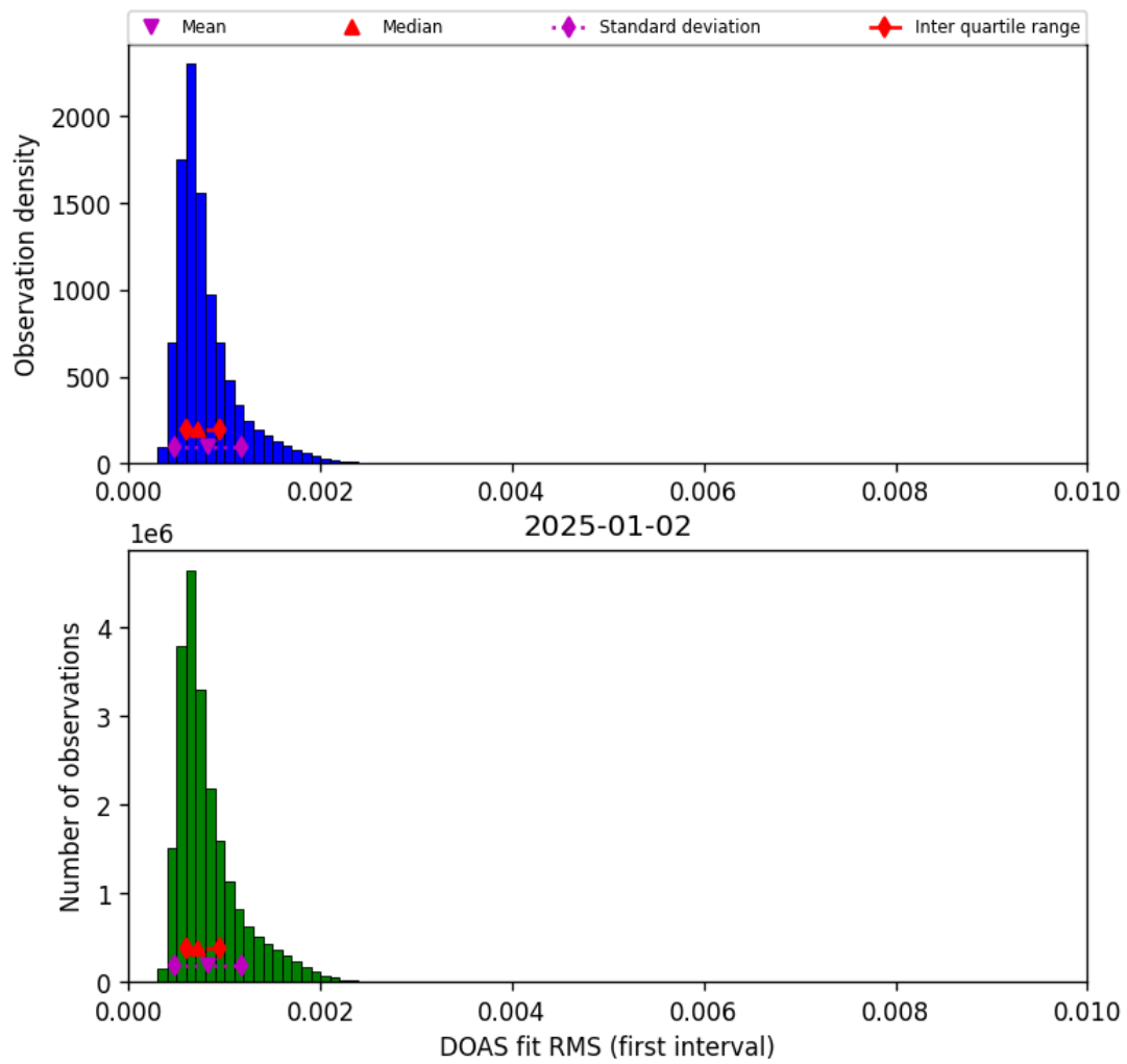
Figure 44: Histogram of "DOAS fit RMS (first interval)" for 2025-01-02 to 2025-01-03
