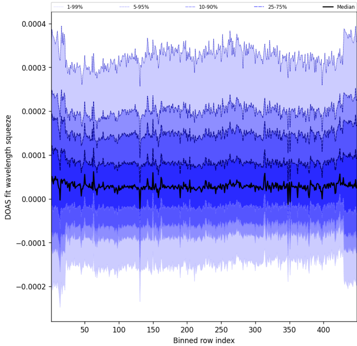
Figure 57: Along track statistics of “DOAS fit wavelength squeeze” for 2025-01-02 to 2025-01-03
