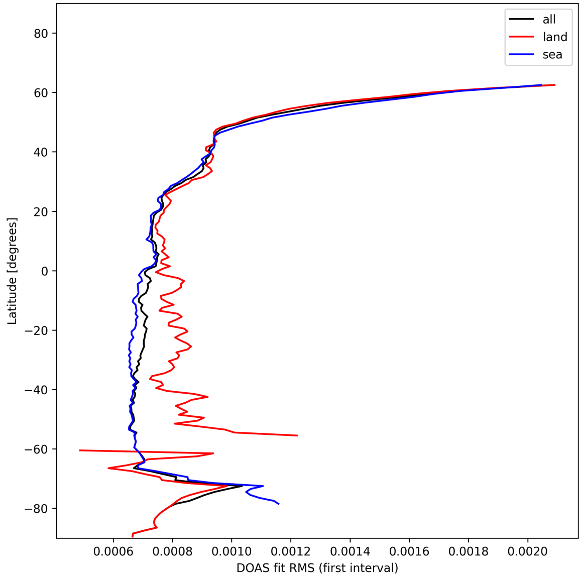
Figure 30: Zonal average of “DOAS fit RMS (first interval)” for 2025-01-02 to 2025-01-03.
