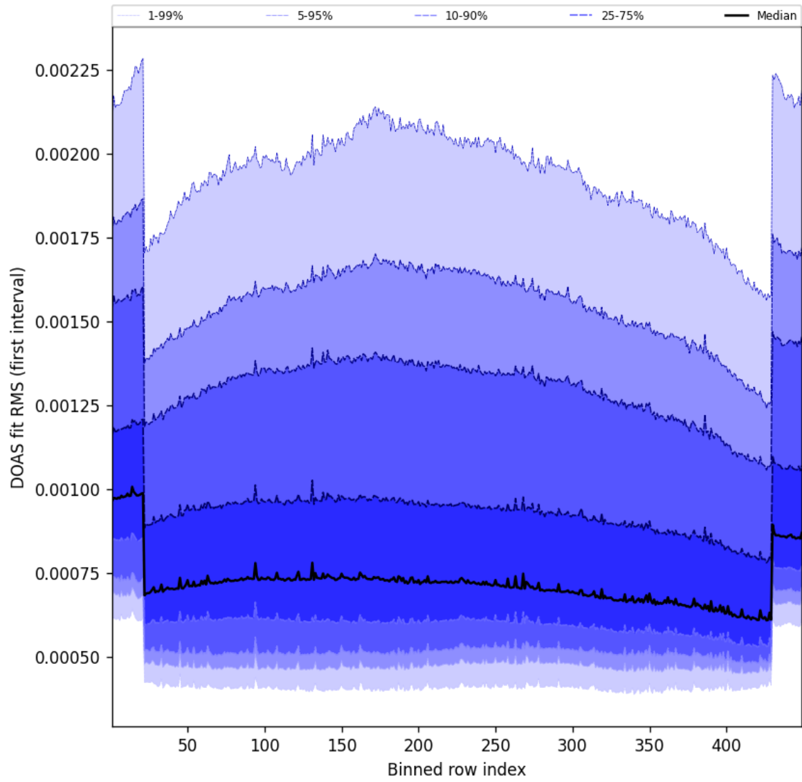
Figure 58: Along track statistics of “DOAS fit RMS (first interval)” for 2025-01-02 to 2025-01-03
