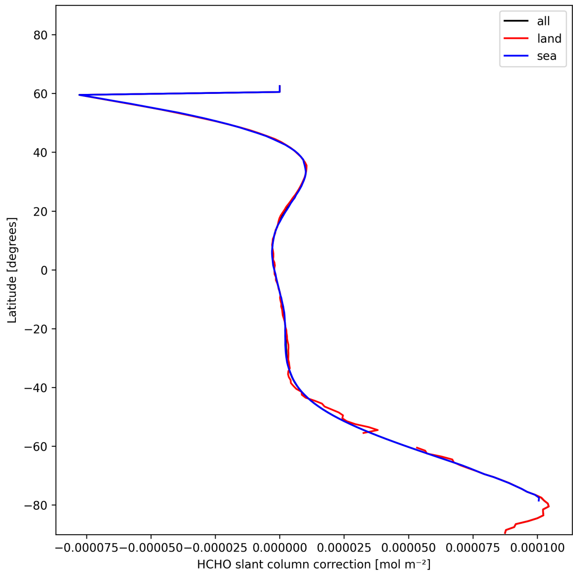
Figure 31: Zonal average of “HCHO slant column correction” for 2025-01-02 to 2025-01-03.
