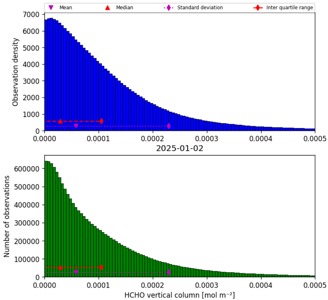
Figure 33: Histogram of “HCHO vertical column” for 2025-01-02 to 2025-01-03
