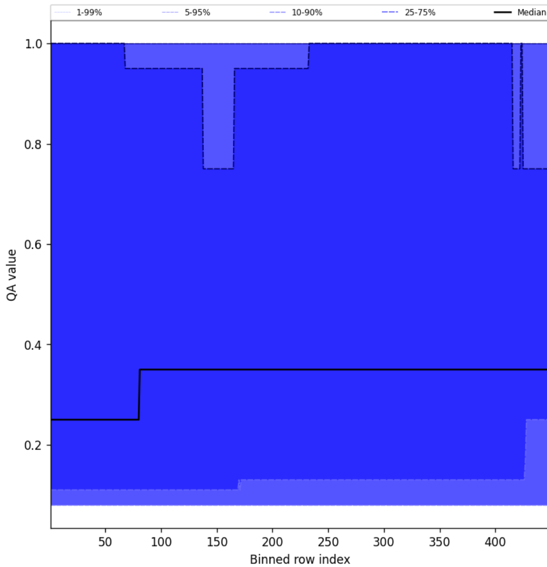
Figure 46: Along track statistics of “QA value” for 2025-01-02 to 2025-01-03
