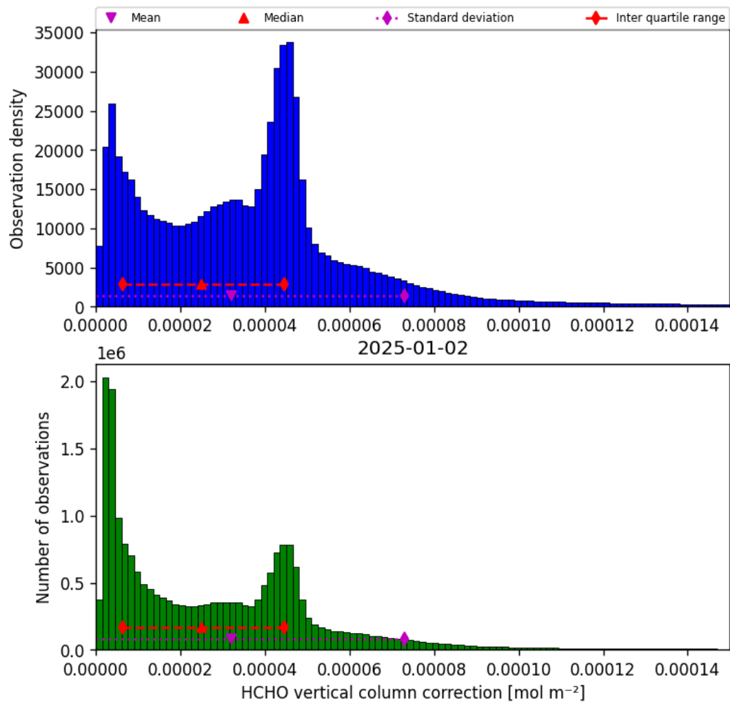
Figure 35: Histogram of “HCHO vertical column correction” for 2025-01-02 to 2025-01-03
