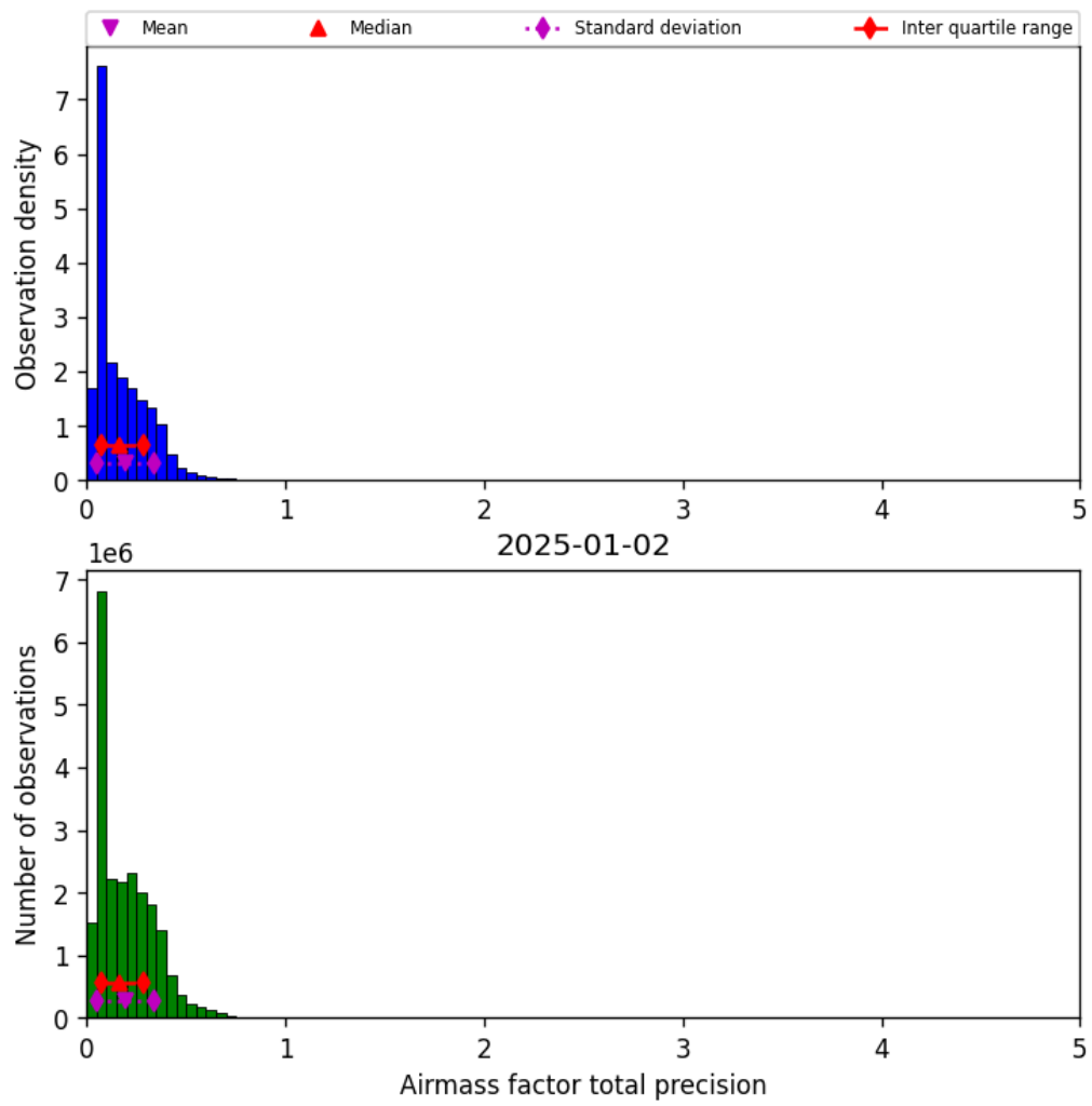
Figure 39: Histogram of “Airmass factor total precision” for 2025-01-02 to 2025-01-03
