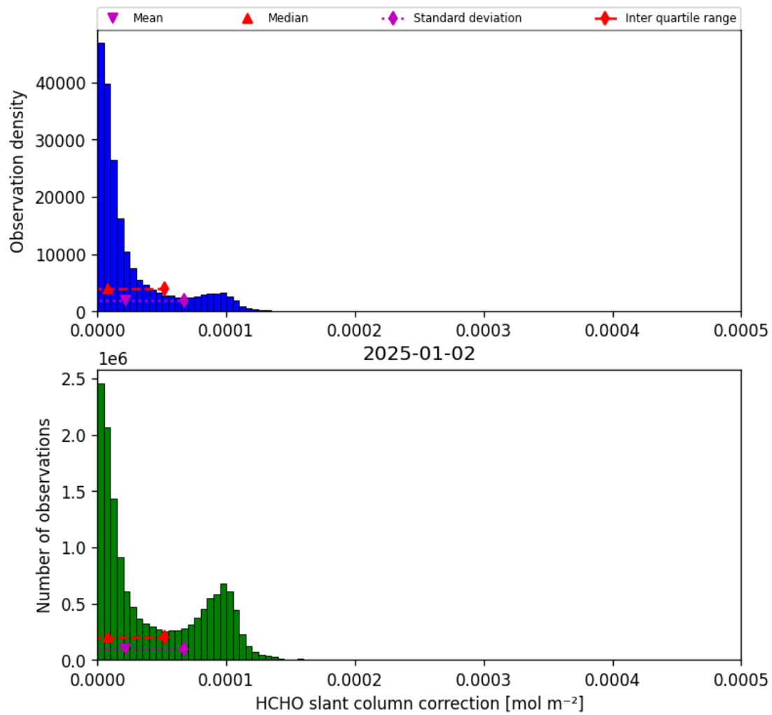
Figure 45: Histogram of “HCHO slant column correction” for 2025-01-02 to 2025-01-03
