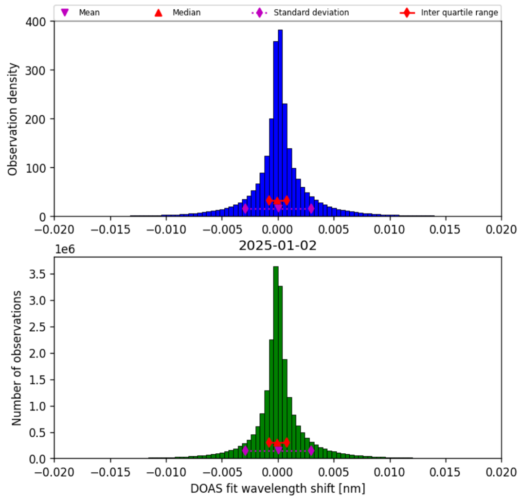
Figure 42: Histogram of “DOAS fit wavelength shift” for 2025-01-02 to 2025-01-03
