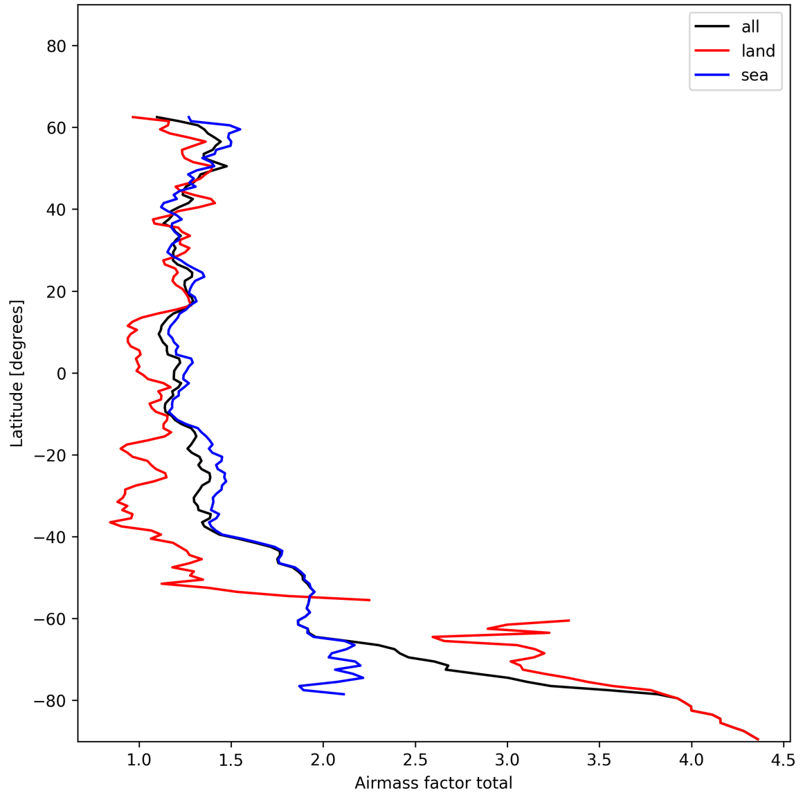
Figure 24: Zonal average of “Airmass factor total” for 2025-01-02 to 2025-01-03.
