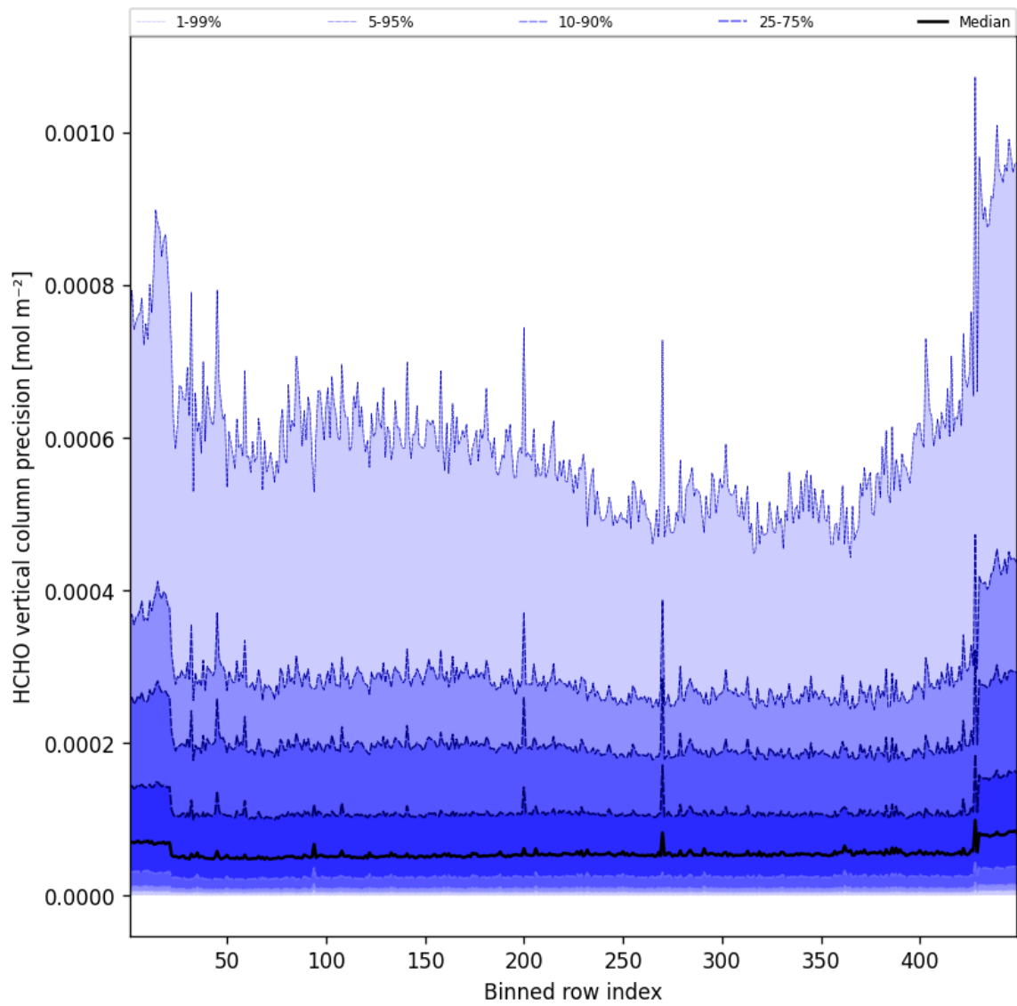
Figure 48: Along track statistics of “HCHO vertical column precision” for 2025-01-02 to 2025-01-03
