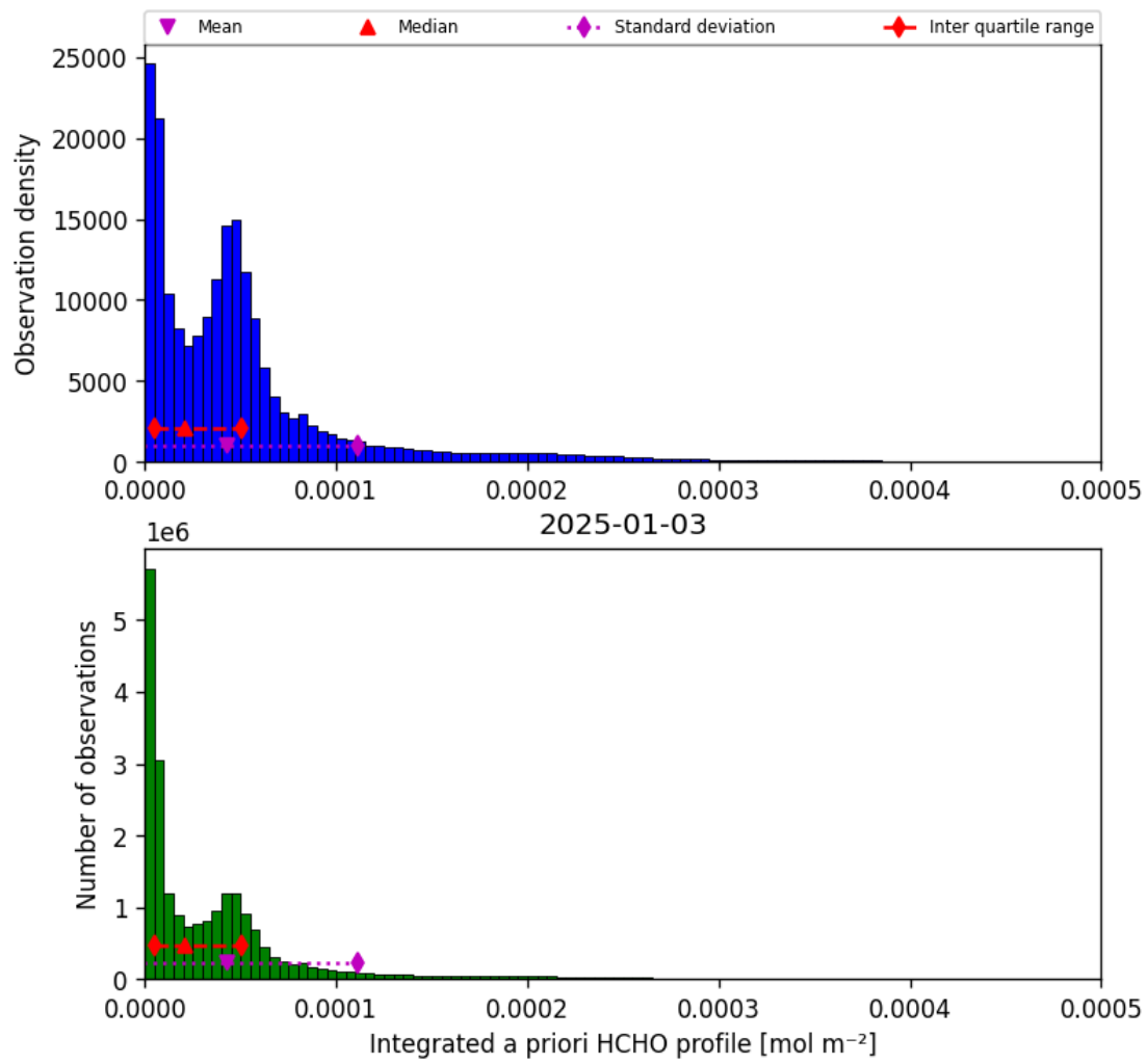
Figure 41: Histogram of “Integrated a priori HCHO profile” for 2025-01-03 to 2025-01-04
