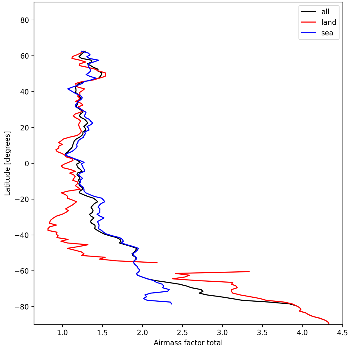
Figure 24: Zonal average of “Airmass factor total” for 2025-01-03 to 2025-01-04.
