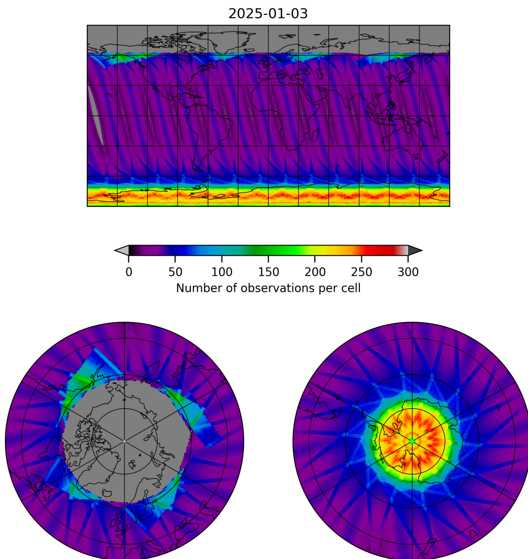
Figure 17: Map of the number of observations for 2025-01-03 to 2025-01-04
