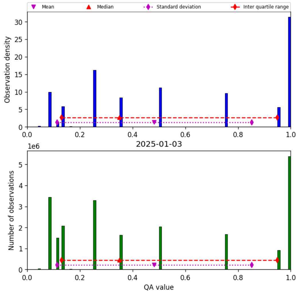
Figure 32: Histogram of “QA value” for 2025-01-03 to 2025-01-04
