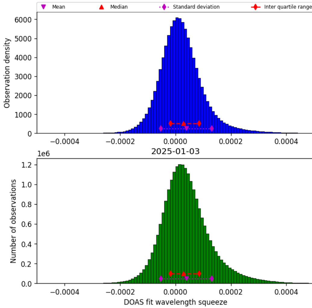
Figure 43: Histogram of “DOAS fit wavelength squeeze” for 2025-01-03 to 2025-01-04
