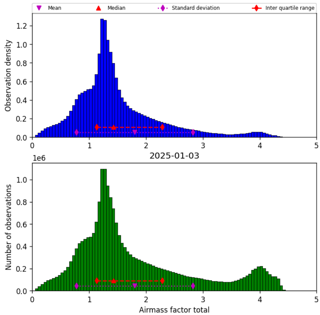
Figure 38: Histogram of “Airmass factor total” for 2025-01-03 to 2025-01-04
