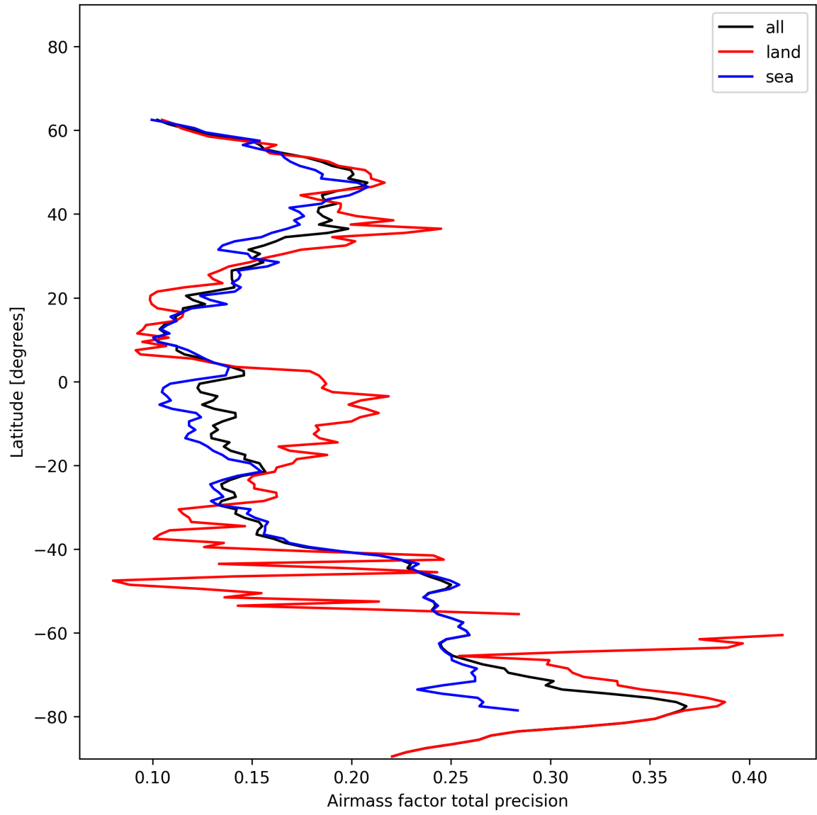
Figure 25: Zonal average of “Airmass factor total precision” for 2025-01-03 to 2025-01-04.
