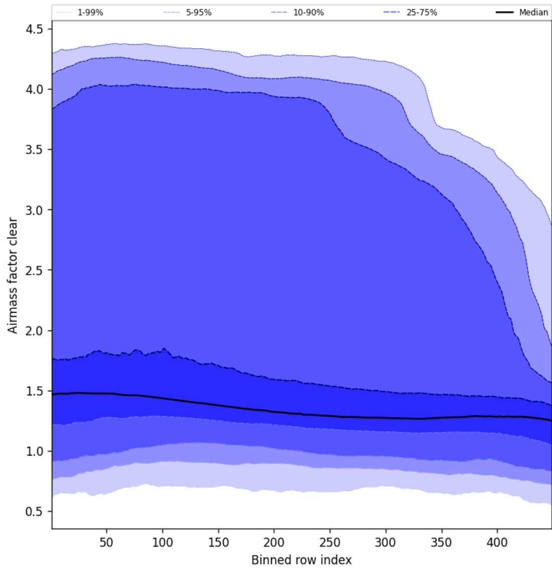
Figure 54: Along track statistics of “Air mass factor clear” for 2025-01-03 to 2025-01-04
