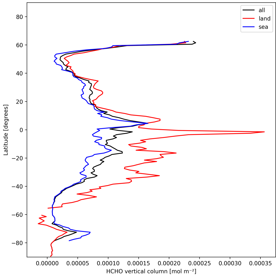
Figure 19: Zonal average of “HCHO vertical column” for 2025-01-03 to 2025-01-04.
