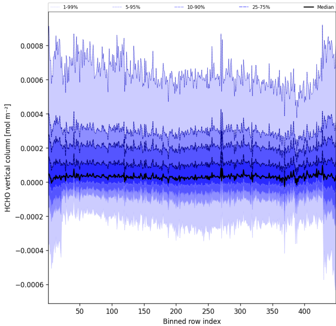
Figure 47: Along track statistics of “HCHO vertical column” for 2025-01-03 to 2025-01-04
