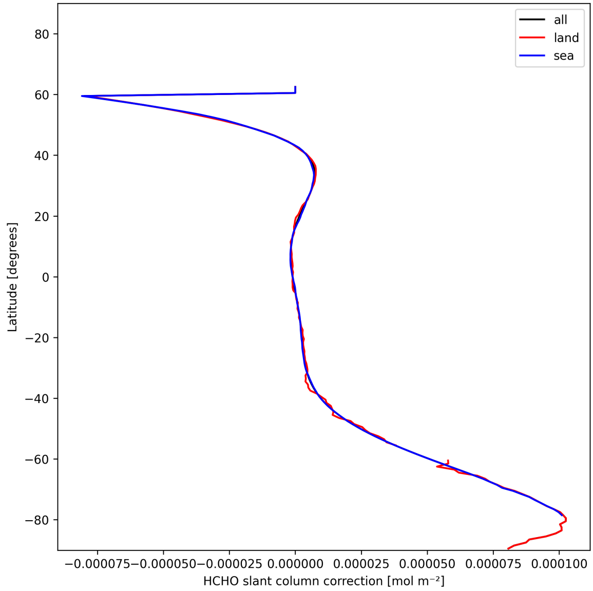
Figure 31: Zonal average of "HCHO slant column correction" for 2025-01-03 to 2025-01-04.
