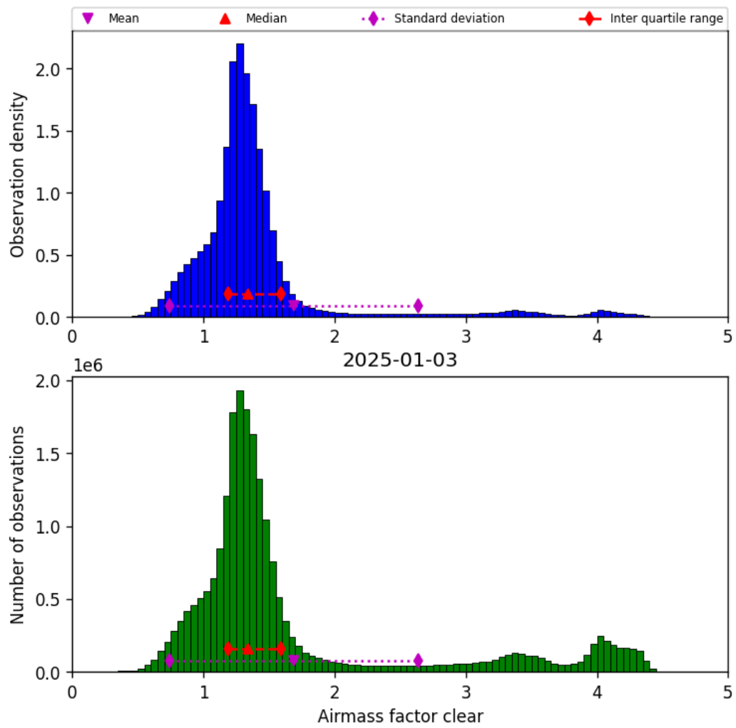
Figure 40: Histogram of “Airmass factor clear” for 2025-01-03 to 2025-01-04
