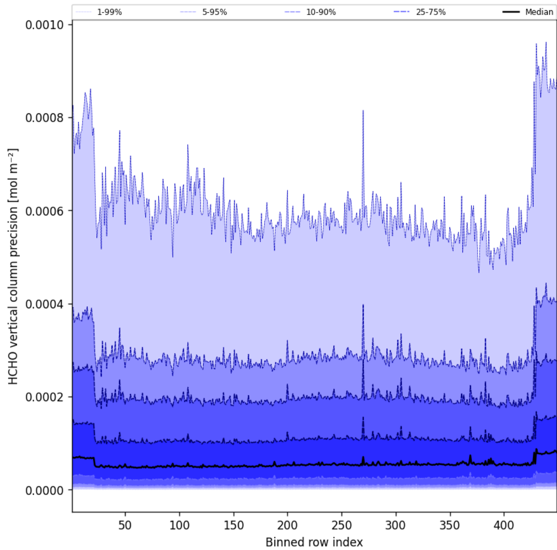
Figure 48: Along track statistics of “HCHO vertical column precision” for 2025-01-03 to 2025-01-04
