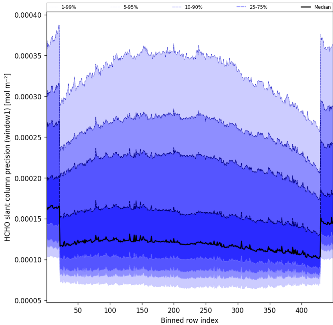
Figure 51: Along track statistics of “HCHO slant column precision (window1)” for 2025-01-03 to 2025-01-04
