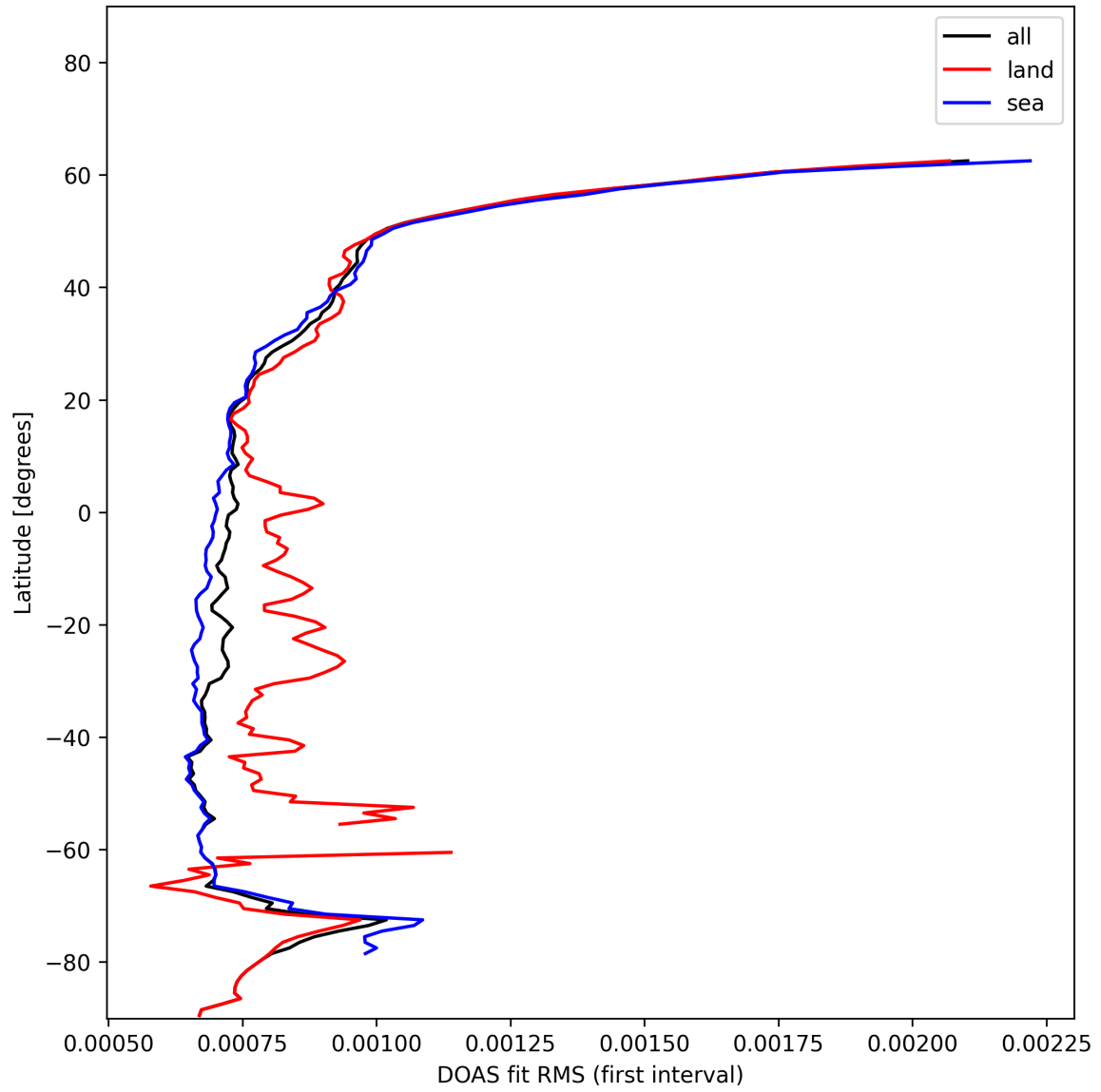
Figure 30: Zonal average of “DOAS fit RMS (first interval)” for 2025-01-03 to 2025-01-04.
