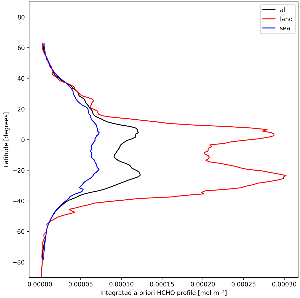
Figure 27: Zonal average of “Integrated a priori HCHO profile” for 2025-01-03 to 2025-01-04.
