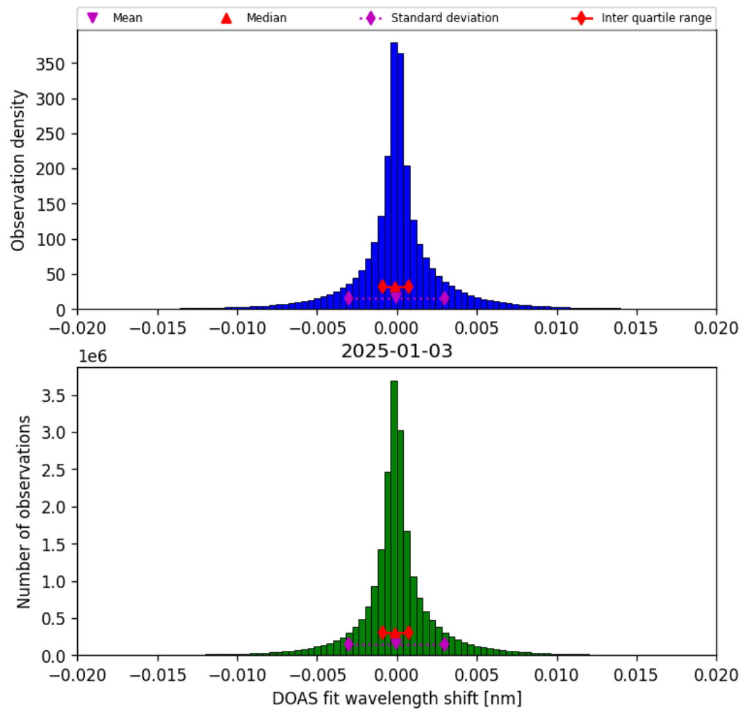
Figure 42: Histogram of “DOAS fit wavelength shift” for 2025-01-03 to 2025-01-04
