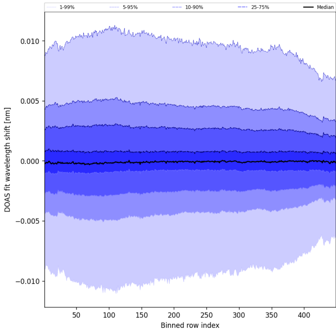
Figure 56: Along track statistics of “DOAS fit wavelength shift” for 2025-01-03 to 2025-01-04
