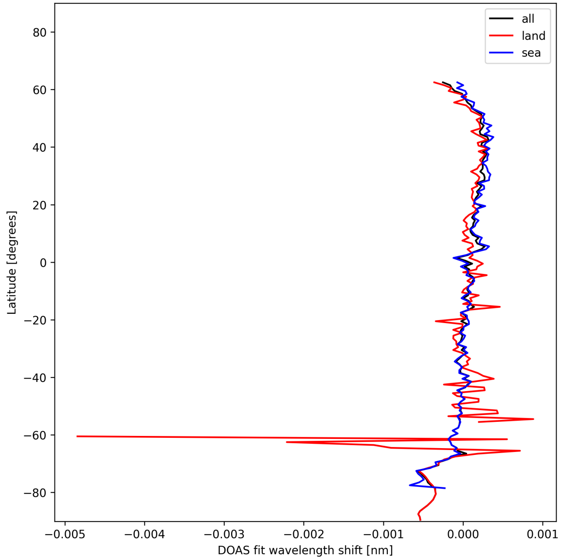
Figure 28: Zonal average of “DOAS fit wavelength shift” for 2025-01-03 to 2025-01-04.
