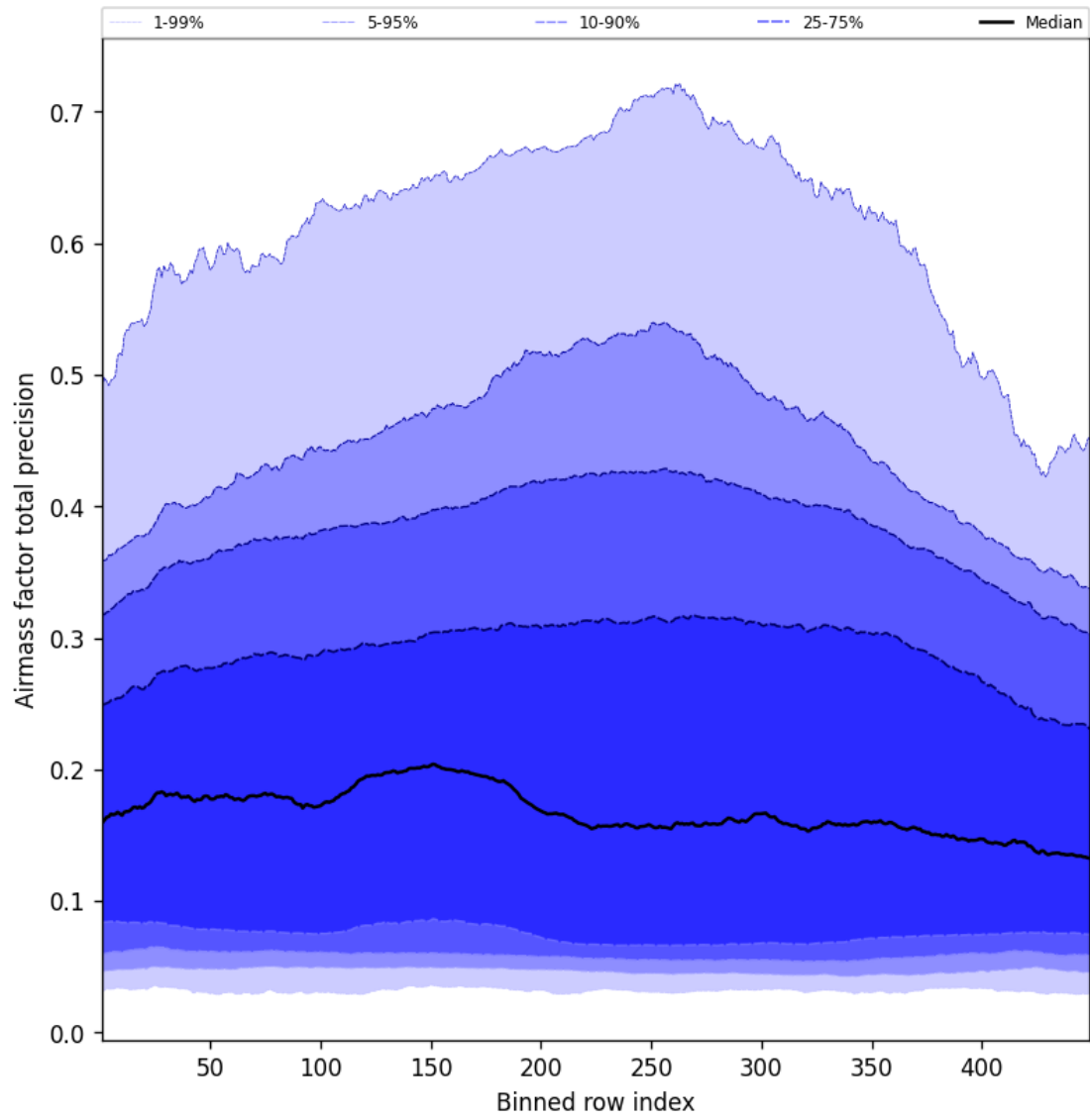
Figure 53: Along track statistics of “Airmass factor total precision” for 2025-01-03 to 2025-01-04
