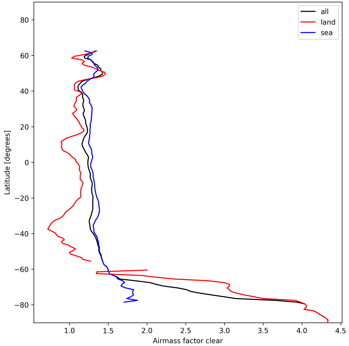
Figure 26: Zonal average of “Airmass factor clear” for 2025-01-03 to 2025-01-04.
