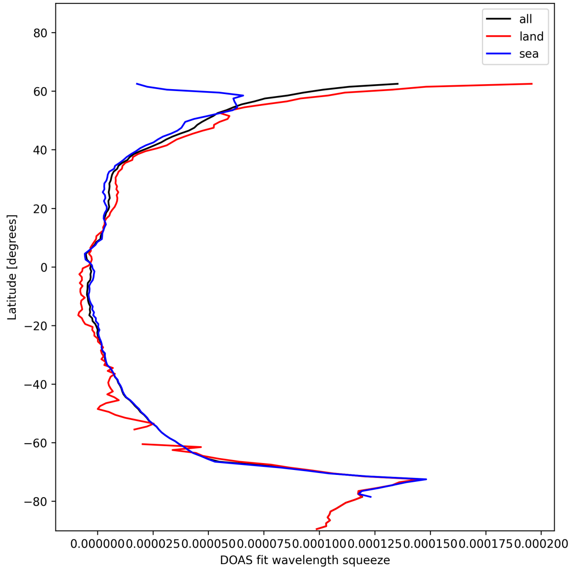
Figure 29: Zonal average of “DOAS fit wavelength squeeze” for 2025-01-03 to 2025-01-04.
