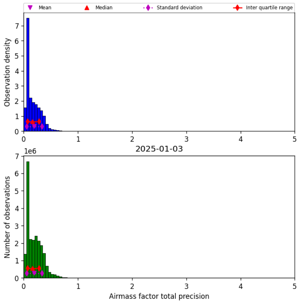
Figure 39: Histogram of “Airmass factor total precision” for 2025-01-03 to 2025-01-04
