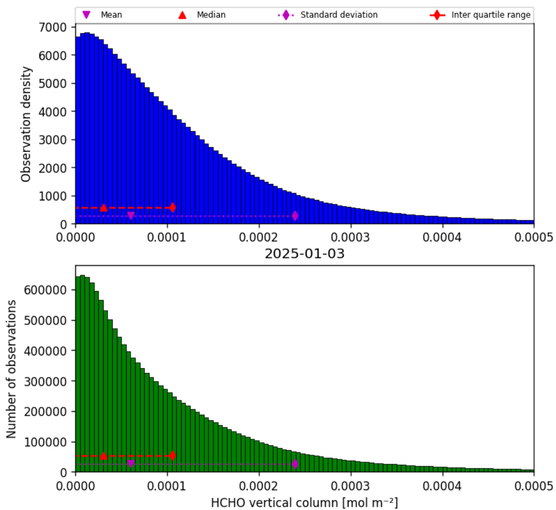
Figure 33: Histogram of “HCHO vertical column” for 2025-01-03 to 2025-01-04
