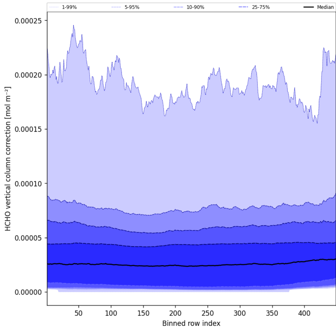
Figure 49: Along track statistics of “HCHO vertical column correction” for 2025-01-03 to 2025-01-04
