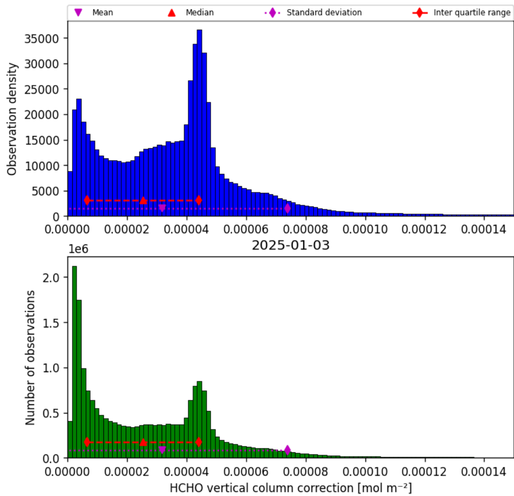
Figure 35: Histogram of “HCHO vertical column correction” for 2025-01-03 to 2025-01-04
