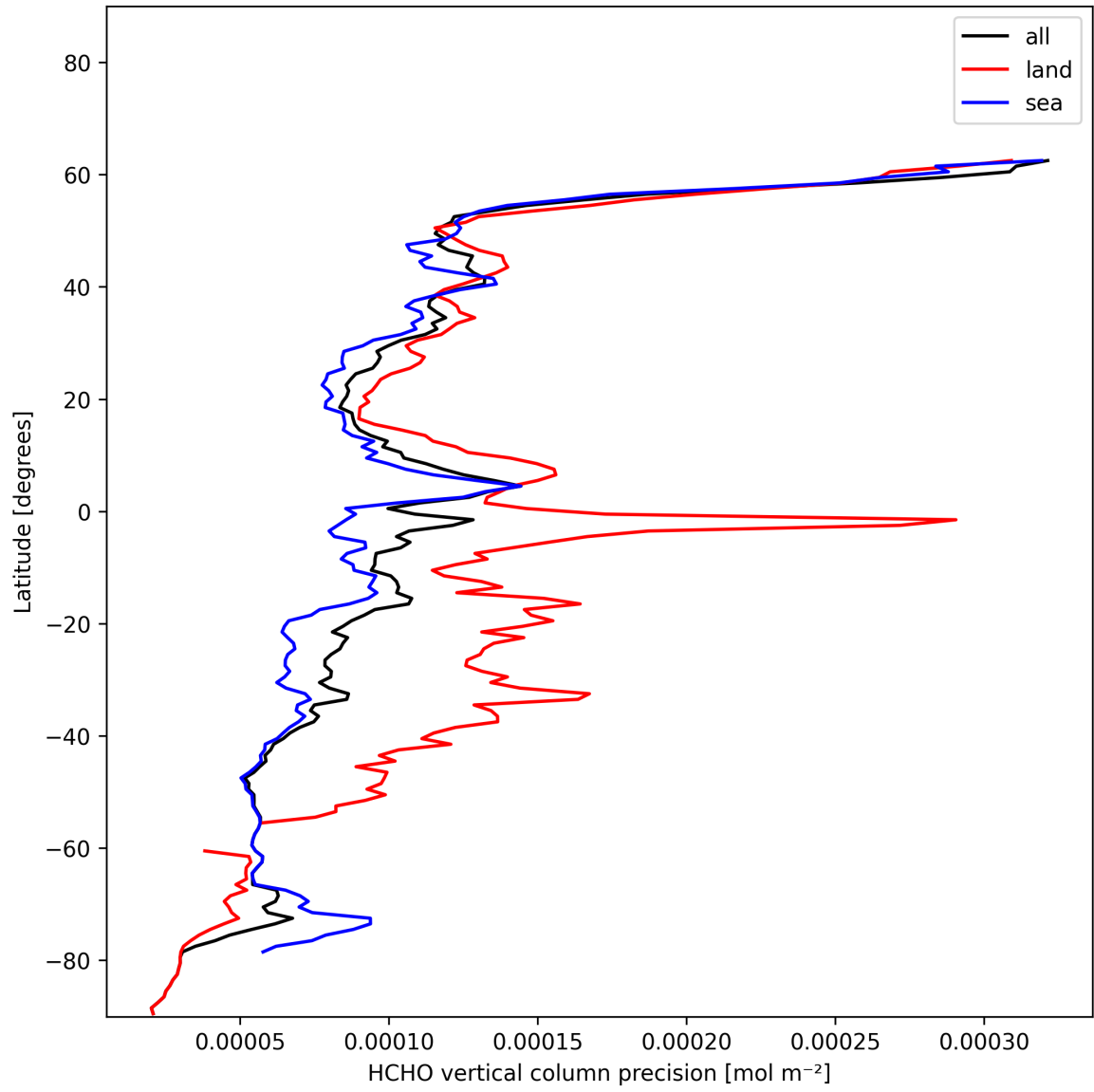
Figure 20: Zonal average of “HCHO vertical column precision” for 2025-01-03 to 2025-01-04.
