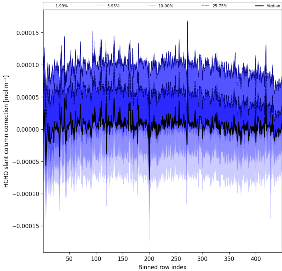
Figure 59: Along track statistics of “HCHO slant column correction” for 2025-01-03 to 2025-01-04
