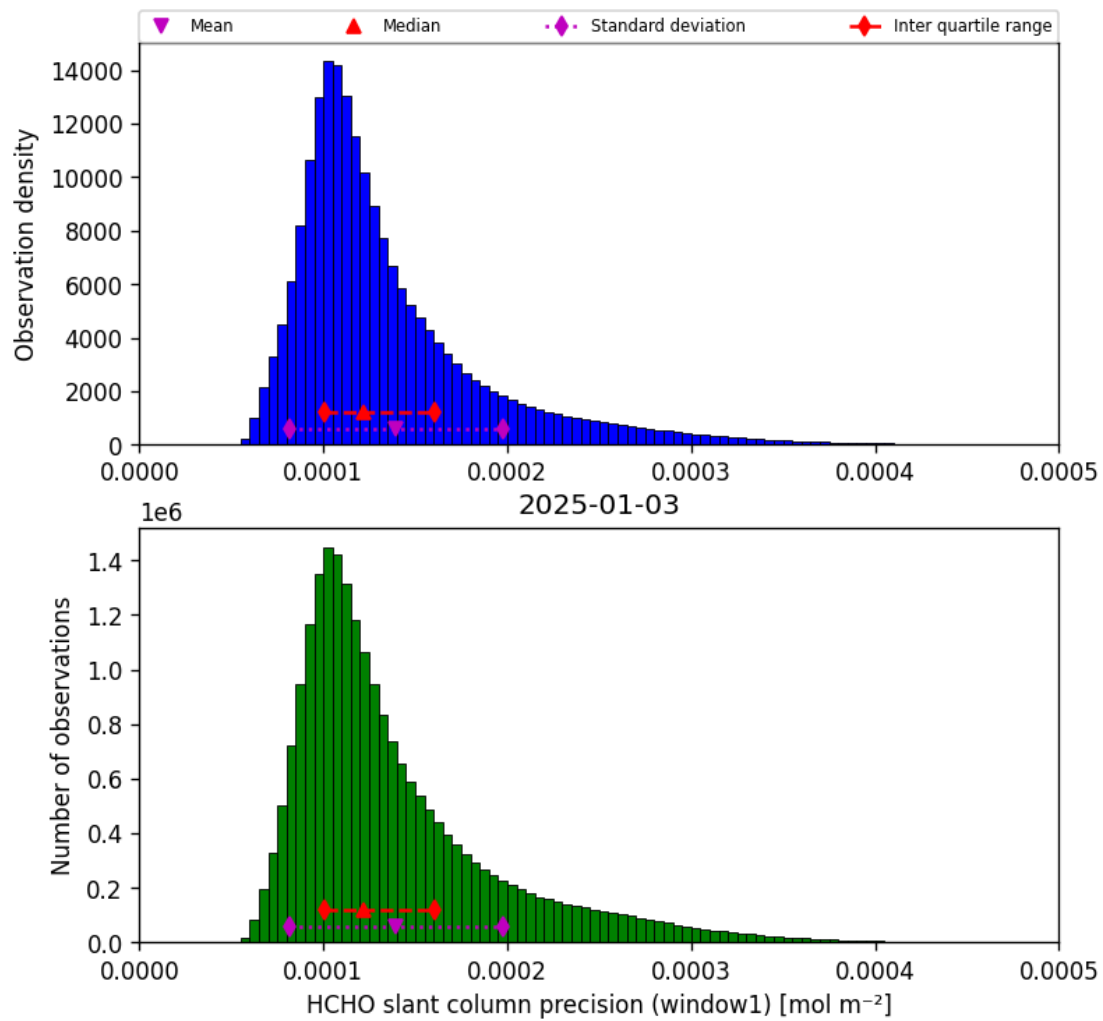
Figure 37: Histogram of “HCHO slant column precision (window1)” for 2025-01-03 to 2025-01-04
