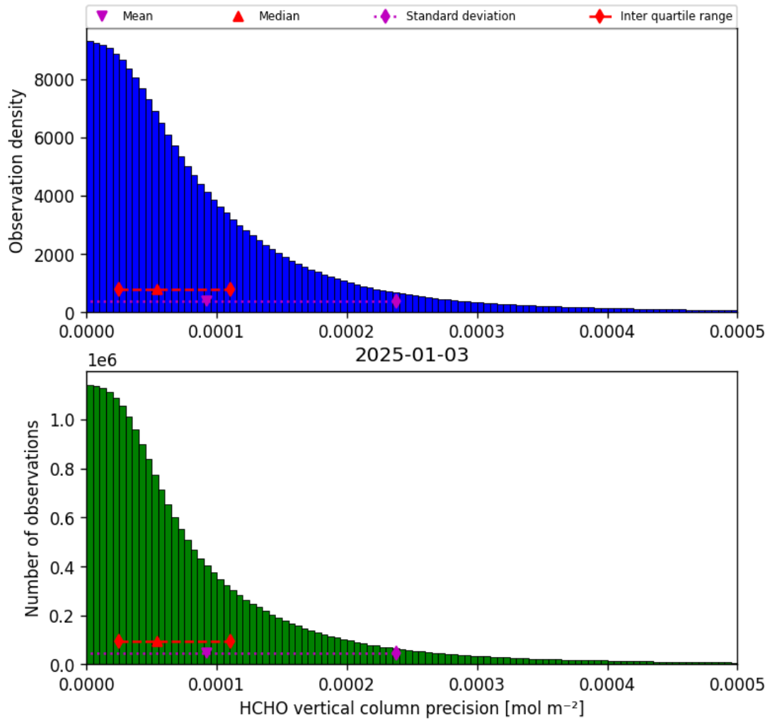
Figure 34: Histogram of “HCHO vertical column precision” for 2025-01-03 to 2025-01-04
