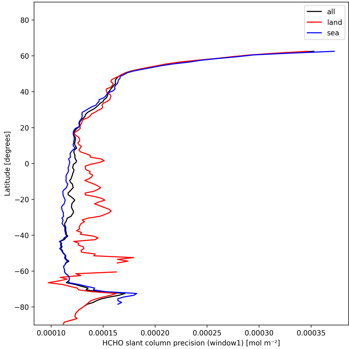
Figure 23: Zonal average of “HCHO slant column precision (window1)” for 2025-01-03 to 2025-01-04.
