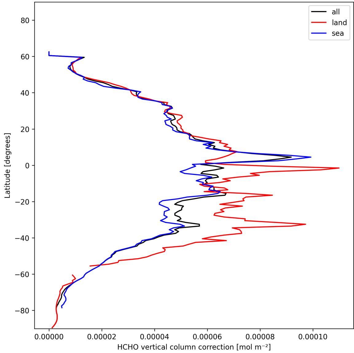
Figure 21: Zonal average of “HCHO vertical column correction” for 2025-01-03 to 2025-01-04.
