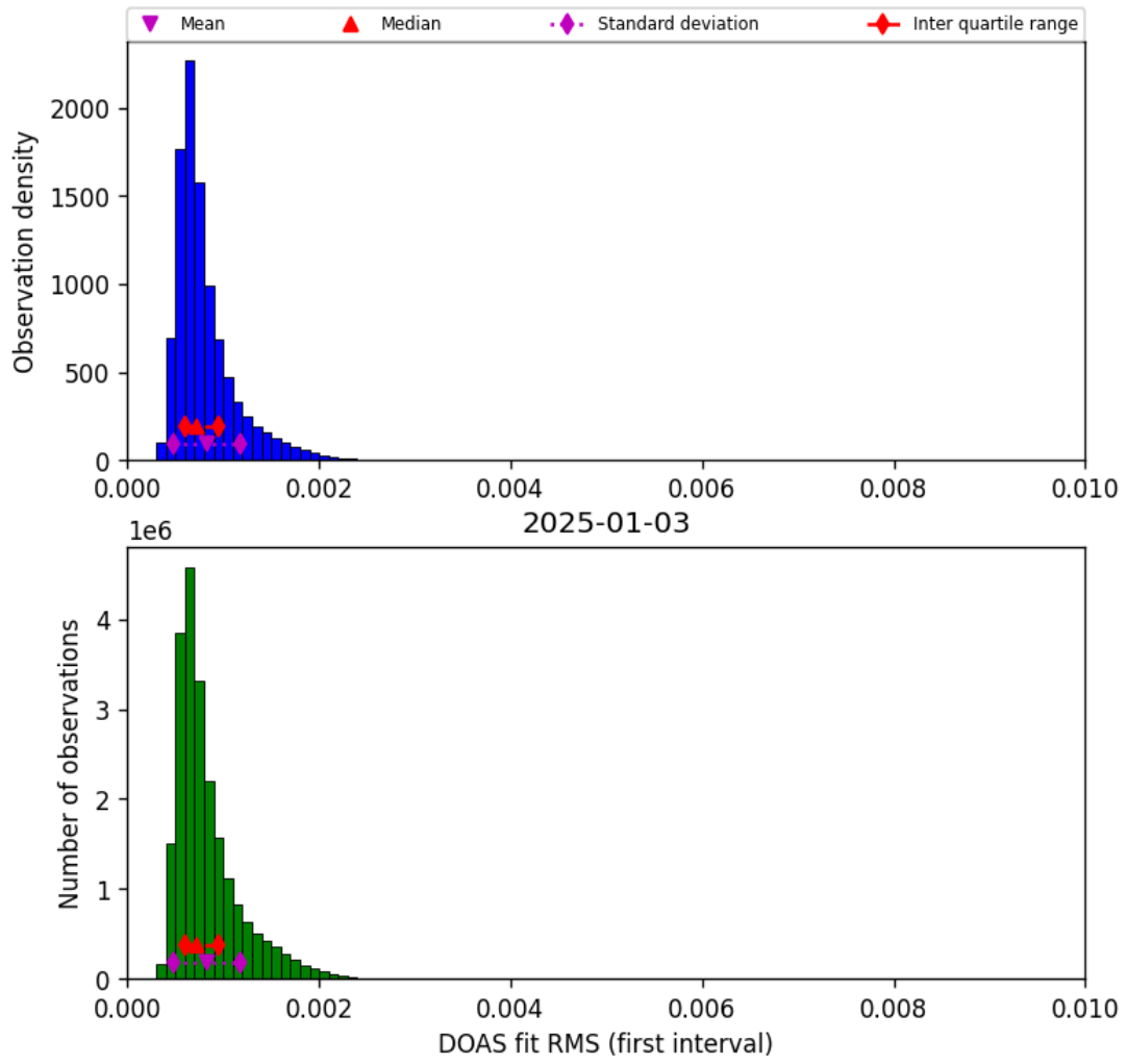
Figure 44: Histogram of “DOAS fit RMS (first interval)” for 2025-01-03 to 2025-01-04
