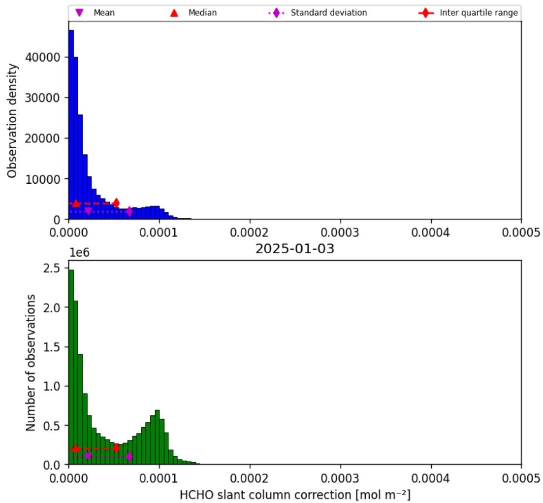
Figure 45: Histogram of “HCHO slant column correction” for 2025-01-03 to 2025-01-04
