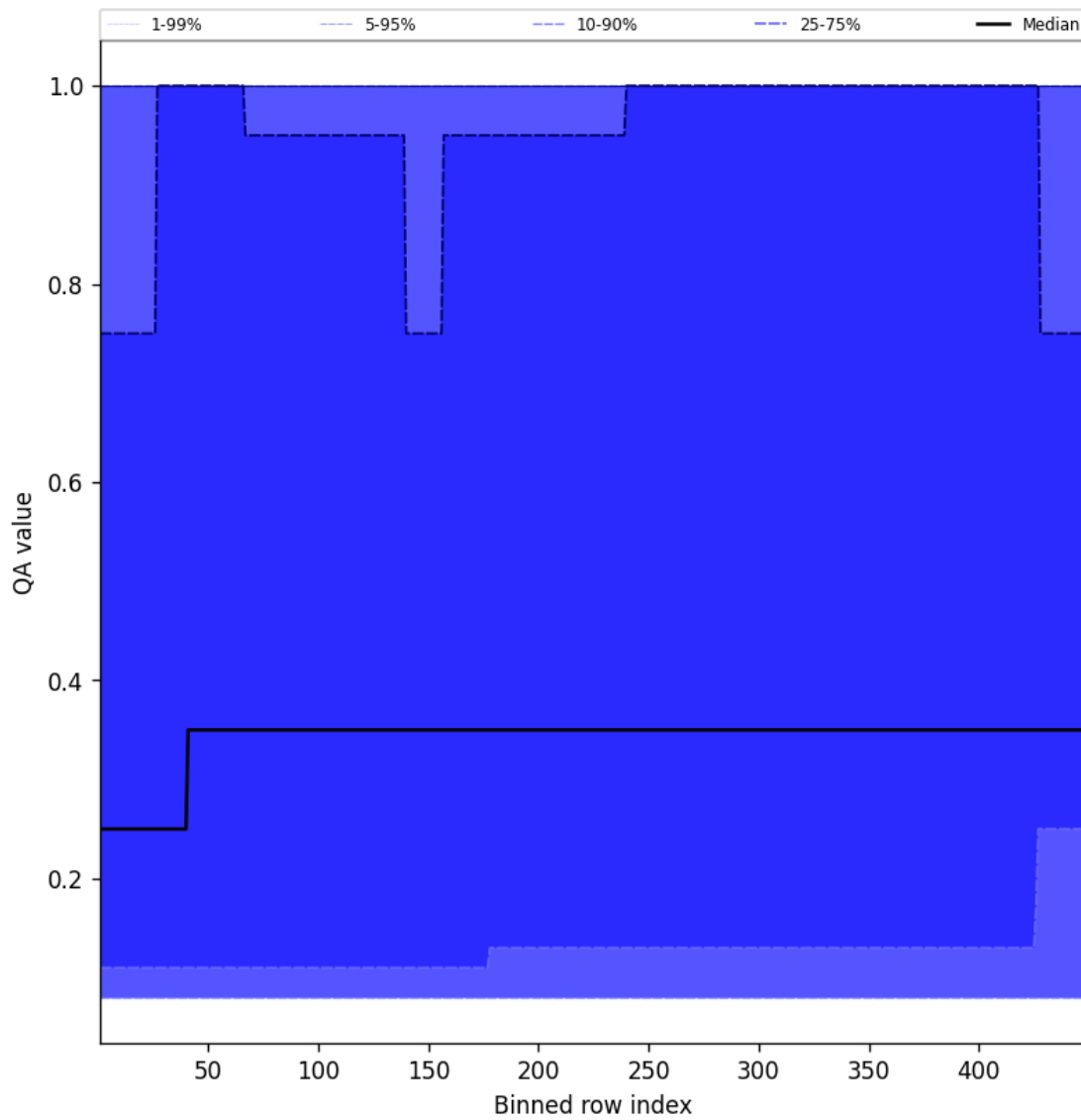
Figure 46: Along track statistics of “QA value” for 2025-01-03 to 2025-01-04
