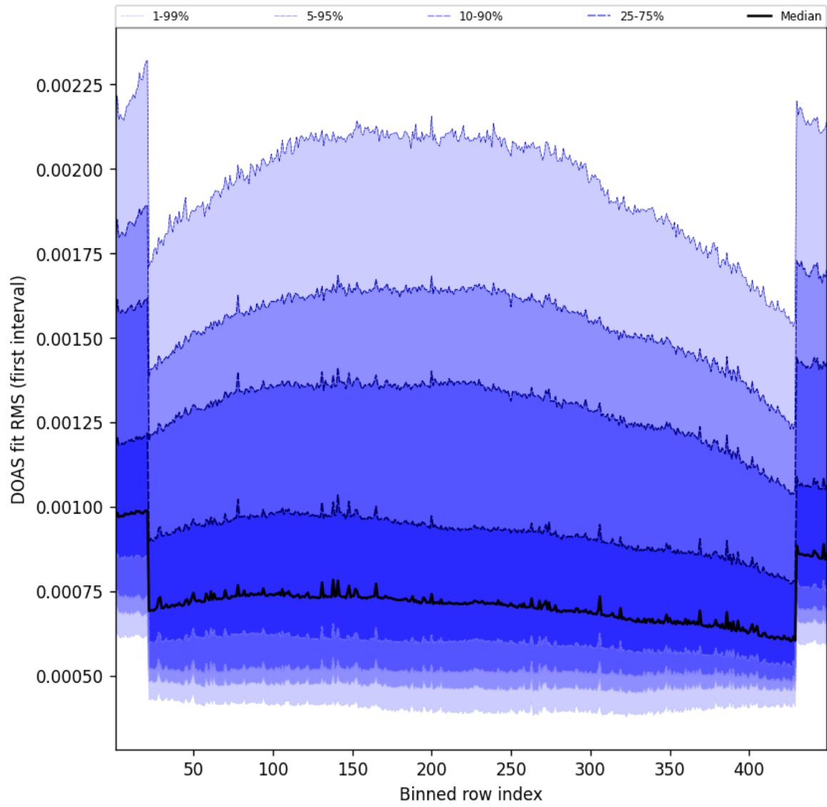
Figure 58: Along track statistics of “DOAS fit RMS (first interval)” for 2025-01-03 to 2025-01-04
