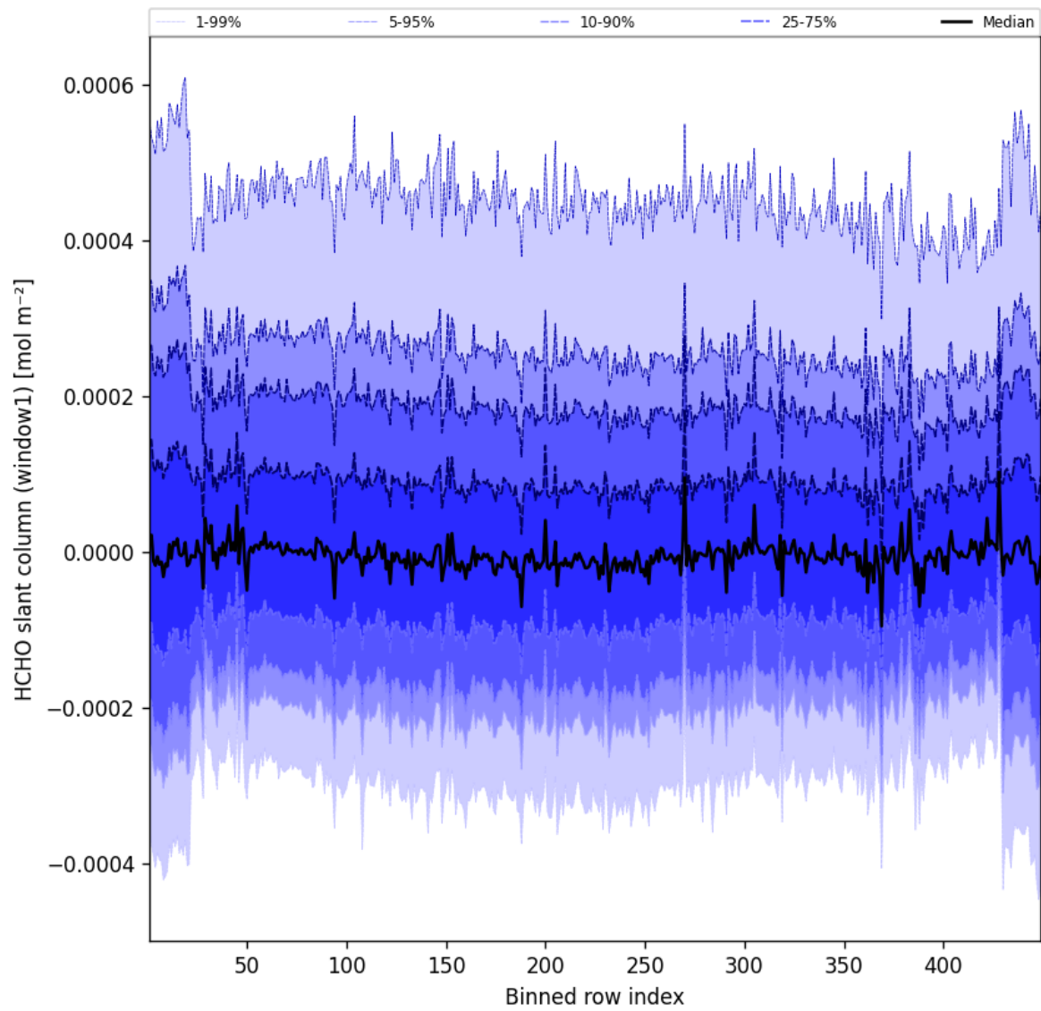
Figure 50: Along track statistics of “HCHO slant column (window1)” for 2025-01-03 to 2025-01-04
