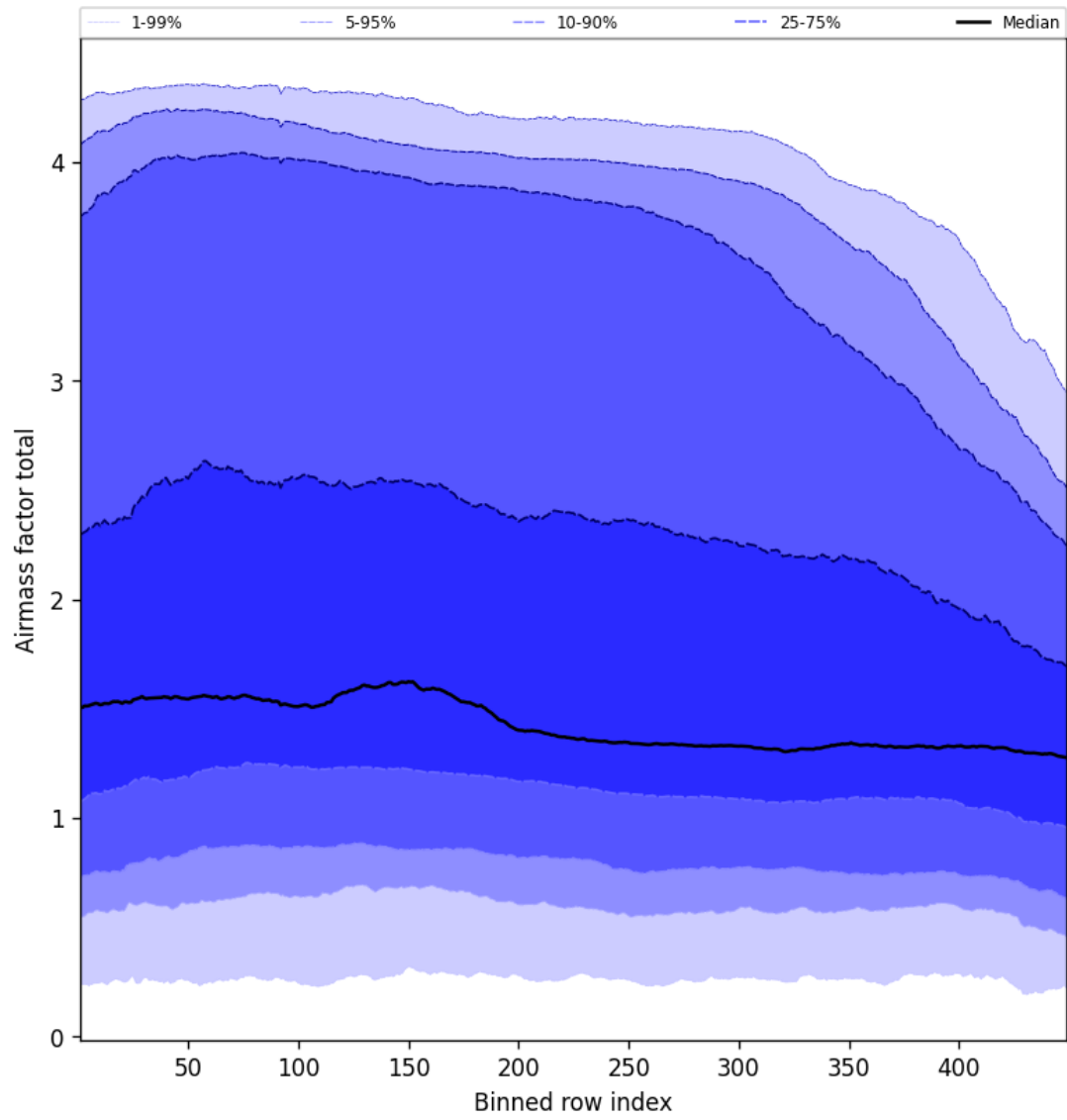
Figure 52: Along track statistics of “Airmass factor total” for 2025-01-03 to 2025-01-04
