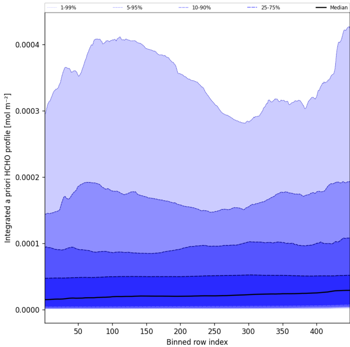
Figure 55: Along track statistics of “Integrated a priori HCHO profile” for 2025-01-03 to 2025-01-04
