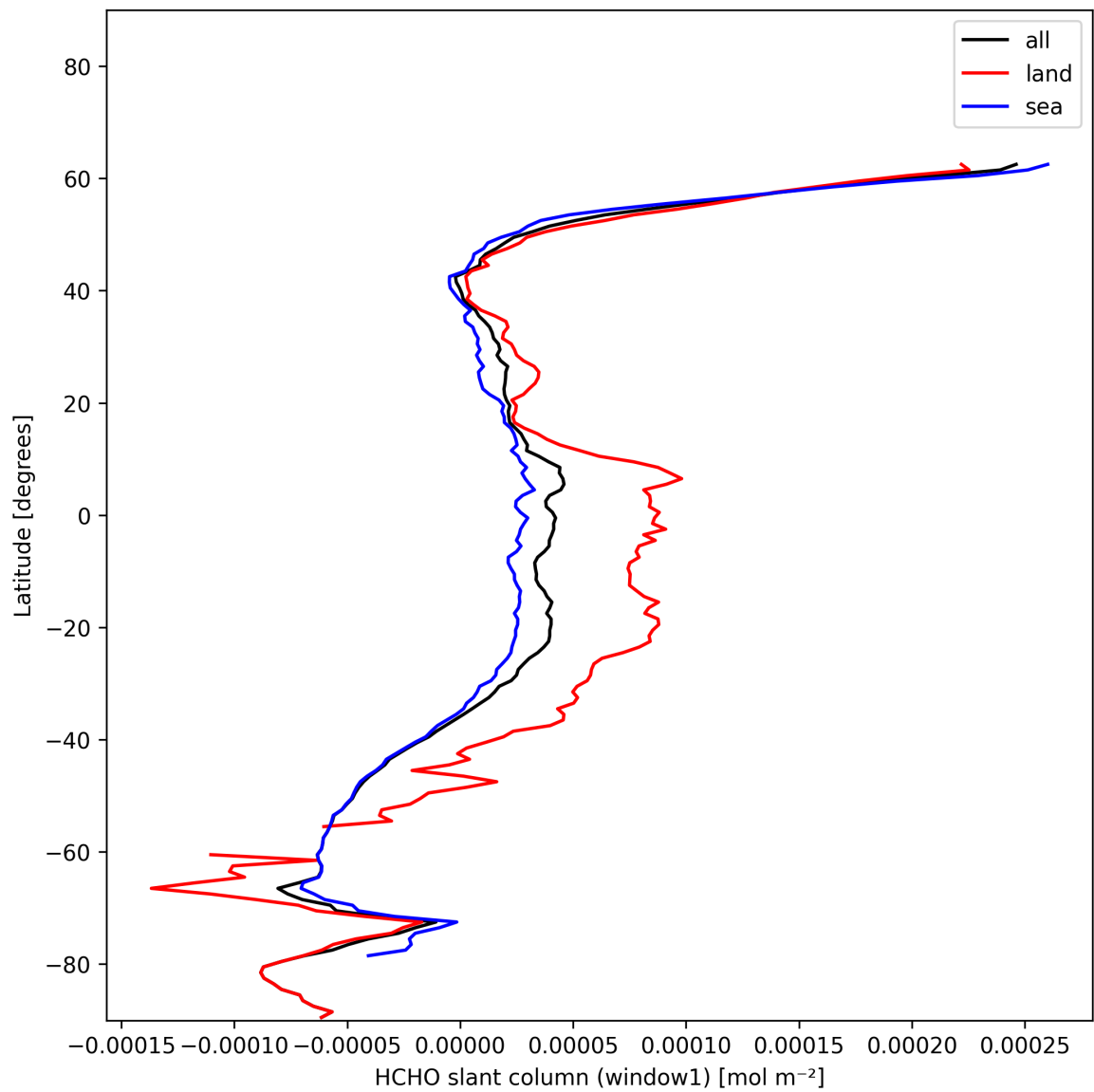
Figure 22: Zonal average of “HCHO slant column (window1)” for 2025-01-03 to 2025-01-04.
