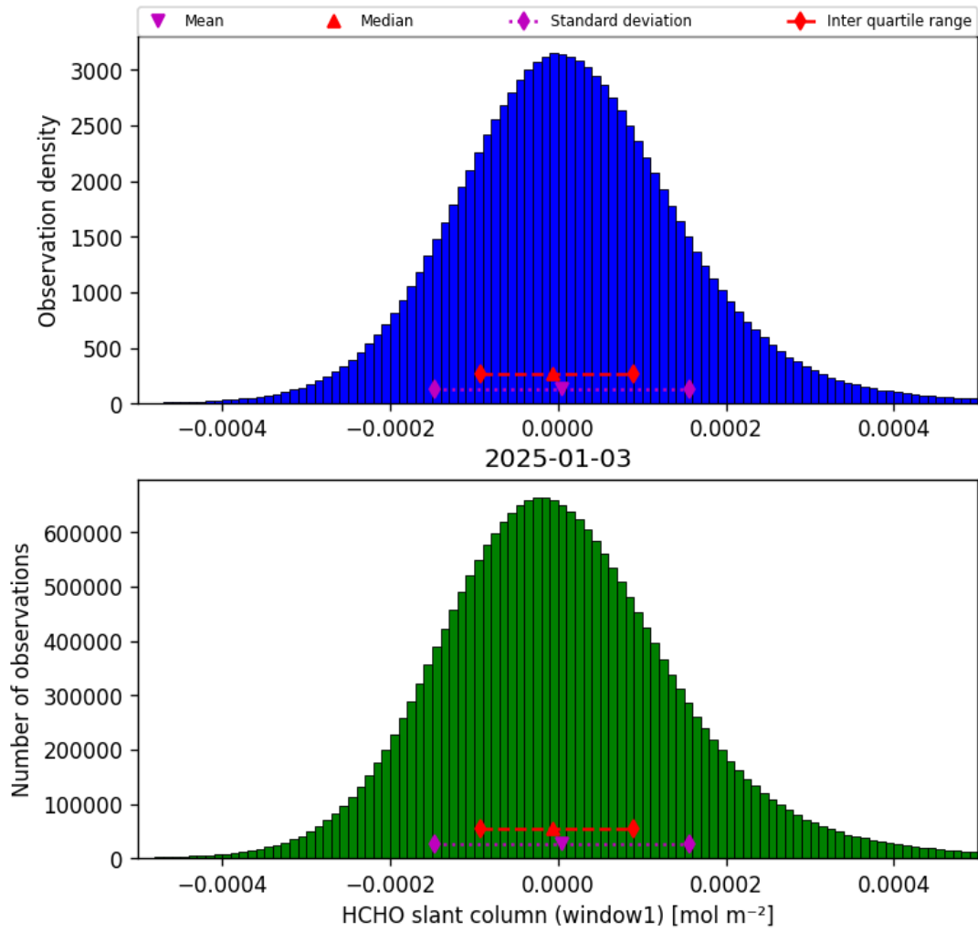
Figure 36: Histogram of “HCHO slant column (window1)” for 2025-01-03 to 2025-01-04
