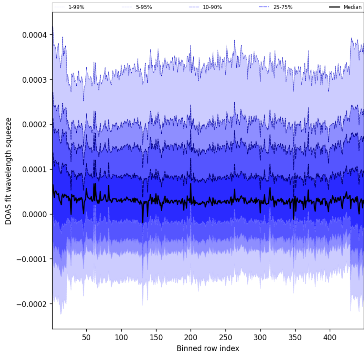
Figure 57: Along track statistics of “DOAS fit wavelength squeeze” for 2025-01-03 to 2025-01-04
