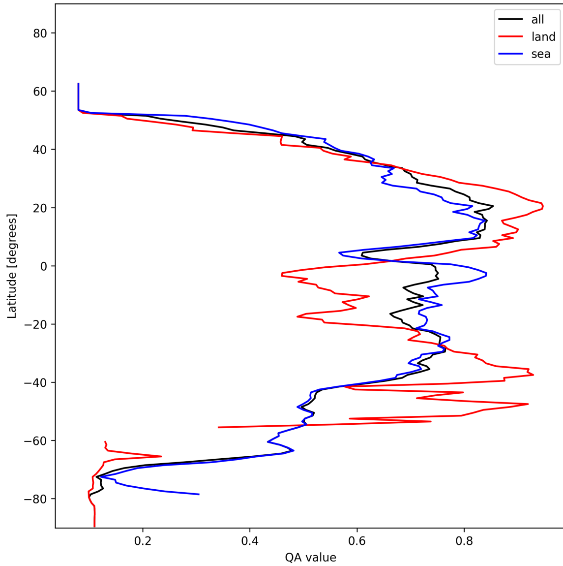
Figure 18: Zonal average of “QA value” for 2025-01-03 to 2025-01-04.
