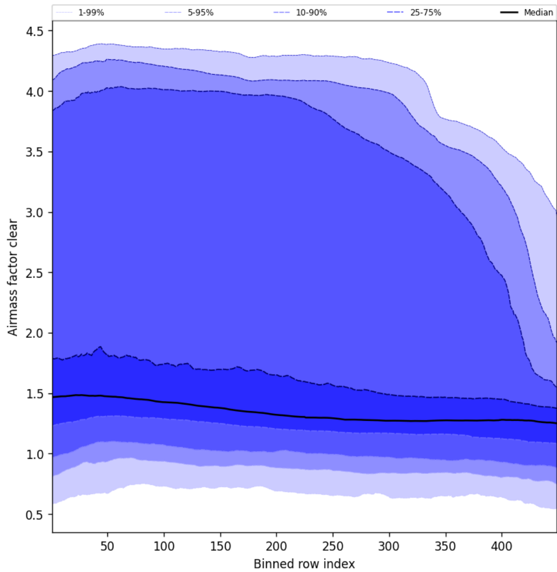
Figure 54: Along track statistics of “Airmass factor clear” for 2025-01-05 to 2025-01-05
