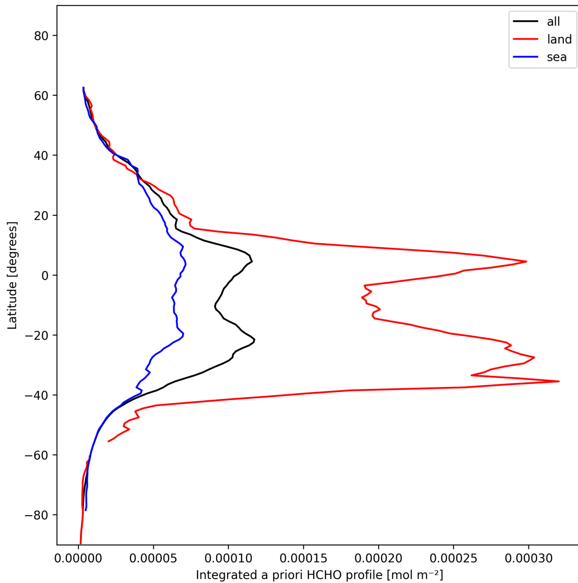
Figure 27: Zonal average of “Integrated a priori HCHO profile” for 2025-01-05 to 2025-01-05.
