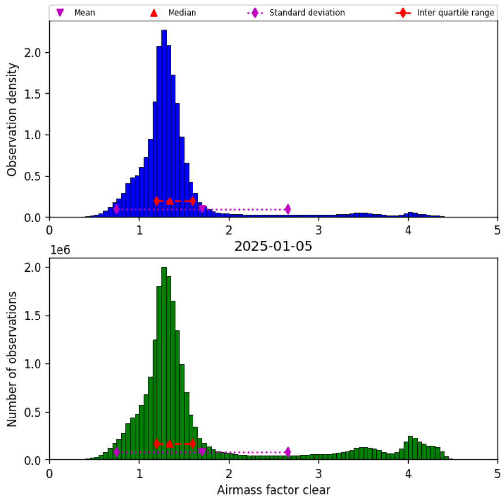
Figure 40: Histogram of “Airmass factor clear” for 2025-01-05 to 2025-01-05
