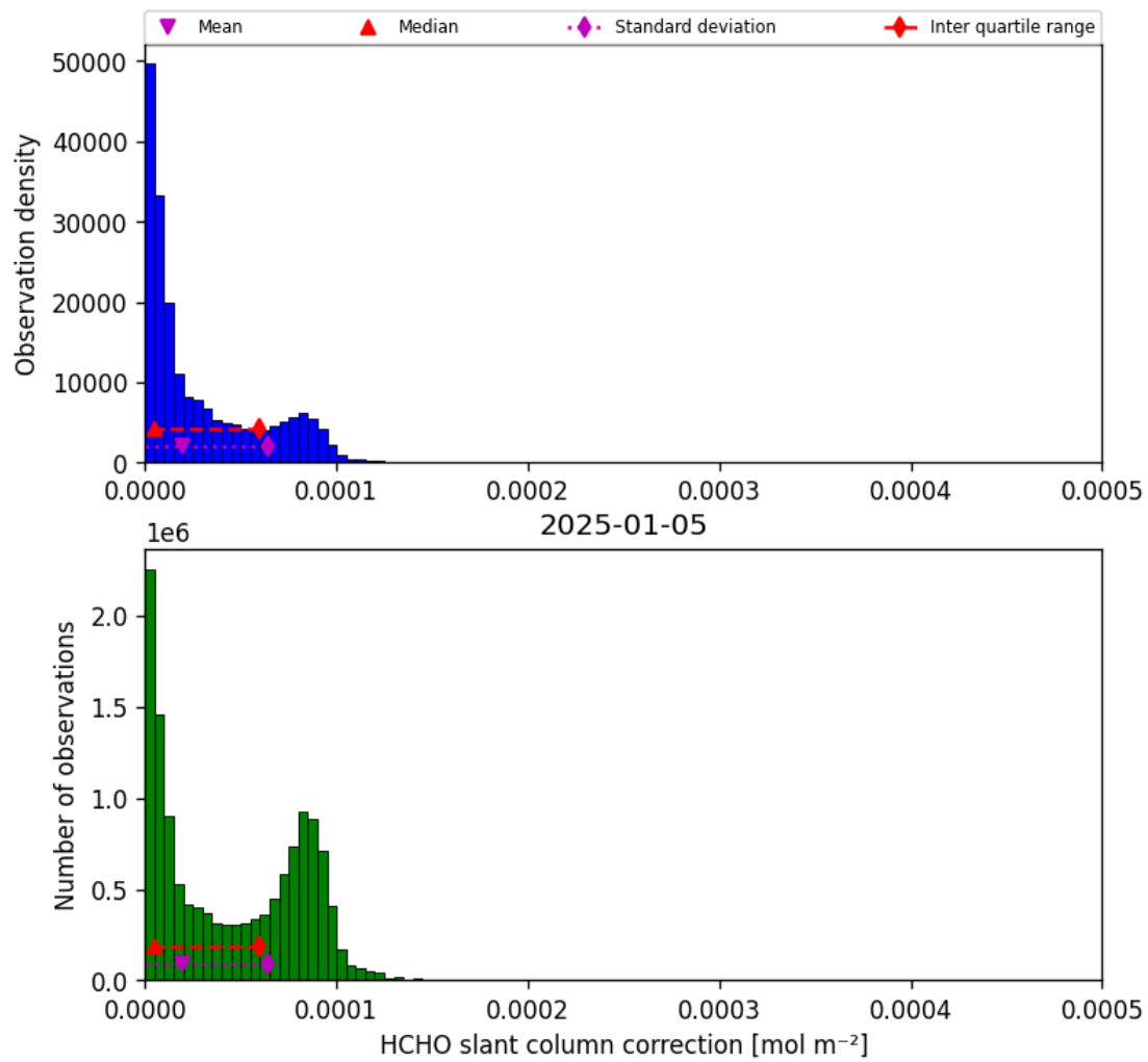
Figure 45: Histogram of “HCHO slant column correction” for 2025-01-05 to 2025-01-05
