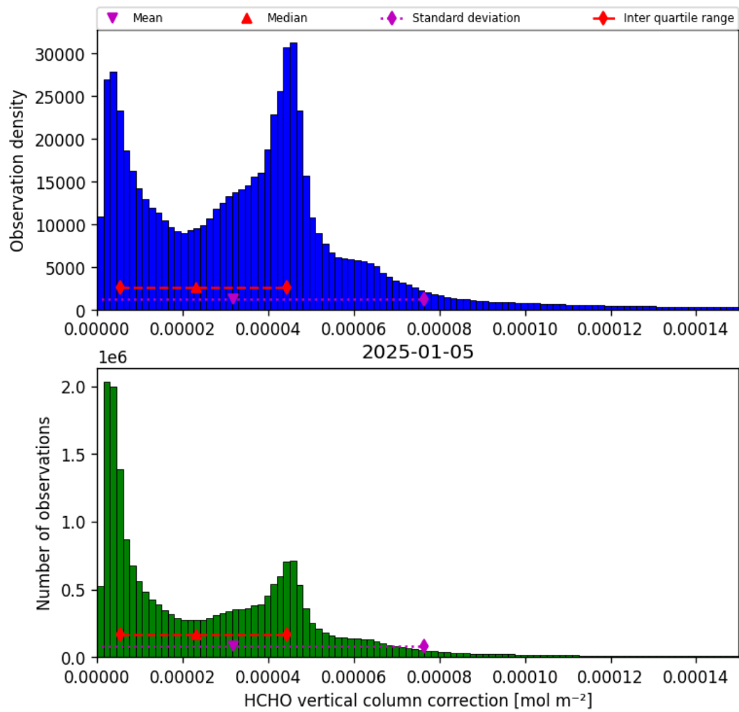
Figure 35: Histogram of “HCHO vertical column correction” for 2025-01-05 to 2025-01-05
