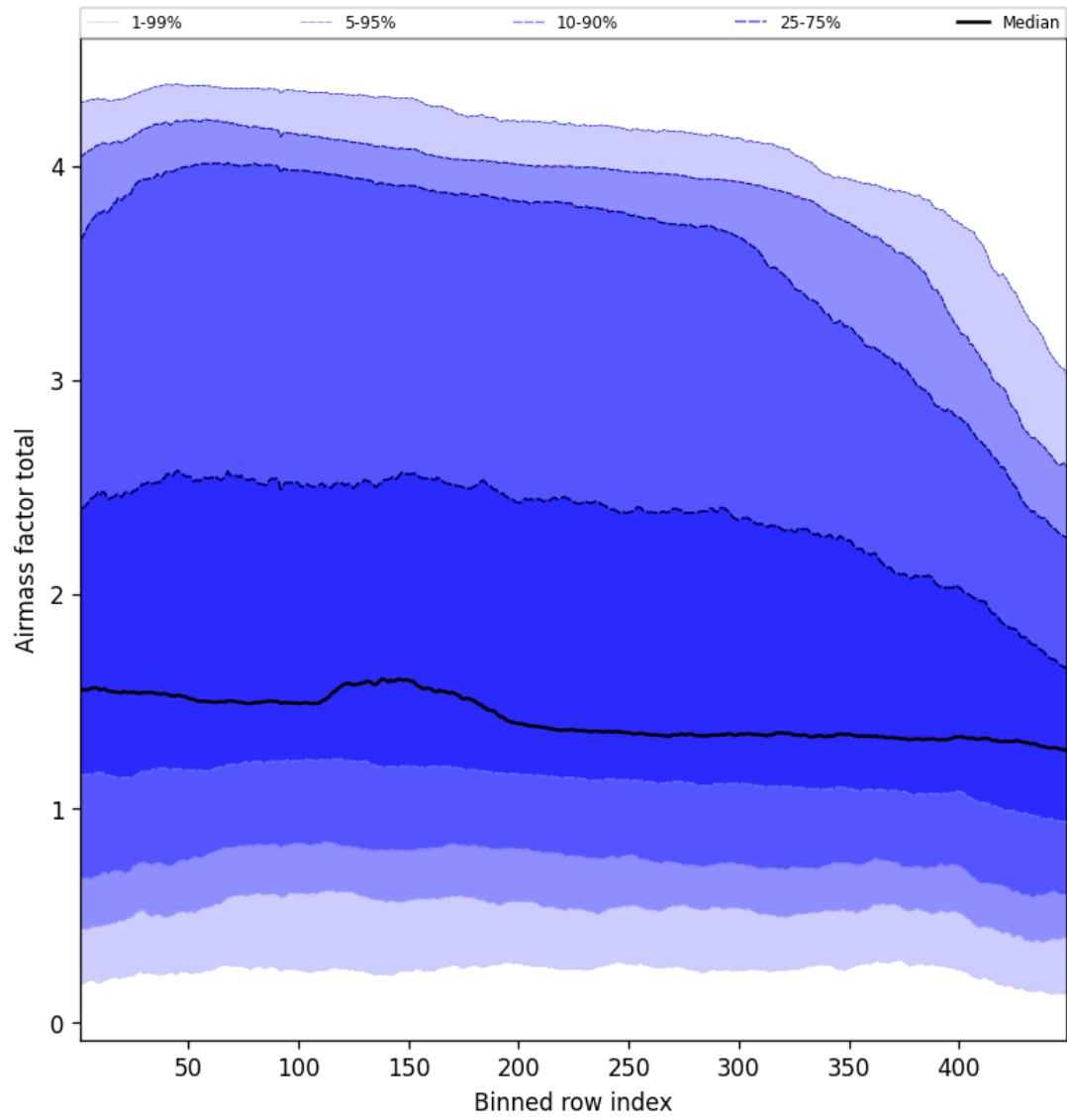
Figure 52: Along track statistics of “Airmass factor total” for 2025-01-05 to 2025-01-05
