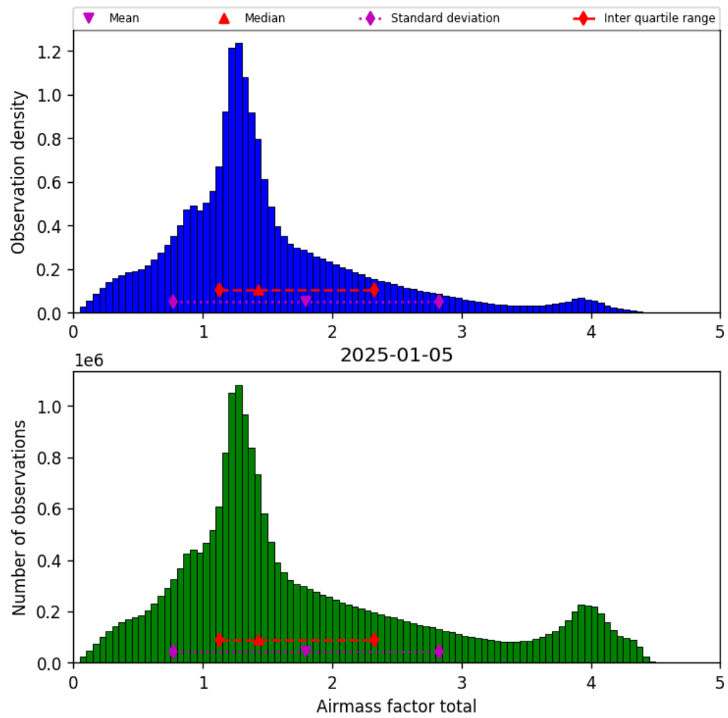
Figure 38: Histogram of “Airmass factor total” for 2025-01-05 to 2025-01-05
