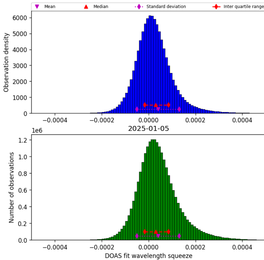
Figure 43: Histogram of “DOAS fit wavelength squeeze” for 2025-01-05 to 2025-01-05
