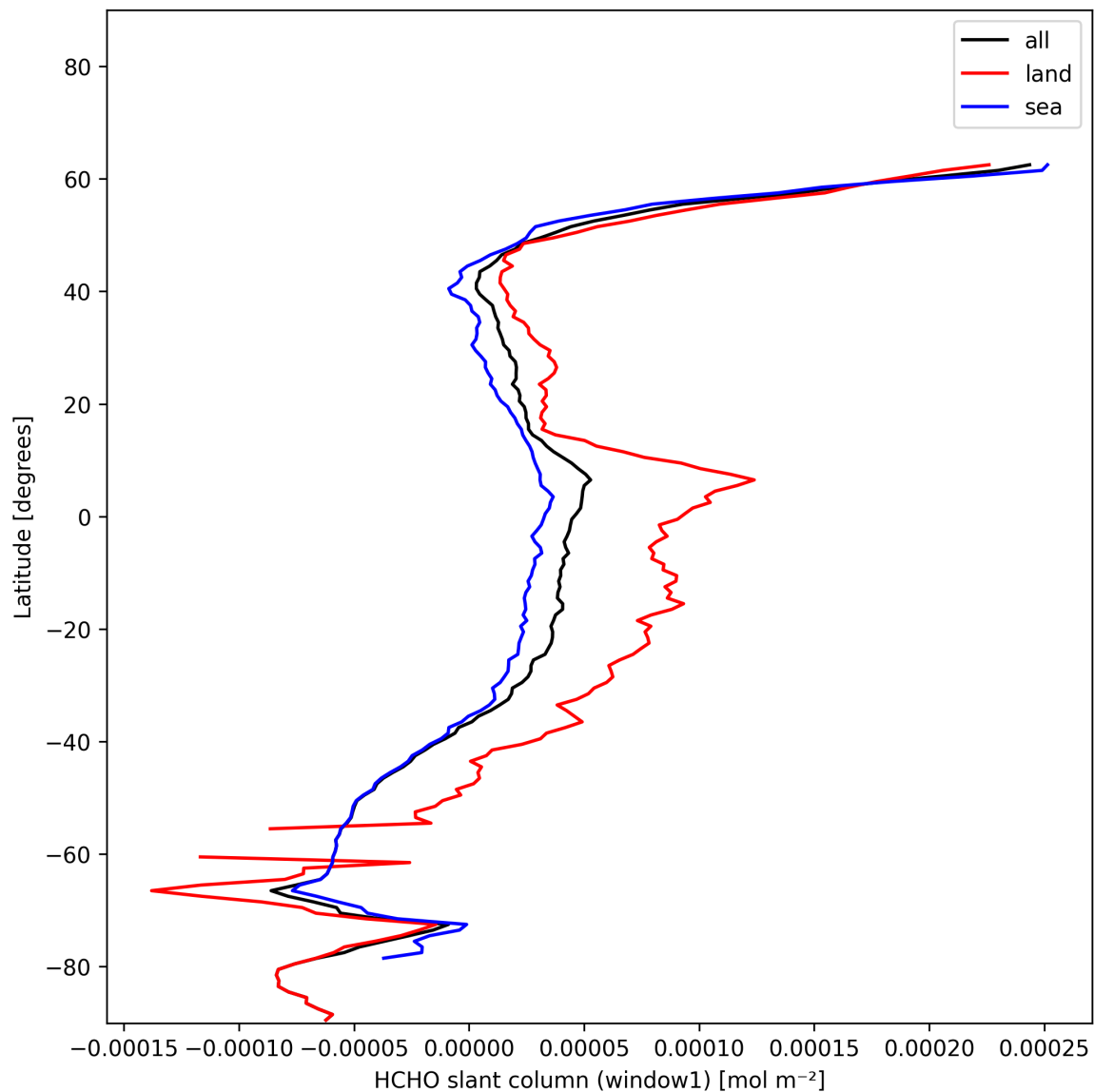
Figure 22: Zonal average of “HCHO slant column (window1)” for 2025-01-05 to 2025-01-05.
