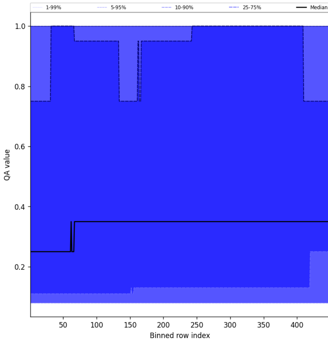
Figure 46: Along track statistics of “QA value” for 2025-01-05 to 2025-01-05
