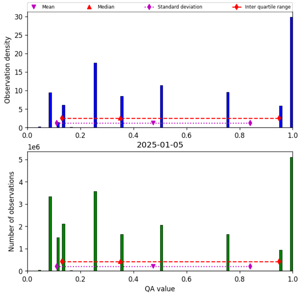
Figure 32: Histogram of “QA value” for 2025-01-05 to 2025-01-05
