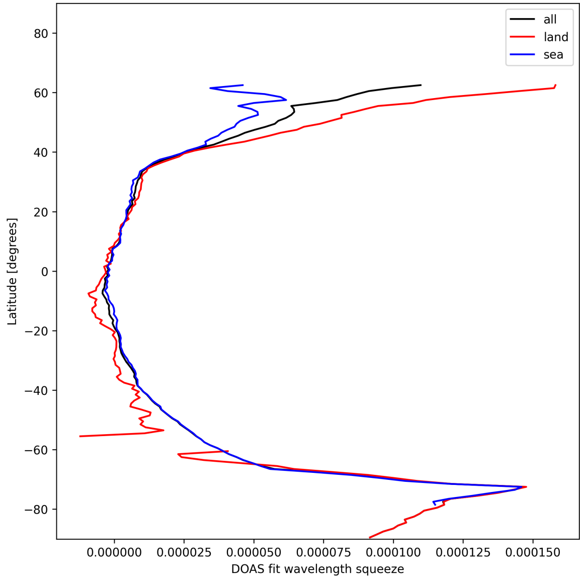
Figure 29: Zonal average of “DOAS fit wavelength squeeze” for 2025-01-05 to 2025-01-05.
