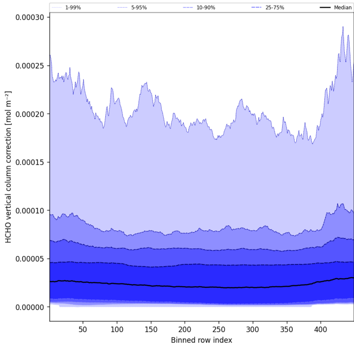
Figure 49: Along track statistics of “HCHO vertical column correction” for 2025-01-05 to 2025-01-05
