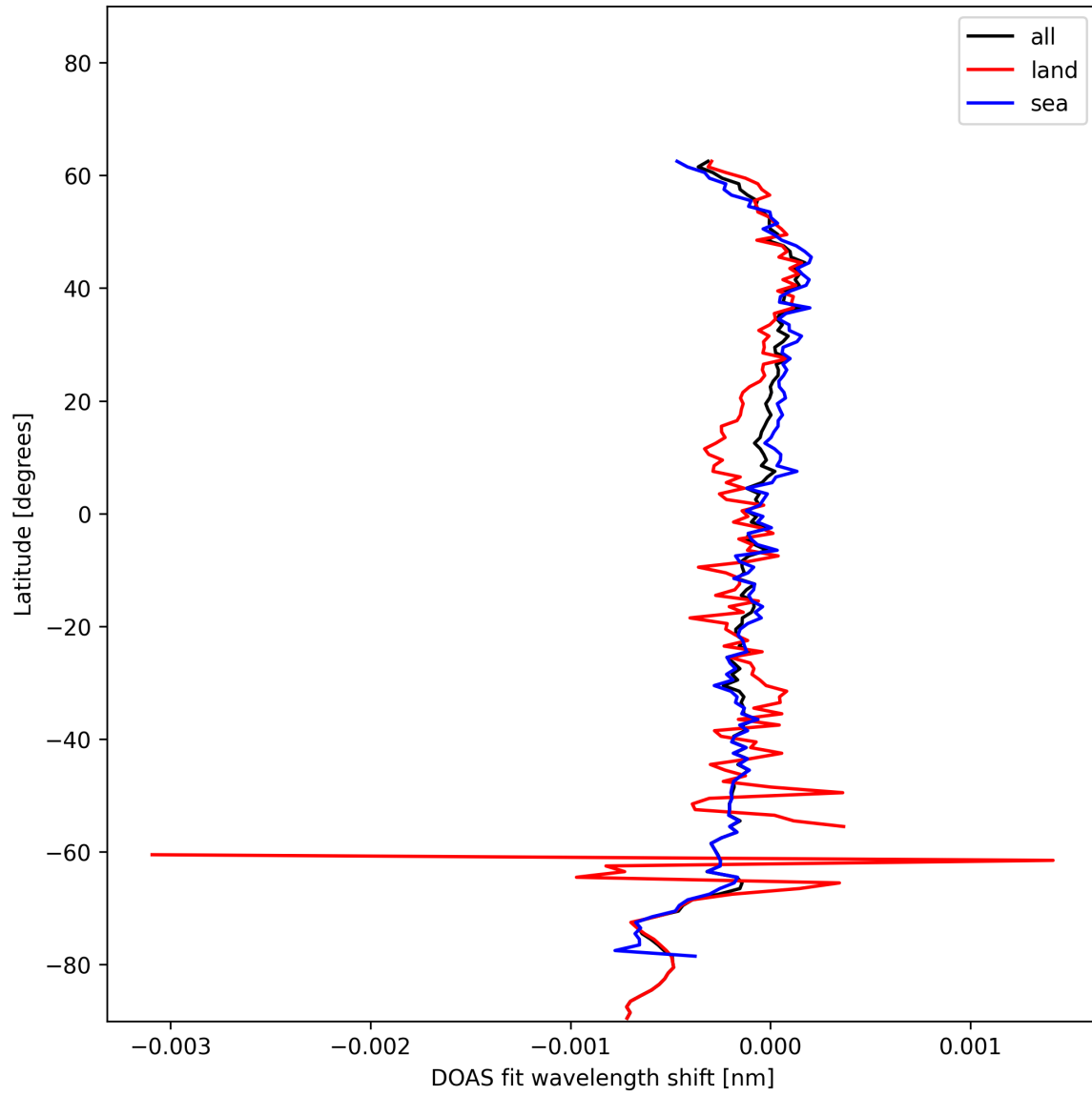
Figure 28: Zonal average of “DOAS fit wavelength shift” for 2025-01-05 to 2025-01-05.
