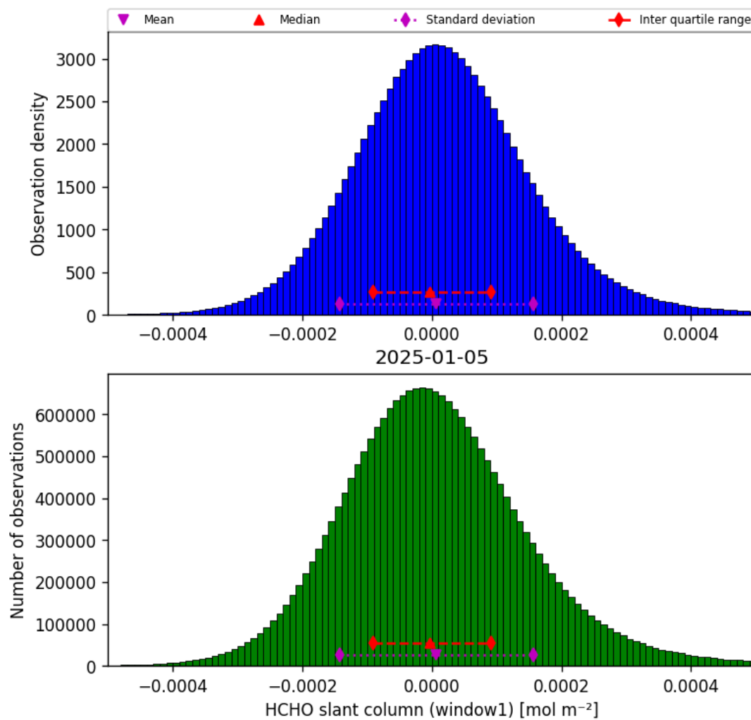
Figure 36: Histogram of “HCHO slant column (window1)” for 2025-01-05 to 2025-01-05
