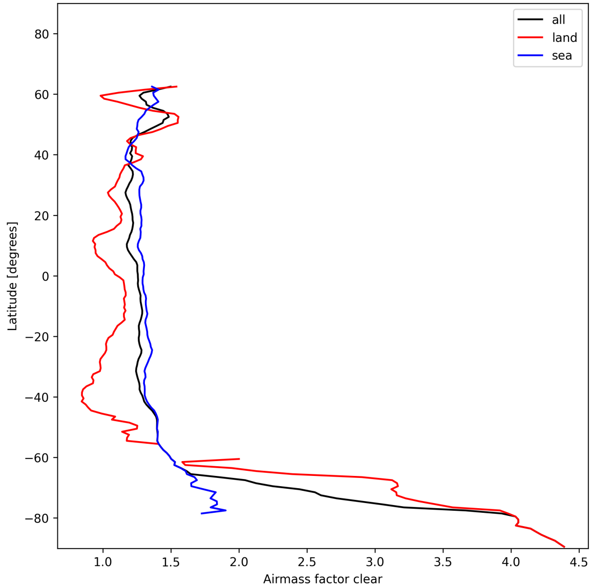
Figure 26: Zonal average of “Airmass factor clear” for 2025-01-05 to 2025-01-05.
