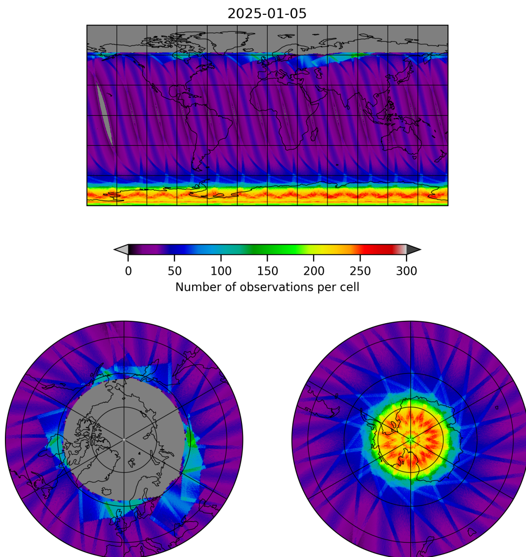
Figure 17: Map of the number of observations for 2025-01-05 to 2025-01-05
