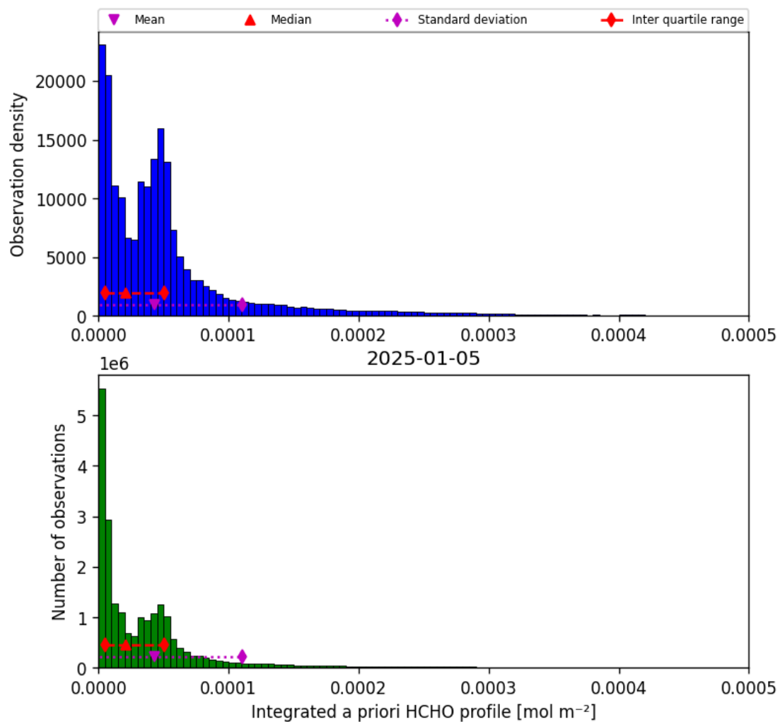
Figure 41: Histogram of “Integrated a priori HCHO profile” for 2025-01-05 to 2025-01-05
