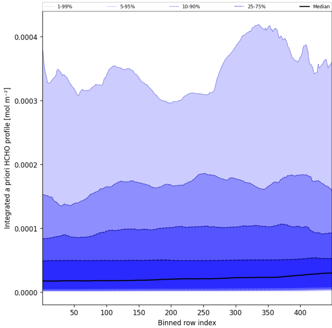
Figure 55: Along track statistics of "Integrated a priori HCHO profile" for 2025-01-05 to 2025-01-05
