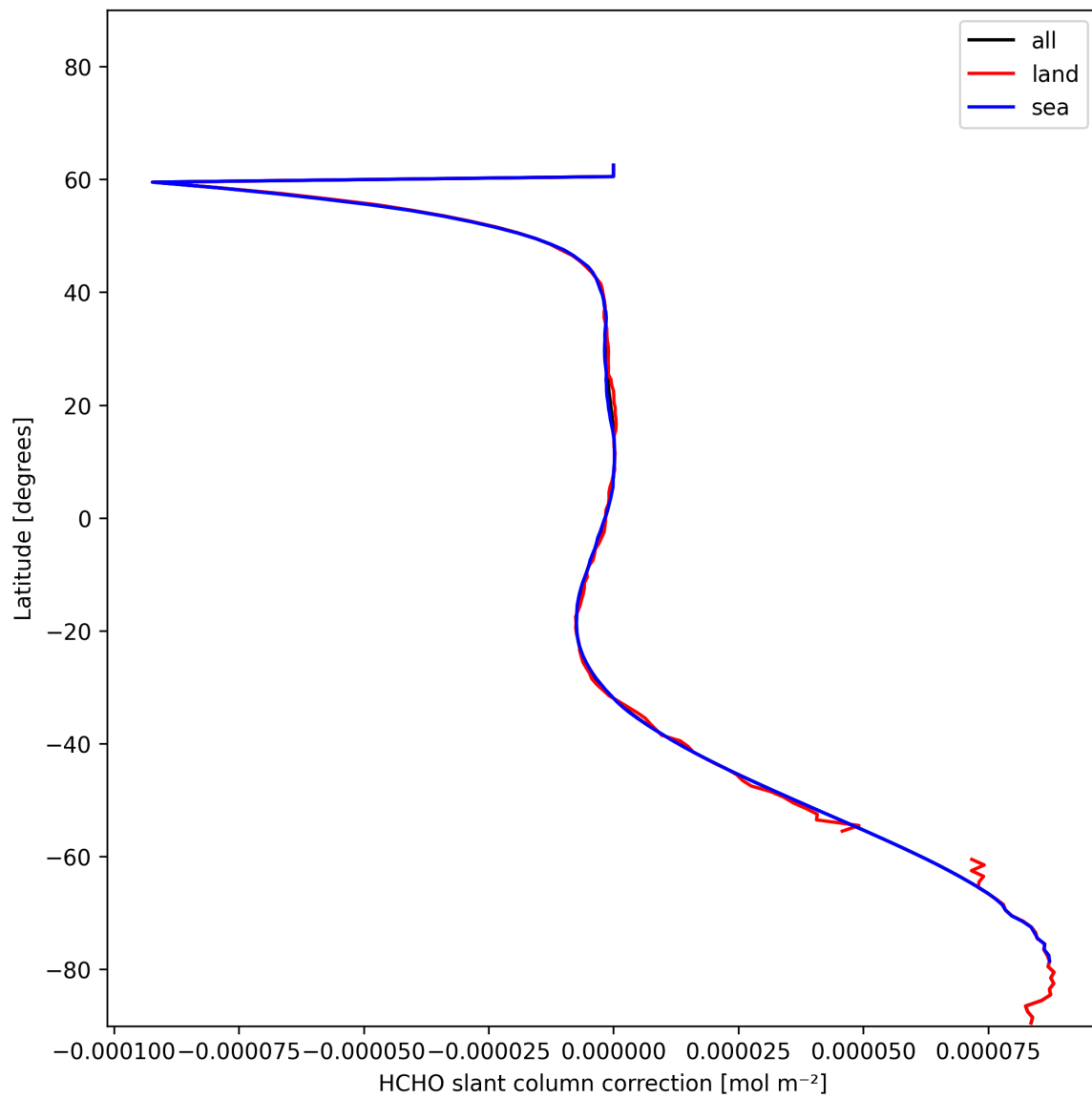
Figure 31: Zonal average of “HCHO slant column correction” for 2025-01-05 to 2025-01-05.
