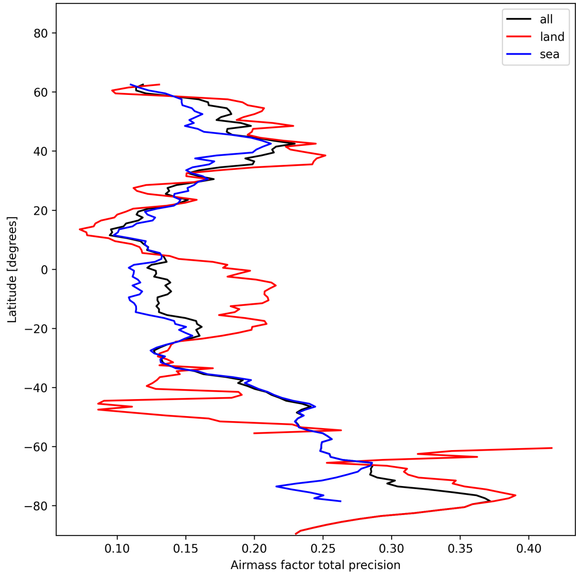
Figure 25: Zonal average of “Airmass factor total precision” for 2025-01-05 to 2025-01-05.
