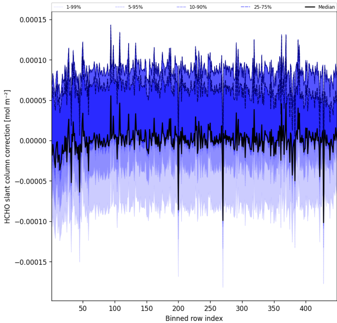
Figure 59: Along track statistics of “HCHO slant column correction” for 2025-01-05 to 2025-01-05
