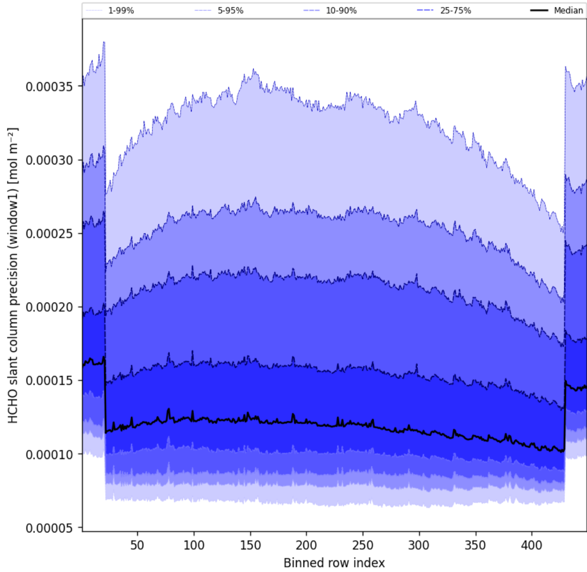
Figure 51: Along track statistics of “HCHO slant column precision (window1)” for 2025-01-05 to 2025-01-05
