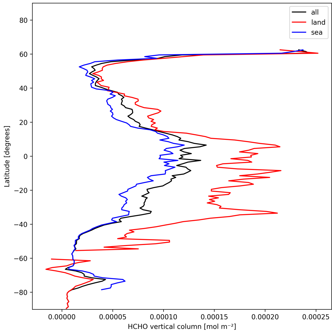
Figure 19: Zonal average of “HCHO vertical column” for 2025-01-05 to 2025-01-05.
