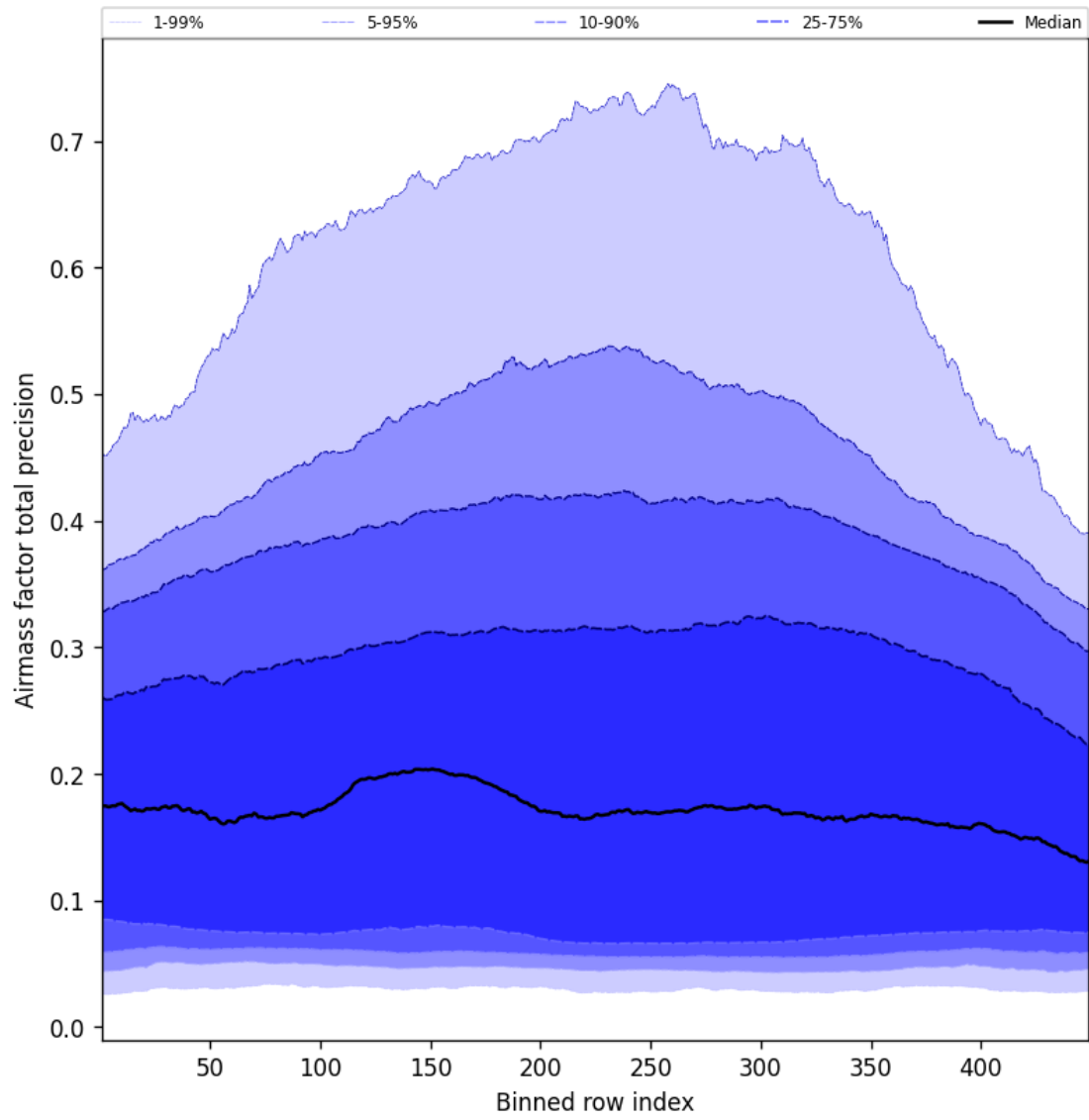
Figure 53: Along track statistics of “Airmass factor total precision” for 2025-01-05 to 2025-01-05
