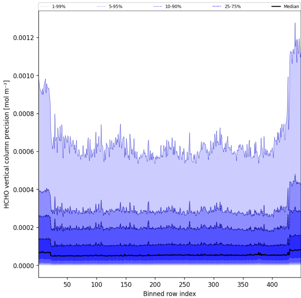
Figure 48: Along track statistics of “HCHO vertical column precision” for 2025-01-05 to 2025-01-05
