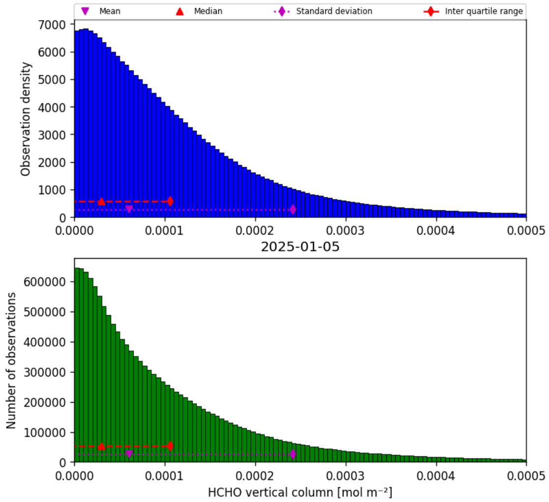
Figure 33: Histogram of “HCHO vertical column” for 2025-01-05 to 2025-01-05
