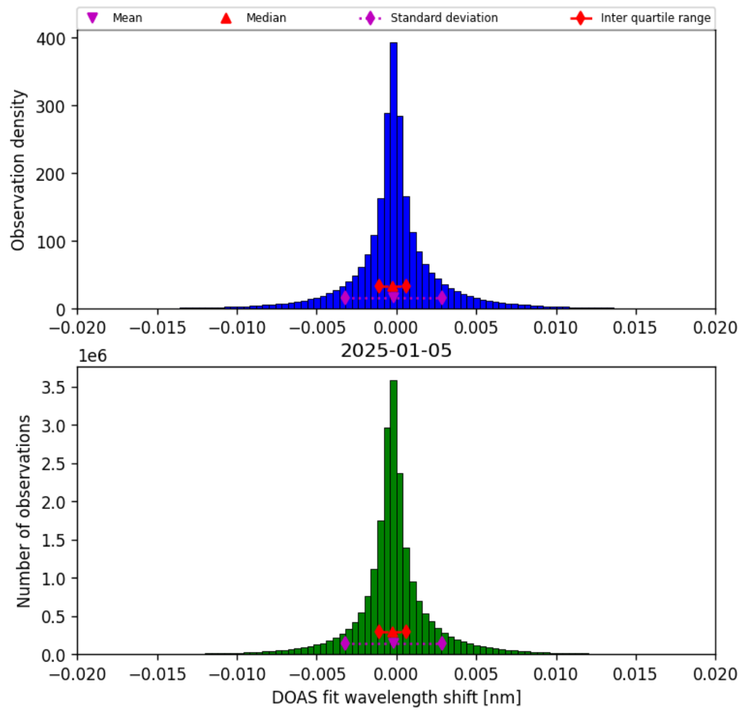
Figure 42: Histogram of “DOAS fit wavelength shift” for 2025-01-05 to 2025-01-05
