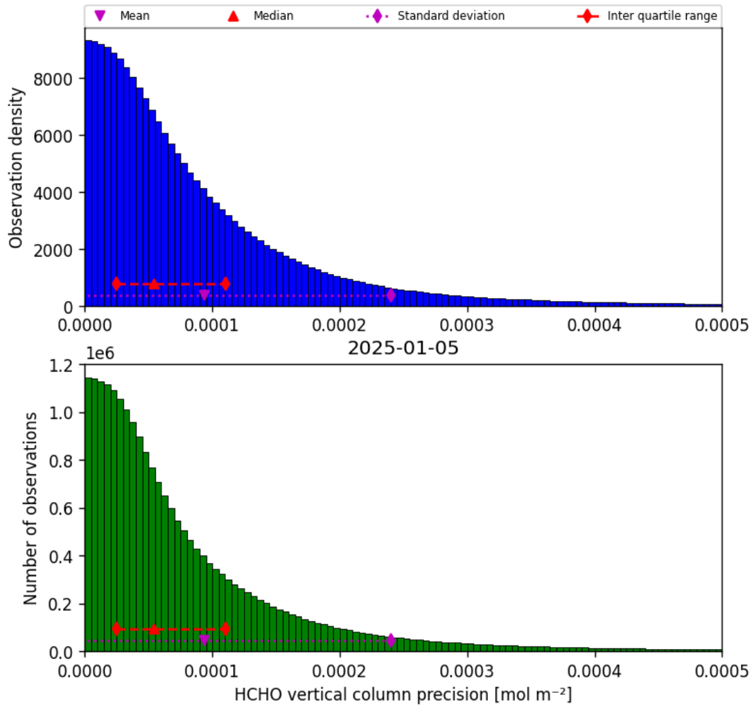
Figure 34: Histogram of “HCHO vertical column precision” for 2025-01-05 to 2025-01-05
