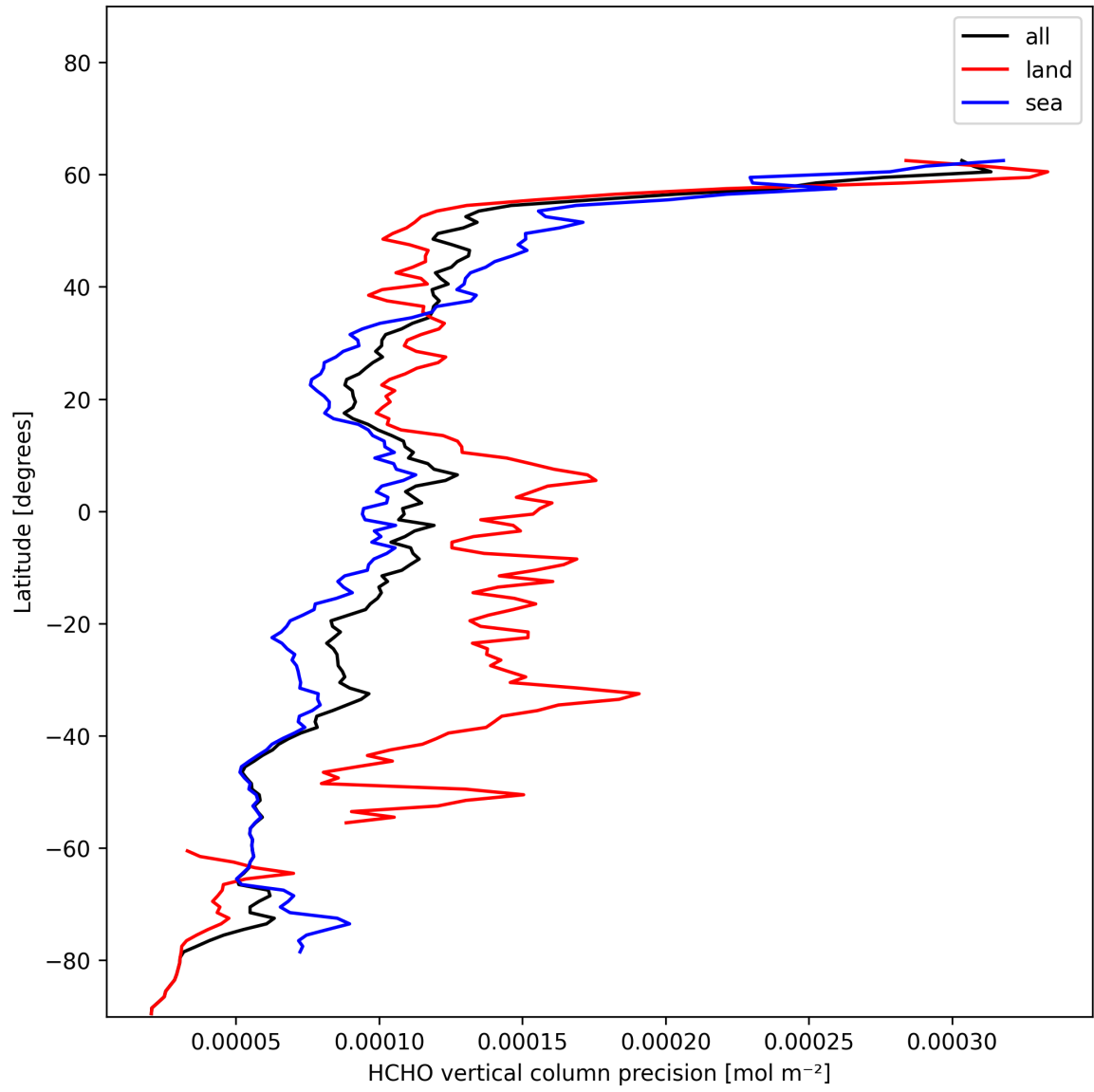
Figure 20: Zonal average of “HCHO vertical column precision” for 2025-01-05 to 2025-01-05.
