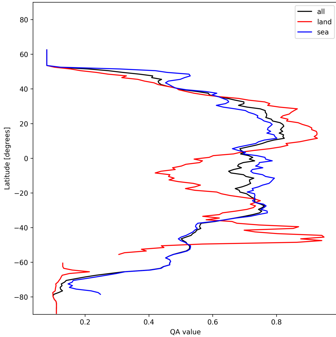
Figure 18: Zonal average of “QA value” for 2025-01-05 to 2025-01-05.
