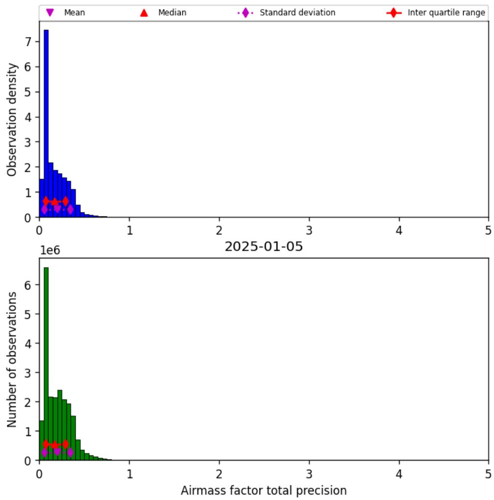
Figure 39: Histogram of “Airmass factor total precision” for 2025-01-05 to 2025-01-05
