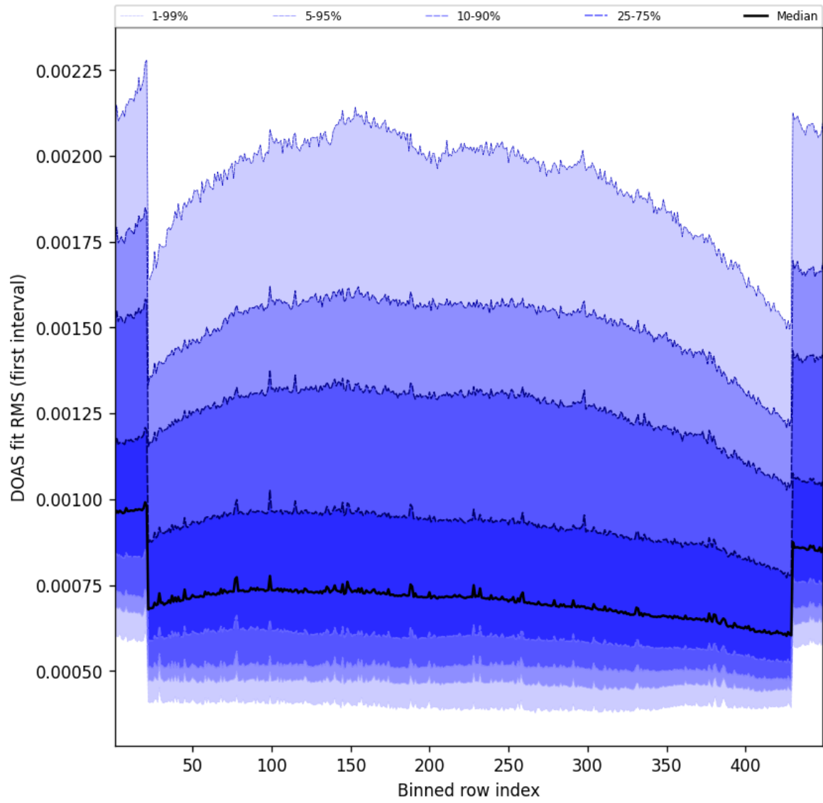
Figure 58: Along track statistics of “DOAS fit RMS (first interval)” for 2025-01-05 to 2025-01-05
