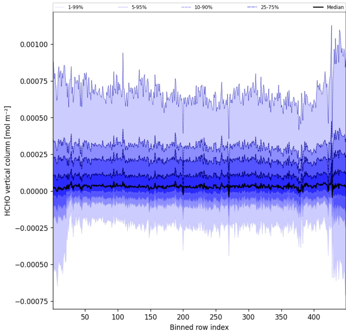
Figure 47: Along track statistics of “HCHO vertical column” for 2025-01-05 to 2025-01-05
