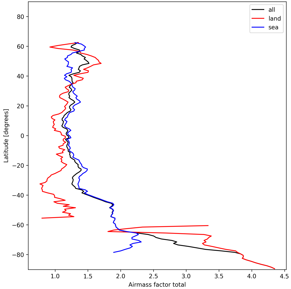
Figure 24: Zonal average of “Airmass factor total” for 2025-01-05 to 2025-01-05.
