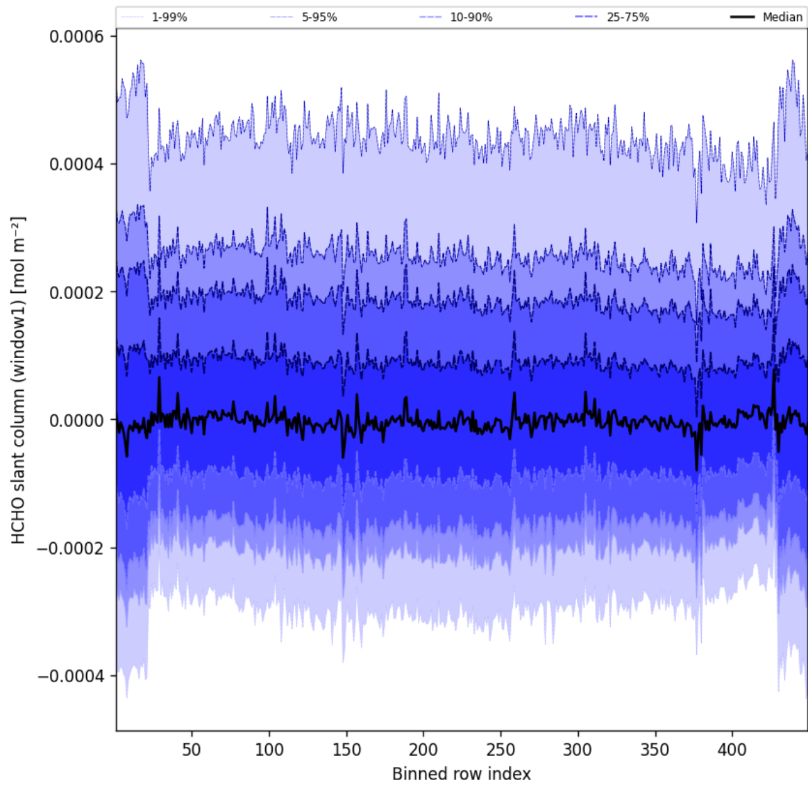
Figure 50: Along track statistics of “HCHO slant column (window1)” for 2025-01-05 to 2025-01-05
