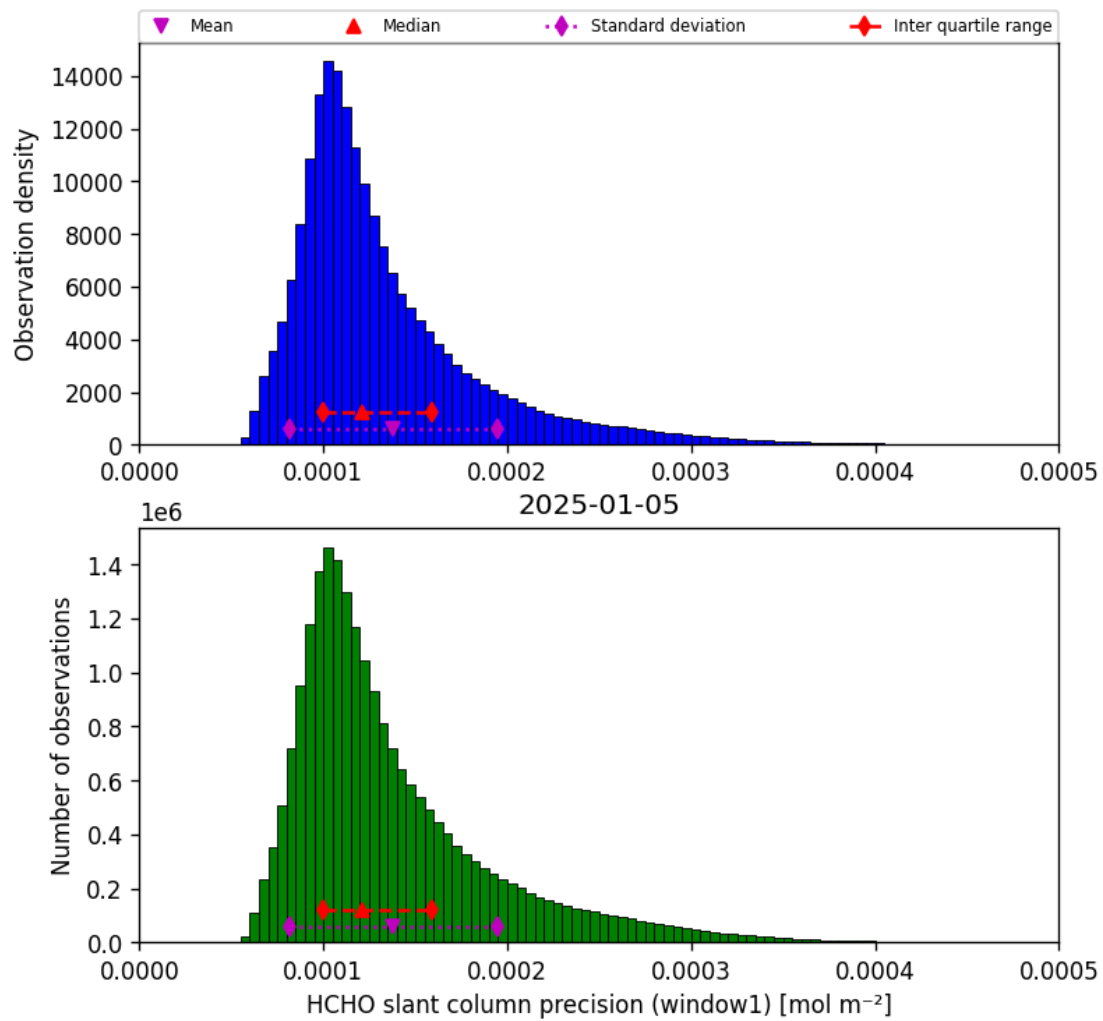
Figure 37: Histogram of “HCHO slant column precision (window1)” for 2025-01-05 to 2025-01-05
