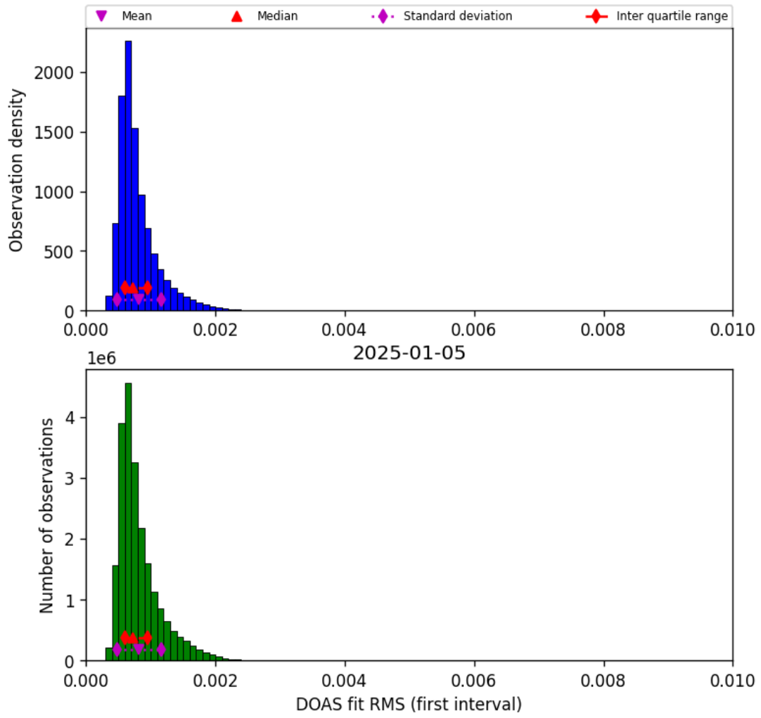
Figure 44: Histogram of “DOAS fit RMS (first interval)” for 2025-01-05 to 2025-01-05
