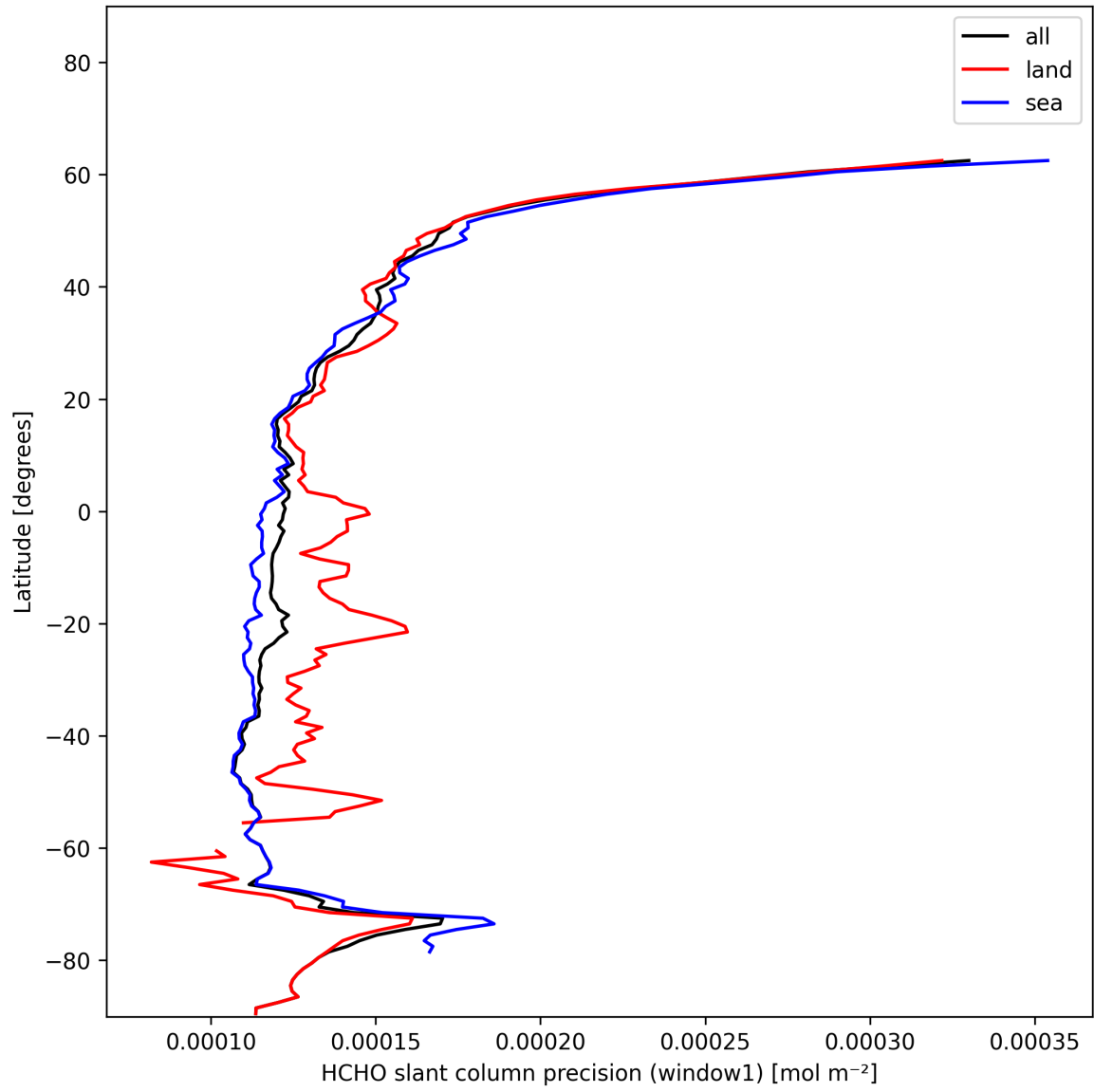
Figure 23: Zonal average of “HCHO slant column precision (window1)” for 2025-01-05 to 2025-01-05.
