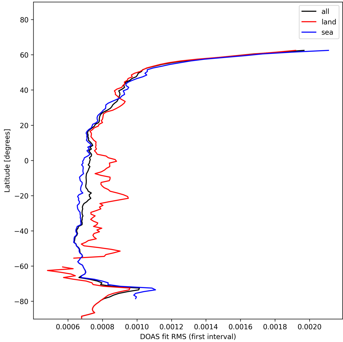
Figure 30: Zonal average of “DOAS fit RMS (first interval)” for 2025-01-05 to 2025-01-05.
