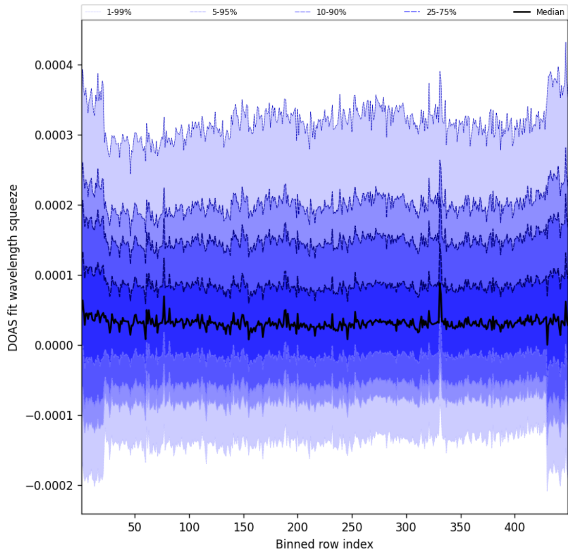
Figure 57: Along track statistics of “DOAS fit wavelength squeeze” for 2025-01-05 to 2025-01-05
