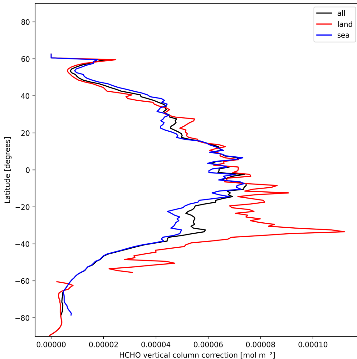
Figure 21: Zonal average of “HCHO vertical column correction” for 2025-01-05 to 2025-01-05.
