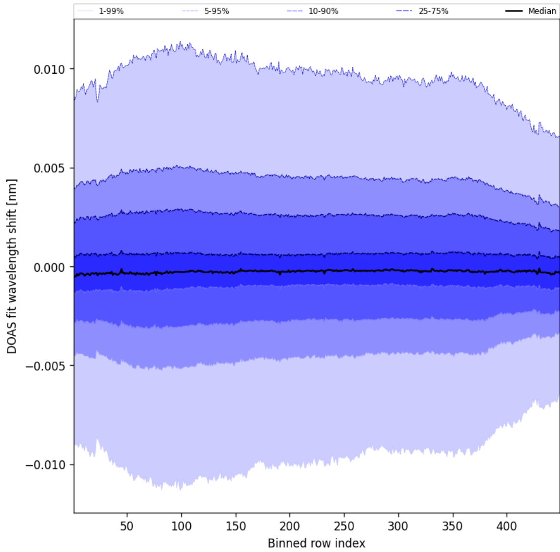
Figure 56: Along track statistics of “DOAS fit wavelength shift” for 2025-01-05 to 2025-01-05
