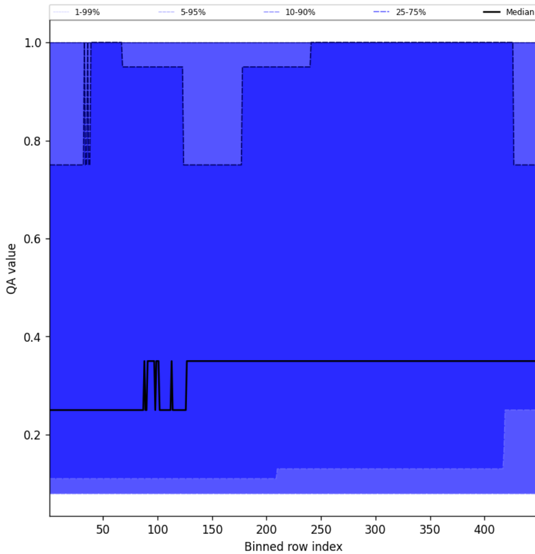
Figure 46: Along track statistics of “QA value” for 2025-01-06 to 2025-01-07
