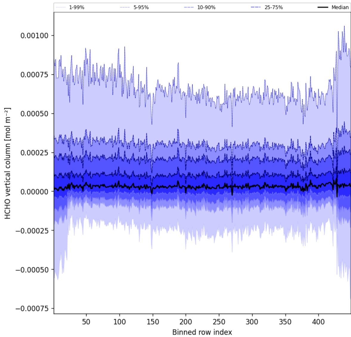
Figure 47: Along track statistics of “HCHO vertical column” for 2025-01-06 to 2025-01-07
