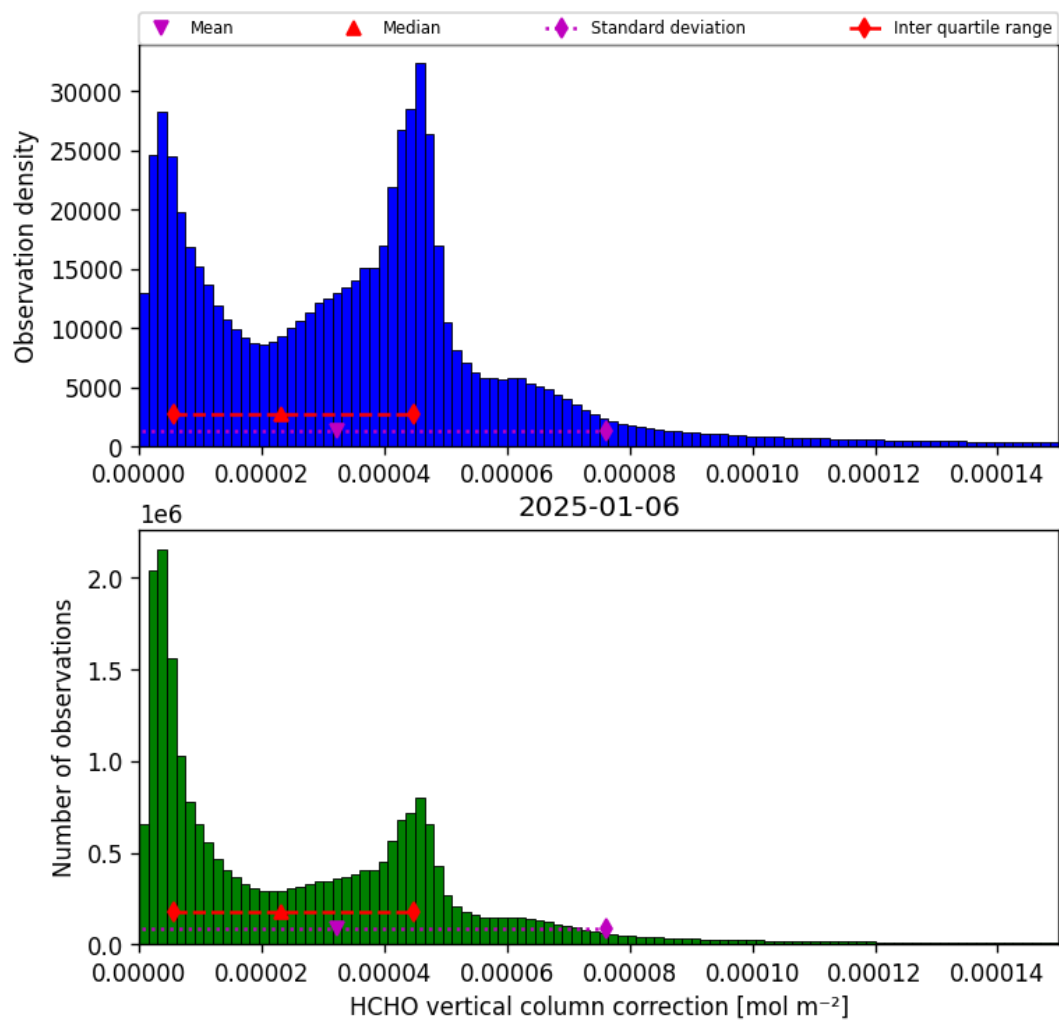
Figure 35: Histogram of “HCHO vertical column correction” for 2025-01-06 to 2025-01-07
