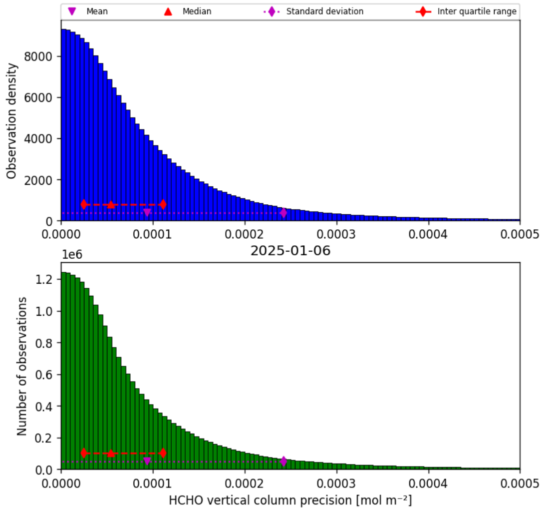
Figure 34: Histogram of “HCHO vertical column precision” for 2025-01-06 to 2025-01-07
