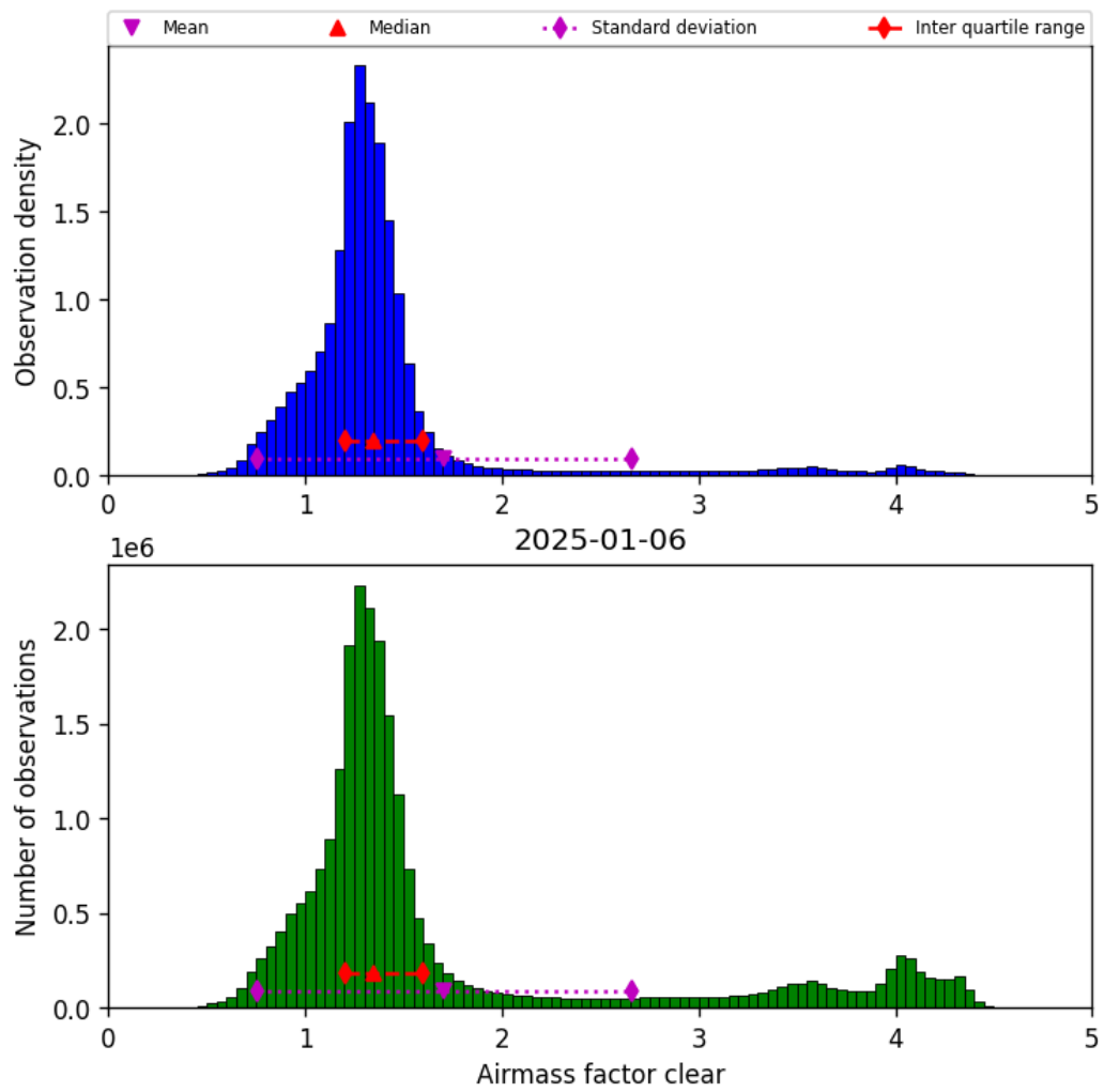
Figure 40: Histogram of “Airmass factor clear” for 2025-01-06 to 2025-01-07
