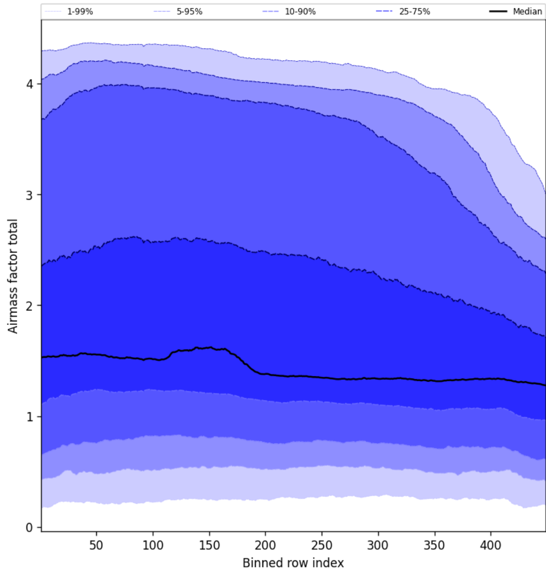
Figure 52: Along track statistics of “Airmass factor total” for 2025-01-06 to 2025-01-07
