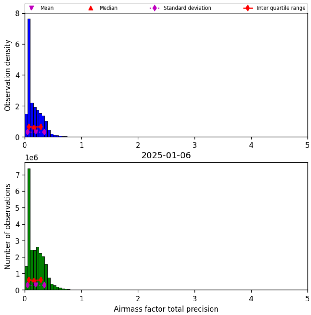
Figure 39: Histogram of “Airmass factor total precision” for 2025-01-06 to 2025-01-07
