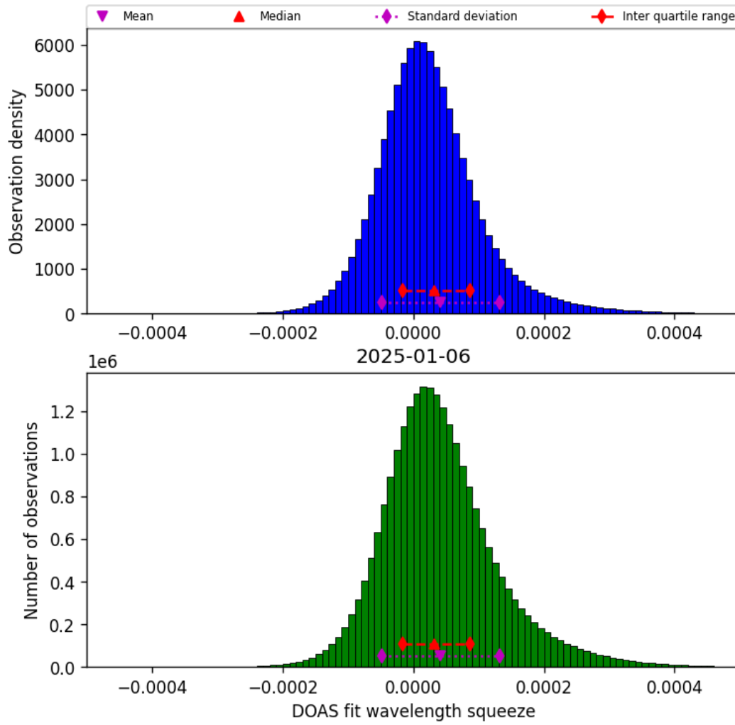
Figure 43: Histogram of “DOAS fit wavelength squeeze” for 2025-01-06 to 2025-01-07
