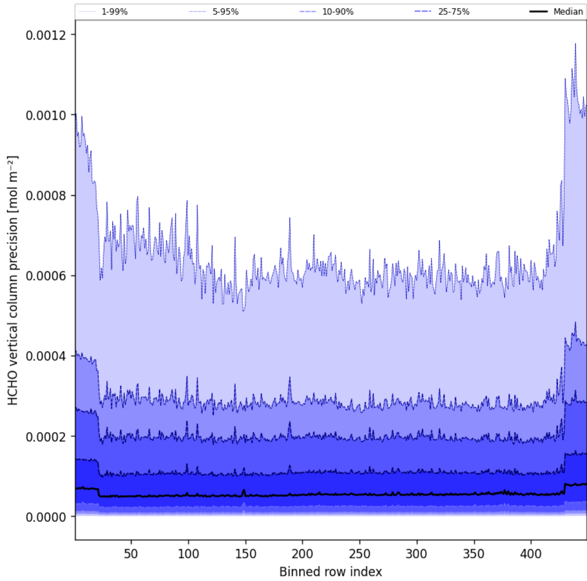
Figure 48: Along track statistics of “HCHO vertical column precision” for 2025-01-06 to 2025-01-07
