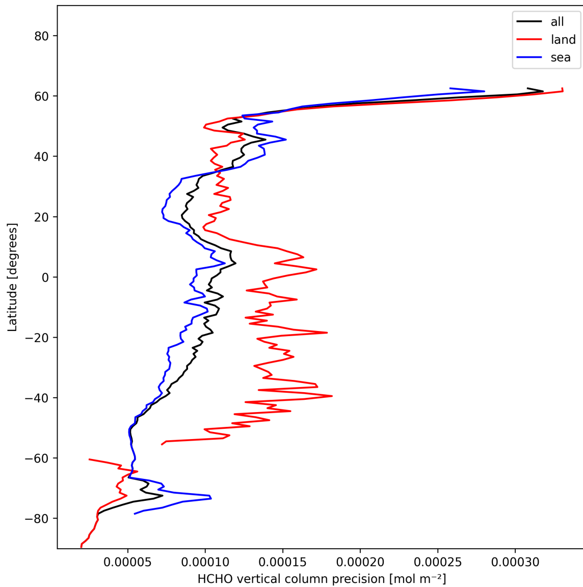
Figure 20: Zonal average of “HCHO vertical column precision” for 2025-01-06 to 2025-01-07.
