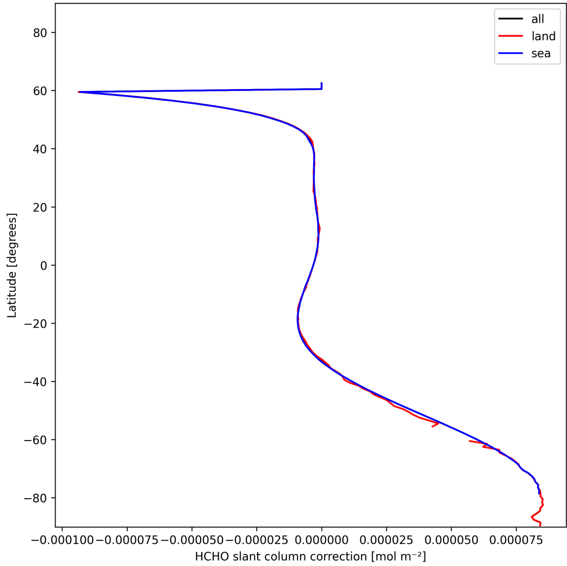
Figure 31: Zonal average of “HCHO slant column correction” for 2025-01-06 to 2025-01-07.
