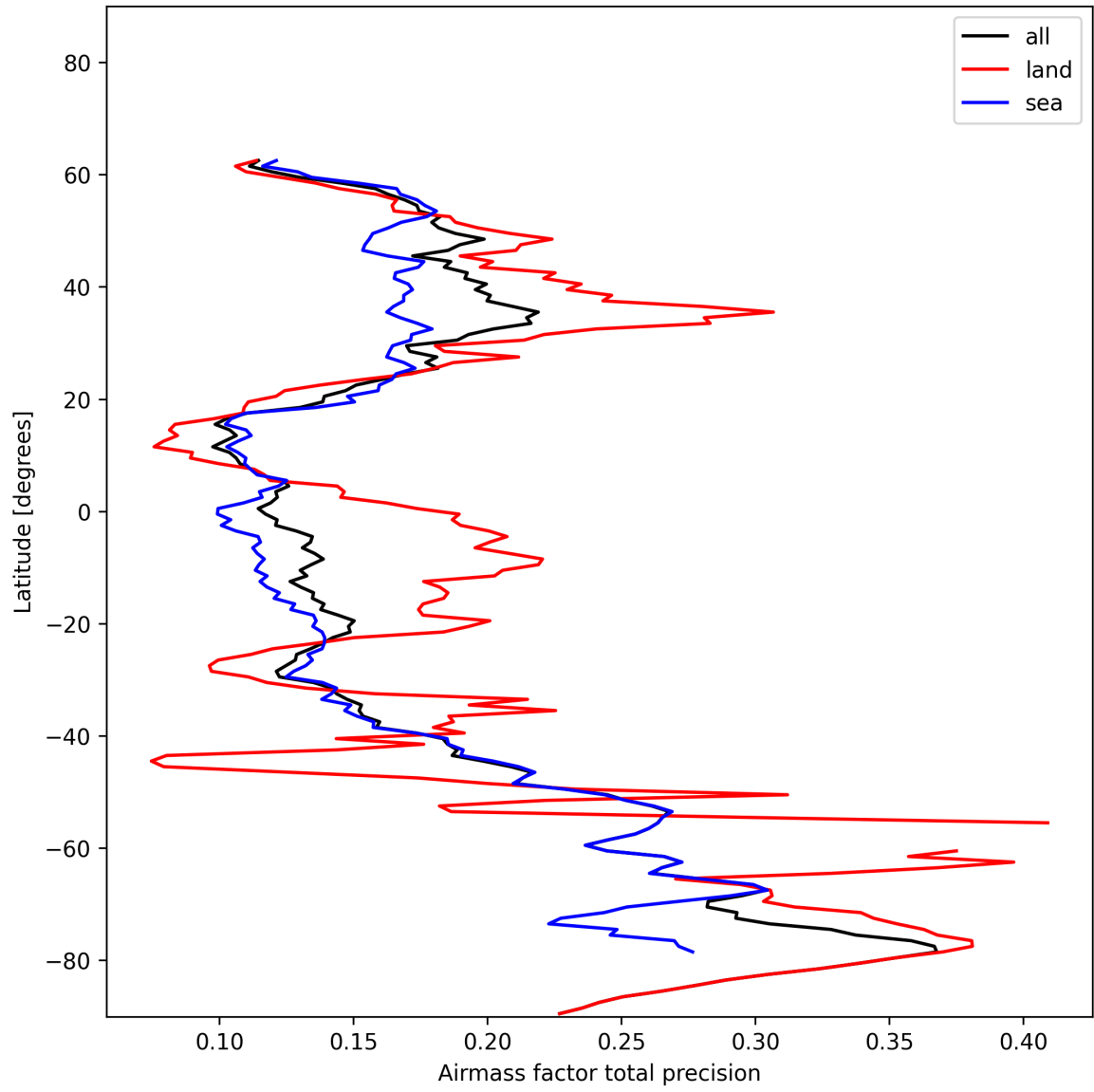
Figure 25: Zonal average of “Airmass factor total precision” for 2025-01-06 to 2025-01-07.
