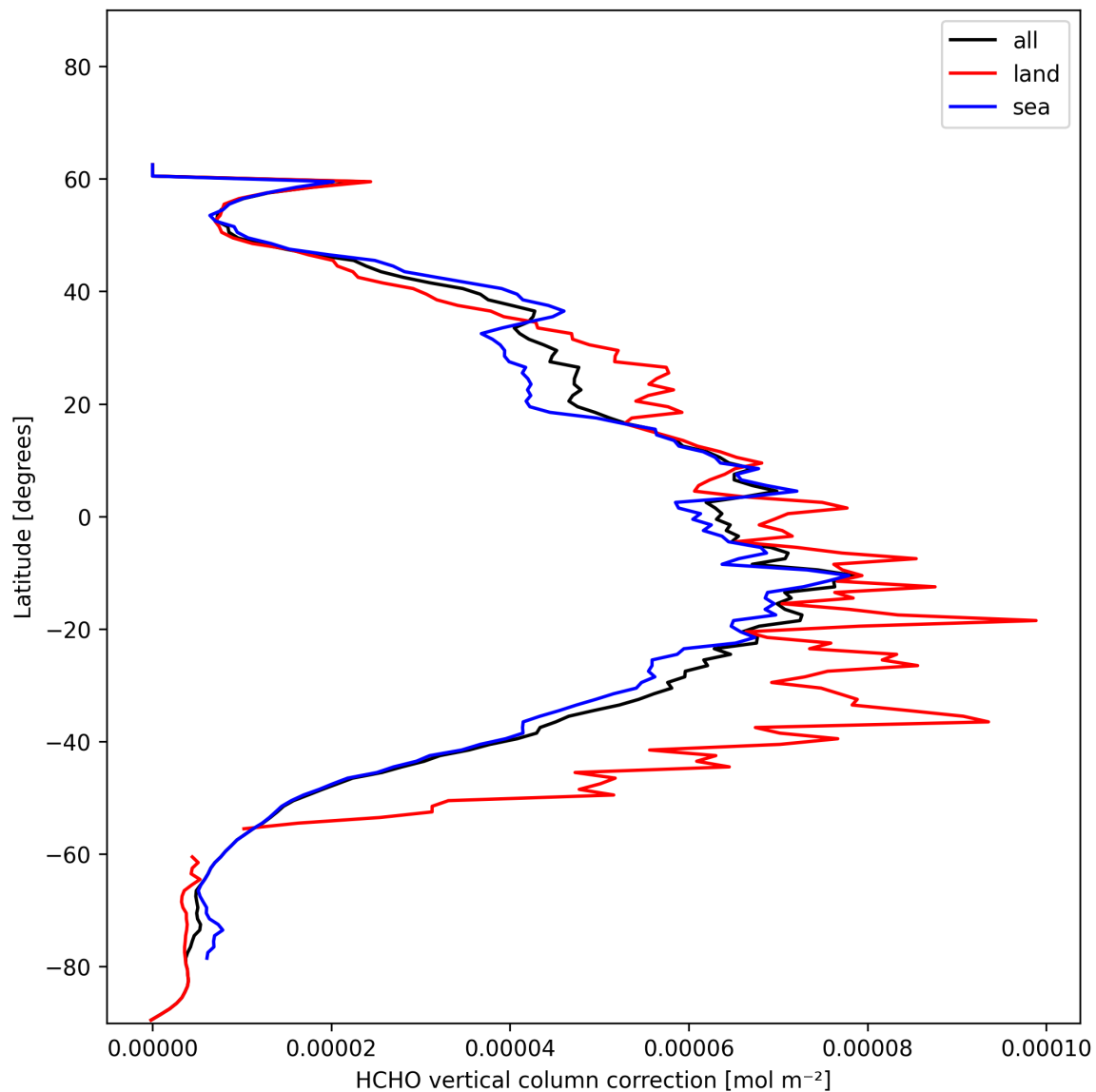
Figure 21: Zonal average of “HCHO vertical column correction” for 2025-01-06 to 2025-01-07.
