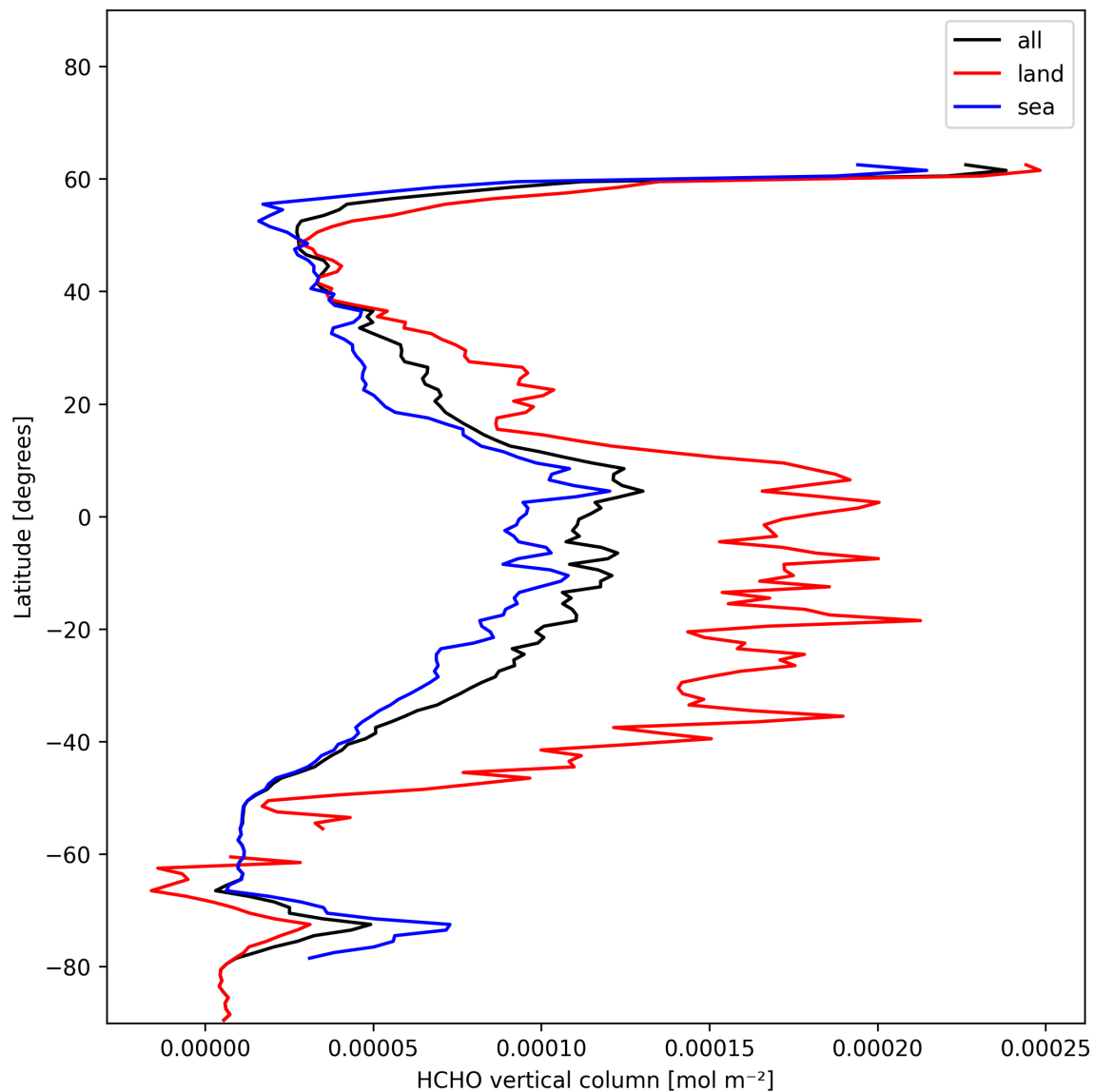
Figure 19: Zonal average of “HCHO vertical column” for 2025-01-06 to 2025-01-07.
