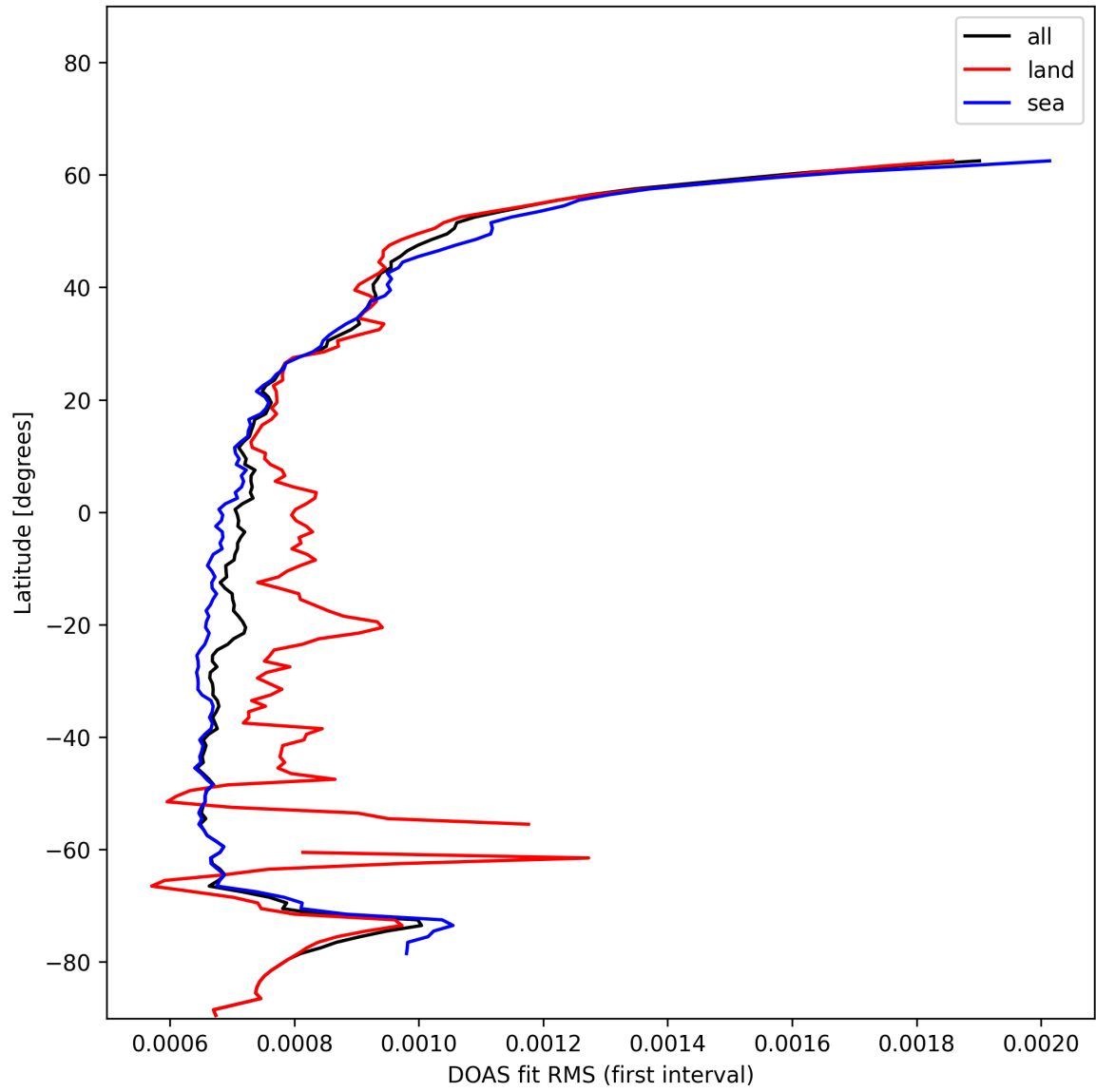
Figure 30: Zonal average of "DOAS fit RMS (first interval)" for 2025-01-06 to 2025-01-07.
