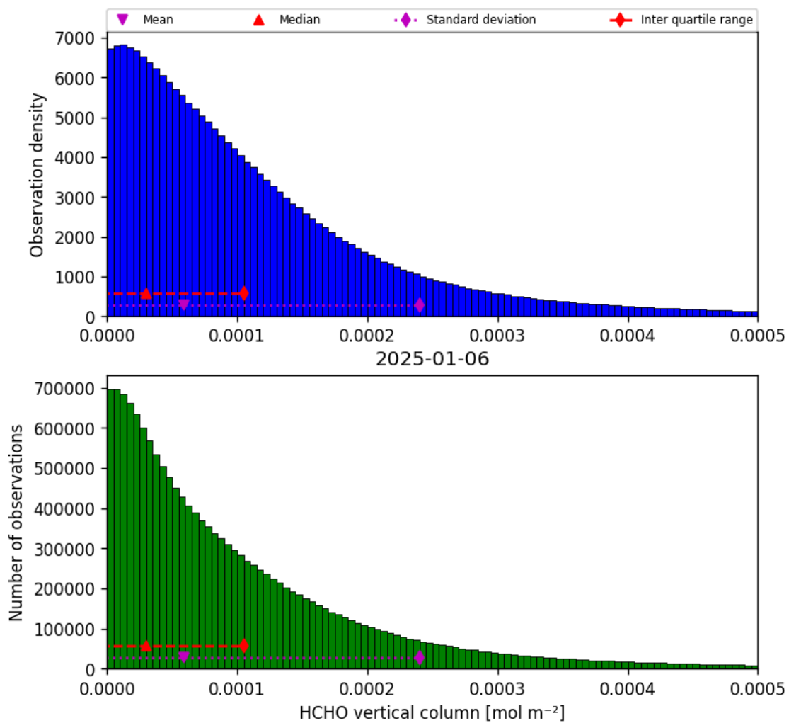
Figure 33: Histogram of “HCHO vertical column” for 2025-01-06 to 2025-01-07
