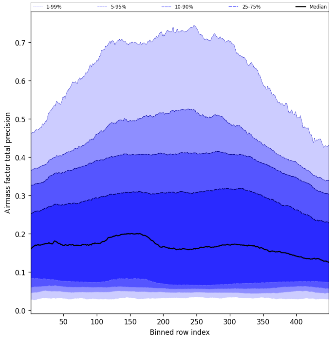
Figure 53: Along track statistics of “Airmass factor total precision” for 2025-01-06 to 2025-01-07
