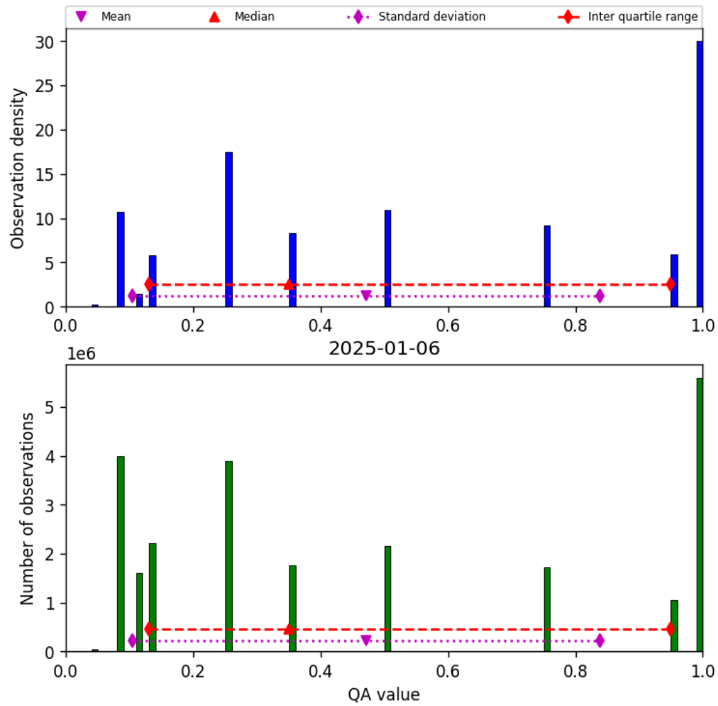
Figure 32: Histogram of “QA value” for 2025-01-06 to 2025-01-07
