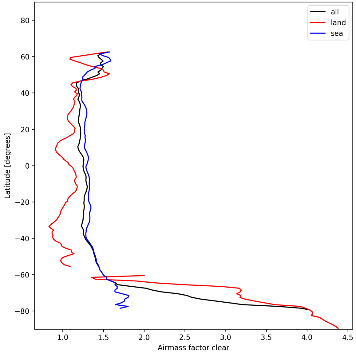
Figure 26: Zonal average of “Airmass factor clear” for 2025-01-06 to 2025-01-07.
