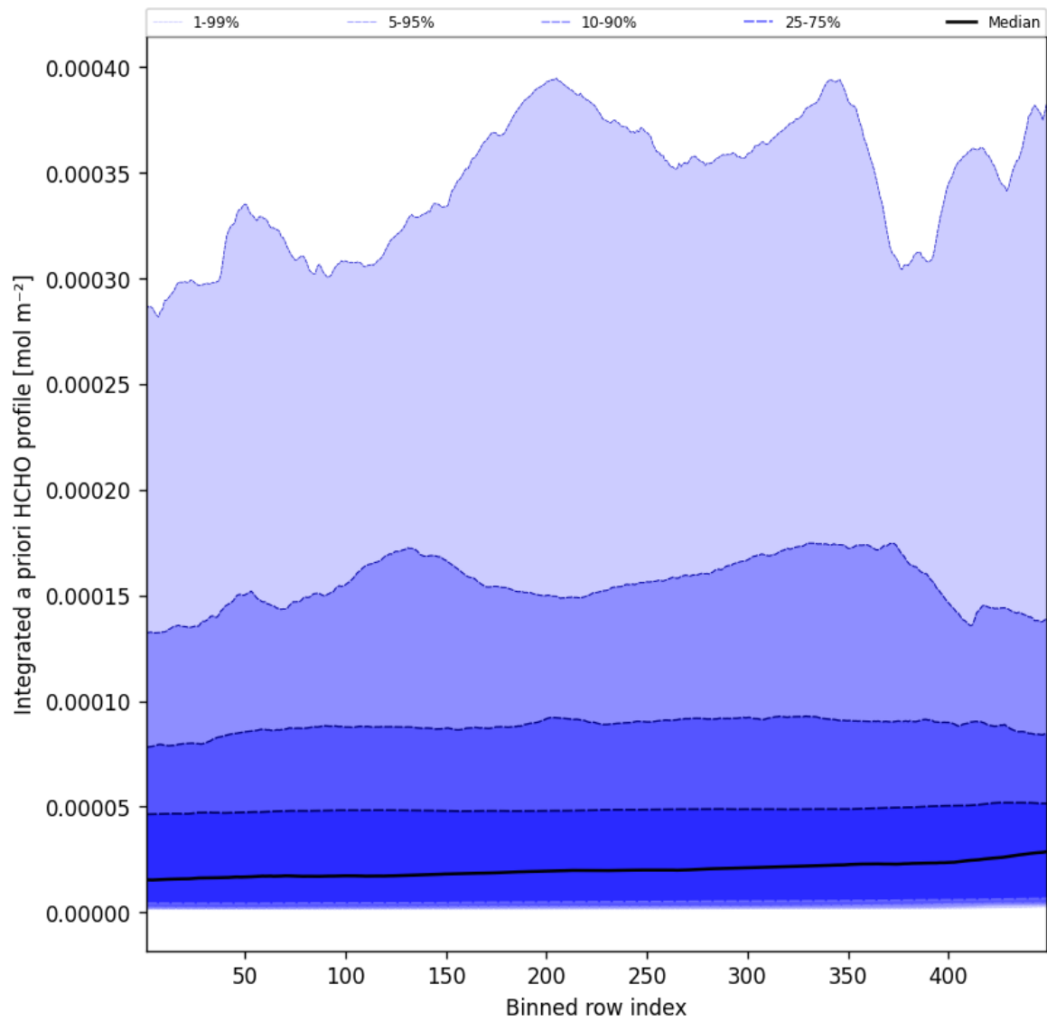
Figure 55: Along track statistics of “Integrated a priori HCHO profile” for 2025-01-06 to 2025-01-07
