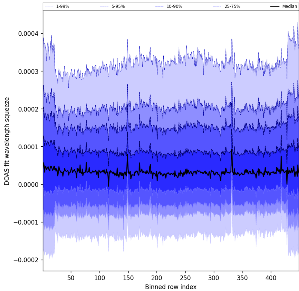
Figure 57: Along track statistics of “DOAS fit wavelength squeeze” for 2025-01-06 to 2025-01-07
