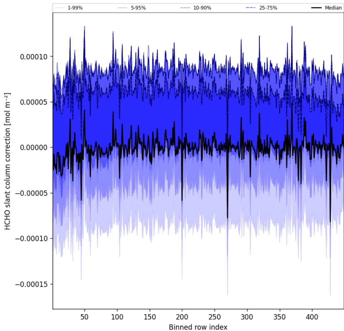
Figure 59: Along track statistics of “HCHO slant column correction” for 2025-01-06 to 2025-01-07
