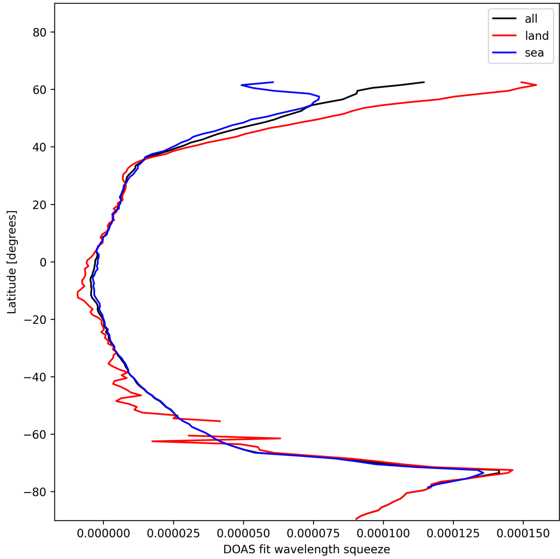
Figure 29: Zonal average of “DOAS fit wavelength squeeze” for 2025-01-06 to 2025-01-07.
