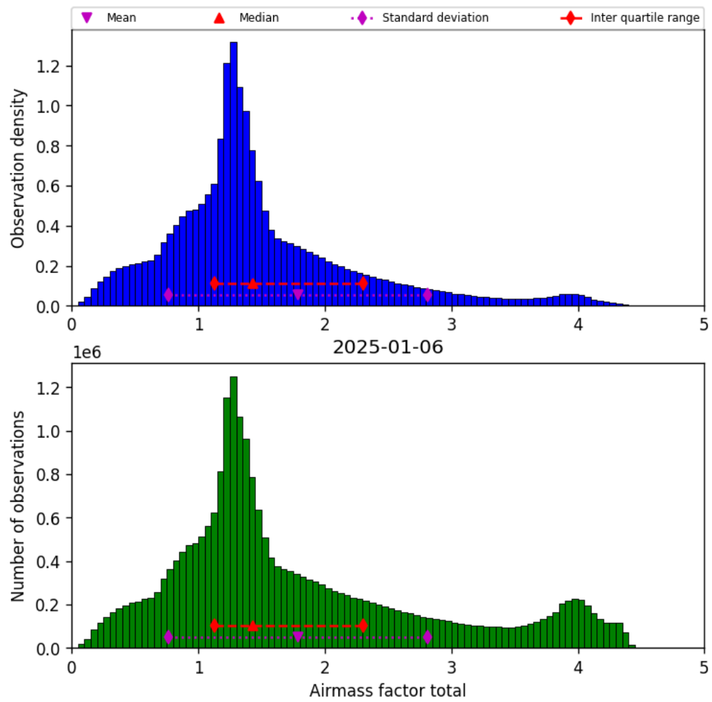
Figure 38: Histogram of “Airmass factor total” for 2025-01-06 to 2025-01-07
