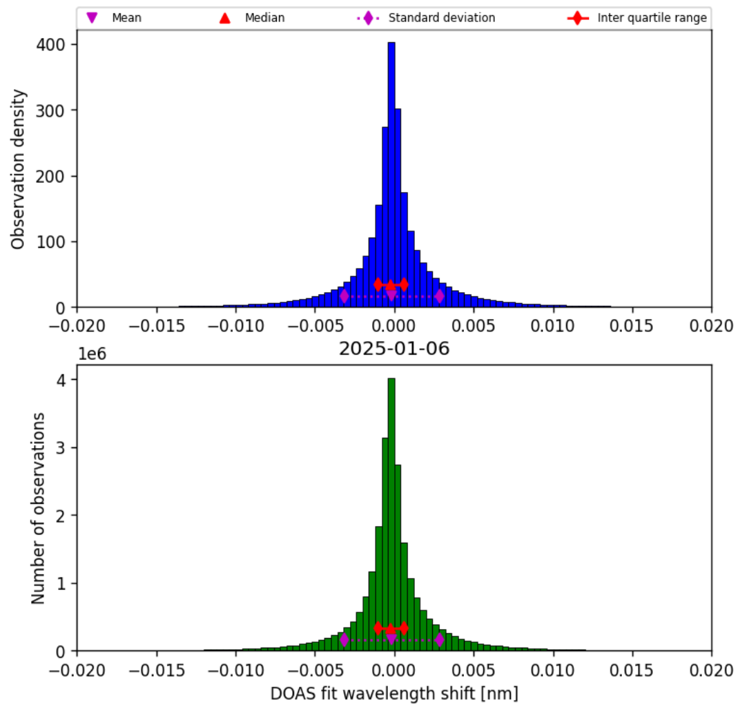
Figure 42: Histogram of “DOAS fit wavelength shift” for 2025-01-06 to 2025-01-07
