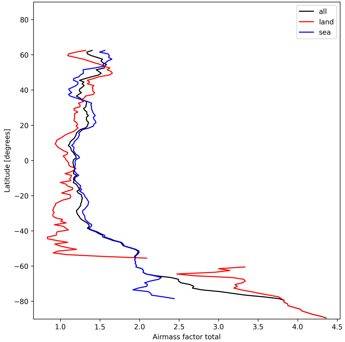
Figure 24: Zonal average of “Airmass factor total” for 2025-01-06 to 2025-01-07.
