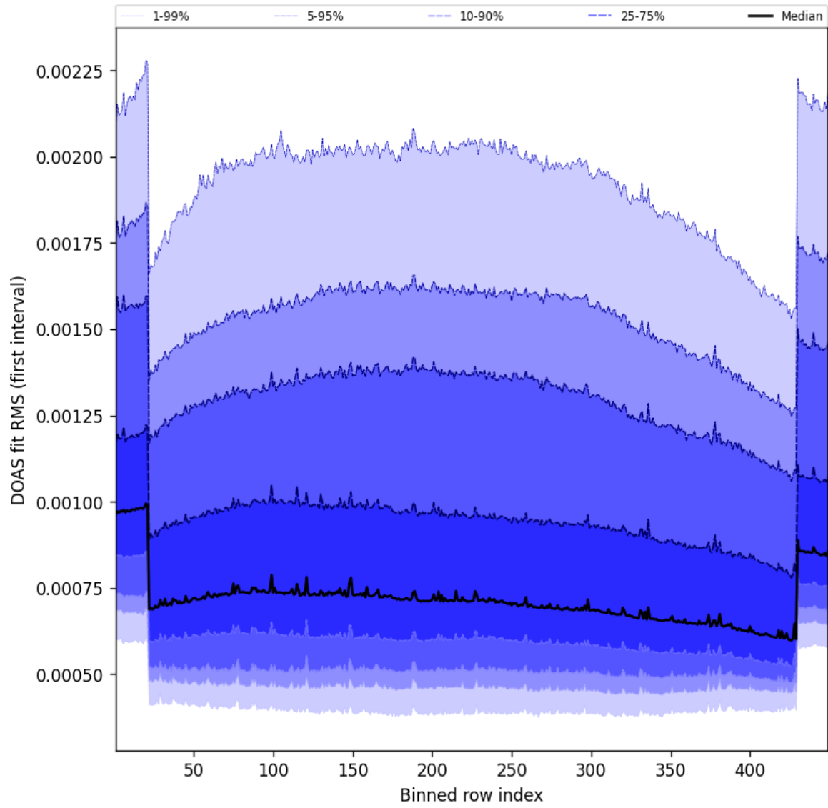
Figure 58: Along track statistics of “DOAS fit RMS (first interval)” for 2025-01-06 to 2025-01-07
