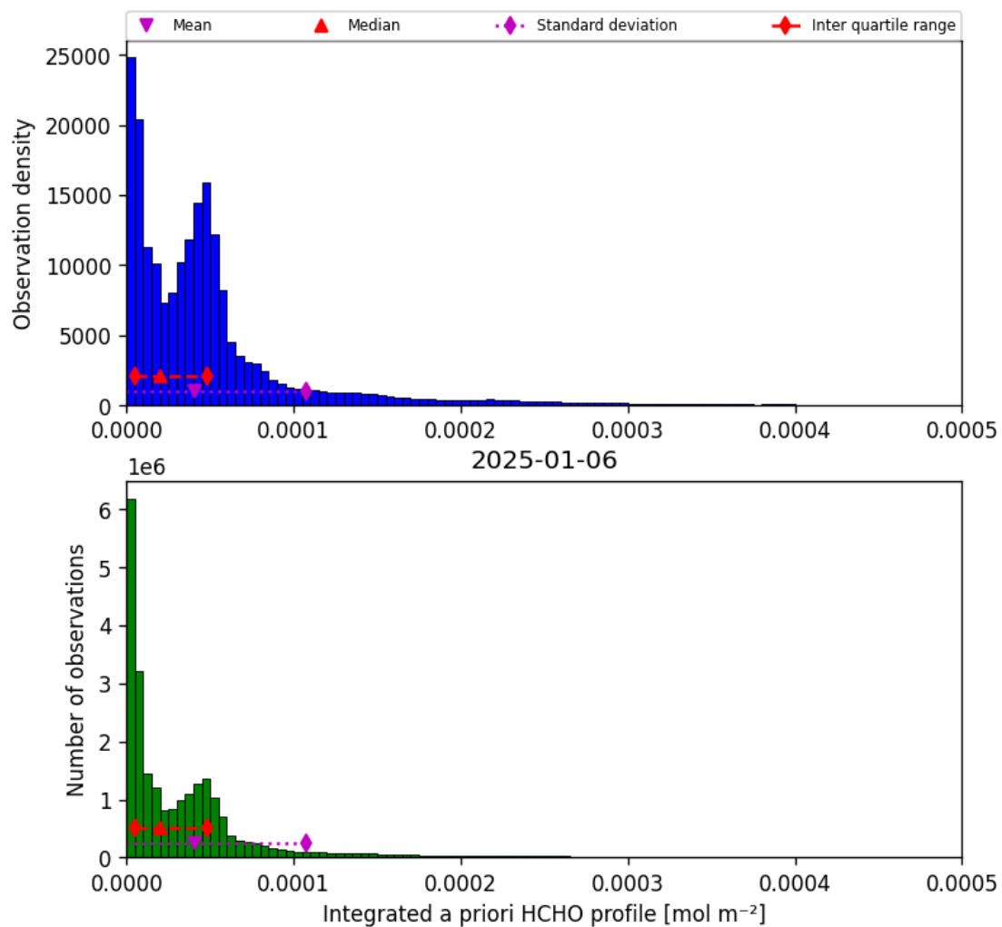
Figure 41: Histogram of “Integrated a priori HCHO profile” for 2025-01-06 to 2025-01-07
