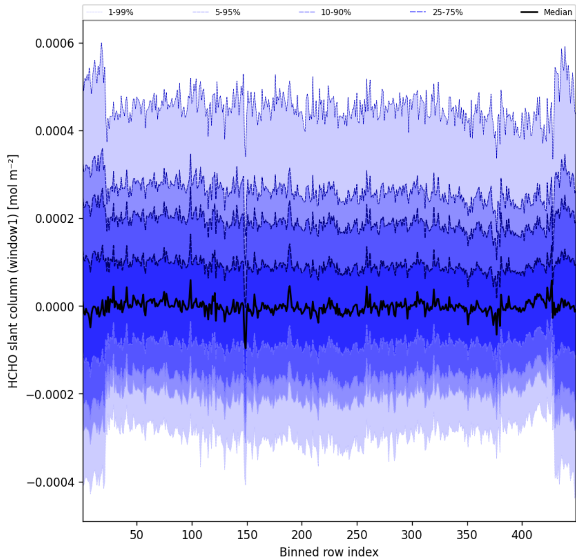
Figure 50: Along track statistics of “HCHO slant column (window1)” for 2025-01-06 to 2025-01-07
