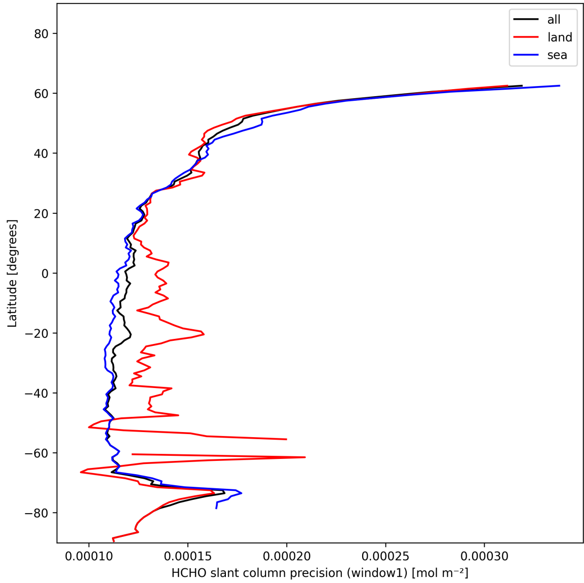
Figure 23: Zonal average of “HCHO slant column precision (window1)” for 2025-01-06 to 2025-01-07.
