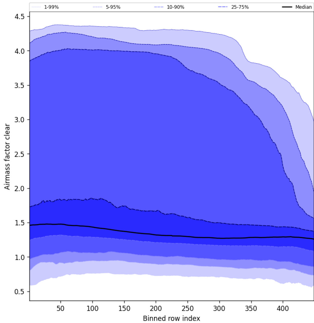
Figure 54: Along track statistics of “Airmass factor clear” for 2025-01-06 to 2025-01-07
