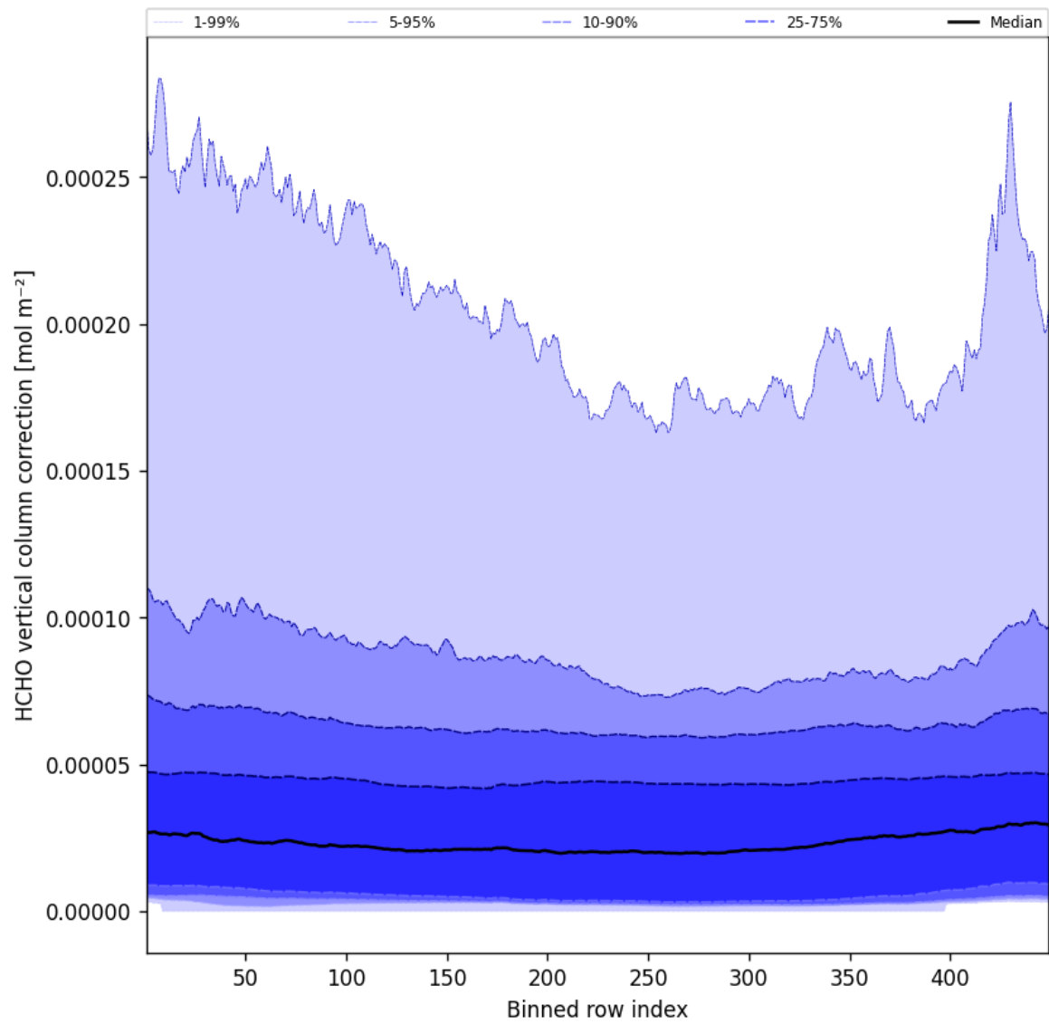
Figure 49: Along track statistics of “HCHO vertical column correction” for 2025-01-06 to 2025-01-07
