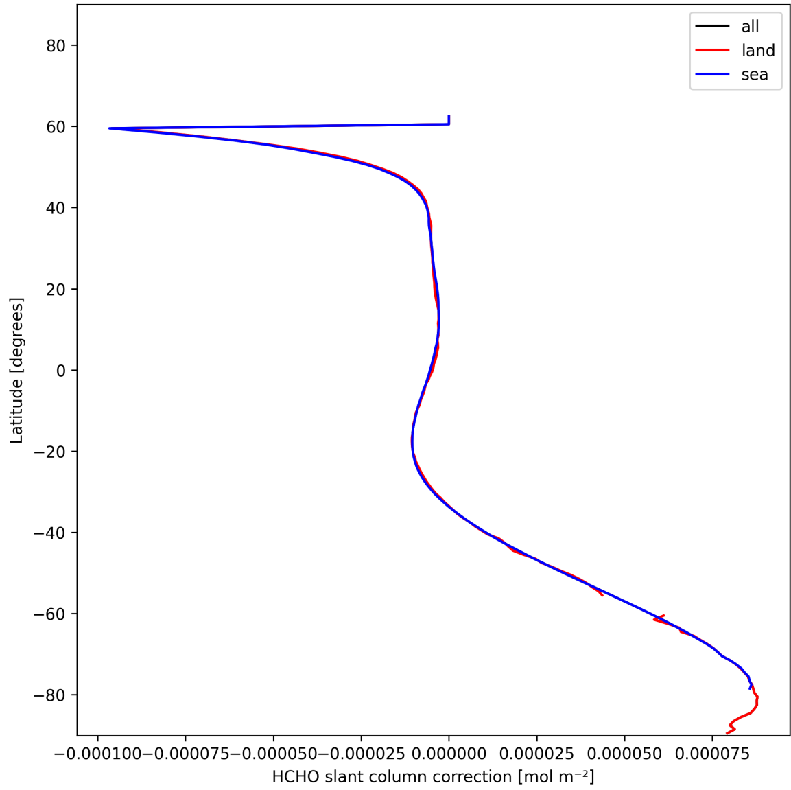
Figure 31: Zonal average of "HCHO slant column correction" for 2025-01-07 to 2025-01-08.
