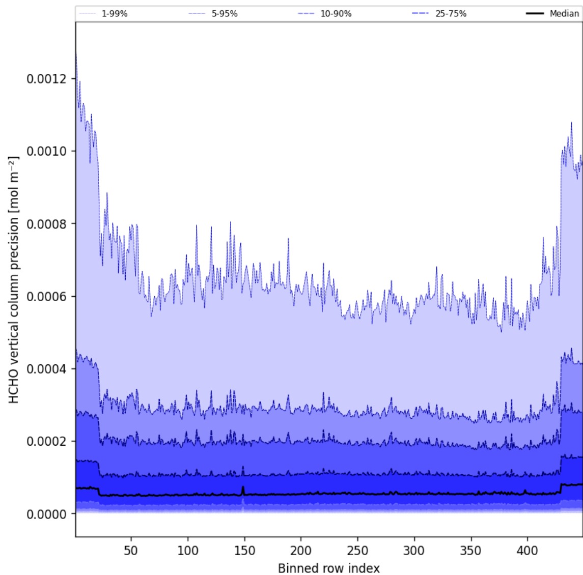
Figure 48: Along track statistics of “HCHO vertical column precision” for 2025-01-07 to 2025-01-08
