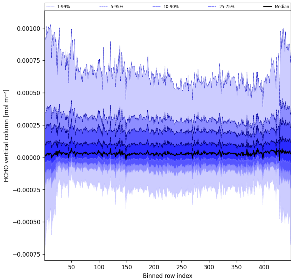
Figure 47: Along track statistics of “HCHO vertical column” for 2025-01-07 to 2025-01-08
