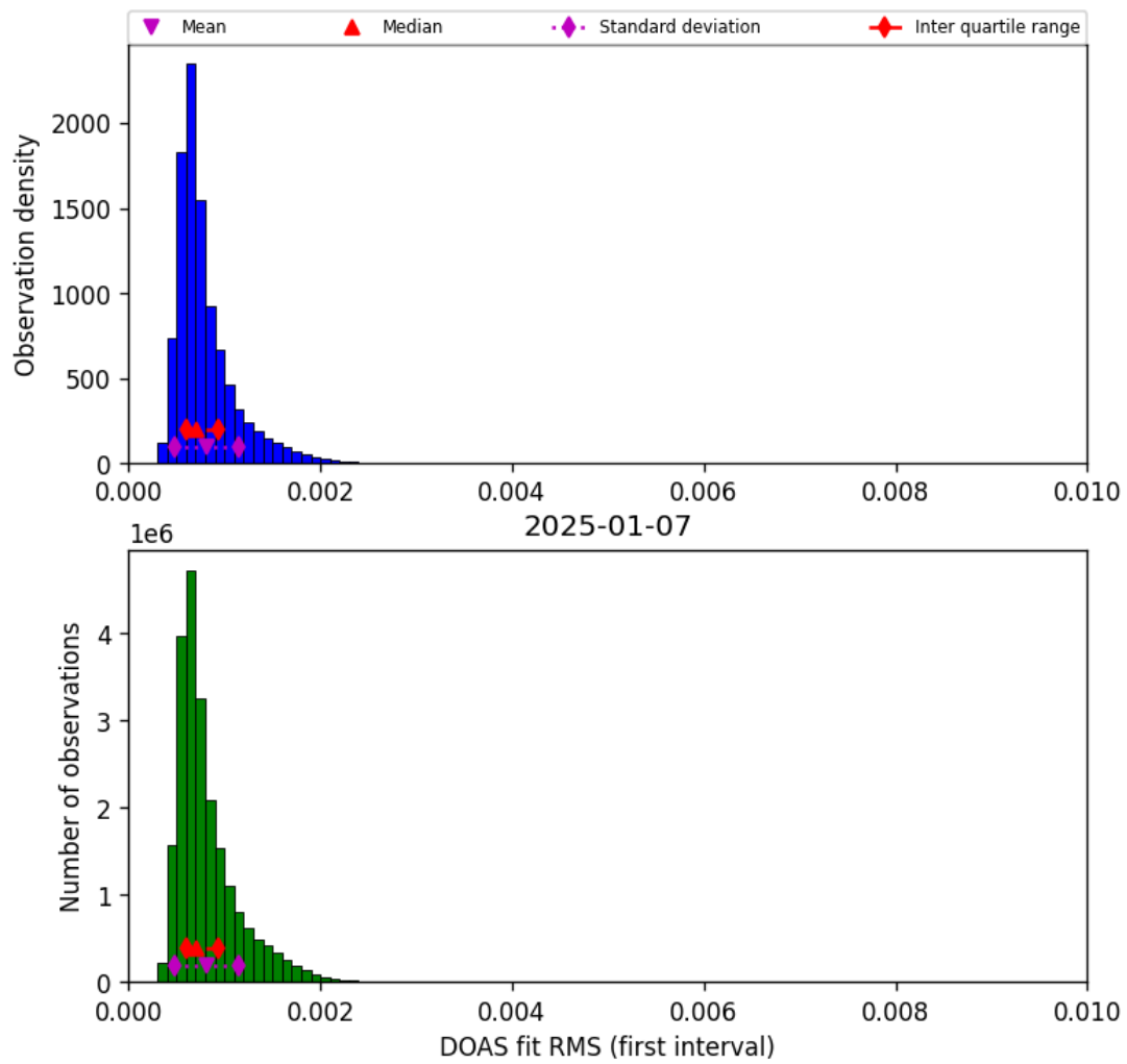
Figure 44: Histogram of “DOAS fit RMS (first interval)” for 2025-01-07 to 2025-01-08
