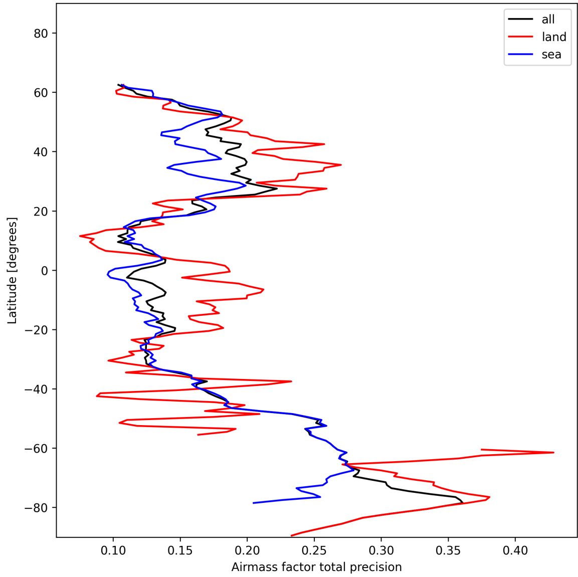
Figure 25: Zonal average of “Airmass factor total precision” for 2025-01-07 to 2025-01-08.
