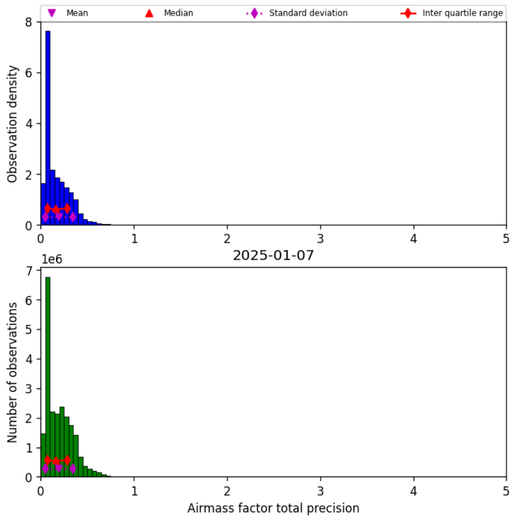
Figure 39: Histogram of “Airmass factor total precision” for 2025-01-07 to 2025-01-08
