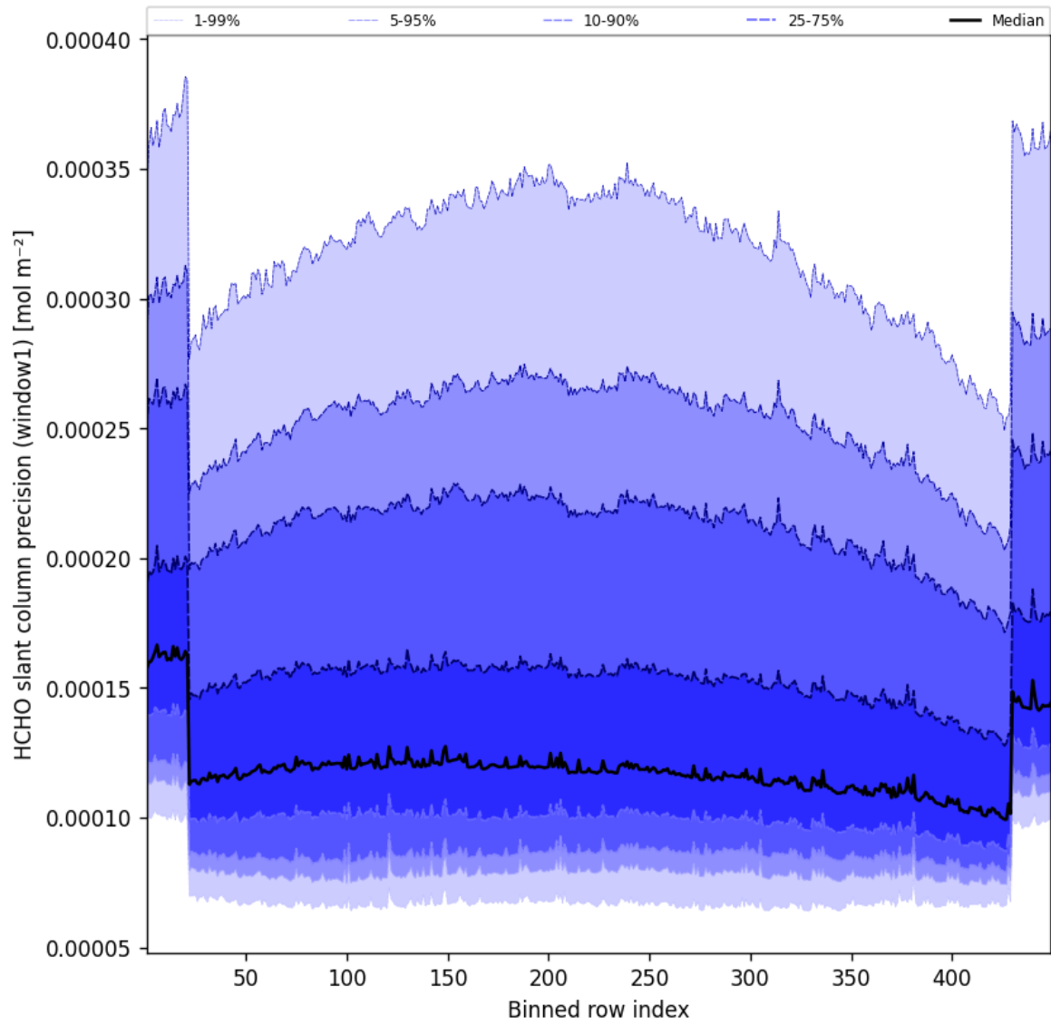
Figure 51: Along track statistics of “HCHO slant column precision (window1)” for 2025-01-07 to 2025-01-08
