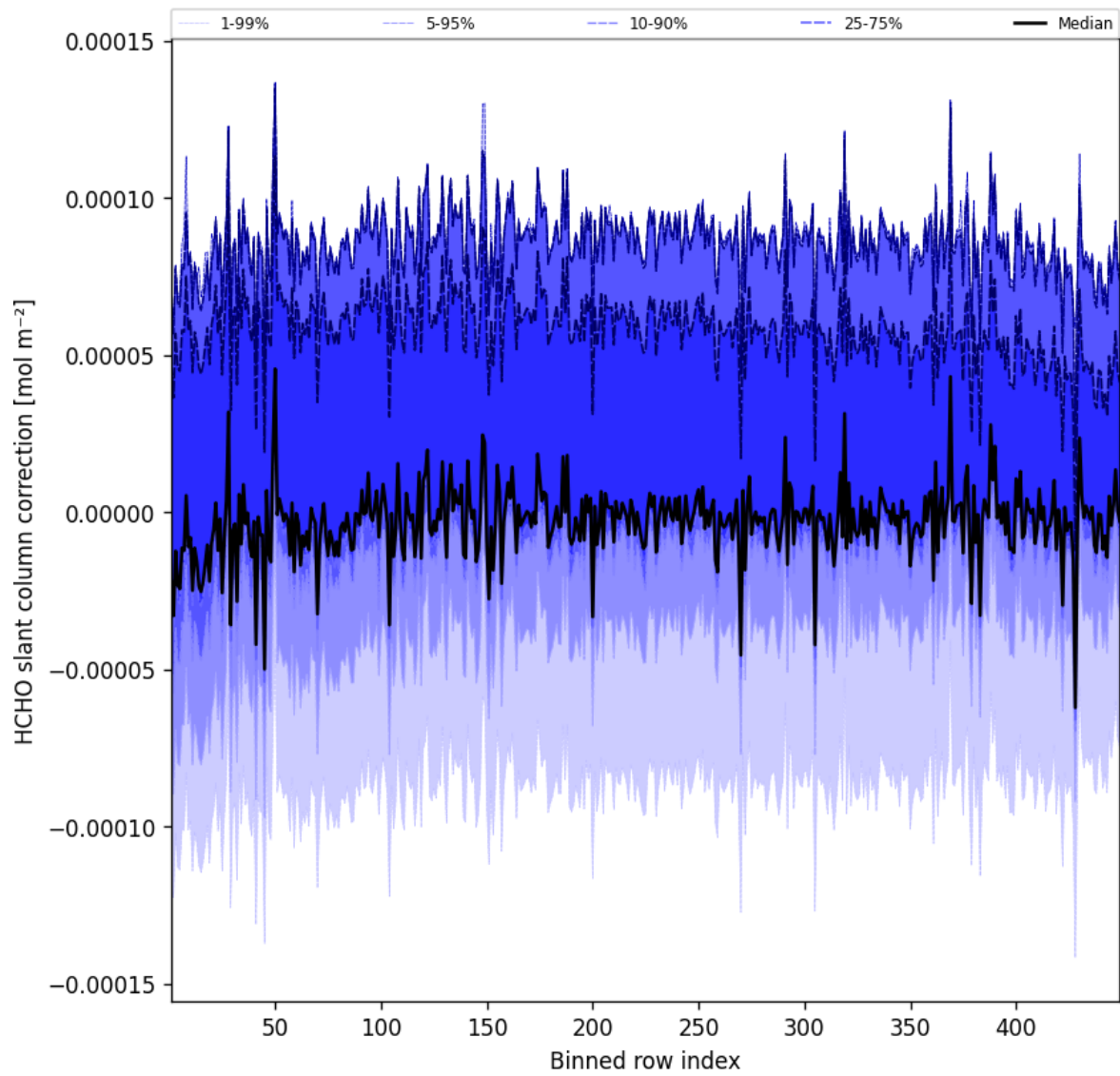
Figure 59: Along track statistics of “HCHO slant column correction” for 2025-01-07 to 2025-01-08
