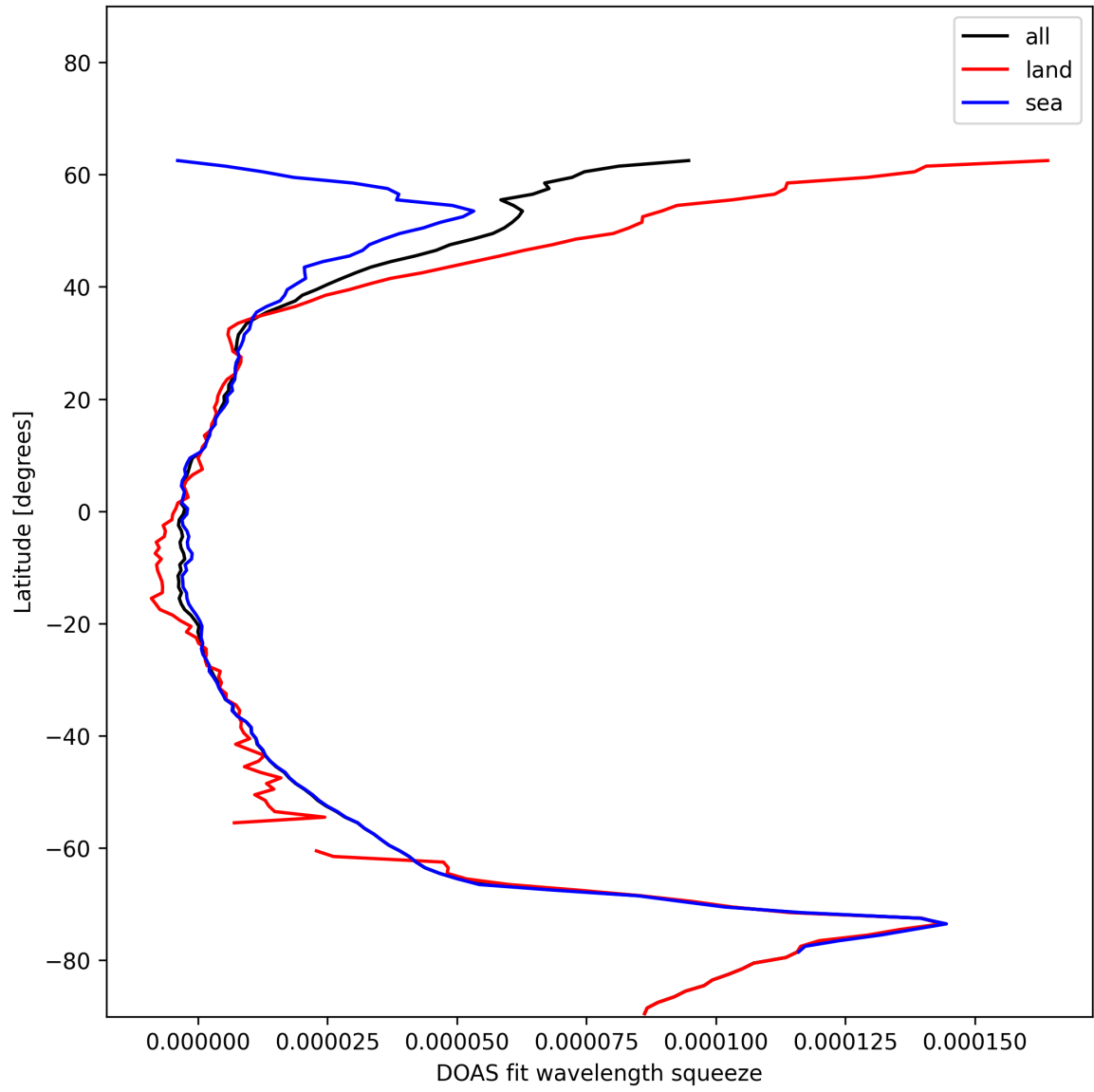
Figure 29: Zonal average of “DOAS fit wavelength squeeze” for 2025-01-07 to 2025-01-08.
