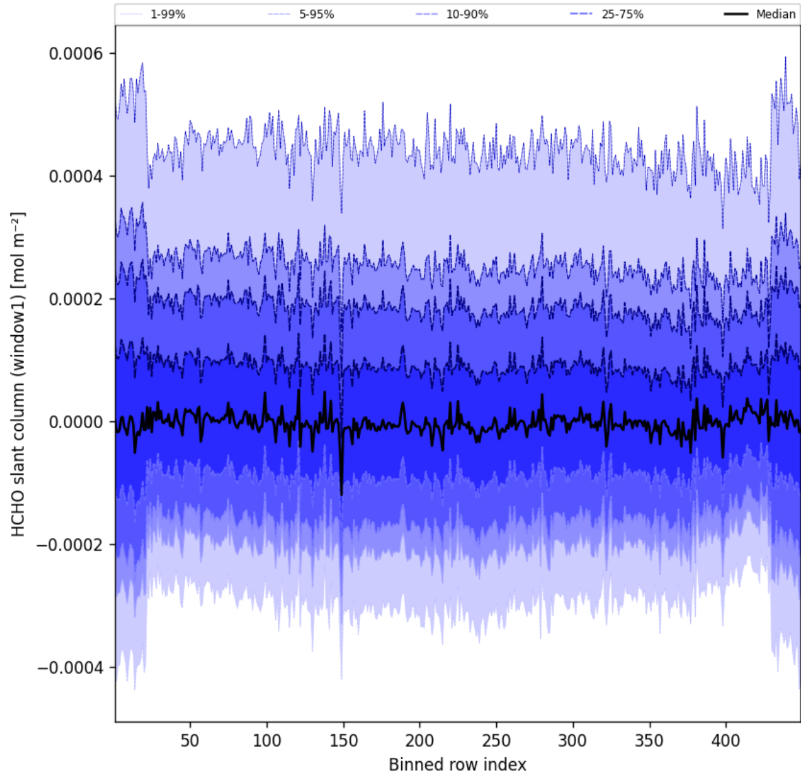
Figure 50: Along track statistics of “HCHO slant column (window1)” for 2025-01-07 to 2025-01-08
