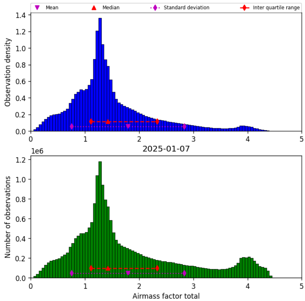
Figure 38: Histogram of “Airmass factor total” for 2025-01-07 to 2025-01-08
