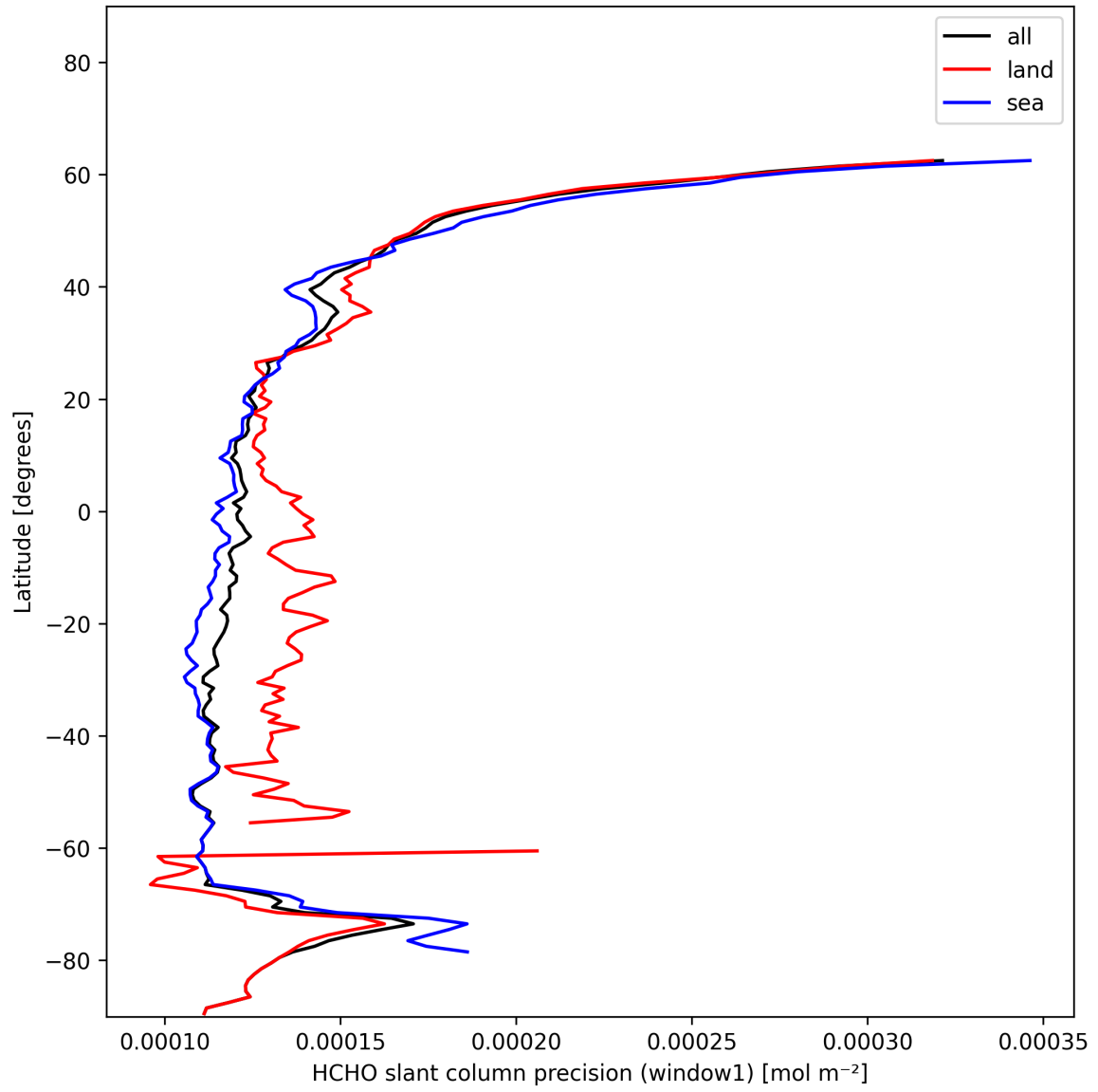
Figure 23: Zonal average of “HCHO slant column precision (window1)” for 2025-01-07 to 2025-01-08.
