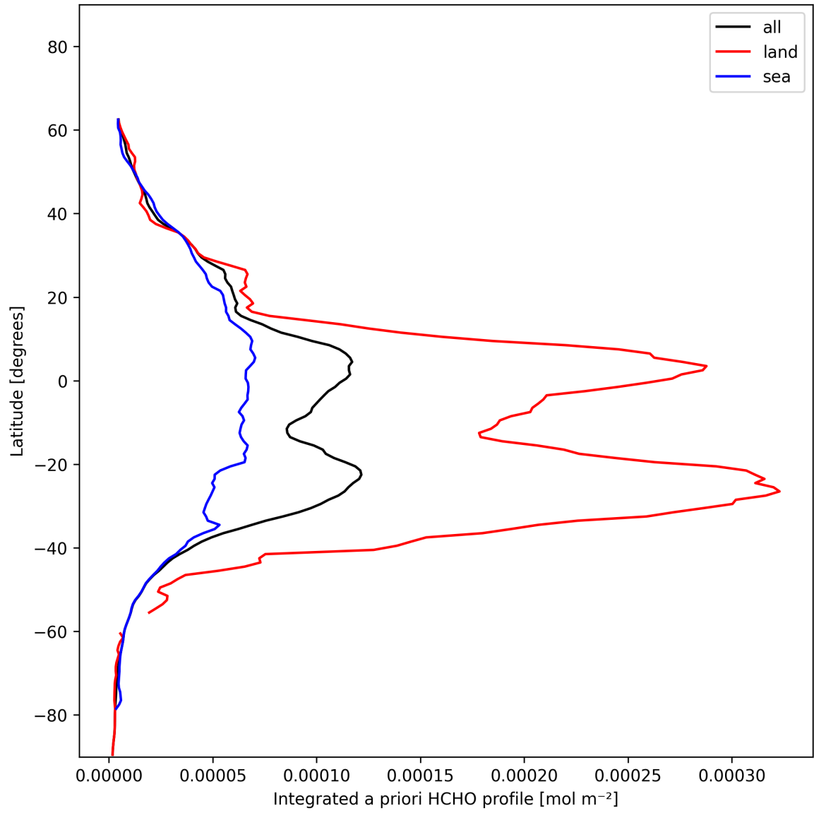
Figure 27: Zonal average of “Integrated a priori HCHO profile” for 2025-01-07 to 2025-01-08.
