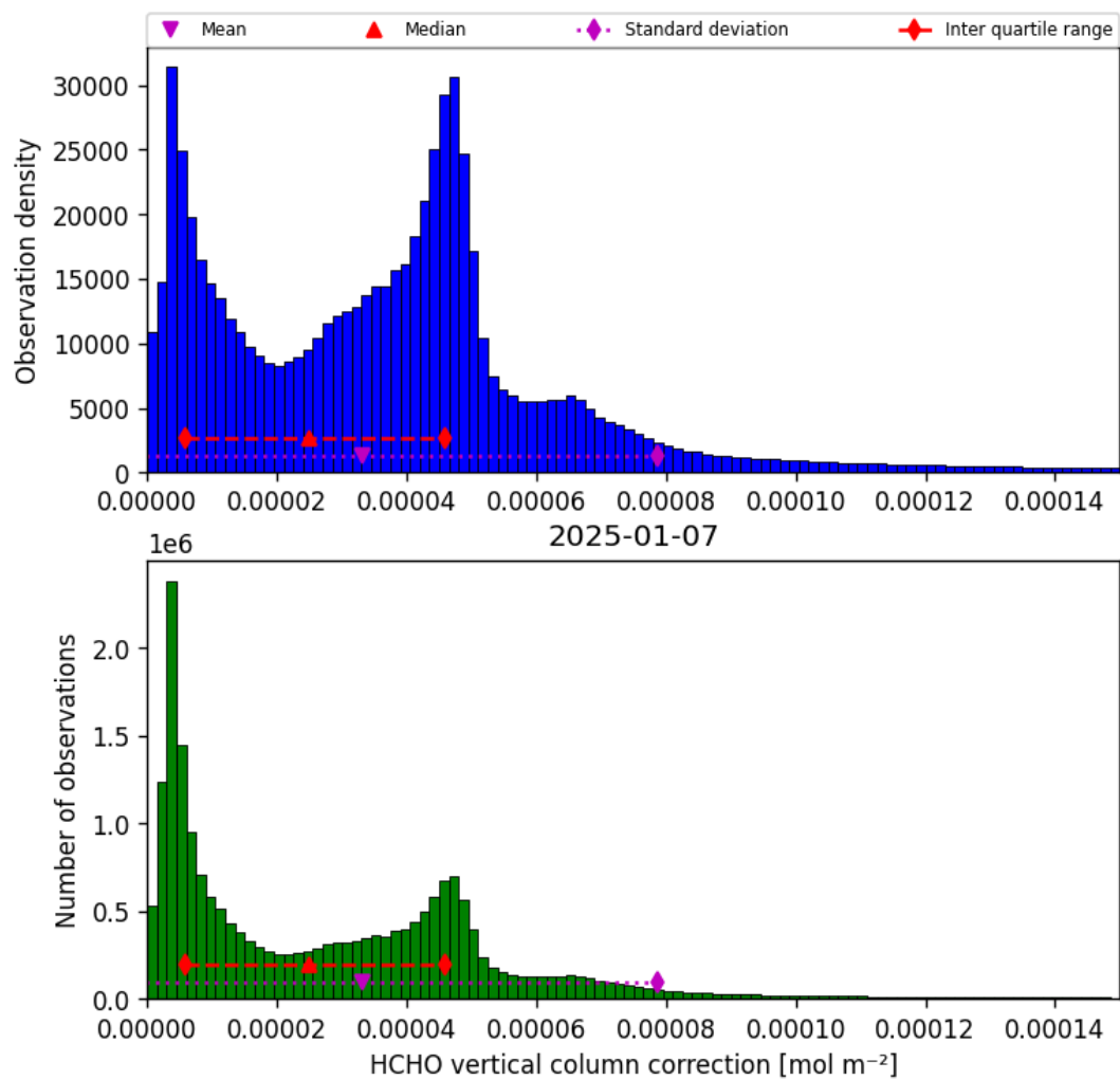
Figure 35: Histogram of “HCHO vertical column correction” for 2025-01-07 to 2025-01-08
