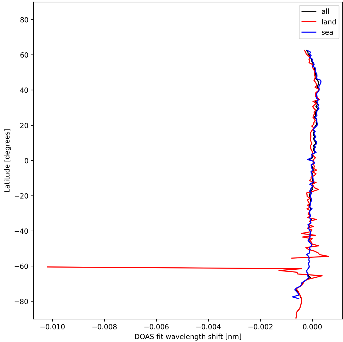
Figure 28: Zonal average of “DOAS fit wavelength shift” for 2025-01-07 to 2025-01-08.
