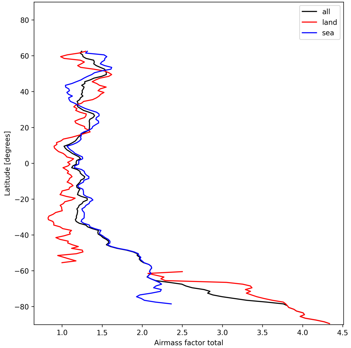
Figure 24: Zonal average of “Airmass factor total” for 2025-01-07 to 2025-01-08.
