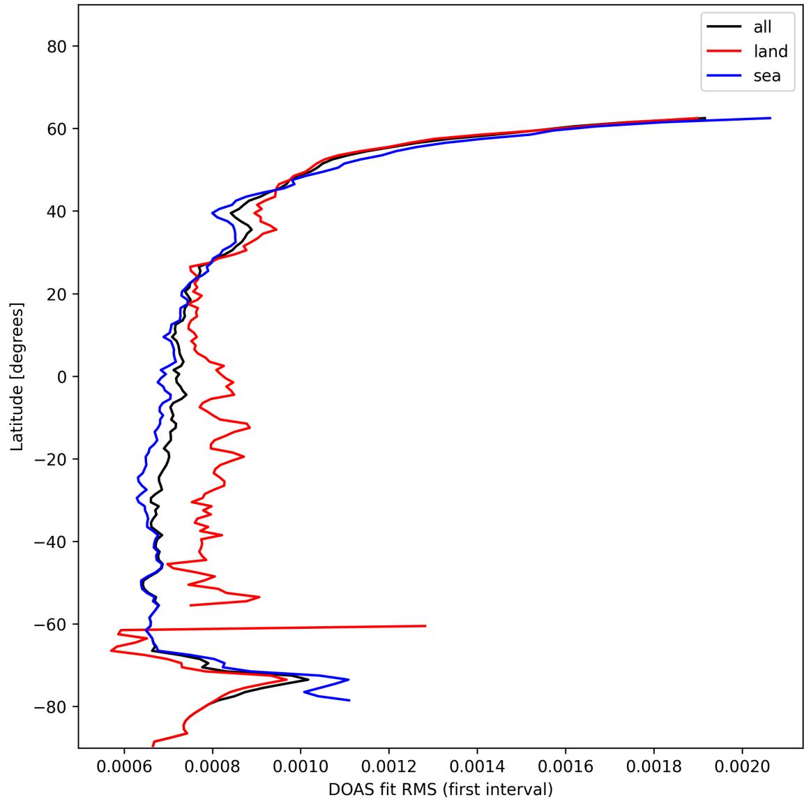
Figure 30: Zonal average of "DOAS fit RMS (first interval)" for 2025-01-07 to 2025-01-08.
