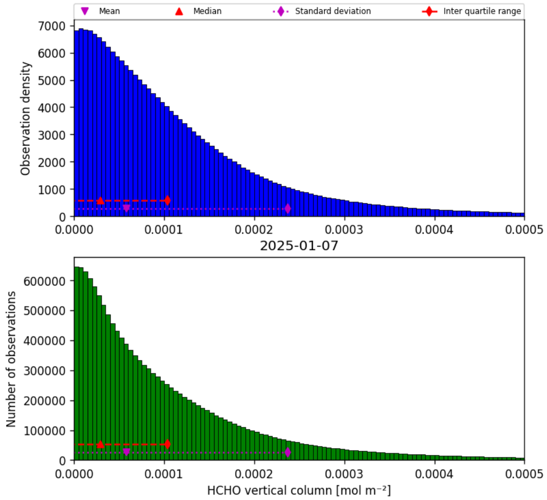
Figure 33: Histogram of “HCHO vertical column” for 2025-01-07 to 2025-01-08
