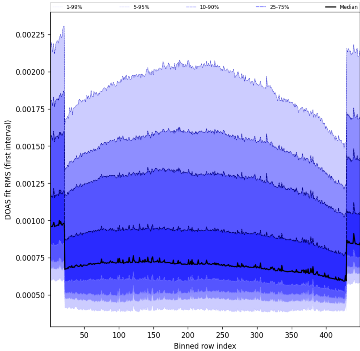
Figure 58: Along track statistics of “DOAS fit RMS (first interval)” for 2025-01-07 to 2025-01-08
