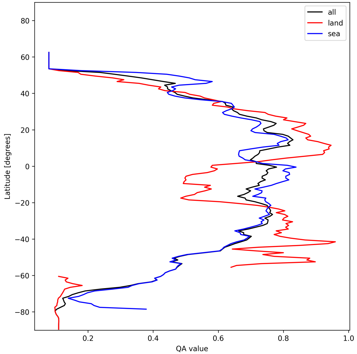
Figure 18: Zonal average of “QA value” for 2025-01-07 to 2025-01-08.
