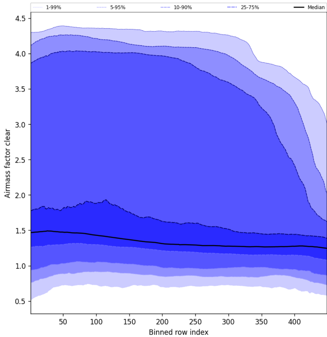
Figure 54: Along track statistics of “Airmass factor clear” for 2025-01-07 to 2025-01-08
