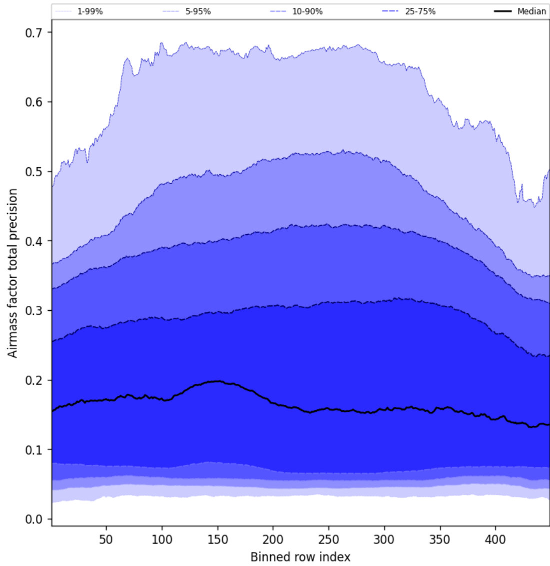
Figure 53: Along track statistics of “Airmass factor total precision” for 2025-01-07 to 2025-01-08
