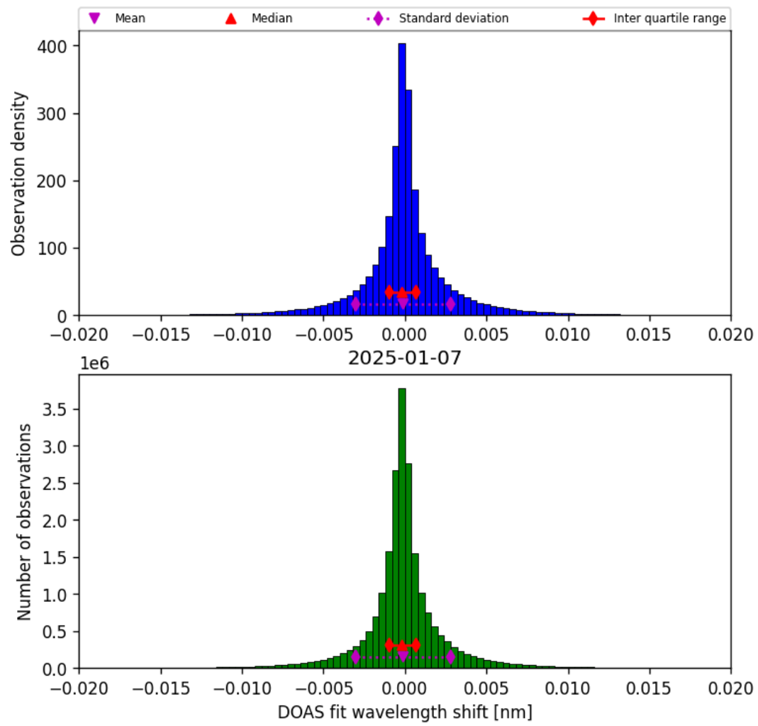
Figure 42: Histogram of “DOAS fit wavelength shift” for 2025-01-07 to 2025-01-08
