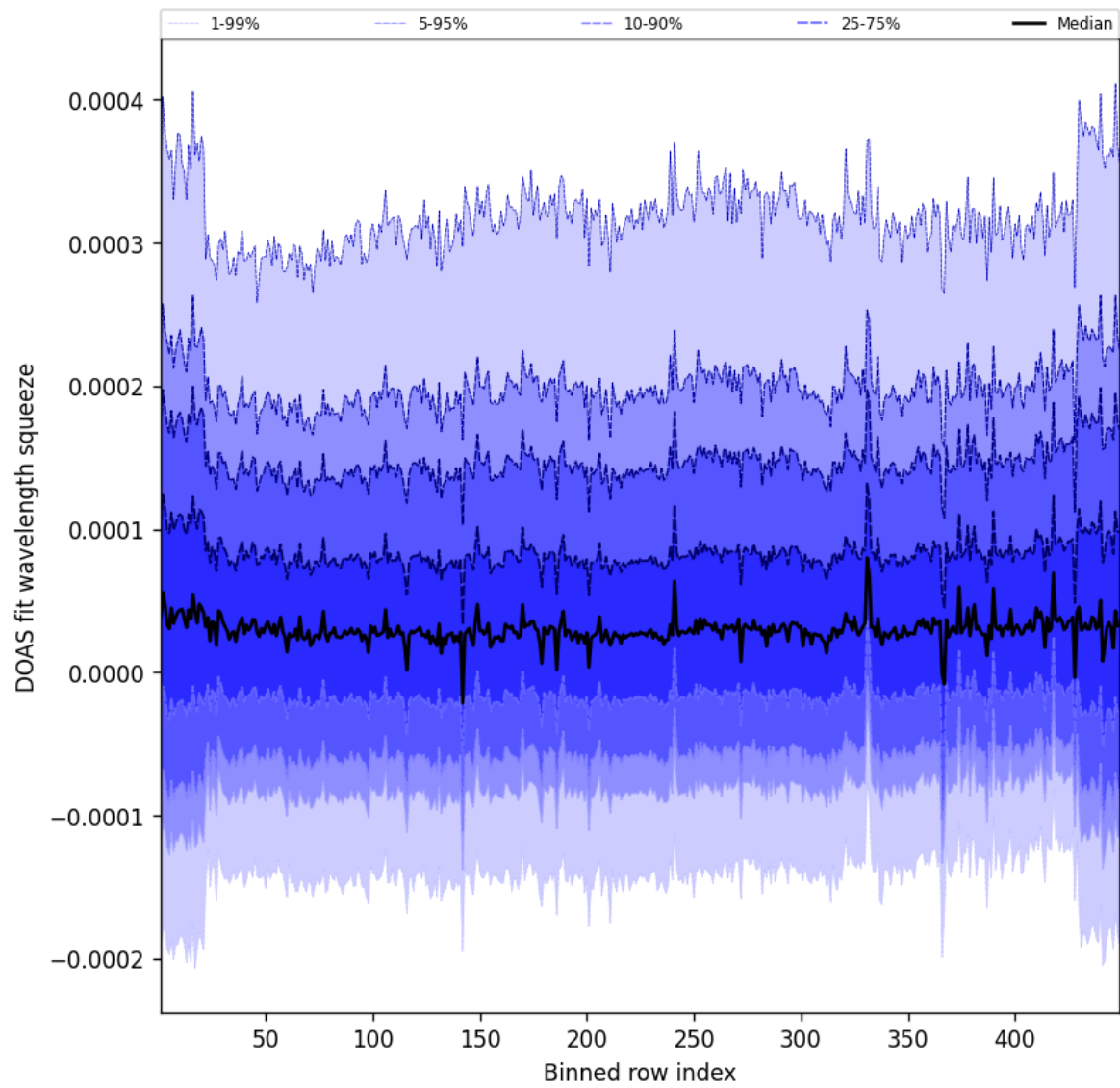
Figure 57: Along track statistics of “DOAS fit wavelength squeeze” for 2025-01-07 to 2025-01-08
