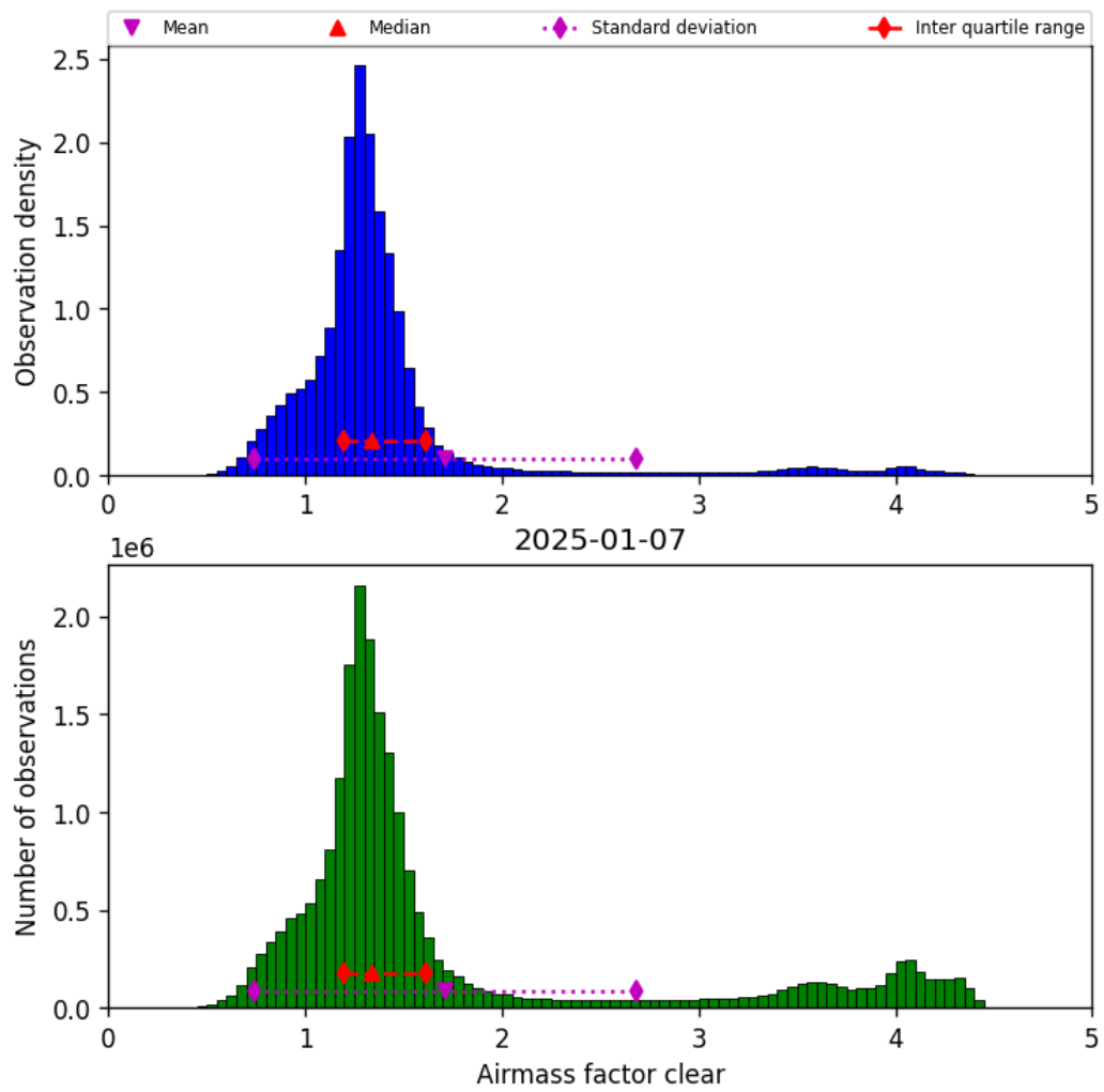
Figure 40: Histogram of “Airmass factor clear” for 2025-01-07 to 2025-01-08
