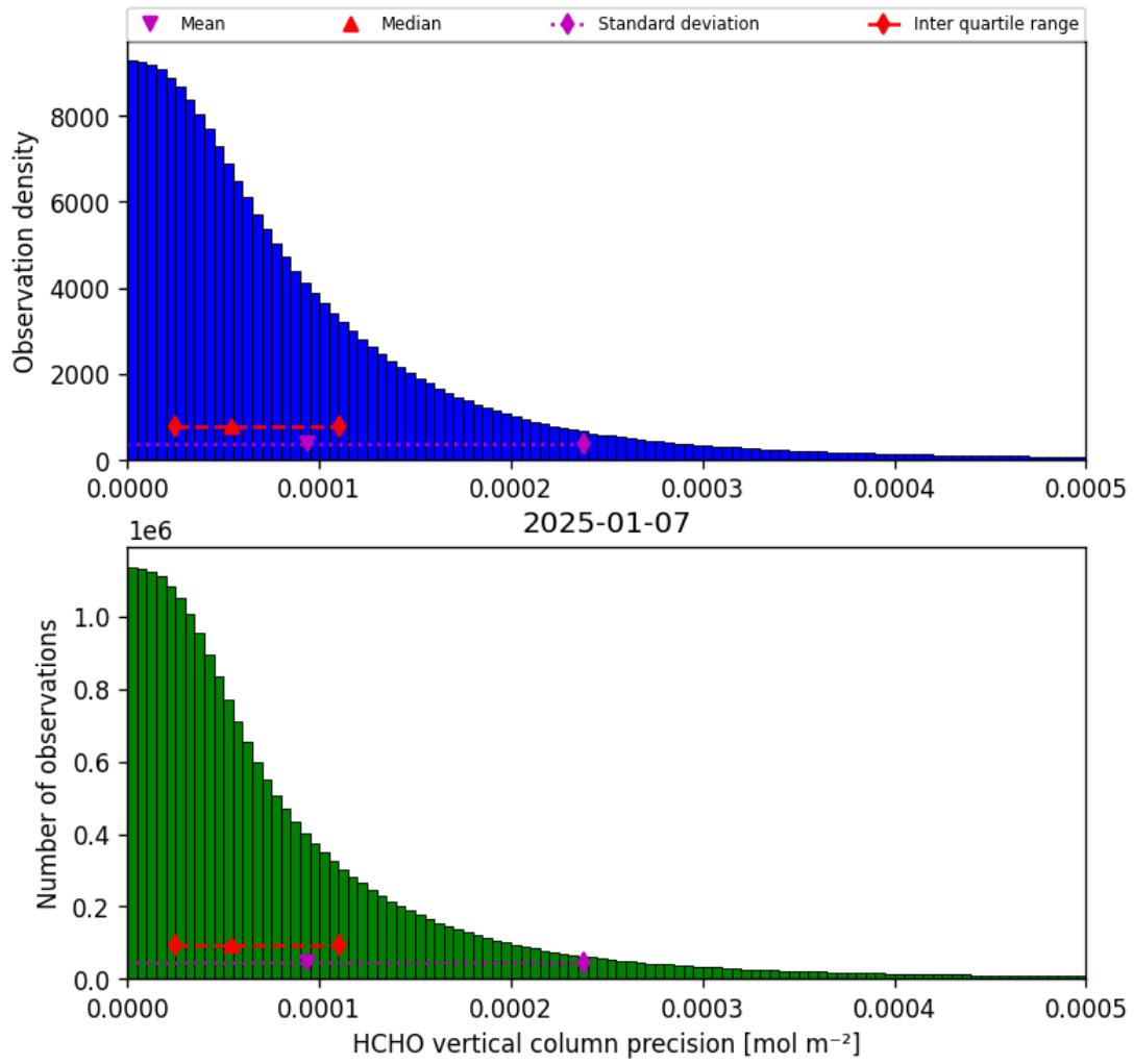
Figure 34: Histogram of “HCHO vertical column precision” for 2025-01-07 to 2025-01-08
