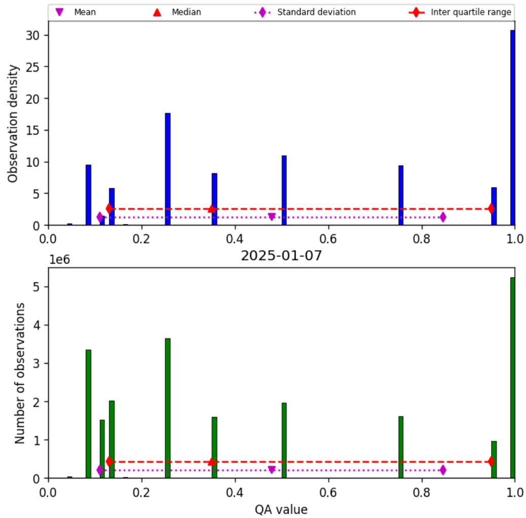
Figure 32: Histogram of “QA value” for 2025-01-07 to 2025-01-08
