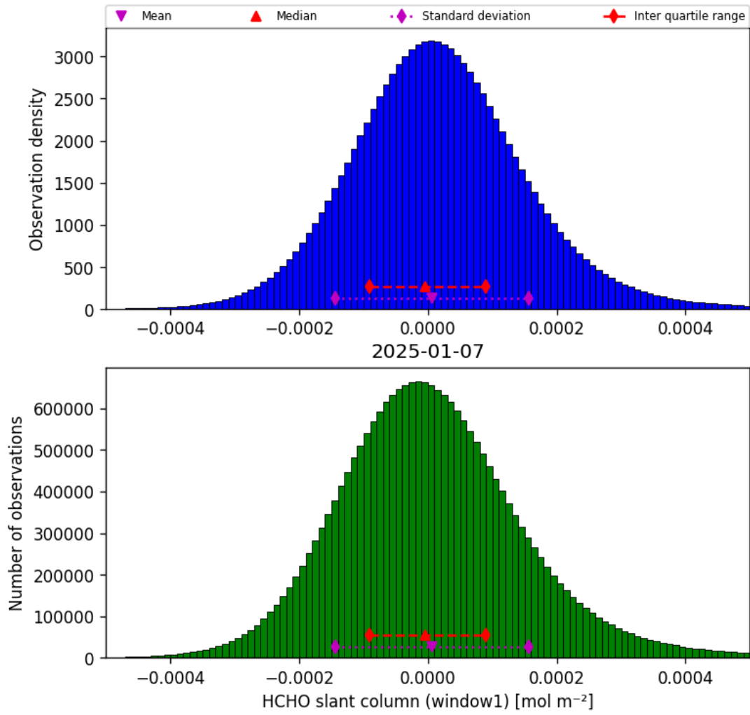
Figure 36: Histogram of “HCHO slant column (window1)” for 2025-01-07 to 2025-01-08
