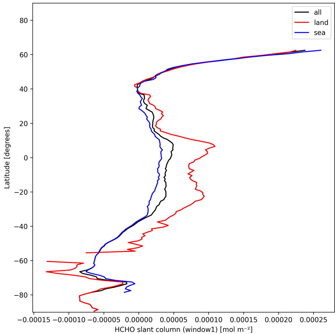
Figure 22: Zonal average of “HCHO slant column (window1)” for 2025-01-07 to 2025-01-08.
