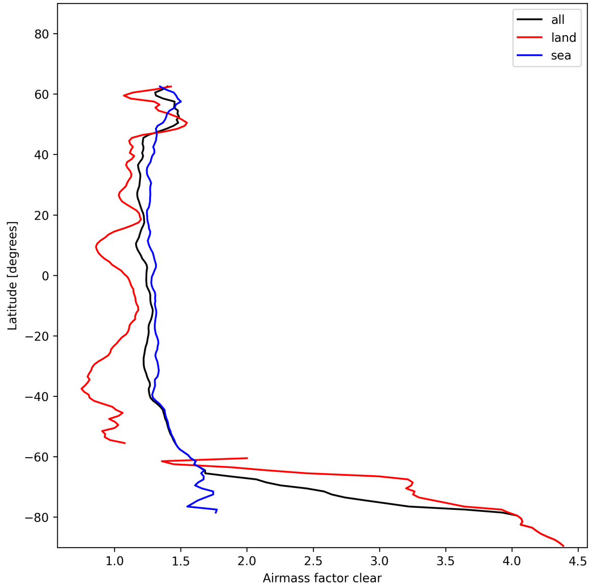
Figure 26: Zonal average of “Airmass factor clear” for 2025-01-07 to 2025-01-08.
