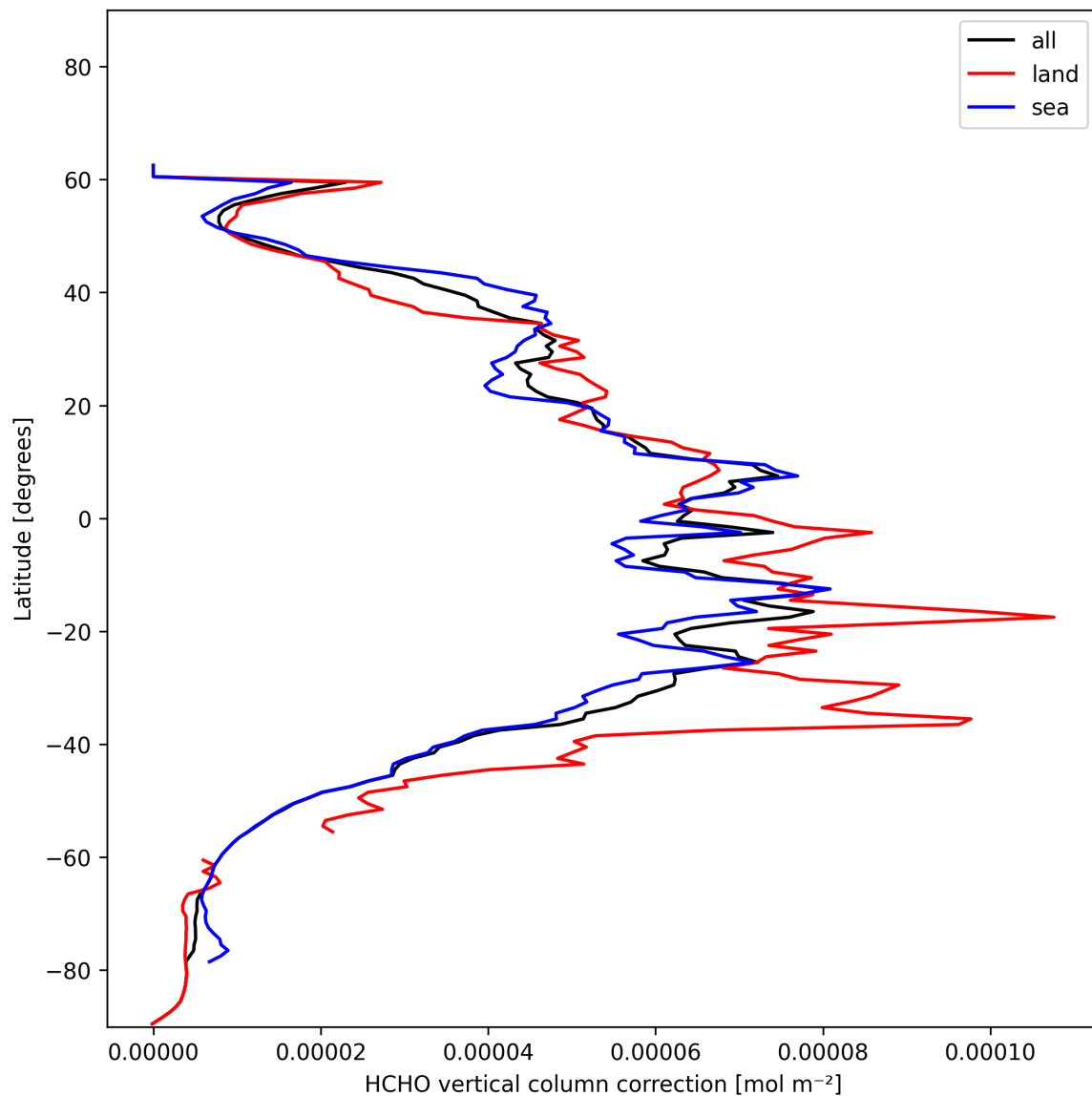
Figure 21: Zonal average of “HCHO vertical column correction” for 2025-01-07 to 2025-01-08.
