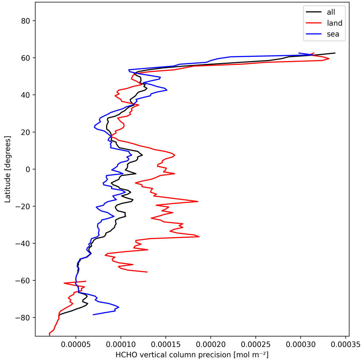
Figure 20: Zonal average of “HCHO vertical column precision” for 2025-01-07 to 2025-01-08.
