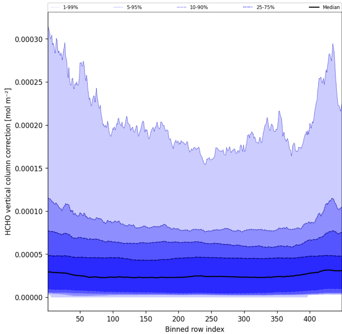
Figure 49: Along track statistics of “HCHO vertical column correction” for 2025-01-07 to 2025-01-08
