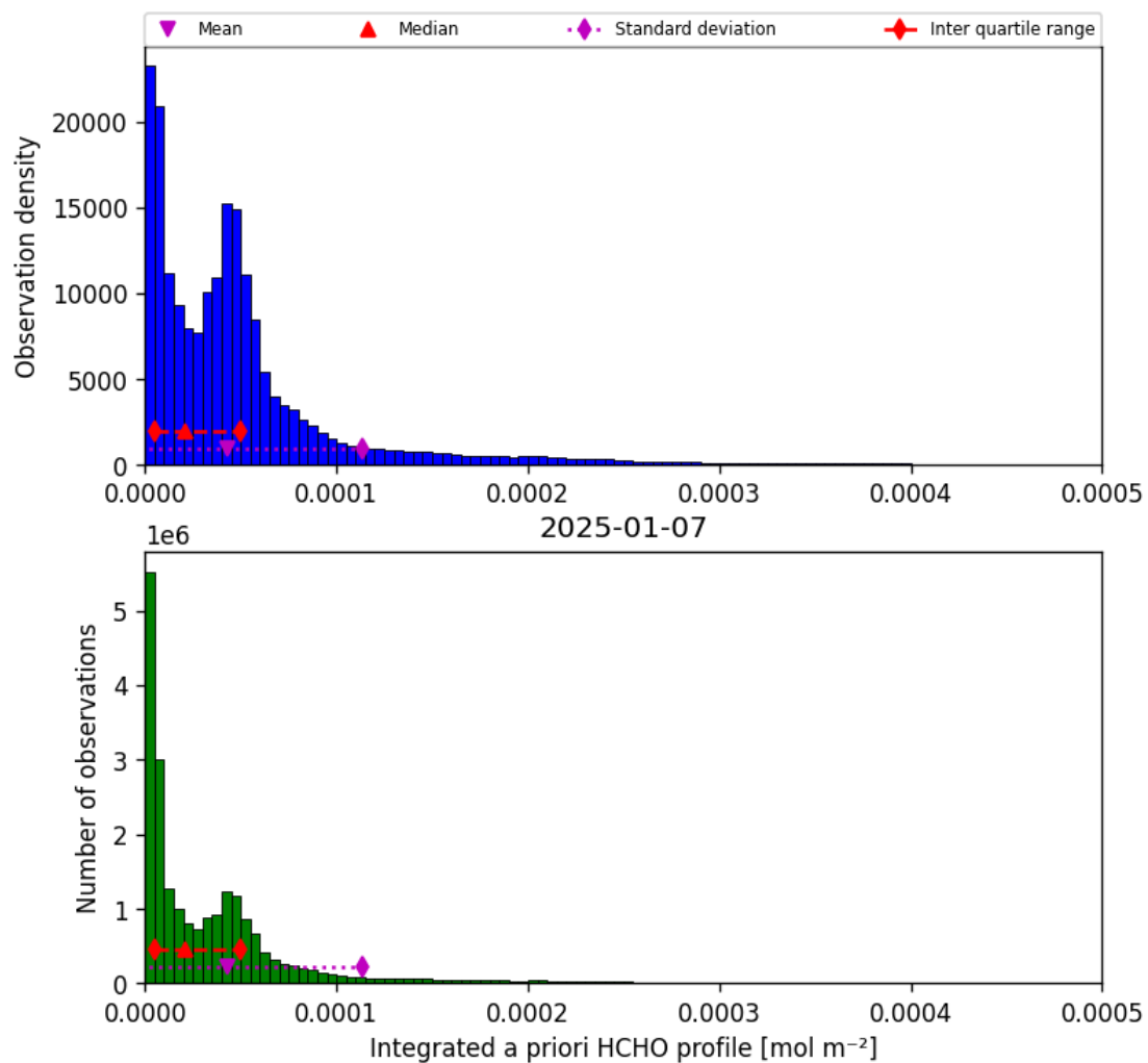
Figure 41: Histogram of “Integrated a priori HCHO profile” for 2025-01-07 to 2025-01-08
