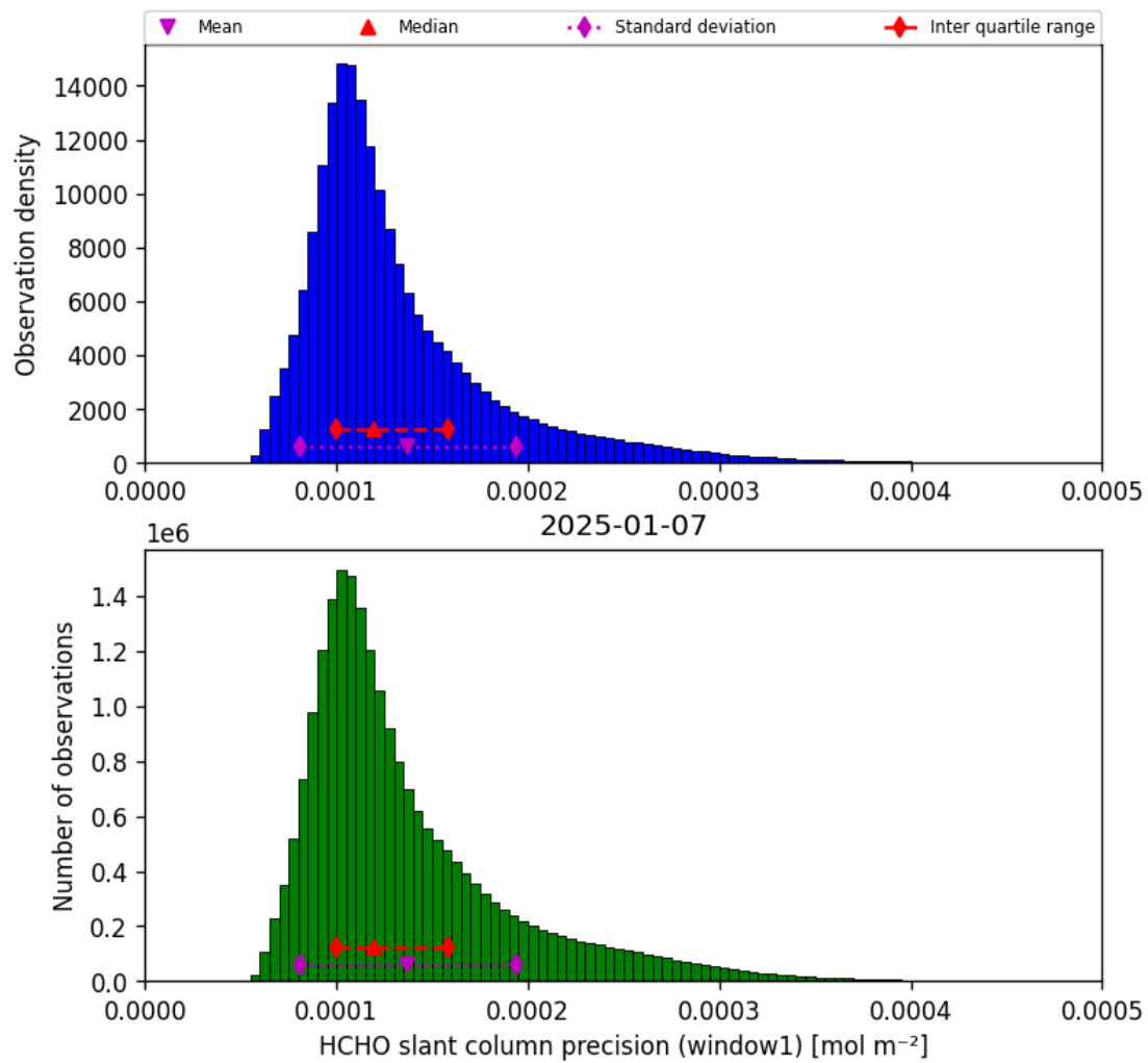
Figure 37: Histogram of “HCHO slant column precision (window1)” for 2025-01-07 to 2025-01-08
