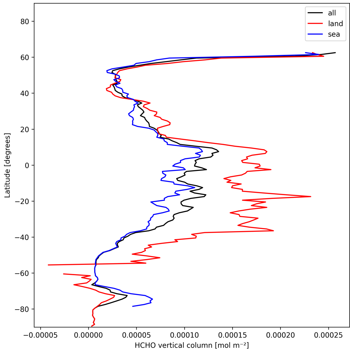
Figure 19: Zonal average of “HCHO vertical column” for 2025-01-07 to 2025-01-08.
