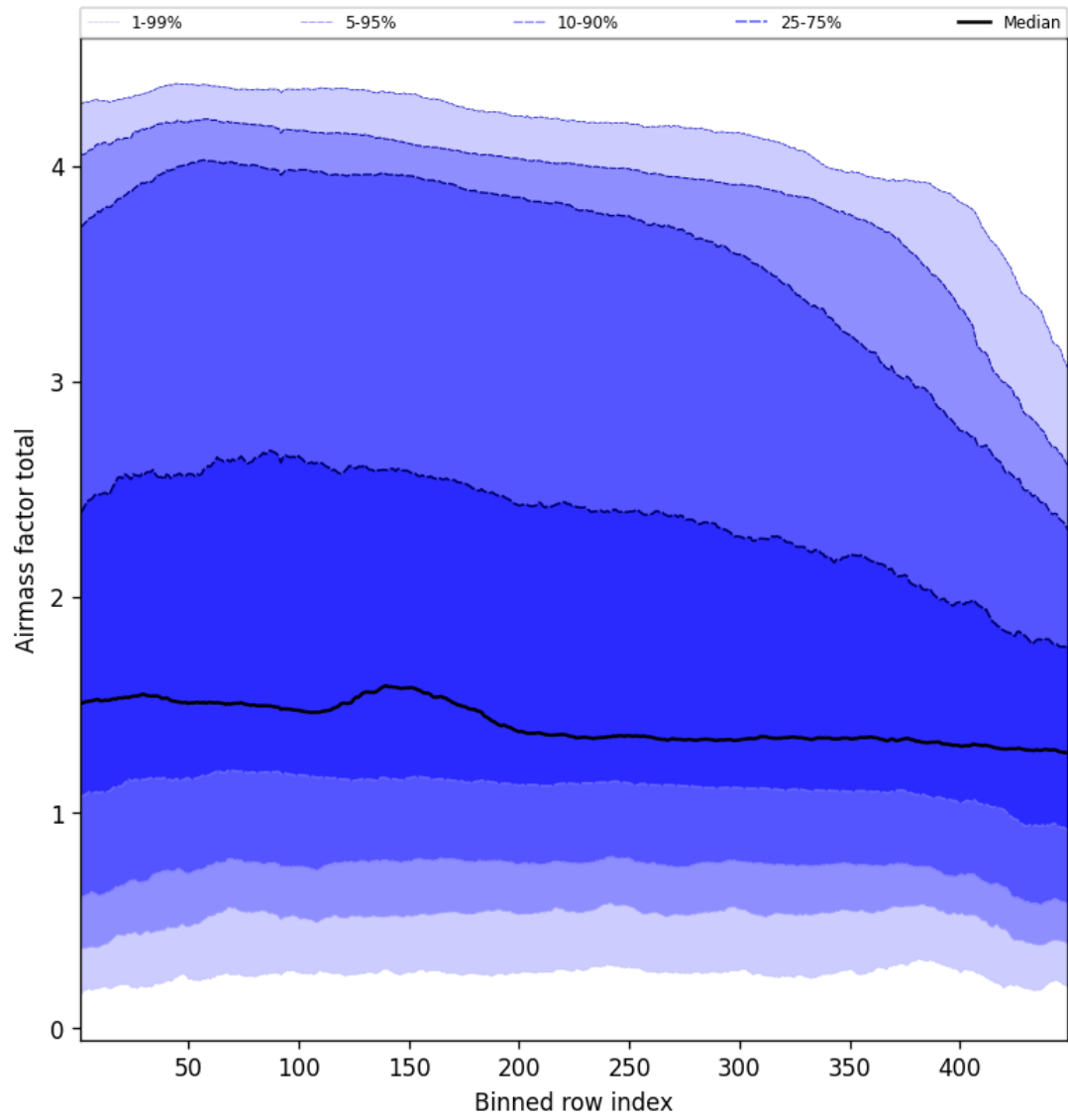
Figure 52: Along track statistics of “Airmass factor total” for 2025-01-07 to 2025-01-08
