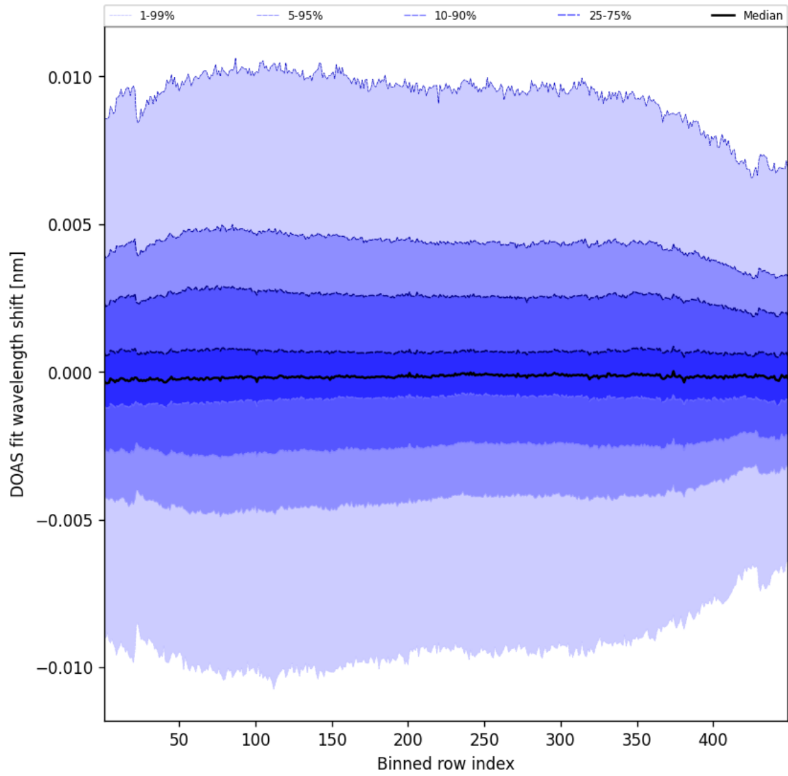
Figure 56: Along track statistics of “DOAS fit wavelength shift” for 2025-01-07 to 2025-01-08
