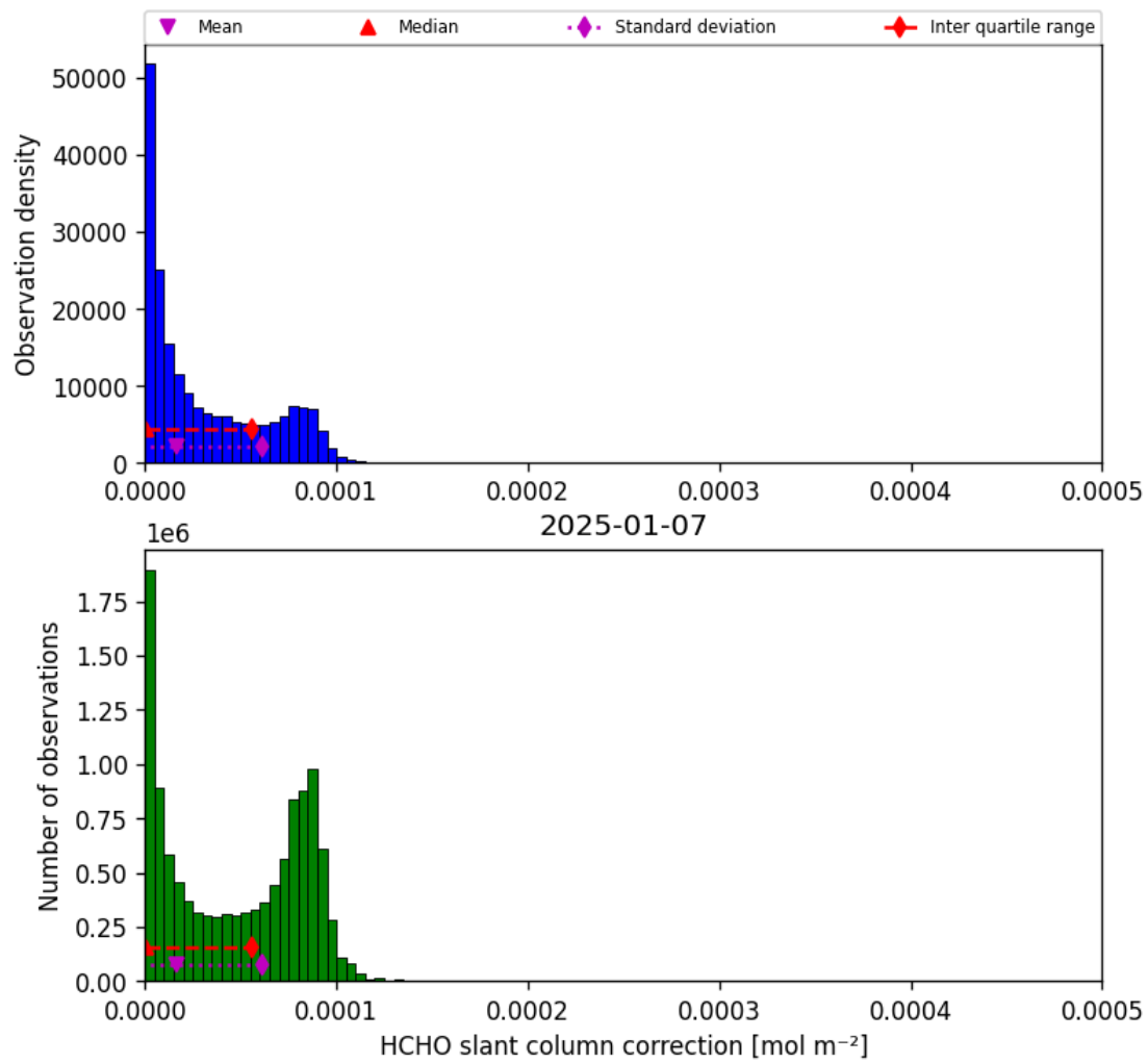
Figure 45: Histogram of “HCHO slant column correction” for 2025-01-07 to 2025-01-08
