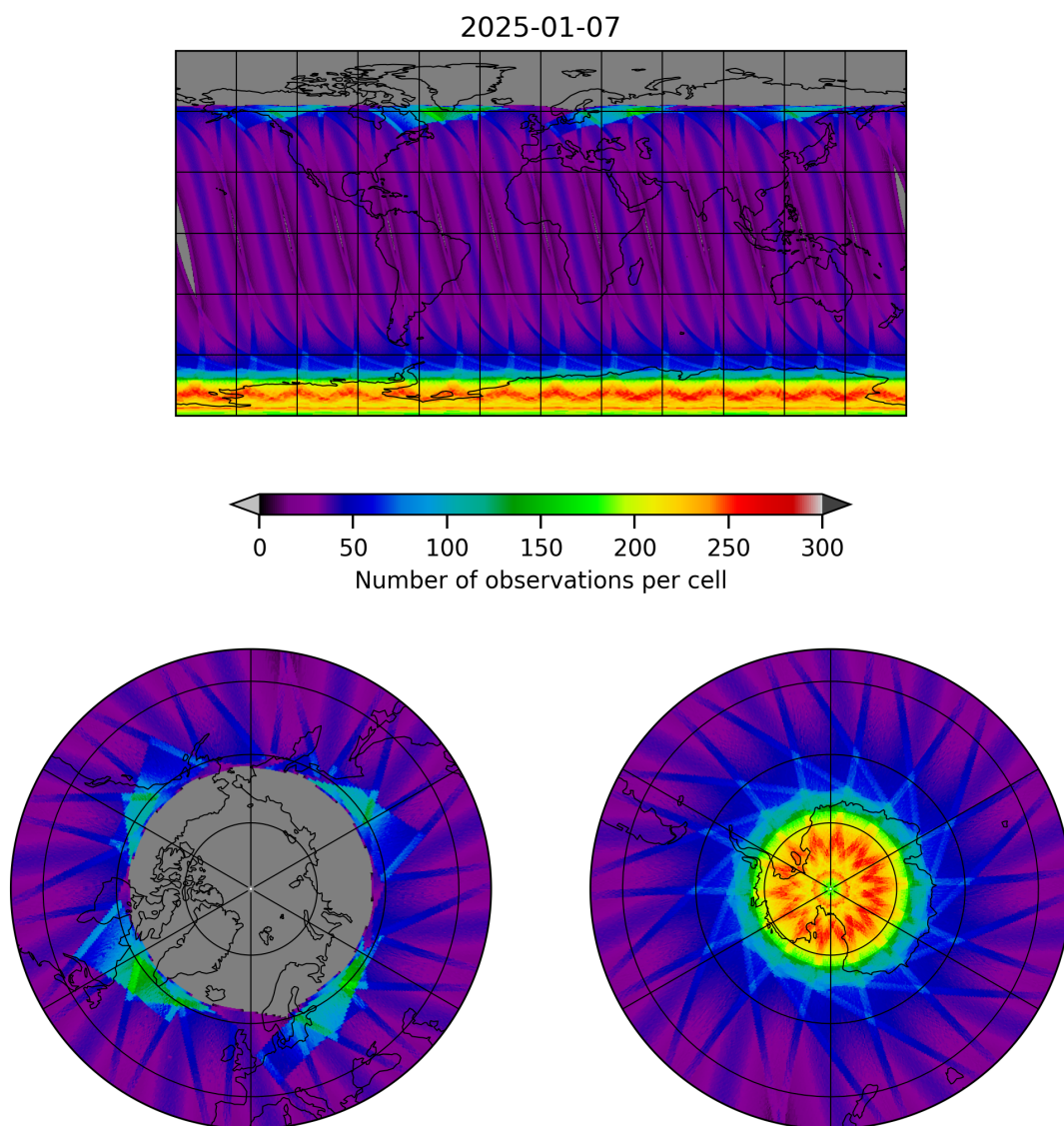
Figure 17: Map of the number of observations for 2025-01-07 to 2025-01-08
