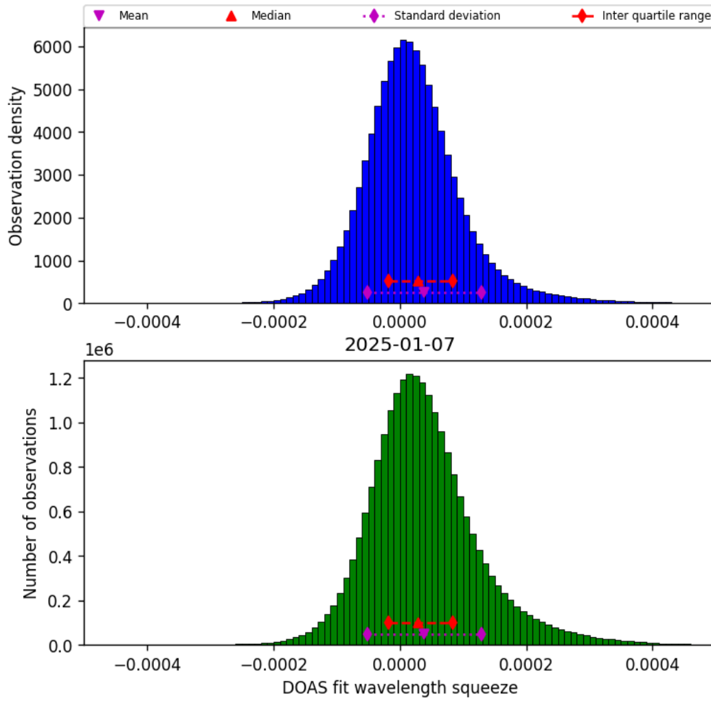
Figure 43: Histogram of “DOAS fit wavelength squeeze” for 2025-01-07 to 2025-01-08
