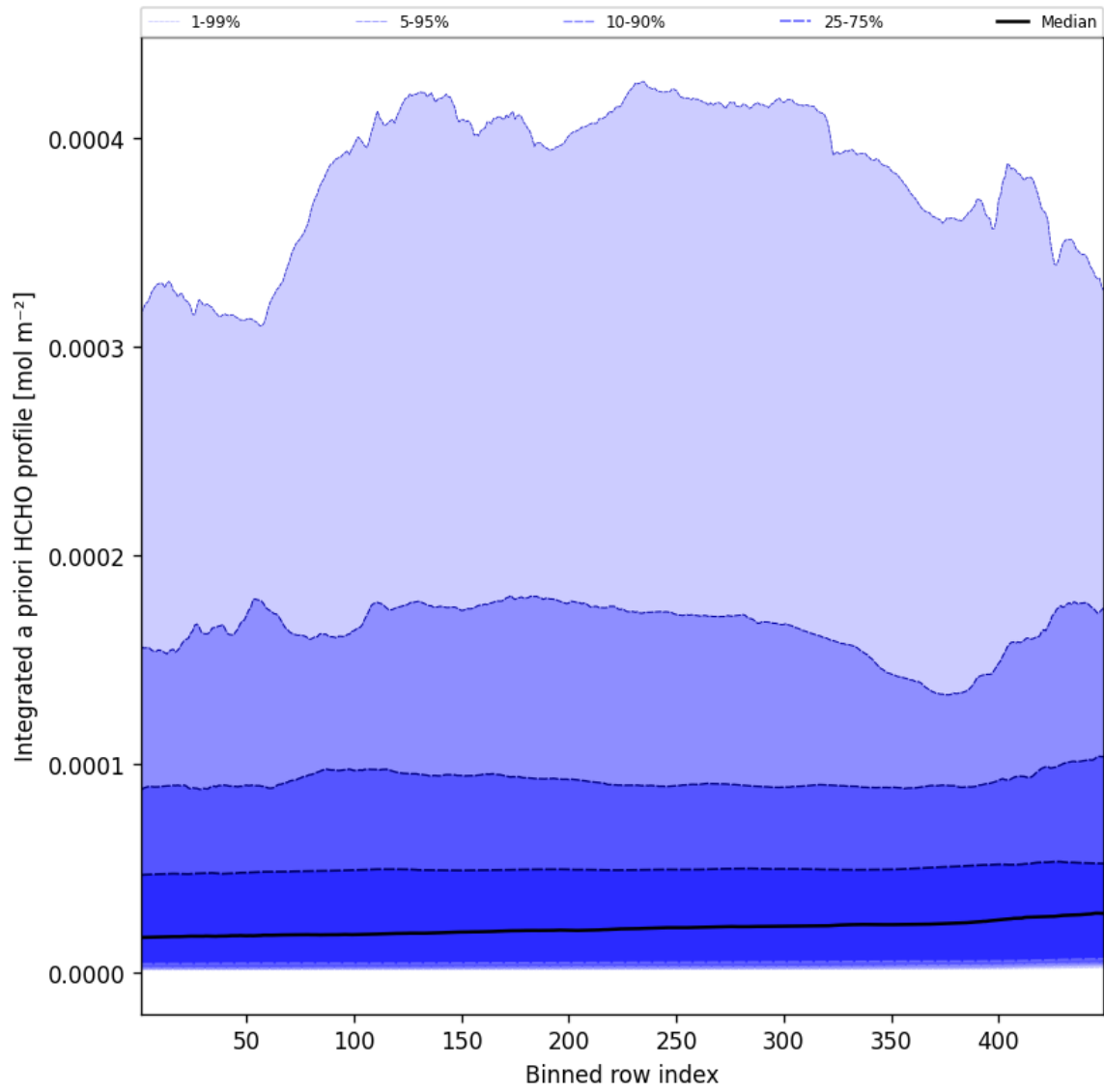
Figure 55: Along track statistics of “Integrated a priori HCHO profile” for 2025-01-07 to 2025-01-08
