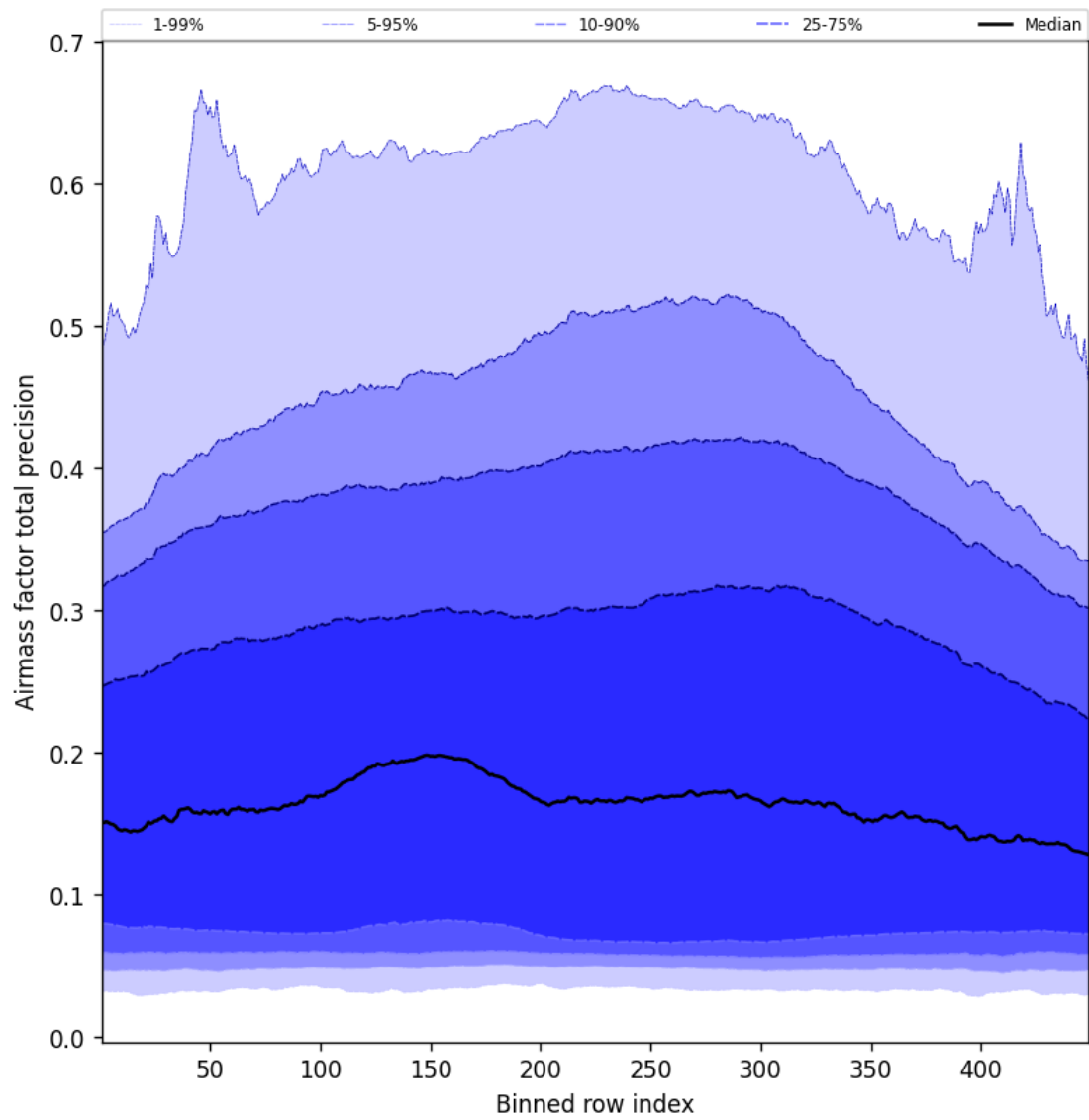
Figure 53: Along track statistics of “Airmass factor total precision” for 2025-01-08 to 2025-01-09
