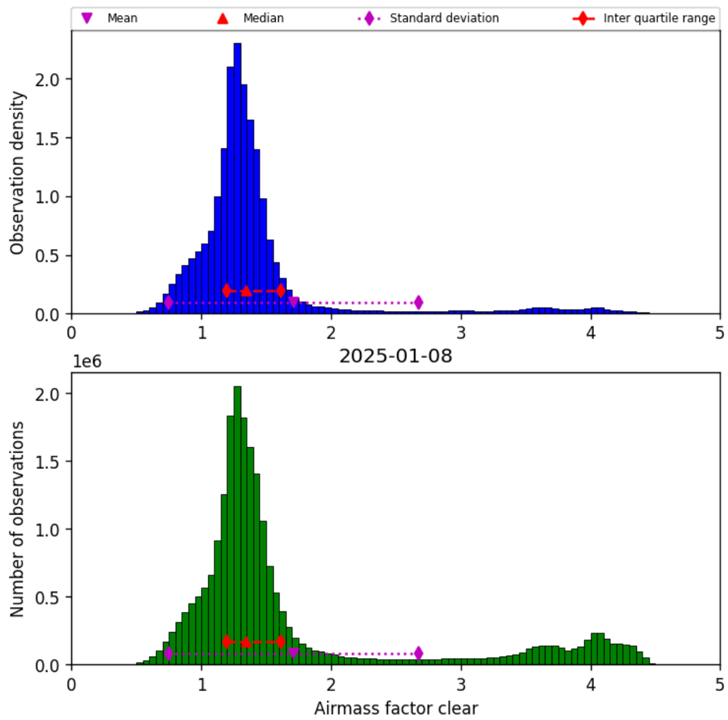
Figure 40: Histogram of “Airmass factor clear” for 2025-01-08 to 2025-01-09
