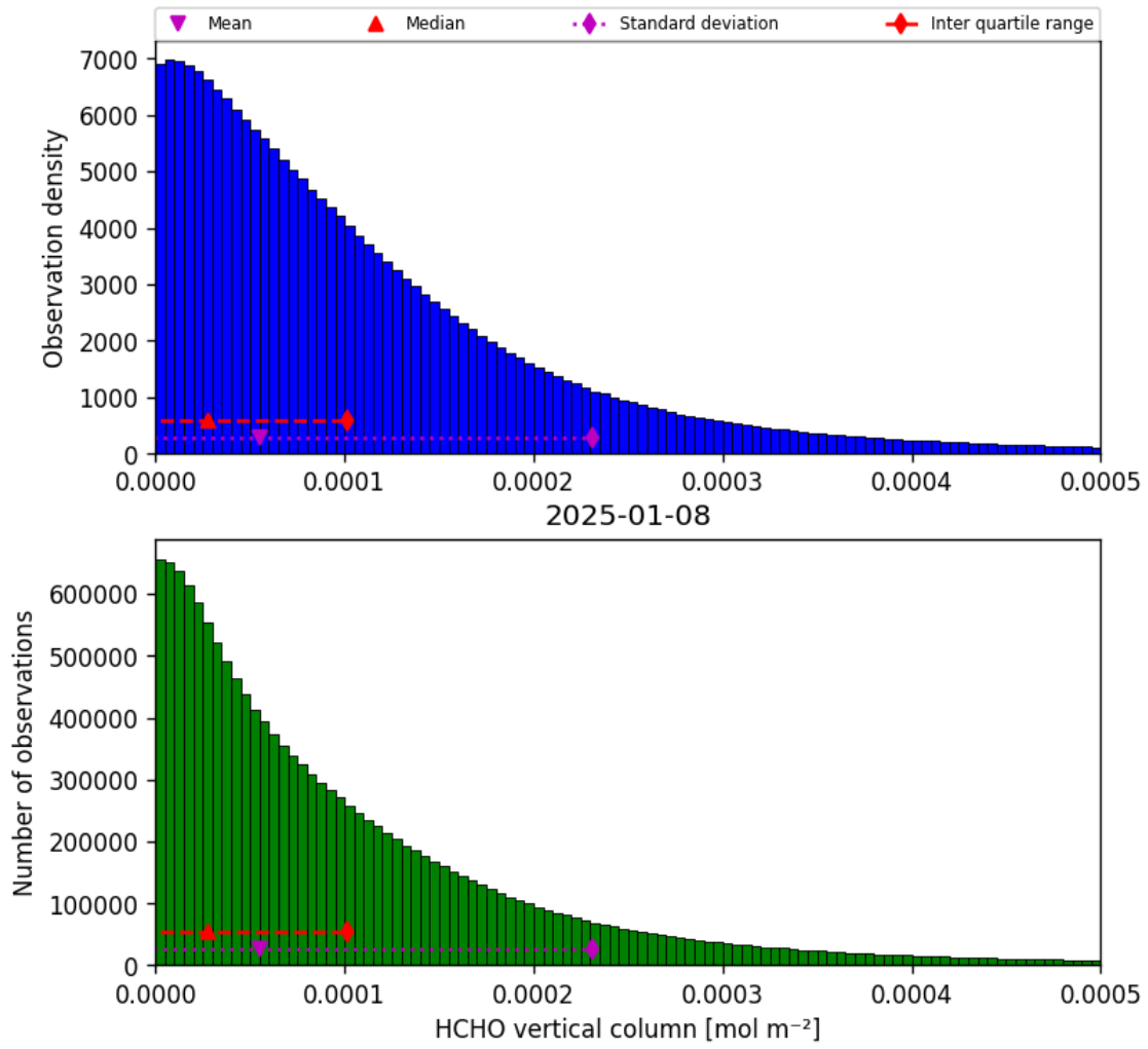
Figure 33: Histogram of “HCHO vertical column” for 2025-01-08 to 2025-01-09
