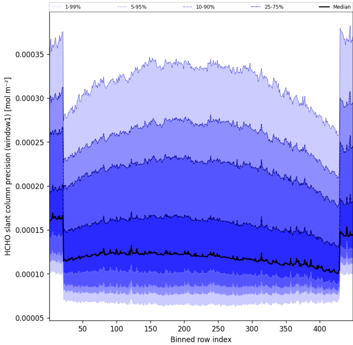
Figure 51: Along track statistics of “HCHO slant column precision (window1)” for 2025-01-08 to 2025-01-09
