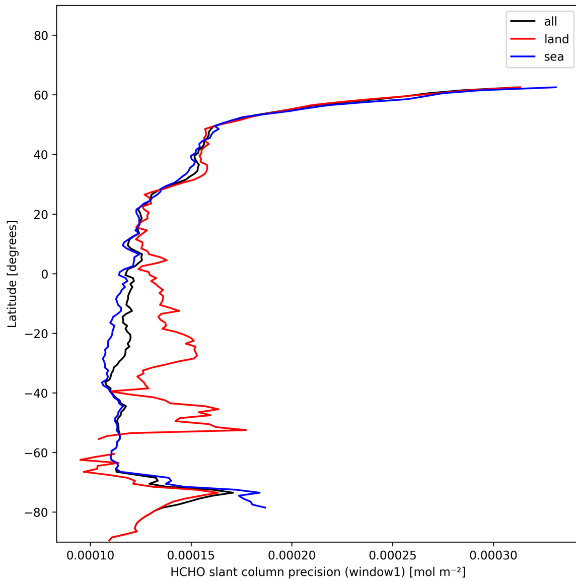
Figure 23: Zonal average of “HCHO slant column precision (window1)” for 2025-01-08 to 2025-01-09.
