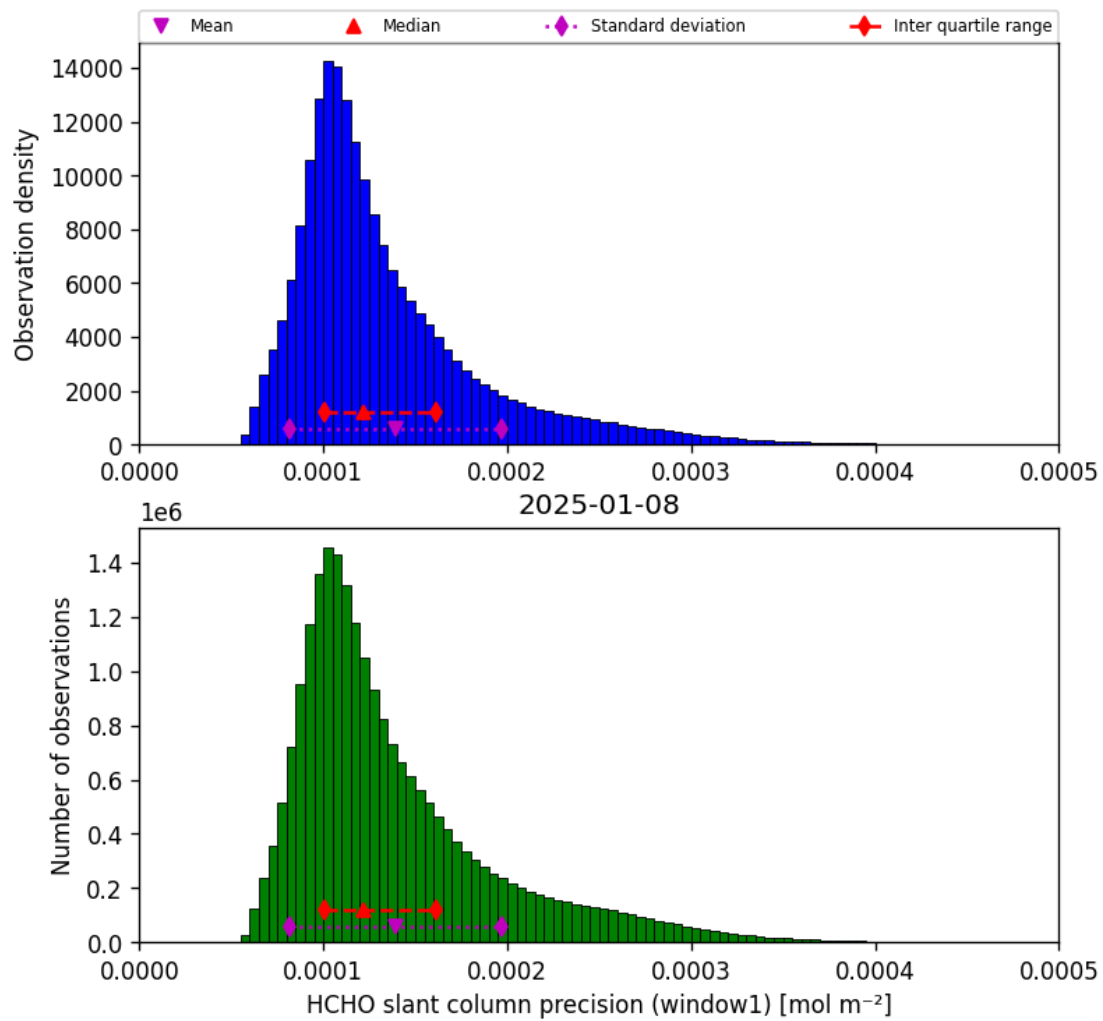
Figure 37: Histogram of “HCHO slant column precision (window1)” for 2025-01-08 to 2025-01-09
