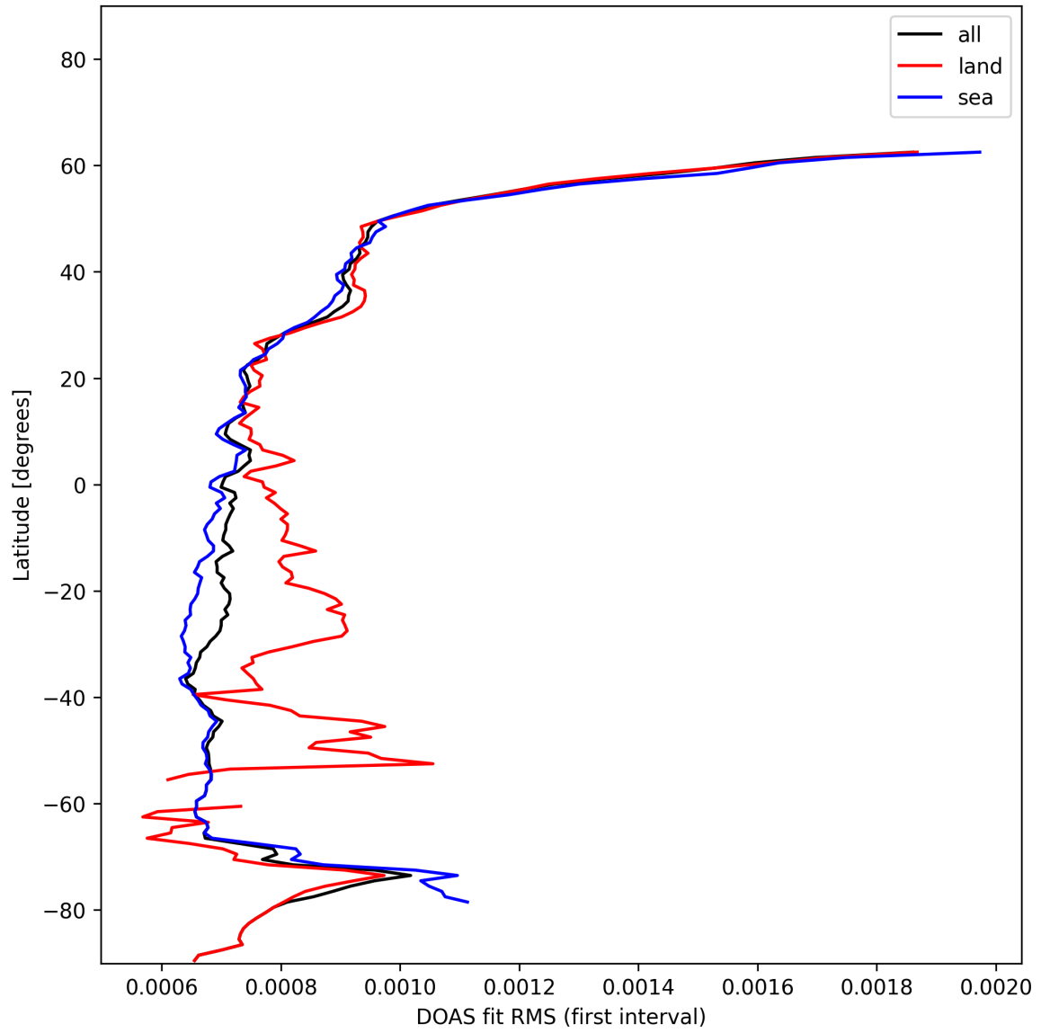
Figure 30: Zonal average of “DOAS fit RMS (first interval)” for 2025-01-08 to 2025-01-09.
