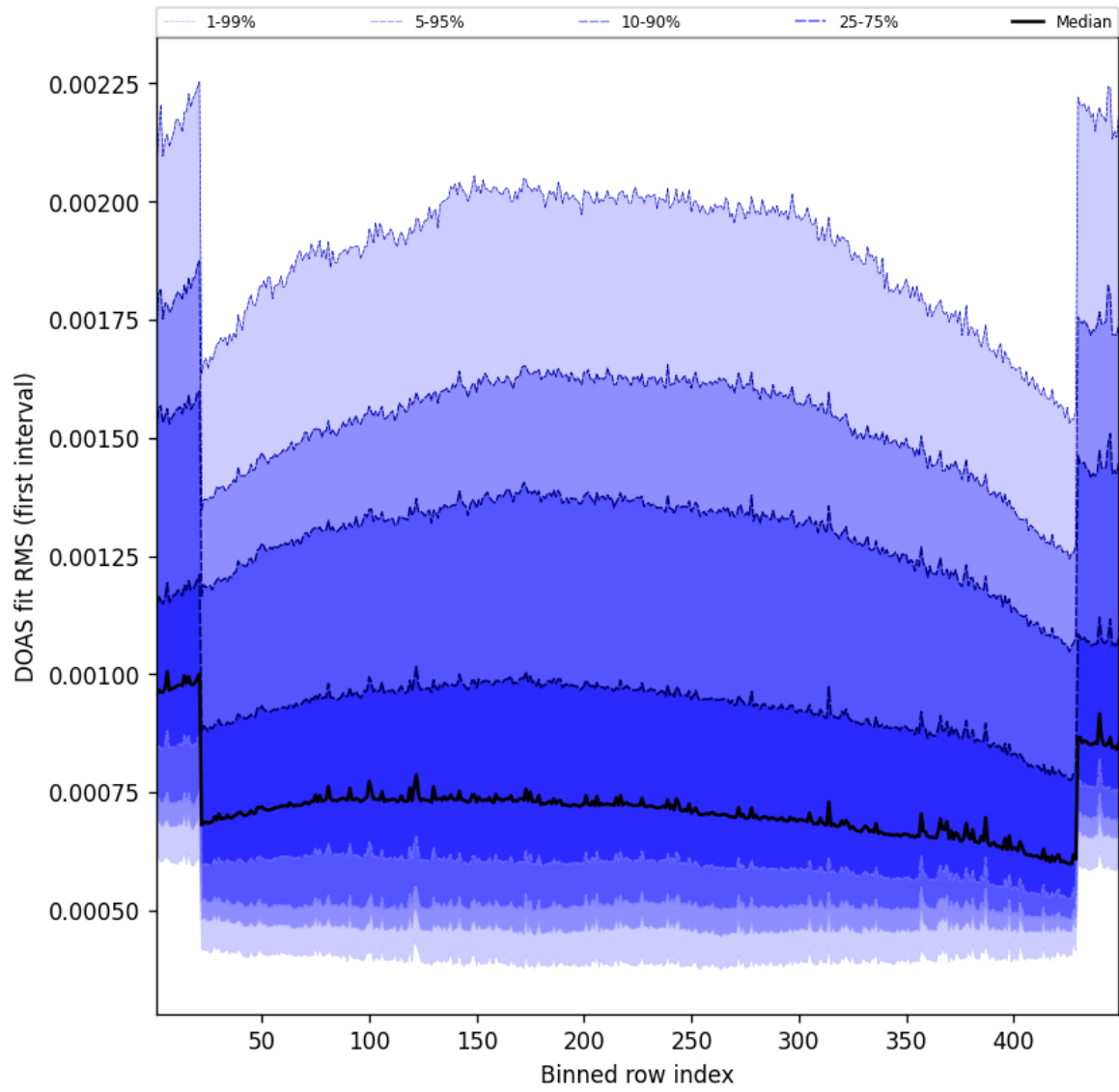
Figure 58: Along track statistics of “DOAS fit RMS (first interval)” for 2025-01-08 to 2025-01-09
