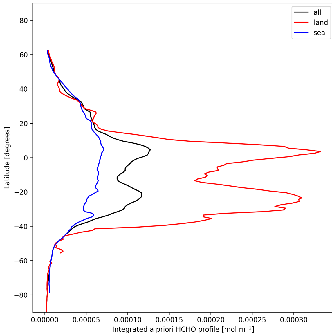
Figure 27: Zonal average of “Integrated a priori HCHO profile” for 2025-01-08 to 2025-01-09.
