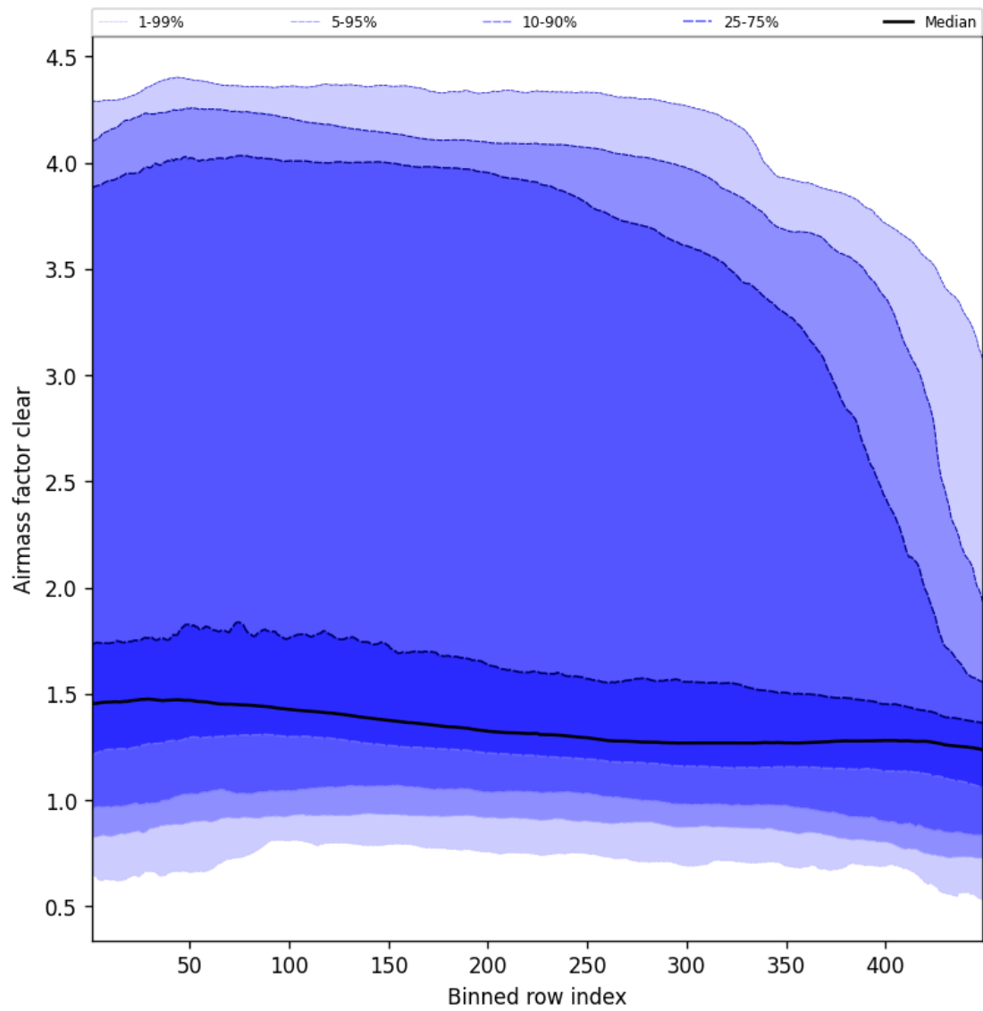
Figure 54: Along track statistics of “Airmass factor clear” for 2025-01-08 to 2025-01-09
