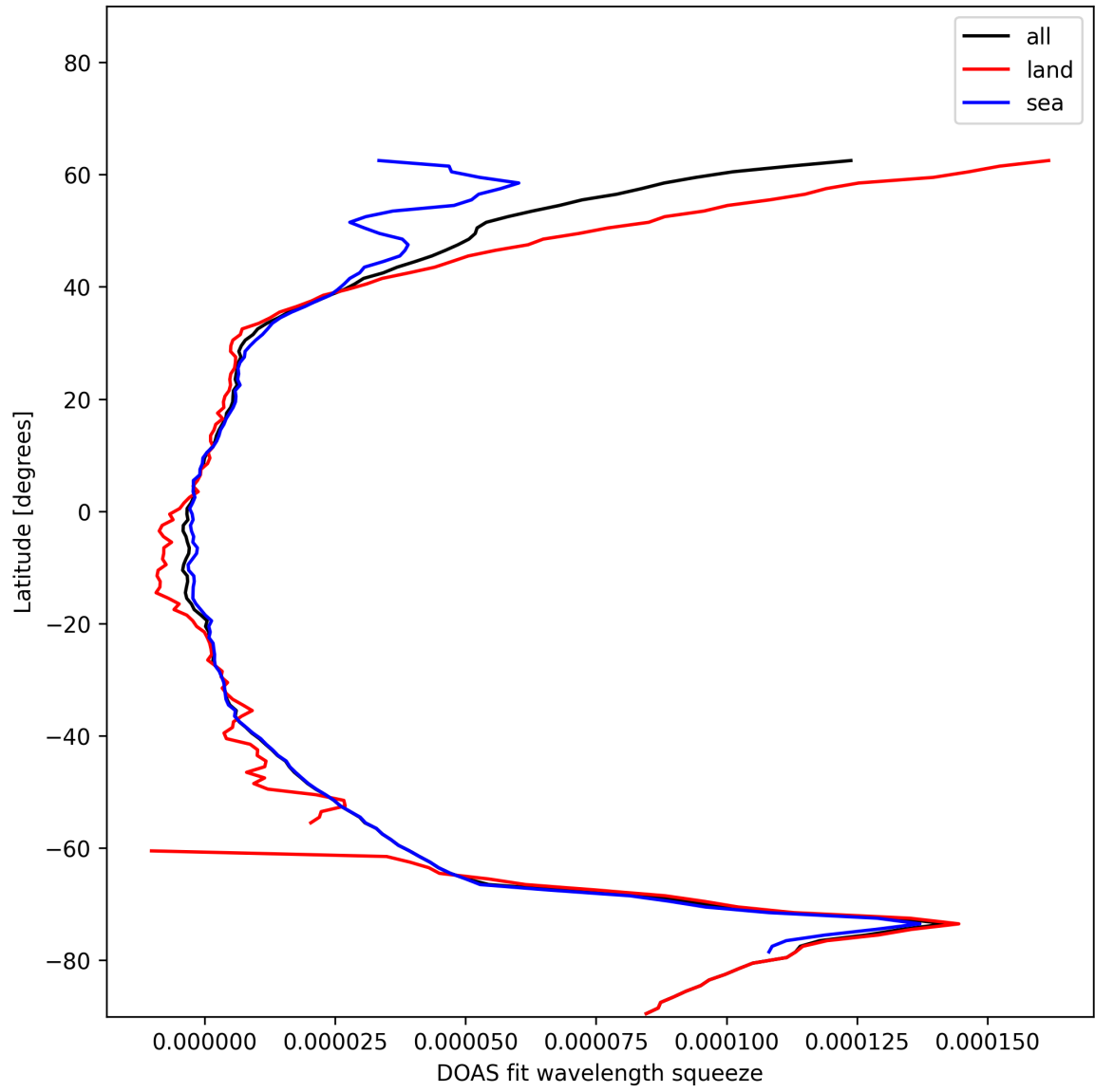
Figure 29: Zonal average of “DOAS fit wavelength squeeze” for 2025-01-08 to 2025-01-09.
