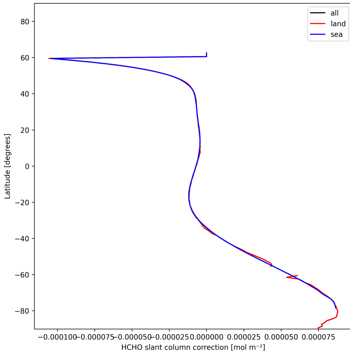
Figure 31: Zonal average of “HCHO slant column correction” for 2025-01-08 to 2025-01-09.
