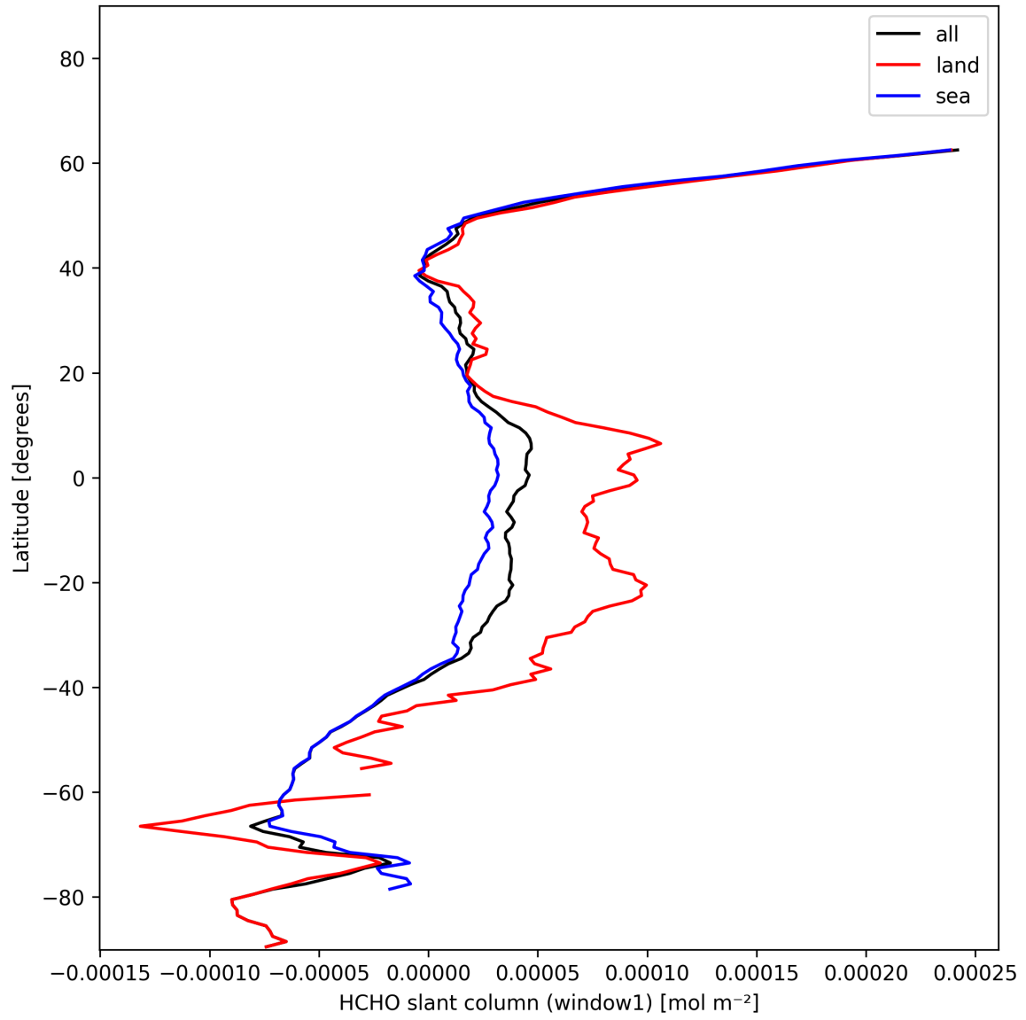
Figure 22: Zonal average of “HCHO slant column (window1)” for 2025-01-08 to 2025-01-09.
