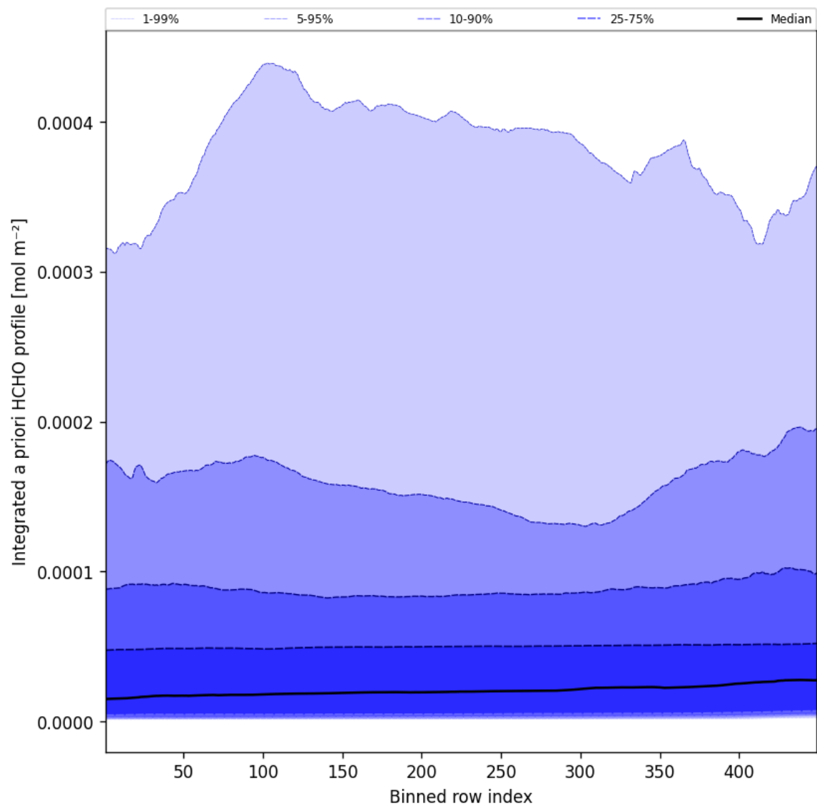
Figure 55: Along track statistics of “Integrated a priori HCHO profile” for 2025-01-08 to 2025-01-09
