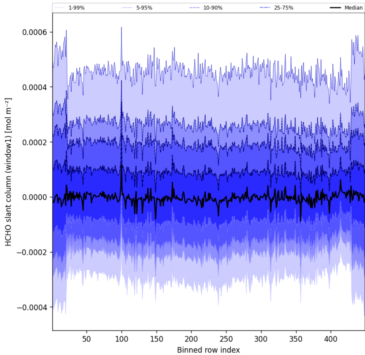
Figure 50: Along track statistics of “HCHO slant column (window1)” for 2025-01-08 to 2025-01-09
