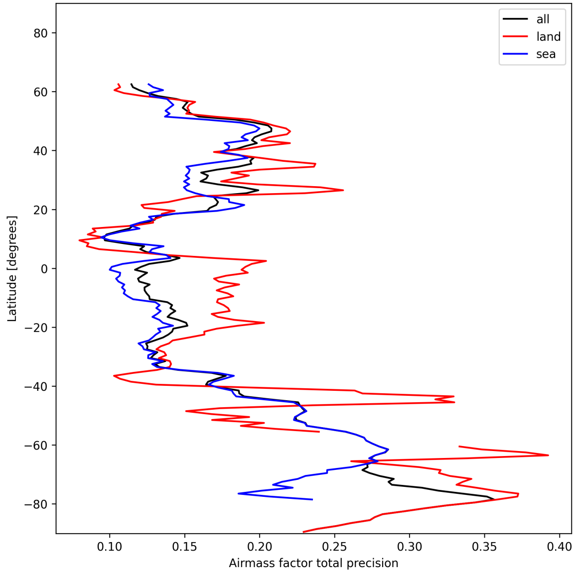
Figure 25: Zonal average of “Airmass factor total precision” for 2025-01-08 to 2025-01-09.
