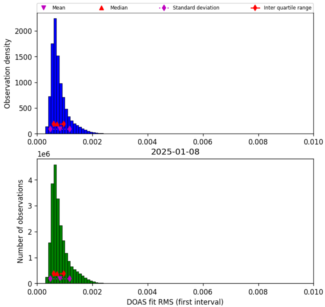
Figure 44: Histogram of "DOAS fit RMS (first interval)" for 2025-01-08 to 2025-01-09
