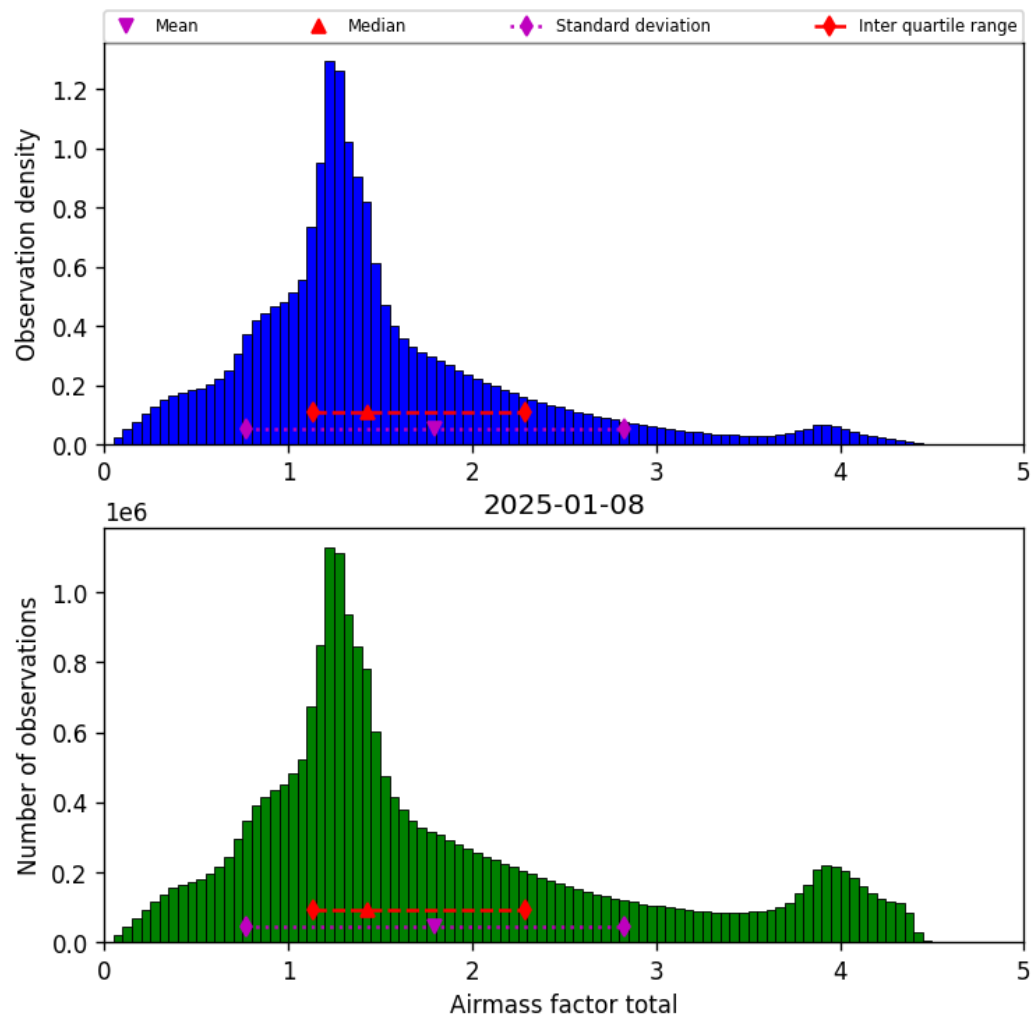
Figure 38: Histogram of “Airmass factor total” for 2025-01-08 to 2025-01-09
