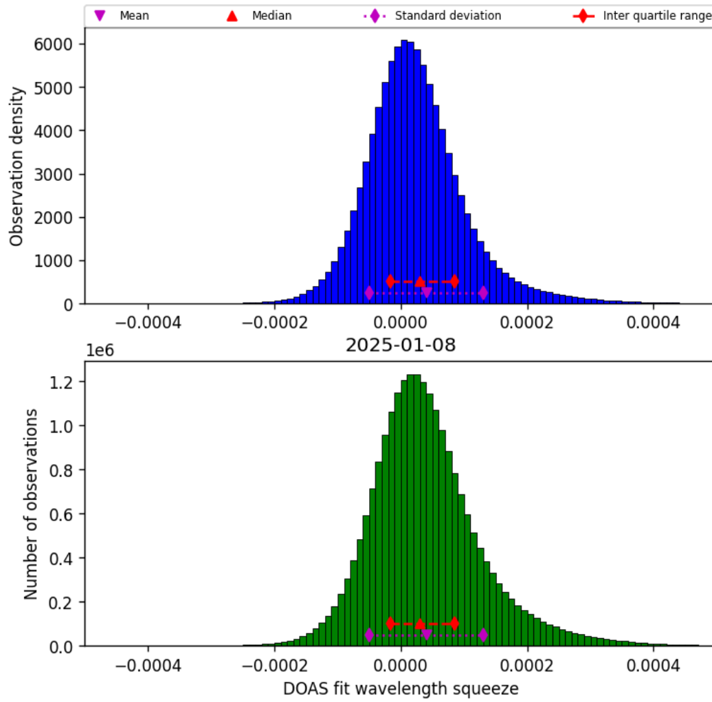
Figure 43: Histogram of “DOAS fit wavelength squeeze” for 2025-01-08 to 2025-01-09
