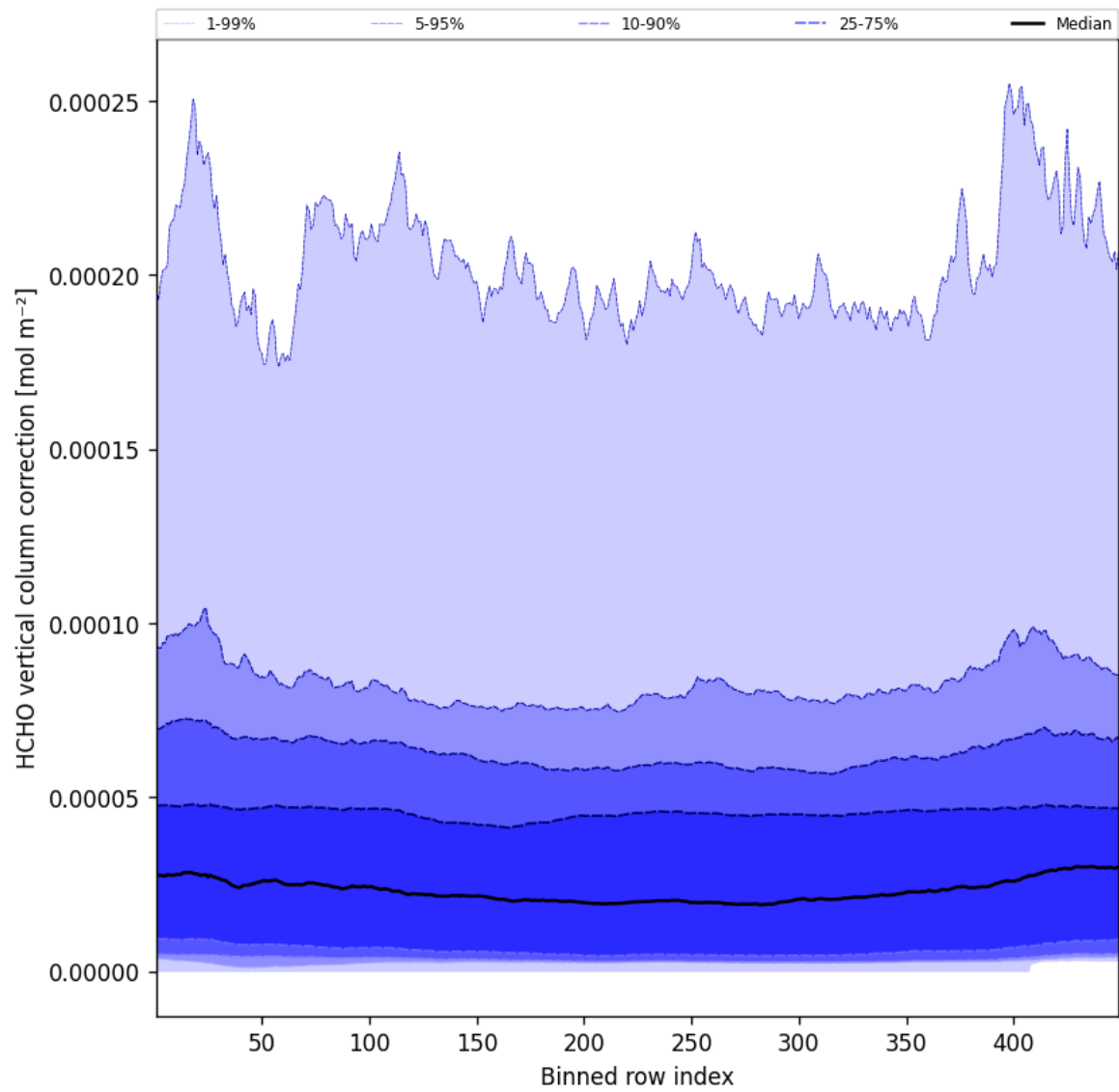
Figure 49: Along track statistics of “HCHO vertical column correction” for 2025-01-08 to 2025-01-09
