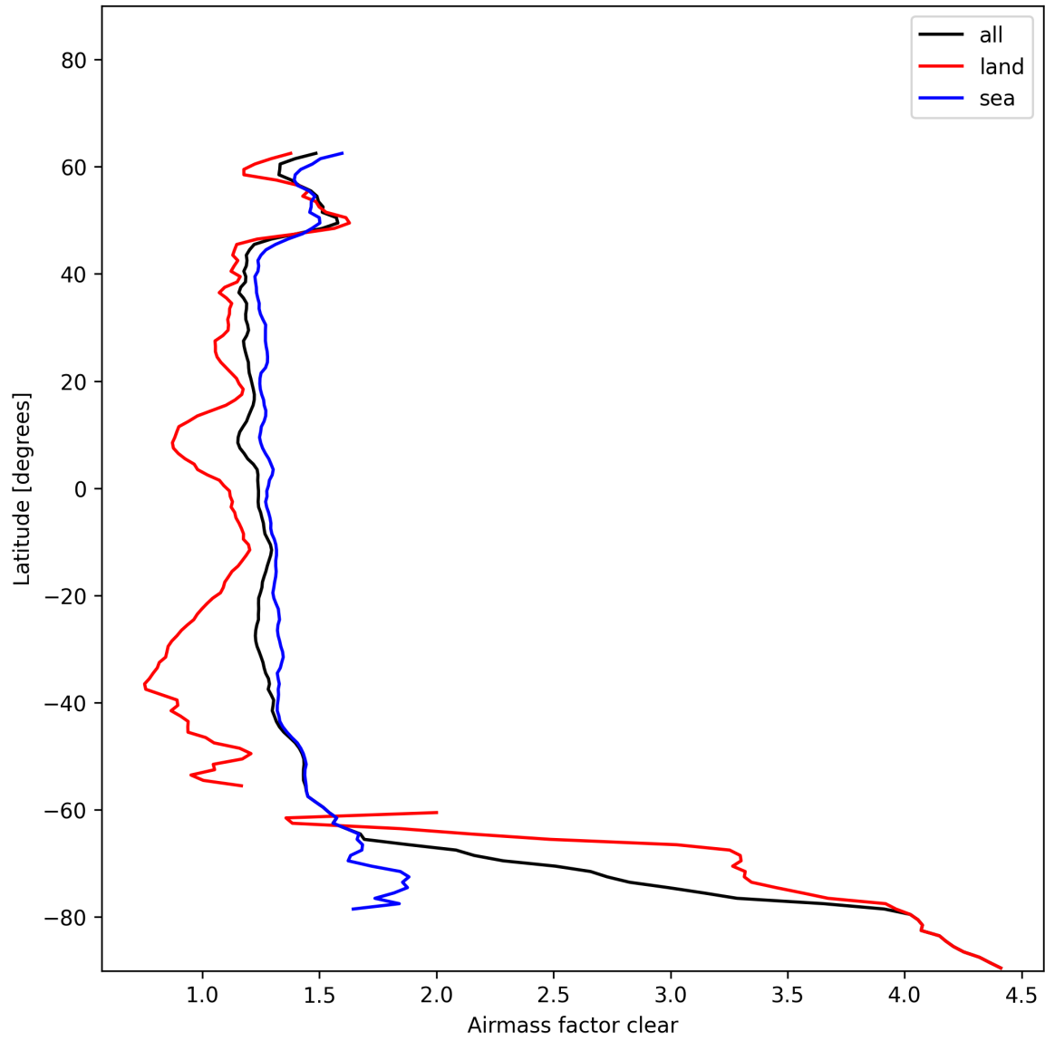
Figure 26: Zonal average of “Airmass factor clear” for 2025-01-08 to 2025-01-09.
