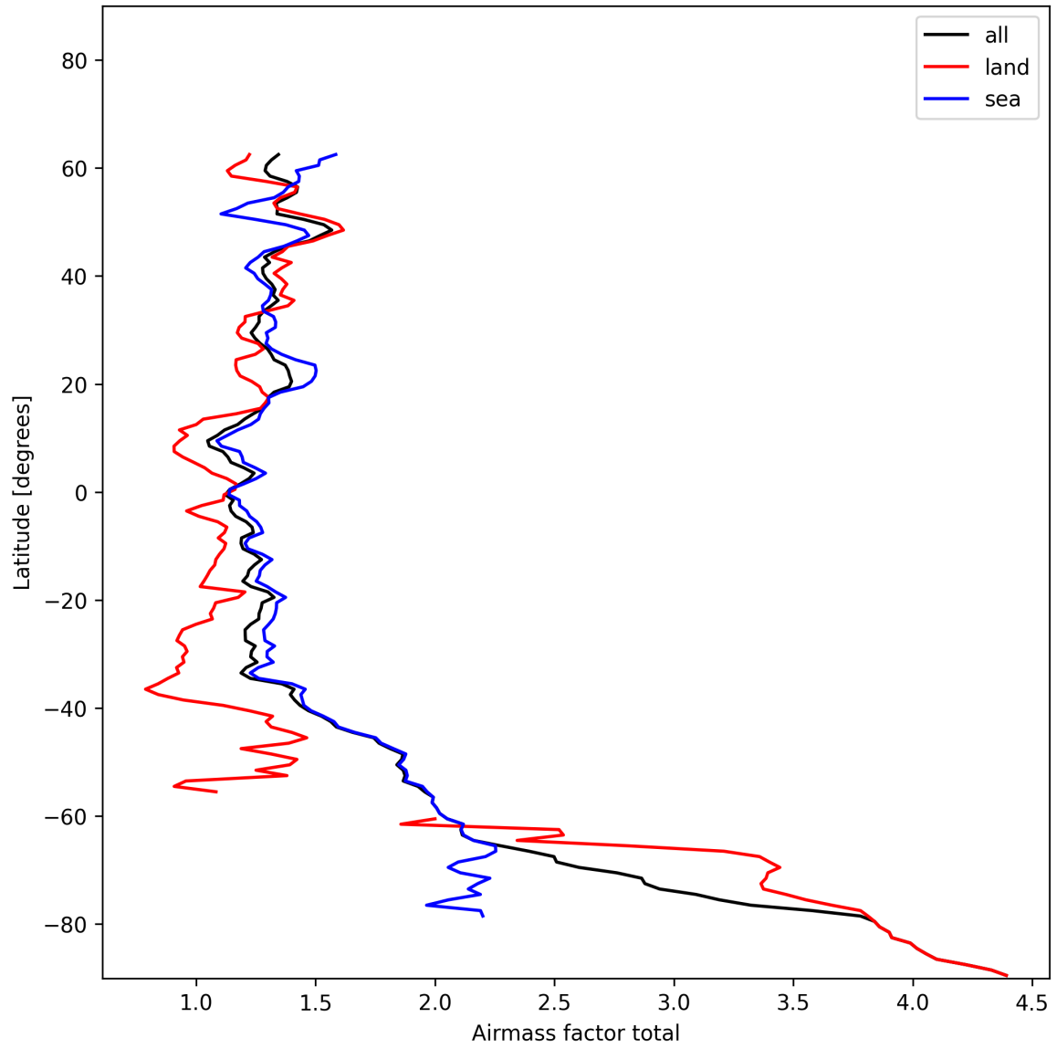
Figure 24: Zonal average of “Airmass factor total” for 2025-01-08 to 2025-01-09.
