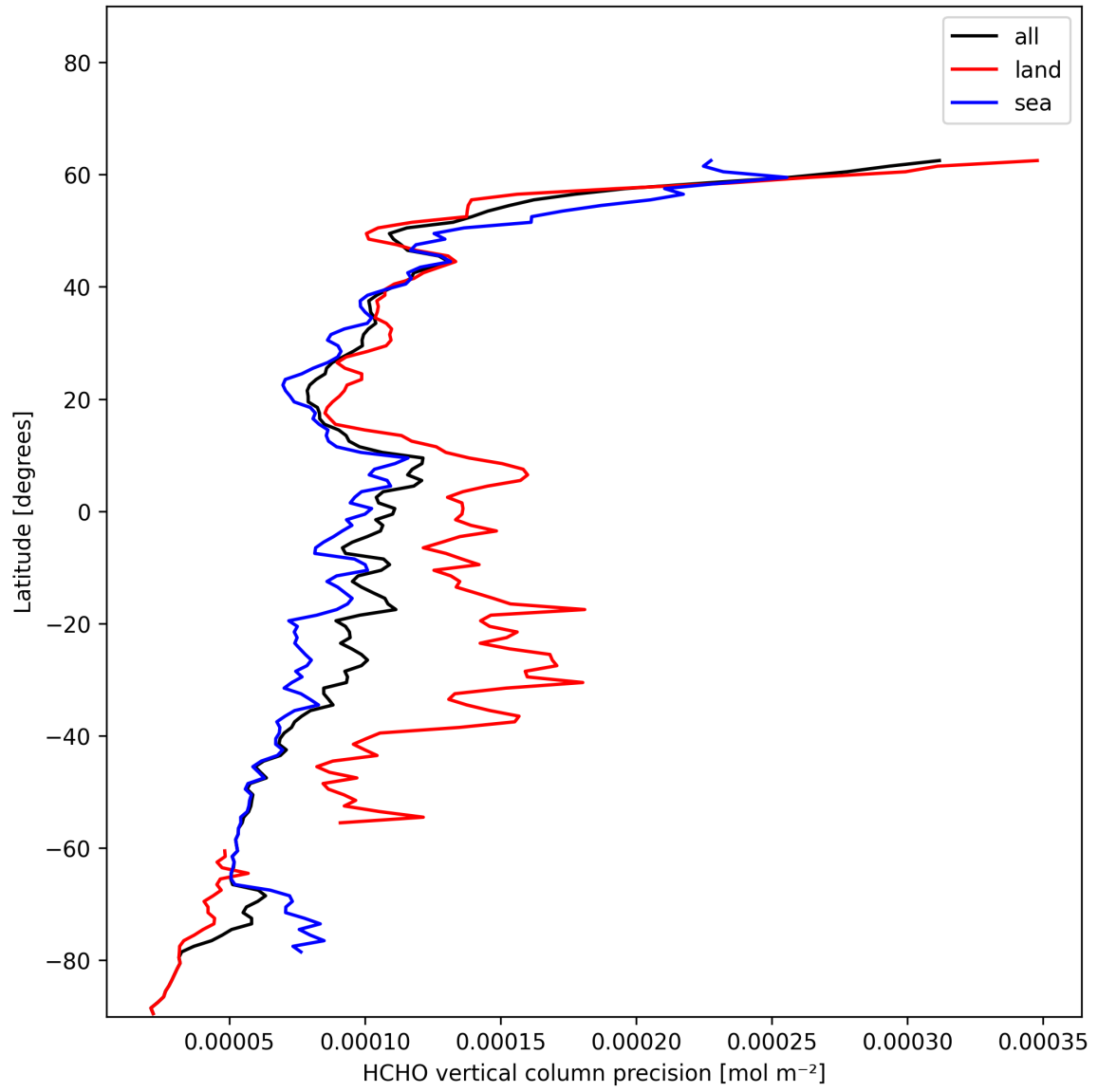
Figure 20: Zonal average of “HCHO vertical column precision” for 2025-01-08 to 2025-01-09.
