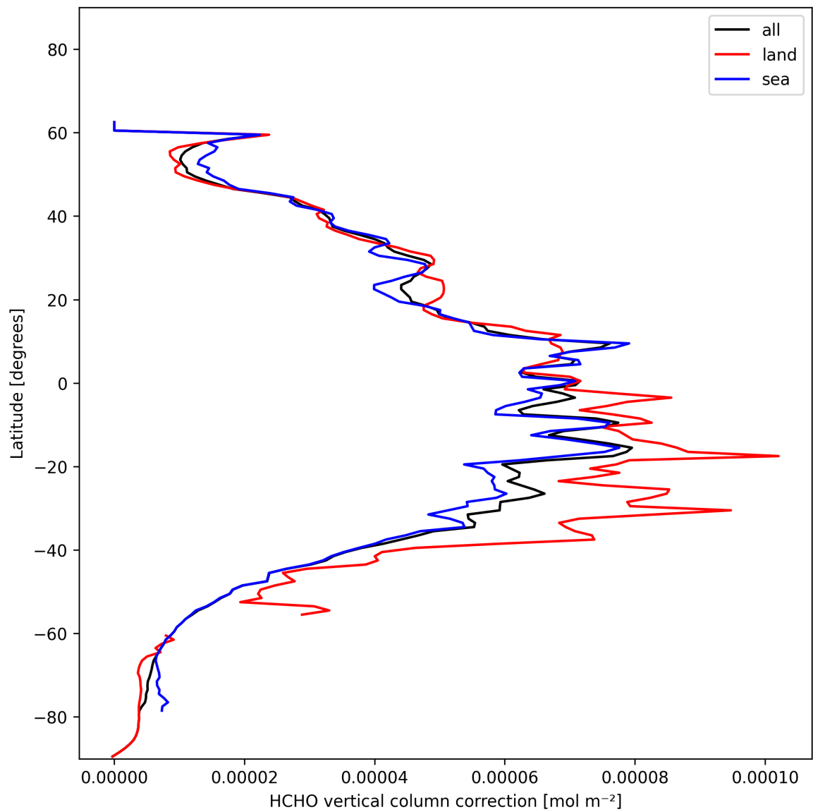
Figure 21: Zonal average of “HCHO vertical column correction” for 2025-01-08 to 2025-01-09.
