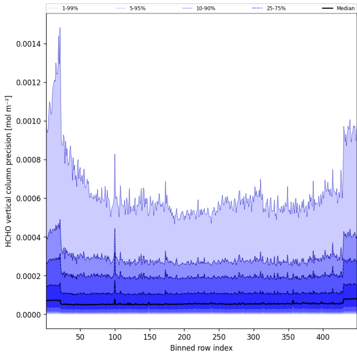
Figure 48: Along track statistics of “HCHO vertical column precision” for 2025-01-08 to 2025-01-09
