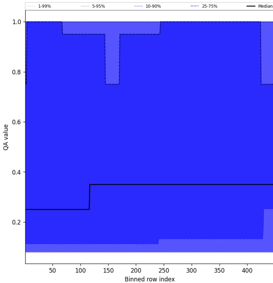
Figure 46: Along track statistics of “QA value” for 2025-01-08 to 2025-01-09
