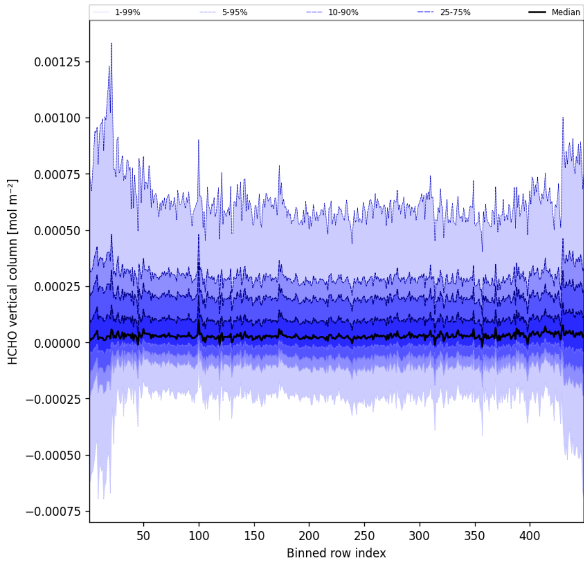
Figure 47: Along track statistics of “HCHO vertical column” for 2025-01-08 to 2025-01-09
