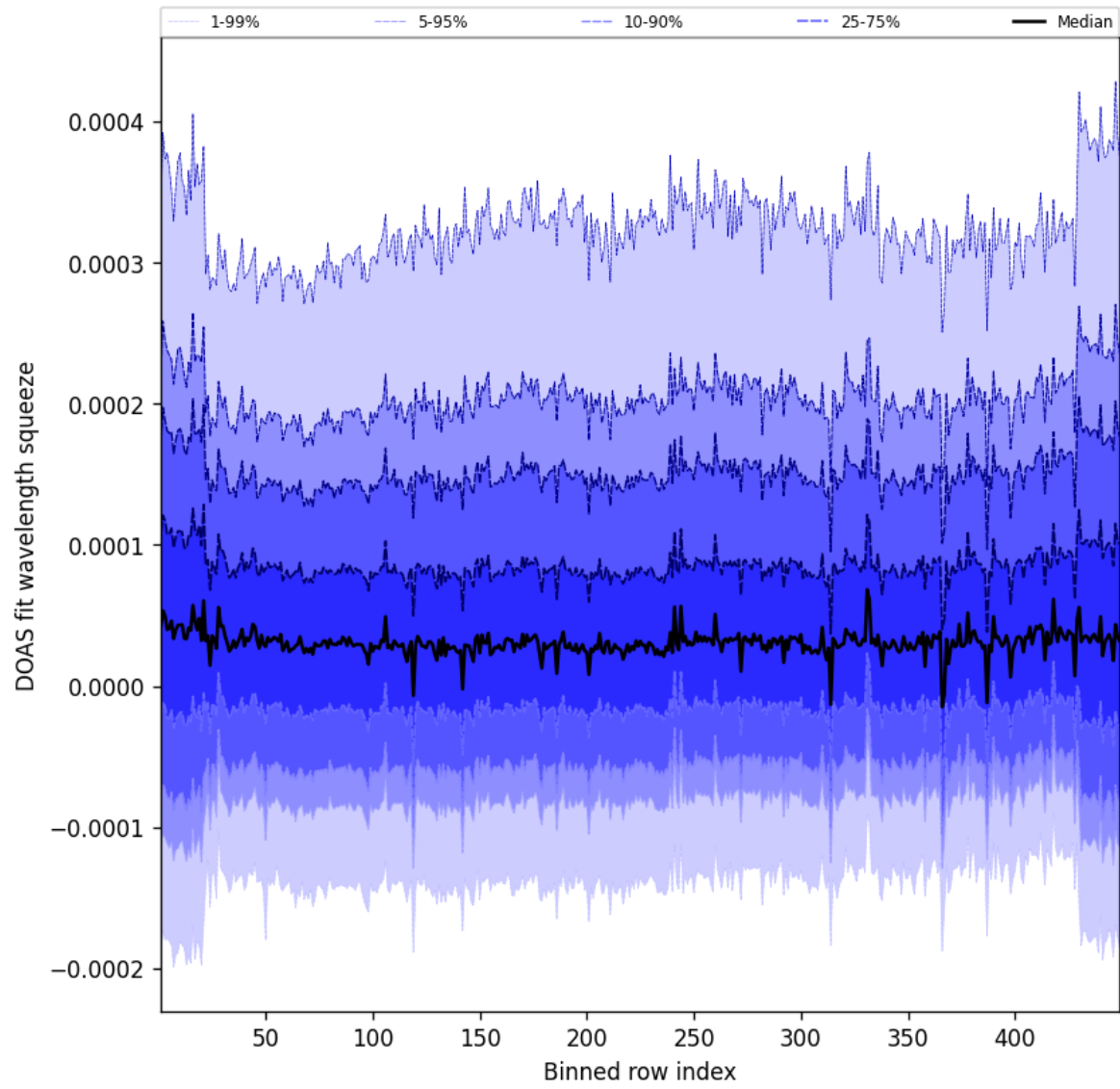
Figure 57: Along track statistics of “DOAS fit wavelength squeeze” for 2025-01-08 to 2025-01-09
