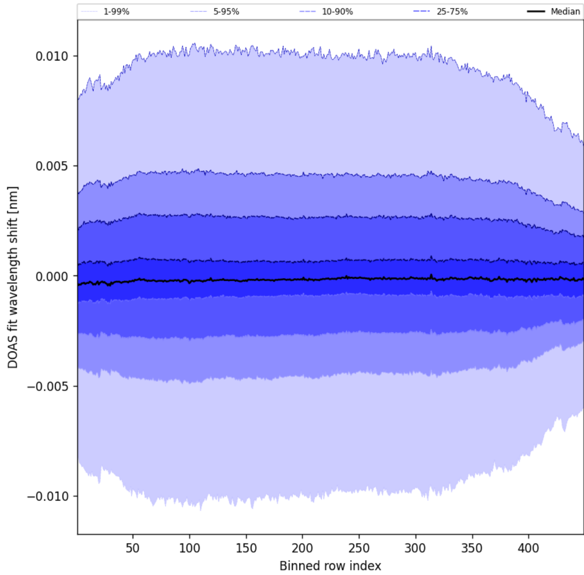
Figure 56: Along track statistics of “DOAS fit wavelength shift” for 2025-01-08 to 2025-01-09
