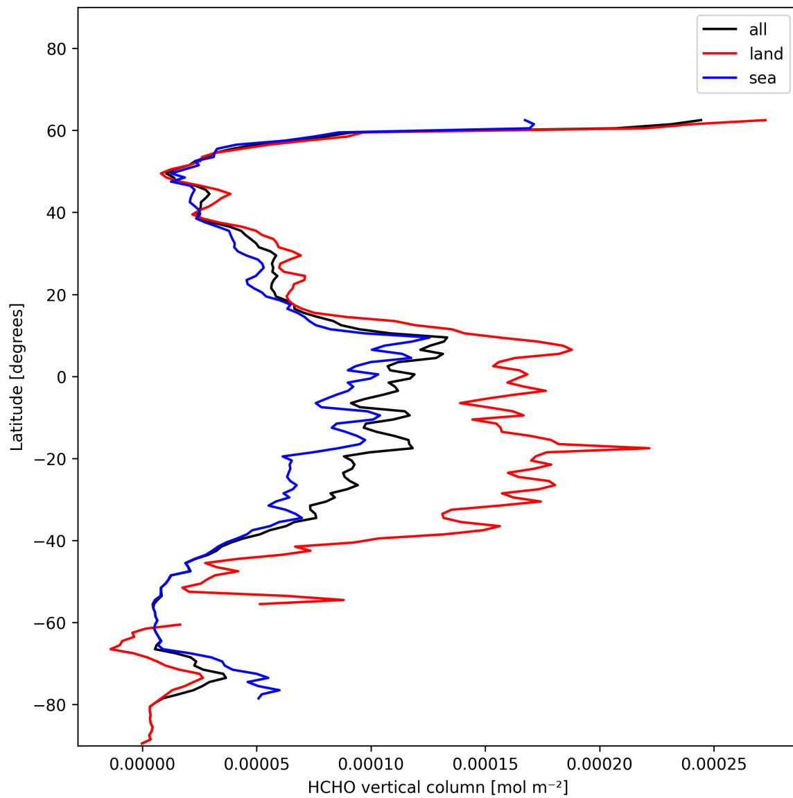
Figure 19: Zonal average of “HCHO vertical column” for 2025-01-08 to 2025-01-09.
