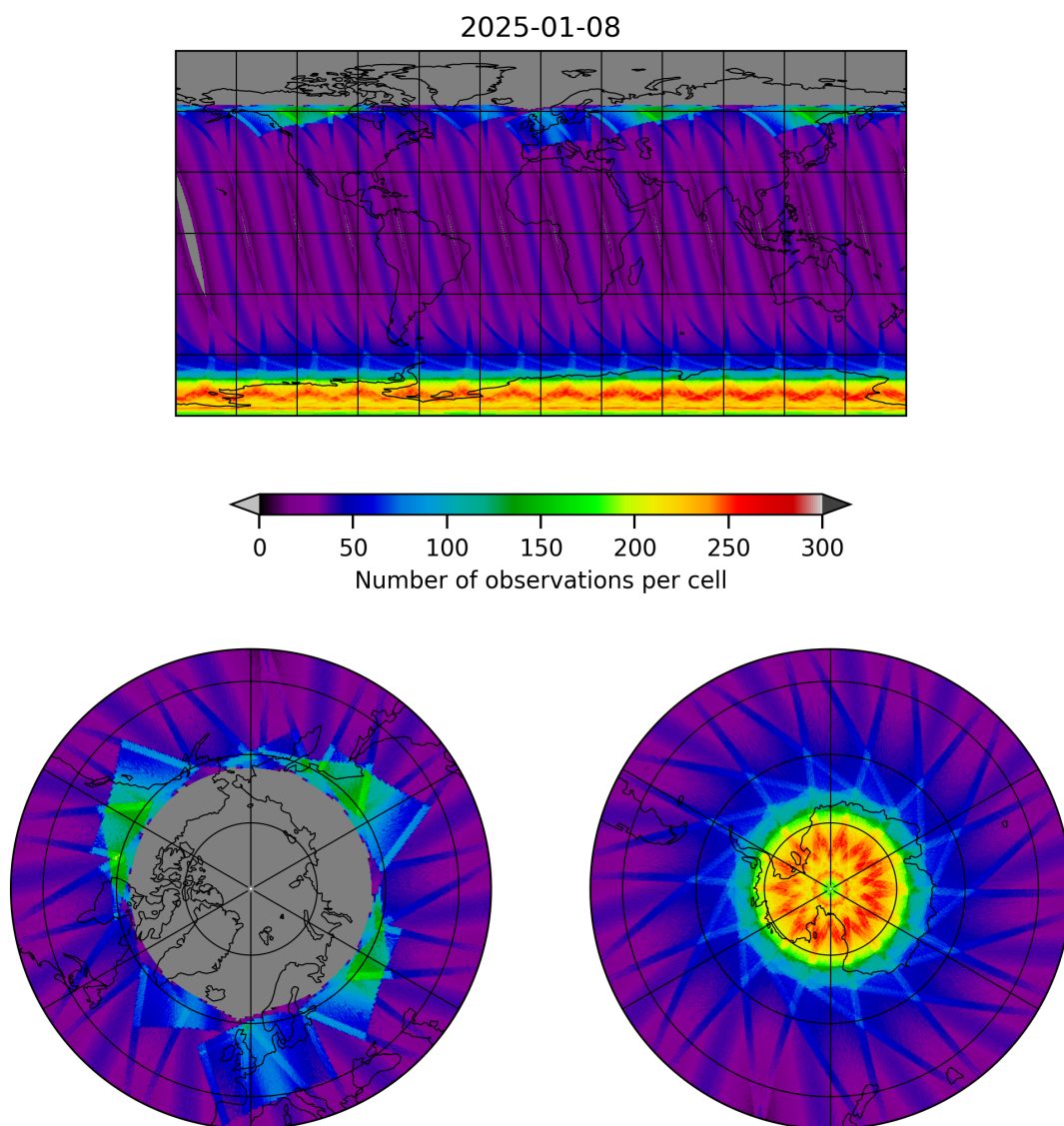
Figure 17: Map of the number of observations for 2025-01-08 to 2025-01-09
