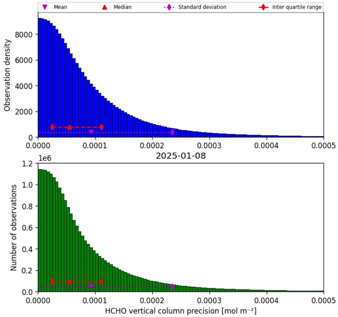
Figure 34: Histogram of “HCHO vertical column precision” for 2025-01-08 to 2025-01-09
