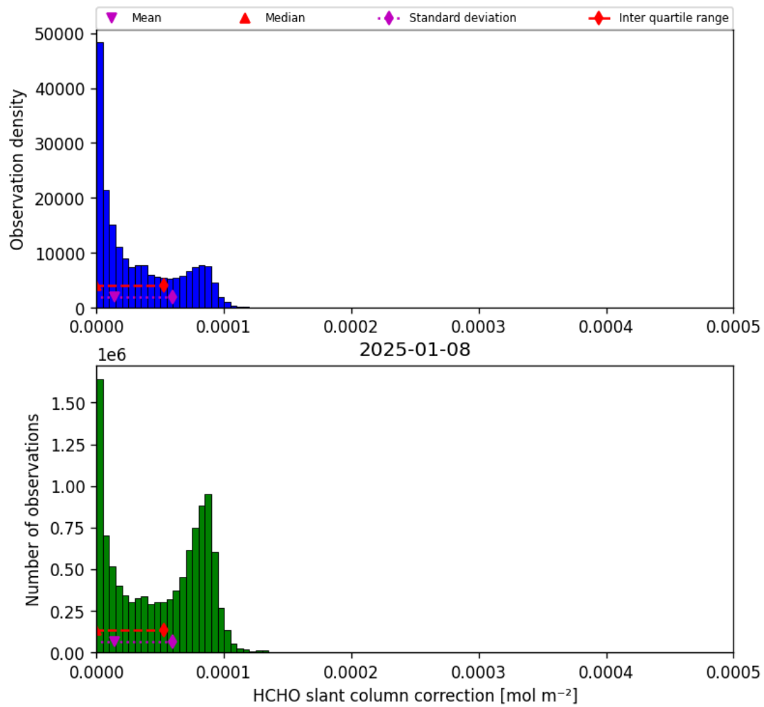
Figure 45: Histogram of “HCHO slant column correction” for 2025-01-08 to 2025-01-09
