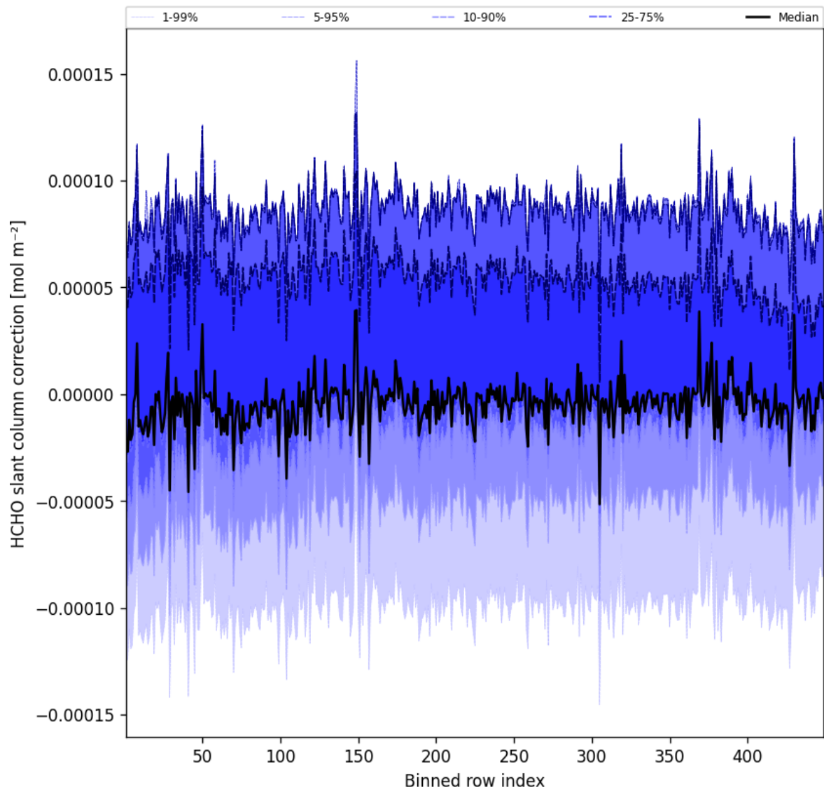
Figure 59: Along track statistics of “HCHO slant column correction” for 2025-01-08 to 2025-01-09
