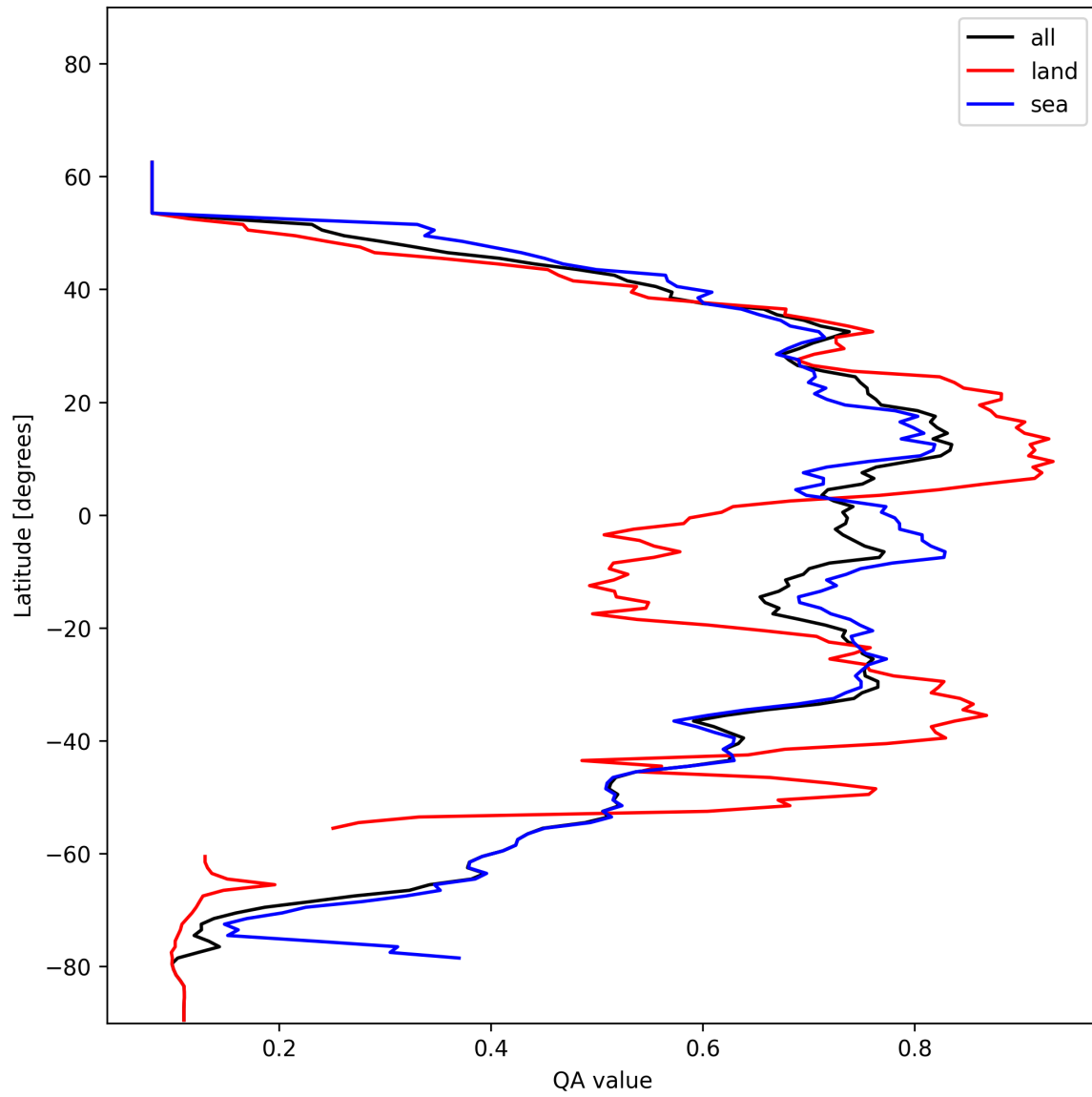
Figure 18: Zonal average of “QA value” for 2025-01-08 to 2025-01-09.
