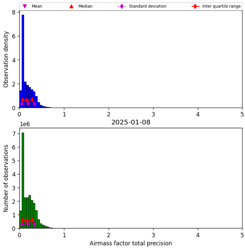
Figure 39: Histogram of “Airmass factor total precision” for 2025-01-08 to 2025-01-09
