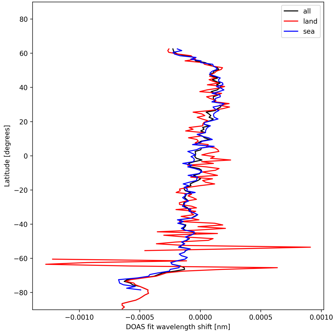
Figure 28: Zonal average of “DOAS fit wavelength shift” for 2025-01-08 to 2025-01-09.
