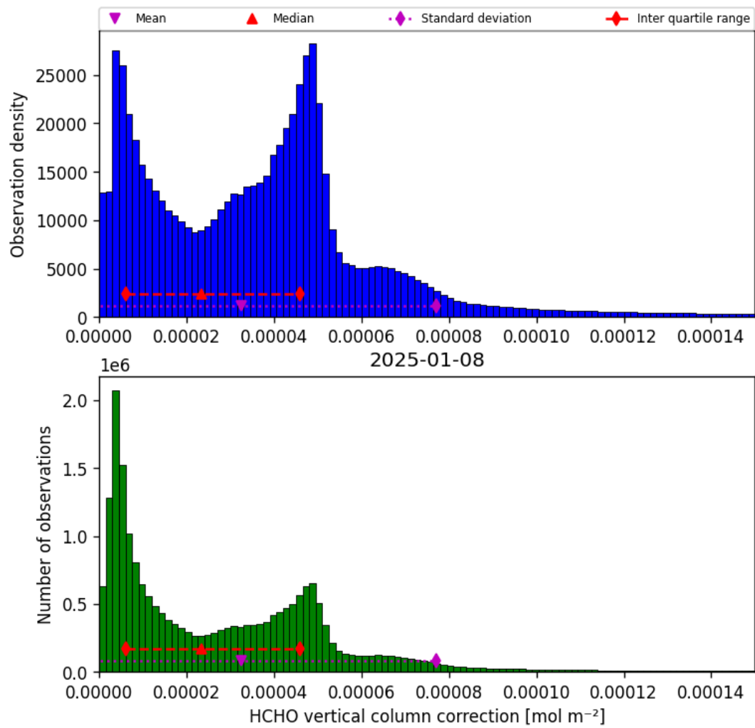
Figure 35: Histogram of “HCHO vertical column correction” for 2025-01-08 to 2025-01-09
