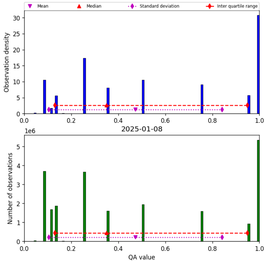
Figure 32: Histogram of “QA value” for 2025-01-08 to 2025-01-09
