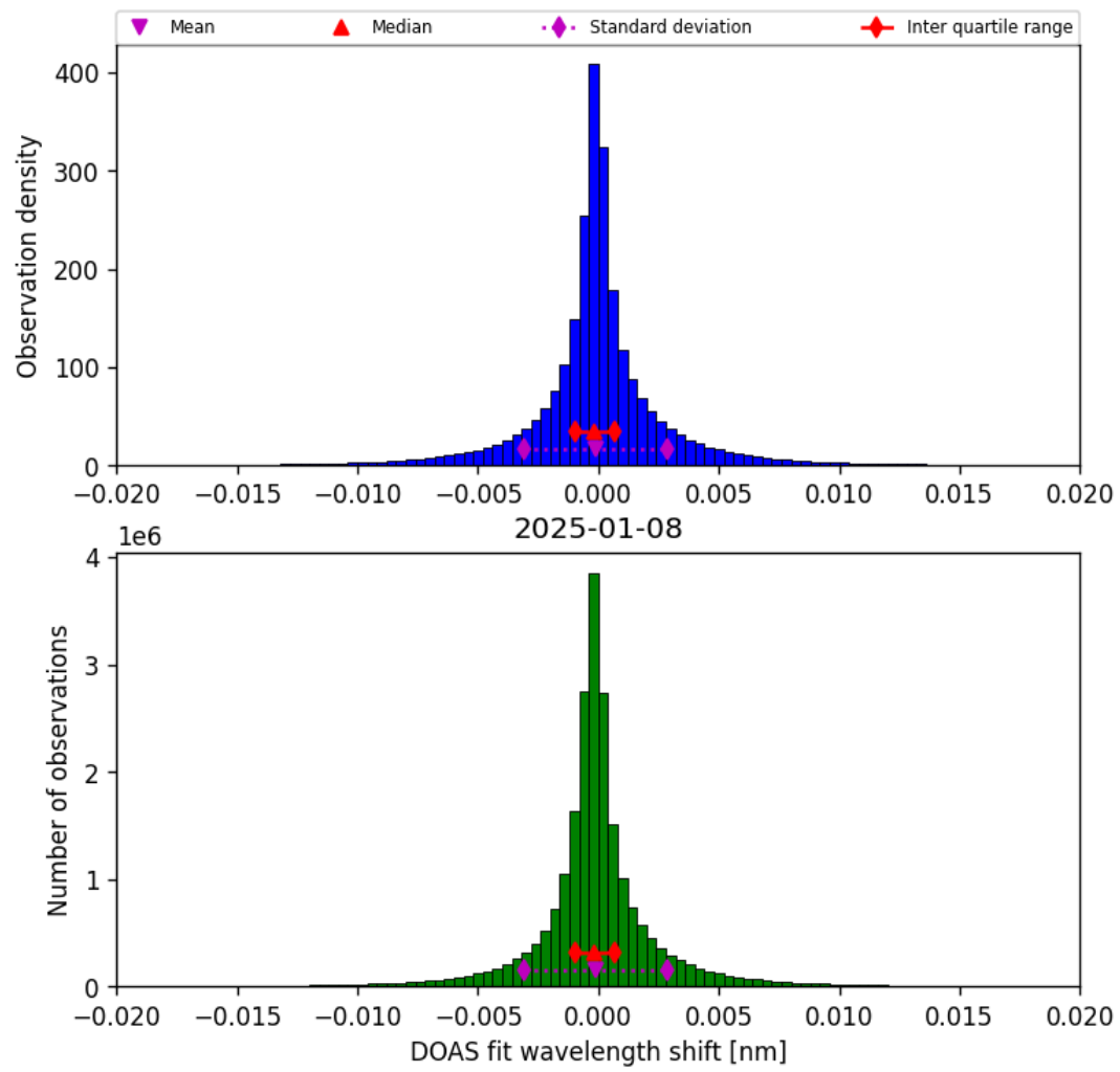
Figure 42: Histogram of “DOAS fit wavelength shift” for 2025-01-08 to 2025-01-09
