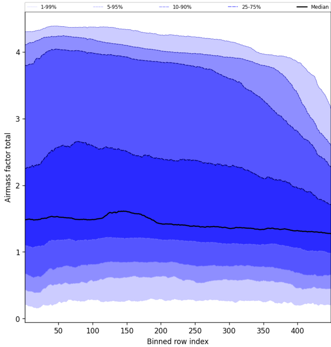
Figure 52: Along track statistics of “Airmass factor total” for 2025-01-08 to 2025-01-09
