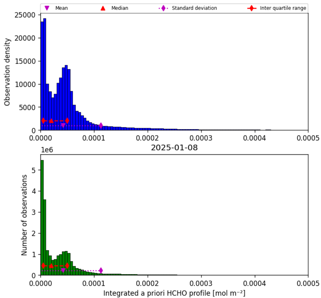
Figure 41: Histogram of “Integrated a priori HCHO profile” for 2025-01-08 to 2025-01-09
