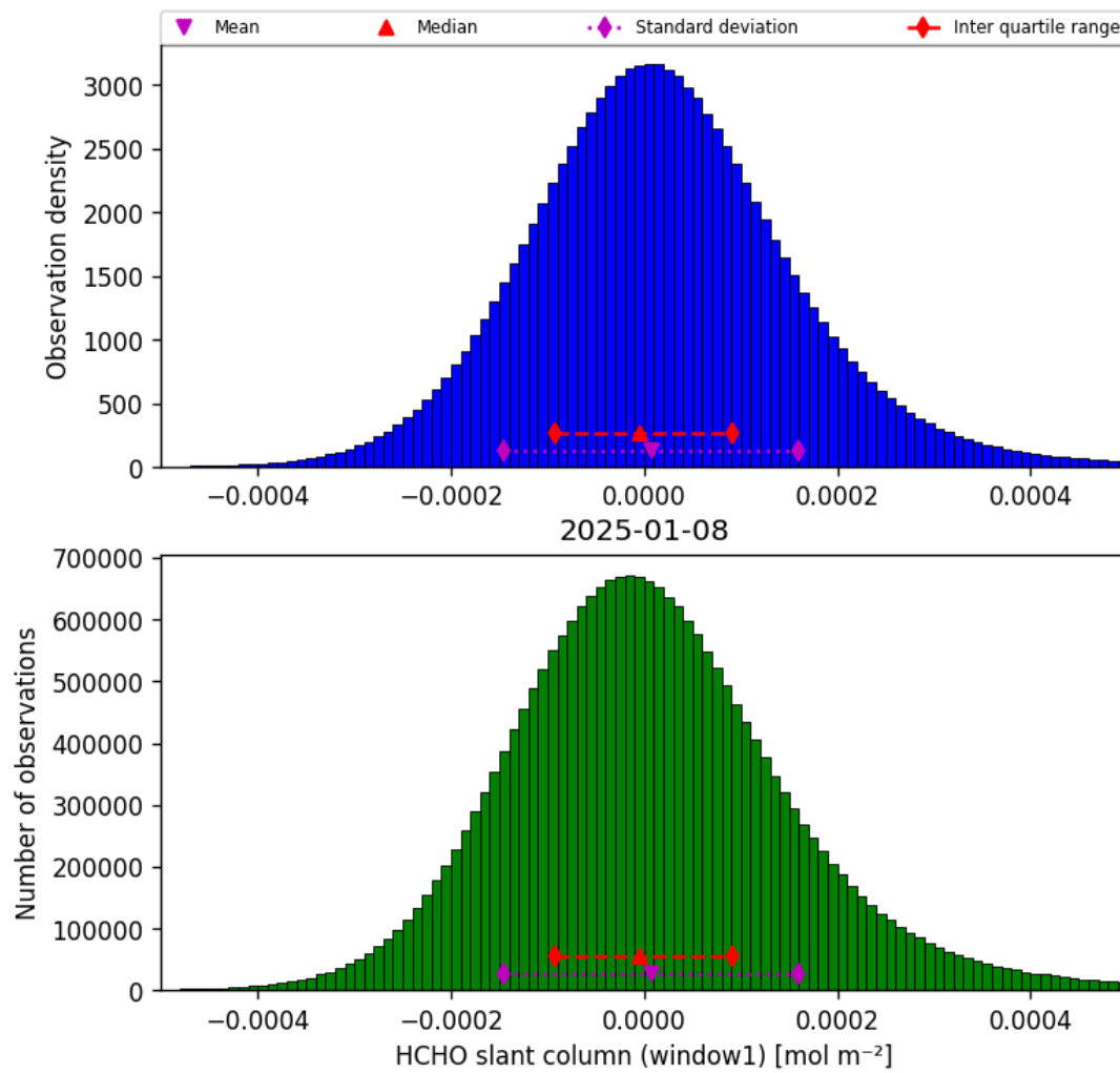
Figure 36: Histogram of “HCHO slant column (window1)” for 2025-01-08 to 2025-01-09
