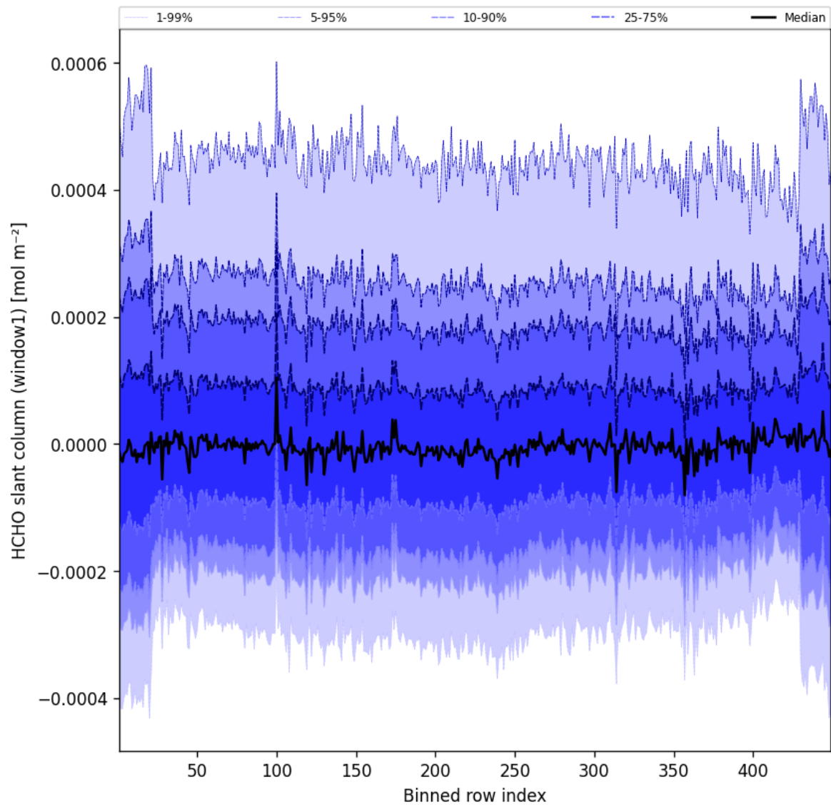
Figure 50: Along track statistics of “HCHO slant column (window1)” for 2025-01-09 to 2025-01-10
