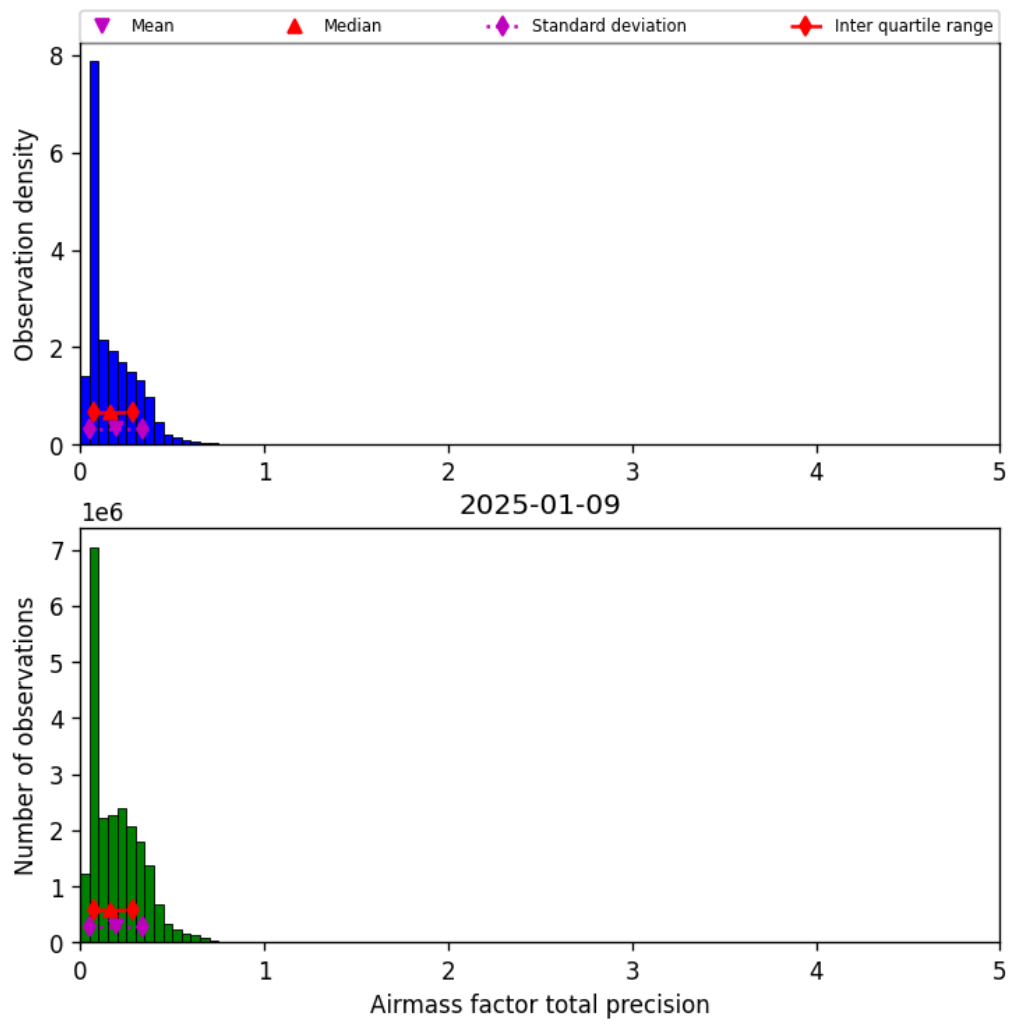
Figure 39: Histogram of “Airmass factor total precision” for 2025-01-09 to 2025-01-10
