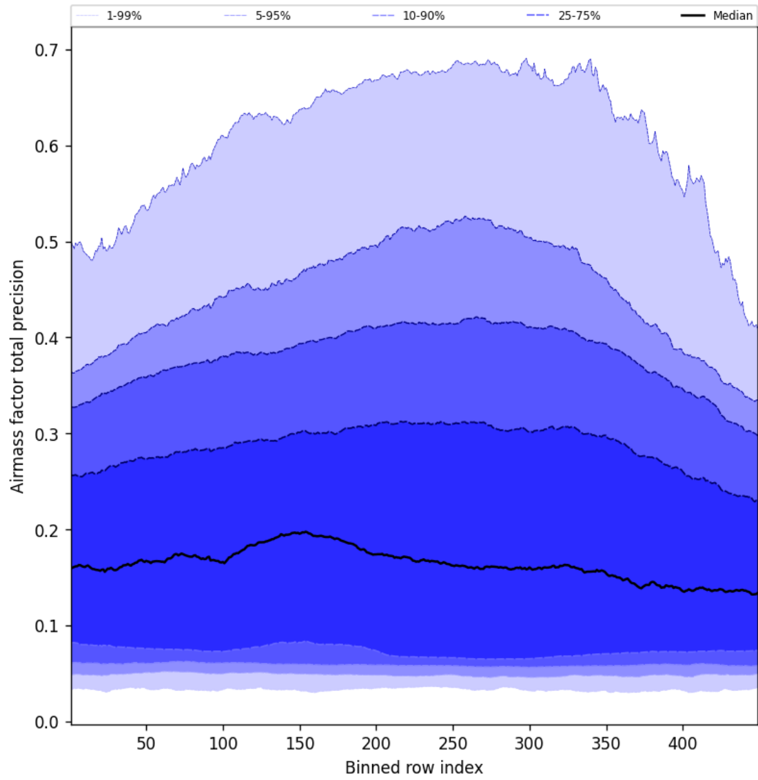
Figure 53: Along track statistics of “Airmass factor total precision” for 2025-01-09 to 2025-01-10
