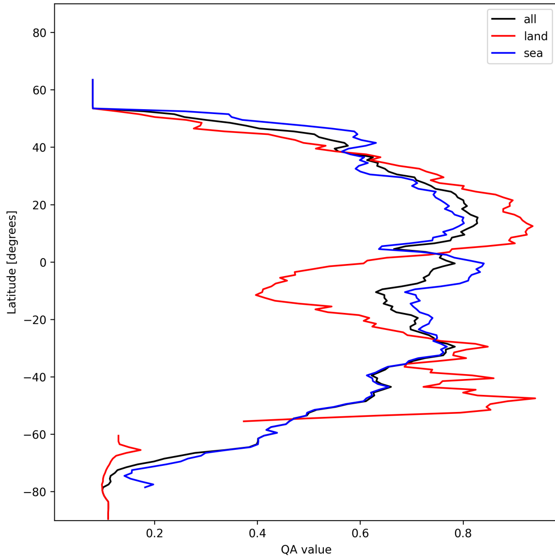
Figure 18: Zonal average of “QA value” for 2025-01-09 to 2025-01-10.
