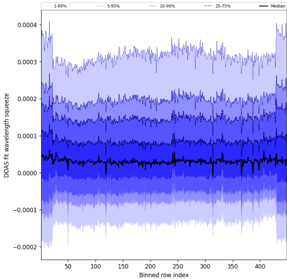
Figure 57: Along track statistics of “DOAS fit wavelength squeeze” for 2025-01-09 to 2025-01-10
