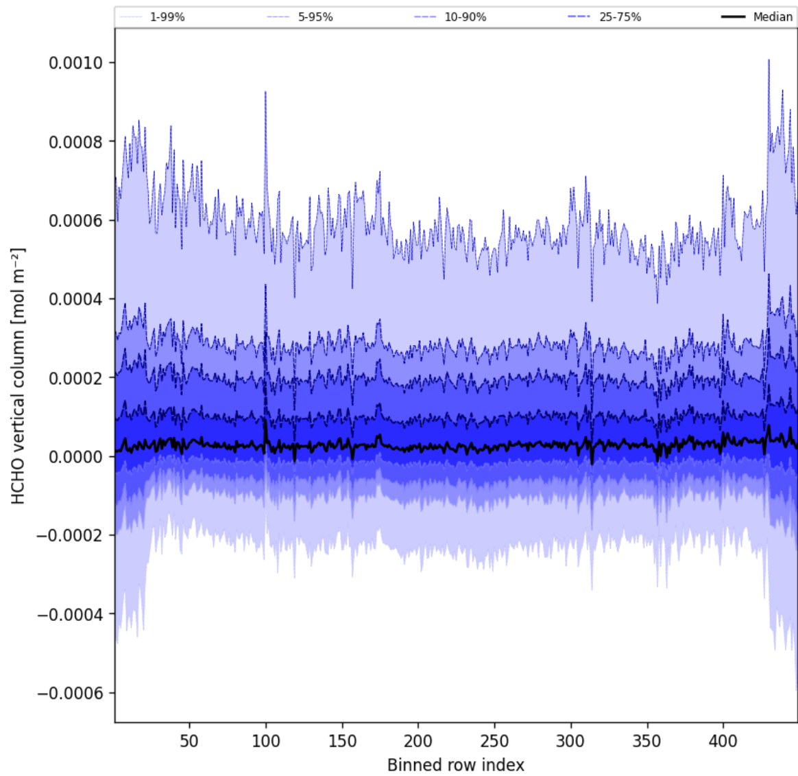
Figure 47: Along track statistics of “HCHO vertical column” for 2025-01-09 to 2025-01-10
