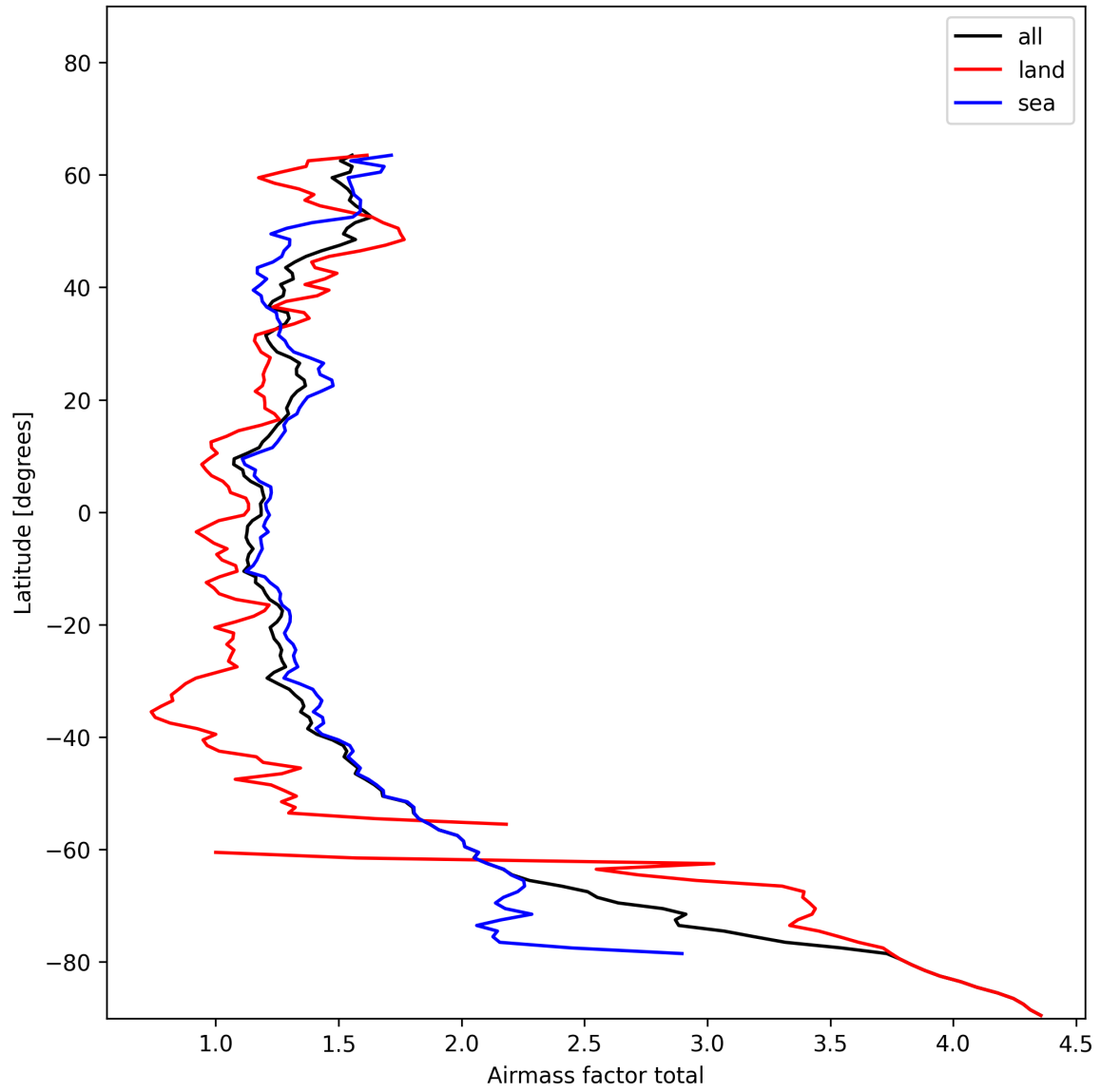
Figure 24: Zonal average of “Airmass factor total” for 2025-01-09 to 2025-01-10.
