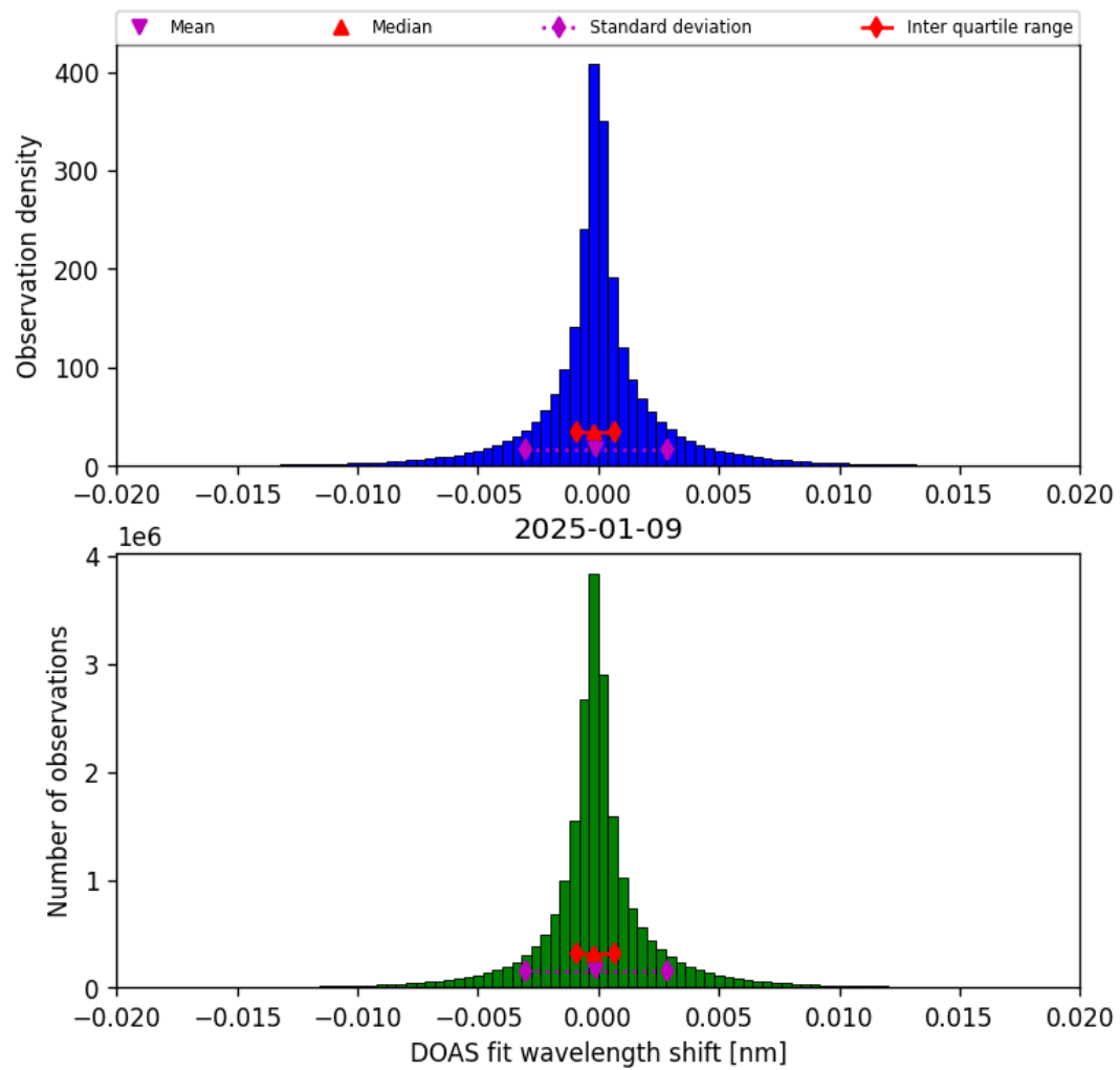
Figure 42: Histogram of “DOAS fit wavelength shift” for 2025-01-09 to 2025-01-10
