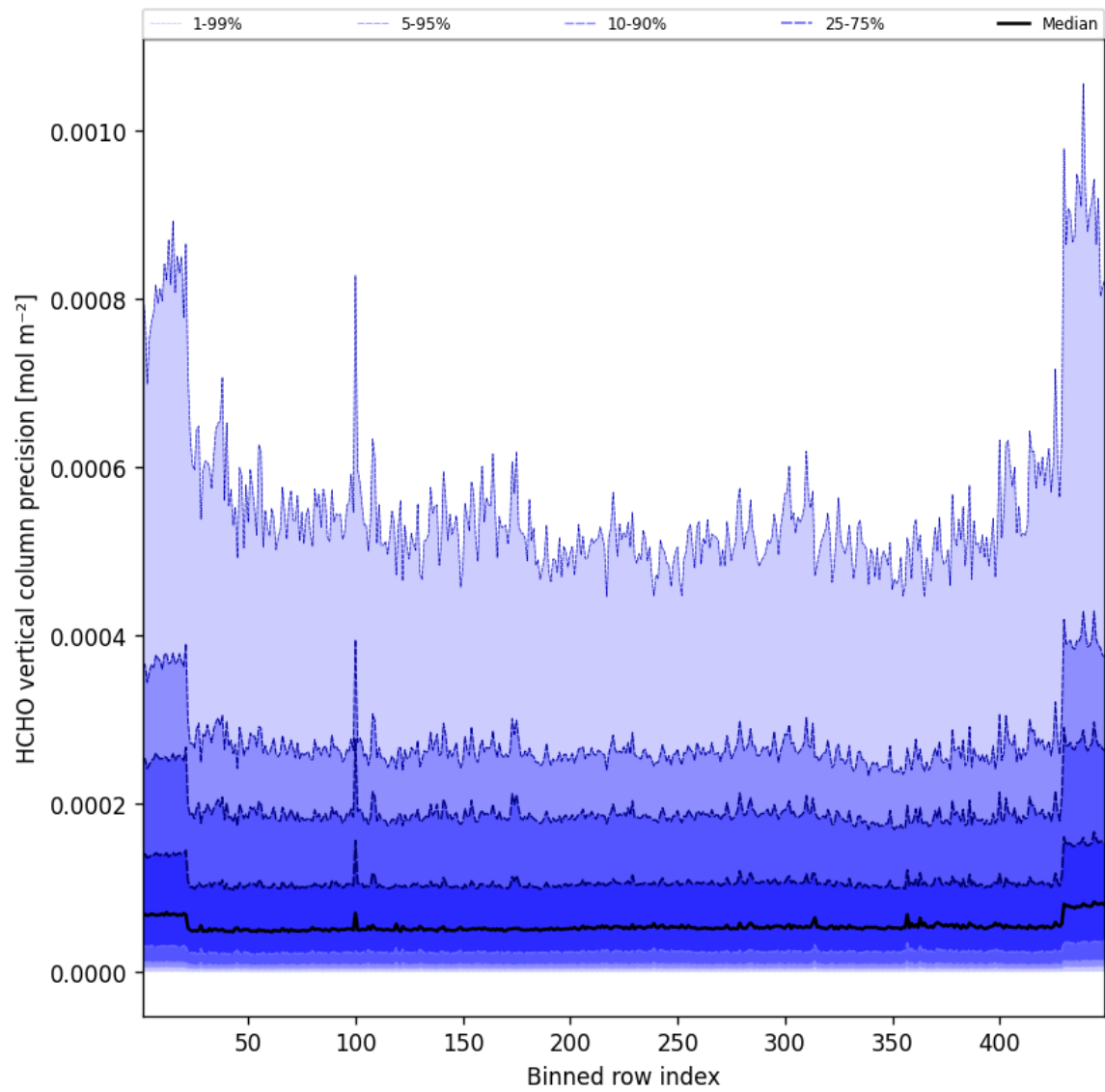
Figure 48: Along track statistics of “HCHO vertical column precision” for 2025-01-09 to 2025-01-10
