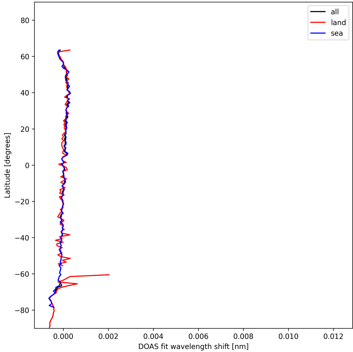
Figure 28: Zonal average of “DOAS fit wavelength shift” for 2025-01-09 to 2025-01-10.
