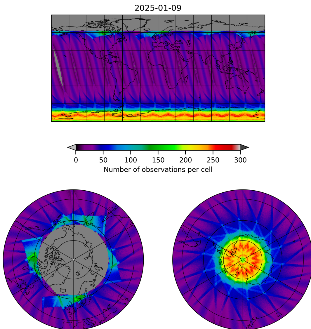
Figure 17: Map of the number of observations for 2025-01-09 to 2025-01-10
