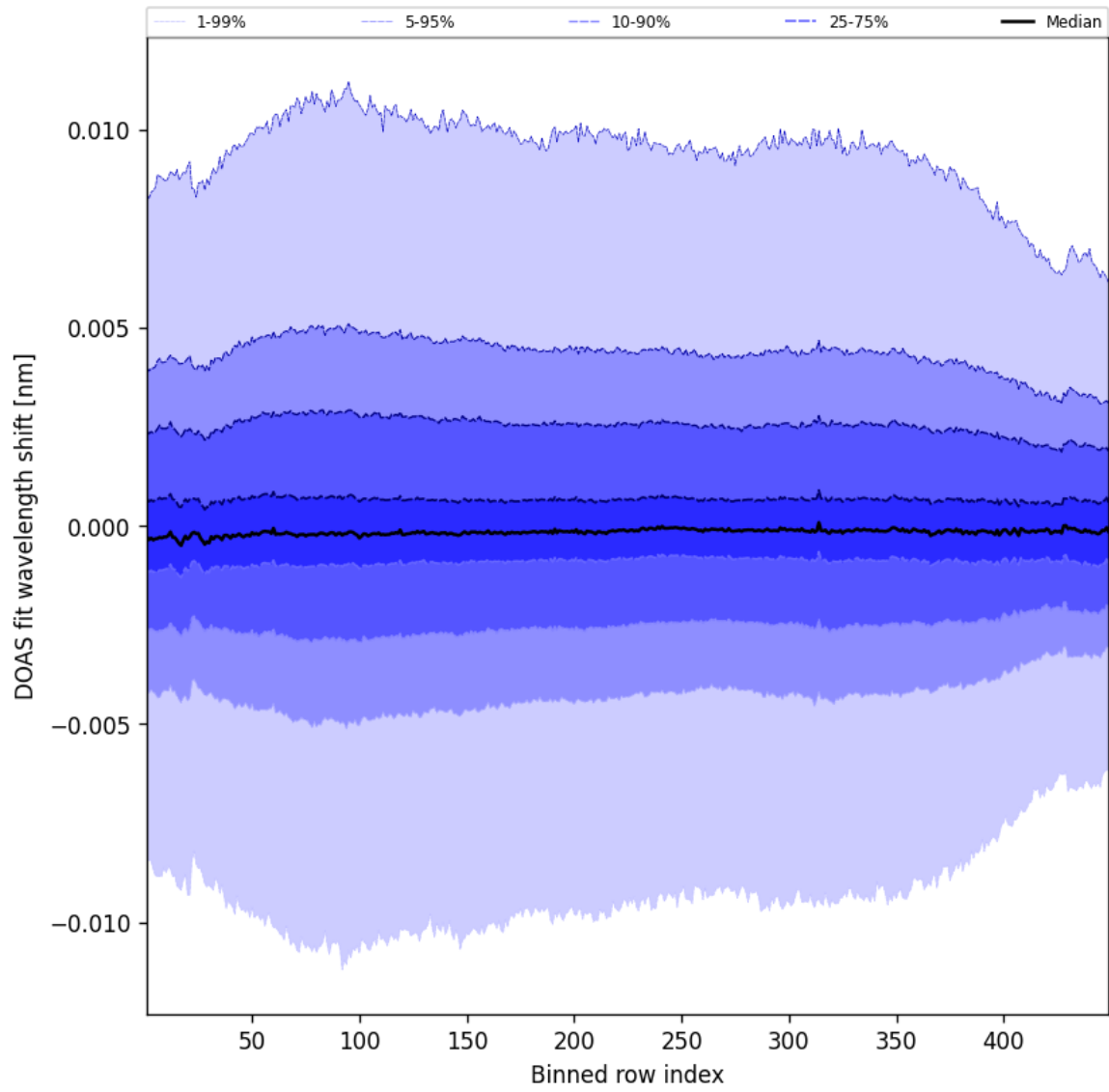
Figure 56: Along track statistics of “DOAS fit wavelength shift” for 2025-01-09 to 2025-01-10
