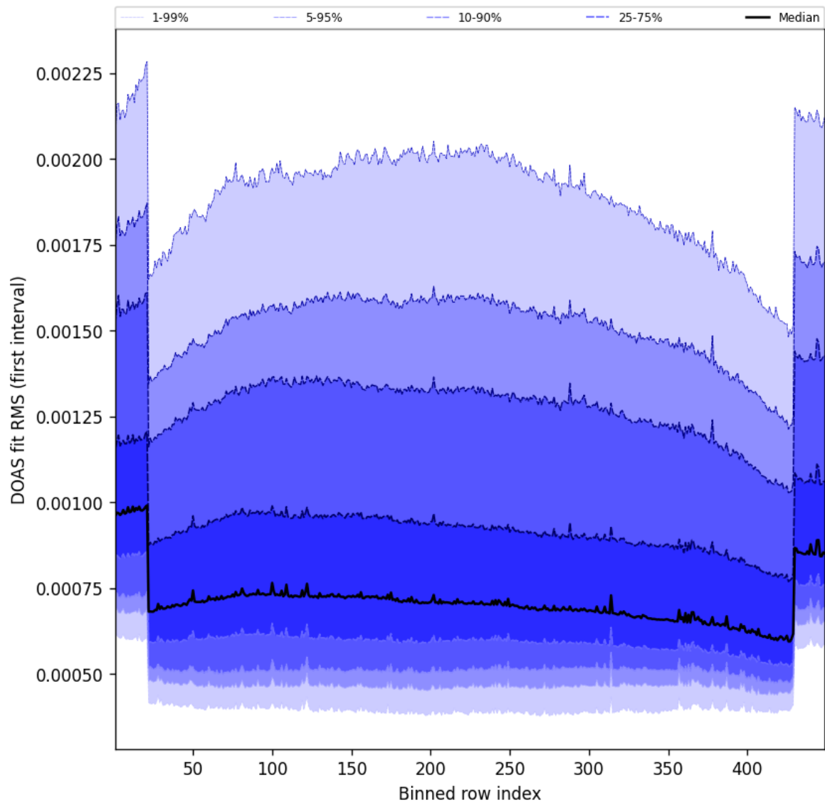
Figure 58: Along track statistics of “DOAS fit RMS (first interval)” for 2025-01-09 to 2025-01-10
