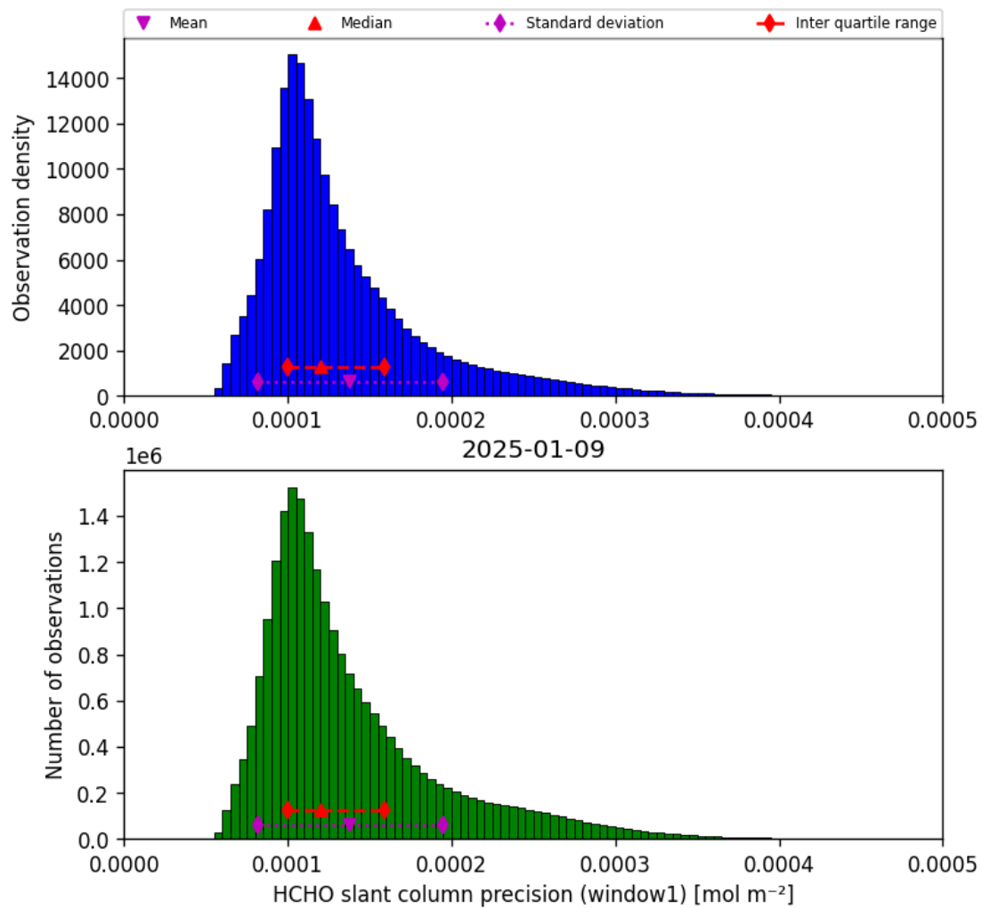
Figure 37: Histogram of “HCHO slant column precision (window1)” for 2025-01-09 to 2025-01-10
