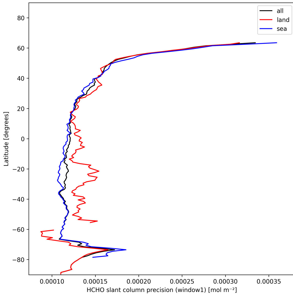
Figure 23: Zonal average of “HCHO slant column precision (window1)” for 2025-01-09 to 2025-01-10.
