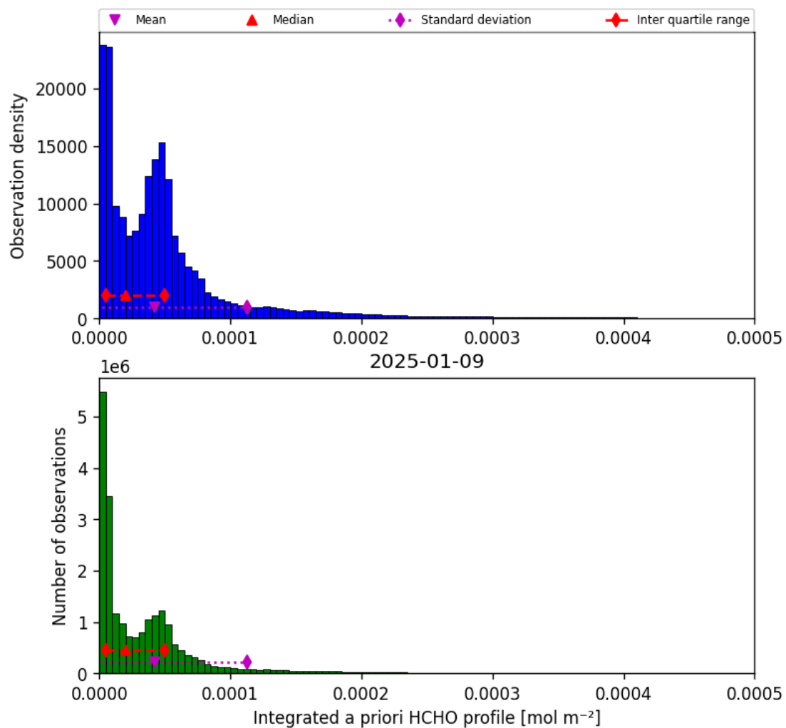
Figure 41: Histogram of “Integrated a priori HCHO profile” for 2025-01-09 to 2025-01-10
