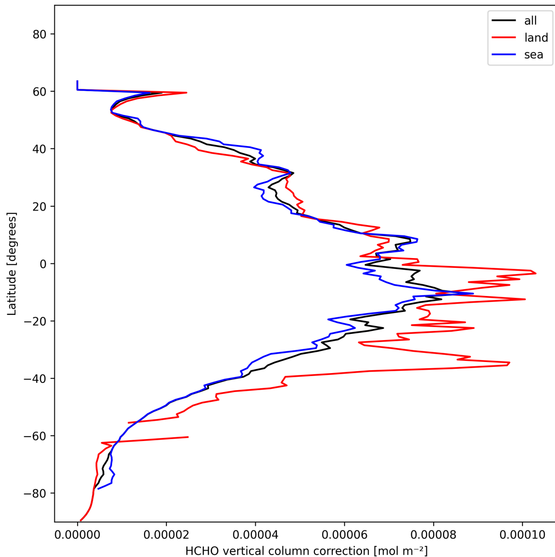
Figure 21: Zonal average of “HCHO vertical column correction” for 2025-01-09 to 2025-01-10.
