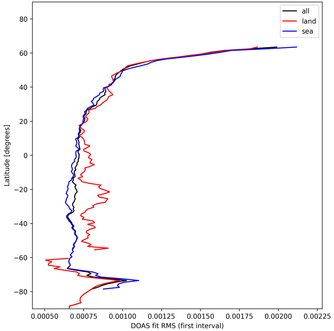
Figure 30: Zonal average of “DOAS fit RMS (first interval)” for 2025-01-09 to 2025-01-10.
