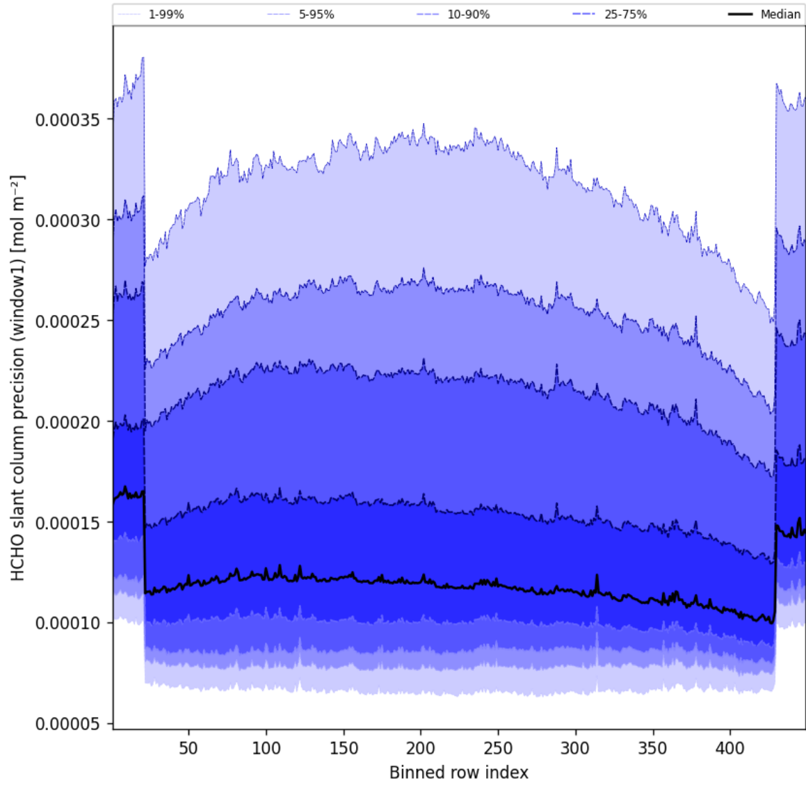
Figure 51: Along track statistics of “HCHO slant column precision (window1)” for 2025-01-09 to 2025-01-10
