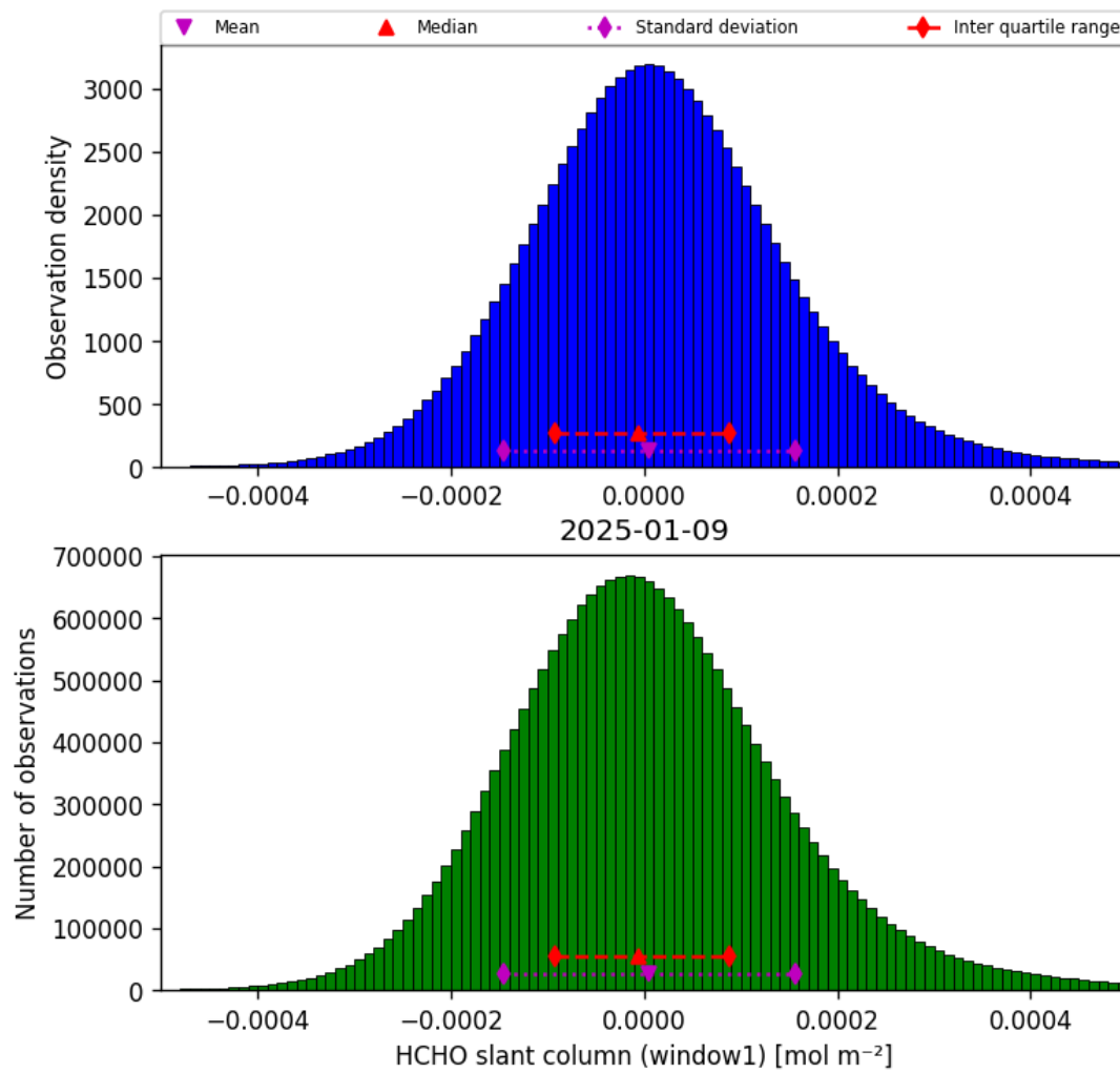
Figure 36: Histogram of “HCHO slant column (window1)” for 2025-01-09 to 2025-01-10
