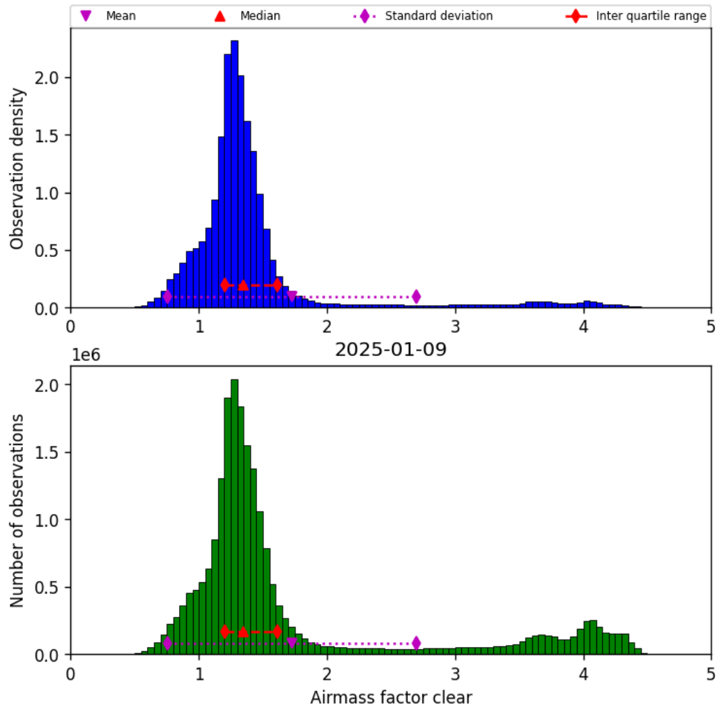
Figure 40: Histogram of “Airmass factor clear” for 2025-01-09 to 2025-01-10
