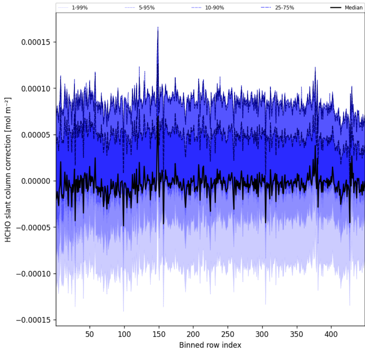
Figure 59: Along track statistics of “HCHO slant column correction” for 2025-01-09 to 2025-01-10
