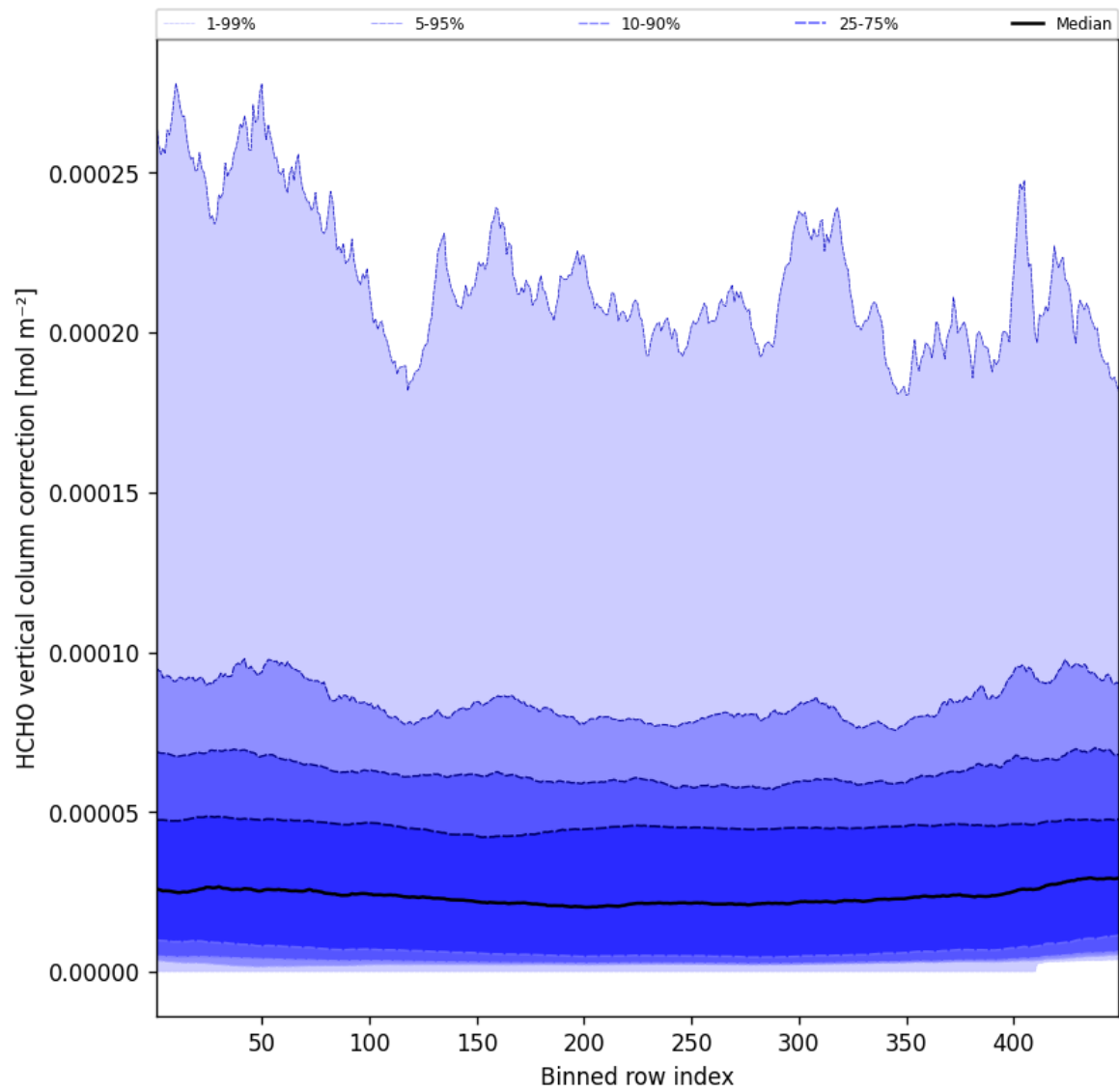
Figure 49: Along track statistics of “HCHO vertical column correction” for 2025-01-09 to 2025-01-10
