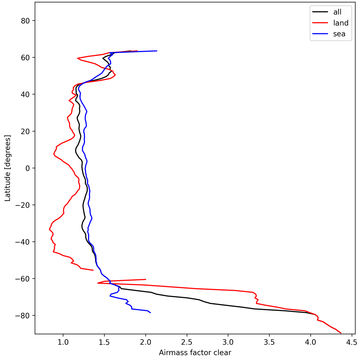
Figure 26: Zonal average of “Airmass factor clear” for 2025-01-09 to 2025-01-10.
