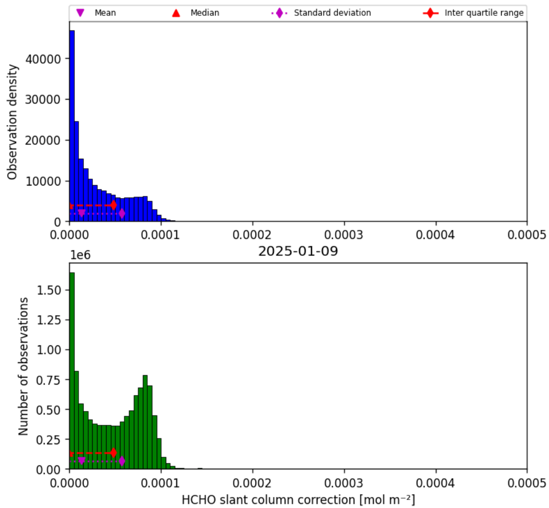
Figure 45: Histogram of “HCHO slant column correction” for 2025-01-09 to 2025-01-10
