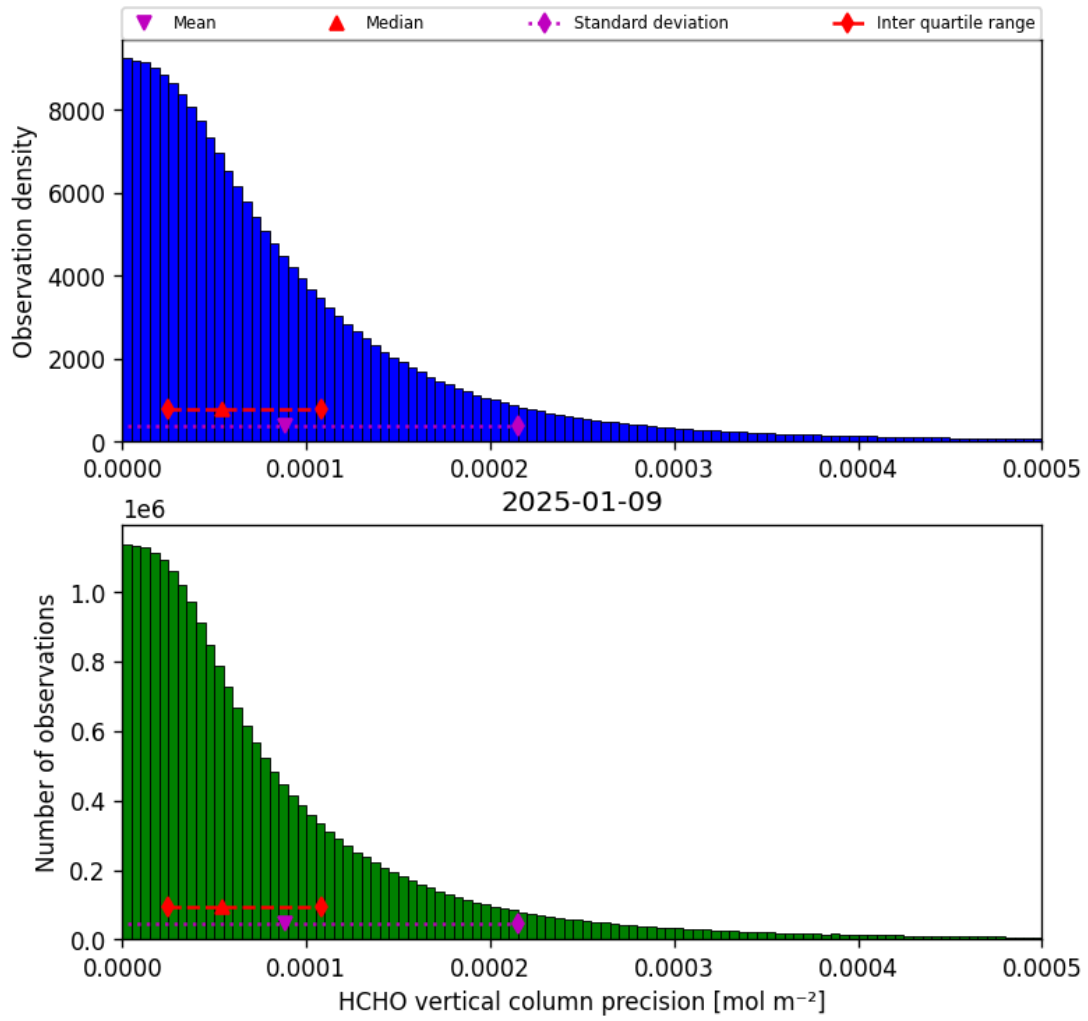
Figure 34: Histogram of “HCHO vertical column precision” for 2025-01-09 to 2025-01-10
