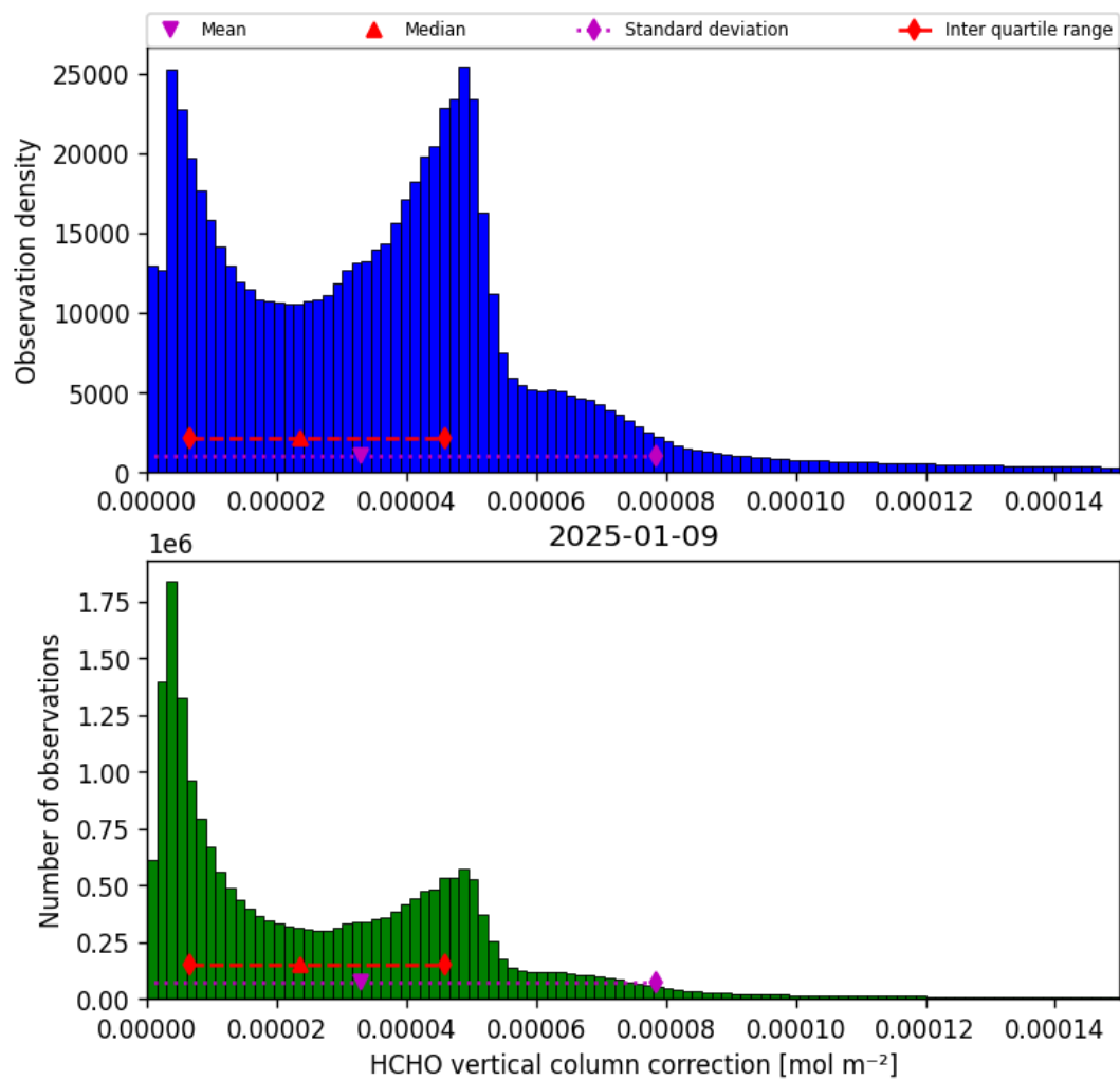
Figure 35: Histogram of “HCHO vertical column correction” for 2025-01-09 to 2025-01-10
