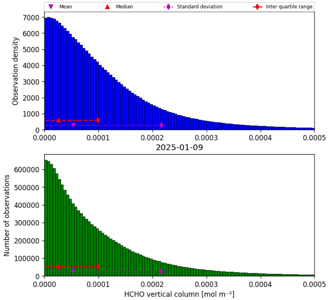
Figure 33: Histogram of “HCHO vertical column” for 2025-01-09 to 2025-01-10
