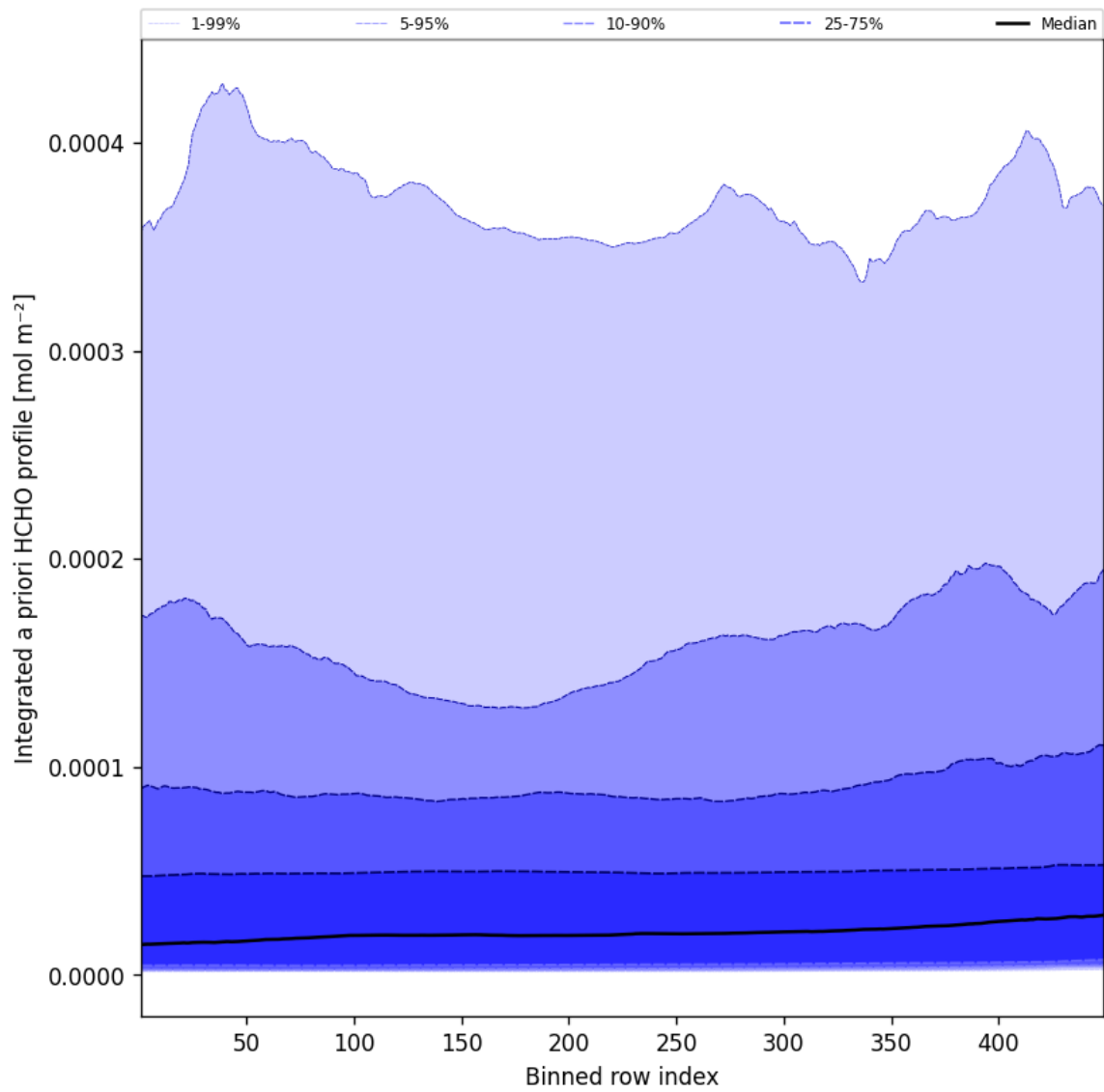
Figure 55: Along track statistics of "Integrated a priori HCHO profile" for 2025-01-09 to 2025-01-10
