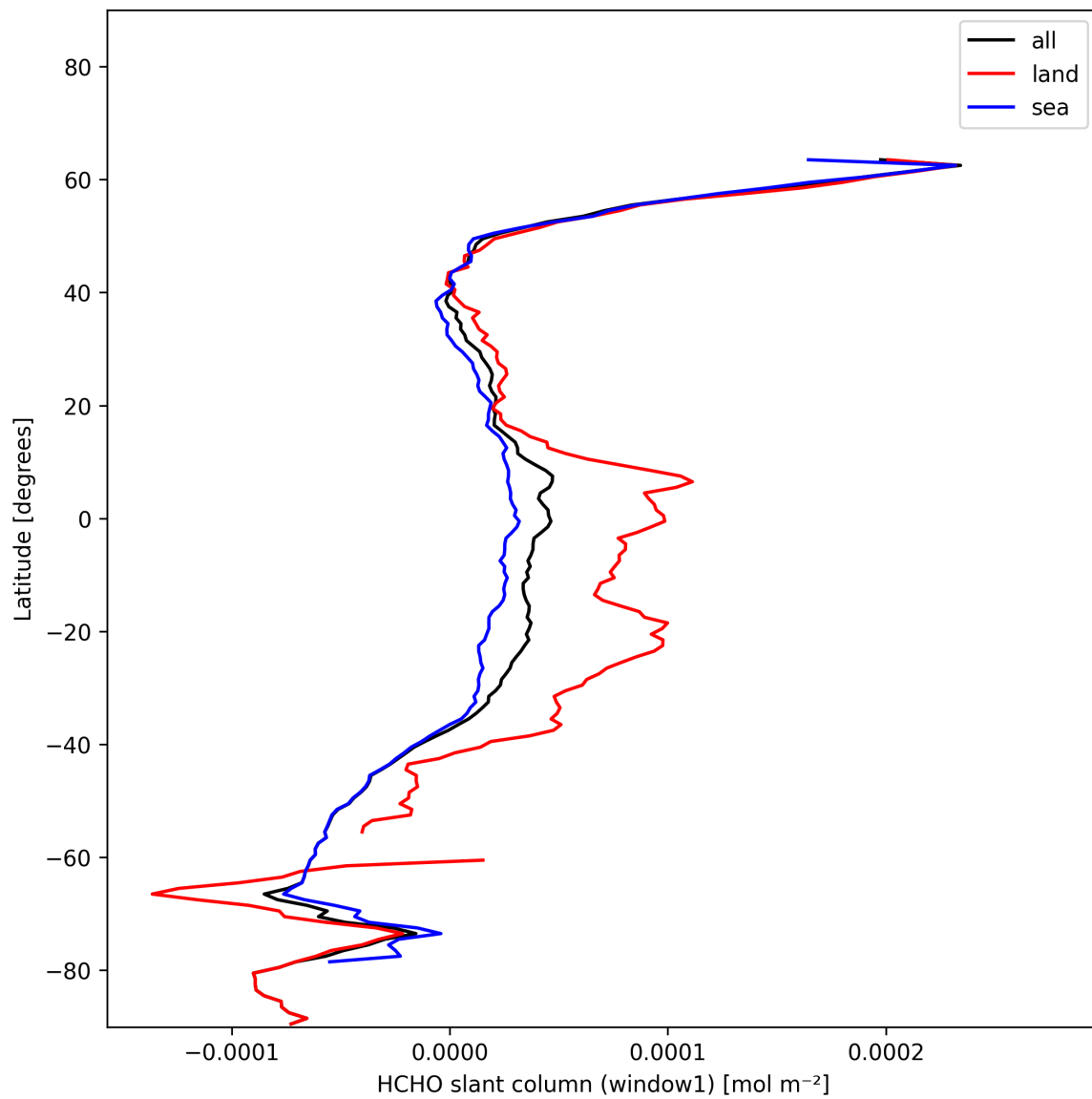
Figure 22: Zonal average of “HCHO slant column (window1)” for 2025-01-09 to 2025-01-10.
