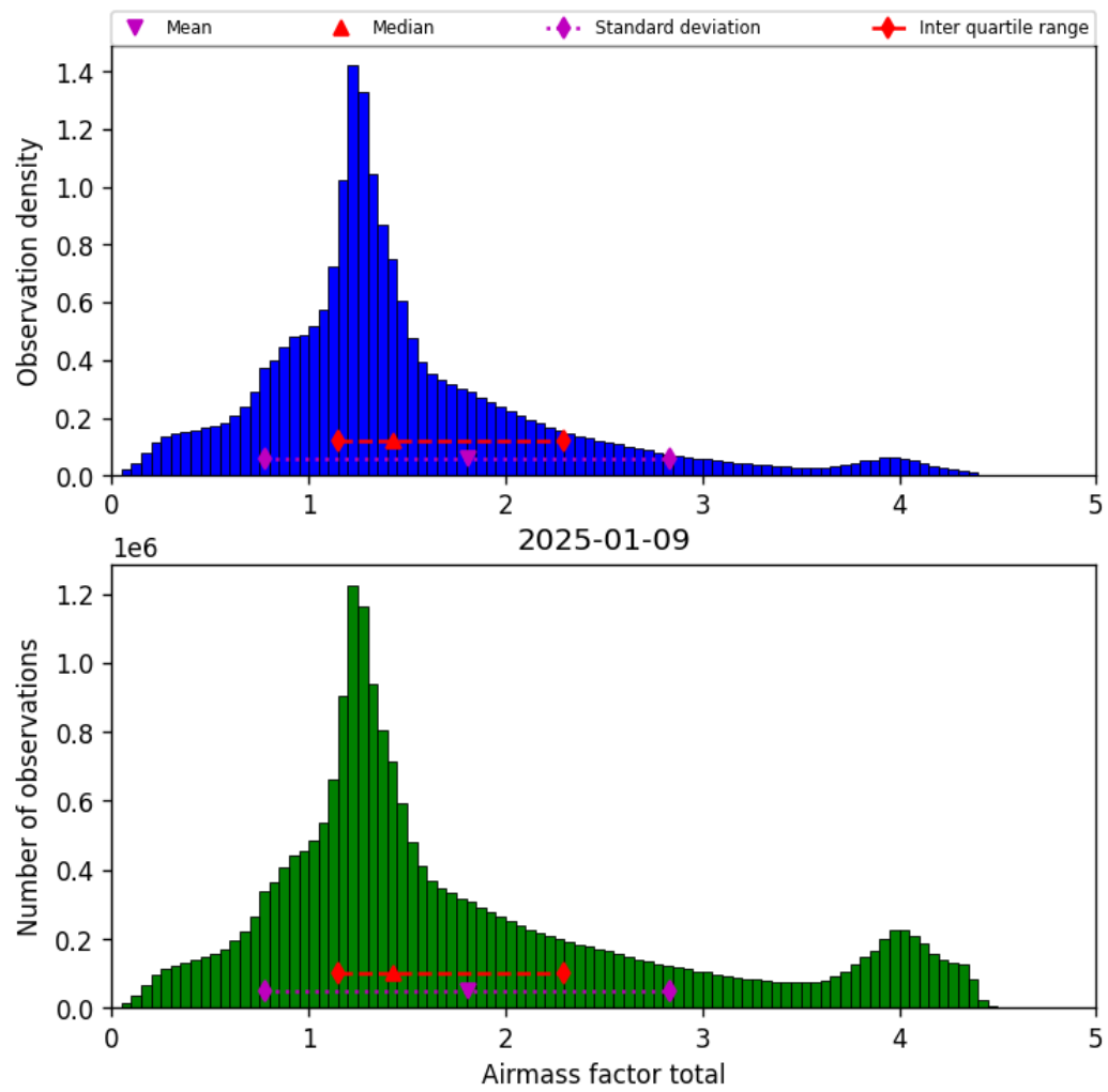
Figure 38: Histogram of “Airmass factor total” for 2025-01-09 to 2025-01-10
