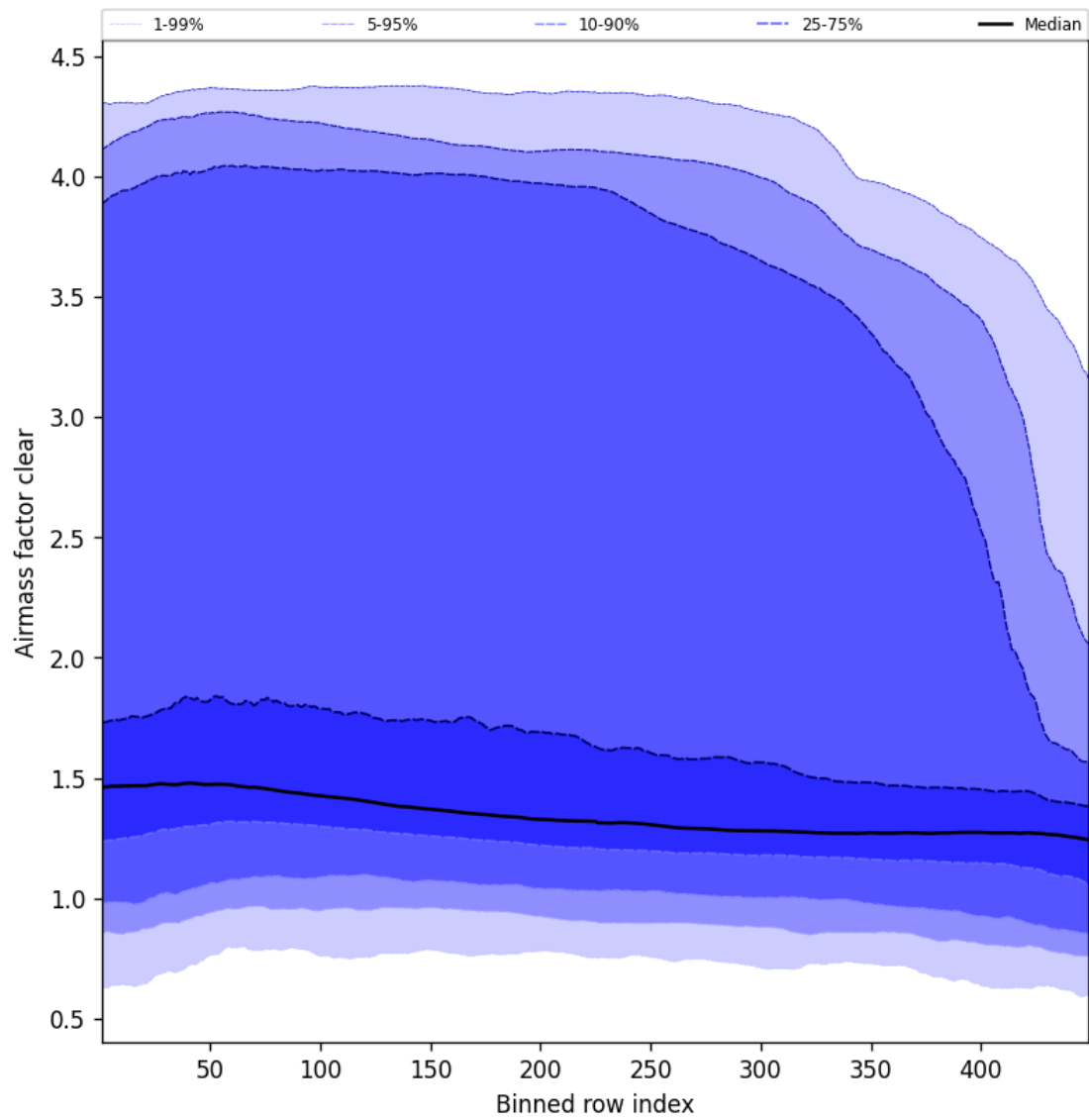
Figure 54: Along track statistics of “Airmass factor clear” for 2025-01-09 to 2025-01-10
