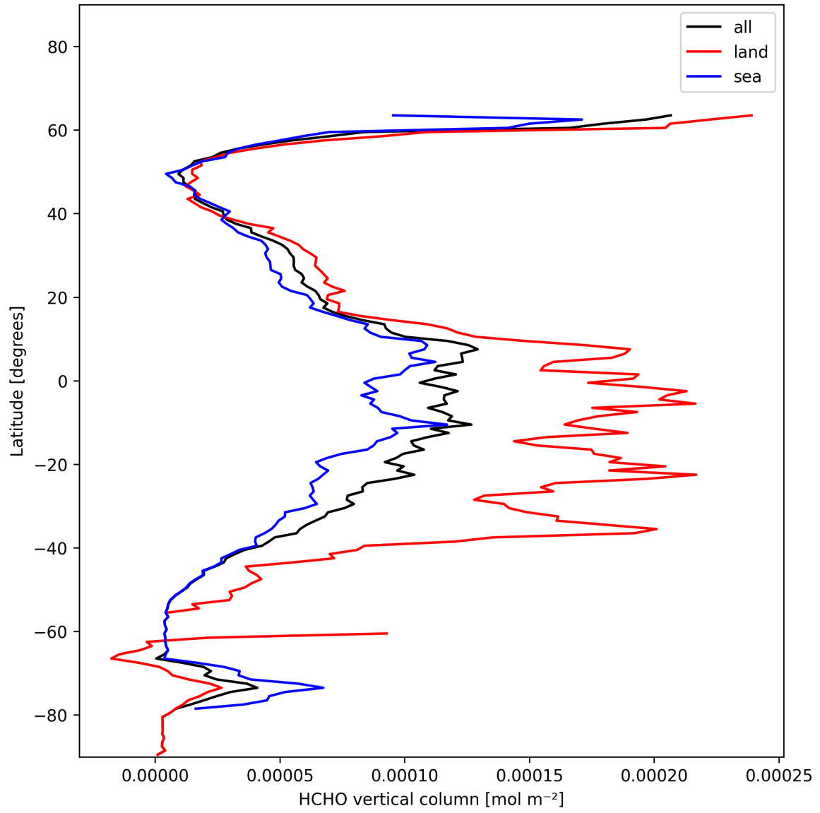
Figure 19: Zonal average of “HCHO vertical column” for 2025-01-09 to 2025-01-10.
