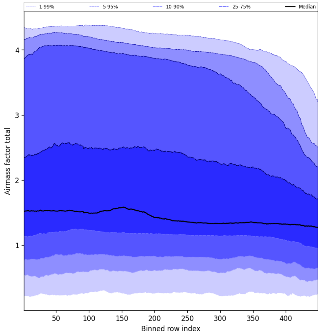
Figure 52: Along track statistics of “Airmass factor total” for 2025-01-09 to 2025-01-10
