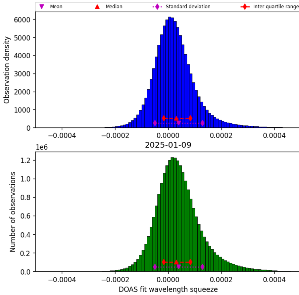
Figure 43: Histogram of “DOAS fit wavelength squeeze” for 2025-01-09 to 2025-01-10
