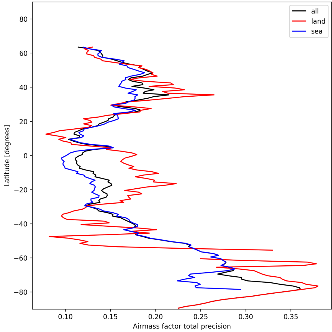
Figure 25: Zonal average of “Airmass factor total precision” for 2025-01-09 to 2025-01-10.
