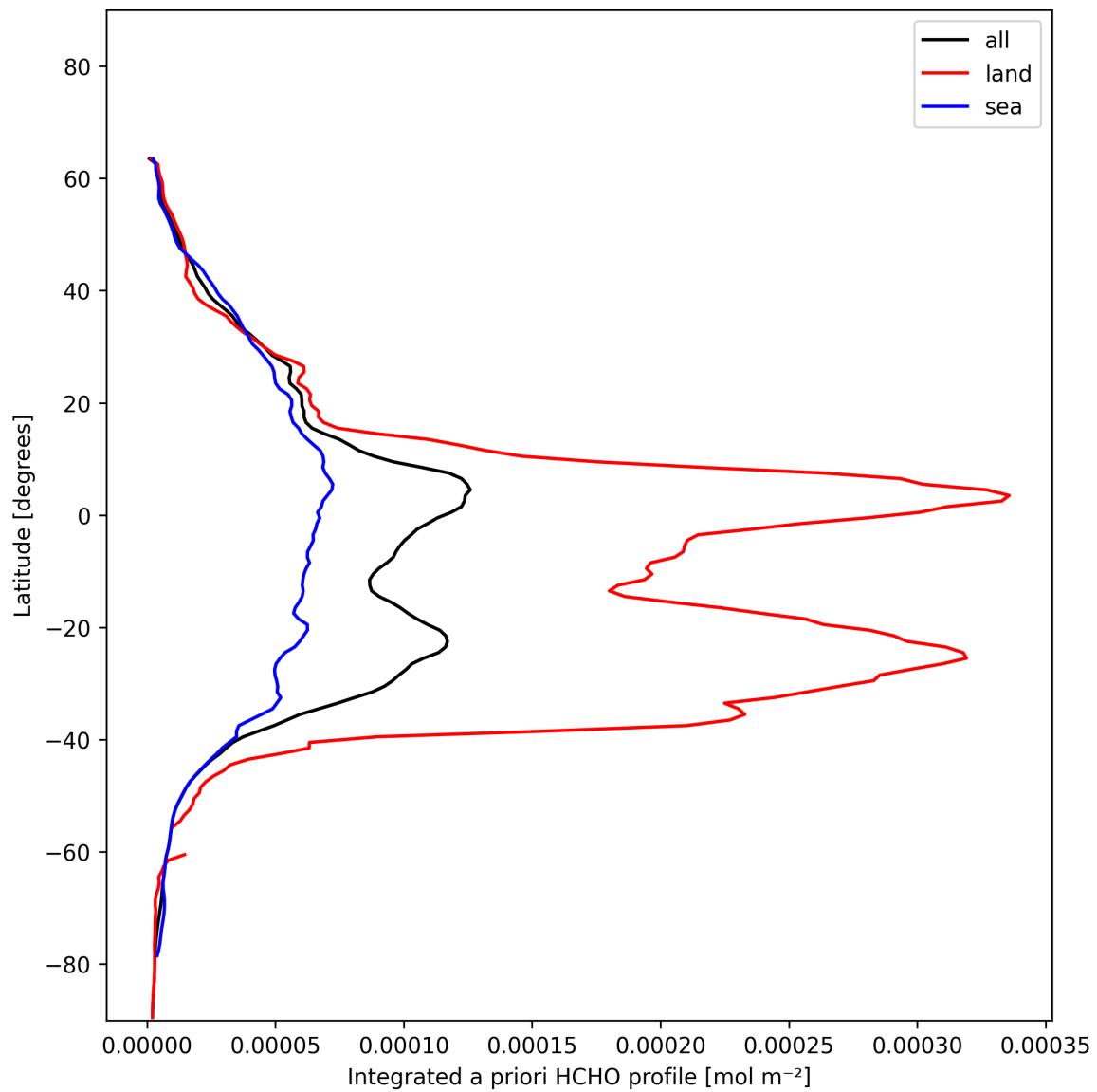
Figure 27: Zonal average of “Integrated a priori HCHO profile” for 2025-01-09 to 2025-01-10.
