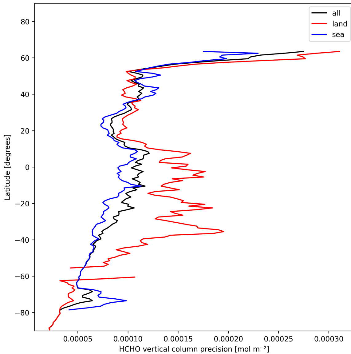
Figure 20: Zonal average of “HCHO vertical column precision” for 2025-01-09 to 2025-01-10.
