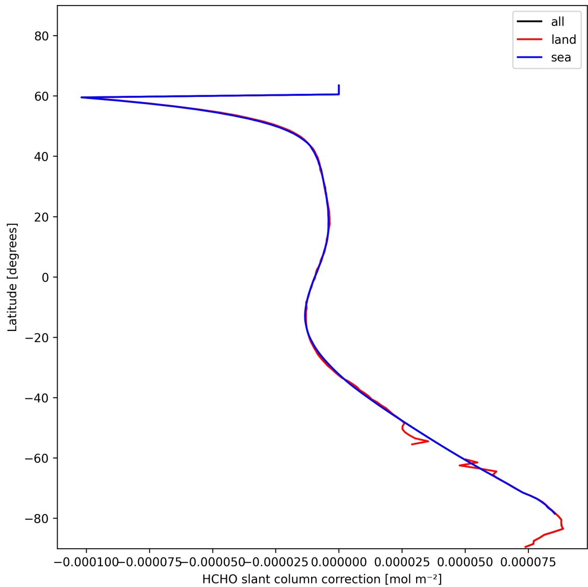
Figure 31: Zonal average of “HCHO slant column correction” for 2025-01-09 to 2025-01-10.
