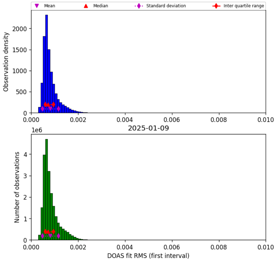
Figure 44: Histogram of "DOAS fit RMS (first interval)" for 2025-01-09 to 2025-01-10
