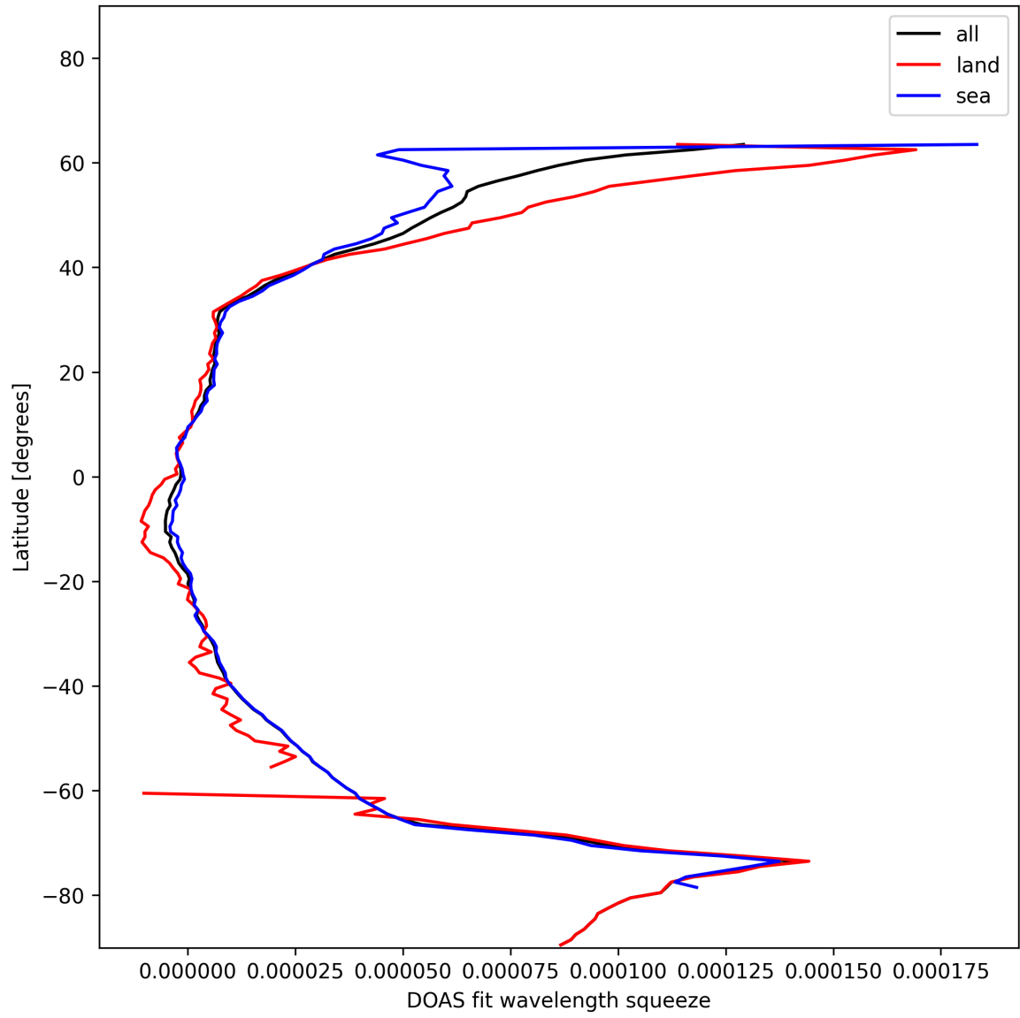
Figure 29: Zonal average of “DOAS fit wavelength squeeze” for 2025-01-09 to 2025-01-10.
