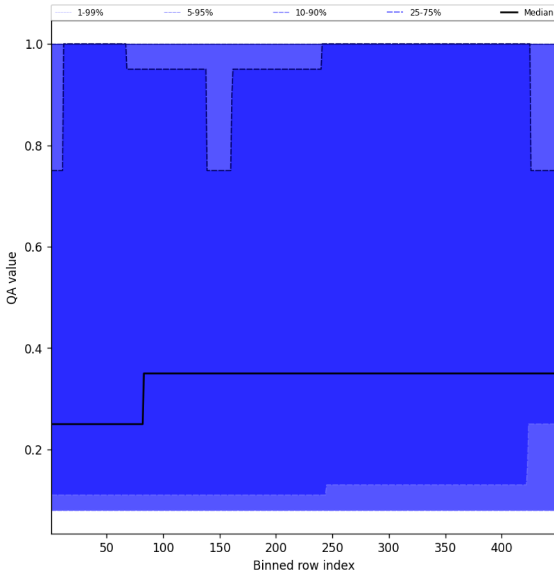
Figure 46: Along track statistics of “QA value” for 2025-01-09 to 2025-01-10
