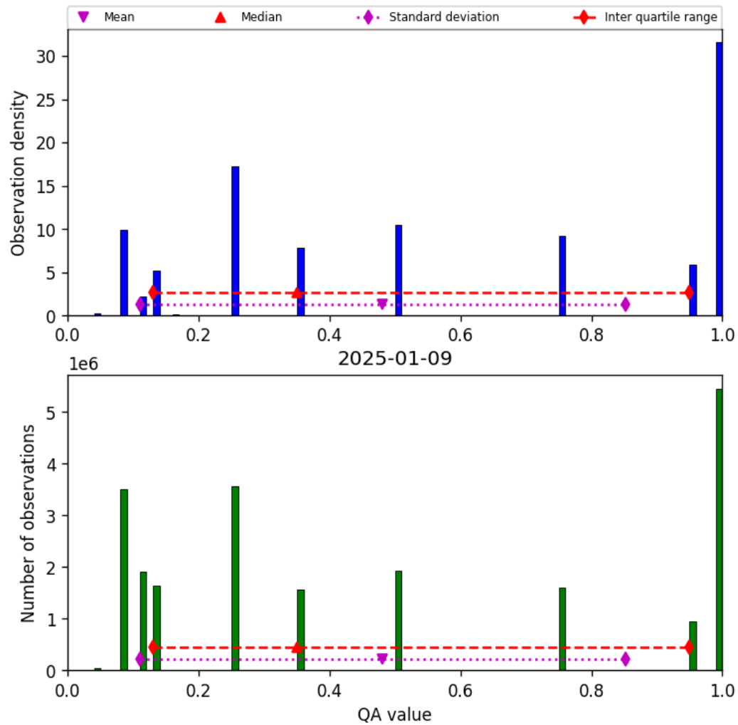
Figure 32: Histogram of “QA value” for 2025-01-09 to 2025-01-10
