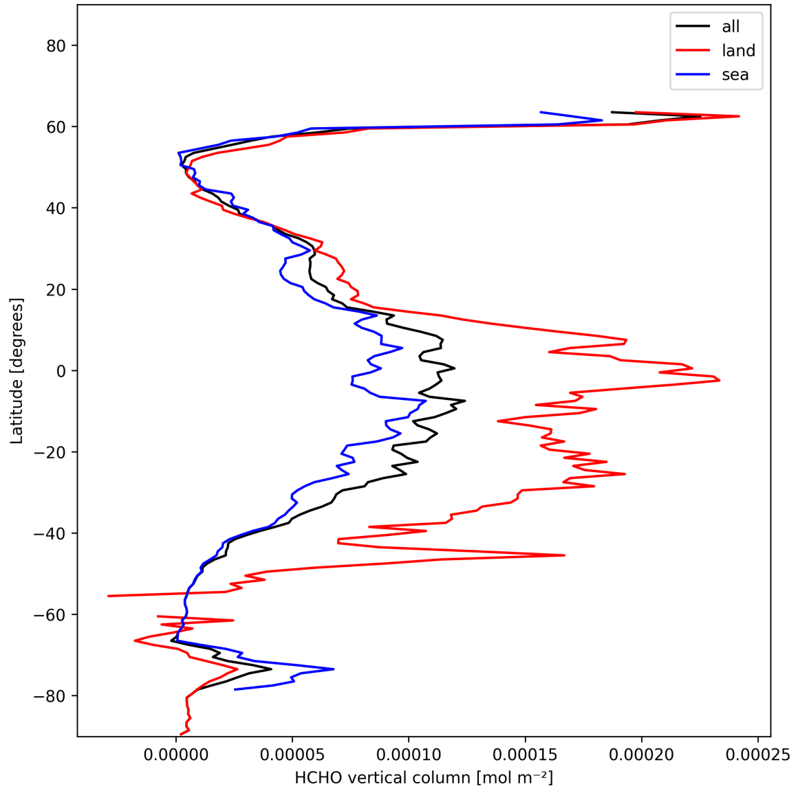
Figure 19: Zonal average of “HCHO vertical column” for 2025-01-10 to 2025-01-10.
