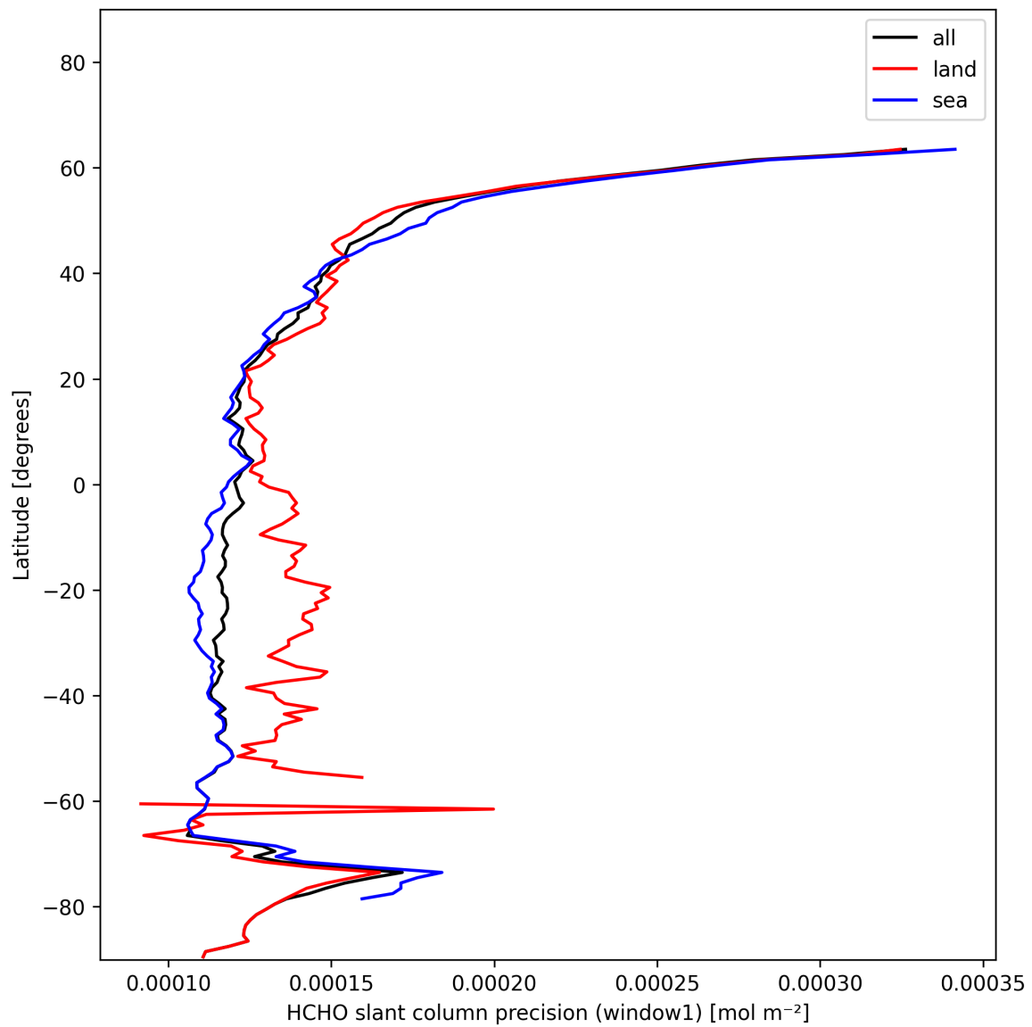
Figure 23: Zonal average of “HCHO slant column precision (window1)” for 2025-01-10 to 2025-01-10.
