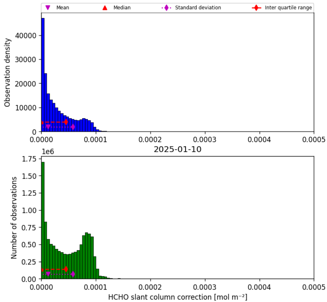
Figure 45: Histogram of “HCHO slant column correction” for 2025-01-10 to 2025-01-10
