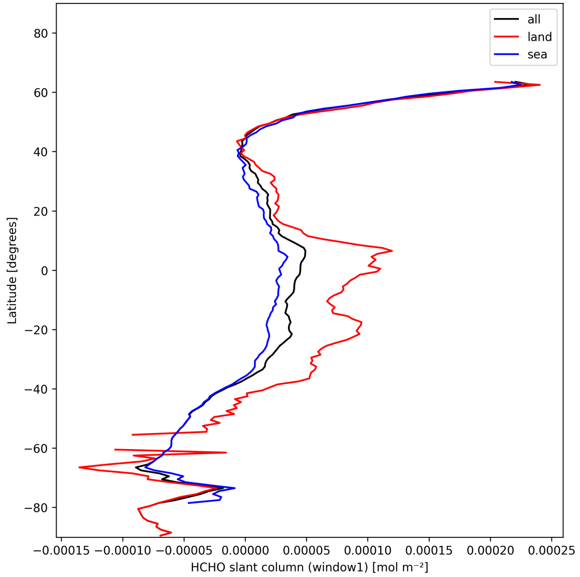
Figure 22: Zonal average of “HCHO slant column (window1)” for 2025-01-10 to 2025-01-10.
