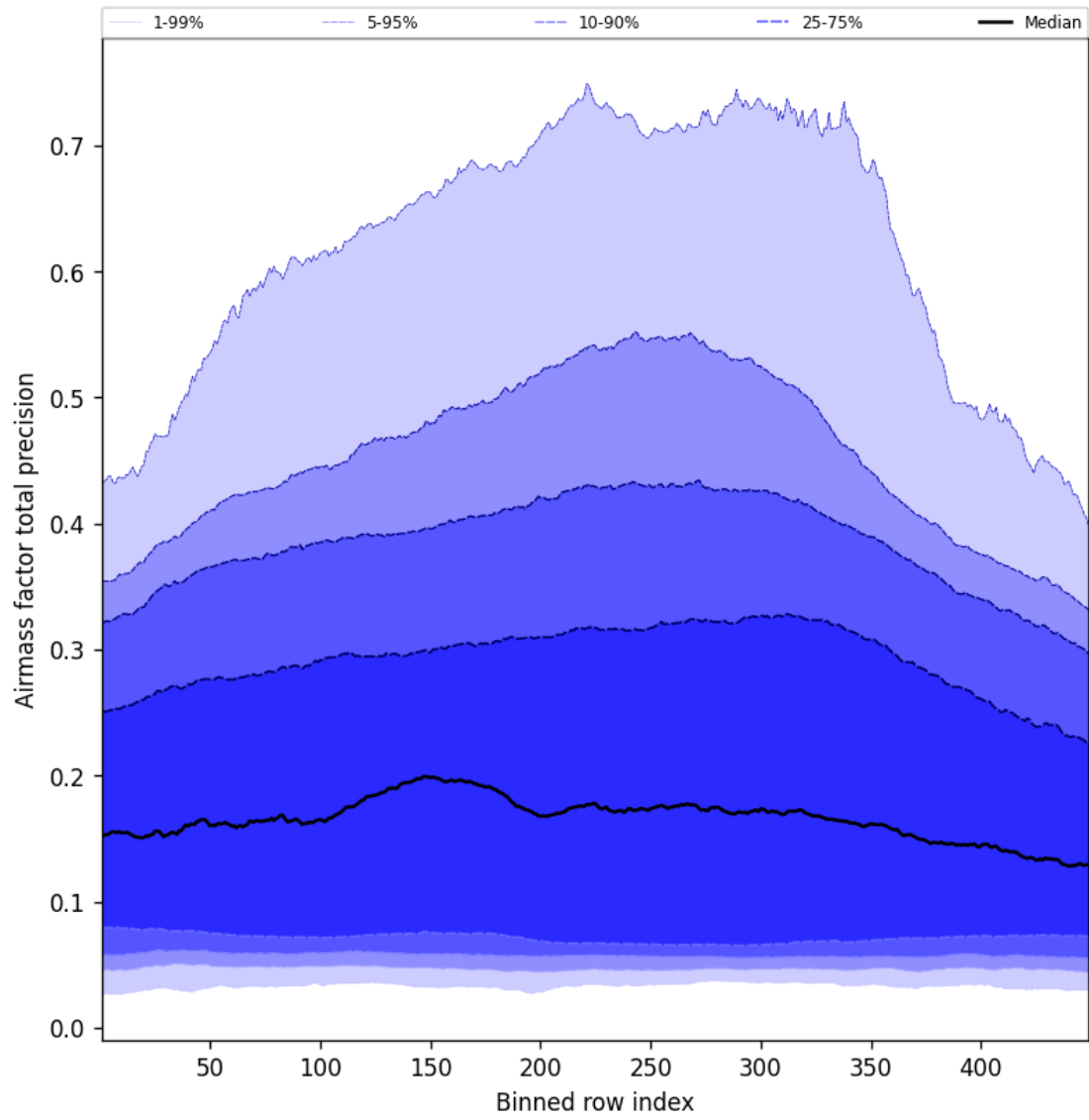
Figure 53: Along track statistics of “Airmass factor total precision” for 2025-01-10 to 2025-01-10
