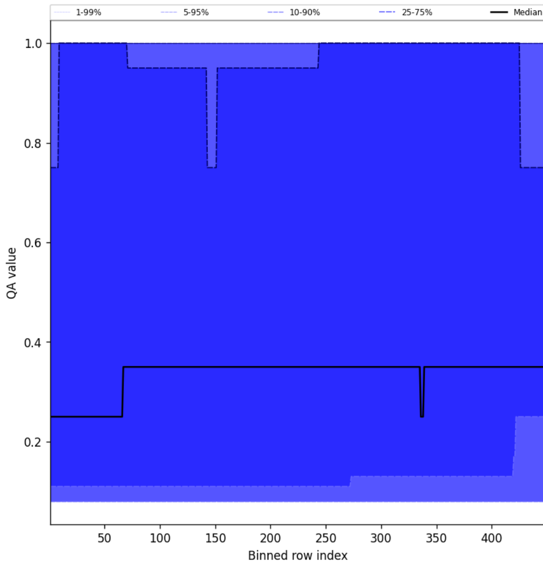
Figure 46: Along track statistics of “QA value” for 2025-01-10 to 2025-01-10
