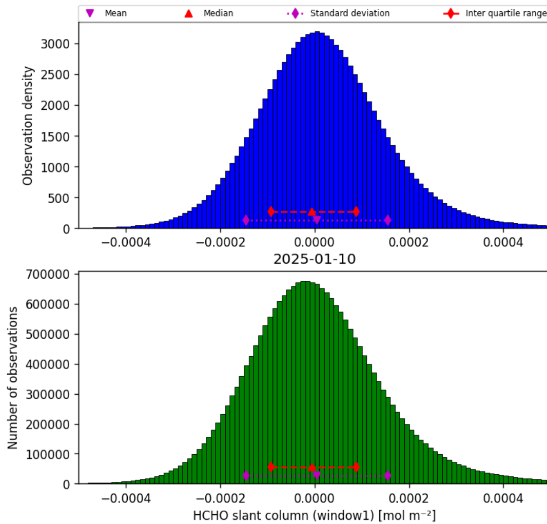
Figure 36: Histogram of “HCHO slant column (window1)” for 2025-01-10 to 2025-01-10
