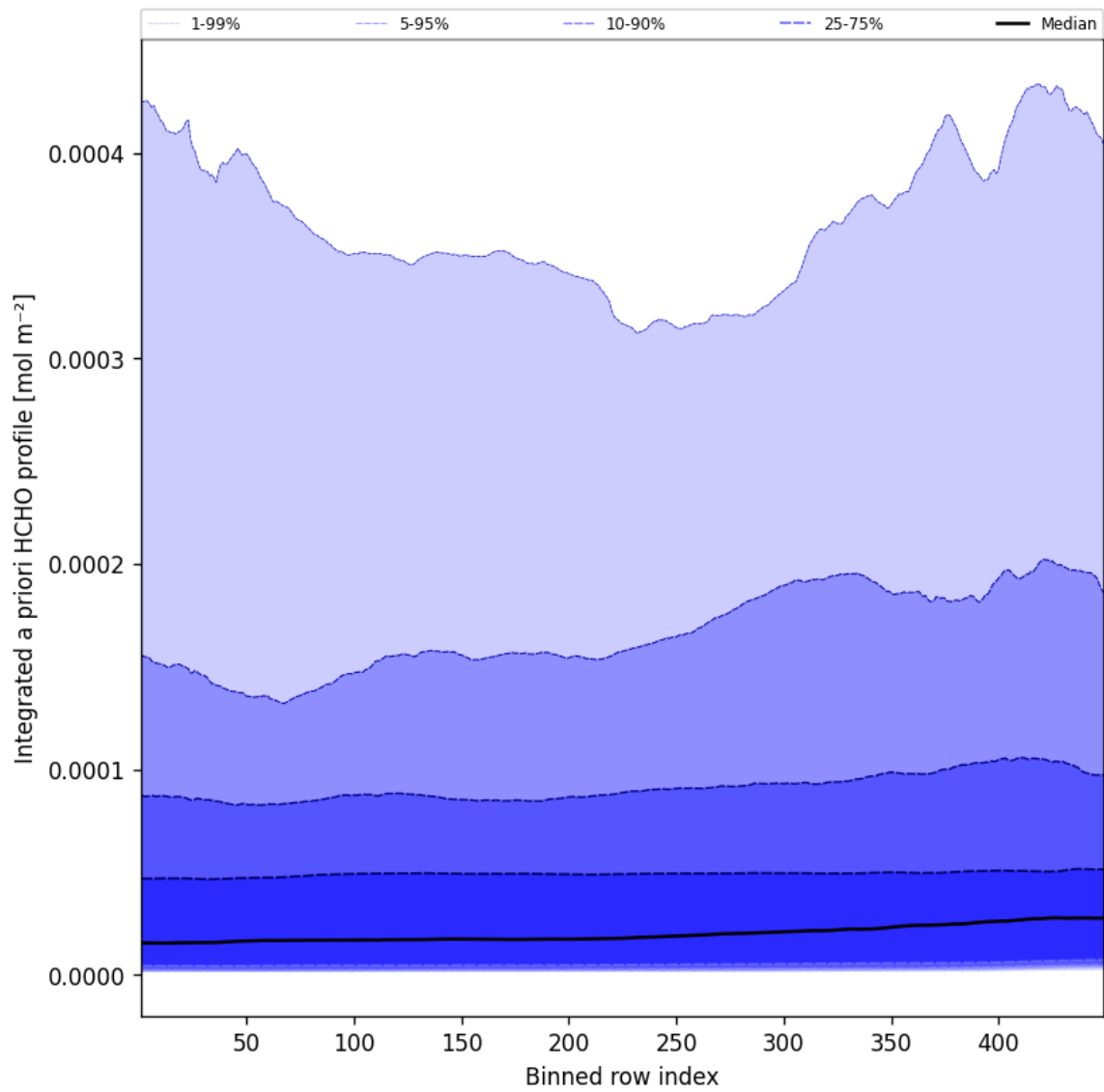
Figure 55: Along track statistics of “Integrated a priori HCHO profile” for 2025-01-10 to 2025-01-10
