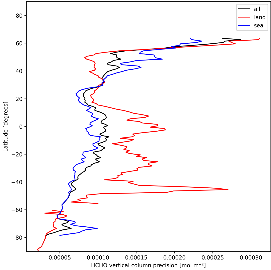
Figure 20: Zonal average of “HCHO vertical column precision” for 2025-01-10 to 2025-01-10.
