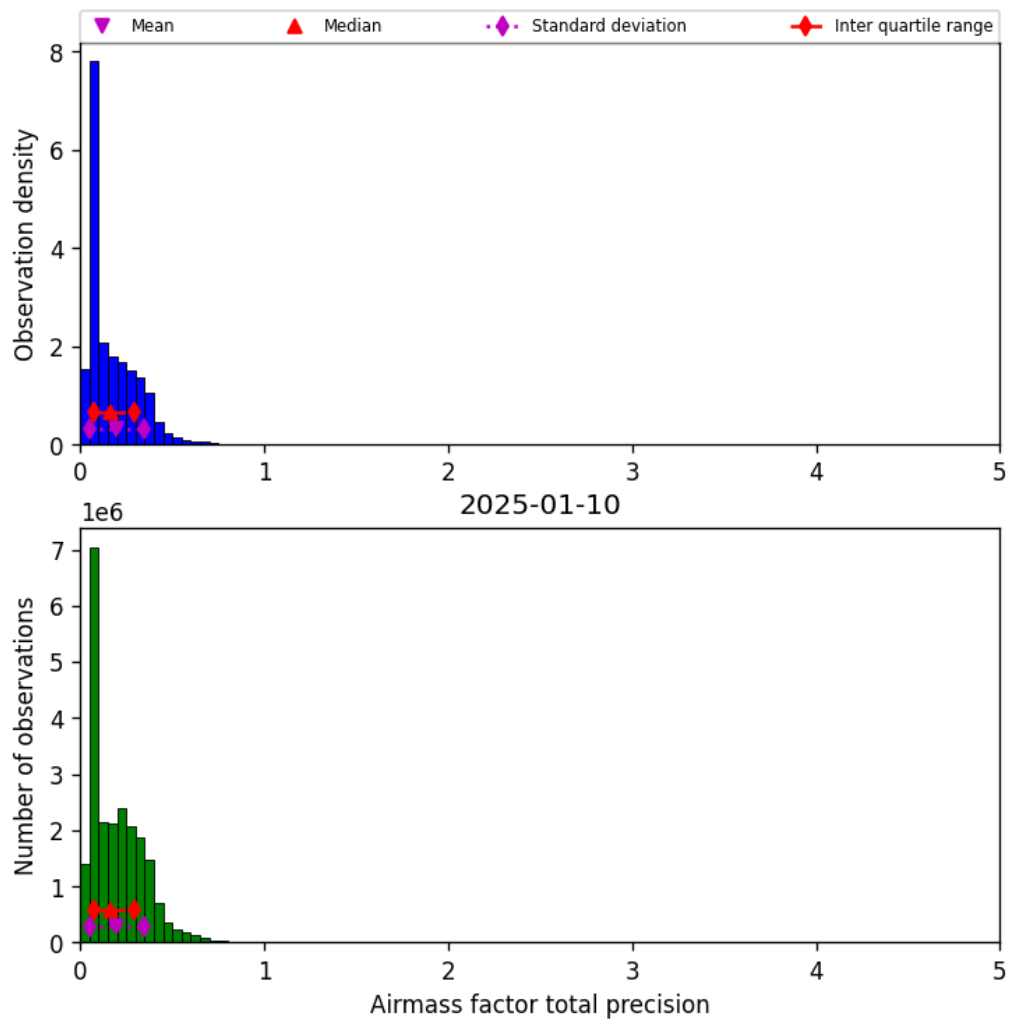
Figure 39: Histogram of “Airmass factor total precision” for 2025-01-10 to 2025-01-10
