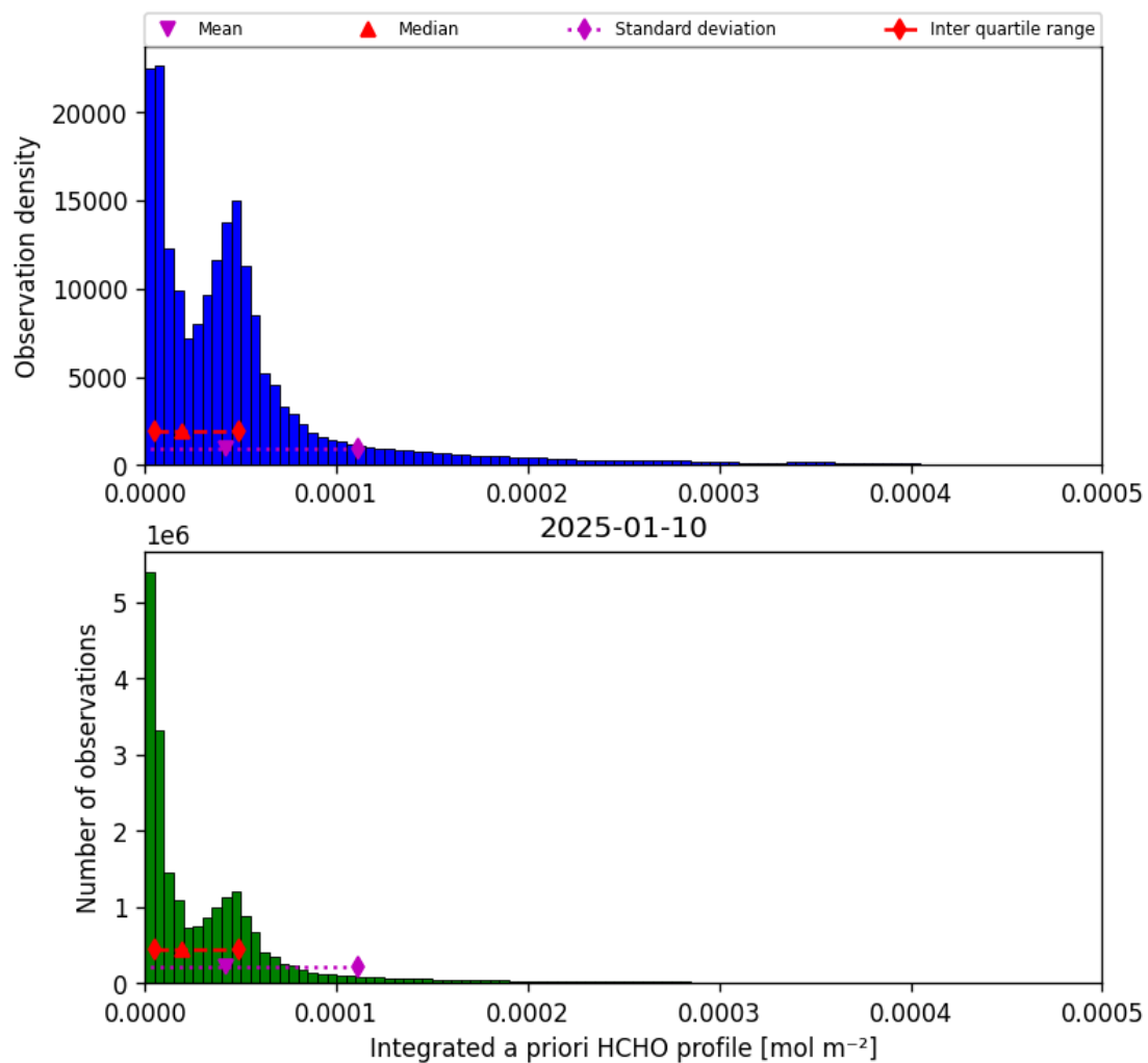
Figure 41: Histogram of “Integrated a priori HCHO profile” for 2025-01-10 to 2025-01-10
