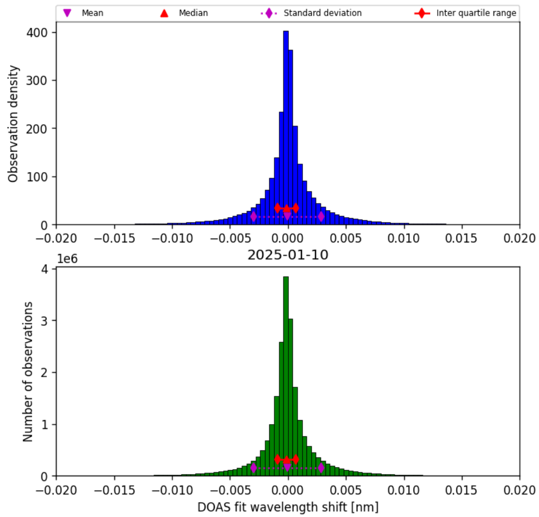
Figure 42: Histogram of “DOAS fit wavelength shift” for 2025-01-10 to 2025-01-10
