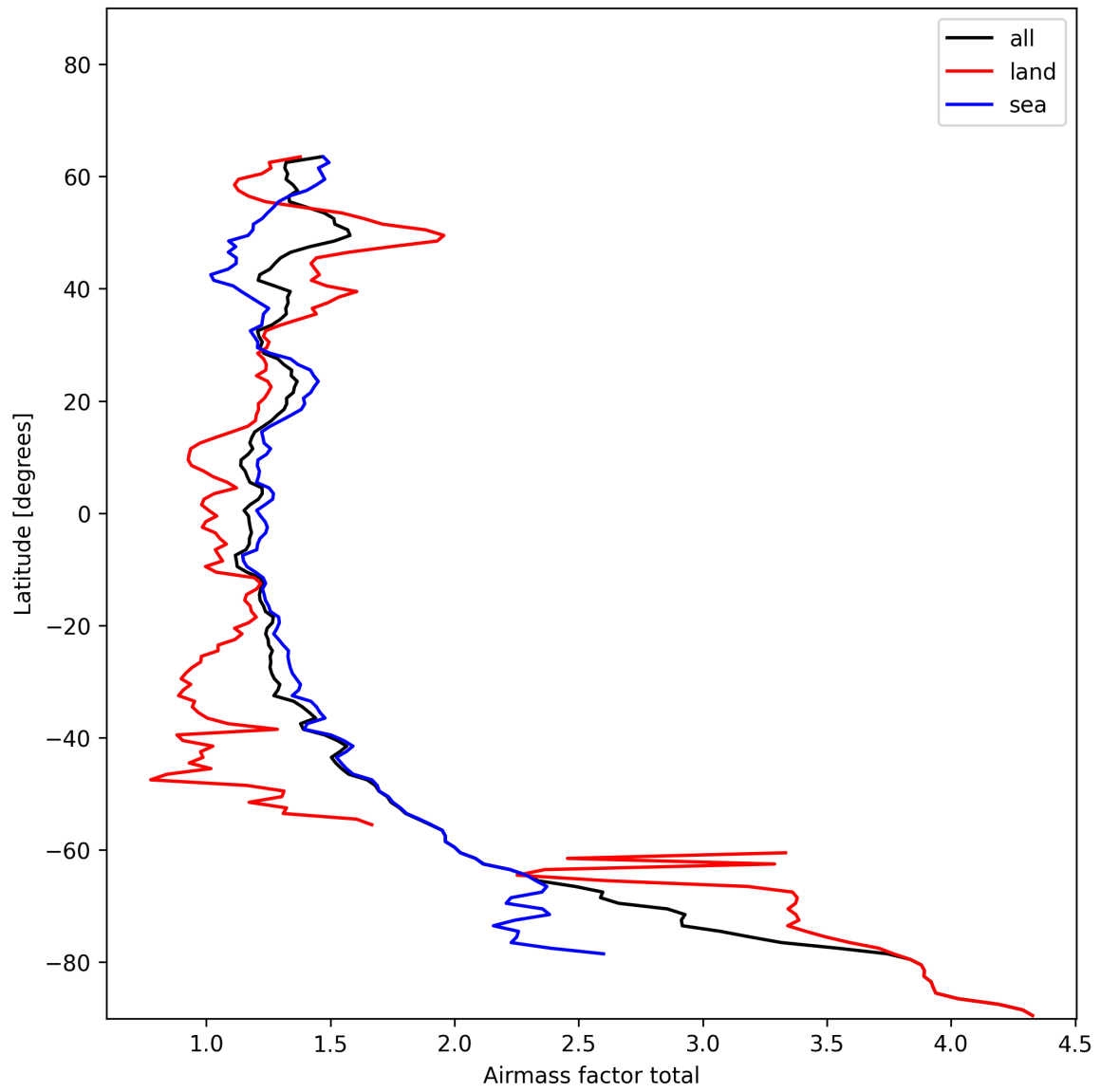
Figure 24: Zonal average of “Airmass factor total” for 2025-01-10 to 2025-01-10.
