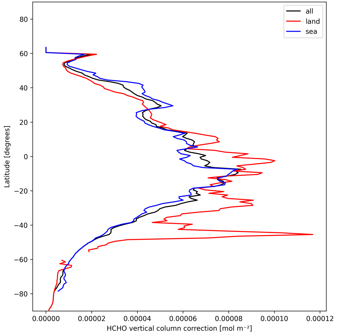
Figure 21: Zonal average of “HCHO vertical column correction” for 2025-01-10 to 2025-01-10.
