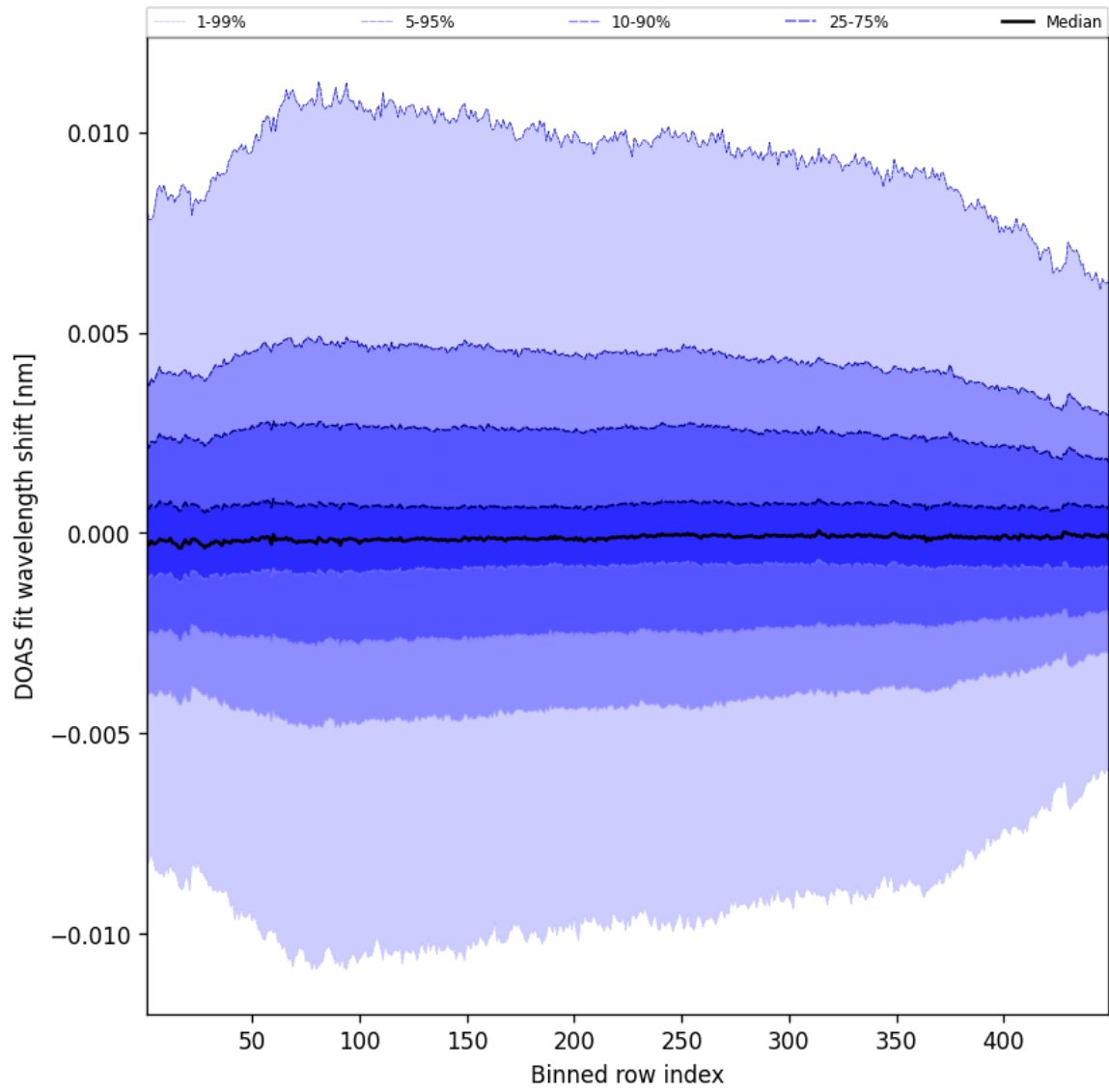
Figure 56: Along track statistics of “DOAS fit wavelength shift” for 2025-01-10 to 2025-01-10
