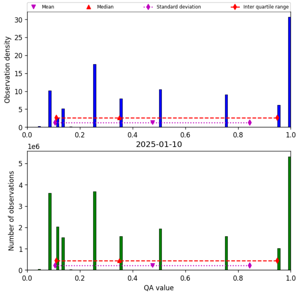
Figure 32: Histogram of “QA value” for 2025-01-10 to 2025-01-10
