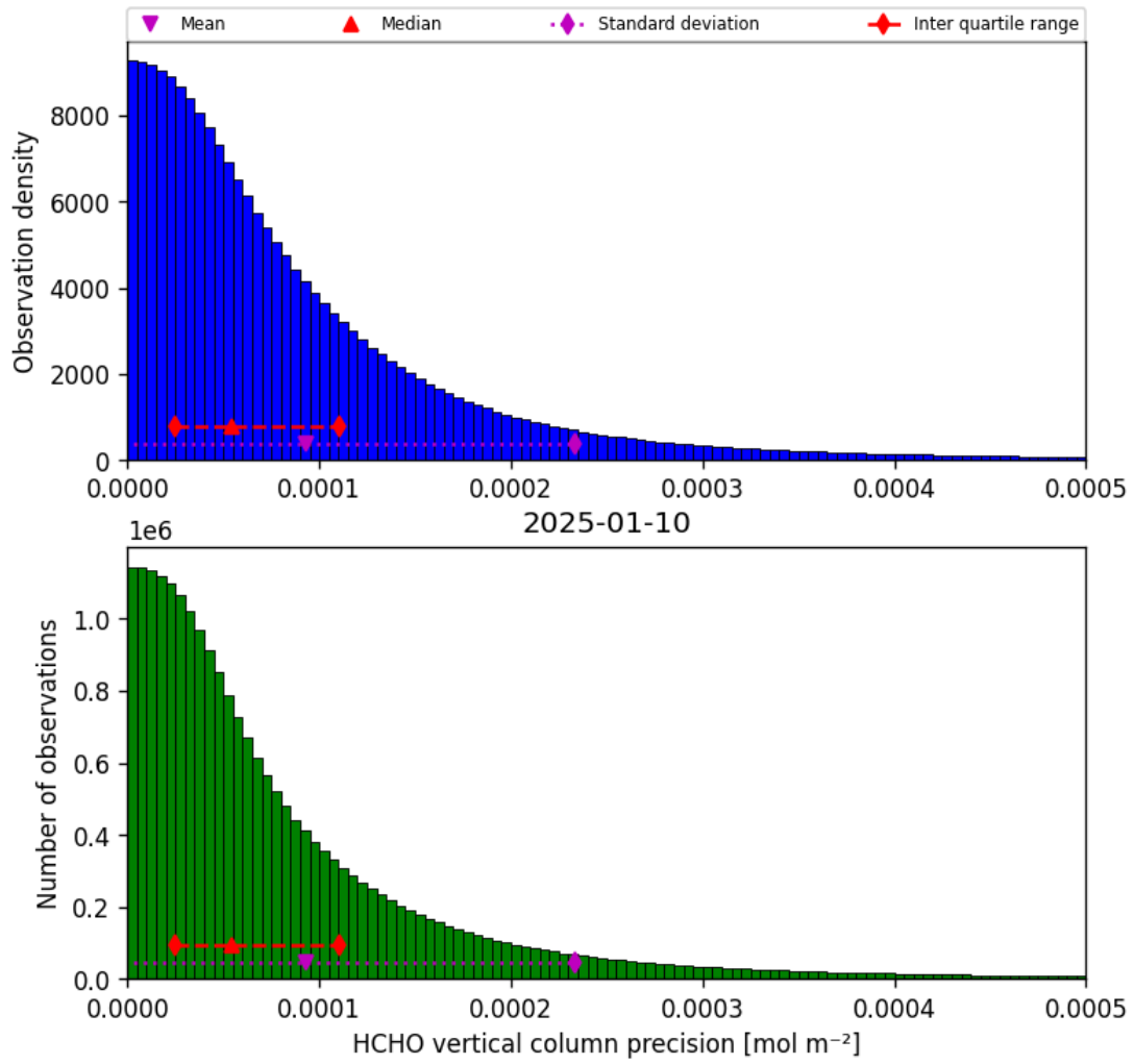
Figure 34: Histogram of “HCHO vertical column precision” for 2025-01-10 to 2025-01-10
