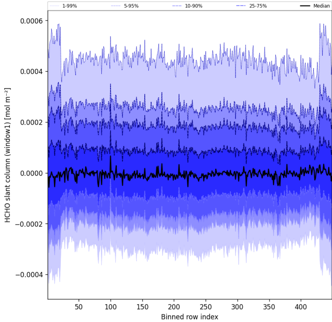
Figure 50: Along track statistics of “HCHO slant column (window1)” for 2025-01-10 to 2025-01-10
