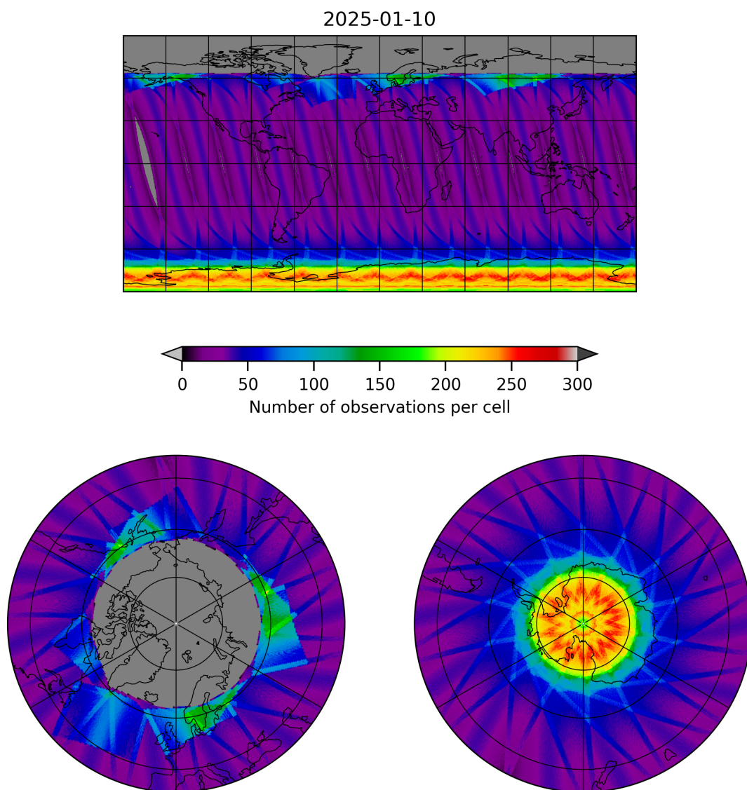
Figure 17: Map of the number of observations for 2025-01-10 to 2025-01-10
