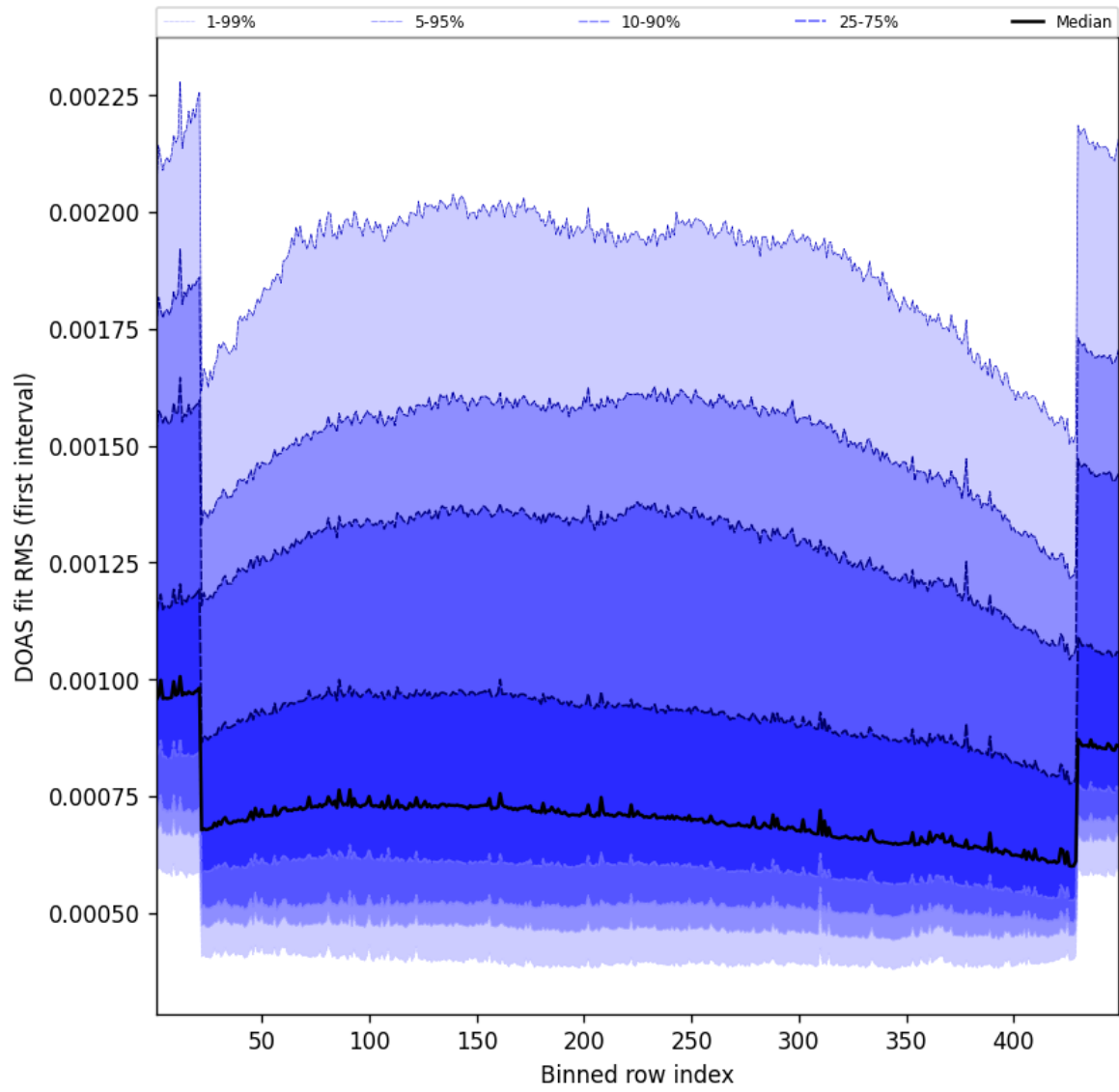
Figure 58: Along track statistics of “DOAS fit RMS (first interval)” for 2025-01-10 to 2025-01-10
