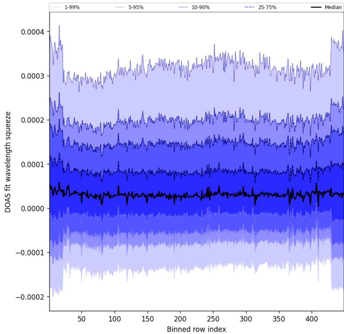
Figure 57: Along track statistics of “DOAS fit wavelength squeeze” for 2025-01-10 to 2025-01-10
