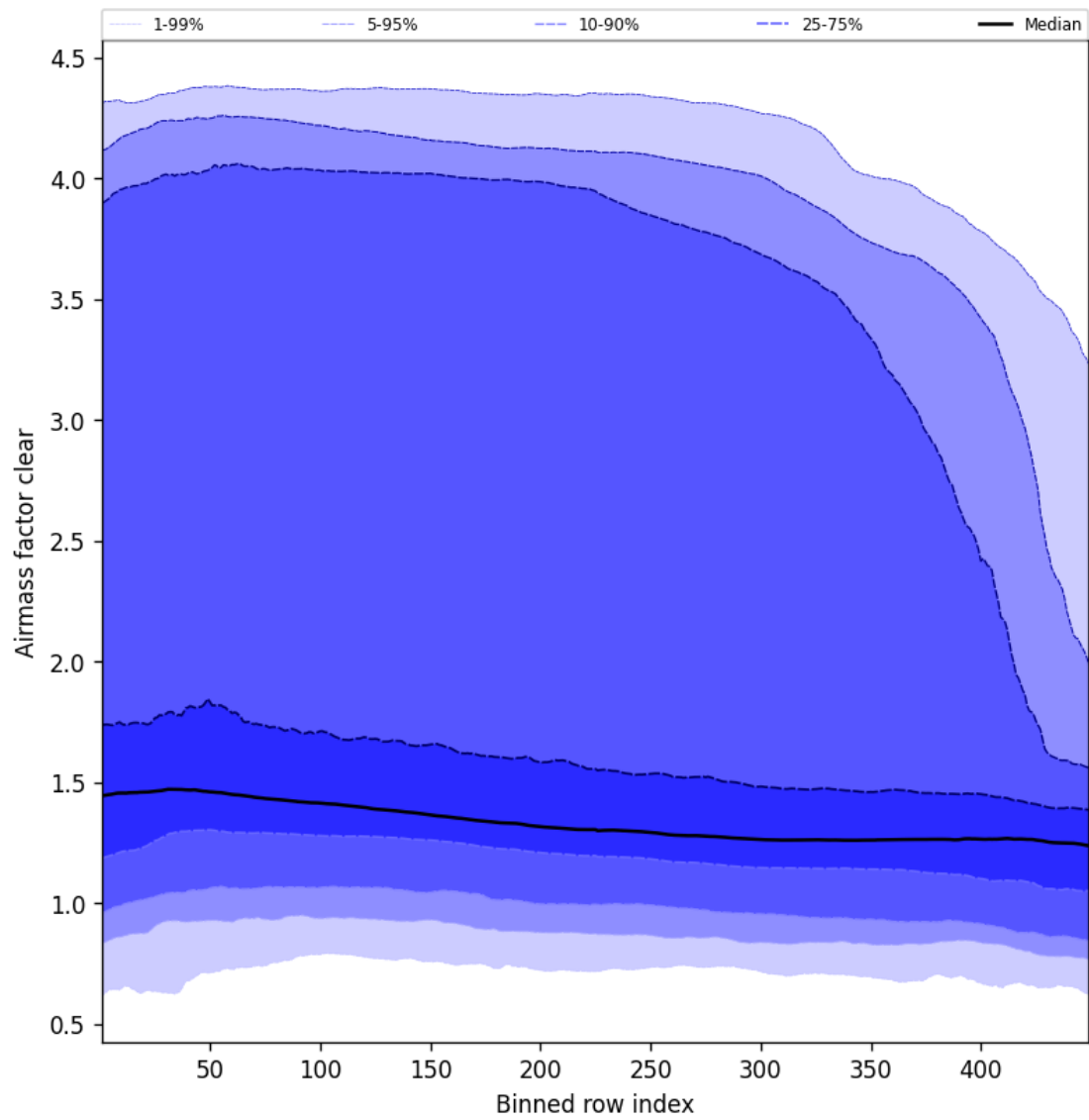
Figure 54: Along track statistics of “Airmass factor clear” for 2025-01-10 to 2025-01-10
