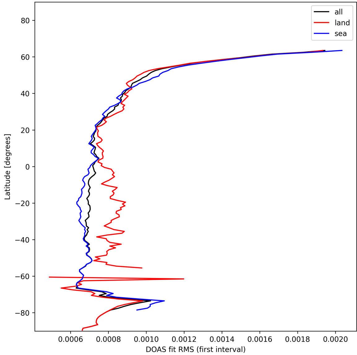
Figure 30: Zonal average of “DOAS fit RMS (first interval)” for 2025-01-10 to 2025-01-10.
