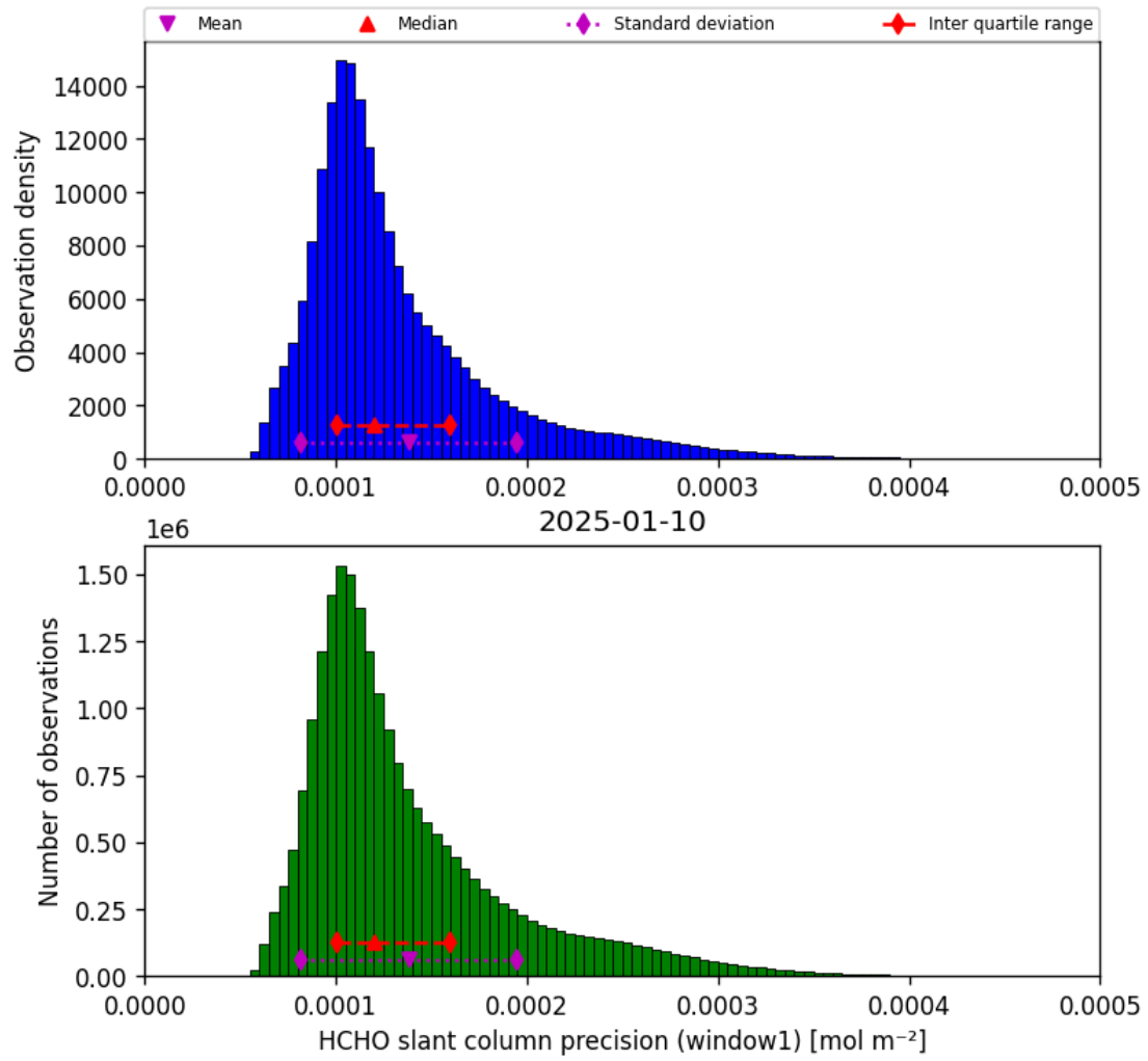
Figure 37: Histogram of “HCHO slant column precision (window1)” for 2025-01-10 to 2025-01-10
