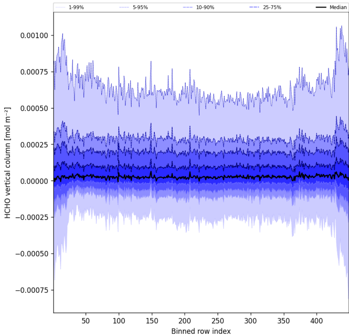
Figure 47: Along track statistics of “HCHO vertical column” for 2025-01-10 to 2025-01-10
