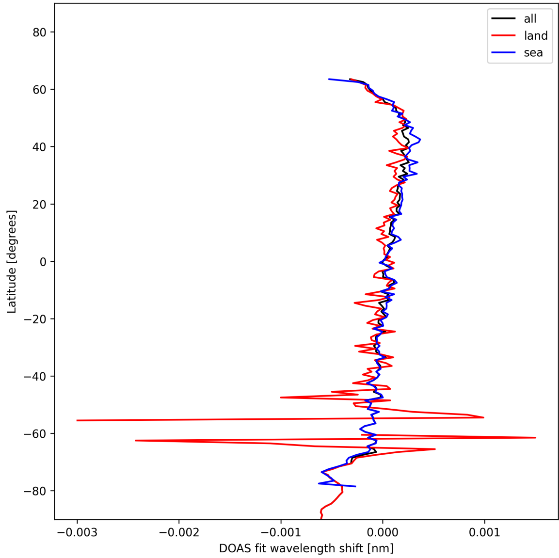
Figure 28: Zonal average of “DOAS fit wavelength shift” for 2025-01-10 to 2025-01-10.
