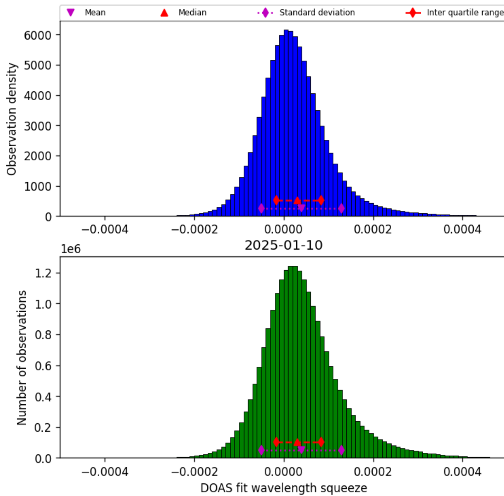
Figure 43: Histogram of “DOAS fit wavelength squeeze” for 2025-01-10 to 2025-01-10
