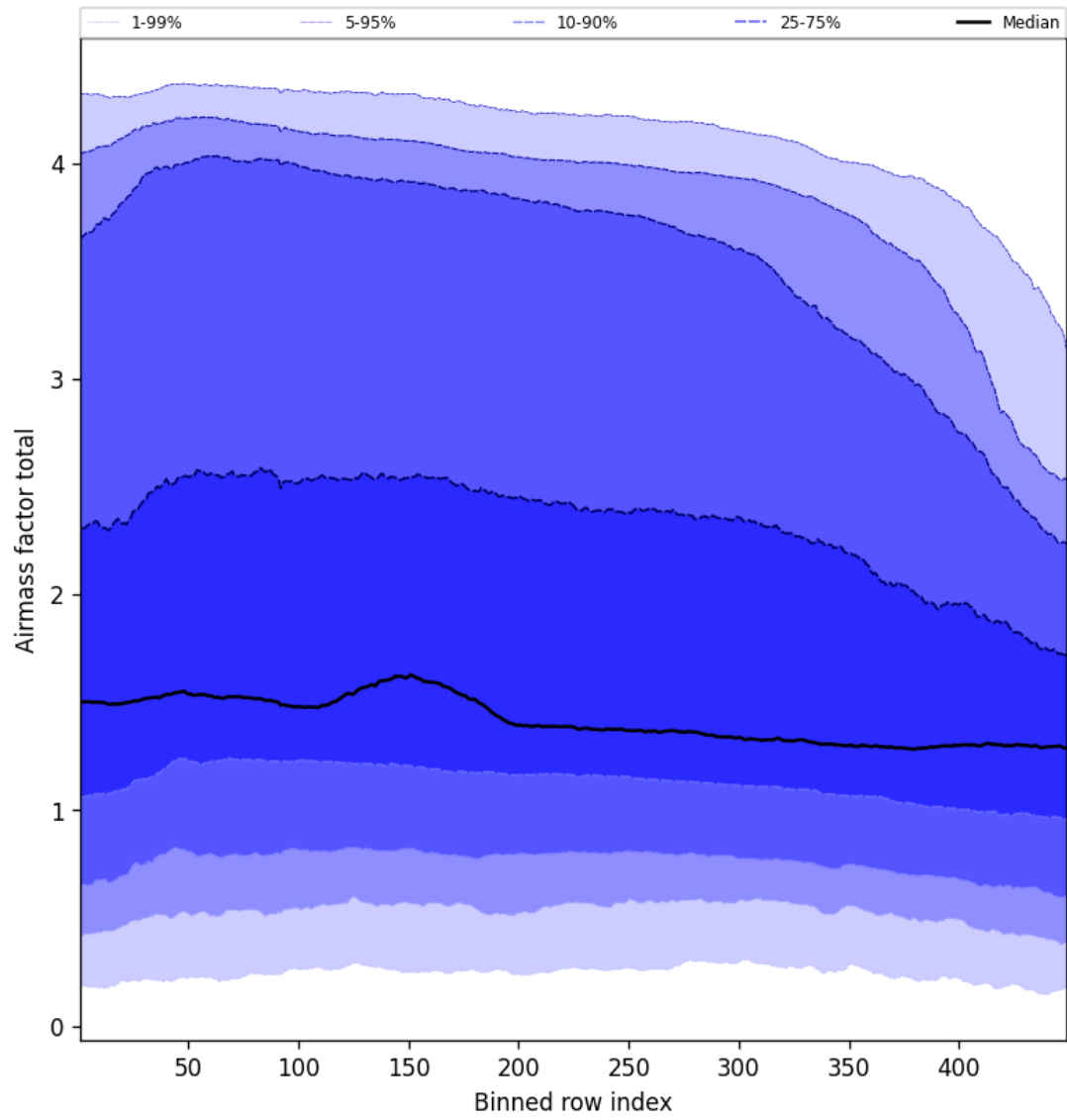
Figure 52: Along track statistics of “Airmass factor total” for 2025-01-10 to 2025-01-10
