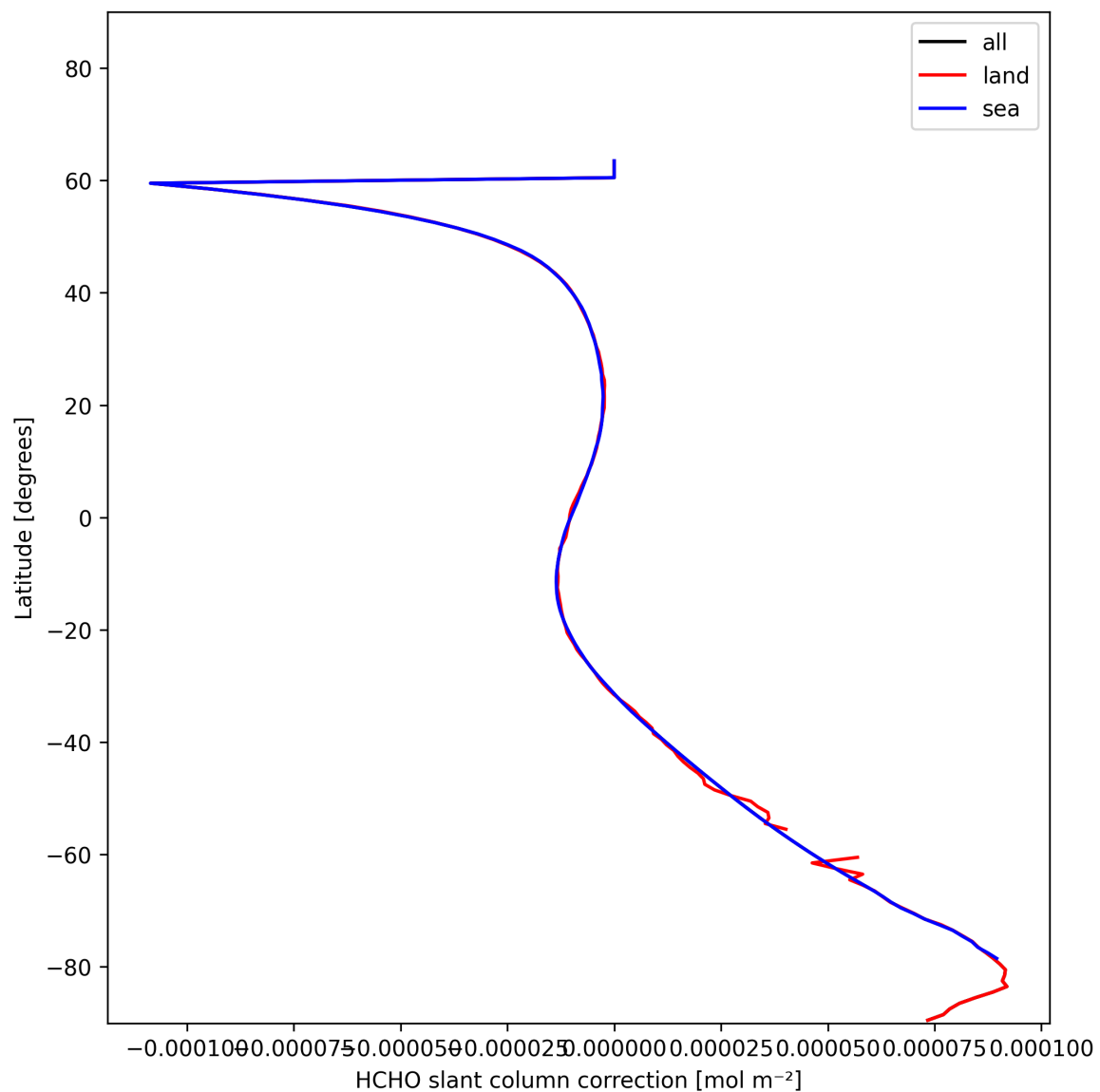
Figure 31: Zonal average of “HCHO slant column correction” for 2025-01-10 to 2025-01-10.
