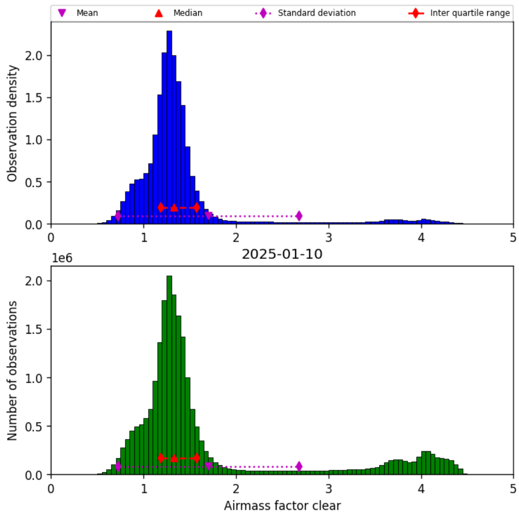
Figure 40: Histogram of “Airmass factor clear” for 2025-01-10 to 2025-01-10
