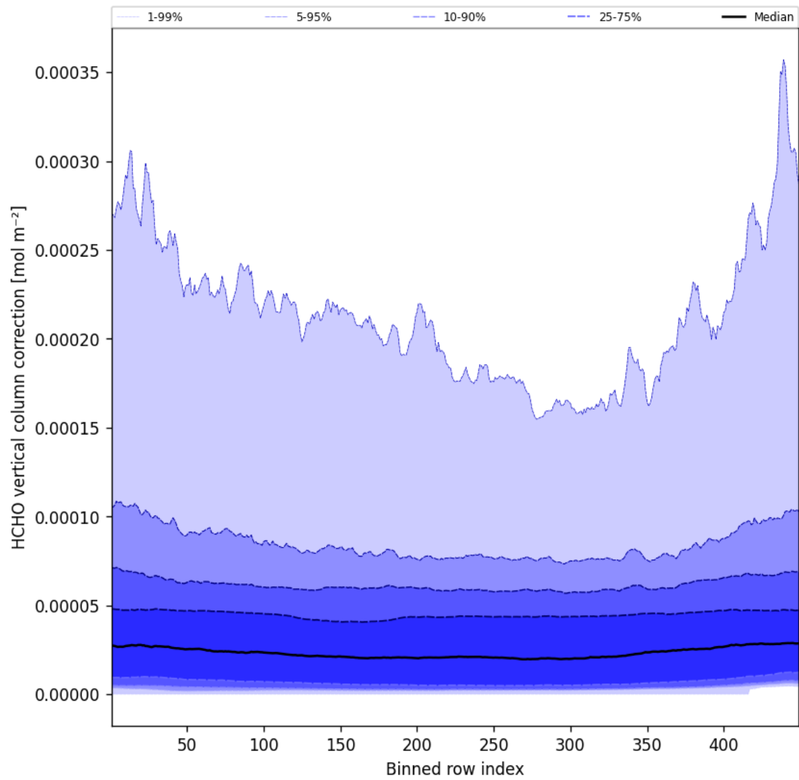
Figure 49: Along track statistics of “HCHO vertical column correction” for 2025-01-10 to 2025-01-10
