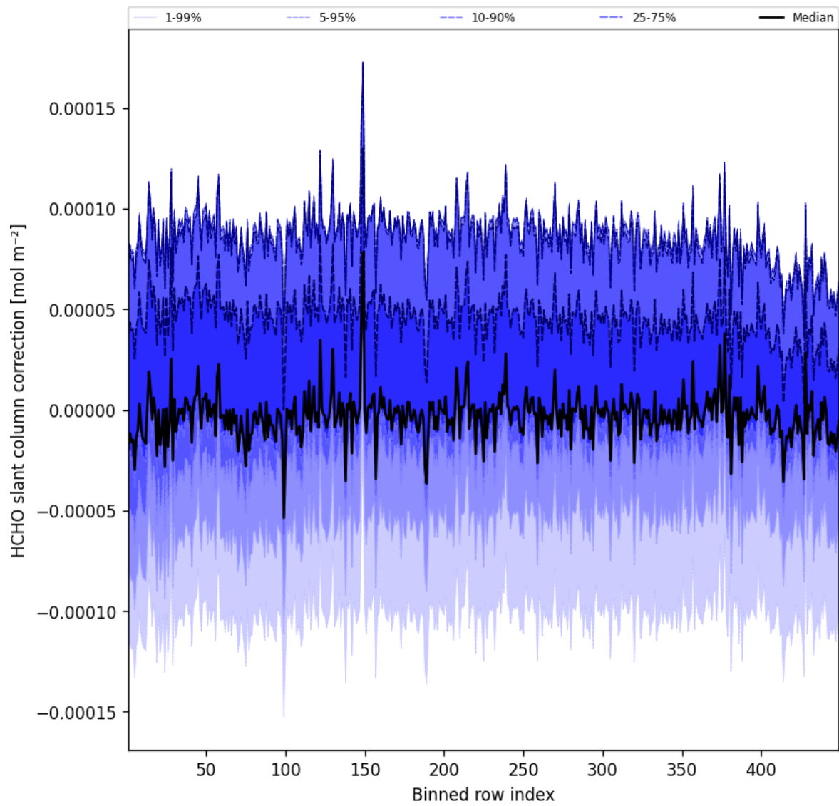
Figure 59: Along track statistics of “HCHO slant column correction” for 2025-01-10 to 2025-01-10
