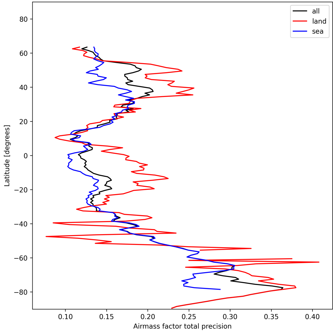
Figure 25: Zonal average of “Airmass factor total precision” for 2025-01-10 to 2025-01-10.
