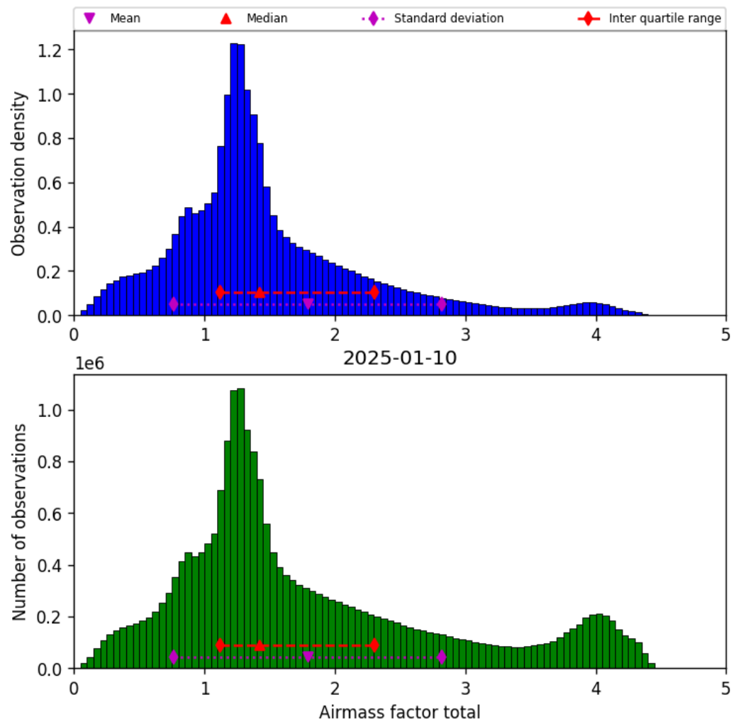
Figure 38: Histogram of “Airmass factor total” for 2025-01-10 to 2025-01-10
