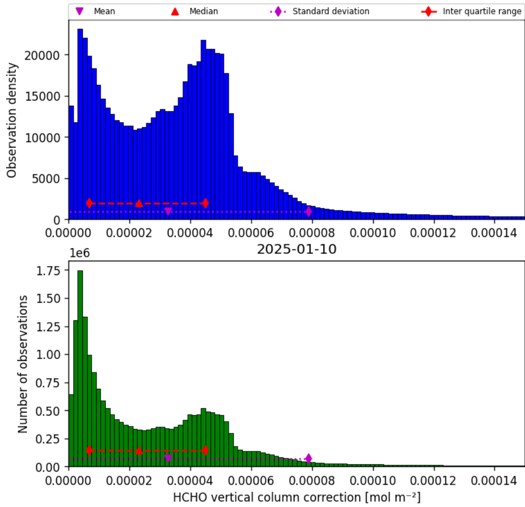
Figure 35: Histogram of “HCHO vertical column correction” for 2025-01-10 to 2025-01-10
