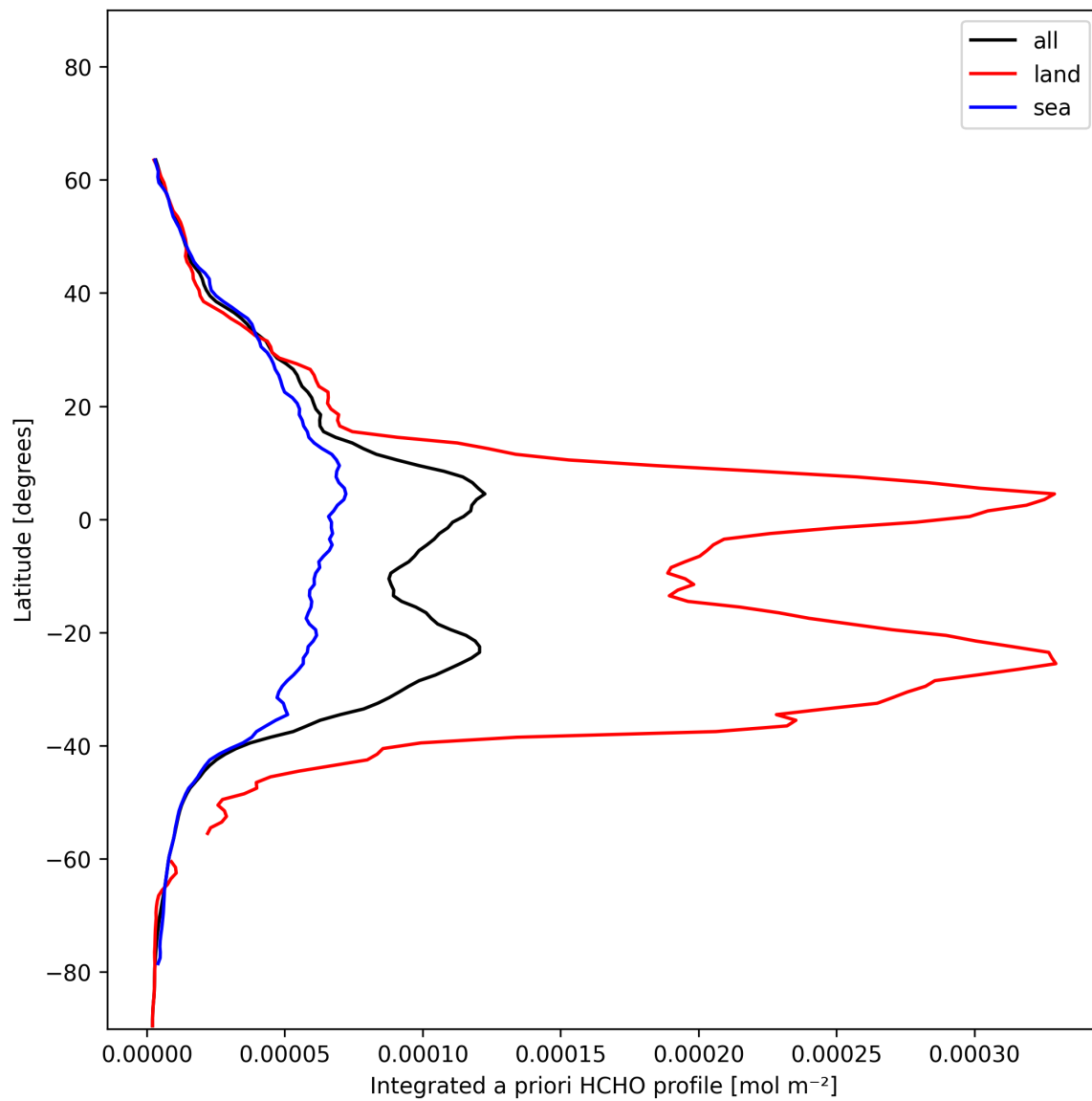
Figure 27: Zonal average of “Integrated a priori HCHO profile” for 2025-01-10 to 2025-01-10.
