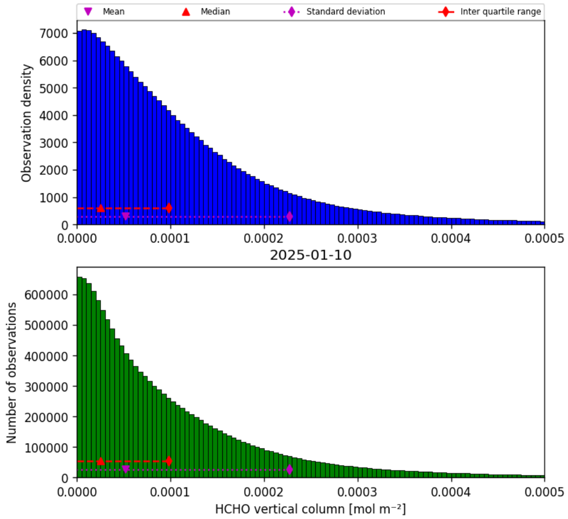
Figure 33: Histogram of “HCHO vertical column” for 2025-01-10 to 2025-01-10
