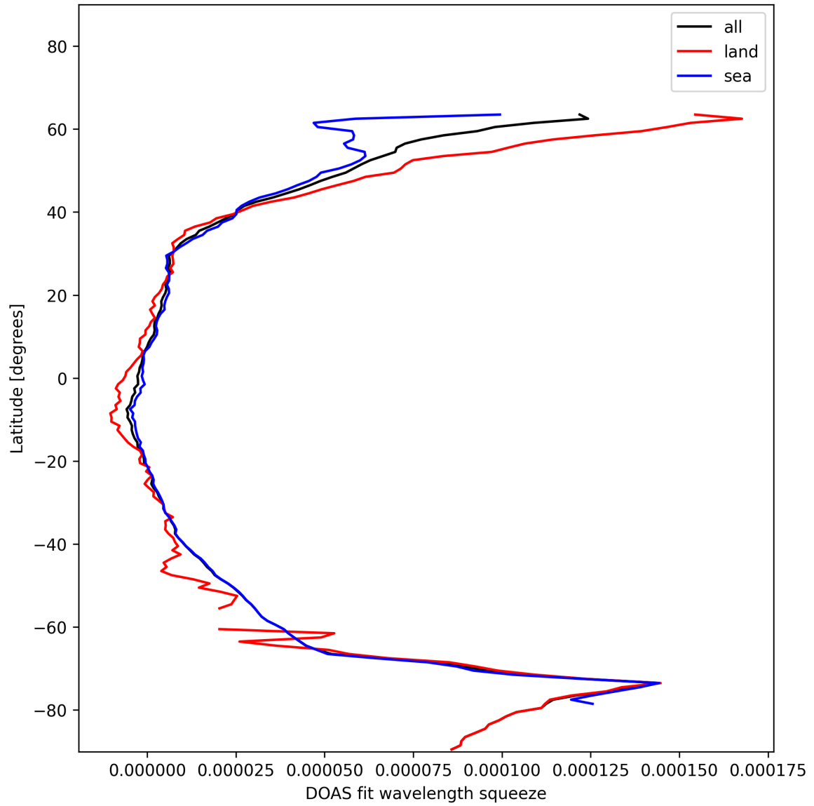
Figure 29: Zonal average of “DOAS fit wavelength squeeze” for 2025-01-10 to 2025-01-10.
