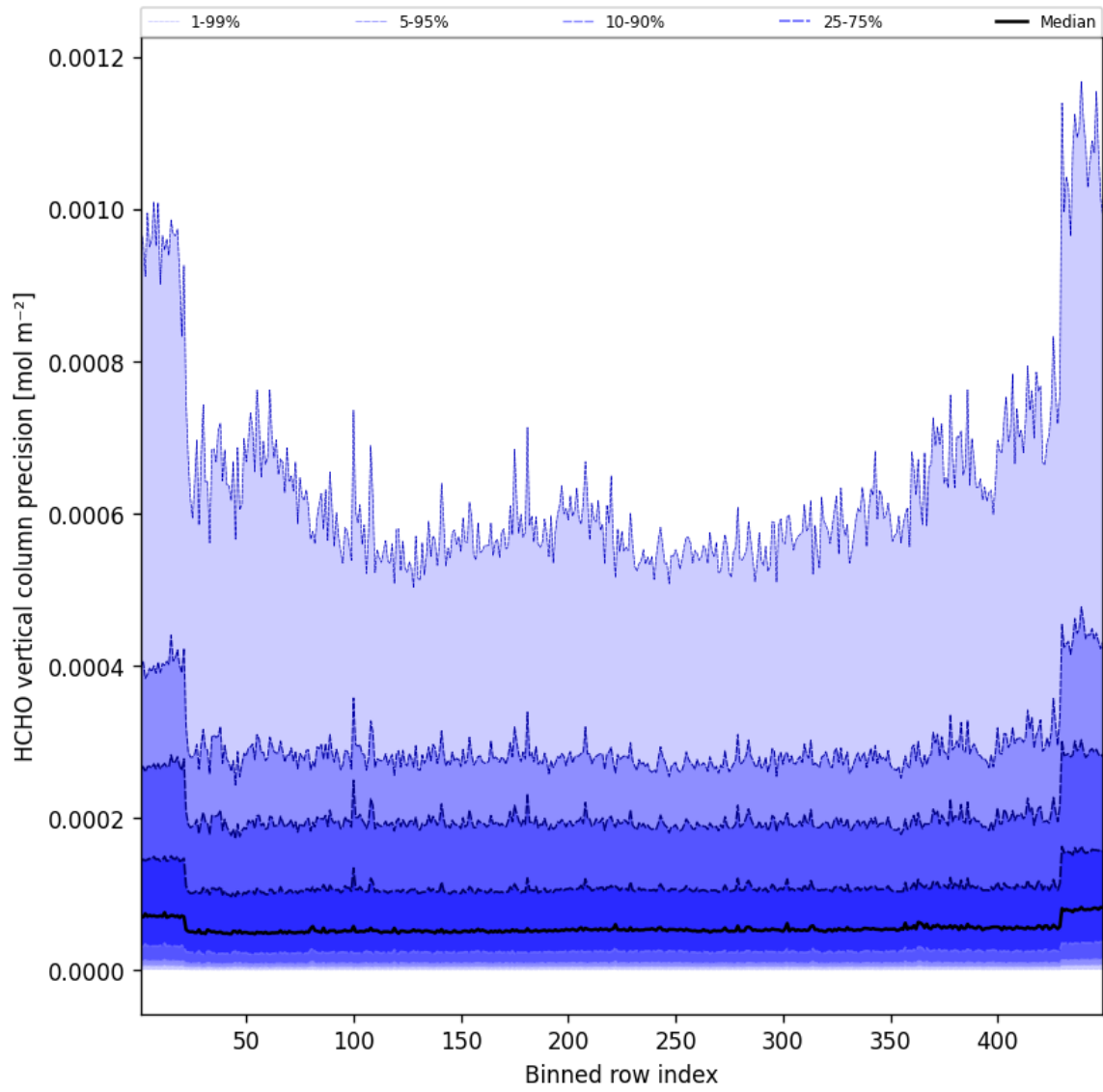
Figure 48: Along track statistics of “HCHO vertical column precision” for 2025-01-10 to 2025-01-10
