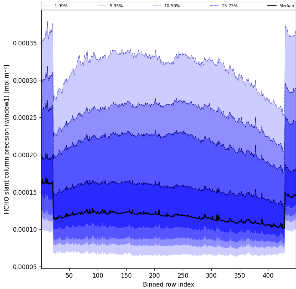
Figure 51: Along track statistics of “HCHO slant column precision (window1)” for 2025-01-10 to 2025-01-10
