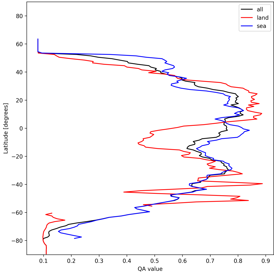
Figure 18: Zonal average of “QA value” for 2025-01-10 to 2025-01-10.
