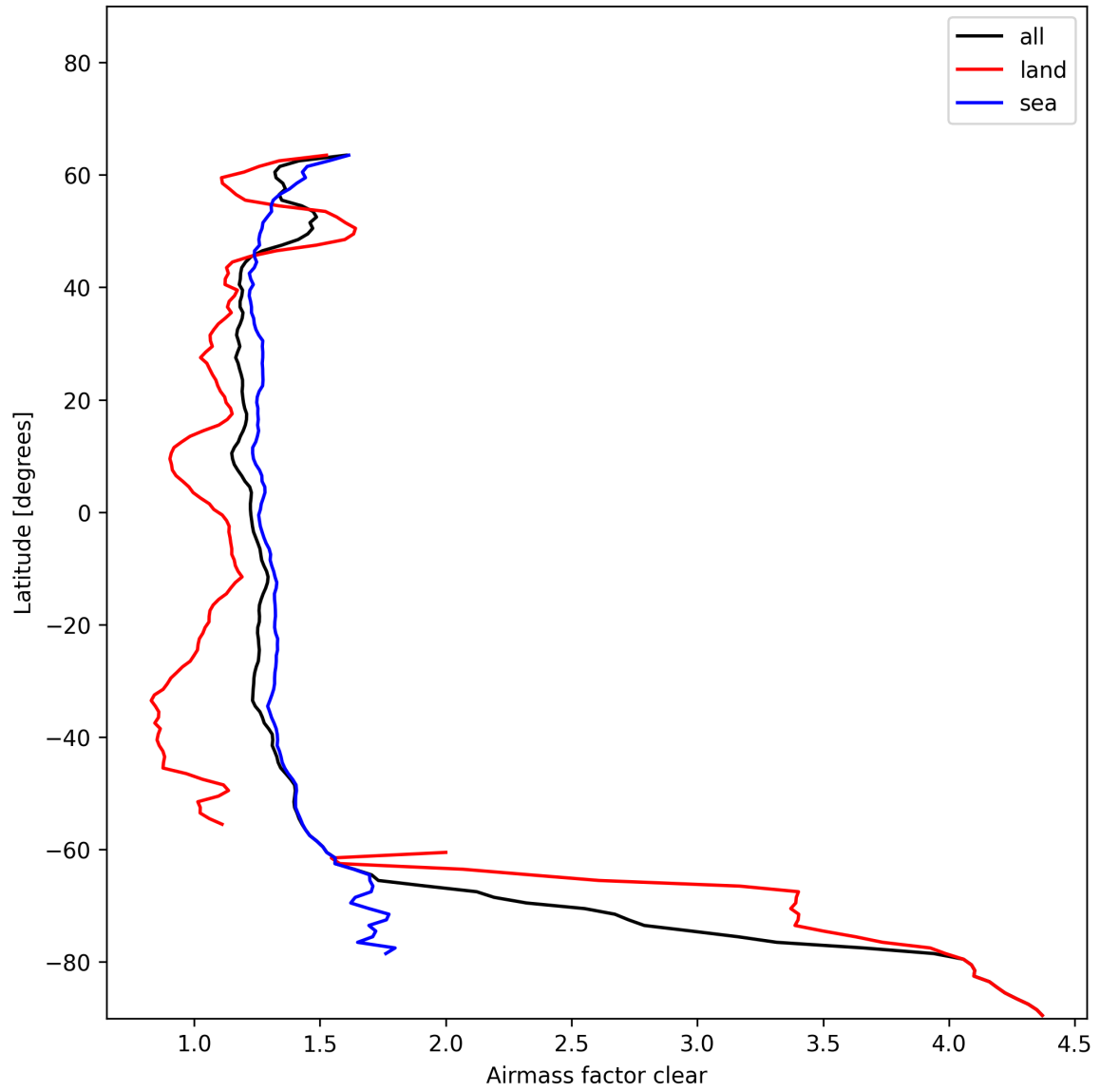
Figure 26: Zonal average of “Airmass factor clear” for 2025-01-10 to 2025-01-10.
