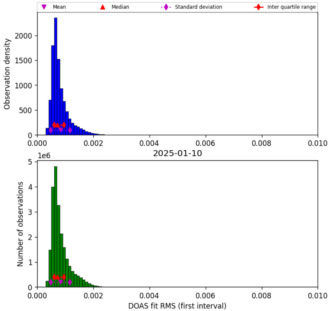
Figure 44: Histogram of “DOAS fit RMS (first interval)” for 2025-01-10 to 2025-01-10
