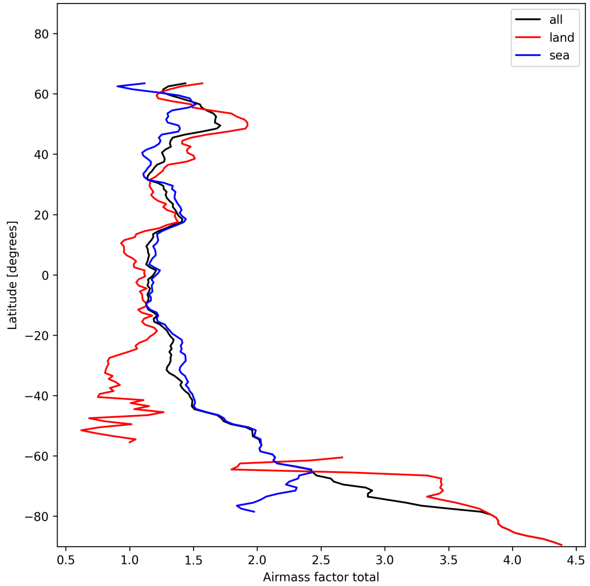
Figure 24: Zonal average of “Airmass factor total” for 2025-01-11 to 2025-01-12.
