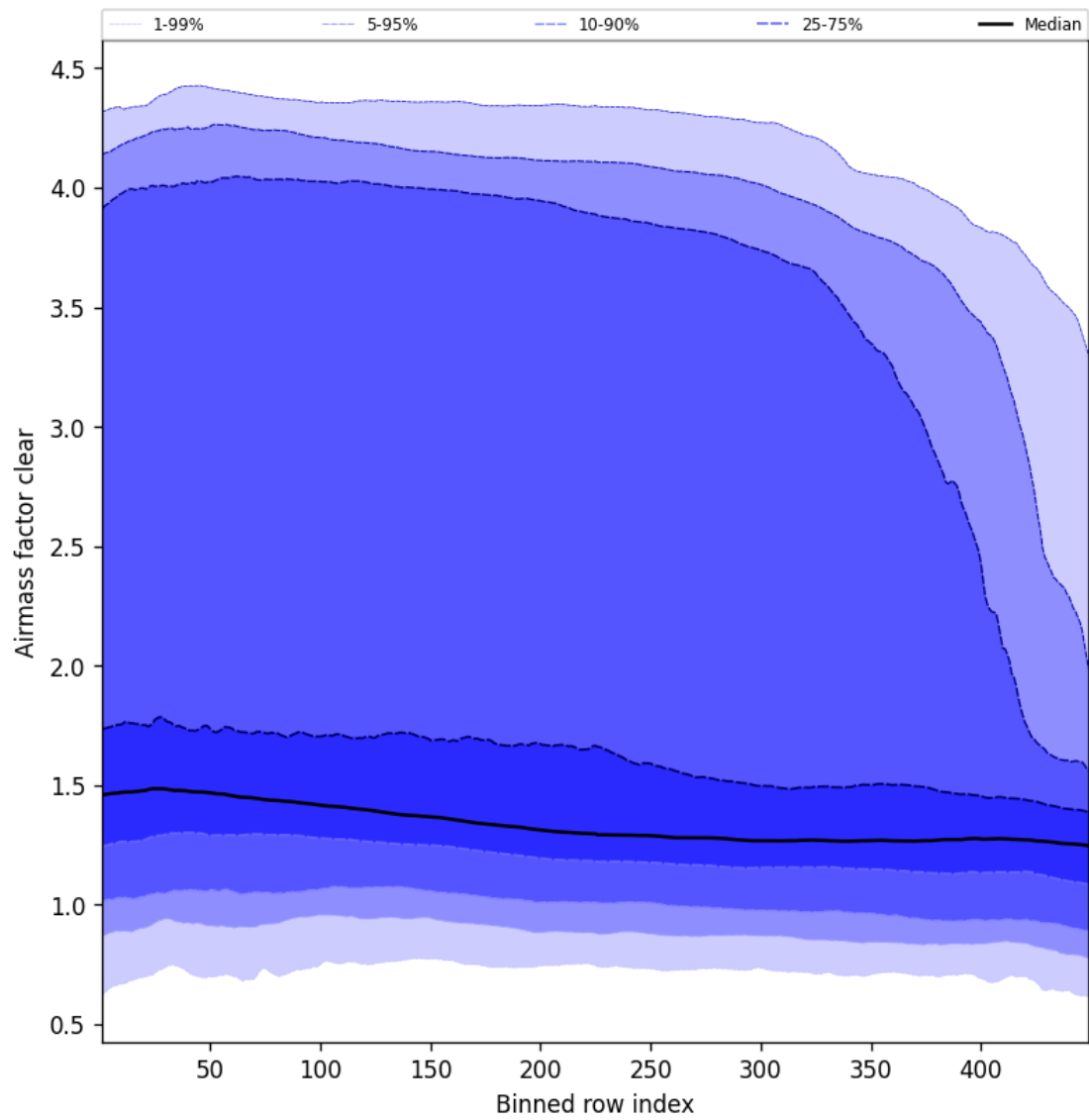
Figure 54: Along track statistics of “Airmass factor clear” for 2025-01-11 to 2025-01-12
