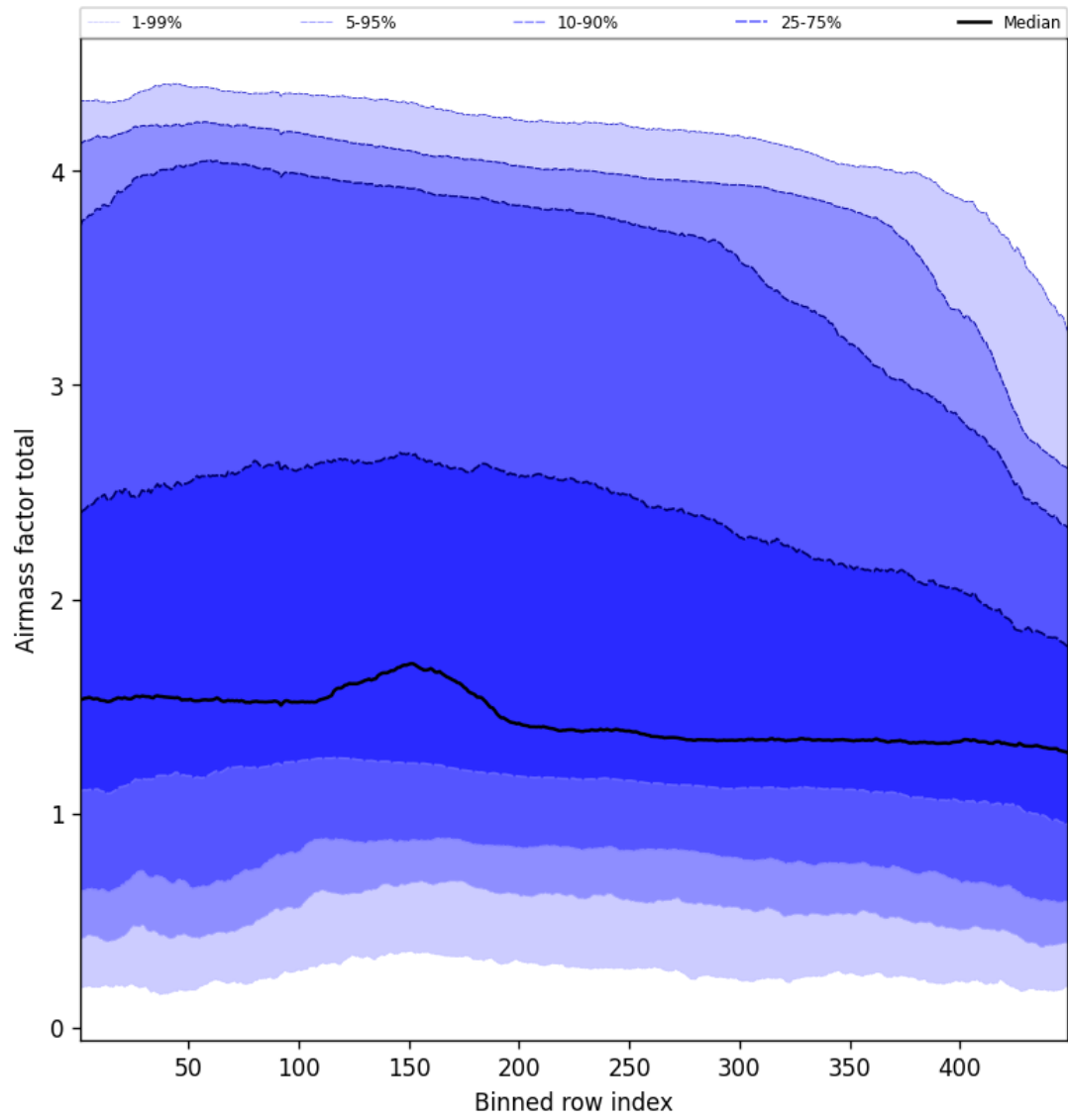
Figure 52: Along track statistics of “Airmass factor total” for 2025-01-11 to 2025-01-12
