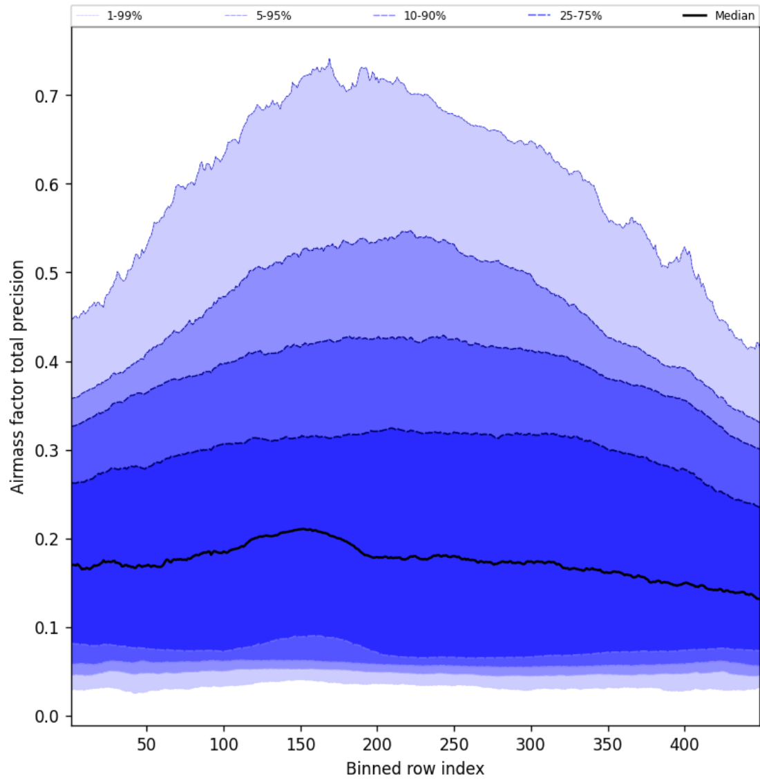
Figure 53: Along track statistics of “Airmass factor total precision” for 2025-01-11 to 2025-01-12
