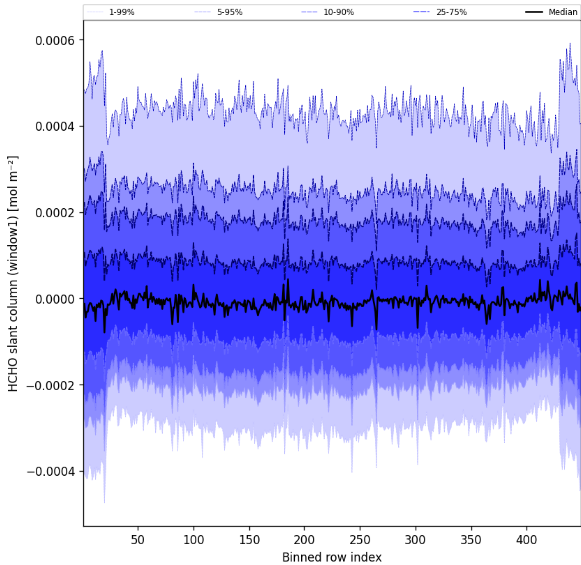
Figure 50: Along track statistics of “HCHO slant column (window1)” for 2025-01-11 to 2025-01-12
