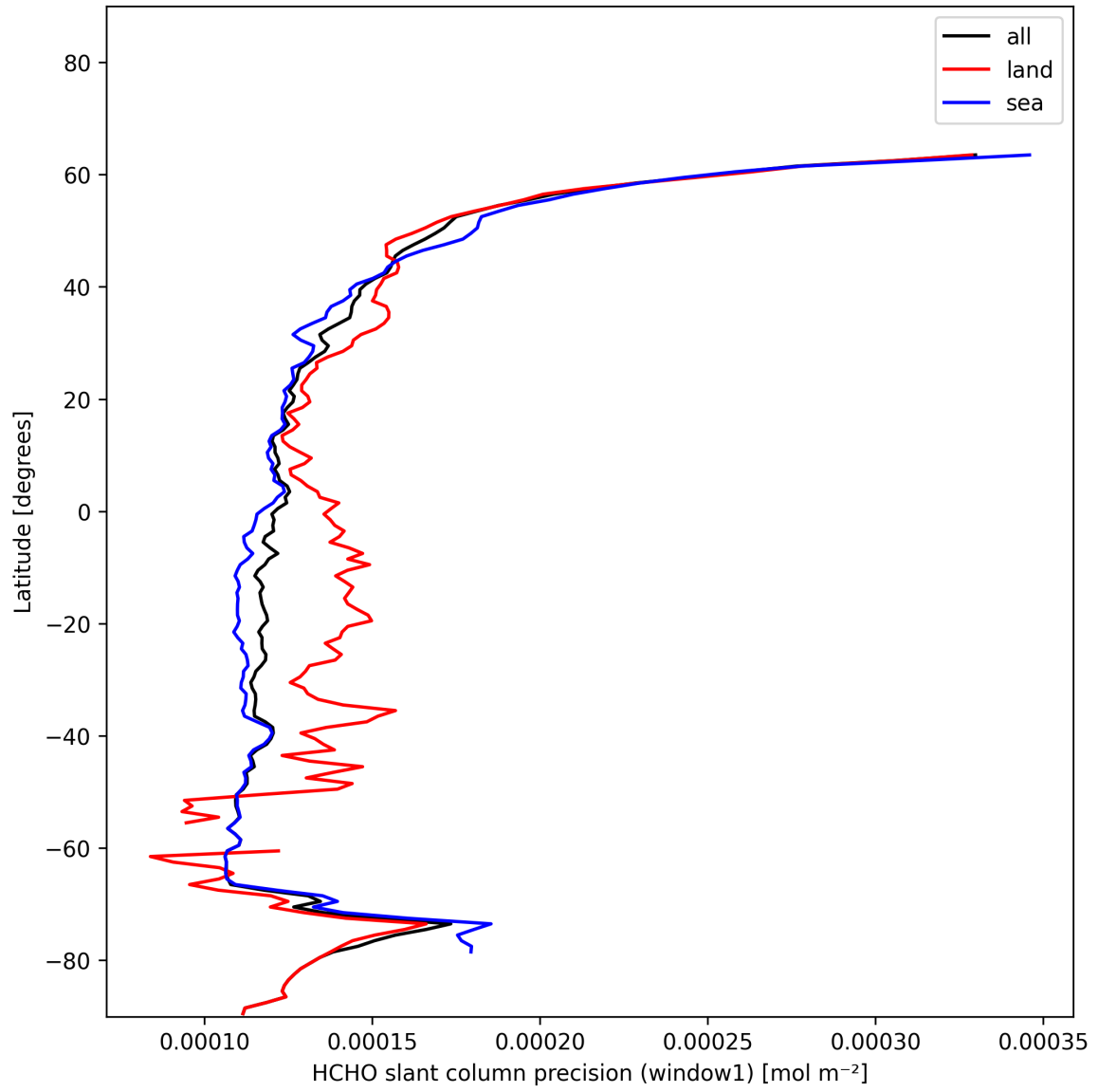
Figure 23: Zonal average of “HCHO slant column precision (window1)” for 2025-01-11 to 2025-01-12.
