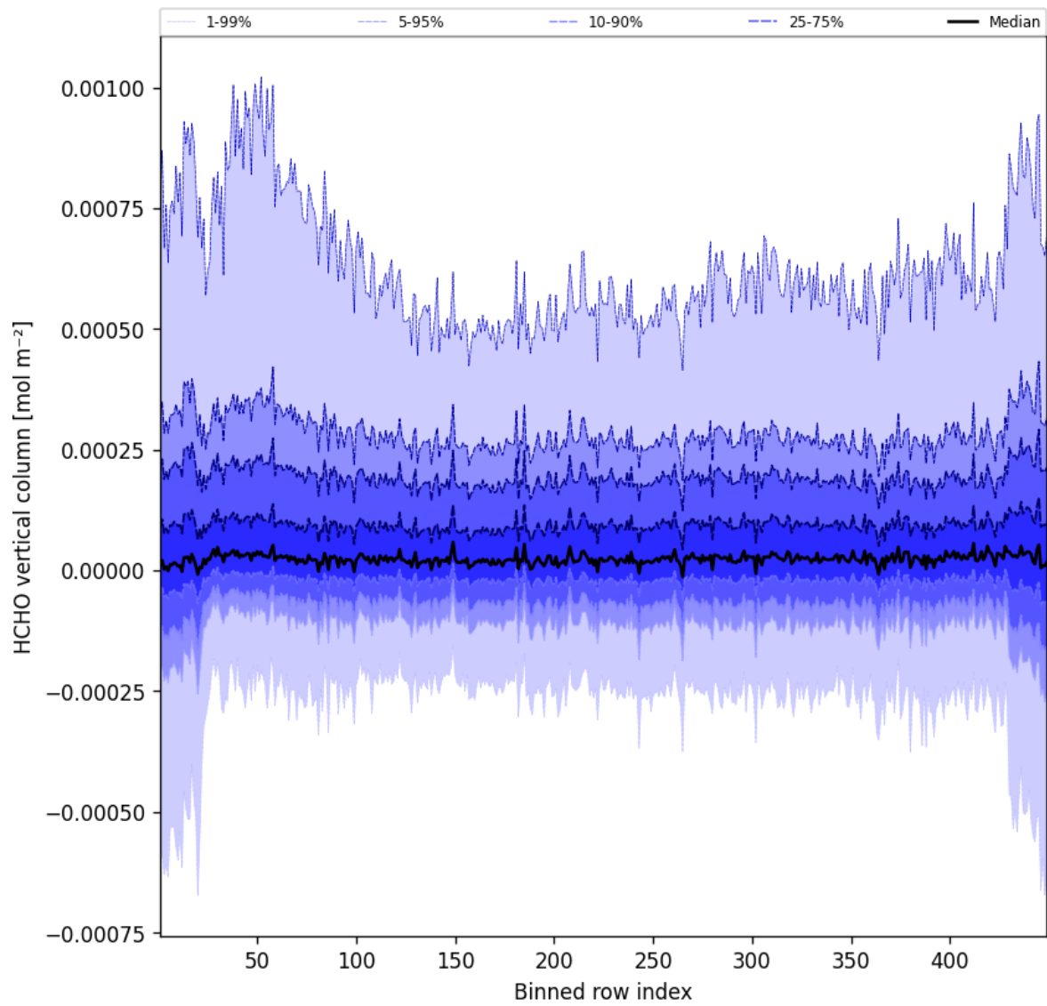
Figure 47: Along track statistics of “HCHO vertical column” for 2025-01-11 to 2025-01-12
