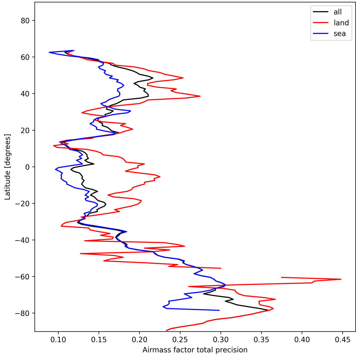
Figure 25: Zonal average of “Airmass factor total precision” for 2025-01-11 to 2025-01-12.
