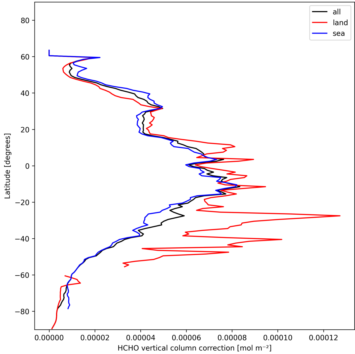
Figure 21: Zonal average of “HCHO vertical column correction” for 2025-01-11 to 2025-01-12.
