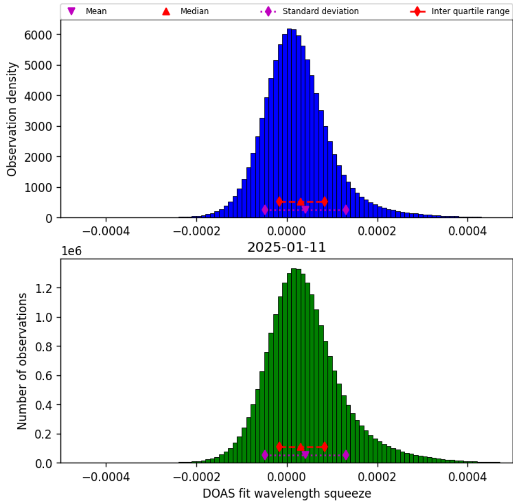
Figure 43: Histogram of “DOAS fit wavelength squeeze” for 2025-01-11 to 2025-01-12
