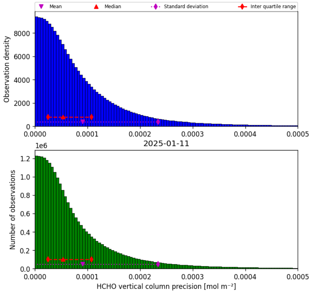
Figure 34: Histogram of “HCHO vertical column precision” for 2025-01-11 to 2025-01-12
