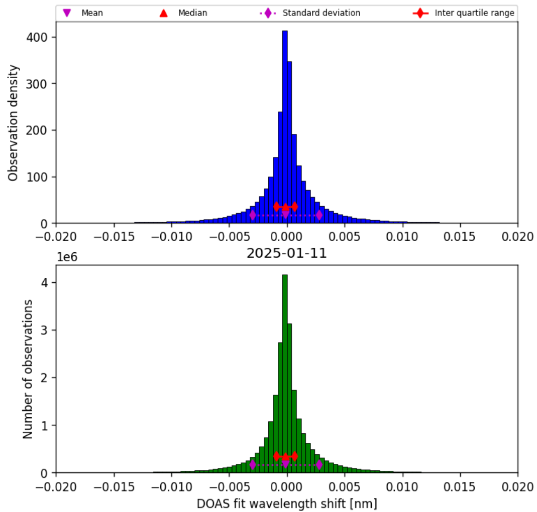
Figure 42: Histogram of “DOAS fit wavelength shift” for 2025-01-11 to 2025-01-12
