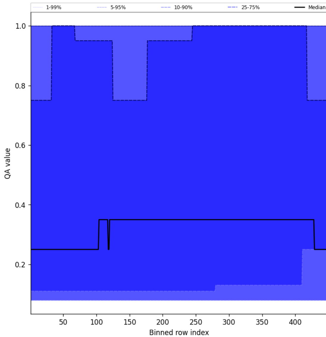
Figure 46: Along track statistics of “QA value” for 2025-01-11 to 2025-01-12
