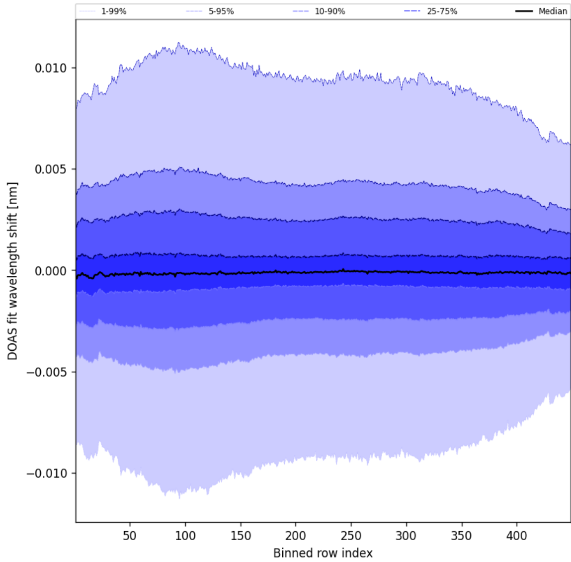
Figure 56: Along track statistics of “DOAS fit wavelength shift” for 2025-01-11 to 2025-01-12
