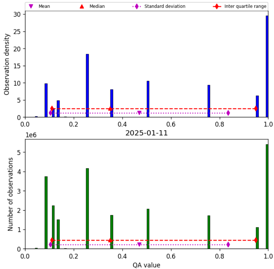
Figure 32: Histogram of “QA value” for 2025-01-11 to 2025-01-12
