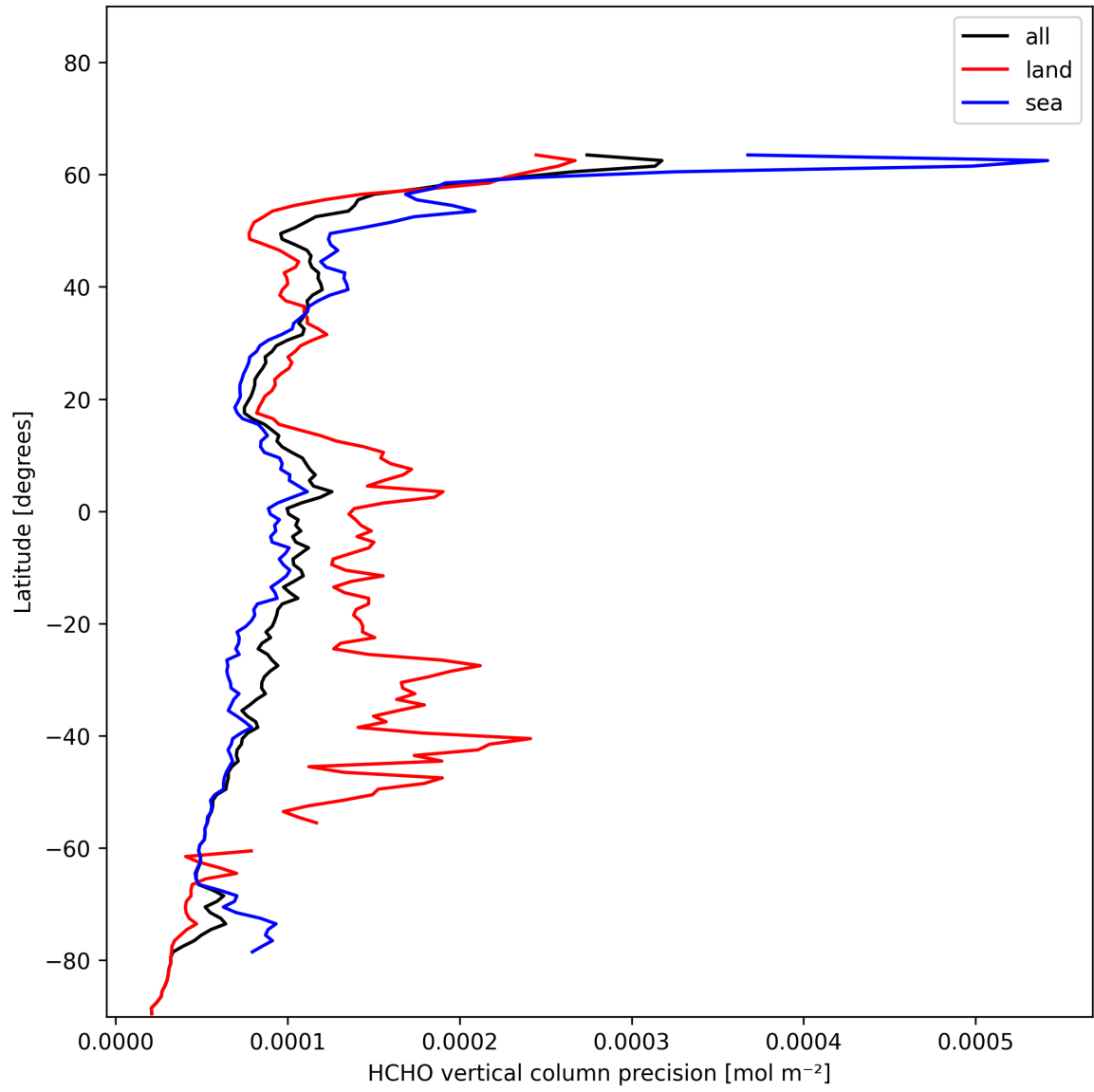
Figure 20: Zonal average of "HCHO vertical column precision" for 2025-01-11 to 2025-01-12.
