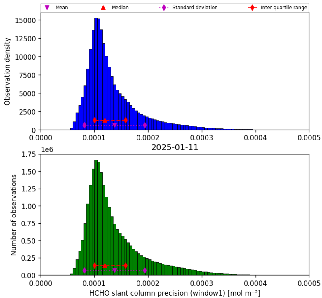
Figure 37: Histogram of “HCHO slant column precision (window1)” for 2025-01-11 to 2025-01-12
