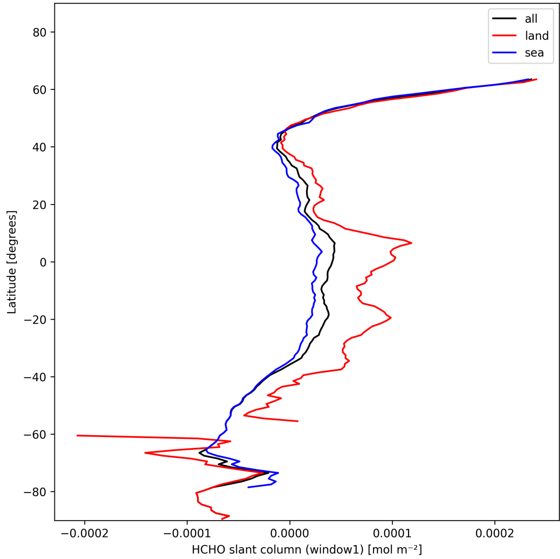
Figure 22: Zonal average of “HCHO slant column (window1)” for 2025-01-11 to 2025-01-12.
