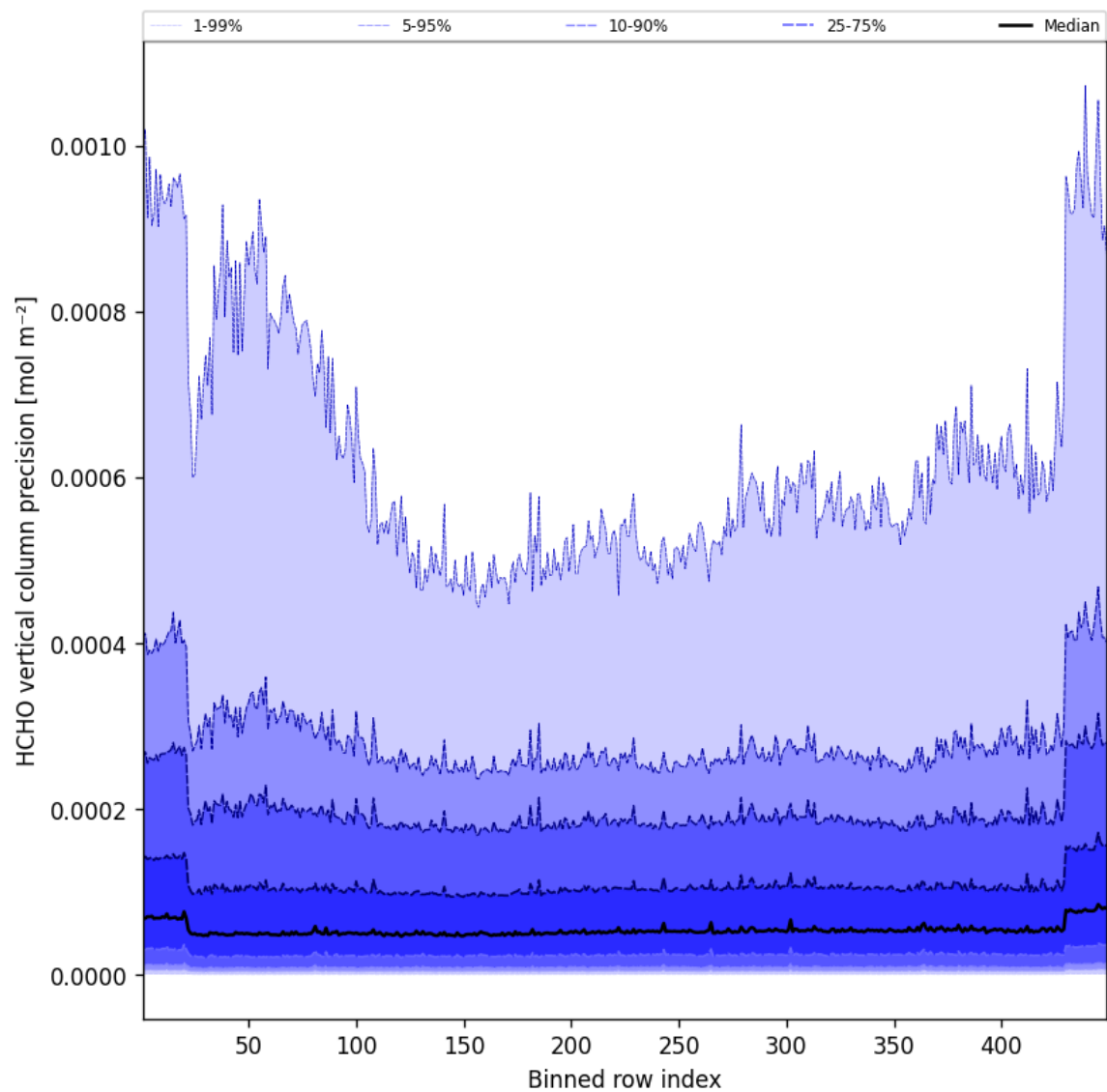
Figure 48: Along track statistics of “HCHO vertical column precision” for 2025-01-11 to 2025-01-12
