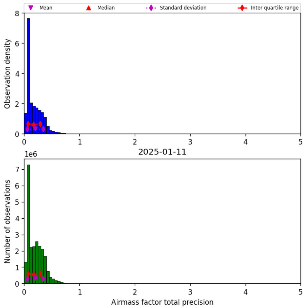
Figure 39: Histogram of “Airmass factor total precision” for 2025-01-11 to 2025-01-12
