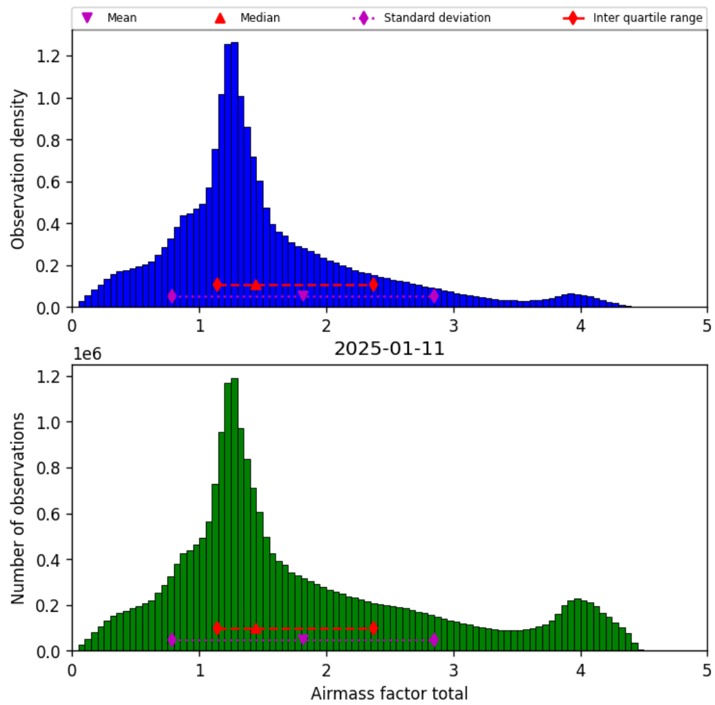
Figure 38: Histogram of “Airmass factor total” for 2025-01-11 to 2025-01-12
