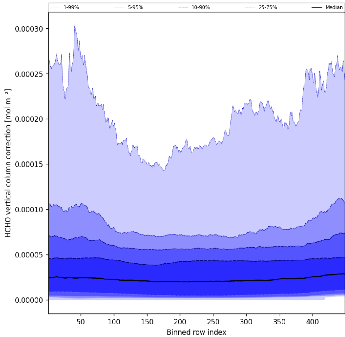
Figure 49: Along track statistics of “HCHO vertical column correction” for 2025-01-11 to 2025-01-12
