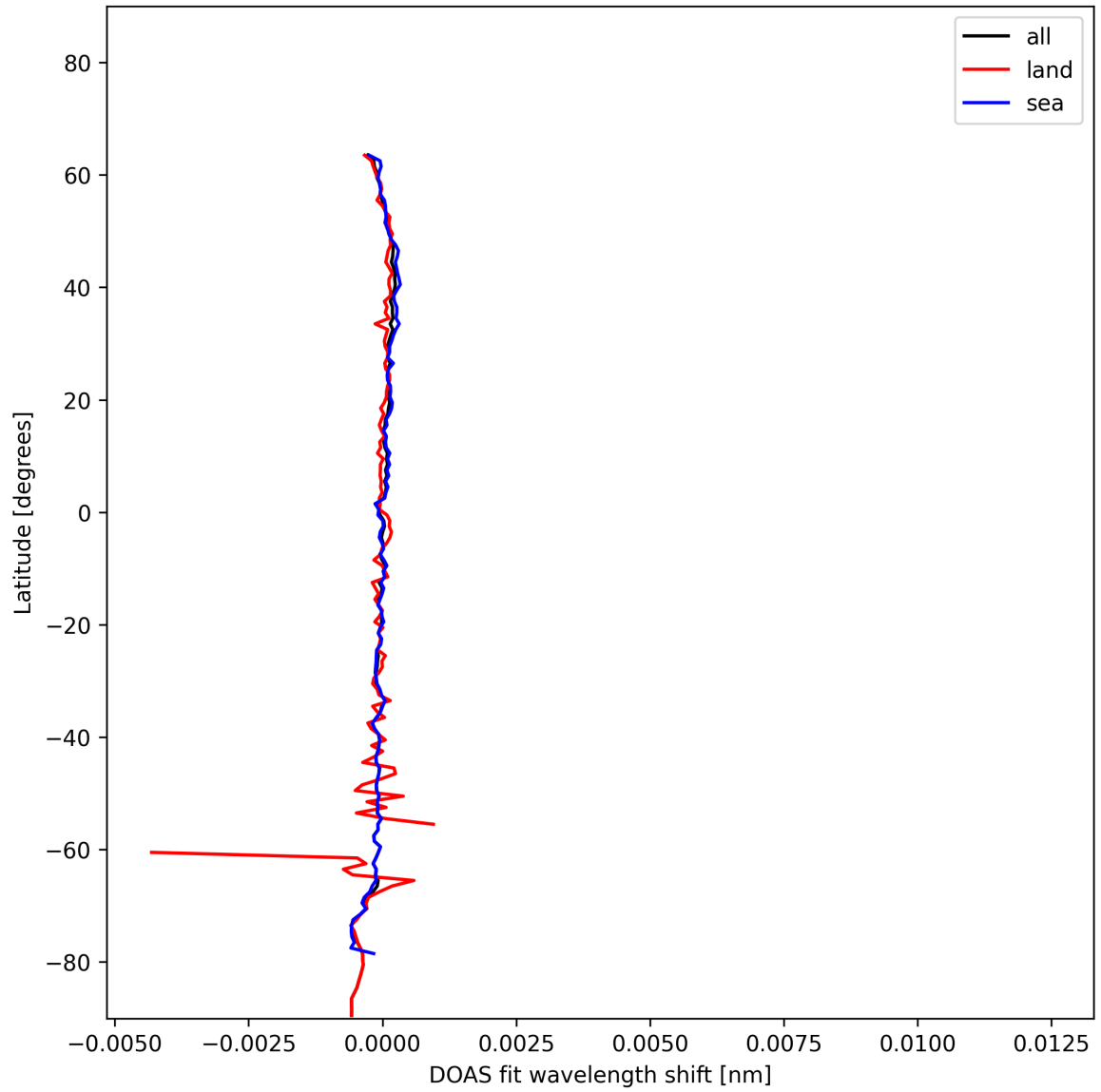
Figure 28: Zonal average of "DOAS fit wavelength shift" for 2025-01-11 to 2025-01-12.
