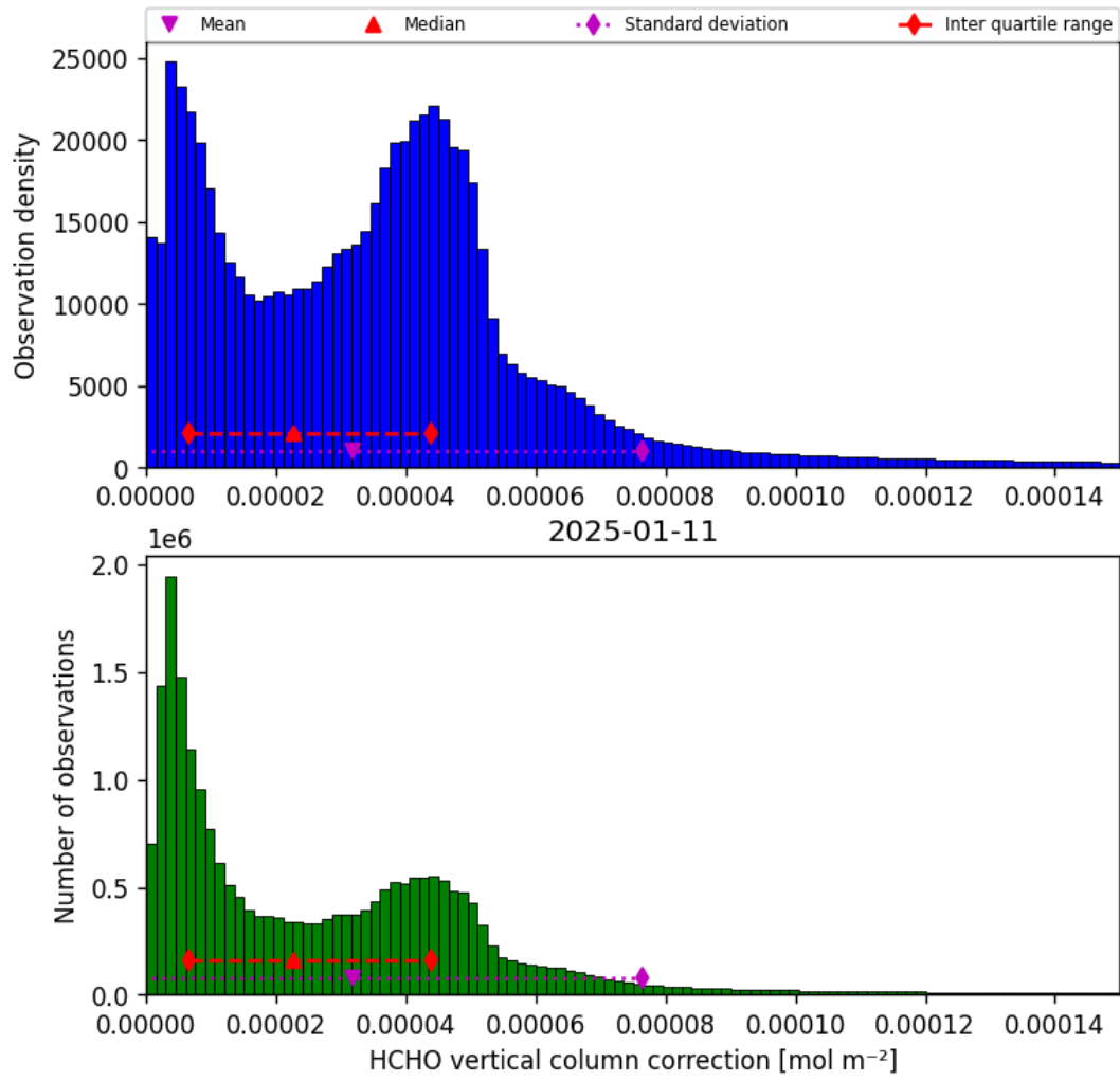
Figure 35: Histogram of “HCHO vertical column correction” for 2025-01-11 to 2025-01-12
