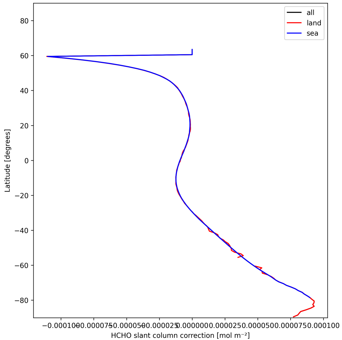
Figure 31: Zonal average of “HCHO slant column correction” for 2025-01-11 to 2025-01-12.
