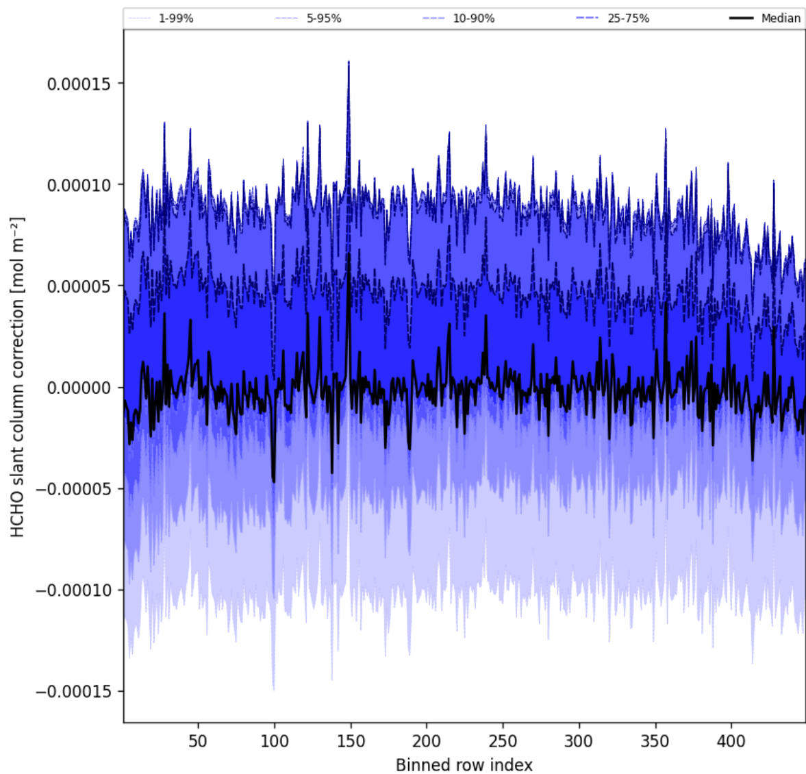
Figure 59: Along track statistics of “HCHO slant column correction” for 2025-01-11 to 2025-01-12
