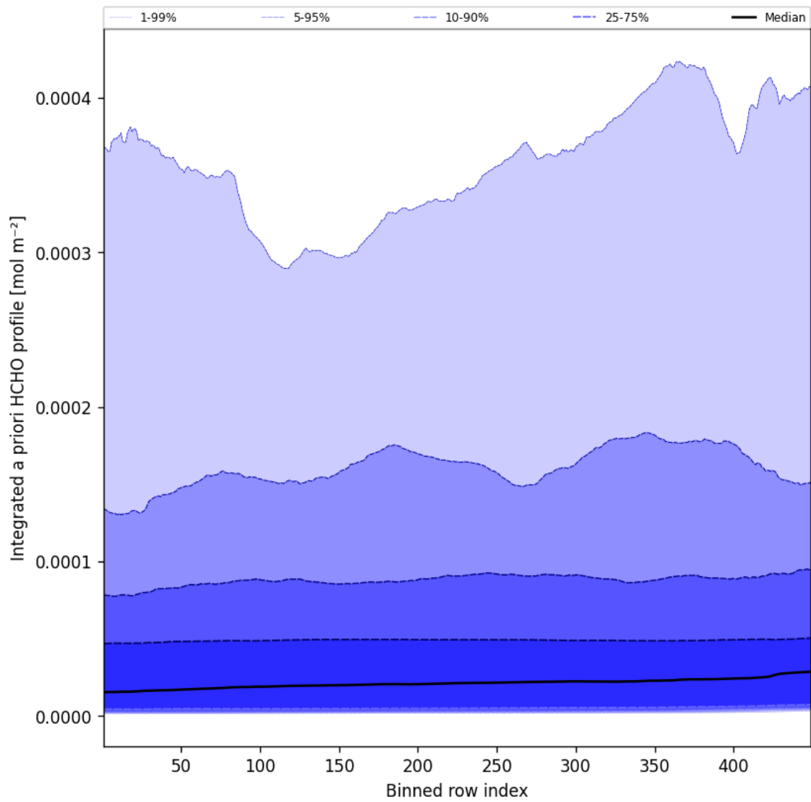
Figure 55: Along track statistics of “Integrated a priori HCHO profile” for 2025-01-11 to 2025-01-12
