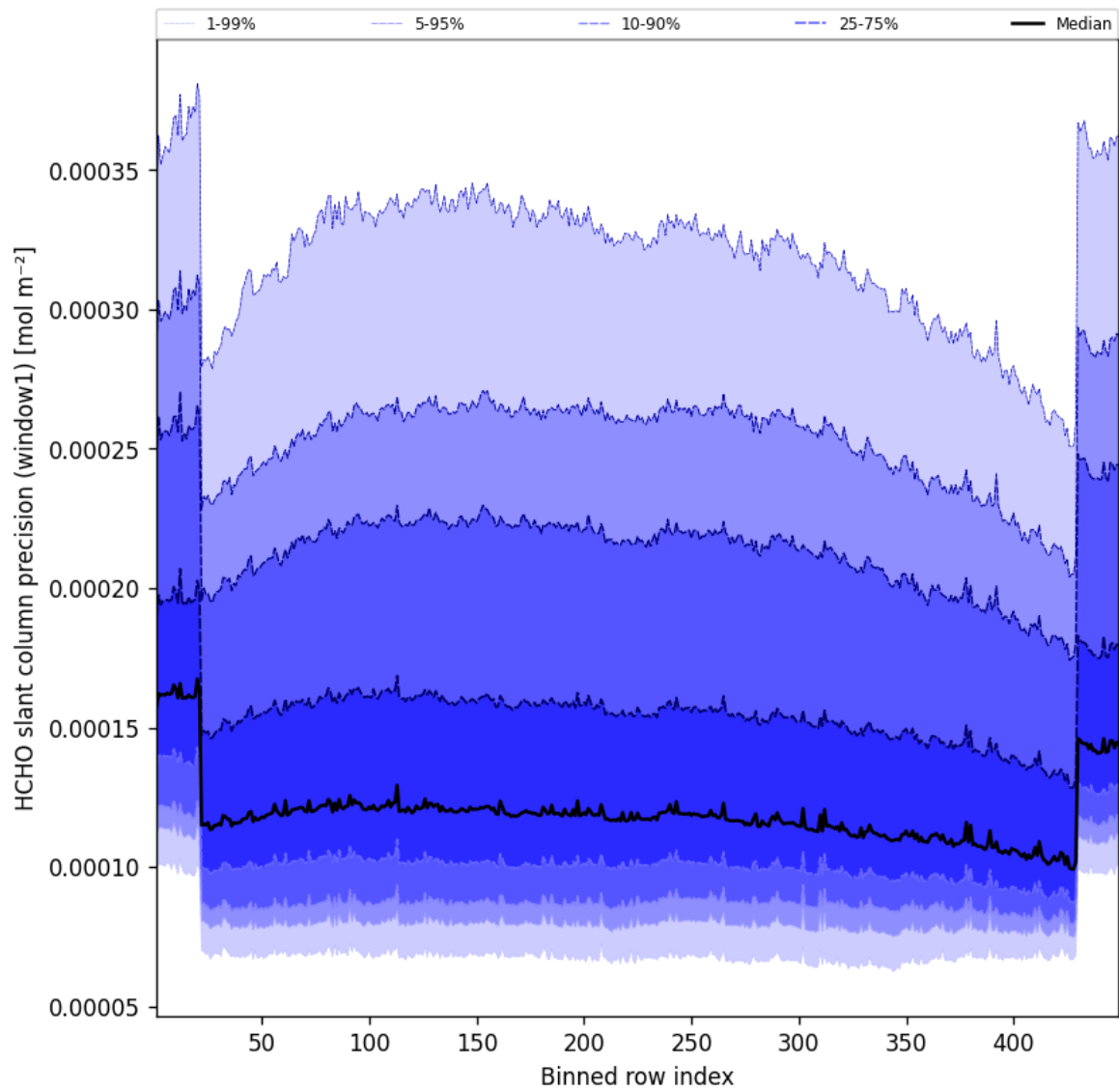
Figure 51: Along track statistics of “HCHO slant column precision (window1)” for 2025-01-11 to 2025-01-12
