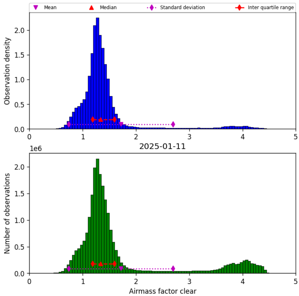
Figure 40: Histogram of “Airmass factor clear” for 2025-01-11 to 2025-01-12
