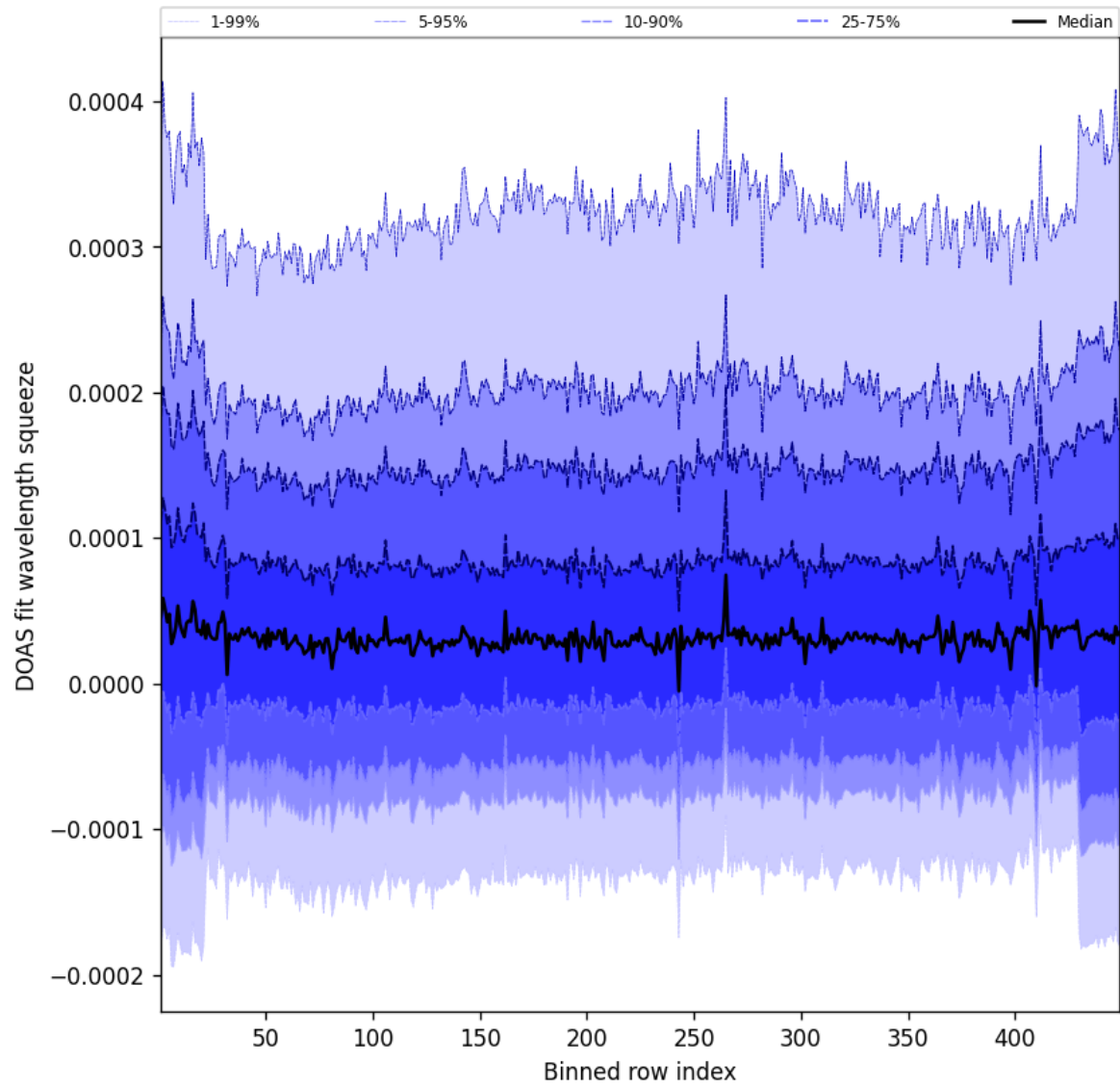
Figure 57: Along track statistics of “DOAS fit wavelength squeeze” for 2025-01-11 to 2025-01-12
