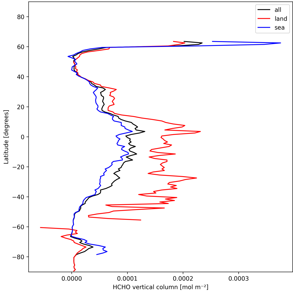
Figure 19: Zonal average of “HCHO vertical column” for 2025-01-11 to 2025-01-12.
