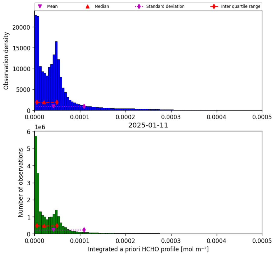
Figure 41: Histogram of “Integrated a priori HCHO profile” for 2025-01-11 to 2025-01-12
