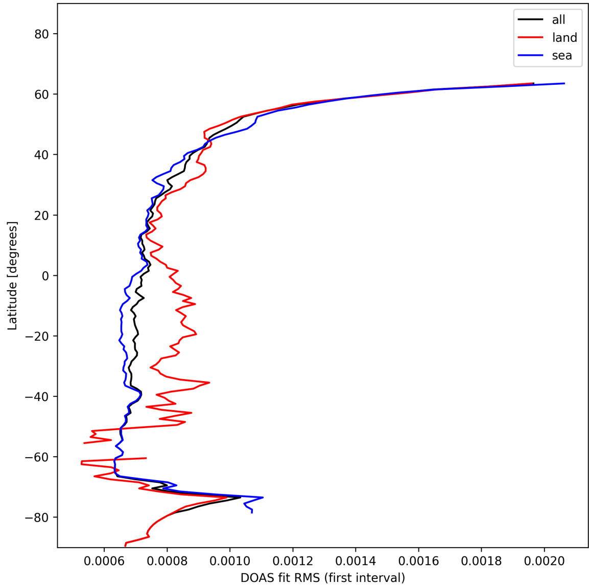
Figure 30: Zonal average of “DOAS fit RMS (first interval)” for 2025-01-11 to 2025-01-12.
