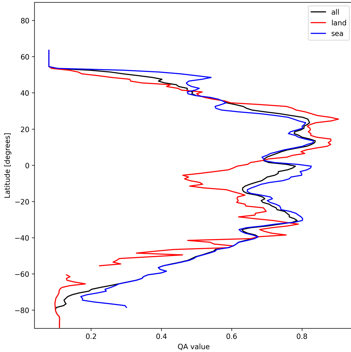
Figure 18: Zonal average of “QA value” for 2025-01-11 to 2025-01-12.
