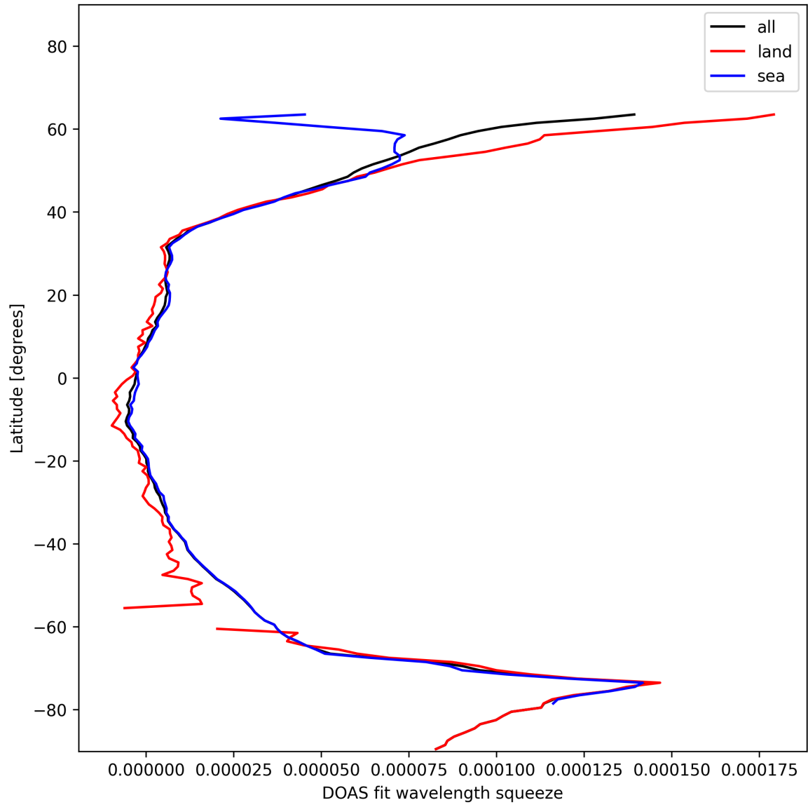
Figure 29: Zonal average of “DOAS fit wavelength squeeze” for 2025-01-11 to 2025-01-12.
