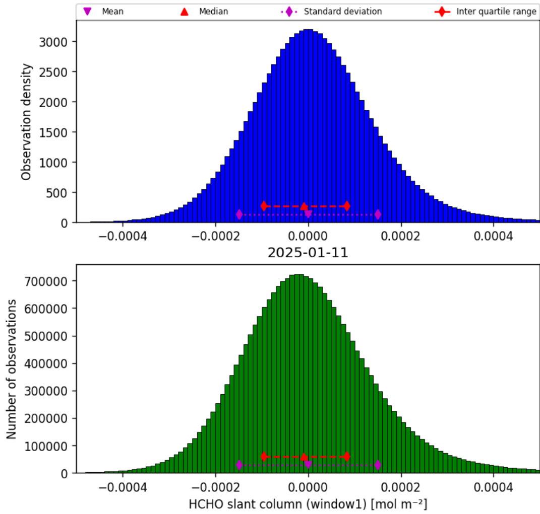
Figure 36: Histogram of “HCHO slant column (window1)” for 2025-01-11 to 2025-01-12
