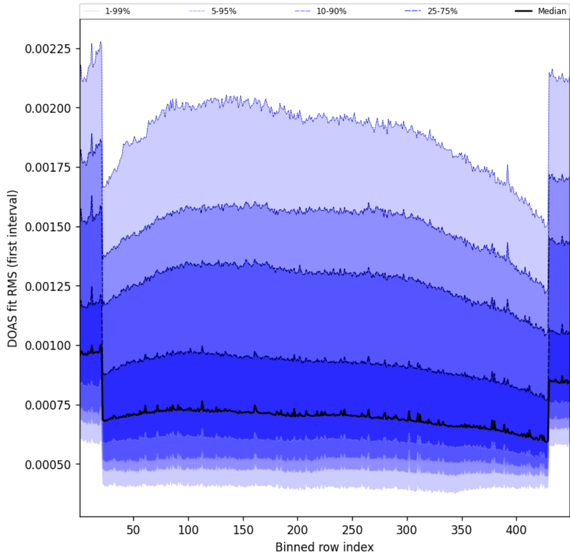
Figure 58: Along track statistics of “DOAS fit RMS (first interval)” for 2025-01-11 to 2025-01-12
