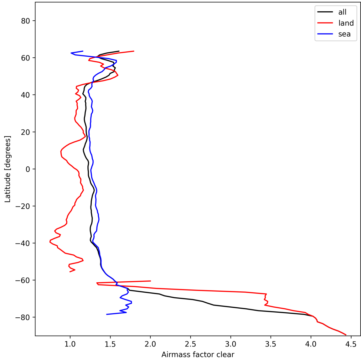
Figure 26: Zonal average of “Airmass factor clear” for 2025-01-11 to 2025-01-12.
