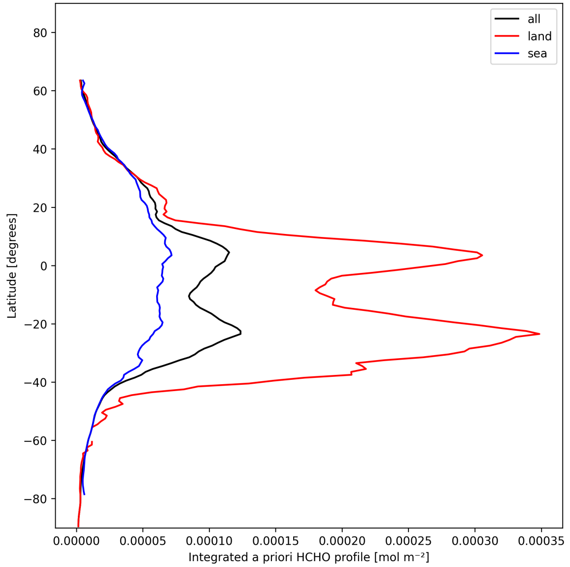
Figure 27: Zonal average of “Integrated a priori HCHO profile” for 2025-01-11 to 2025-01-12.
