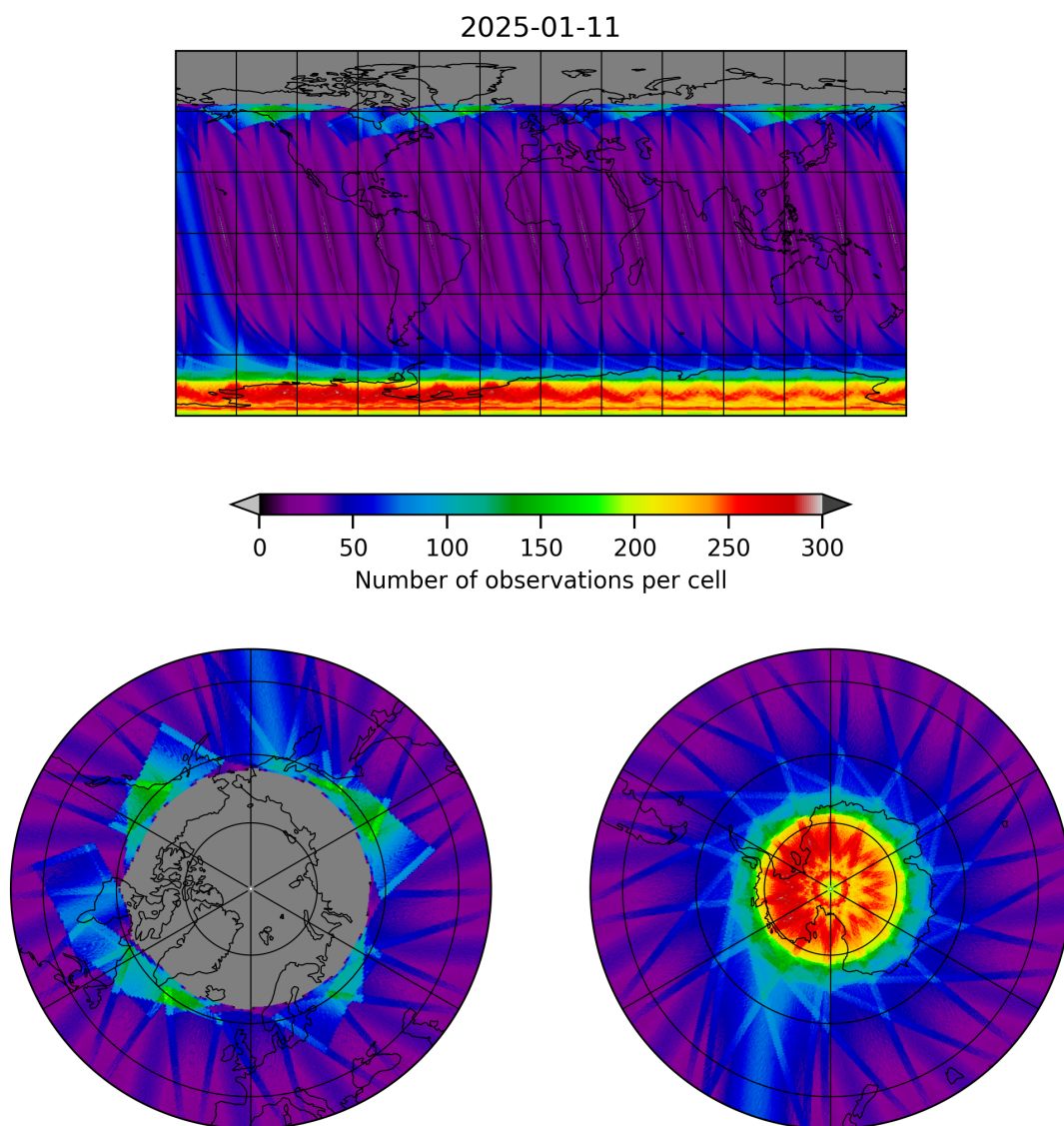
Figure 17: Map of the number of observations for 2025-01-11 to 2025-01-12
