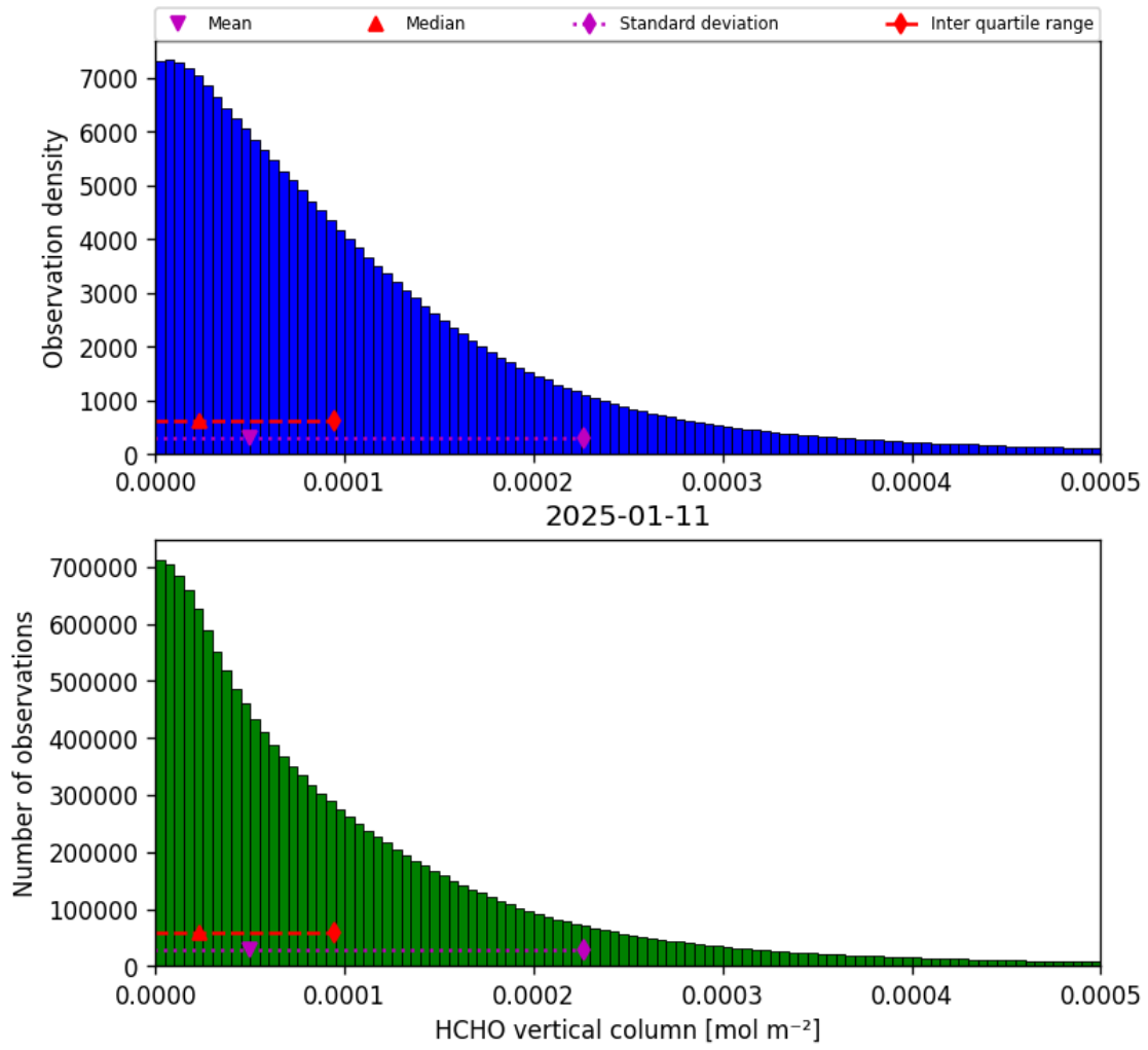
Figure 33: Histogram of “HCHO vertical column” for 2025-01-11 to 2025-01-12
