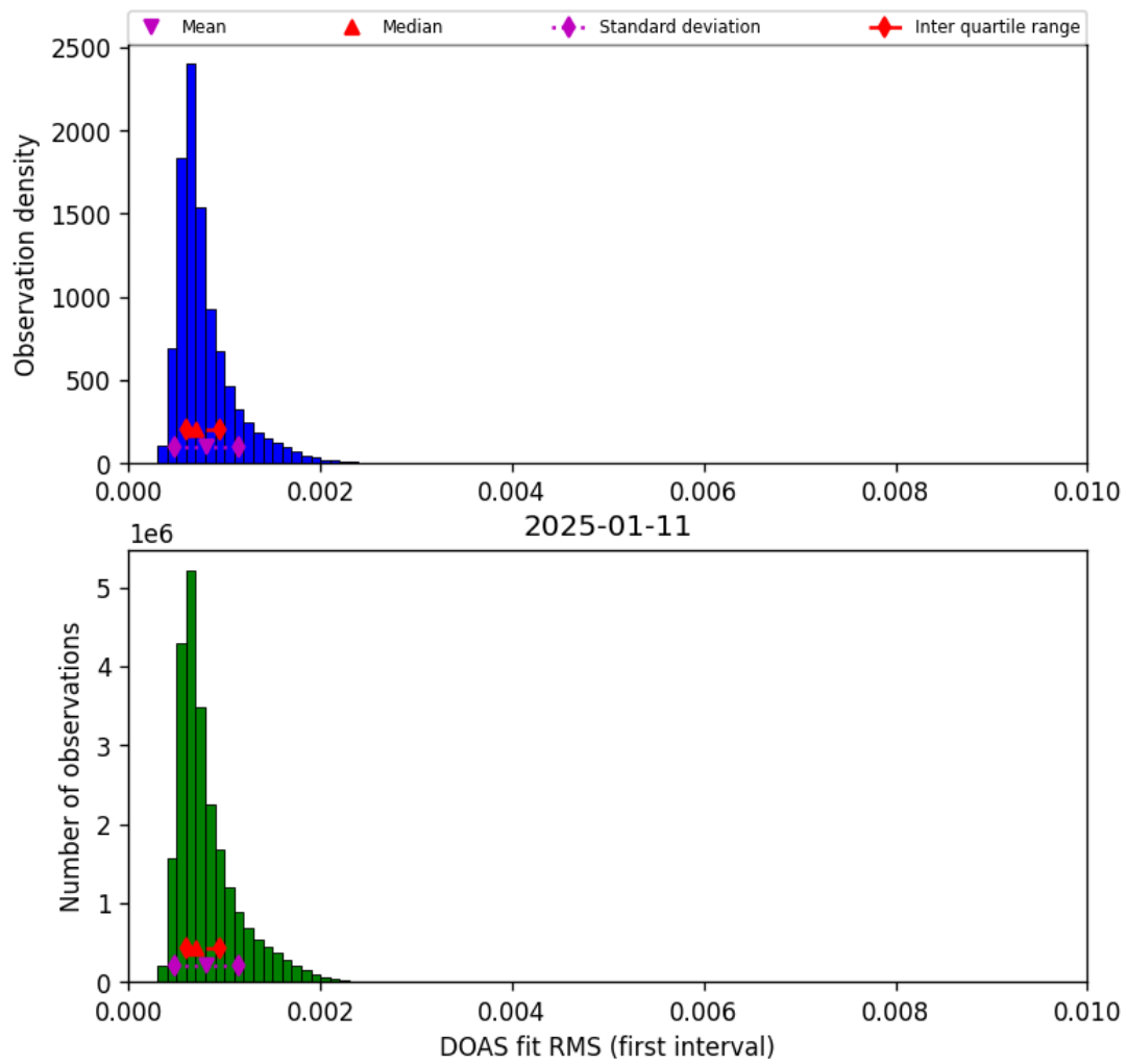
Figure 44: Histogram of “DOAS fit RMS (first interval)” for 2025-01-11 to 2025-01-12
