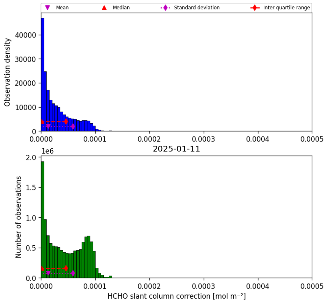
Figure 45: Histogram of “HCHO slant column correction” for 2025-01-11 to 2025-01-12
