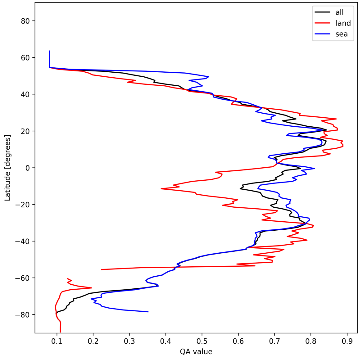
Figure 18: Zonal average of “QA value” for 2025-01-12 to 2025-01-13.
