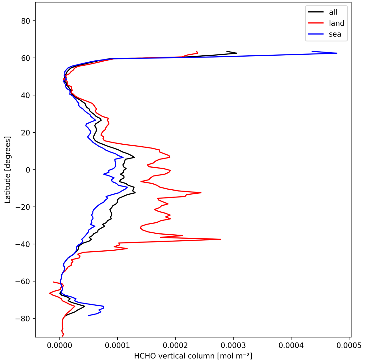
Figure 19: Zonal average of “HCHO vertical column” for 2025-01-12 to 2025-01-13.
