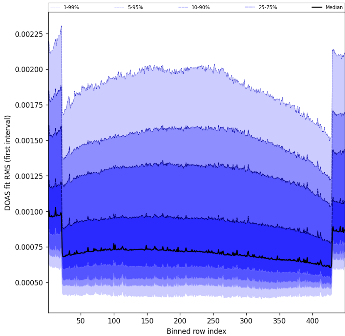
Figure 58: Along track statistics of “DOAS fit RMS (first interval)” for 2025-01-12 to 2025-01-13
