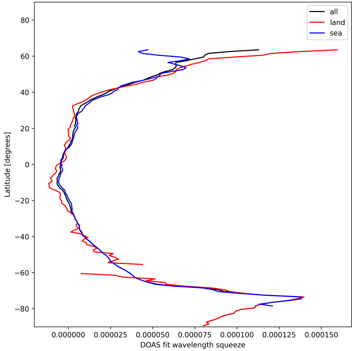
Figure 29: Zonal average of “DOAS fit wavelength squeeze” for 2025-01-12 to 2025-01-13.
