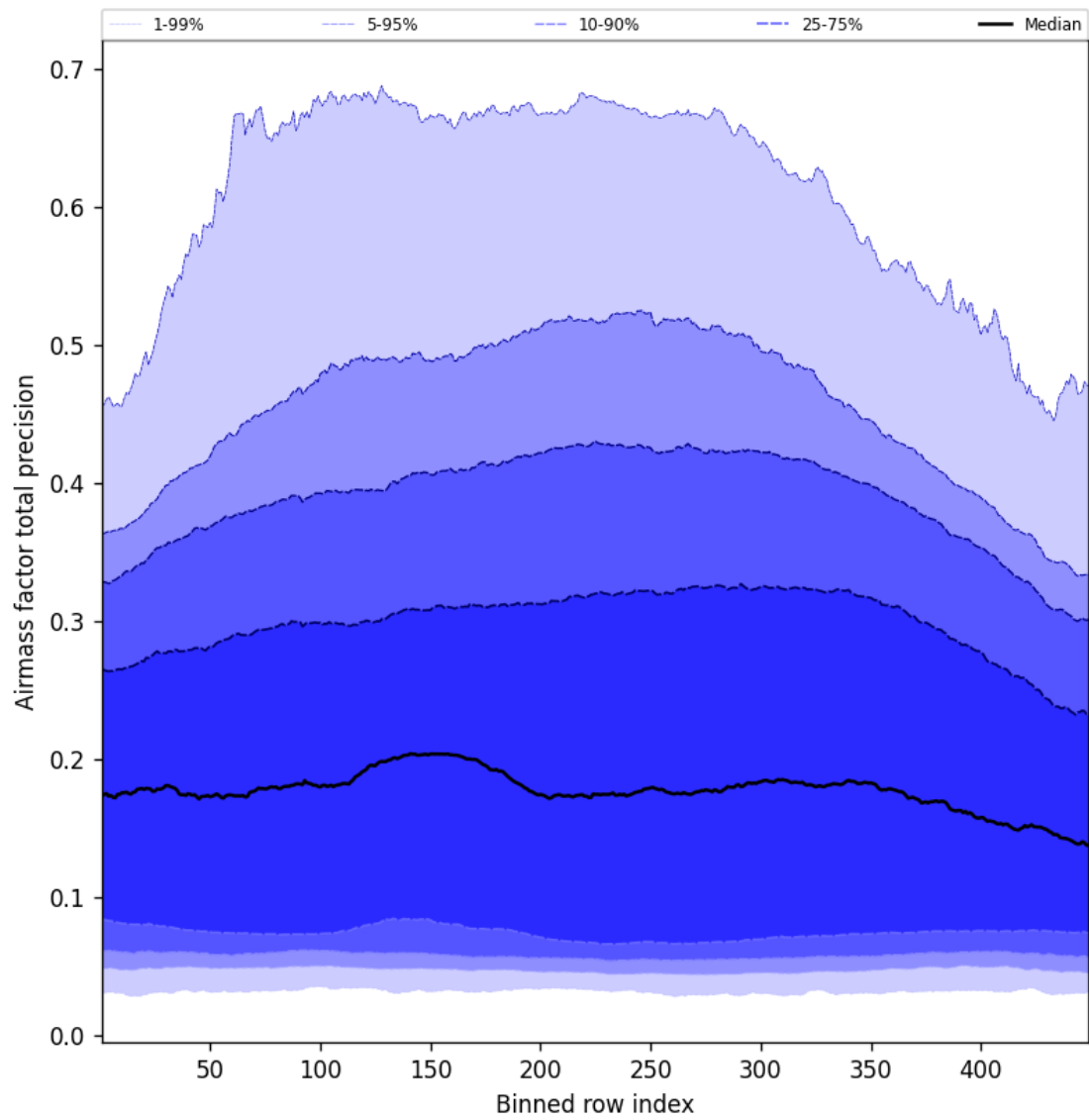
Figure 53: Along track statistics of “Airmass factor total precision” for 2025-01-12 to 2025-01-13
