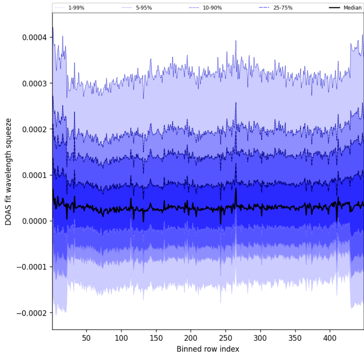
Figure 57: Along track statistics of “DOAS fit wavelength squeeze” for 2025-01-12 to 2025-01-13
