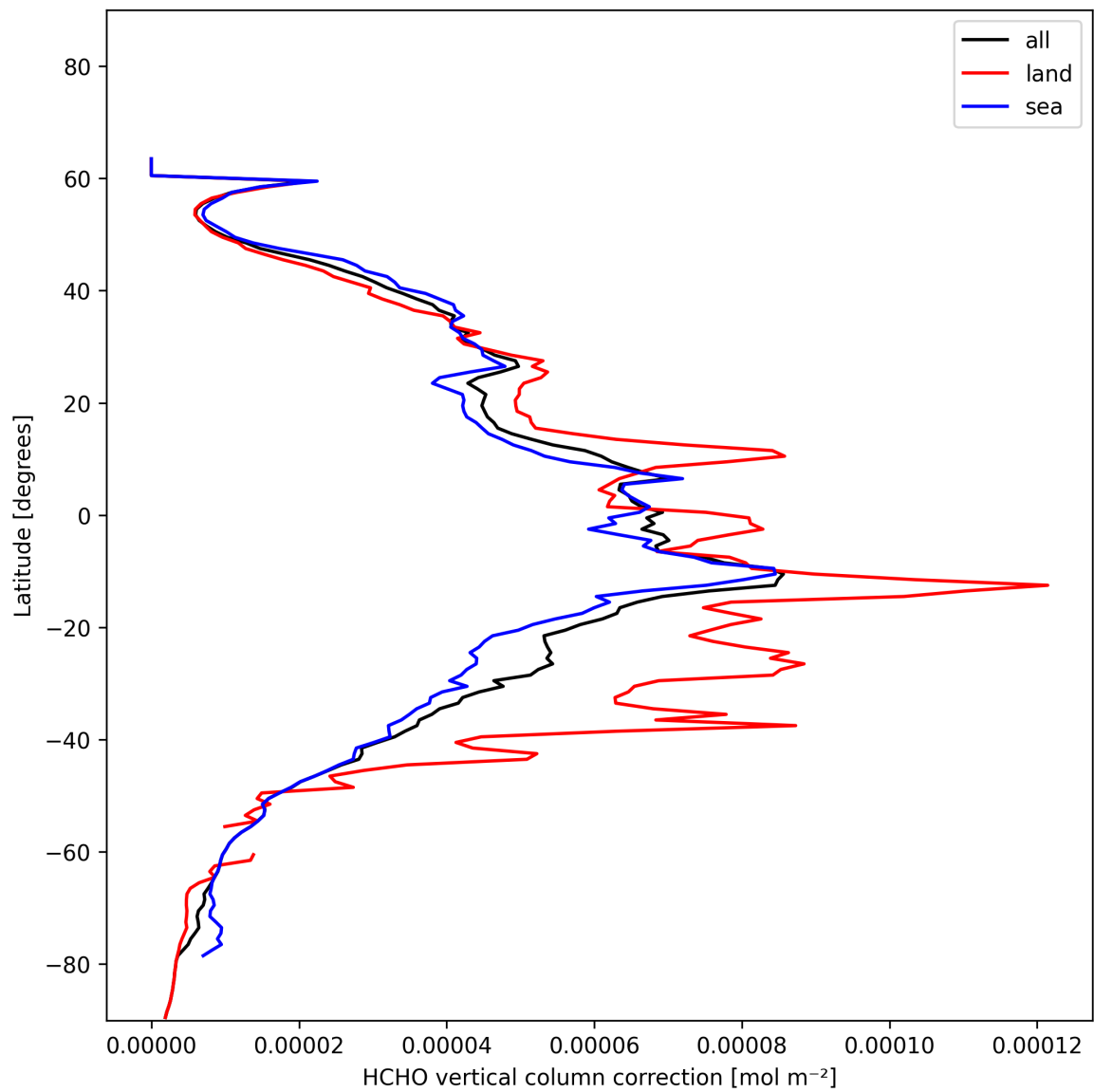
Figure 21: Zonal average of “HCHO vertical column correction” for 2025-01-12 to 2025-01-13.
