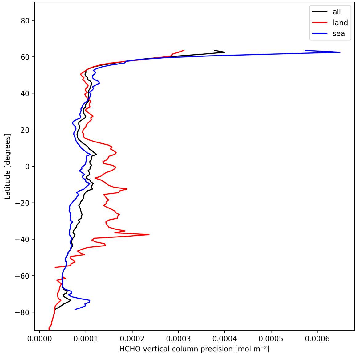
Figure 20: Zonal average of “HCHO vertical column precision” for 2025-01-12 to 2025-01-13.
