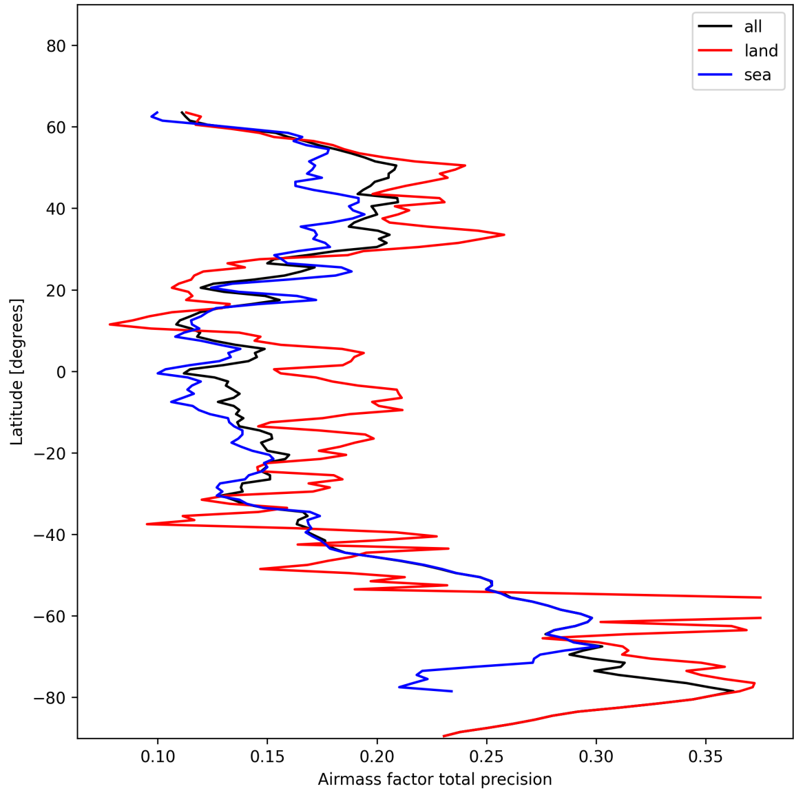
Figure 25: Zonal average of “Airmass factor total precision” for 2025-01-12 to 2025-01-13.
