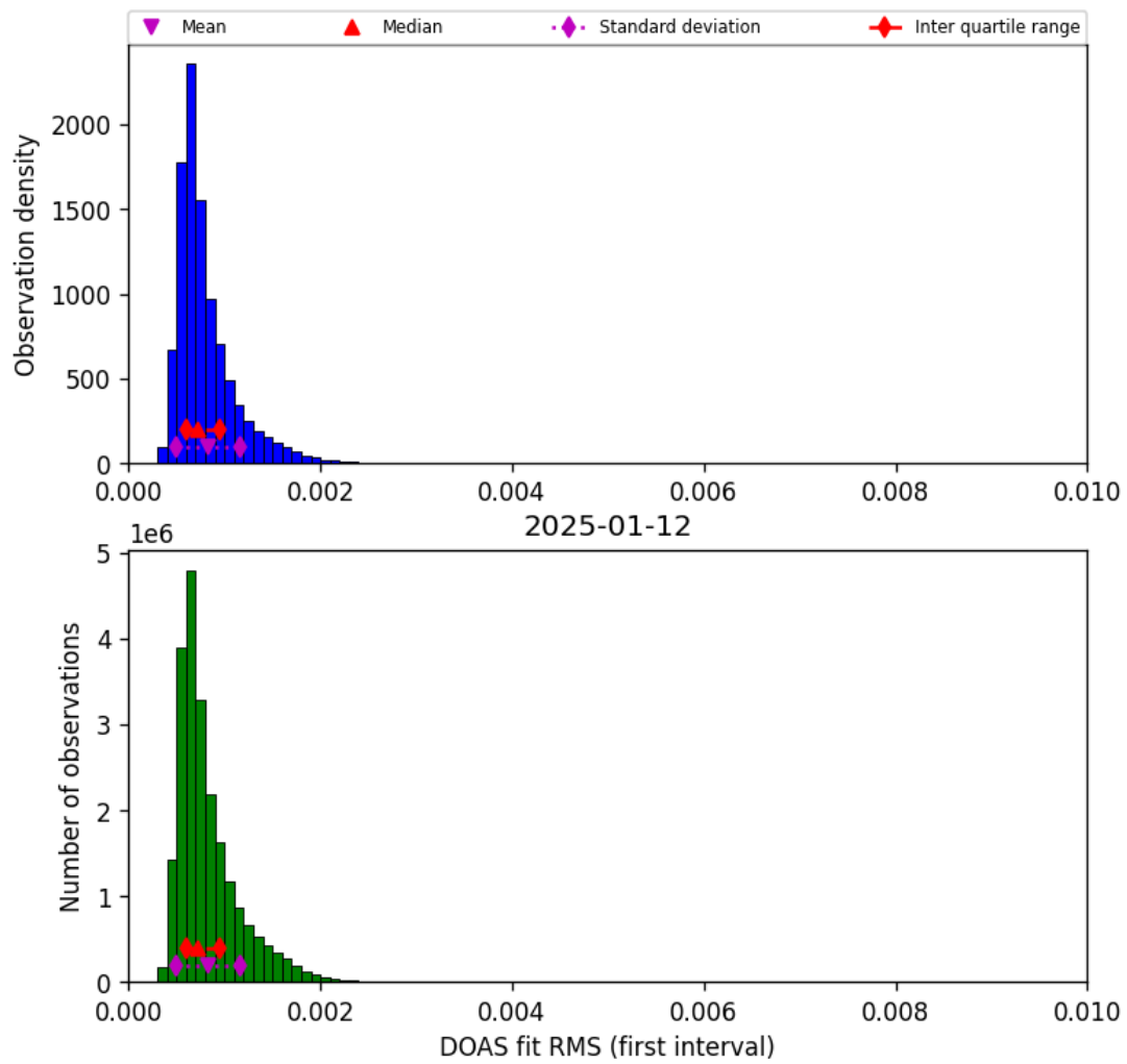
Figure 44: Histogram of “DOAS fit RMS (first interval)” for 2025-01-12 to 2025-01-13
