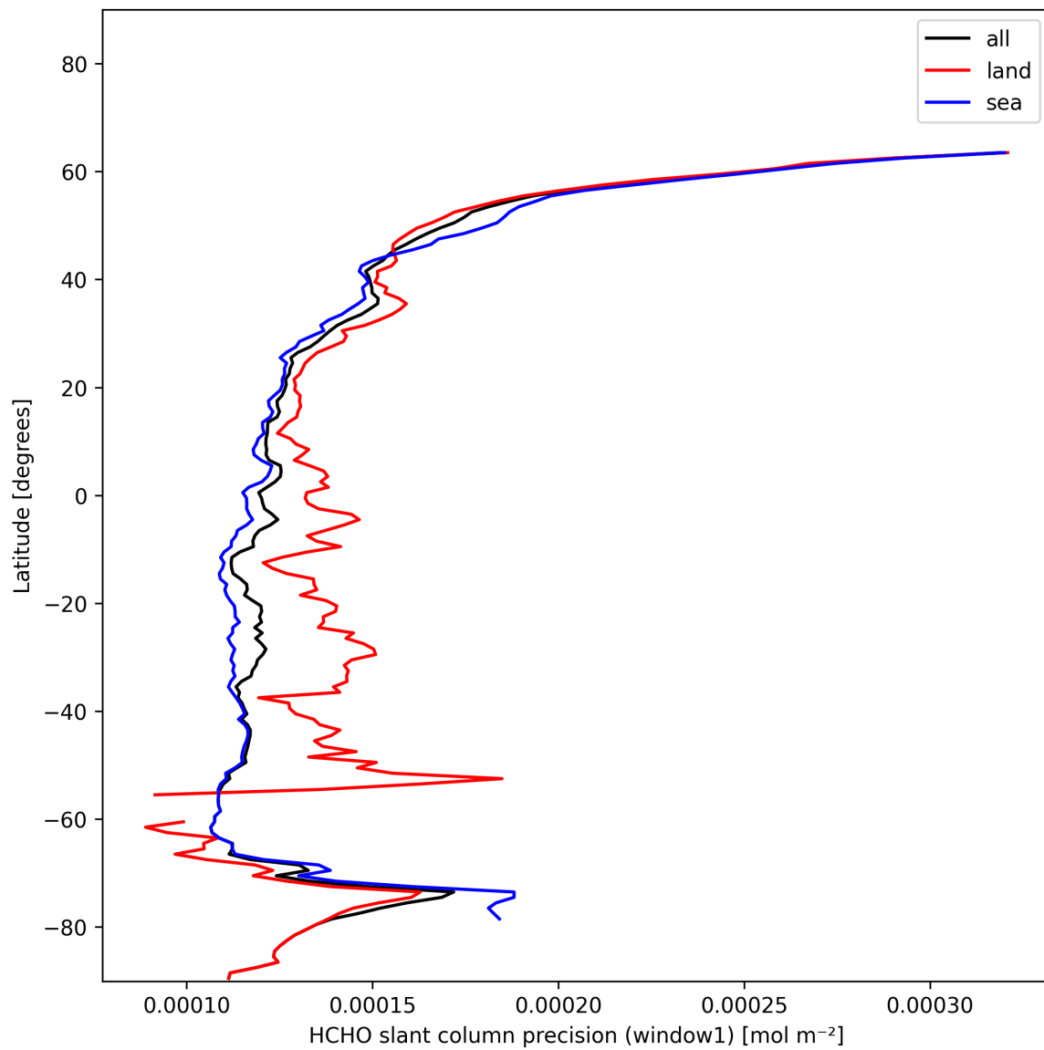
Figure 23: Zonal average of “HCHO slant column precision (window1)” for 2025-01-12 to 2025-01-13.
