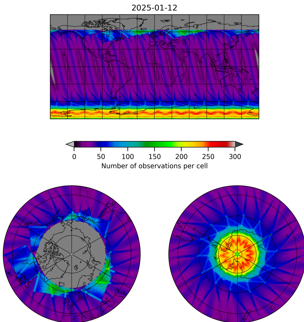
Figure 17: Map of the number of observations for 2025-01-12 to 2025-01-13
