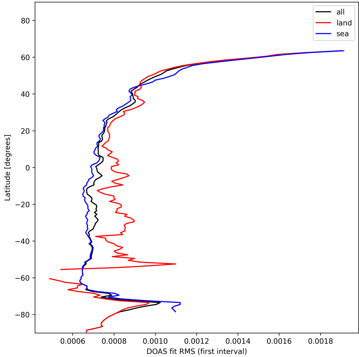
Figure 30: Zonal average of “DOAS fit RMS (first interval)” for 2025-01-12 to 2025-01-13.
