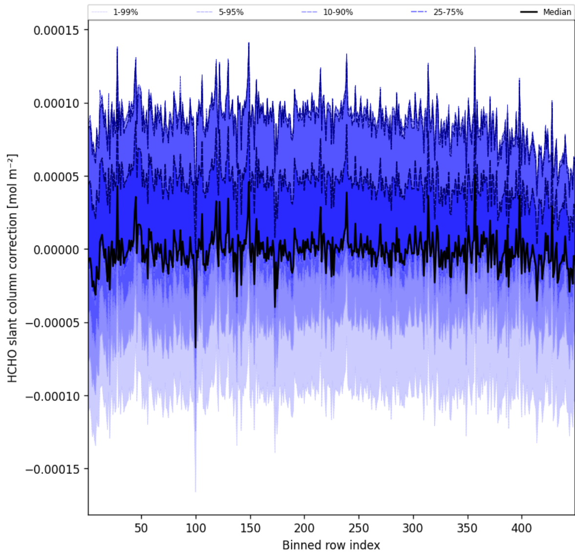
Figure 59: Along track statistics of "HCHO slant column correction" for 2025-01-12 to 2025-01-13
