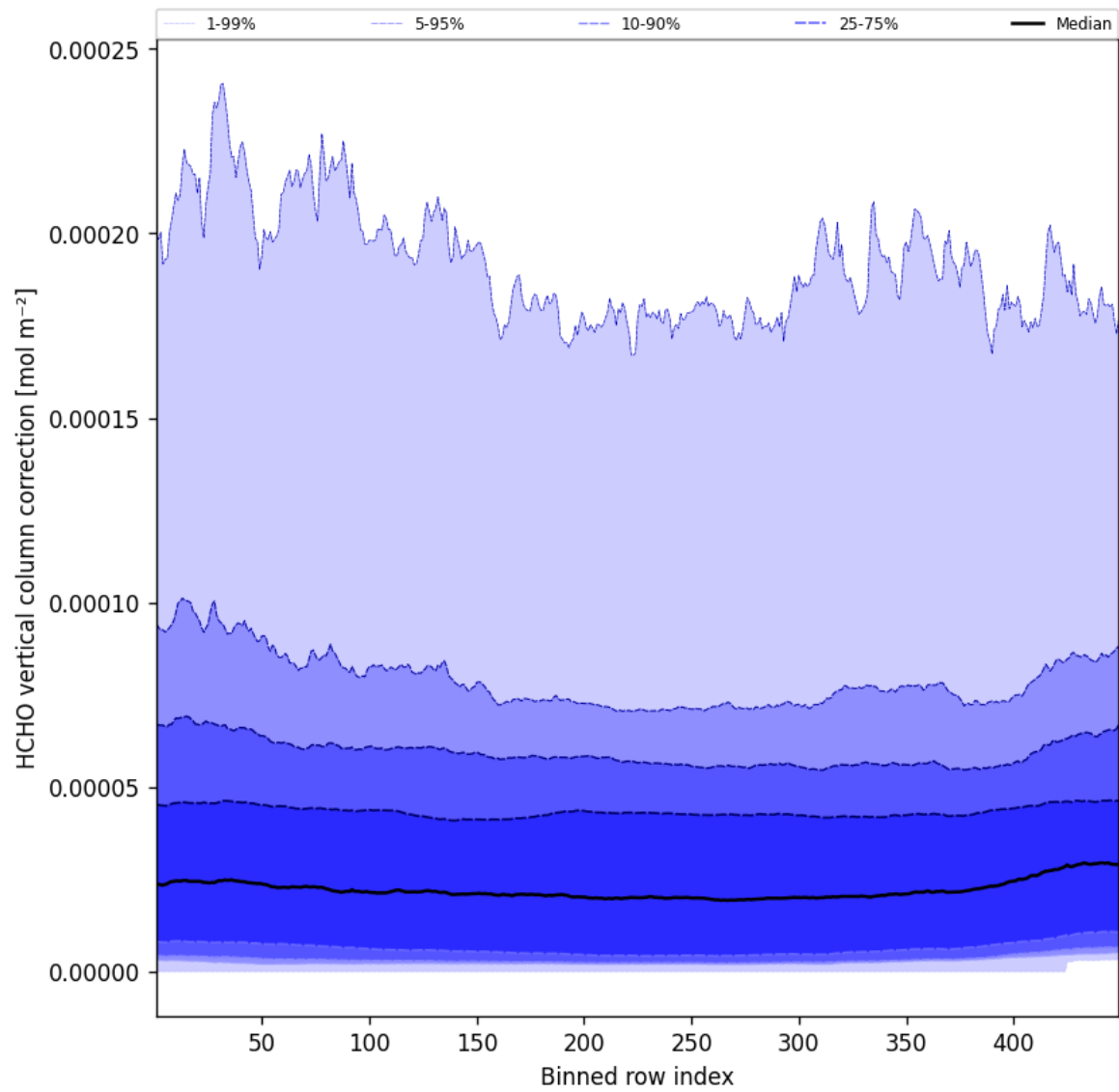
Figure 49: Along track statistics of “HCHO vertical column correction” for 2025-01-12 to 2025-01-13
