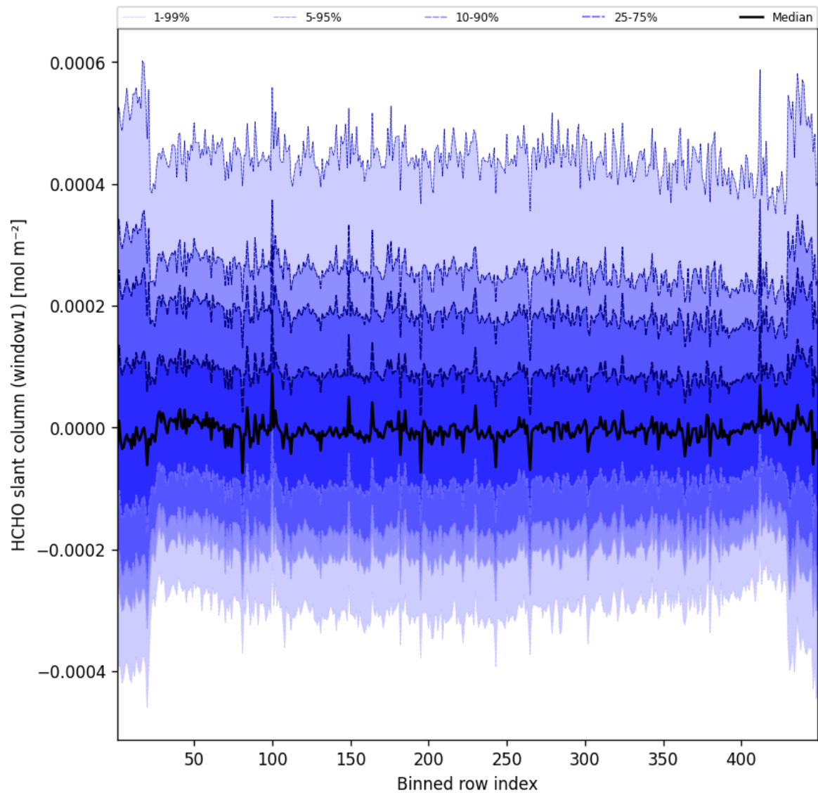
Figure 50: Along track statistics of “HCHO slant column (window1)” for 2025-01-12 to 2025-01-13
