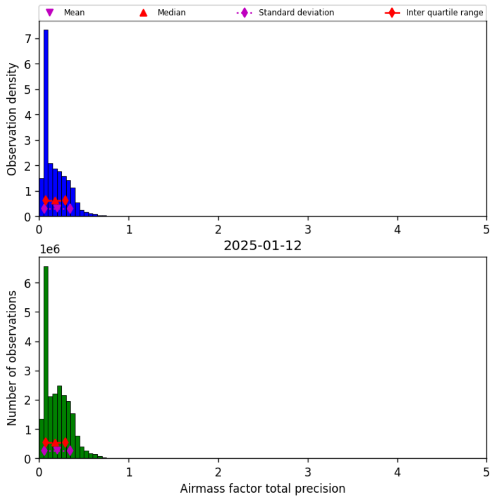
Figure 39: Histogram of “Airmass factor total precision” for 2025-01-12 to 2025-01-13
