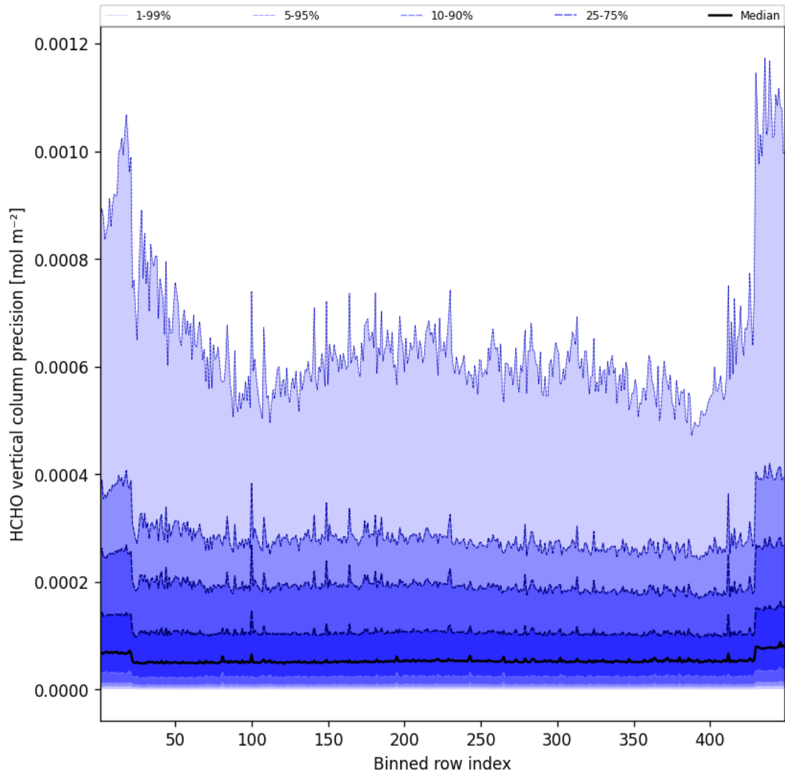
Figure 48: Along track statistics of “HCHO vertical column precision” for 2025-01-12 to 2025-01-13
