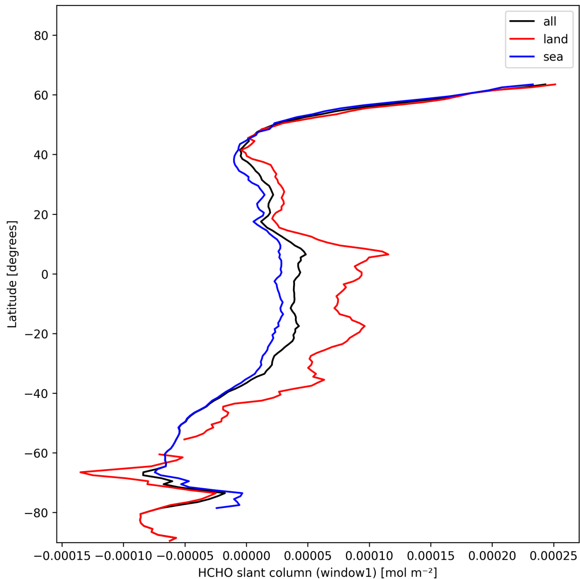
Figure 22: Zonal average of “HCHO slant column (window1)” for 2025-01-12 to 2025-01-13.
