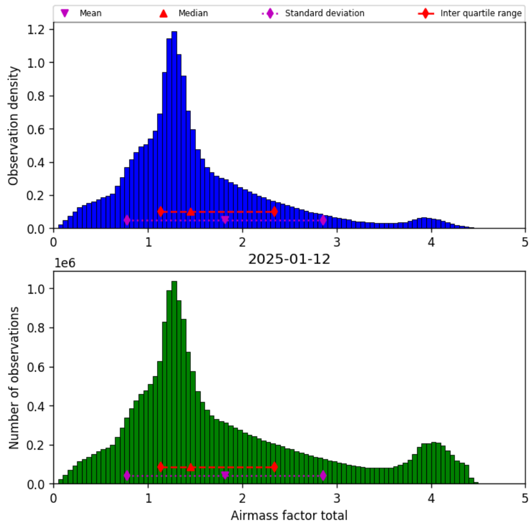
Figure 38: Histogram of “Airmass factor total” for 2025-01-12 to 2025-01-13
