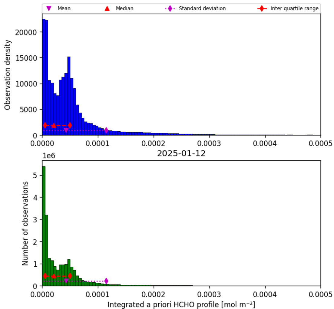
Figure 41: Histogram of “Integrated a priori HCHO profile” for 2025-01-12 to 2025-01-13
