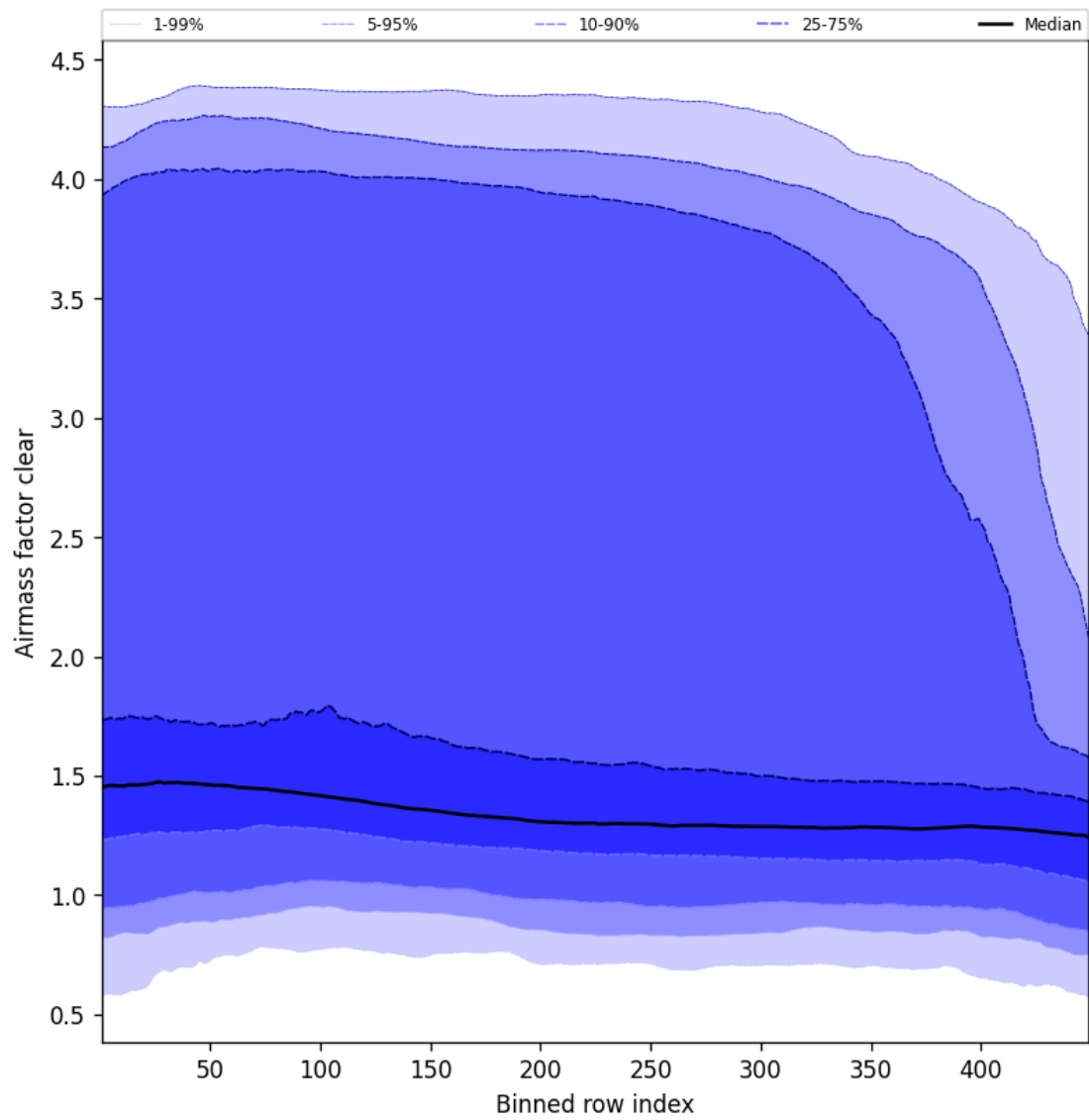
Figure 54: Along track statistics of “Airmass factor clear” for 2025-01-12 to 2025-01-13
