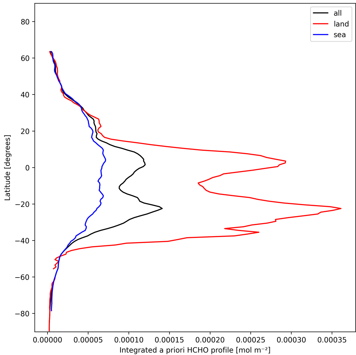
Figure 27: Zonal average of “Integrated a priori HCHO profile” for 2025-01-12 to 2025-01-13.
