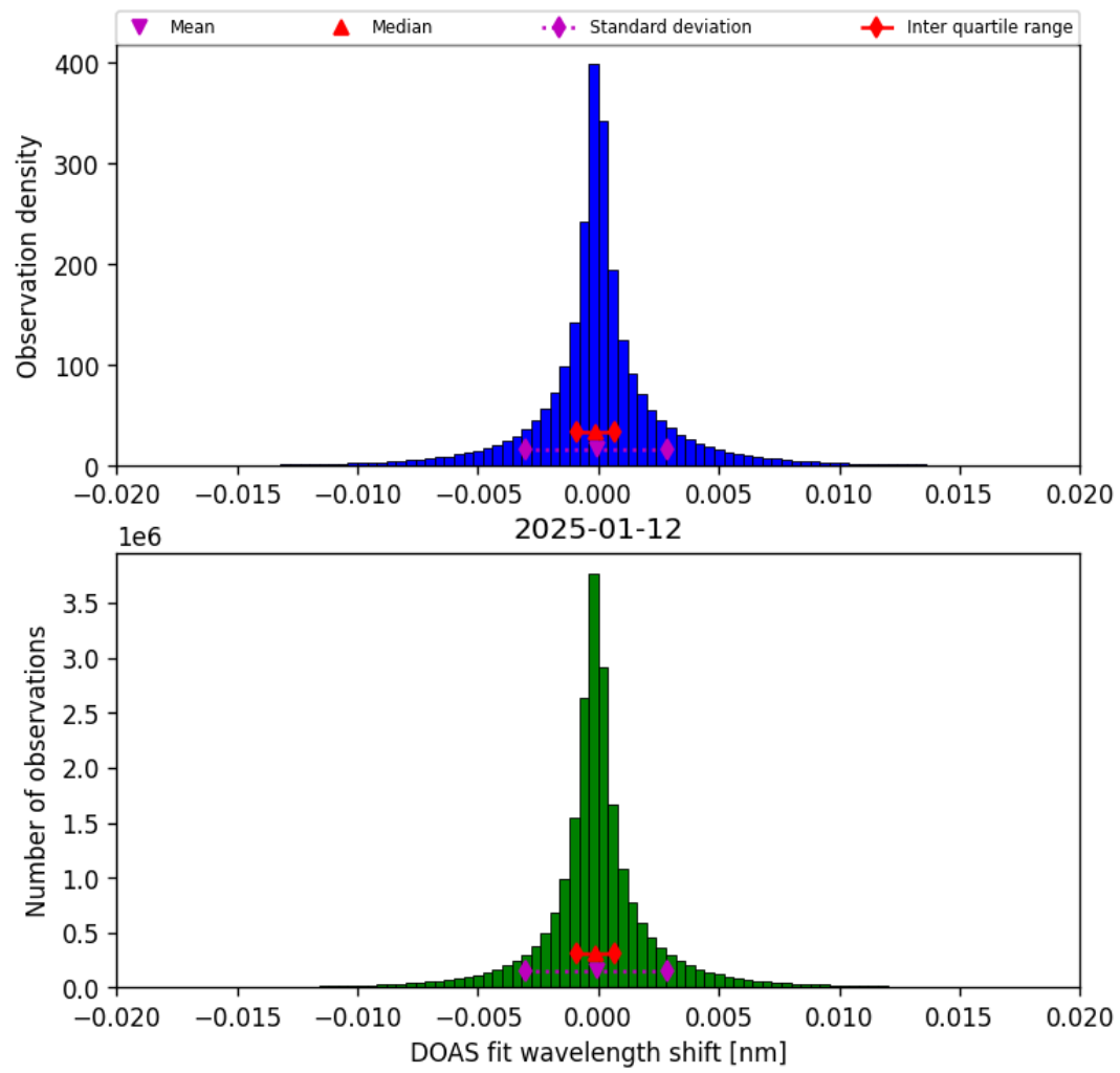
Figure 42: Histogram of “DOAS fit wavelength shift” for 2025-01-12 to 2025-01-13
