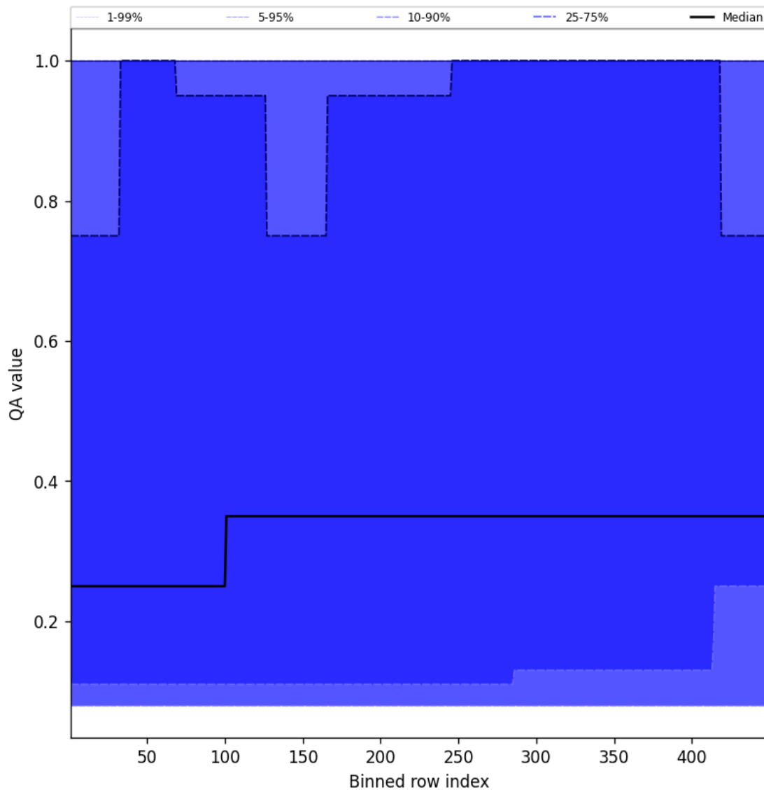
Figure 46: Along track statistics of “QA value” for 2025-01-12 to 2025-01-13
