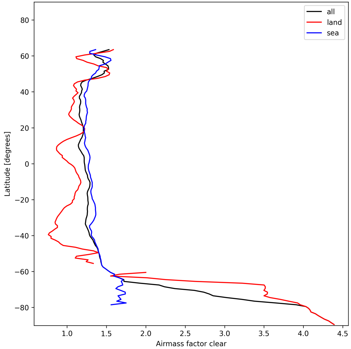
Figure 26: Zonal average of “Airmass factor clear” for 2025-01-12 to 2025-01-13.
