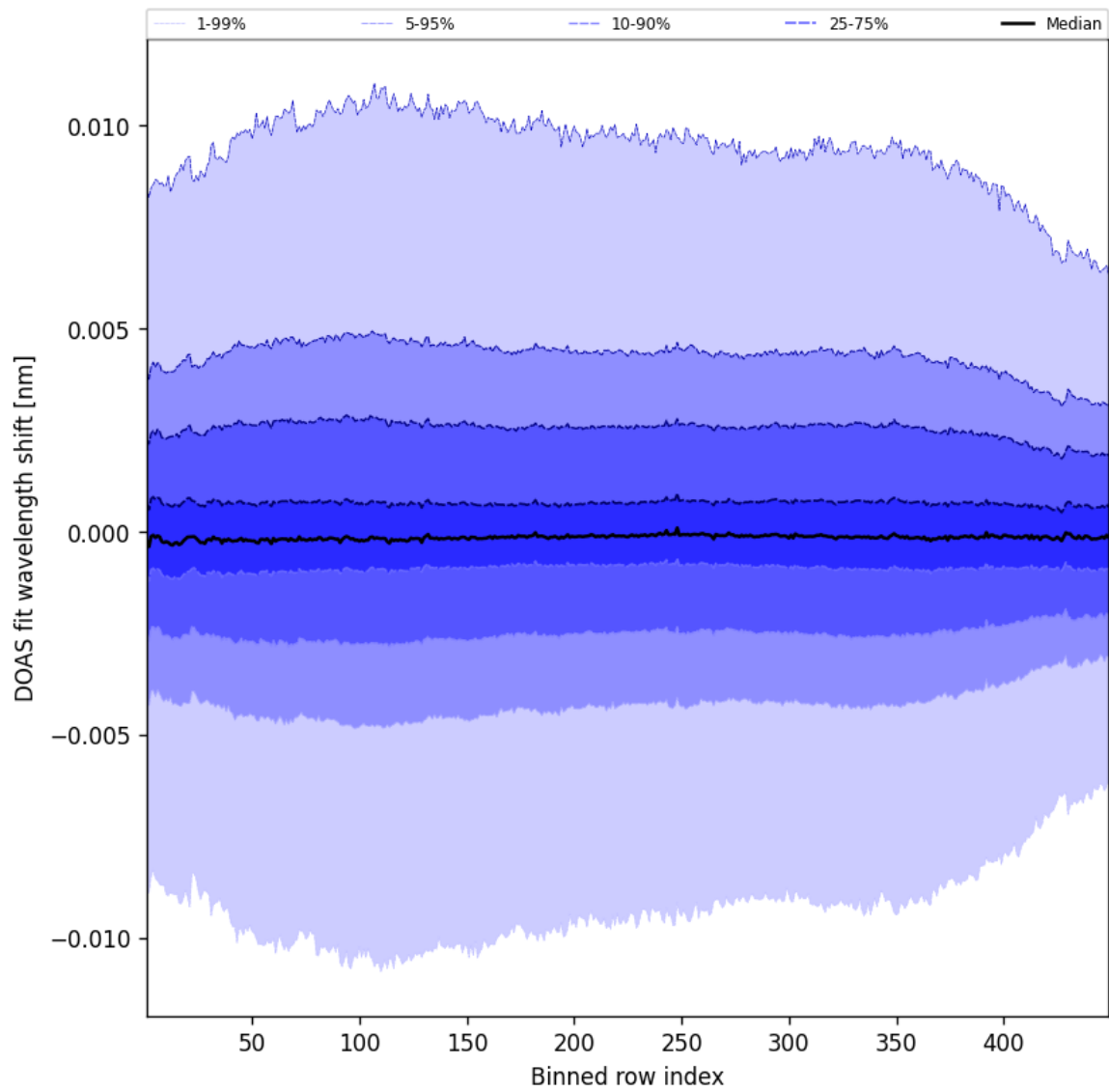
Figure 56: Along track statistics of “DOAS fit wavelength shift” for 2025-01-12 to 2025-01-13
