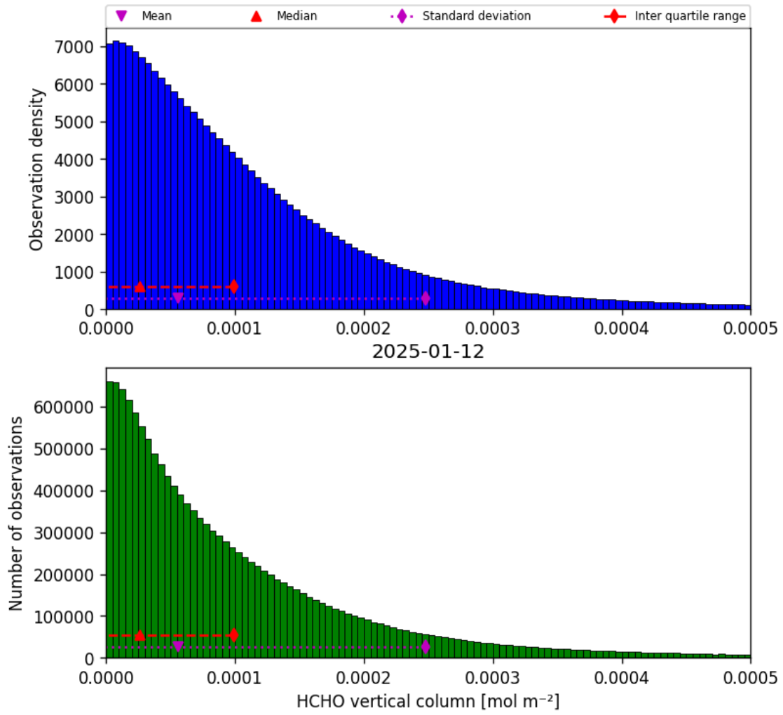
Figure 33: Histogram of “HCHO vertical column” for 2025-01-12 to 2025-01-13
