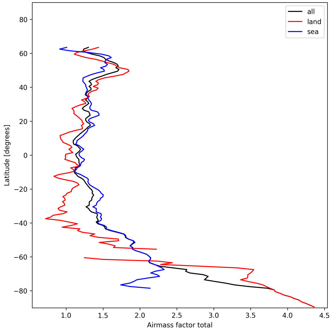
Figure 24: Zonal average of “Airmass factor total” for 2025-01-12 to 2025-01-13.
