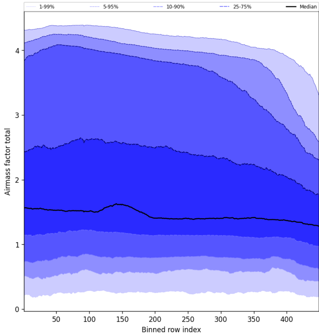
Figure 52: Along track statistics of “Airmass factor total” for 2025-01-12 to 2025-01-13
