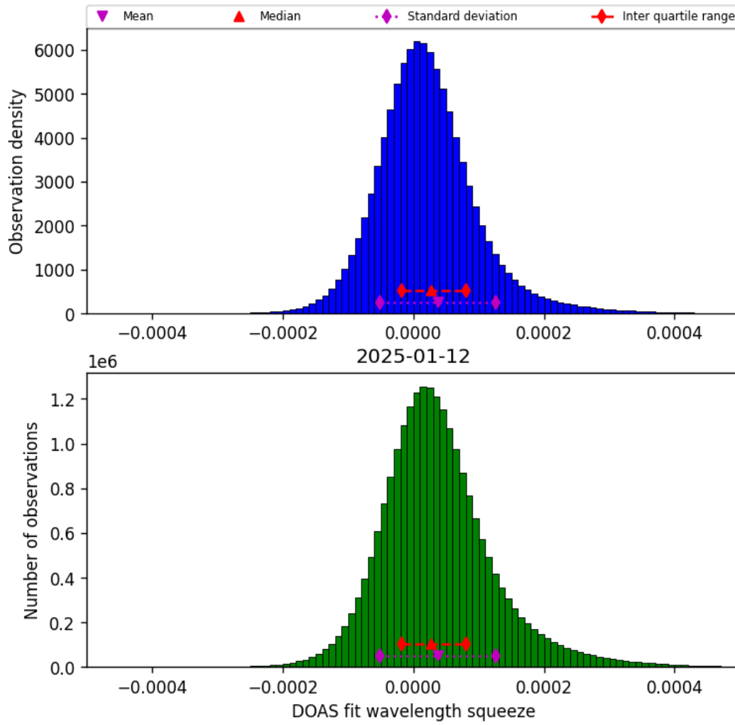
Figure 43: Histogram of “DOAS fit wavelength squeeze” for 2025-01-12 to 2025-01-13
