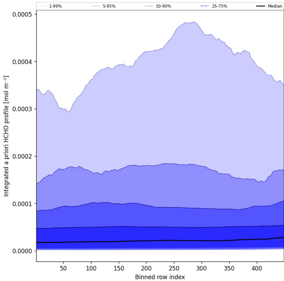
Figure 55: Along track statistics of “Integrated a priori HCHO profile” for 2025-01-12 to 2025-01-13
