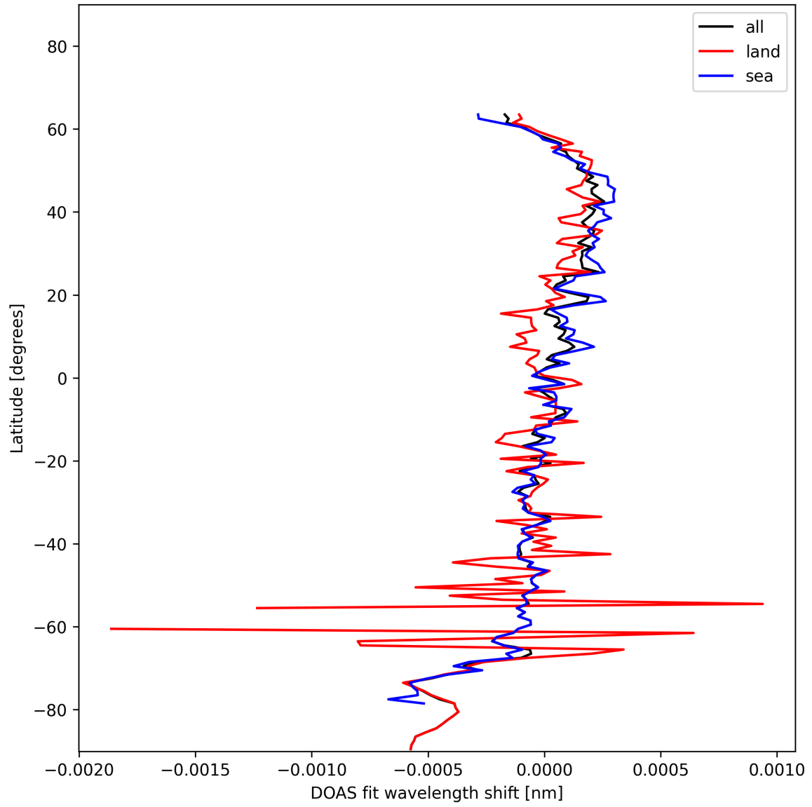
Figure 28: Zonal average of “DOAS fit wavelength shift” for 2025-01-12 to 2025-01-13.
