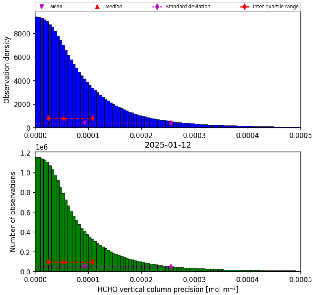
Figure 34: Histogram of “HCHO vertical column precision” for 2025-01-12 to 2025-01-13
