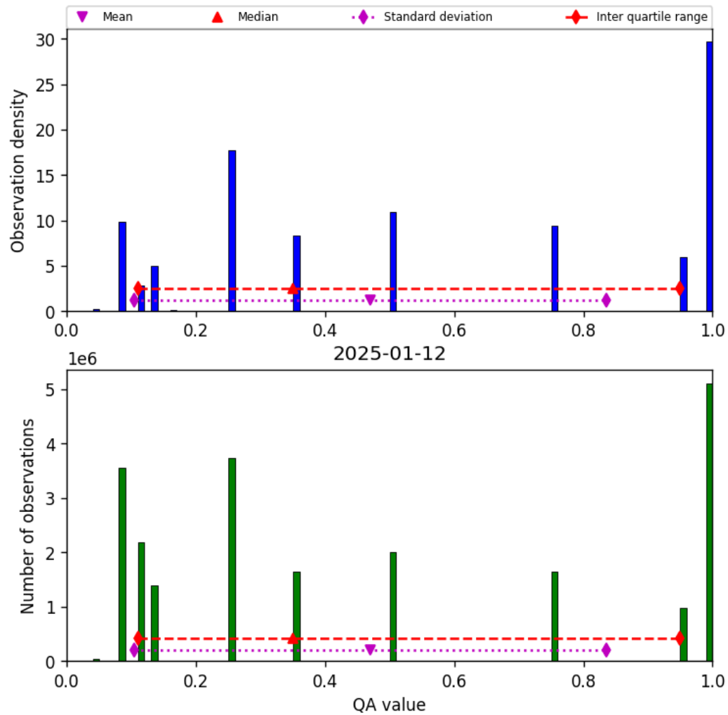
Figure 32: Histogram of “QA value” for 2025-01-12 to 2025-01-13
