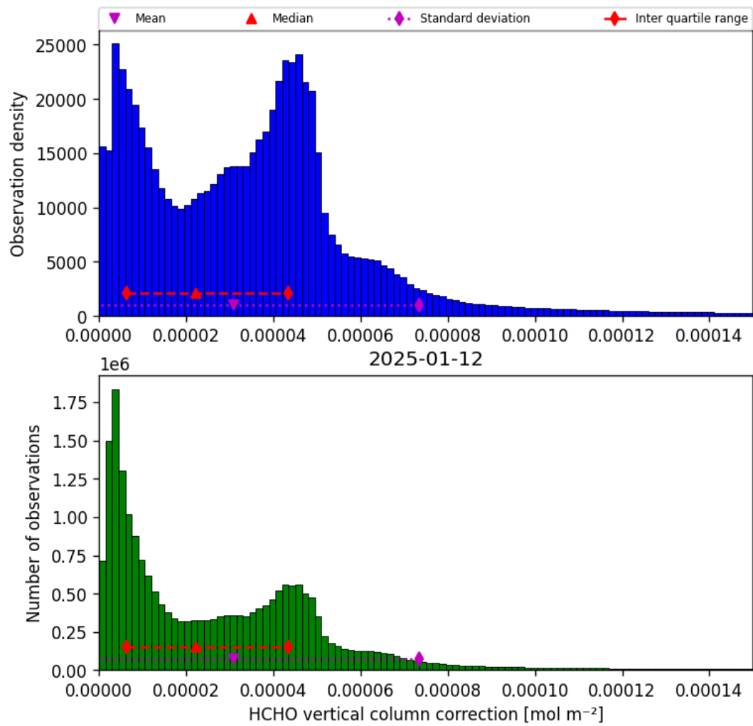
Figure 35: Histogram of “HCHO vertical column correction” for 2025-01-12 to 2025-01-13
