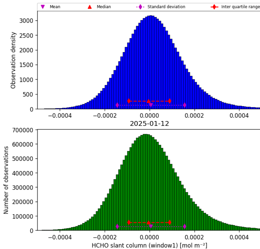
Figure 36: Histogram of “HCHO slant column (window1)” for 2025-01-12 to 2025-01-13
