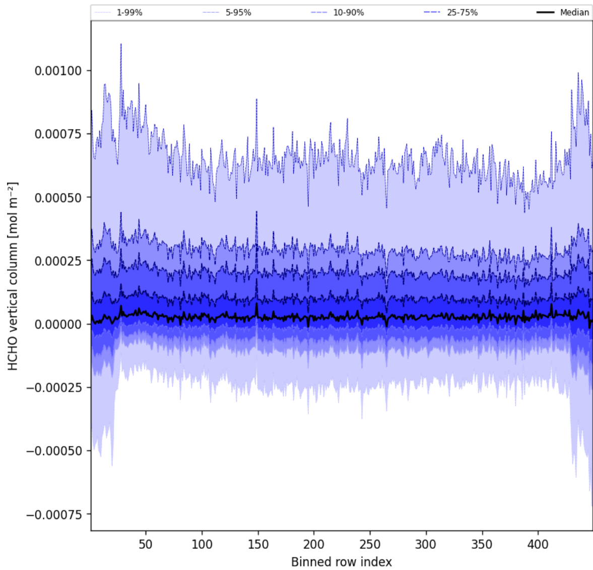
Figure 47: Along track statistics of “HCHO vertical column” for 2025-01-12 to 2025-01-13
