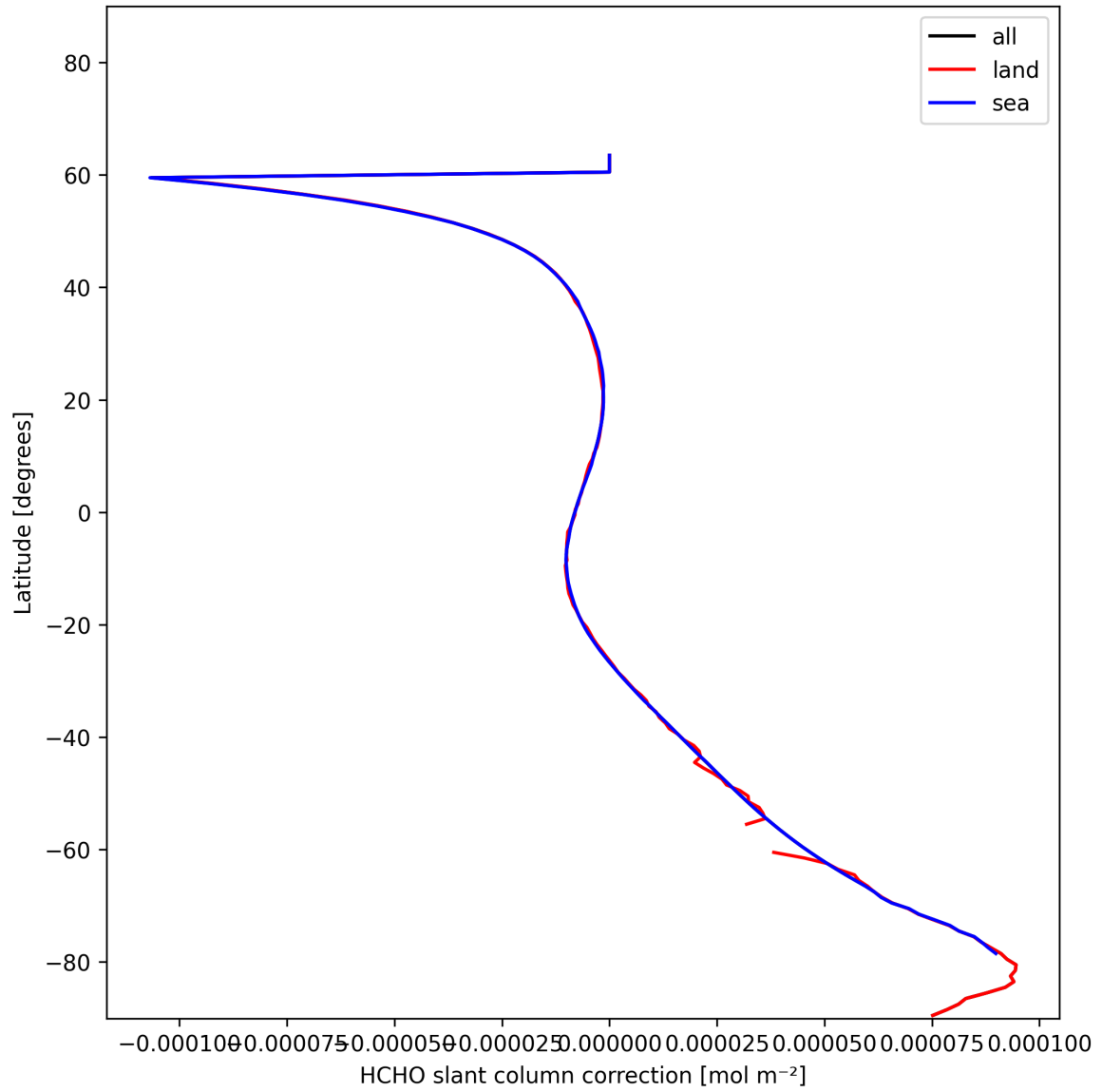
Figure 31: Zonal average of “HCHO slant column correction” for 2025-01-12 to 2025-01-13.
