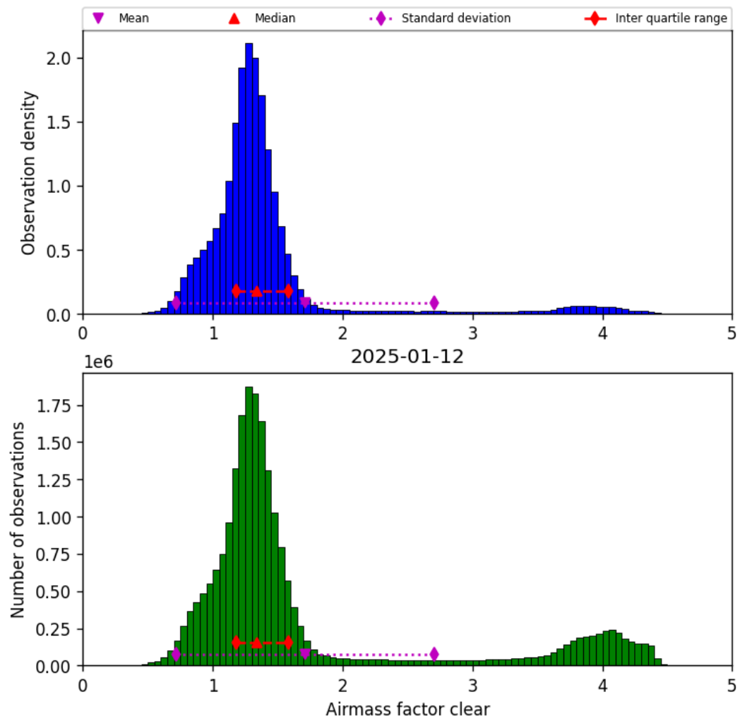
Figure 40: Histogram of “Airmass factor clear” for 2025-01-12 to 2025-01-13
