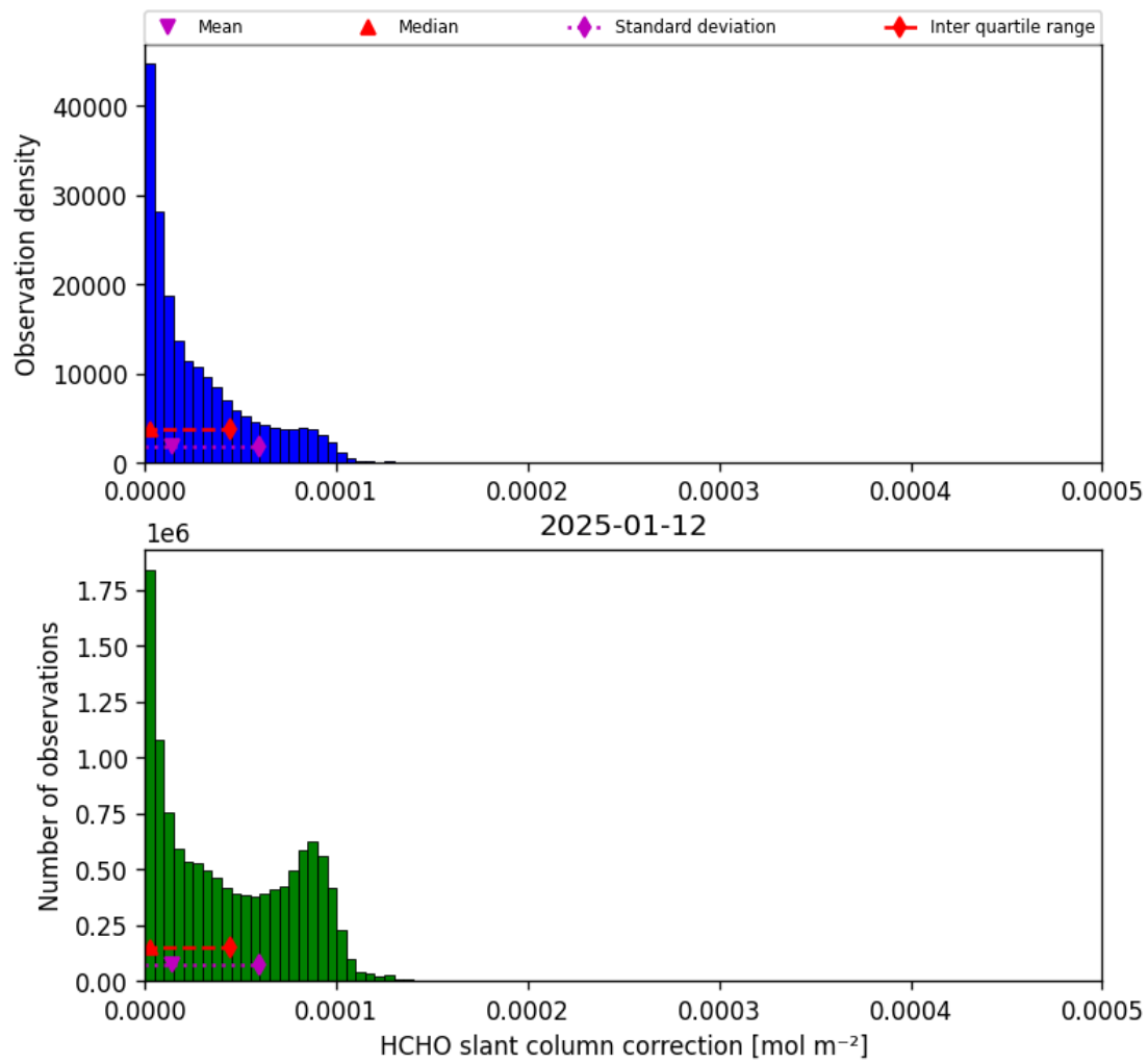
Figure 45: Histogram of “HCHO slant column correction” for 2025-01-12 to 2025-01-13
