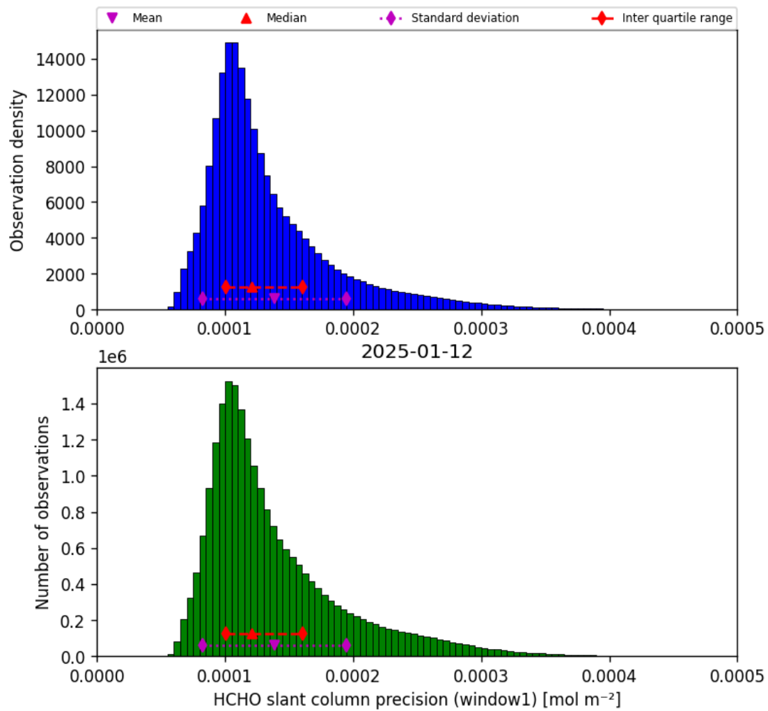
Figure 37: Histogram of “HCHO slant column precision (window1)” for 2025-01-12 to 2025-01-13
