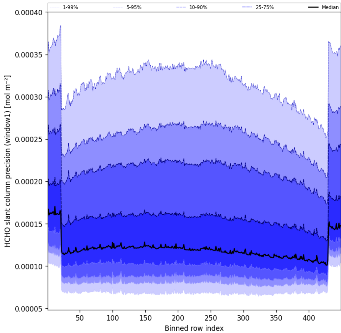
Figure 51: Along track statistics of “HCHO slant column precision (window1)” for 2025-01-12 to 2025-01-13
