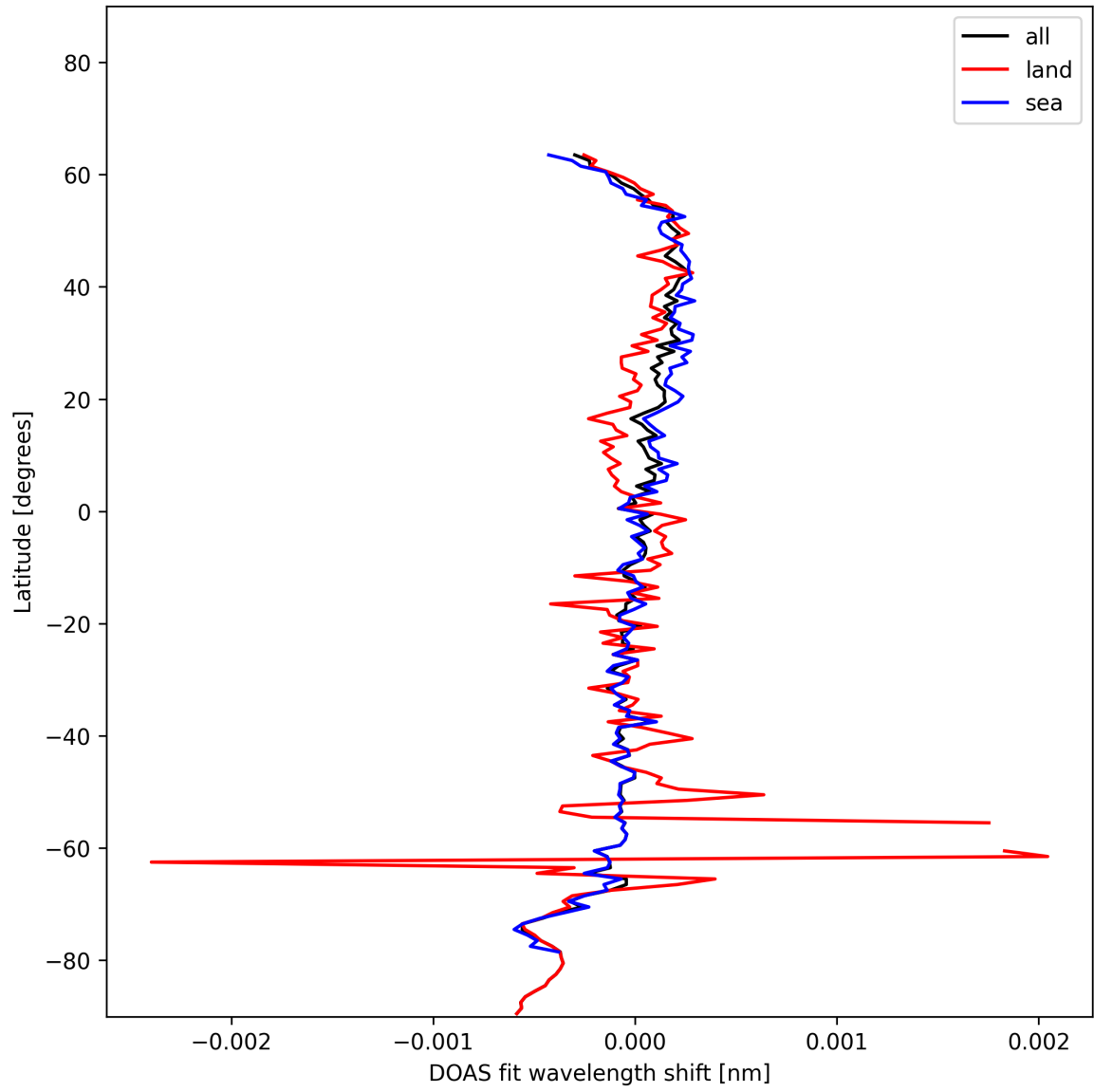
Figure 28: Zonal average of “DOAS fit wavelength shift” for 2025-01-13 to 2025-01-14.
