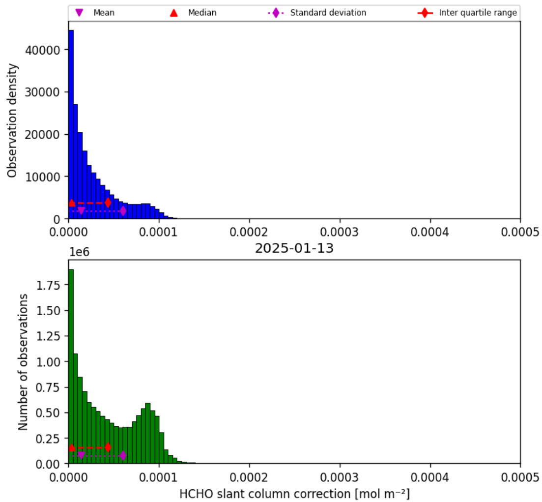
Figure 45: Histogram of “HCHO slant column correction” for 2025-01-13 to 2025-01-14
