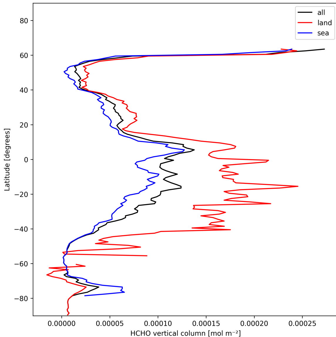
Figure 19: Zonal average of “HCHO vertical column” for 2025-01-13 to 2025-01-14.
