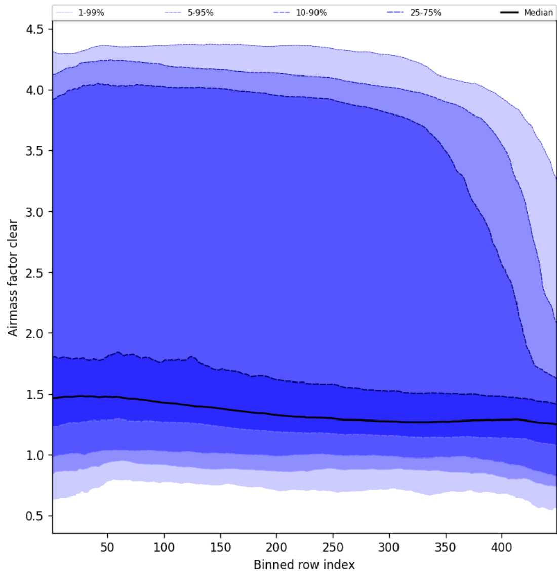
Figure 54: Along track statistics of “Airmass factor clear” for 2025-01-13 to 2025-01-14
