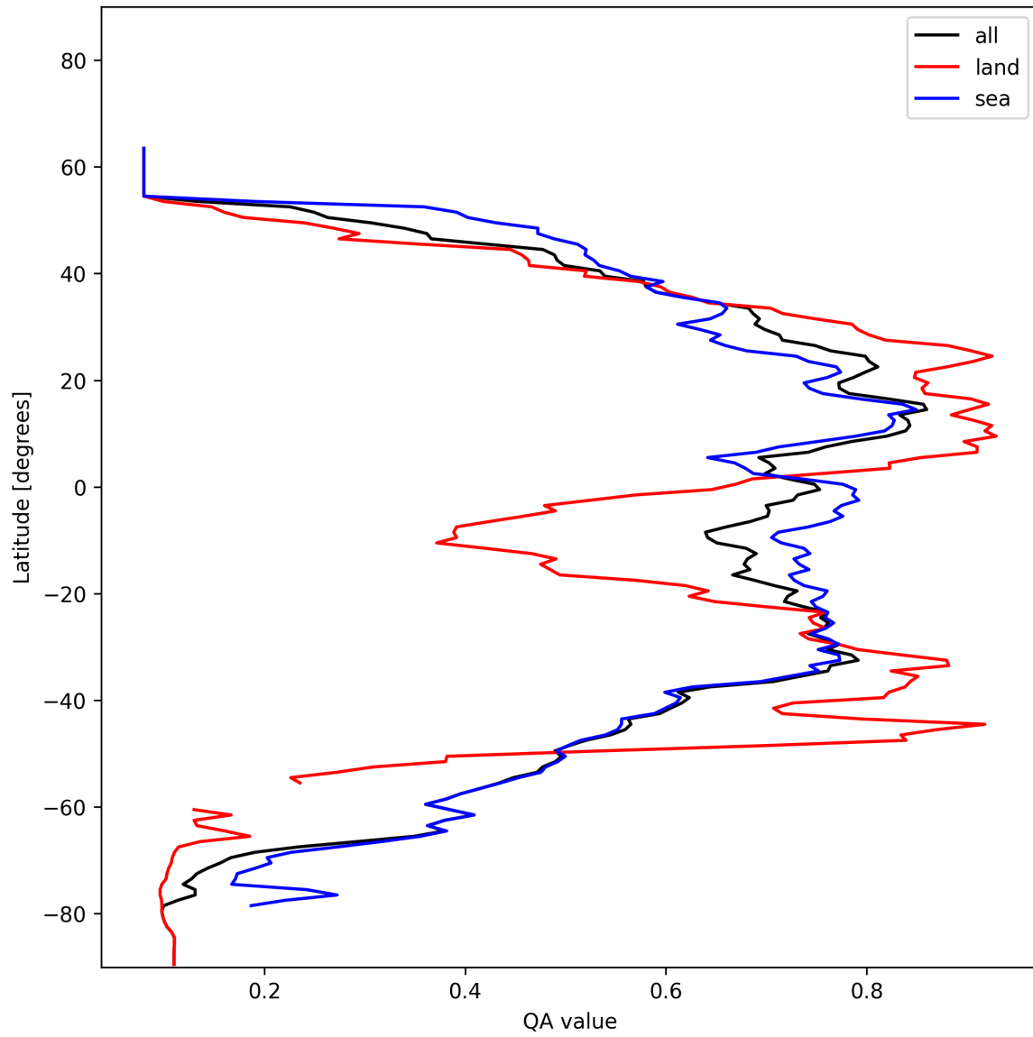
Figure 18: Zonal average of “QA value” for 2025-01-13 to 2025-01-14.
