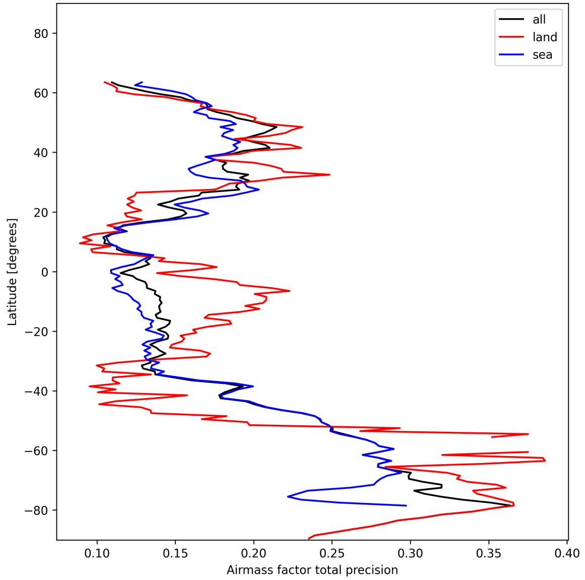
Figure 25: Zonal average of “Airmass factor total precision” for 2025-01-13 to 2025-01-14.
