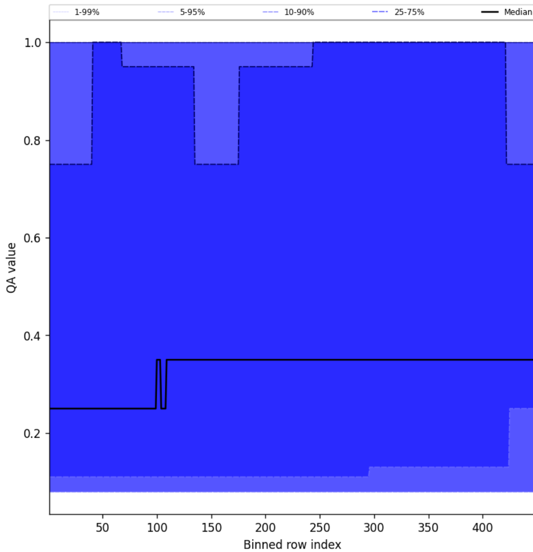
Figure 46: Along track statistics of “QA value” for 2025-01-13 to 2025-01-14
