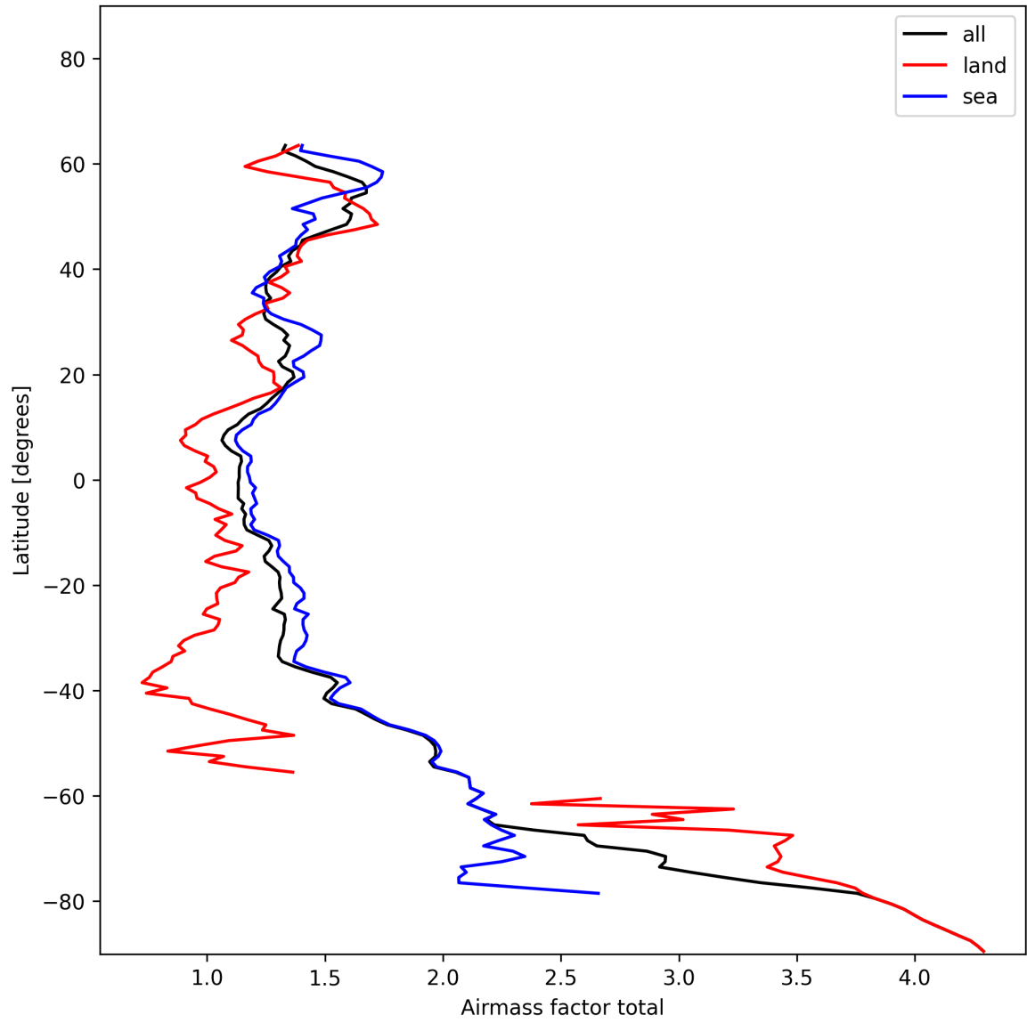
Figure 24: Zonal average of “Airmass factor total” for 2025-01-13 to 2025-01-14.
