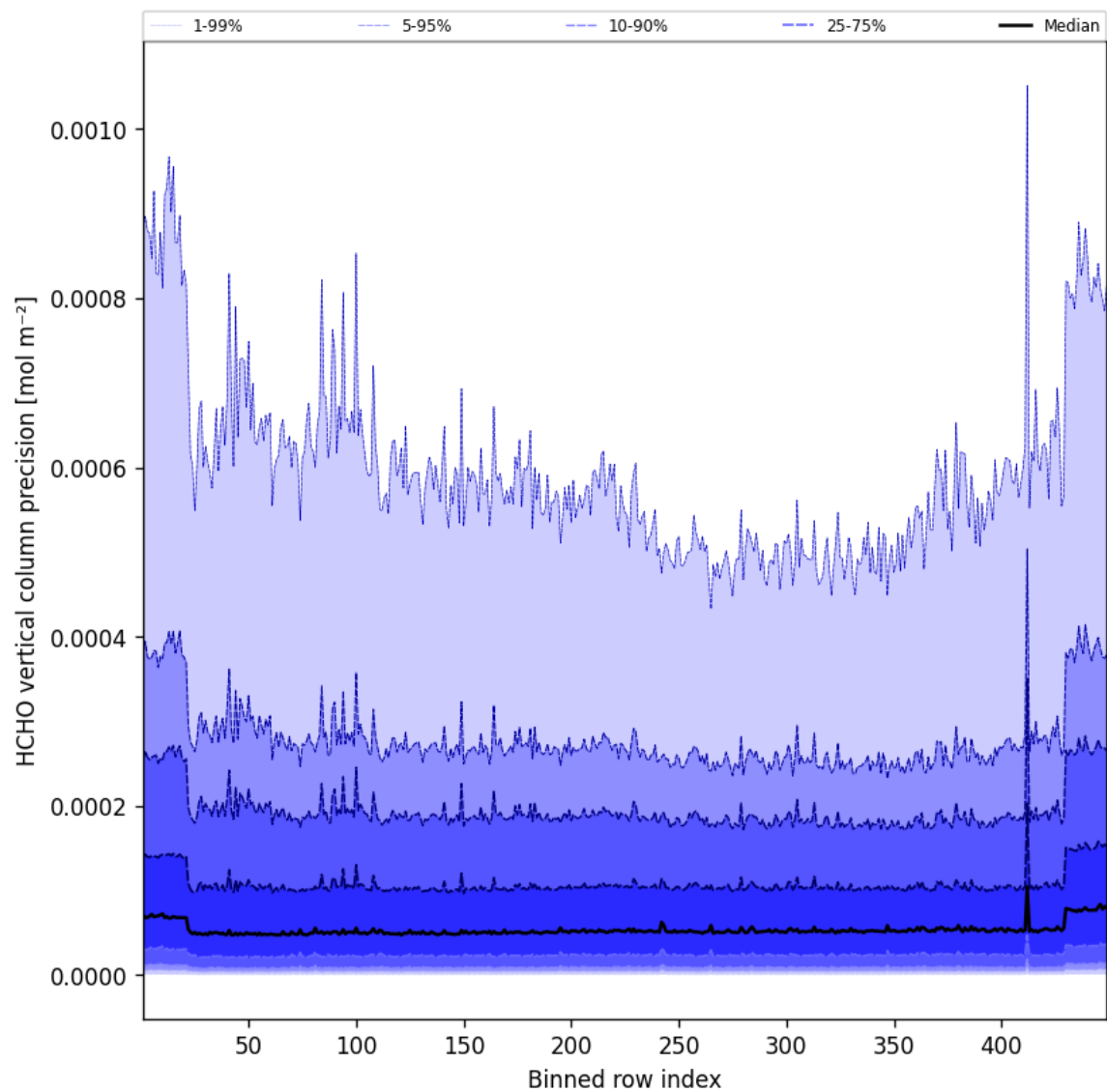
Figure 48: Along track statistics of “HCHO vertical column precision” for 2025-01-13 to 2025-01-14
