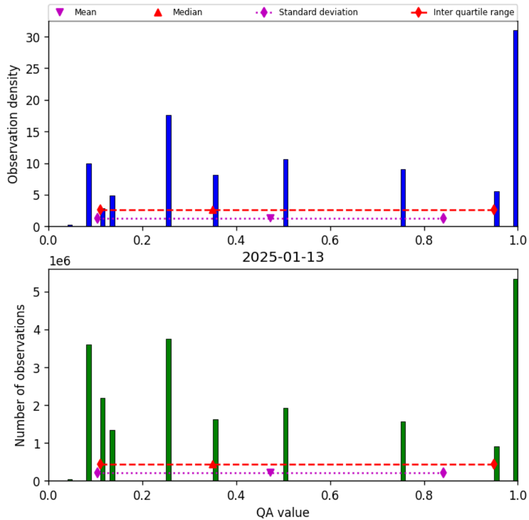
Figure 32: Histogram of “QA value” for 2025-01-13 to 2025-01-14
