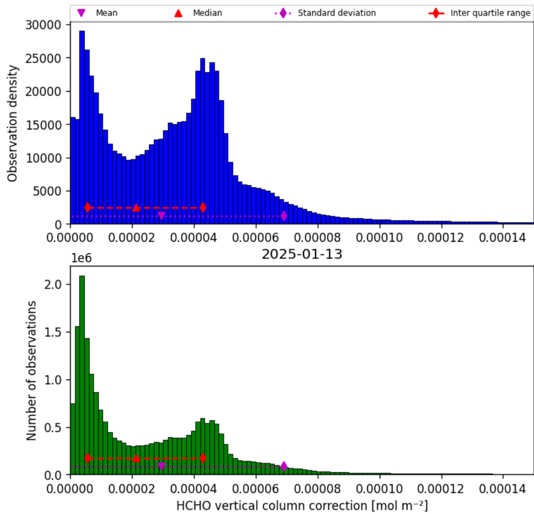
Figure 35: Histogram of “HCHO vertical column correction” for 2025-01-13 to 2025-01-14
