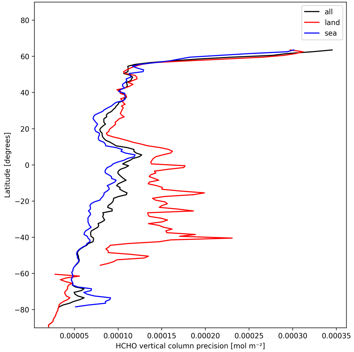
Figure 20: Zonal average of “HCHO vertical column precision” for 2025-01-13 to 2025-01-14.
