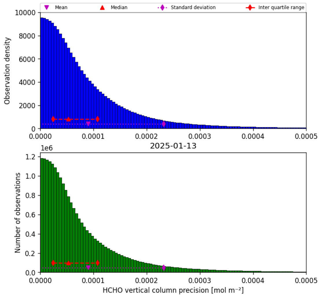
Figure 34: Histogram of “HCHO vertical column precision” for 2025-01-13 to 2025-01-14
