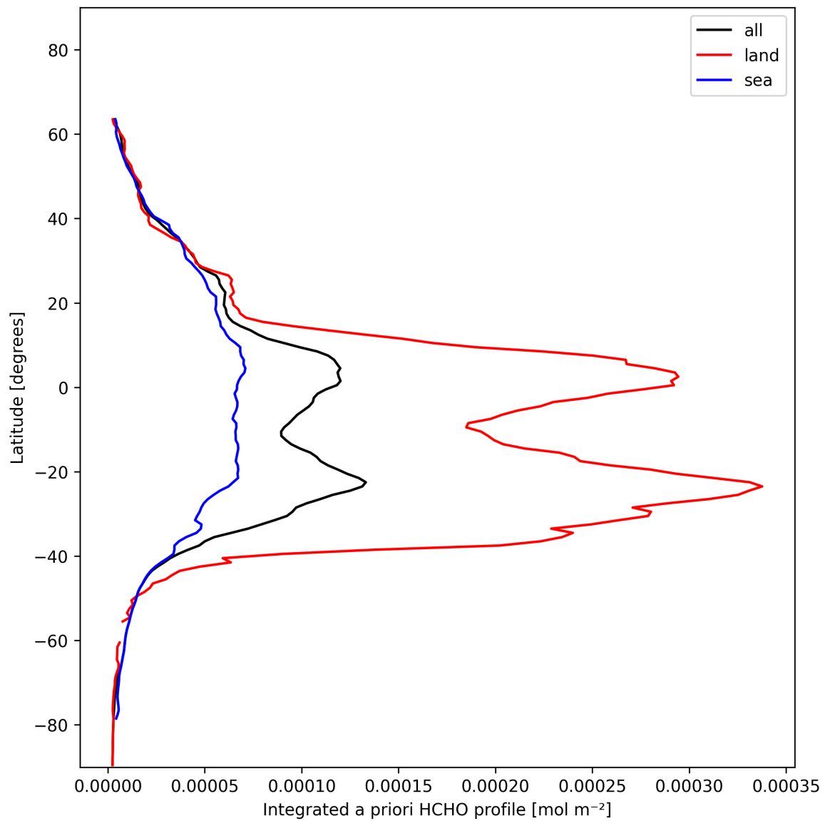
Figure 27: Zonal average of “Integrated a priori HCHO profile” for 2025-01-13 to 2025-01-14.
