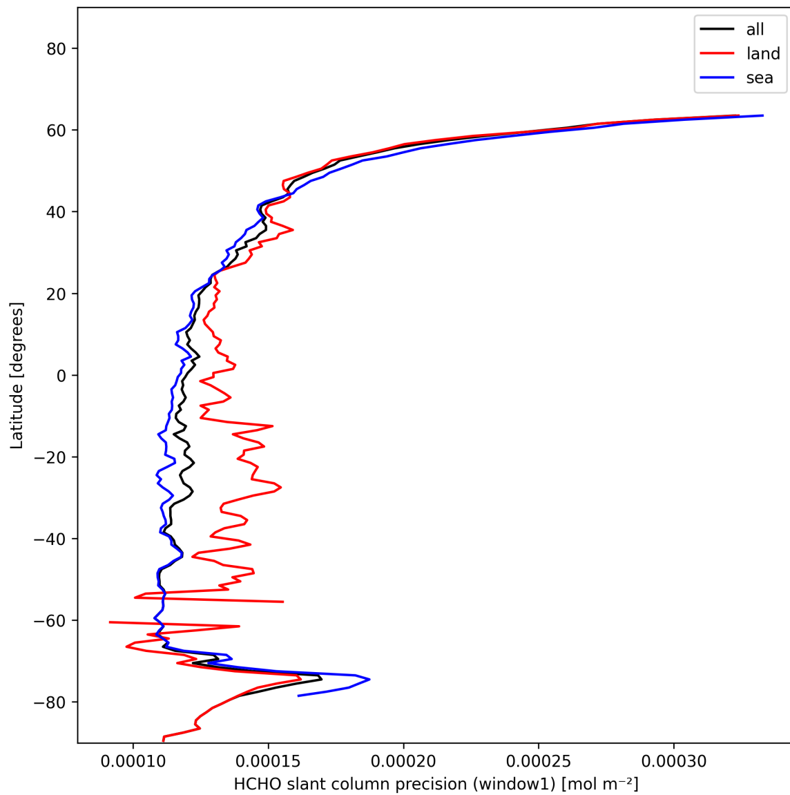
Figure 23: Zonal average of “HCHO slant column precision (window1)” for 2025-01-13 to 2025-01-14.
