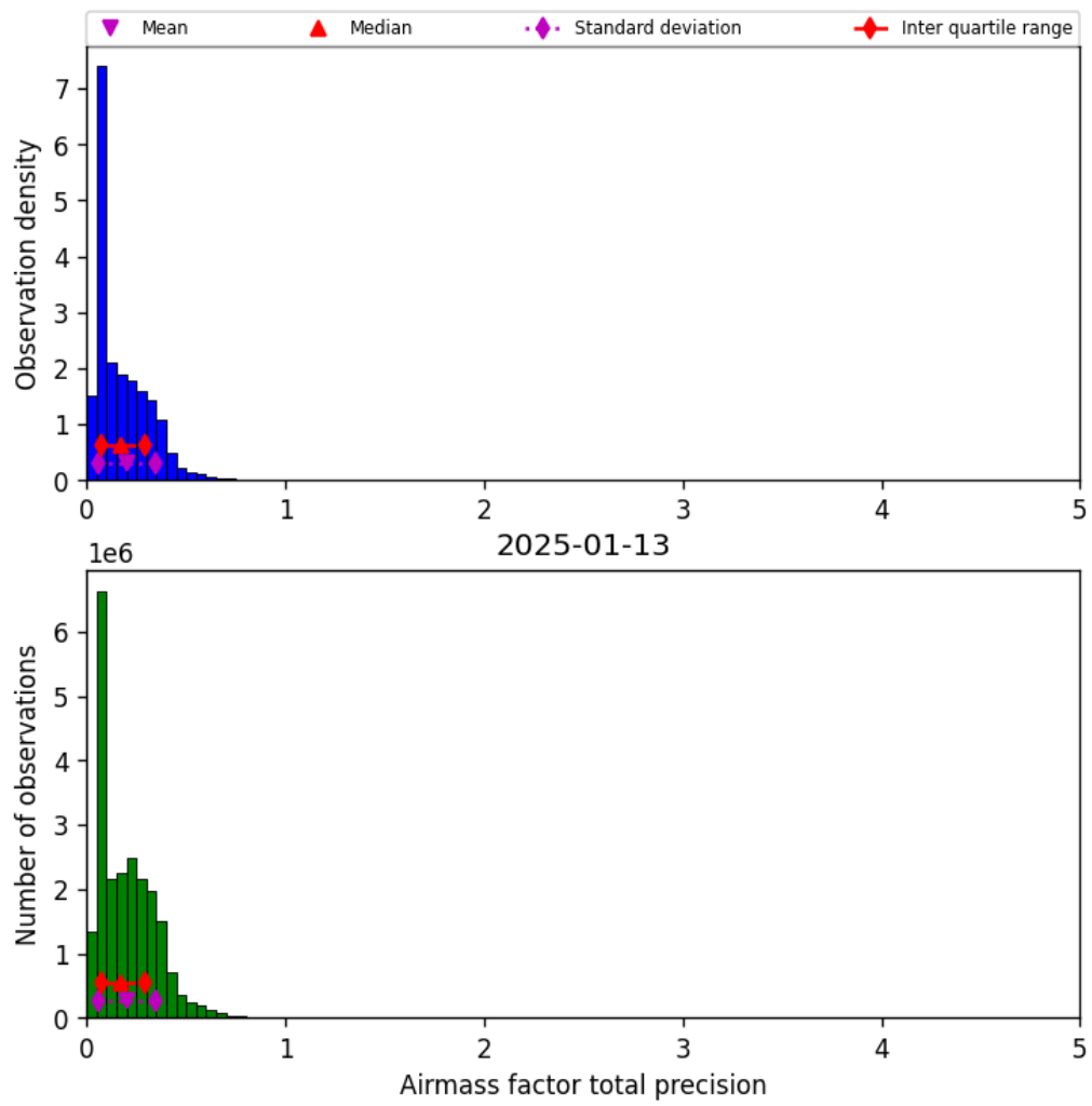
Figure 39: Histogram of “Airmass factor total precision” for 2025-01-13 to 2025-01-14
