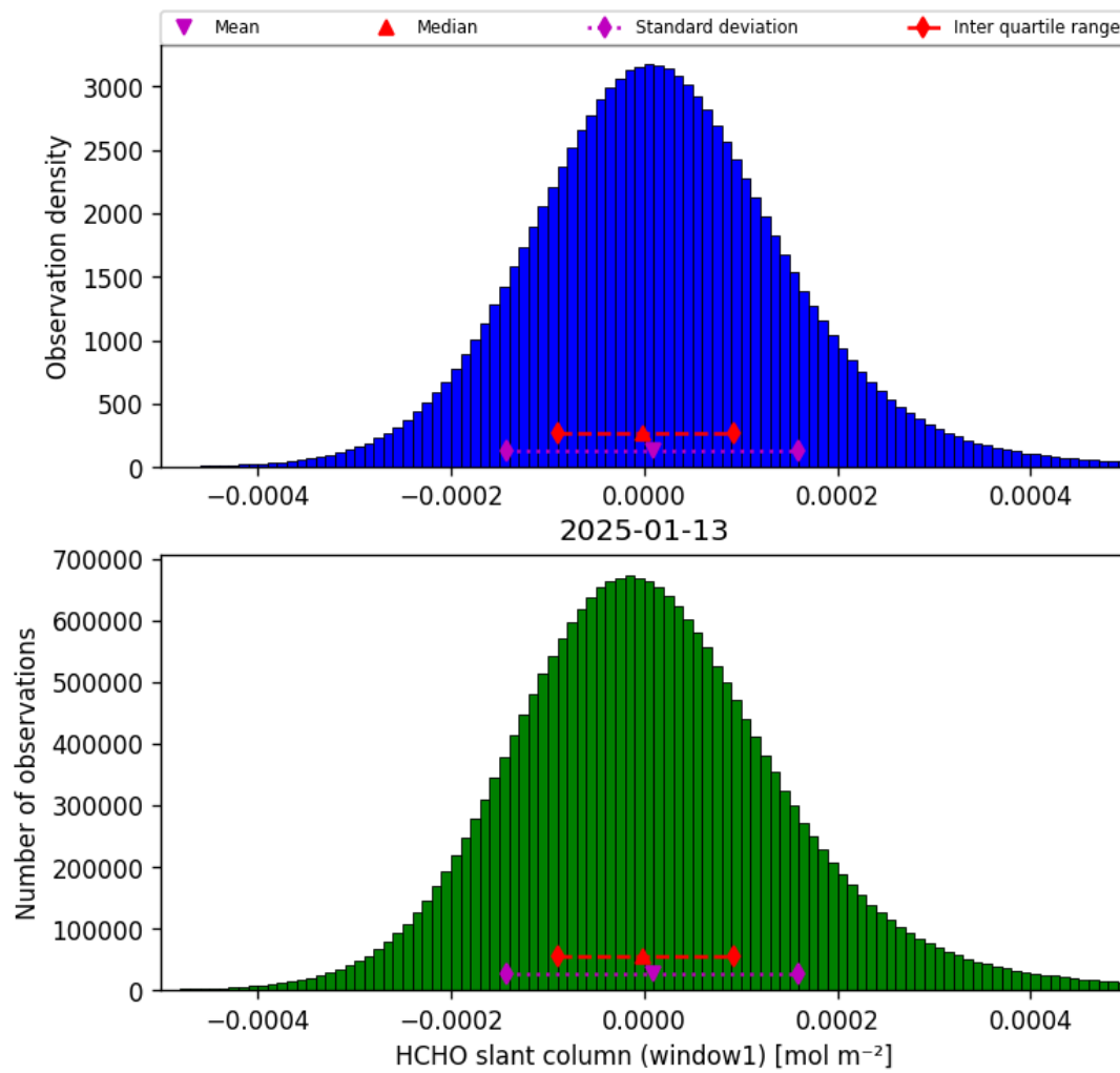
Figure 36: Histogram of “HCHO slant column (window1)” for 2025-01-13 to 2025-01-14
