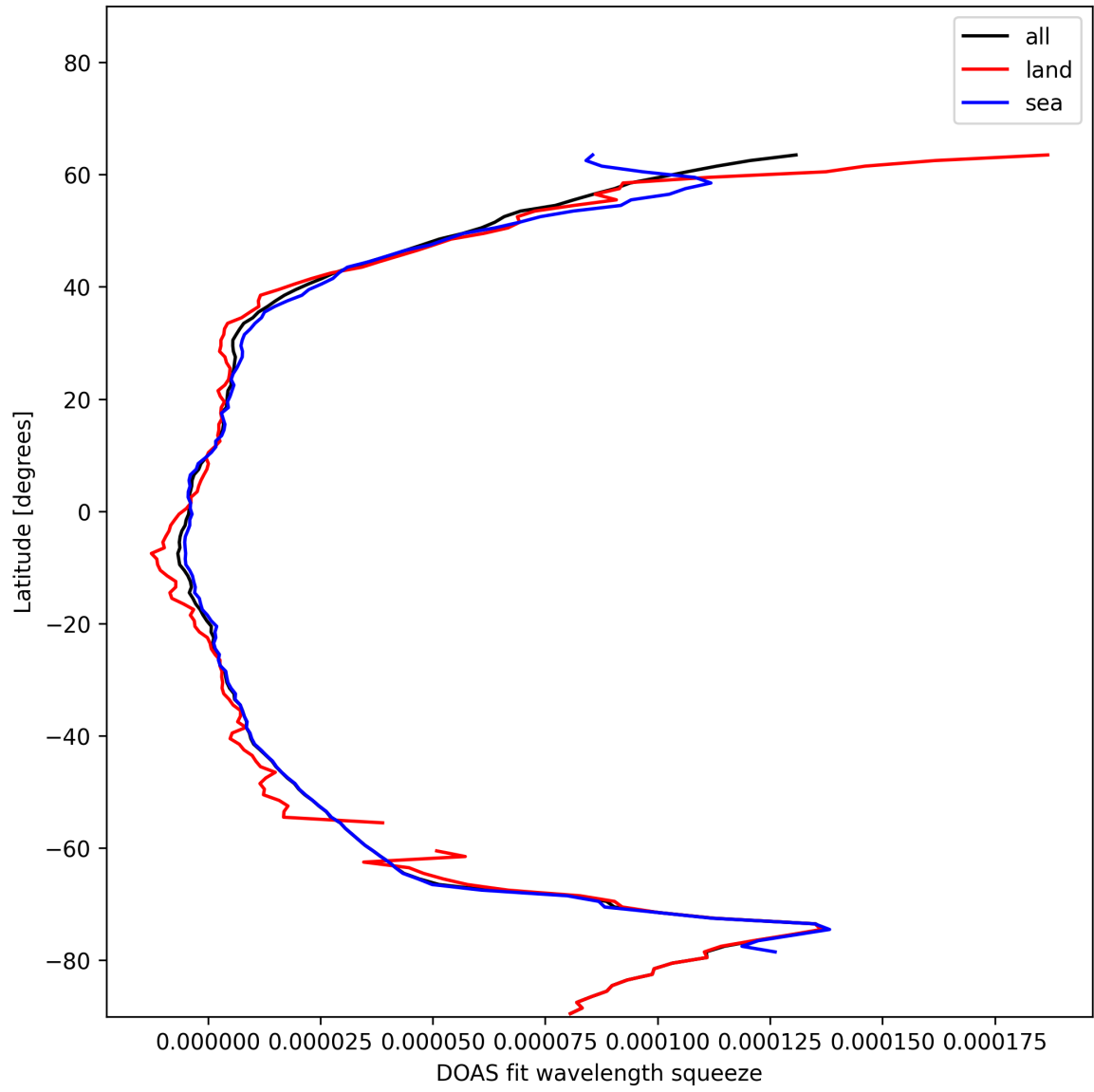
Figure 29: Zonal average of “DOAS fit wavelength squeeze” for 2025-01-13 to 2025-01-14.
