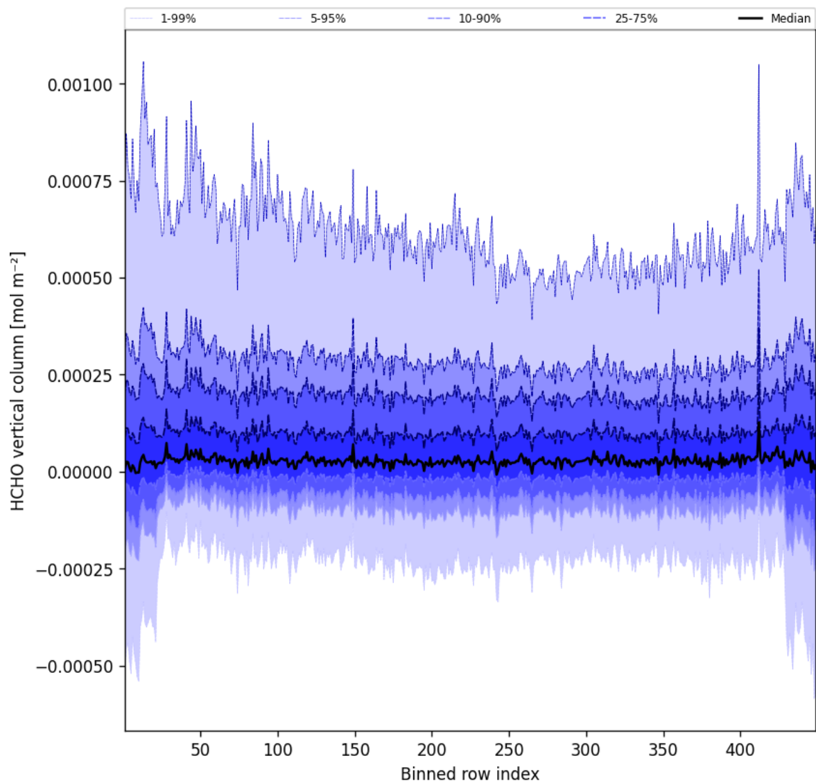
Figure 47: Along track statistics of “HCHO vertical column” for 2025-01-13 to 2025-01-14
