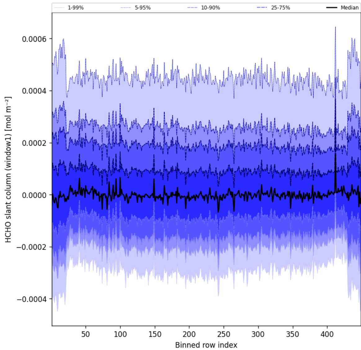
Figure 50: Along track statistics of “HCHO slant column (window1)” for 2025-01-13 to 2025-01-14
