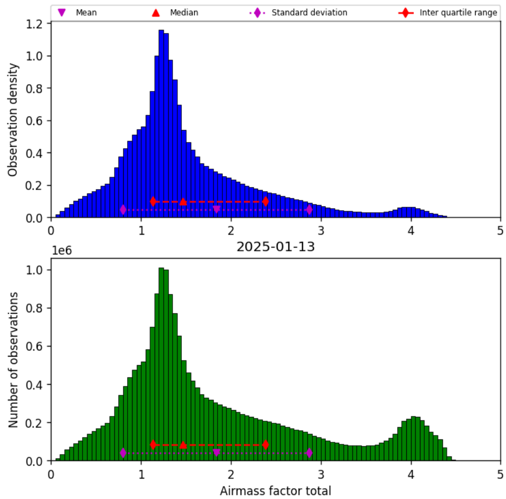
Figure 38: Histogram of “Airmass factor total” for 2025-01-13 to 2025-01-14
