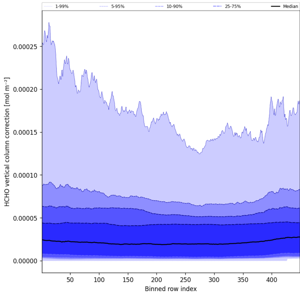
Figure 49: Along track statistics of “HCHO vertical column correction” for 2025-01-13 to 2025-01-14
