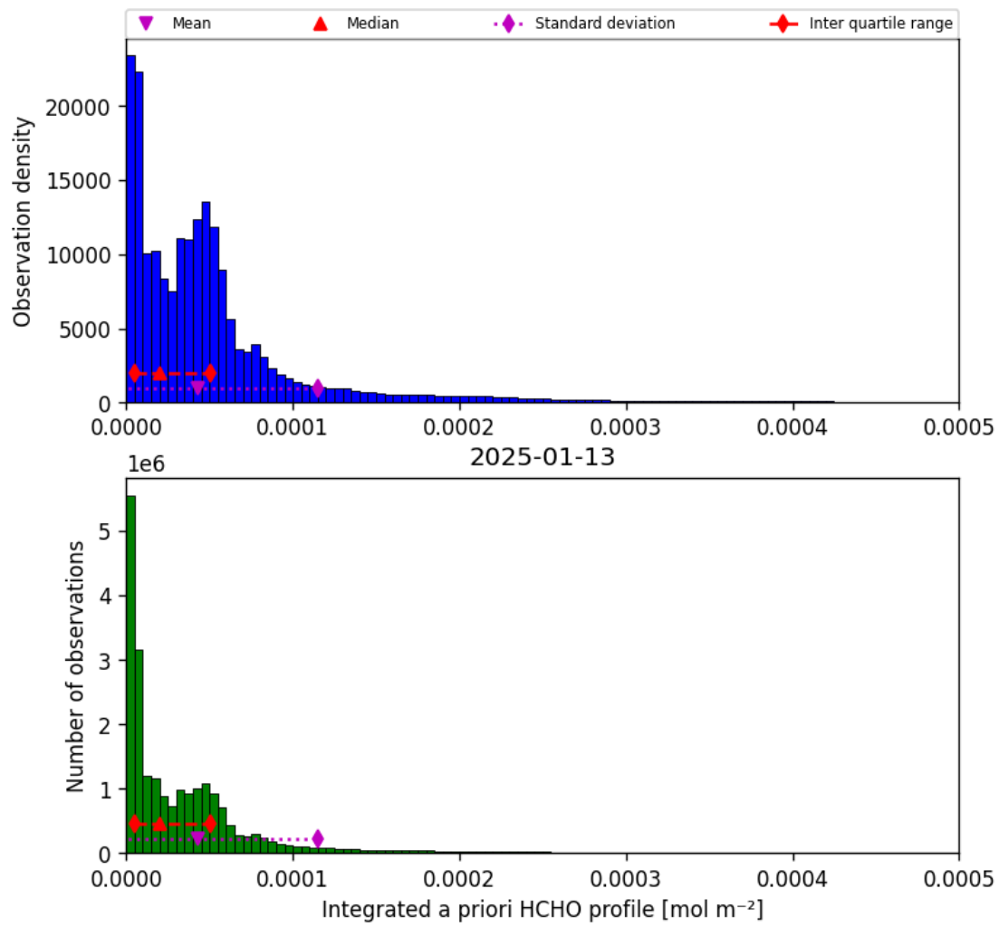
Figure 41: Histogram of “Integrated a priori HCHO profile” for 2025-01-13 to 2025-01-14
