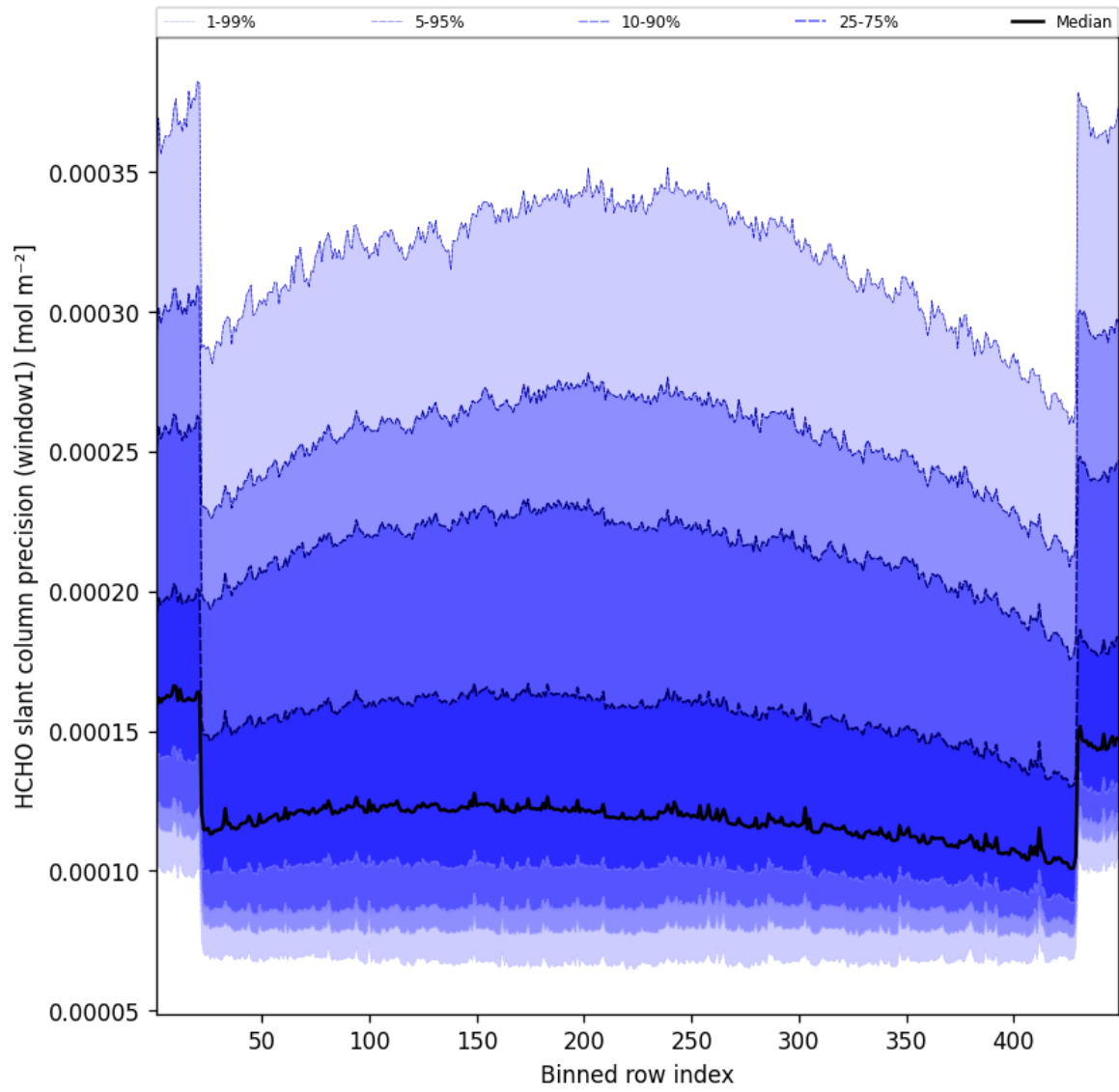
Figure 51: Along track statistics of “HCHO slant column precision (window1)” for 2025-01-13 to 2025-01-14
