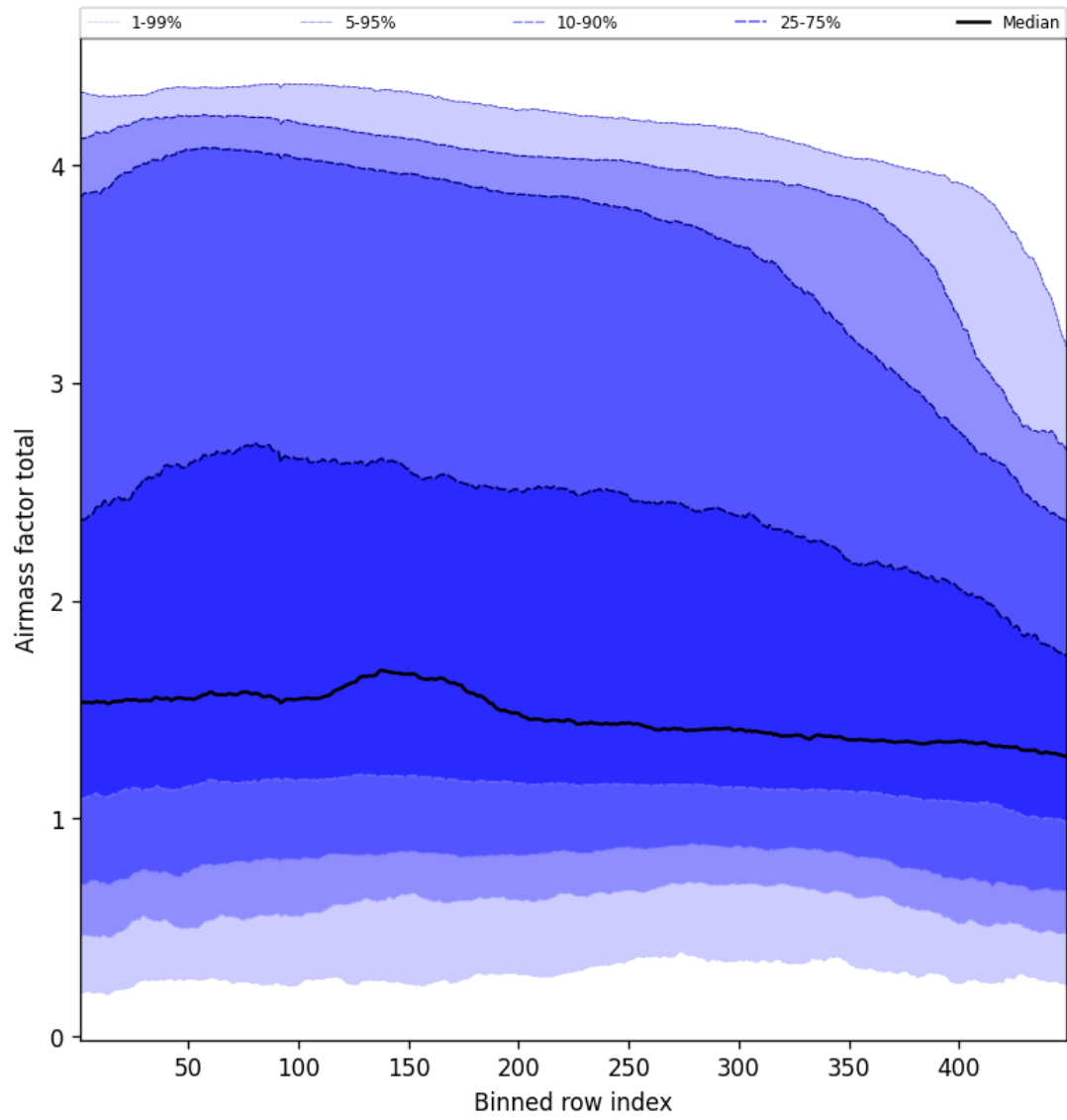
Figure 52: Along track statistics of “Airmass factor total” for 2025-01-13 to 2025-01-14
