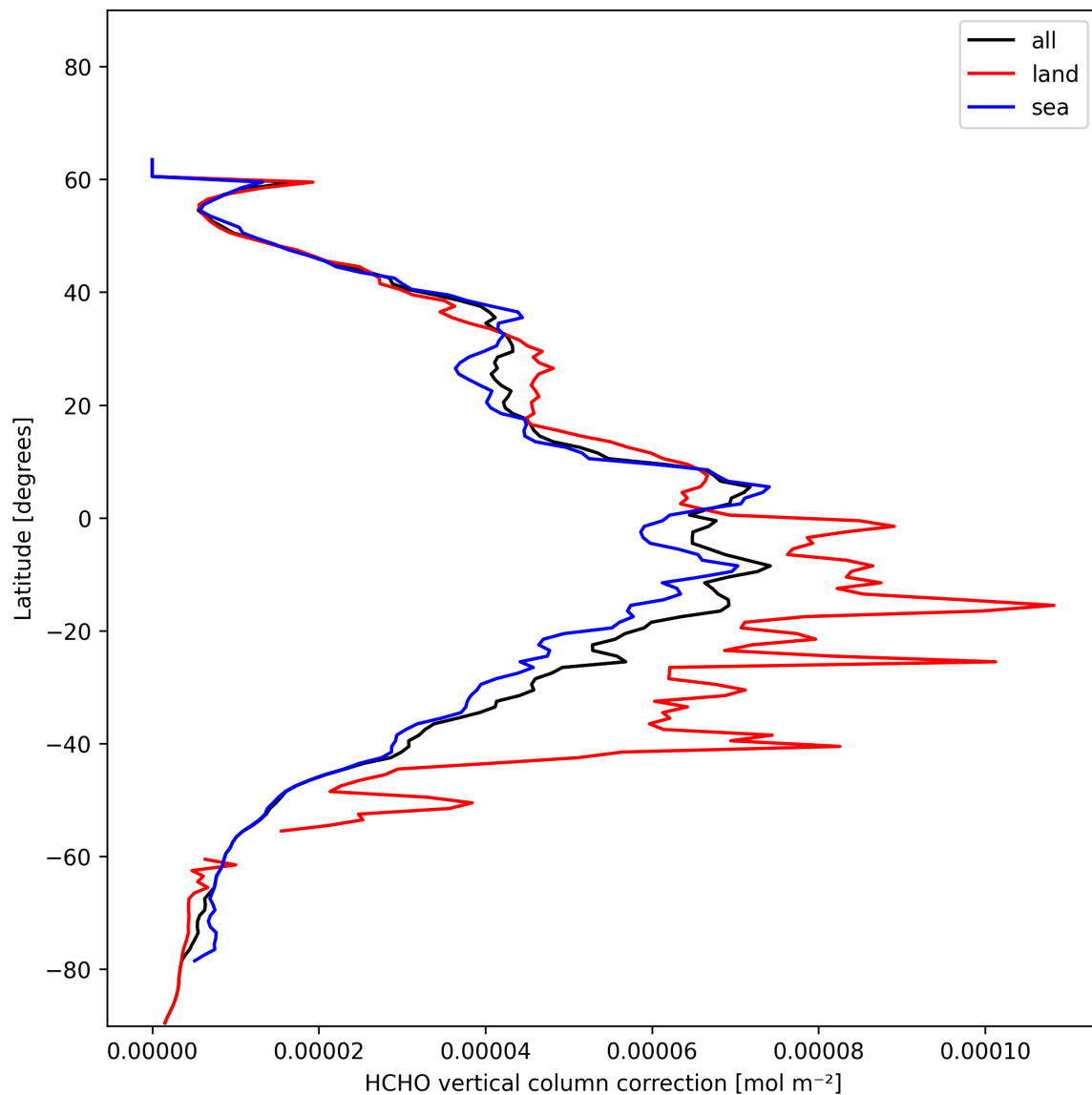
Figure 21: Zonal average of “HCHO vertical column correction” for 2025-01-13 to 2025-01-14.
