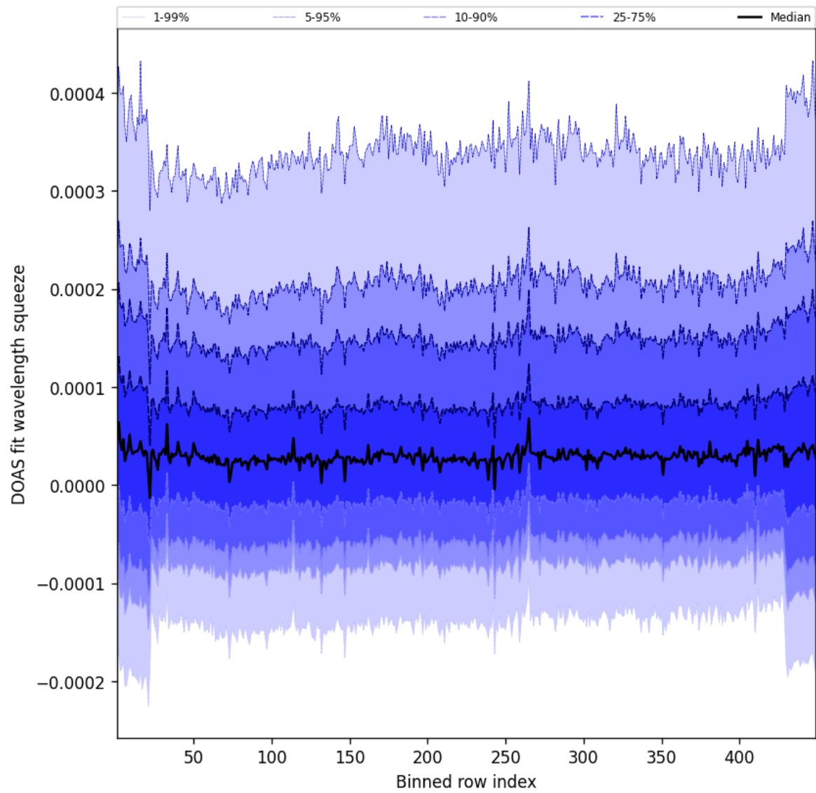
Figure 57: Along track statistics of “DOAS fit wavelength squeeze” for 2025-01-13 to 2025-01-14
