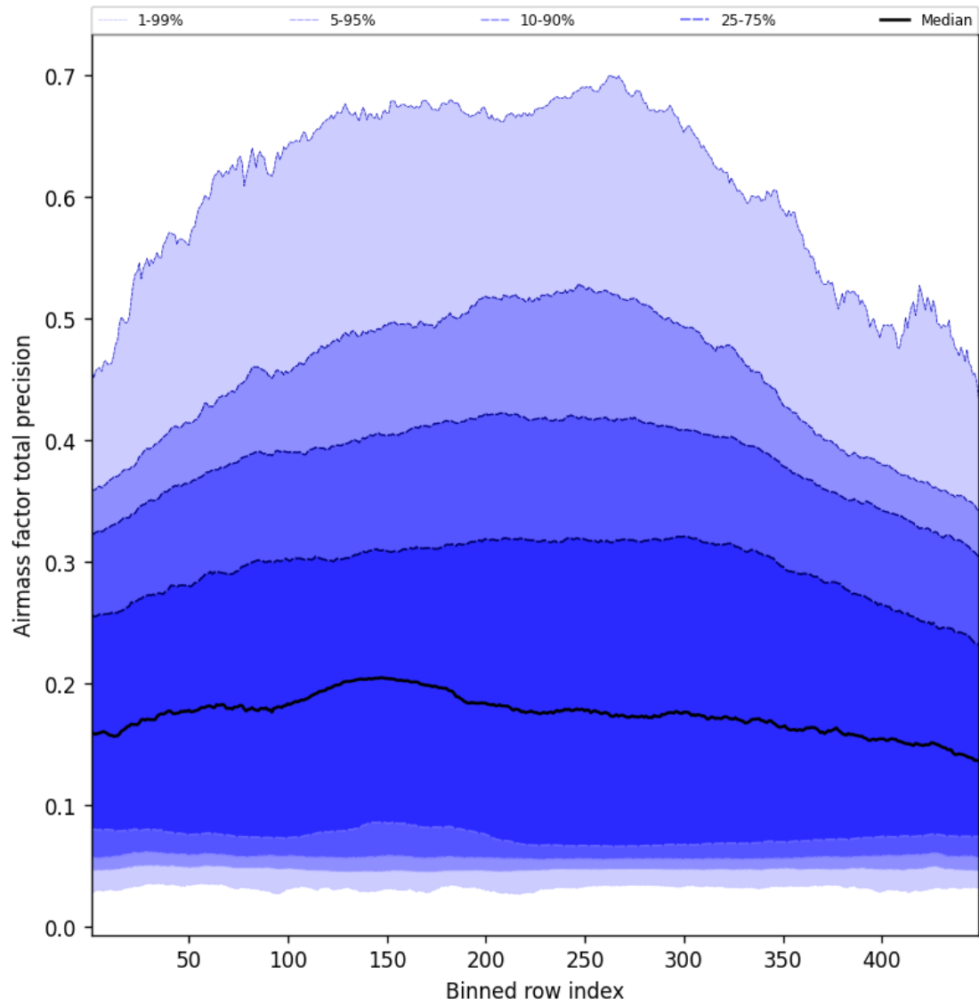
Figure 53: Along track statistics of “Airmass factor total precision” for 2025-01-13 to 2025-01-14
