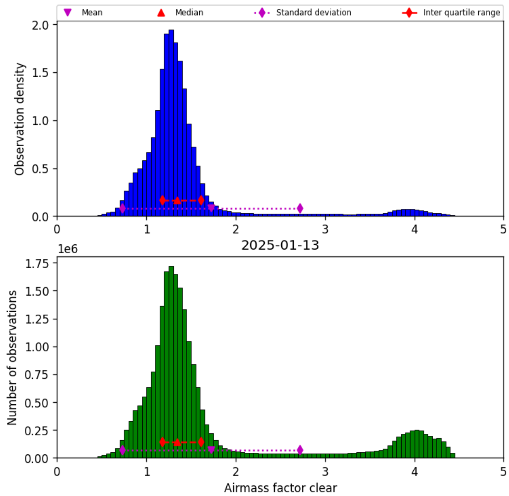
Figure 40: Histogram of “Airmass factor clear” for 2025-01-13 to 2025-01-14
