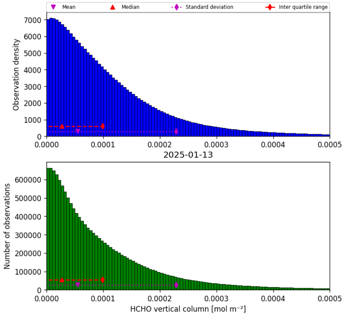
Figure 33: Histogram of “HCHO vertical column” for 2025-01-13 to 2025-01-14
