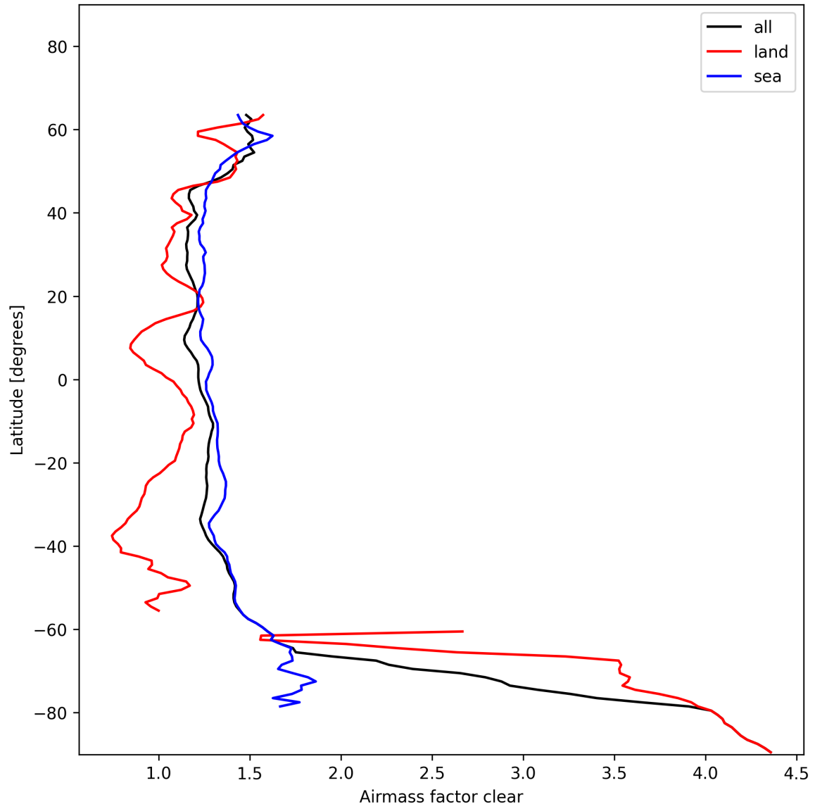
Figure 26: Zonal average of “Airmass factor clear” for 2025-01-13 to 2025-01-14.
