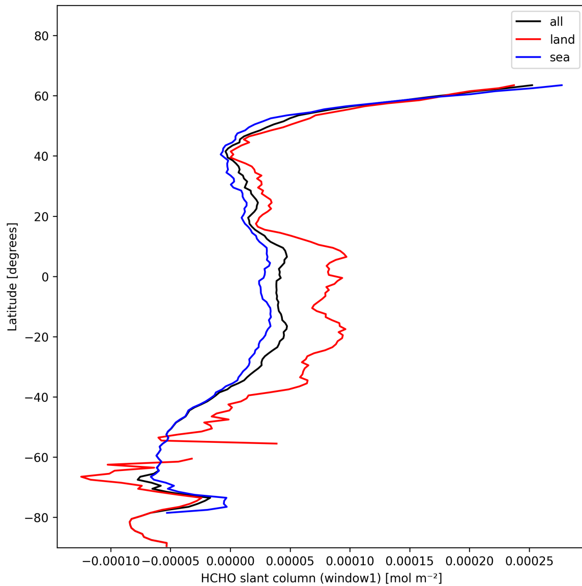
Figure 22: Zonal average of “HCHO slant column (window1)” for 2025-01-13 to 2025-01-14.
