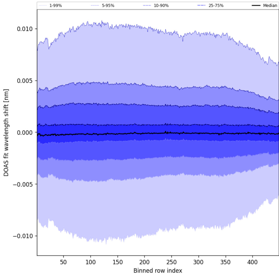
Figure 56: Along track statistics of “DOAS fit wavelength shift” for 2025-01-13 to 2025-01-14
