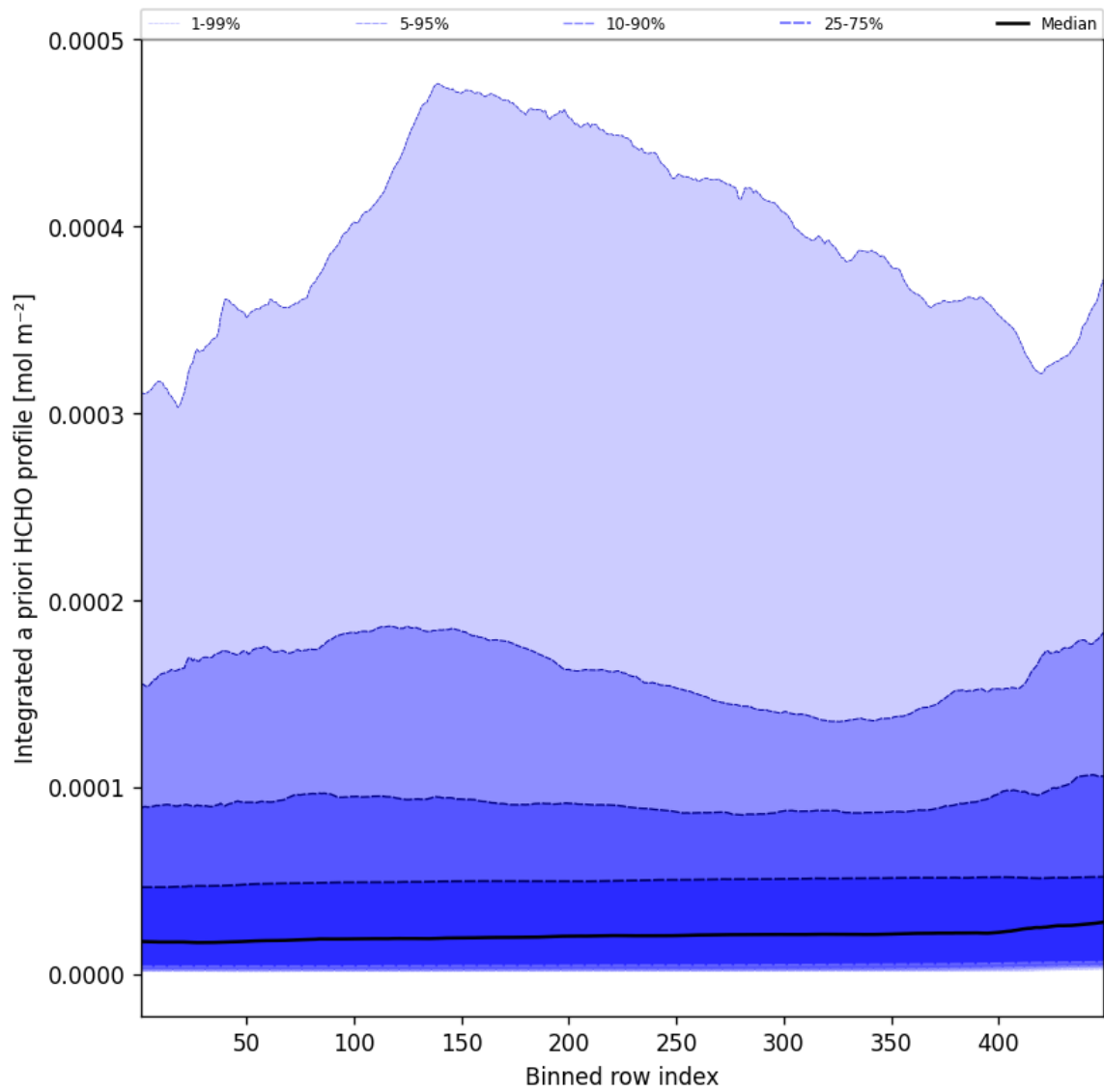
Figure 55: Along track statistics of “Integrated a priori HCHO profile” for 2025-01-13 to 2025-01-14
