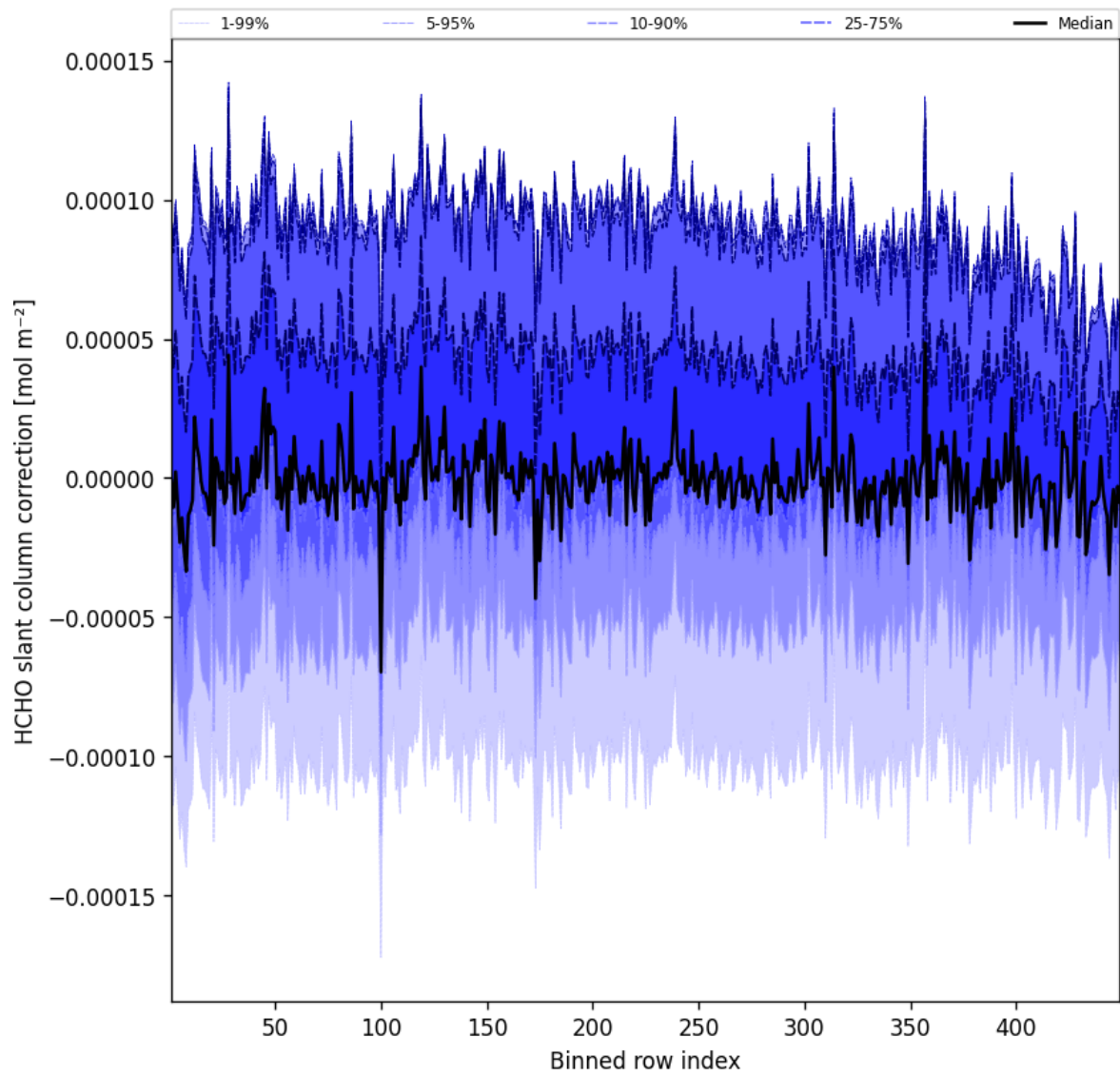
Figure 59: Along track statistics of “HCHO slant column correction” for 2025-01-13 to 2025-01-14
