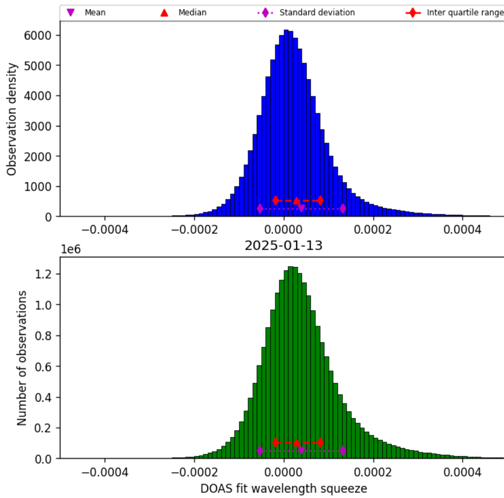
Figure 43: Histogram of “DOAS fit wavelength squeeze” for 2025-01-13 to 2025-01-14
