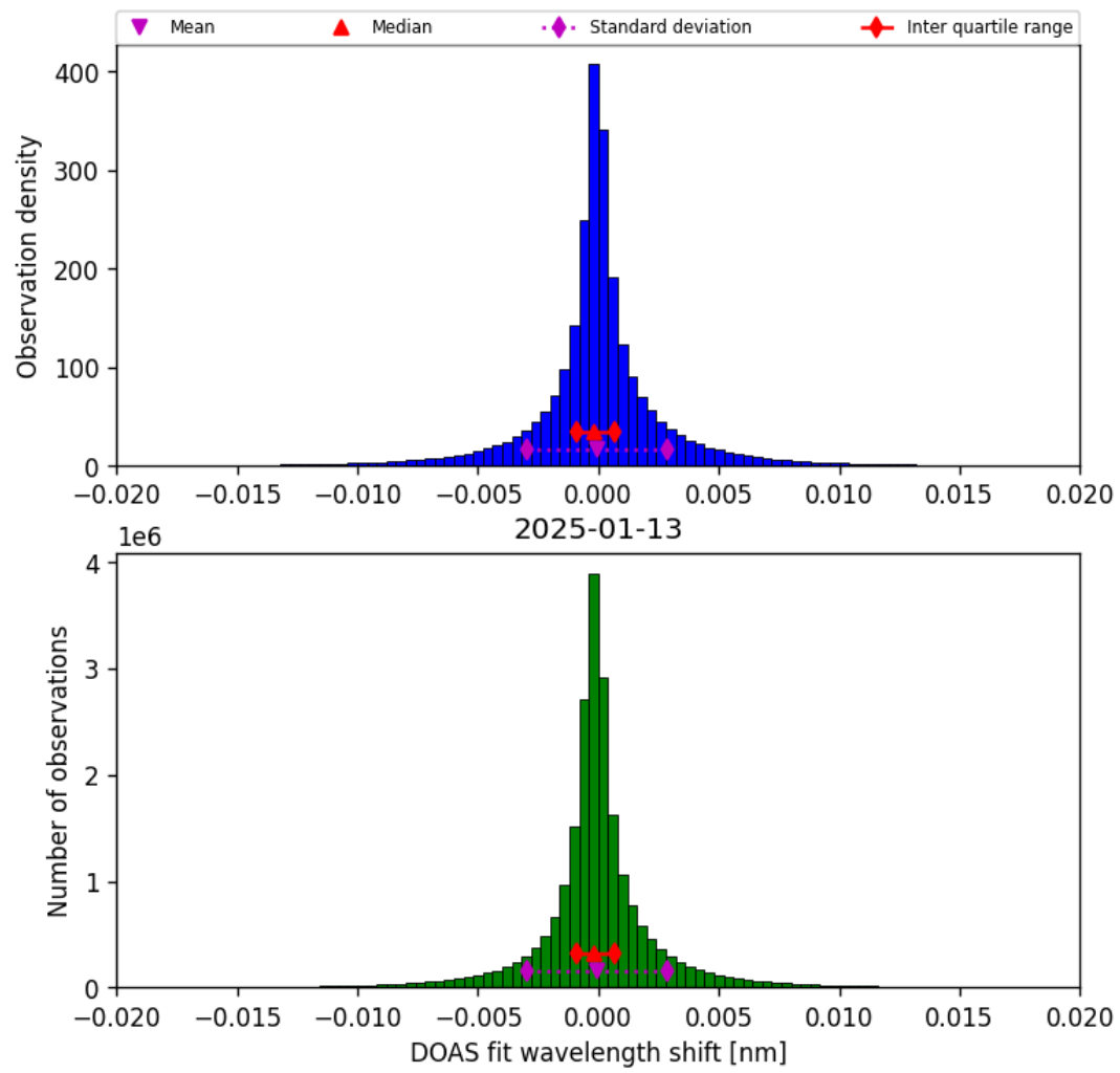
Figure 42: Histogram of “DOAS fit wavelength shift” for 2025-01-13 to 2025-01-14
