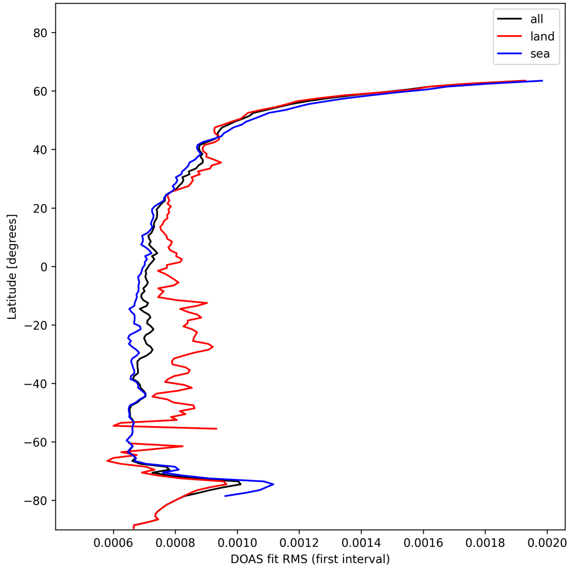
Figure 30: Zonal average of “DOAS fit RMS (first interval)” for 2025-01-13 to 2025-01-14.
