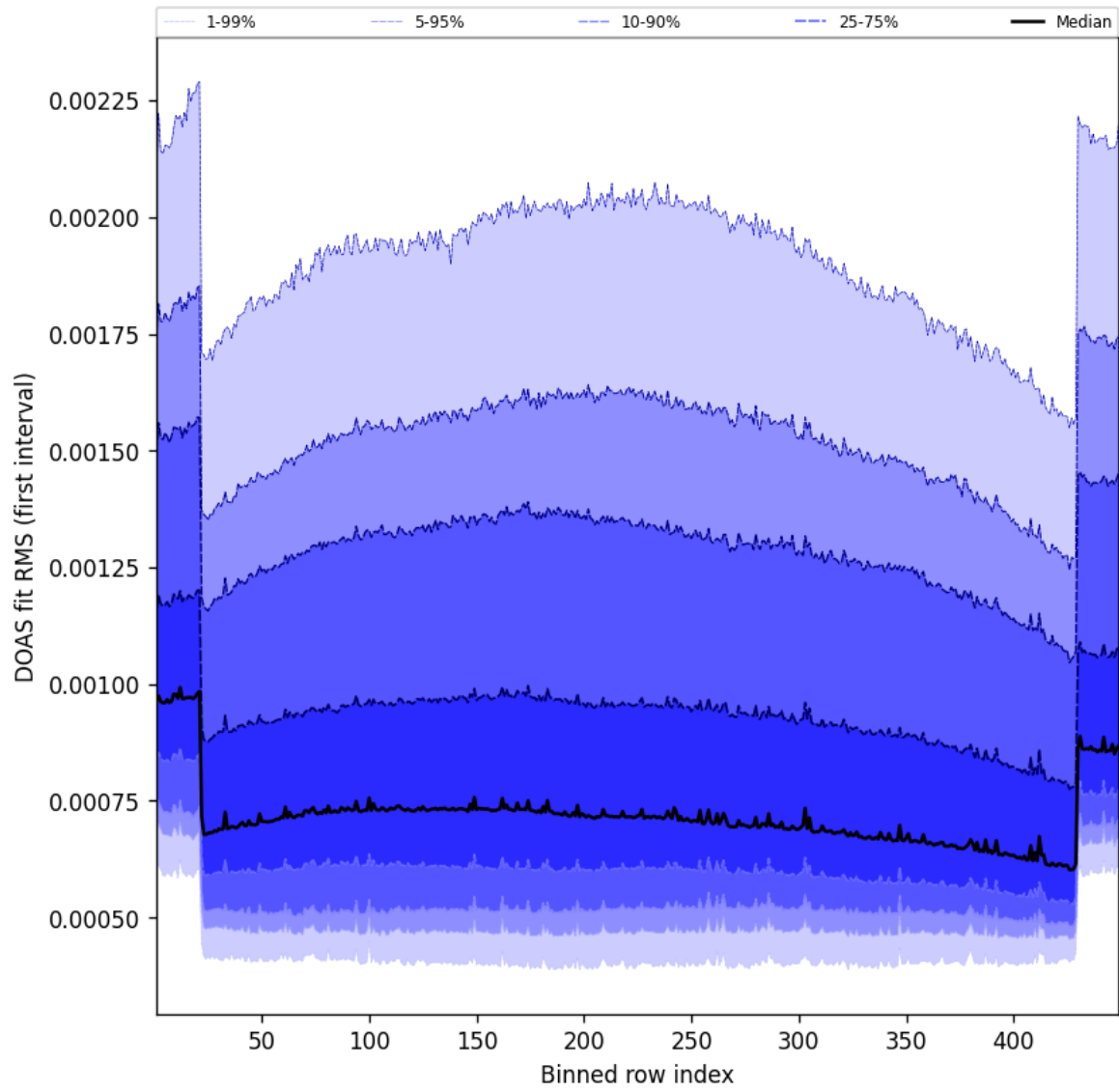
Figure 58: Along track statistics of “DOAS fit RMS (first interval)” for 2025-01-13 to 2025-01-14
