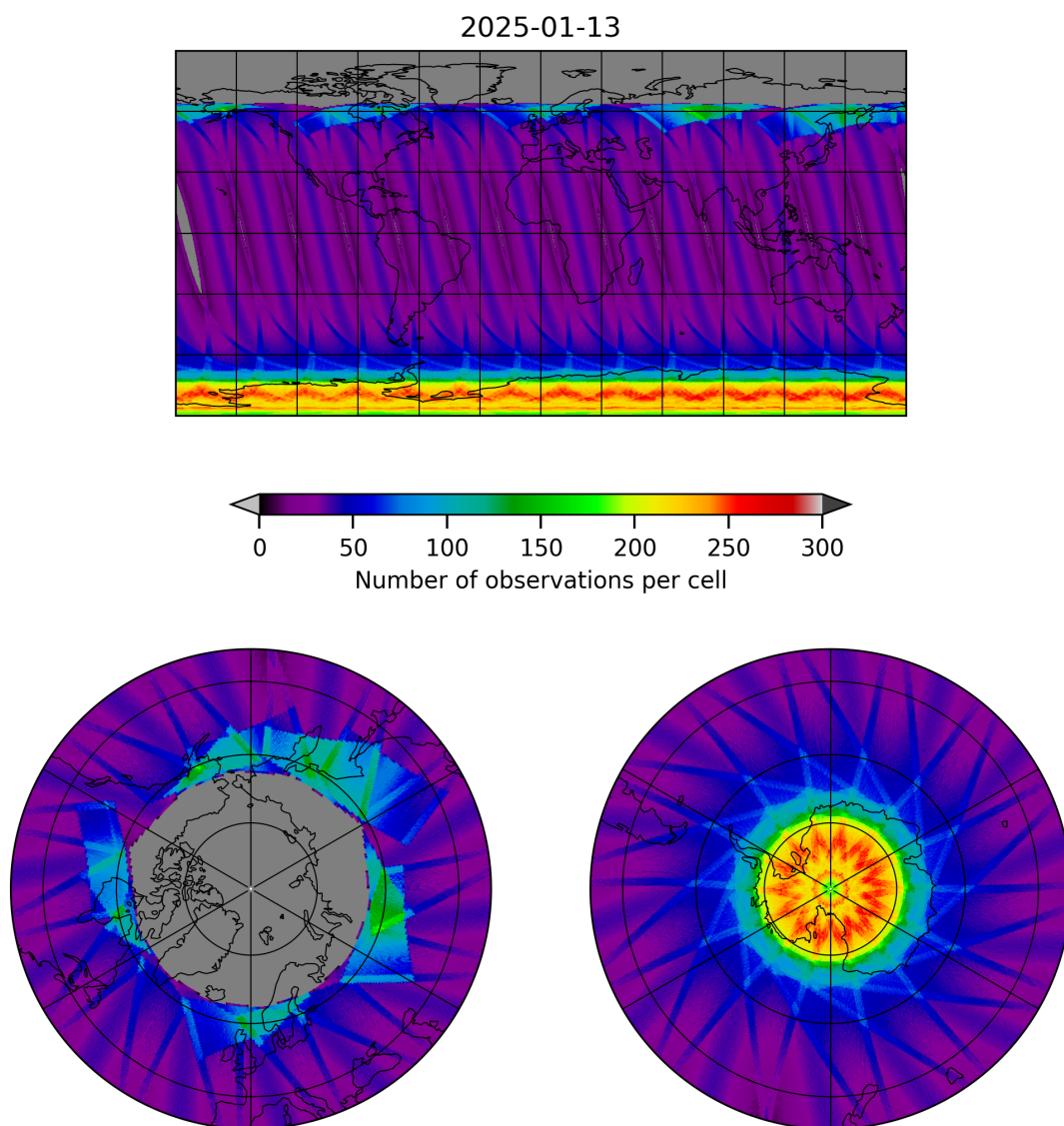
Figure 17: Map of the number of observations for 2025-01-13 to 2025-01-14
