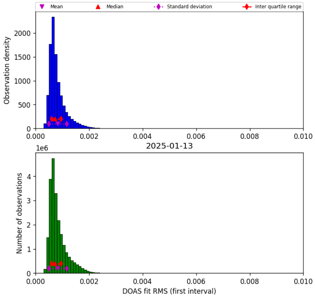
Figure 44: Histogram of "DOAS fit RMS (first interval)" for 2025-01-13 to 2025-01-14
