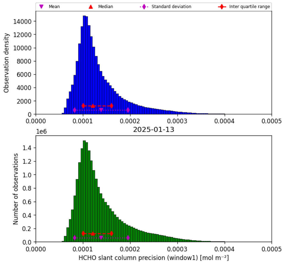
Figure 37: Histogram of “HCHO slant column precision (window1)” for 2025-01-13 to 2025-01-14
