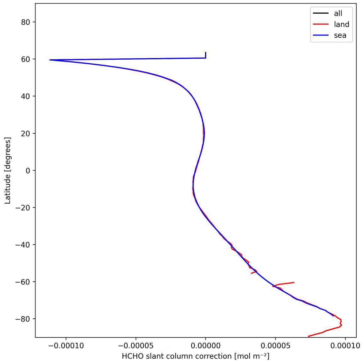
Figure 31: Zonal average of “HCHO slant column correction” for 2025-01-13 to 2025-01-14.
