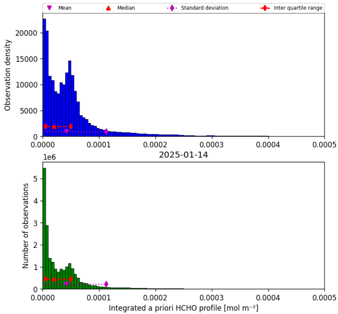
Figure 41: Histogram of “Integrated a priori HCHO profile” for 2025-01-14 to 2025-01-15
