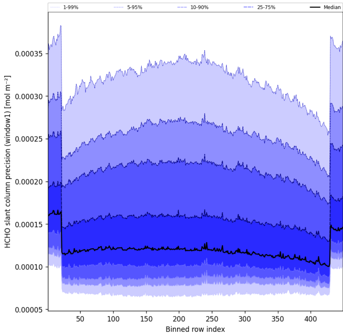
Figure 51: Along track statistics of “HCHO slant column precision (window1)” for 2025-01-14 to 2025-01-15
