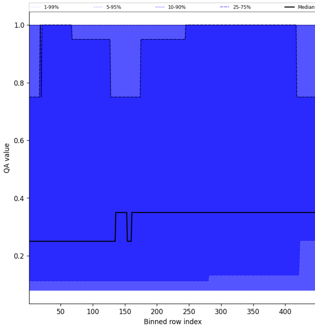
Figure 46: Along track statistics of “QA value” for 2025-01-14 to 2025-01-15
