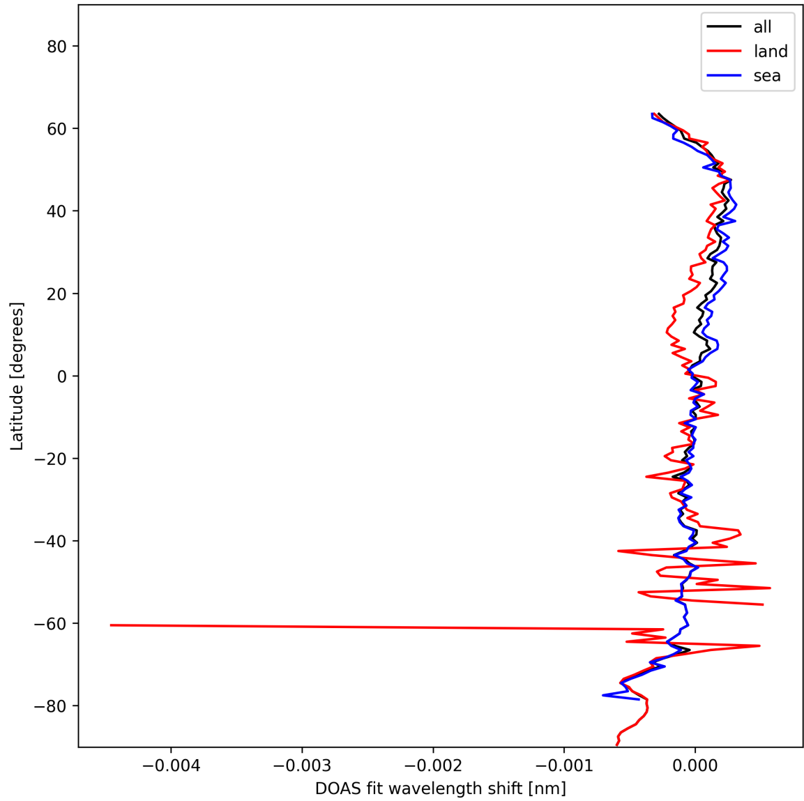
Figure 28: Zonal average of "DOAS fit wavelength shift" for 2025-01-14 to 2025-01-15.
