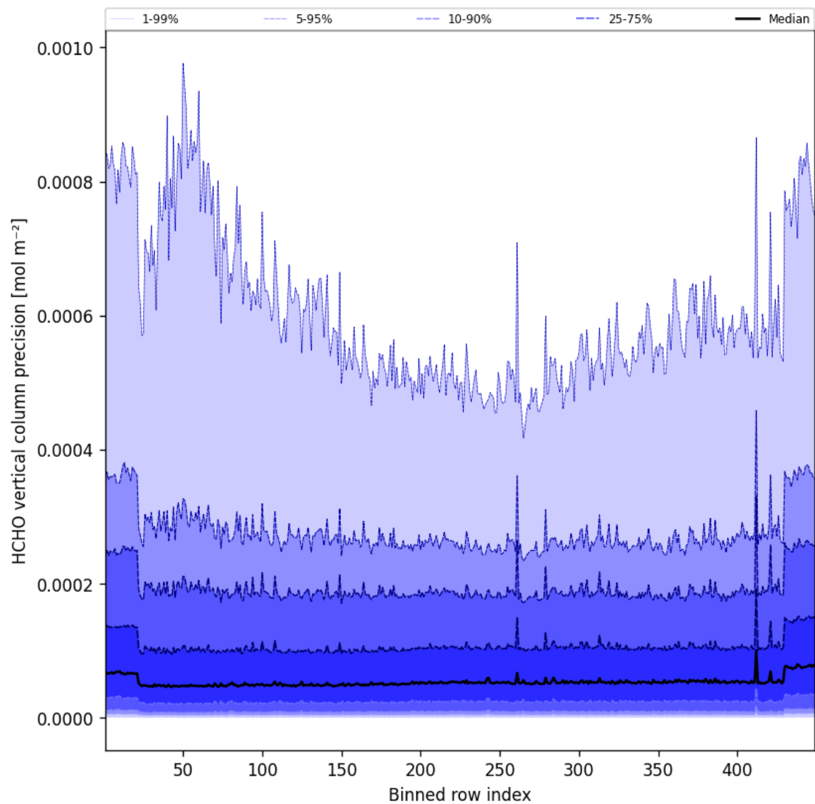
Figure 48: Along track statistics of “HCHO vertical column precision” for 2025-01-14 to 2025-01-15
