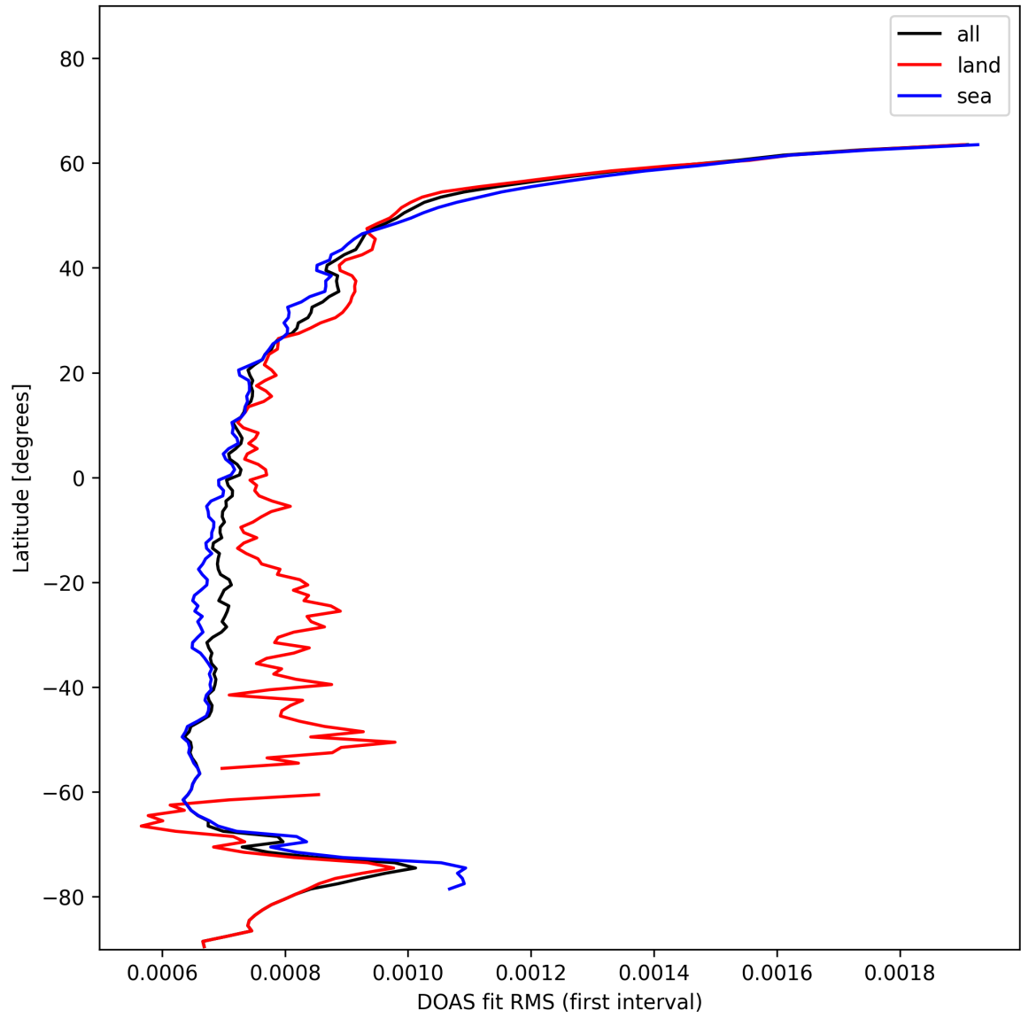
Figure 30: Zonal average of “DOAS fit RMS (first interval)” for 2025-01-14 to 2025-01-15.
