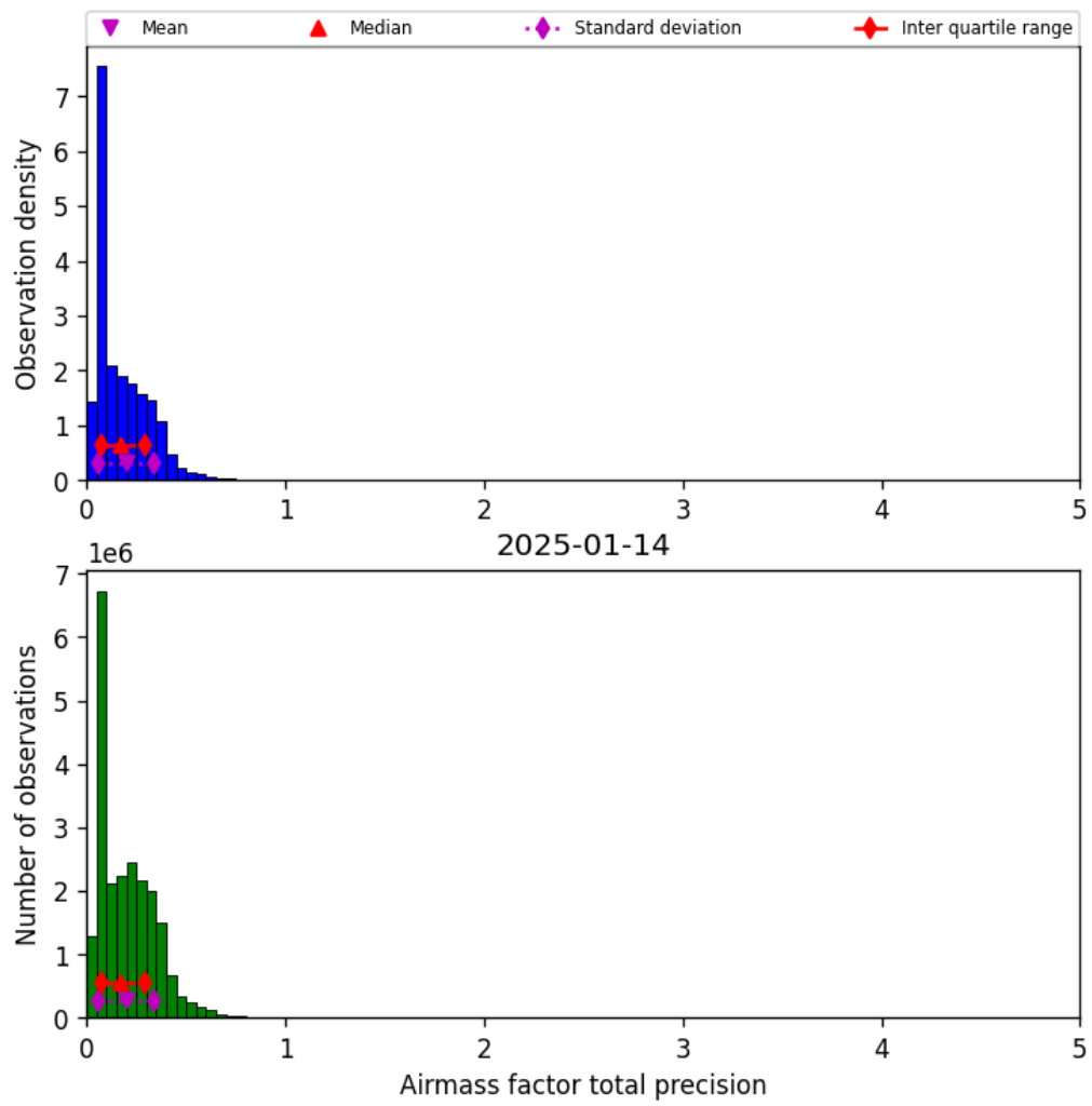
Figure 39: Histogram of “Airmass factor total precision” for 2025-01-14 to 2025-01-15
