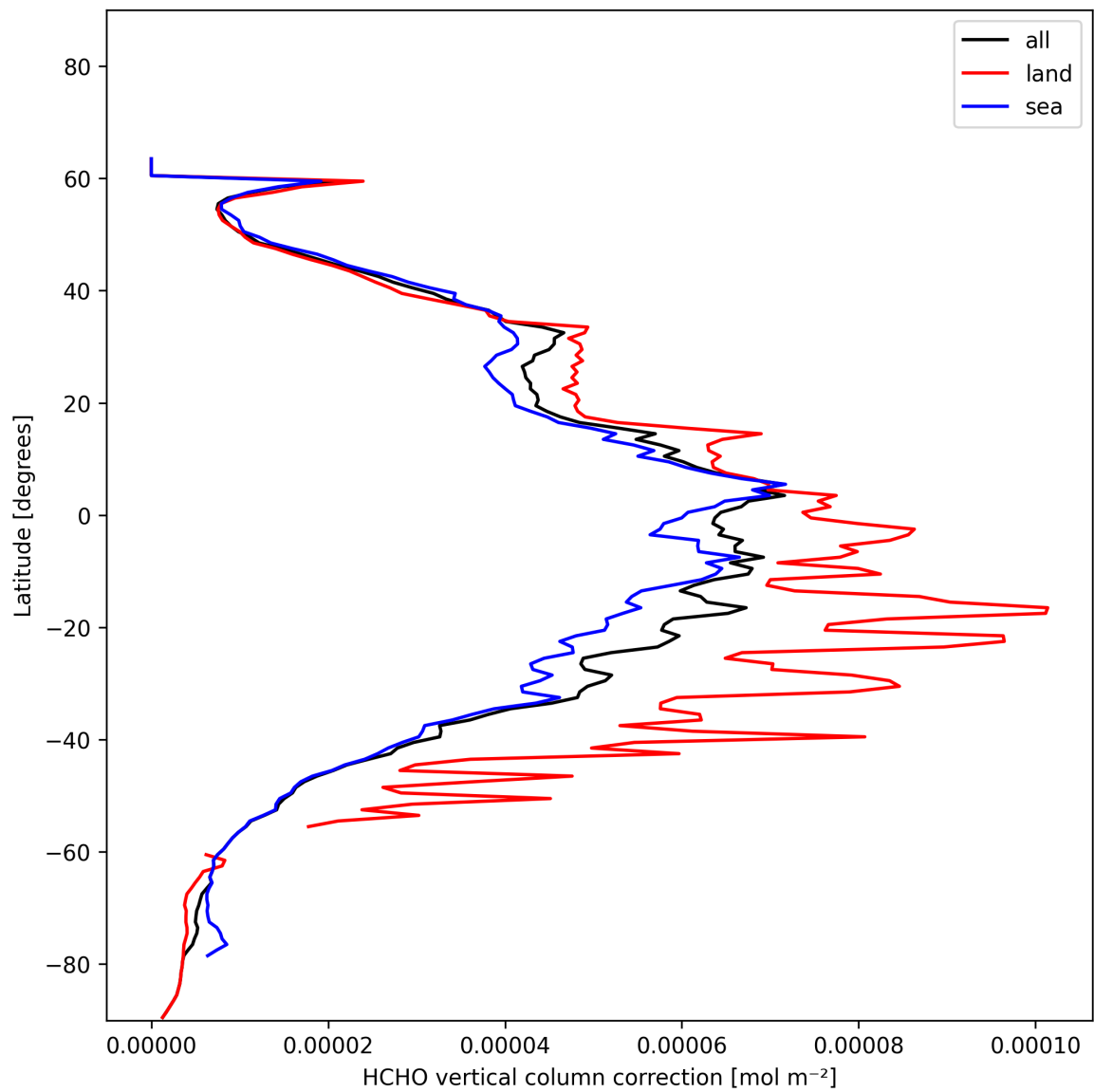
Figure 21: Zonal average of “HCHO vertical column correction” for 2025-01-14 to 2025-01-15.
