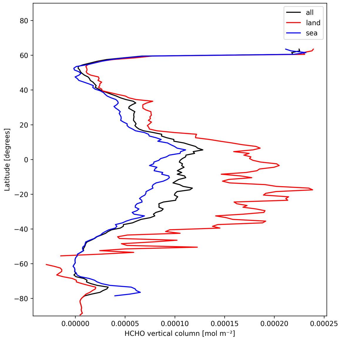
Figure 19: Zonal average of “HCHO vertical column” for 2025-01-14 to 2025-01-15.
