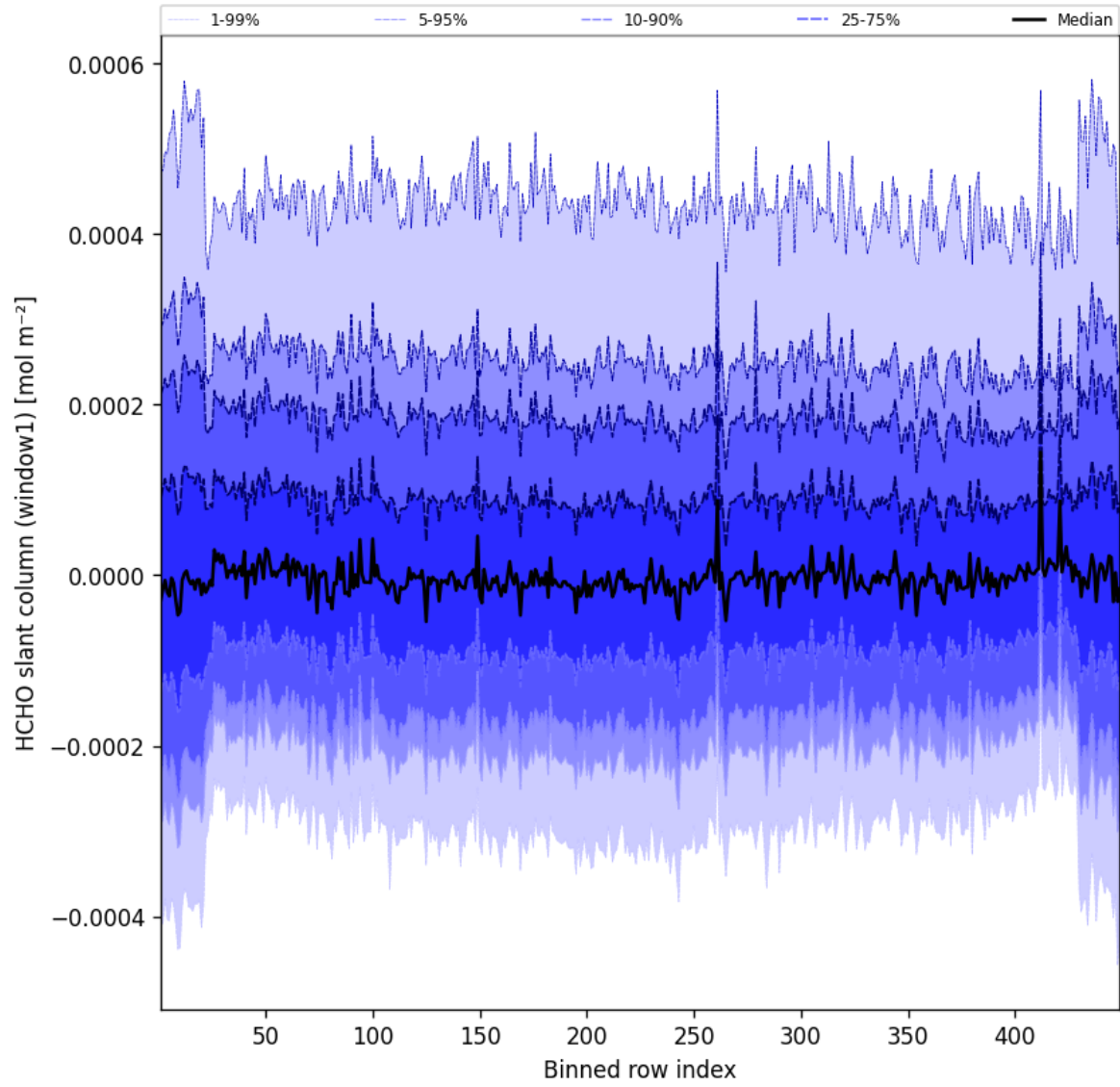
Figure 50: Along track statistics of “HCHO slant column (window1)” for 2025-01-14 to 2025-01-15
