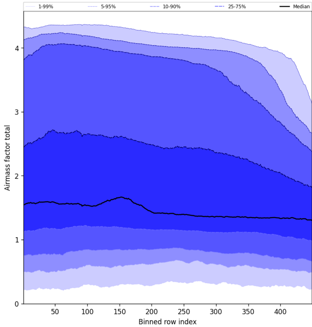
Figure 52: Along track statistics of “Airmass factor total” for 2025-01-14 to 2025-01-15
