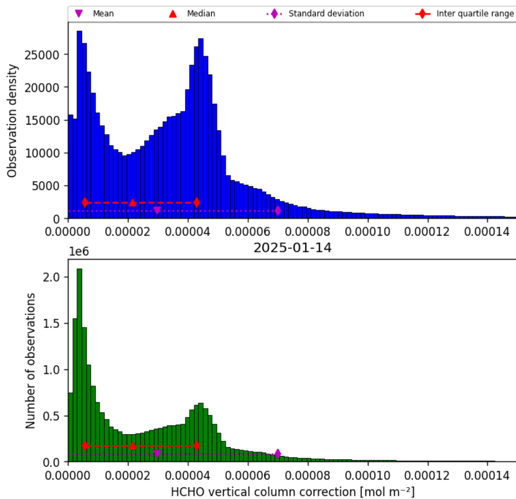
Figure 35: Histogram of “HCHO vertical column correction” for 2025-01-14 to 2025-01-15
