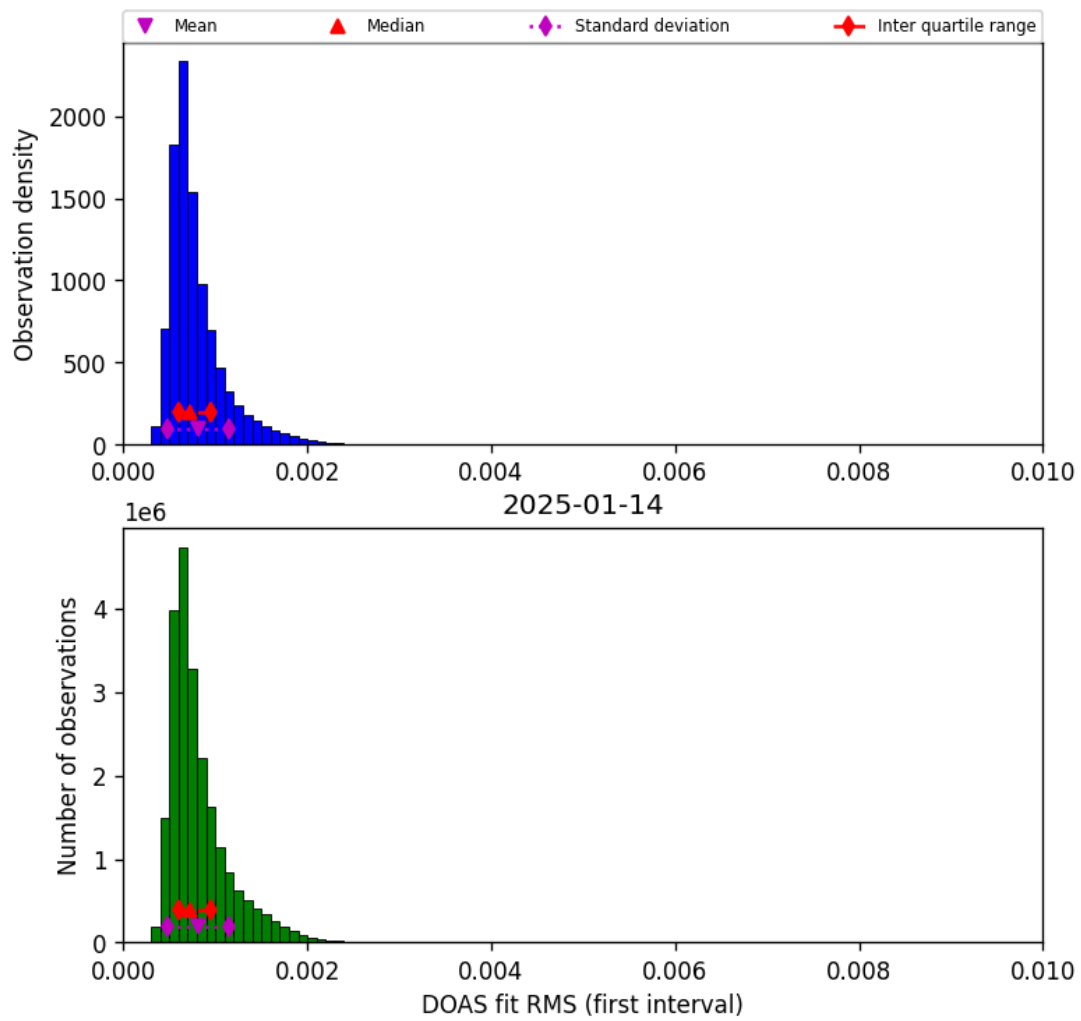
Figure 44: Histogram of "DOAS fit RMS (first interval)" for 2025-01-14 to 2025-01-15
