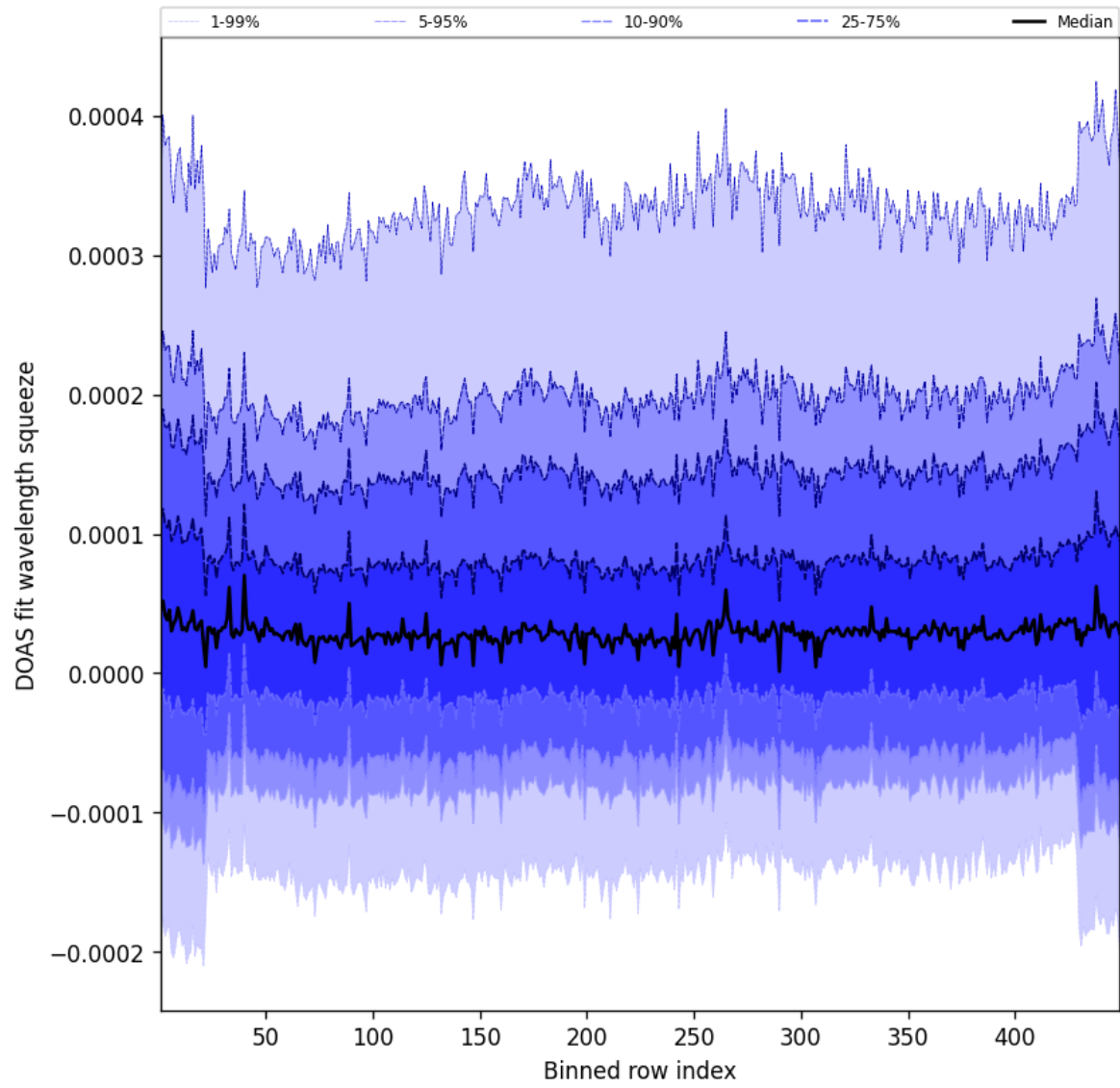
Figure 57: Along track statistics of “DOAS fit wavelength squeeze” for 2025-01-14 to 2025-01-15
