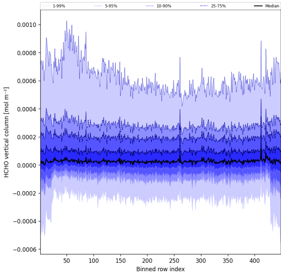
Figure 47: Along track statistics of “HCHO vertical column” for 2025-01-14 to 2025-01-15
