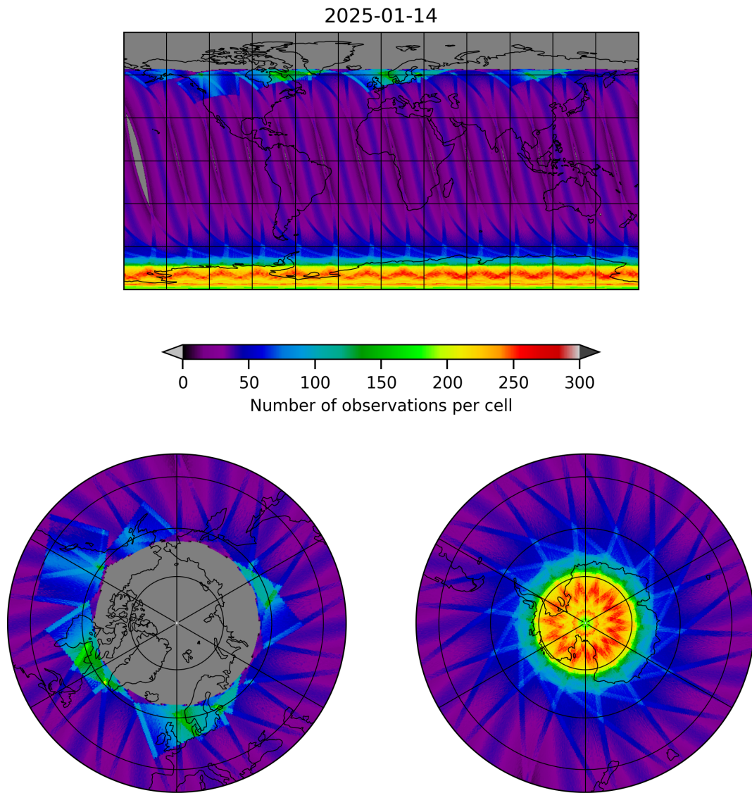
Figure 17: Map of the number of observations for 2025-01-14 to 2025-01-15
