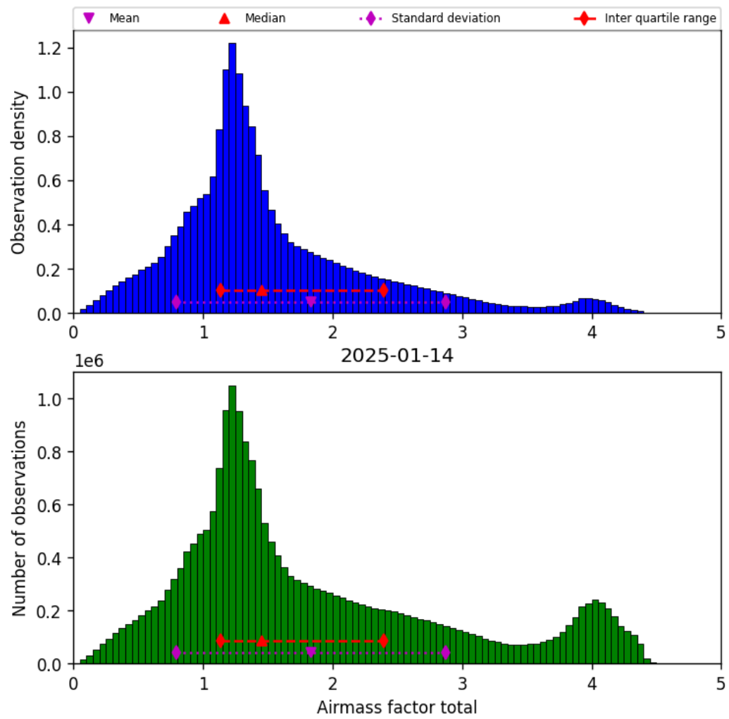
Figure 38: Histogram of “Airmass factor total” for 2025-01-14 to 2025-01-15
