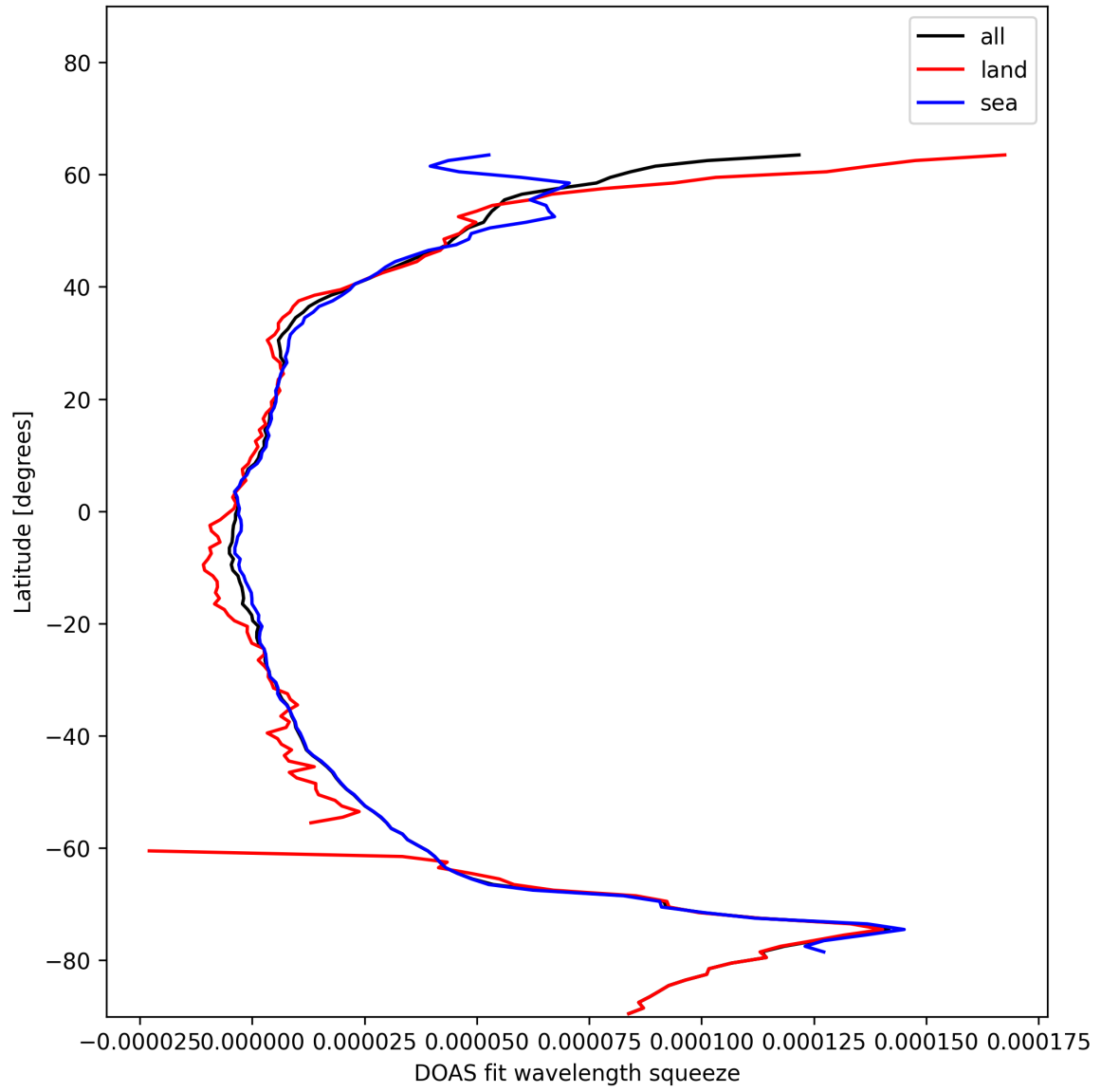
Figure 29: Zonal average of “DOAS fit wavelength squeeze” for 2025-01-14 to 2025-01-15.
