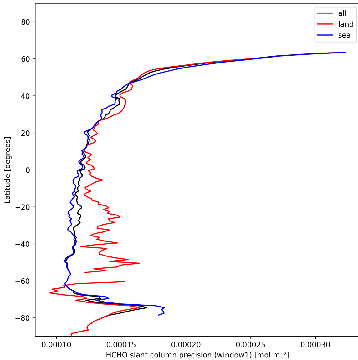
Figure 23: Zonal average of “HCHO slant column precision (window1)” for 2025-01-14 to 2025-01-15.
