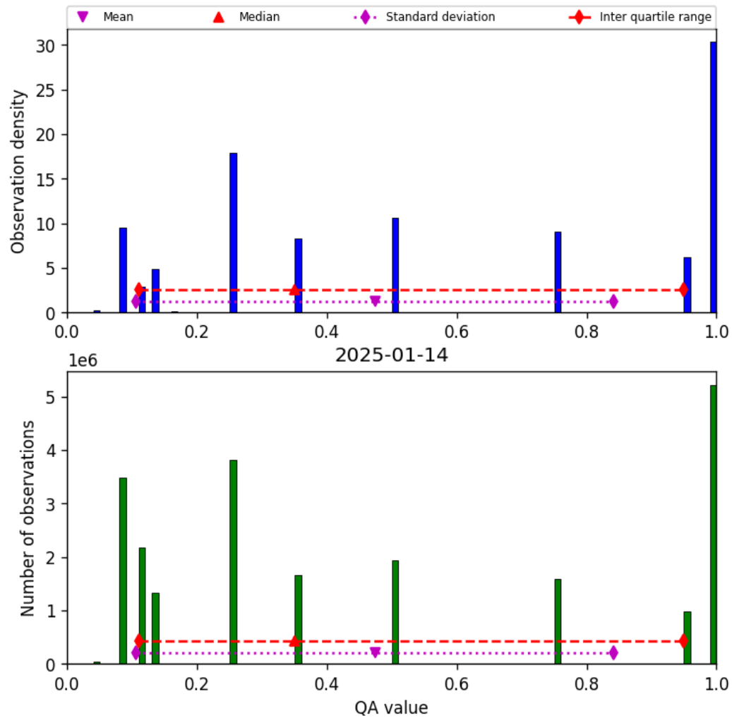
Figure 32: Histogram of “QA value” for 2025-01-14 to 2025-01-15
