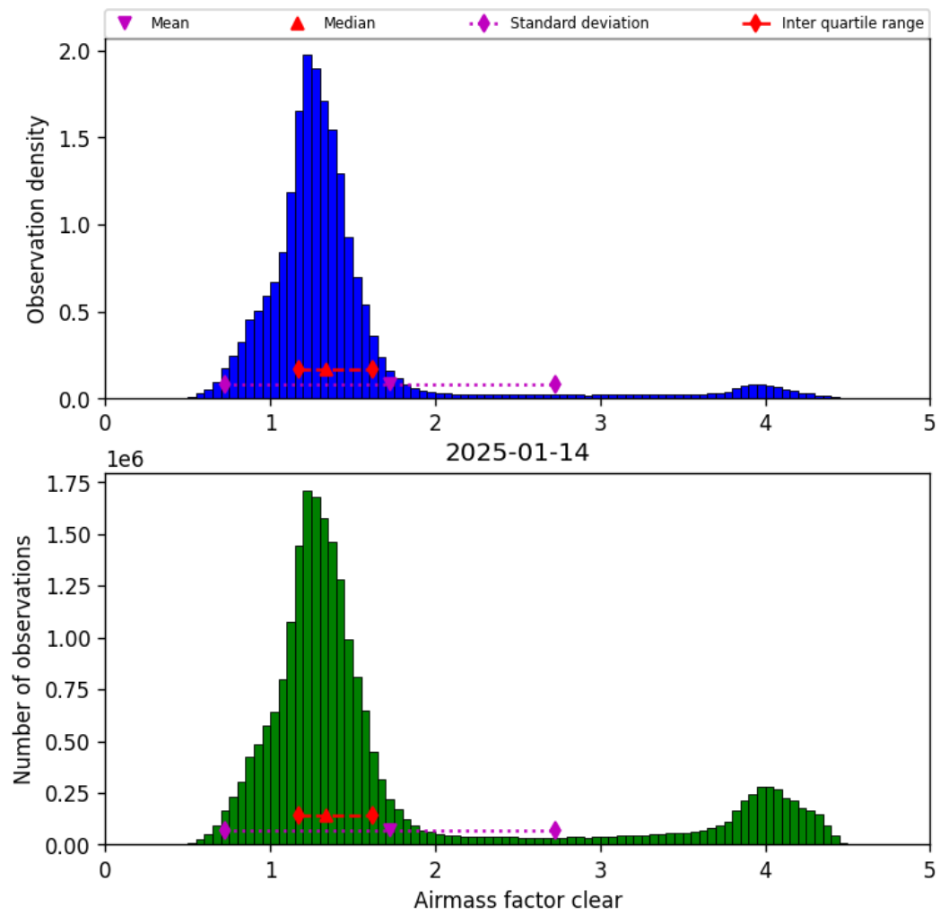
Figure 40: Histogram of “Airmass factor clear” for 2025-01-14 to 2025-01-15
