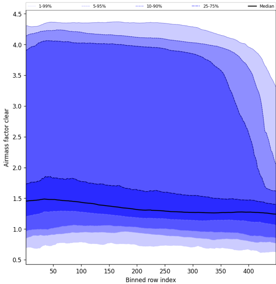
Figure 54: Along track statistics of “Airmass factor clear” for 2025-01-14 to 2025-01-15
