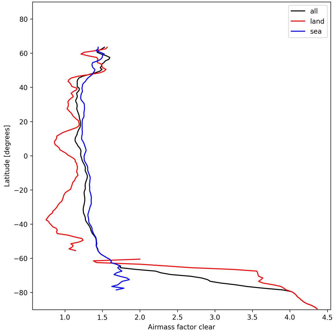
Figure 26: Zonal average of “Airmass factor clear” for 2025-01-14 to 2025-01-15.
