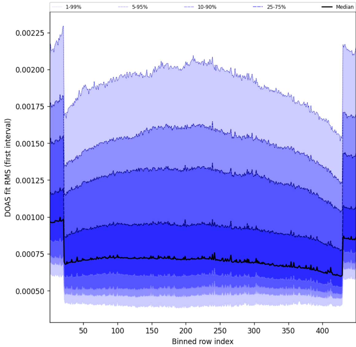
Figure 58: Along track statistics of “DOAS fit RMS (first interval)” for 2025-01-14 to 2025-01-15
