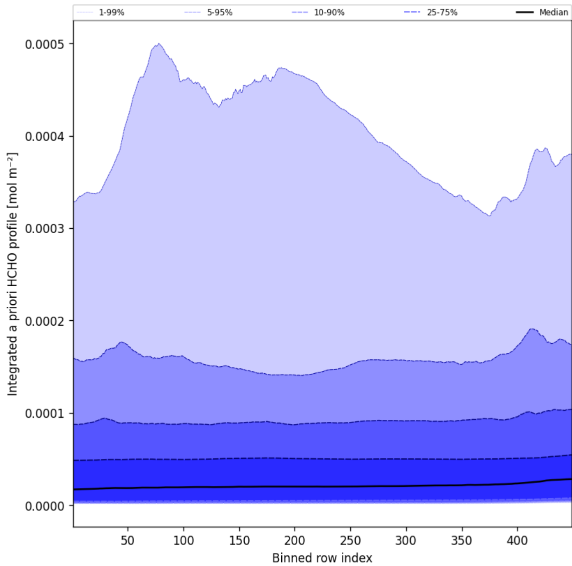
Figure 55: Along track statistics of “Integrated a priori HCHO profile” for 2025-01-14 to 2025-01-15
