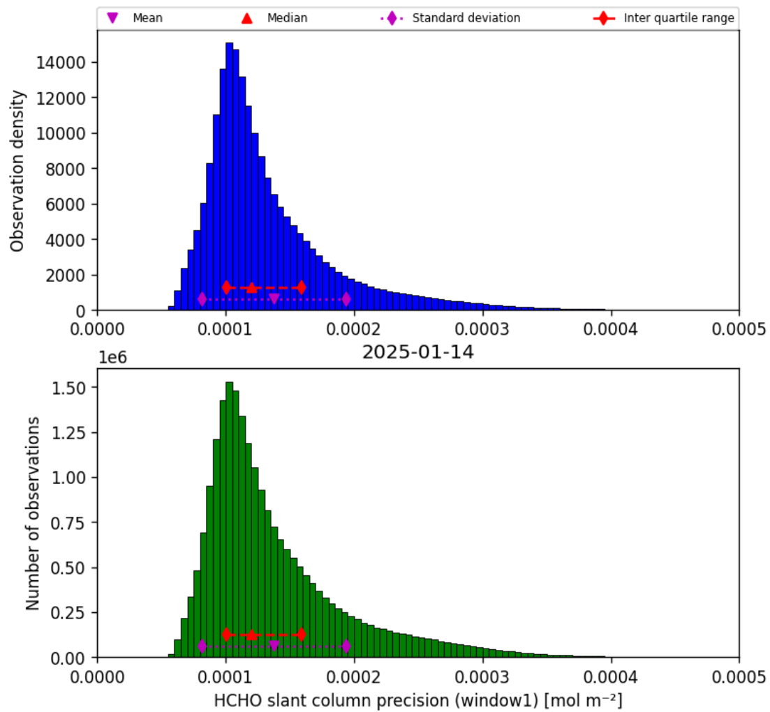
Figure 37: Histogram of “HCHO slant column precision (window1)” for 2025-01-14 to 2025-01-15
