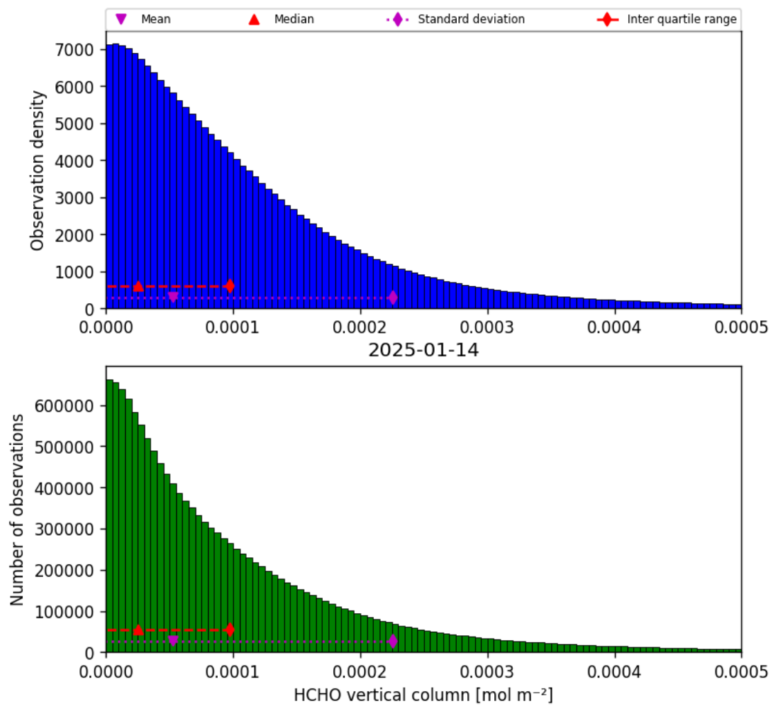
Figure 33: Histogram of “HCHO vertical column” for 2025-01-14 to 2025-01-15
