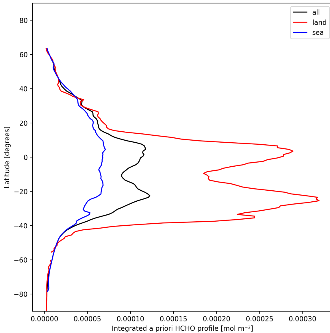
Figure 27: Zonal average of “Integrated a priori HCHO profile” for 2025-01-14 to 2025-01-15.
