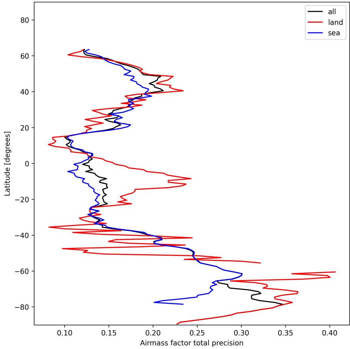
Figure 25: Zonal average of “Airmass factor total precision” for 2025-01-14 to 2025-01-15.
