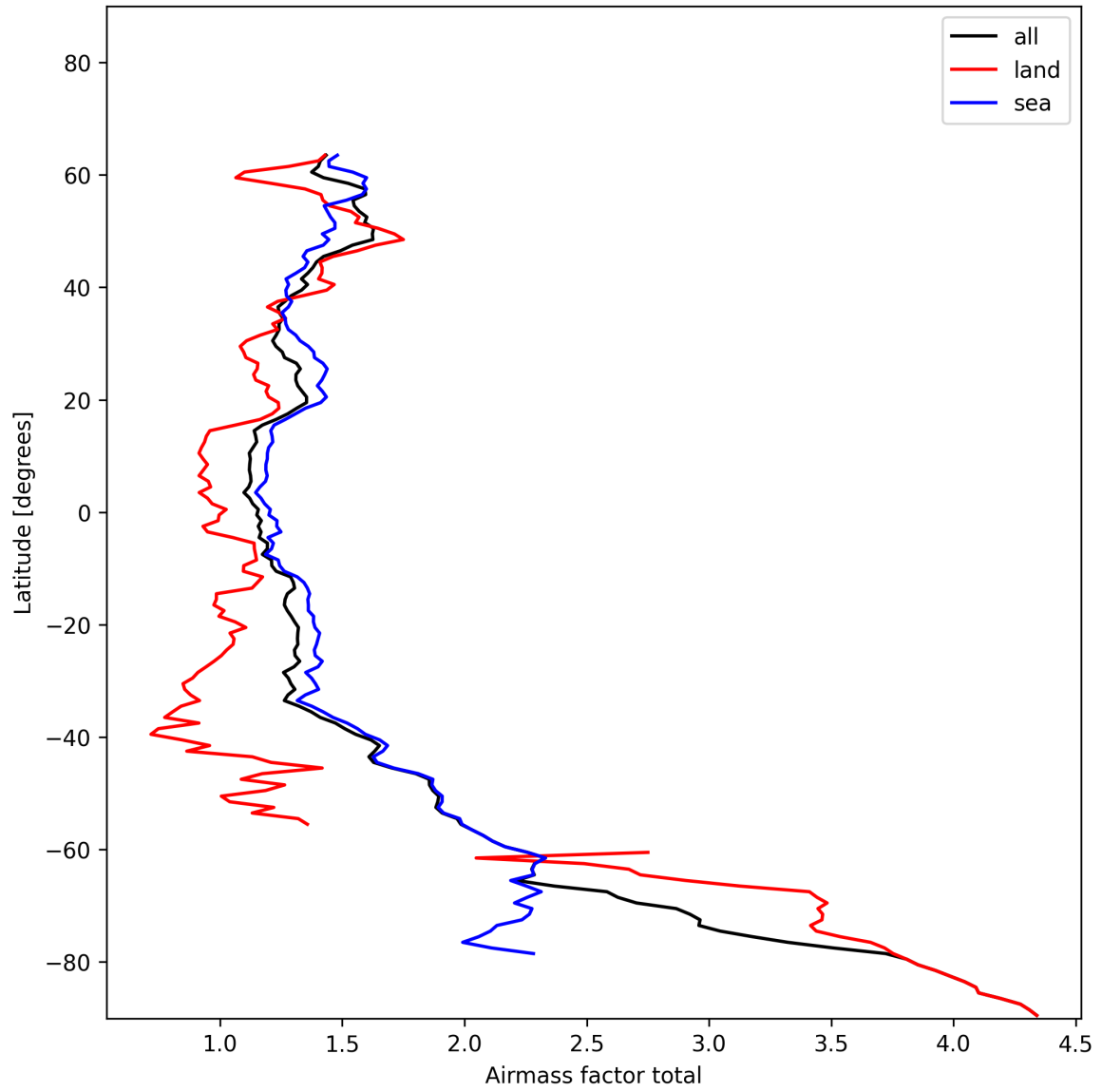
Figure 24: Zonal average of “Airmass factor total” for 2025-01-14 to 2025-01-15.
