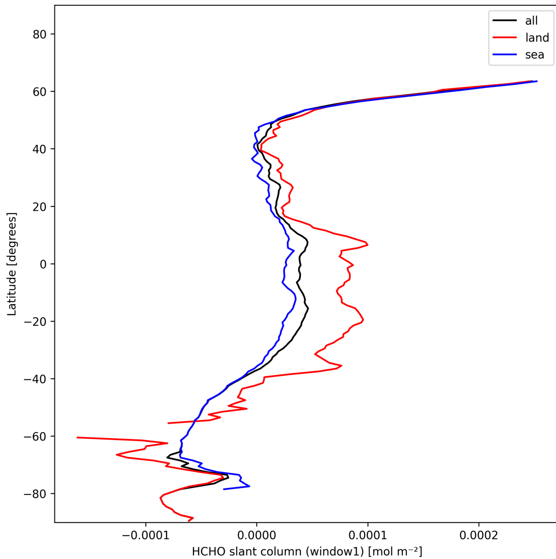
Figure 22: Zonal average of “HCHO slant column (window1)” for 2025-01-14 to 2025-01-15.
