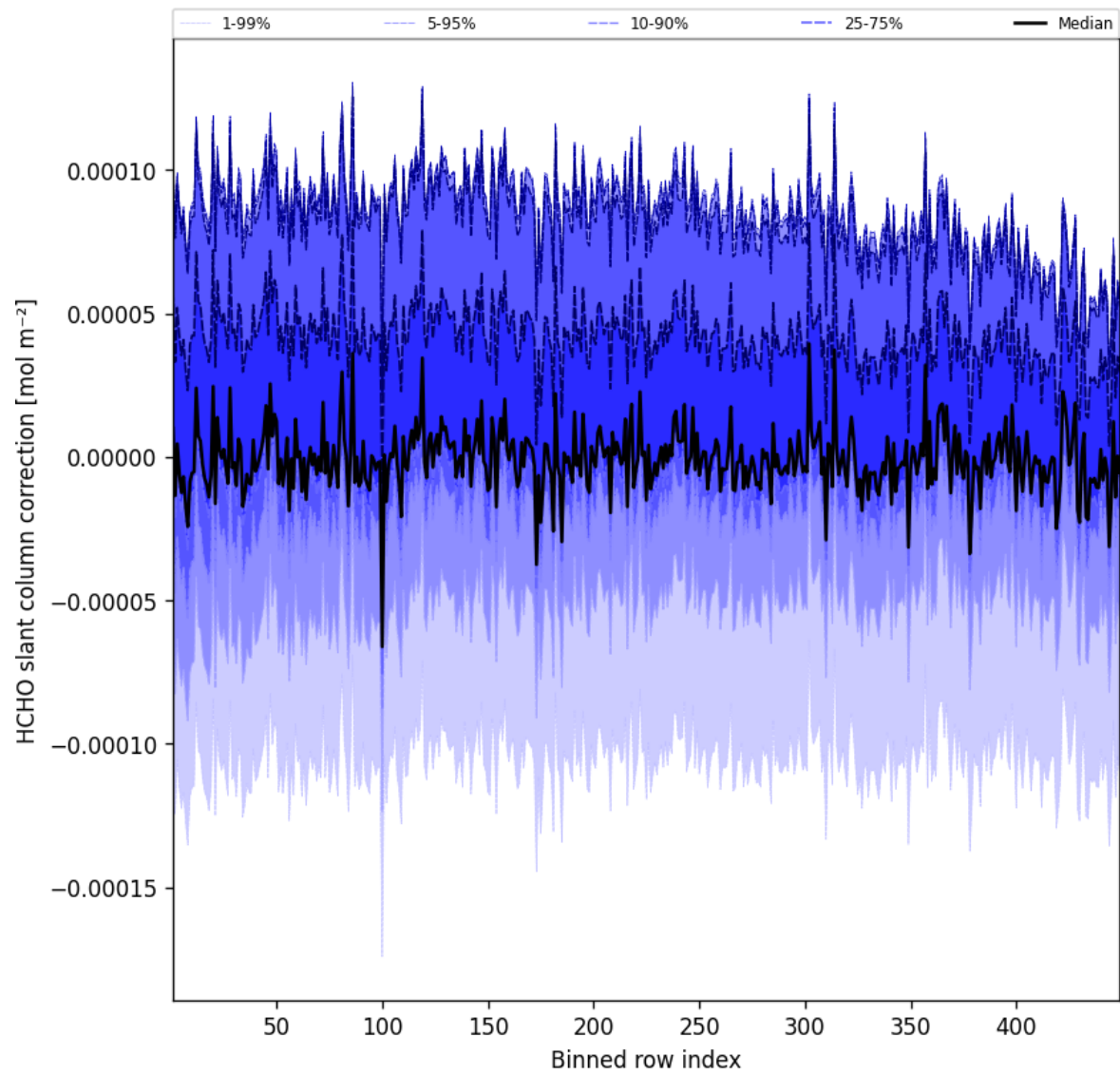
Figure 59: Along track statistics of “HCHO slant column correction” for 2025-01-14 to 2025-01-15
