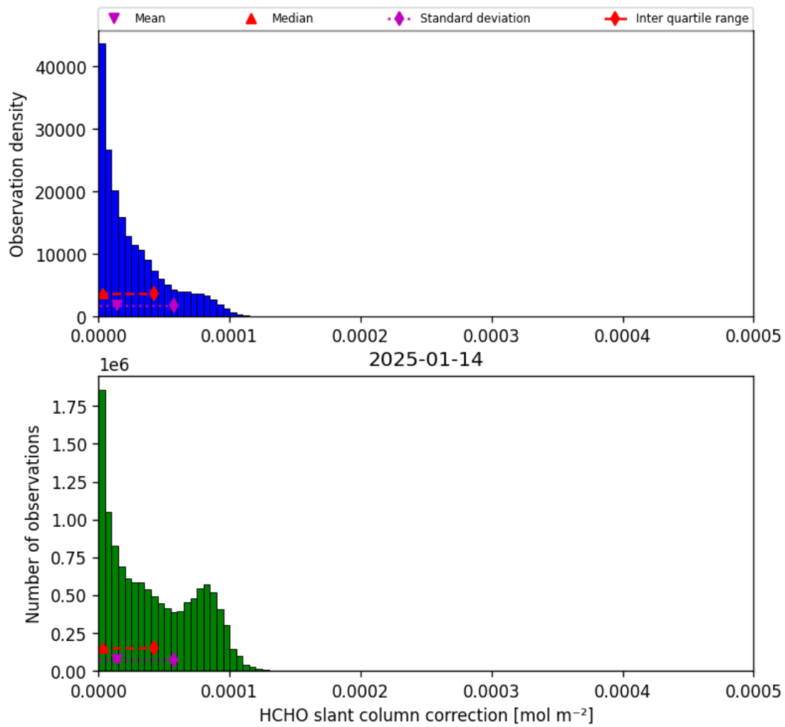
Figure 45: Histogram of “HCHO slant column correction” for 2025-01-14 to 2025-01-15
