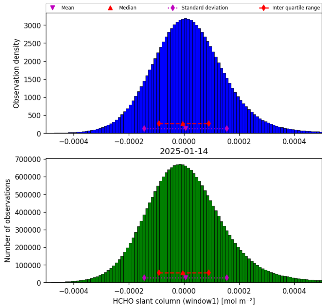
Figure 36: Histogram of “HCHO slant column (window1)” for 2025-01-14 to 2025-01-15
