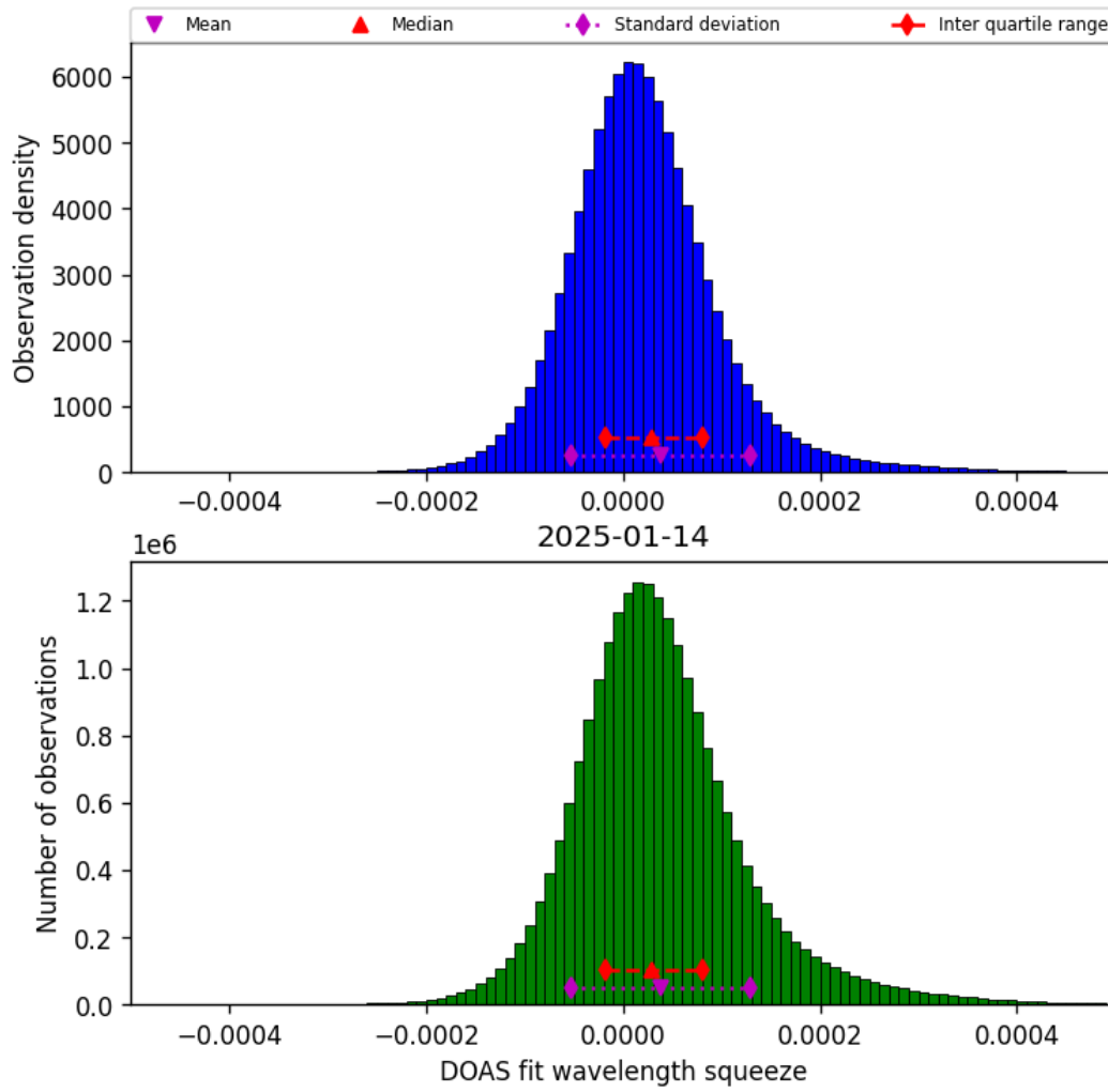
Figure 43: Histogram of “DOAS fit wavelength squeeze” for 2025-01-14 to 2025-01-15
