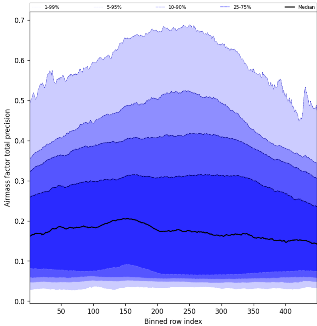
Figure 53: Along track statistics of “Airmass factor total precision” for 2025-01-14 to 2025-01-15
