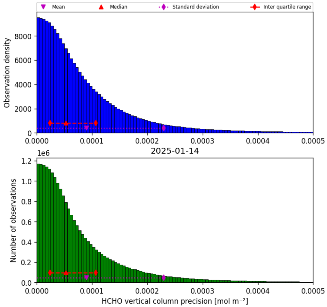
Figure 34: Histogram of “HCHO vertical column precision” for 2025-01-14 to 2025-01-15
