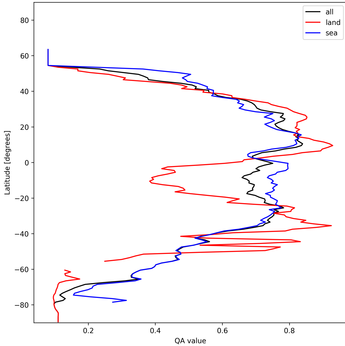
Figure 18: Zonal average of “QA value” for 2025-01-14 to 2025-01-15.
