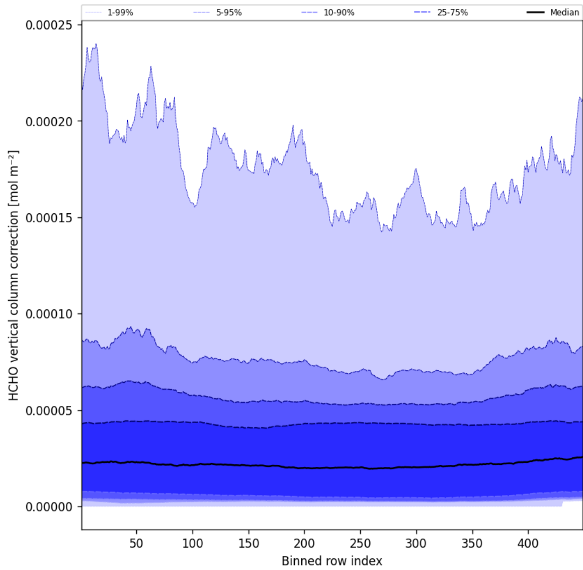
Figure 49: Along track statistics of “HCHO vertical column correction” for 2025-01-14 to 2025-01-15
