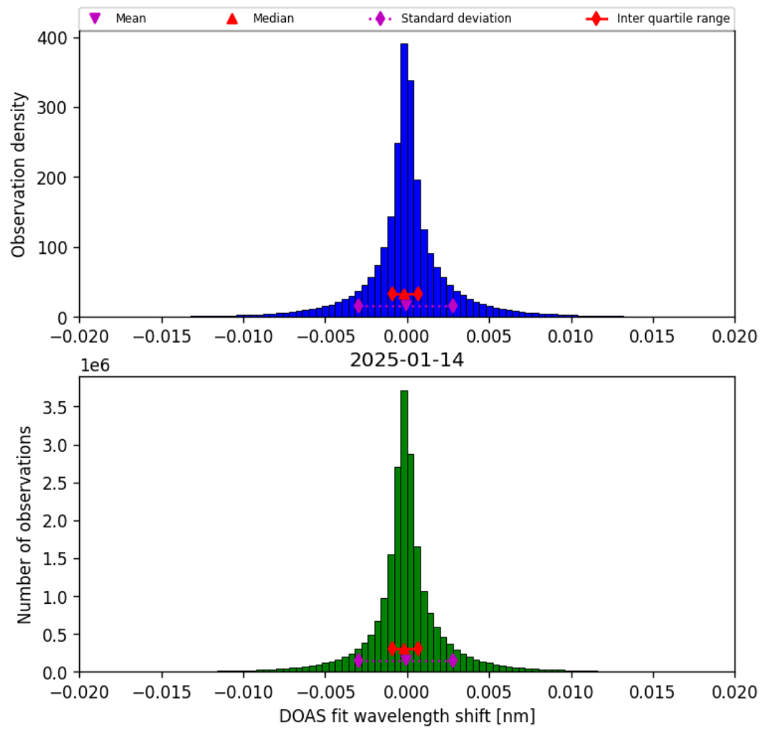
Figure 42: Histogram of “DOAS fit wavelength shift” for 2025-01-14 to 2025-01-15
