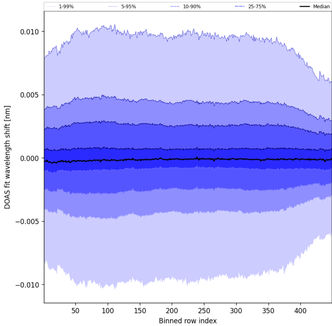
Figure 56: Along track statistics of “DOAS fit wavelength shift” for 2025-01-14 to 2025-01-15
