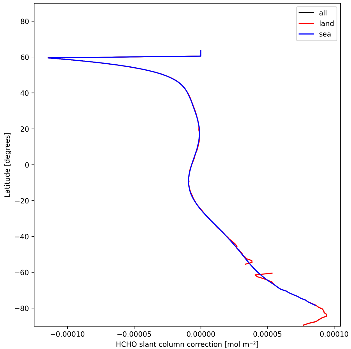
Figure 31: Zonal average of “HCHO slant column correction” for 2025-01-14 to 2025-01-15.
