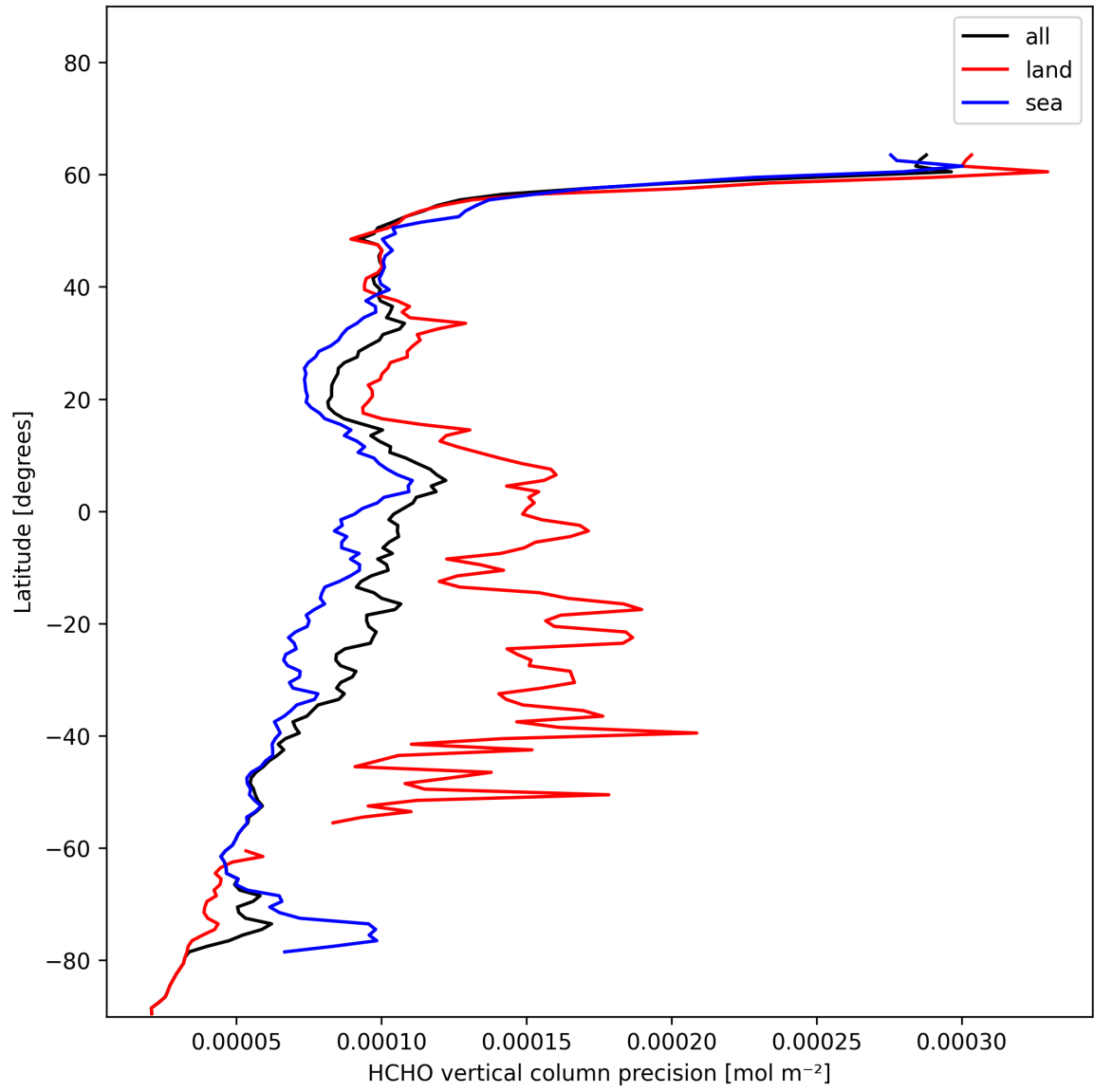
Figure 20: Zonal average of “HCHO vertical column precision” for 2025-01-14 to 2025-01-15.
