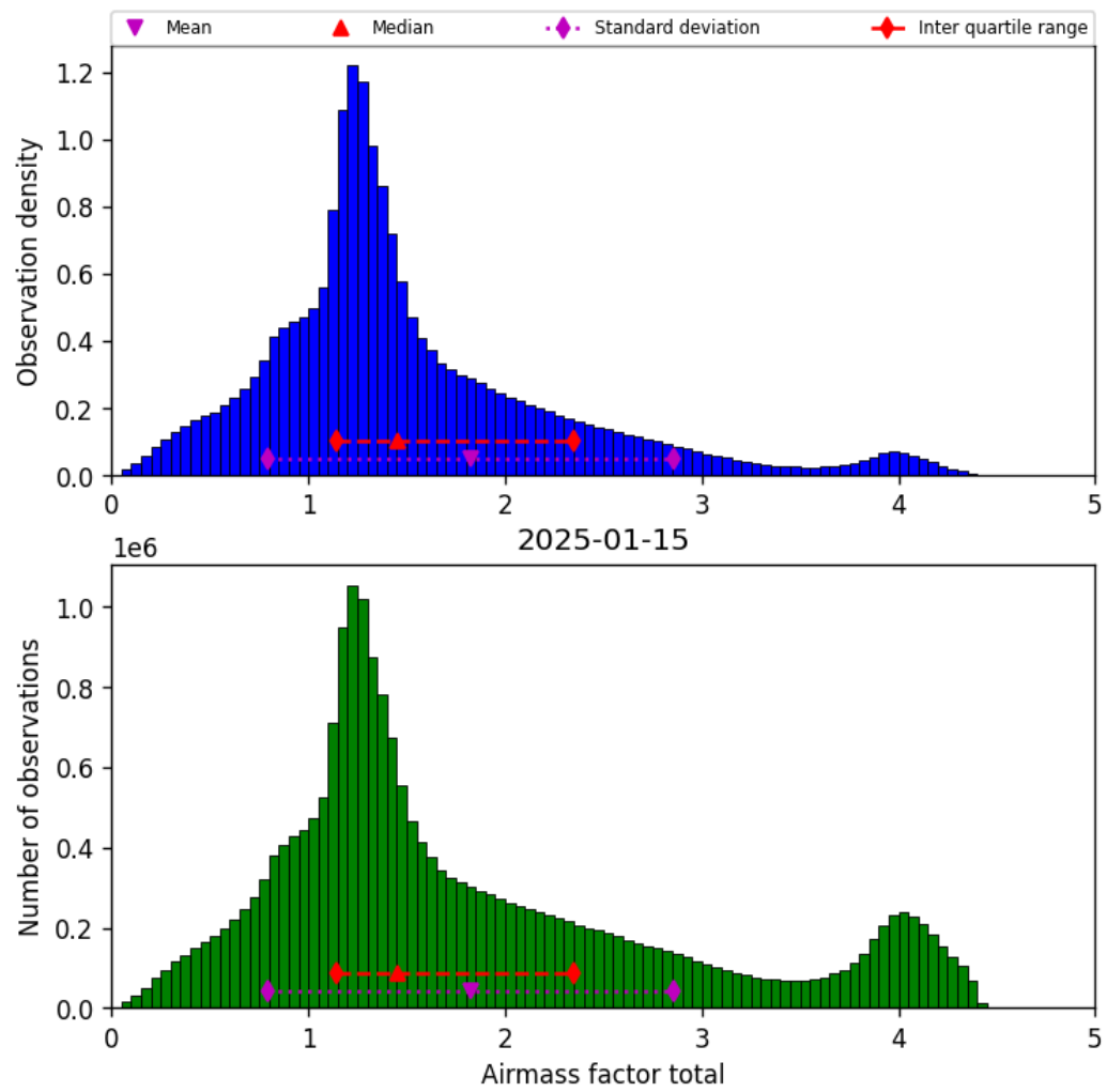
Figure 38: Histogram of “Airmass factor total” for 2025-01-15 to 2025-01-15
