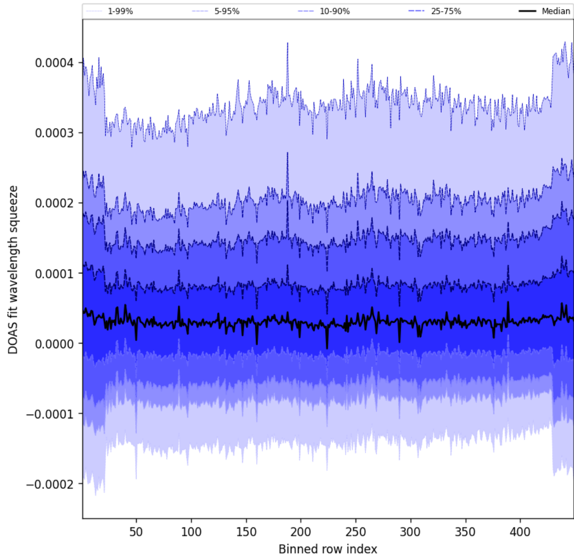
Figure 57: Along track statistics of “DOAS fit wavelength squeeze” for 2025-01-15 to 2025-01-15
