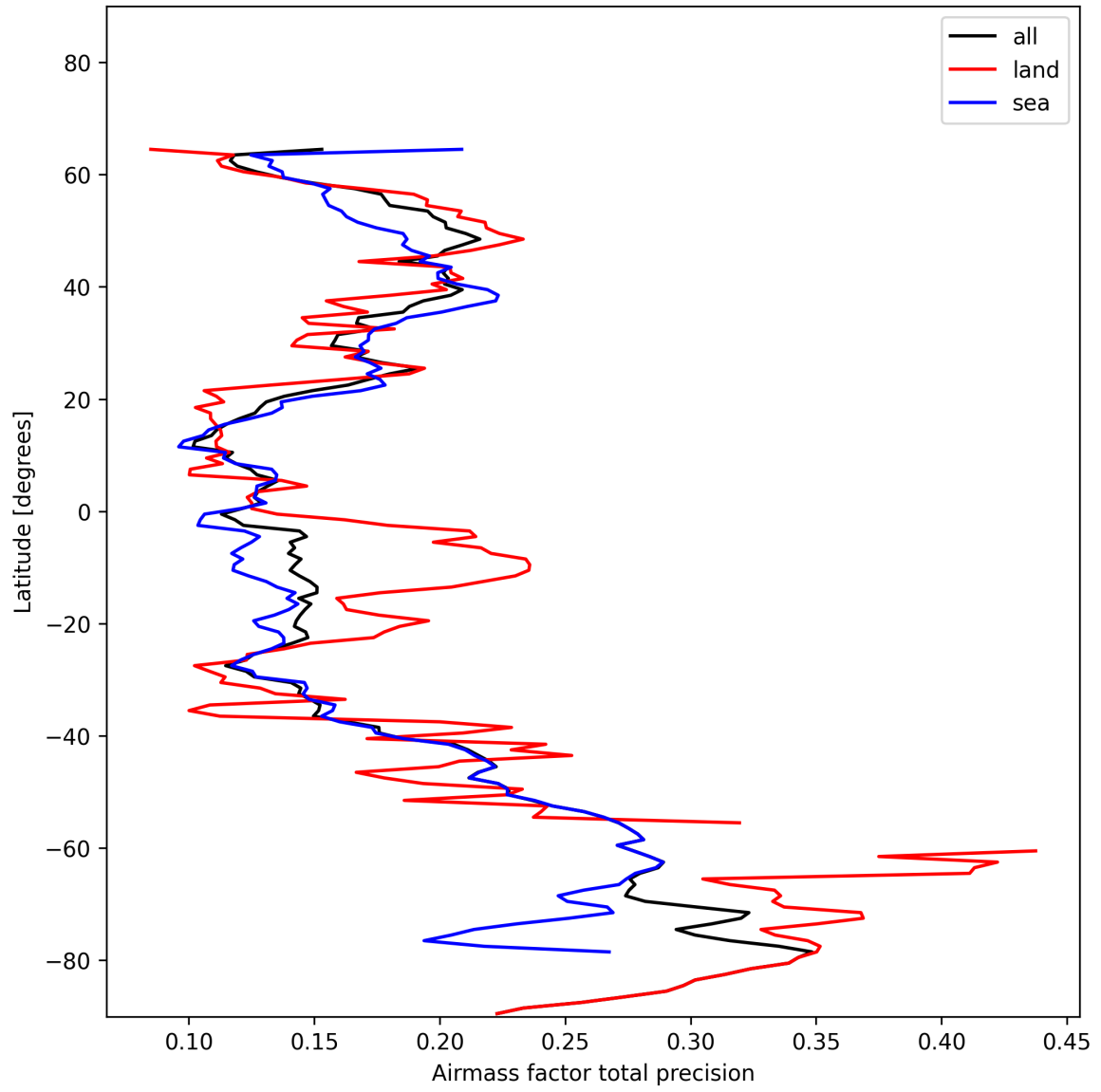
Figure 25: Zonal average of “Airmass factor total precision” for 2025-01-15 to 2025-01-15.
