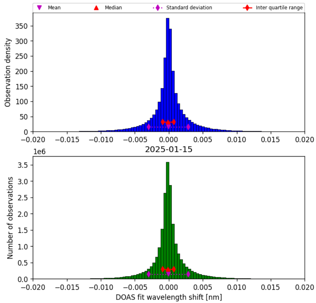
Figure 42: Histogram of “DOAS fit wavelength shift” for 2025-01-15 to 2025-01-15
