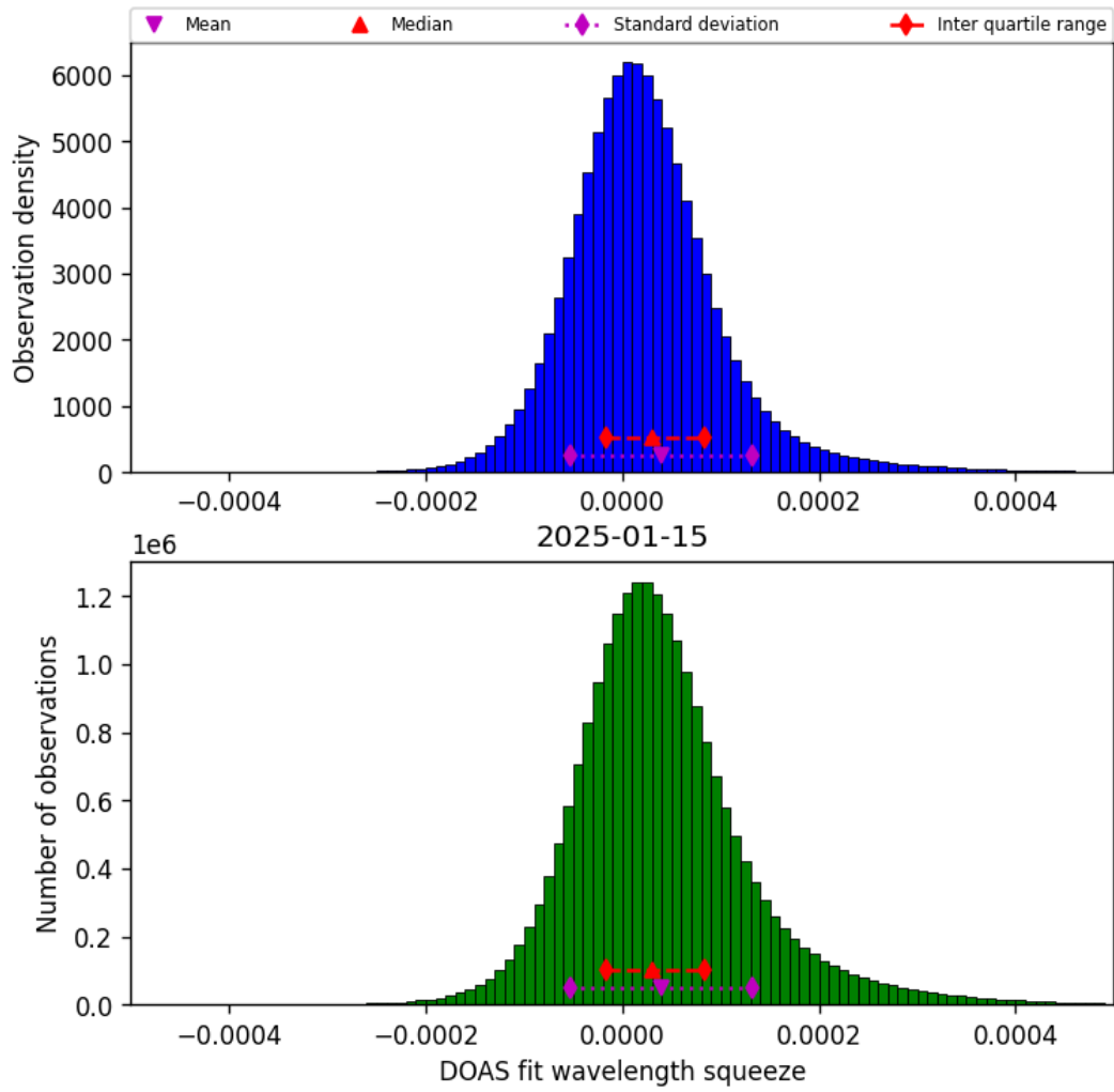
Figure 43: Histogram of “DOAS fit wavelength squeeze” for 2025-01-15 to 2025-01-15
