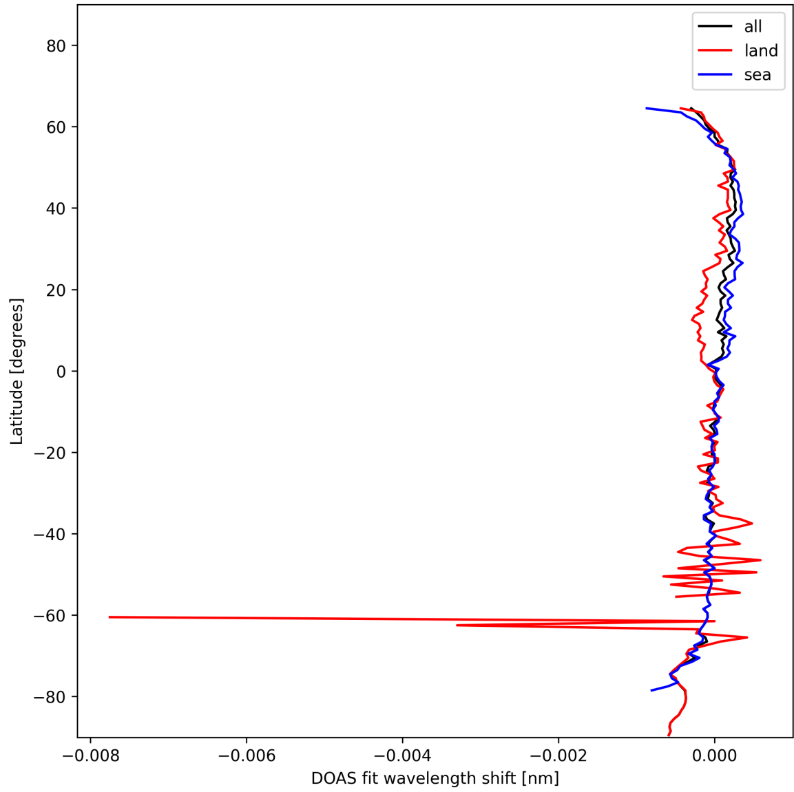
Figure 28: Zonal average of "DOAS fit wavelength shift" for 2025-01-15 to 2025-01-15.
