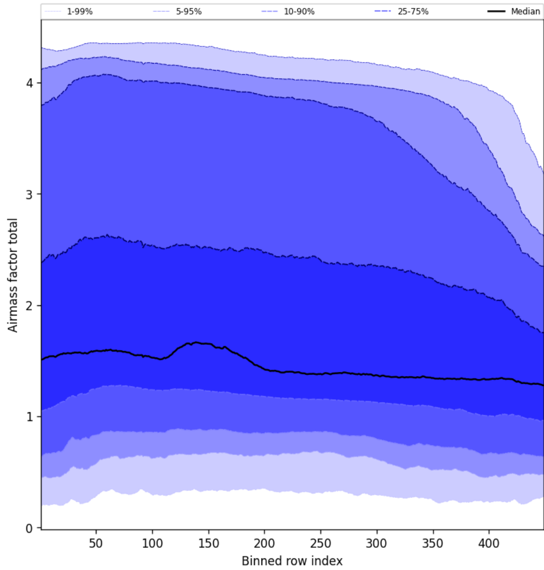
Figure 52: Along track statistics of “Airmass factor total” for 2025-01-15 to 2025-01-15
