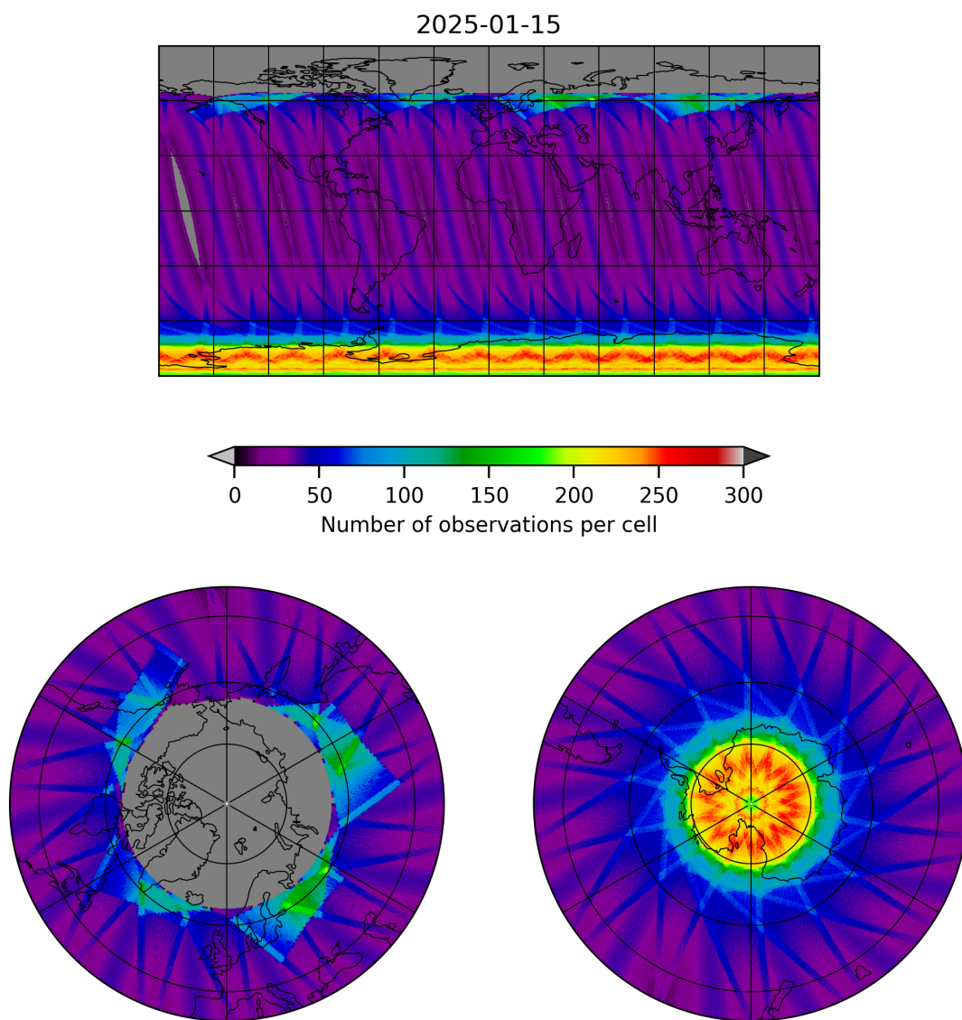
Figure 17: Map of the number of observations for 2025-01-15 to 2025-01-15
