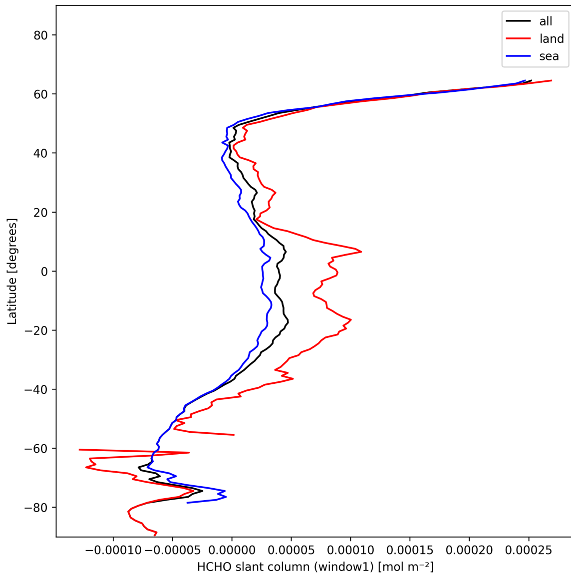
Figure 22: Zonal average of “HCHO slant column (window1)” for 2025-01-15 to 2025-01-15.
