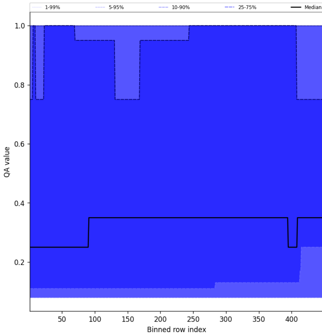
Figure 46: Along track statistics of “QA value” for 2025-01-15 to 2025-01-15
