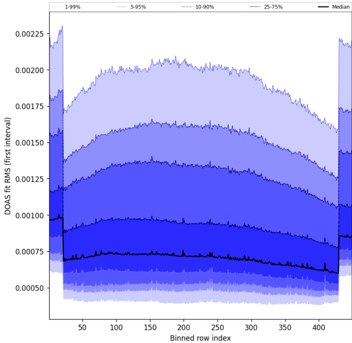
Figure 58: Along track statistics of “DOAS fit RMS (first interval)” for 2025-01-15 to 2025-01-15
