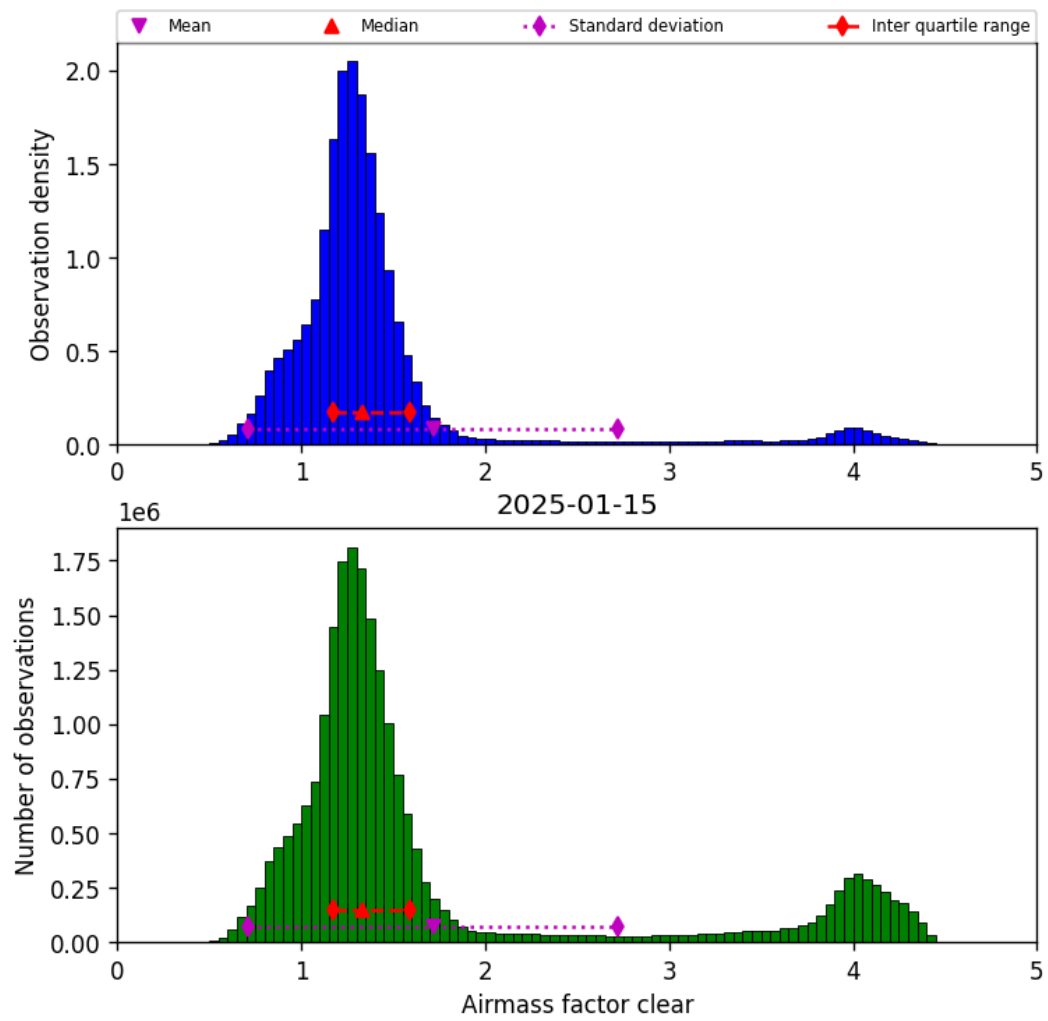
Figure 40: Histogram of “Airmass factor clear” for 2025-01-15 to 2025-01-15
