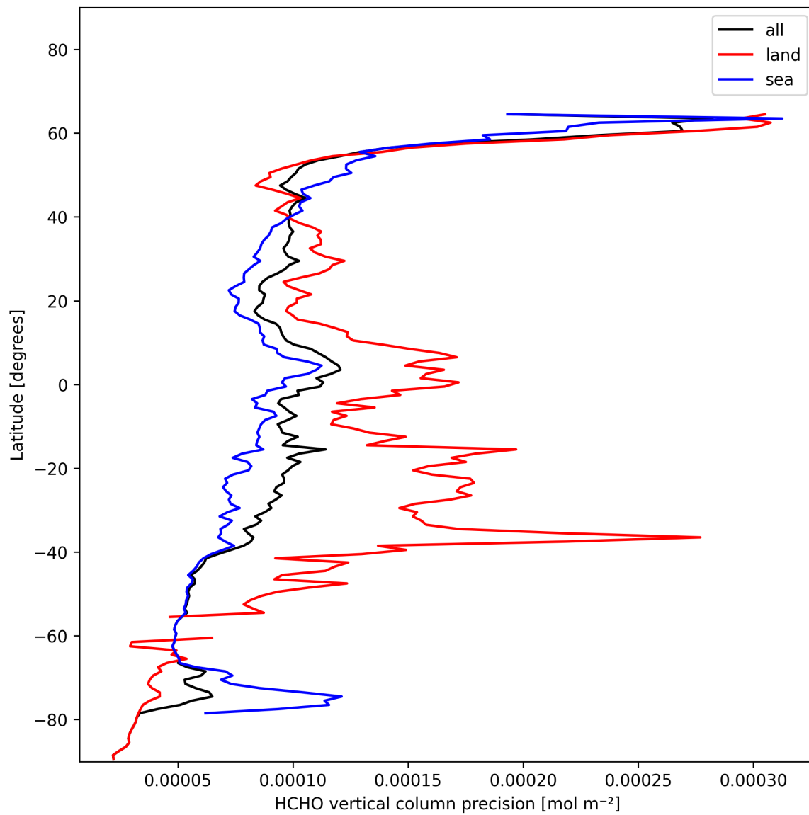
Figure 20: Zonal average of “HCHO vertical column precision” for 2025-01-15 to 2025-01-15.
