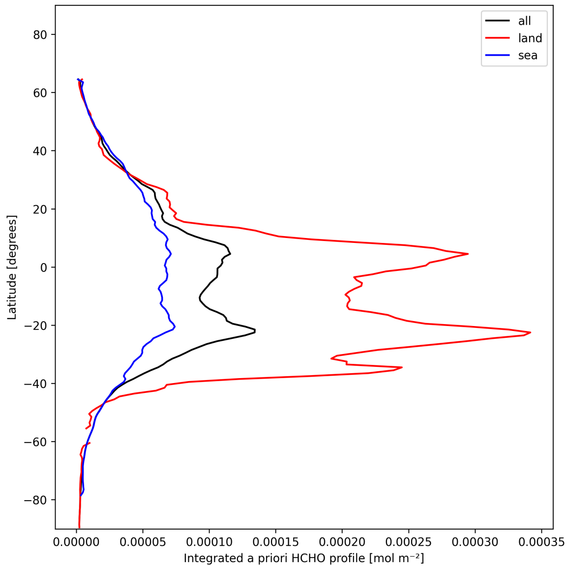
Figure 27: Zonal average of “Integrated a priori HCHO profile” for 2025-01-15 to 2025-01-15.
