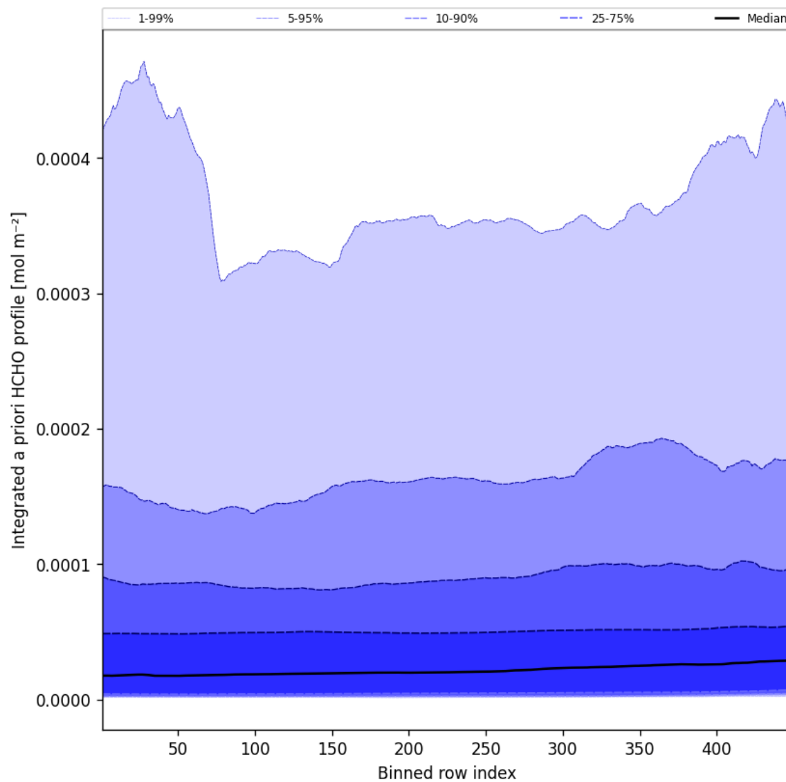
Figure 55: Along track statistics of “Integrated a priori HCHO profile” for 2025-01-15 to 2025-01-15
