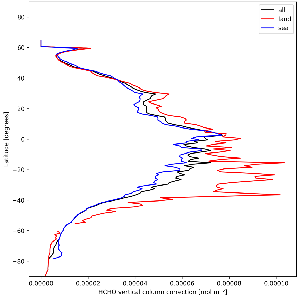
Figure 21: Zonal average of “HCHO vertical column correction” for 2025-01-15 to 2025-01-15.
