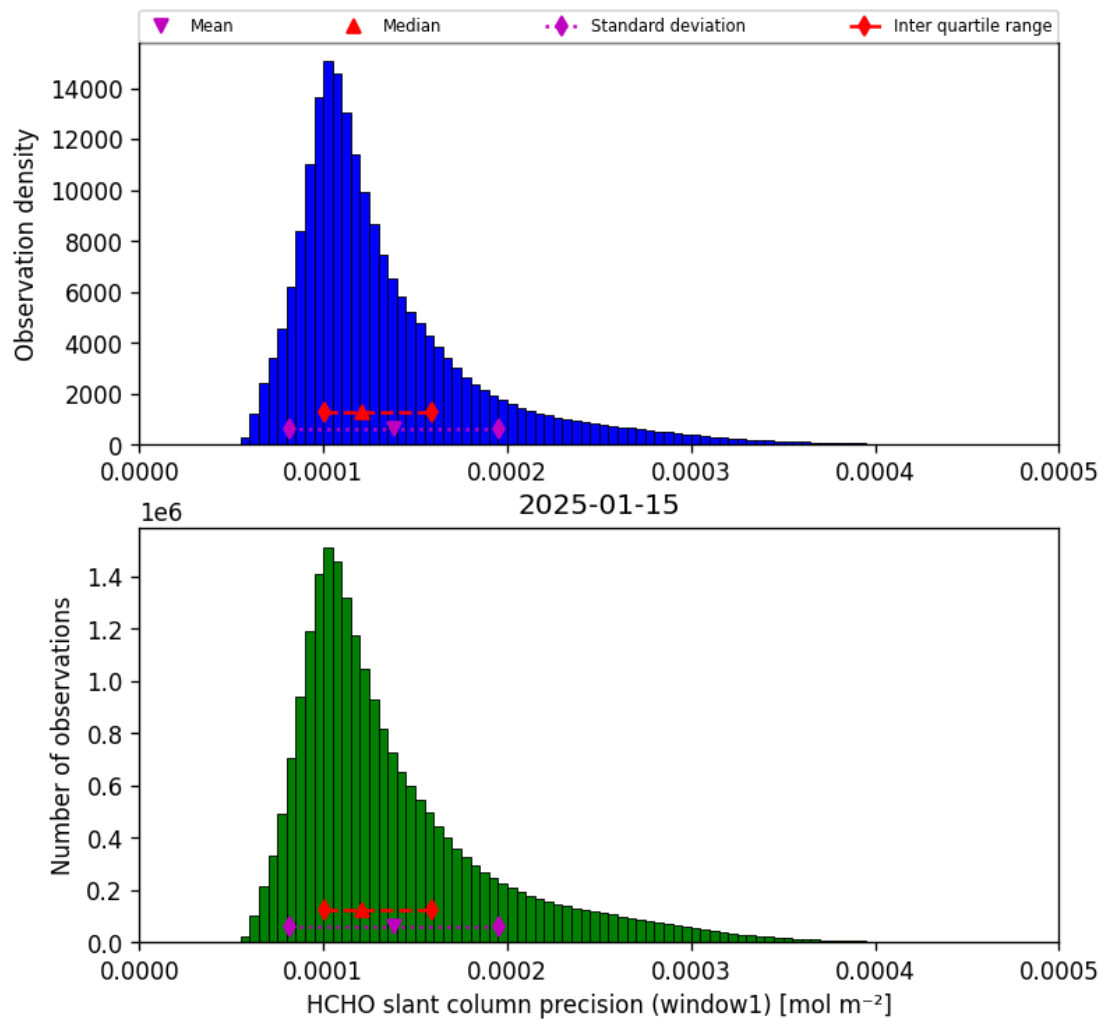
Figure 37: Histogram of “HCHO slant column precision (window1)” for 2025-01-15 to 2025-01-15
