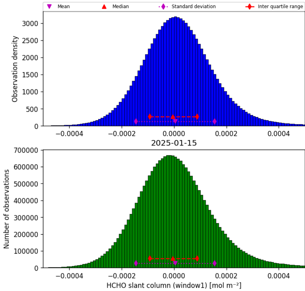
Figure 36: Histogram of “HCHO slant column (window1)” for 2025-01-15 to 2025-01-15
