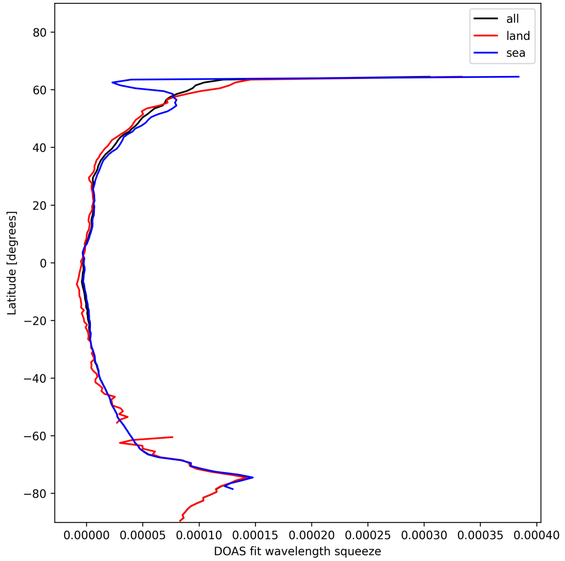
Figure 29: Zonal average of “DOAS fit wavelength squeeze” for 2025-01-15 to 2025-01-15.
