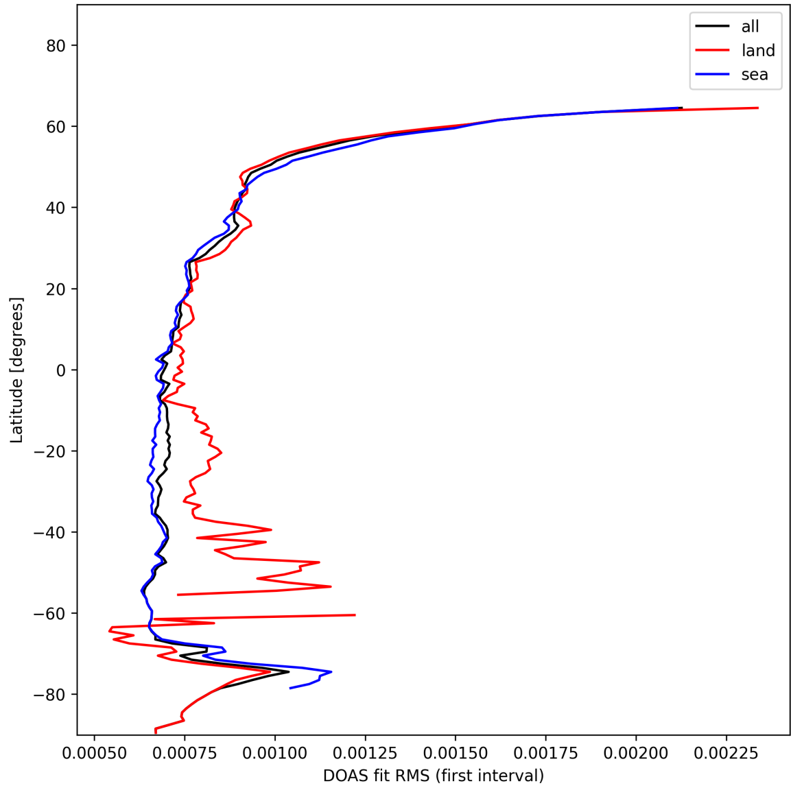
Figure 30: Zonal average of “DOAS fit RMS (first interval)” for 2025-01-15 to 2025-01-15.
