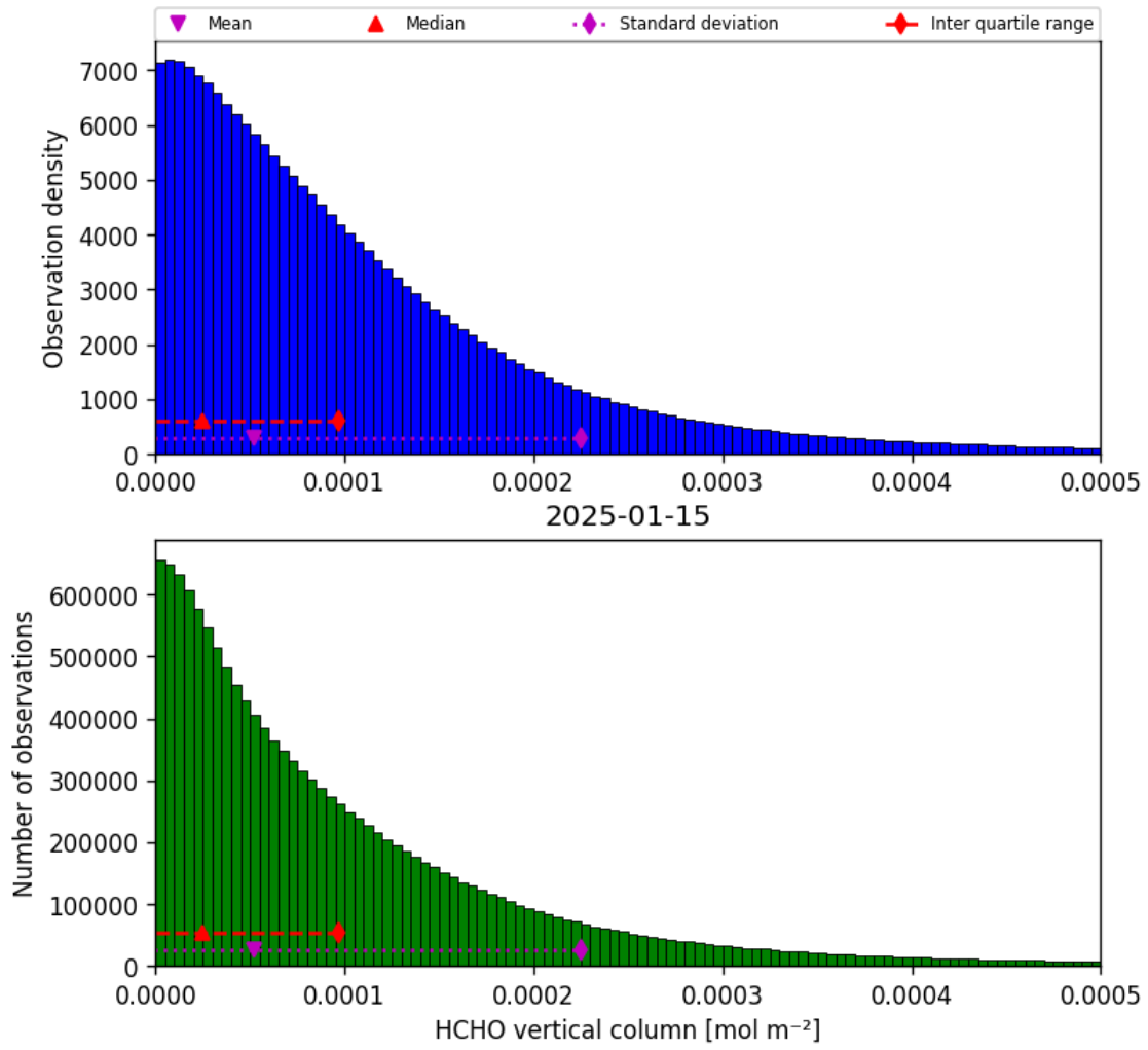
Figure 33: Histogram of “HCHO vertical column” for 2025-01-15 to 2025-01-15
