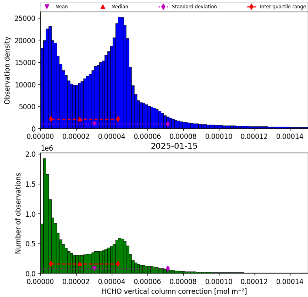
Figure 35: Histogram of “HCHO vertical column correction” for 2025-01-15 to 2025-01-15
