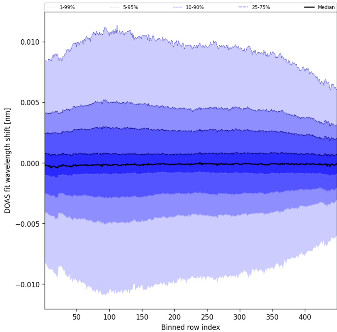
Figure 56: Along track statistics of “DOAS fit wavelength shift” for 2025-01-15 to 2025-01-15
