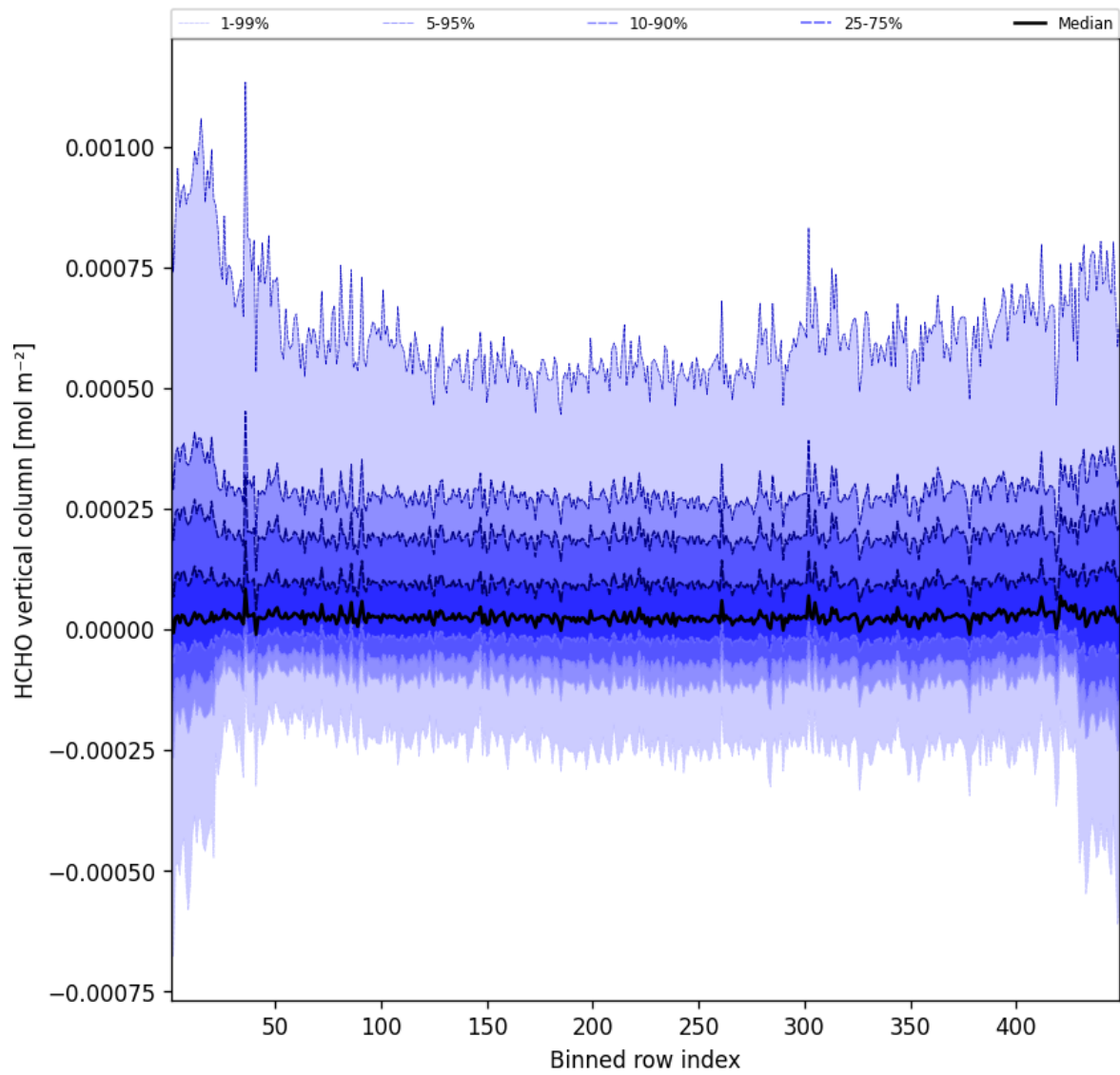
Figure 47: Along track statistics of “HCHO vertical column” for 2025-01-15 to 2025-01-15
