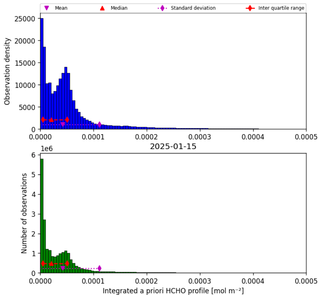
Figure 41: Histogram of “Integrated a priori HCHO profile” for 2025-01-15 to 2025-01-15
