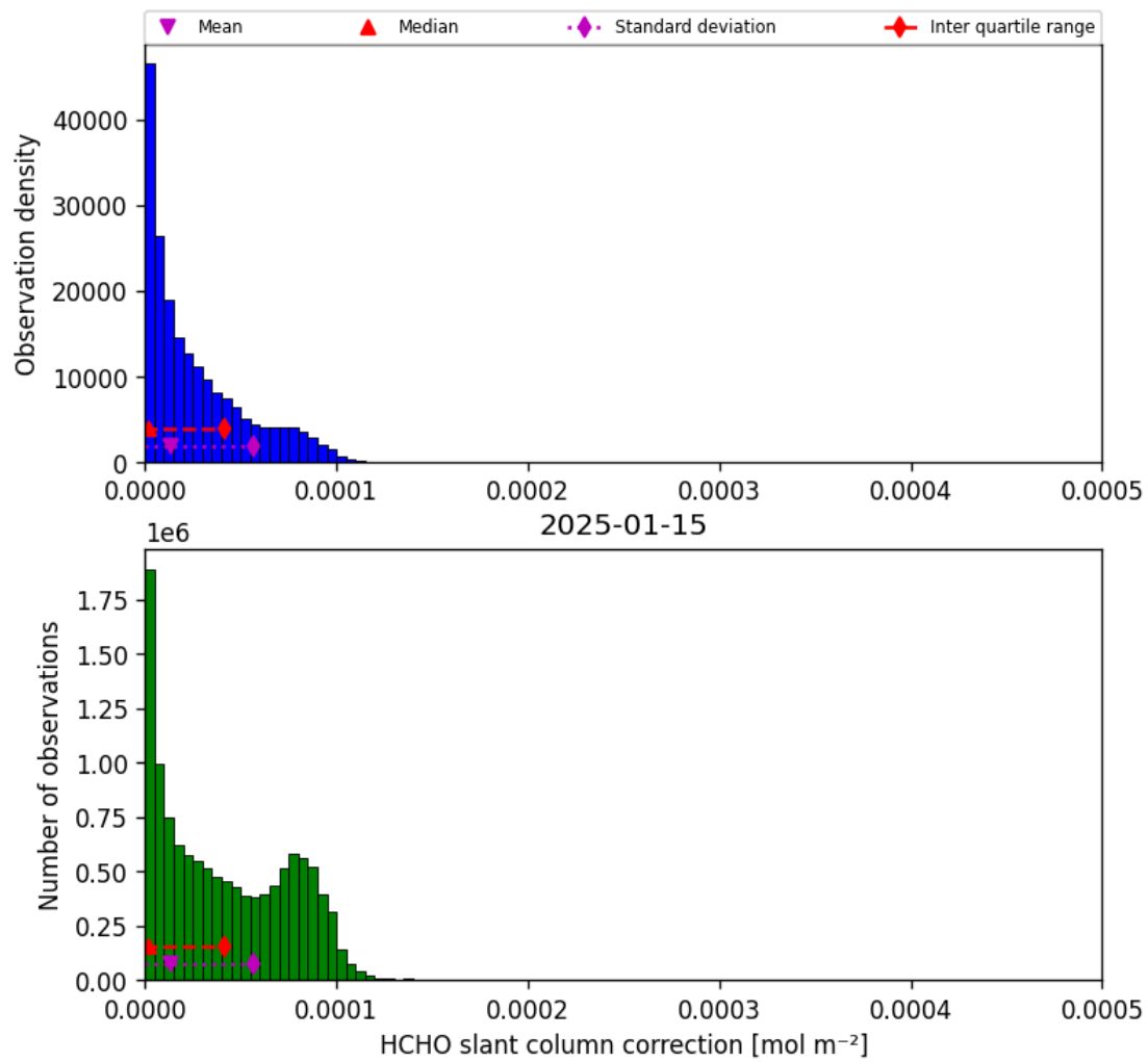
Figure 45: Histogram of “HCHO slant column correction” for 2025-01-15 to 2025-01-15
