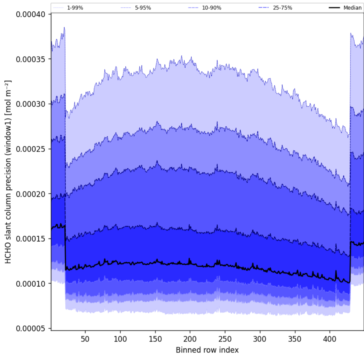
Figure 51: Along track statistics of “HCHO slant column precision (window1)” for 2025-01-15 to 2025-01-15
