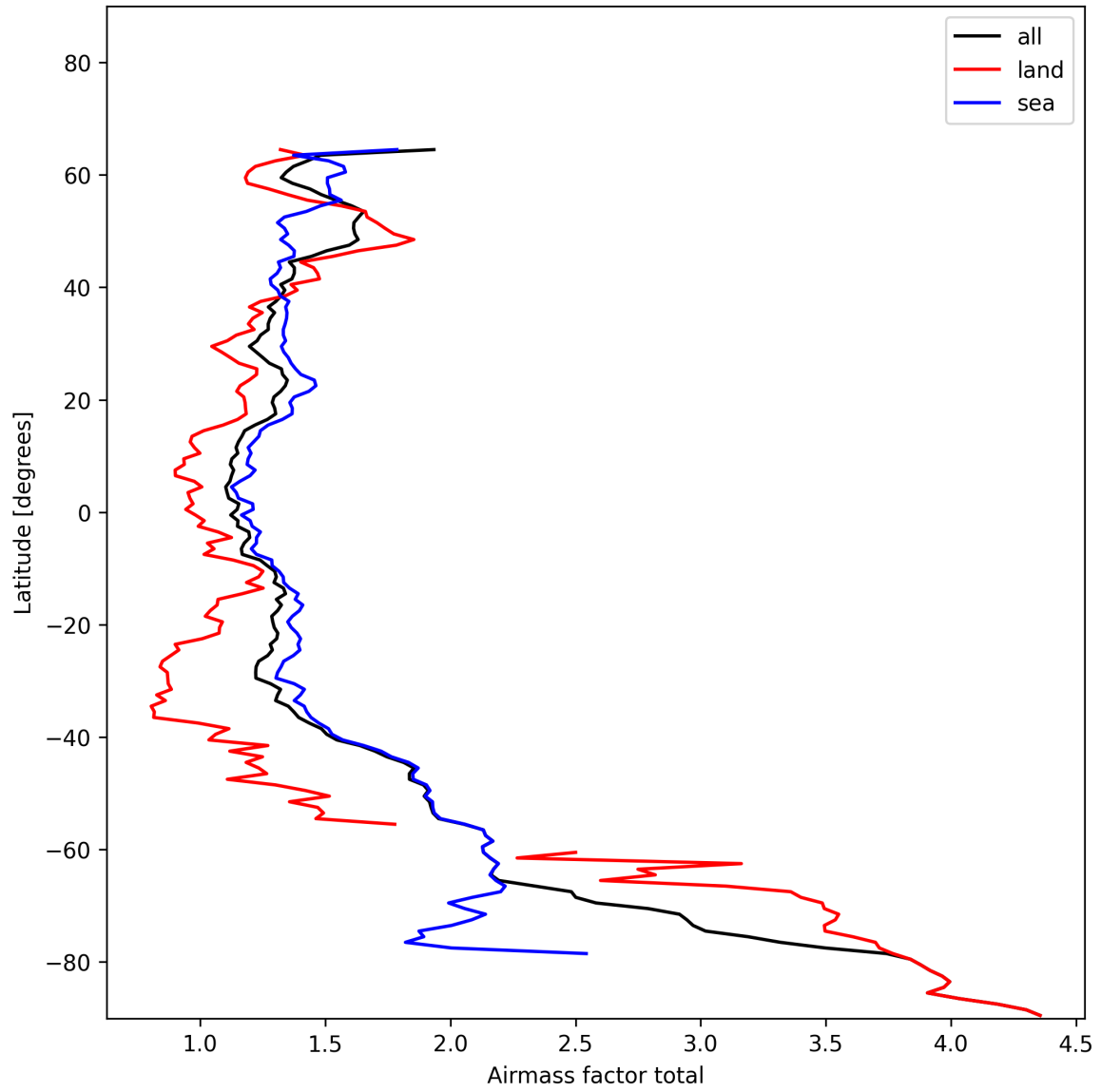
Figure 24: Zonal average of “Airmass factor total” for 2025-01-15 to 2025-01-15.
