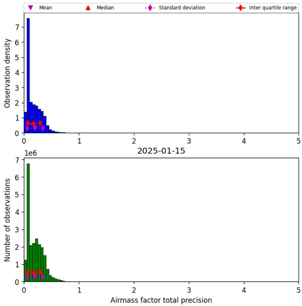
Figure 39: Histogram of “Airmass factor total precision” for 2025-01-15 to 2025-01-15
