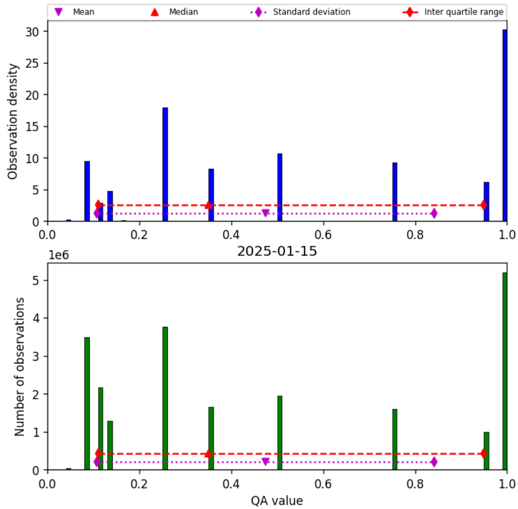
Figure 32: Histogram of “QA value” for 2025-01-15 to 2025-01-15
