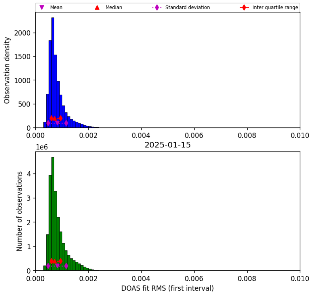
Figure 44: Histogram of “DOAS fit RMS (first interval)” for 2025-01-15 to 2025-01-15
