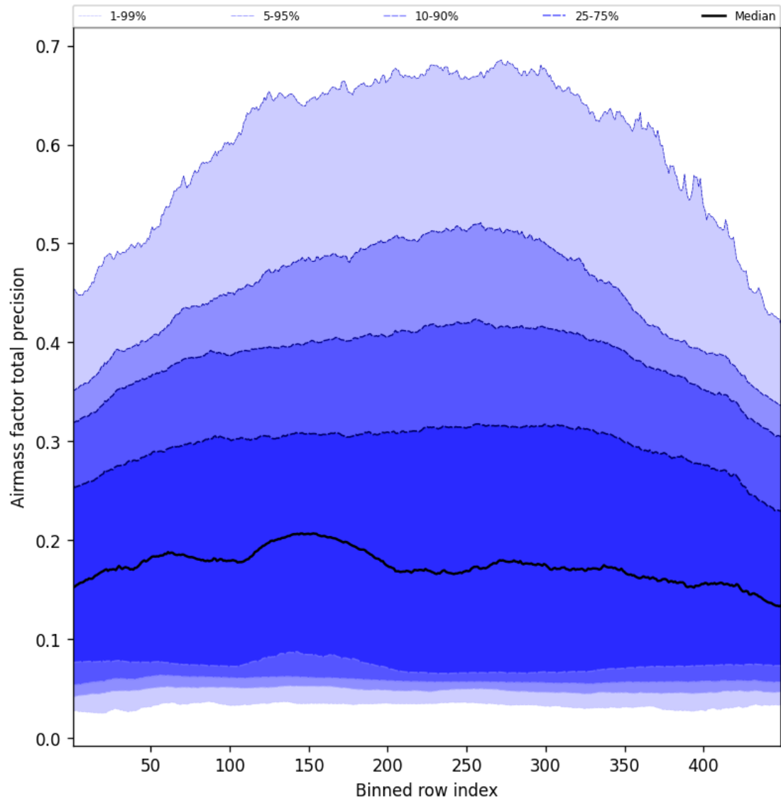
Figure 53: Along track statistics of “Airmass factor total precision” for 2025-01-15 to 2025-01-15
