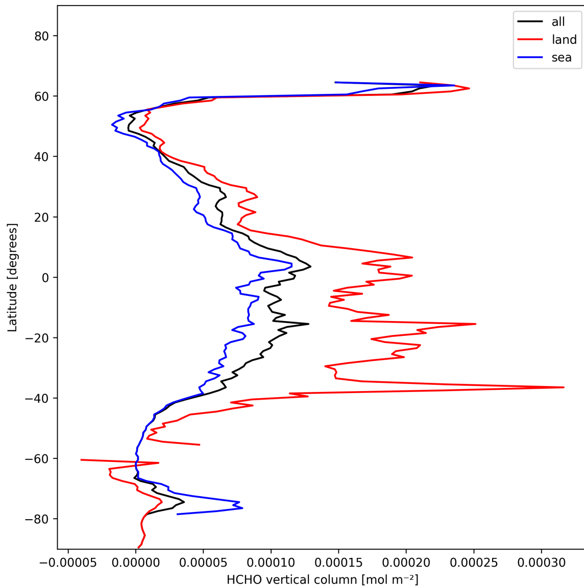
Figure 19: Zonal average of “HCHO vertical column” for 2025-01-15 to 2025-01-15.
