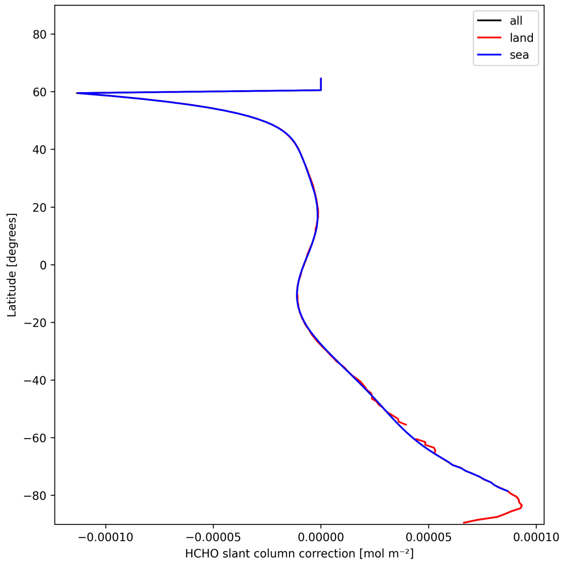
Figure 31: Zonal average of “HCHO slant column correction” for 2025-01-15 to 2025-01-15.
