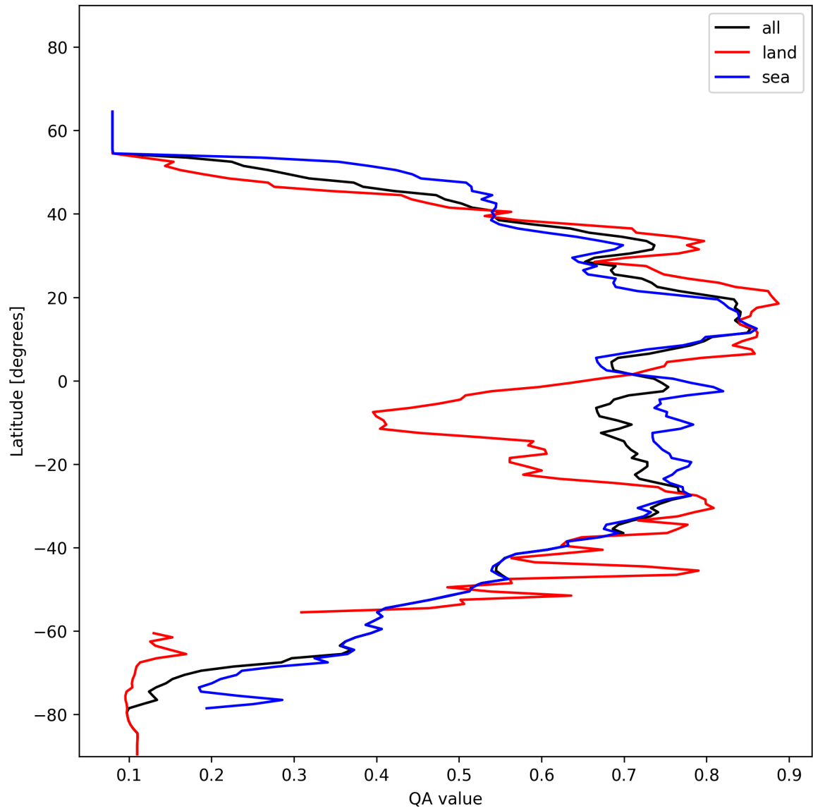
Figure 18: Zonal average of “QA value” for 2025-01-15 to 2025-01-15.
