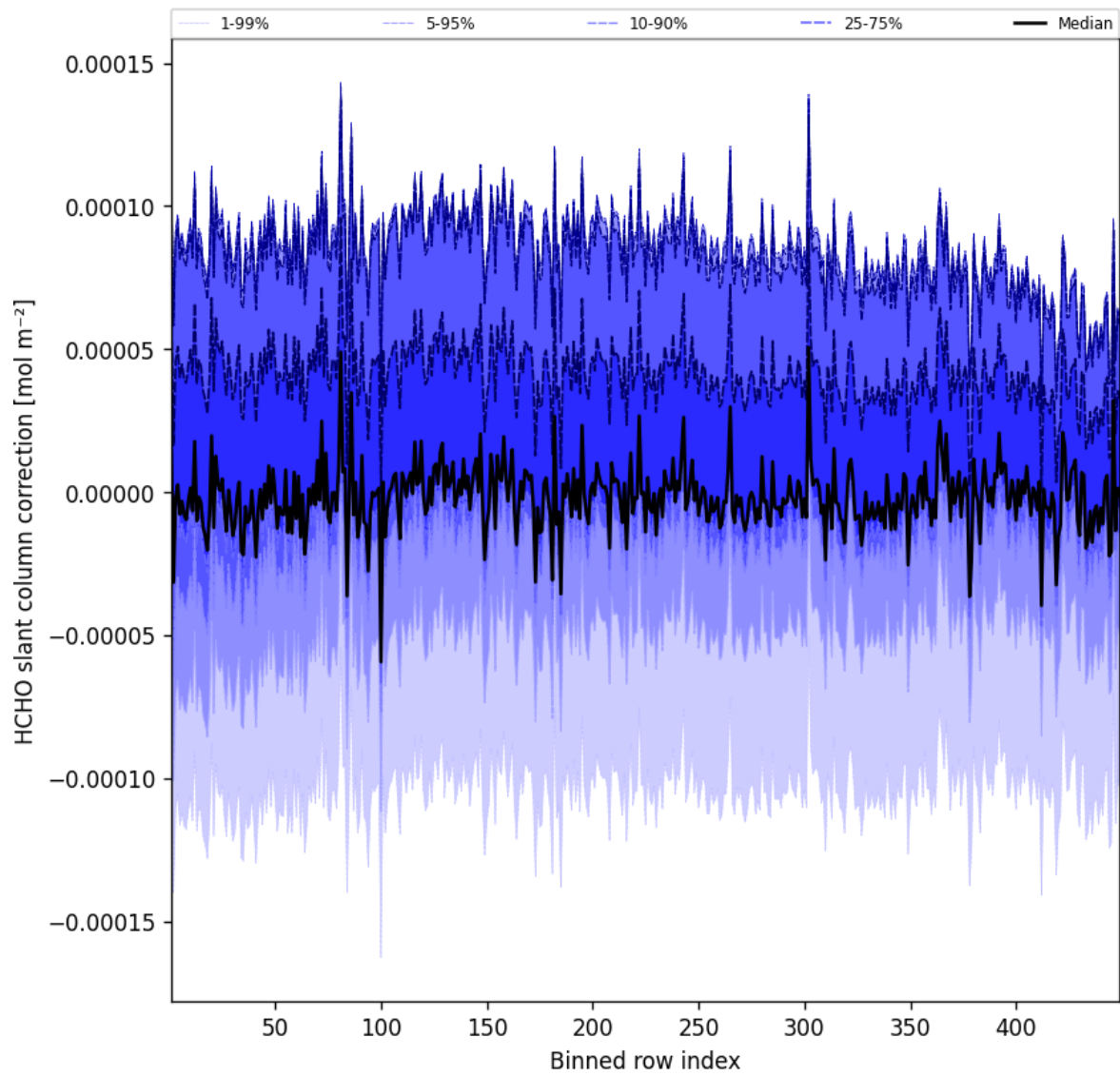
Figure 59: Along track statistics of “HCHO slant column correction” for 2025-01-15 to 2025-01-15
