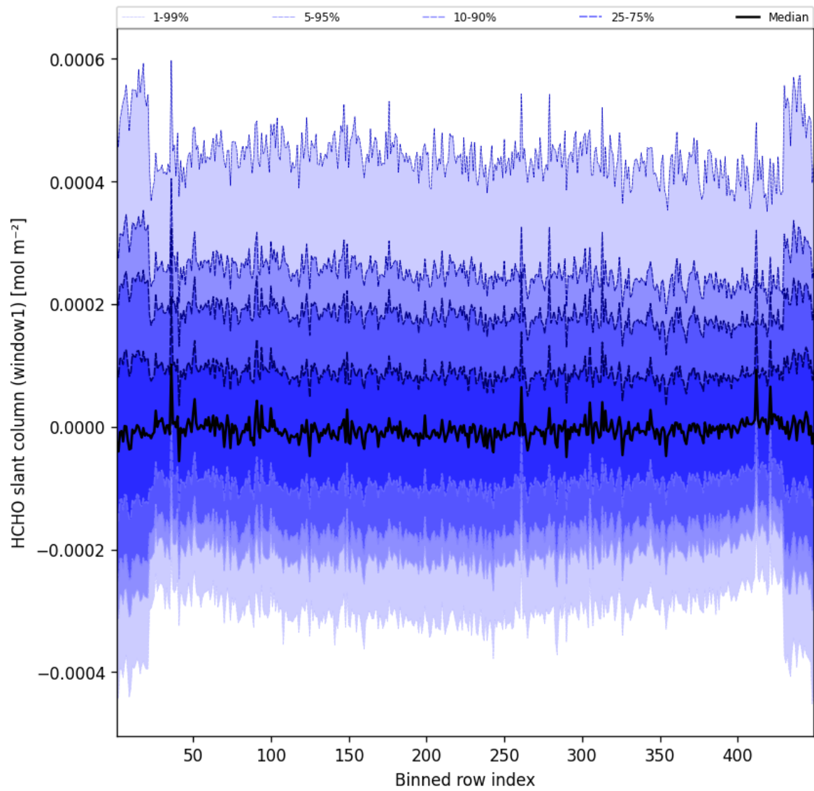
Figure 50: Along track statistics of “HCHO slant column (window1)” for 2025-01-15 to 2025-01-15
