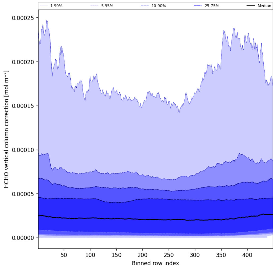
Figure 49: Along track statistics of “HCHO vertical column correction” for 2025-01-15 to 2025-01-15
