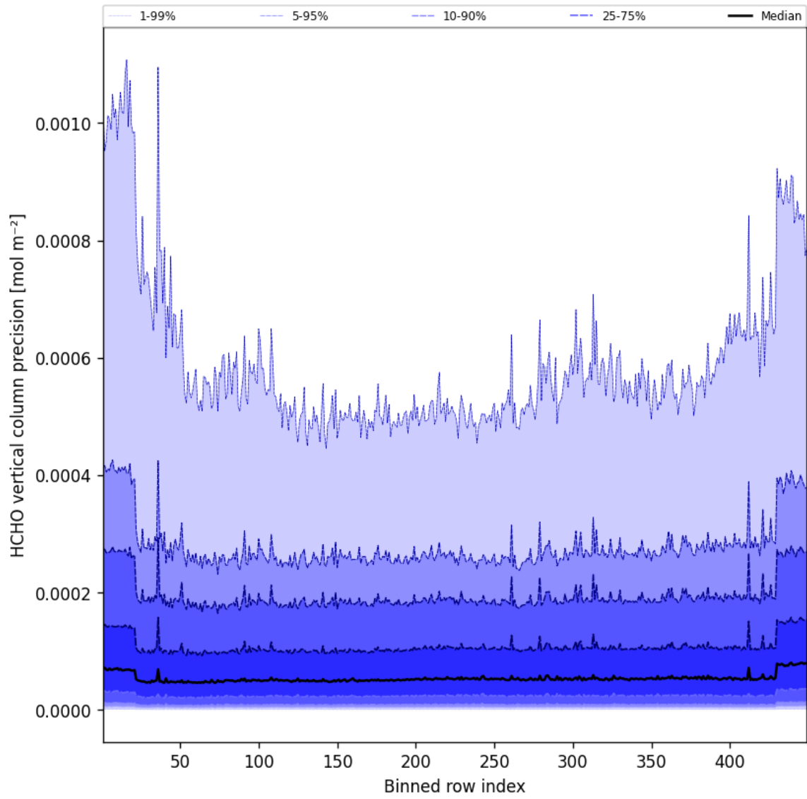
Figure 48: Along track statistics of “HCHO vertical column precision” for 2025-01-15 to 2025-01-15
