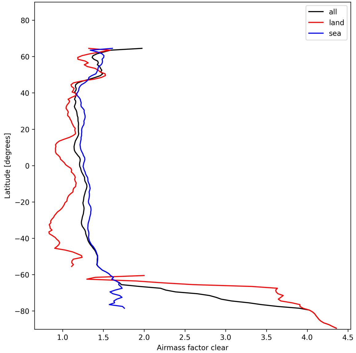
Figure 26: Zonal average of “Airmass factor clear” for 2025-01-15 to 2025-01-15.
