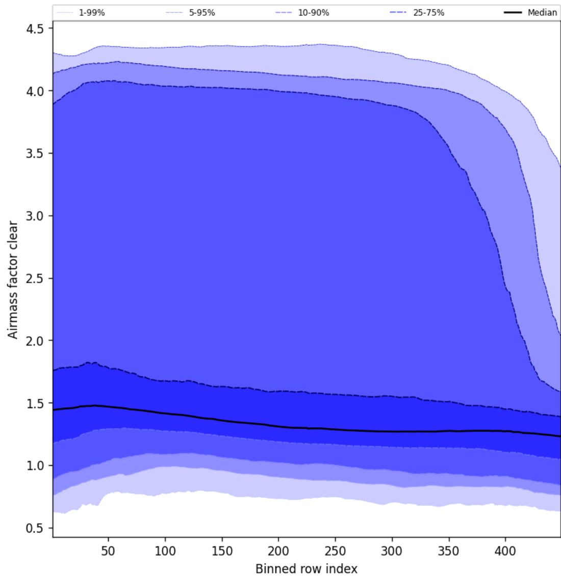
Figure 54: Along track statistics of “Airmass factor clear” for 2025-01-15 to 2025-01-15
