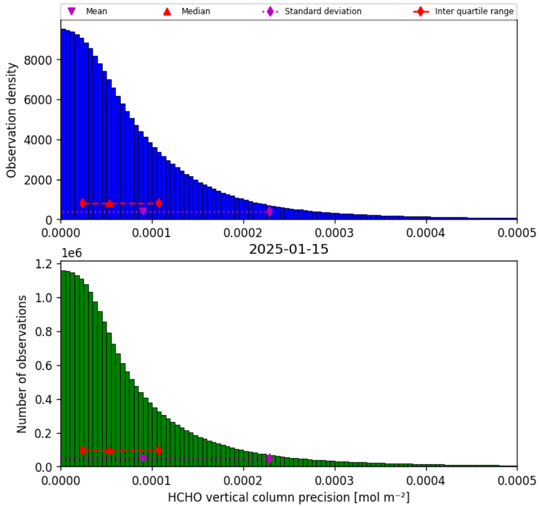
Figure 34: Histogram of “HCHO vertical column precision” for 2025-01-15 to 2025-01-15
