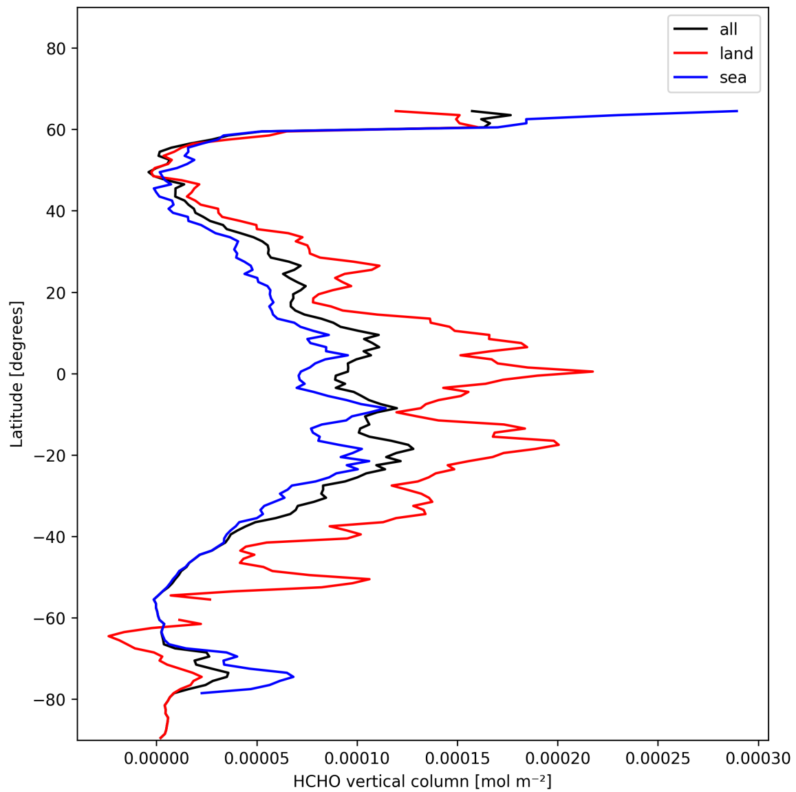
Figure 19: Zonal average of “HCHO vertical column” for 2025-01-16 to 2025-01-17.
