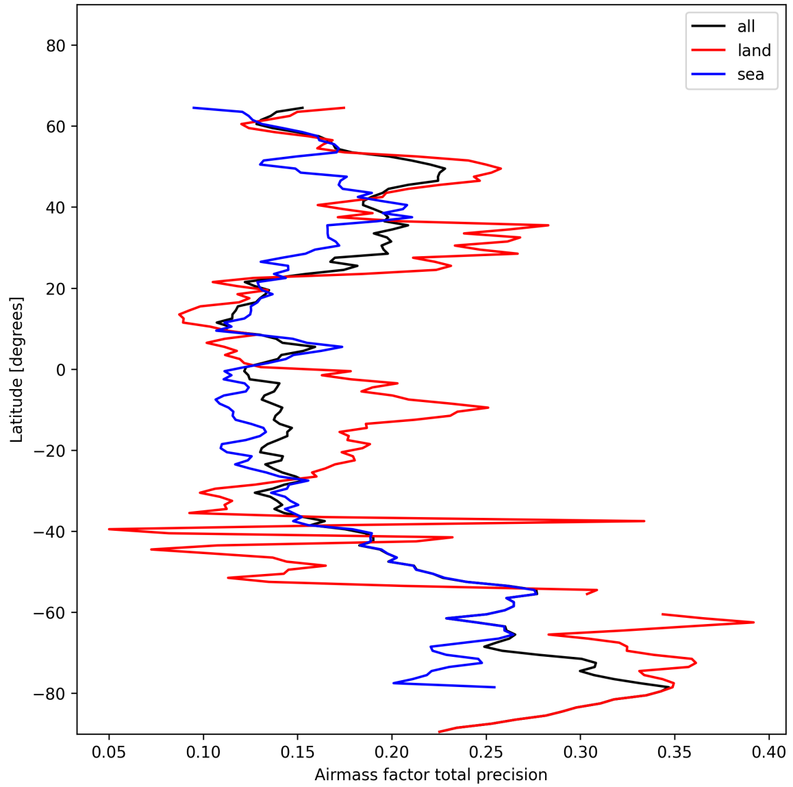
Figure 25: Zonal average of “Airmass factor total precision” for 2025-01-16 to 2025-01-17.
