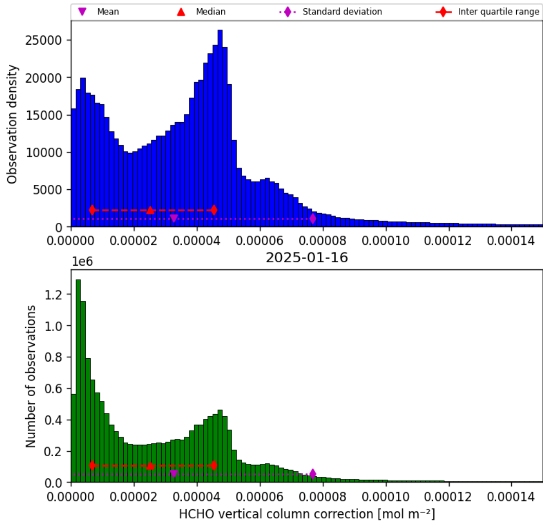
Figure 35: Histogram of “HCHO vertical column correction” for 2025-01-16 to 2025-01-17
