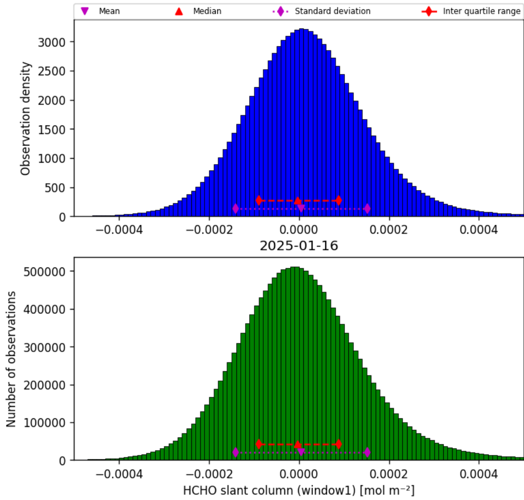
Figure 36: Histogram of “HCHO slant column (window1)” for 2025-01-16 to 2025-01-17
