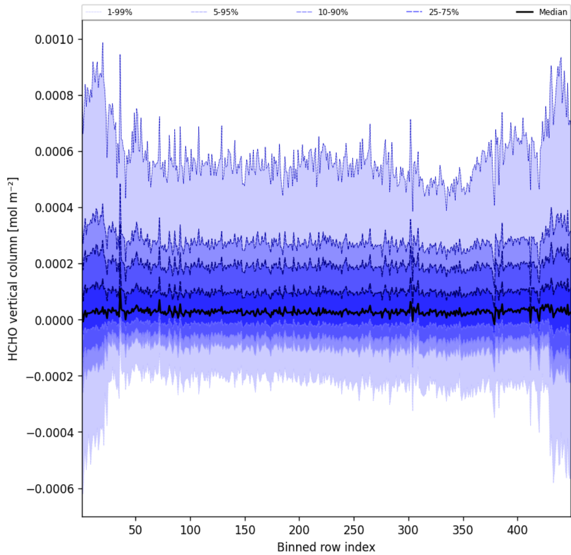
Figure 47: Along track statistics of “HCHO vertical column” for 2025-01-16 to 2025-01-17
