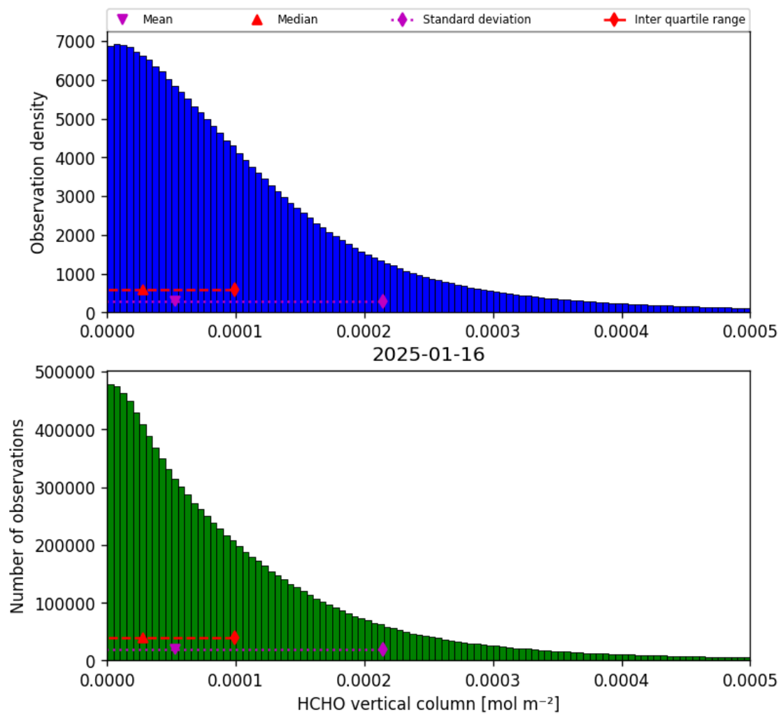
Figure 33: Histogram of “HCHO vertical column” for 2025-01-16 to 2025-01-17
