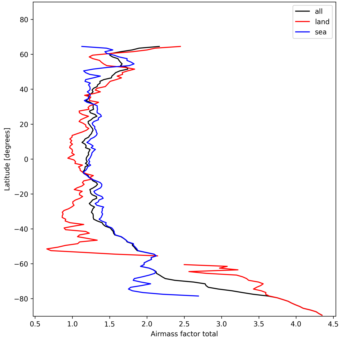
Figure 24: Zonal average of “Airmass factor total” for 2025-01-16 to 2025-01-17.
