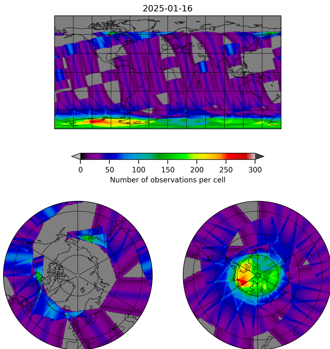
Figure 17: Map of the number of observations for 2025-01-16 to 2025-01-17
