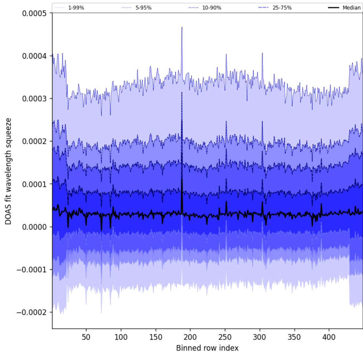
Figure 57: Along track statistics of “DOAS fit wavelength squeeze” for 2025-01-16 to 2025-01-17
