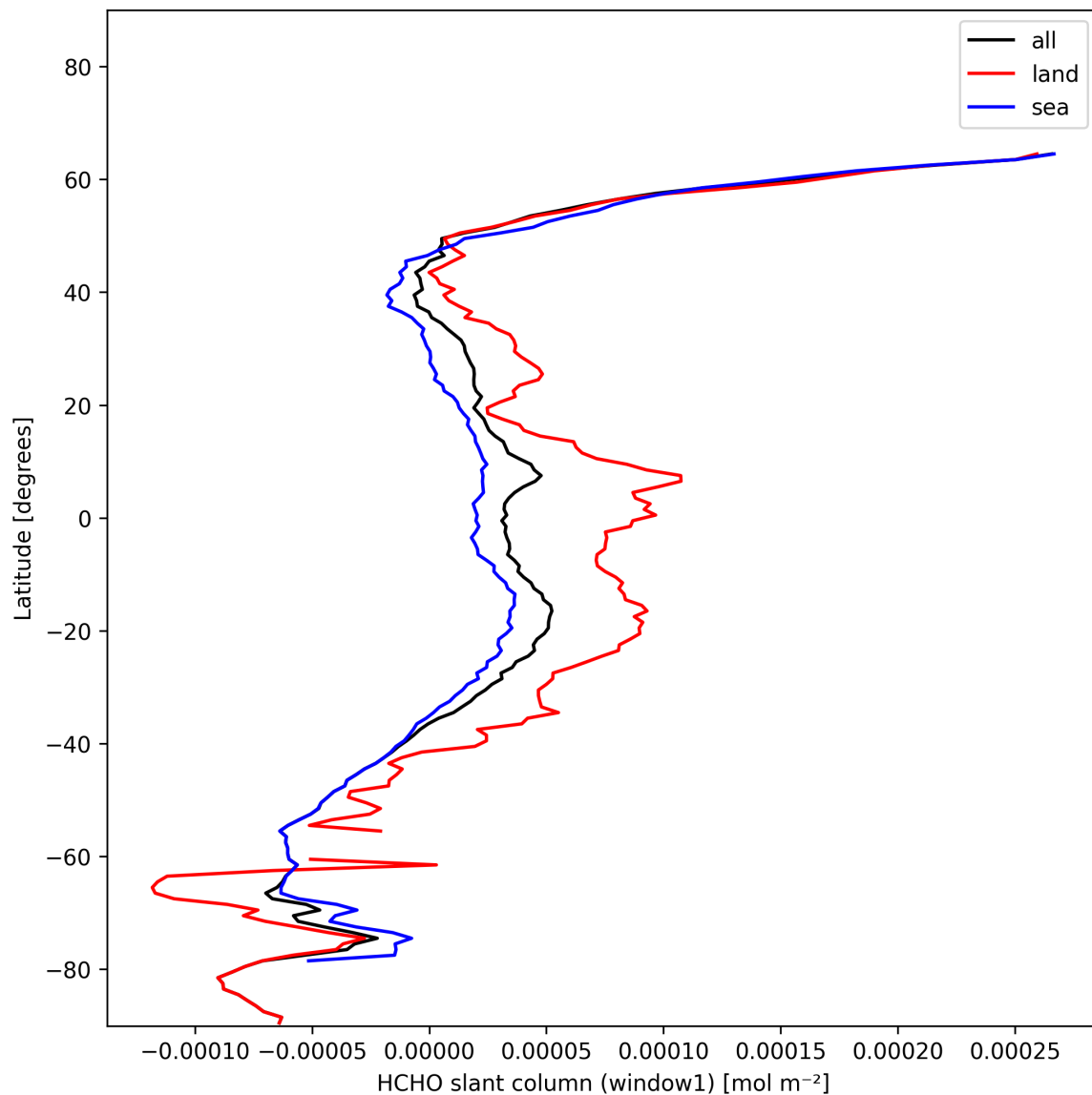
Figure 22: Zonal average of “HCHO slant column (window1)” for 2025-01-16 to 2025-01-17.
