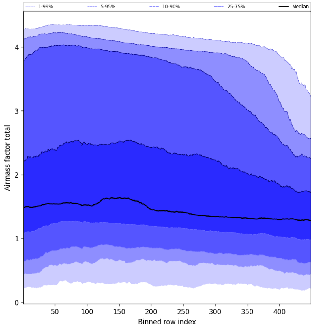
Figure 52: Along track statistics of “Airmass factor total” for 2025-01-16 to 2025-01-17
