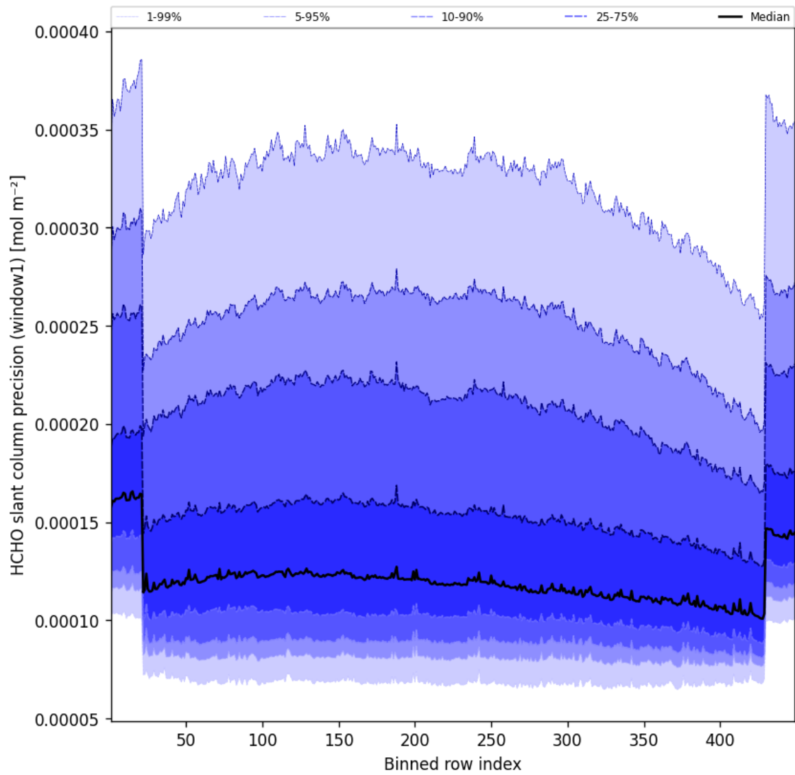
Figure 51: Along track statistics of “HCHO slant column precision (window1)” for 2025-01-16 to 2025-01-17
