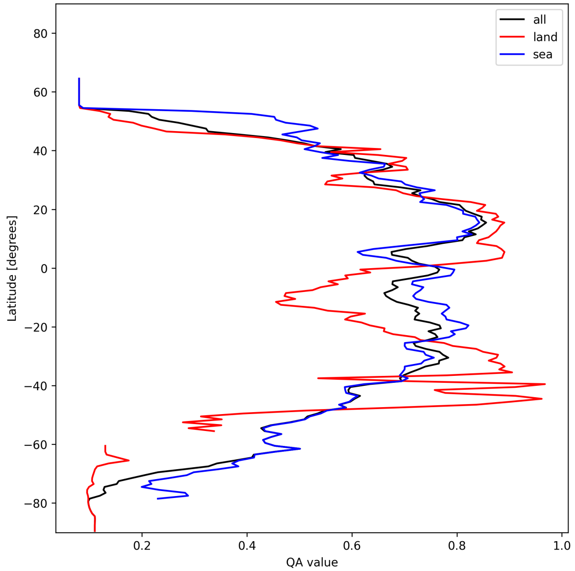
Figure 18: Zonal average of “QA value” for 2025-01-16 to 2025-01-17.
