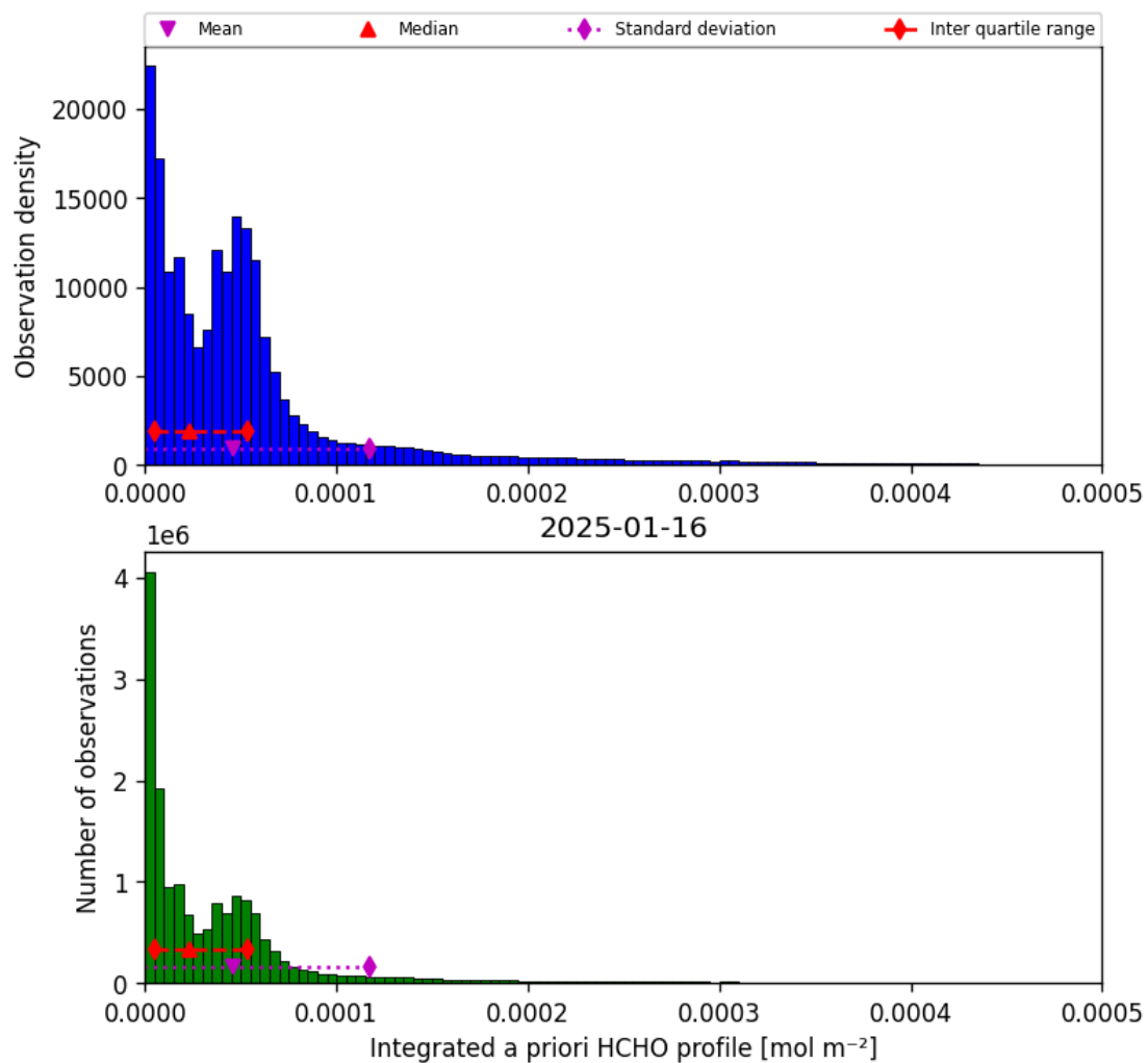
Figure 41: Histogram of “Integrated a priori HCHO profile” for 2025-01-16 to 2025-01-17
