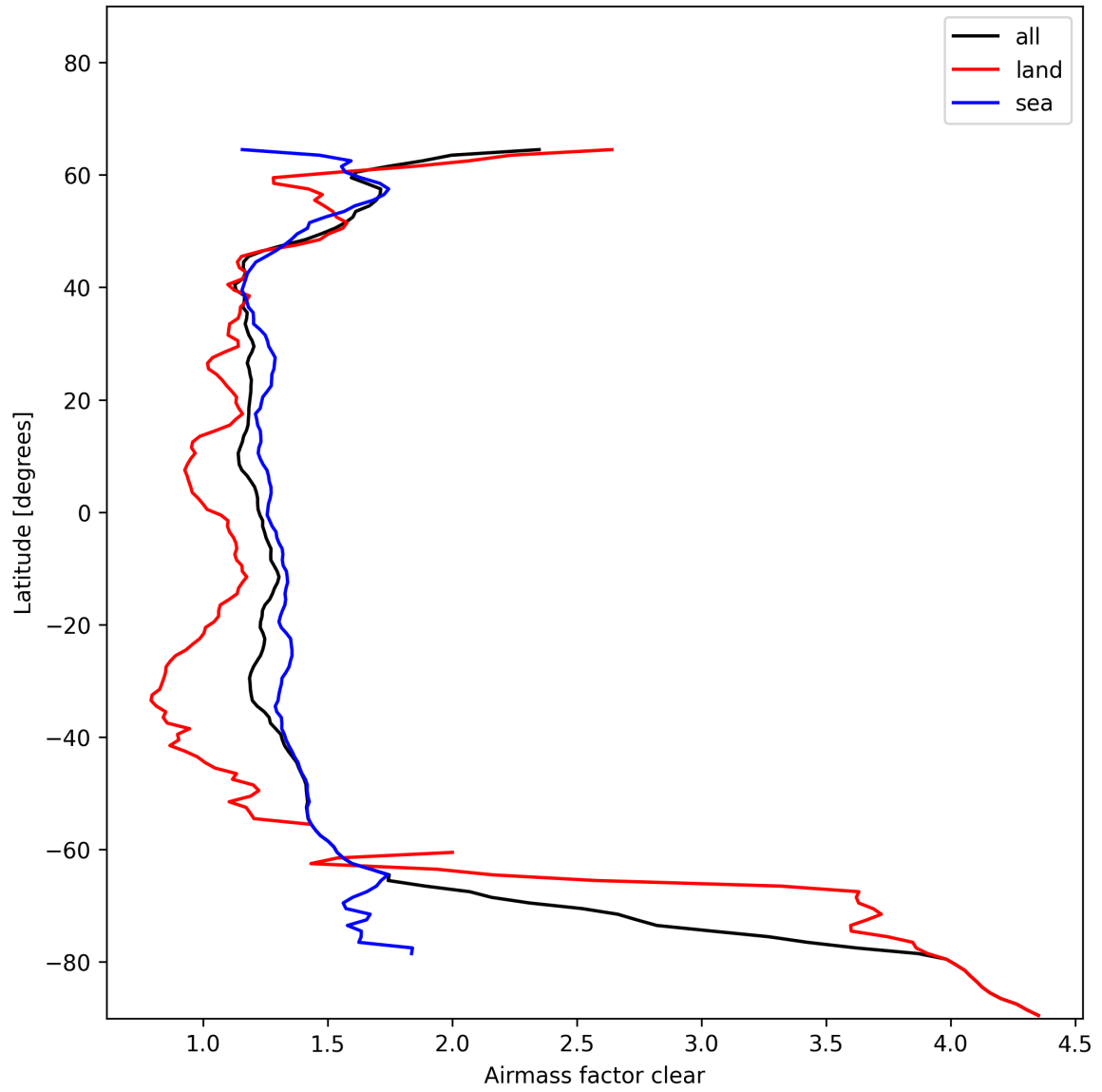
Figure 26: Zonal average of “Airmass factor clear” for 2025-01-16 to 2025-01-17.
