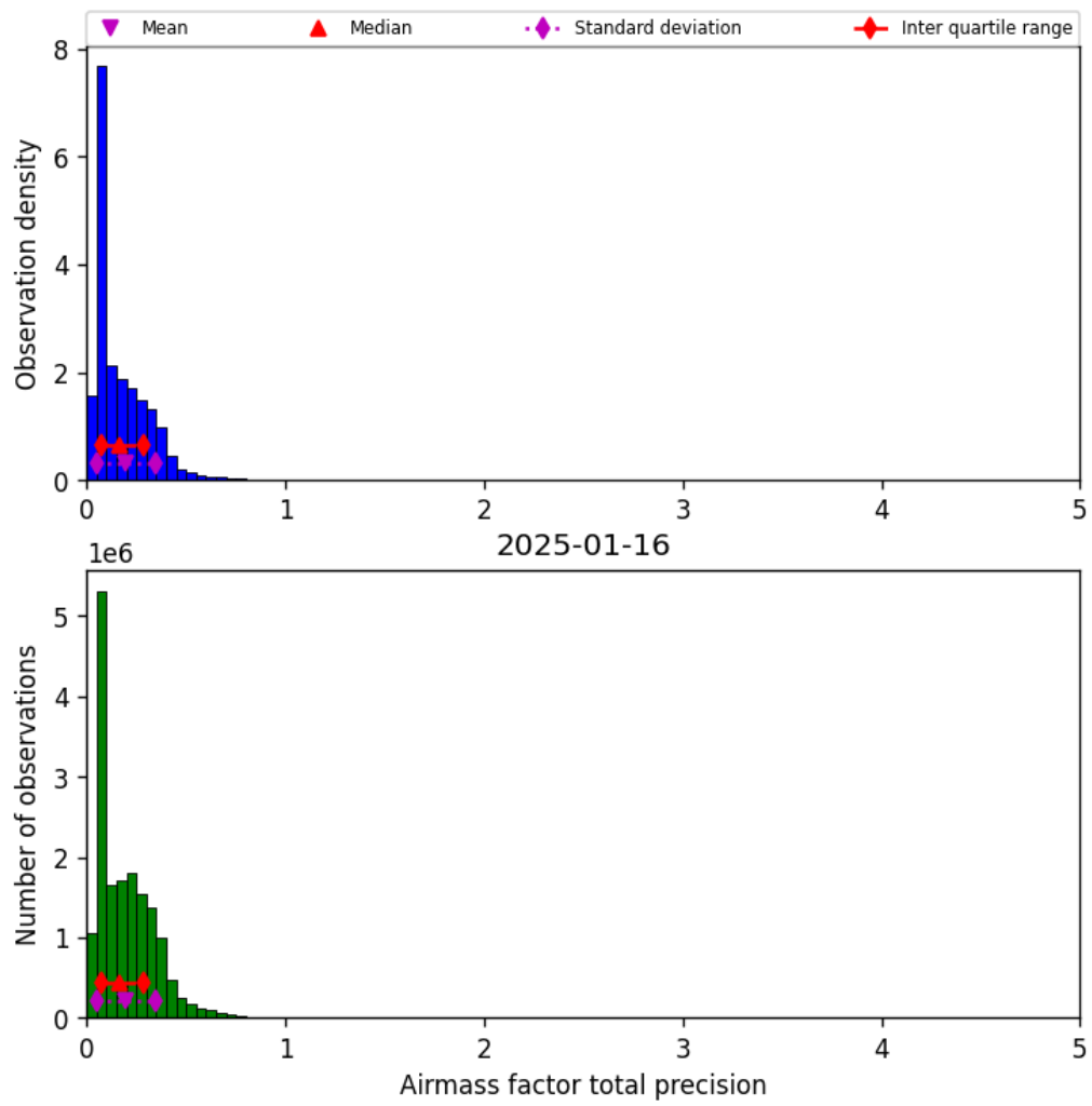
Figure 39: Histogram of “Airmass factor total precision” for 2025-01-16 to 2025-01-17
