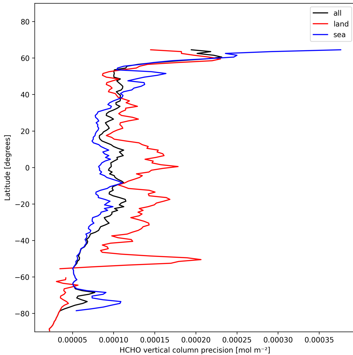
Figure 20: Zonal average of “HCHO vertical column precision” for 2025-01-16 to 2025-01-17.
