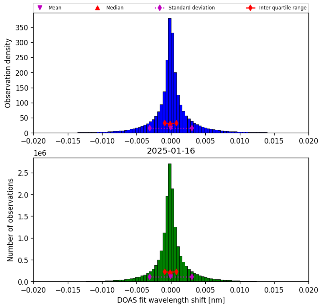
Figure 42: Histogram of “DOAS fit wavelength shift” for 2025-01-16 to 2025-01-17
