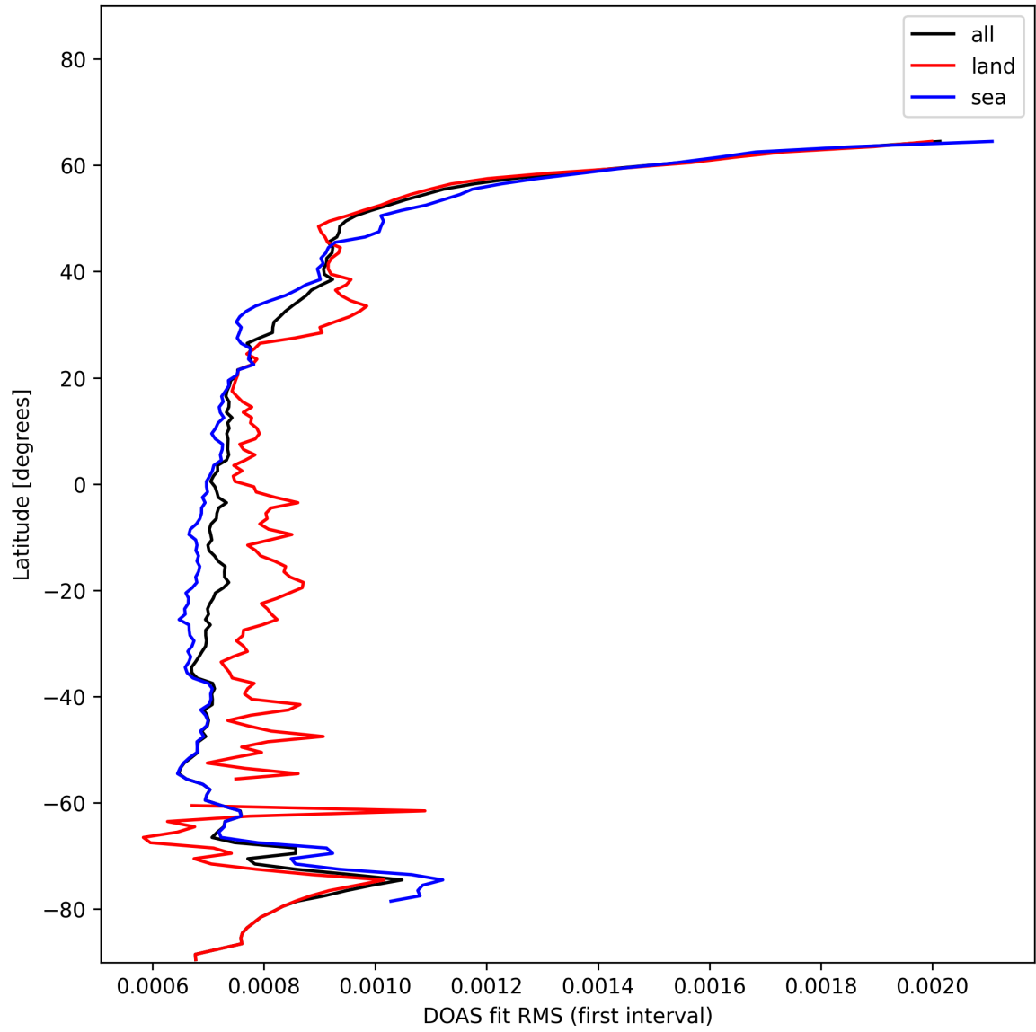
Figure 30: Zonal average of “DOAS fit RMS (first interval)” for 2025-01-16 to 2025-01-17.
