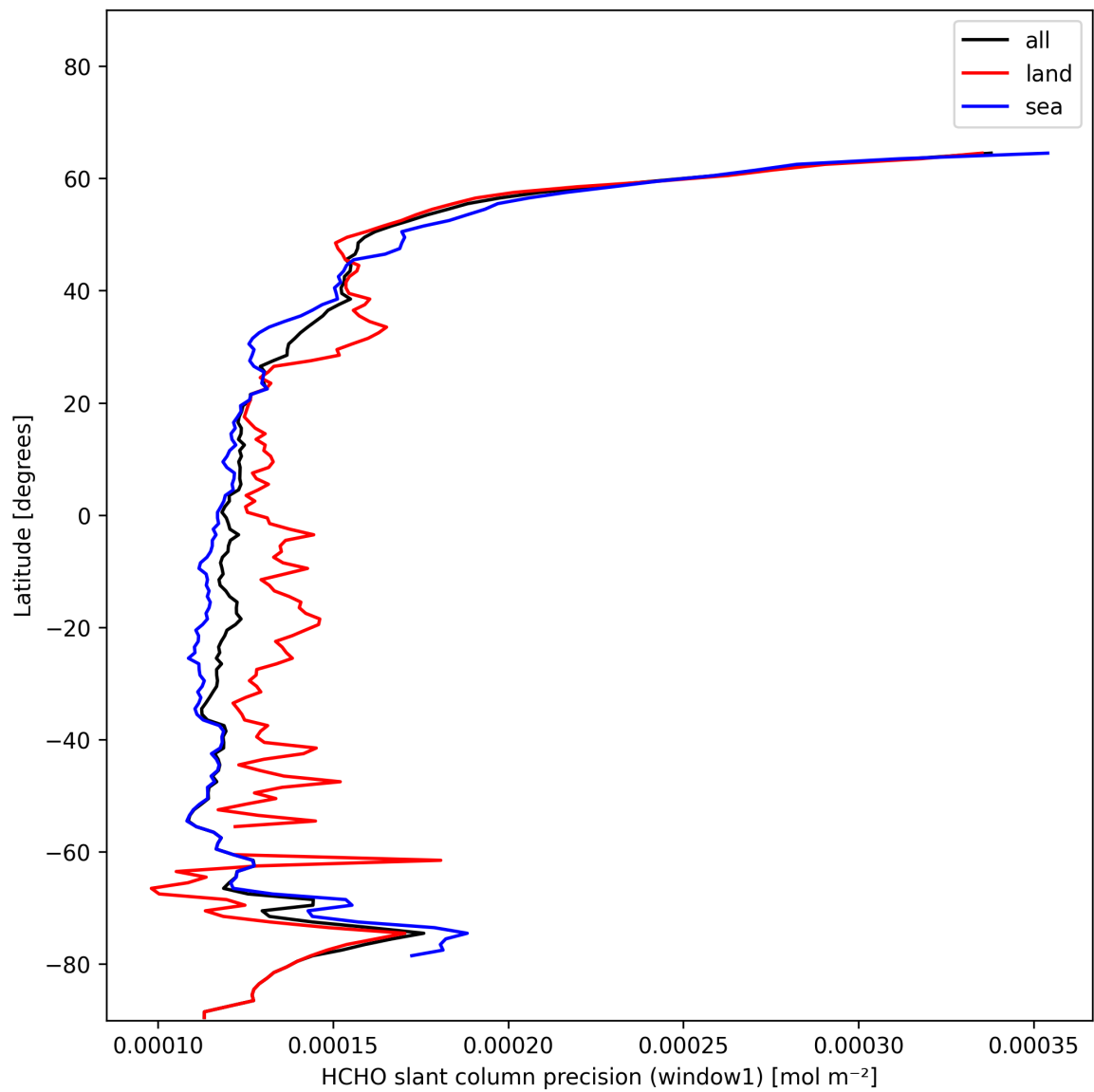
Figure 23: Zonal average of "HCHO slant column precision (window1)" for 2025-01-16 to 2025-01-17.
