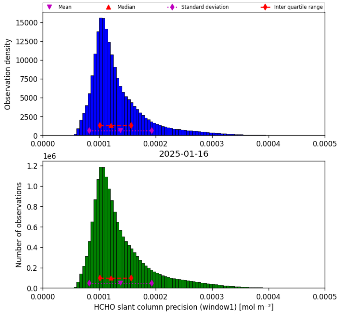
Figure 37: Histogram of “HCHO slant column precision (window1)” for 2025-01-16 to 2025-01-17
