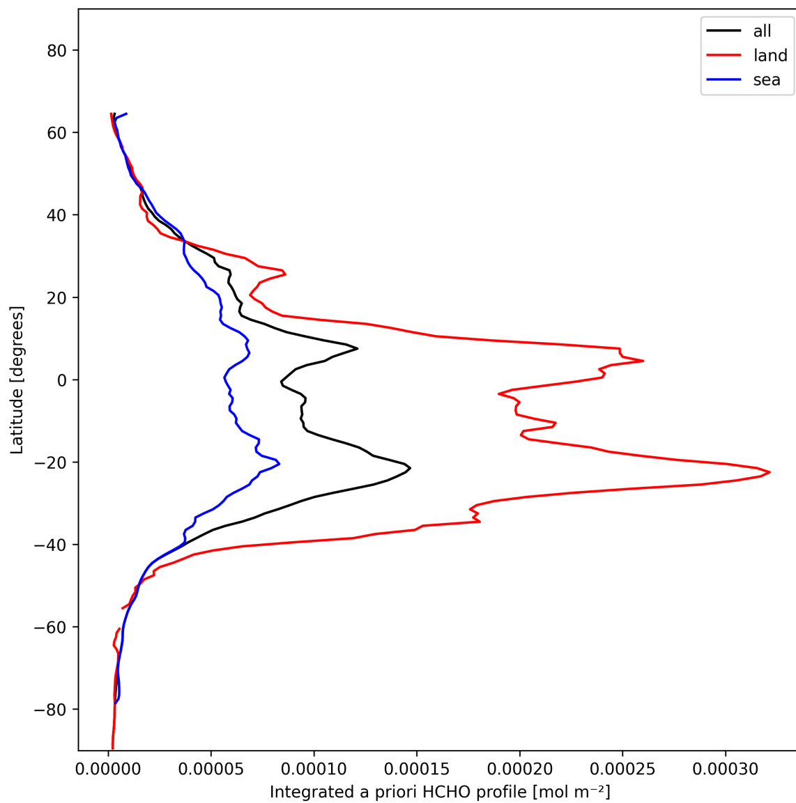
Figure 27: Zonal average of “Integrated a priori HCHO profile” for 2025-01-16 to 2025-01-17.
