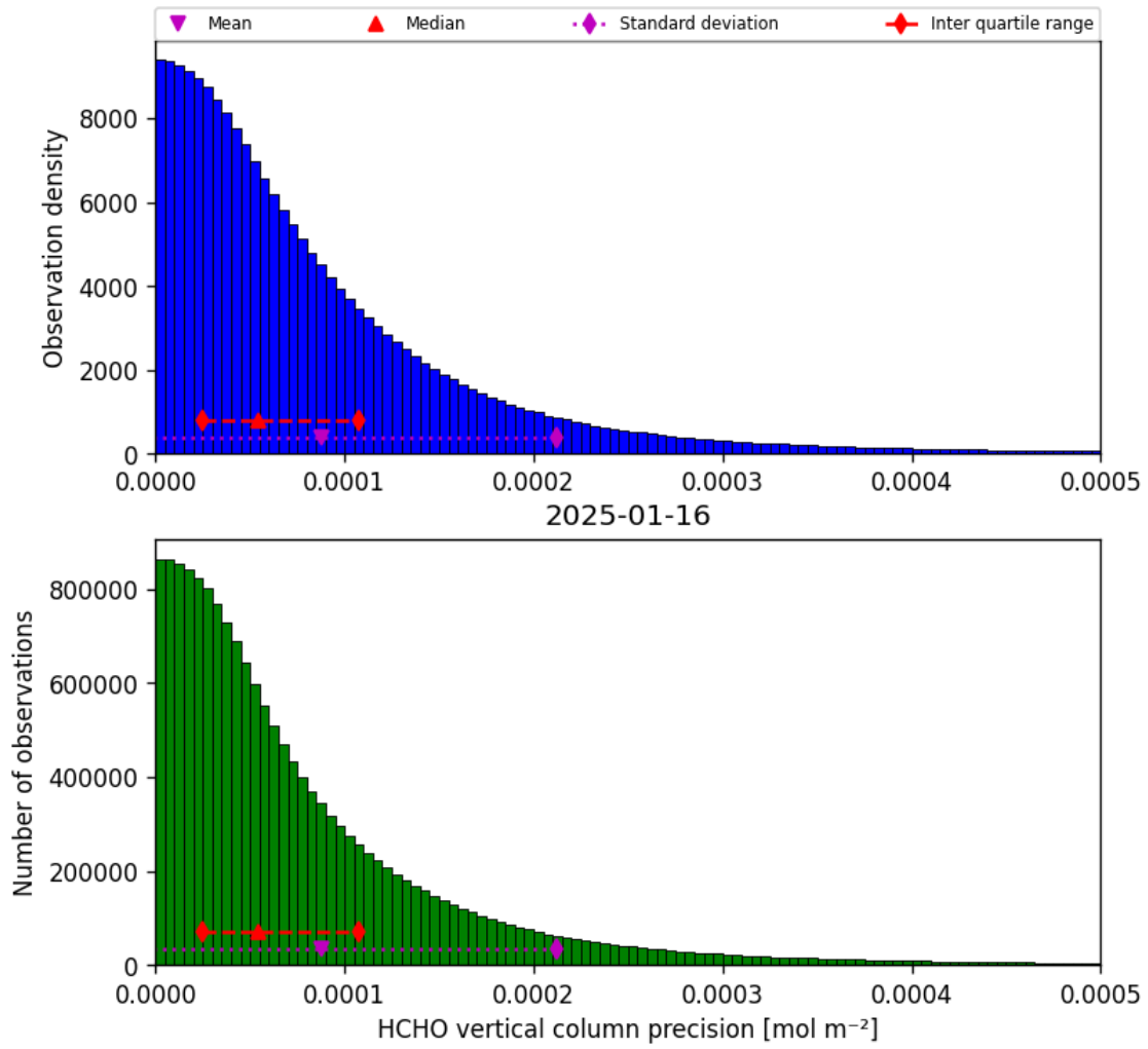
Figure 34: Histogram of “HCHO vertical column precision” for 2025-01-16 to 2025-01-17
