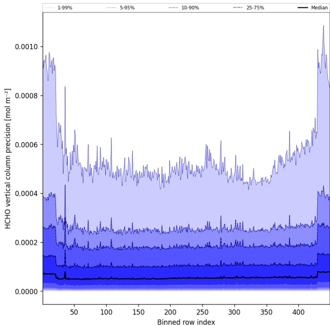
Figure 48: Along track statistics of “HCHO vertical column precision” for 2025-01-16 to 2025-01-17
