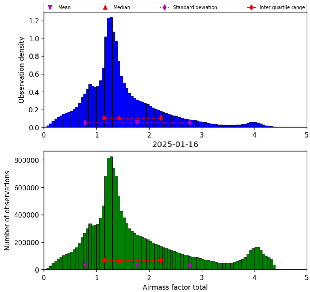
Figure 38: Histogram of “Airmass factor total” for 2025-01-16 to 2025-01-17
