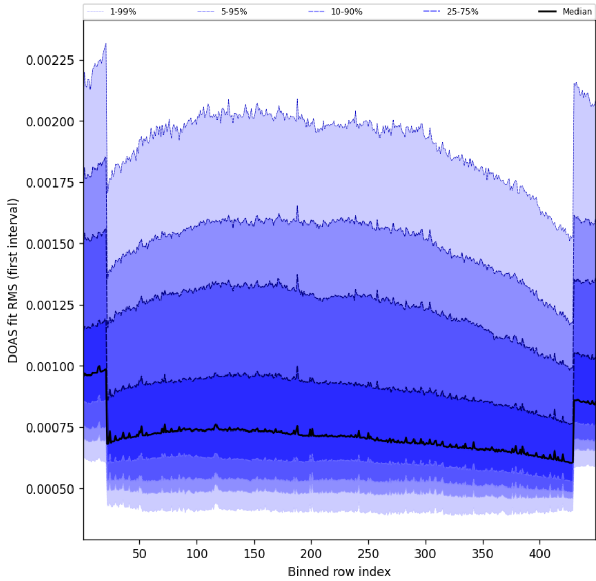
Figure 58: Along track statistics of “DOAS fit RMS (first interval)” for 2025-01-16 to 2025-01-17
