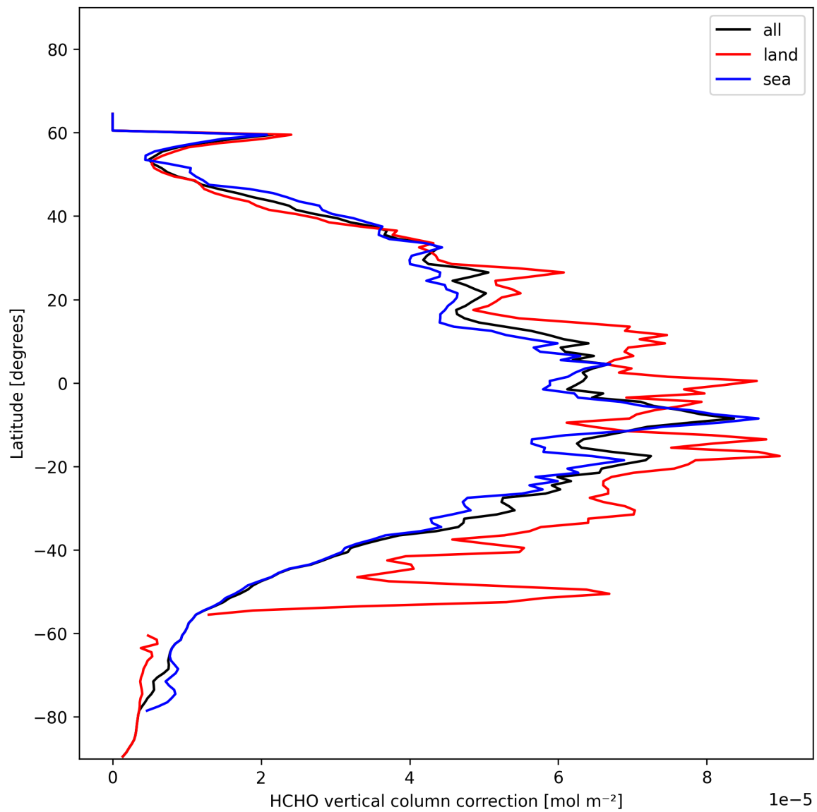
Figure 21: Zonal average of “HCHO vertical column correction” for 2025-01-16 to 2025-01-17.
