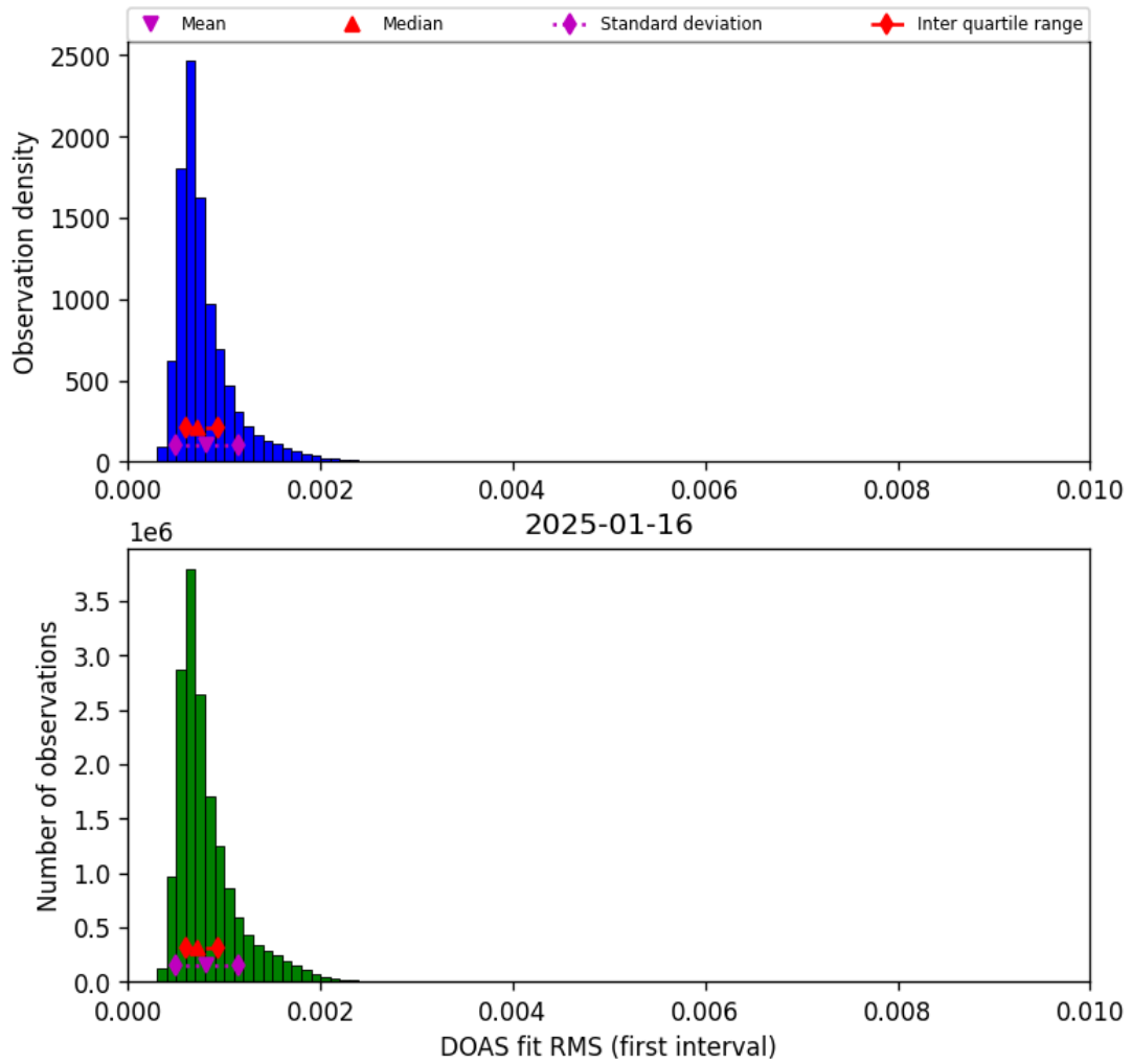
Figure 44: Histogram of “DOAS fit RMS (first interval)” for 2025-01-16 to 2025-01-17
