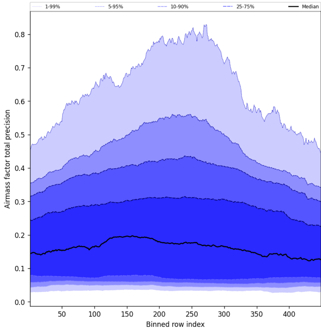
Figure 53: Along track statistics of “Airmass factor total precision” for 2025-01-16 to 2025-01-17
