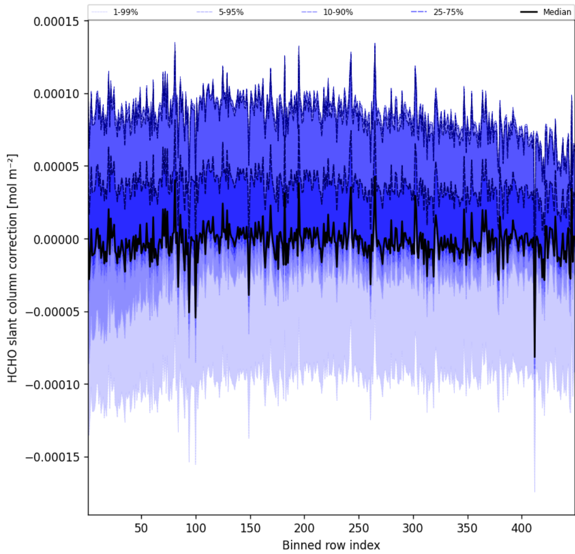
Figure 59: Along track statistics of “HCHO slant column correction” for 2025-01-16 to 2025-01-17
