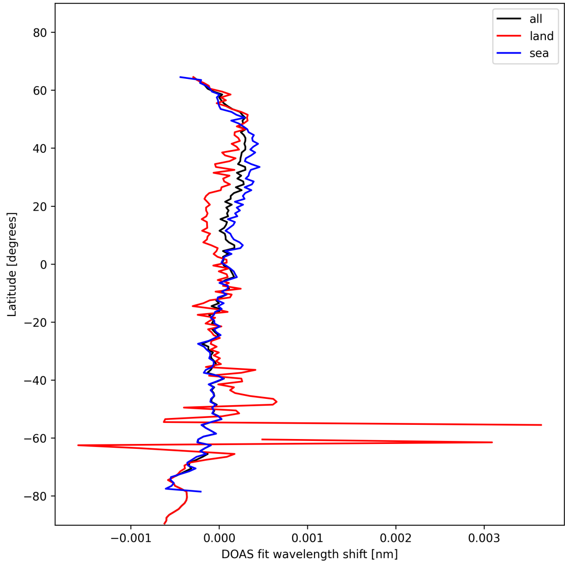
Figure 28: Zonal average of “DOAS fit wavelength shift” for 2025-01-16 to 2025-01-17.
