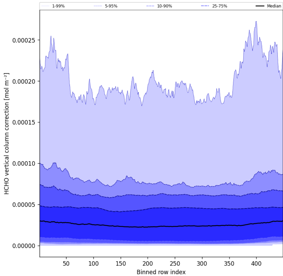
Figure 49: Along track statistics of “HCHO vertical column correction” for 2025-01-16 to 2025-01-17
