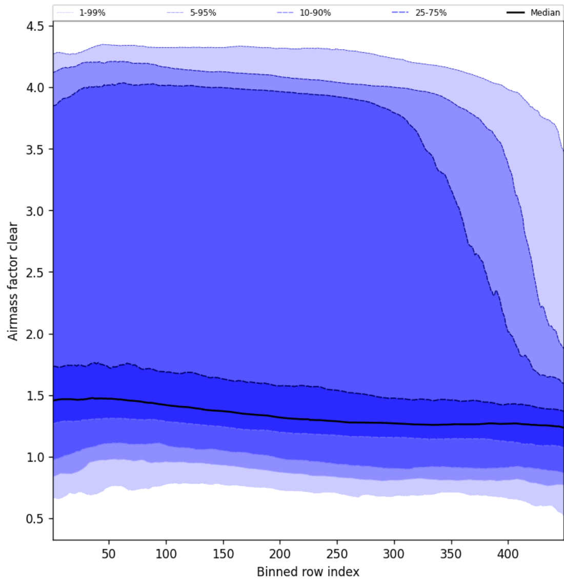
Figure 54: Along track statistics of “Airmass factor clear” for 2025-01-16 to 2025-01-17
