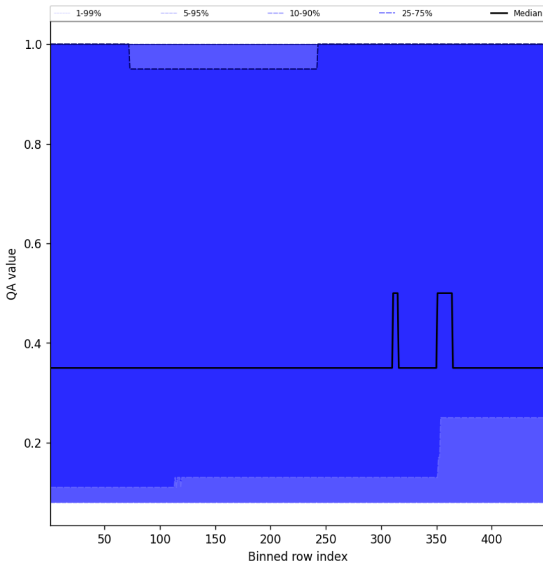
Figure 46: Along track statistics of “QA value” for 2025-01-16 to 2025-01-17
