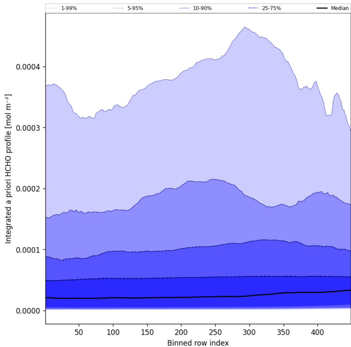
Figure 55: Along track statistics of "Integrated a priori HCHO profile" for 2025-01-16 to 2025-01-17
