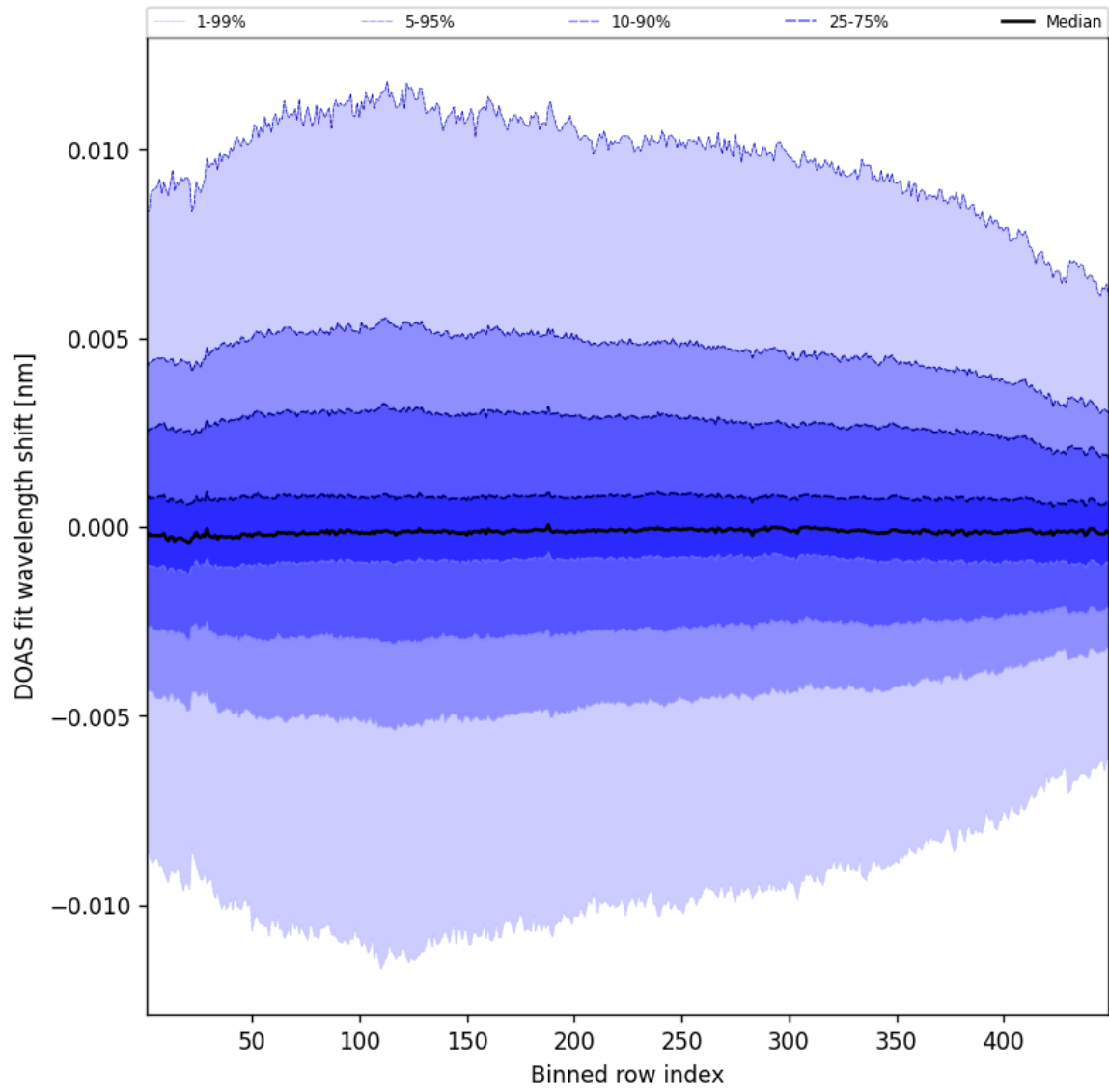
Figure 56: Along track statistics of “DOAS fit wavelength shift” for 2025-01-16 to 2025-01-17
