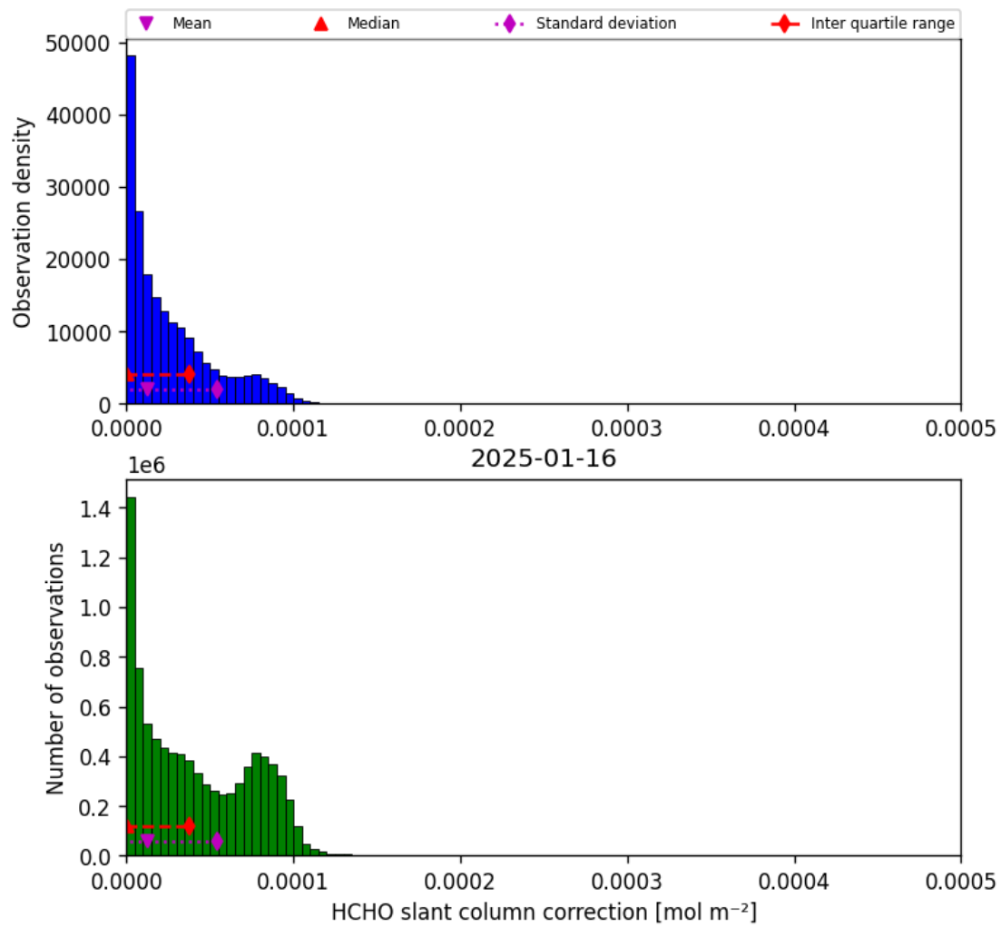
Figure 45: Histogram of “HCHO slant column correction” for 2025-01-16 to 2025-01-17
