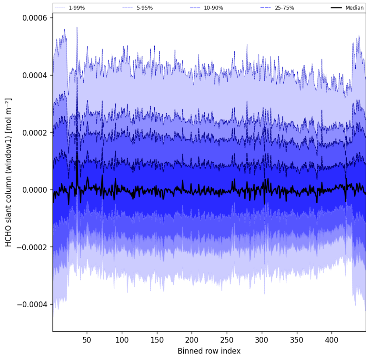
Figure 50: Along track statistics of “HCHO slant column (window1)” for 2025-01-16 to 2025-01-17
