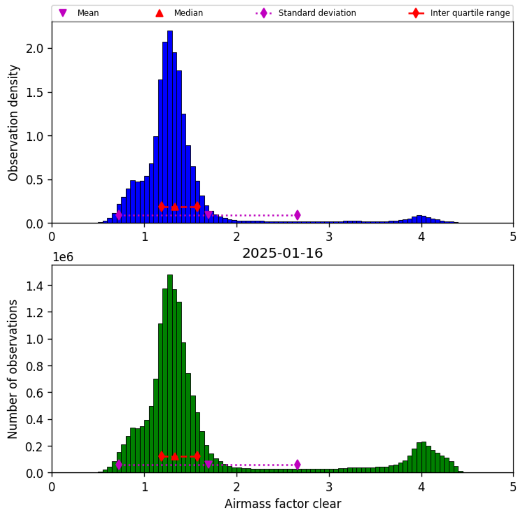
Figure 40: Histogram of “Airmass factor clear” for 2025-01-16 to 2025-01-17
