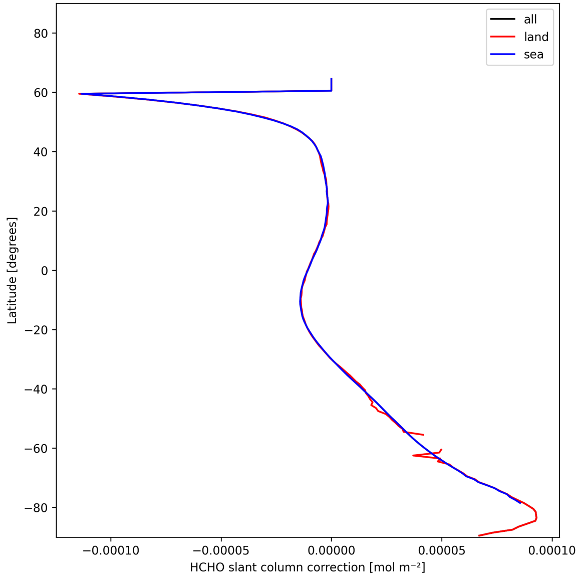
Figure 31: Zonal average of “HCHO slant column correction” for 2025-01-16 to 2025-01-17.
