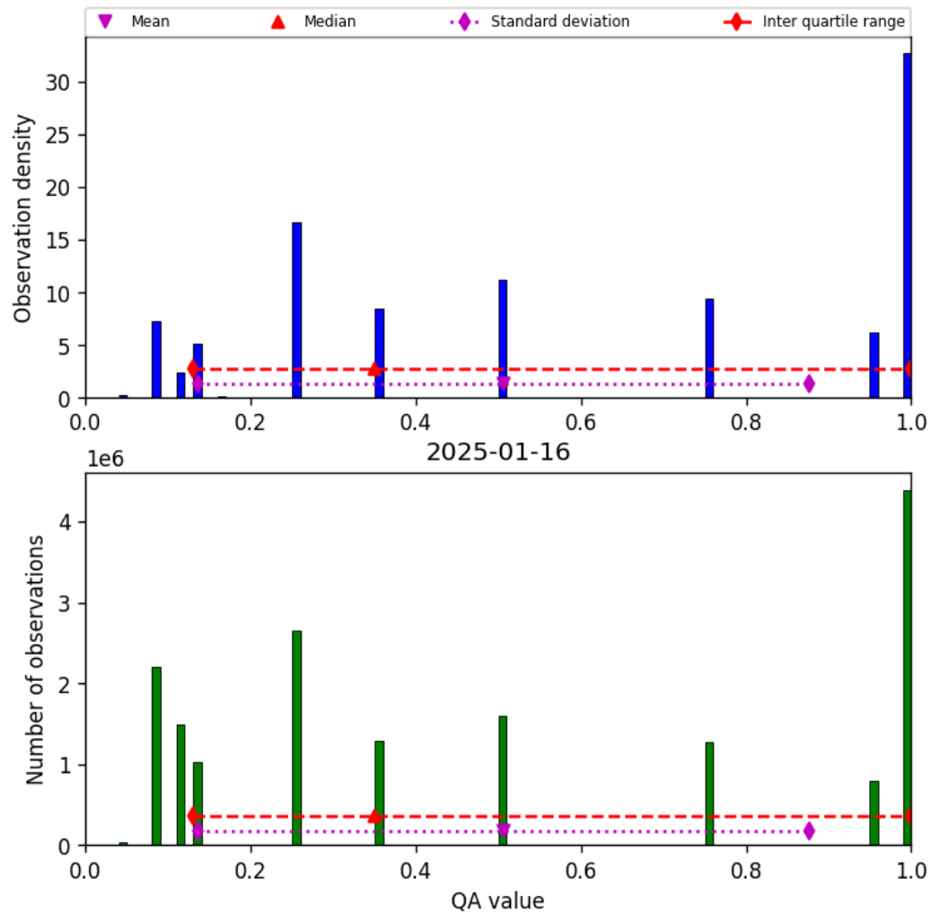
Figure 32: Histogram of “QA value” for 2025-01-16 to 2025-01-17
