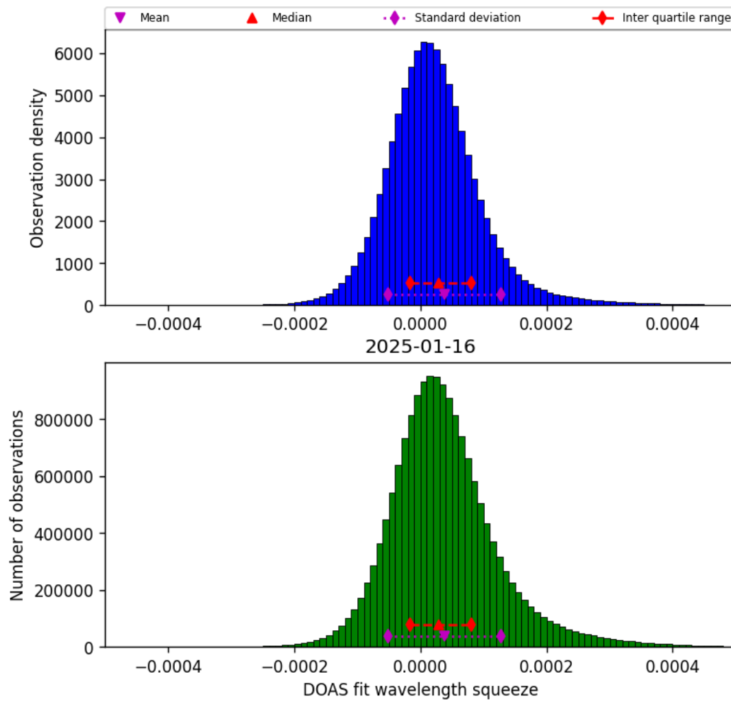
Figure 43: Histogram of “DOAS fit wavelength squeeze” for 2025-01-16 to 2025-01-17
