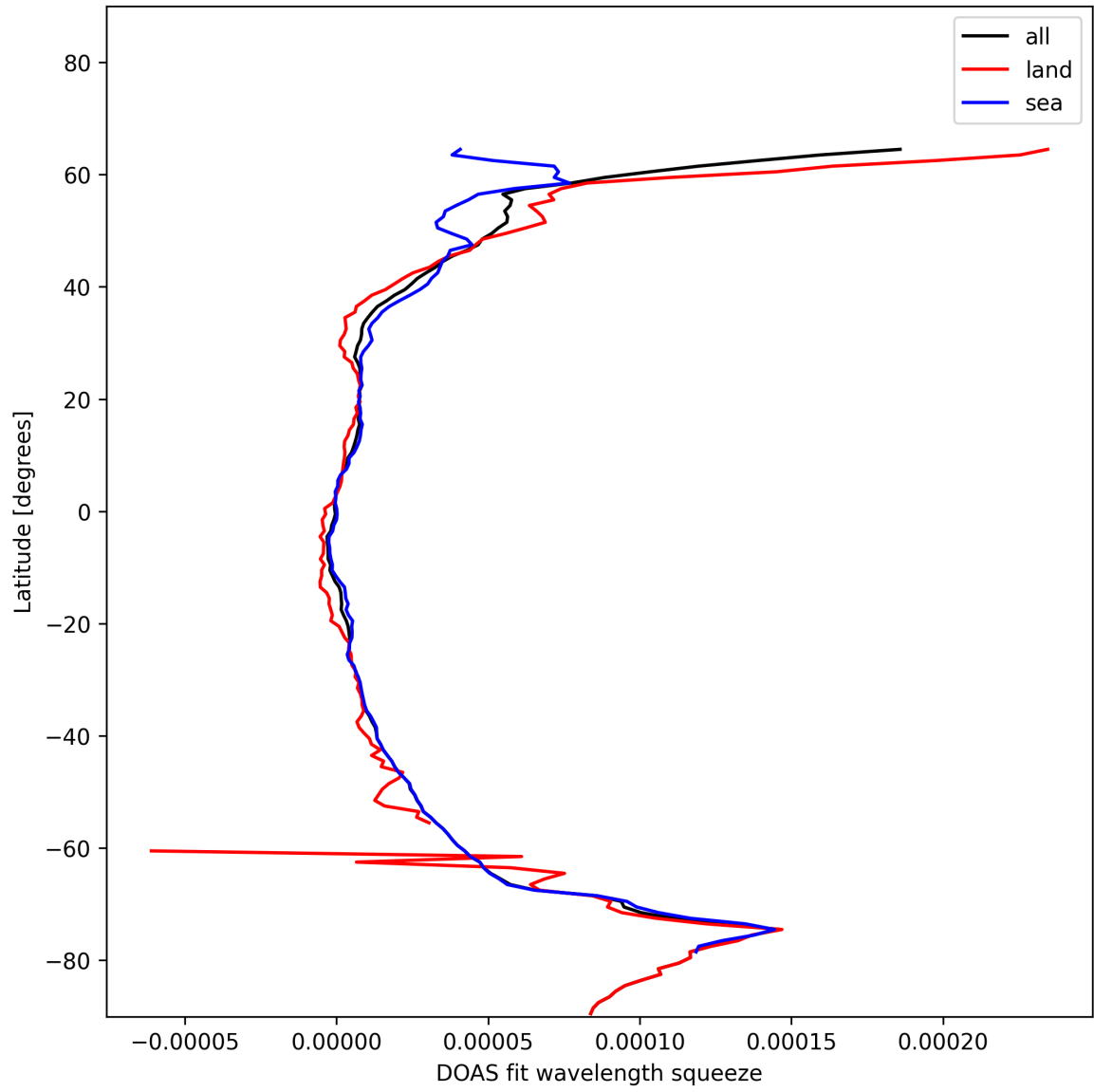
Figure 29: Zonal average of “DOAS fit wavelength squeeze” for 2025-01-16 to 2025-01-17.
