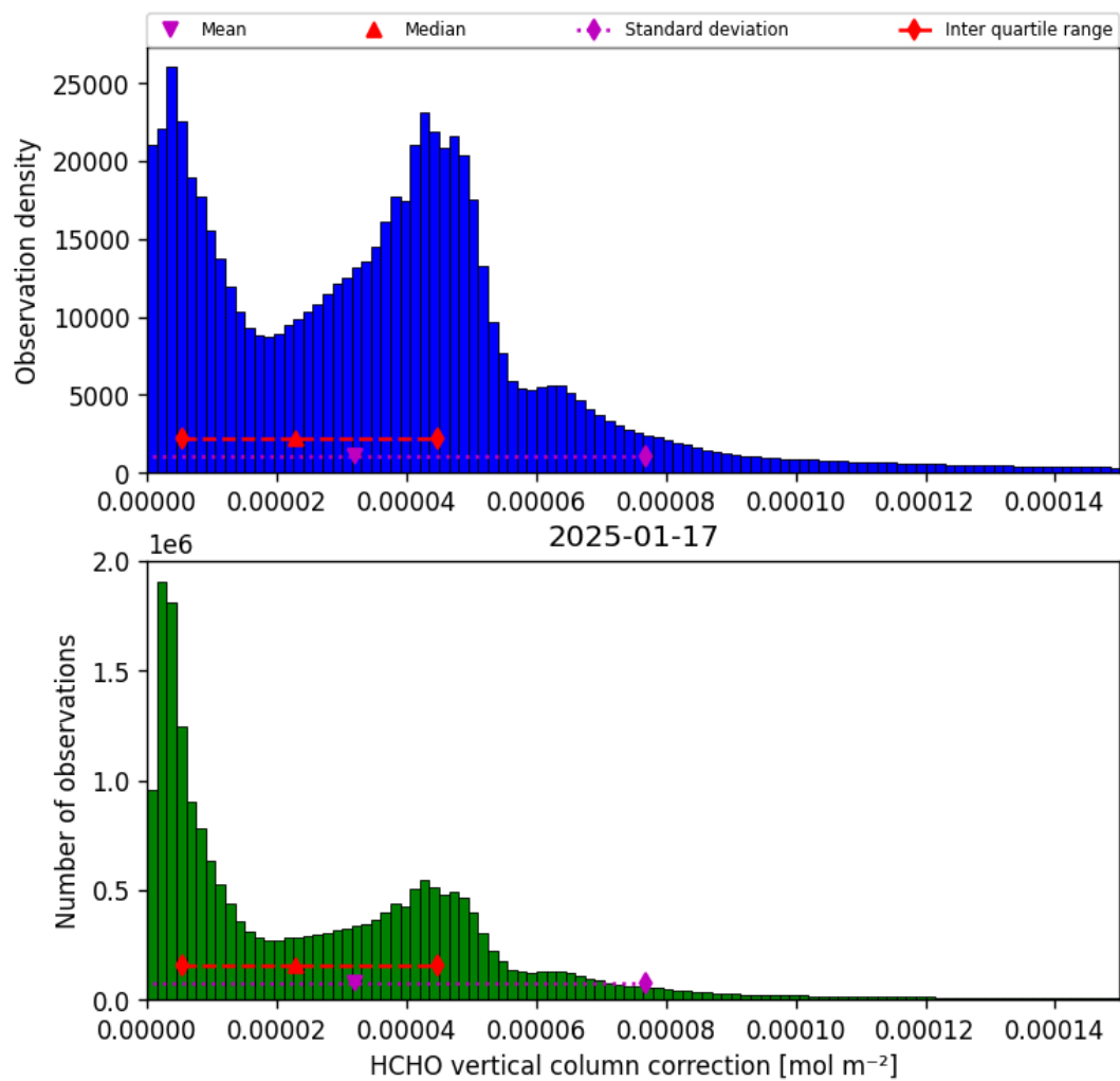
Figure 35: Histogram of “HCHO vertical column correction” for 2025-01-17 to 2025-01-18
