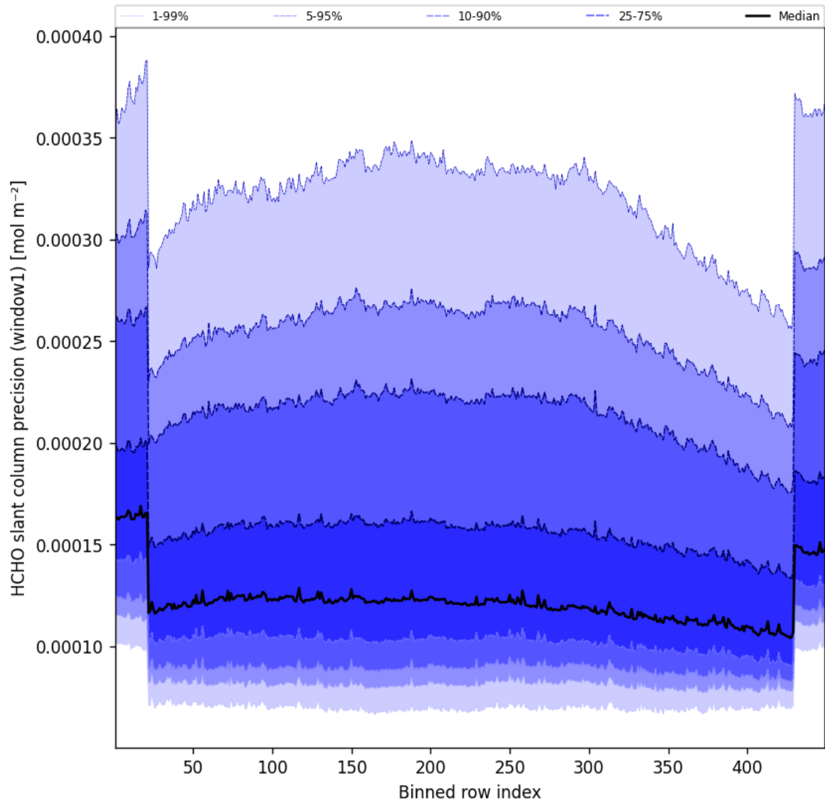
Figure 51: Along track statistics of “HCHO slant column precision (window1)” for 2025-01-17 to 2025-01-18
