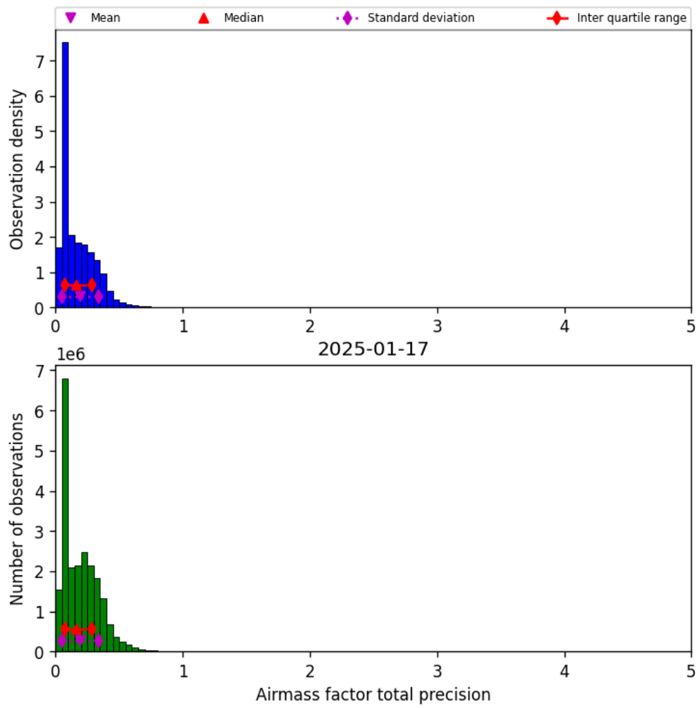
Figure 39: Histogram of “Airmass factor total precision” for 2025-01-17 to 2025-01-18
