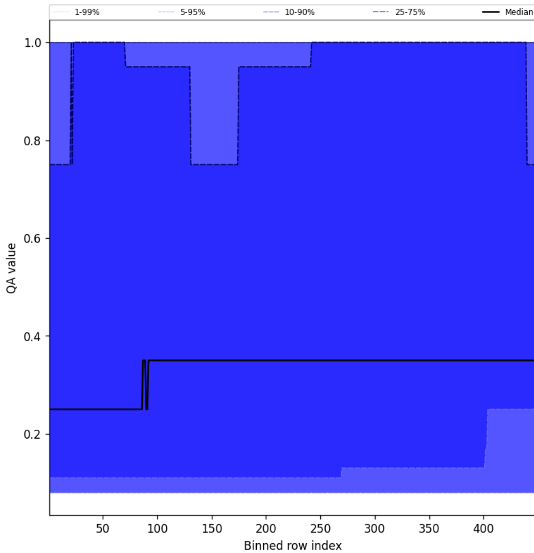
Figure 46: Along track statistics of “QA value” for 2025-01-17 to 2025-01-18
