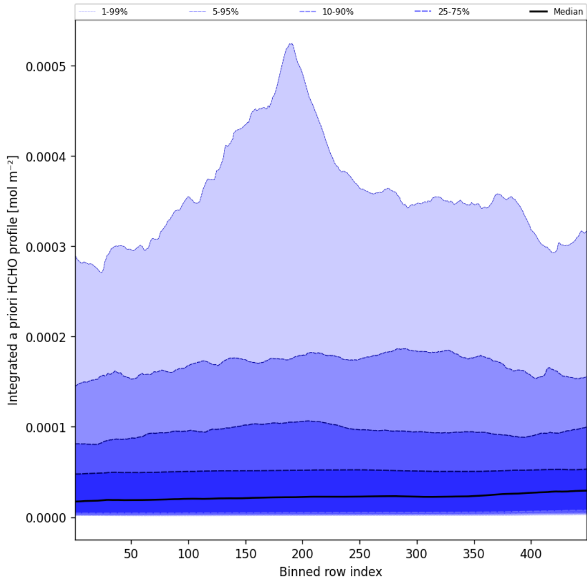
Figure 55: Along track statistics of “Integrated a priori HCHO profile” for 2025-01-17 to 2025-01-18
