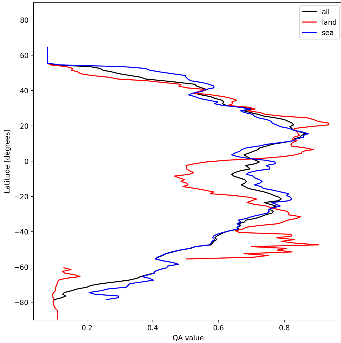
Figure 18: Zonal average of “QA value” for 2025-01-17 to 2025-01-18.
