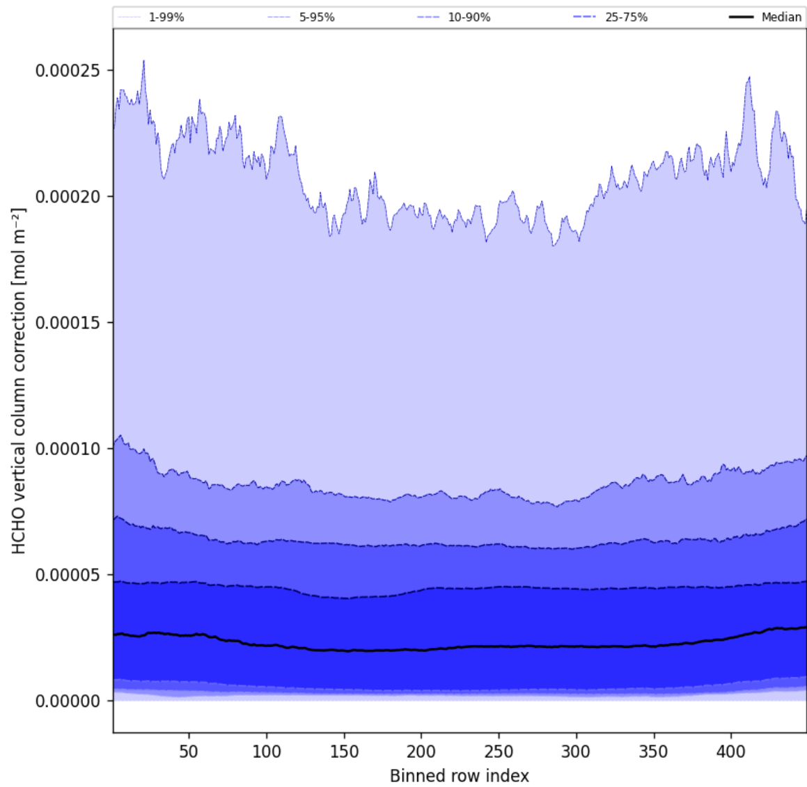
Figure 49: Along track statistics of “HCHO vertical column correction” for 2025-01-17 to 2025-01-18
