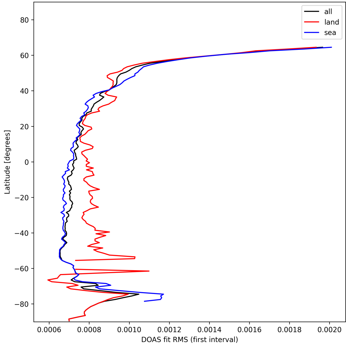
Figure 30: Zonal average of “DOAS fit RMS (first interval)” for 2025-01-17 to 2025-01-18.
