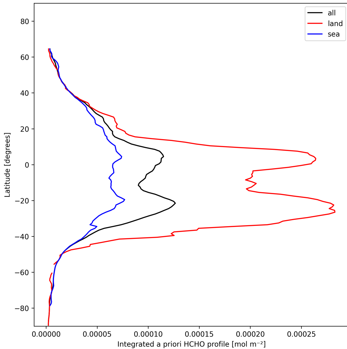
Figure 27: Zonal average of “Integrated a priori HCHO profile” for 2025-01-17 to 2025-01-18.
