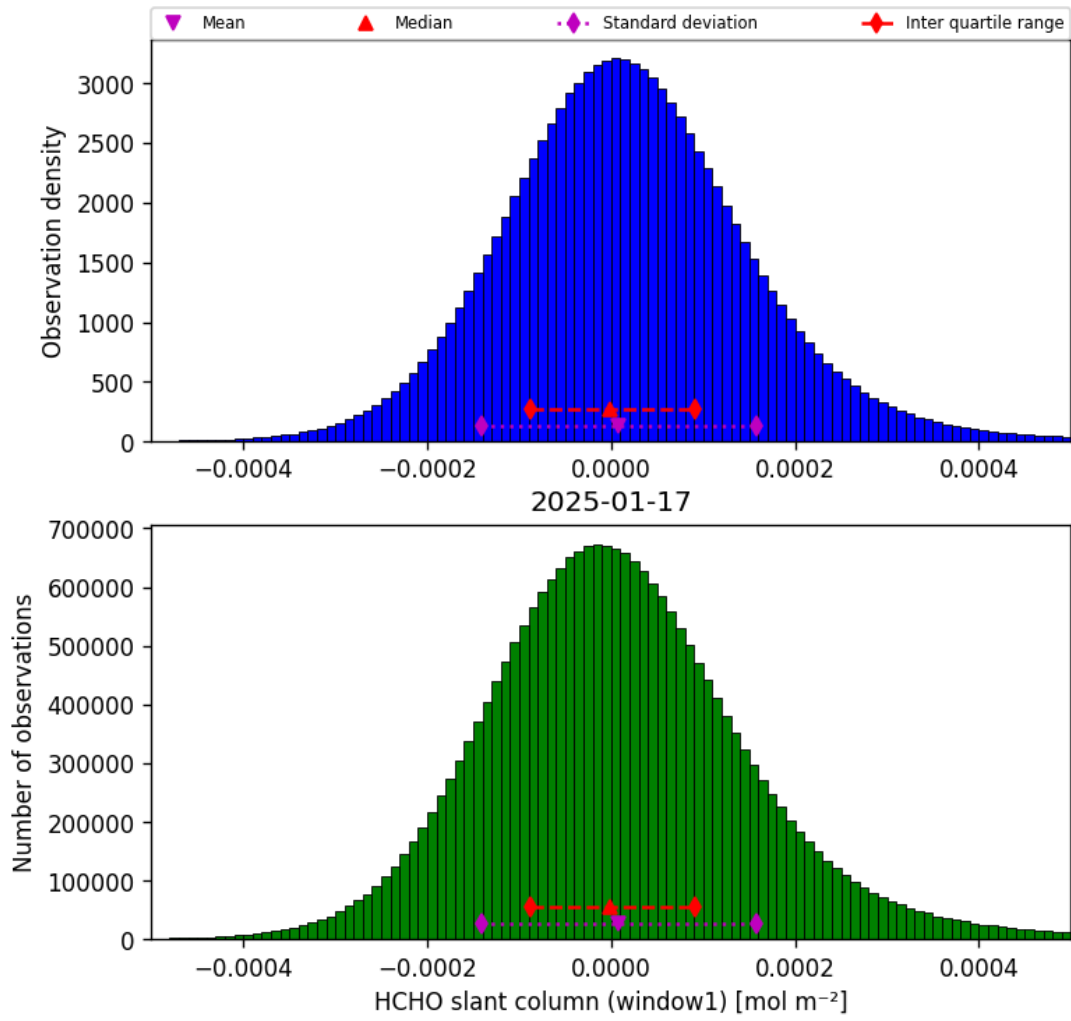
Figure 36: Histogram of “HCHO slant column (window1)” for 2025-01-17 to 2025-01-18
