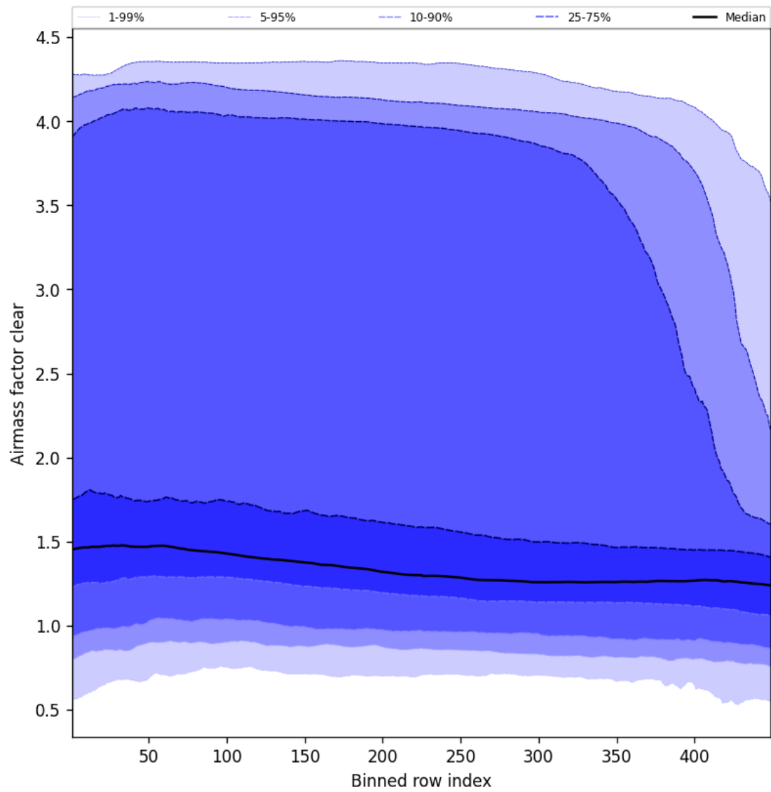
Figure 54: Along track statistics of “Airmass factor clear” for 2025-01-17 to 2025-01-18
