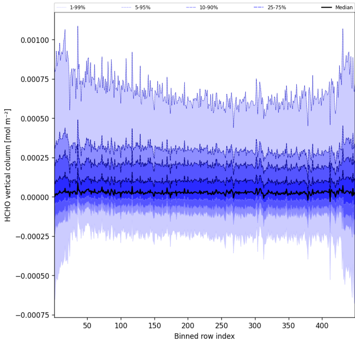
Figure 47: Along track statistics of “HCHO vertical column” for 2025-01-17 to 2025-01-18
