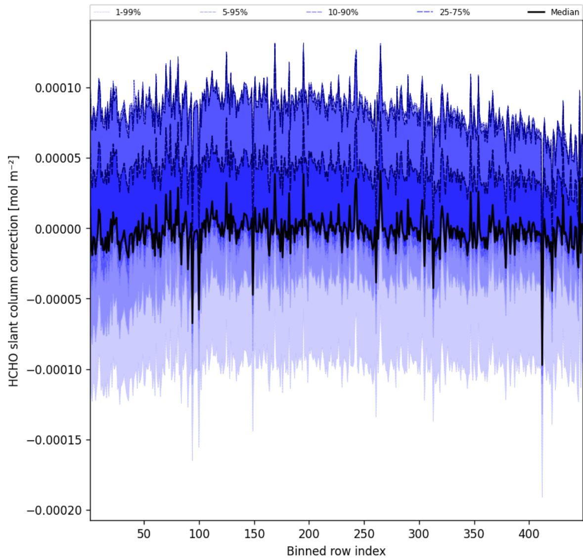
Figure 59: Along track statistics of “HCHO slant column correction” for 2025-01-17 to 2025-01-18
