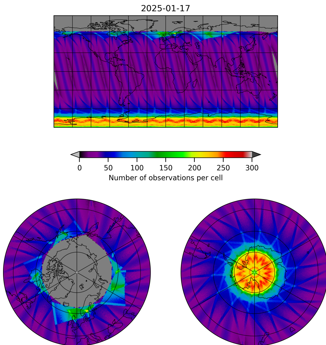
Figure 17: Map of the number of observations for 2025-01-17 to 2025-01-18
