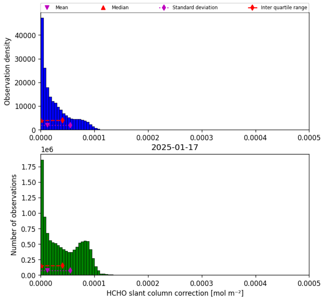
Figure 45: Histogram of “HCHO slant column correction” for 2025-01-17 to 2025-01-18
