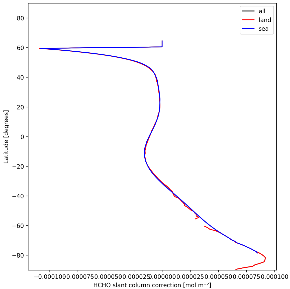
Figure 31: Zonal average of “HCHO slant column correction” for 2025-01-17 to 2025-01-18.
