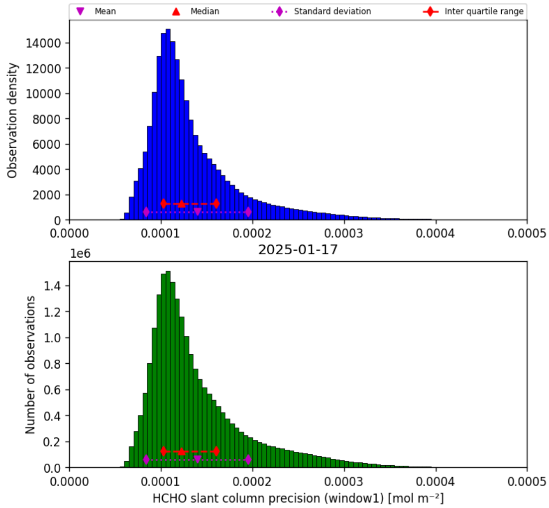
Figure 37: Histogram of “HCHO slant column precision (window1)” for 2025-01-17 to 2025-01-18
