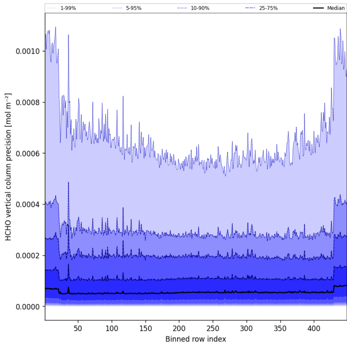
Figure 48: Along track statistics of “HCHO vertical column precision” for 2025-01-17 to 2025-01-18
