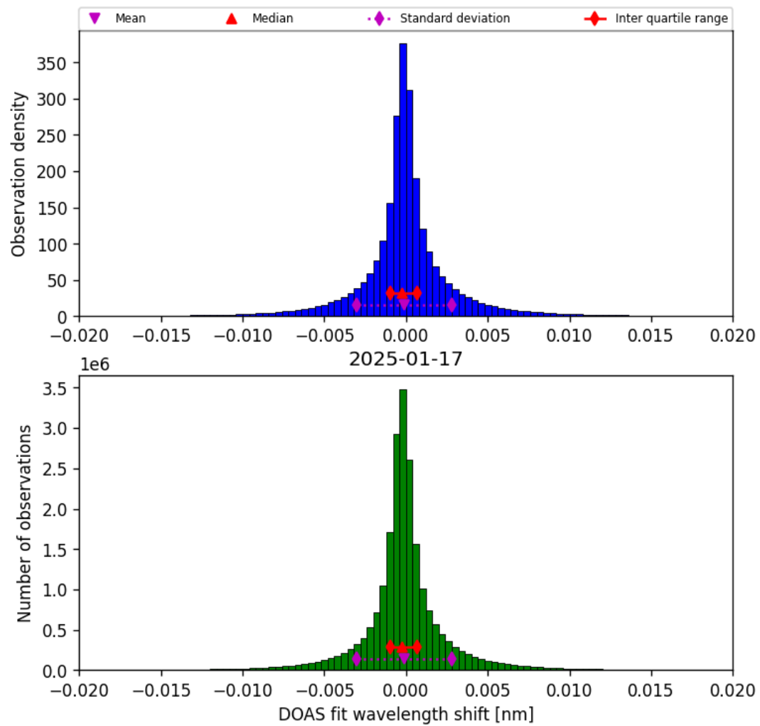
Figure 42: Histogram of “DOAS fit wavelength shift” for 2025-01-17 to 2025-01-18
