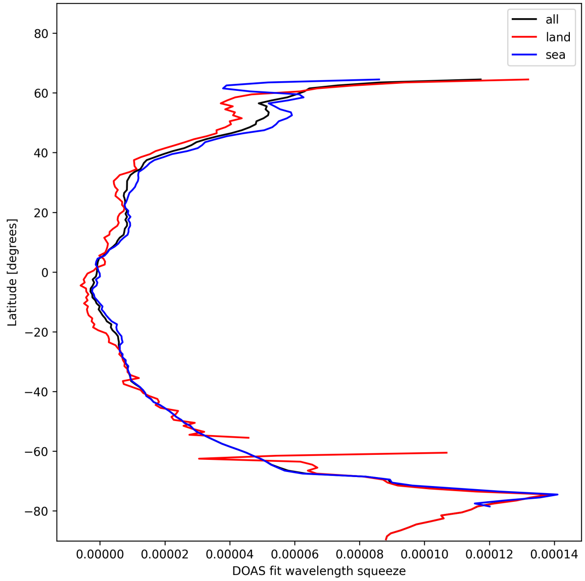
Figure 29: Zonal average of “DOAS fit wavelength squeeze” for 2025-01-17 to 2025-01-18.
