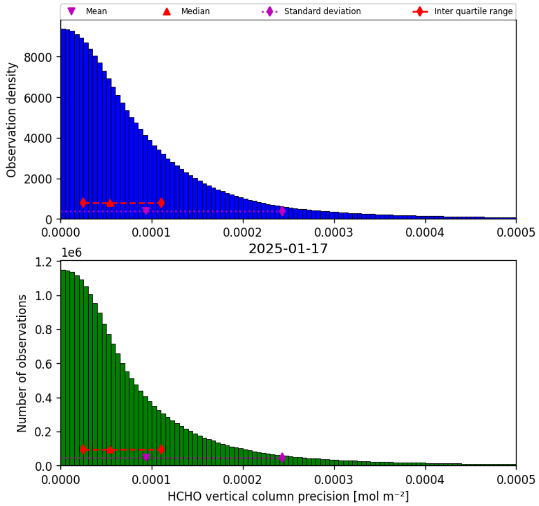
Figure 34: Histogram of “HCHO vertical column precision” for 2025-01-17 to 2025-01-18
