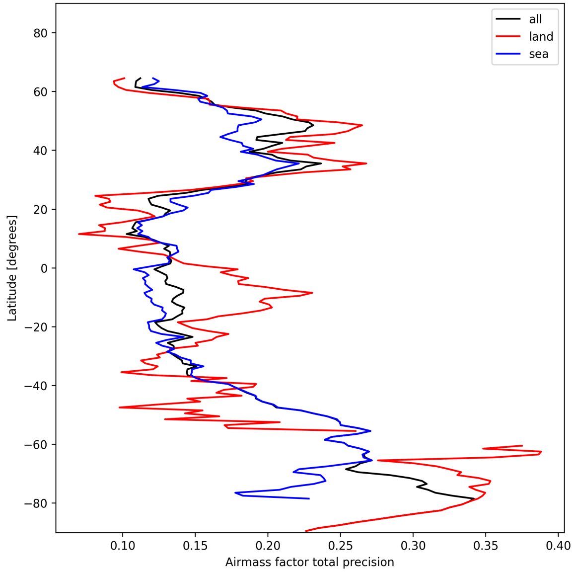
Figure 25: Zonal average of “Airmass factor total precision” for 2025-01-17 to 2025-01-18.
