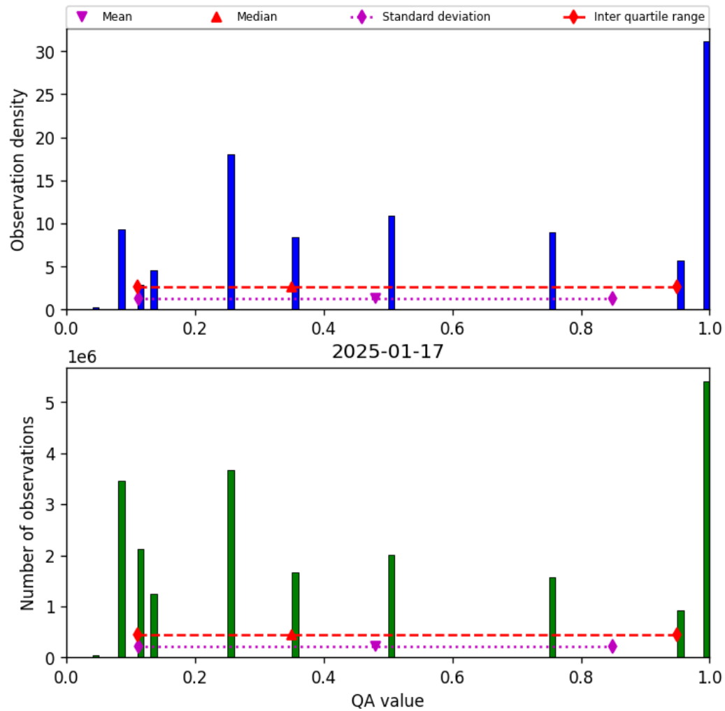
Figure 32: Histogram of “QA value” for 2025-01-17 to 2025-01-18
