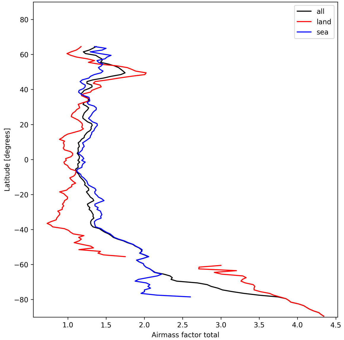
Figure 24: Zonal average of “Airmass factor total” for 2025-01-17 to 2025-01-18.
