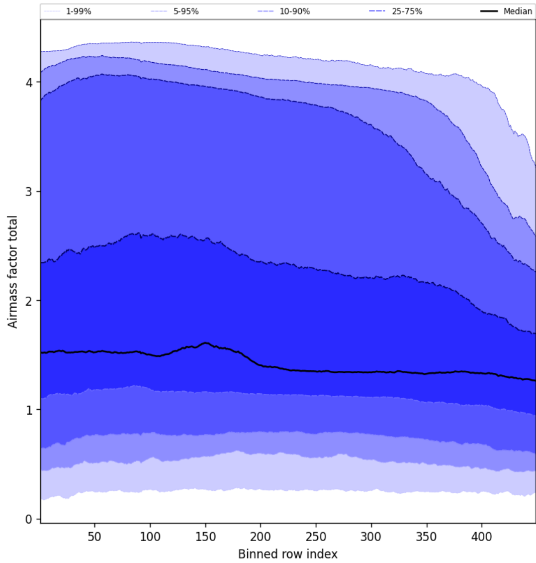
Figure 52: Along track statistics of “Airmass factor total” for 2025-01-17 to 2025-01-18
