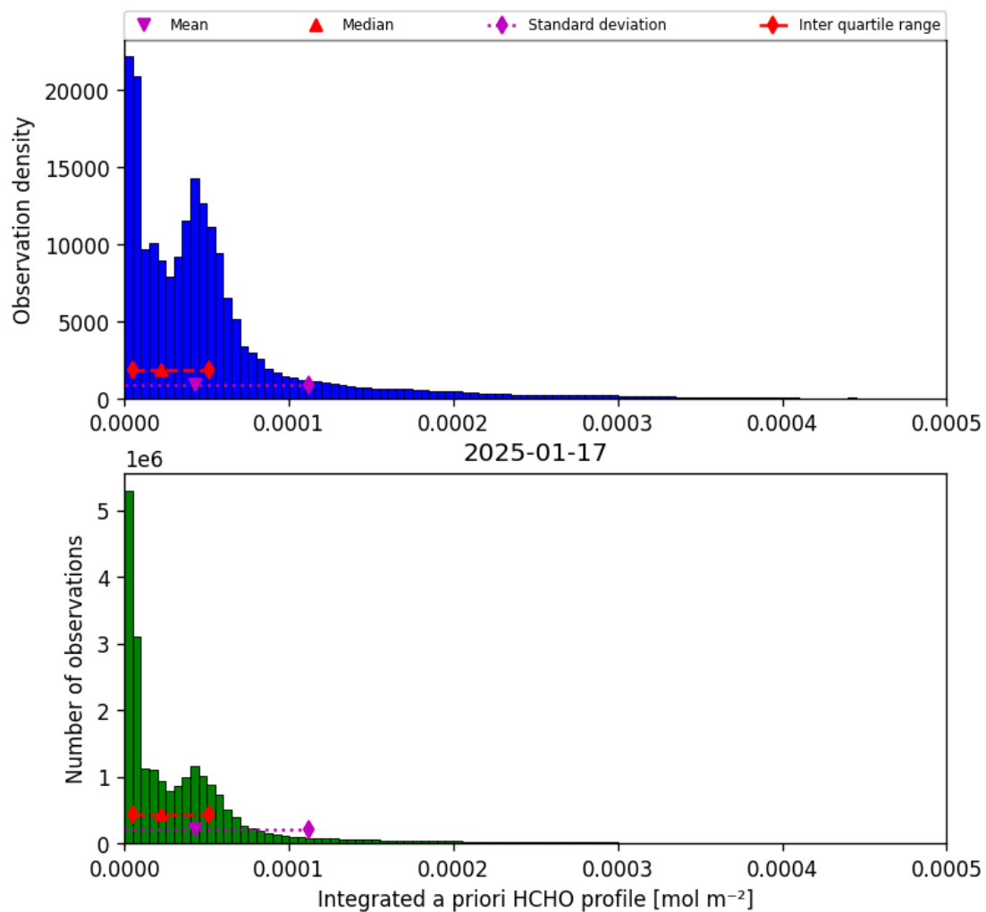
Figure 41: Histogram of “Integrated a priori HCHO profile” for 2025-01-17 to 2025-01-18
