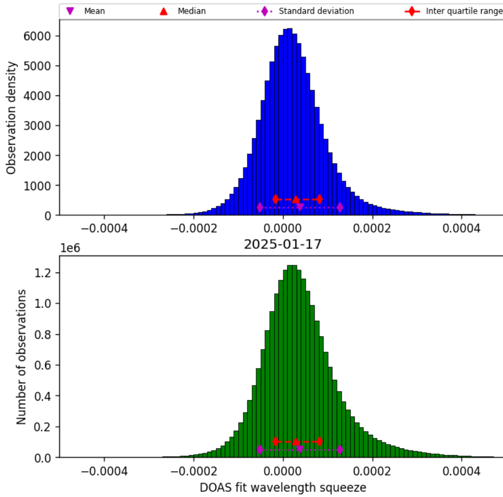
Figure 43: Histogram of “DOAS fit wavelength squeeze” for 2025-01-17 to 2025-01-18
