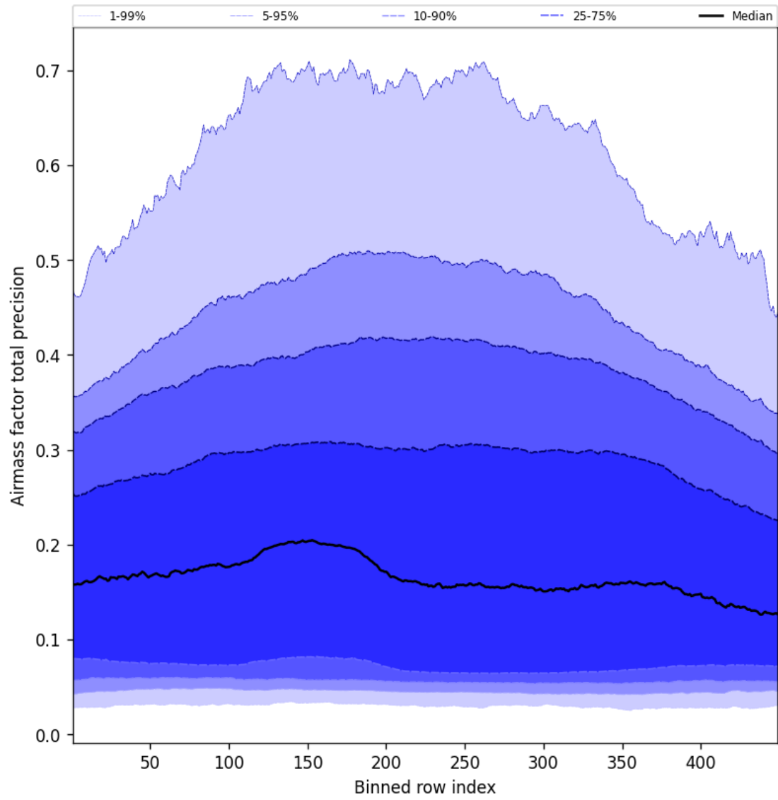
Figure 53: Along track statistics of “Airmass factor total precision” for 2025-01-17 to 2025-01-18
