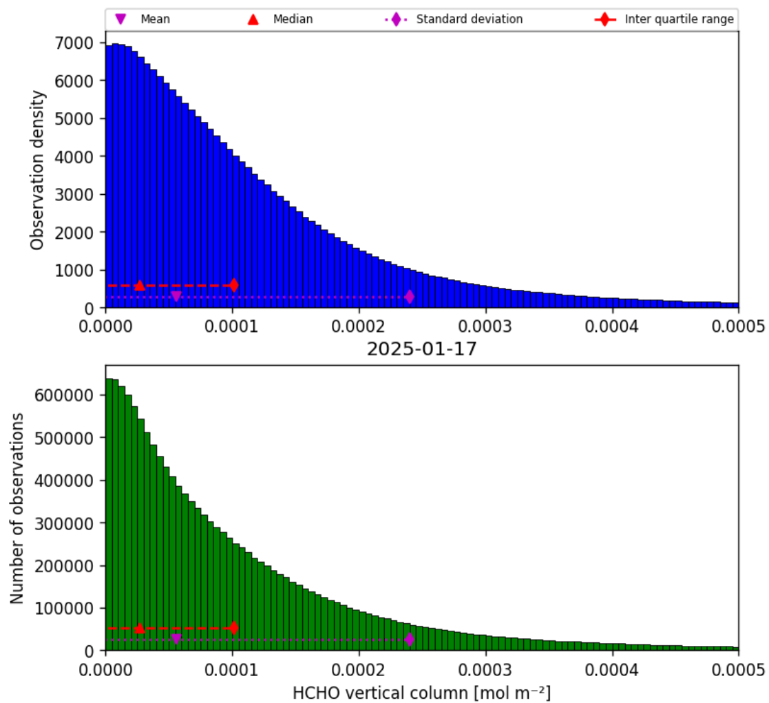
Figure 33: Histogram of “HCHO vertical column” for 2025-01-17 to 2025-01-18
