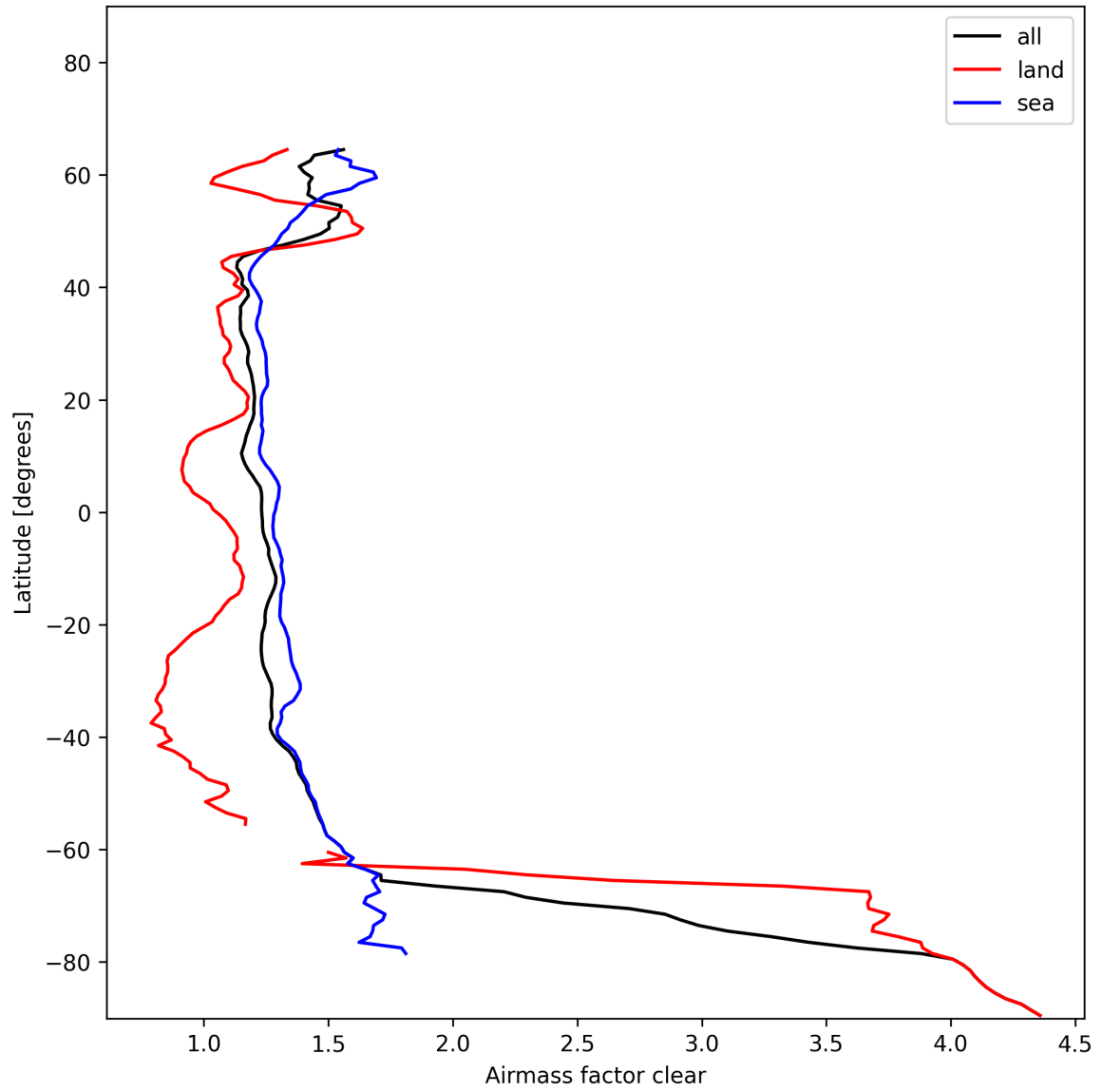
Figure 26: Zonal average of “Airmass factor clear” for 2025-01-17 to 2025-01-18.
