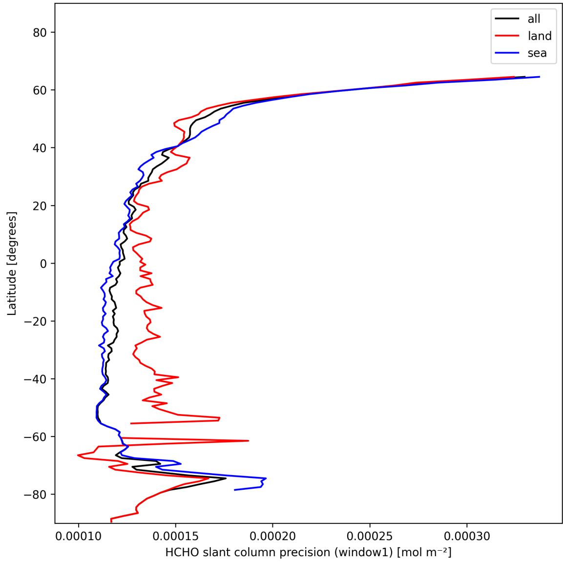
Figure 23: Zonal average of "HCHO slant column precision (window1)" for 2025-01-17 to 2025-01-18.
