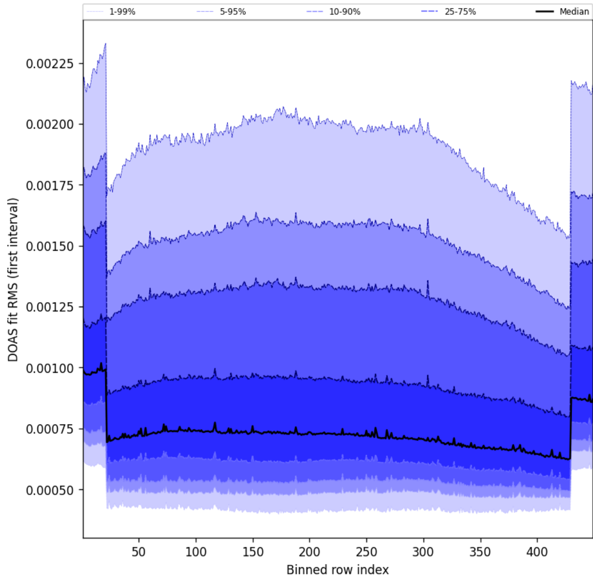
Figure 58: Along track statistics of “DOAS fit RMS (first interval)” for 2025-01-17 to 2025-01-18
