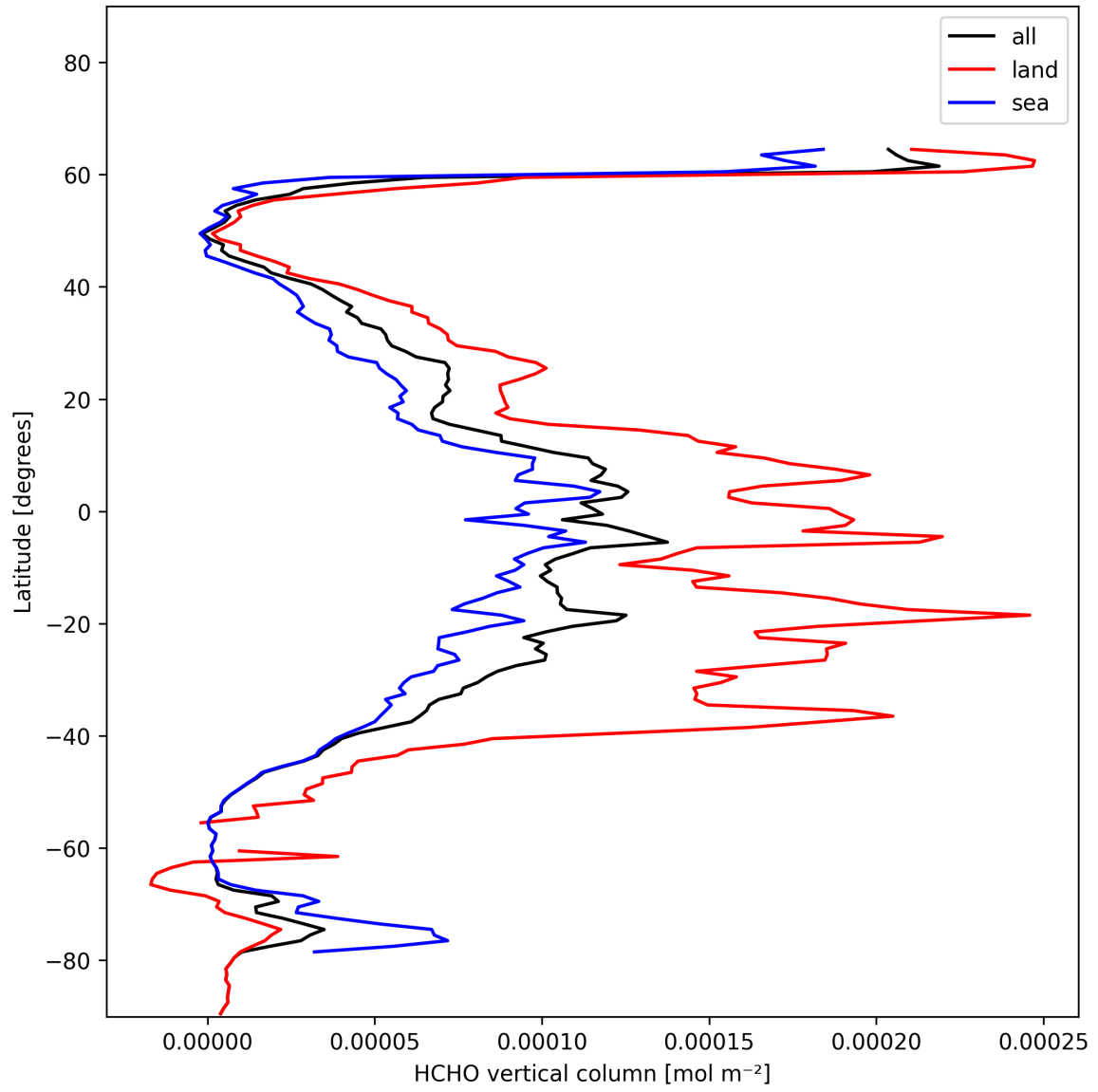
Figure 19: Zonal average of “HCHO vertical column” for 2025-01-17 to 2025-01-18.
