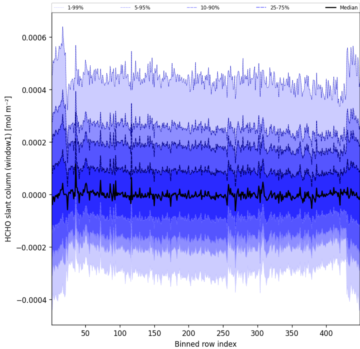
Figure 50: Along track statistics of “HCHO slant column (window1)” for 2025-01-17 to 2025-01-18
