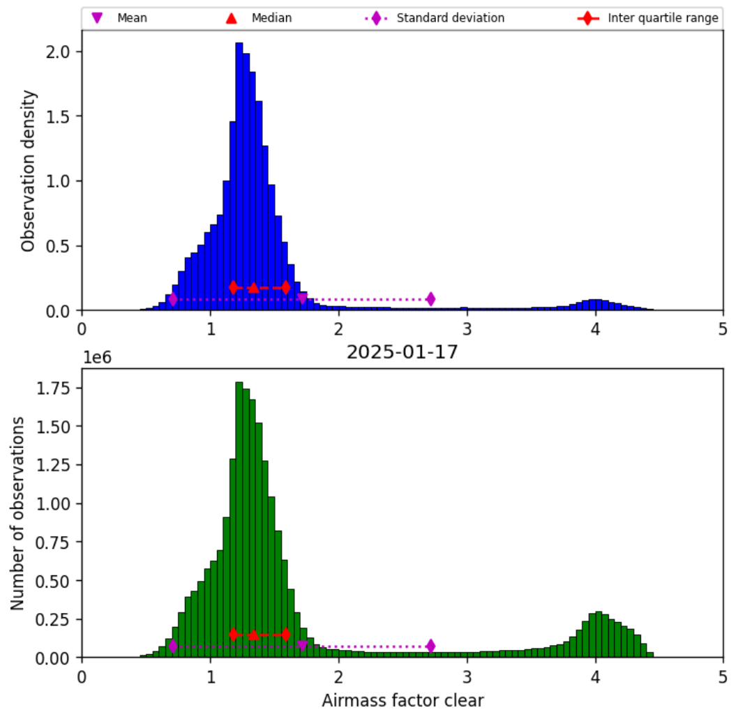
Figure 40: Histogram of “Airmass factor clear” for 2025-01-17 to 2025-01-18
