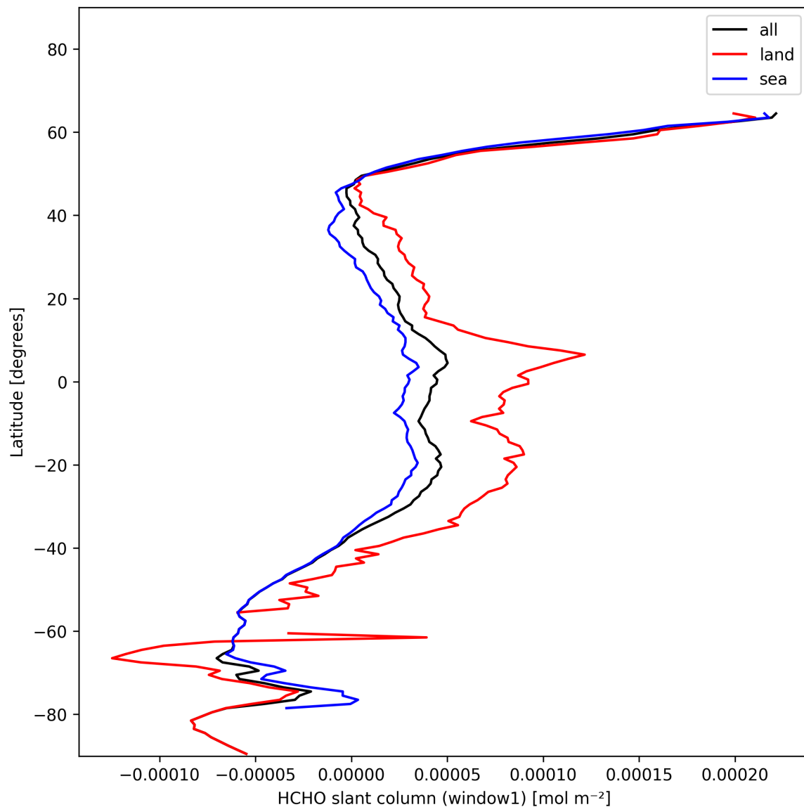
Figure 22: Zonal average of “HCHO slant column (window1)” for 2025-01-17 to 2025-01-18.
