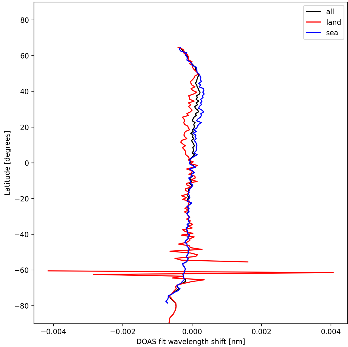
Figure 28: Zonal average of “DOAS fit wavelength shift” for 2025-01-17 to 2025-01-18.
