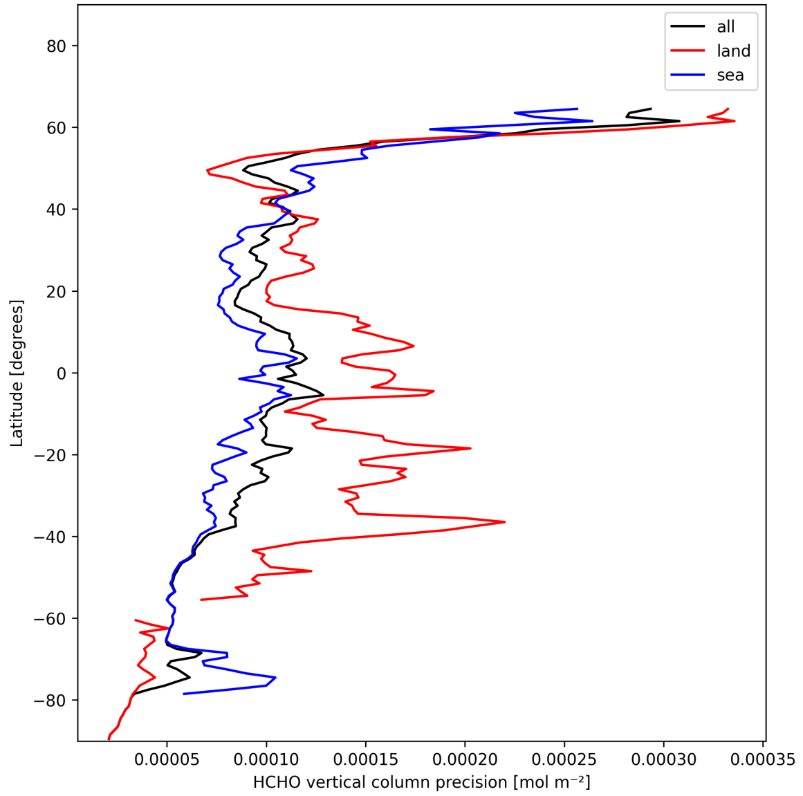
Figure 20: Zonal average of “HCHO vertical column precision” for 2025-01-17 to 2025-01-18.
