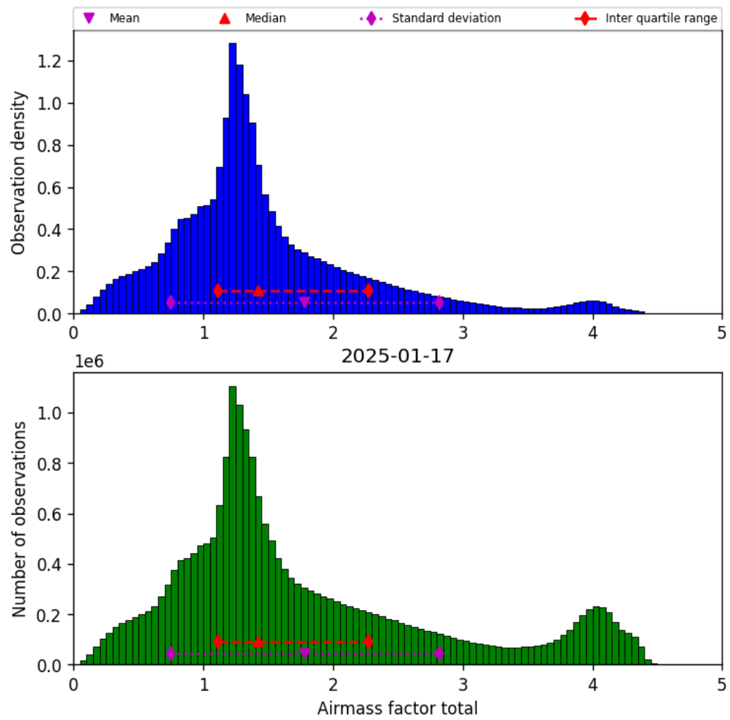
Figure 38: Histogram of “Airmass factor total” for 2025-01-17 to 2025-01-18
