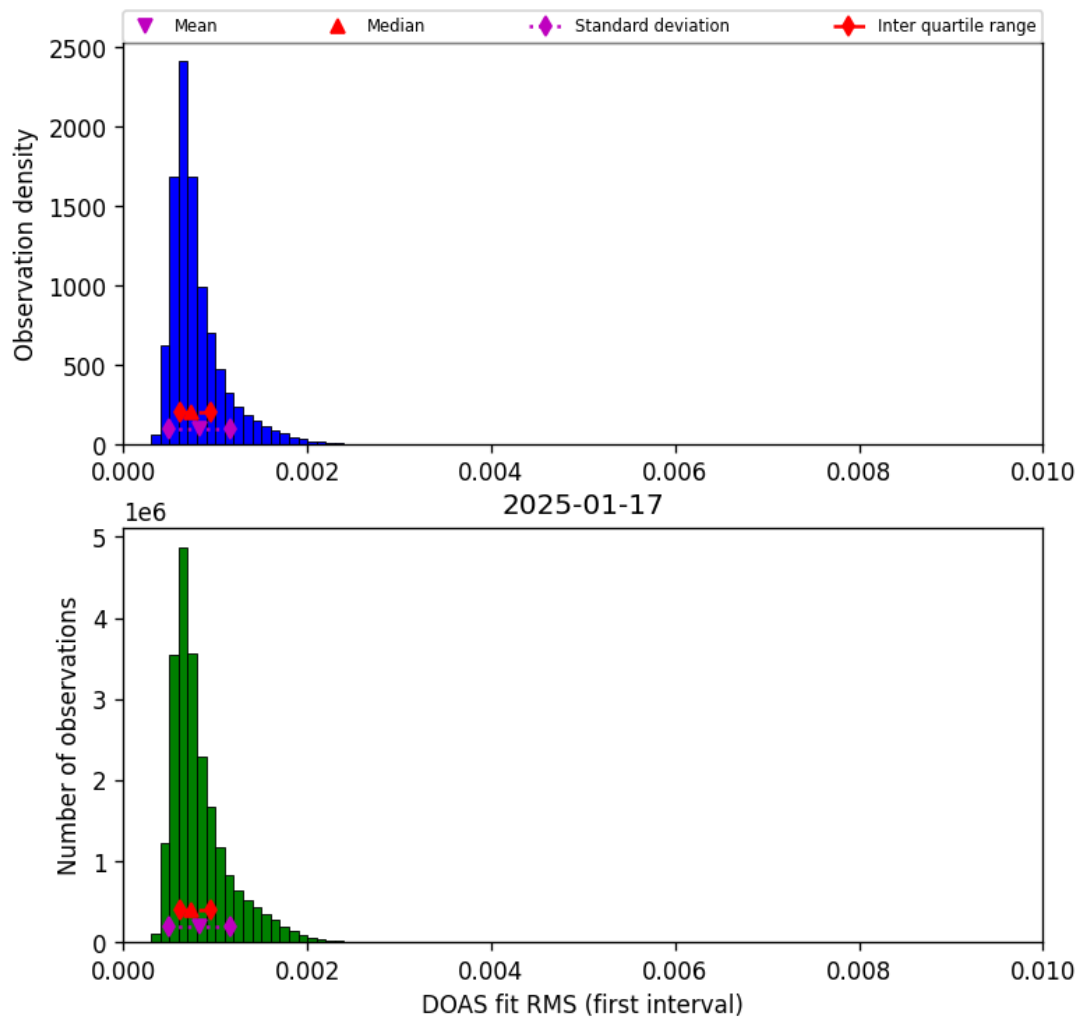
Figure 44: Histogram of “DOAS fit RMS (first interval)” for 2025-01-17 to 2025-01-18
