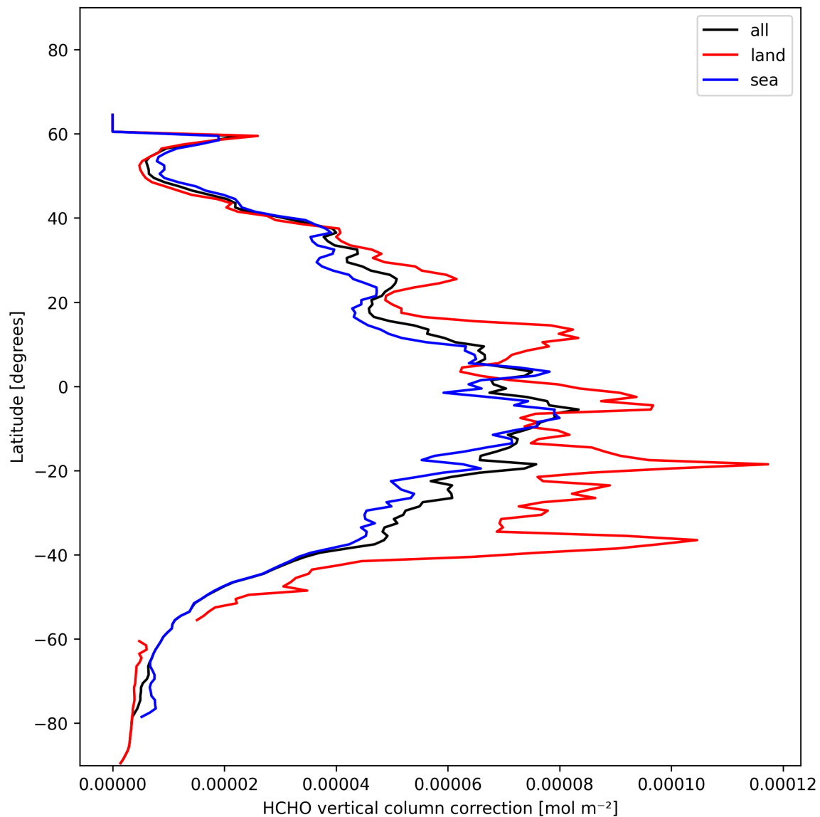
Figure 21: Zonal average of “HCHO vertical column correction” for 2025-01-17 to 2025-01-18.
