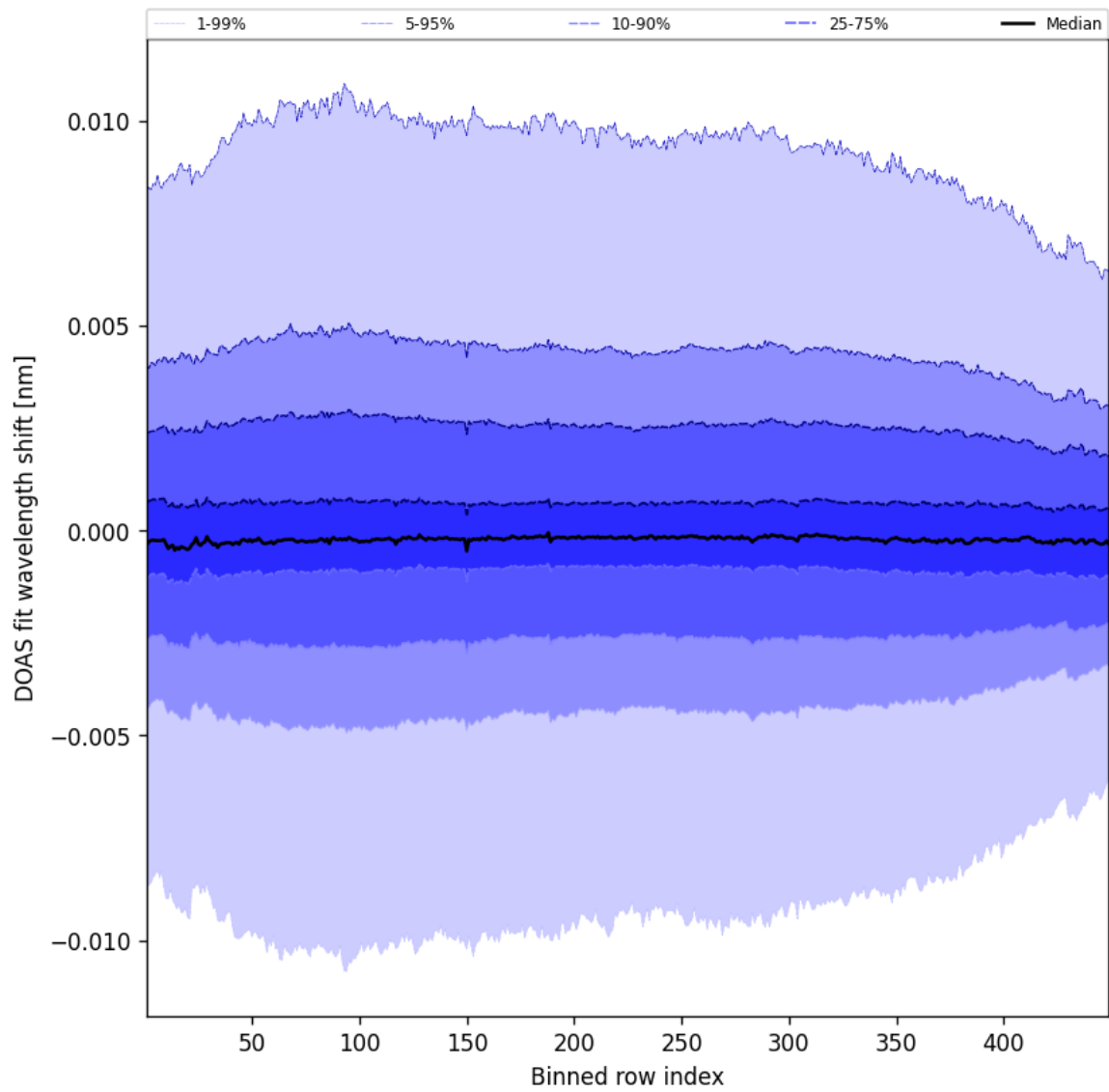
Figure 56: Along track statistics of “DOAS fit wavelength shift” for 2025-01-17 to 2025-01-18
