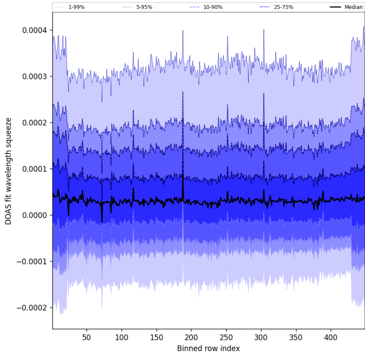
Figure 57: Along track statistics of “DOAS fit wavelength squeeze” for 2025-01-17 to 2025-01-18
