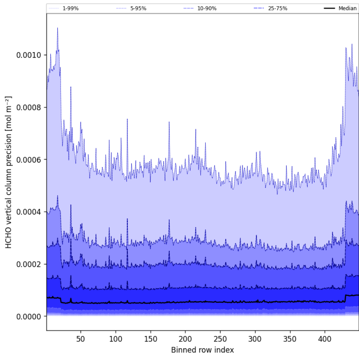
Figure 48: Along track statistics of “HCHO vertical column precision” for 2025-01-18 to 2025-01-19
