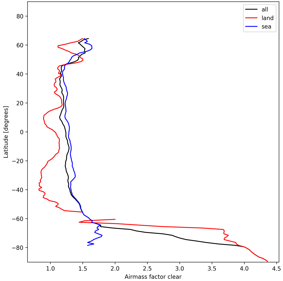
Figure 26: Zonal average of “Airmass factor clear” for 2025-01-18 to 2025-01-19.
