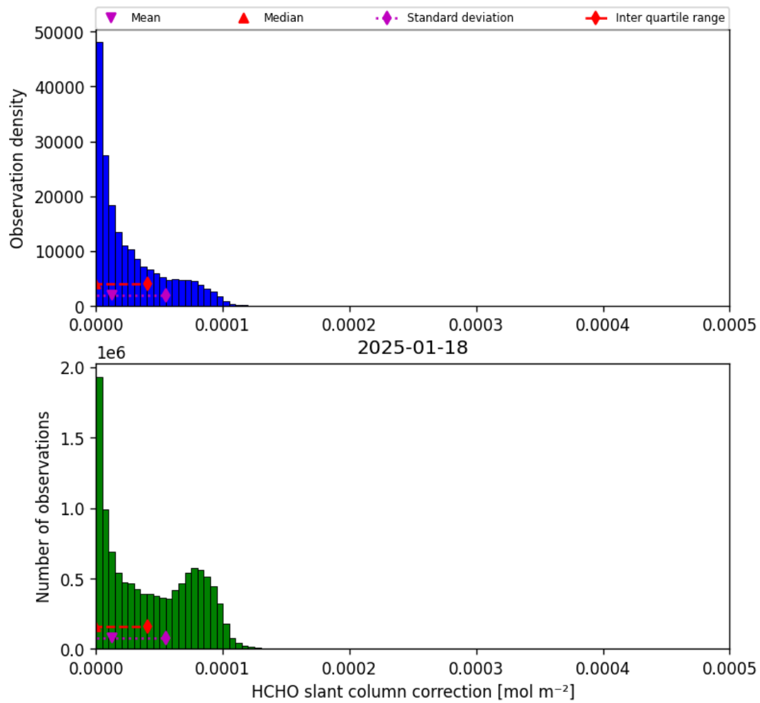
Figure 45: Histogram of “HCHO slant column correction” for 2025-01-18 to 2025-01-19
