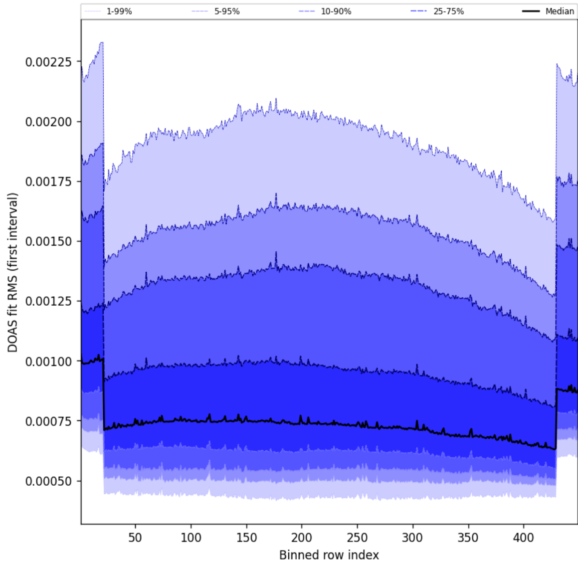
Figure 58: Along track statistics of “DOAS fit RMS (first interval)” for 2025-01-18 to 2025-01-19
