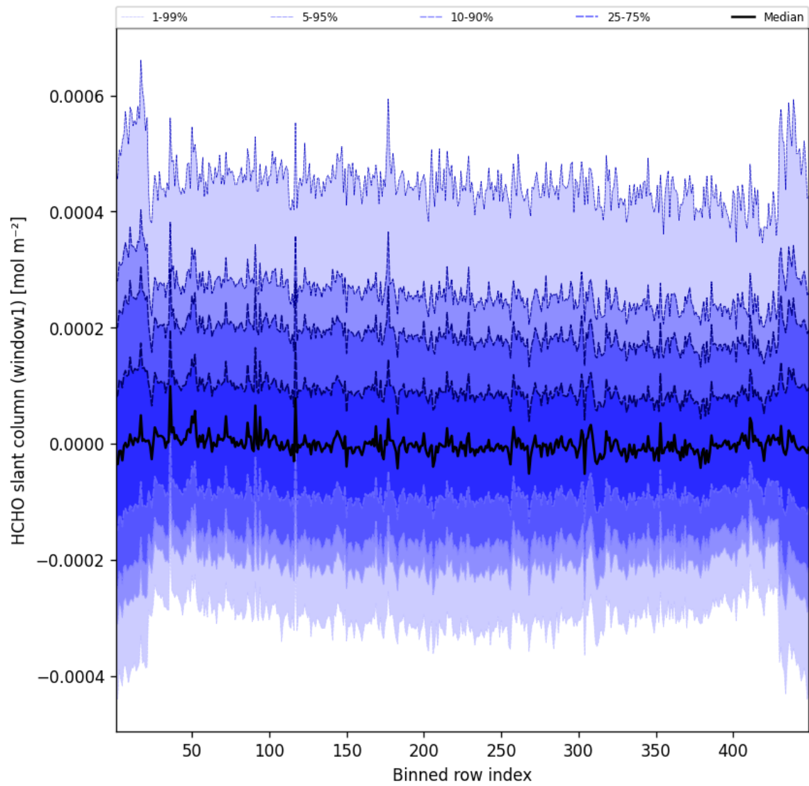
Figure 50: Along track statistics of “HCHO slant column (window1)” for 2025-01-18 to 2025-01-19
