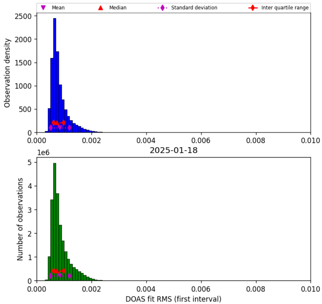
Figure 44: Histogram of “DOAS fit RMS (first interval)” for 2025-01-18 to 2025-01-19
