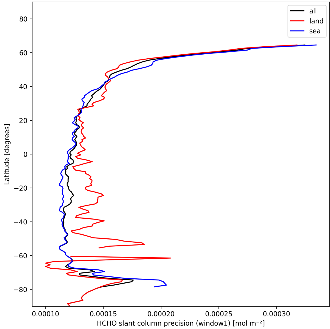
Figure 23: Zonal average of “HCHO slant column precision (window1)” for 2025-01-18 to 2025-01-19.
