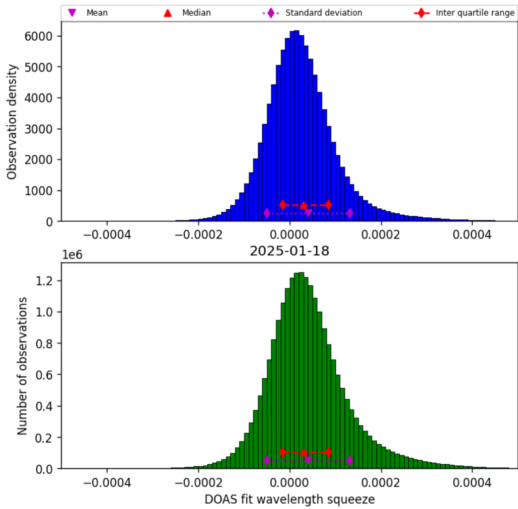
Figure 43: Histogram of “DOAS fit wavelength squeeze” for 2025-01-18 to 2025-01-19
