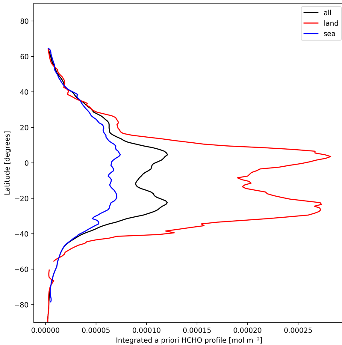
Figure 27: Zonal average of “Integrated a priori HCHO profile” for 2025-01-18 to 2025-01-19.
