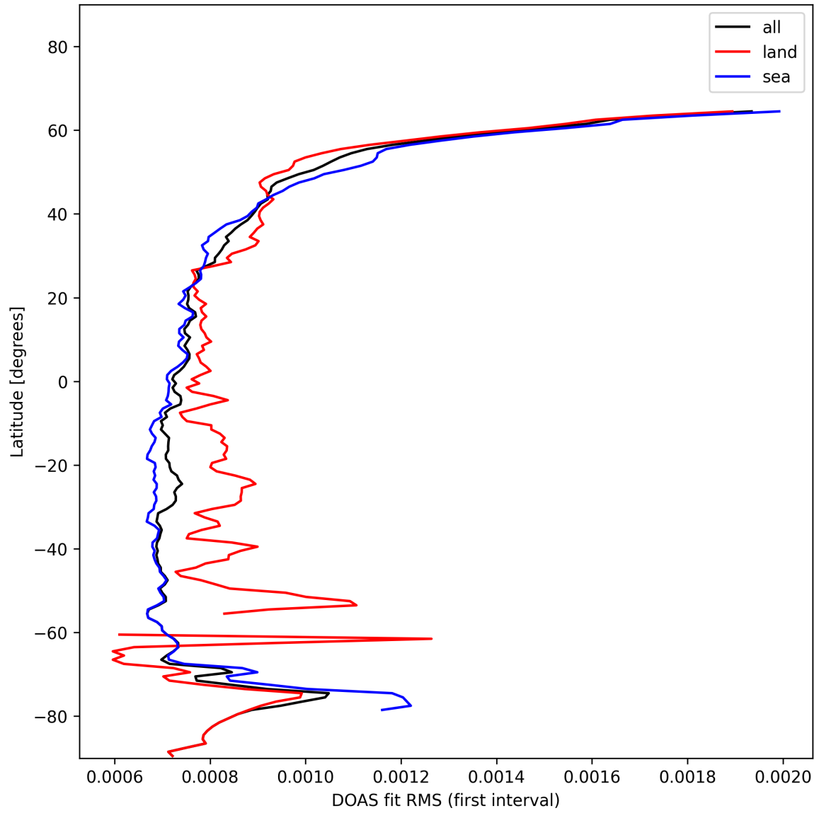
Figure 30: Zonal average of "DOAS fit RMS (first interval)" for 2025-01-18 to 2025-01-19.
