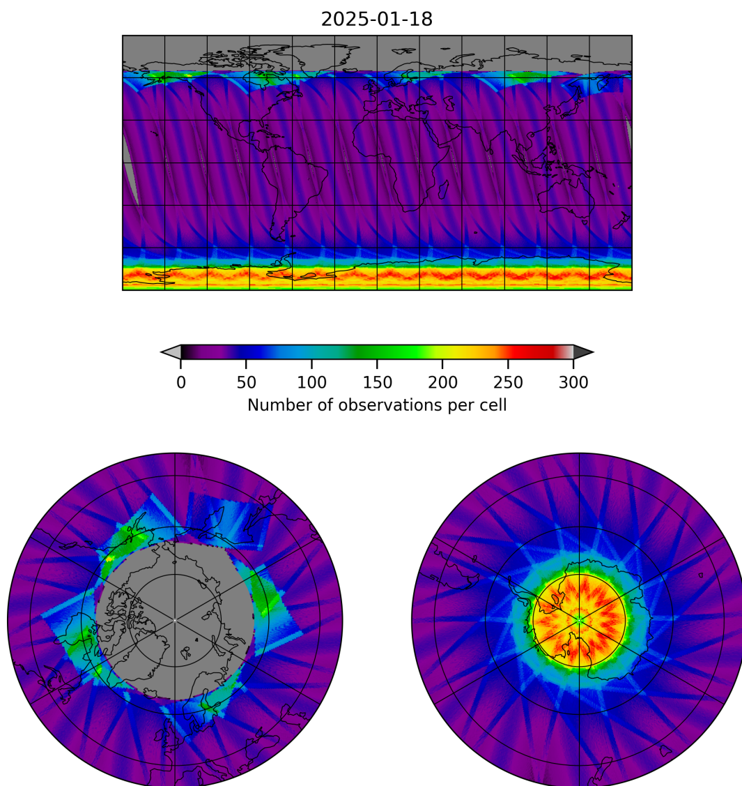
Figure 17: Map of the number of observations for 2025-01-18 to 2025-01-19
