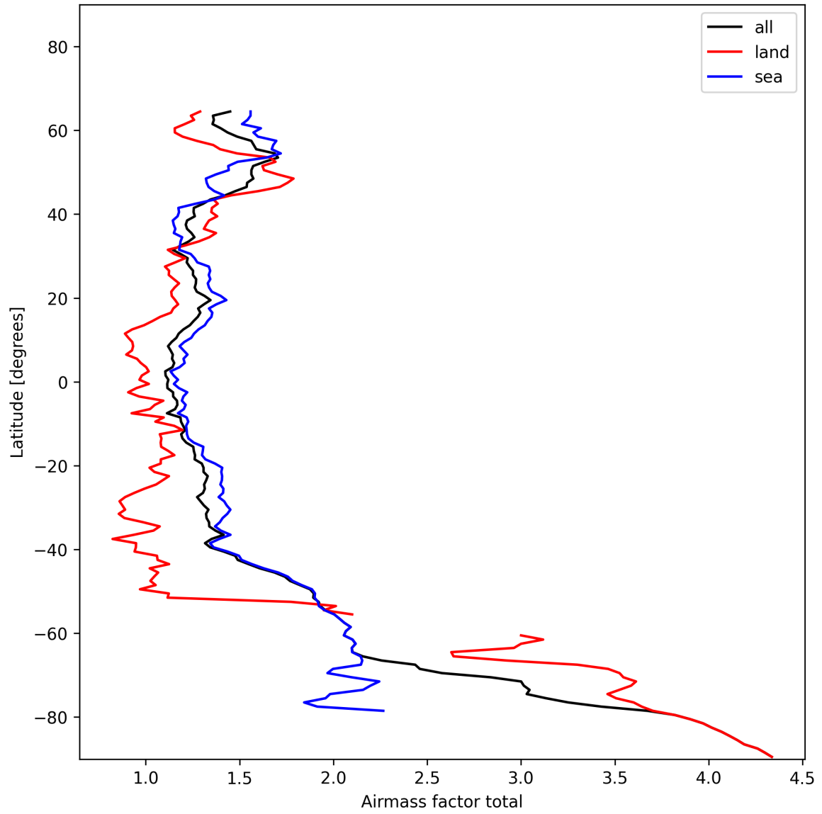
Figure 24: Zonal average of “Airmass factor total” for 2025-01-18 to 2025-01-19.
