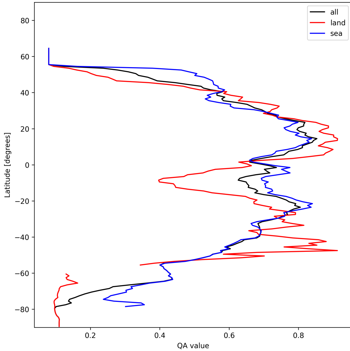
Figure 18: Zonal average of “QA value” for 2025-01-18 to 2025-01-19.
