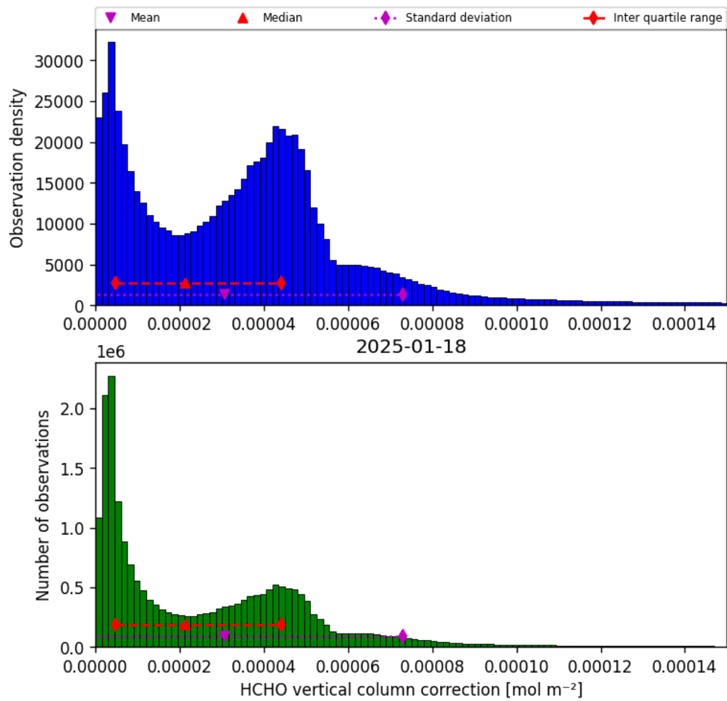
Figure 35: Histogram of “HCHO vertical column correction” for 2025-01-18 to 2025-01-19
