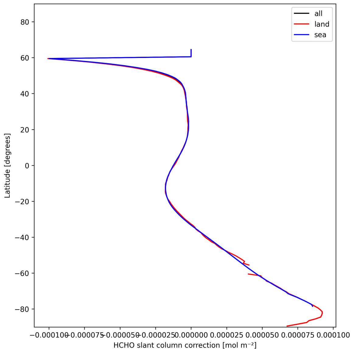
Figure 31: Zonal average of “HCHO slant column correction” for 2025-01-18 to 2025-01-19.
