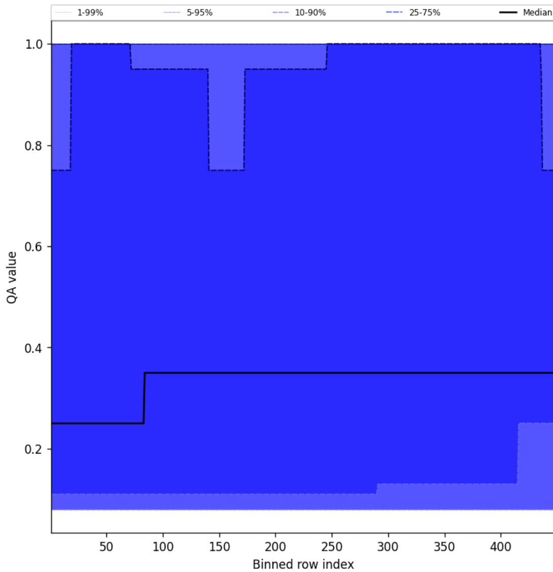
Figure 46: Along track statistics of “QA value” for 2025-01-18 to 2025-01-19
