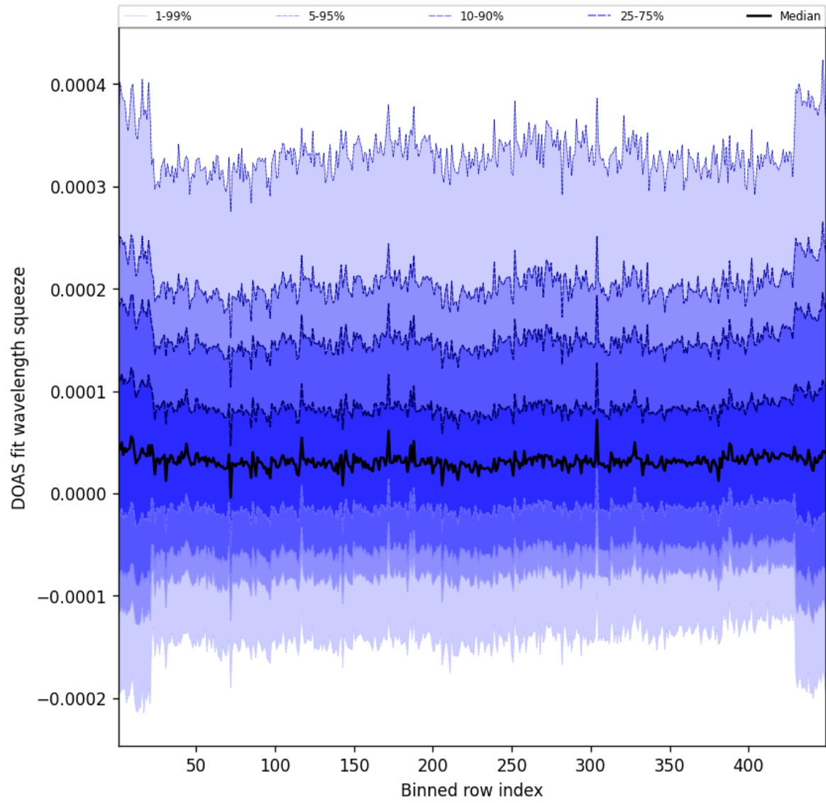
Figure 57: Along track statistics of “DOAS fit wavelength squeeze” for 2025-01-18 to 2025-01-19
