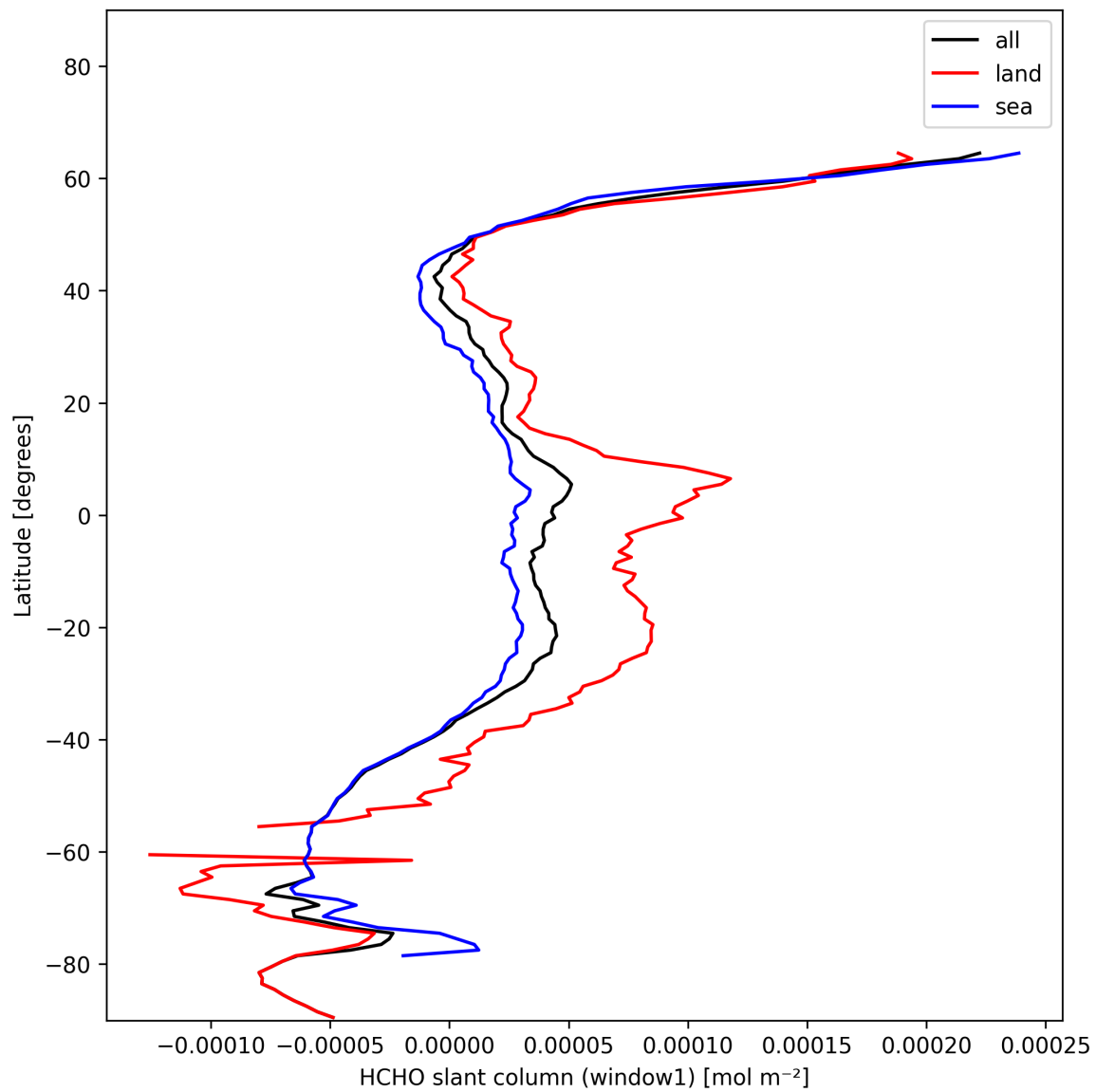
Figure 22: Zonal average of “HCHO slant column (window1)” for 2025-01-18 to 2025-01-19.
