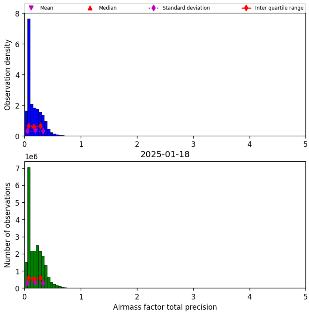
Figure 39: Histogram of “Airmass factor total precision” for 2025-01-18 to 2025-01-19
