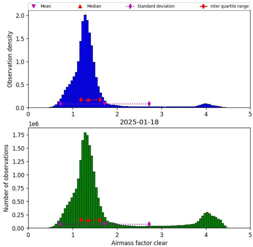
Figure 40: Histogram of “Airmass factor clear” for 2025-01-18 to 2025-01-19
