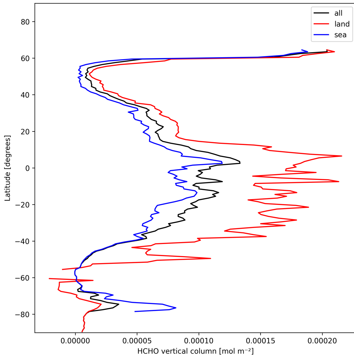
Figure 19: Zonal average of “HCHO vertical column” for 2025-01-18 to 2025-01-19.
