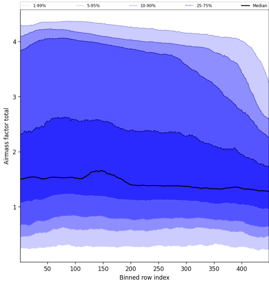
Figure 52: Along track statistics of “Airmass factor total” for 2025-01-18 to 2025-01-19
