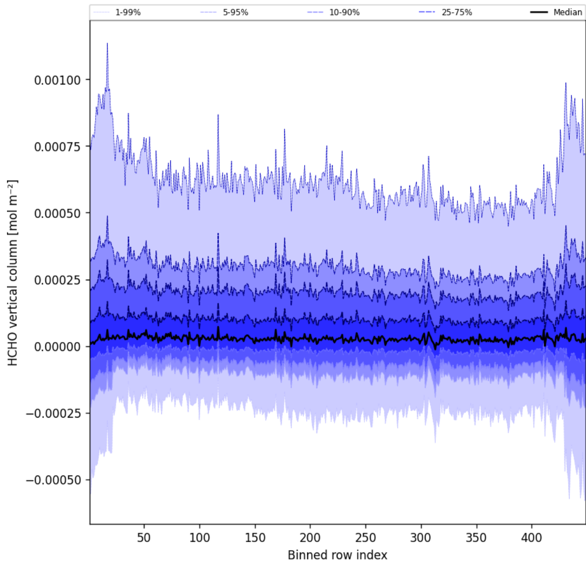
Figure 47: Along track statistics of “HCHO vertical column” for 2025-01-18 to 2025-01-19
