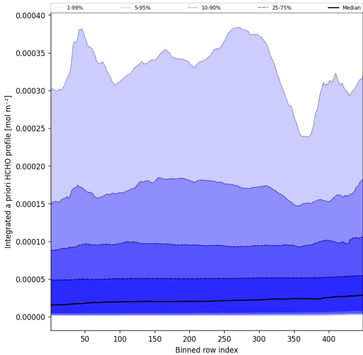
Figure 55: Along track statistics of "Integrated a priori HCHO profile" for 2025-01-18 to 2025-01-19
