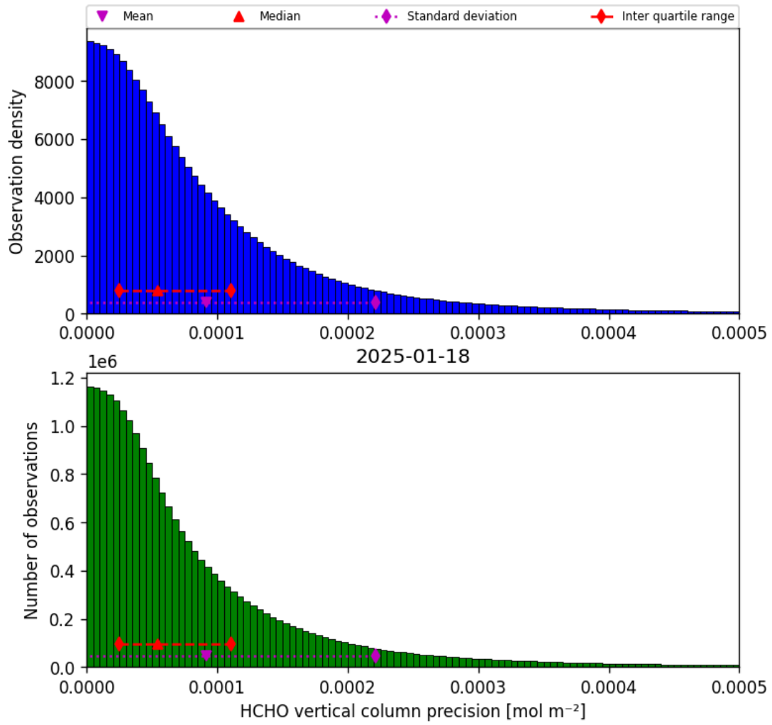
Figure 34: Histogram of “HCHO vertical column precision” for 2025-01-18 to 2025-01-19
