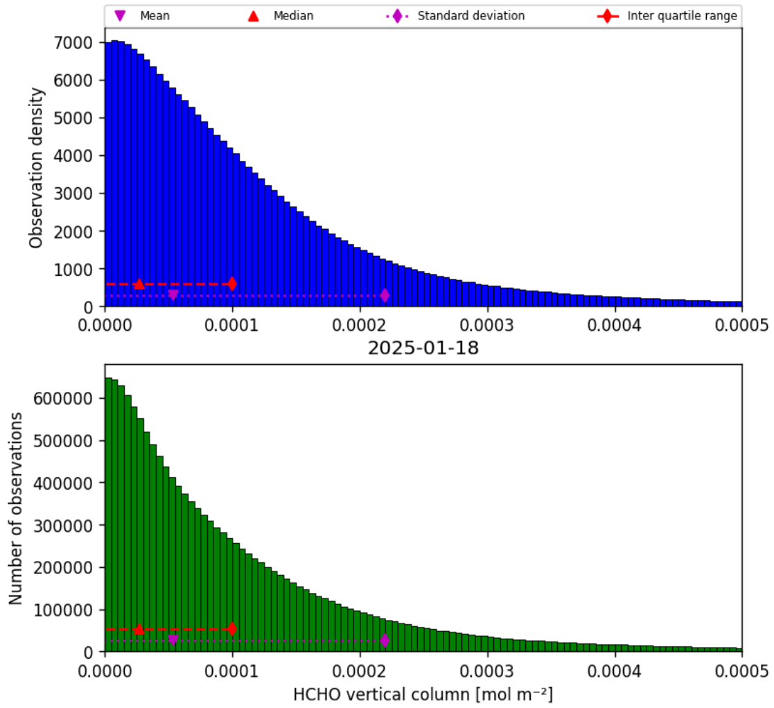
Figure 33: Histogram of “HCHO vertical column” for 2025-01-18 to 2025-01-19
