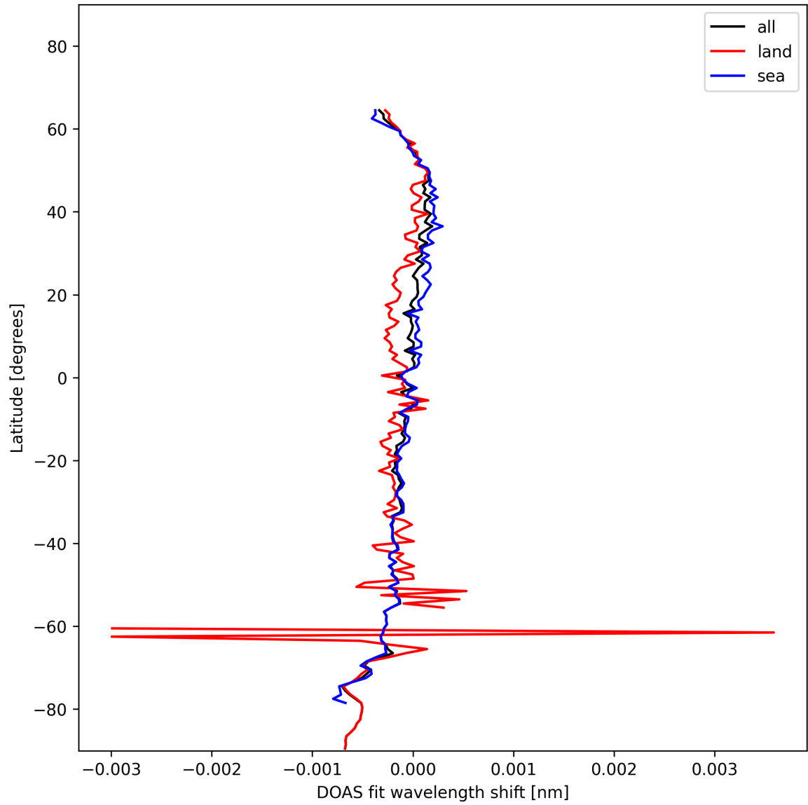
Figure 28: Zonal average of “DOAS fit wavelength shift” for 2025-01-18 to 2025-01-19.
