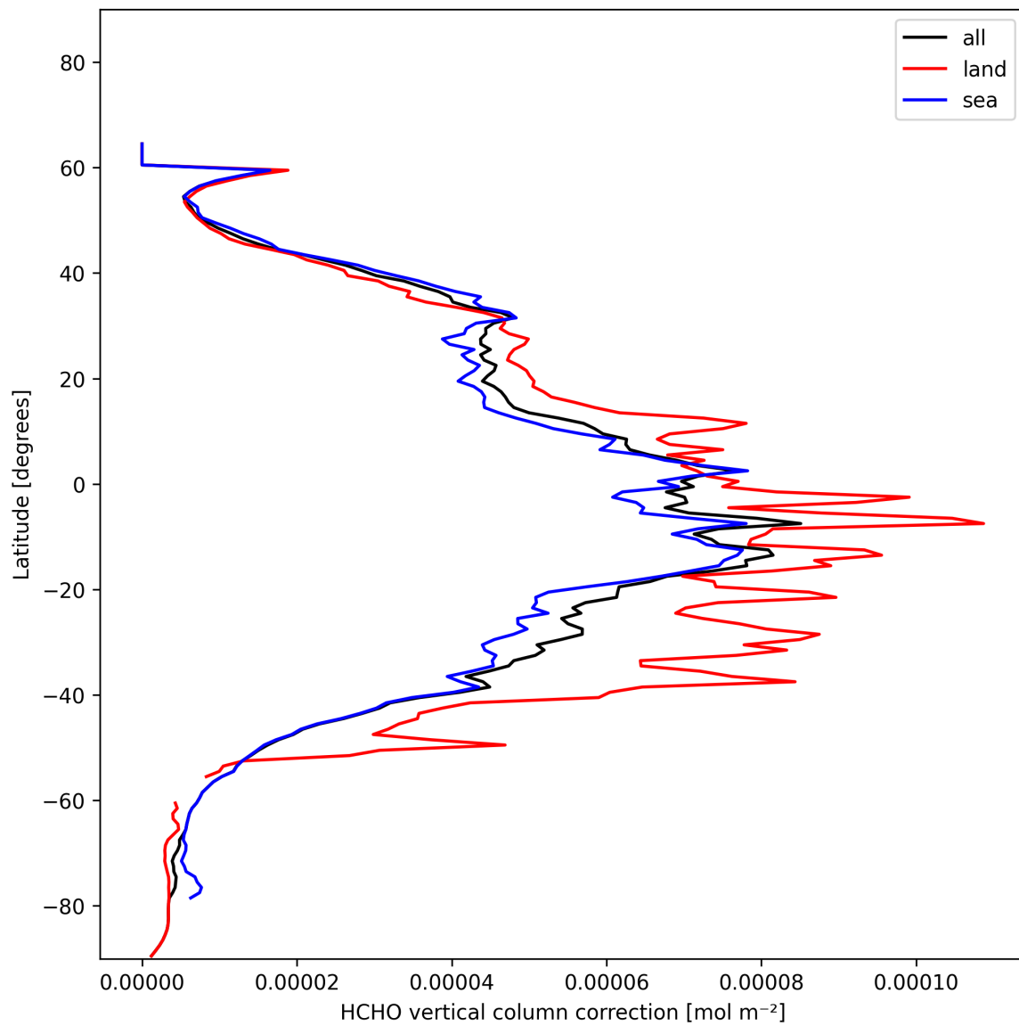
Figure 21: Zonal average of “HCHO vertical column correction” for 2025-01-18 to 2025-01-19.
