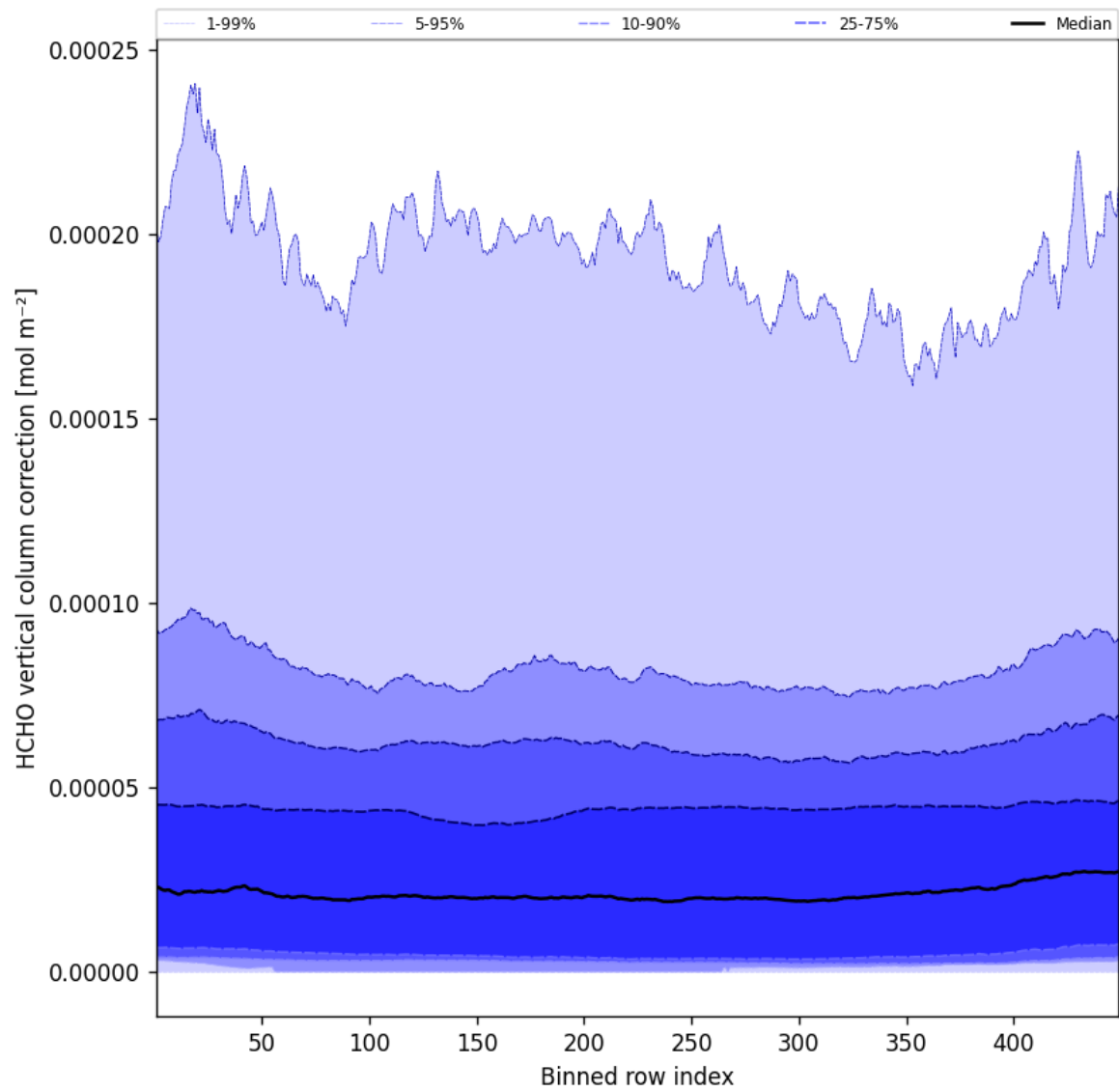
Figure 49: Along track statistics of “HCHO vertical column correction” for 2025-01-18 to 2025-01-19
