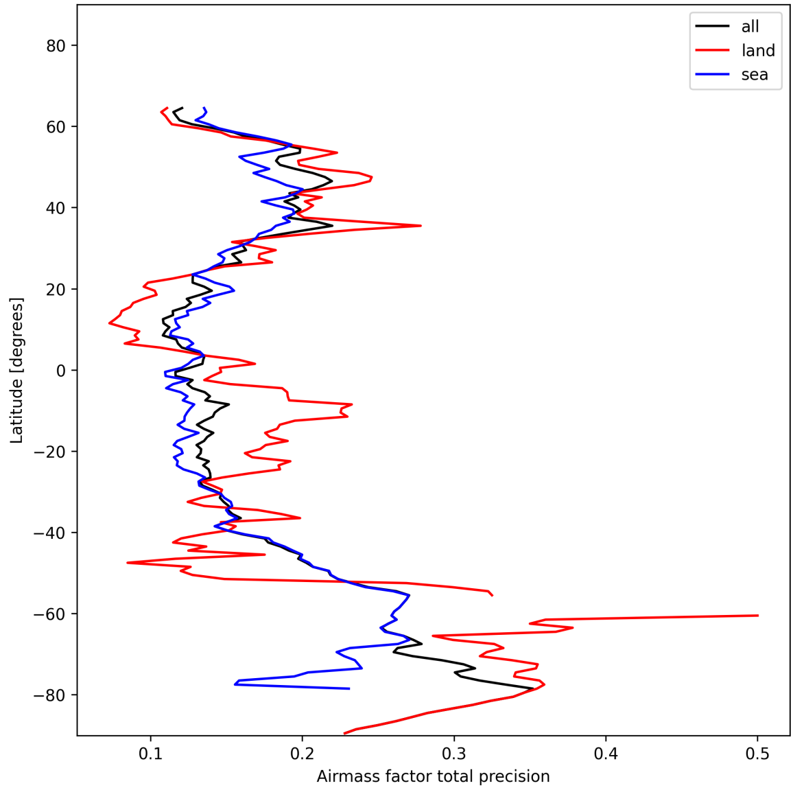
Figure 25: Zonal average of “Airmass factor total precision” for 2025-01-18 to 2025-01-19.
