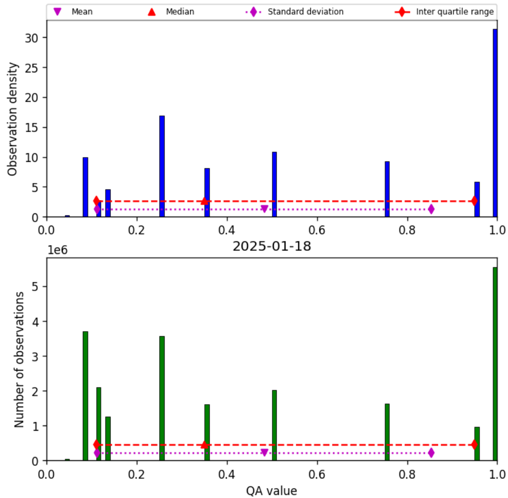
Figure 32: Histogram of “QA value” for 2025-01-18 to 2025-01-19
