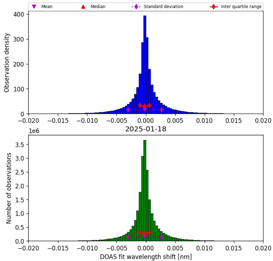
Figure 42: Histogram of “DOAS fit wavelength shift” for 2025-01-18 to 2025-01-19
