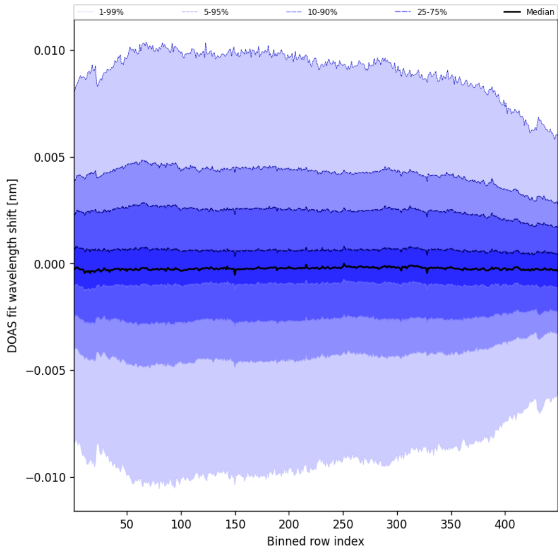
Figure 56: Along track statistics of “DOAS fit wavelength shift” for 2025-01-18 to 2025-01-19
