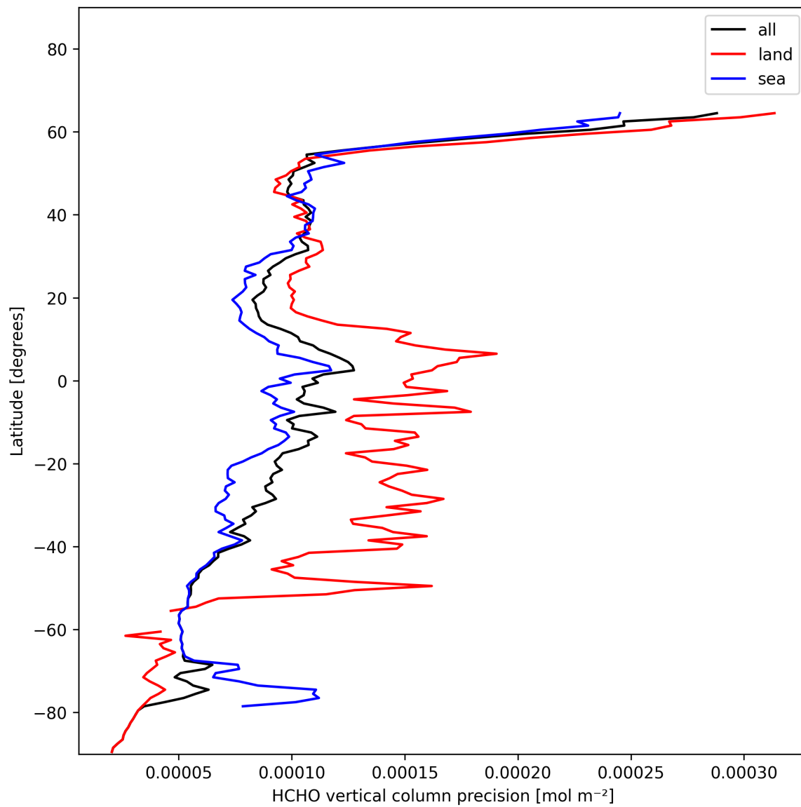
Figure 20: Zonal average of “HCHO vertical column precision” for 2025-01-18 to 2025-01-19.
