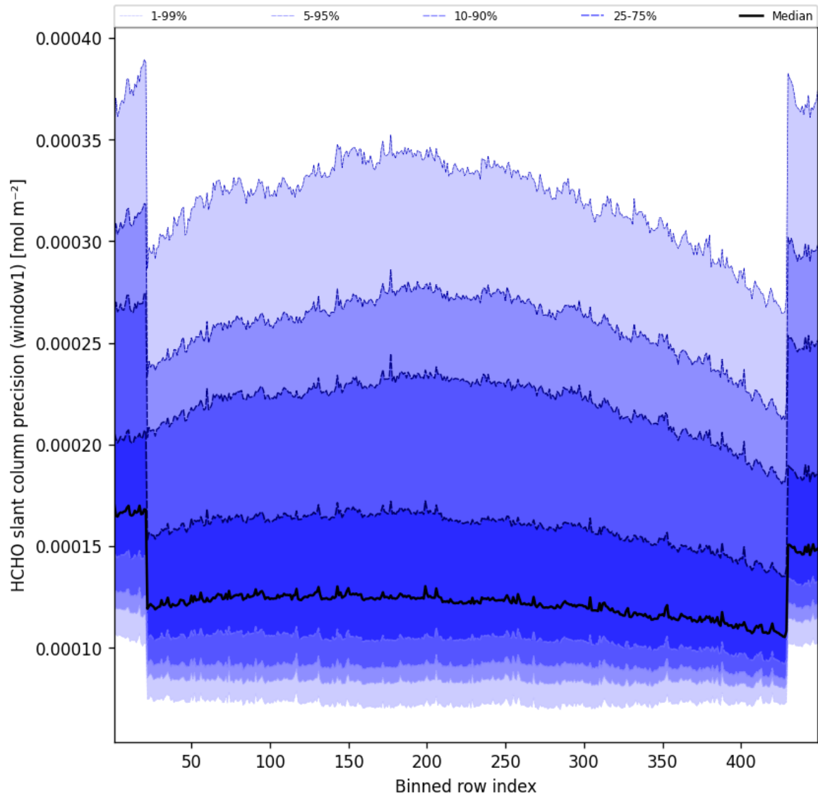
Figure 51: Along track statistics of “HCHO slant column precision (window1)” for 2025-01-18 to 2025-01-19
