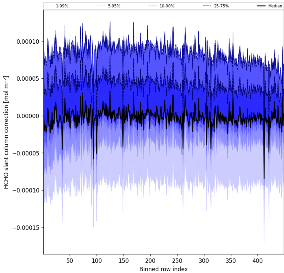
Figure 59: Along track statistics of “HCHO slant column correction” for 2025-01-18 to 2025-01-19
