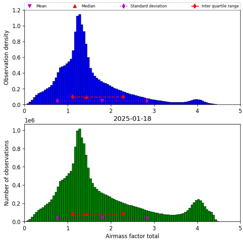
Figure 38: Histogram of “Airmass factor total” for 2025-01-18 to 2025-01-19
