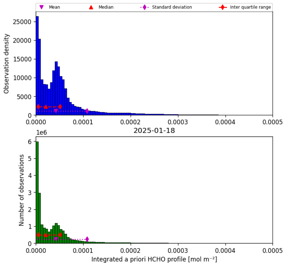
Figure 41: Histogram of “Integrated a priori HCHO profile” for 2025-01-18 to 2025-01-19
