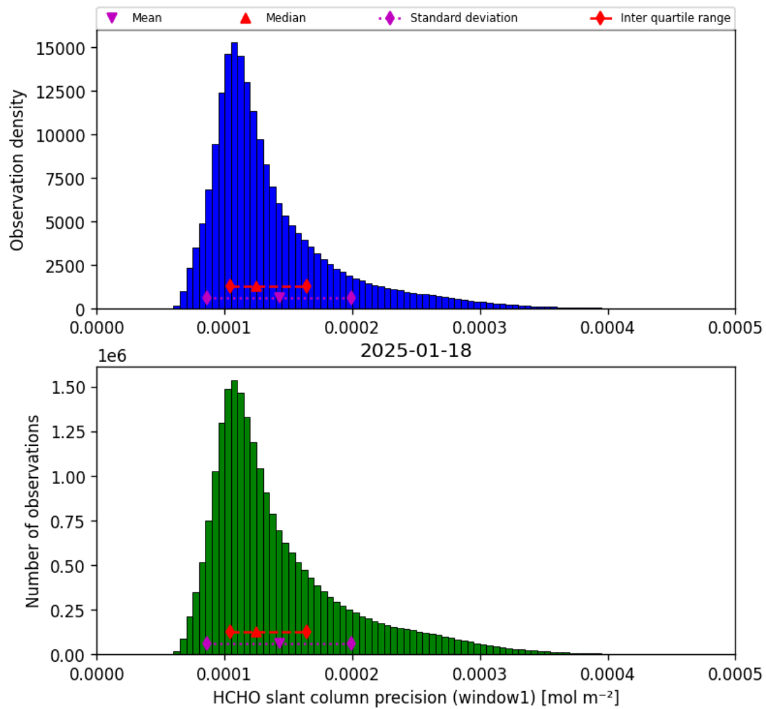
Figure 37: Histogram of “HCHO slant column precision (window1)” for 2025-01-18 to 2025-01-19
