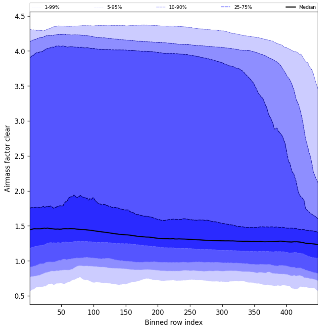
Figure 54: Along track statistics of “Airmass factor clear” for 2025-01-18 to 2025-01-19
