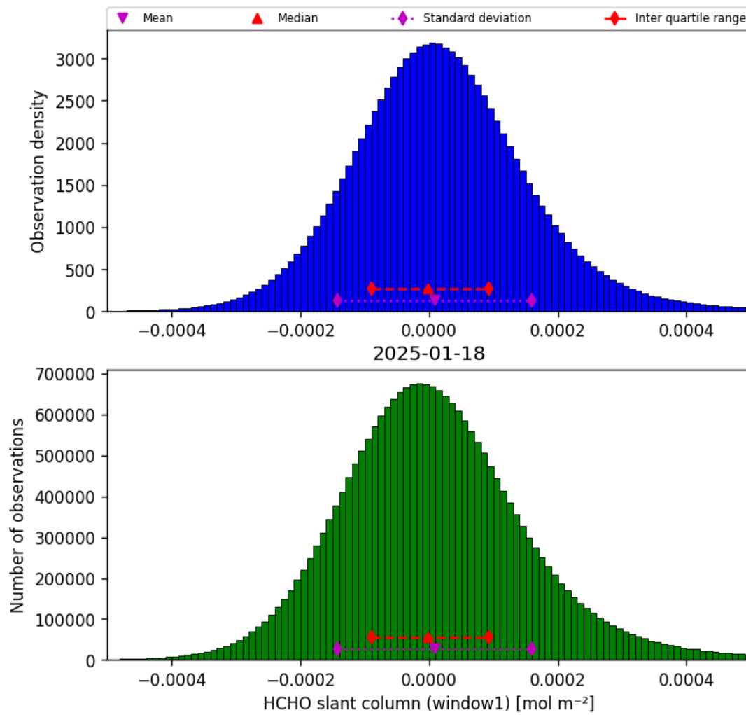
Figure 36: Histogram of “HCHO slant column (window1)” for 2025-01-18 to 2025-01-19
