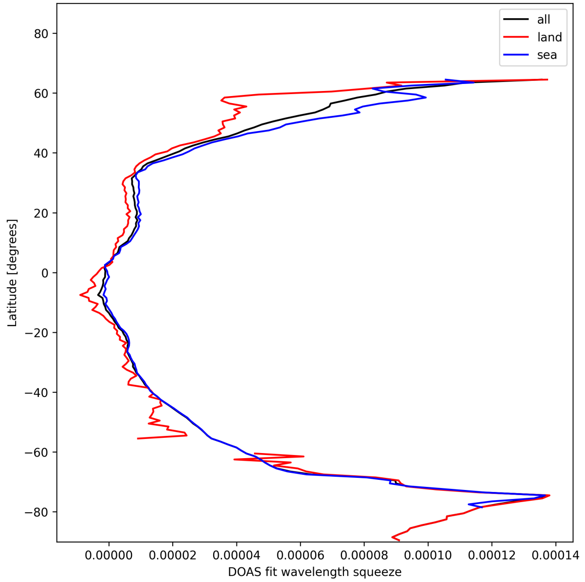
Figure 29: Zonal average of “DOAS fit wavelength squeeze” for 2025-01-18 to 2025-01-19.
