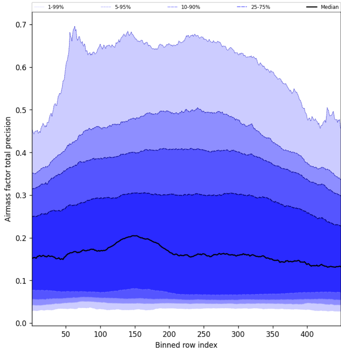
Figure 53: Along track statistics of “Airmass factor total precision” for 2025-01-18 to 2025-01-19
