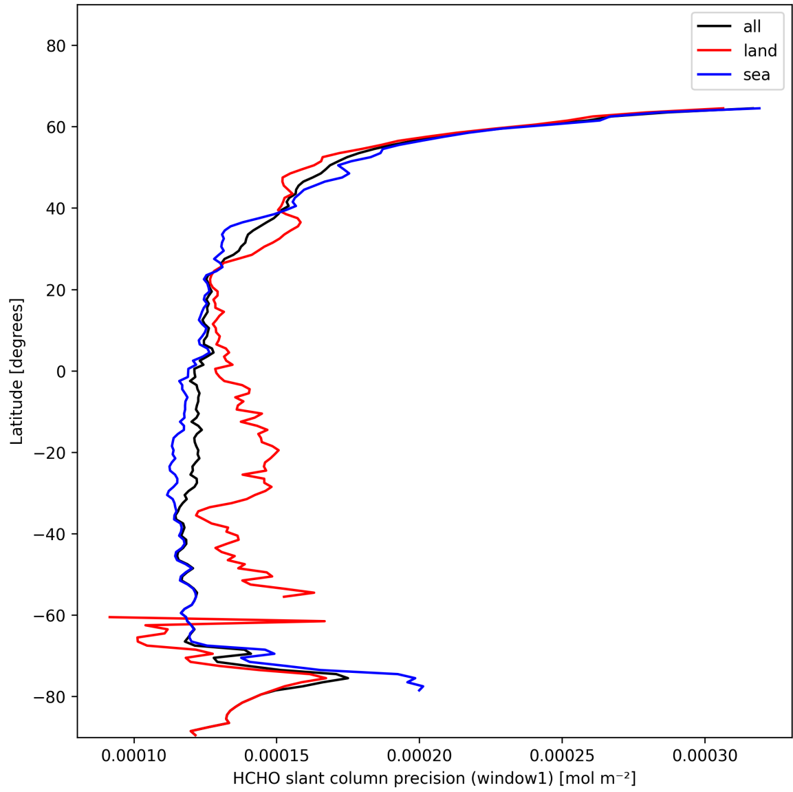
Figure 23: Zonal average of "HCHO slant column precision (window1)" for 2025-01-19 to 2025-01-20.
