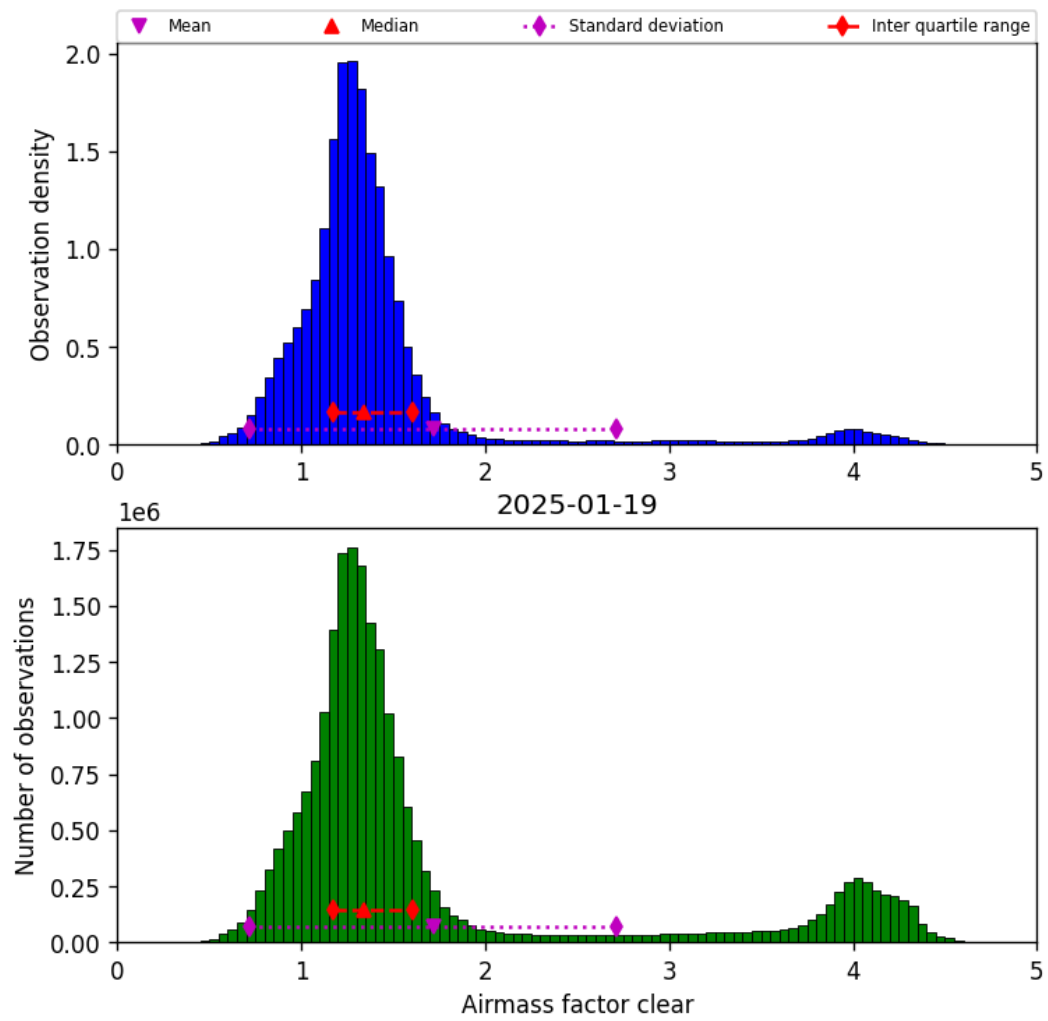
Figure 40: Histogram of “Airmass factor clear” for 2025-01-19 to 2025-01-20
