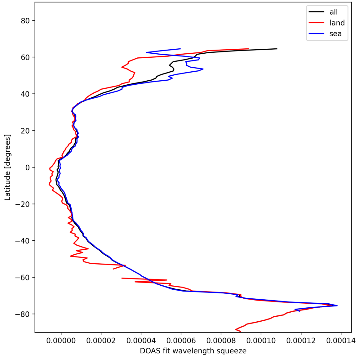
Figure 29: Zonal average of “DOAS fit wavelength squeeze” for 2025-01-19 to 2025-01-20.
