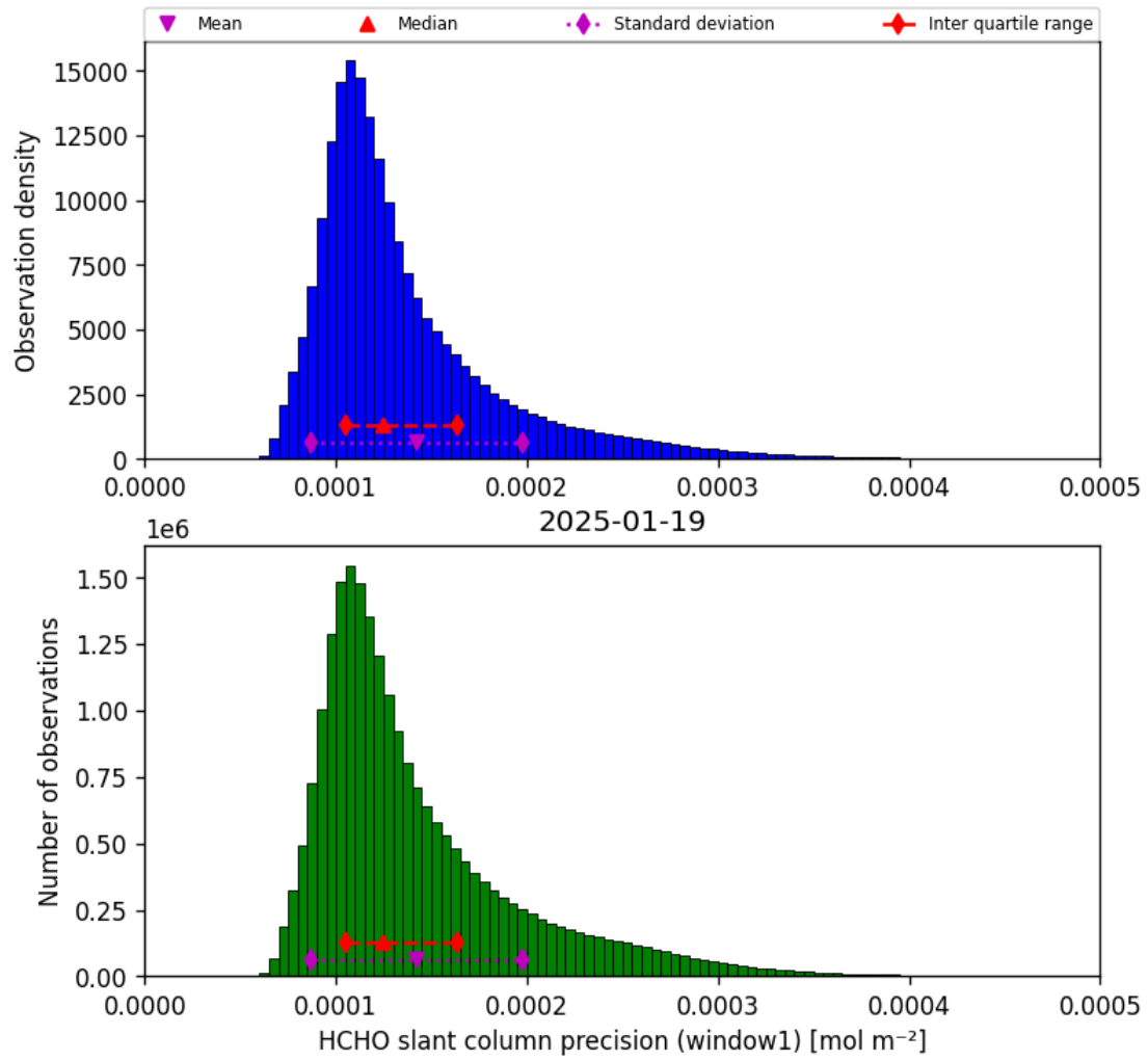
Figure 37: Histogram of “HCHO slant column precision (window1)” for 2025-01-19 to 2025-01-20
