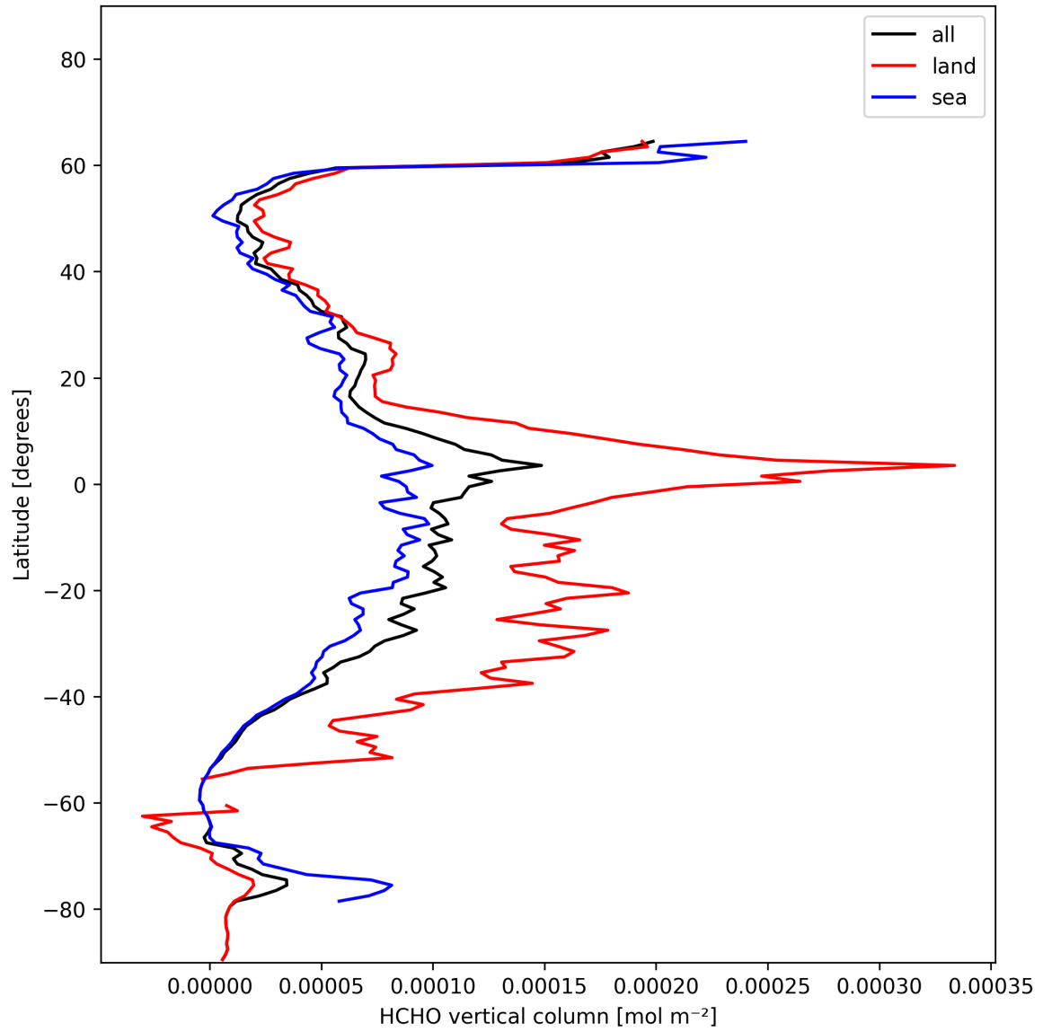
Figure 19: Zonal average of “HCHO vertical column” for 2025-01-19 to 2025-01-20.
