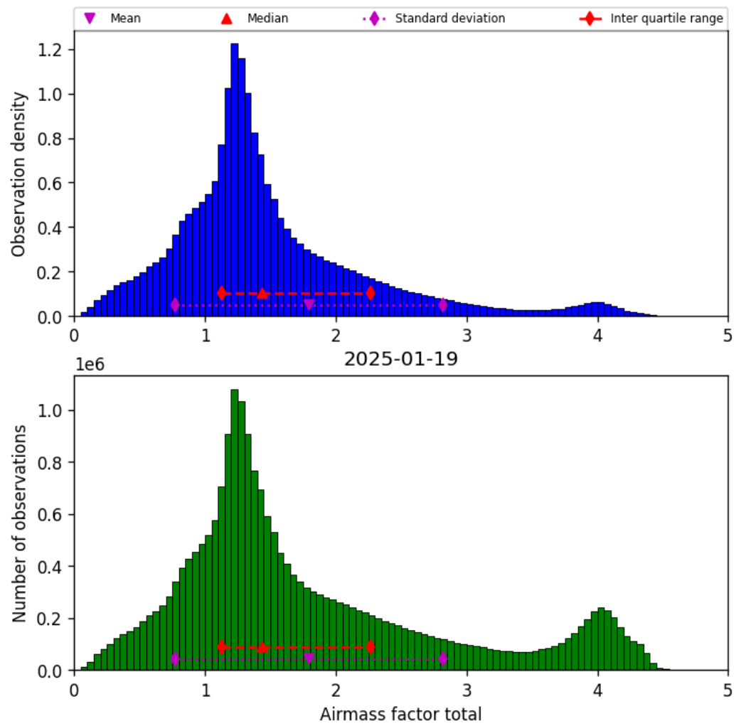
Figure 38: Histogram of “Airmass factor total” for 2025-01-19 to 2025-01-20
