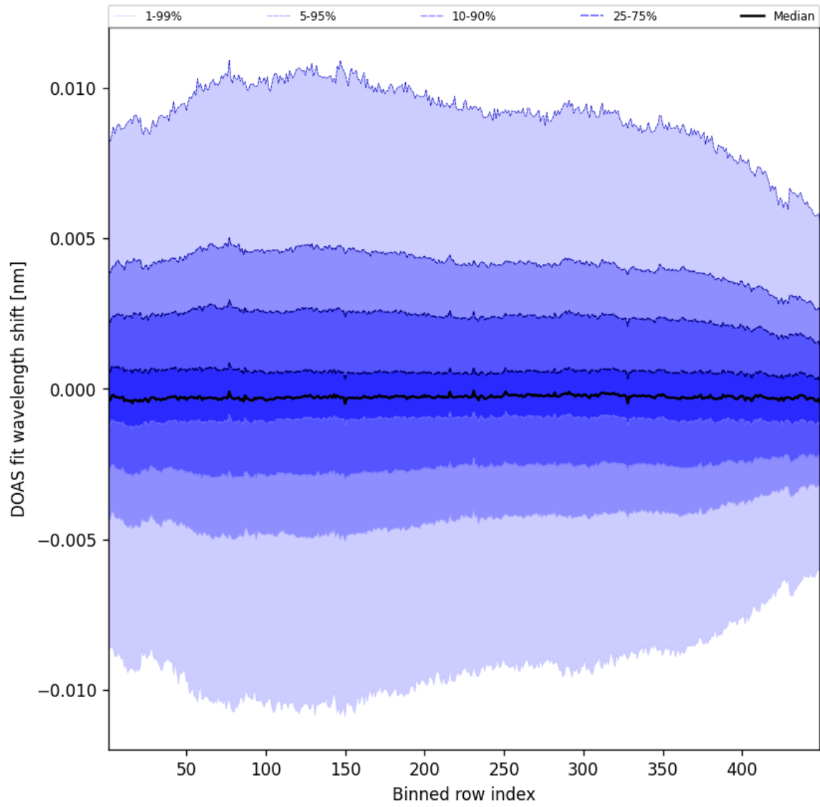
Figure 56: Along track statistics of “DOAS fit wavelength shift” for 2025-01-19 to 2025-01-20
