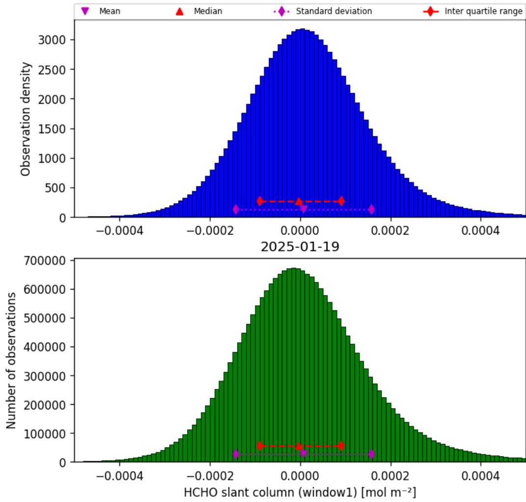
Figure 36: Histogram of “HCHO slant column (window1)” for 2025-01-19 to 2025-01-20
