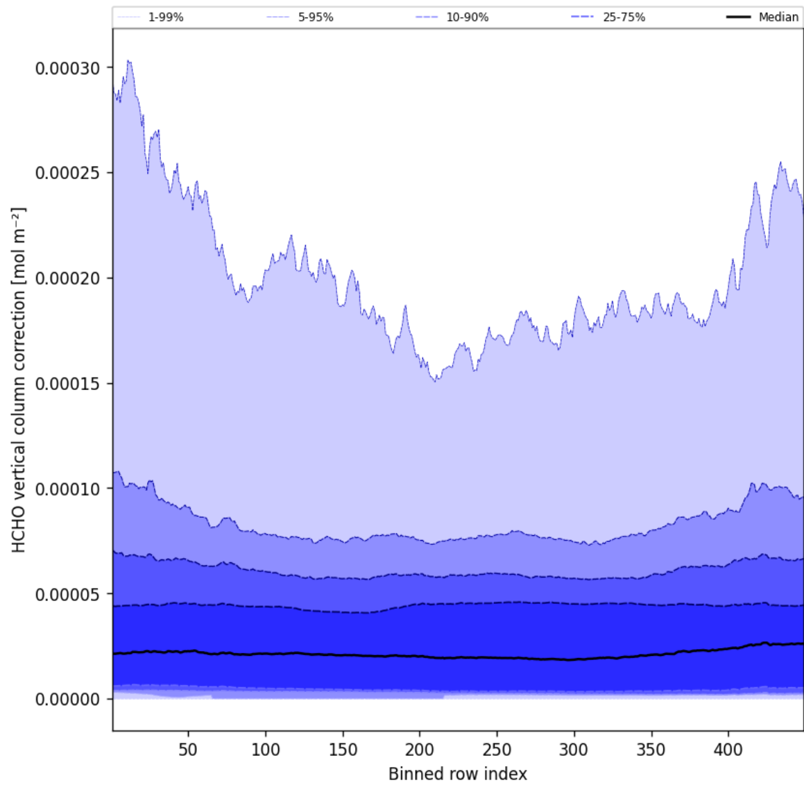
Figure 49: Along track statistics of “HCHO vertical column correction” for 2025-01-19 to 2025-01-20
