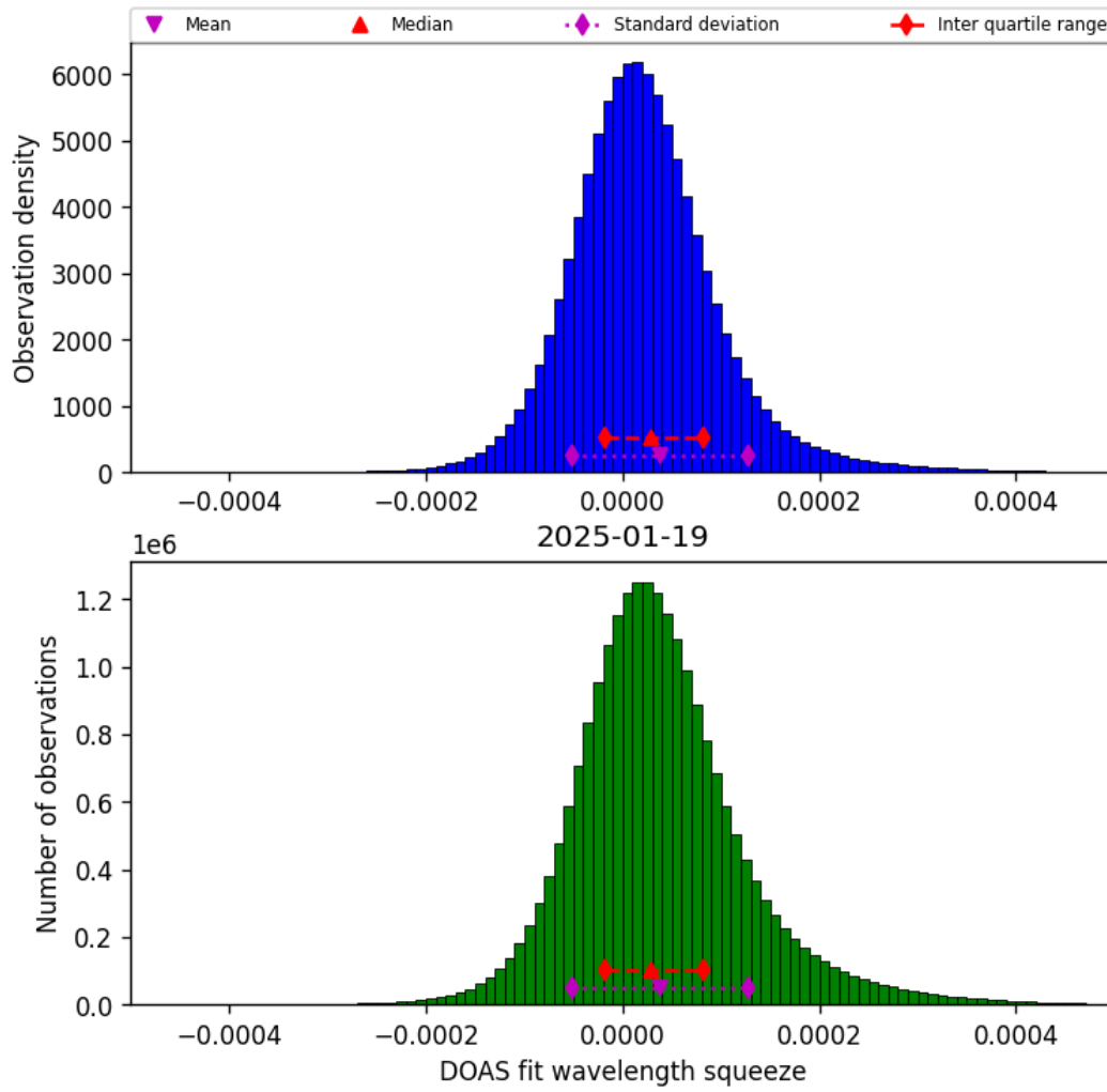
Figure 43: Histogram of “DOAS fit wavelength squeeze” for 2025-01-19 to 2025-01-20
