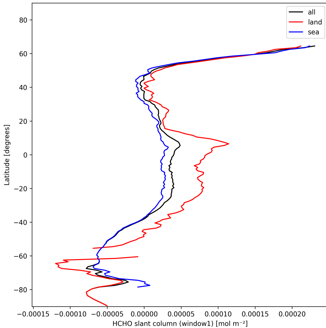
Figure 22: Zonal average of “HCHO slant column (window1)” for 2025-01-19 to 2025-01-20.
