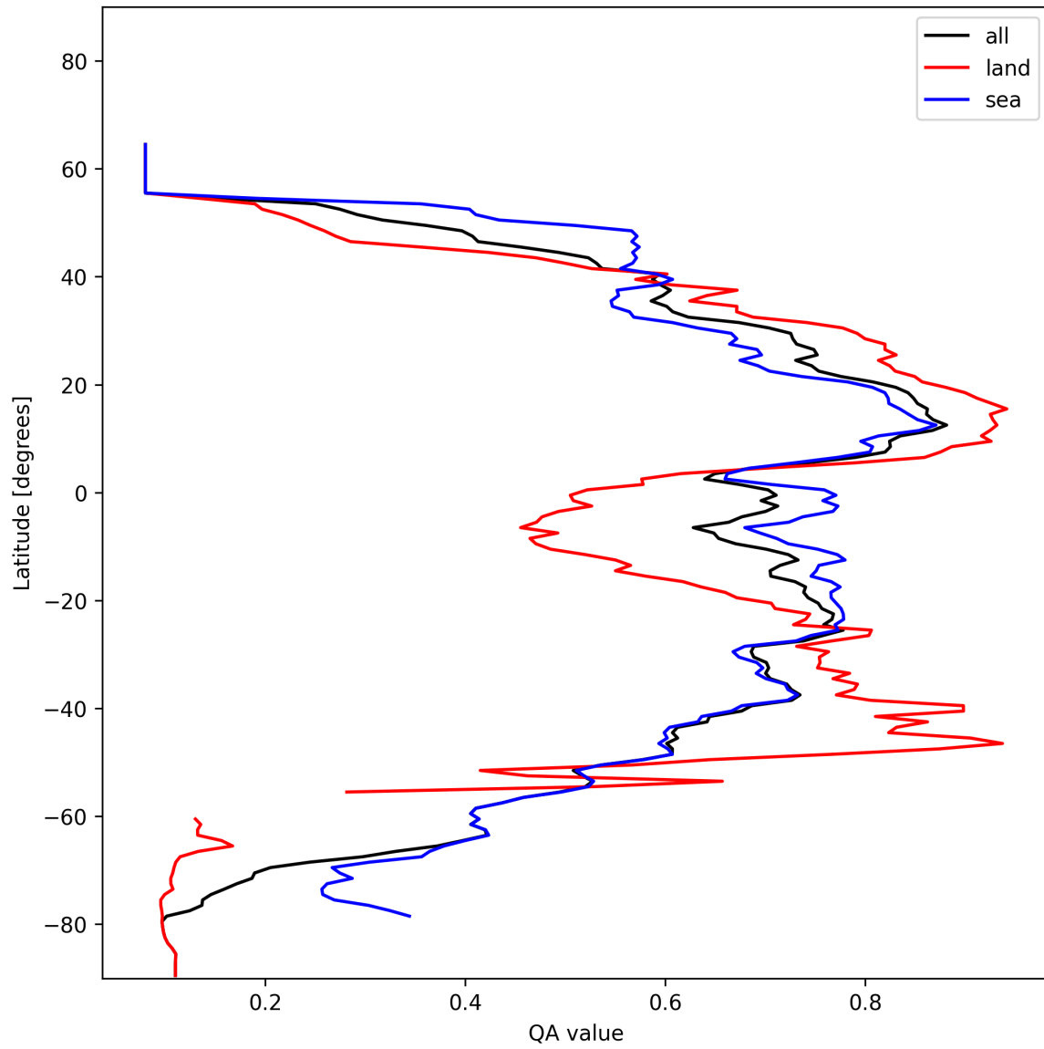
Figure 18: Zonal average of “QA value” for 2025-01-19 to 2025-01-20.
