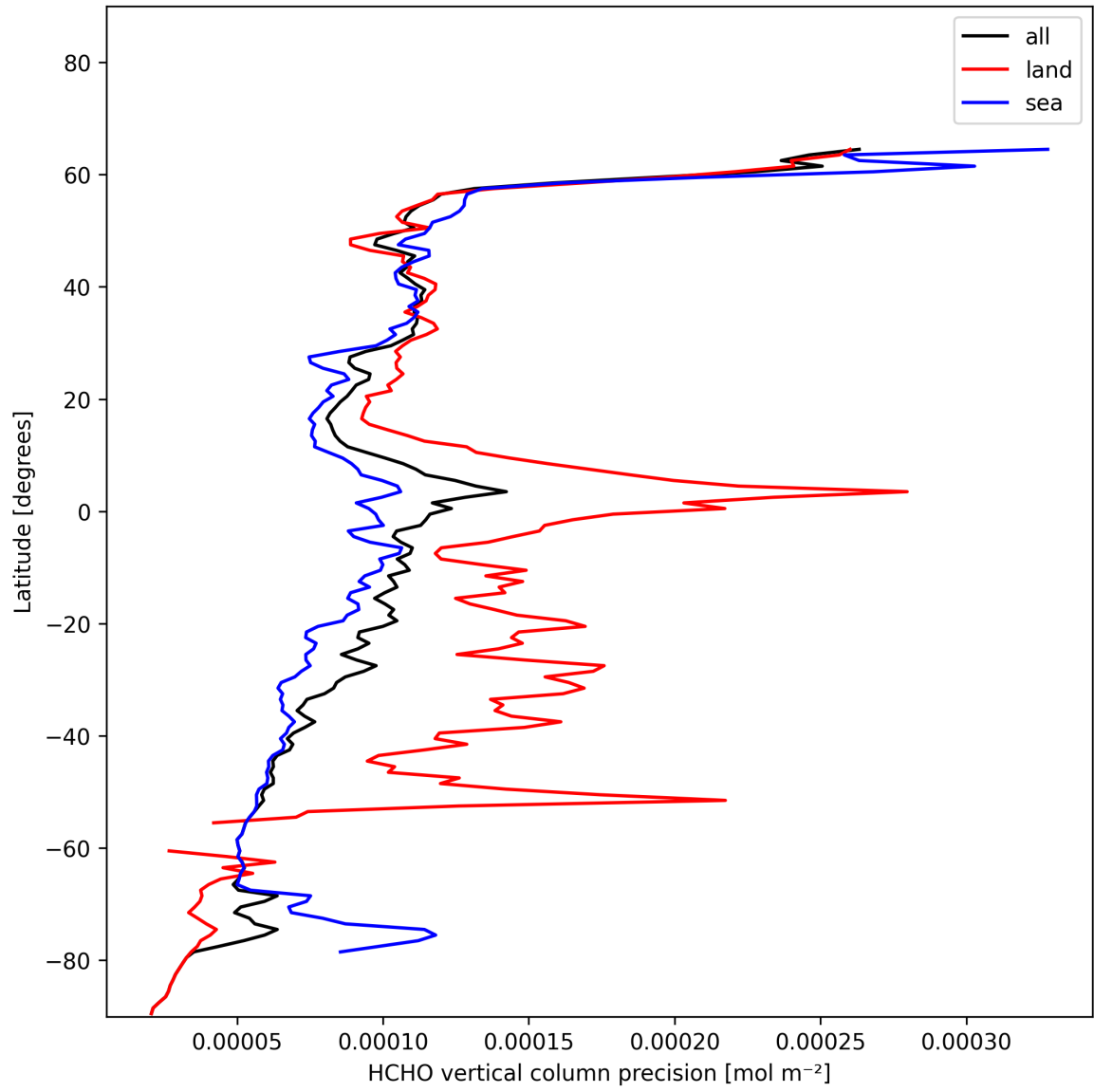
Figure 20: Zonal average of “HCHO vertical column precision” for 2025-01-19 to 2025-01-20.
