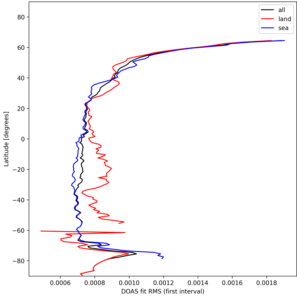
Figure 30: Zonal average of “DOAS fit RMS (first interval)” for 2025-01-19 to 2025-01-20.
