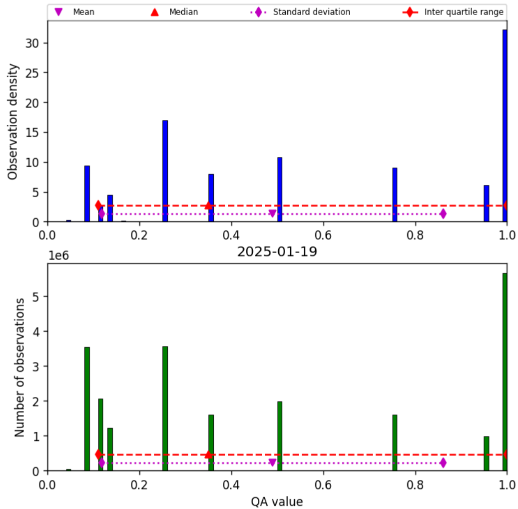
Figure 32: Histogram of “QA value” for 2025-01-19 to 2025-01-20
