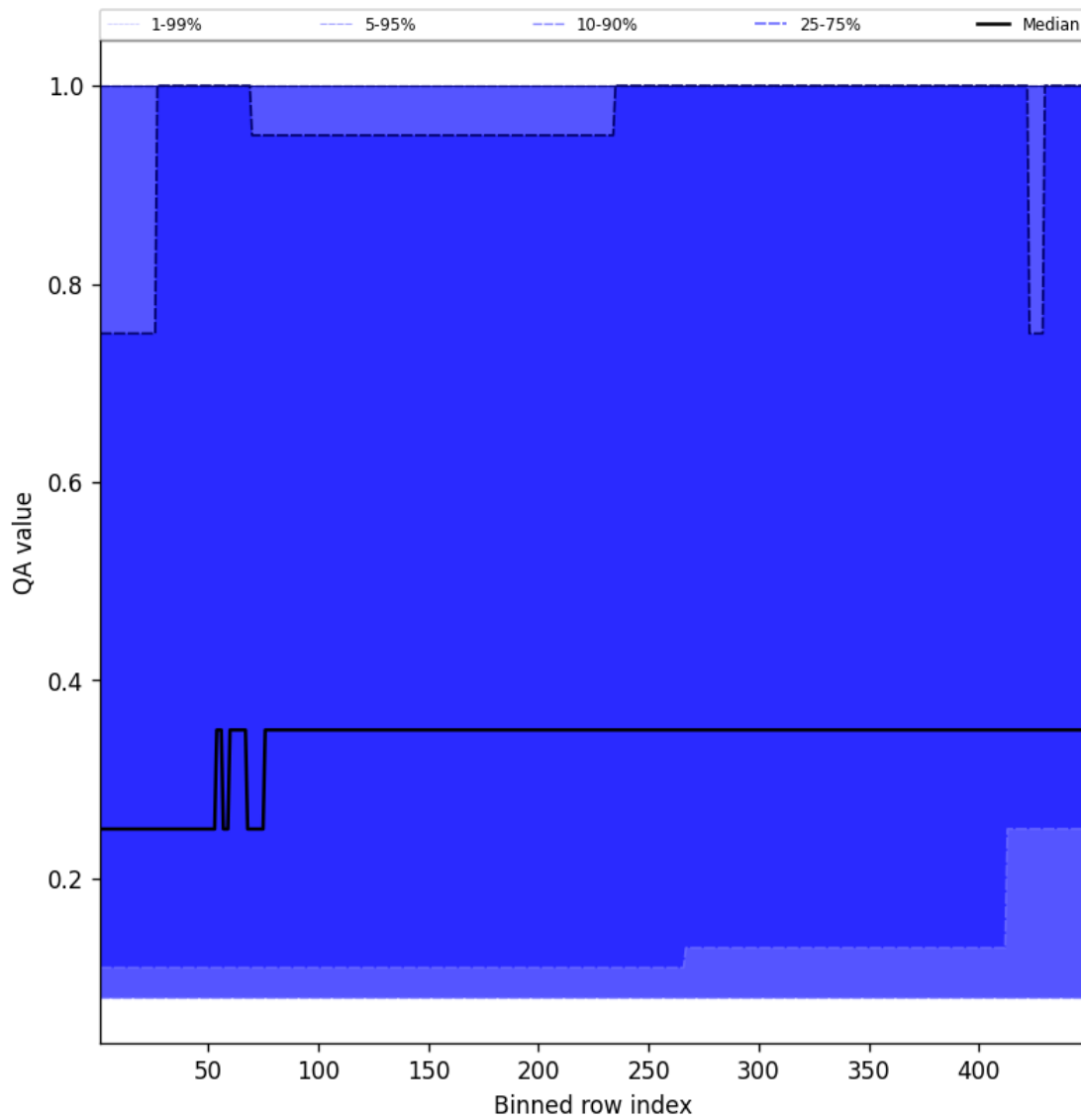
Figure 46: Along track statistics of “QA value” for 2025-01-19 to 2025-01-20
