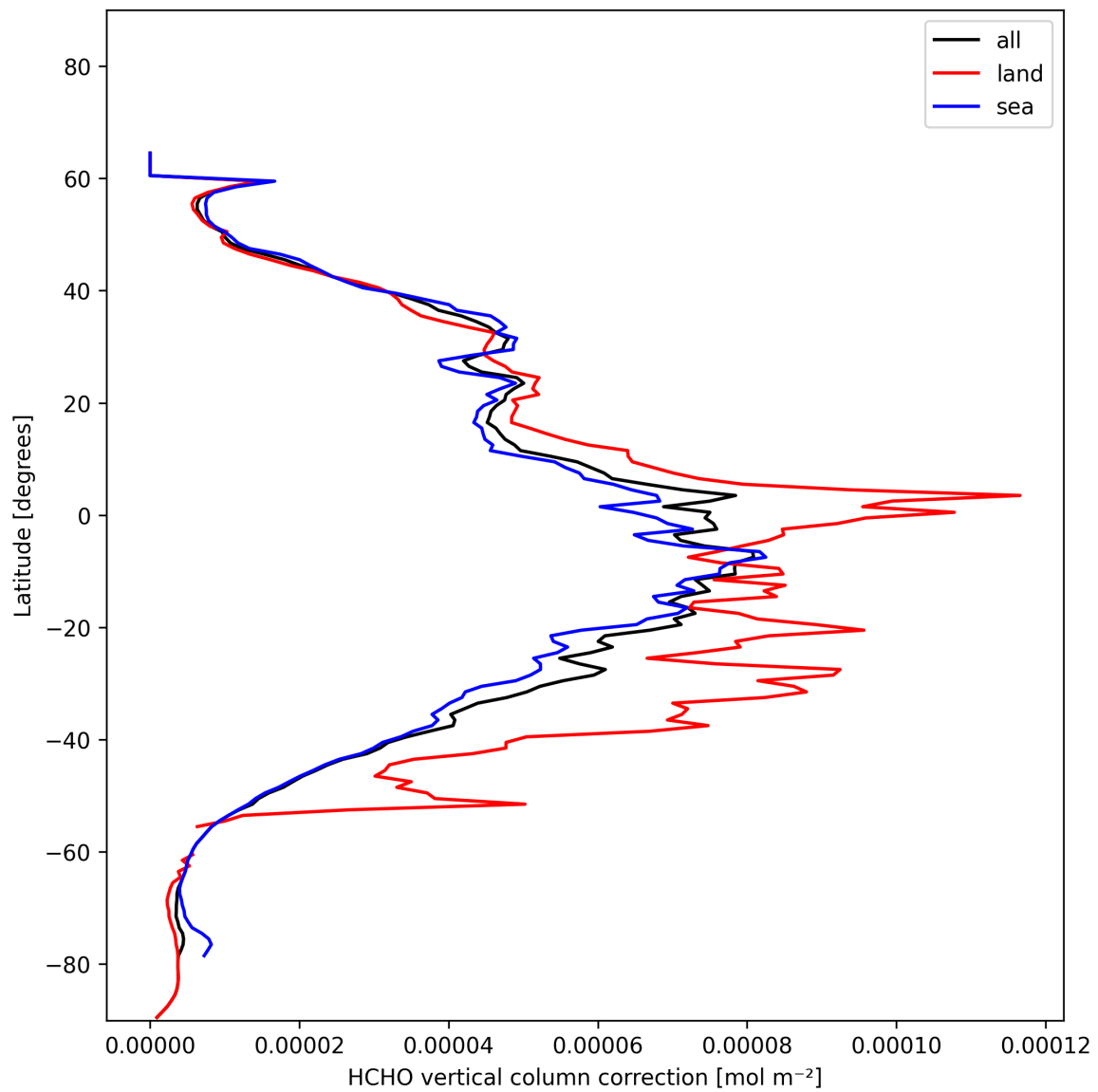
Figure 21: Zonal average of “HCHO vertical column correction” for 2025-01-19 to 2025-01-20.
