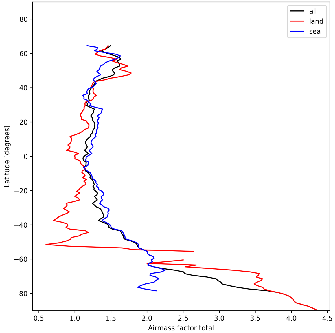
Figure 24: Zonal average of “Airmass factor total” for 2025-01-19 to 2025-01-20.
