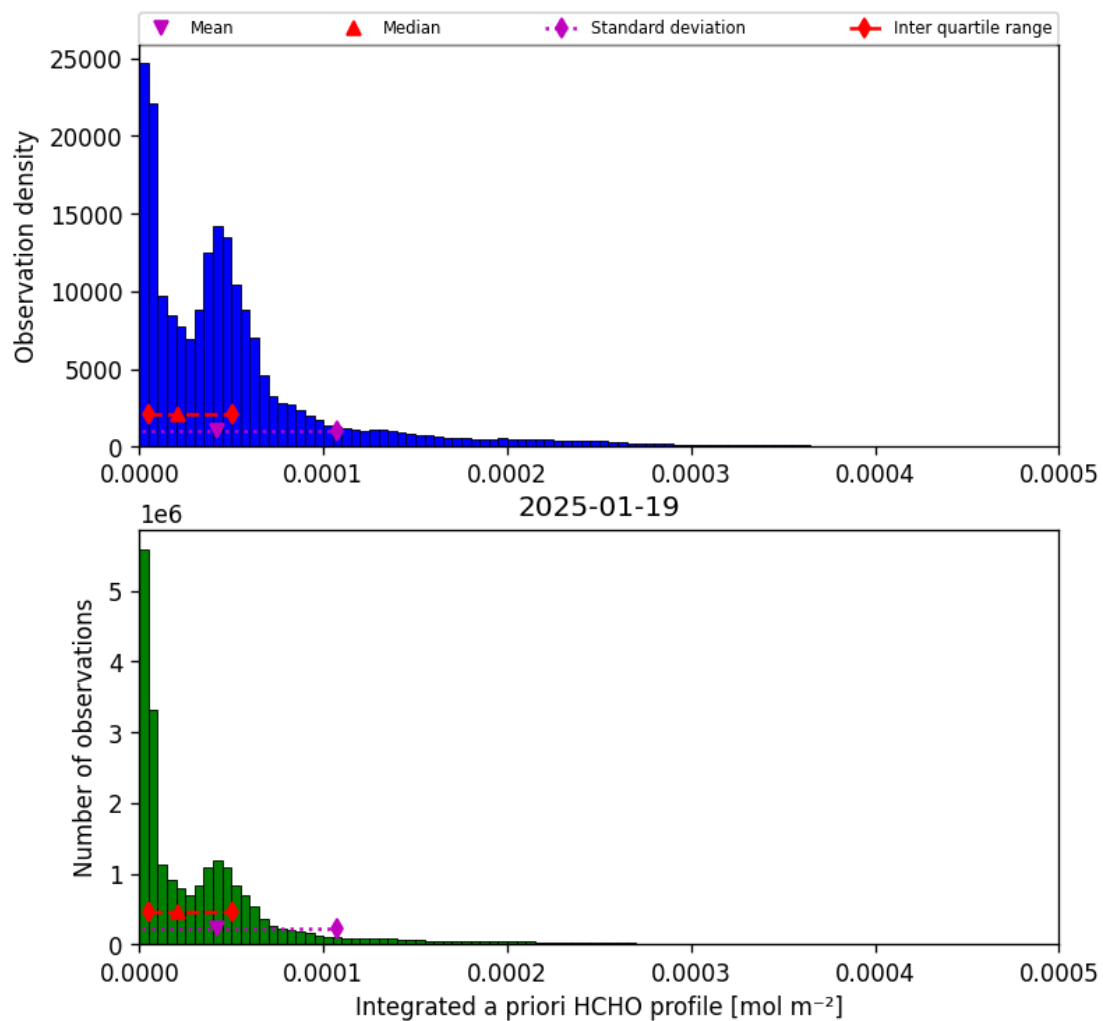
Figure 41: Histogram of “Integrated a priori HCHO profile” for 2025-01-19 to 2025-01-20
