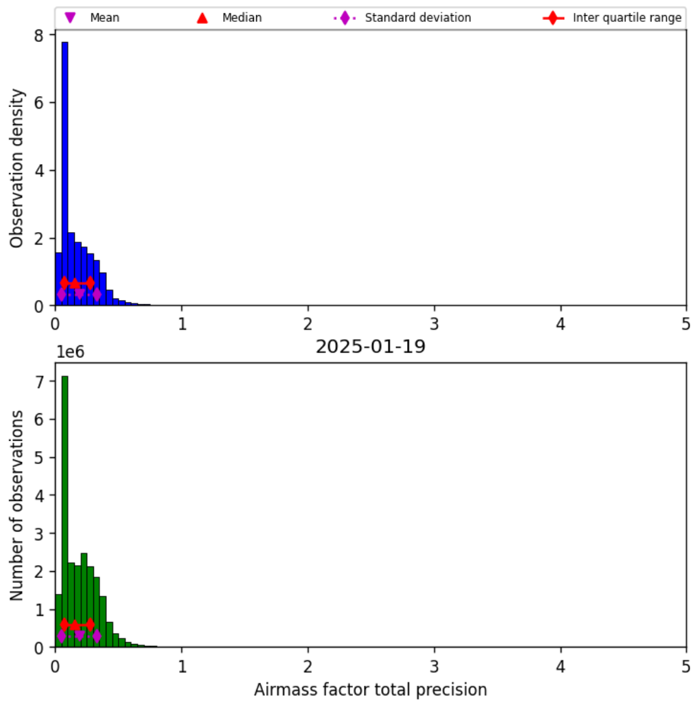
Figure 39: Histogram of “Airmass factor total precision” for 2025-01-19 to 2025-01-20
