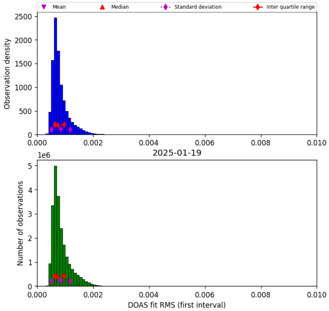
Figure 44: Histogram of “DOAS fit RMS (first interval)” for 2025-01-19 to 2025-01-20
