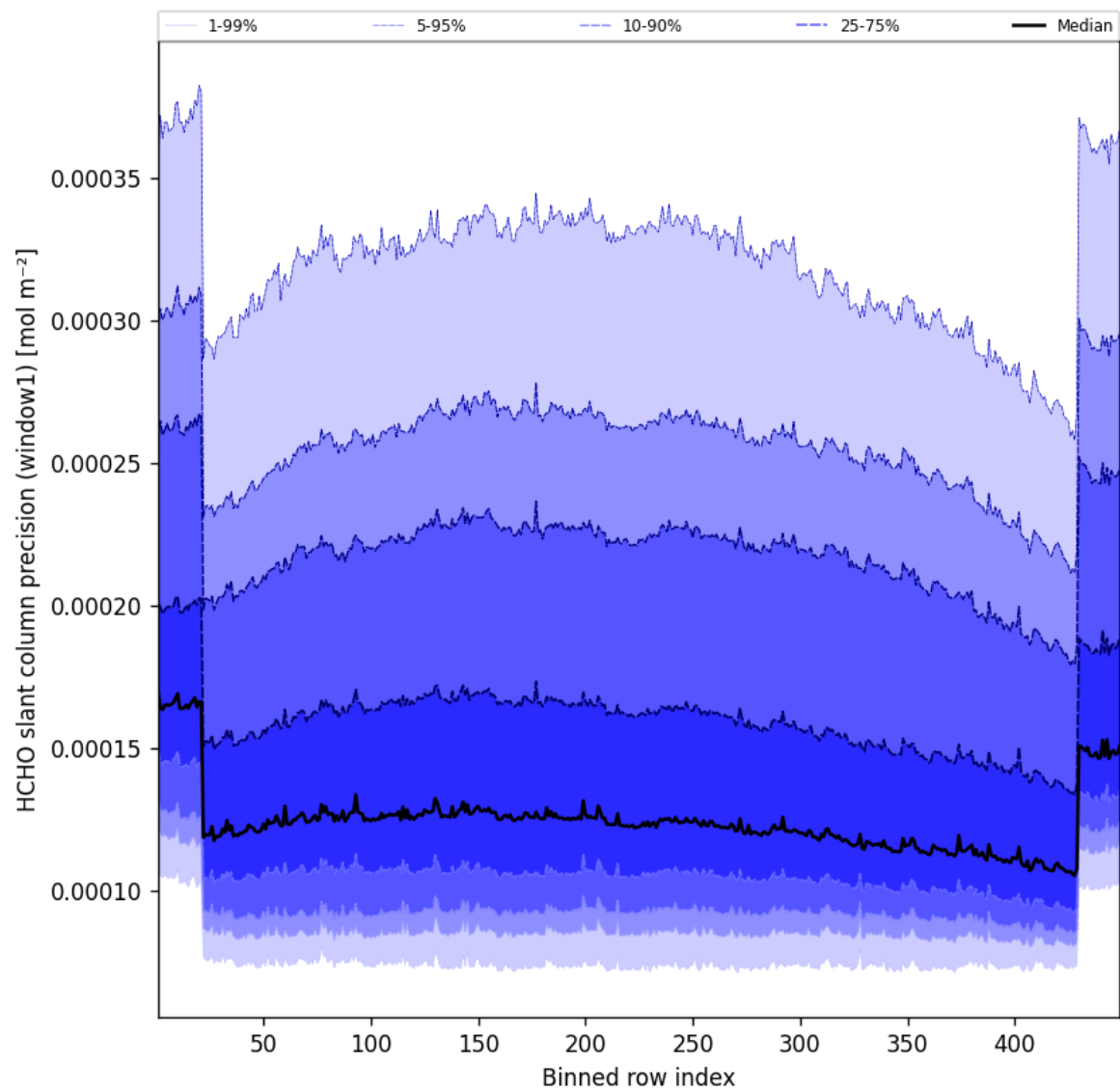
Figure 51: Along track statistics of “HCHO slant column precision (window1)” for 2025-01-19 to 2025-01-20
