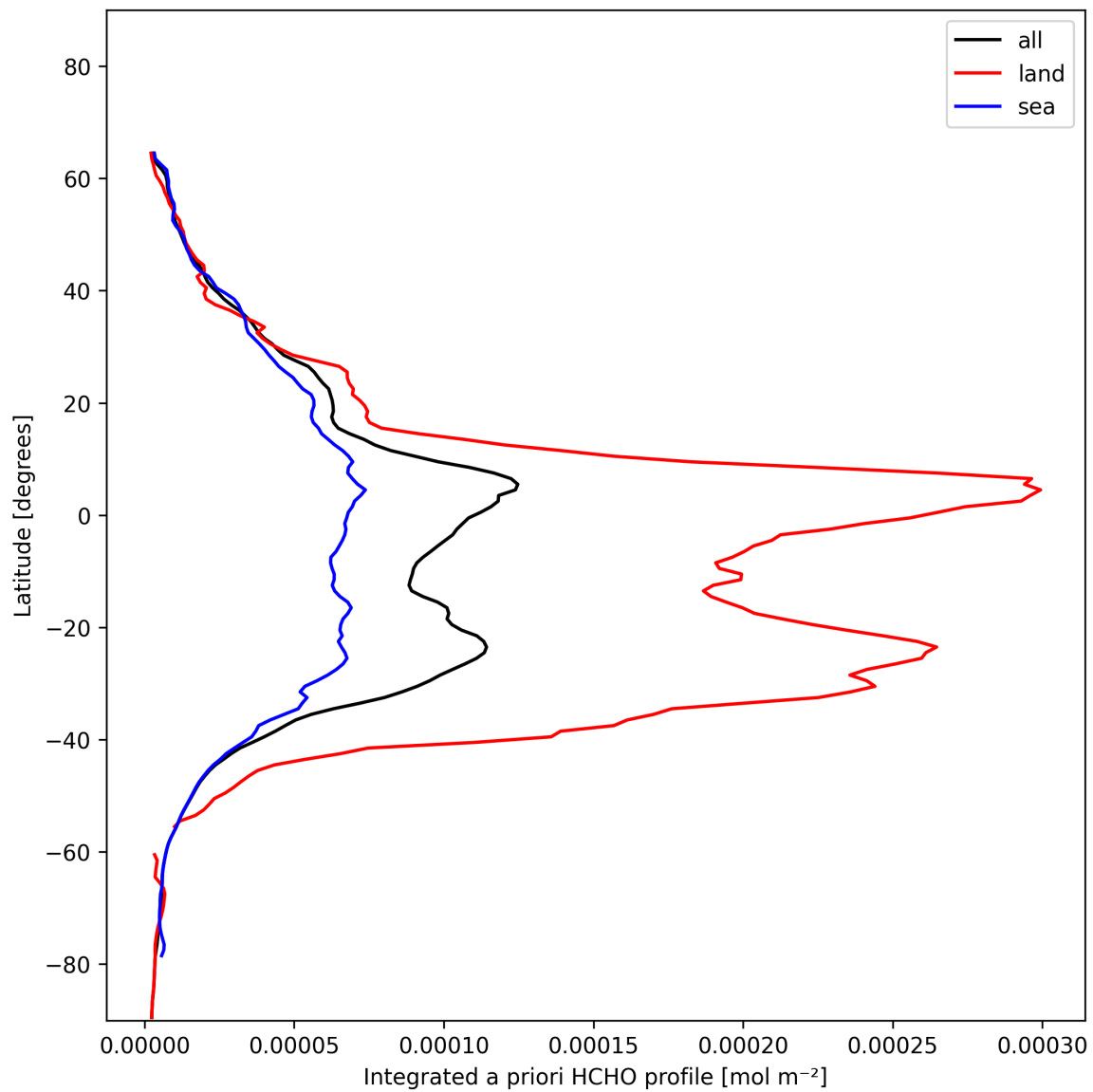
Figure 27: Zonal average of “Integrated a priori HCHO profile” for 2025-01-19 to 2025-01-20.
