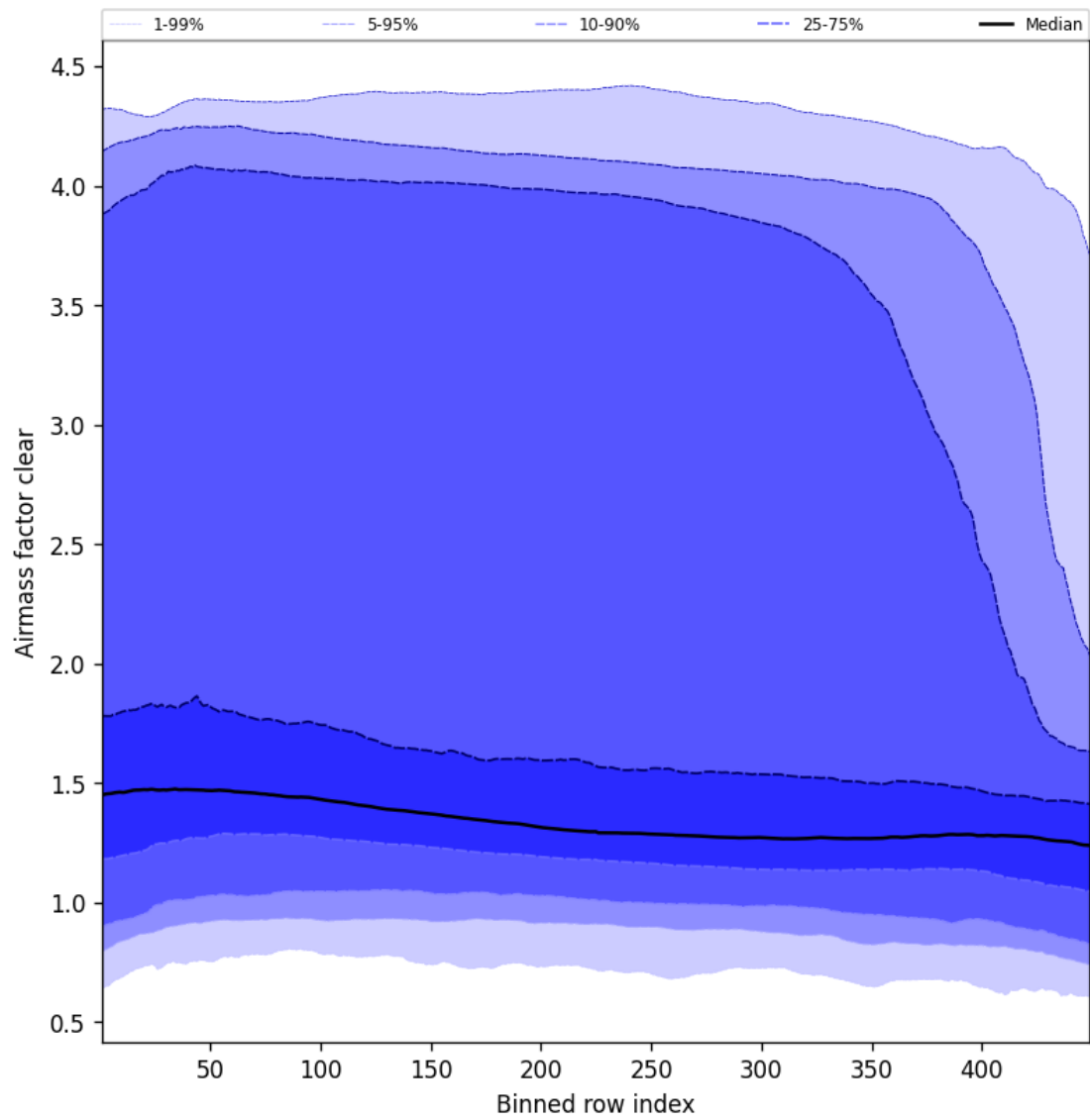
Figure 54: Along track statistics of “Airmass factor clear” for 2025-01-19 to 2025-01-20
