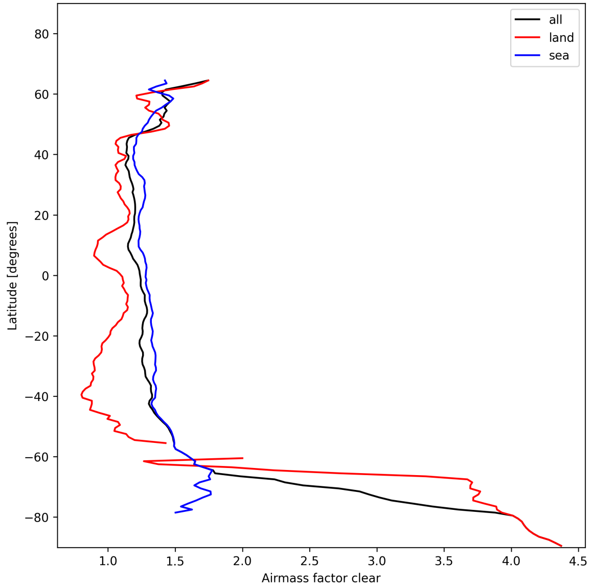
Figure 26: Zonal average of “Airmass factor clear” for 2025-01-19 to 2025-01-20.
