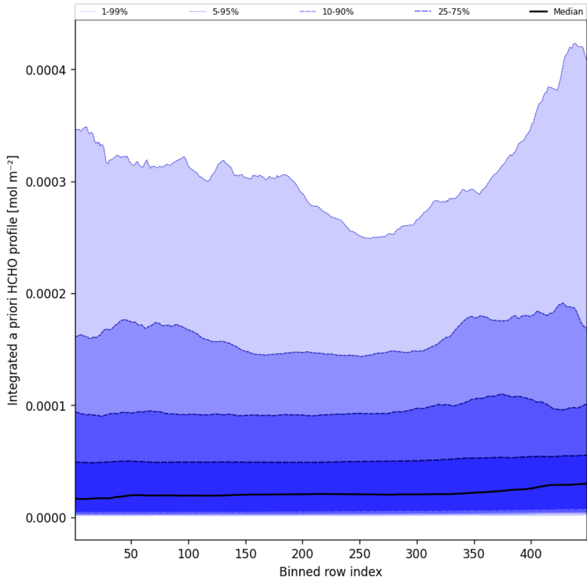
Figure 55: Along track statistics of "Integrated a priori HCHO profile" for 2025-01-19 to 2025-01-20
