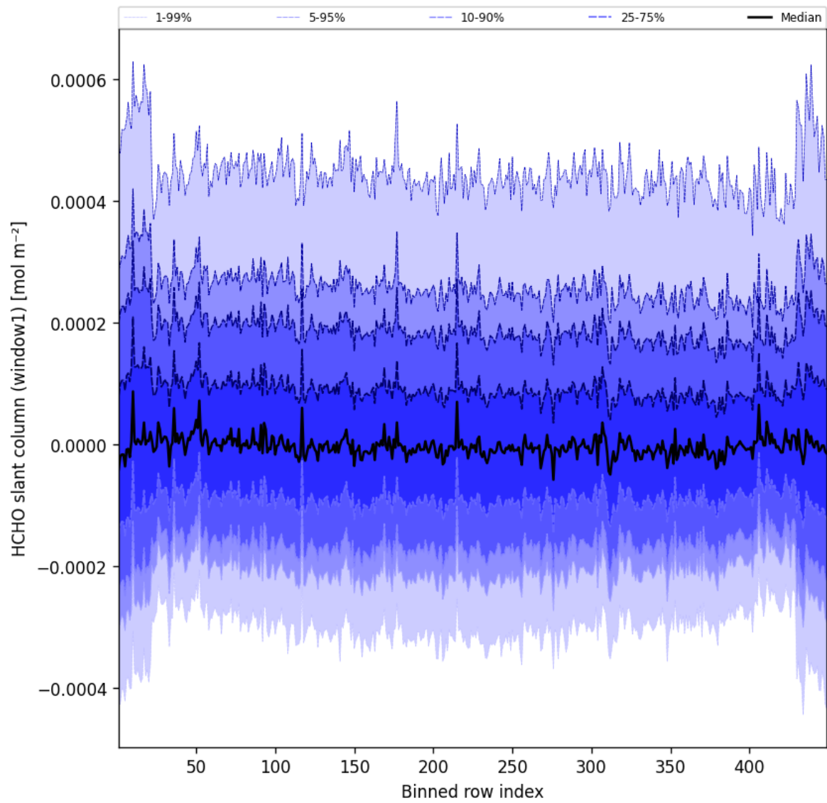
Figure 50: Along track statistics of “HCHO slant column (window1)” for 2025-01-19 to 2025-01-20
