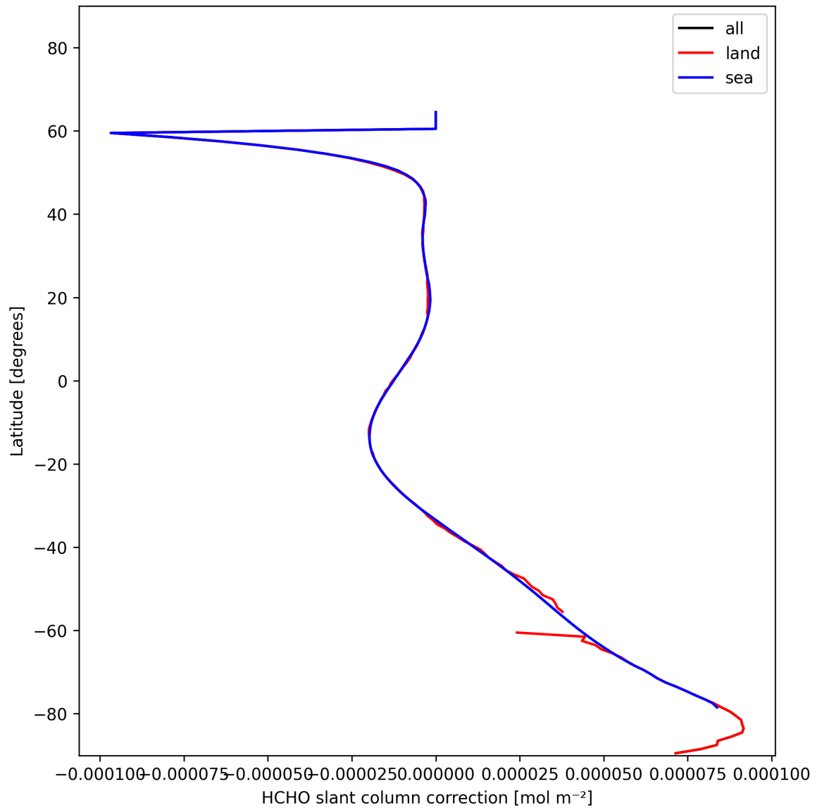
Figure 31: Zonal average of “HCHO slant column correction” for 2025-01-19 to 2025-01-20.
