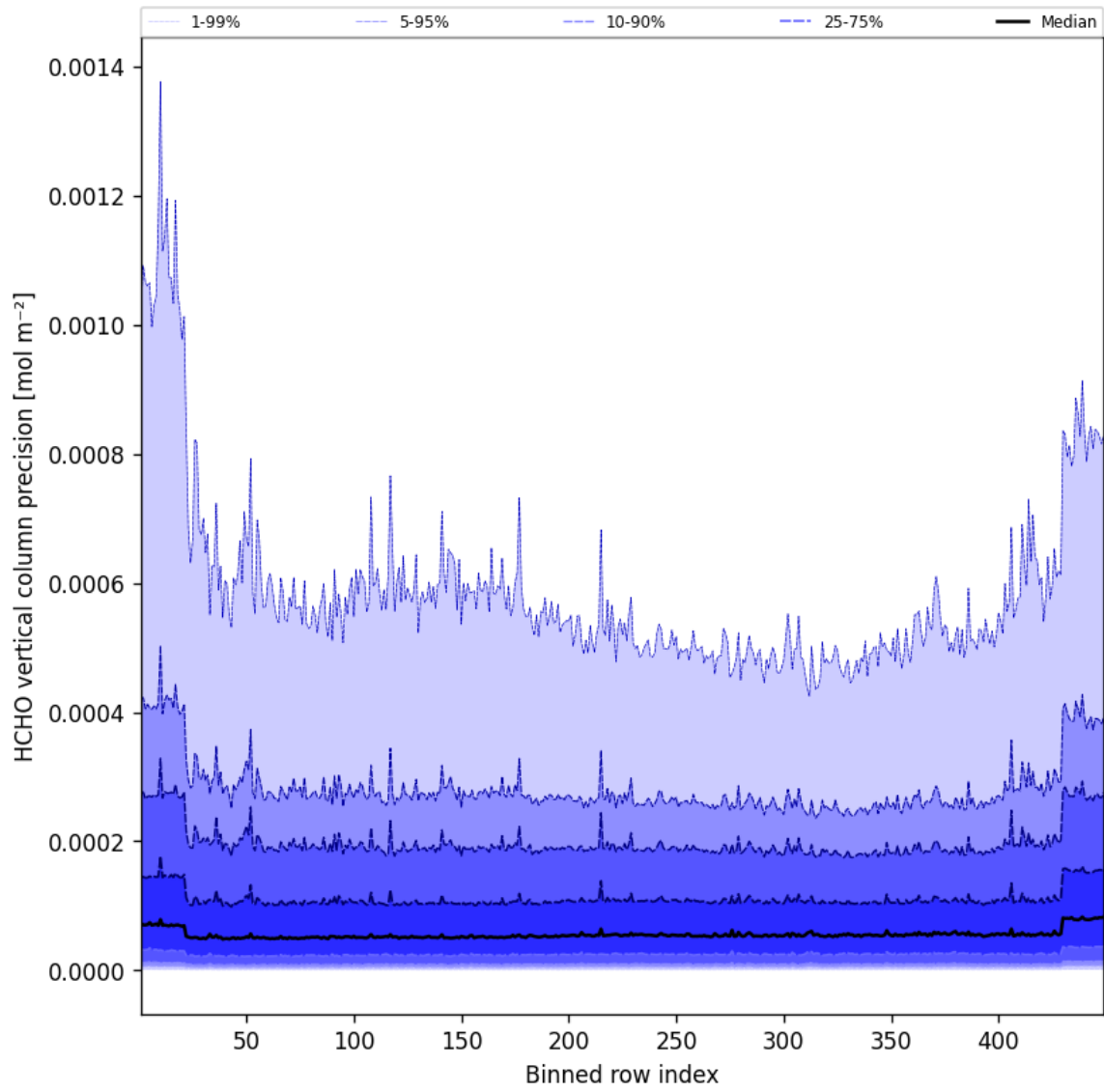
Figure 48: Along track statistics of “HCHO vertical column precision” for 2025-01-19 to 2025-01-20
