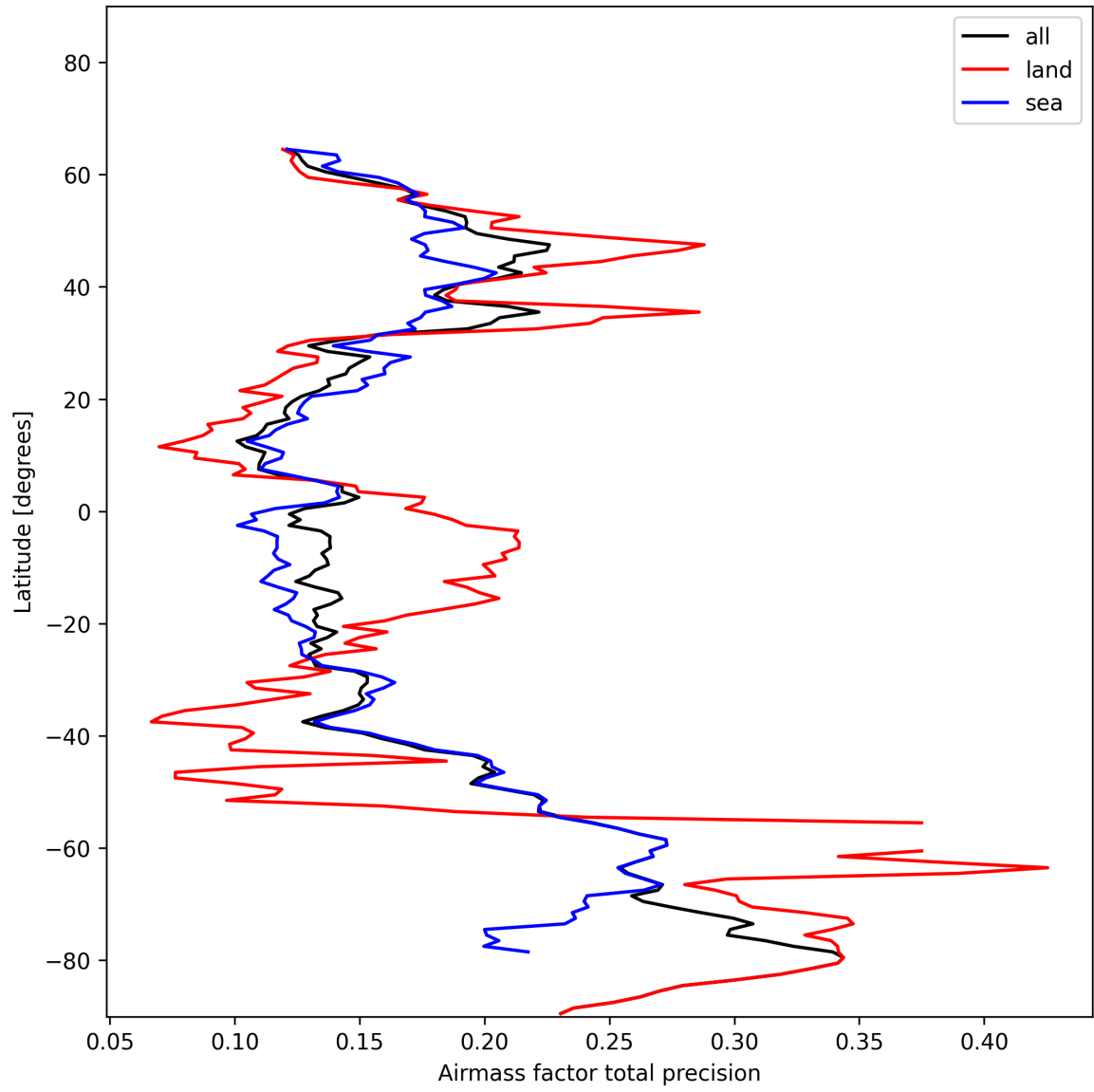
Figure 25: Zonal average of “Airmass factor total precision” for 2025-01-19 to 2025-01-20.
