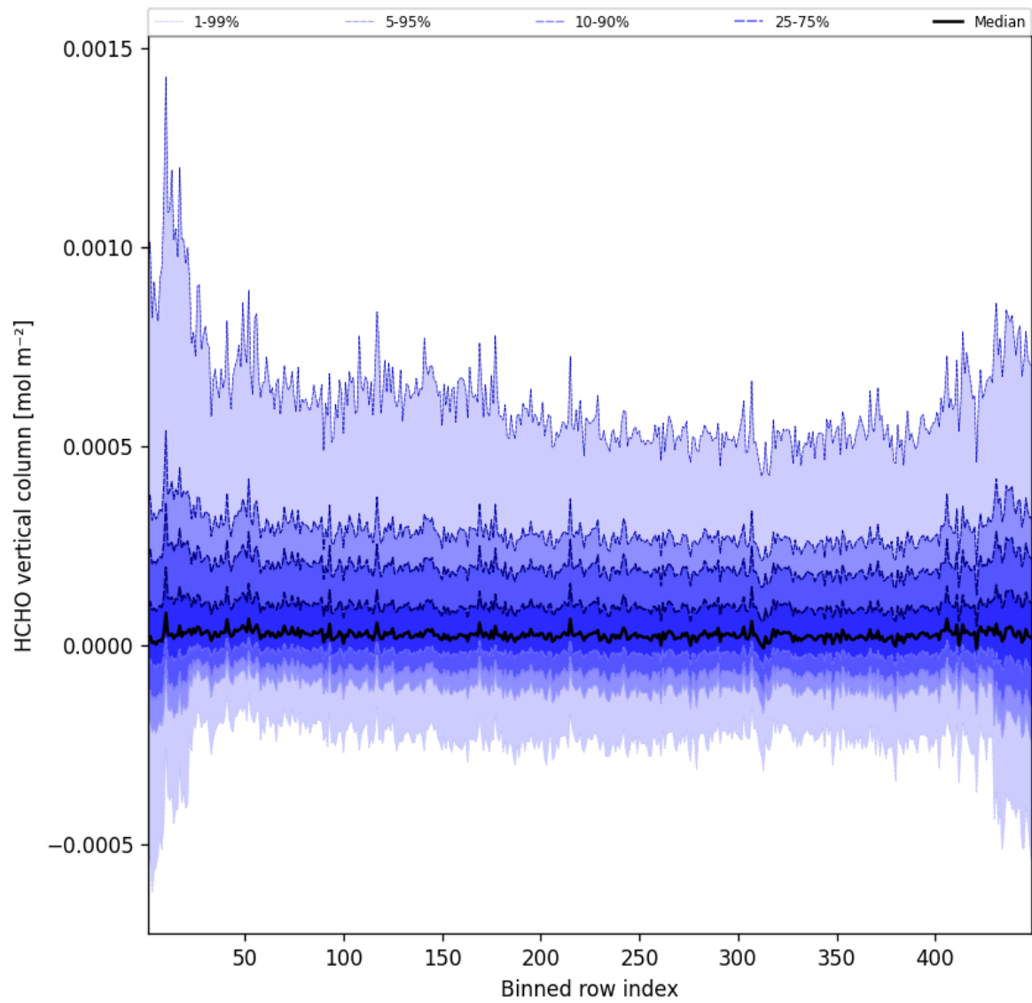
Figure 47: Along track statistics of “HCHO vertical column” for 2025-01-19 to 2025-01-20
