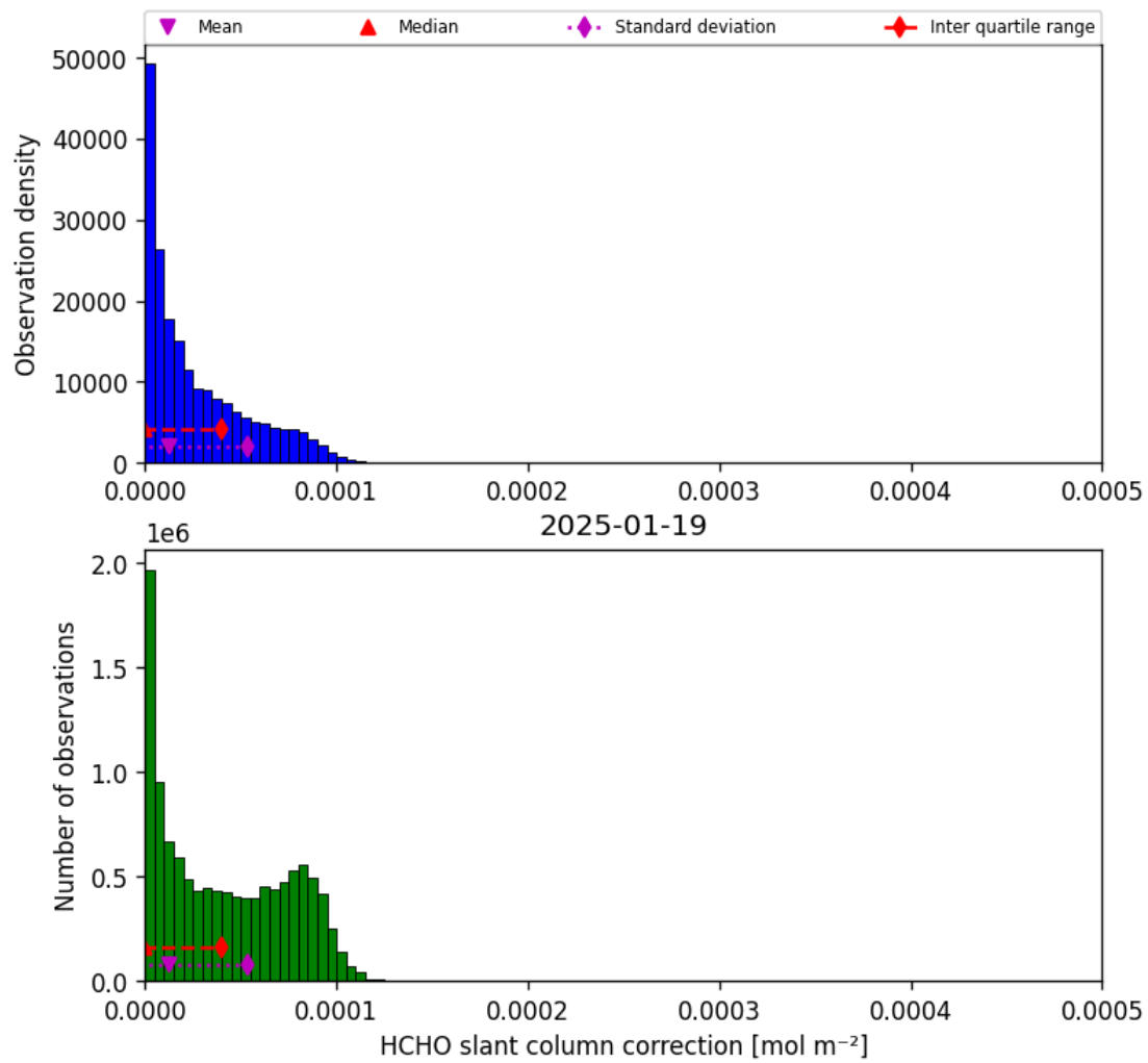
Figure 45: Histogram of “HCHO slant column correction” for 2025-01-19 to 2025-01-20
