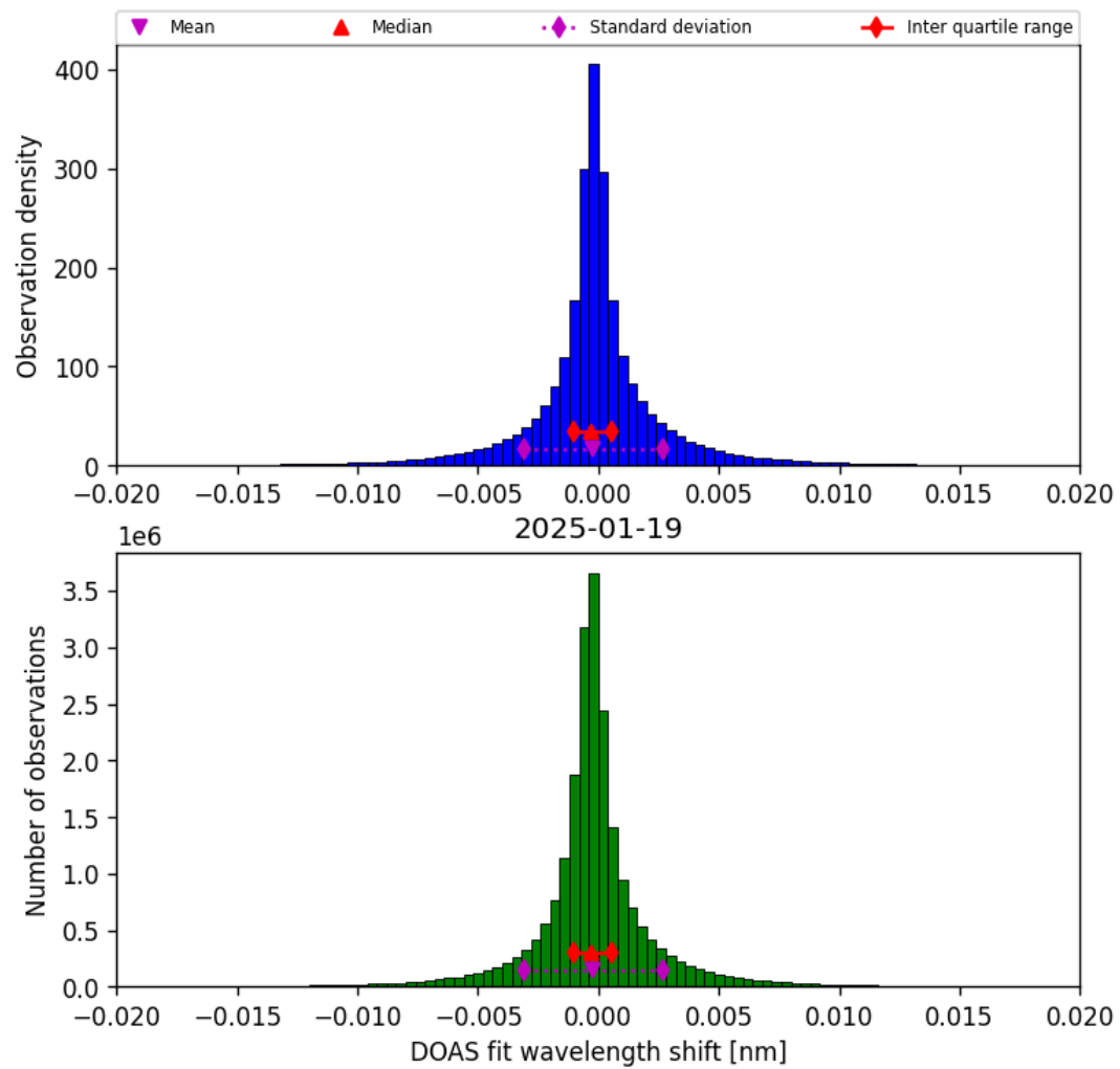
Figure 42: Histogram of “DOAS fit wavelength shift” for 2025-01-19 to 2025-01-20
