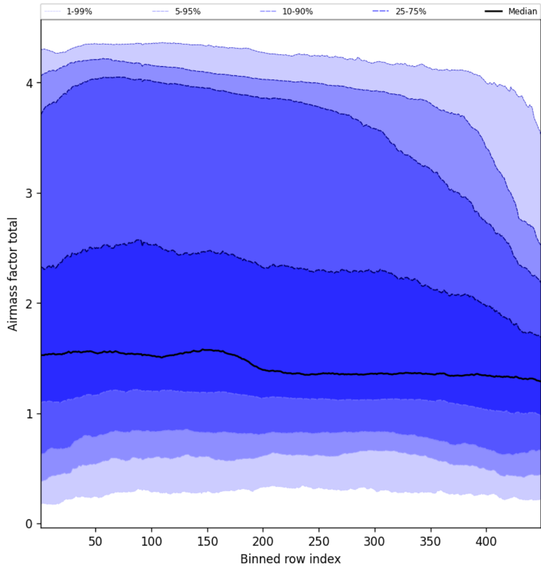
Figure 52: Along track statistics of “Airmass factor total” for 2025-01-19 to 2025-01-20
