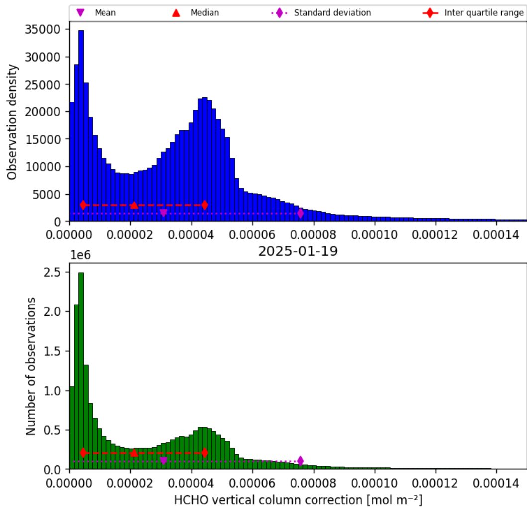
Figure 35: Histogram of “HCHO vertical column correction” for 2025-01-19 to 2025-01-20
