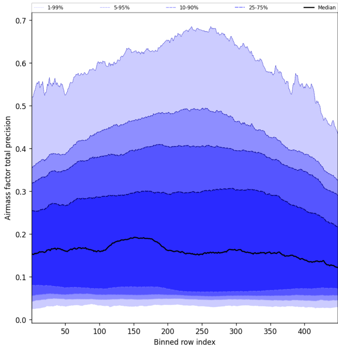
Figure 53: Along track statistics of “Airmass factor total precision” for 2025-01-19 to 2025-01-20
