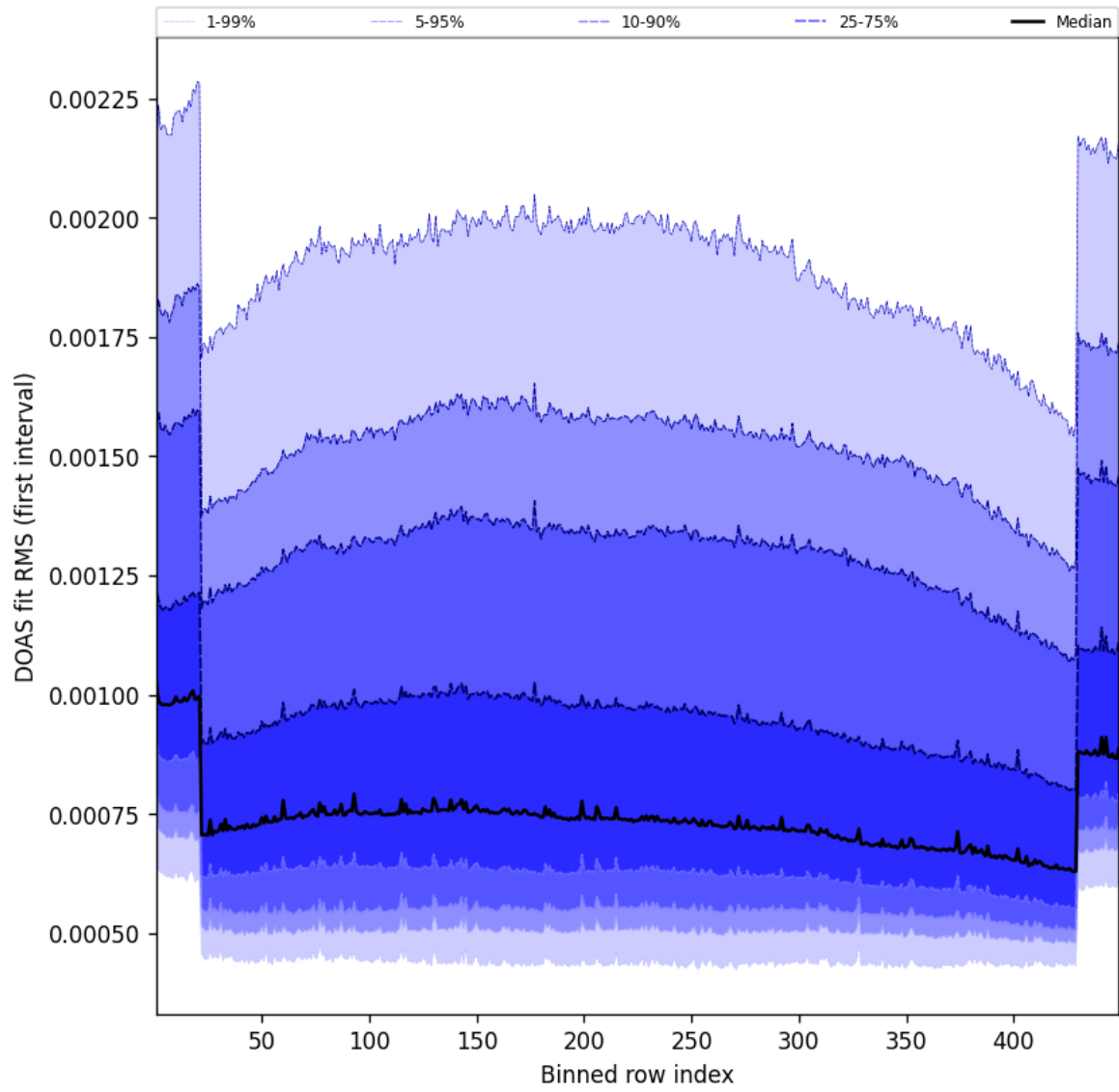
Figure 58: Along track statistics of “DOAS fit RMS (first interval)” for 2025-01-19 to 2025-01-20
