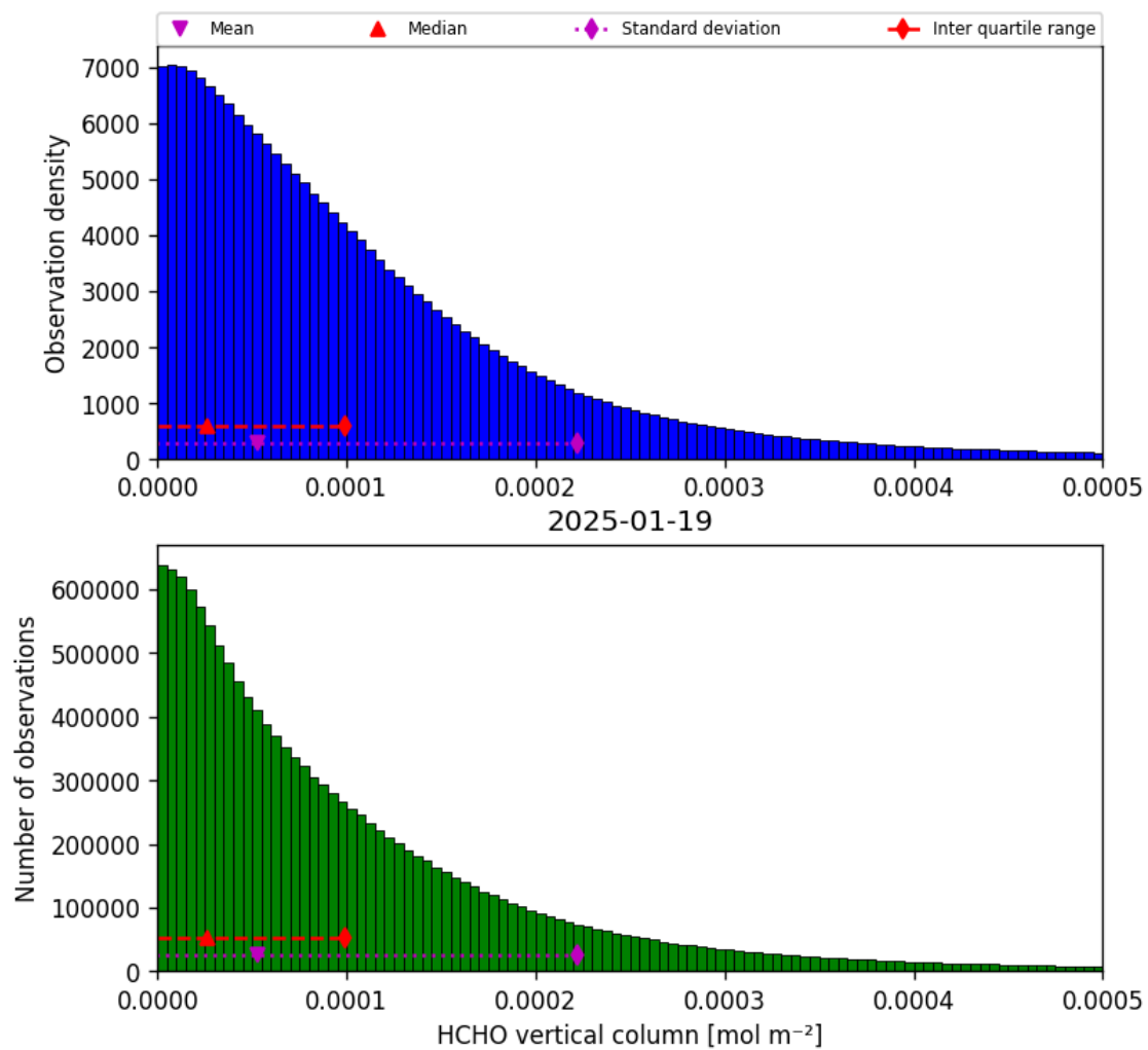
Figure 33: Histogram of “HCHO vertical column” for 2025-01-19 to 2025-01-20
