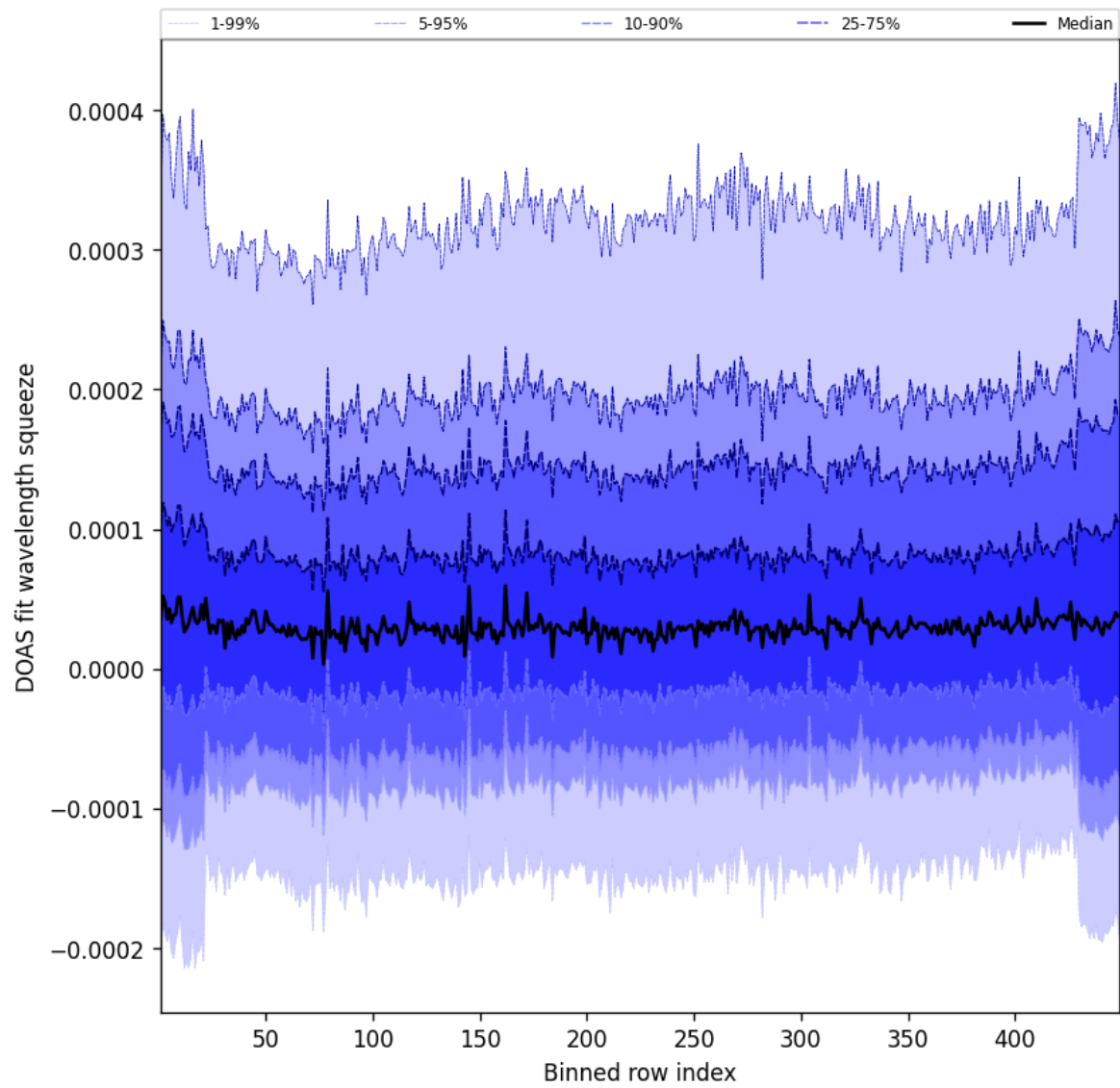
Figure 57: Along track statistics of “DOAS fit wavelength squeeze” for 2025-01-19 to 2025-01-20
