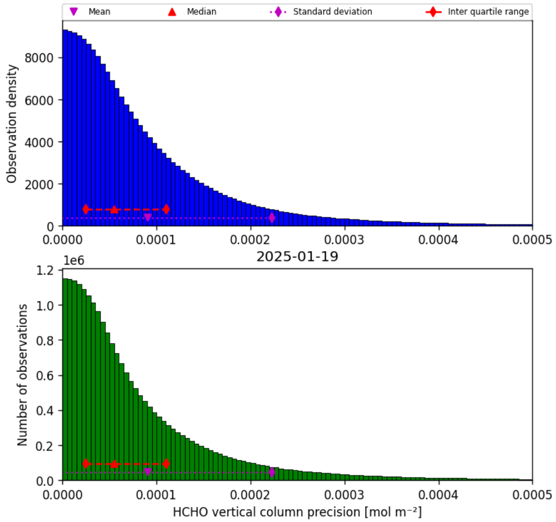
Figure 34: Histogram of “HCHO vertical column precision” for 2025-01-19 to 2025-01-20
