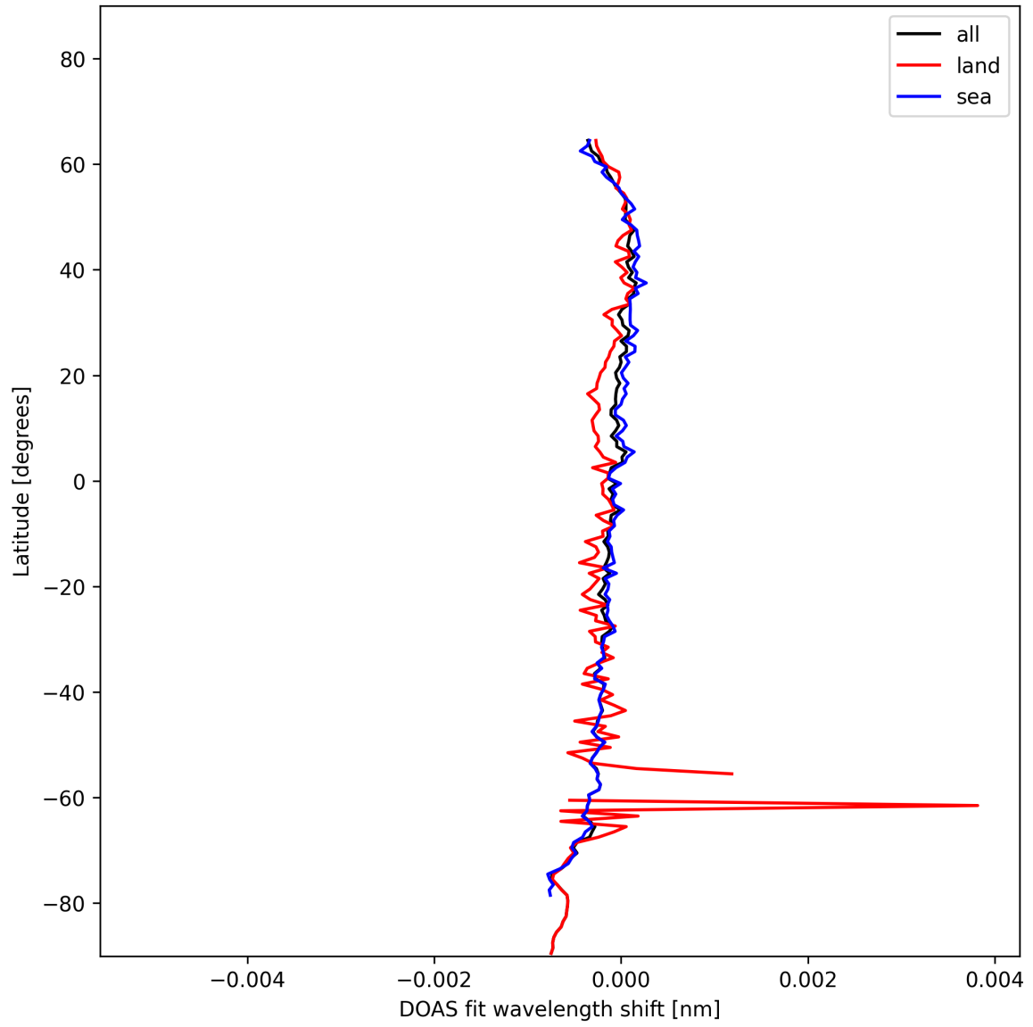
Figure 28: Zonal average of “DOAS fit wavelength shift” for 2025-01-19 to 2025-01-20.
