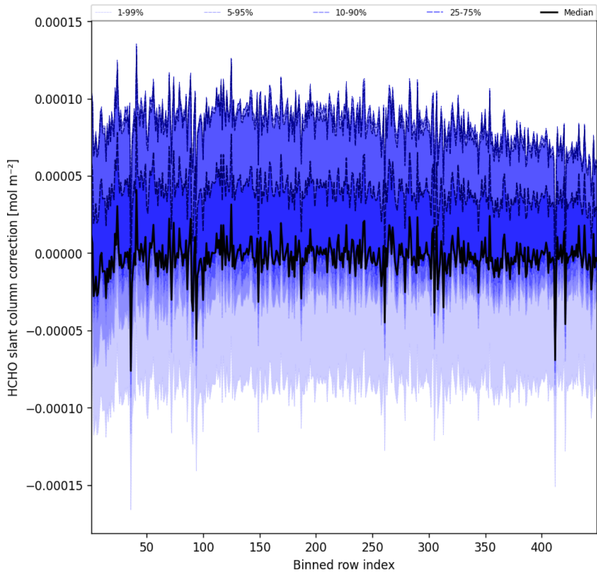
Figure 59: Along track statistics of “HCHO slant column correction” for 2025-01-19 to 2025-01-20
