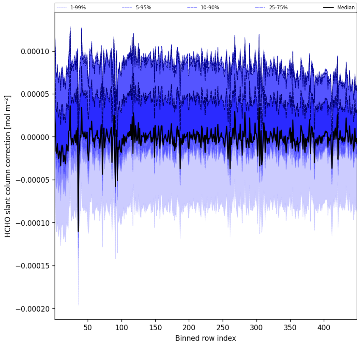
Figure 59: Along track statistics of “HCHO slant column correction” for 2025-01-20 to 2025-01-21
