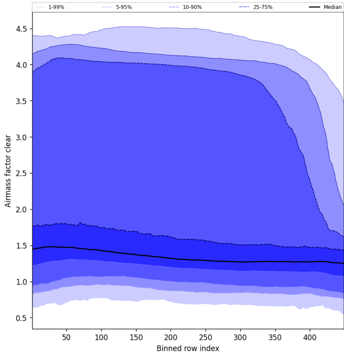
Figure 54: Along track statistics of “Airmass factor clear” for 2025-01-20 to 2025-01-21
