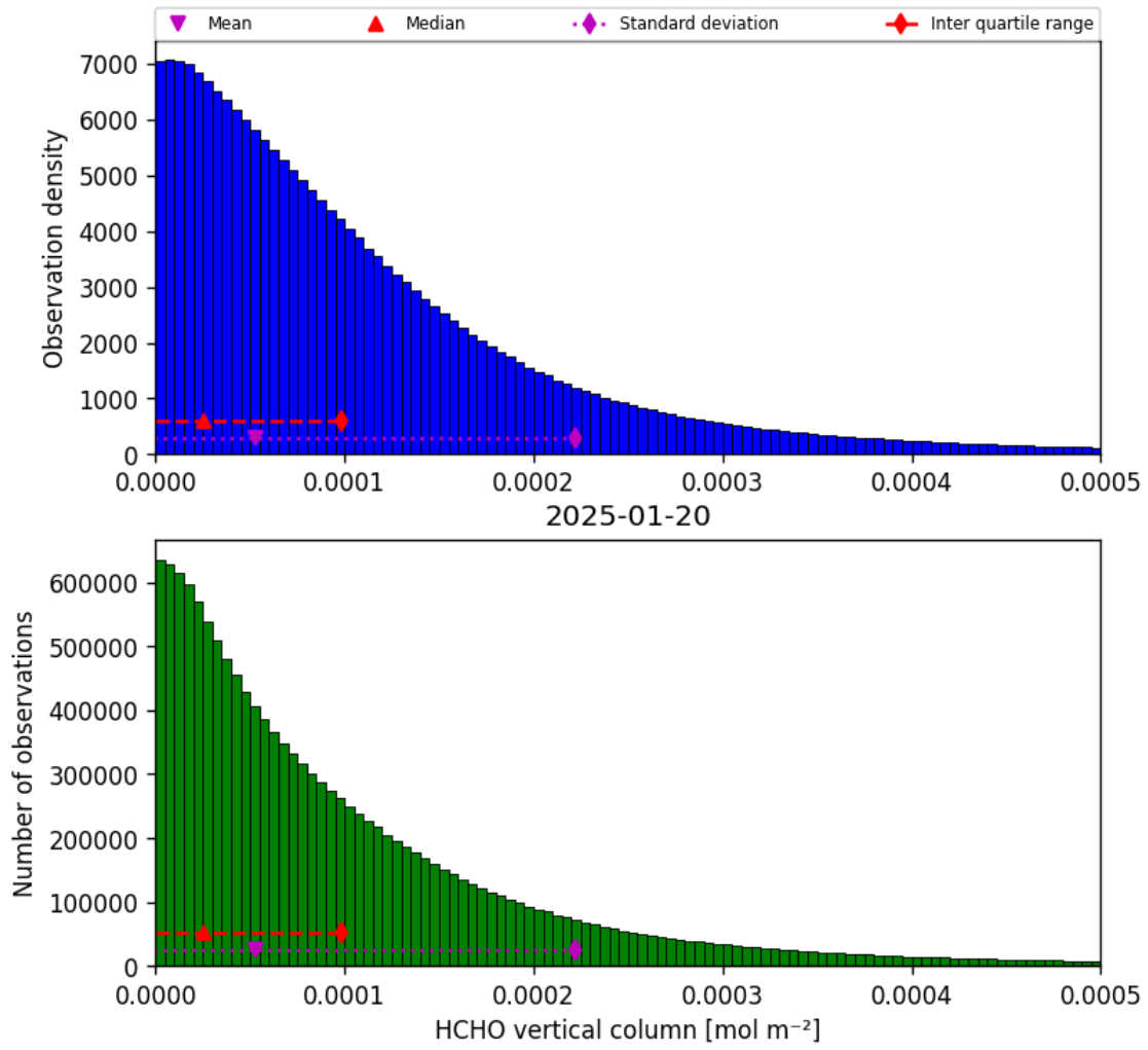
Figure 33: Histogram of “HCHO vertical column” for 2025-01-20 to 2025-01-21
