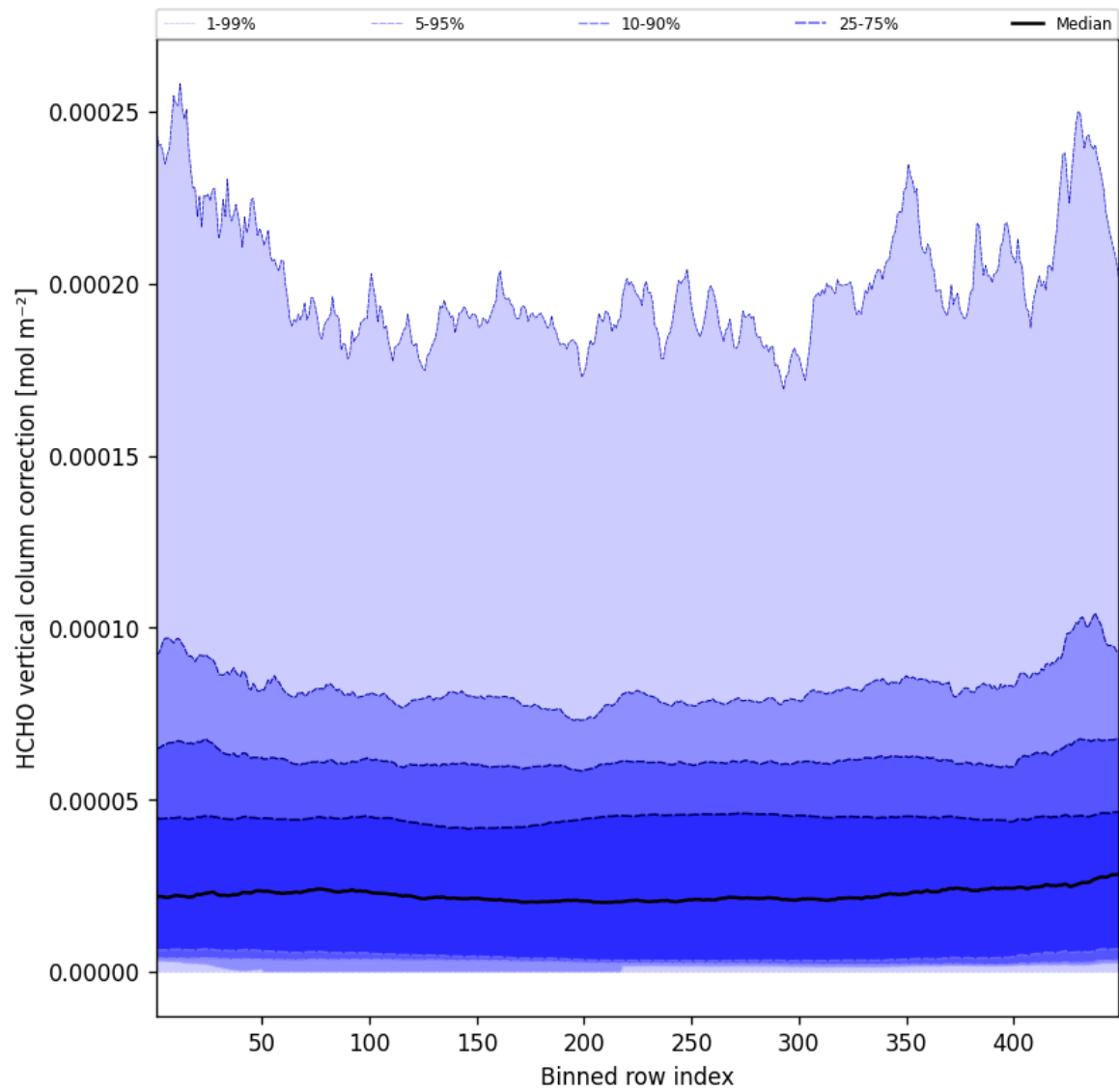
Figure 49: Along track statistics of “HCHO vertical column correction” for 2025-01-20 to 2025-01-21
