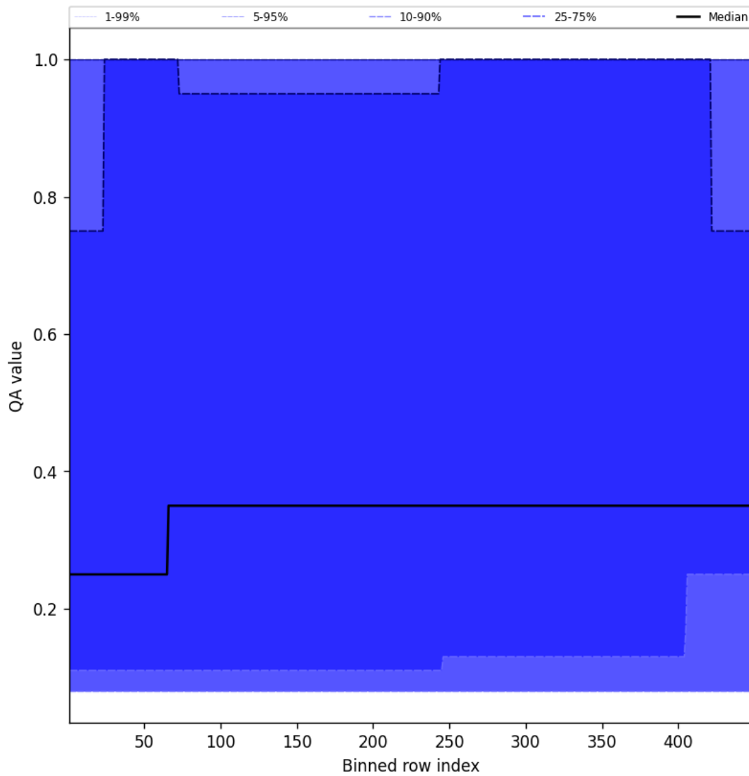
Figure 46: Along track statistics of “QA value” for 2025-01-20 to 2025-01-21
