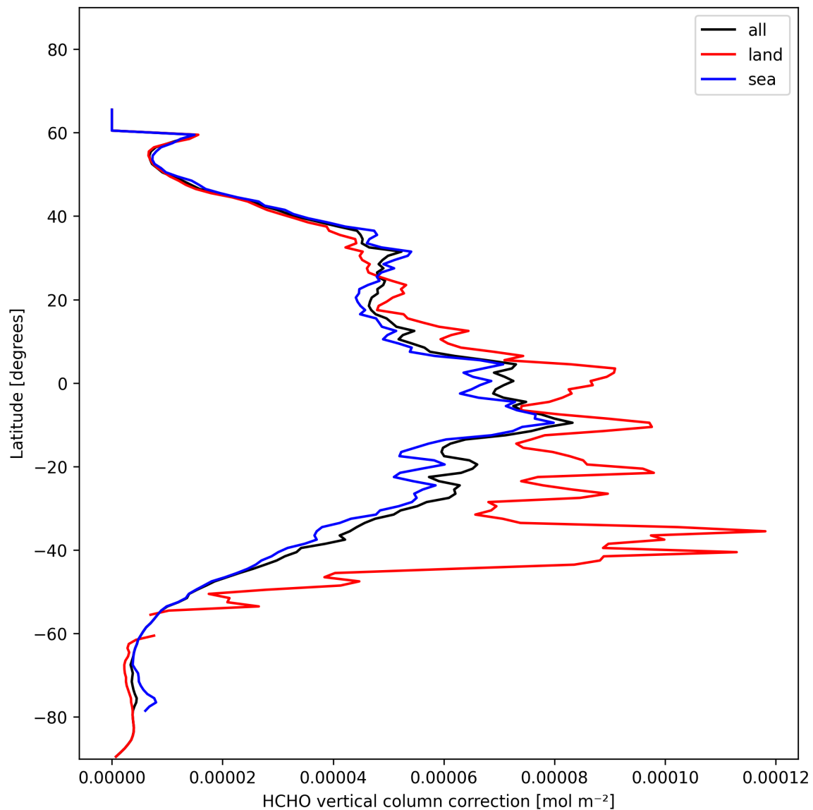
Figure 21: Zonal average of “HCHO vertical column correction” for 2025-01-20 to 2025-01-21.
