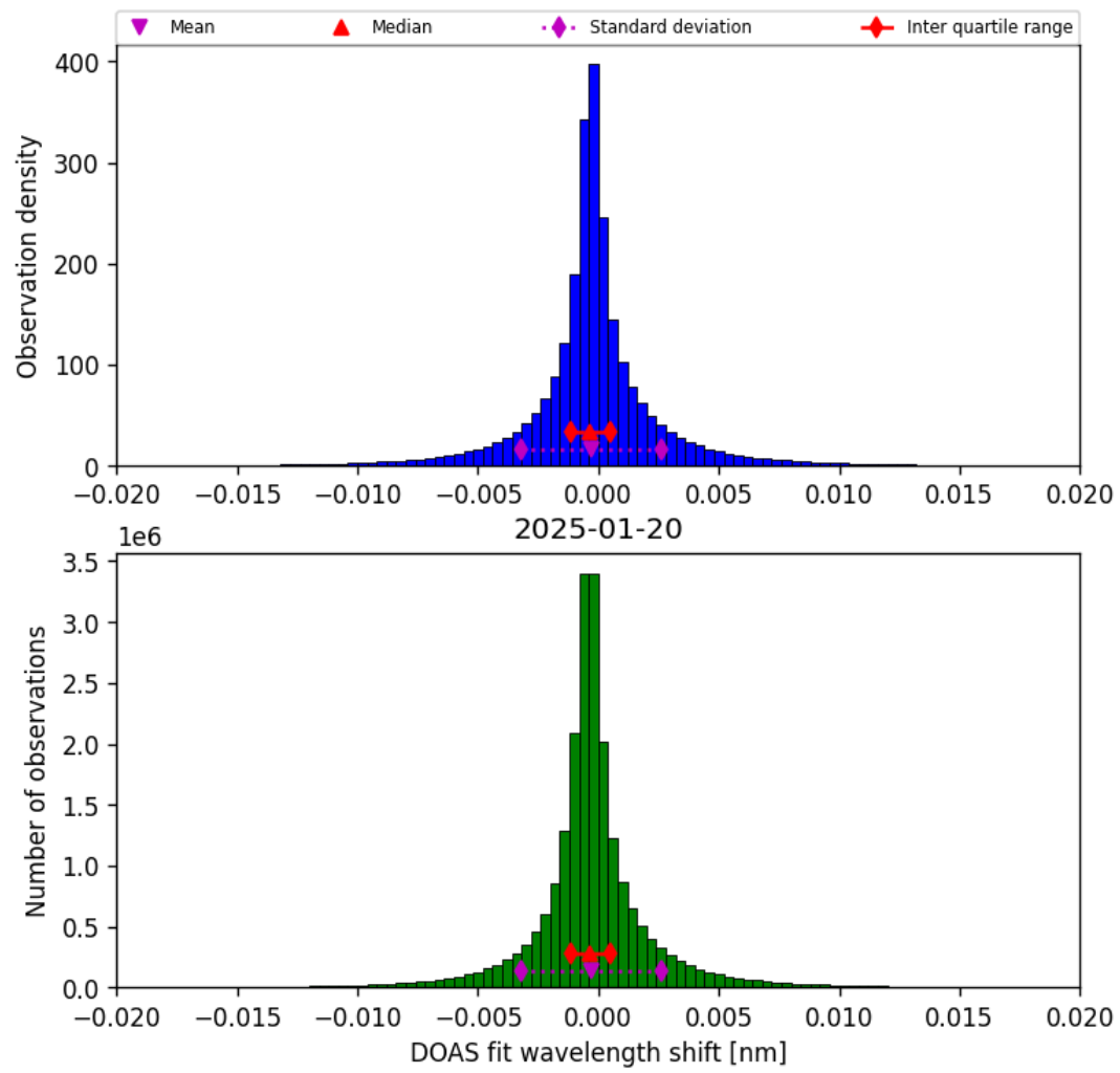
Figure 42: Histogram of “DOAS fit wavelength shift” for 2025-01-20 to 2025-01-21
