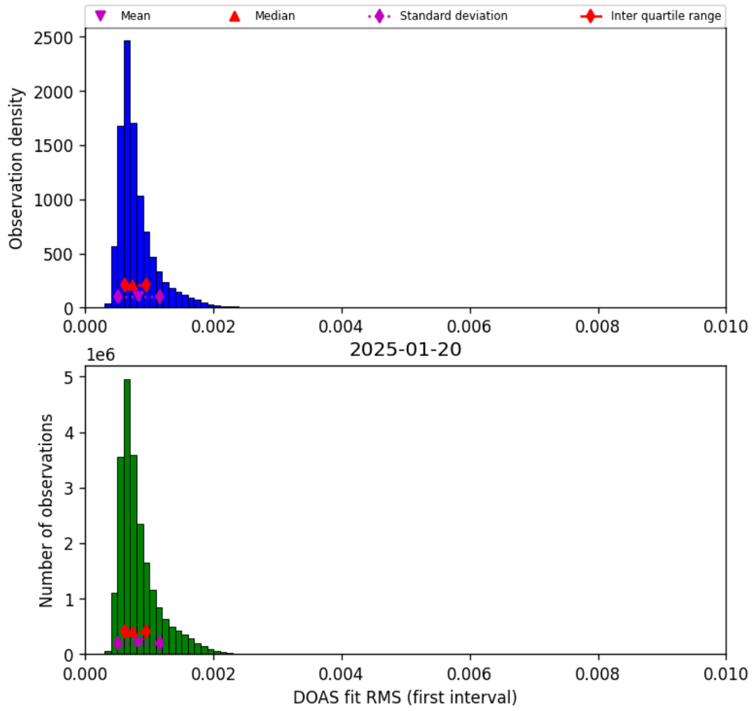
Figure 44: Histogram of “DOAS fit RMS (first interval)” for 2025-01-20 to 2025-01-21
