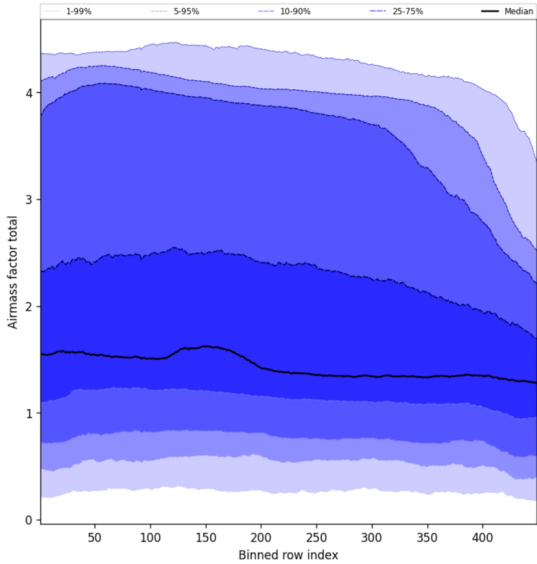
Figure 52: Along track statistics of “Airmass factor total” for 2025-01-20 to 2025-01-21
