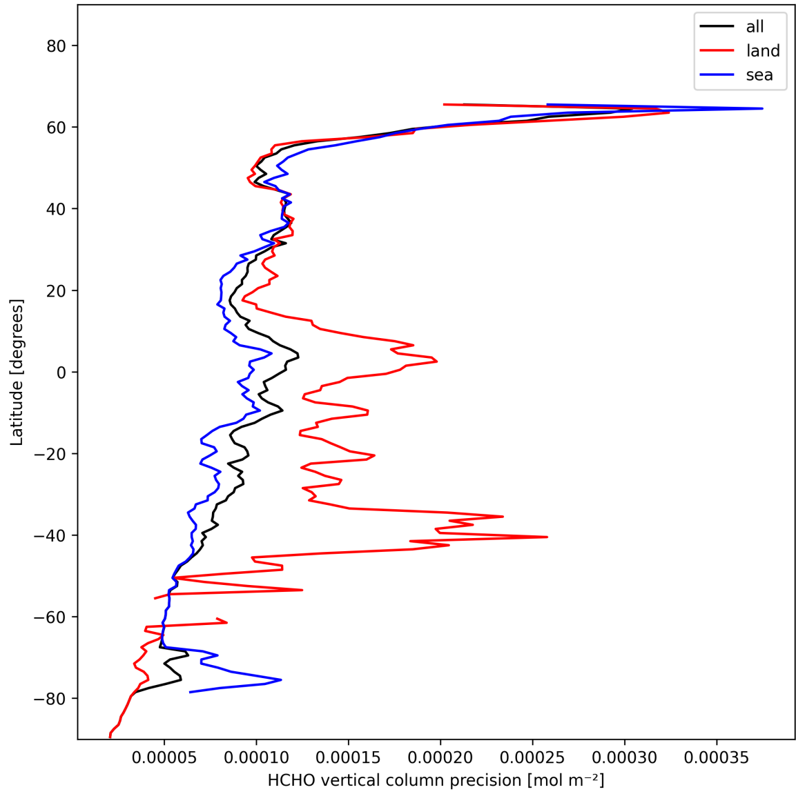
Figure 20: Zonal average of “HCHO vertical column precision” for 2025-01-20 to 2025-01-21.
