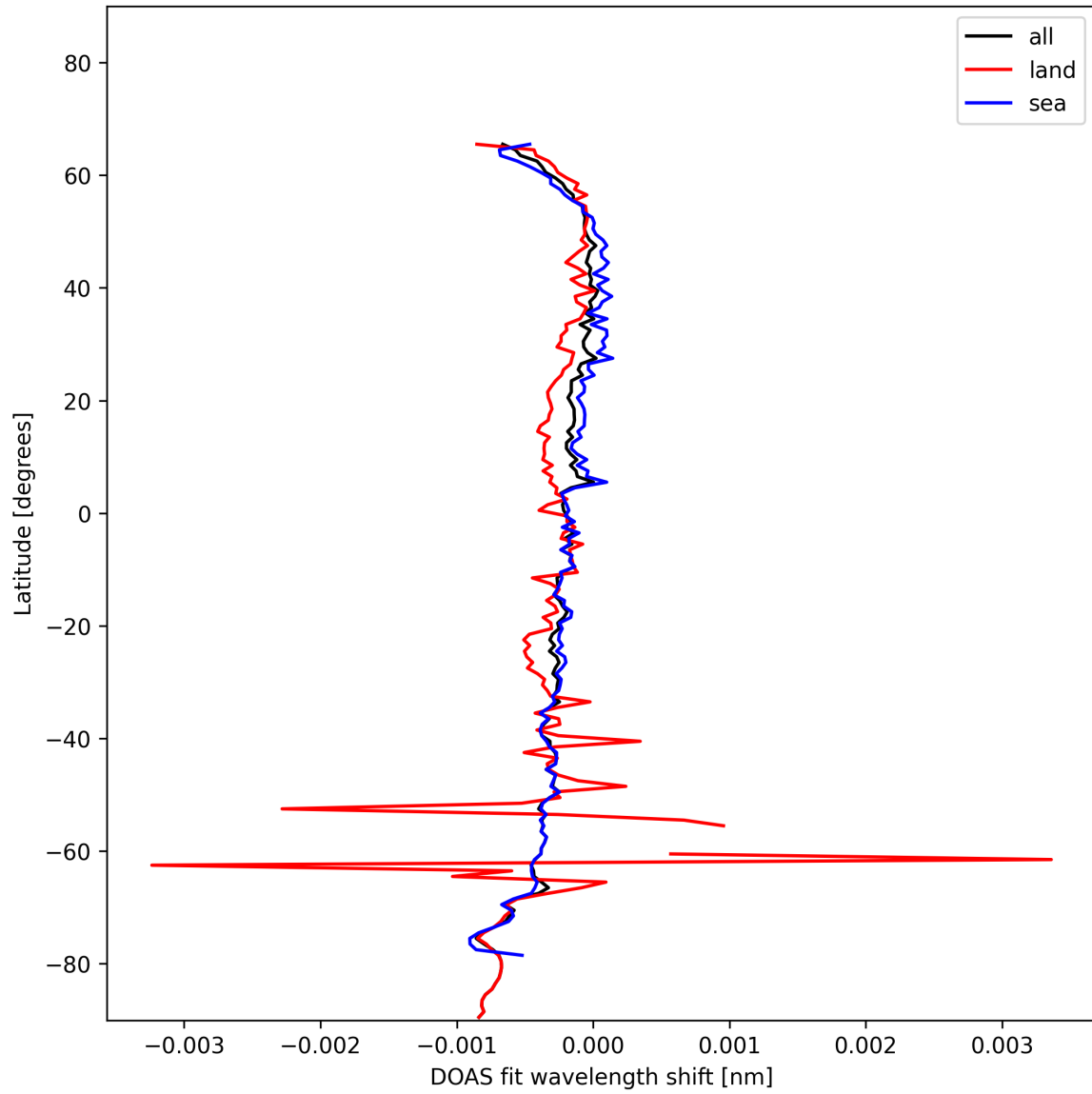
Figure 28: Zonal average of “DOAS fit wavelength shift” for 2025-01-20 to 2025-01-21.
