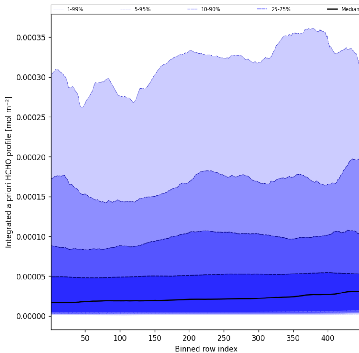
Figure 55: Along track statistics of “Integrated a priori HCHO profile” for 2025-01-20 to 2025-01-21
