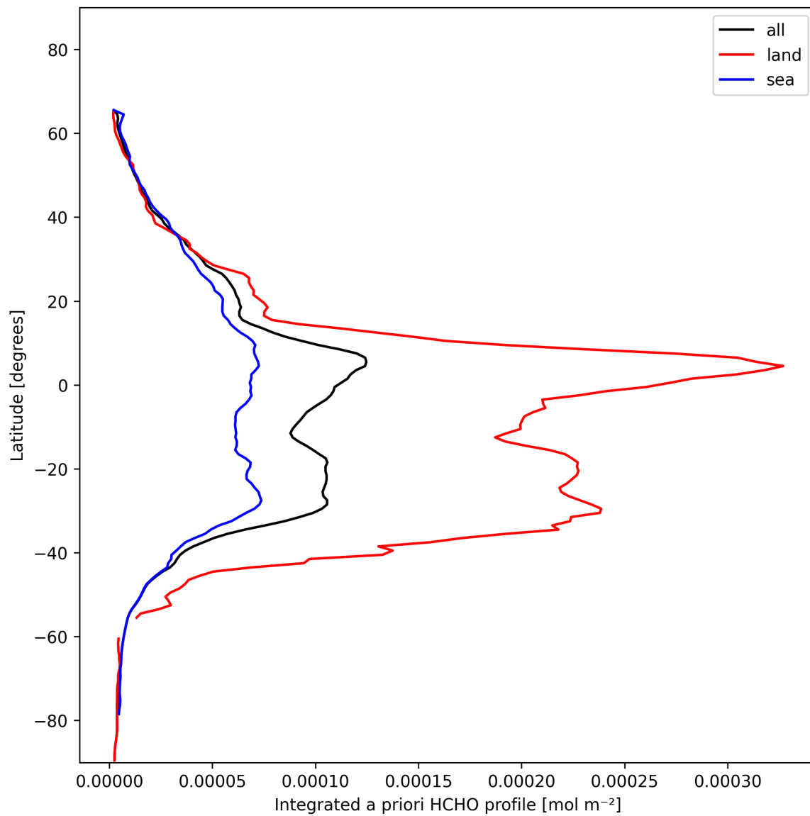
Figure 27: Zonal average of “Integrated a priori HCHO profile” for 2025-01-20 to 2025-01-21.
