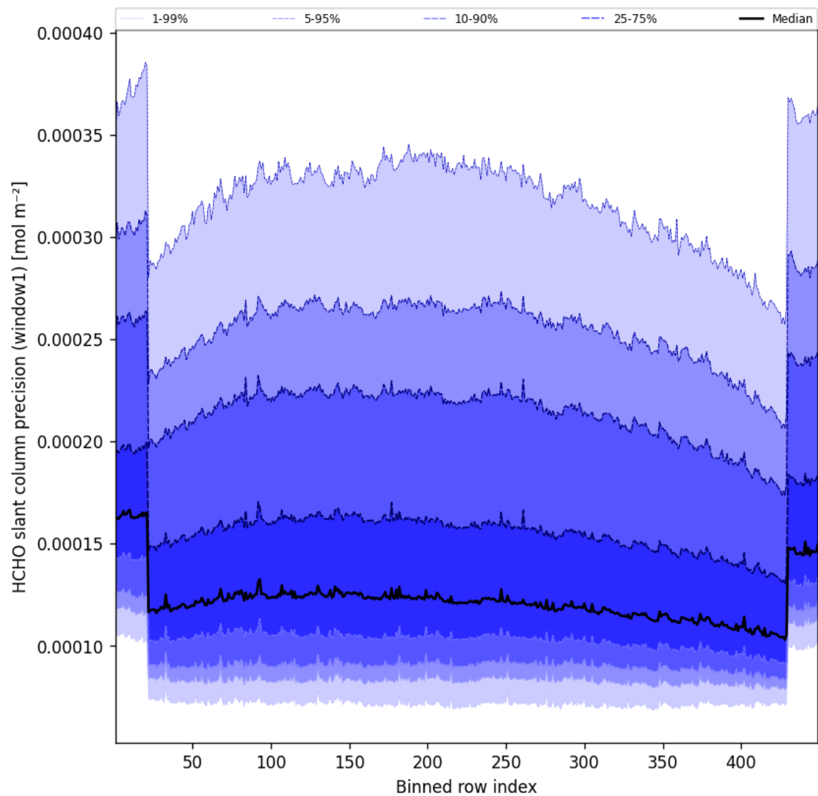
Figure 51: Along track statistics of “HCHO slant column precision (window1)” for 2025-01-20 to 2025-01-21
