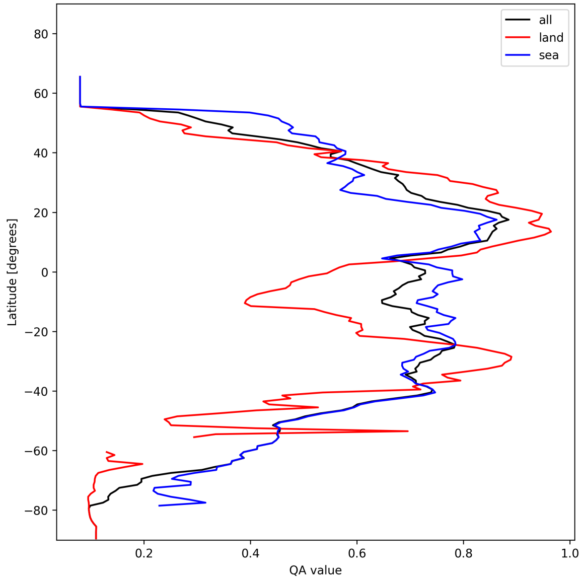
Figure 18: Zonal average of “QA value” for 2025-01-20 to 2025-01-21.
