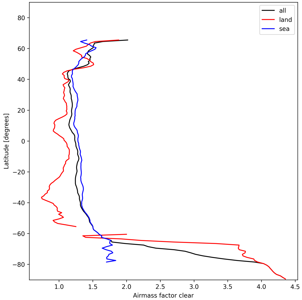
Figure 26: Zonal average of “Airmass factor clear” for 2025-01-20 to 2025-01-21.
