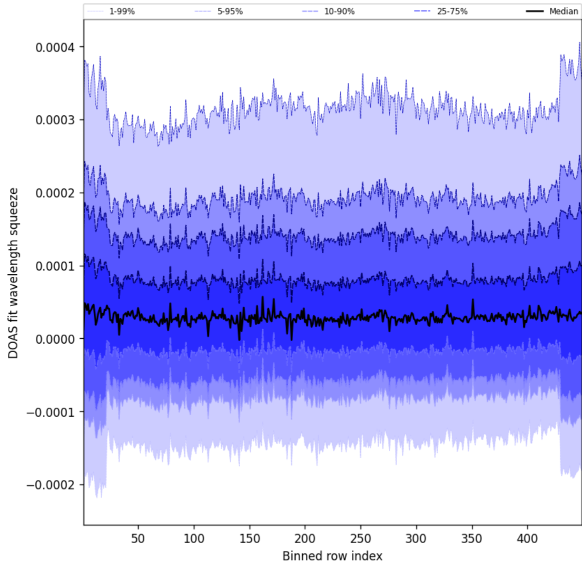
Figure 57: Along track statistics of “DOAS fit wavelength squeeze” for 2025-01-20 to 2025-01-21
