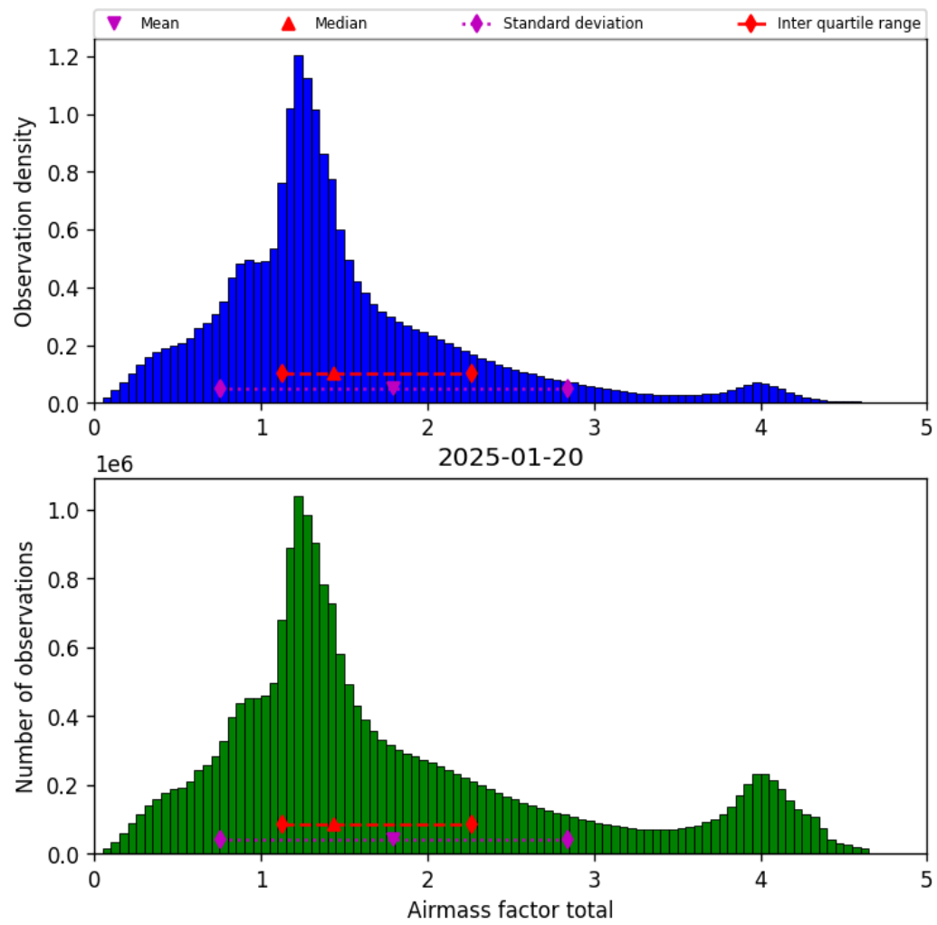
Figure 38: Histogram of “Airmass factor total” for 2025-01-20 to 2025-01-21
