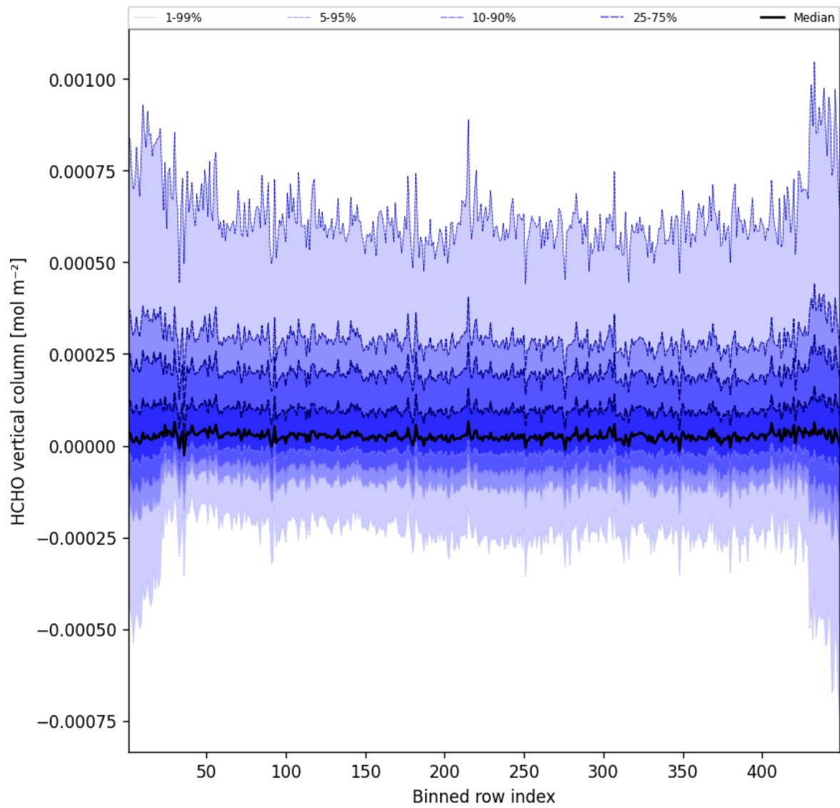
Figure 47: Along track statistics of “HCHO vertical column” for 2025-01-20 to 2025-01-21
