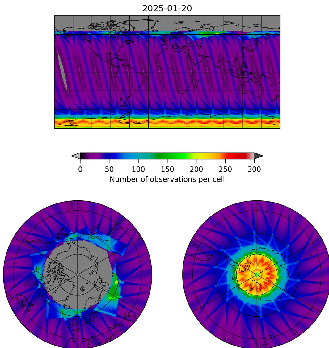
Figure 17: Map of the number of observations for 2025-01-20 to 2025-01-21
