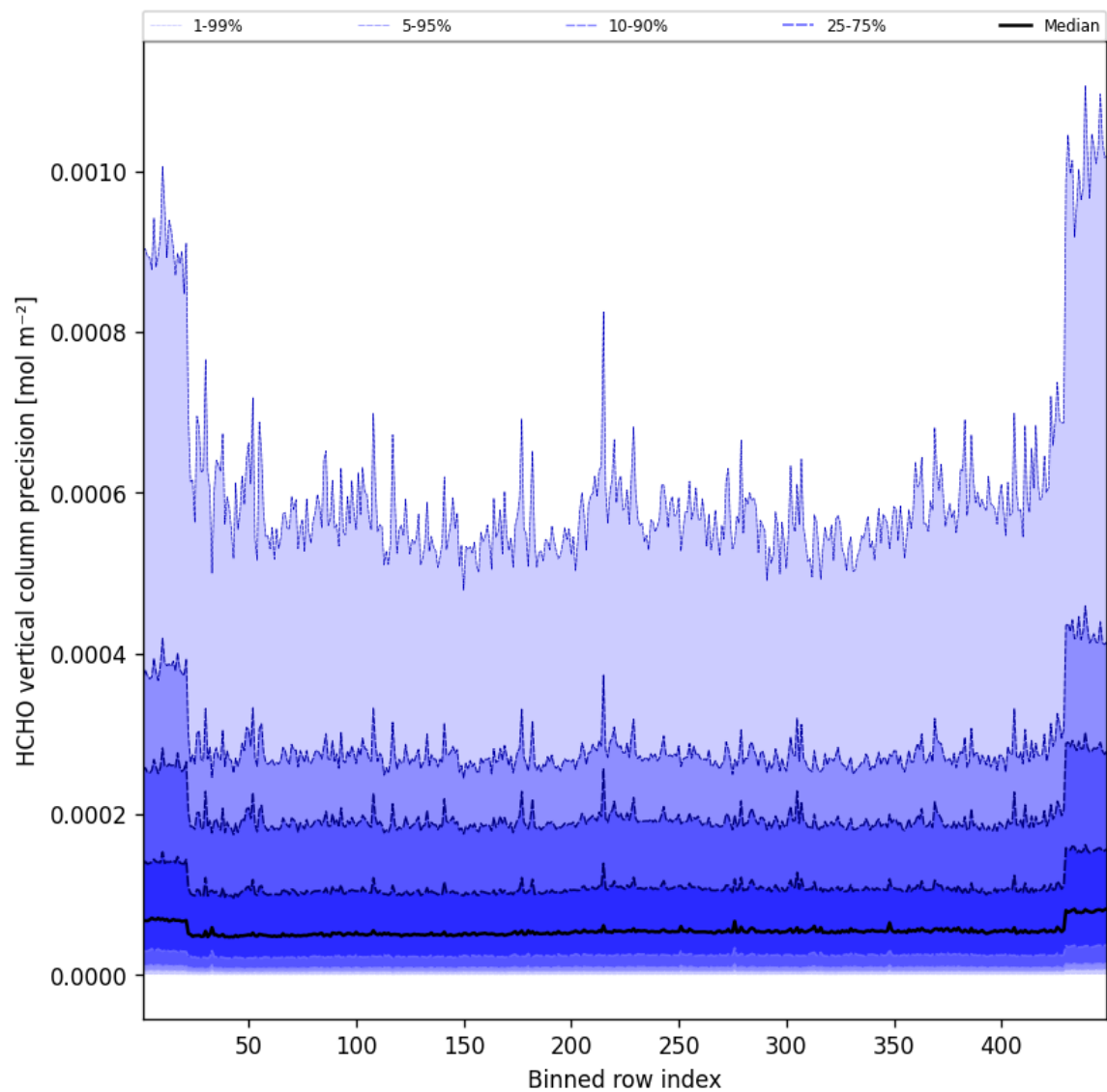
Figure 48: Along track statistics of “HCHO vertical column precision” for 2025-01-20 to 2025-01-21
