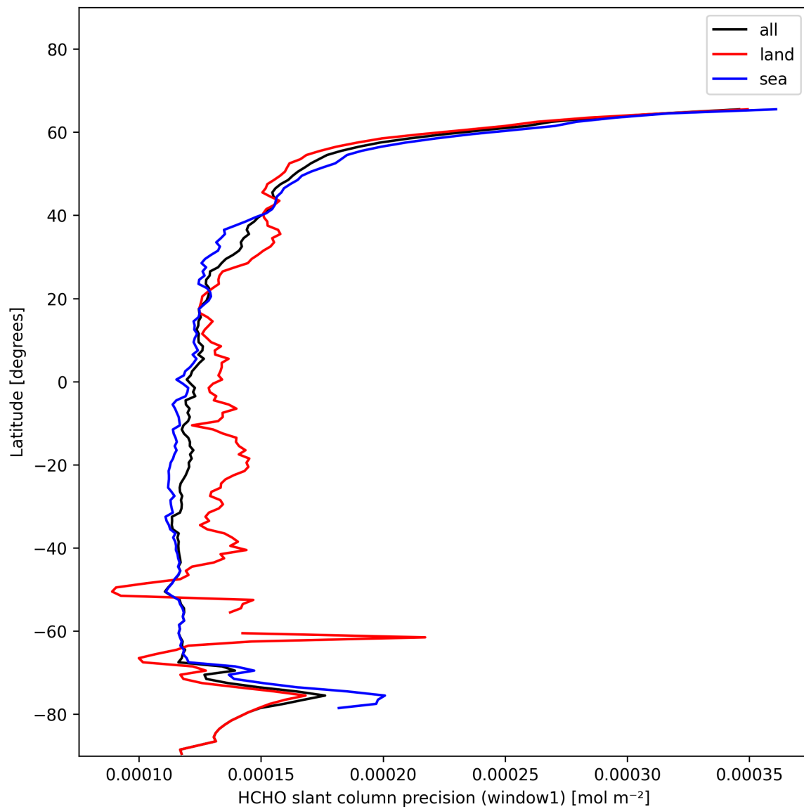
Figure 23: Zonal average of “HCHO slant column precision (window1)” for 2025-01-20 to 2025-01-21.
