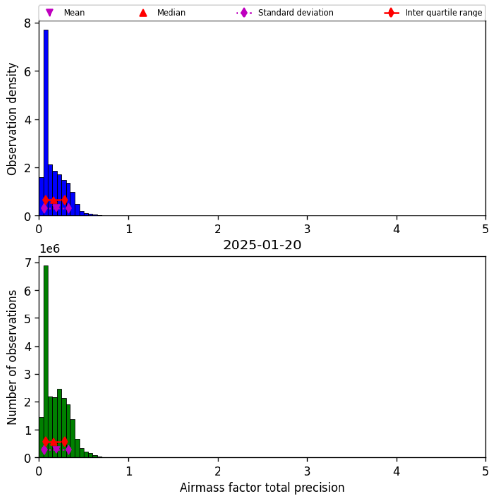
Figure 39: Histogram of “Airmass factor total precision” for 2025-01-20 to 2025-01-21
