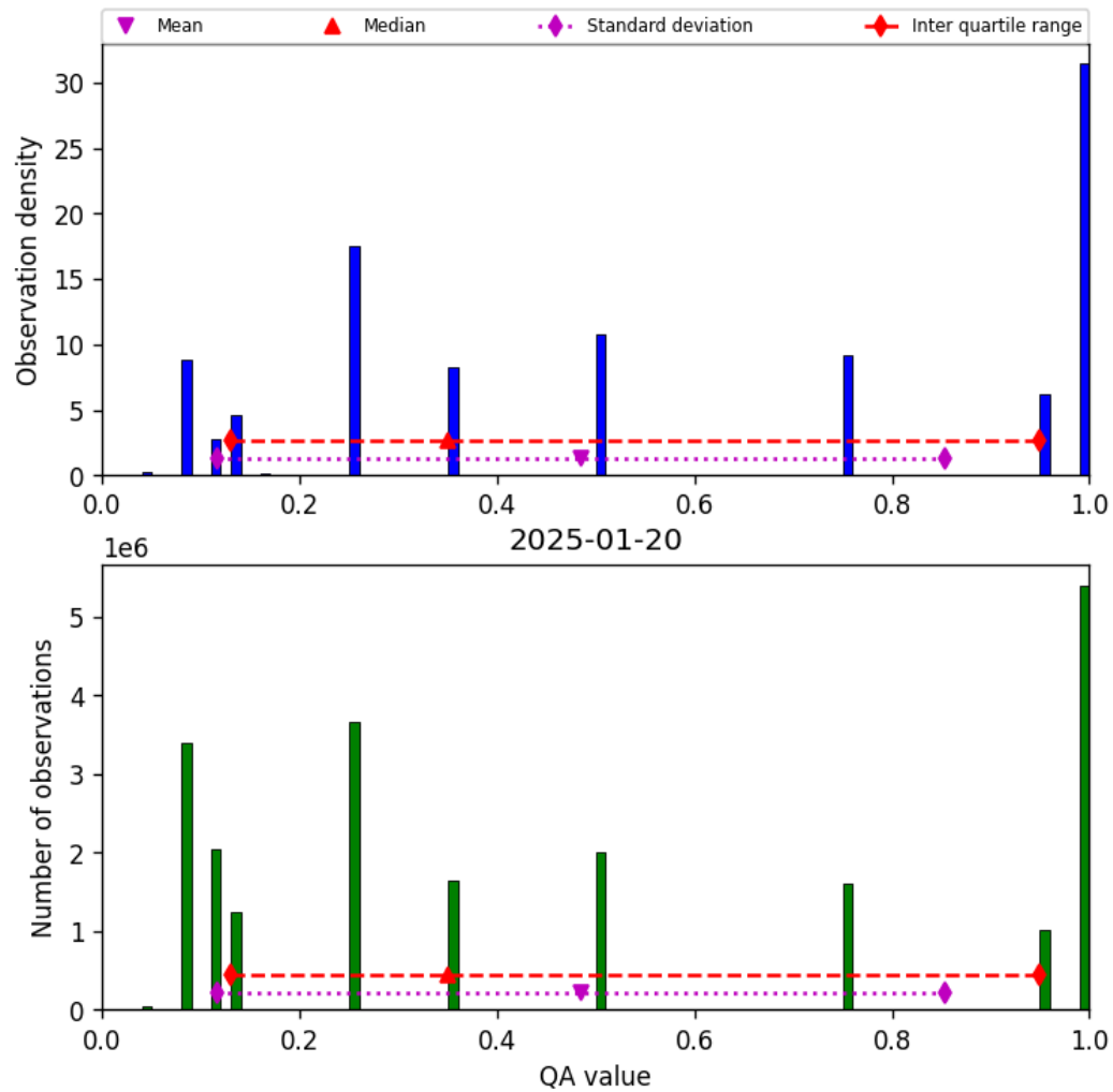
Figure 32: Histogram of “QA value” for 2025-01-20 to 2025-01-21
