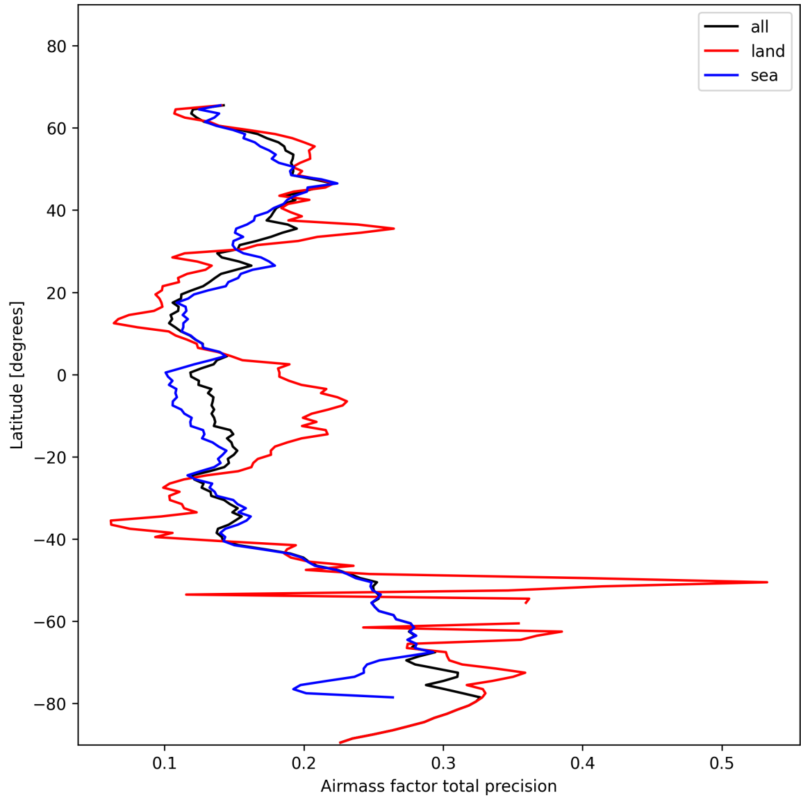
Figure 25: Zonal average of “Airmass factor total precision” for 2025-01-20 to 2025-01-21.
