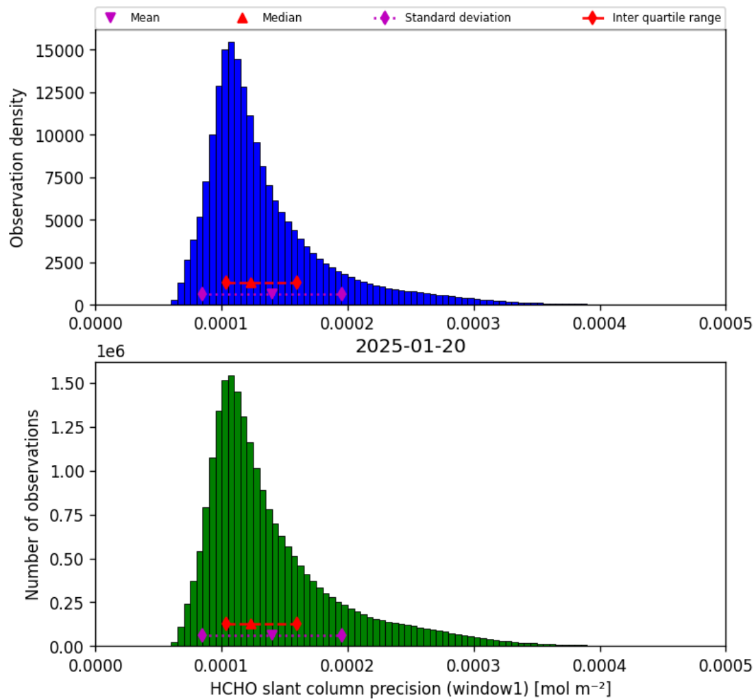
Figure 37: Histogram of “HCHO slant column precision (window1)” for 2025-01-20 to 2025-01-21
