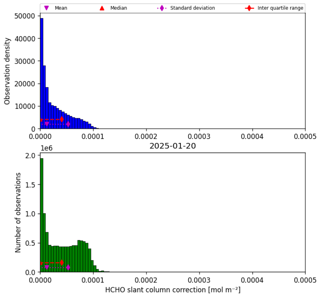
Figure 45: Histogram of “HCHO slant column correction” for 2025-01-20 to 2025-01-21
