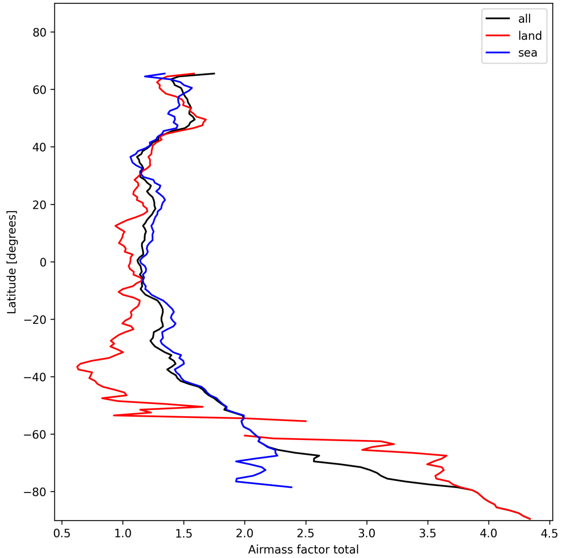
Figure 24: Zonal average of “Airmass factor total” for 2025-01-20 to 2025-01-21.
