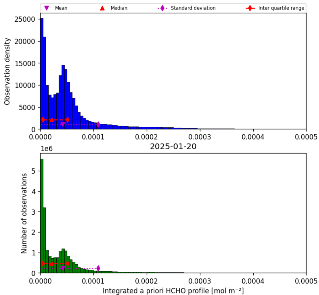
Figure 41: Histogram of “Integrated a priori HCHO profile” for 2025-01-20 to 2025-01-21
