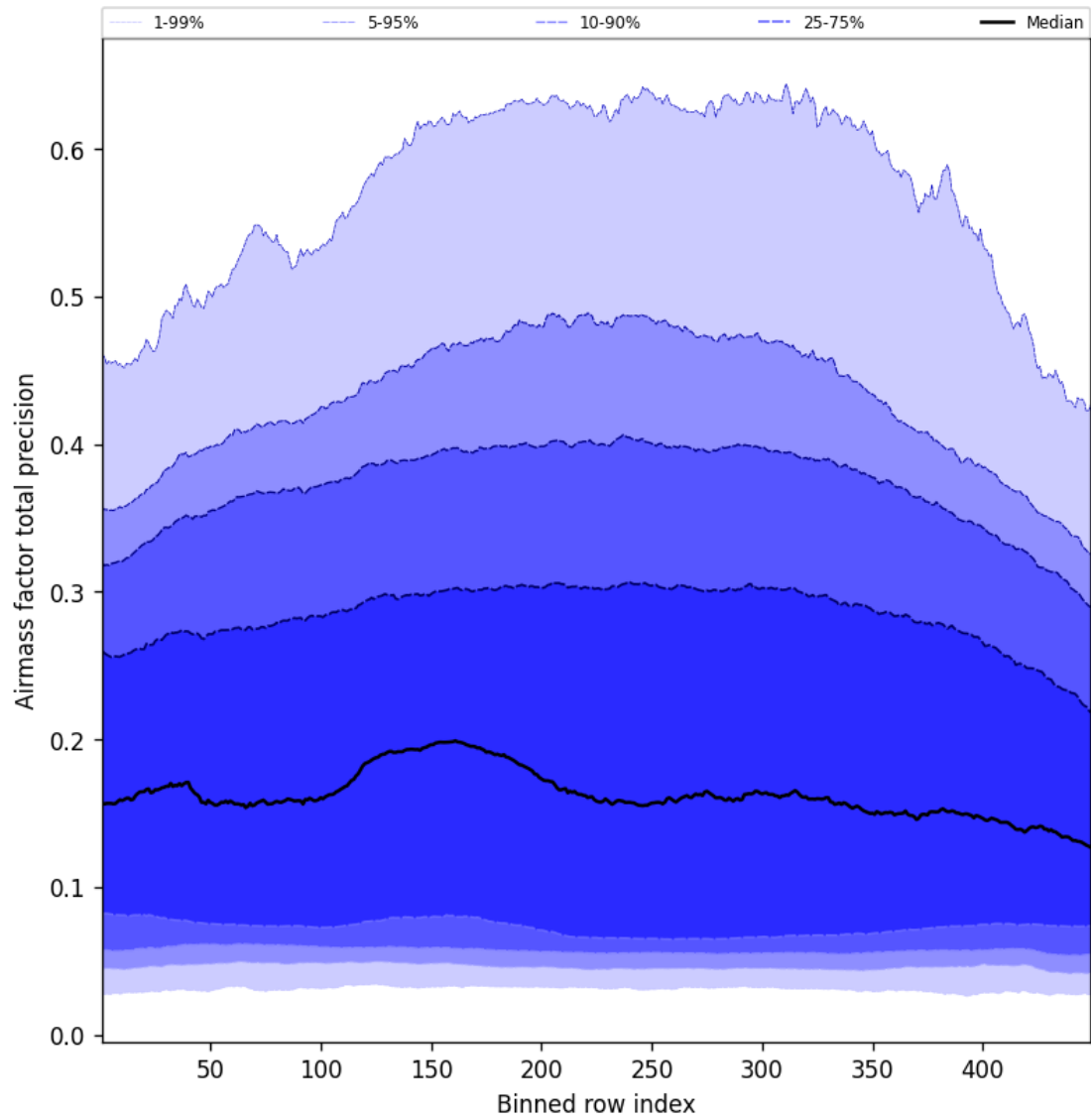
Figure 53: Along track statistics of “Airmass factor total precision” for 2025-01-20 to 2025-01-21
