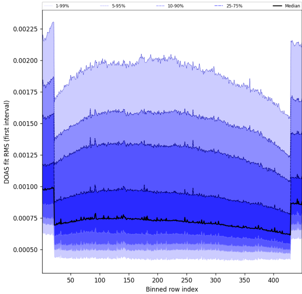
Figure 58: Along track statistics of “DOAS fit RMS (first interval)” for 2025-01-20 to 2025-01-21
