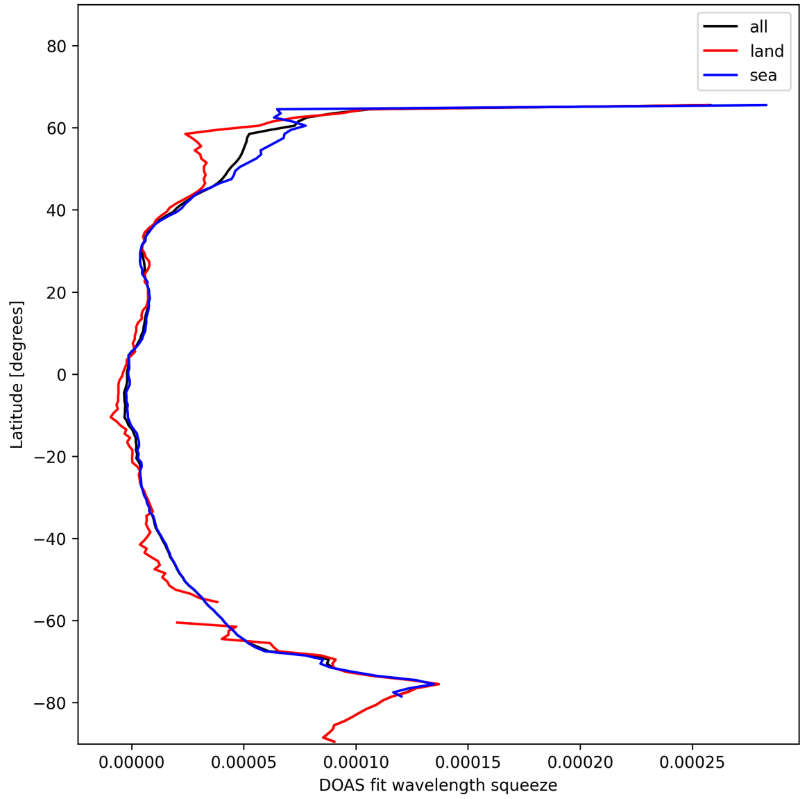
Figure 29: Zonal average of “DOAS fit wavelength squeeze” for 2025-01-20 to 2025-01-21.
