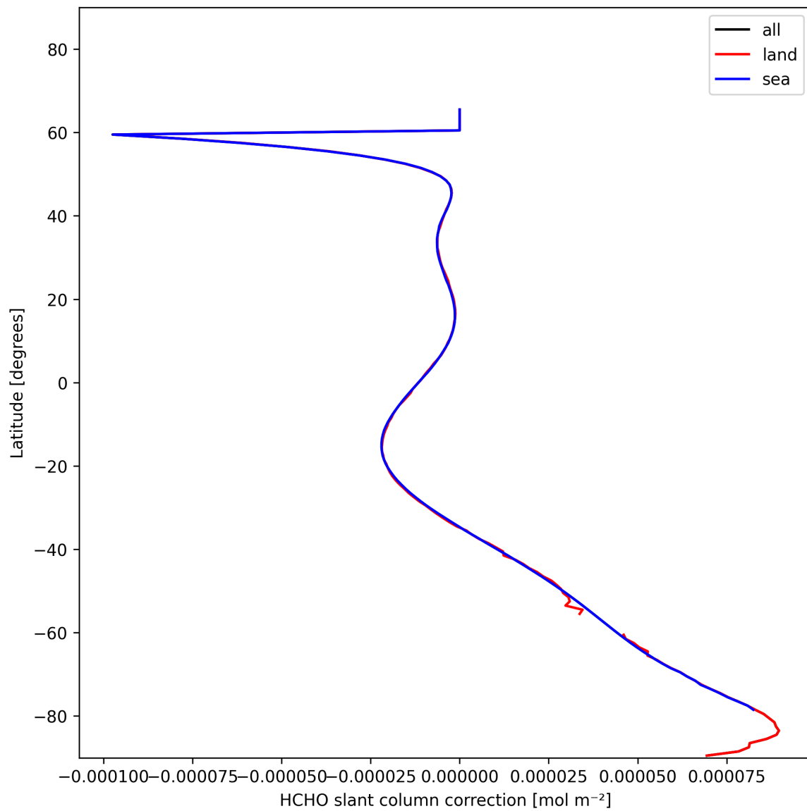
Figure 31: Zonal average of “HCHO slant column correction” for 2025-01-20 to 2025-01-21.
