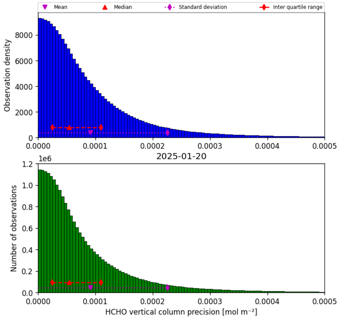
Figure 34: Histogram of “HCHO vertical column precision” for 2025-01-20 to 2025-01-21
