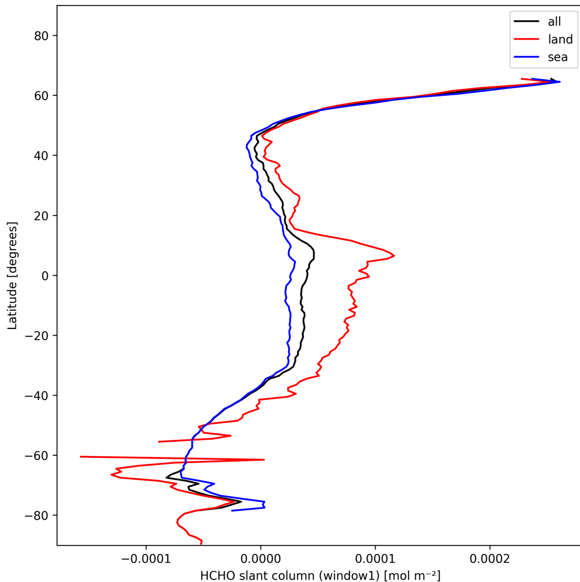
Figure 22: Zonal average of “HCHO slant column (window1)” for 2025-01-20 to 2025-01-21.
