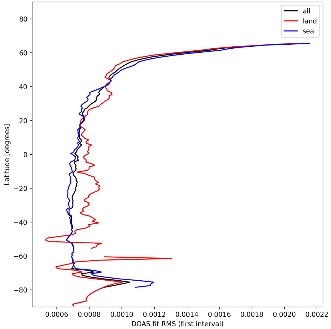
Figure 30: Zonal average of “DOAS fit RMS (first interval)” for 2025-01-20 to 2025-01-21.
