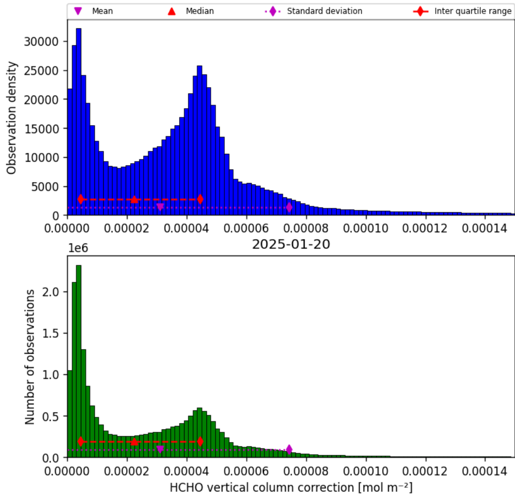
Figure 35: Histogram of “HCHO vertical column correction” for 2025-01-20 to 2025-01-21
