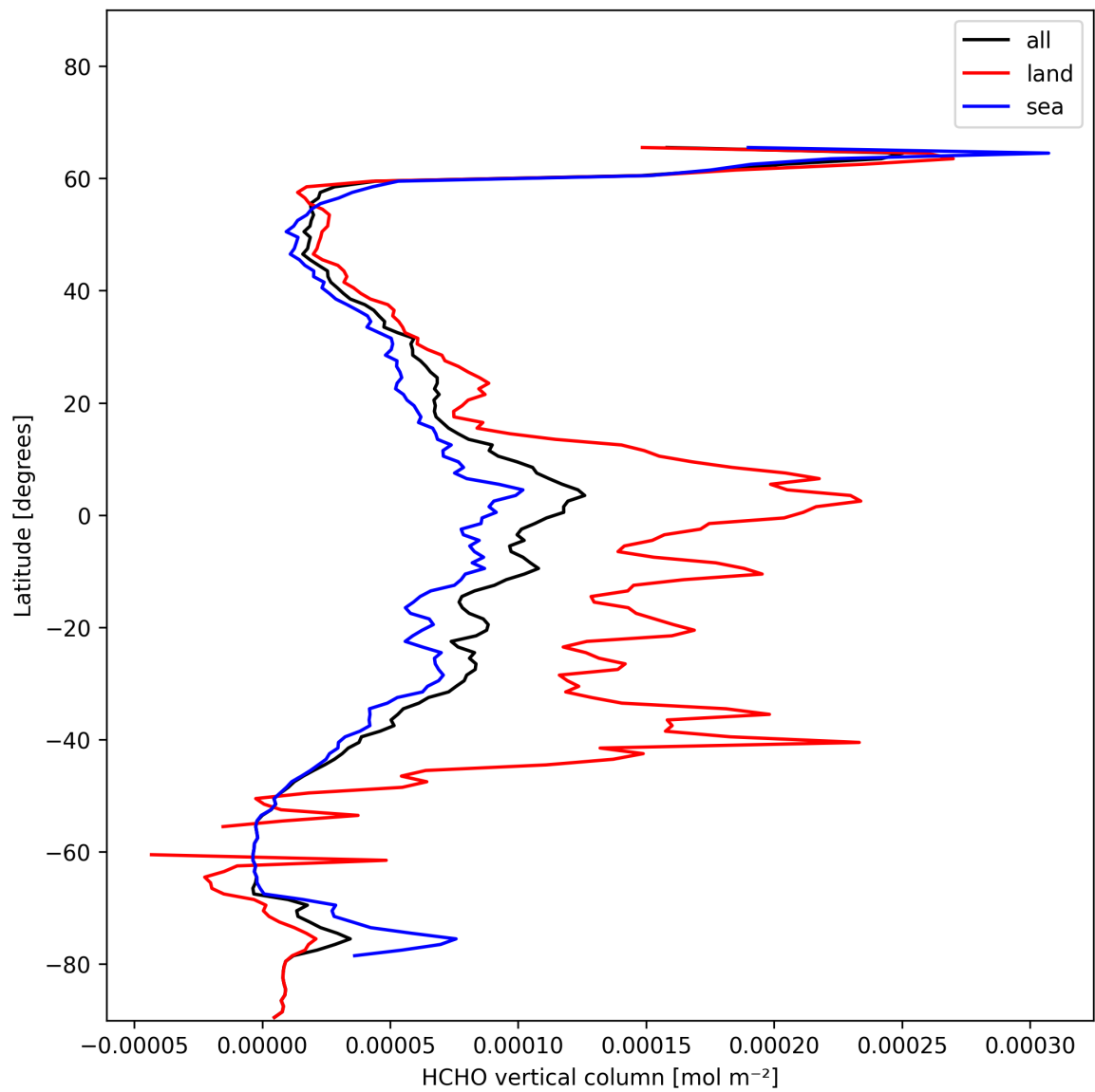
Figure 19: Zonal average of “HCHO vertical column” for 2025-01-20 to 2025-01-21.
