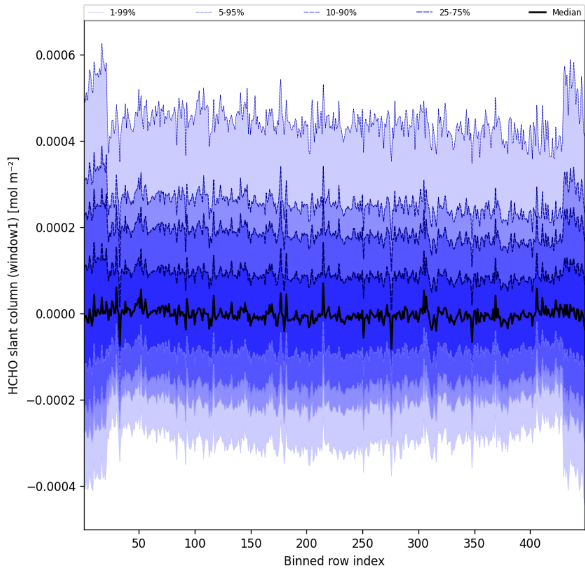
Figure 50: Along track statistics of “HCHO slant column (window1)” for 2025-01-20 to 2025-01-21
