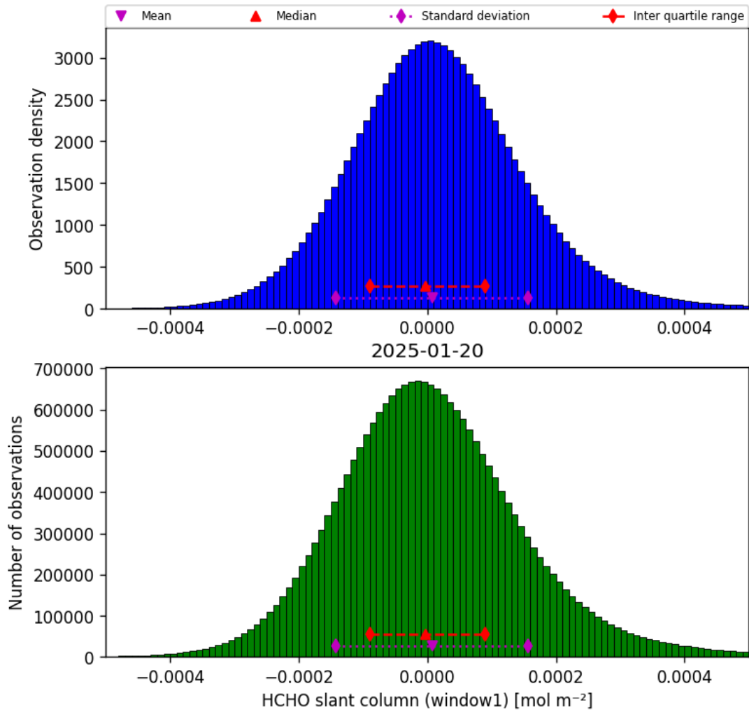
Figure 36: Histogram of “HCHO slant column (window1)” for 2025-01-20 to 2025-01-21
