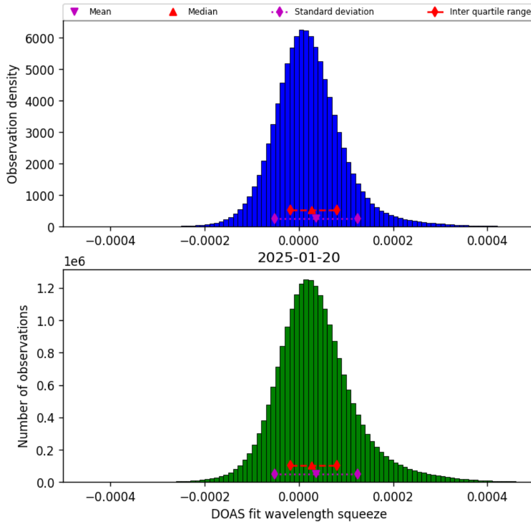
Figure 43: Histogram of “DOAS fit wavelength squeeze” for 2025-01-20 to 2025-01-21
