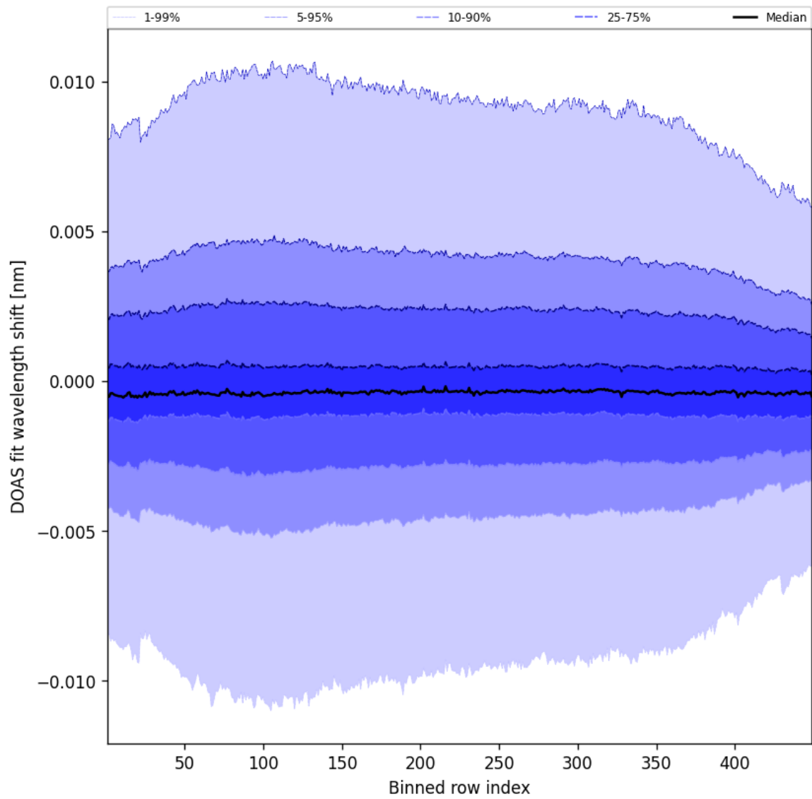
Figure 56: Along track statistics of “DOAS fit wavelength shift” for 2025-01-20 to 2025-01-21
