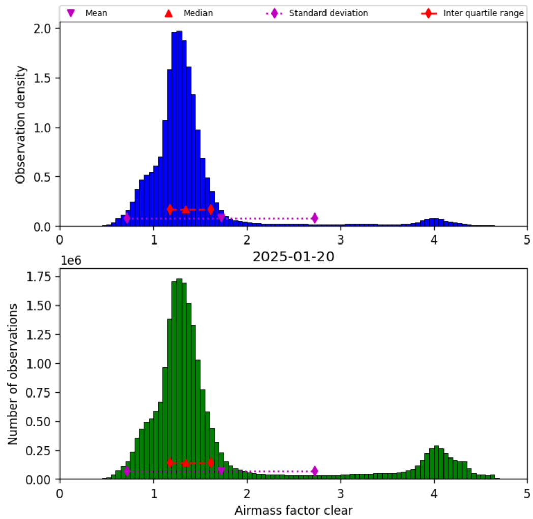
Figure 40: Histogram of “Airmass factor clear” for 2025-01-20 to 2025-01-21
