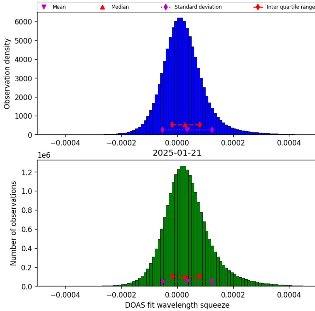
Figure 43: Histogram of “DOAS fit wavelength squeeze” for 2025-01-21 to 2025-01-21
