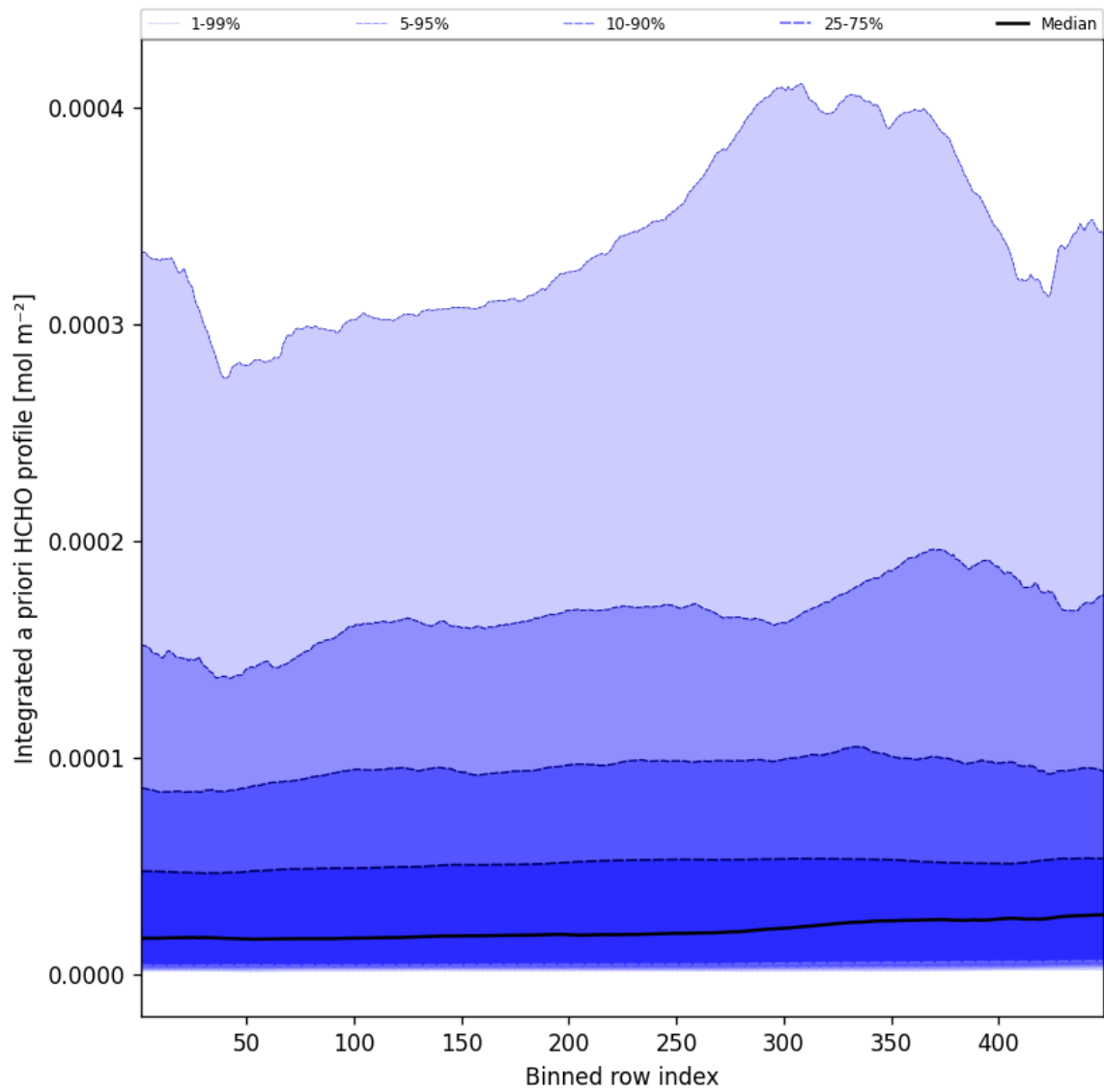
Figure 55: Along track statistics of “Integrated a priori HCHO profile” for 2025-01-21 to 2025-01-21
