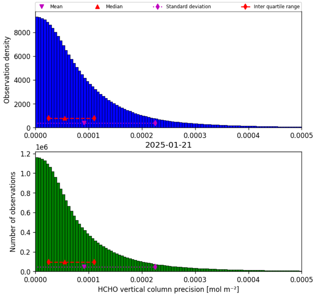
Figure 34: Histogram of “HCHO vertical column precision” for 2025-01-21 to 2025-01-21
