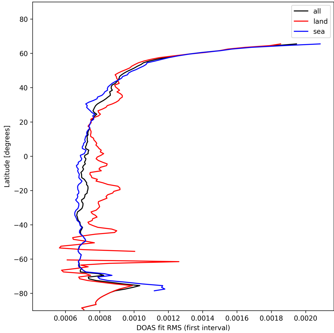
Figure 30: Zonal average of “DOAS fit RMS (first interval)” for 2025-01-21 to 2025-01-21.
