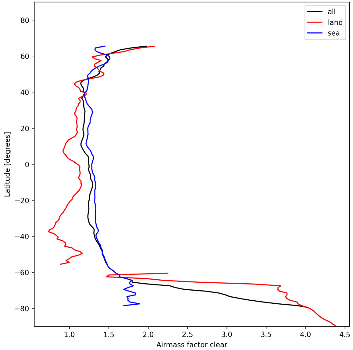
Figure 26: Zonal average of “Airmass factor clear” for 2025-01-21 to 2025-01-21.
