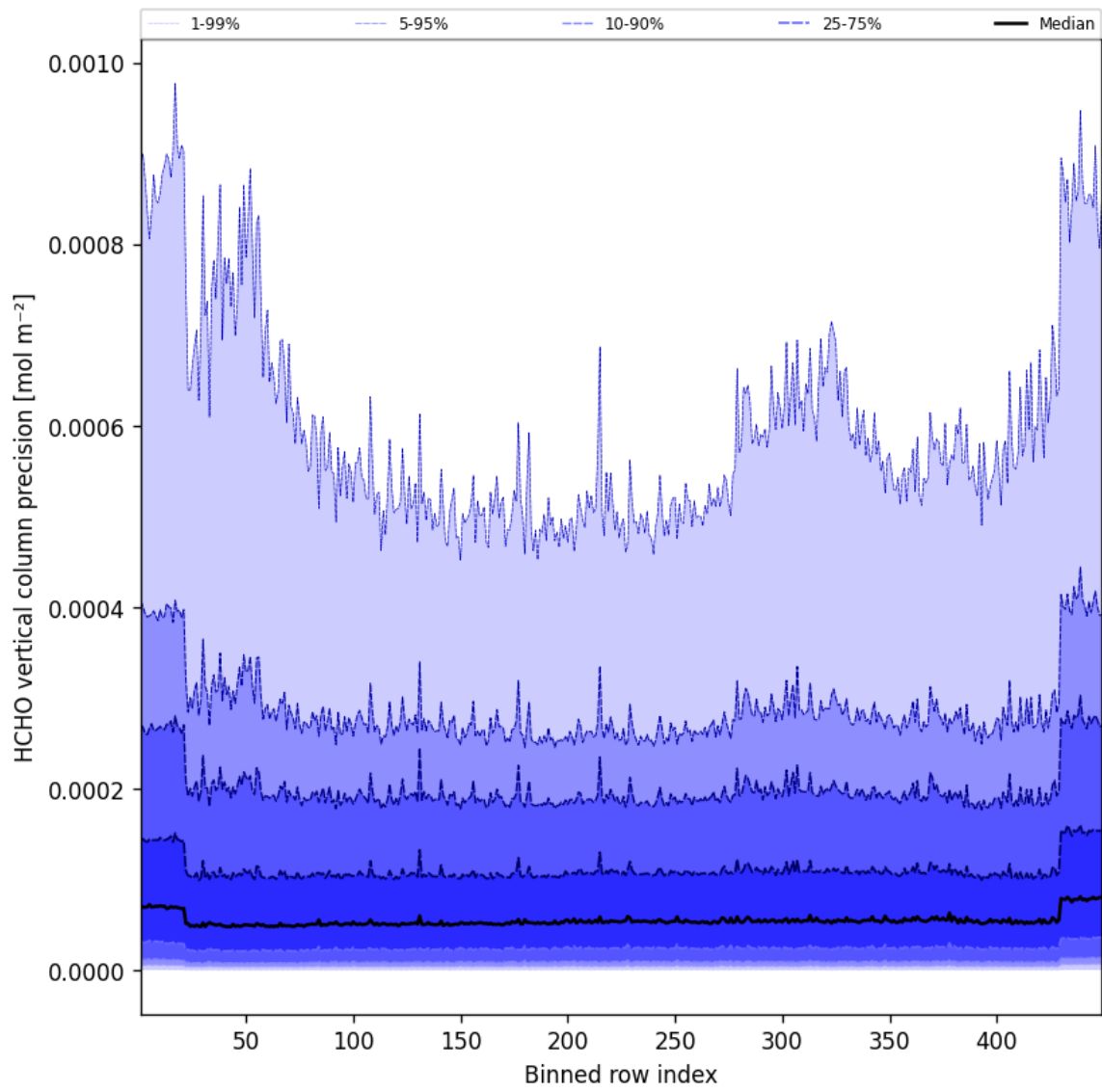
Figure 48: Along track statistics of “HCHO vertical column precision” for 2025-01-21 to 2025-01-21
