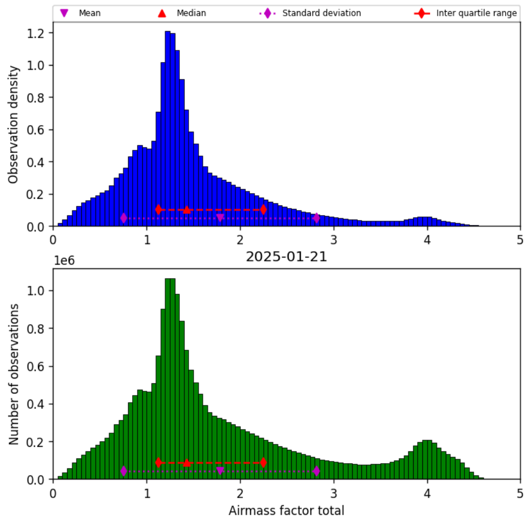
Figure 38: Histogram of “Airmass factor total” for 2025-01-21 to 2025-01-21
