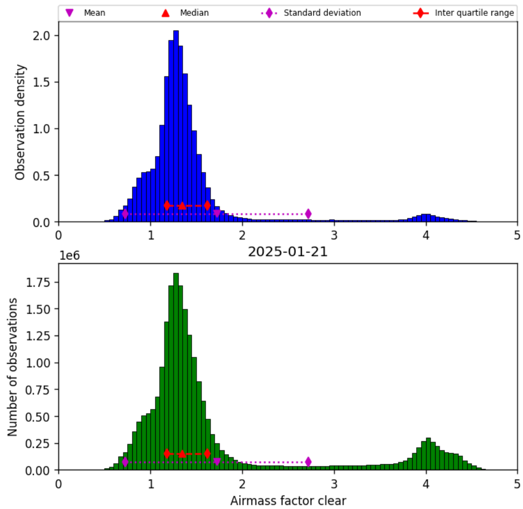
Figure 40: Histogram of “Airmass factor clear” for 2025-01-21 to 2025-01-21
