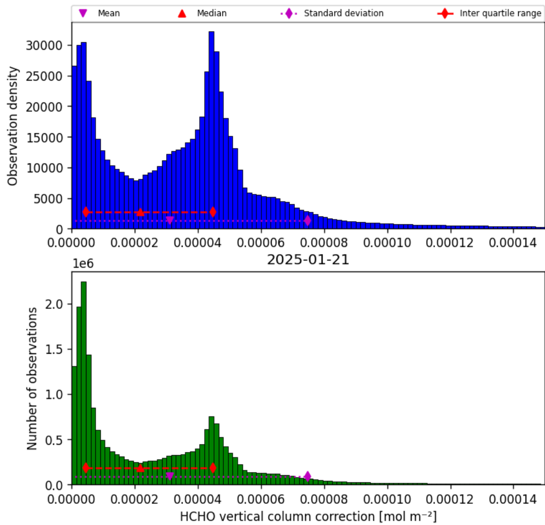
Figure 35: Histogram of “HCHO vertical column correction” for 2025-01-21 to 2025-01-21
