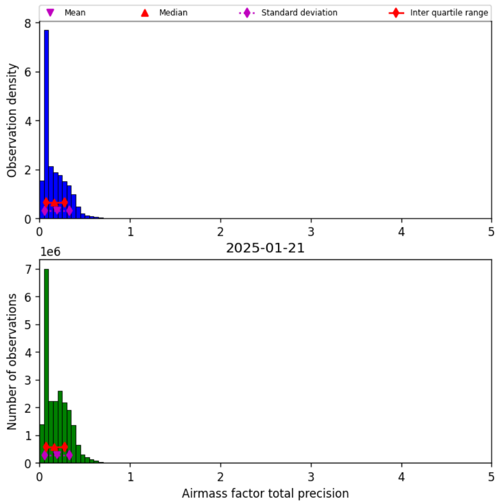
Figure 39: Histogram of “Airmass factor total precision” for 2025-01-21 to 2025-01-21
