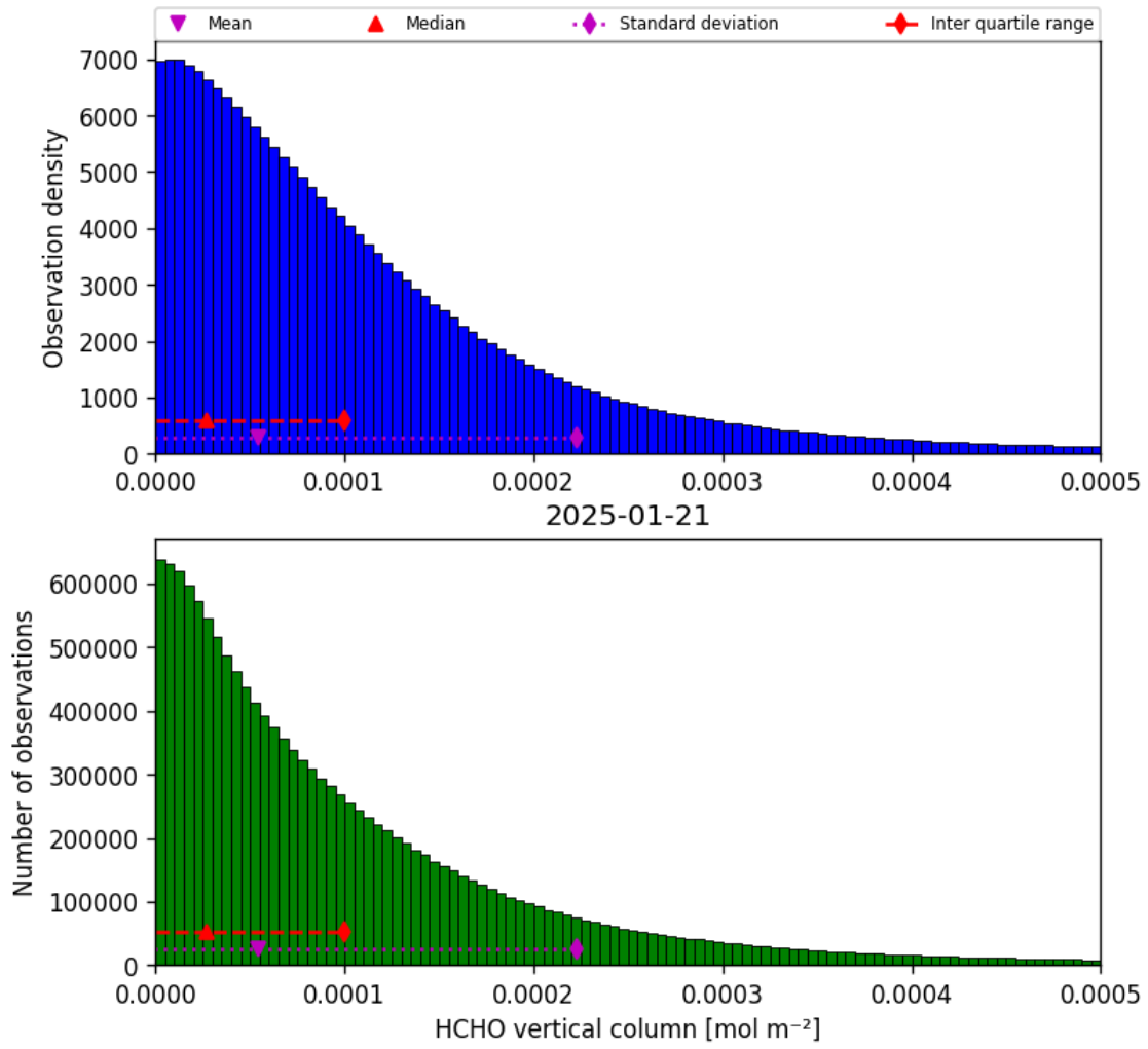
Figure 33: Histogram of “HCHO vertical column” for 2025-01-21 to 2025-01-21
