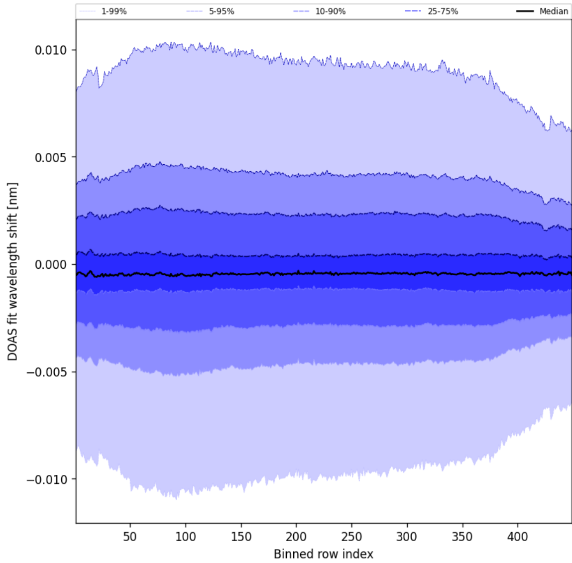
Figure 56: Along track statistics of “DOAS fit wavelength shift” for 2025-01-21 to 2025-01-21
