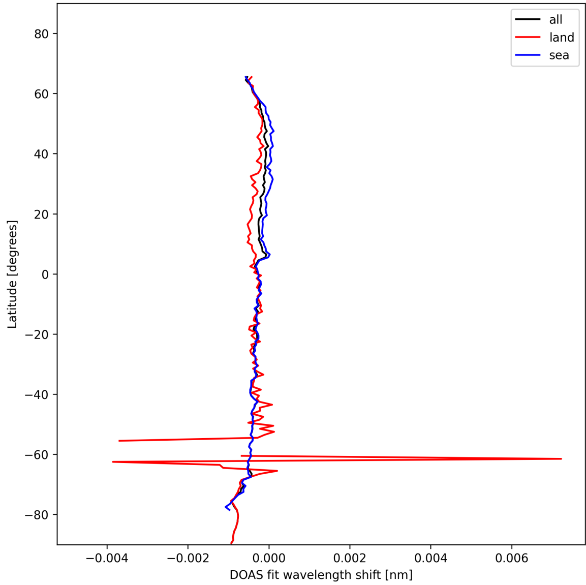
Figure 28: Zonal average of “DOAS fit wavelength shift” for 2025-01-21 to 2025-01-21.
