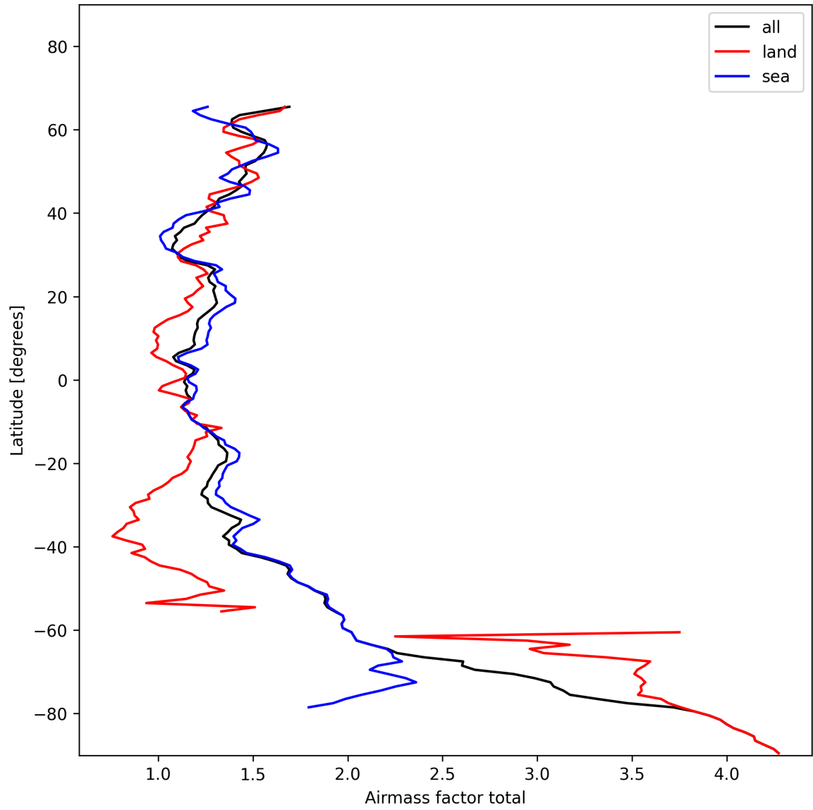
Figure 24: Zonal average of “Airmass factor total” for 2025-01-21 to 2025-01-21.
