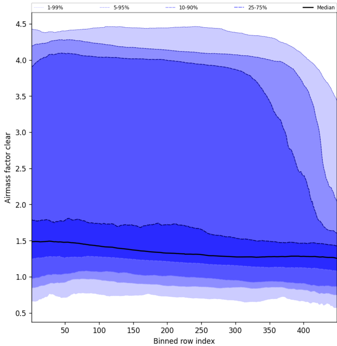
Figure 54: Along track statistics of “Airmass factor clear” for 2025-01-21 to 2025-01-21
