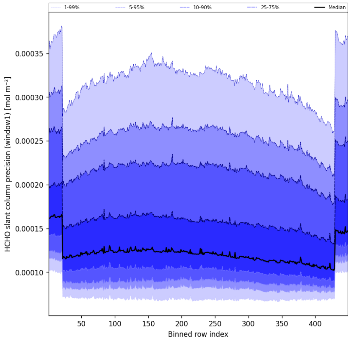
Figure 51: Along track statistics of “HCHO slant column precision (window1)” for 2025-01-21 to 2025-01-21
