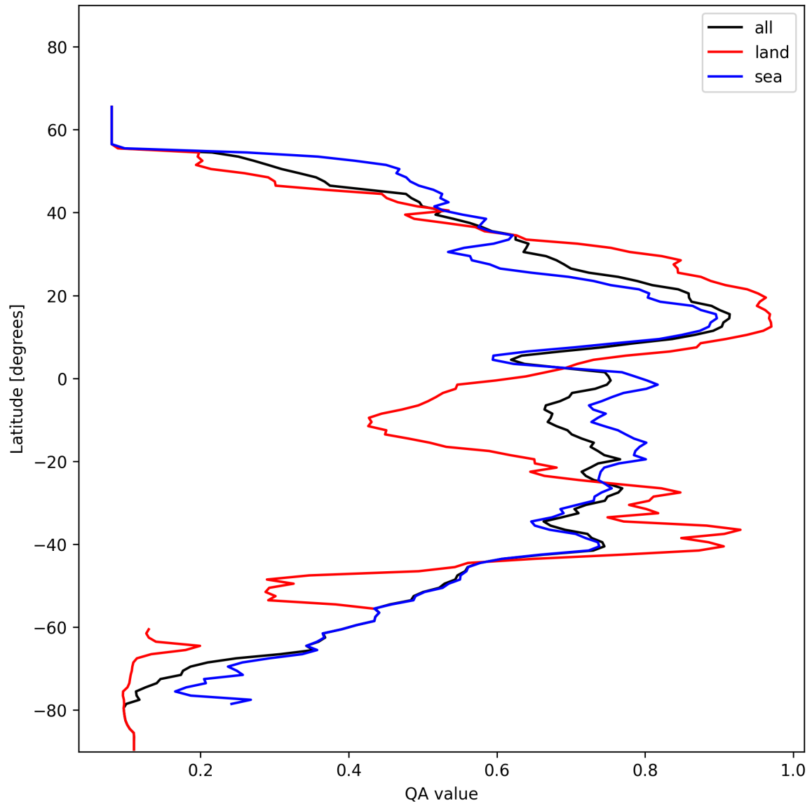
Figure 18: Zonal average of “QA value” for 2025-01-21 to 2025-01-21.
