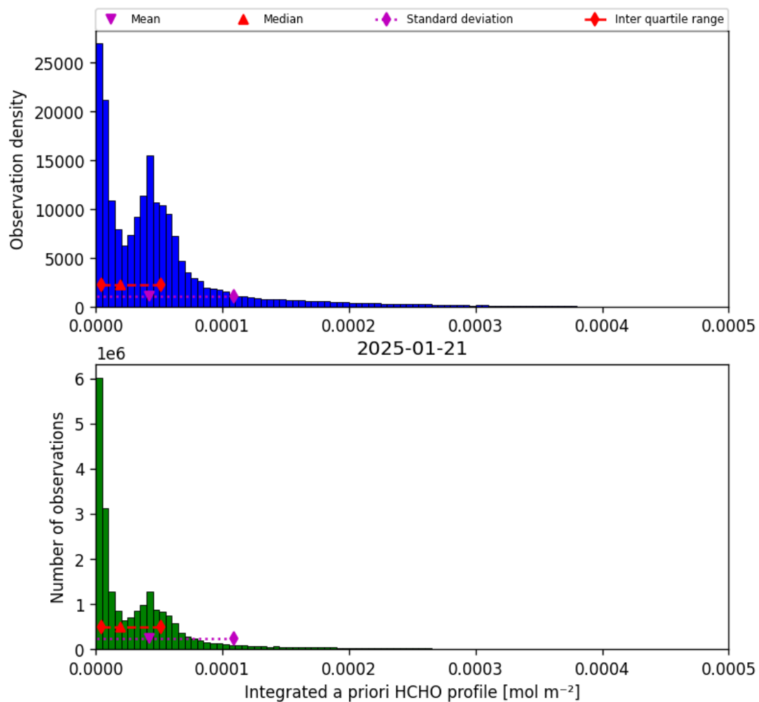
Figure 41: Histogram of “Integrated a priori HCHO profile” for 2025-01-21 to 2025-01-21
