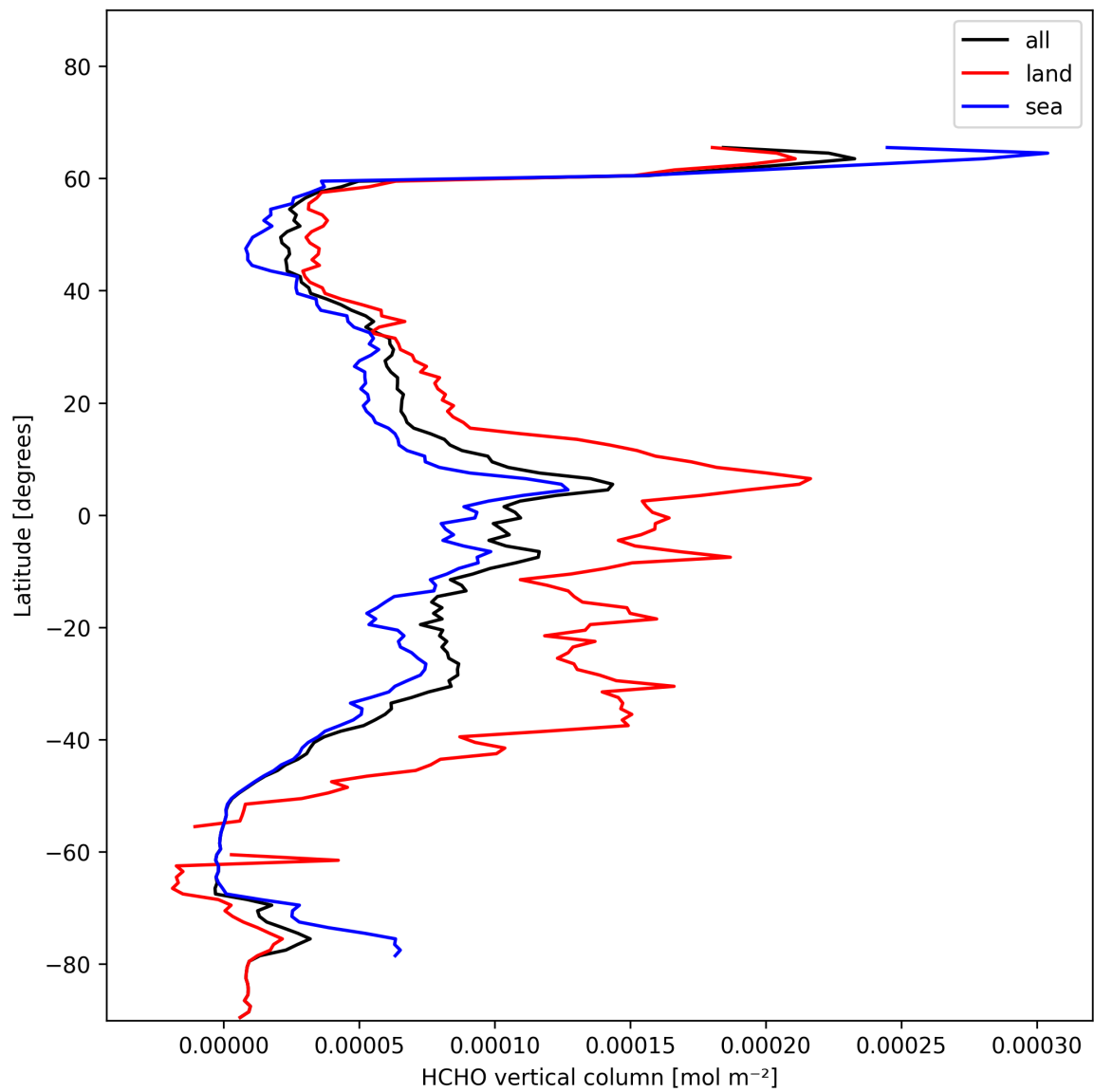
Figure 19: Zonal average of “HCHO vertical column” for 2025-01-21 to 2025-01-21.
