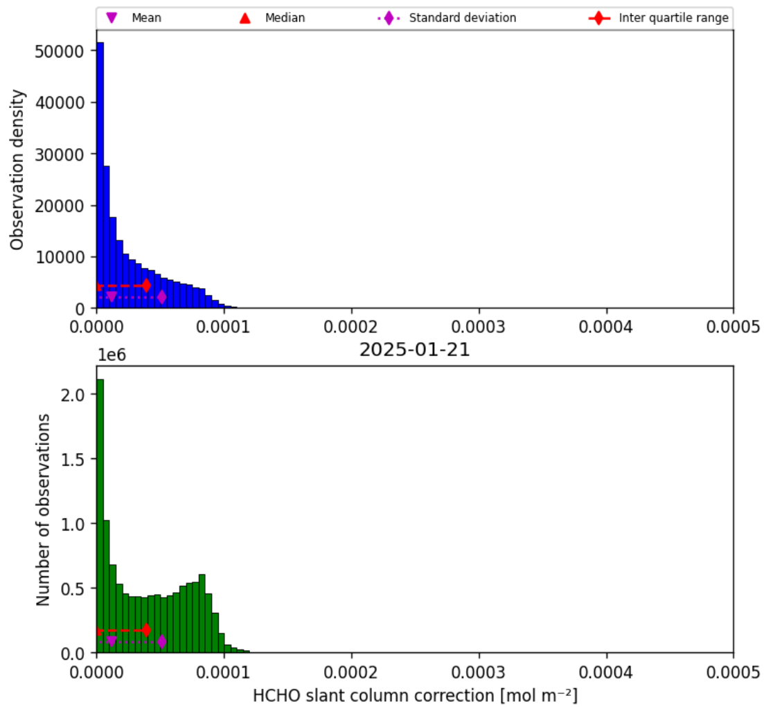
Figure 45: Histogram of “HCHO slant column correction” for 2025-01-21 to 2025-01-21
