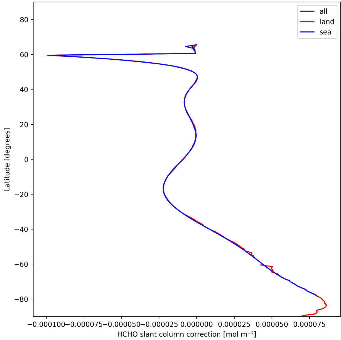
Figure 31: Zonal average of “HCHO slant column correction” for 2025-01-21 to 2025-01-21.
