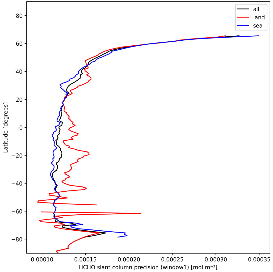
Figure 23: Zonal average of “HCHO slant column precision (window1)” for 2025-01-21 to 2025-01-21.
