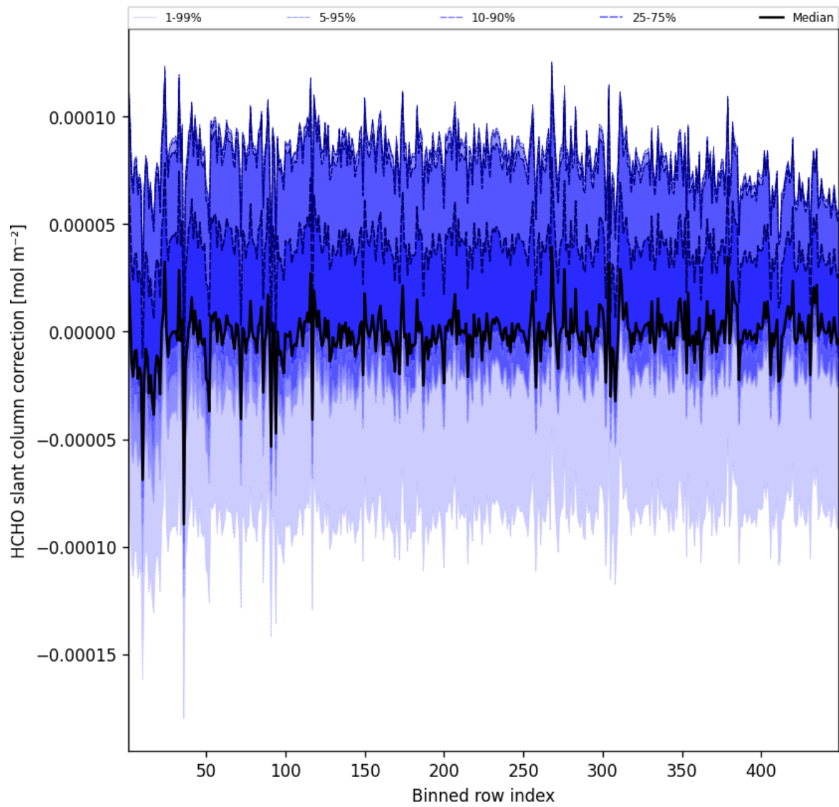
Figure 59: Along track statistics of "HCHO slant column correction" for 2025-01-21 to 2025-01-21
