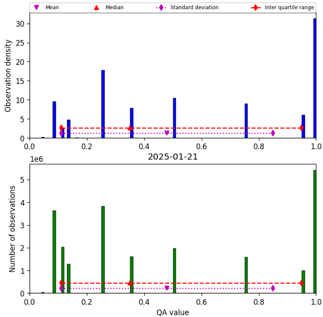
Figure 32: Histogram of “QA value” for 2025-01-21 to 2025-01-21
