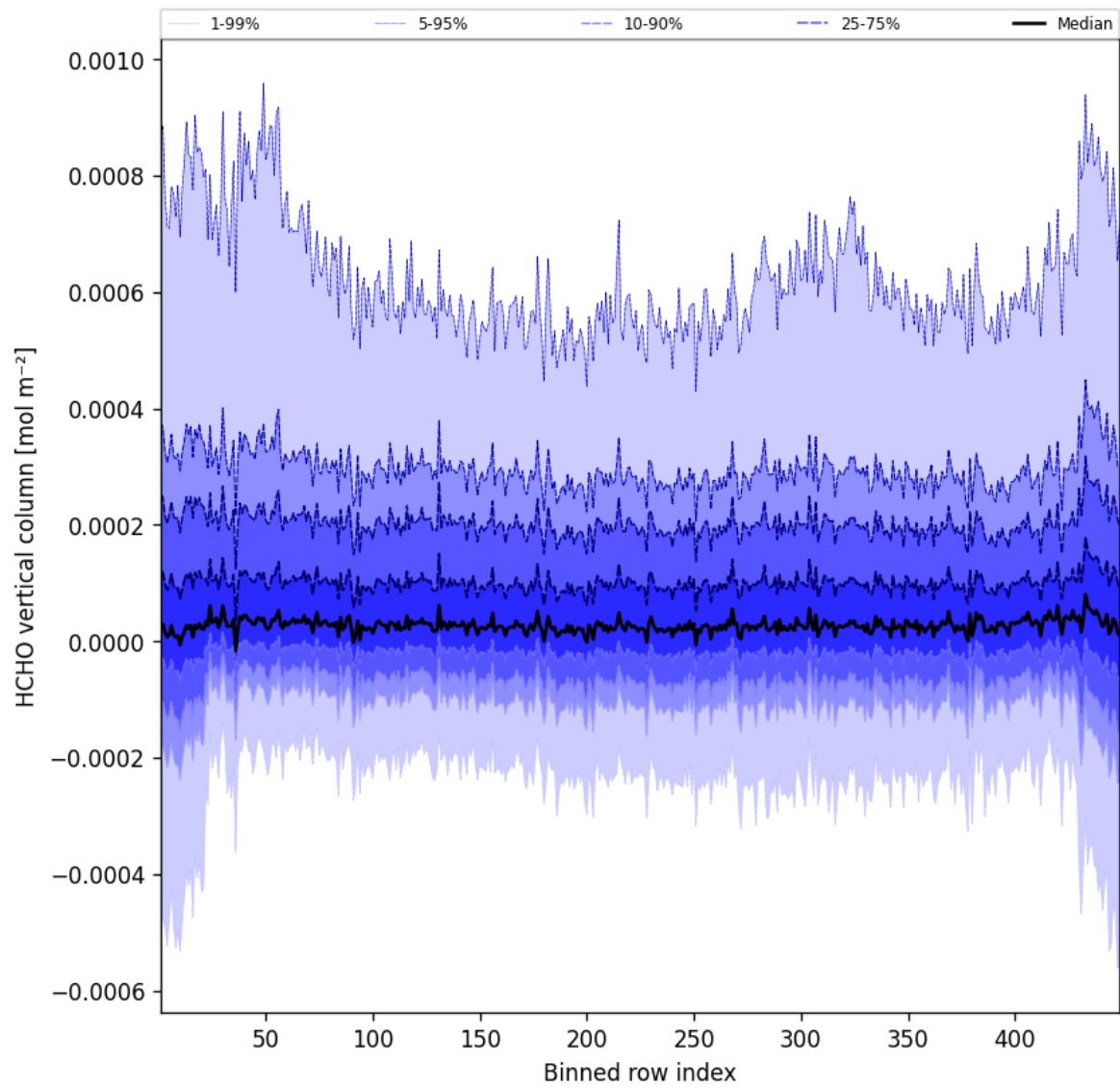
Figure 47: Along track statistics of “HCHO vertical column” for 2025-01-21 to 2025-01-21
