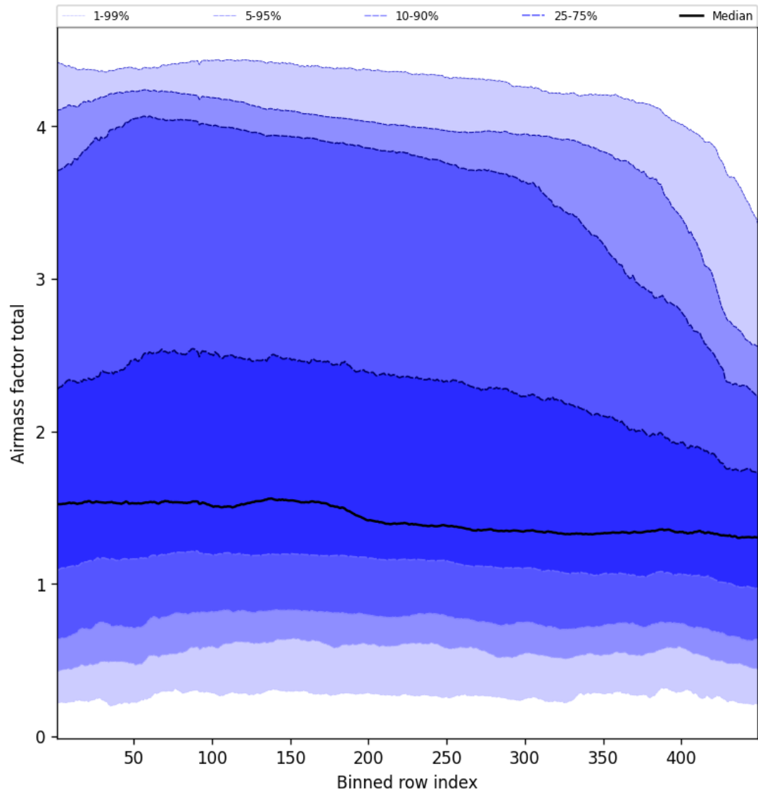
Figure 52: Along track statistics of “Airmass factor total” for 2025-01-21 to 2025-01-21
