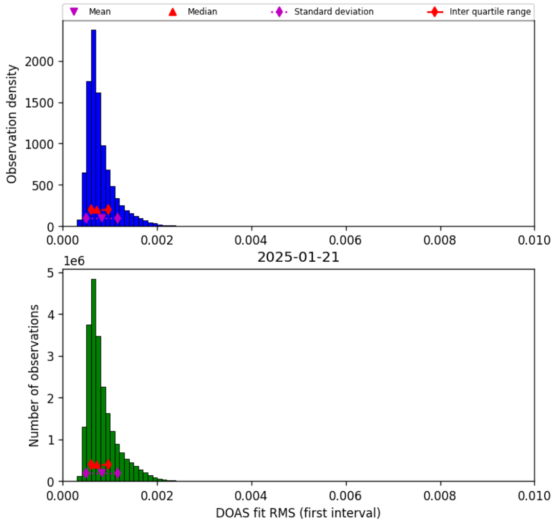
Figure 44: Histogram of “DOAS fit RMS (first interval)” for 2025-01-21 to 2025-01-21
