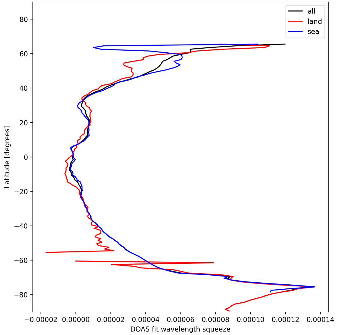
Figure 29: Zonal average of “DOAS fit wavelength squeeze” for 2025-01-21 to 2025-01-21.
