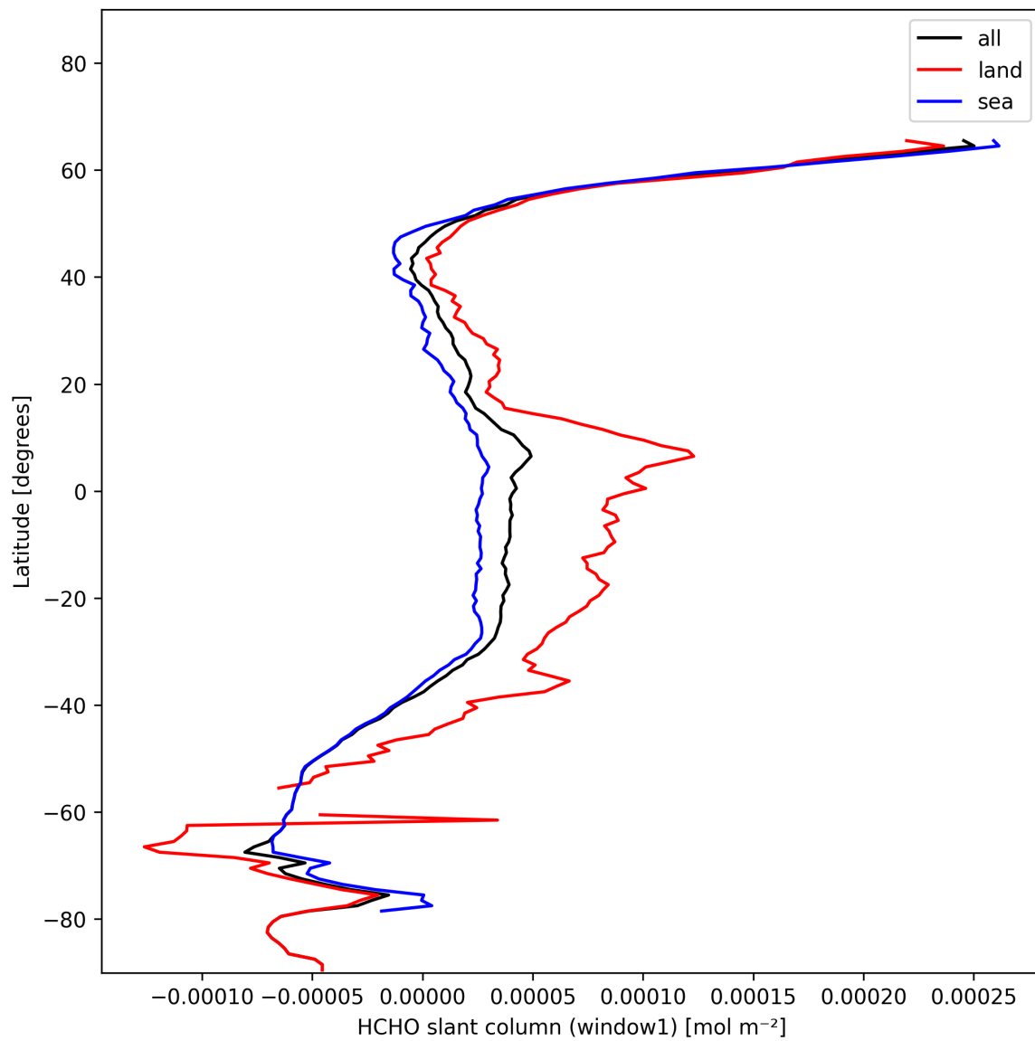
Figure 22: Zonal average of “HCHO slant column (window1)” for 2025-01-21 to 2025-01-21.
