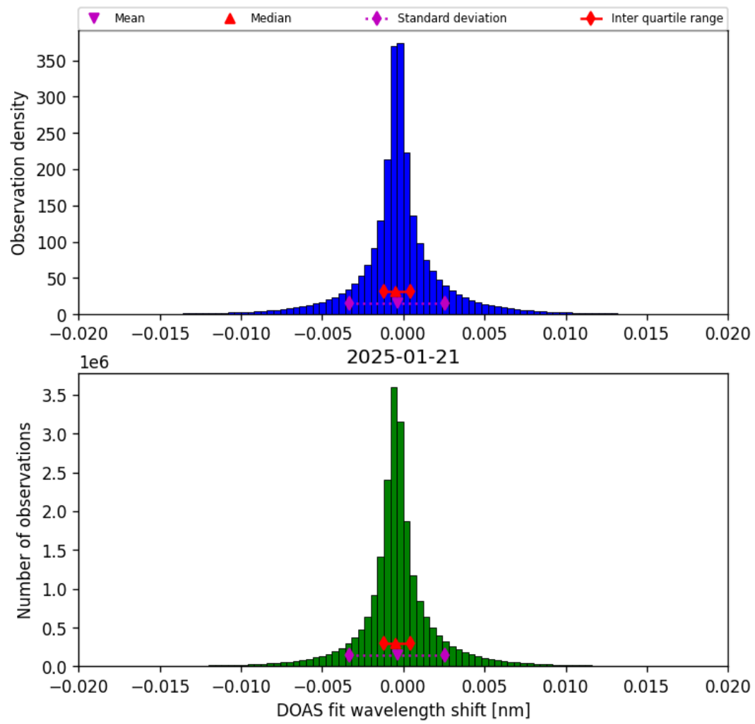
Figure 42: Histogram of “DOAS fit wavelength shift” for 2025-01-21 to 2025-01-21
