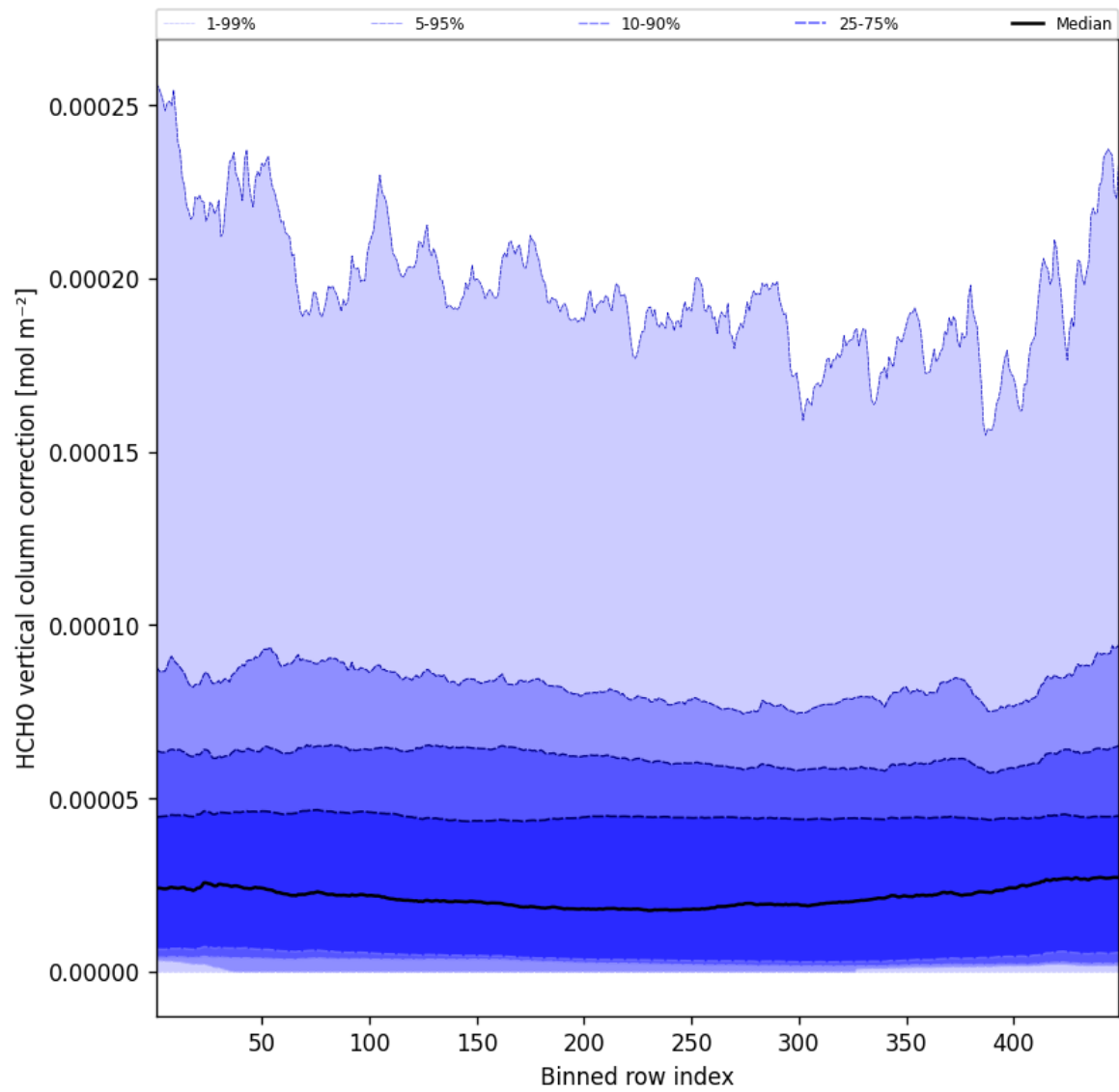
Figure 49: Along track statistics of “HCHO vertical column correction” for 2025-01-21 to 2025-01-21
