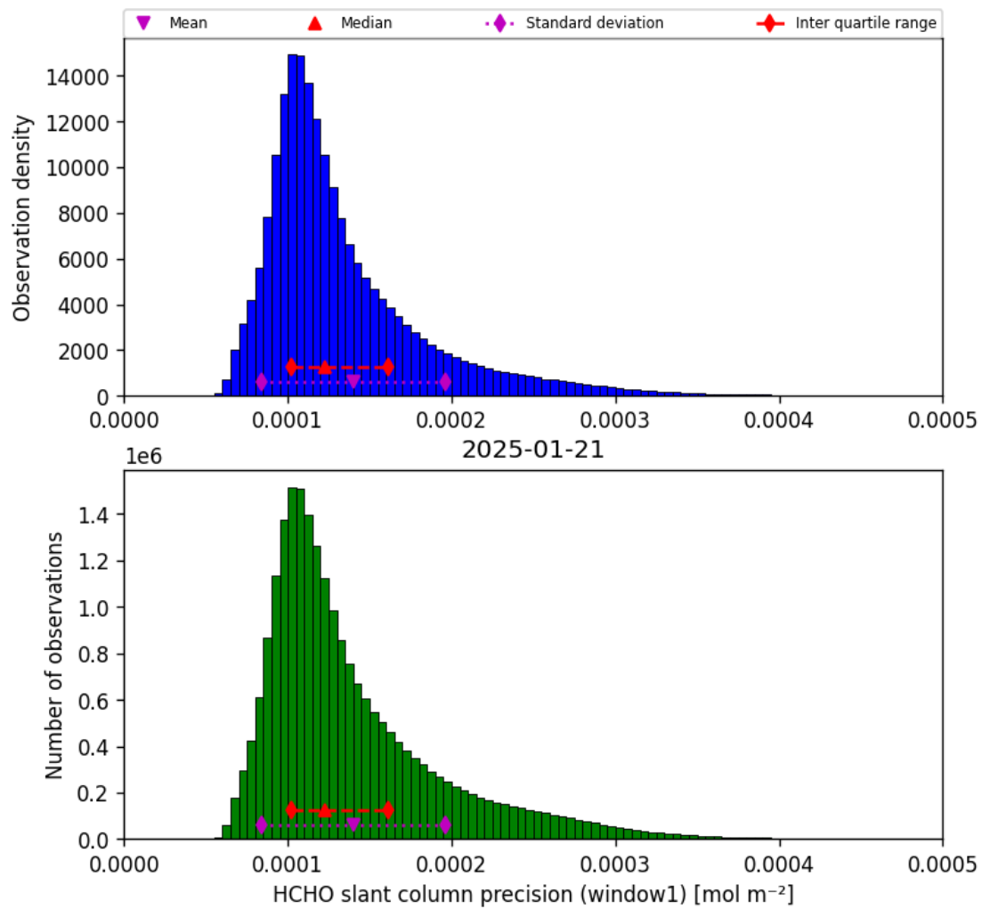
Figure 37: Histogram of “HCHO slant column precision (window1)” for 2025-01-21 to 2025-01-21
