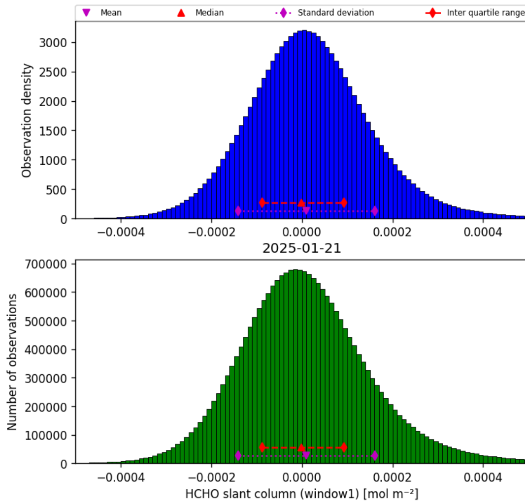
Figure 36: Histogram of “HCHO slant column (window1)” for 2025-01-21 to 2025-01-21
