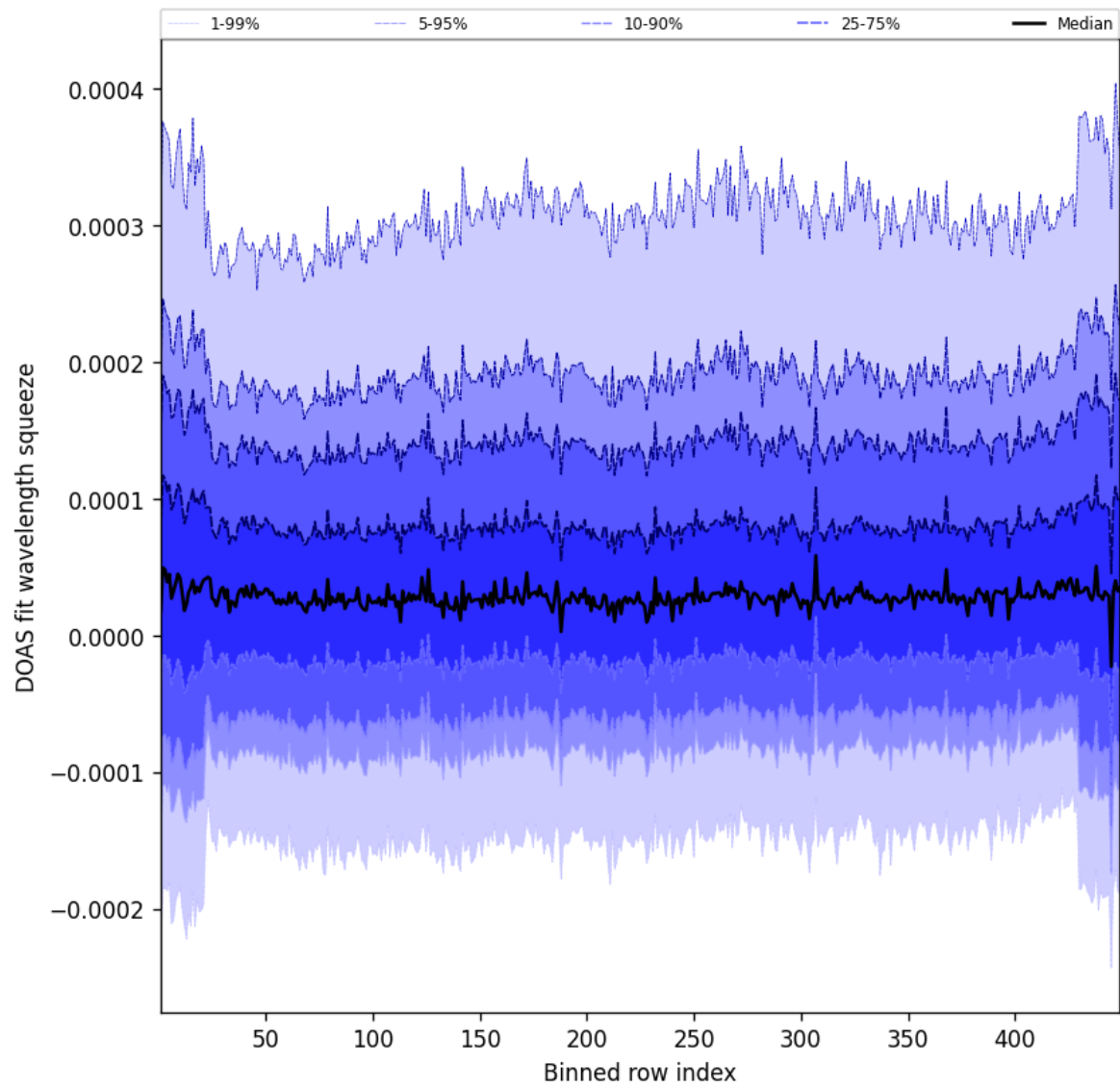
Figure 57: Along track statistics of “DOAS fit wavelength squeeze” for 2025-01-21 to 2025-01-21
