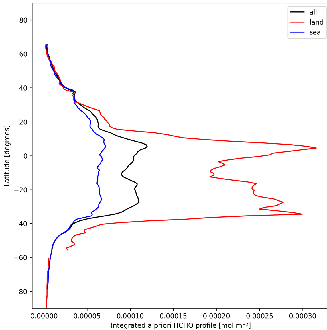
Figure 27: Zonal average of “Integrated a priori HCHO profile” for 2025-01-21 to 2025-01-21.
