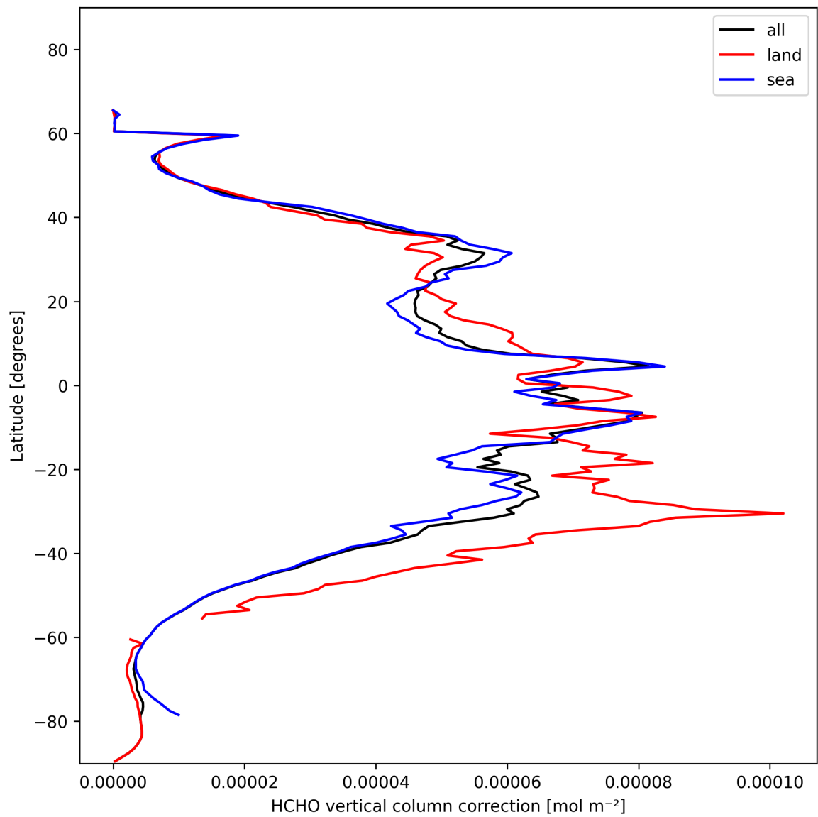
Figure 21: Zonal average of “HCHO vertical column correction” for 2025-01-21 to 2025-01-21.
