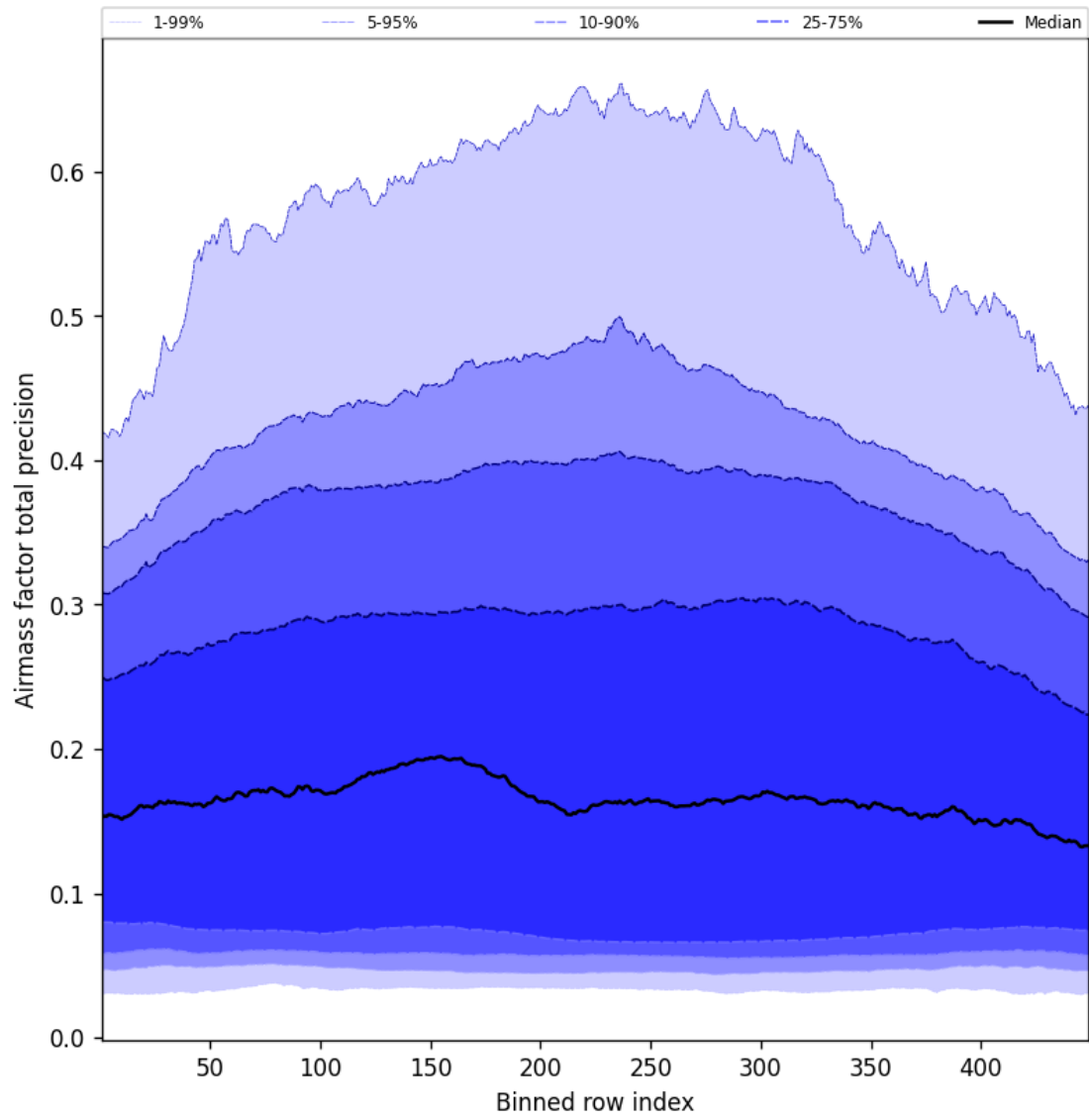
Figure 53: Along track statistics of “Airmass factor total precision” for 2025-01-21 to 2025-01-21
