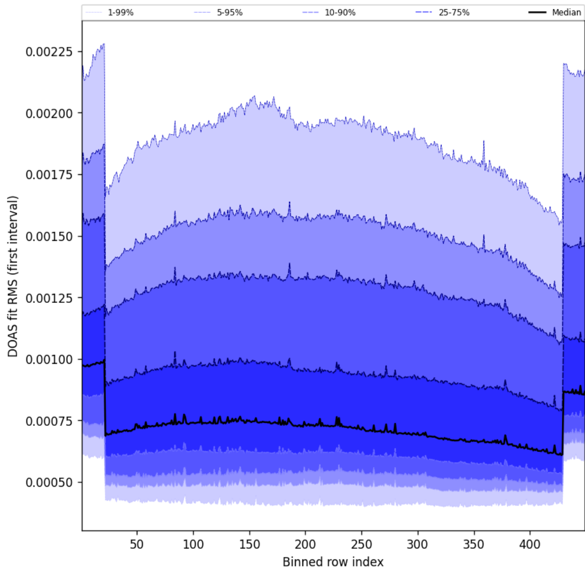
Figure 58: Along track statistics of “DOAS fit RMS (first interval)” for 2025-01-21 to 2025-01-21
