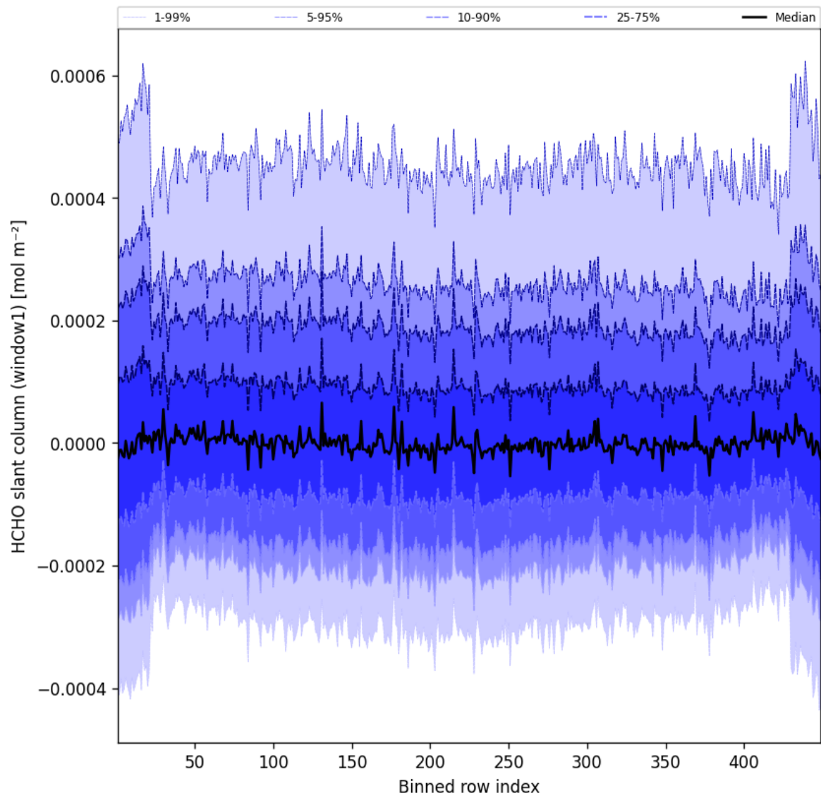
Figure 50: Along track statistics of “HCHO slant column (window1)” for 2025-01-21 to 2025-01-21
