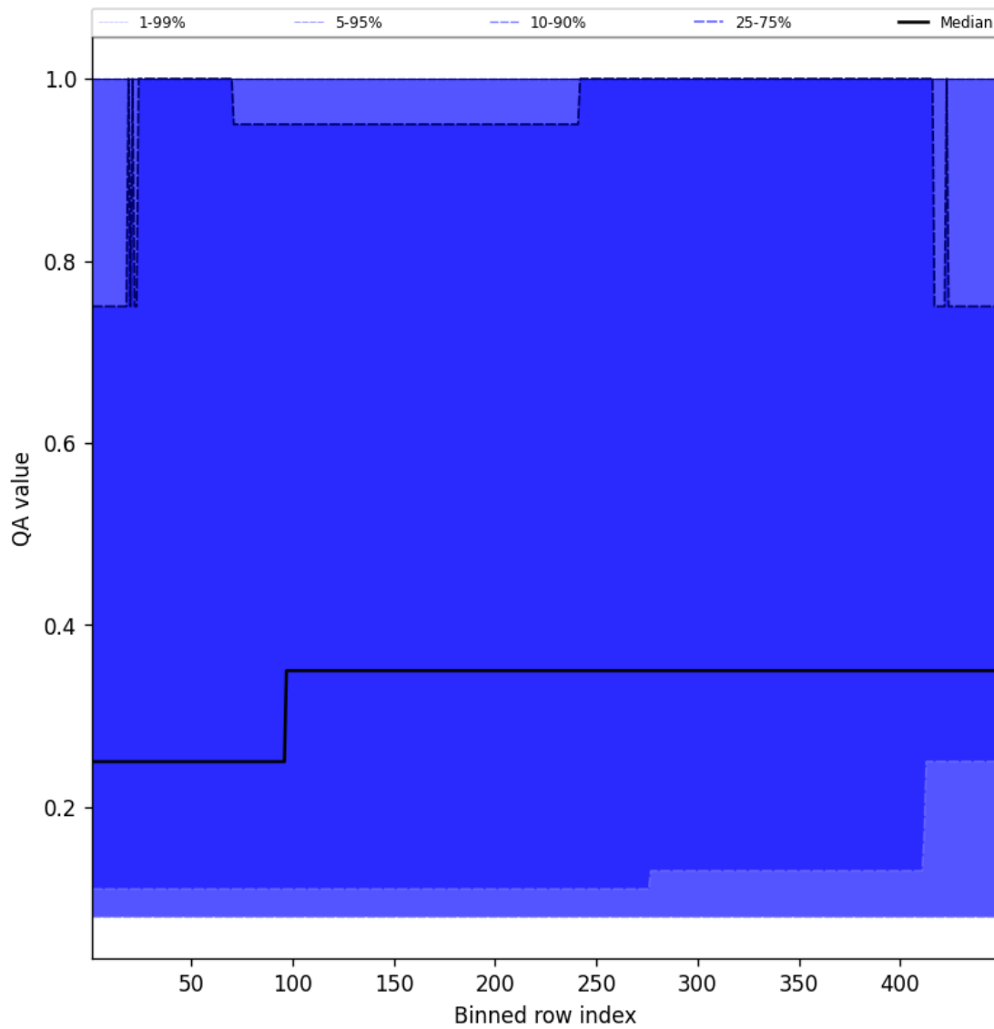
Figure 46: Along track statistics of “QA value” for 2025-01-21 to 2025-01-21
