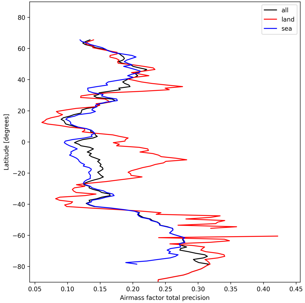
Figure 25: Zonal average of “Airmass factor total precision” for 2025-01-21 to 2025-01-21.
