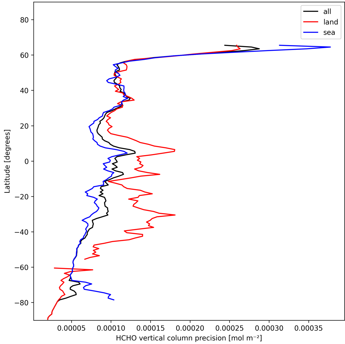
Figure 20: Zonal average of “HCHO vertical column precision” for 2025-01-21 to 2025-01-21.
