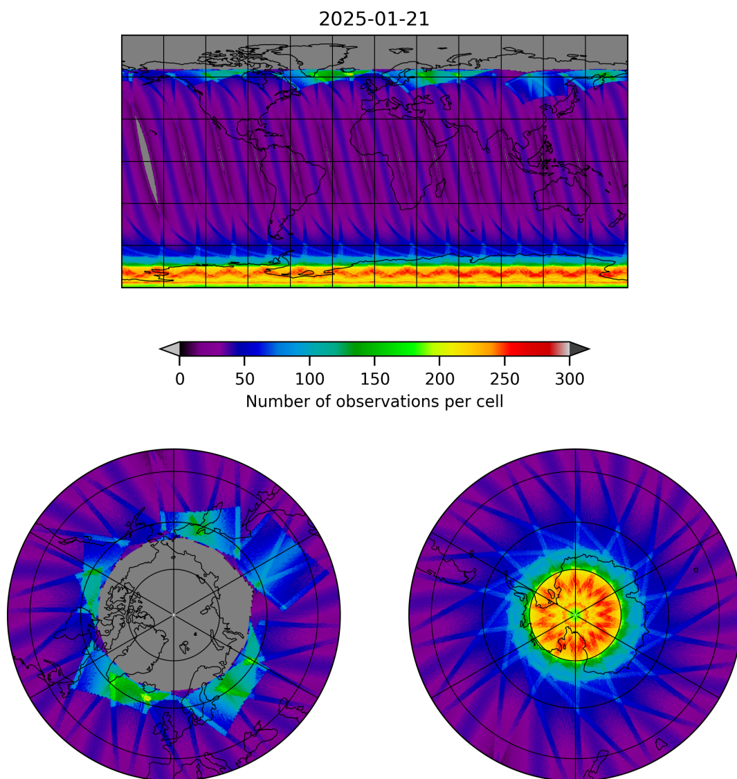
Figure 17: Map of the number of observations for 2025-01-21 to 2025-01-21
