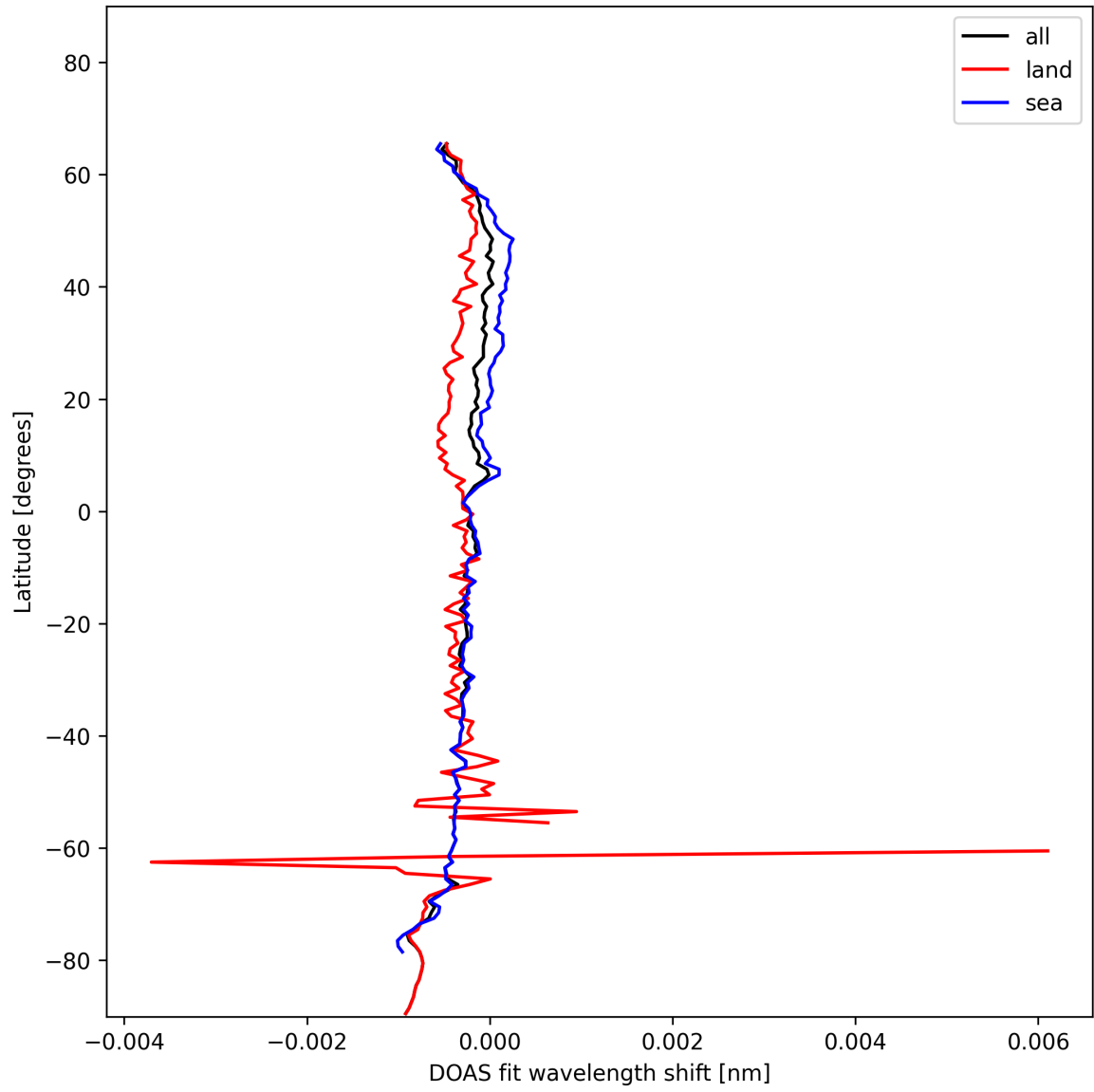
Figure 28: Zonal average of “DOAS fit wavelength shift” for 2025-01-22 to 2025-01-23.
