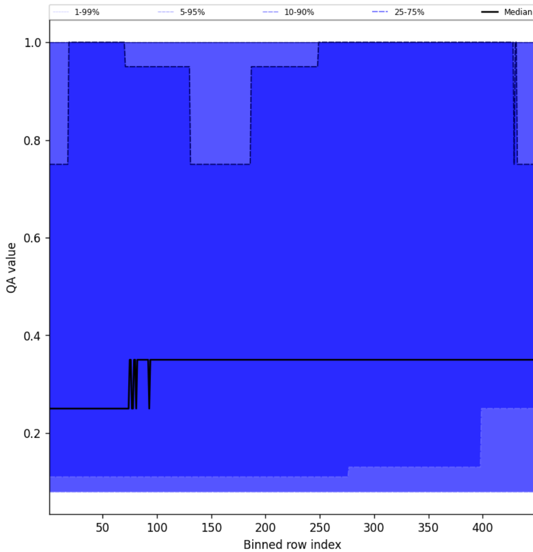
Figure 46: Along track statistics of “QA value” for 2025-01-22 to 2025-01-23
