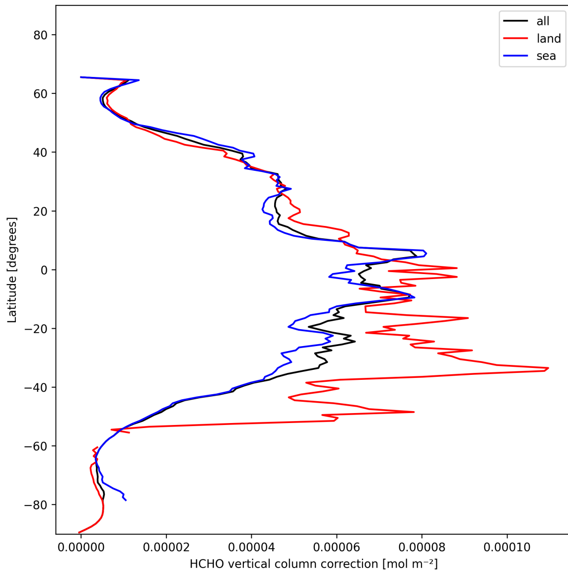
Figure 21: Zonal average of “HCHO vertical column correction” for 2025-01-22 to 2025-01-23.
