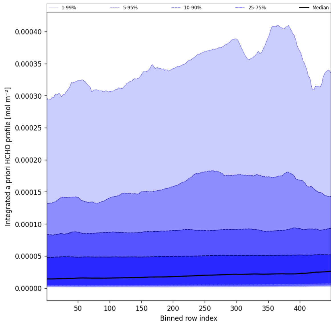
Figure 55: Along track statistics of "Integrated a priori HCHO profile" for 2025-01-22 to 2025-01-23
