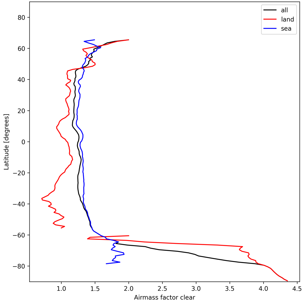
Figure 26: Zonal average of “Airmass factor clear” for 2025-01-22 to 2025-01-23.
