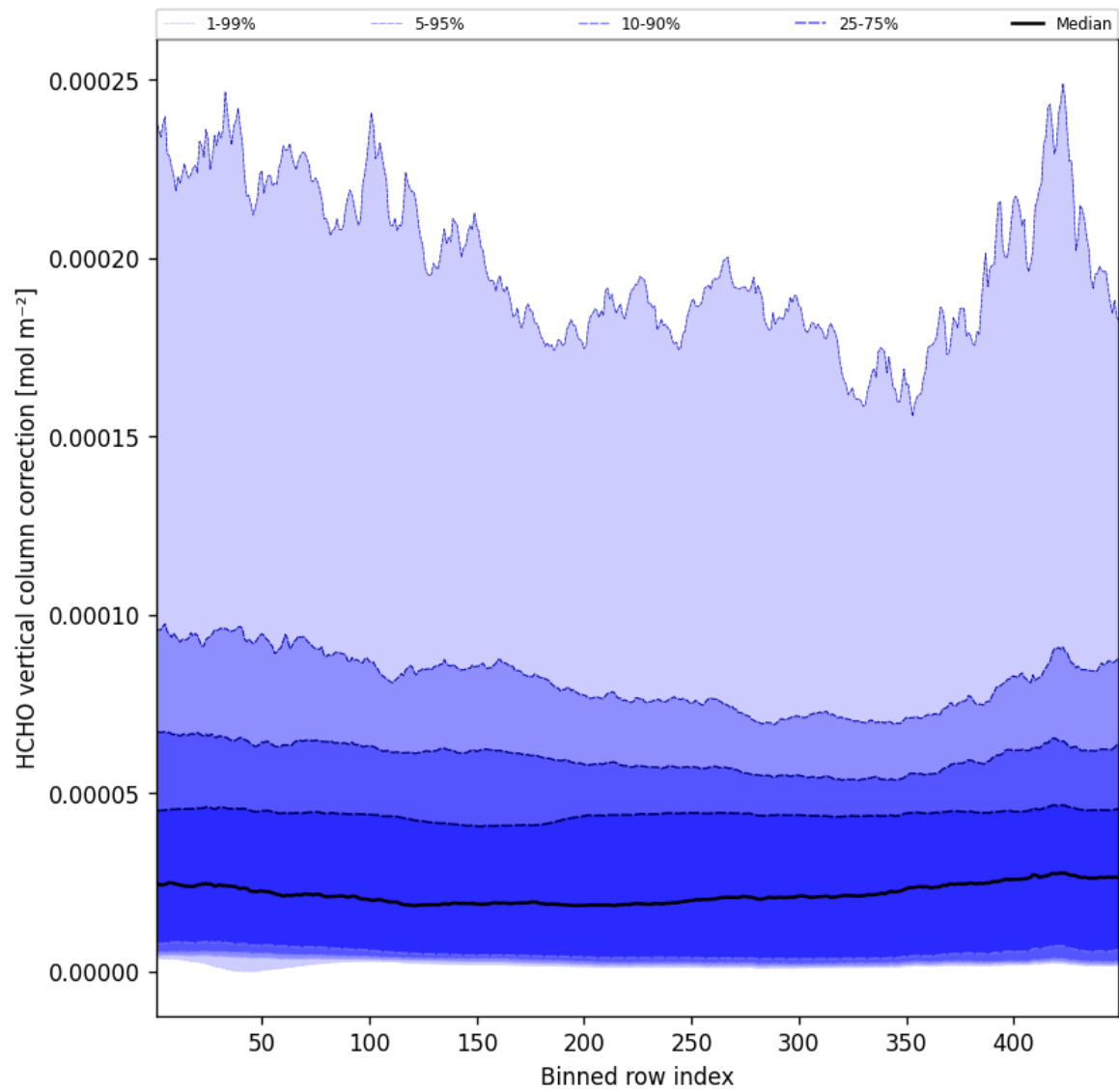
Figure 49: Along track statistics of “HCHO vertical column correction” for 2025-01-22 to 2025-01-23
