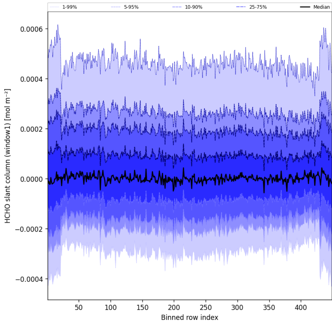
Figure 50: Along track statistics of “HCHO slant column (window1)” for 2025-01-22 to 2025-01-23
