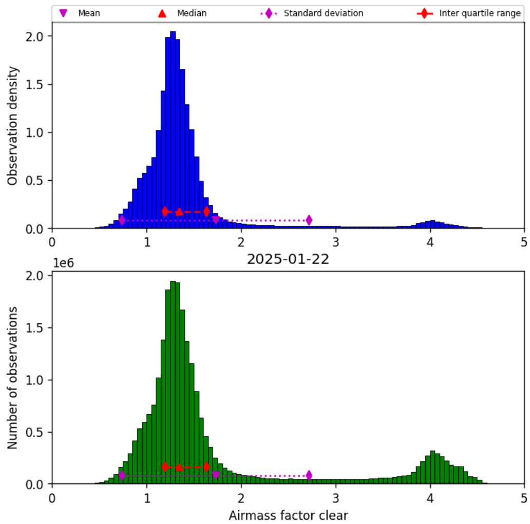
Figure 40: Histogram of “Airmass factor clear” for 2025-01-22 to 2025-01-23
