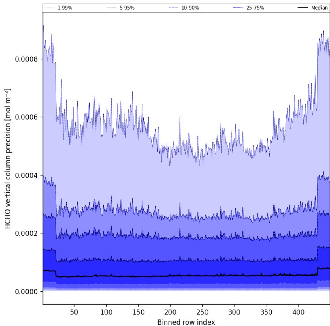
Figure 48: Along track statistics of “HCHO vertical column precision” for 2025-01-22 to 2025-01-23
