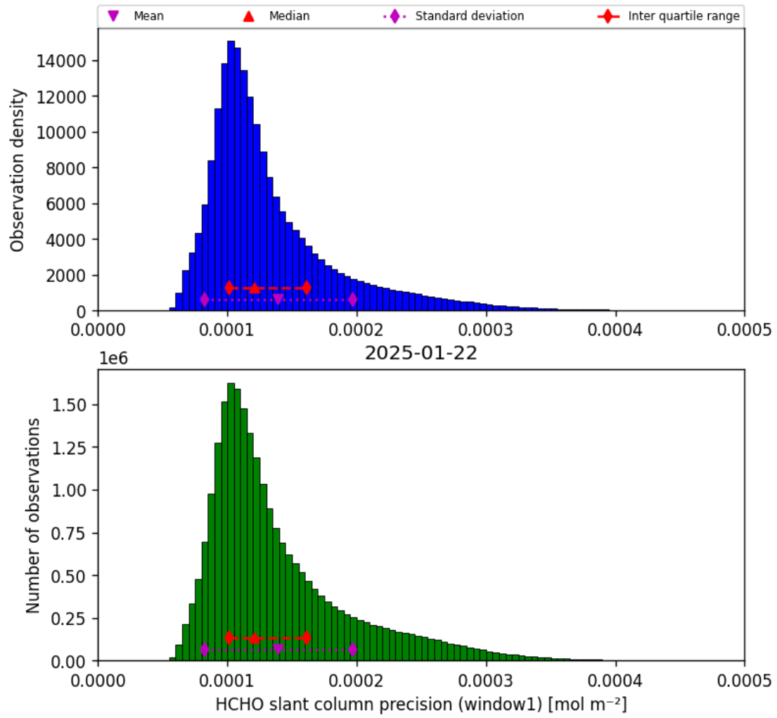
Figure 37: Histogram of “HCHO slant column precision (window1)” for 2025-01-22 to 2025-01-23
