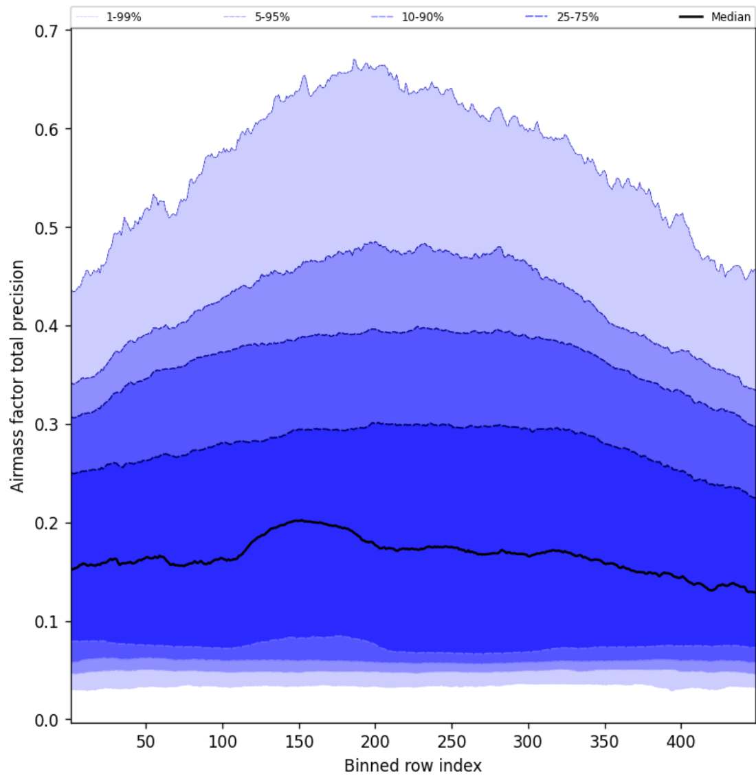
Figure 53: Along track statistics of “Airmass factor total precision” for 2025-01-22 to 2025-01-23
