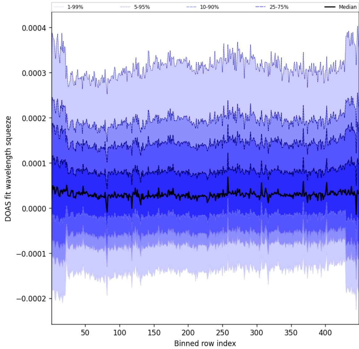
Figure 57: Along track statistics of “DOAS fit wavelength squeeze” for 2025-01-22 to 2025-01-23
