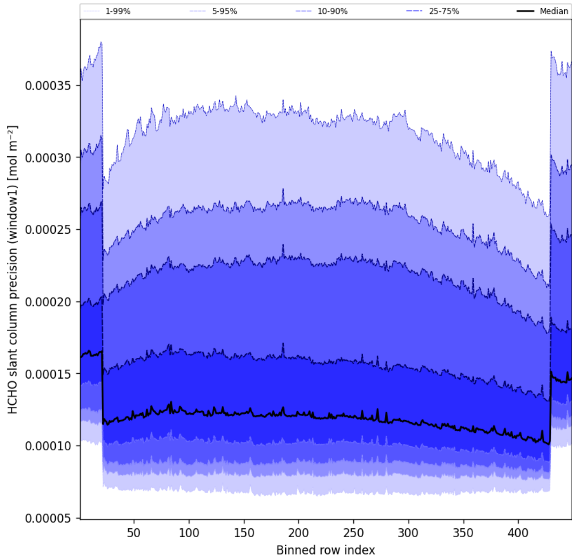
Figure 51: Along track statistics of “HCHO slant column precision (window1)” for 2025-01-22 to 2025-01-23
