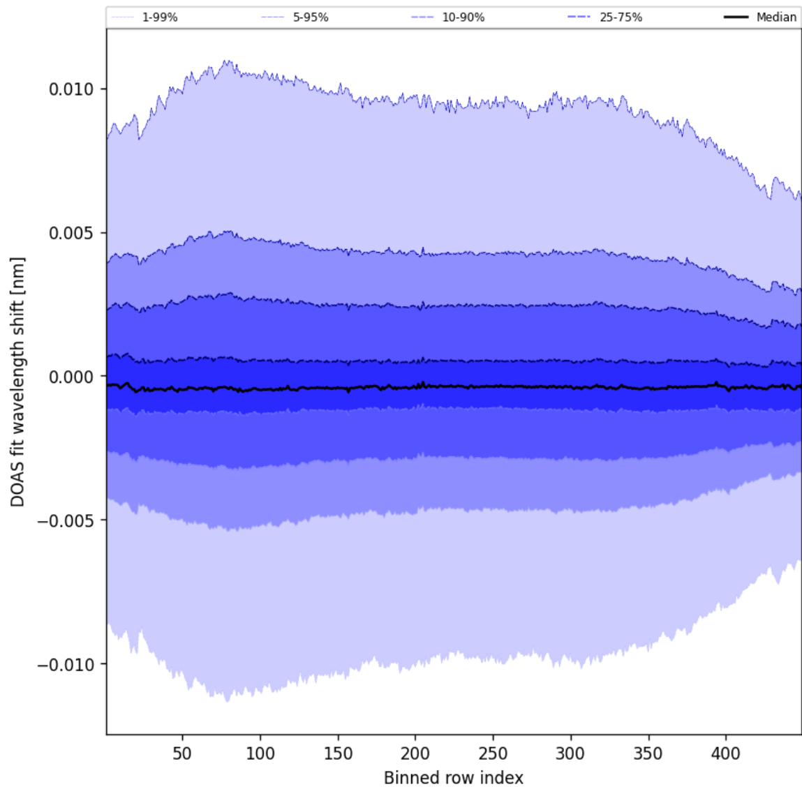
Figure 56: Along track statistics of “DOAS fit wavelength shift” for 2025-01-22 to 2025-01-23
