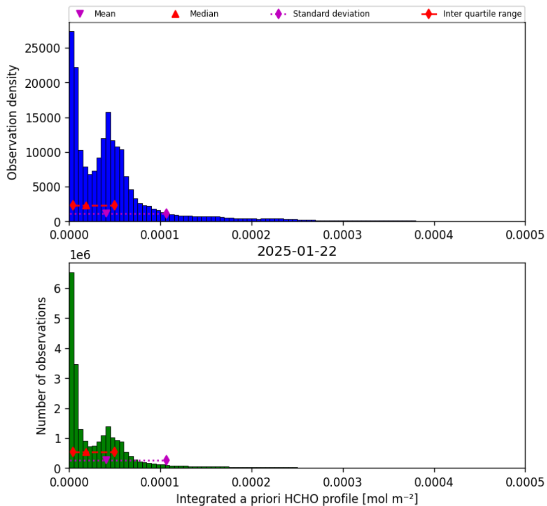
Figure 41: Histogram of “Integrated a priori HCHO profile” for 2025-01-22 to 2025-01-23
