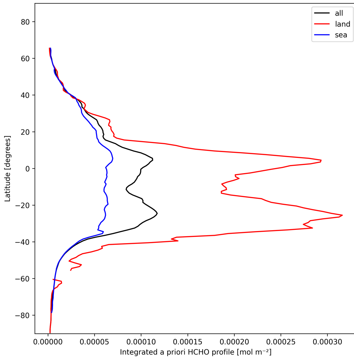
Figure 27: Zonal average of “Integrated a priori HCHO profile” for 2025-01-22 to 2025-01-23.
