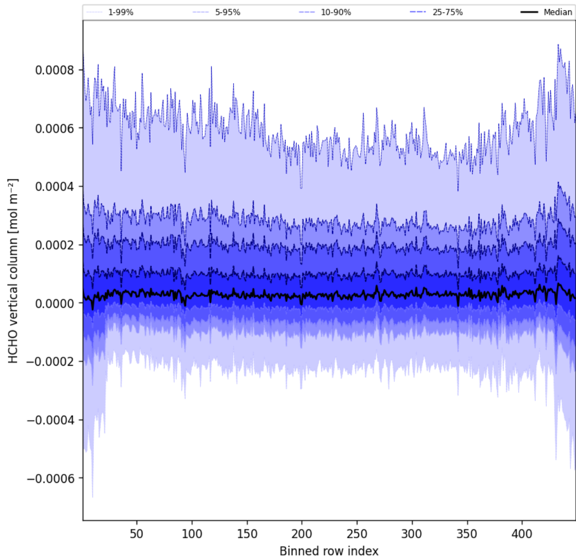
Figure 47: Along track statistics of “HCHO vertical column” for 2025-01-22 to 2025-01-23
