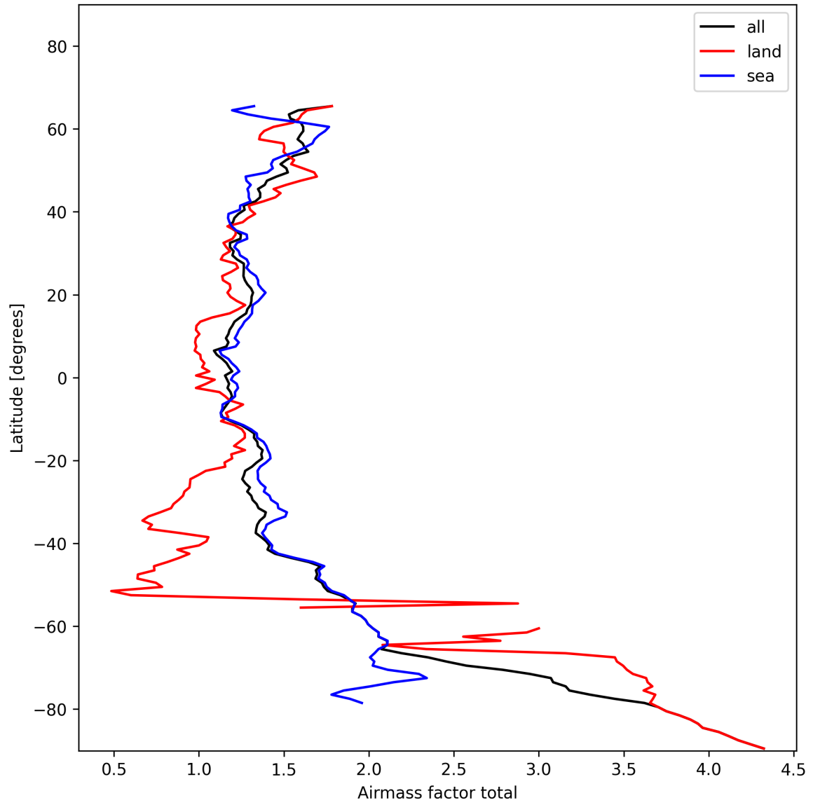
Figure 24: Zonal average of “Airmass factor total” for 2025-01-22 to 2025-01-23.
