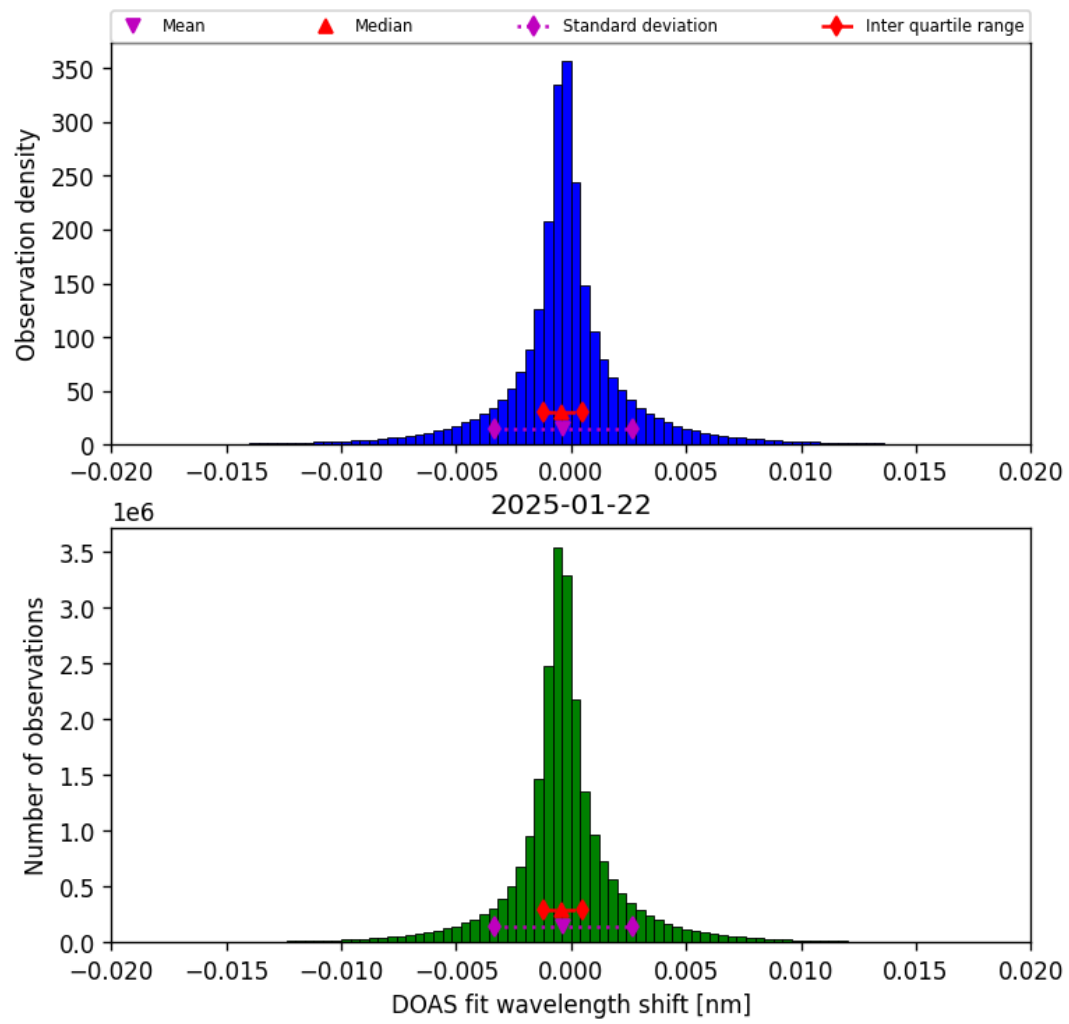
Figure 42: Histogram of “DOAS fit wavelength shift” for 2025-01-22 to 2025-01-23
