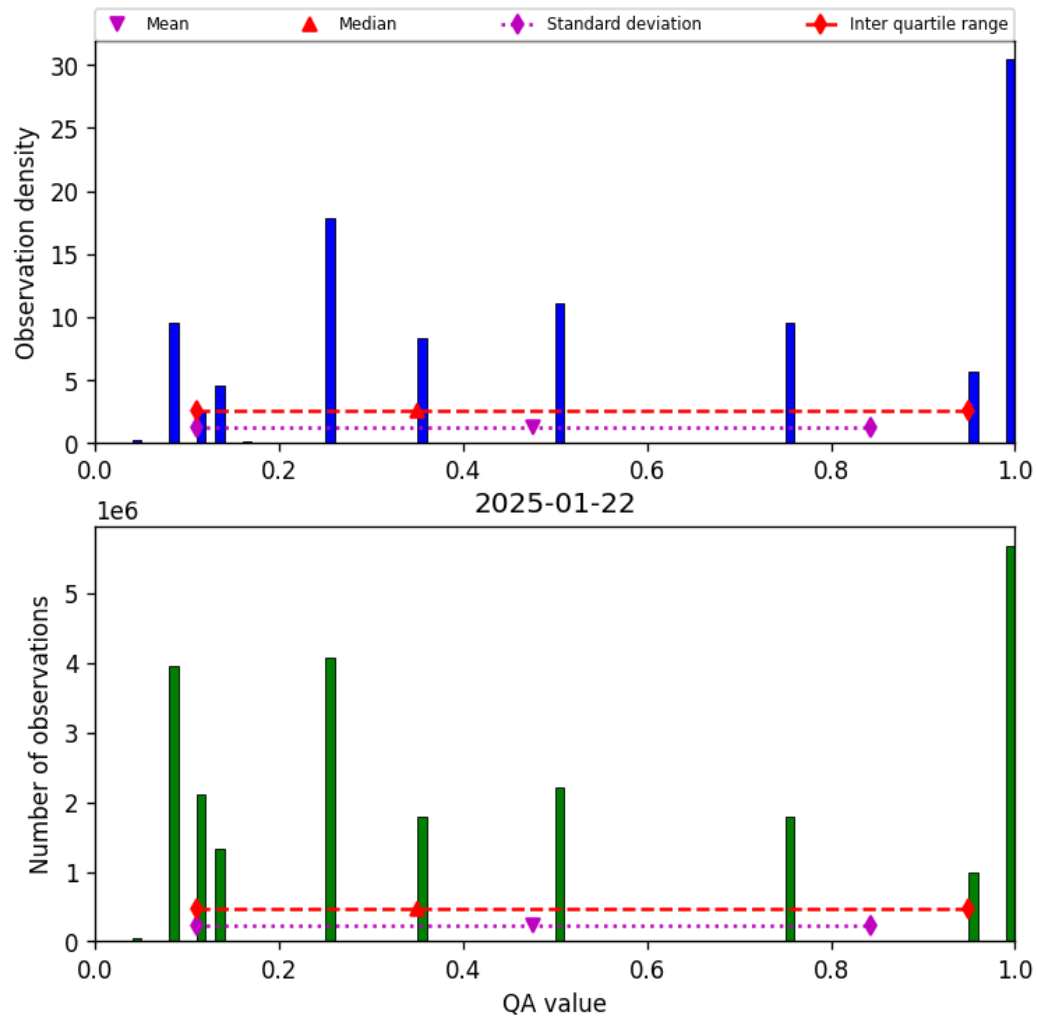
Figure 32: Histogram of “QA value” for 2025-01-22 to 2025-01-23
