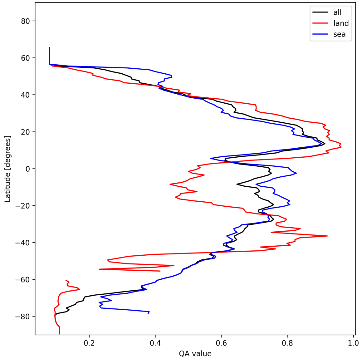
Figure 18: Zonal average of “QA value” for 2025-01-22 to 2025-01-23.
