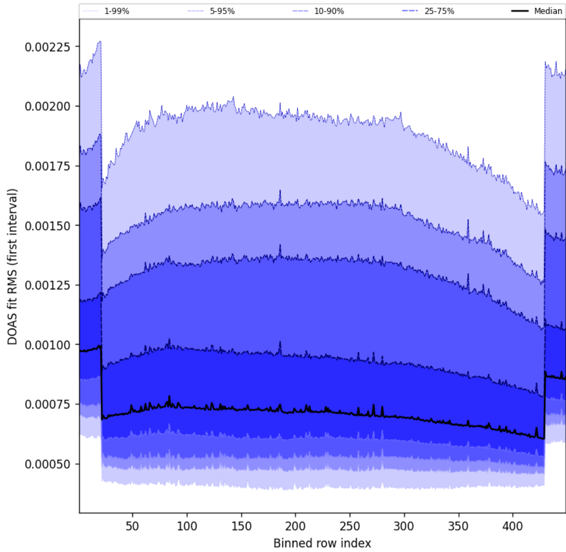
Figure 58: Along track statistics of “DOAS fit RMS (first interval)” for 2025-01-22 to 2025-01-23
