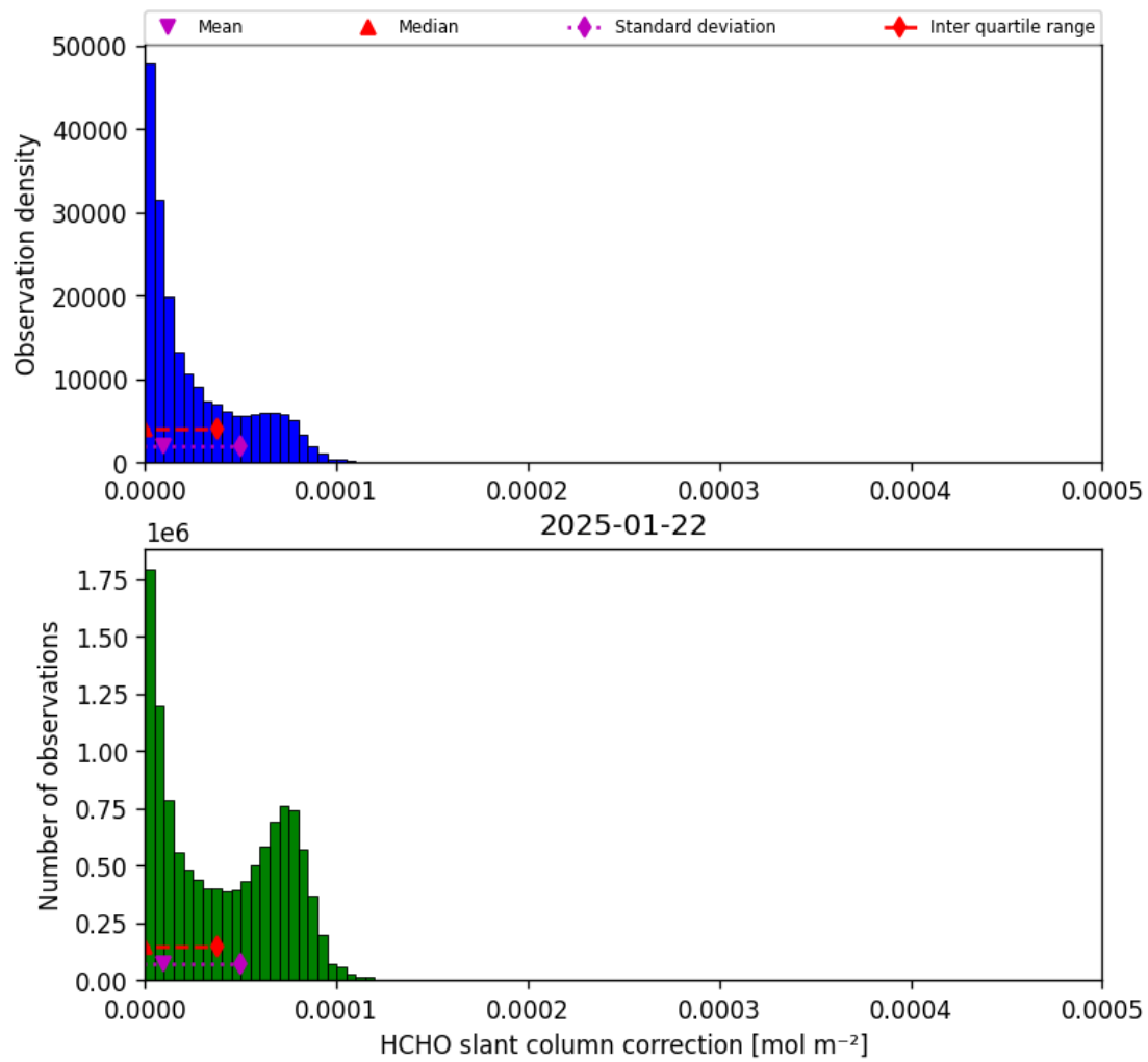
Figure 45: Histogram of "HCHO slant column correction" for 2025-01-22 to 2025-01-23
