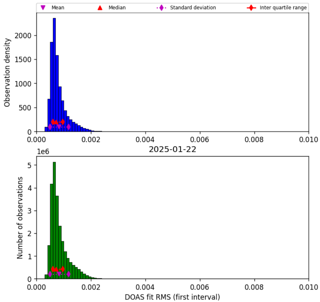
Figure 44: Histogram of “DOAS fit RMS (first interval)” for 2025-01-22 to 2025-01-23
