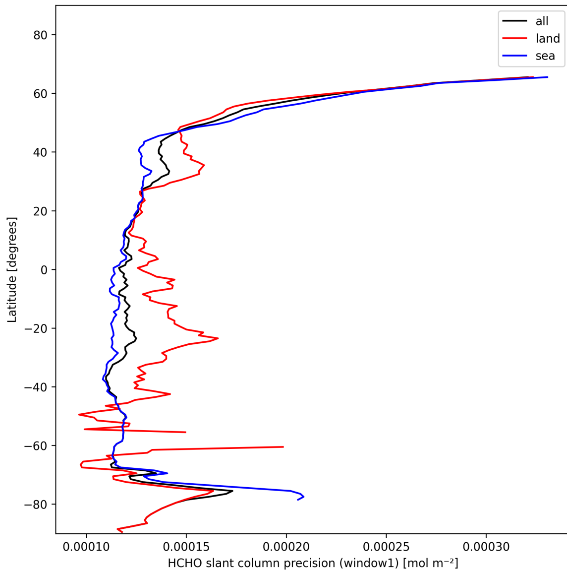
Figure 23: Zonal average of “HCHO slant column precision (window1)” for 2025-01-22 to 2025-01-23.
