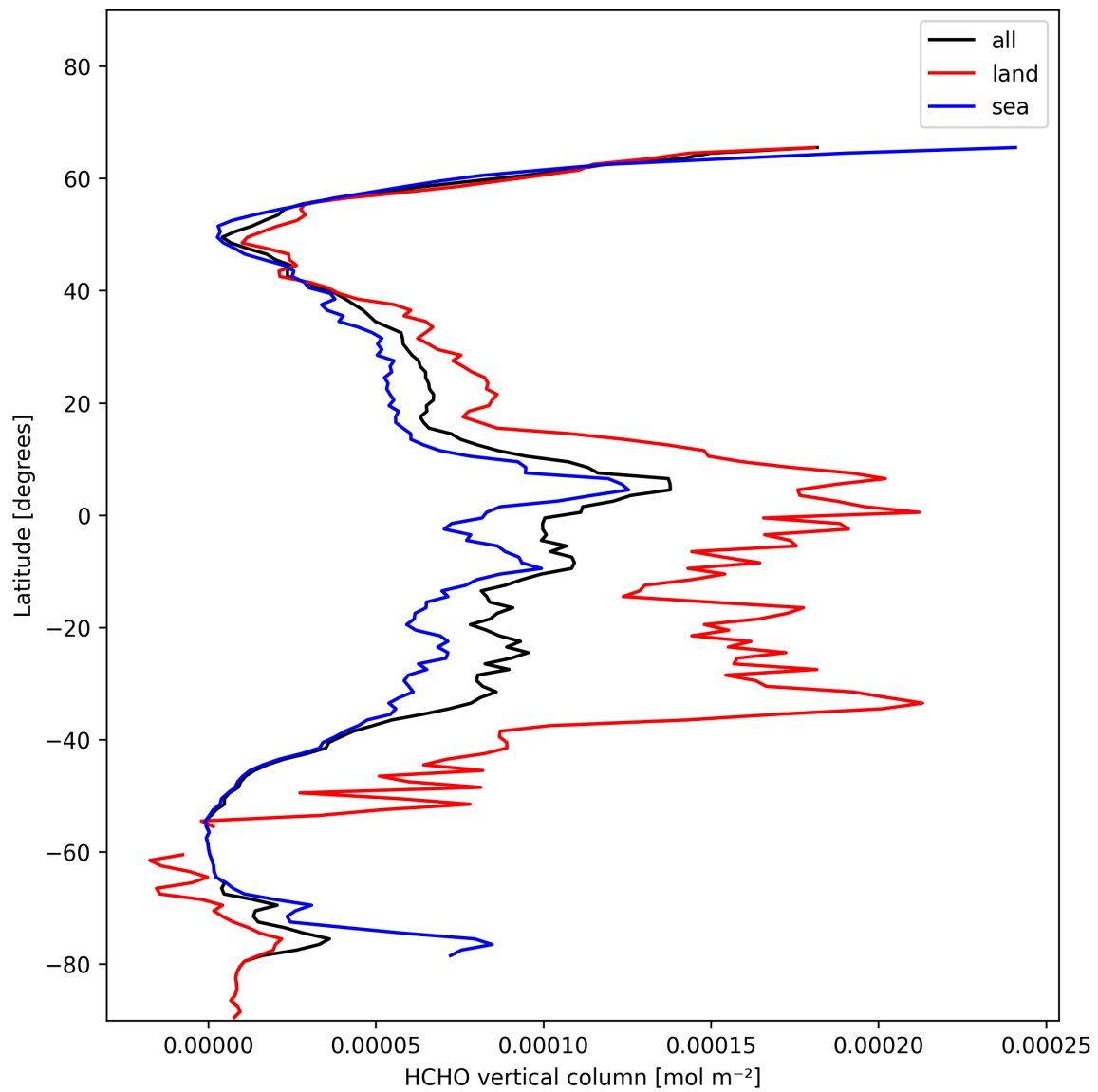
Figure 19: Zonal average of “HCHO vertical column” for 2025-01-22 to 2025-01-23.
