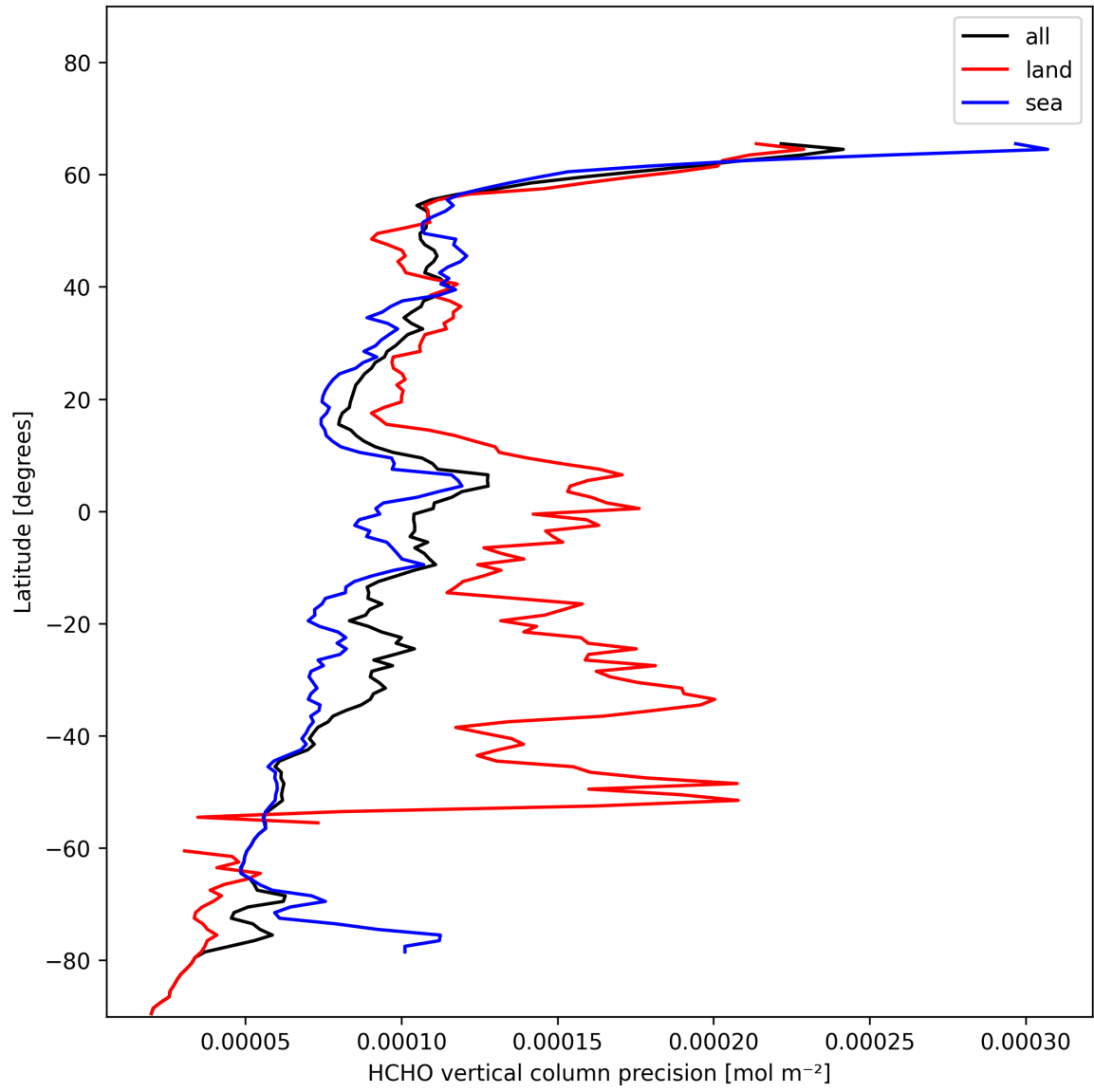
Figure 20: Zonal average of “HCHO vertical column precision” for 2025-01-22 to 2025-01-23.
