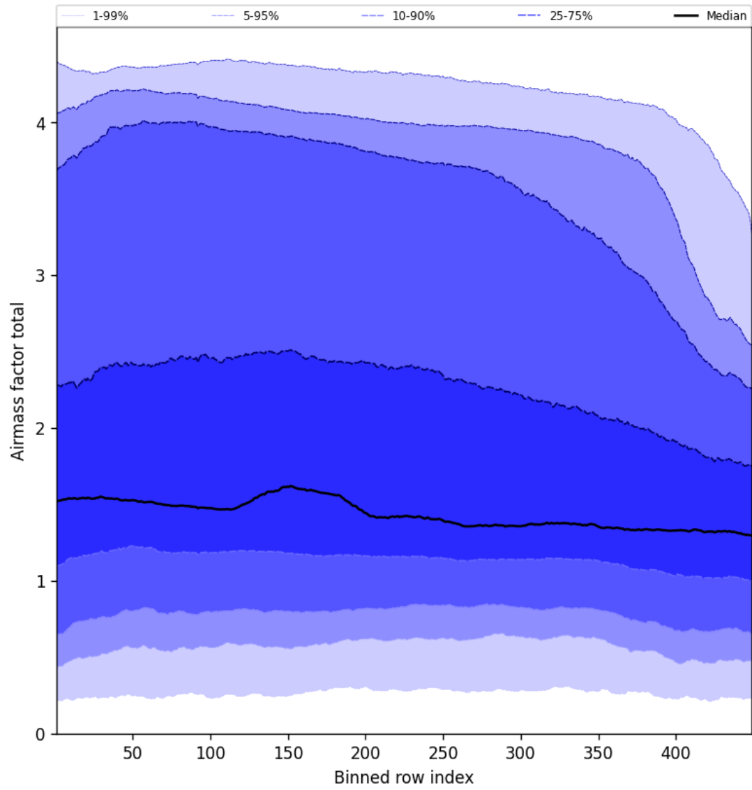
Figure 52: Along track statistics of “Airmass factor total” for 2025-01-22 to 2025-01-23
