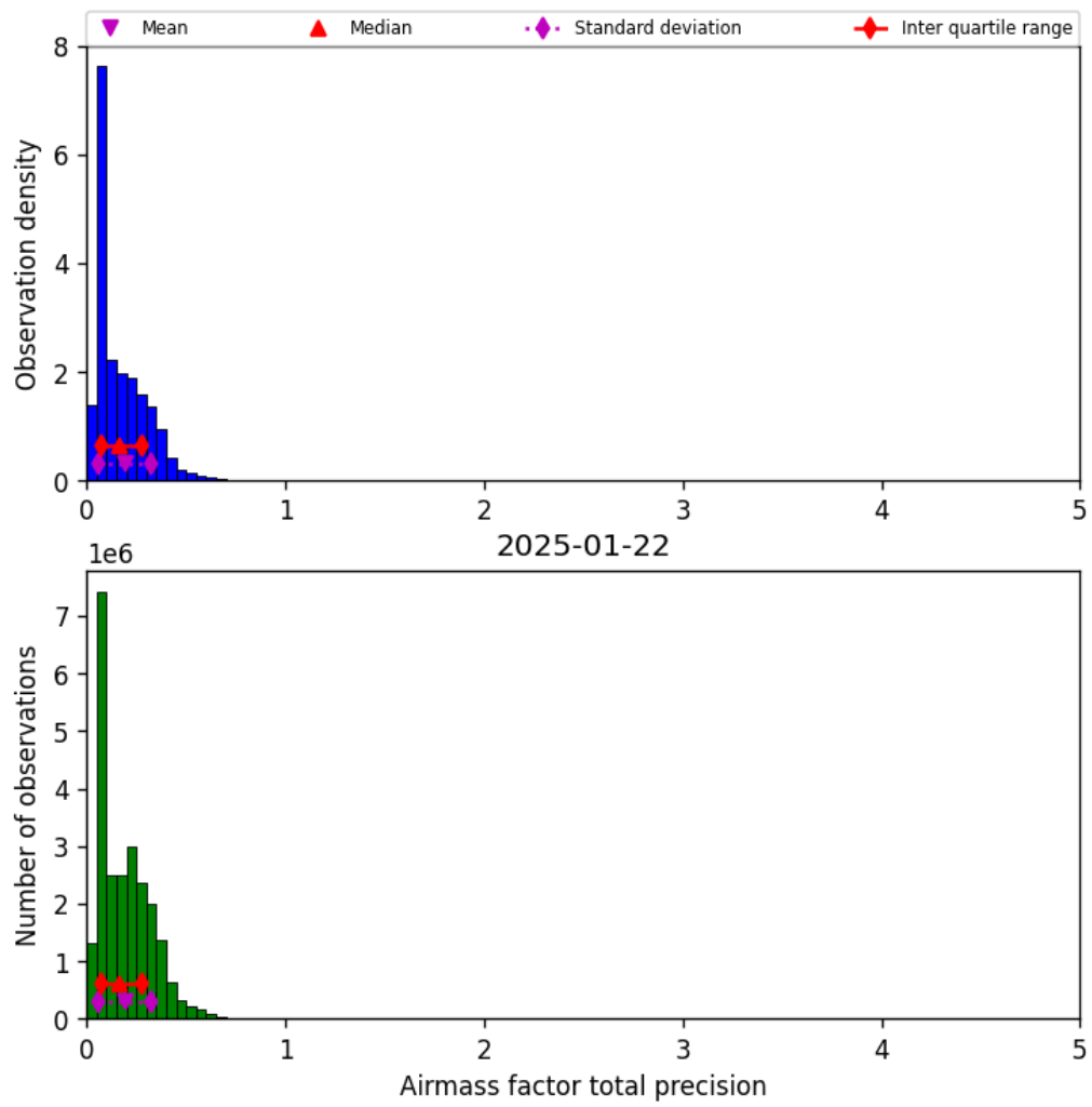
Figure 39: Histogram of “Airmass factor total precision” for 2025-01-22 to 2025-01-23
