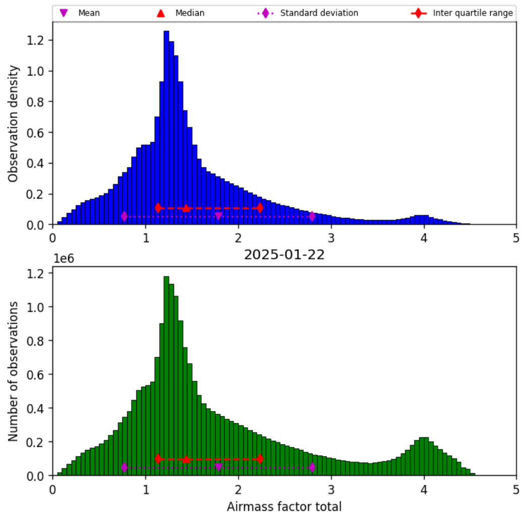
Figure 38: Histogram of “Airmass factor total” for 2025-01-22 to 2025-01-23
