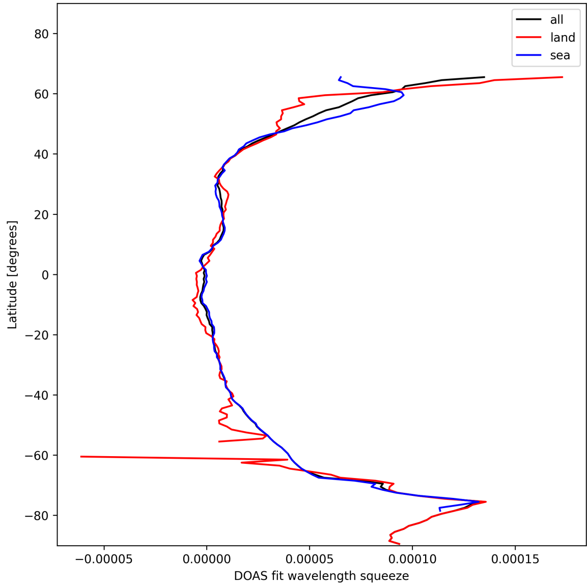
Figure 29: Zonal average of “DOAS fit wavelength squeeze” for 2025-01-22 to 2025-01-23.
