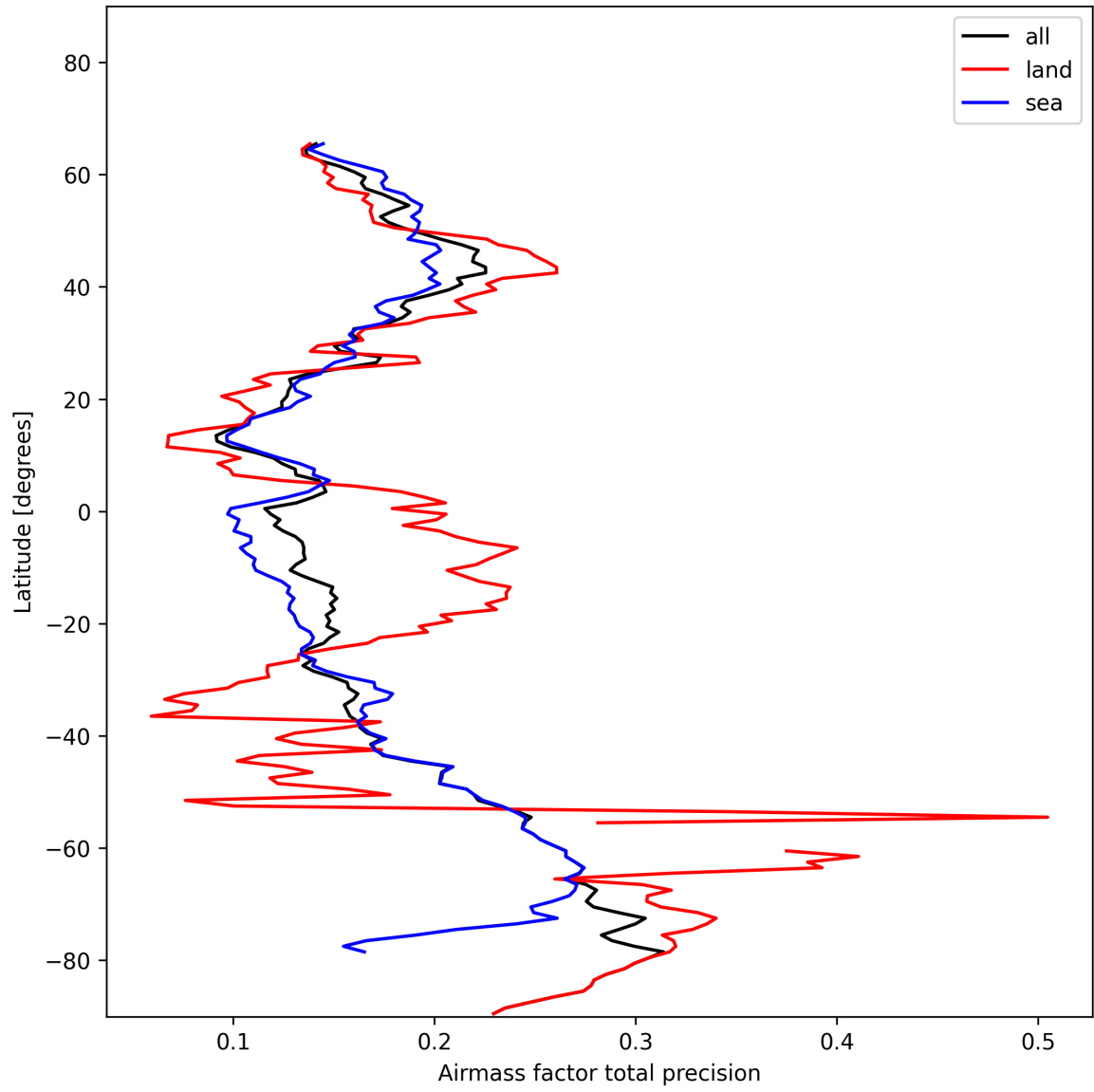
Figure 25: Zonal average of “Airmass factor total precision” for 2025-01-22 to 2025-01-23.
