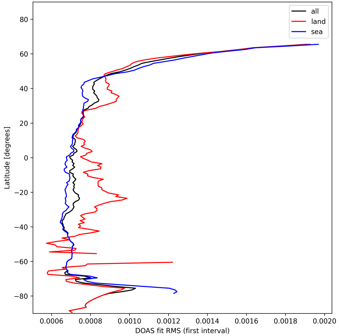
Figure 30: Zonal average of "DOAS fit RMS (first interval)" for 2025-01-22 to 2025-01-23.
