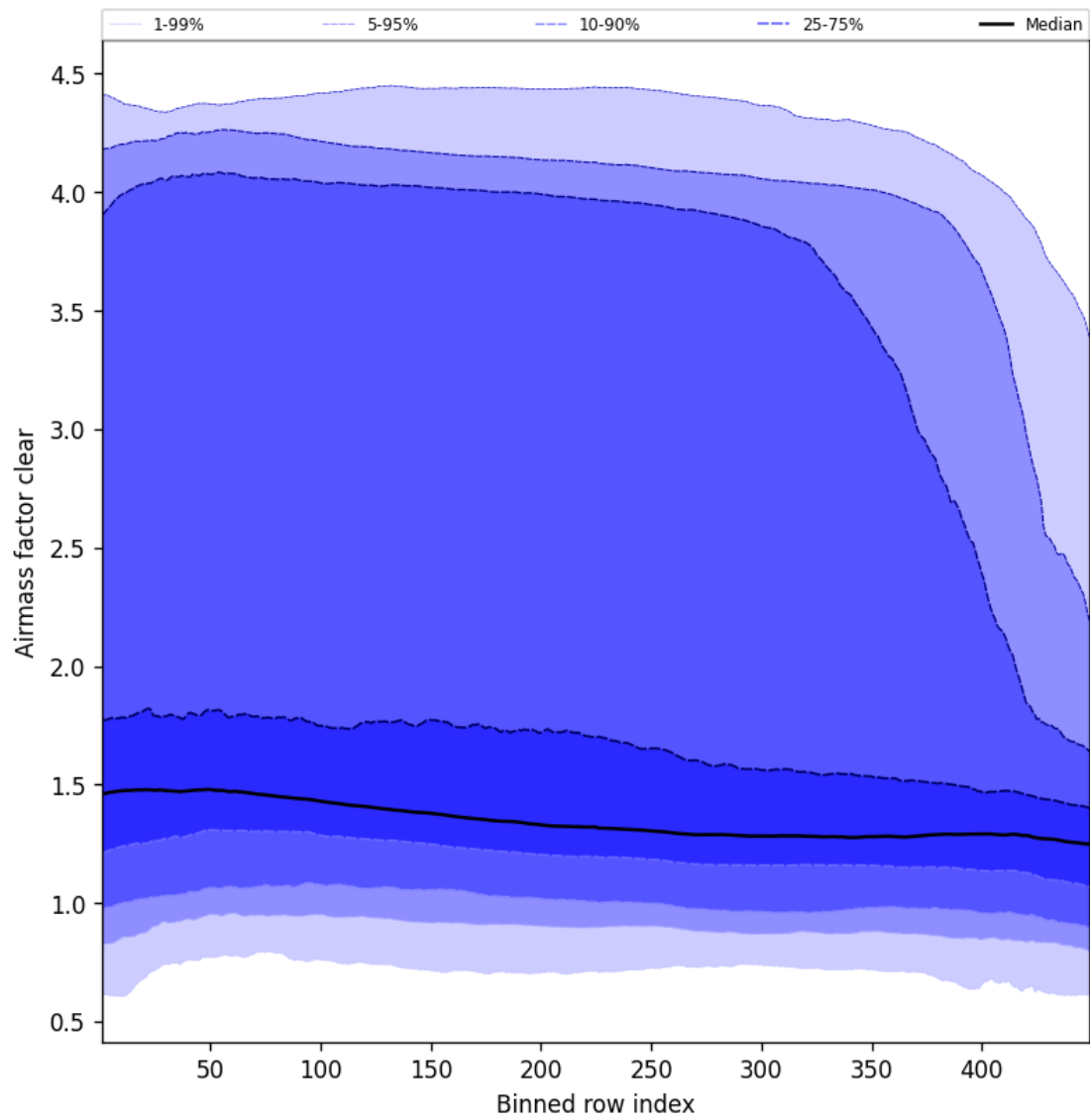
Figure 54: Along track statistics of “Airmass factor clear” for 2025-01-22 to 2025-01-23
