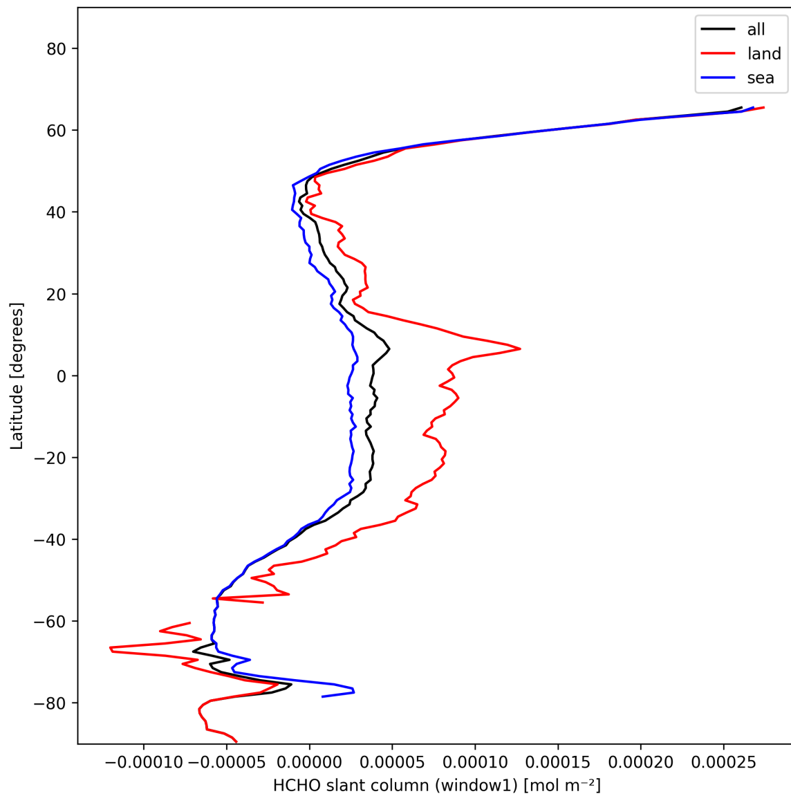
Figure 22: Zonal average of “HCHO slant column (window1)” for 2025-01-22 to 2025-01-23.
