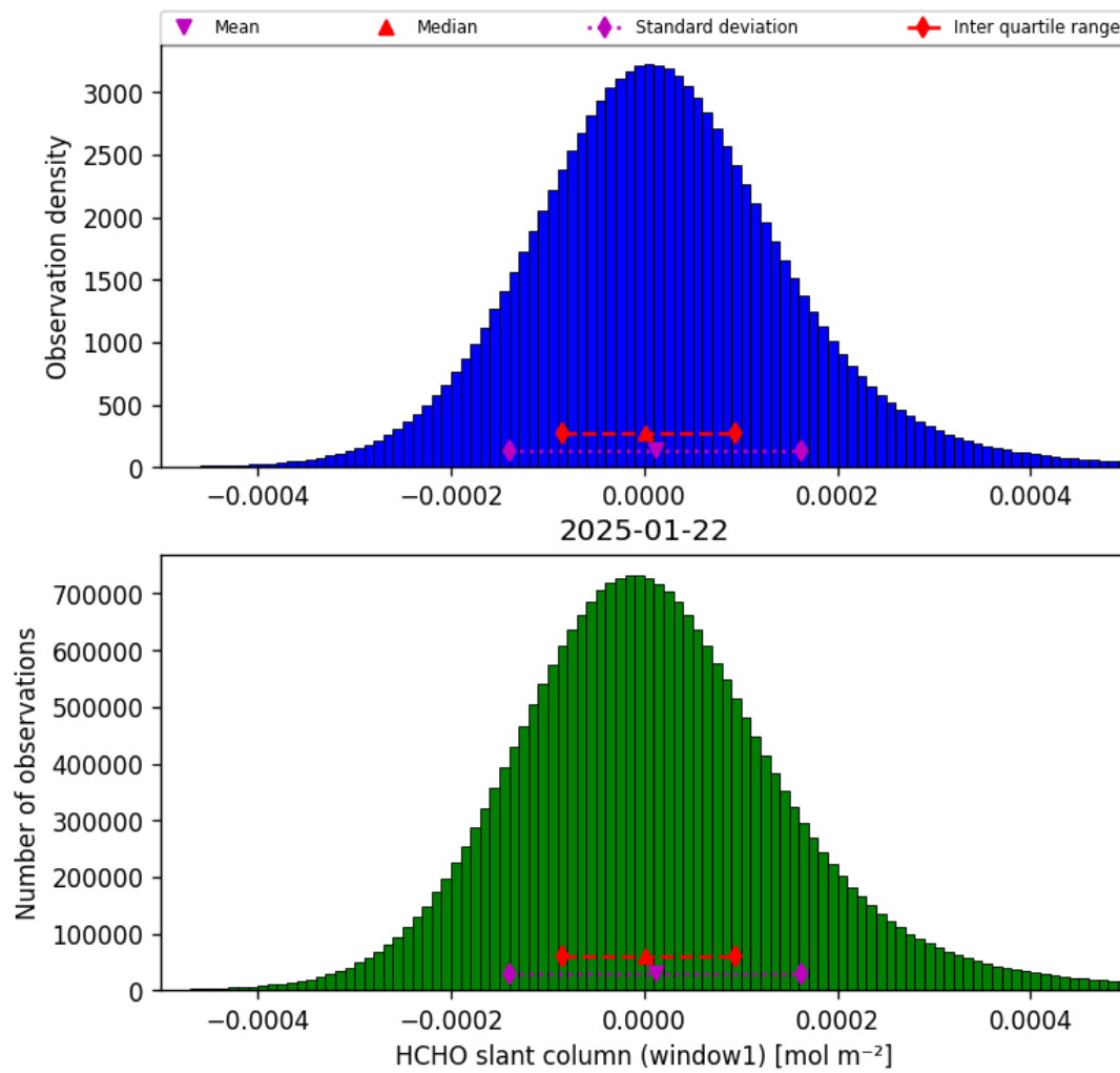
Figure 36: Histogram of “HCHO slant column (window1)” for 2025-01-22 to 2025-01-23
