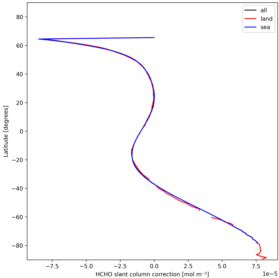
Figure 31: Zonal average of “HCHO slant column correction” for 2025-01-22 to 2025-01-23.
