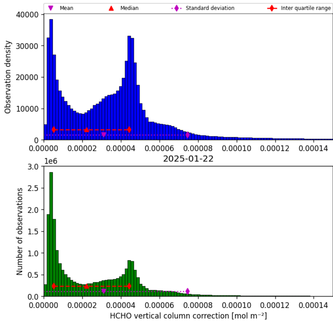
Figure 35: Histogram of “HCHO vertical column correction” for 2025-01-22 to 2025-01-23
