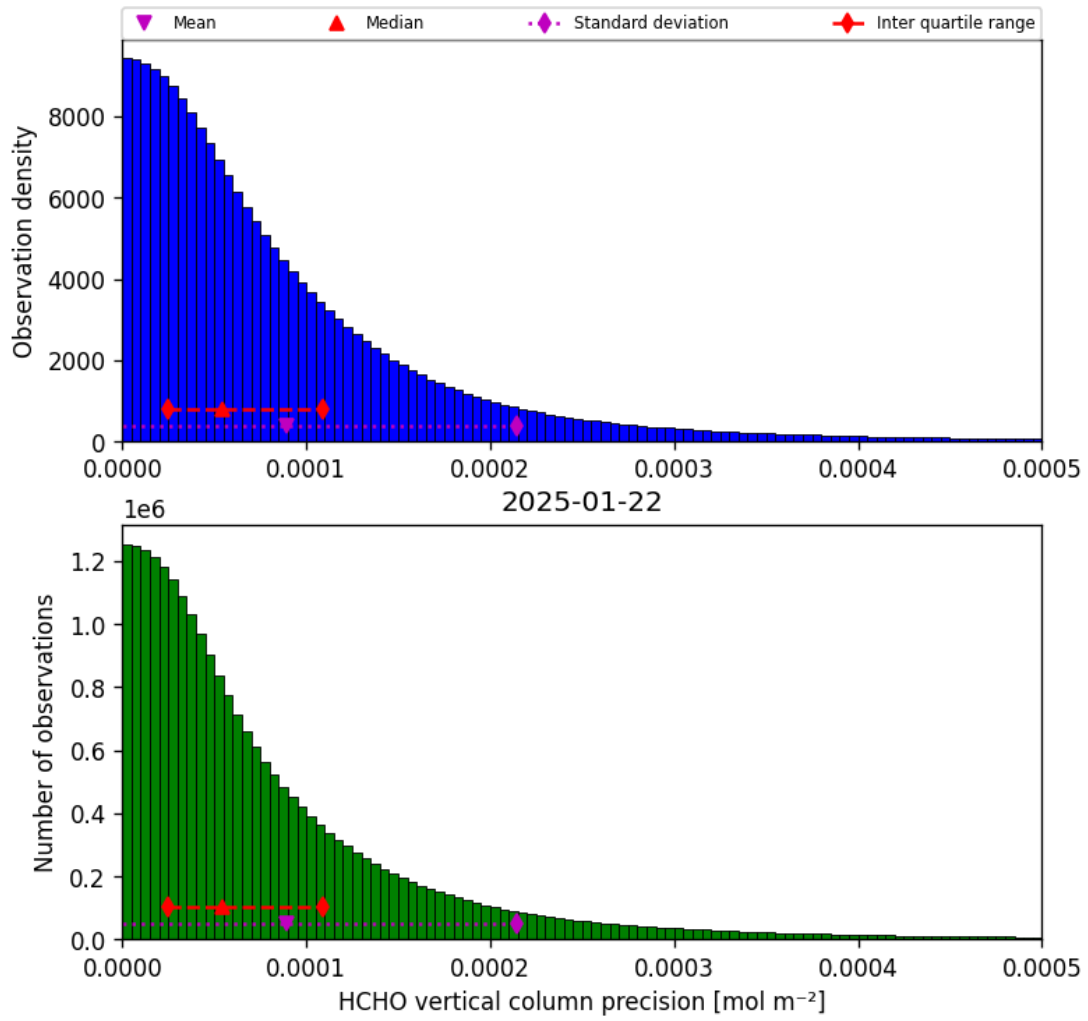
Figure 34: Histogram of “HCHO vertical column precision” for 2025-01-22 to 2025-01-23
