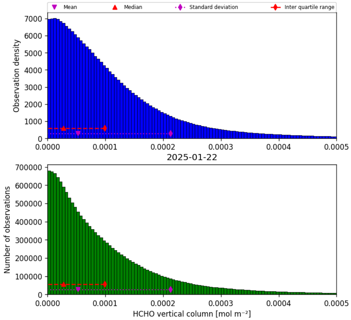
Figure 33: Histogram of “HCHO vertical column” for 2025-01-22 to 2025-01-23
