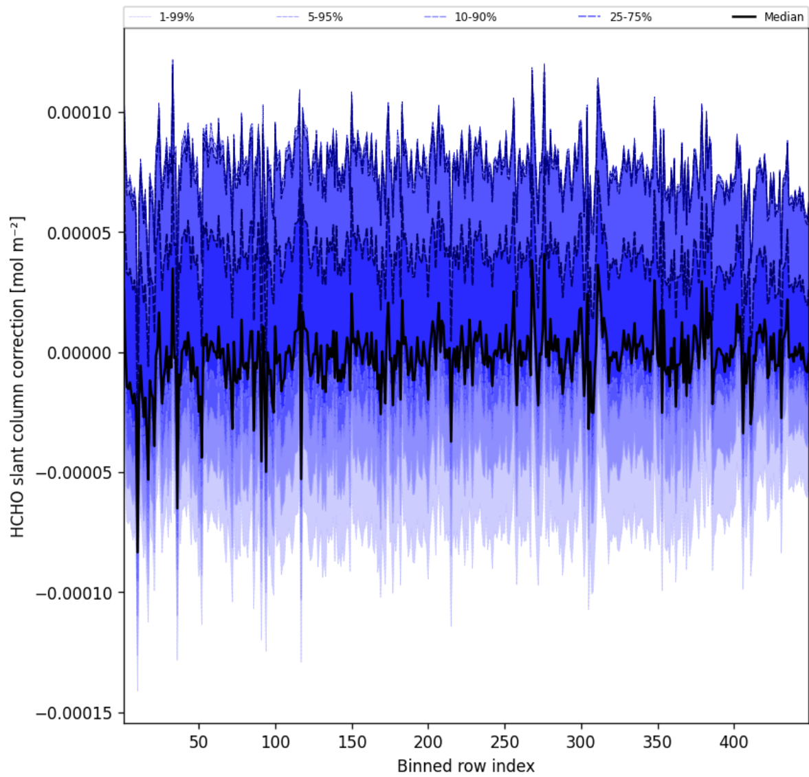
Figure 59: Along track statistics of “HCHO slant column correction” for 2025-01-22 to 2025-01-23
