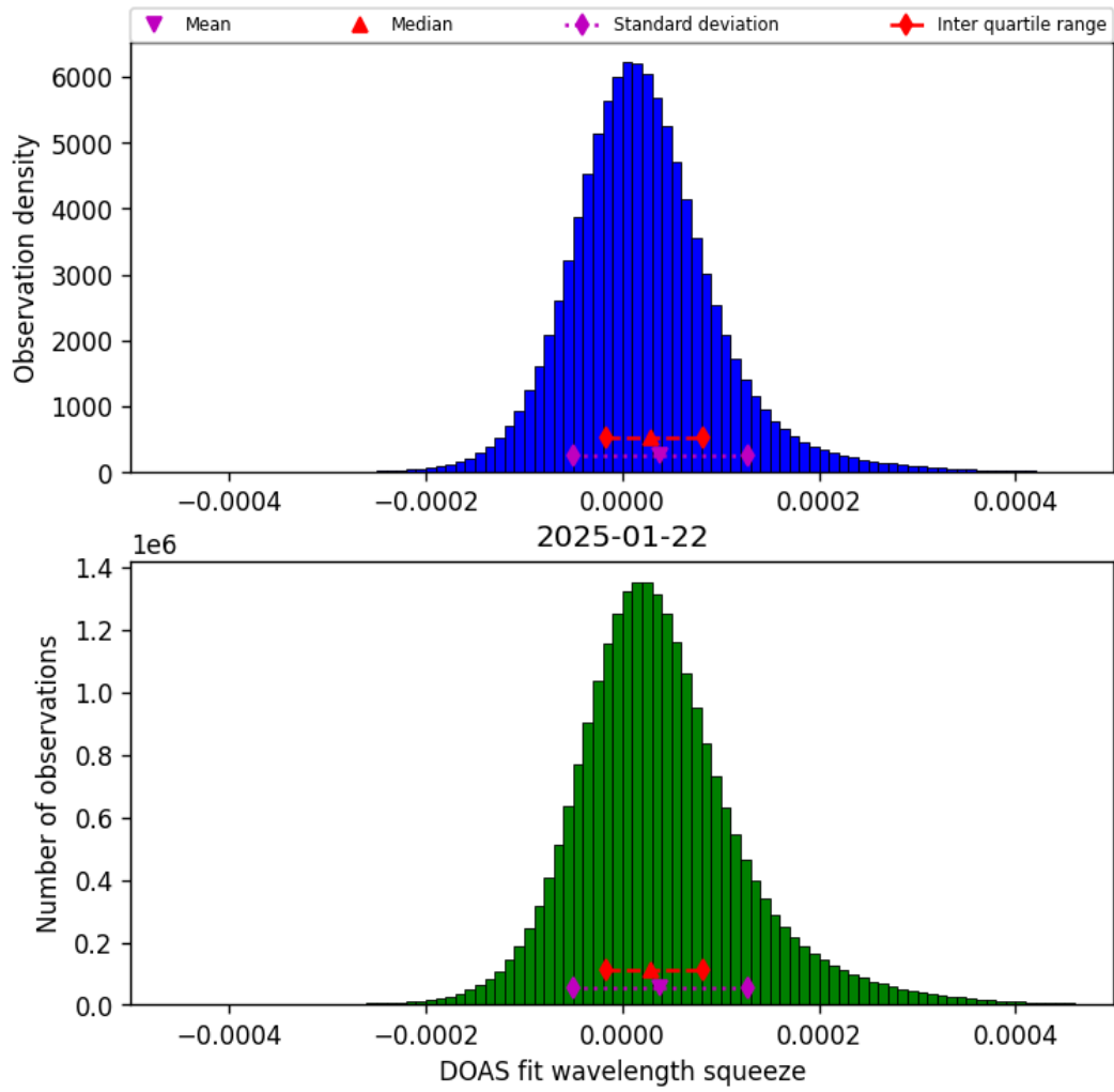
Figure 43: Histogram of “DOAS fit wavelength squeeze” for 2025-01-22 to 2025-01-23
