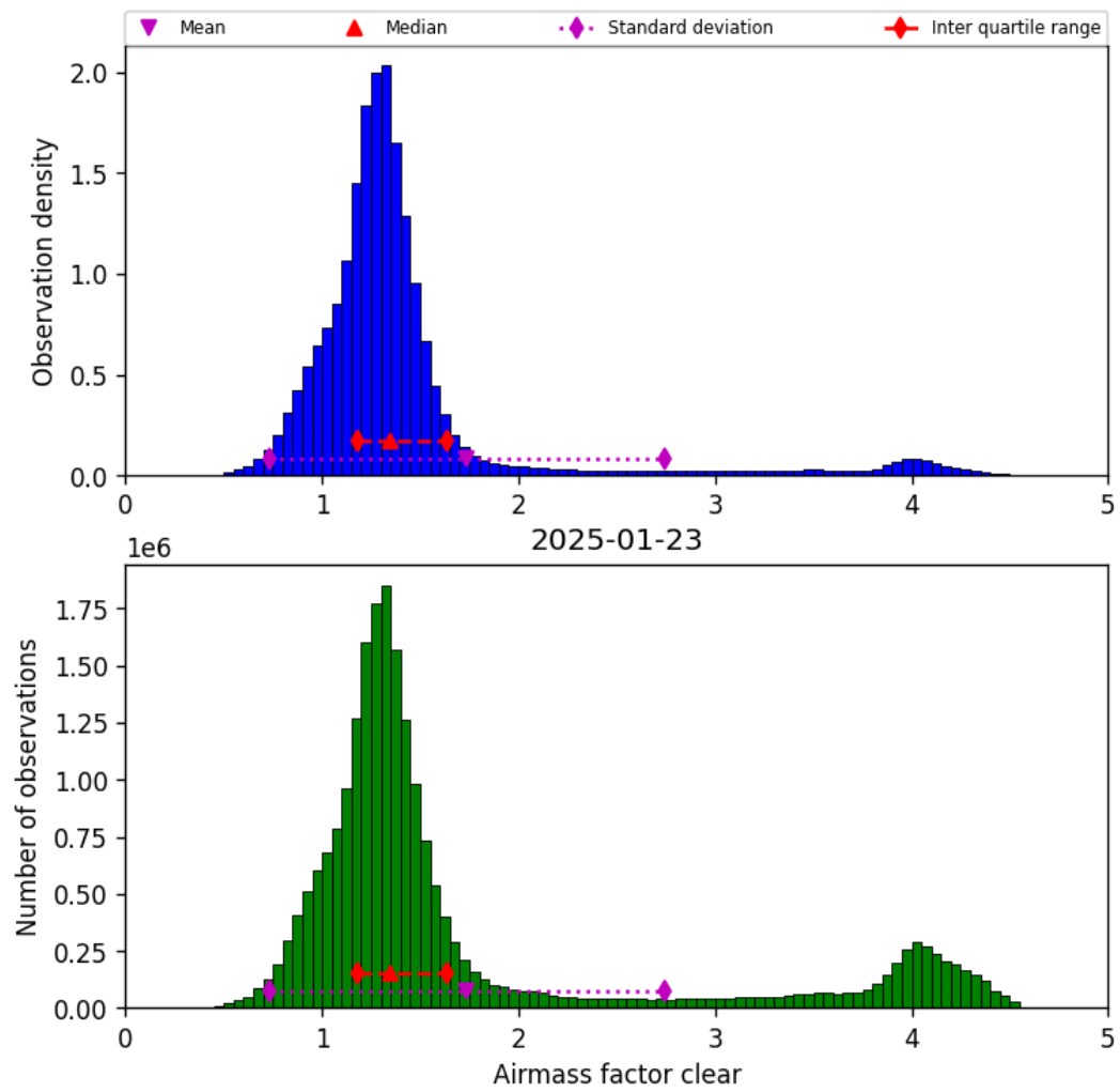
Figure 40: Histogram of “Airmass factor clear” for 2025-01-23 to 2025-01-24
