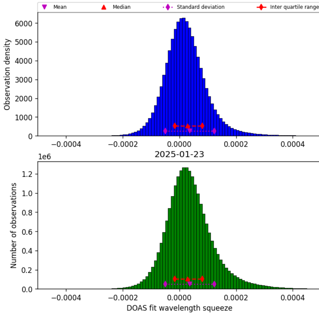
Figure 43: Histogram of “DOAS fit wavelength squeeze” for 2025-01-23 to 2025-01-24
