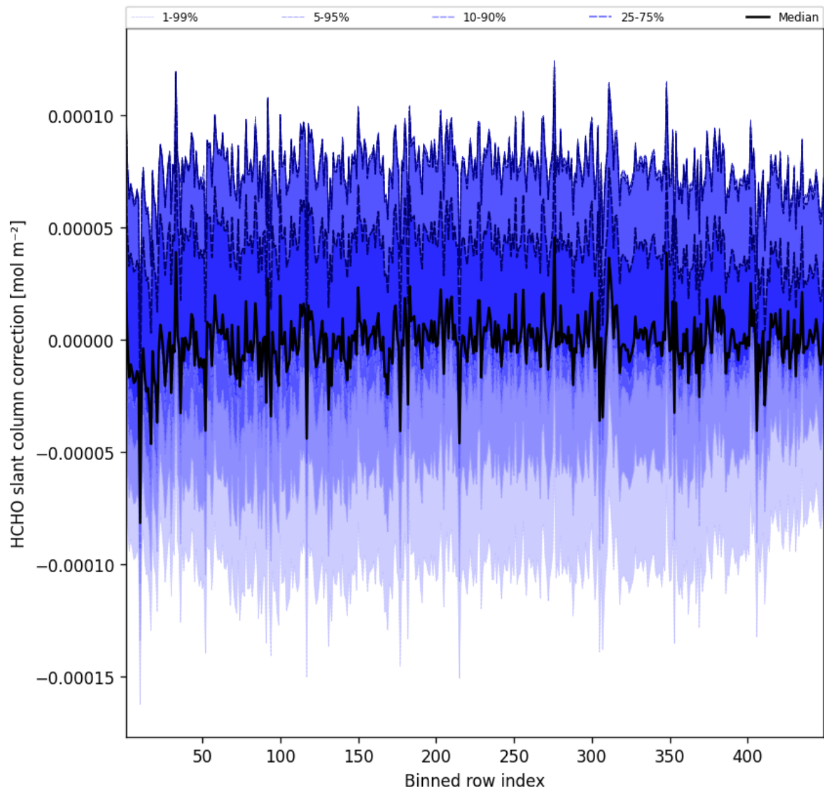
Figure 59: Along track statistics of “HCHO slant column correction” for 2025-01-23 to 2025-01-24
