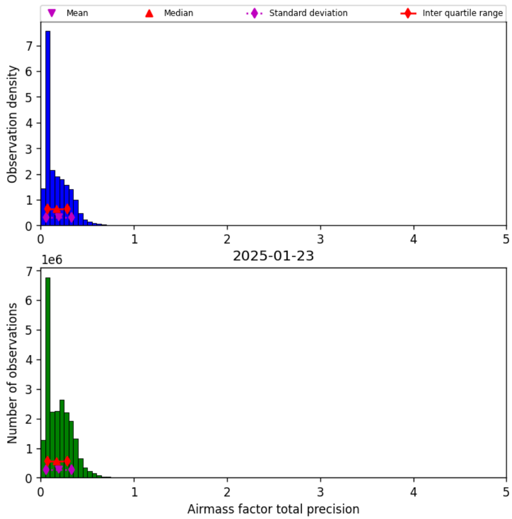
Figure 39: Histogram of “Airmass factor total precision” for 2025-01-23 to 2025-01-24
