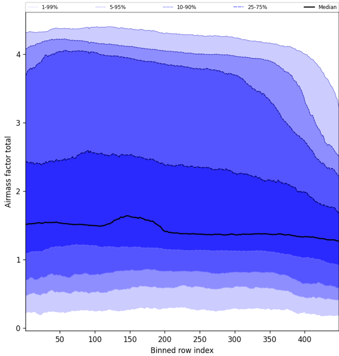
Figure 52: Along track statistics of “Airmass factor total” for 2025-01-23 to 2025-01-24
