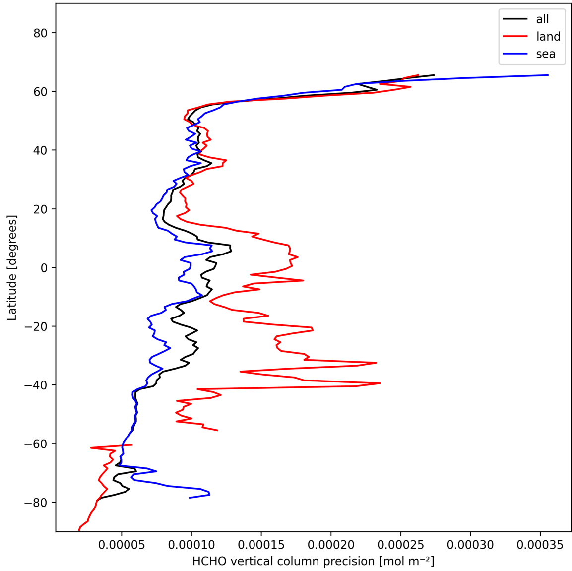
Figure 20: Zonal average of “HCHO vertical column precision” for 2025-01-23 to 2025-01-24.
