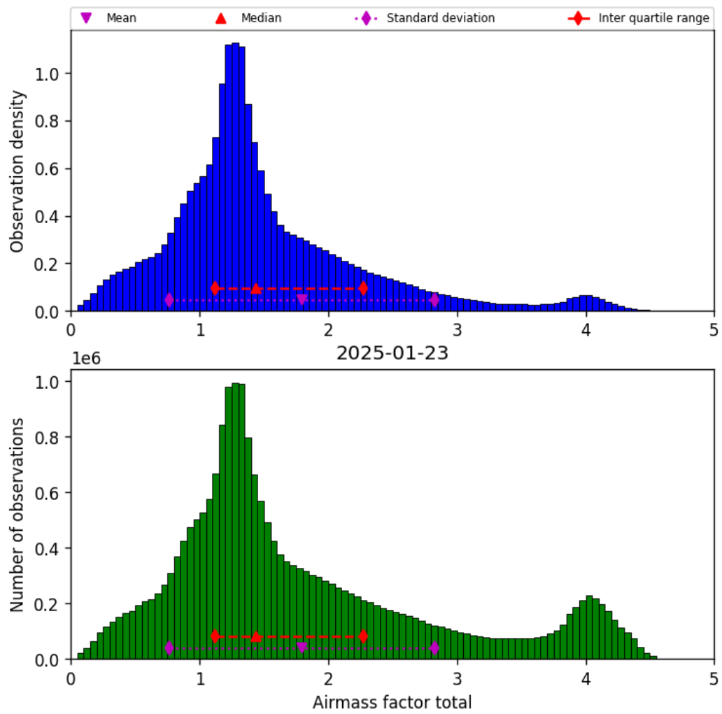
Figure 38: Histogram of “Airmass factor total” for 2025-01-23 to 2025-01-24
