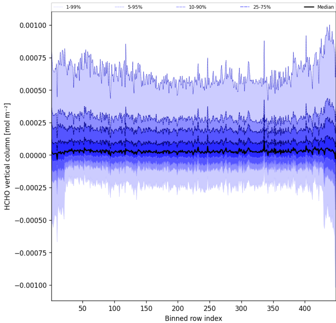
Figure 47: Along track statistics of “HCHO vertical column” for 2025-01-23 to 2025-01-24
