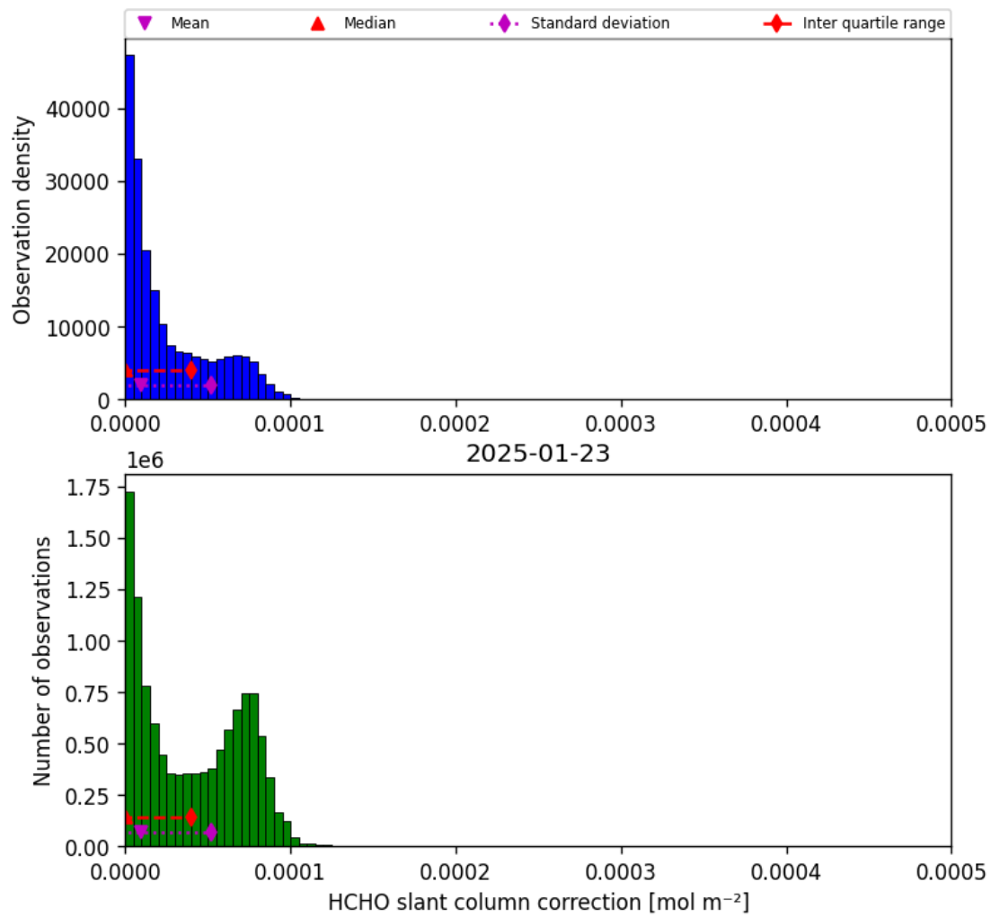
Figure 45: Histogram of “HCHO slant column correction” for 2025-01-23 to 2025-01-24
