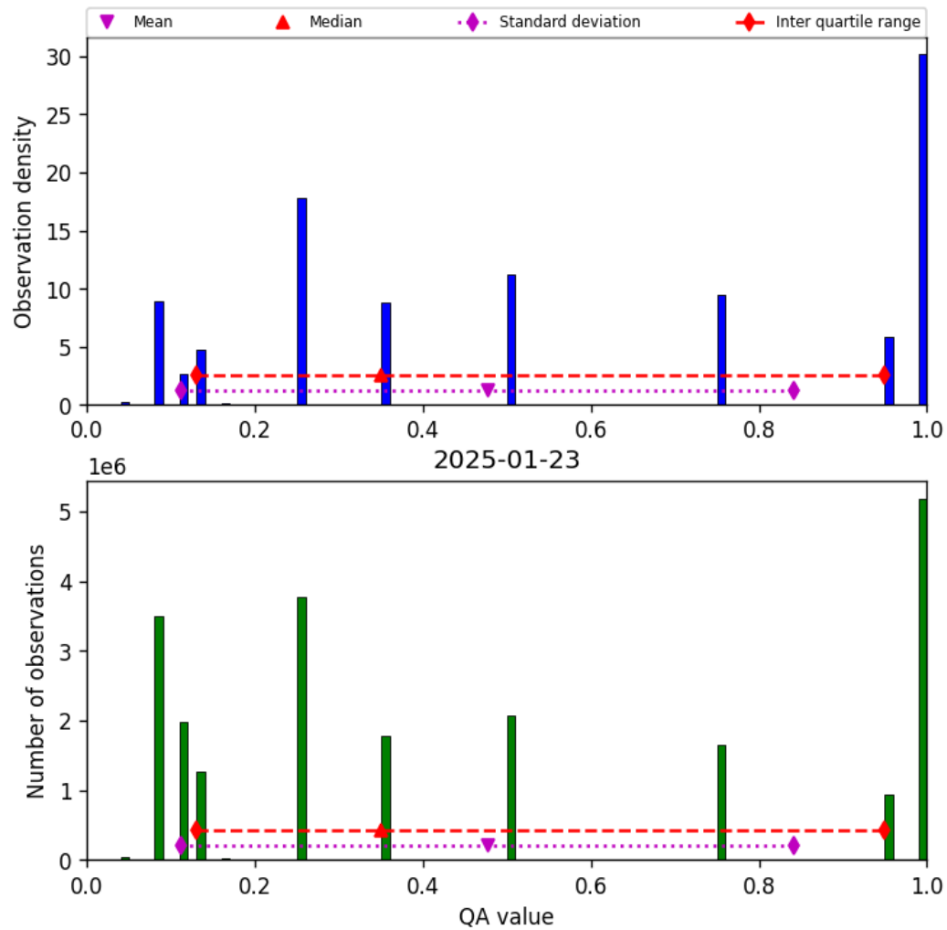
Figure 32: Histogram of “QA value” for 2025-01-23 to 2025-01-24
