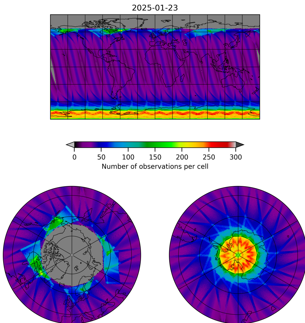
Figure 17: Map of the number of observations for 2025-01-23 to 2025-01-24
