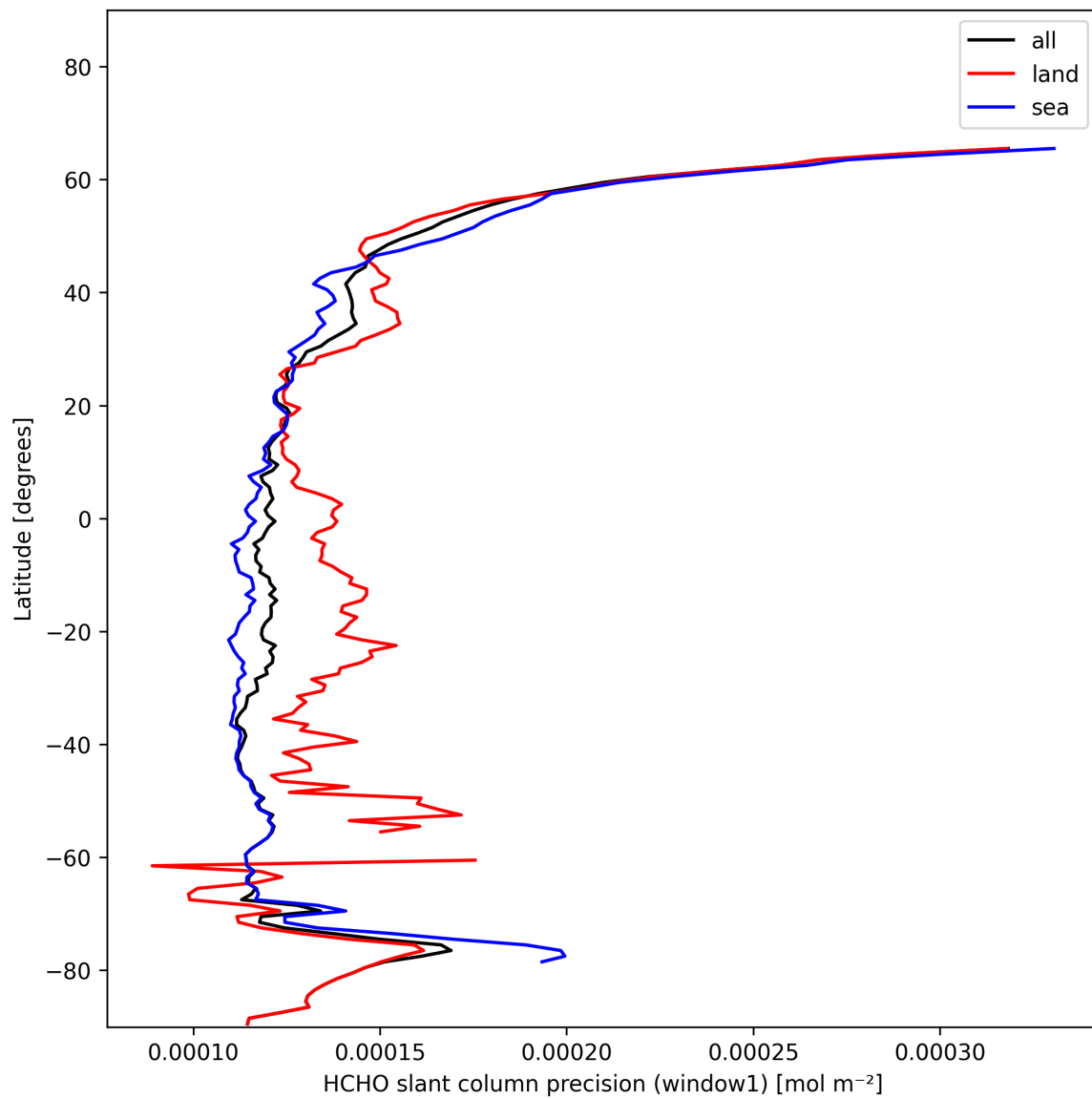
Figure 23: Zonal average of “HCHO slant column precision (window1)” for 2025-01-23 to 2025-01-24.
