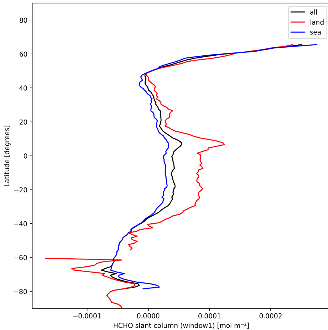
Figure 22: Zonal average of “HCHO slant column (window1)” for 2025-01-23 to 2025-01-24.
