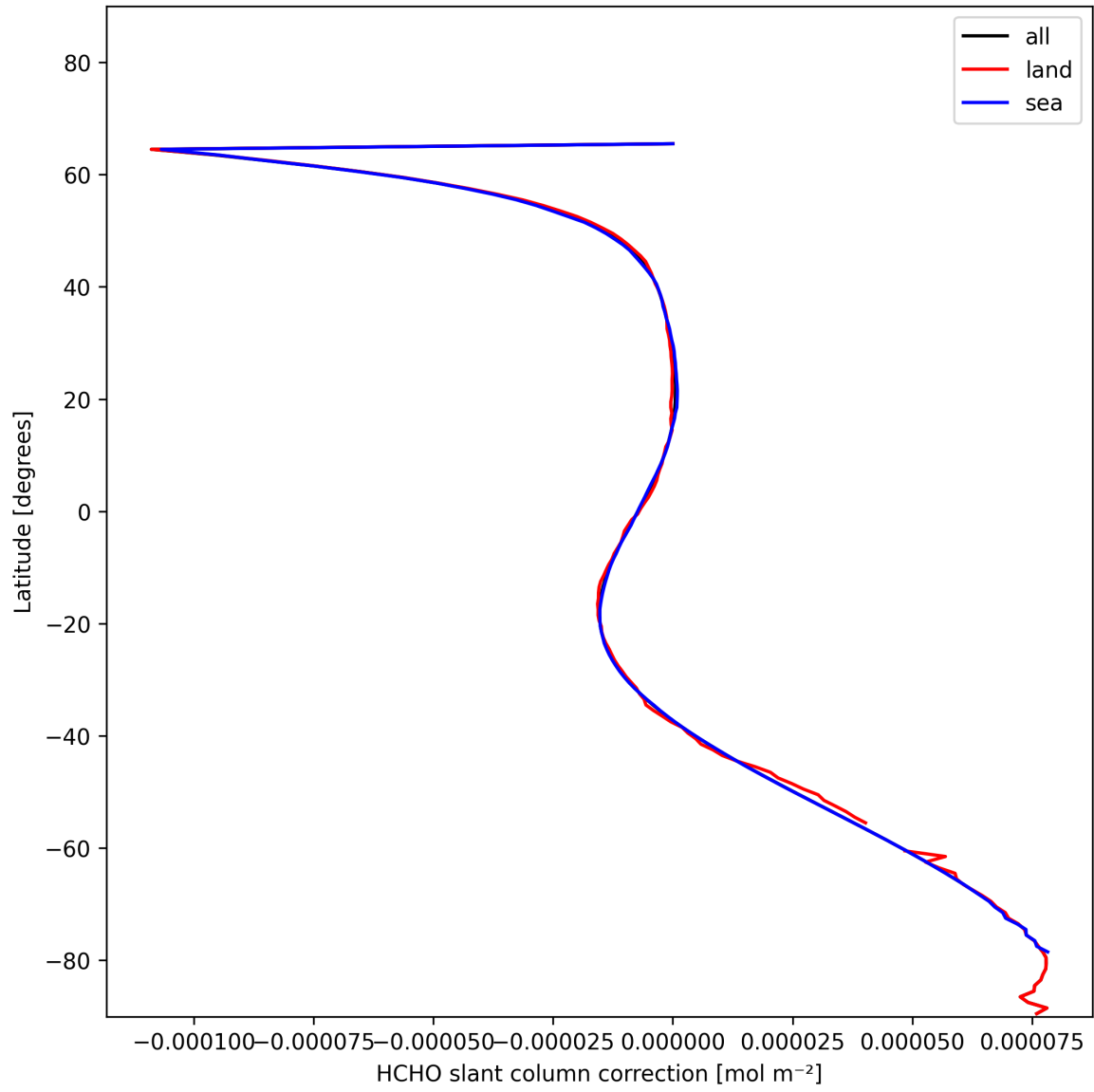
Figure 31: Zonal average of “HCHO slant column correction” for 2025-01-23 to 2025-01-24.
