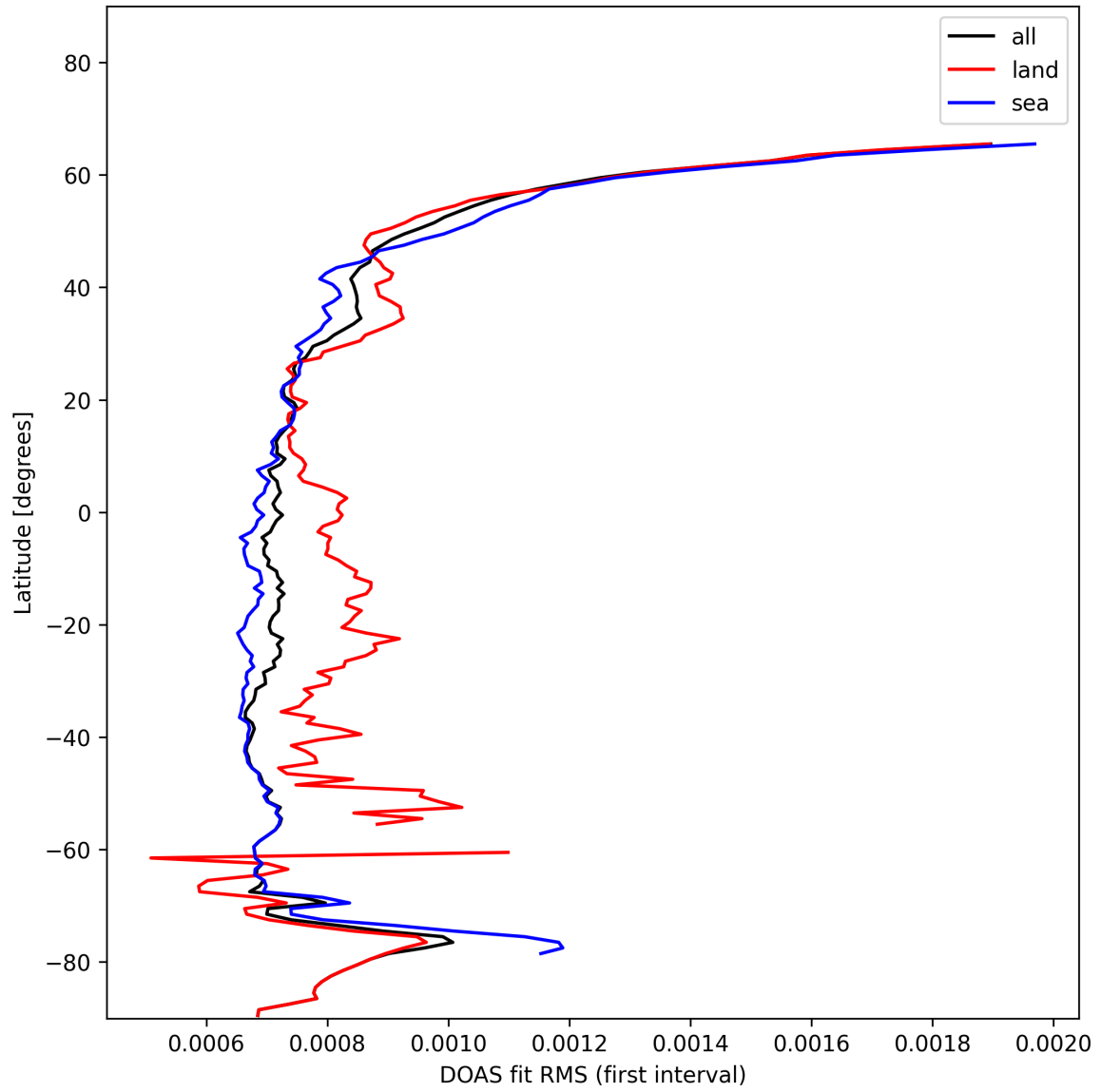
Figure 30: Zonal average of “DOAS fit RMS (first interval)” for 2025-01-23 to 2025-01-24.
