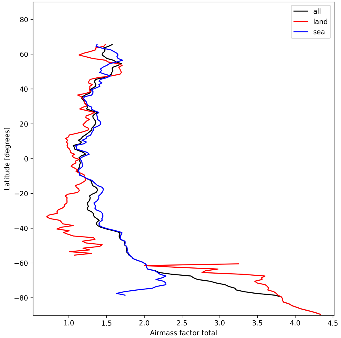
Figure 24: Zonal average of “Airmass factor total” for 2025-01-23 to 2025-01-24.
