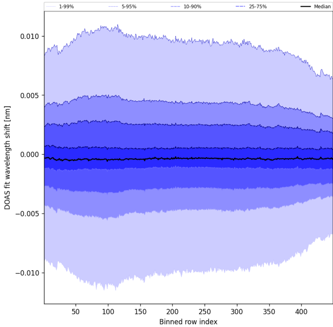
Figure 56: Along track statistics of “DOAS fit wavelength shift” for 2025-01-23 to 2025-01-24
