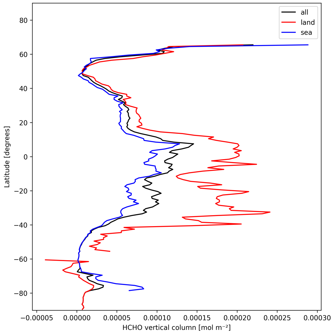
Figure 19: Zonal average of “HCHO vertical column” for 2025-01-23 to 2025-01-24.
