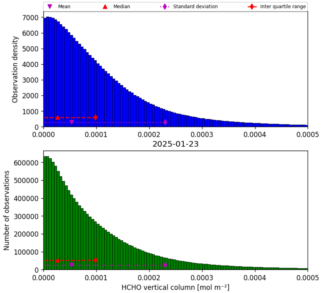
Figure 33: Histogram of “HCHO vertical column” for 2025-01-23 to 2025-01-24
