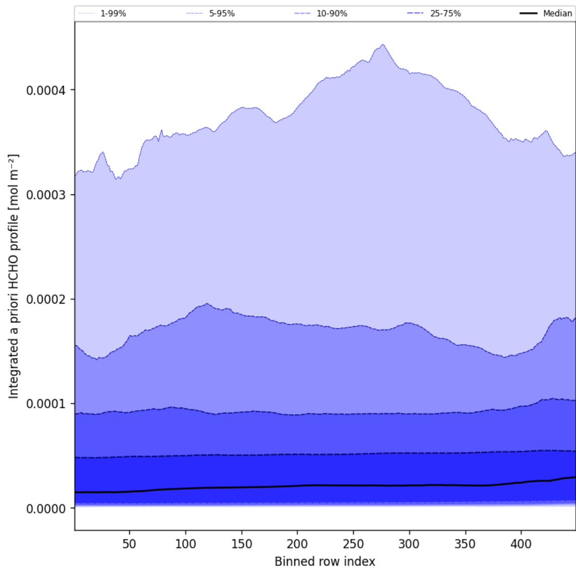
Figure 55: Along track statistics of “Integrated a priori HCHO profile” for 2025-01-23 to 2025-01-24
