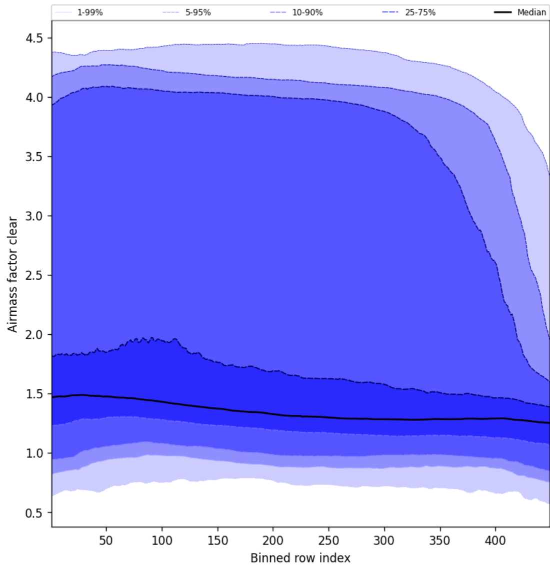
Figure 54: Along track statistics of “Airmass factor clear” for 2025-01-23 to 2025-01-24
