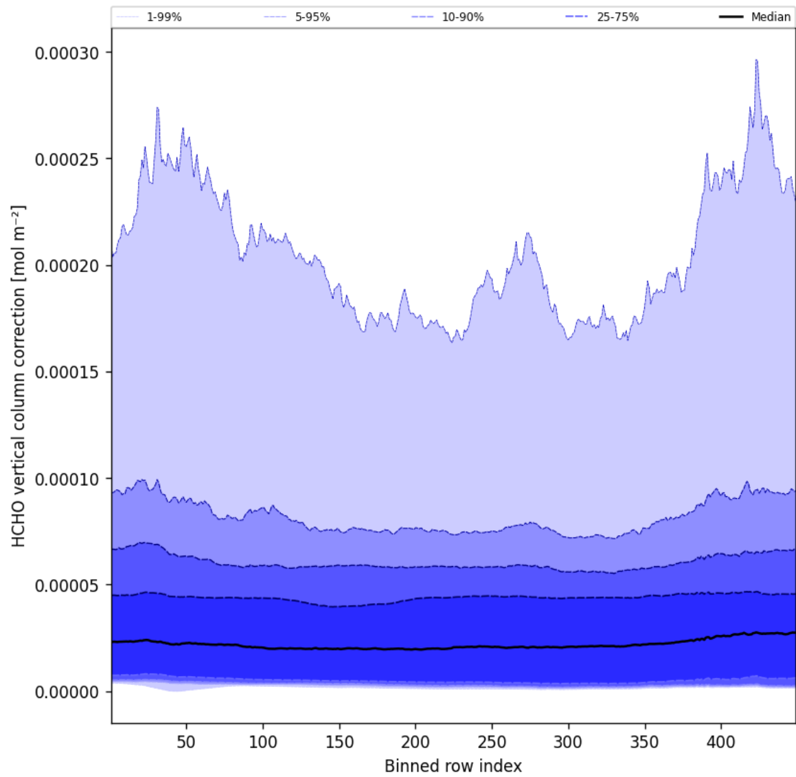
Figure 49: Along track statistics of “HCHO vertical column correction” for 2025-01-23 to 2025-01-24
