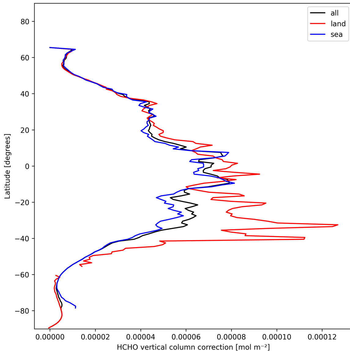
Figure 21: Zonal average of “HCHO vertical column correction” for 2025-01-23 to 2025-01-24.
