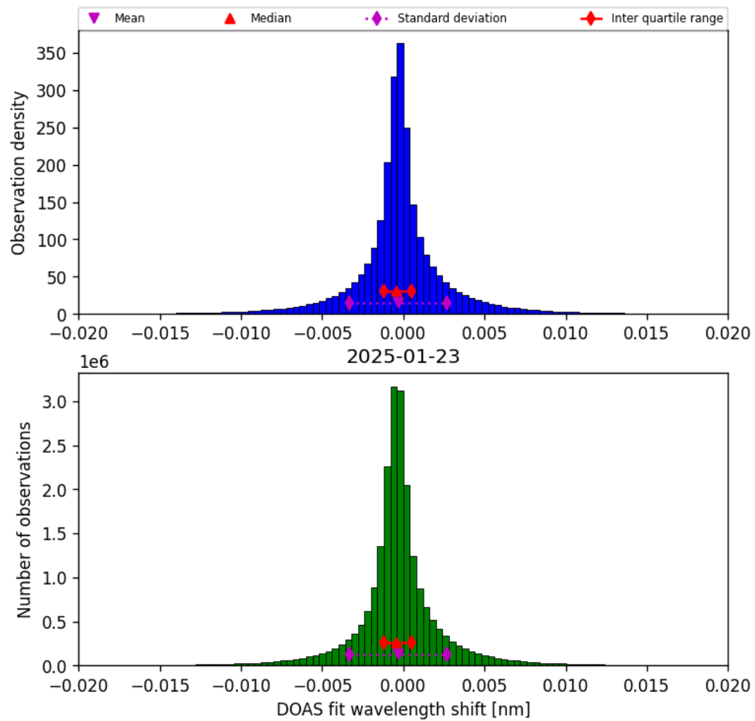
Figure 42: Histogram of “DOAS fit wavelength shift” for 2025-01-23 to 2025-01-24
