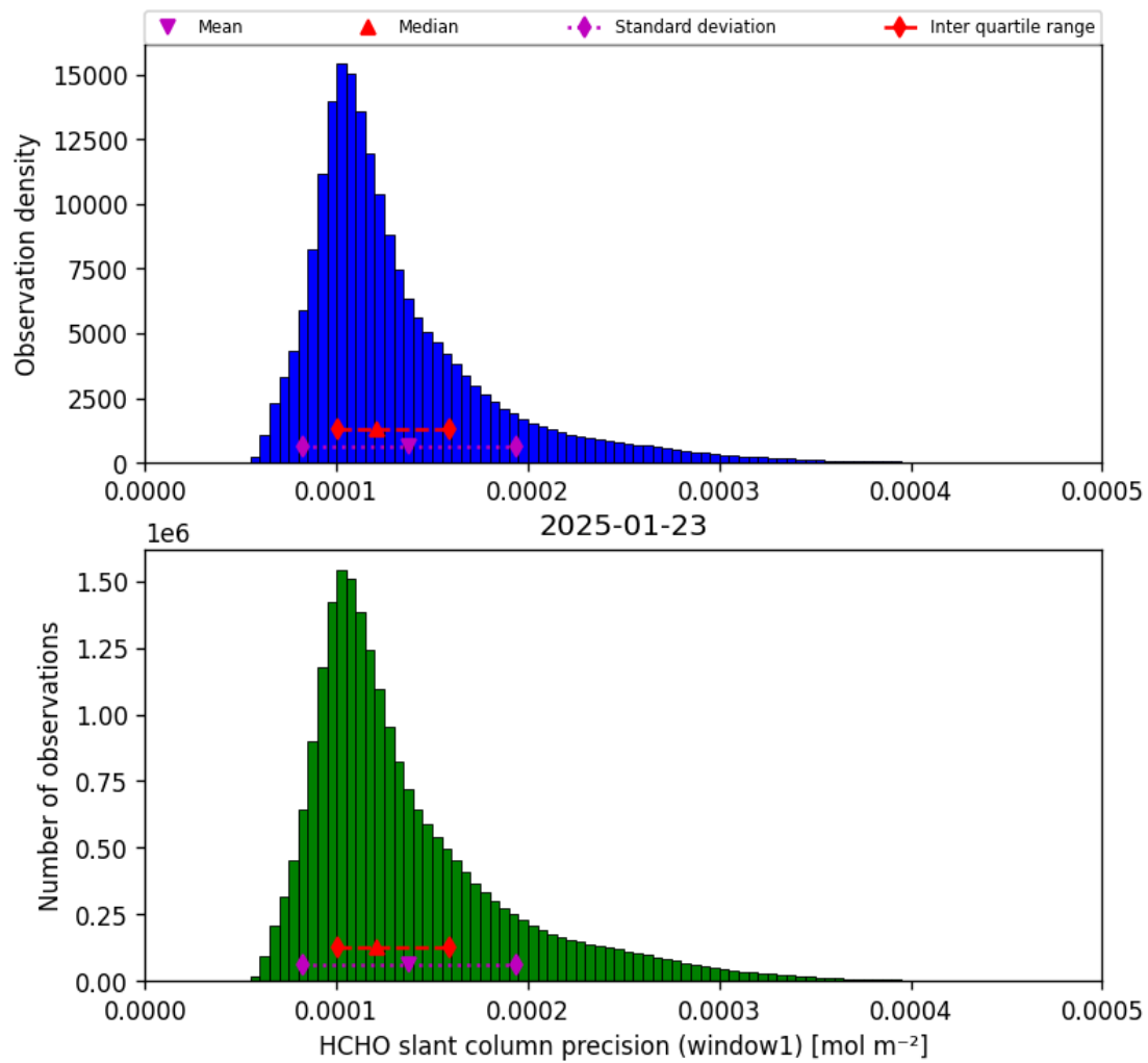
Figure 37: Histogram of “HCHO slant column precision (window1)” for 2025-01-23 to 2025-01-24
