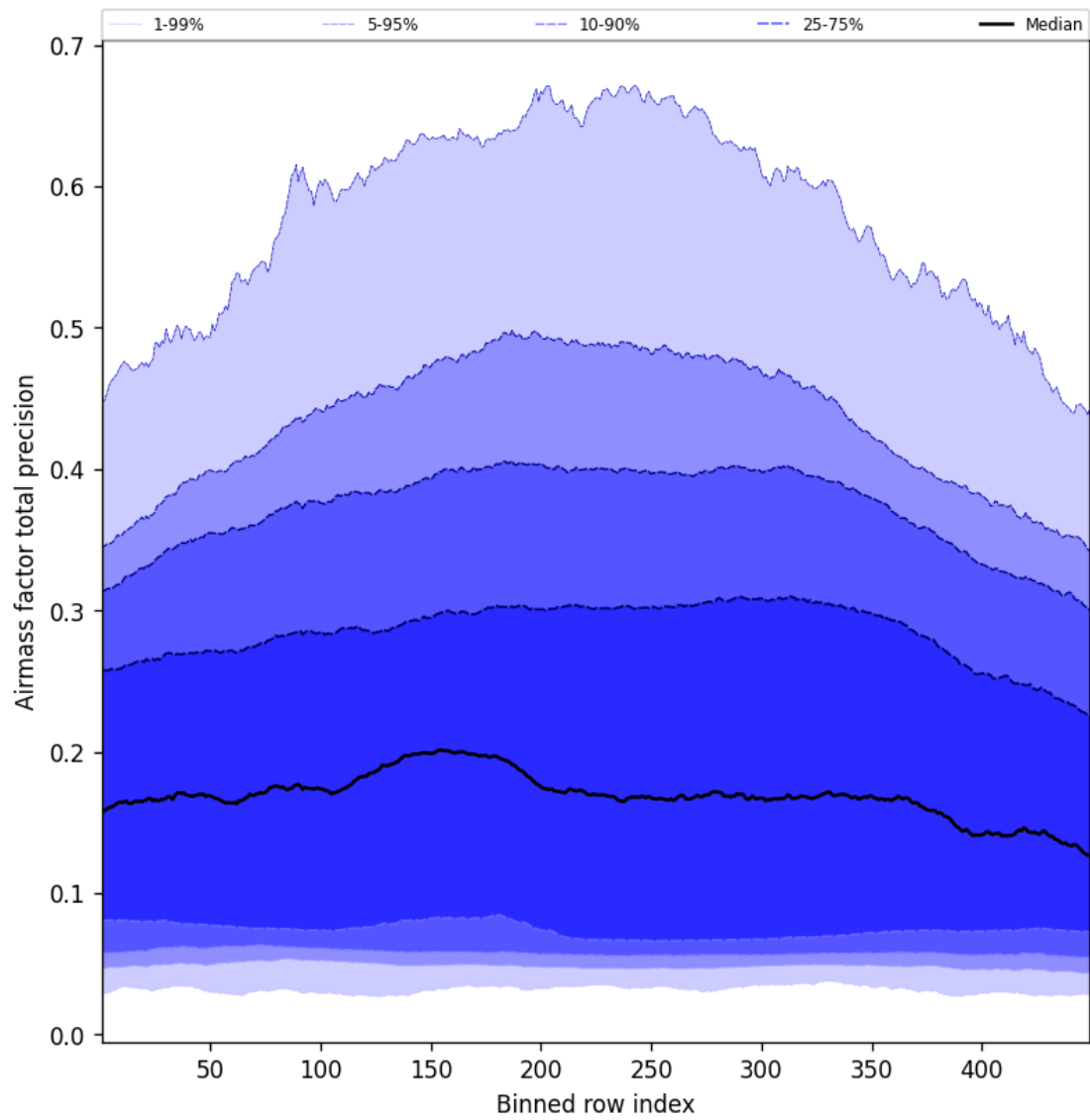
Figure 53: Along track statistics of “Airmass factor total precision” for 2025-01-23 to 2025-01-24
