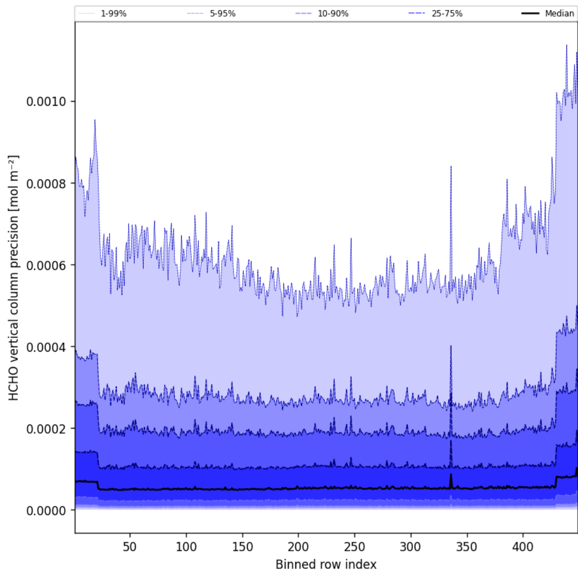
Figure 48: Along track statistics of “HCHO vertical column precision” for 2025-01-23 to 2025-01-24
