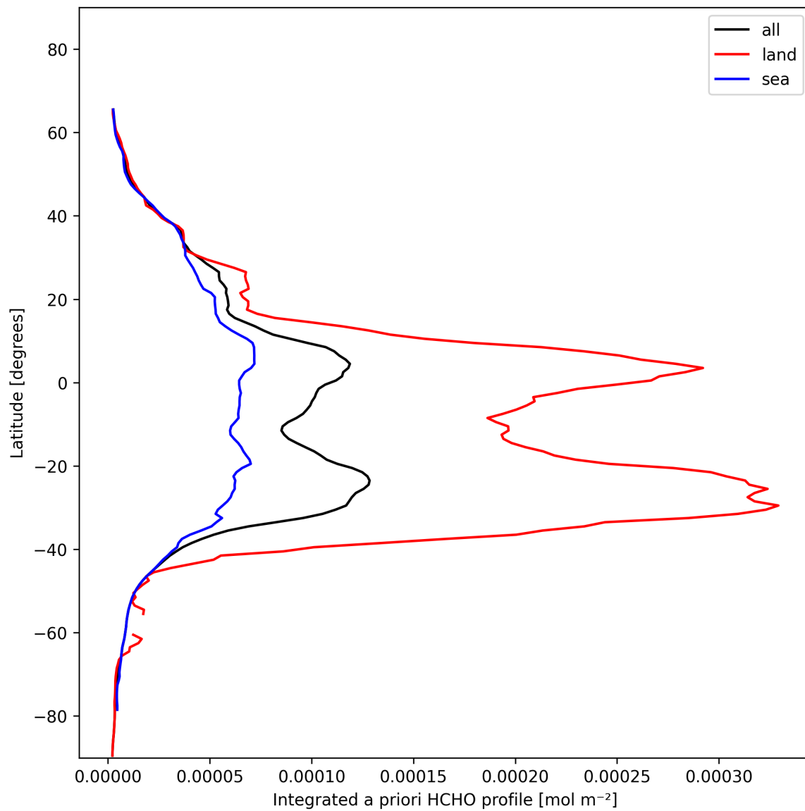
Figure 27: Zonal average of “Integrated a priori HCHO profile” for 2025-01-23 to 2025-01-24.
