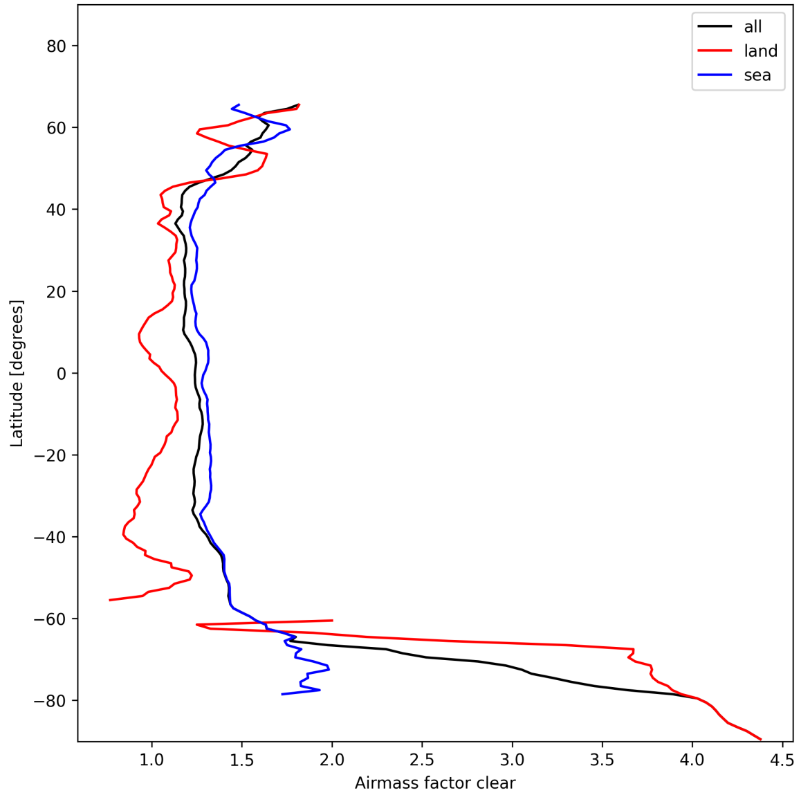
Figure 26: Zonal average of “Airmass factor clear” for 2025-01-23 to 2025-01-24.
