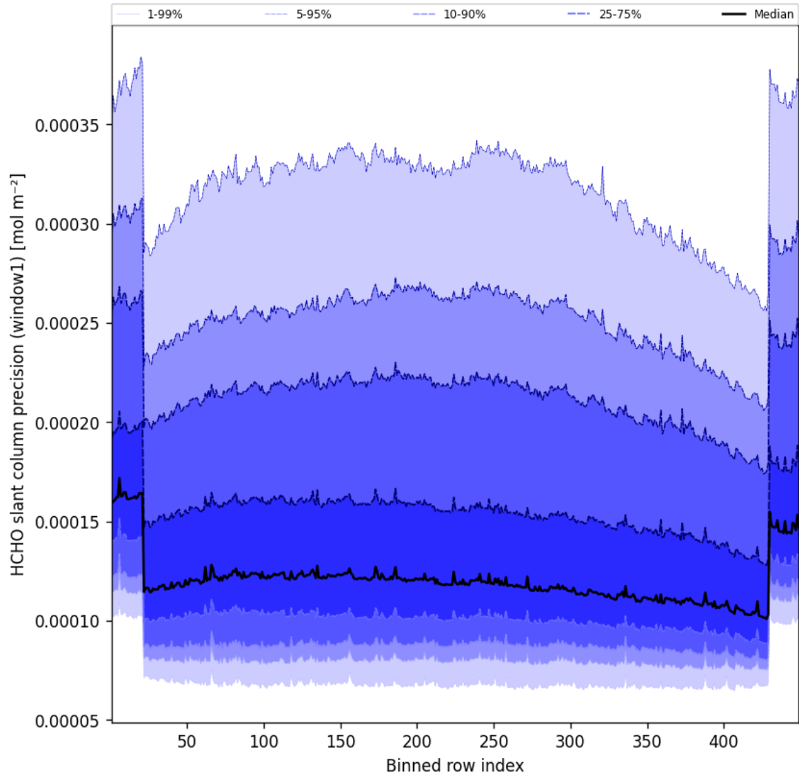
Figure 51: Along track statistics of “HCHO slant column precision (window1)” for 2025-01-23 to 2025-01-24
