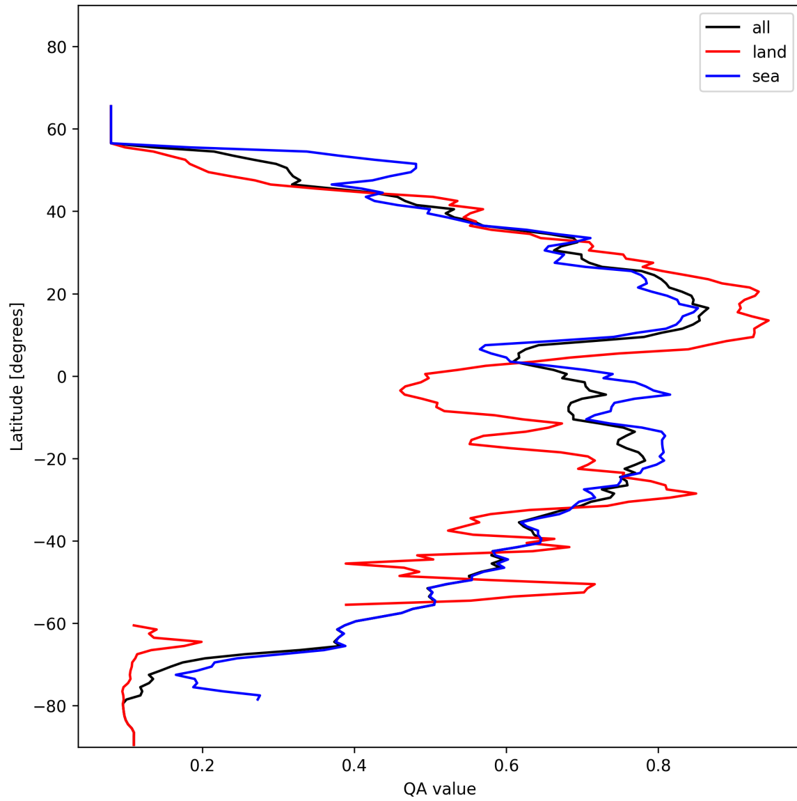
Figure 18: Zonal average of “QA value” for 2025-01-23 to 2025-01-24.
