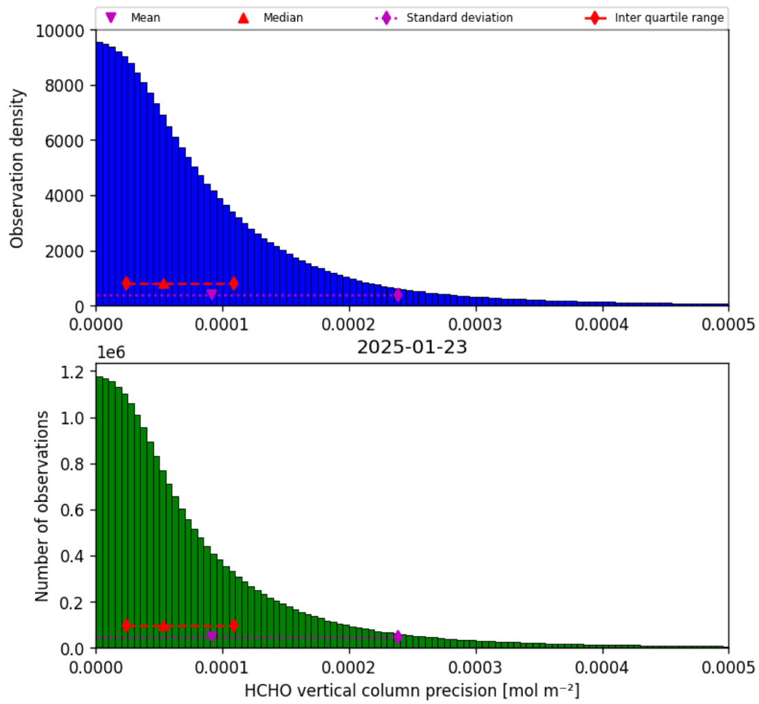
Figure 34: Histogram of “HCHO vertical column precision” for 2025-01-23 to 2025-01-24
