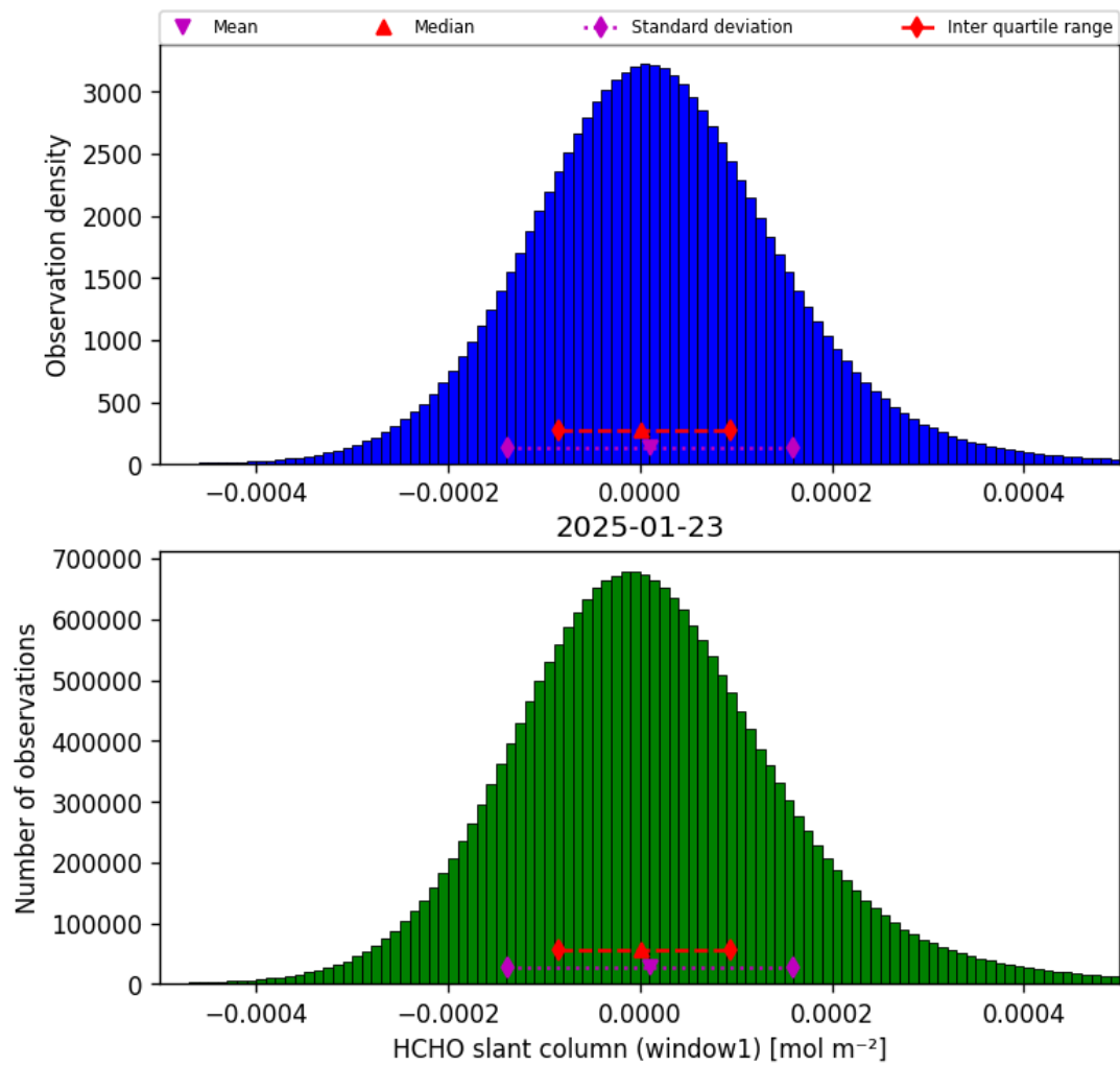
Figure 36: Histogram of “HCHO slant column (window1)” for 2025-01-23 to 2025-01-24
