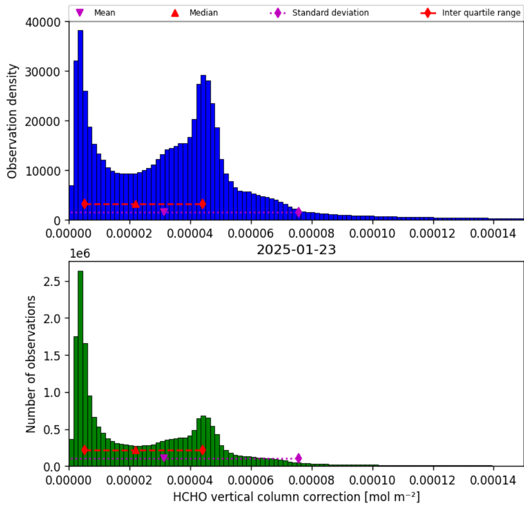
Figure 35: Histogram of “HCHO vertical column correction” for 2025-01-23 to 2025-01-24
