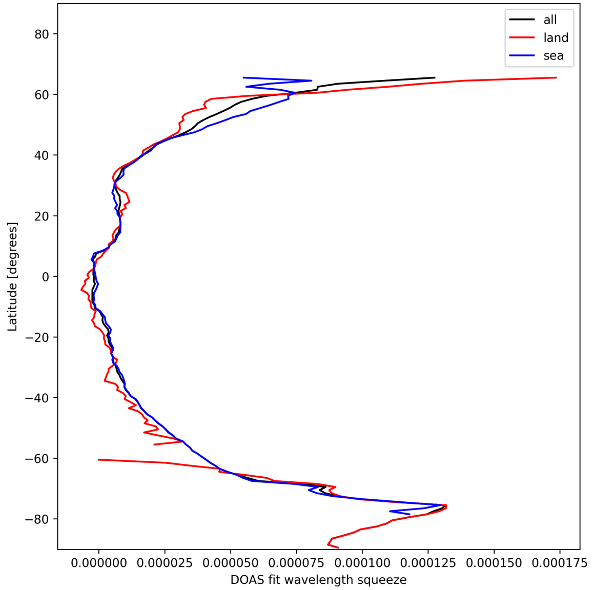
Figure 29: Zonal average of “DOAS fit wavelength squeeze” for 2025-01-23 to 2025-01-24.
