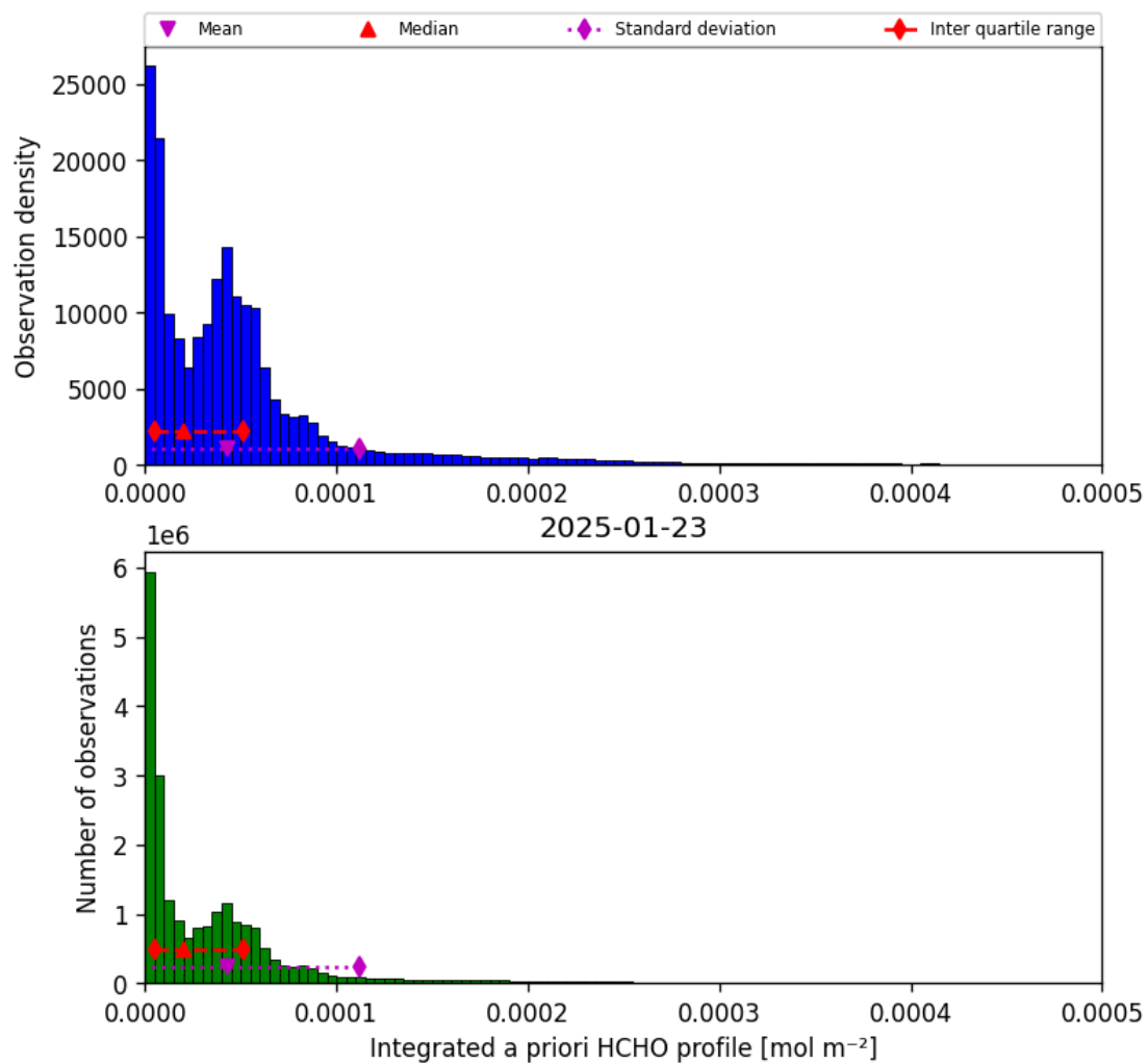
Figure 41: Histogram of “Integrated a priori HCHO profile” for 2025-01-23 to 2025-01-24
