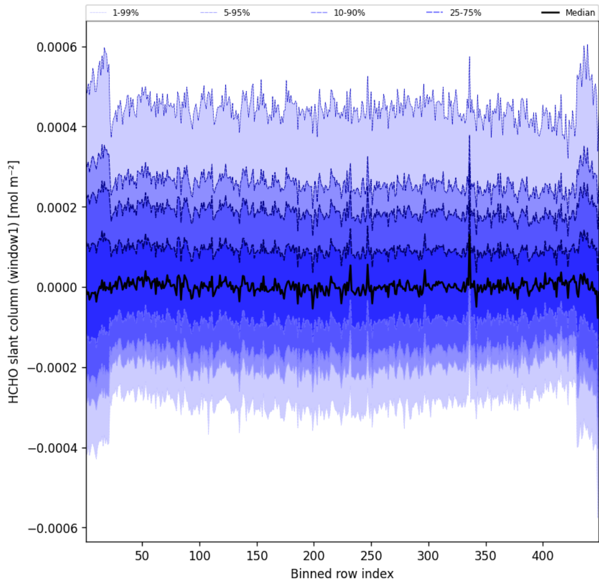
Figure 50: Along track statistics of “HCHO slant column (window1)” for 2025-01-23 to 2025-01-24
