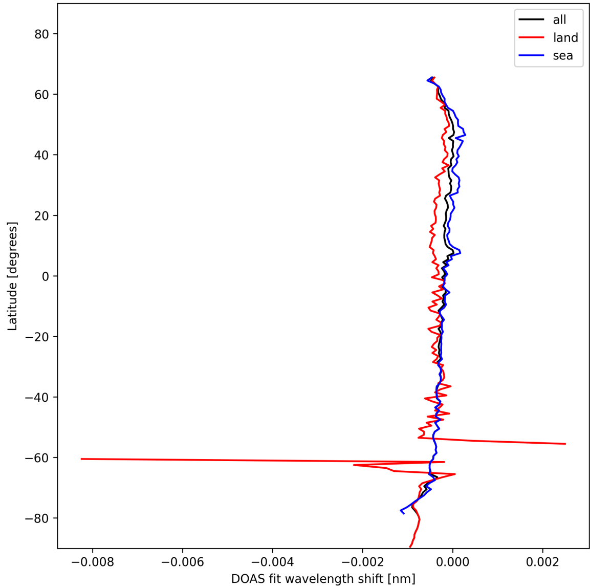
Figure 28: Zonal average of “DOAS fit wavelength shift” for 2025-01-23 to 2025-01-24.
