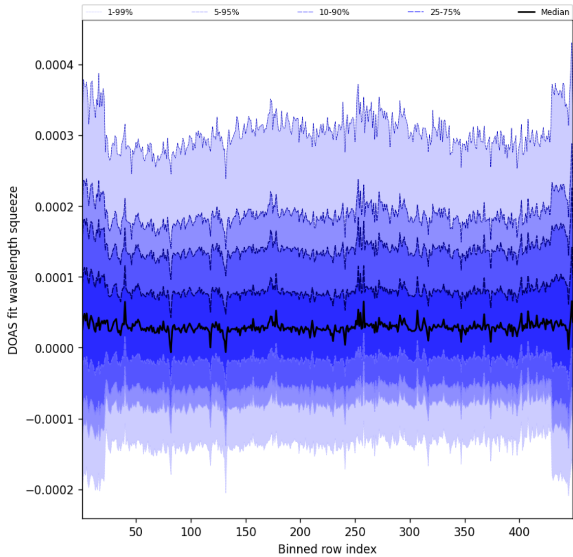
Figure 57: Along track statistics of “DOAS fit wavelength squeeze” for 2025-01-23 to 2025-01-24
