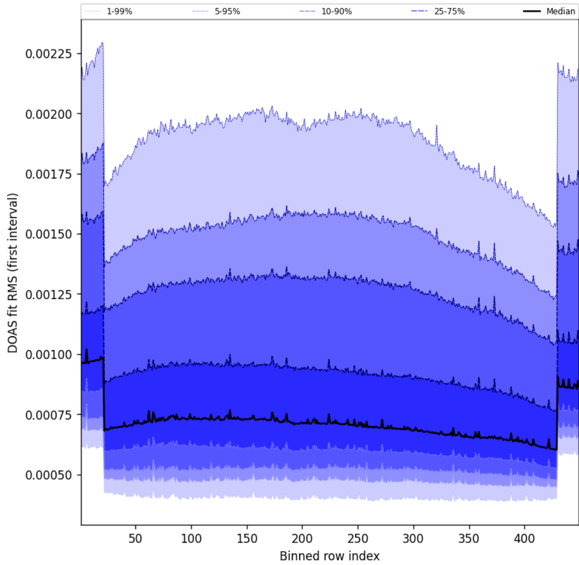
Figure 58: Along track statistics of “DOAS fit RMS (first interval)” for 2025-01-23 to 2025-01-24
