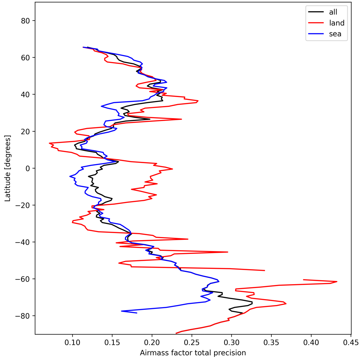
Figure 25: Zonal average of “Airmass factor total precision” for 2025-01-23 to 2025-01-24.
