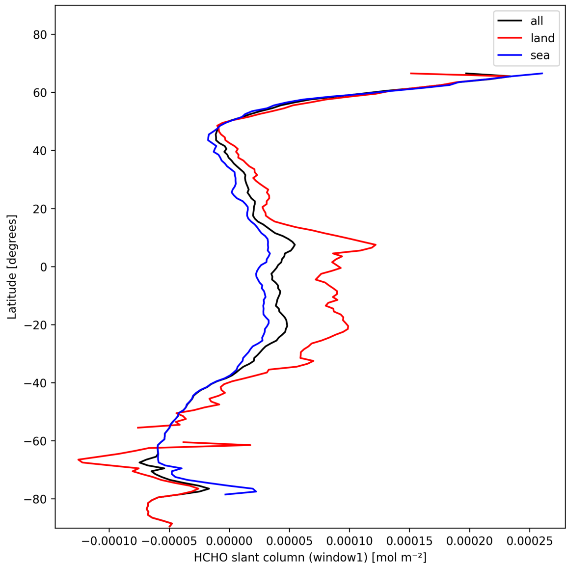
Figure 22: Zonal average of “HCHO slant column (window1)” for 2025-01-24 to 2025-01-25.
