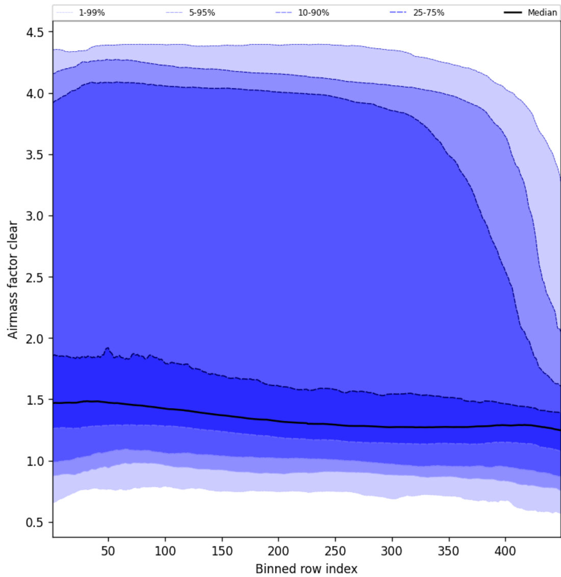
Figure 54: Along track statistics of “Airmass factor clear” for 2025-01-24 to 2025-01-25
