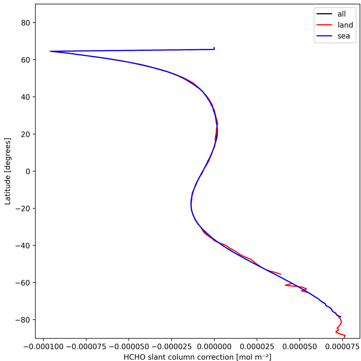
Figure 31: Zonal average of “HCHO slant column correction” for 2025-01-24 to 2025-01-25.
