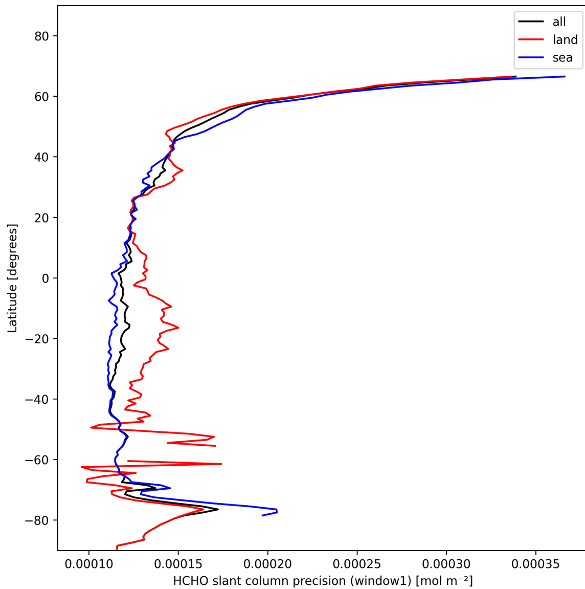
Figure 23: Zonal average of “HCHO slant column precision (window1)” for 2025-01-24 to 2025-01-25.
