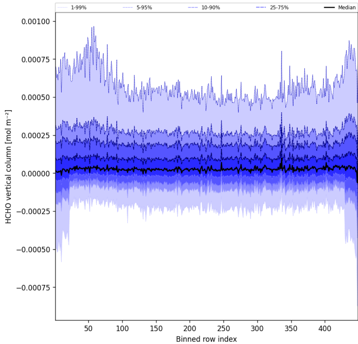
Figure 47: Along track statistics of “HCHO vertical column” for 2025-01-24 to 2025-01-25
