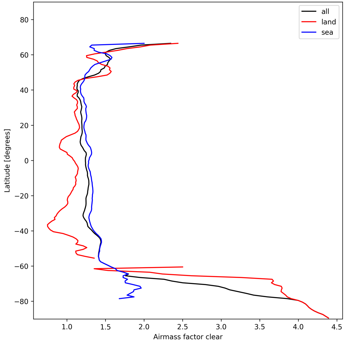
Figure 26: Zonal average of “Airmass factor clear” for 2025-01-24 to 2025-01-25.
