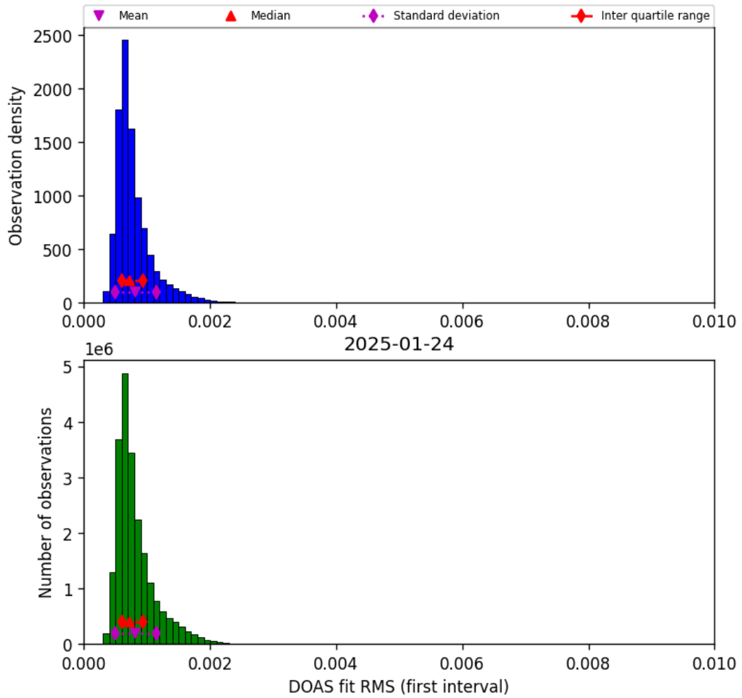
Figure 44: Histogram of “DOAS fit RMS (first interval)” for 2025-01-24 to 2025-01-25
