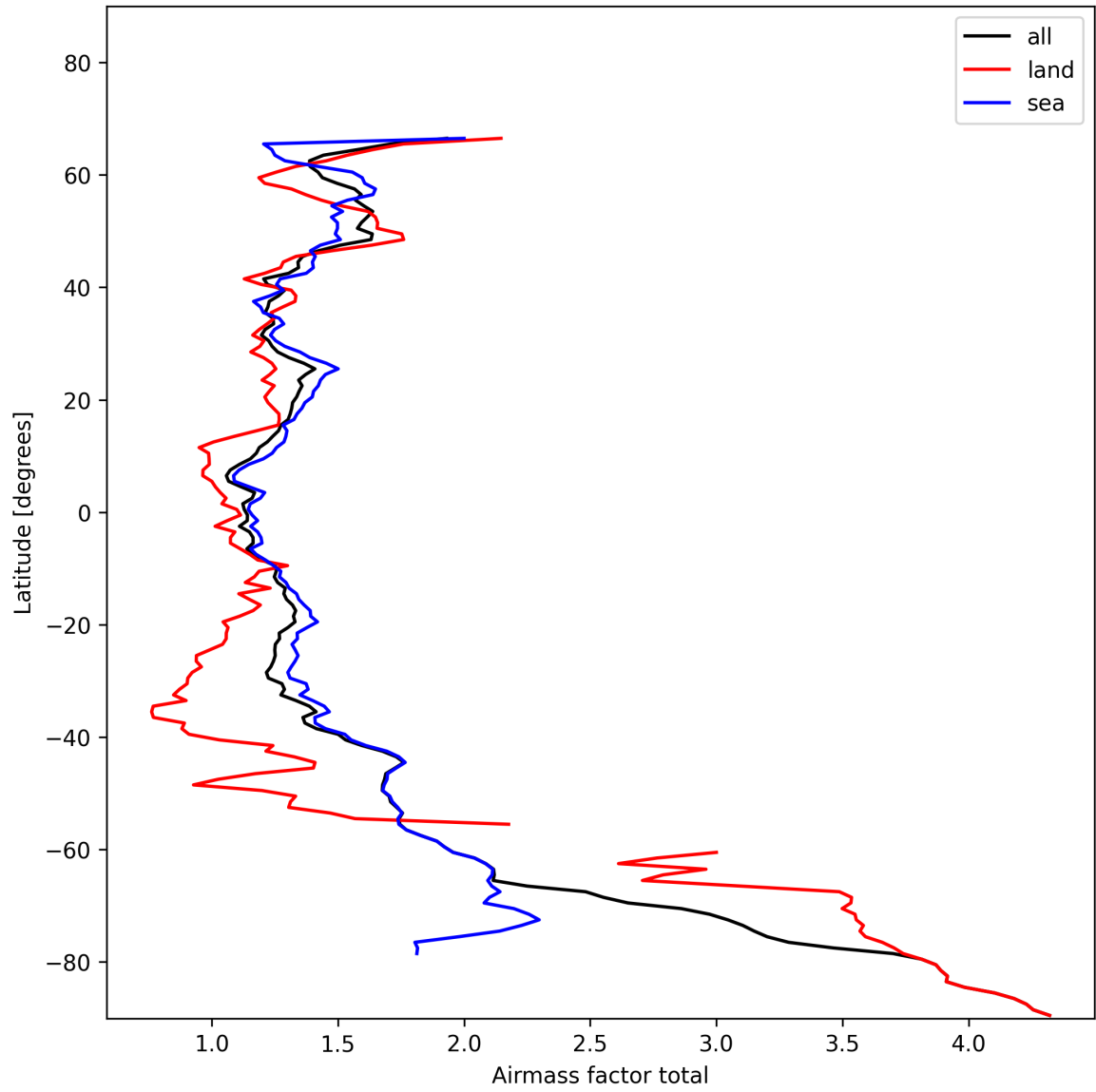
Figure 24: Zonal average of “Airmass factor total” for 2025-01-24 to 2025-01-25.
