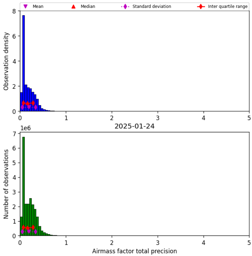
Figure 39: Histogram of “Airmass factor total precision” for 2025-01-24 to 2025-01-25
