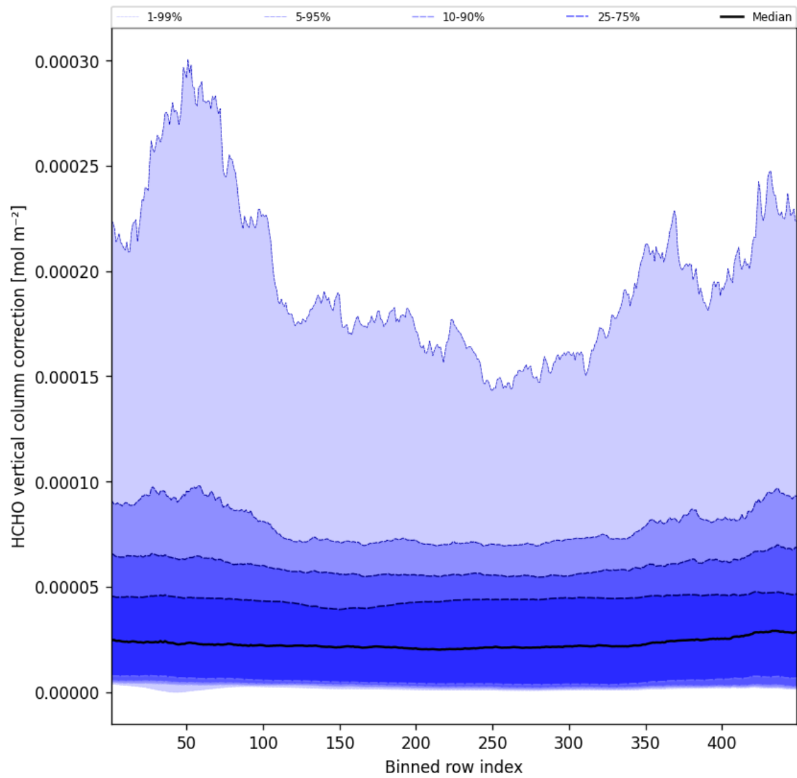
Figure 49: Along track statistics of “HCHO vertical column correction” for 2025-01-24 to 2025-01-25
