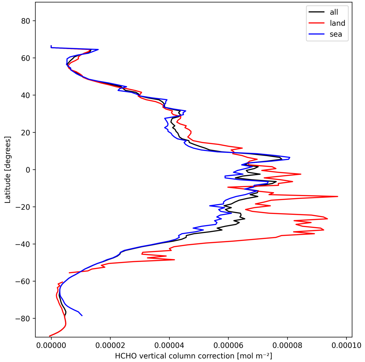
Figure 21: Zonal average of “HCHO vertical column correction” for 2025-01-24 to 2025-01-25.
