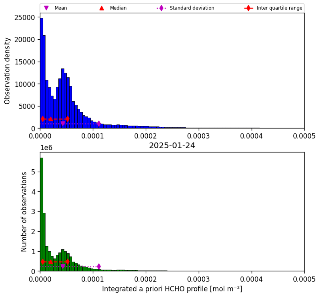
Figure 41: Histogram of “Integrated a priori HCHO profile” for 2025-01-24 to 2025-01-25
