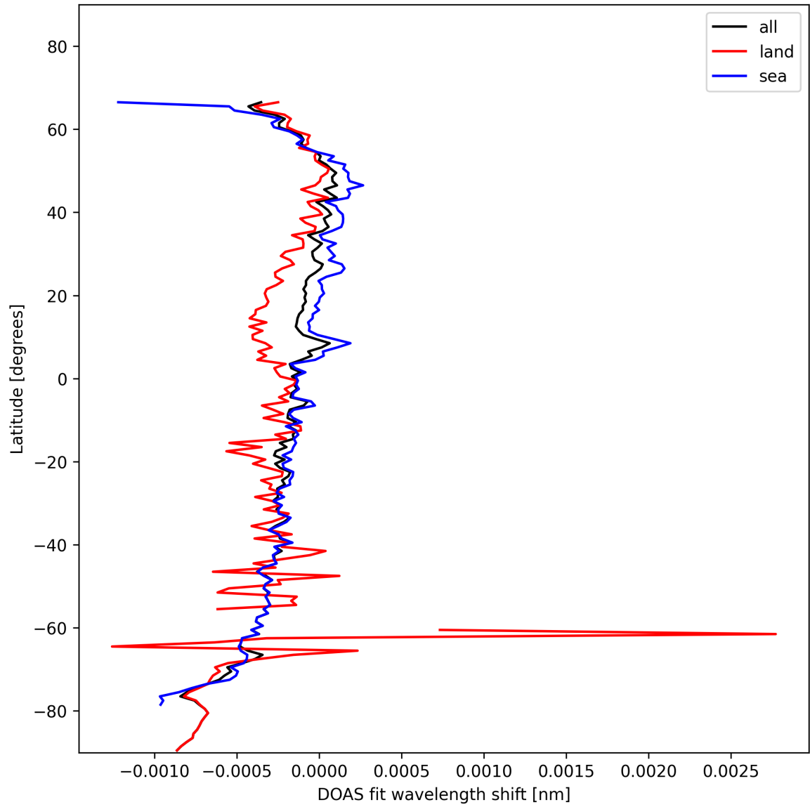
Figure 28: Zonal average of “DOAS fit wavelength shift” for 2025-01-24 to 2025-01-25.
