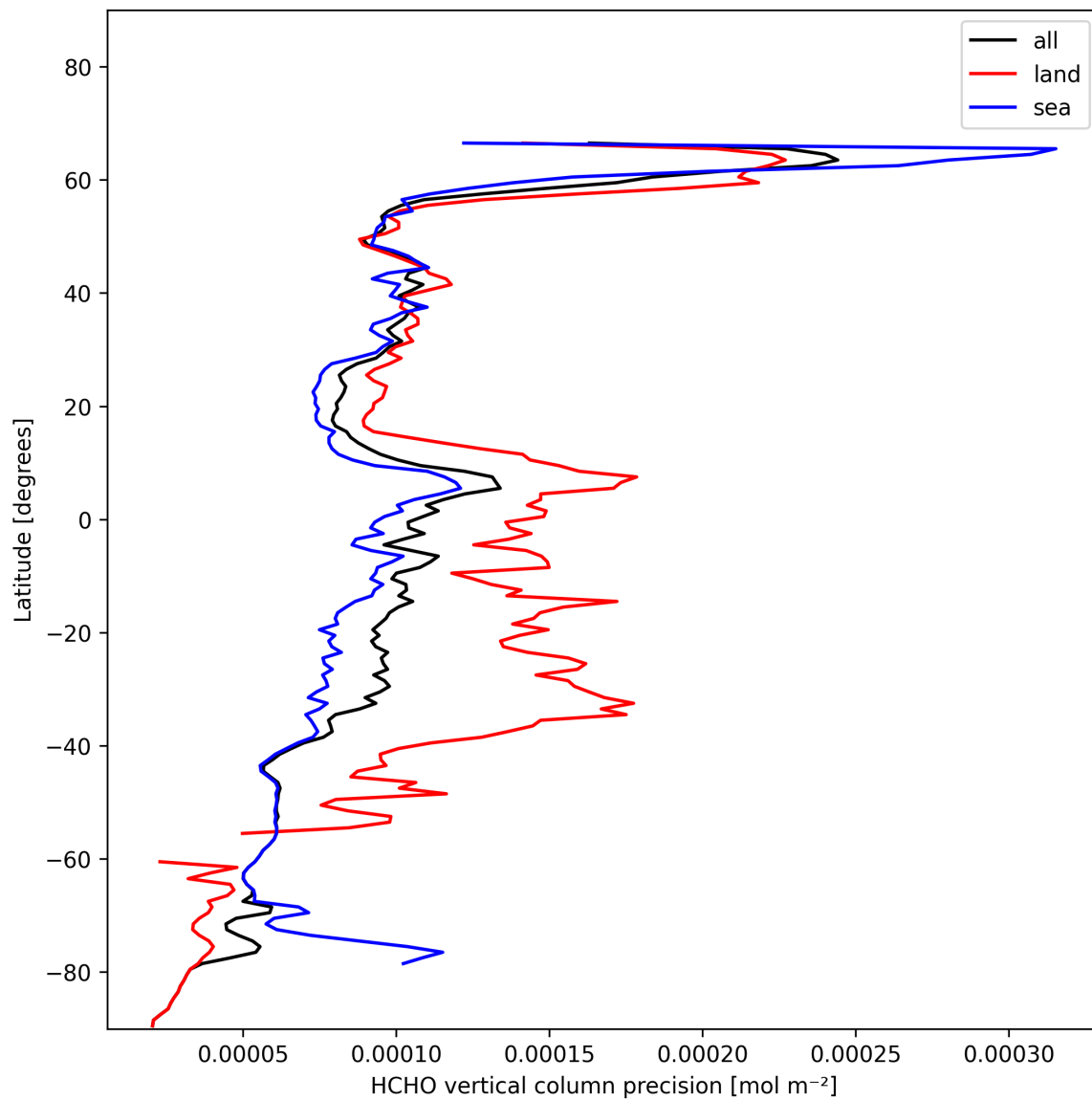
Figure 20: Zonal average of “HCHO vertical column precision” for 2025-01-24 to 2025-01-25.
