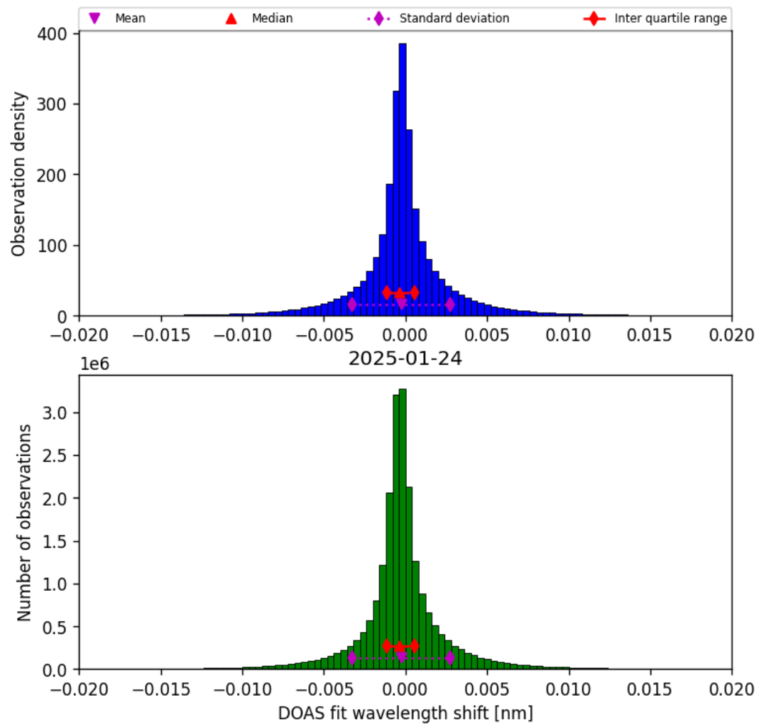
Figure 42: Histogram of “DOAS fit wavelength shift” for 2025-01-24 to 2025-01-25
