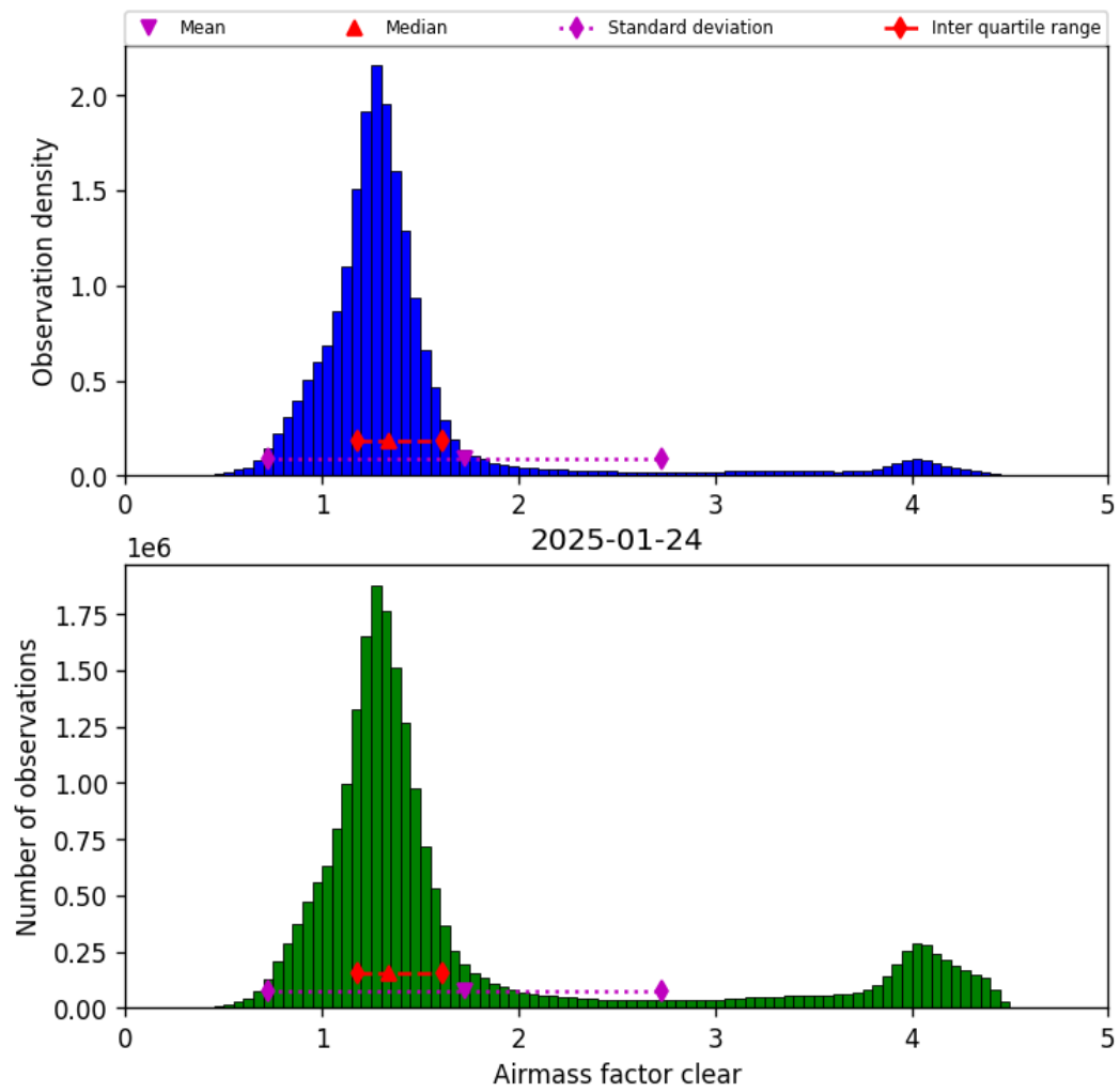
Figure 40: Histogram of “Airmass factor clear” for 2025-01-24 to 2025-01-25
