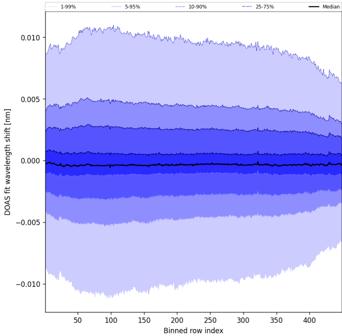
Figure 56: Along track statistics of “DOAS fit wavelength shift” for 2025-01-24 to 2025-01-25
