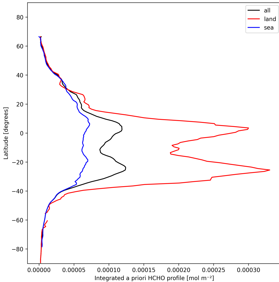
Figure 27: Zonal average of “Integrated a priori HCHO profile” for 2025-01-24 to 2025-01-25.
