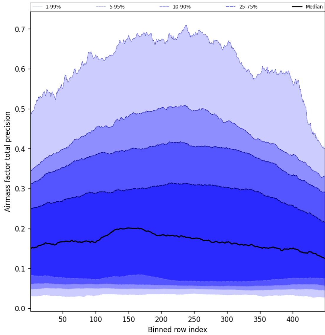
Figure 53: Along track statistics of “Airmass factor total precision” for 2025-01-24 to 2025-01-25
