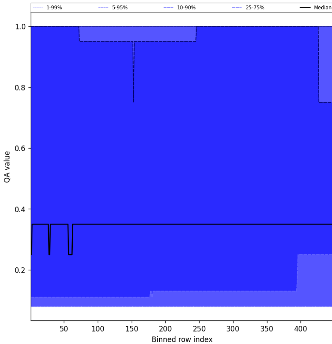
Figure 46: Along track statistics of “QA value” for 2025-01-24 to 2025-01-25
