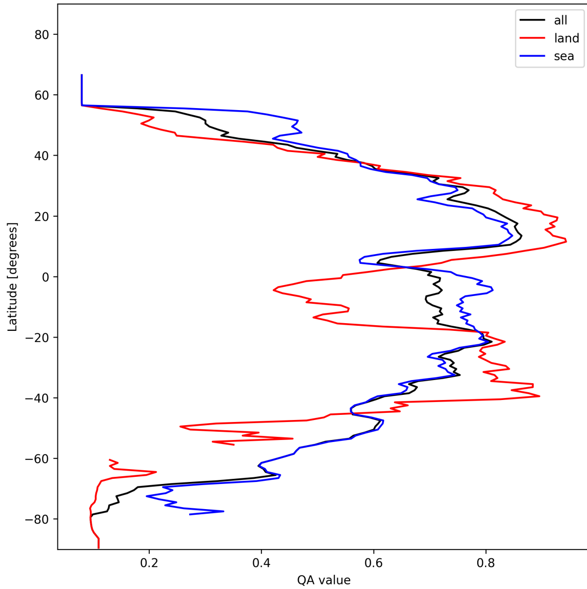
Figure 18: Zonal average of “QA value” for 2025-01-24 to 2025-01-25.
