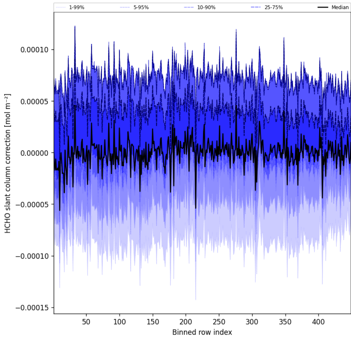
Figure 59: Along track statistics of “HCHO slant column correction” for 2025-01-24 to 2025-01-25
