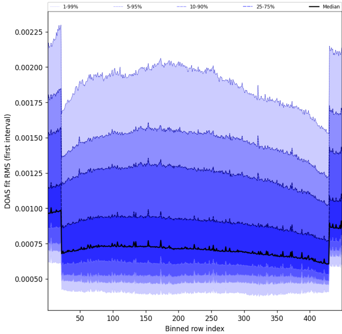
Figure 58: Along track statistics of “DOAS fit RMS (first interval)” for 2025-01-24 to 2025-01-25
