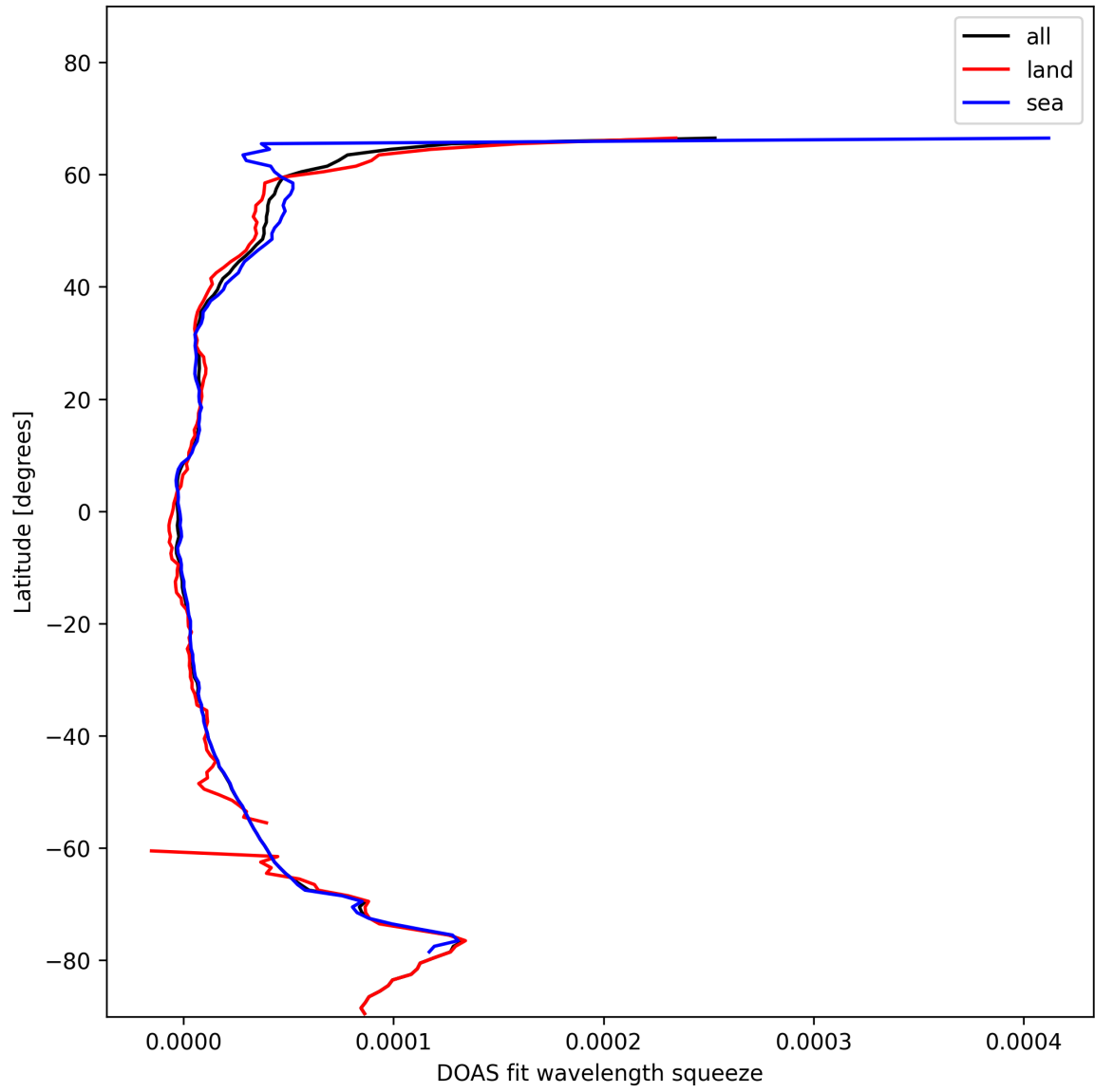
Figure 29: Zonal average of “DOAS fit wavelength squeeze” for 2025-01-24 to 2025-01-25.
