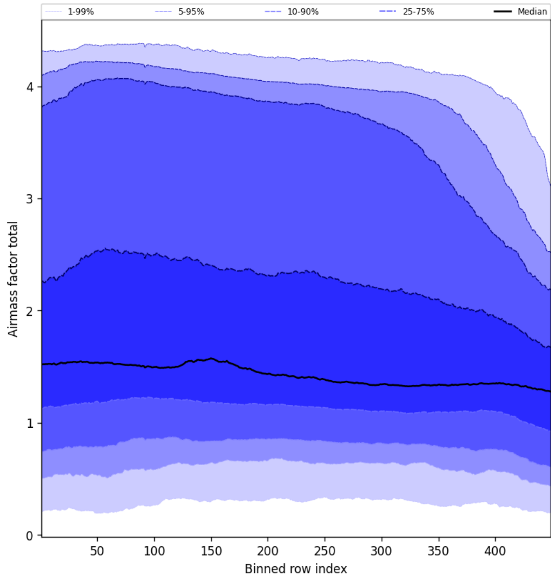
Figure 52: Along track statistics of “Airmass factor total” for 2025-01-24 to 2025-01-25
