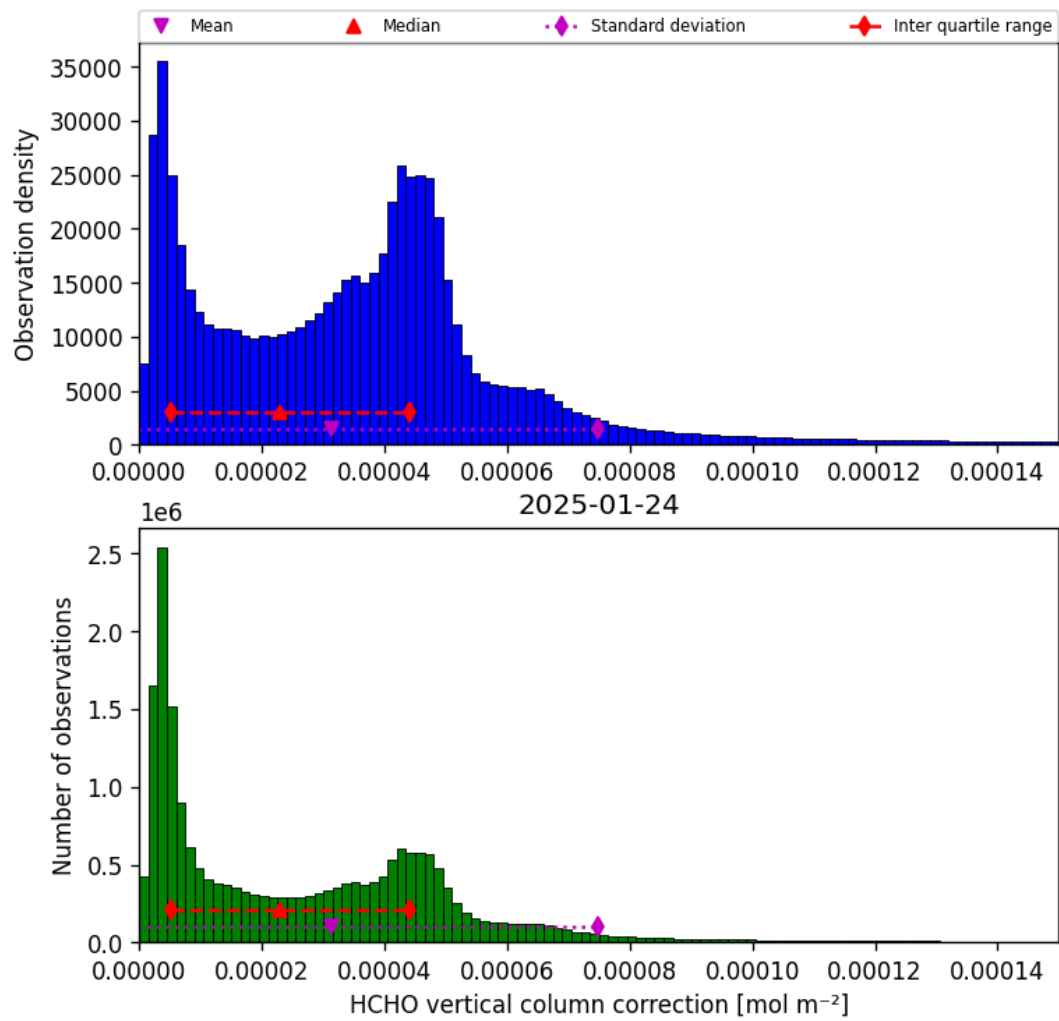
Figure 35: Histogram of “HCHO vertical column correction” for 2025-01-24 to 2025-01-25
