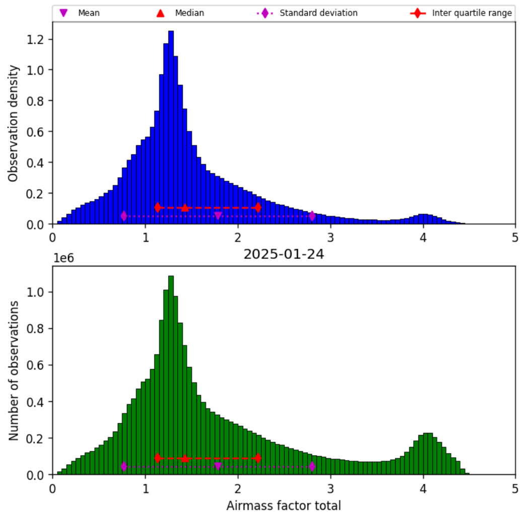
Figure 38: Histogram of “Airmass factor total” for 2025-01-24 to 2025-01-25
