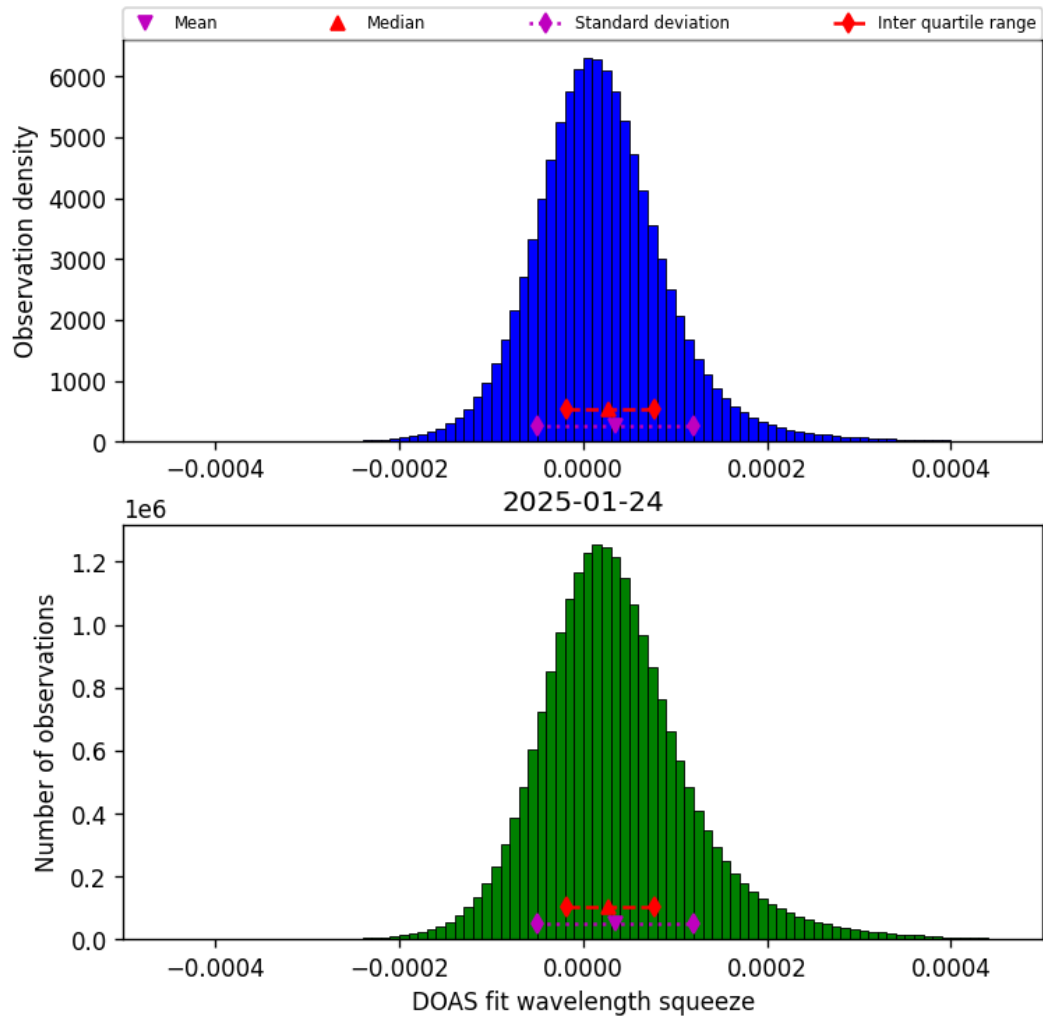
Figure 43: Histogram of “DOAS fit wavelength squeeze” for 2025-01-24 to 2025-01-25
