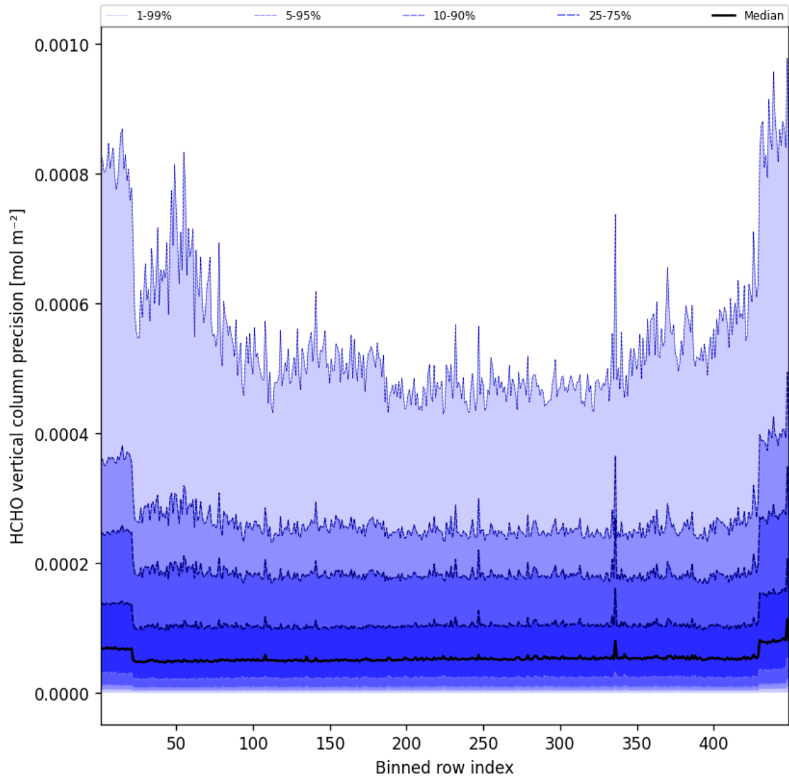
Figure 48: Along track statistics of “HCHO vertical column precision” for 2025-01-24 to 2025-01-25
