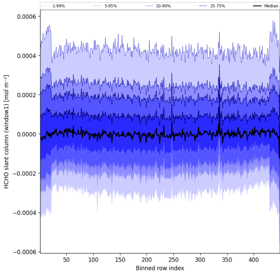
Figure 50: Along track statistics of “HCHO slant column (window1)” for 2025-01-24 to 2025-01-25
