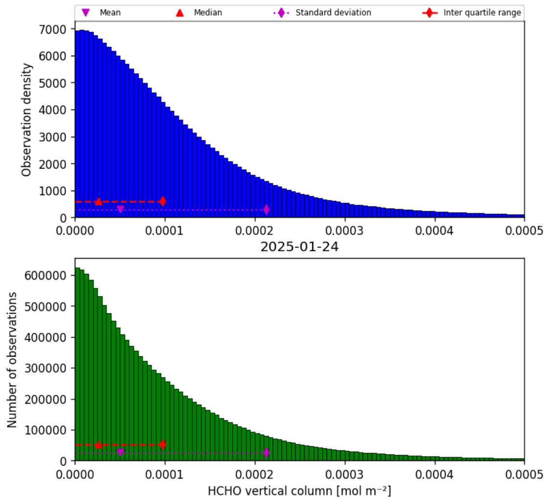
Figure 33: Histogram of “HCHO vertical column” for 2025-01-24 to 2025-01-25
