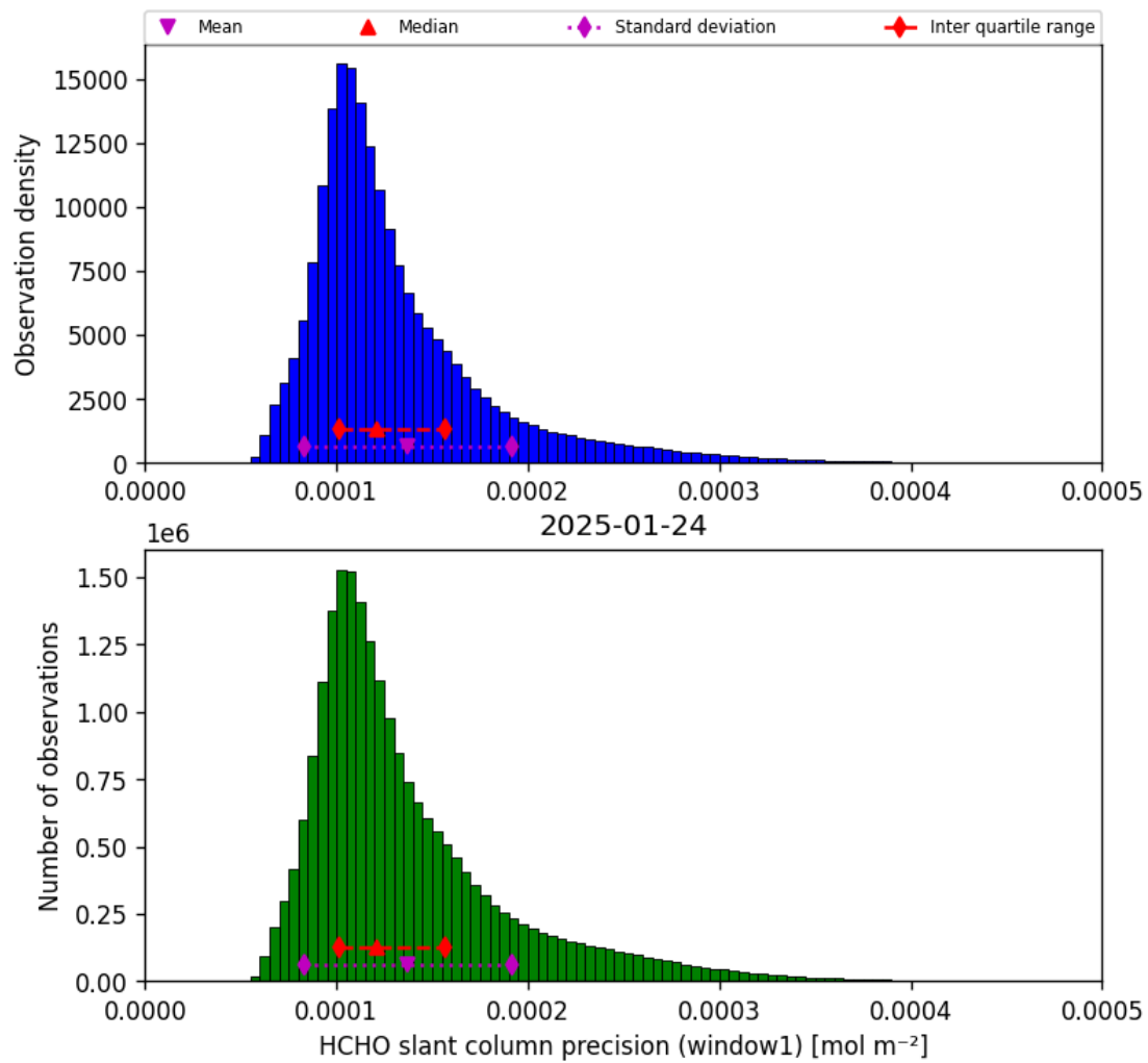
Figure 37: Histogram of “HCHO slant column precision (window1)” for 2025-01-24 to 2025-01-25
