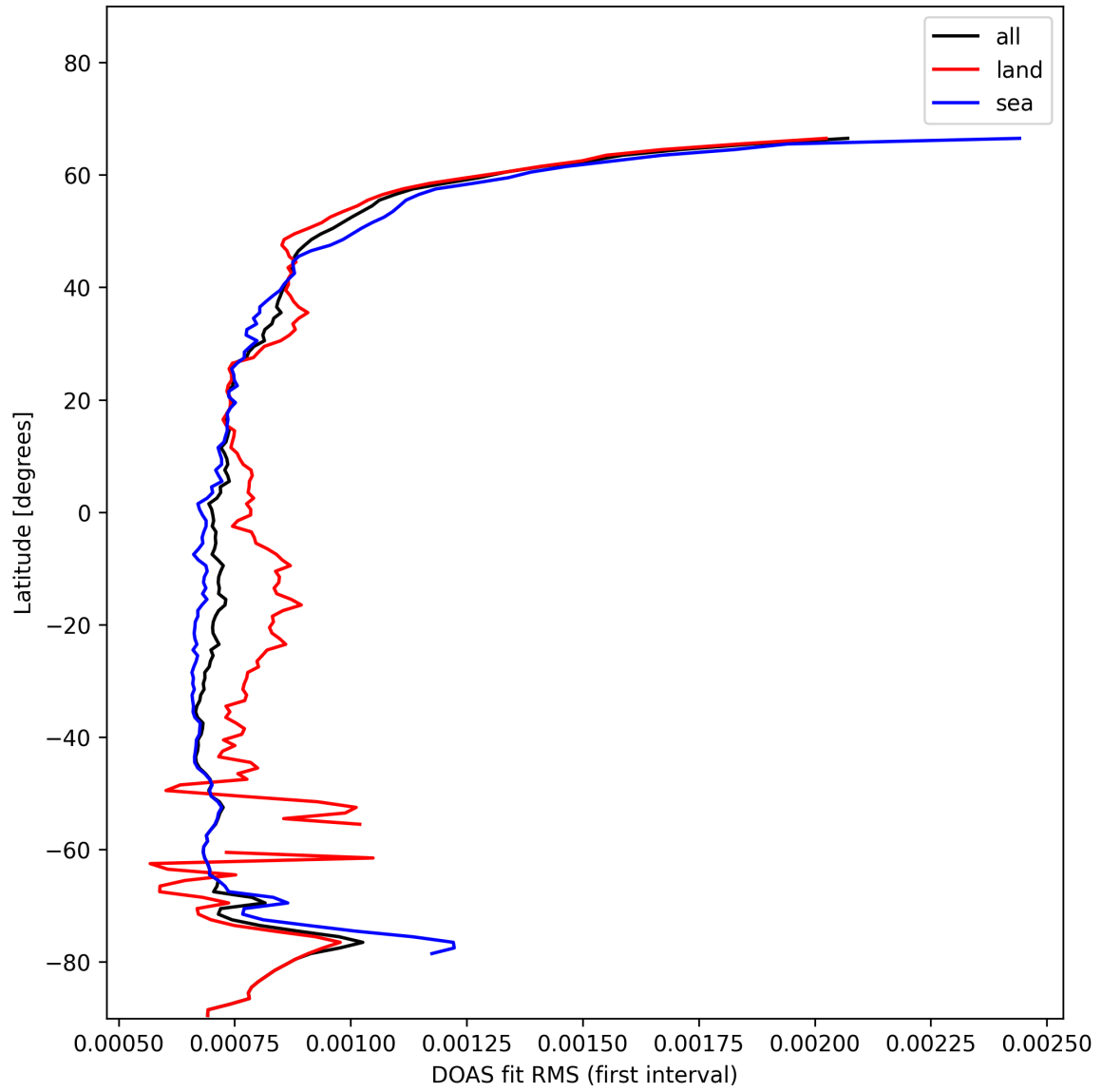
Figure 30: Zonal average of “DOAS fit RMS (first interval)” for 2025-01-24 to 2025-01-25.
