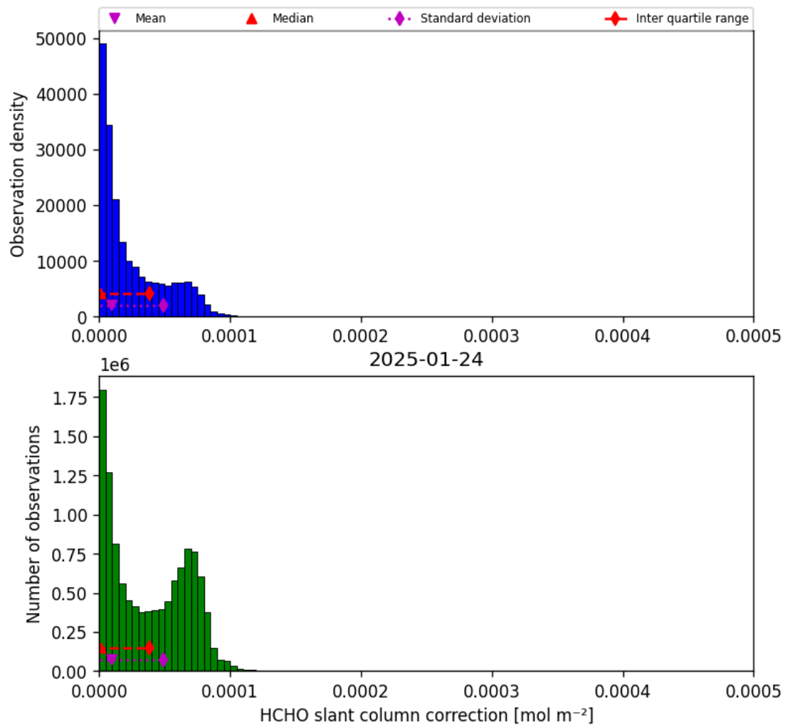
Figure 45: Histogram of “HCHO slant column correction” for 2025-01-24 to 2025-01-25
