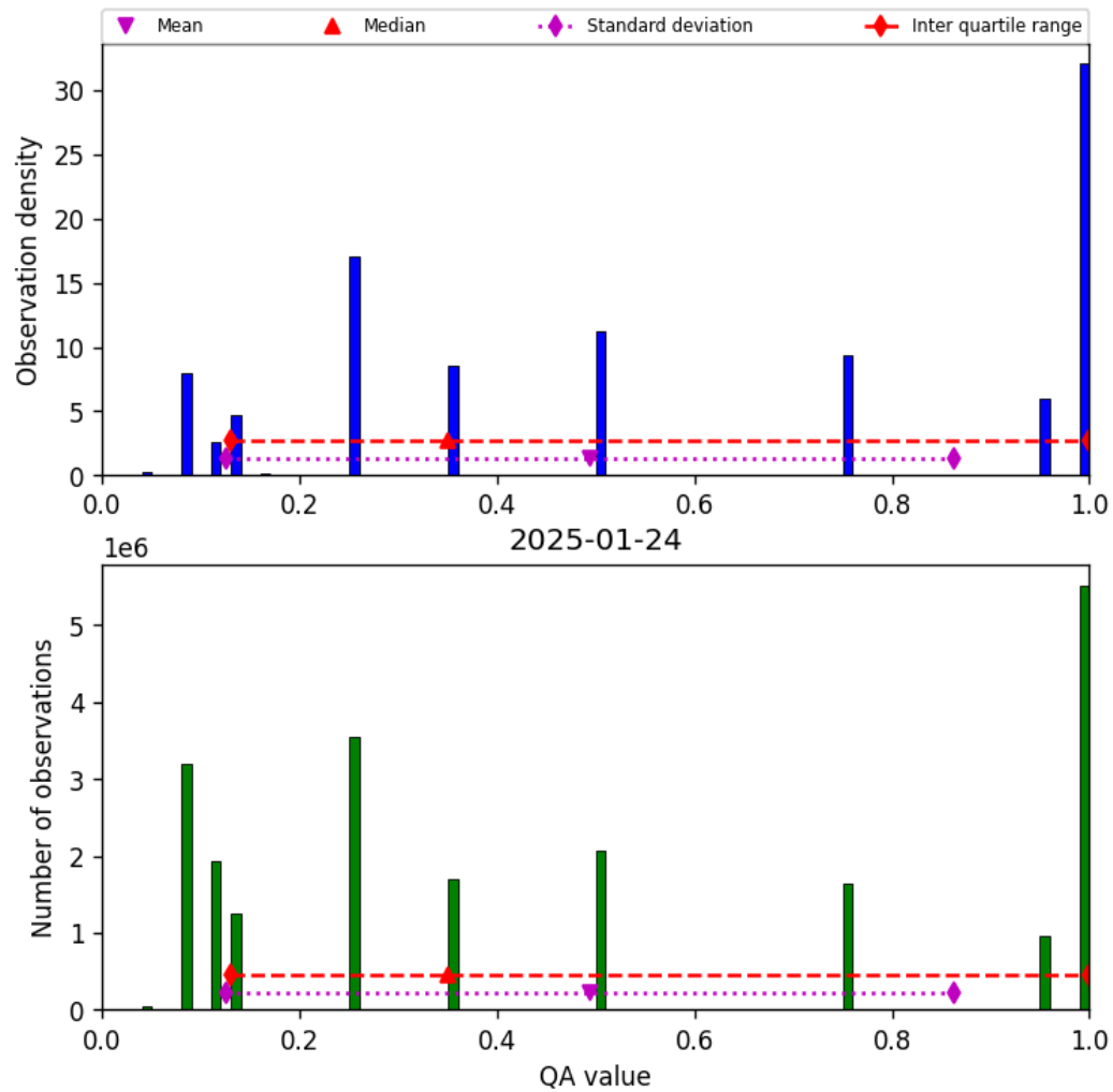
Figure 32: Histogram of “QA value” for 2025-01-24 to 2025-01-25
