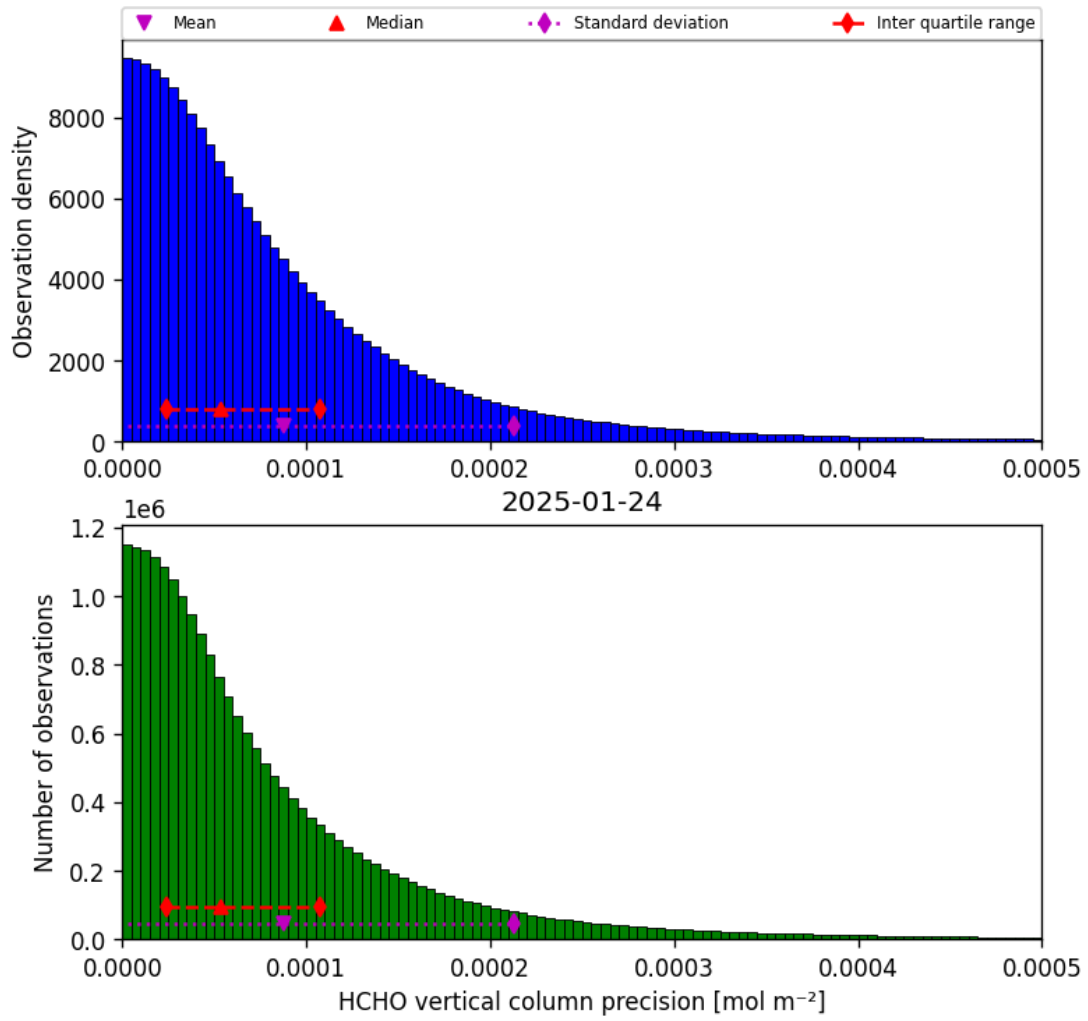
Figure 34: Histogram of “HCHO vertical column precision” for 2025-01-24 to 2025-01-25
