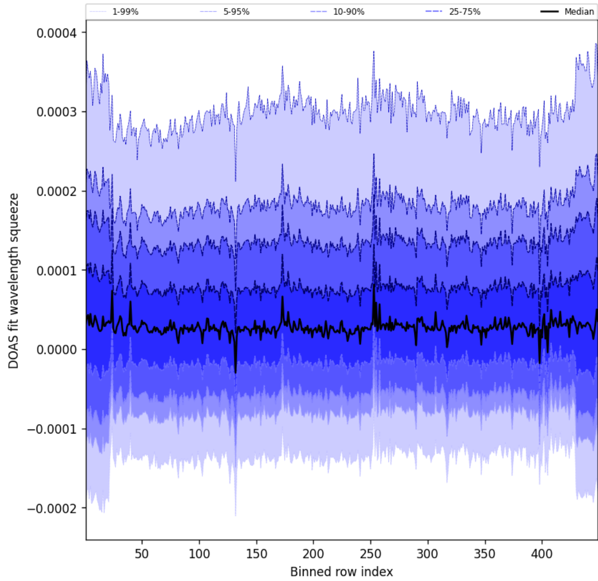
Figure 57: Along track statistics of “DOAS fit wavelength squeeze” for 2025-01-24 to 2025-01-25
