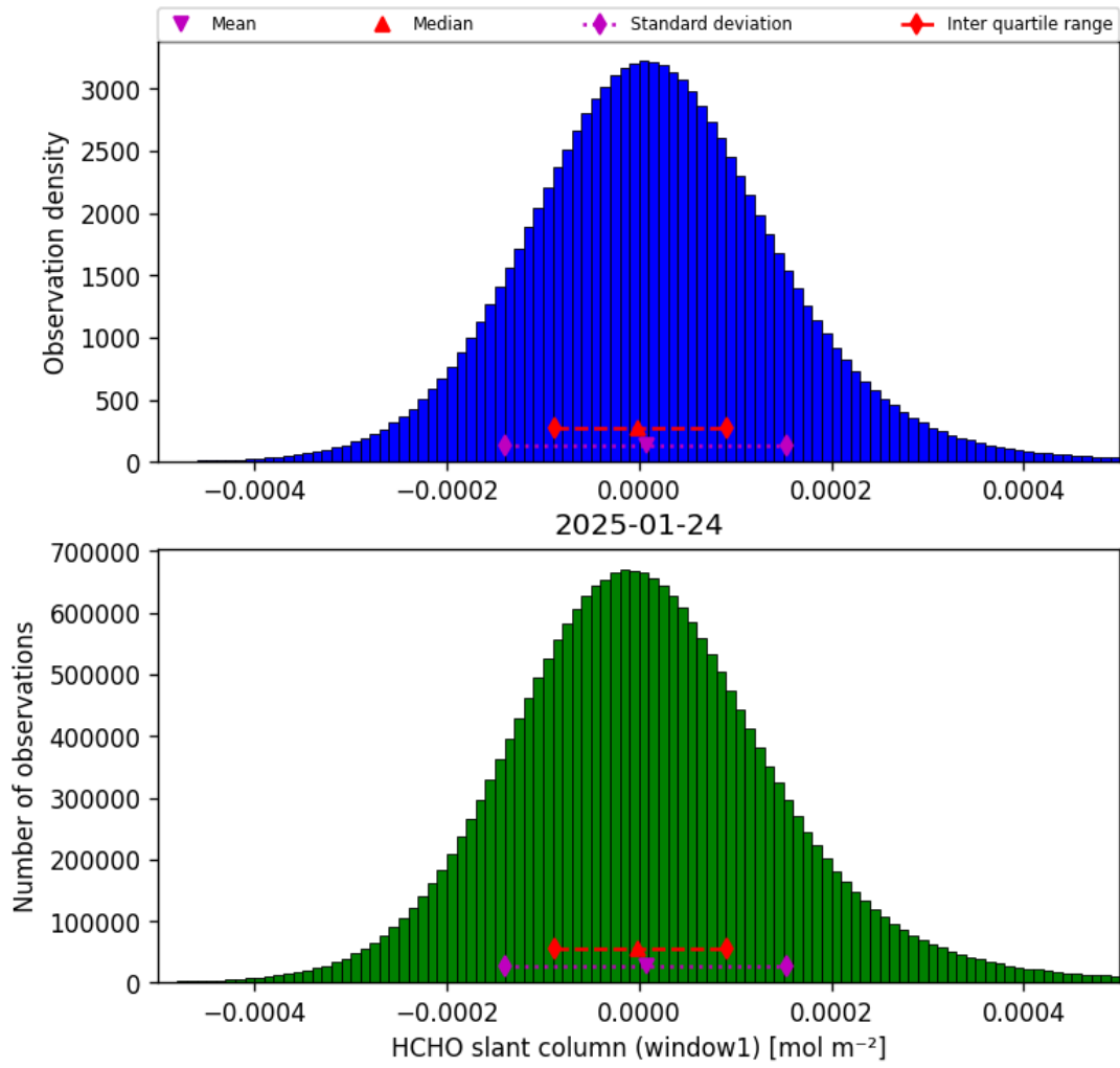
Figure 36: Histogram of “HCHO slant column (window1)” for 2025-01-24 to 2025-01-25
