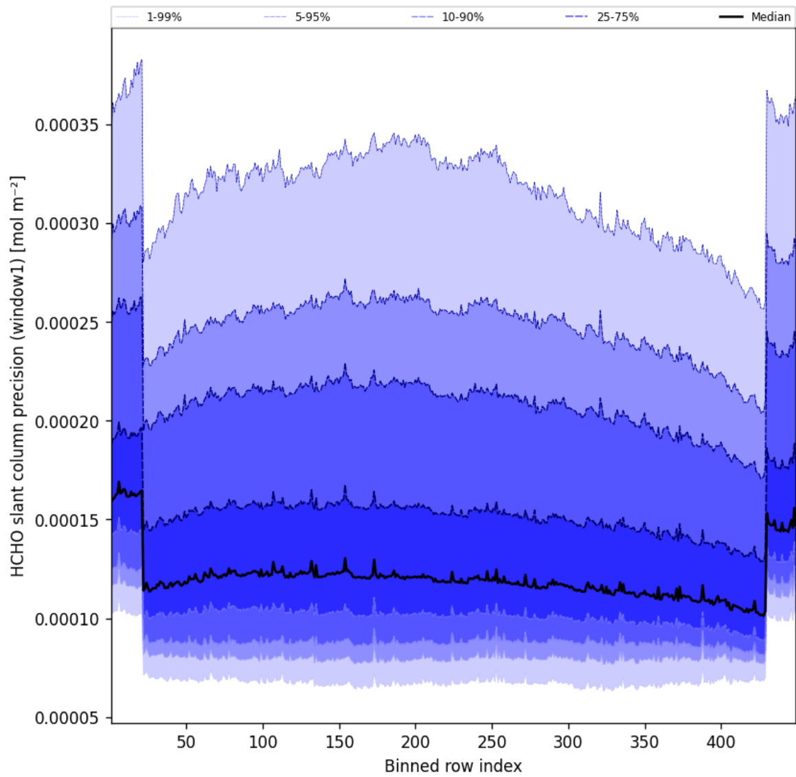
Figure 51: Along track statistics of “HCHO slant column precision (window1)” for 2025-01-24 to 2025-01-25
