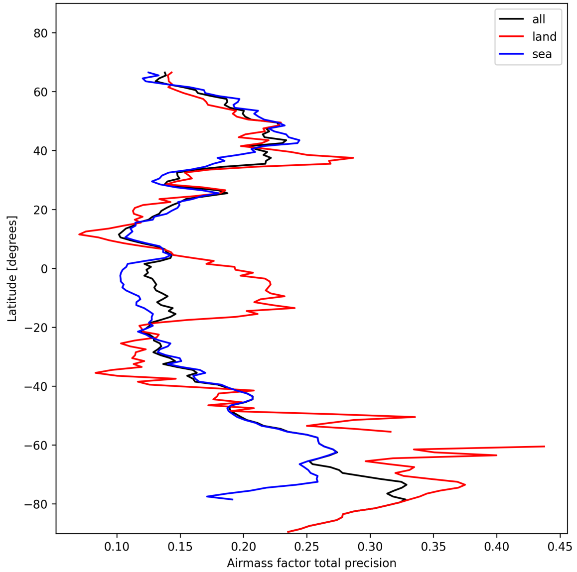
Figure 25: Zonal average of “Airmass factor total precision” for 2025-01-24 to 2025-01-25.
