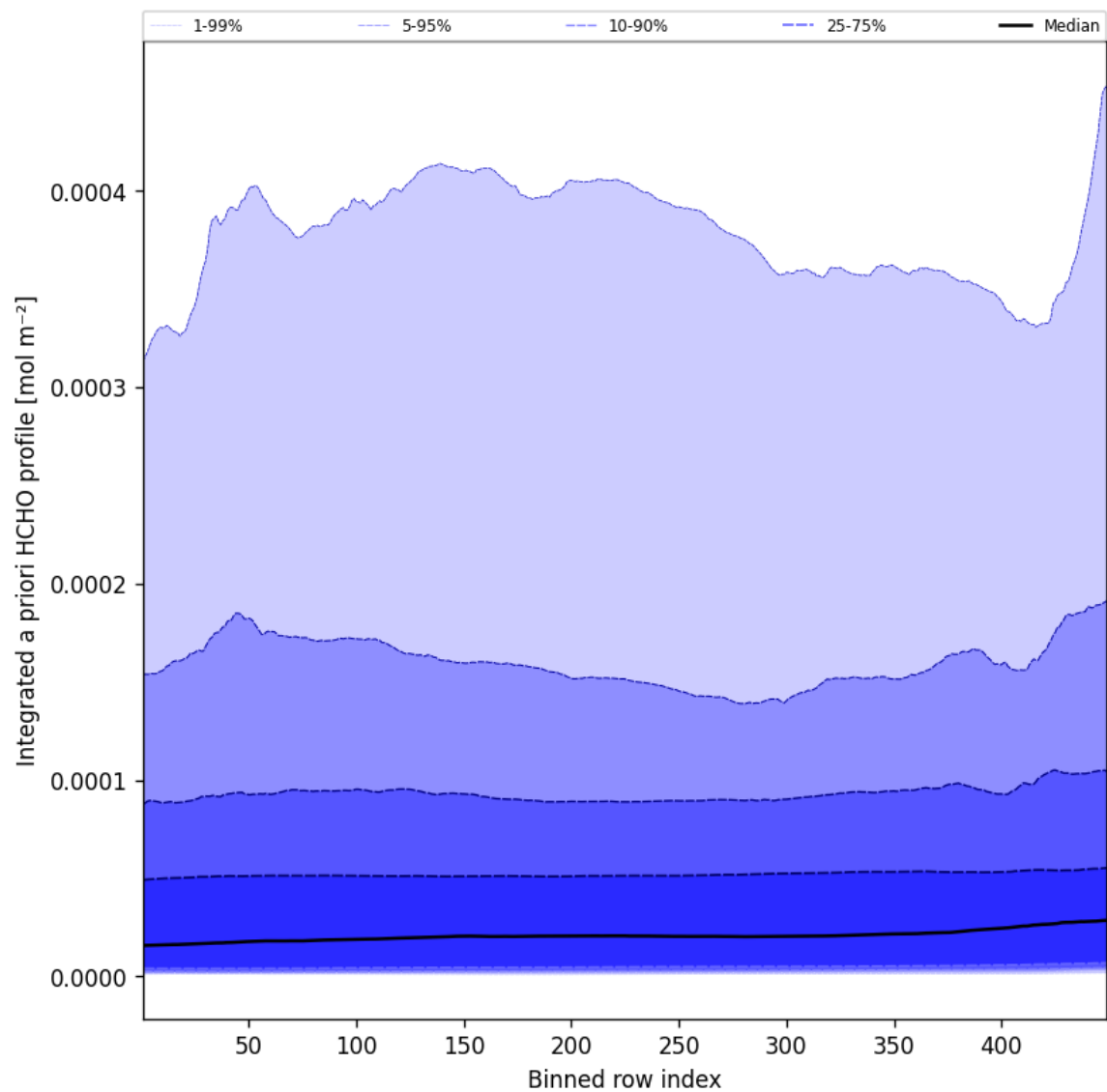
Figure 55: Along track statistics of “Integrated a priori HCHO profile” for 2025-01-24 to 2025-01-25
