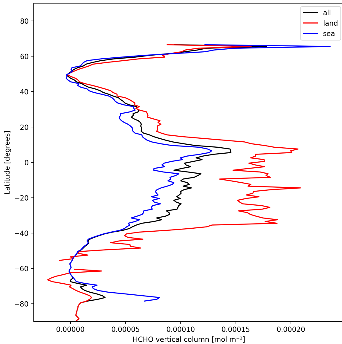
Figure 19: Zonal average of “HCHO vertical column” for 2025-01-24 to 2025-01-25.
