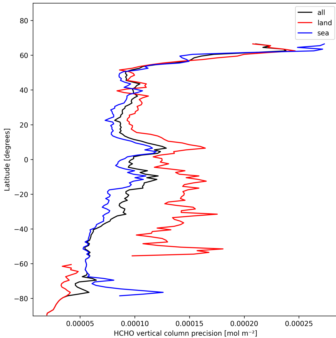
Figure 20: Zonal average of “HCHO vertical column precision” for 2025-01-26 to 2025-01-26.
