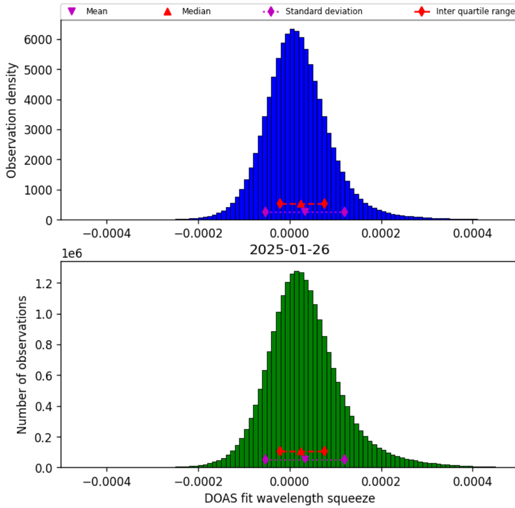
Figure 43: Histogram of “DOAS fit wavelength squeeze” for 2025-01-26 to 2025-01-26
