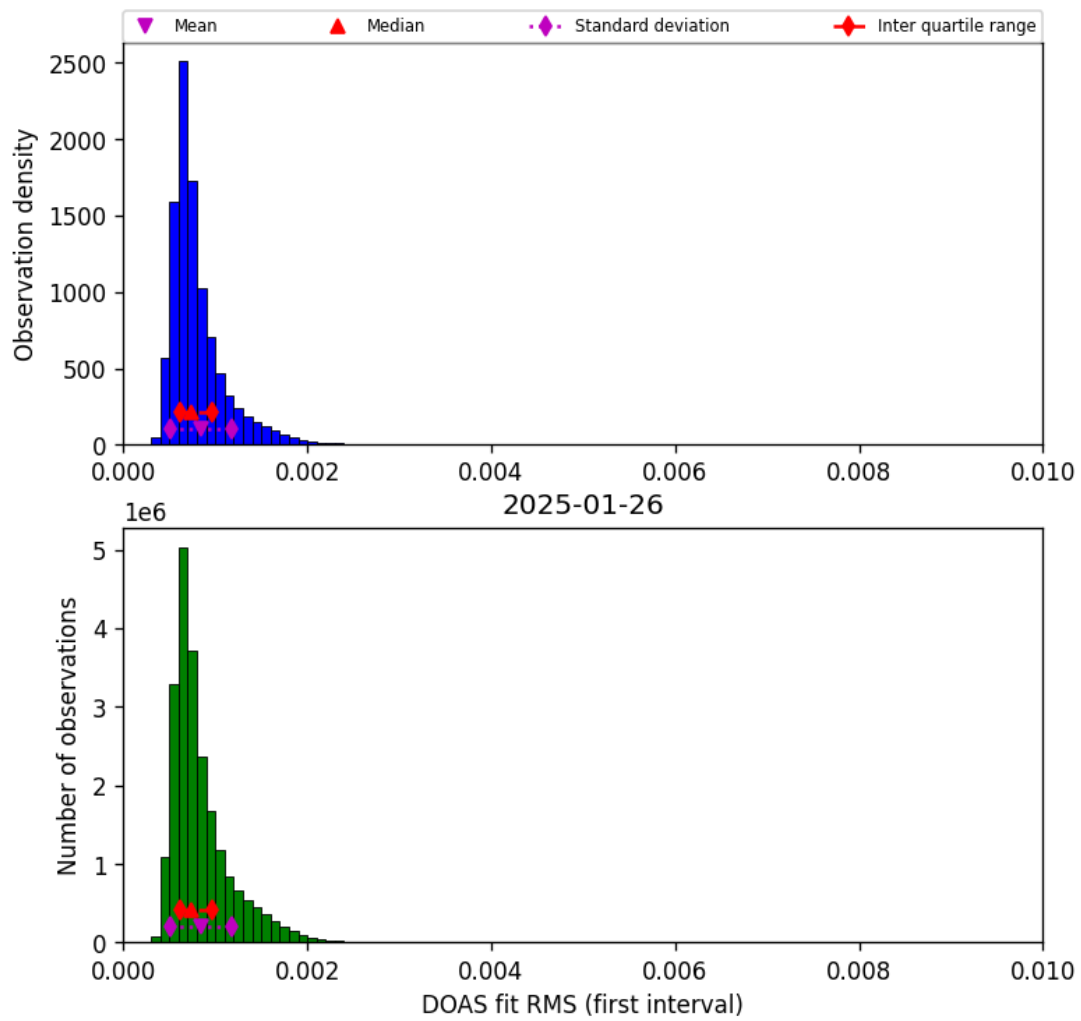
Figure 44: Histogram of “DOAS fit RMS (first interval)” for 2025-01-26 to 2025-01-26
