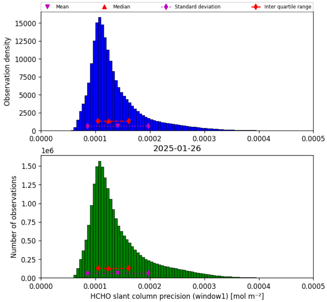
Figure 37: Histogram of “HCHO slant column precision (window1)” for 2025-01-26 to 2025-01-26
