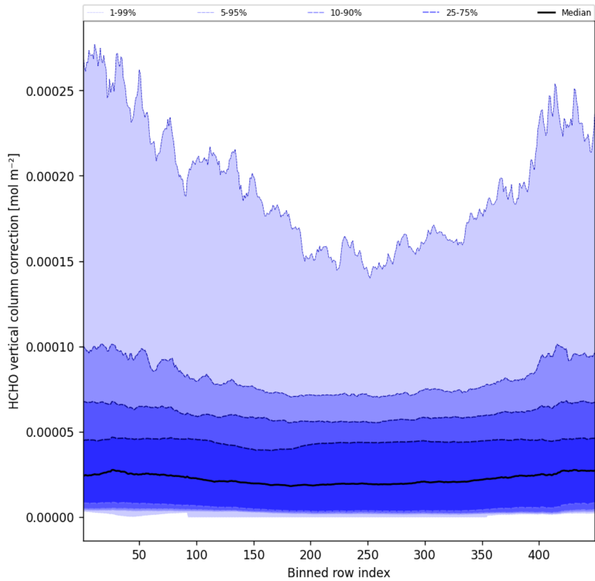
Figure 49: Along track statistics of “HCHO vertical column correction” for 2025-01-26 to 2025-01-26
