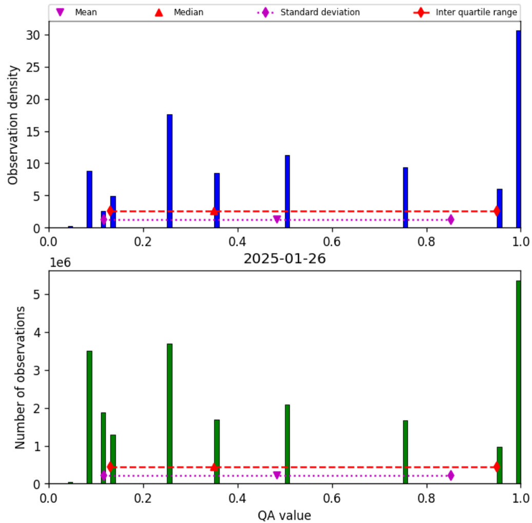
Figure 32: Histogram of “QA value” for 2025-01-26 to 2025-01-26
