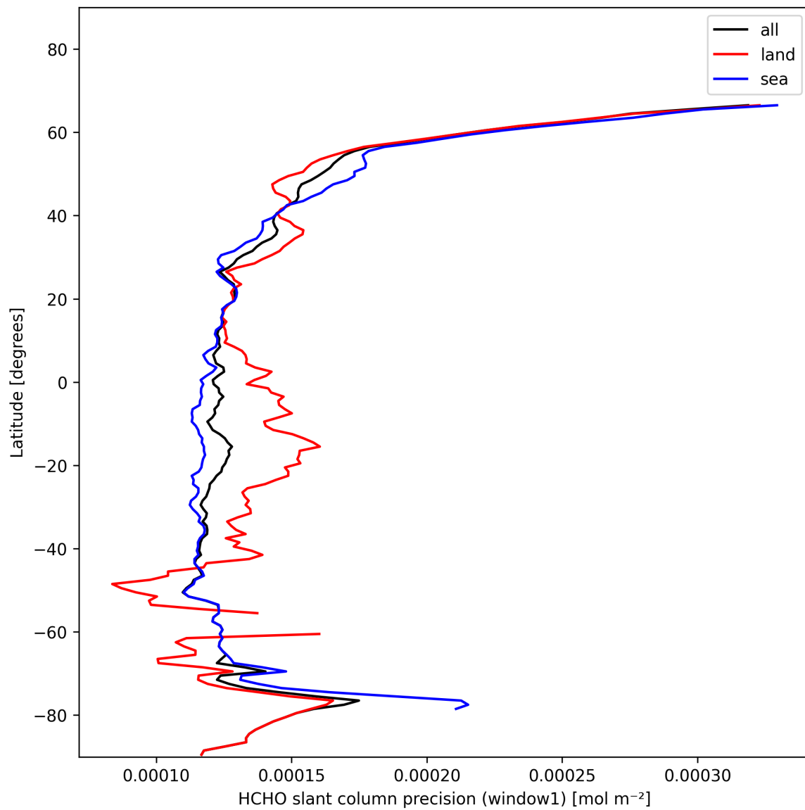
Figure 23: Zonal average of "HCHO slant column precision (window1)" for 2025-01-26 to 2025-01-26.
