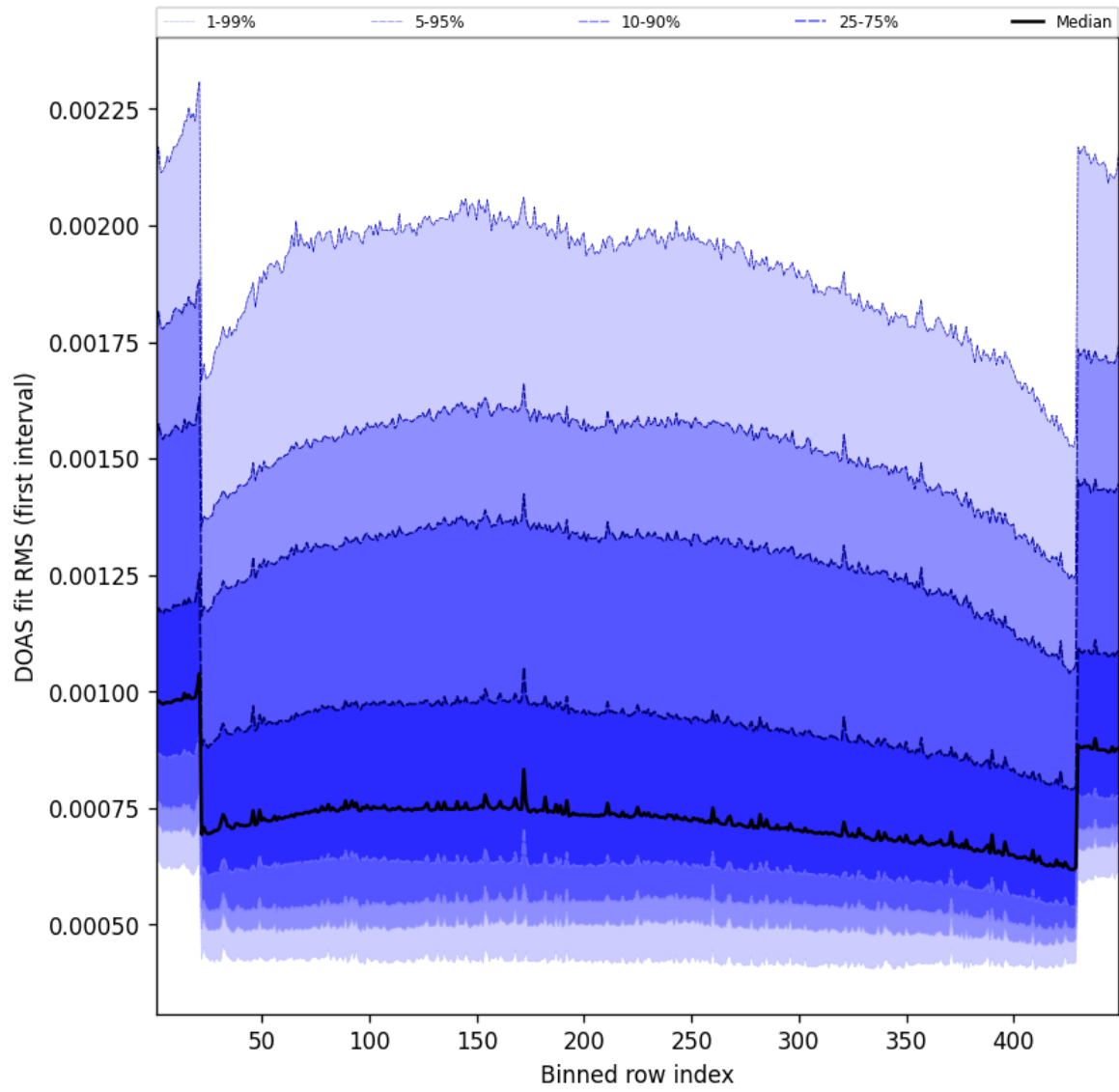
Figure 58: Along track statistics of “DOAS fit RMS (first interval)” for 2025-01-26 to 2025-01-26
