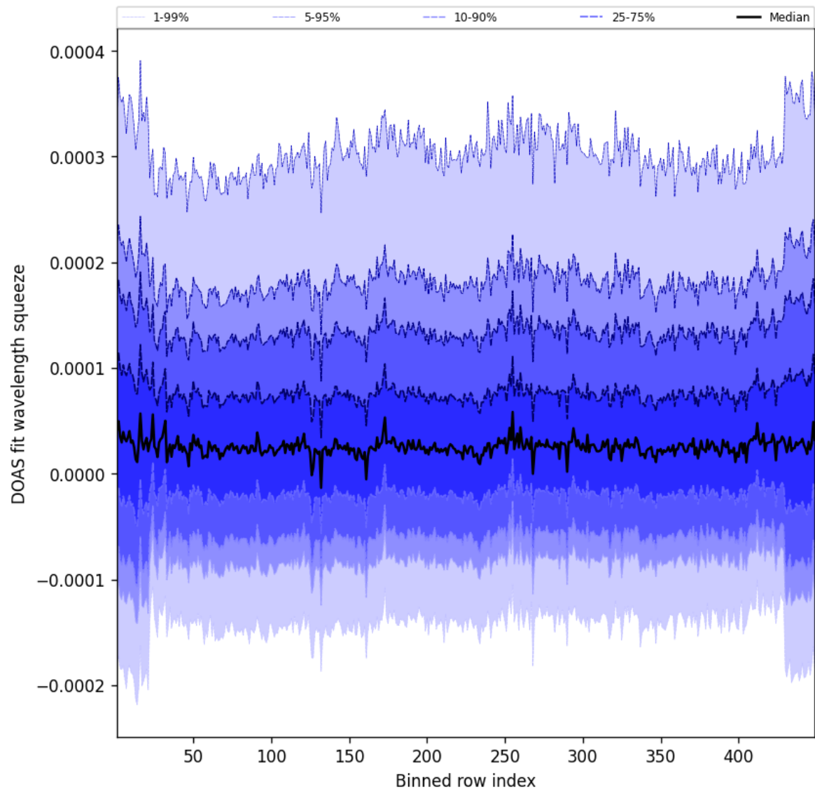
Figure 57: Along track statistics of “DOAS fit wavelength squeeze” for 2025-01-26 to 2025-01-26
