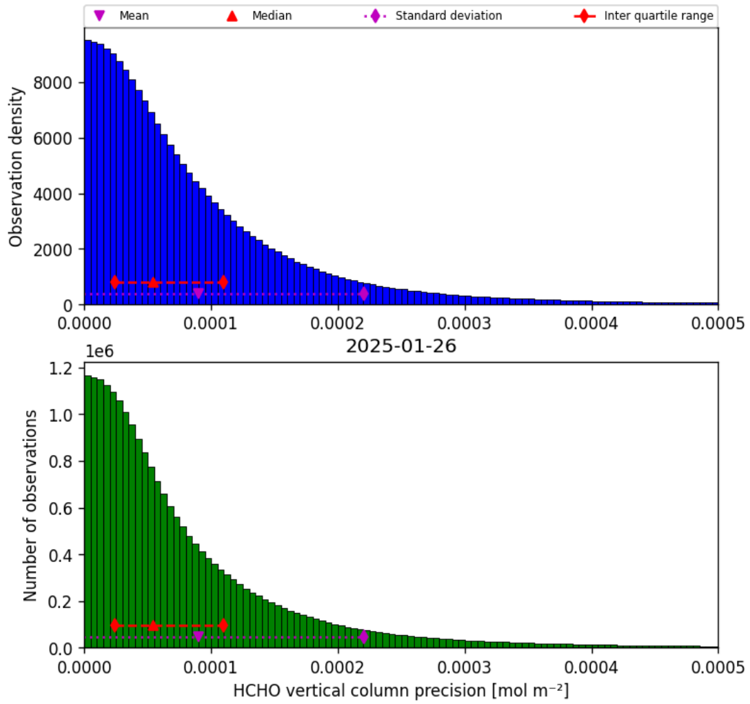
Figure 34: Histogram of “HCHO vertical column precision” for 2025-01-26 to 2025-01-26
