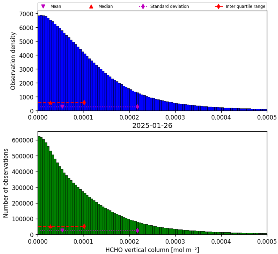
Figure 33: Histogram of “HCHO vertical column” for 2025-01-26 to 2025-01-26
