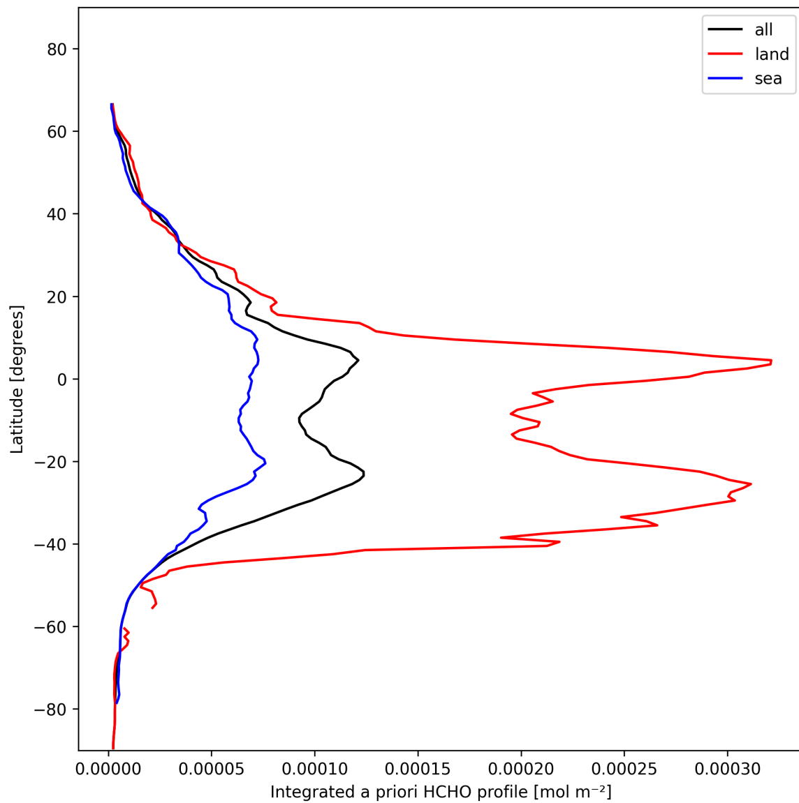
Figure 27: Zonal average of “Integrated a priori HCHO profile” for 2025-01-26 to 2025-01-26.
