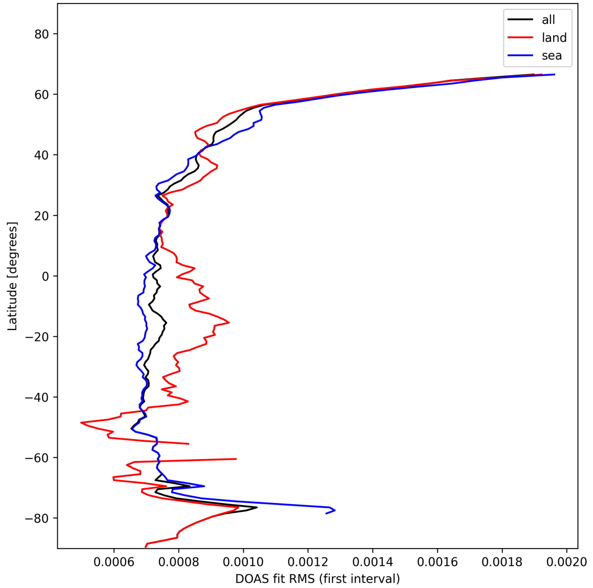
Figure 30: Zonal average of "DOAS fit RMS (first interval)" for 2025-01-26 to 2025-01-26.
