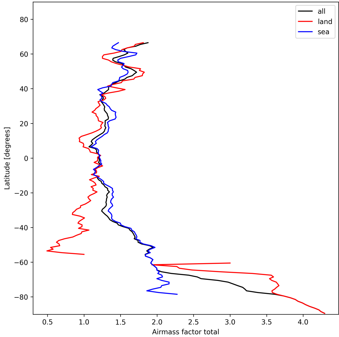
Figure 24: Zonal average of “Airmass factor total” for 2025-01-26 to 2025-01-26.
