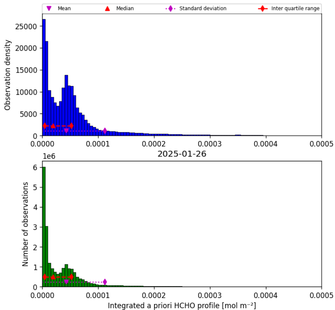
Figure 41: Histogram of “Integrated a priori HCHO profile” for 2025-01-26 to 2025-01-26
