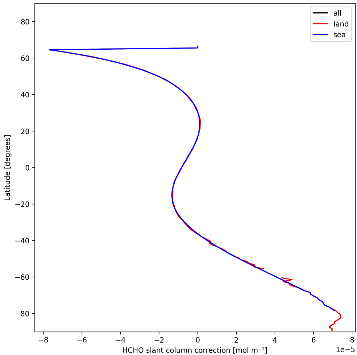
Figure 31: Zonal average of “HCHO slant column correction” for 2025-01-26 to 2025-01-26.
