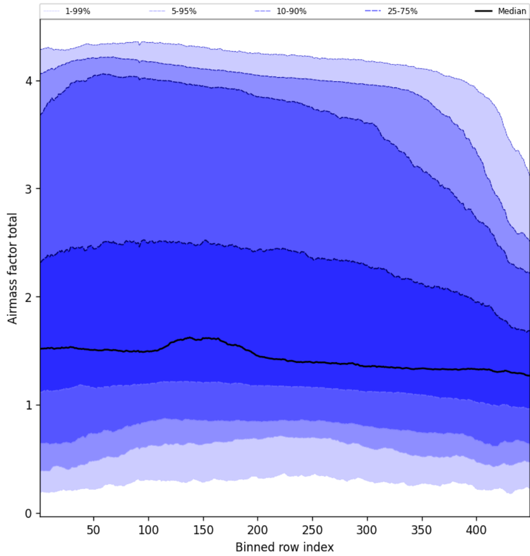
Figure 52: Along track statistics of “Airmass factor total” for 2025-01-26 to 2025-01-26
