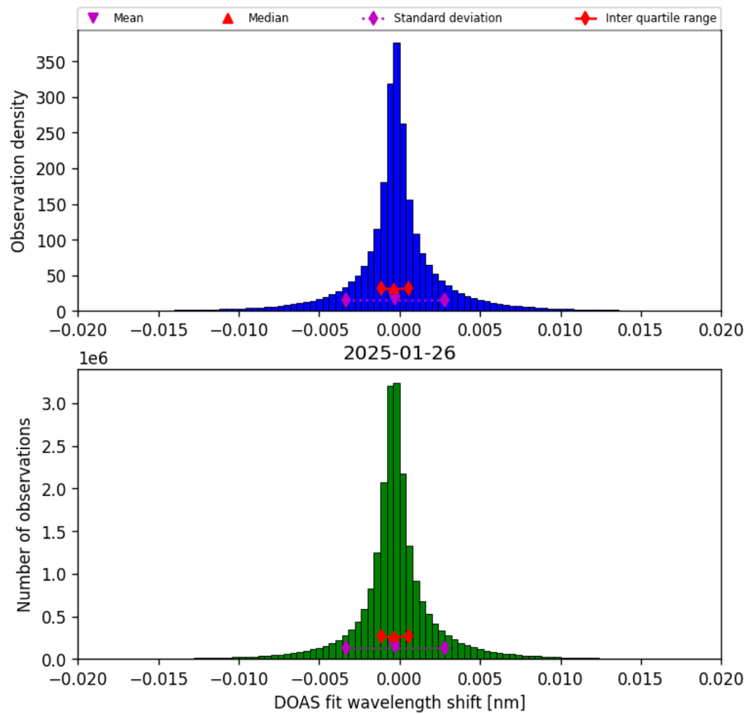
Figure 42: Histogram of “DOAS fit wavelength shift” for 2025-01-26 to 2025-01-26
