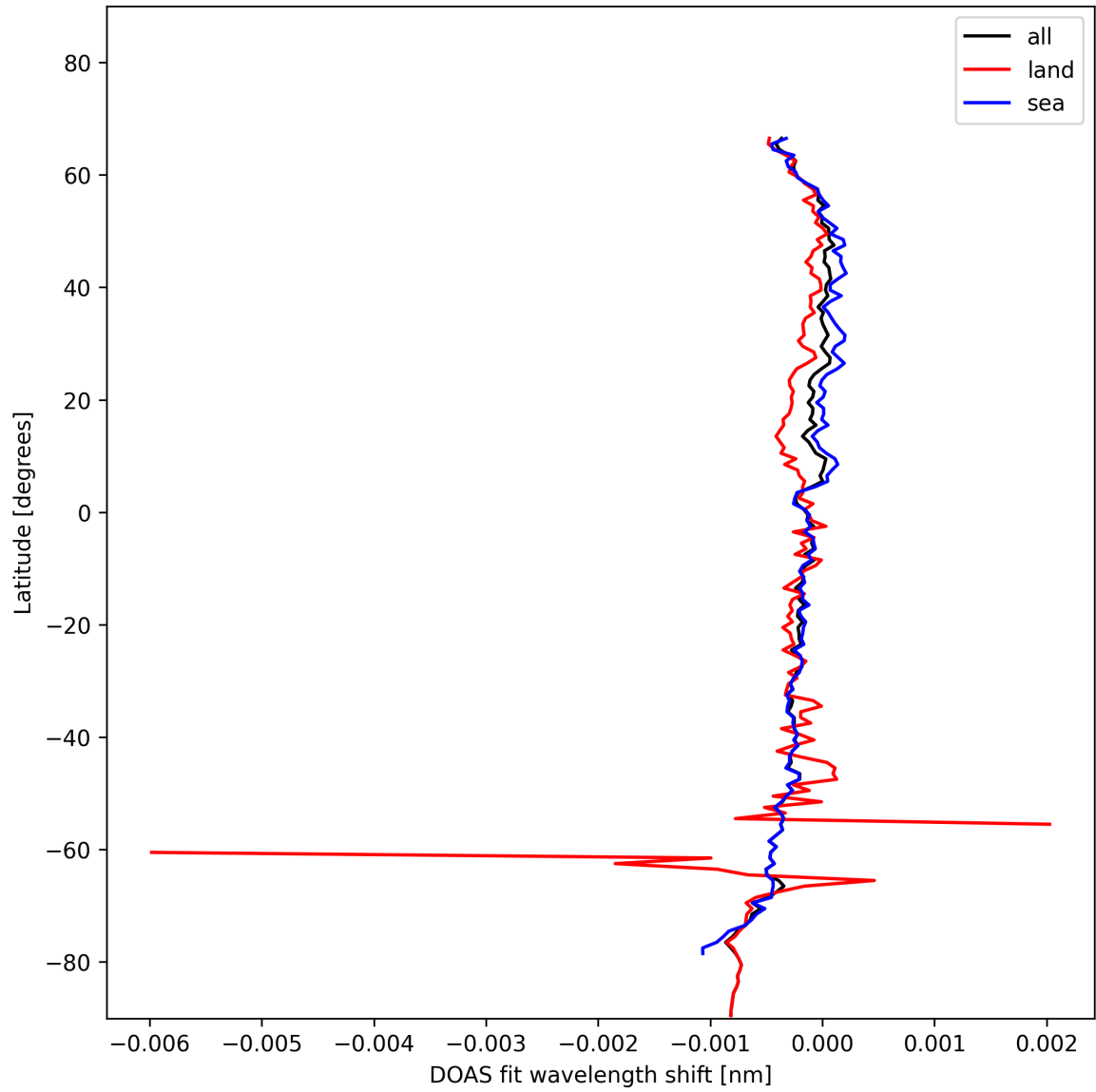
Figure 28: Zonal average of “DOAS fit wavelength shift” for 2025-01-26 to 2025-01-26.
