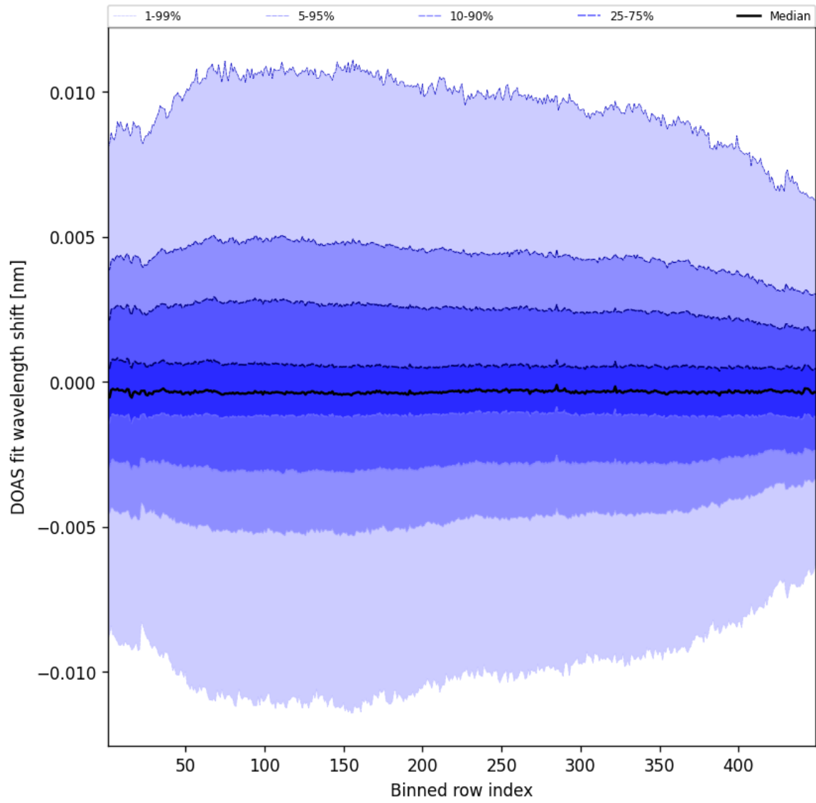
Figure 56: Along track statistics of “DOAS fit wavelength shift” for 2025-01-26 to 2025-01-26
