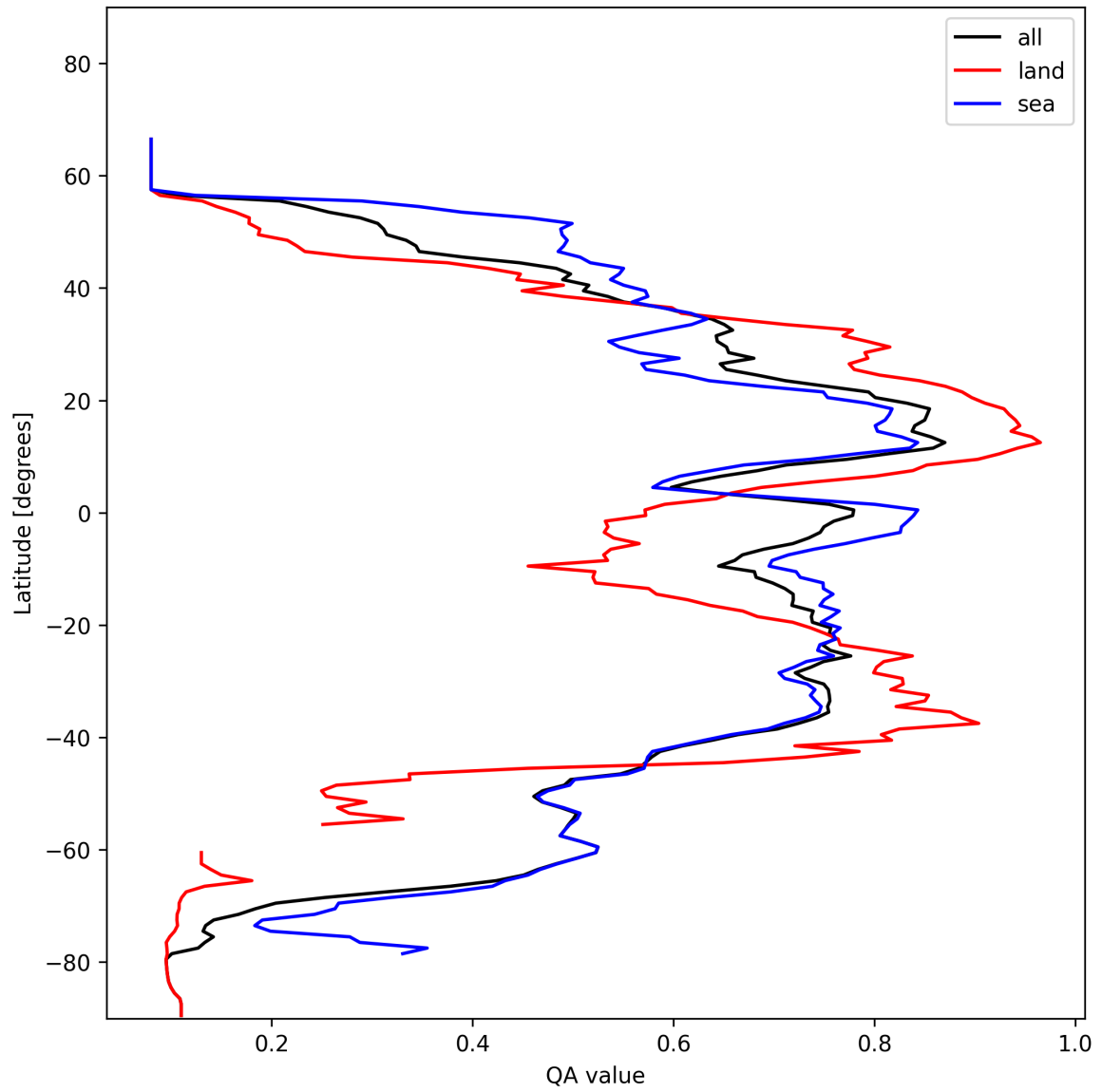
Figure 18: Zonal average of “QA value” for 2025-01-26 to 2025-01-26.
