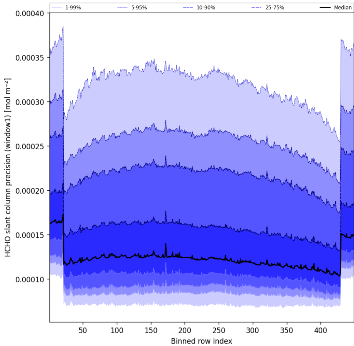
Figure 51: Along track statistics of “HCHO slant column precision (window1)” for 2025-01-26 to 2025-01-26
