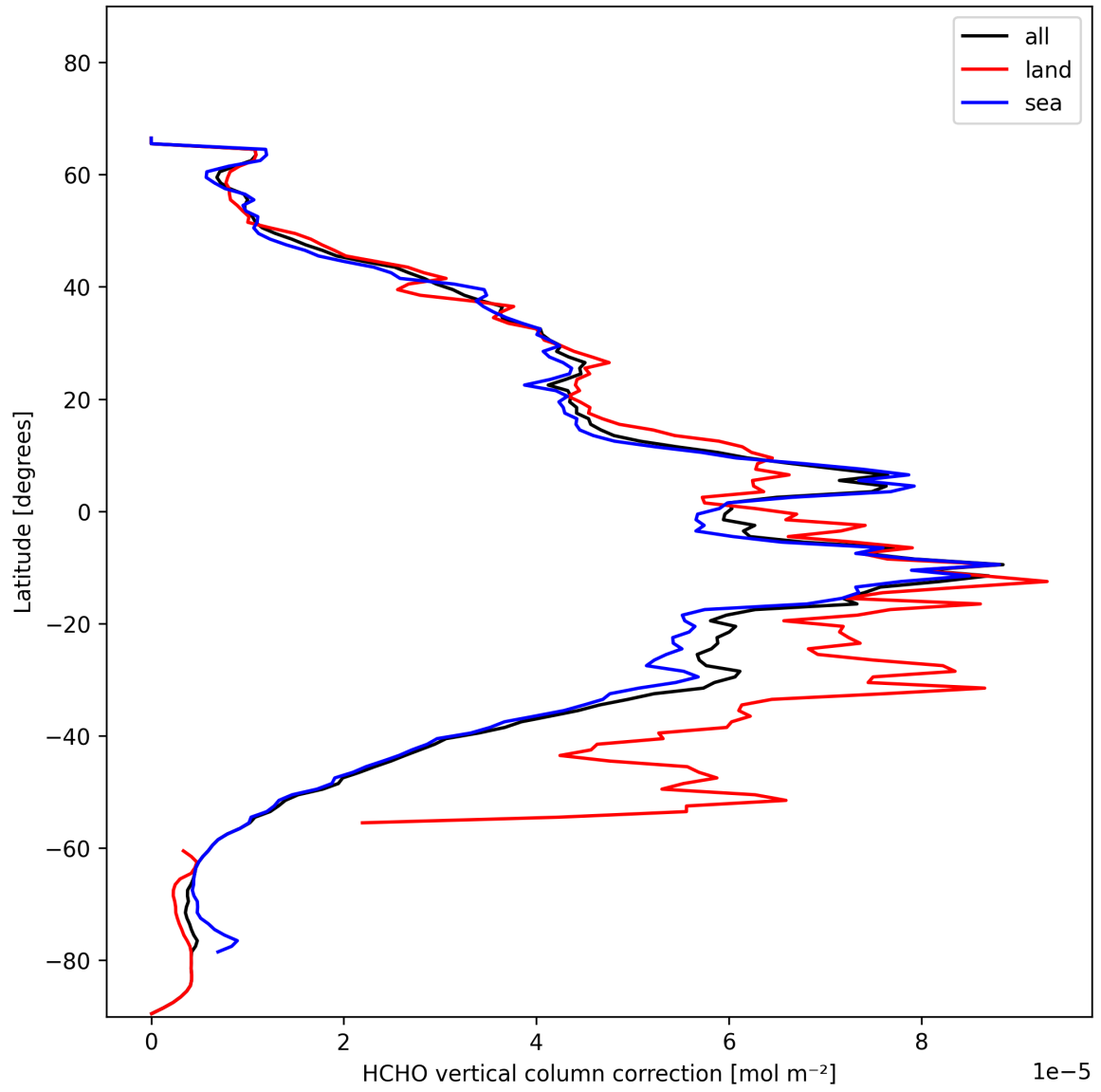
Figure 21: Zonal average of “HCHO vertical column correction” for 2025-01-26 to 2025-01-26.
