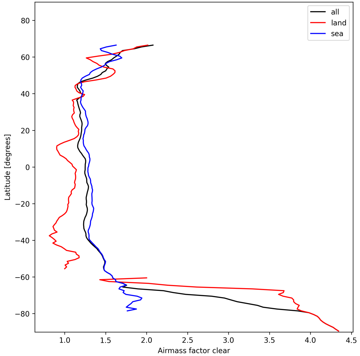
Figure 26: Zonal average of “Airmass factor clear” for 2025-01-26 to 2025-01-26.
