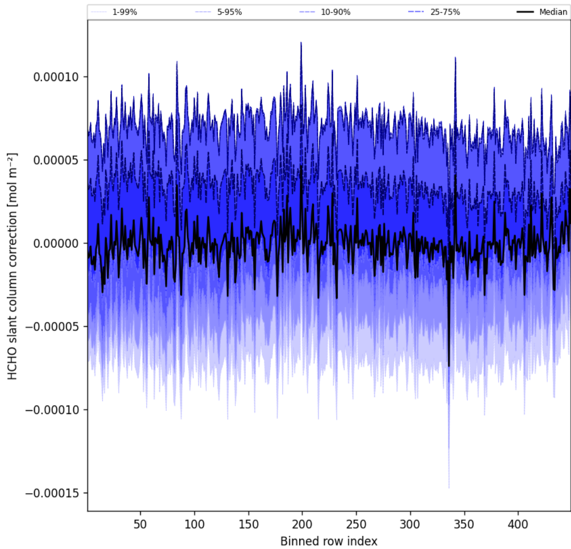
Figure 59: Along track statistics of “HCHO slant column correction” for 2025-01-26 to 2025-01-26
