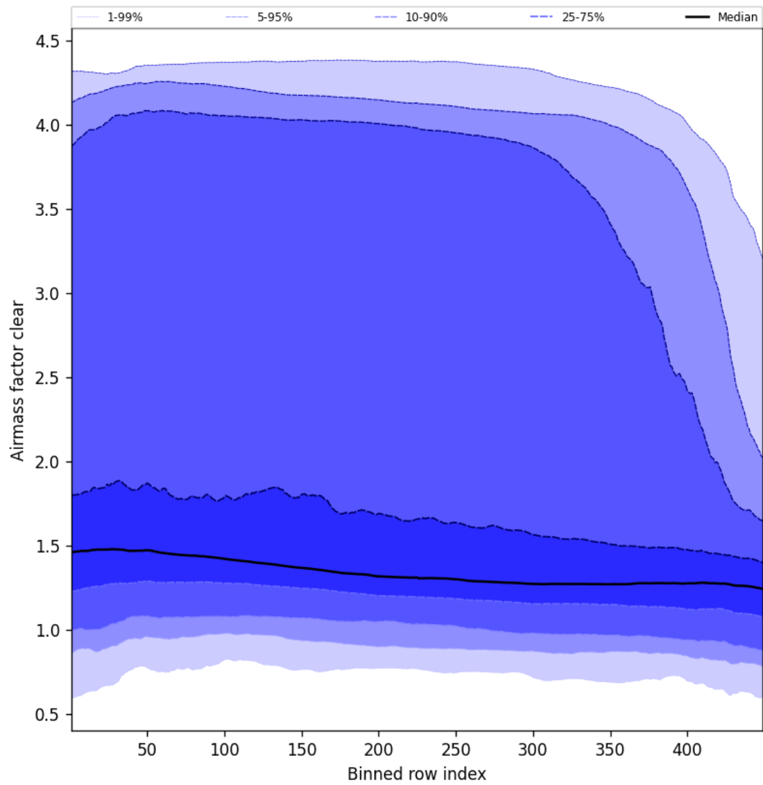
Figure 54: Along track statistics of “Airmass factor clear” for 2025-01-26 to 2025-01-26
