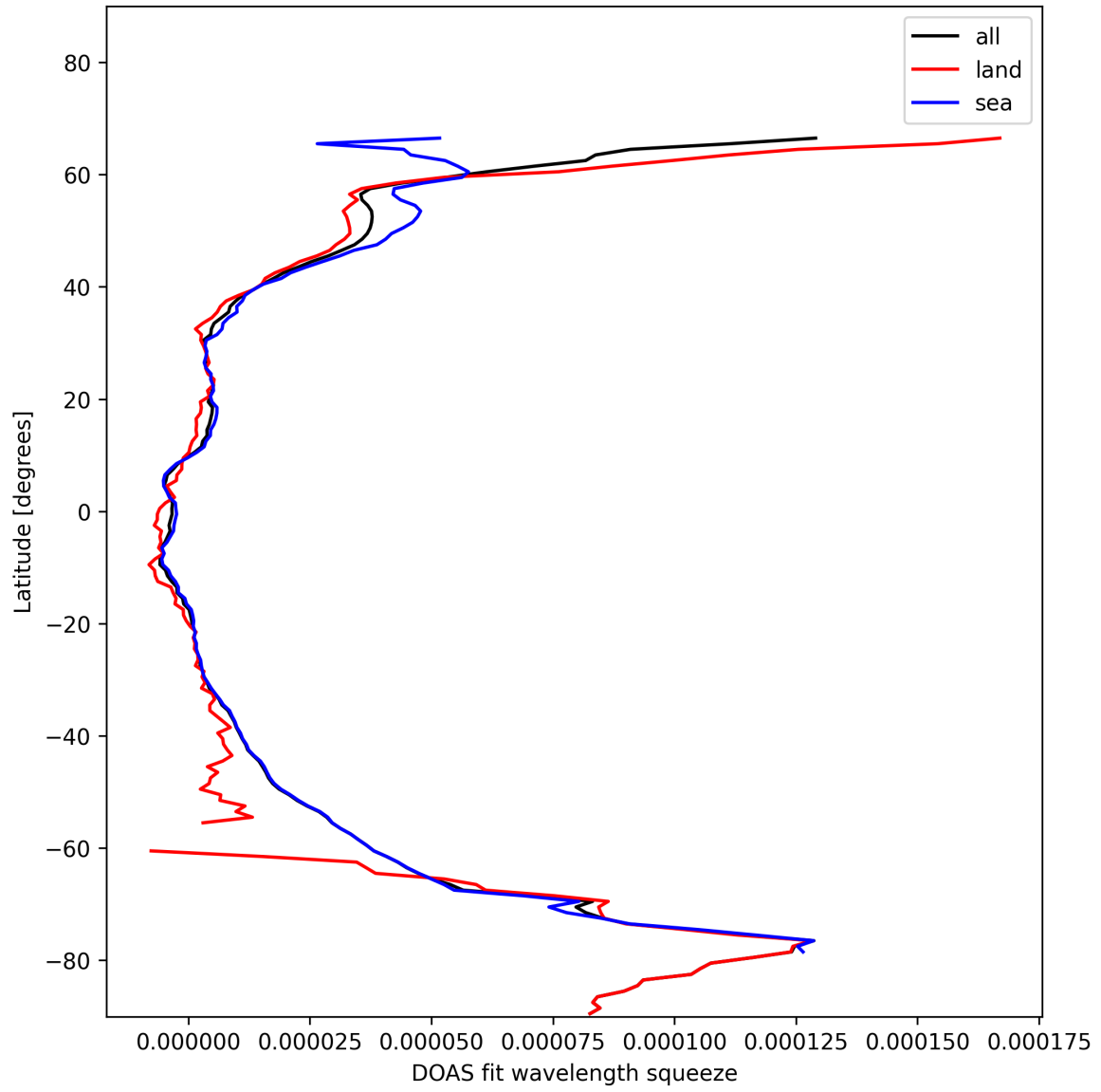
Figure 29: Zonal average of “DOAS fit wavelength squeeze” for 2025-01-26 to 2025-01-26.
