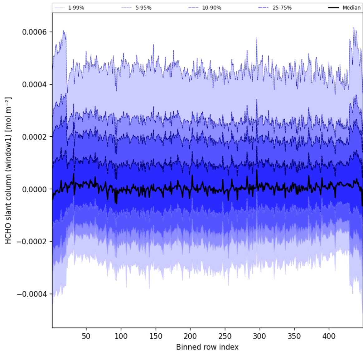
Figure 50: Along track statistics of “HCHO slant column (window1)” for 2025-01-26 to 2025-01-26
