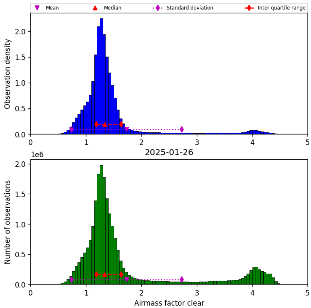
Figure 40: Histogram of “Airmass factor clear” for 2025-01-26 to 2025-01-26
