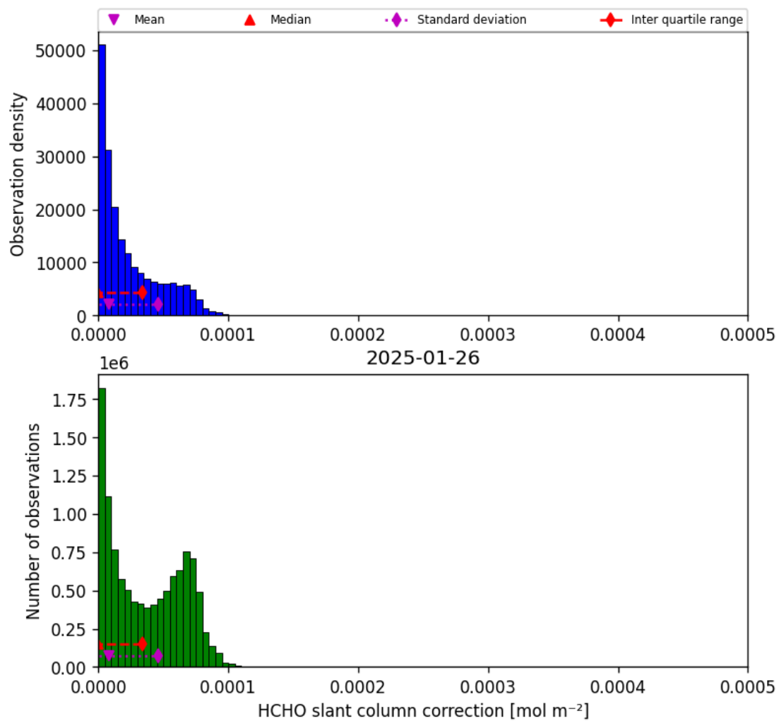
Figure 45: Histogram of “HCHO slant column correction” for 2025-01-26 to 2025-01-26
