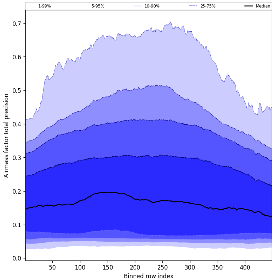
Figure 53: Along track statistics of “Airmass factor total precision” for 2025-01-26 to 2025-01-26
