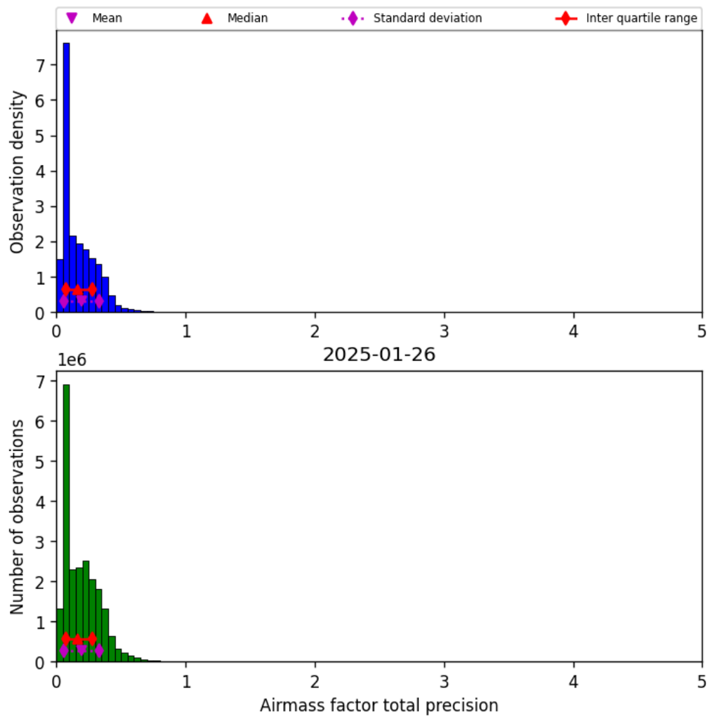
Figure 39: Histogram of “Airmass factor total precision” for 2025-01-26 to 2025-01-26
