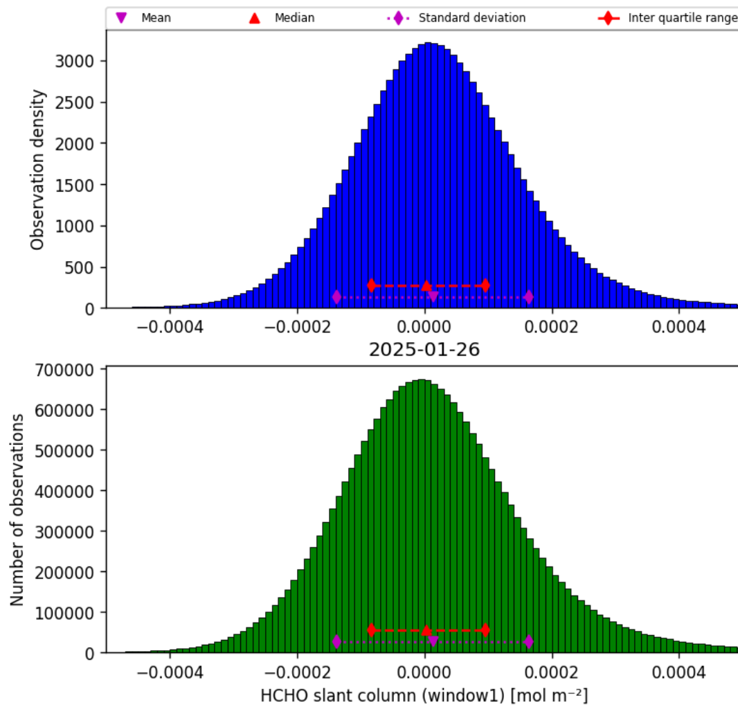
Figure 36: Histogram of “HCHO slant column (window1)” for 2025-01-26 to 2025-01-26
