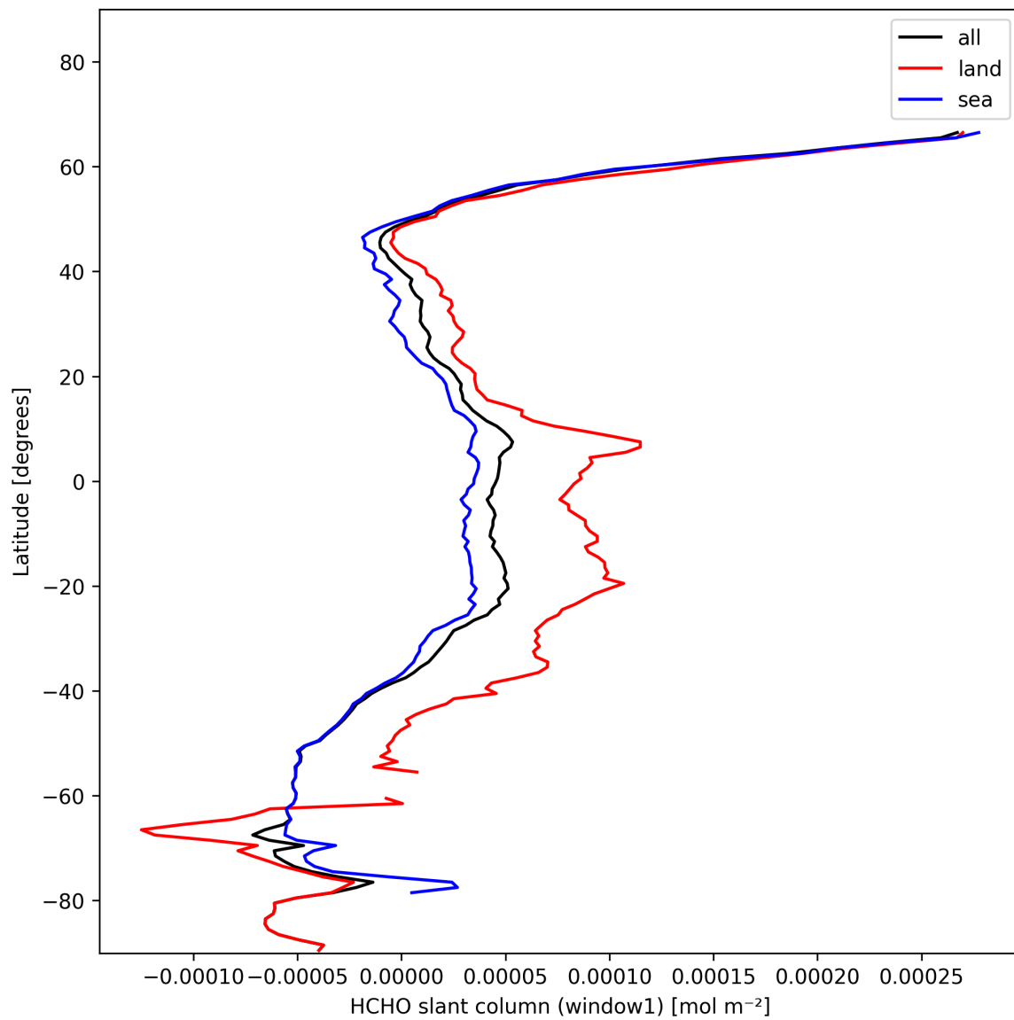
Figure 22: Zonal average of “HCHO slant column (window1)” for 2025-01-26 to 2025-01-26.
