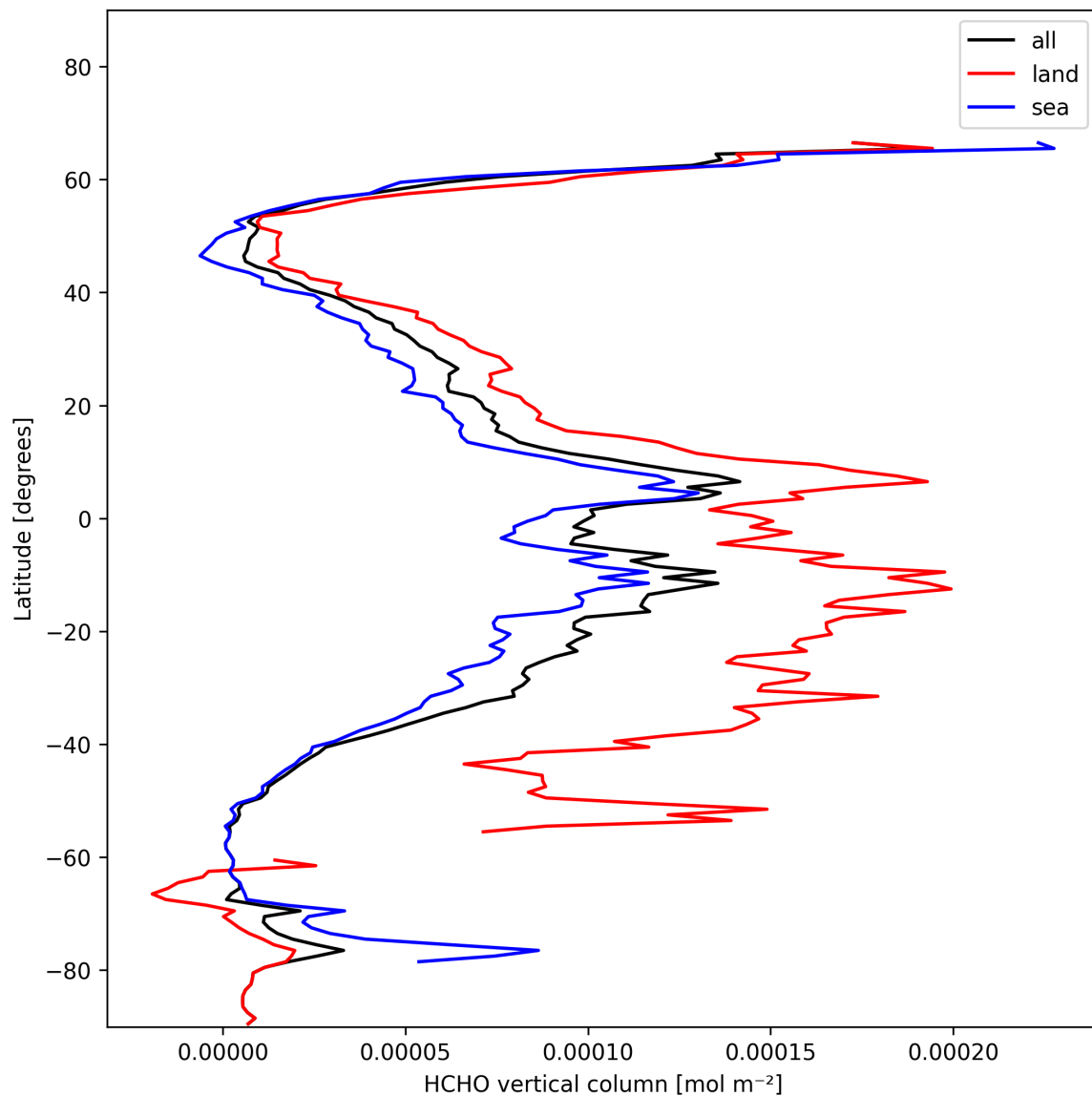
Figure 19: Zonal average of “HCHO vertical column” for 2025-01-26 to 2025-01-26.
