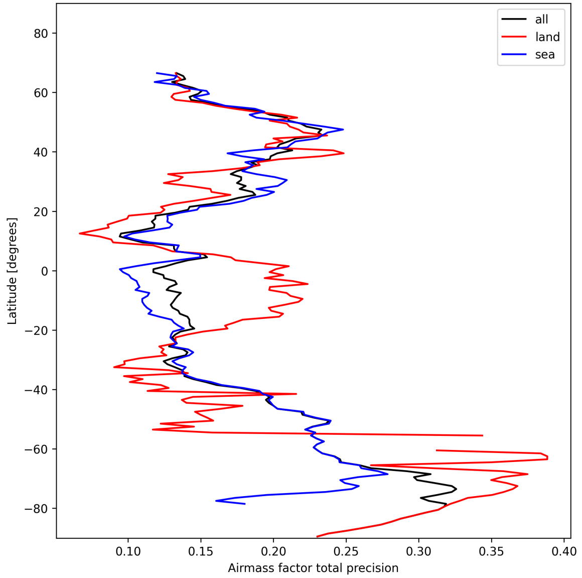
Figure 25: Zonal average of “Airmass factor total precision” for 2025-01-26 to 2025-01-26.
