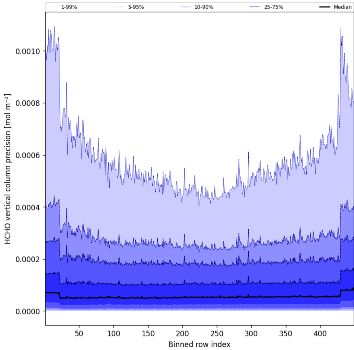
Figure 48: Along track statistics of “HCHO vertical column precision” for 2025-01-26 to 2025-01-26
