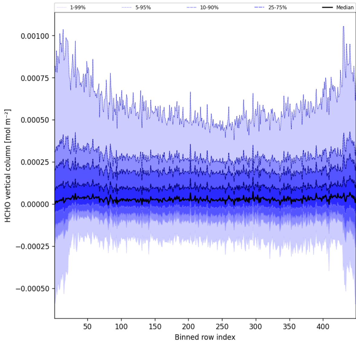
Figure 47: Along track statistics of “HCHO vertical column” for 2025-01-26 to 2025-01-26
