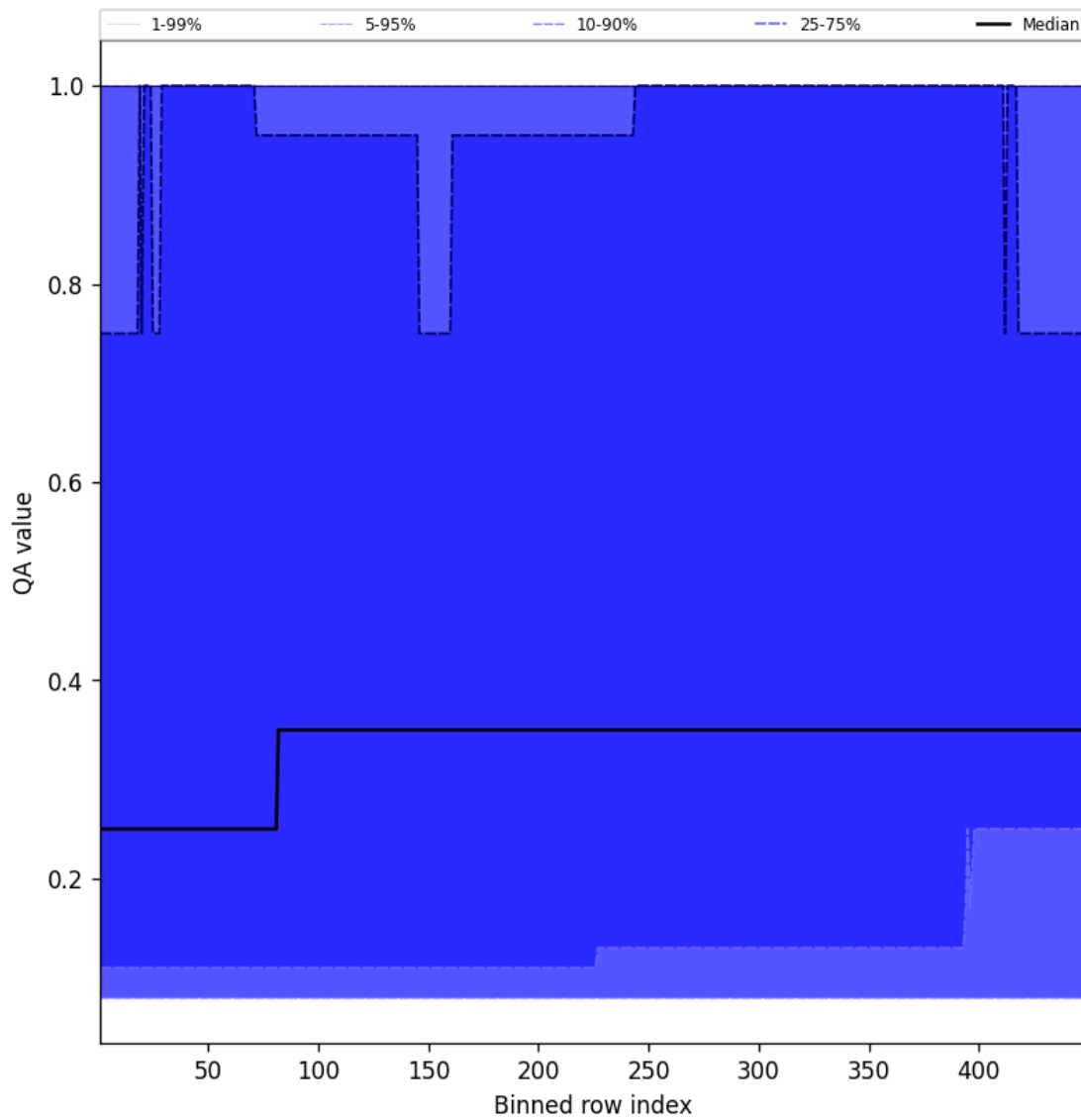
Figure 46: Along track statistics of “QA value” for 2025-01-26 to 2025-01-26
