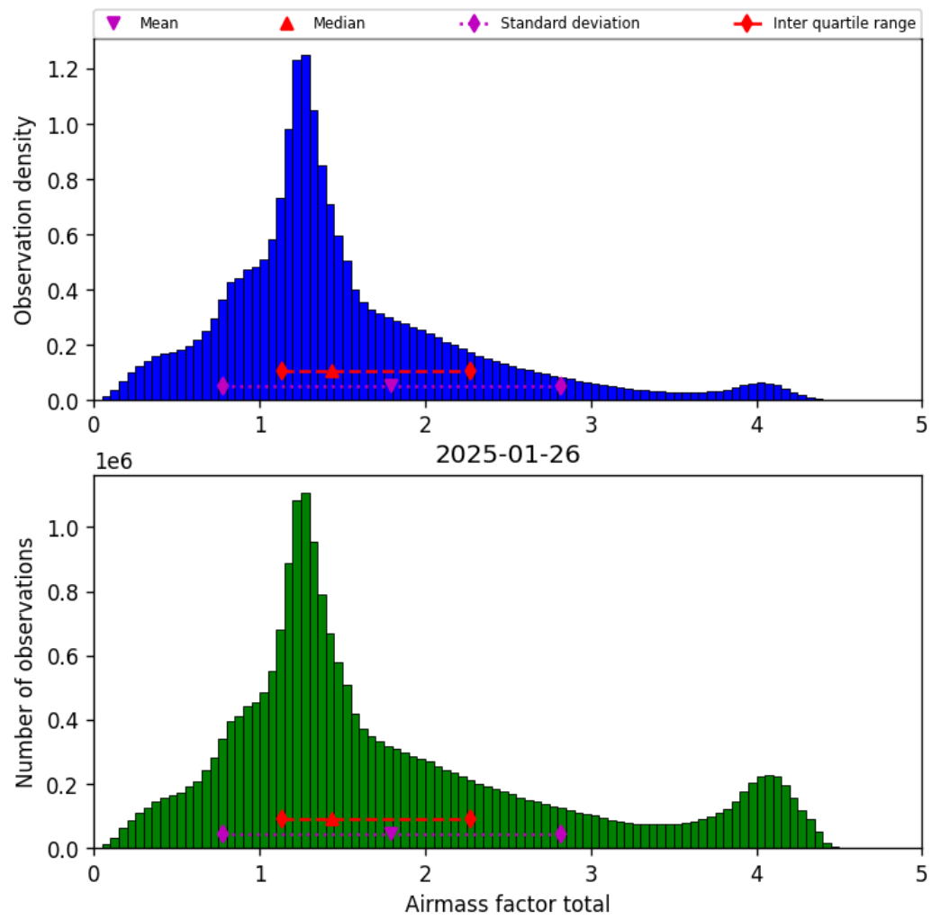
Figure 38: Histogram of “Airmass factor total” for 2025-01-26 to 2025-01-26
