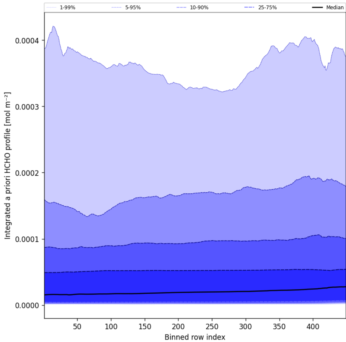
Figure 55: Along track statistics of "Integrated a priori HCHO profile" for 2025-01-26 to 2025-01-26
