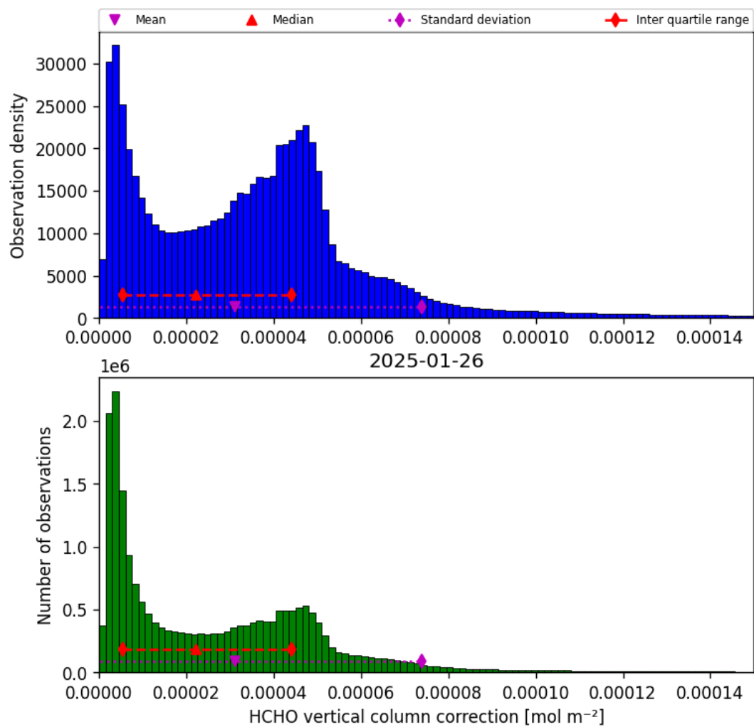
Figure 35: Histogram of “HCHO vertical column correction” for 2025-01-26 to 2025-01-26
