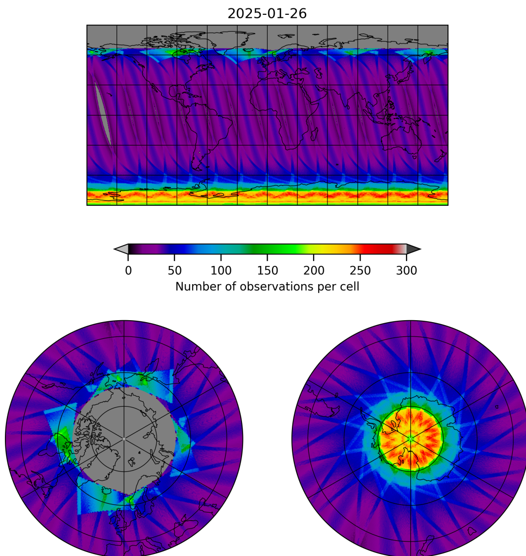
Figure 17: Map of the number of observations for 2025-01-26 to 2025-01-26
