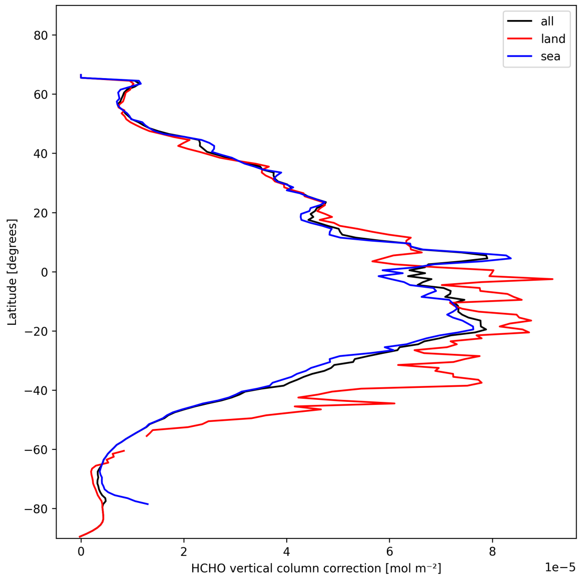
Figure 21: Zonal average of “HCHO vertical column correction” for 2025-01-27 to 2025-01-28.
