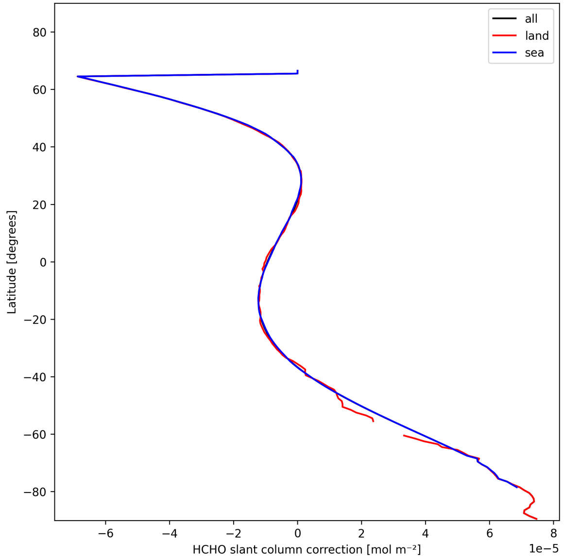
Figure 31: Zonal average of “HCHO slant column correction” for 2025-01-27 to 2025-01-28.
