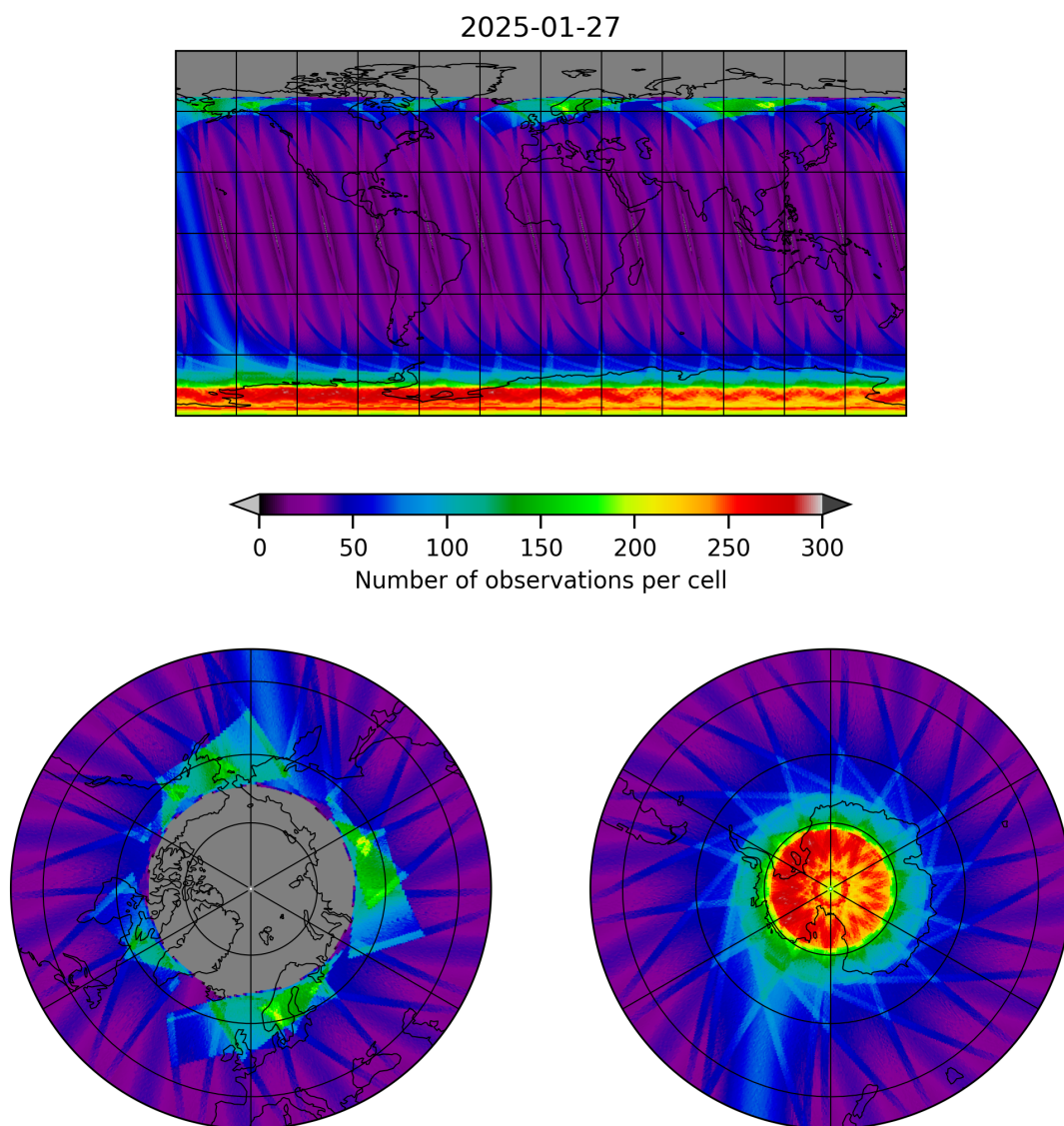
Figure 17: Map of the number of observations for 2025-01-27 to 2025-01-28
