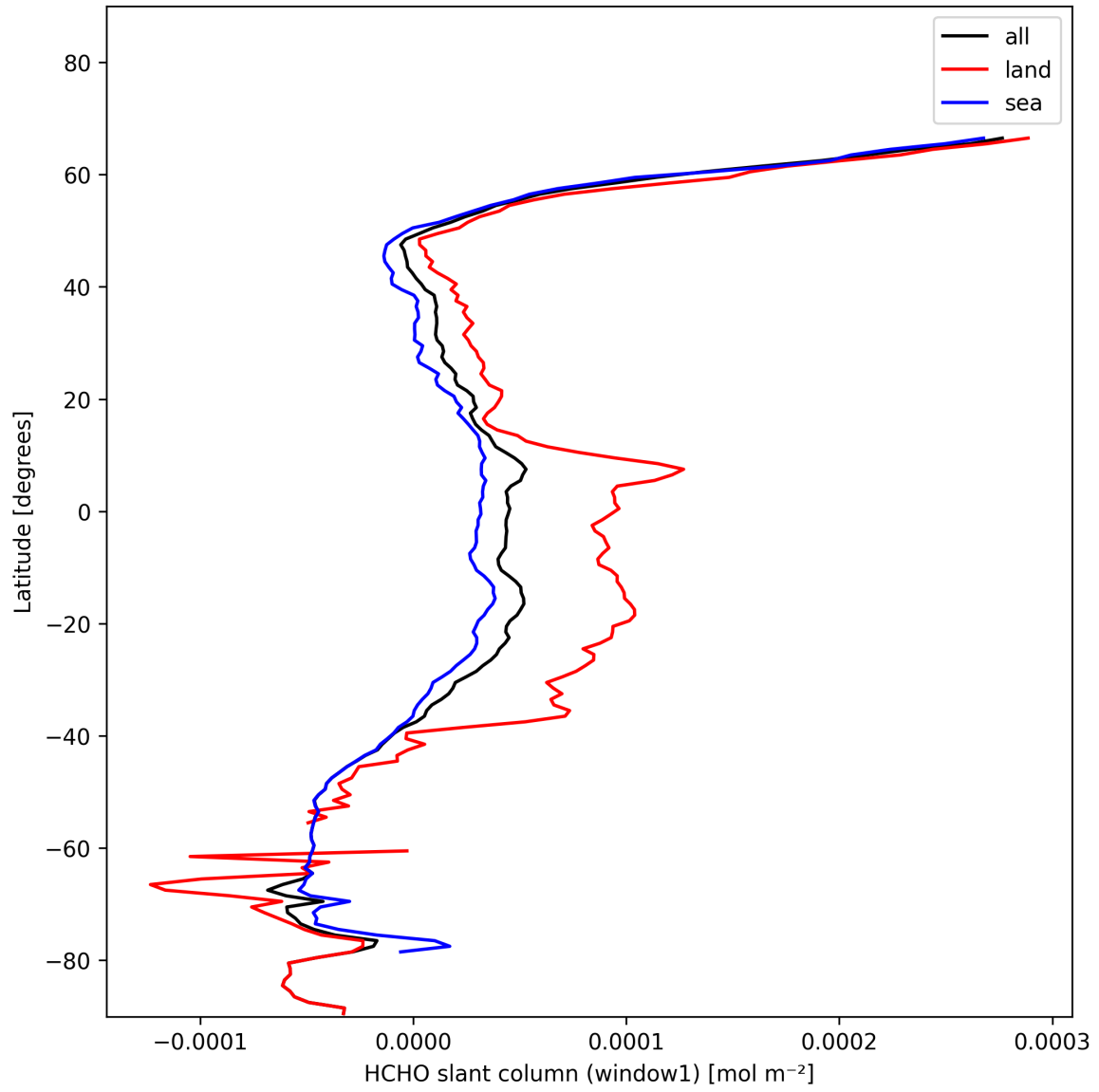
Figure 22: Zonal average of “HCHO slant column (window1)” for 2025-01-27 to 2025-01-28.
