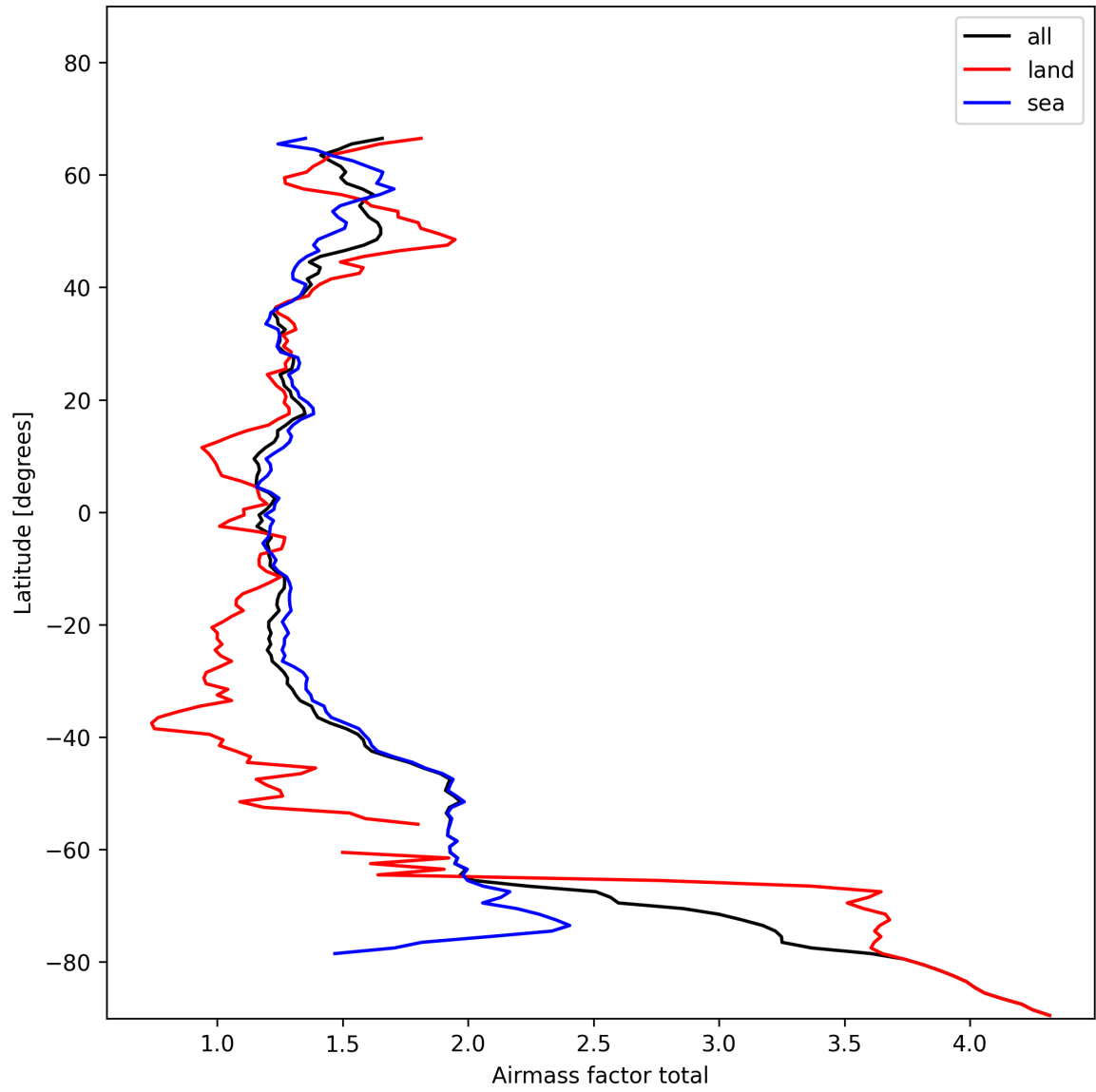
Figure 24: Zonal average of “Airmass factor total” for 2025-01-27 to 2025-01-28.
