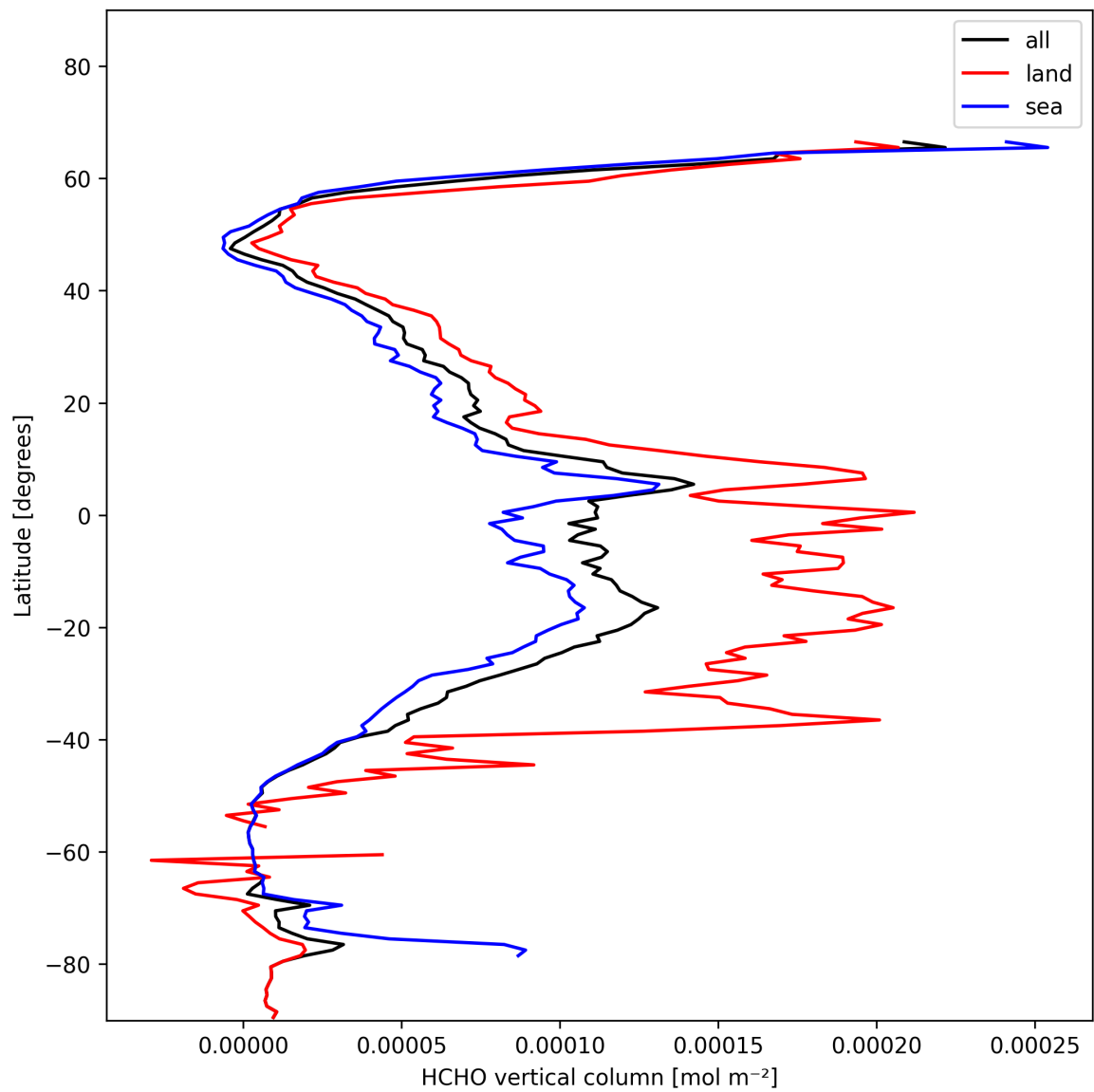
Figure 19: Zonal average of “HCHO vertical column” for 2025-01-27 to 2025-01-28.
