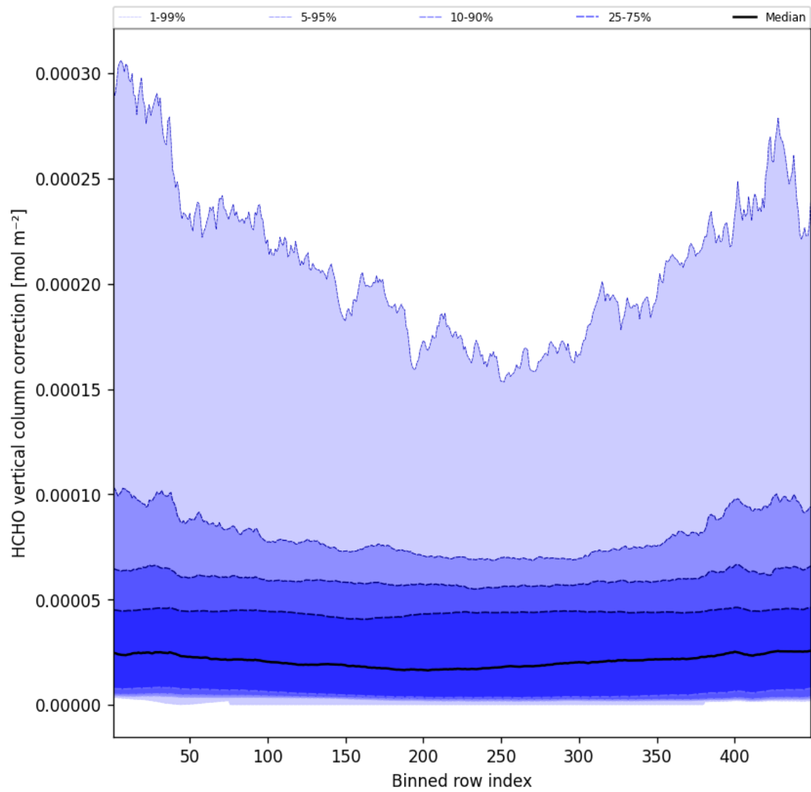
Figure 49: Along track statistics of “HCHO vertical column correction” for 2025-01-27 to 2025-01-28
