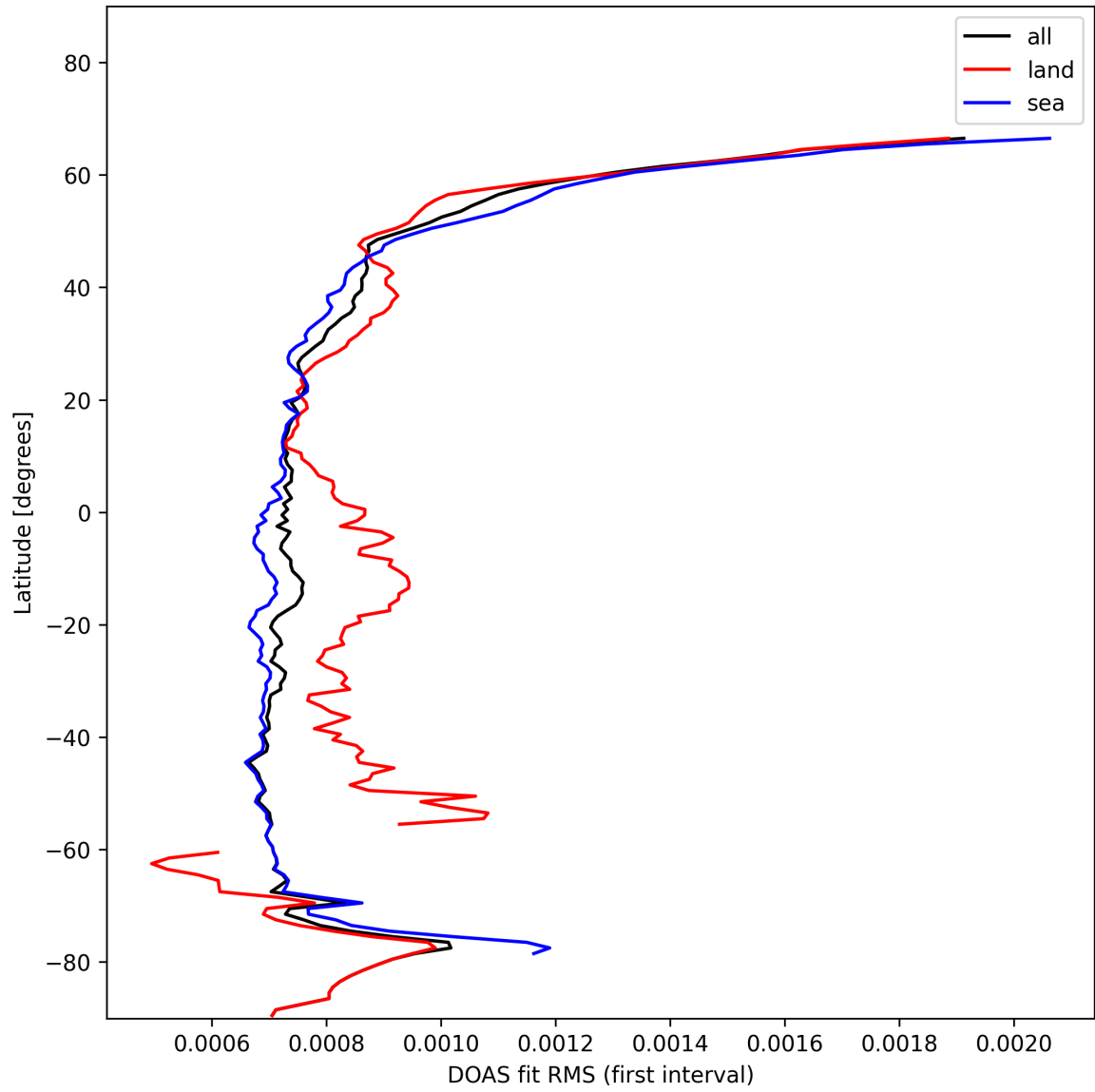
Figure 30: Zonal average of “DOAS fit RMS (first interval)” for 2025-01-27 to 2025-01-28.
