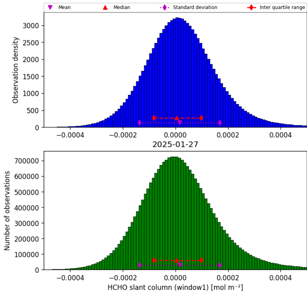
Figure 36: Histogram of “HCHO slant column (window1)” for 2025-01-27 to 2025-01-28
