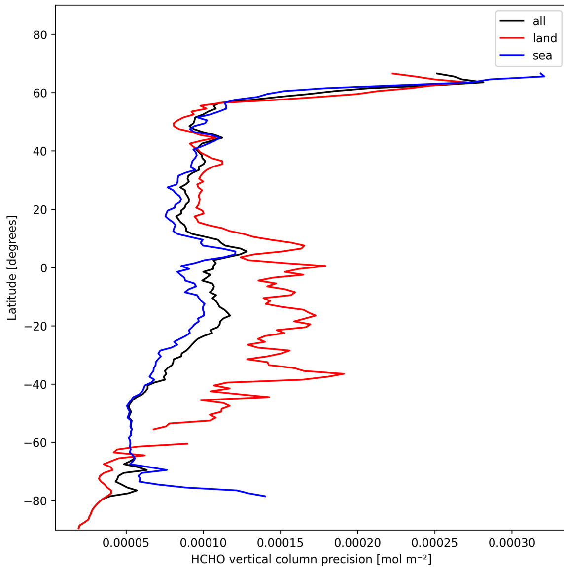
Figure 20: Zonal average of “HCHO vertical column precision” for 2025-01-27 to 2025-01-28.
