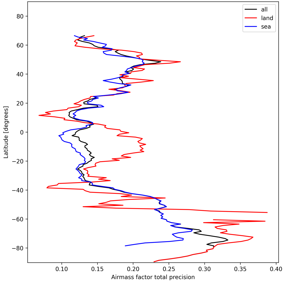
Figure 25: Zonal average of “Airmass factor total precision” for 2025-01-27 to 2025-01-28.
