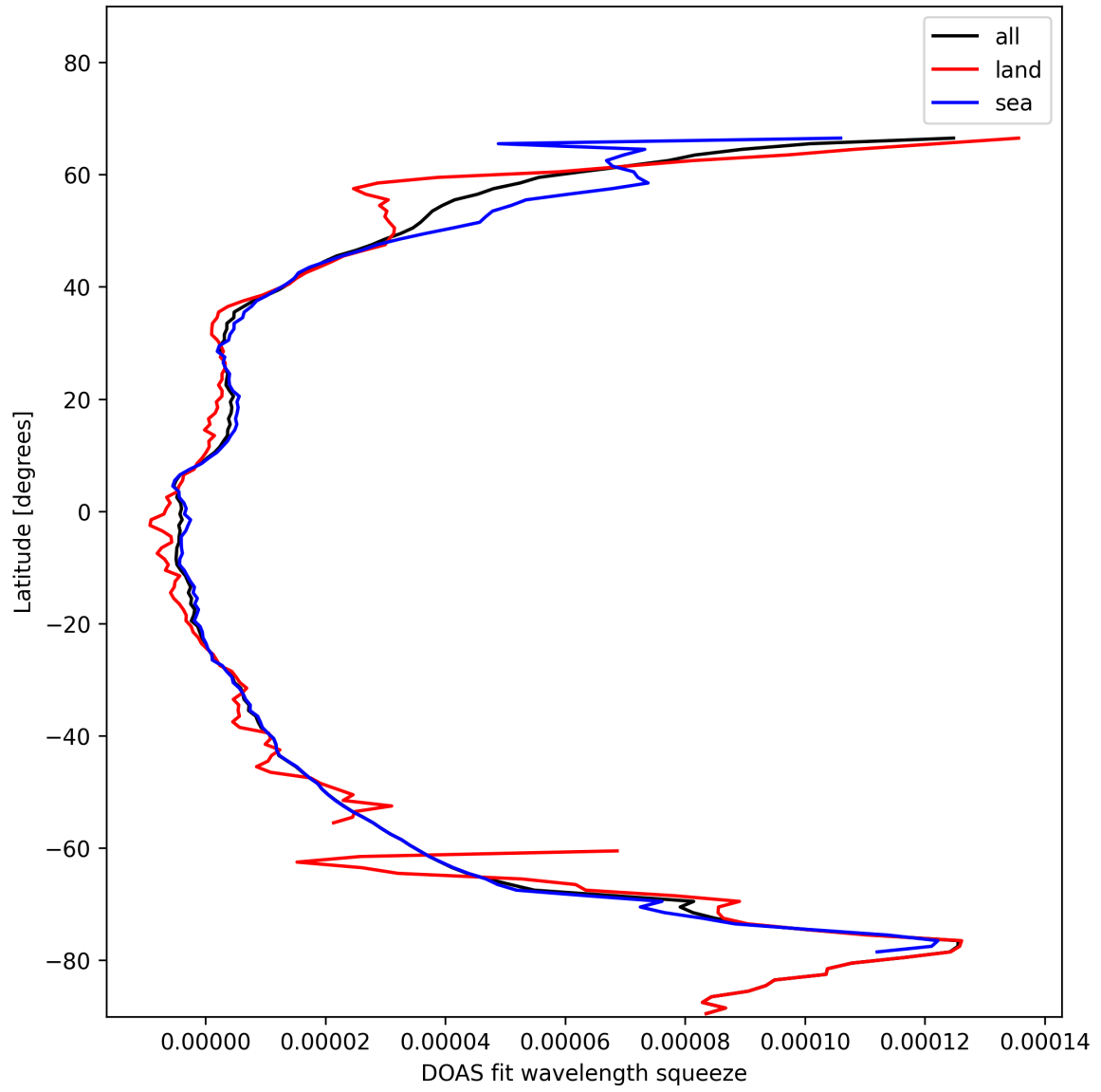
Figure 29: Zonal average of “DOAS fit wavelength squeeze” for 2025-01-27 to 2025-01-28.
