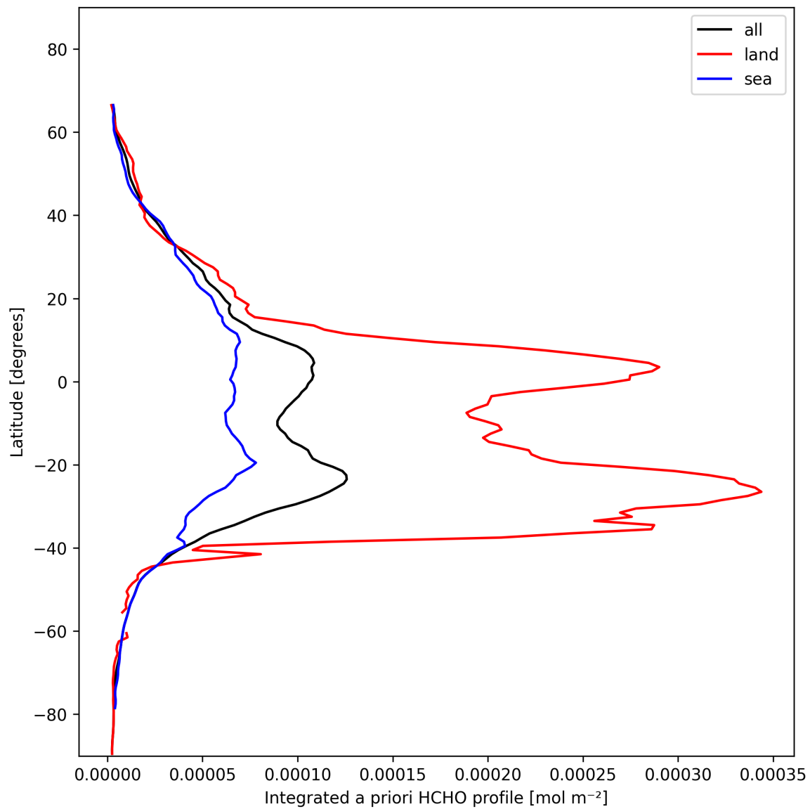
Figure 27: Zonal average of “Integrated a priori HCHO profile” for 2025-01-27 to 2025-01-28.
