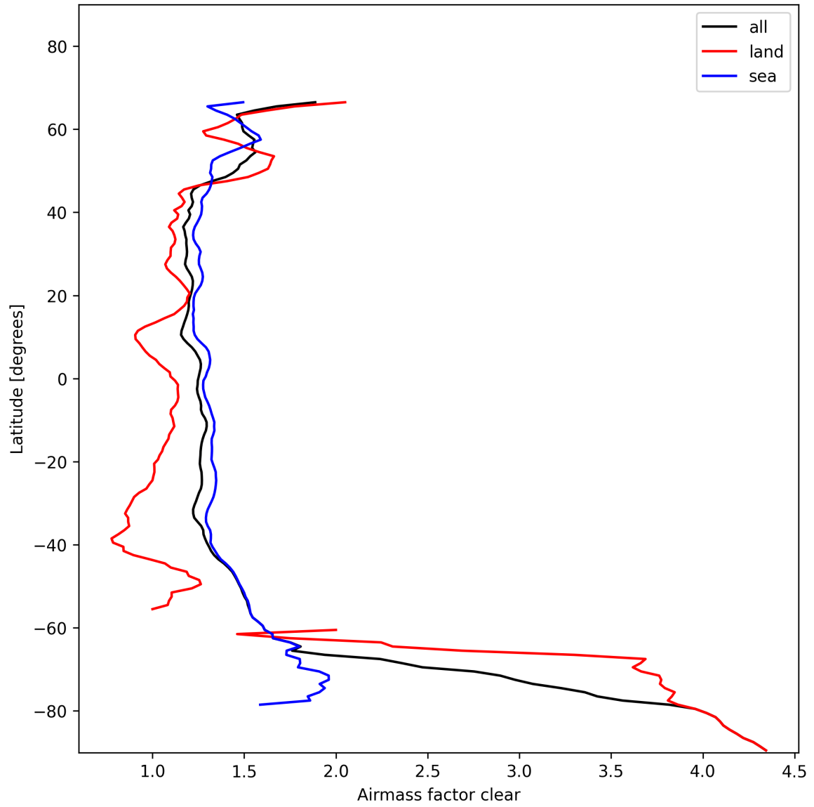
Figure 26: Zonal average of “Airmass factor clear” for 2025-01-27 to 2025-01-28.
