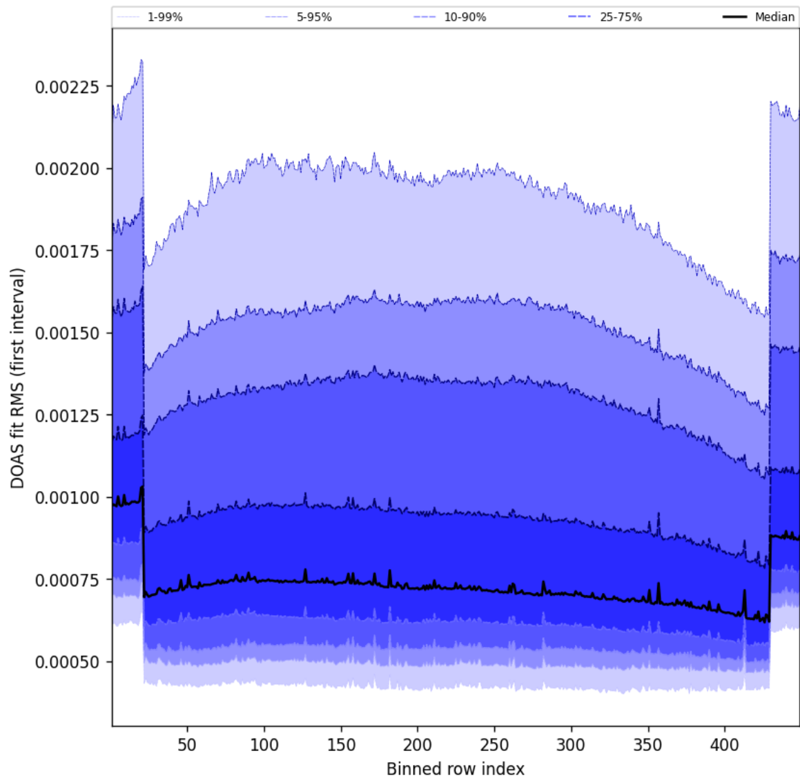
Figure 58: Along track statistics of “DOAS fit RMS (first interval)” for 2025-01-27 to 2025-01-28
