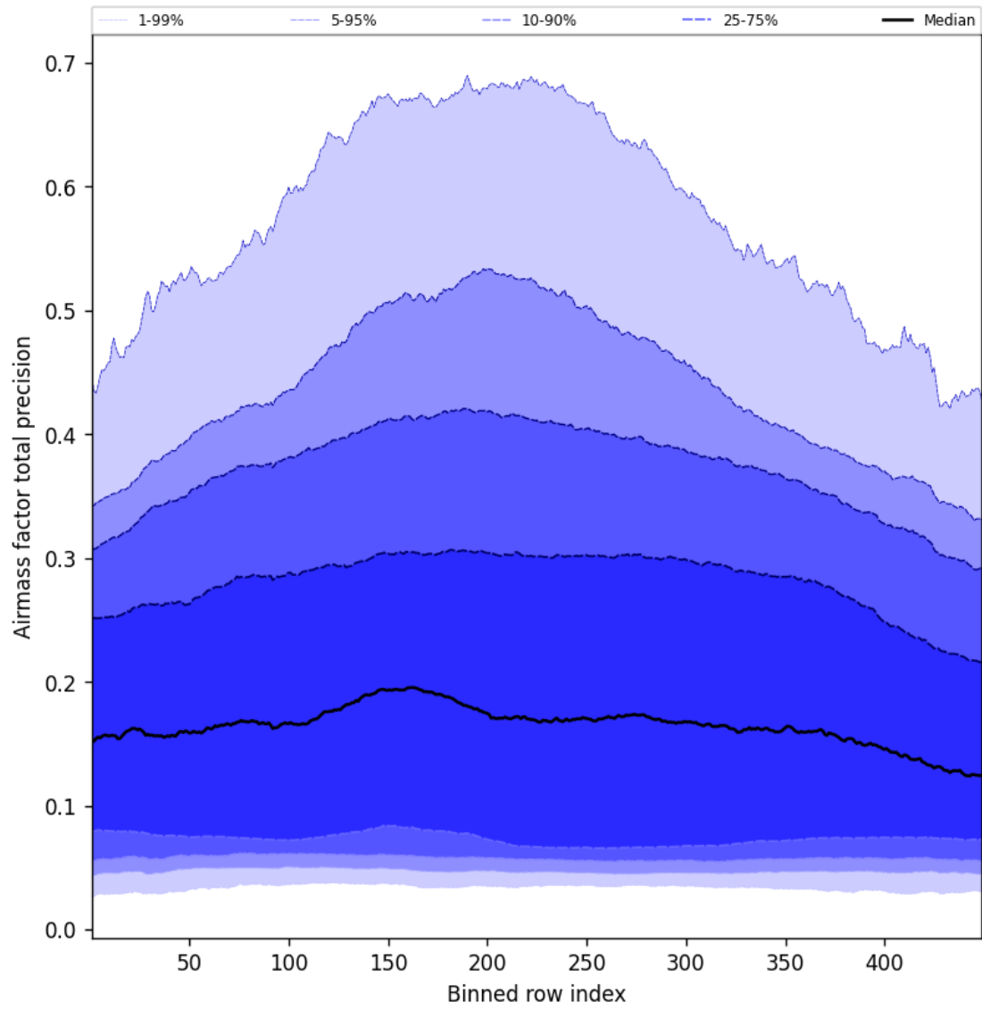
Figure 53: Along track statistics of “Airmass factor total precision” for 2025-01-27 to 2025-01-28
