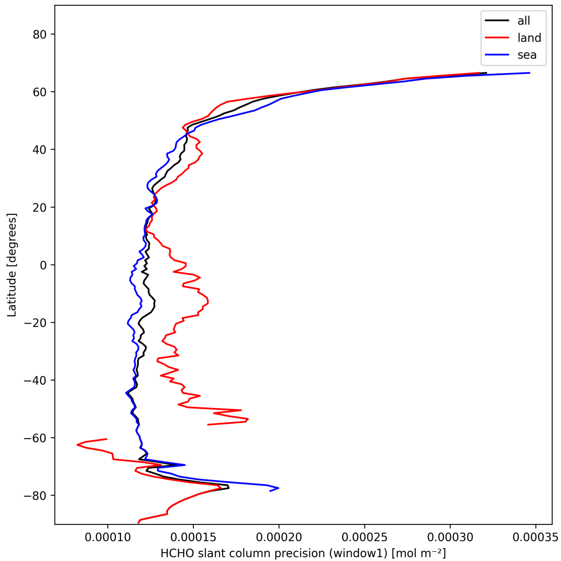
Figure 23: Zonal average of “HCHO slant column precision (window1)” for 2025-01-27 to 2025-01-28.
