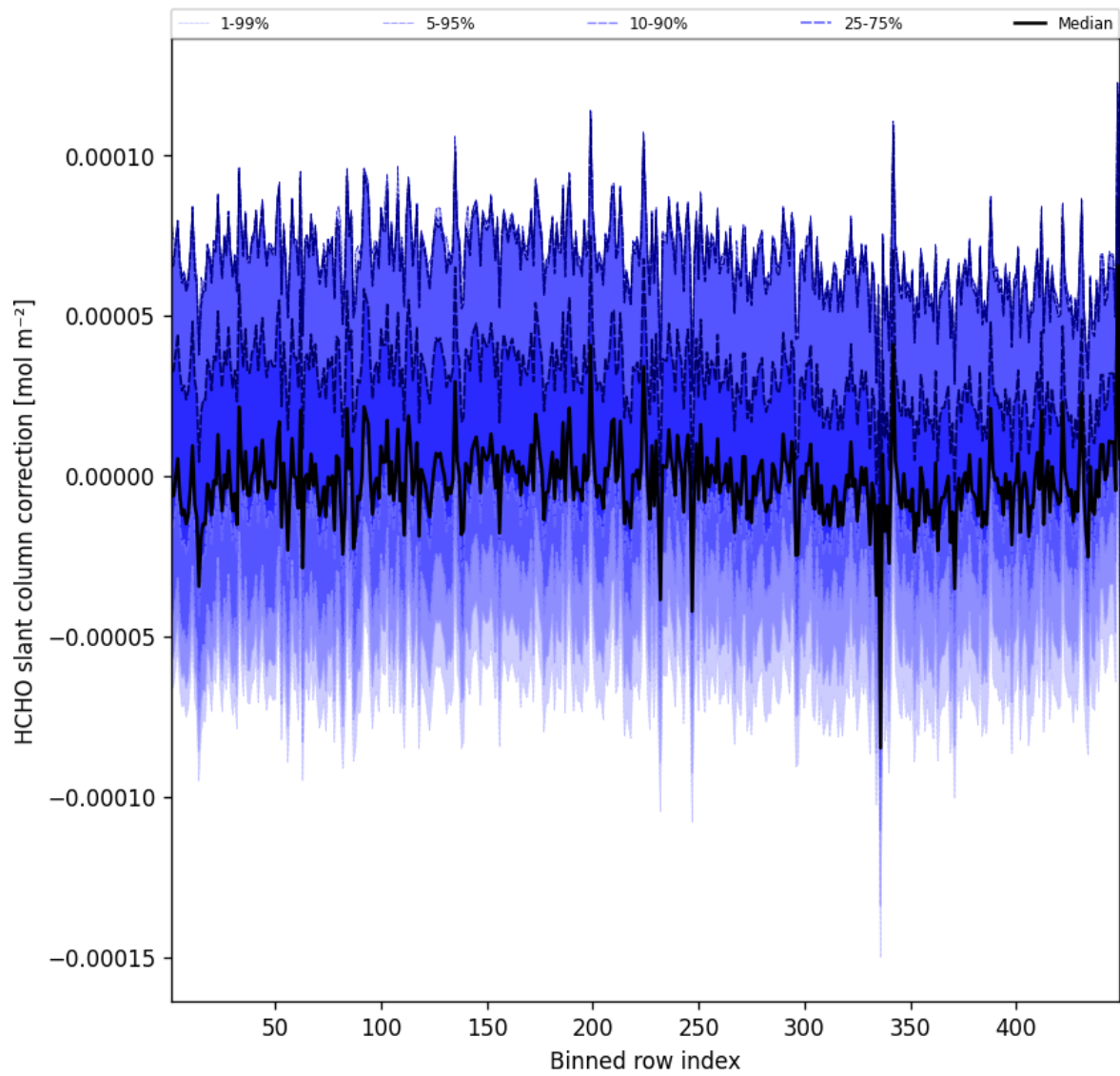
Figure 59: Along track statistics of “HCHO slant column correction” for 2025-01-27 to 2025-01-28
