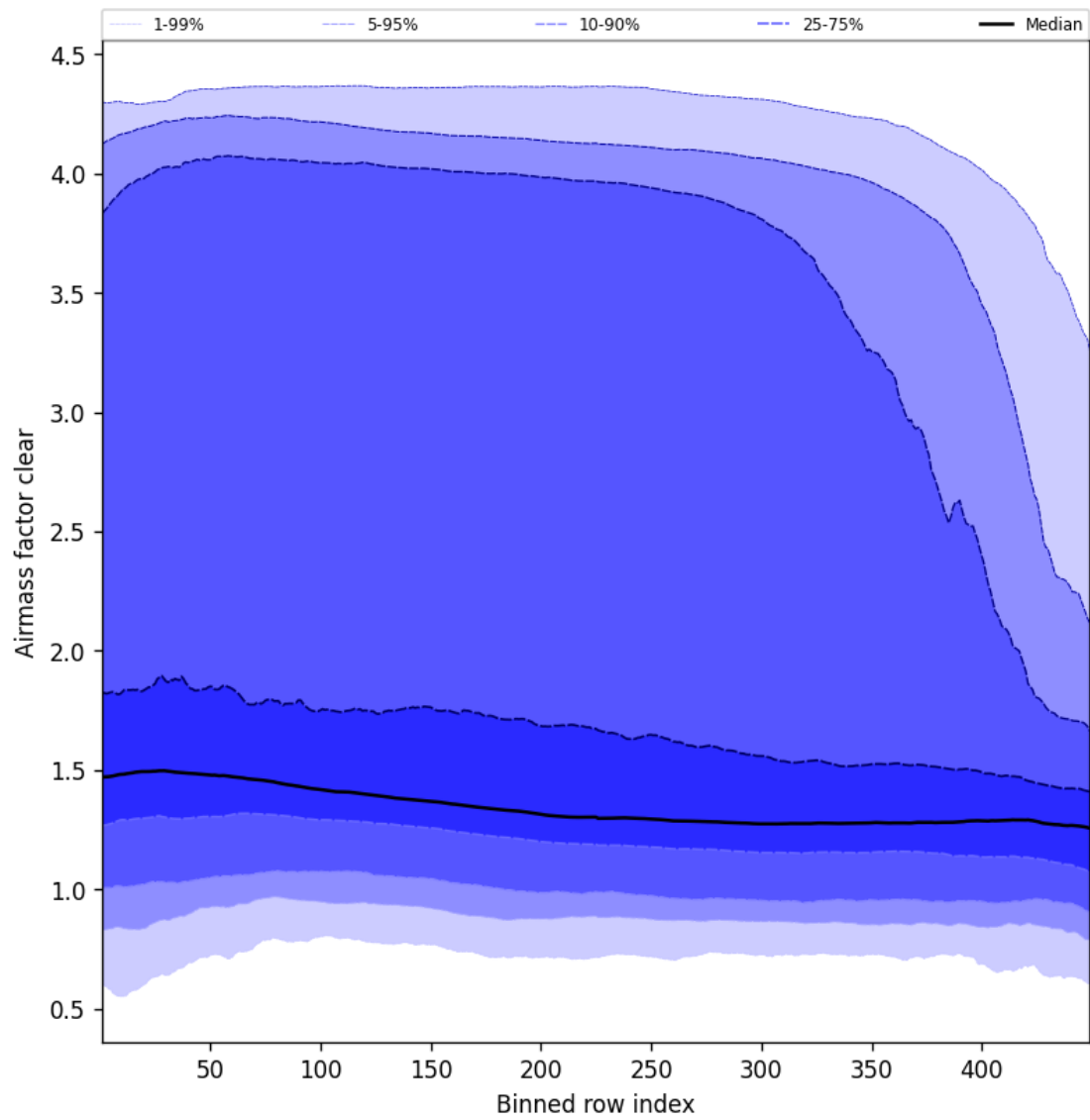
Figure 54: Along track statistics of “Airmass factor clear” for 2025-01-27 to 2025-01-28
