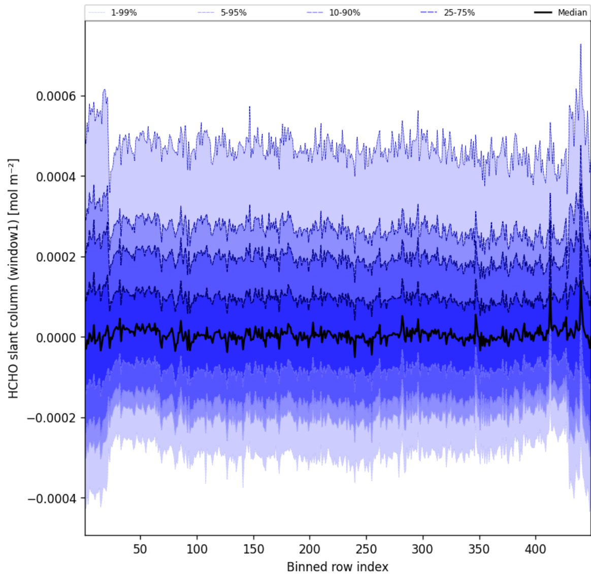
Figure 50: Along track statistics of “HCHO slant column (window1)” for 2025-01-27 to 2025-01-28
