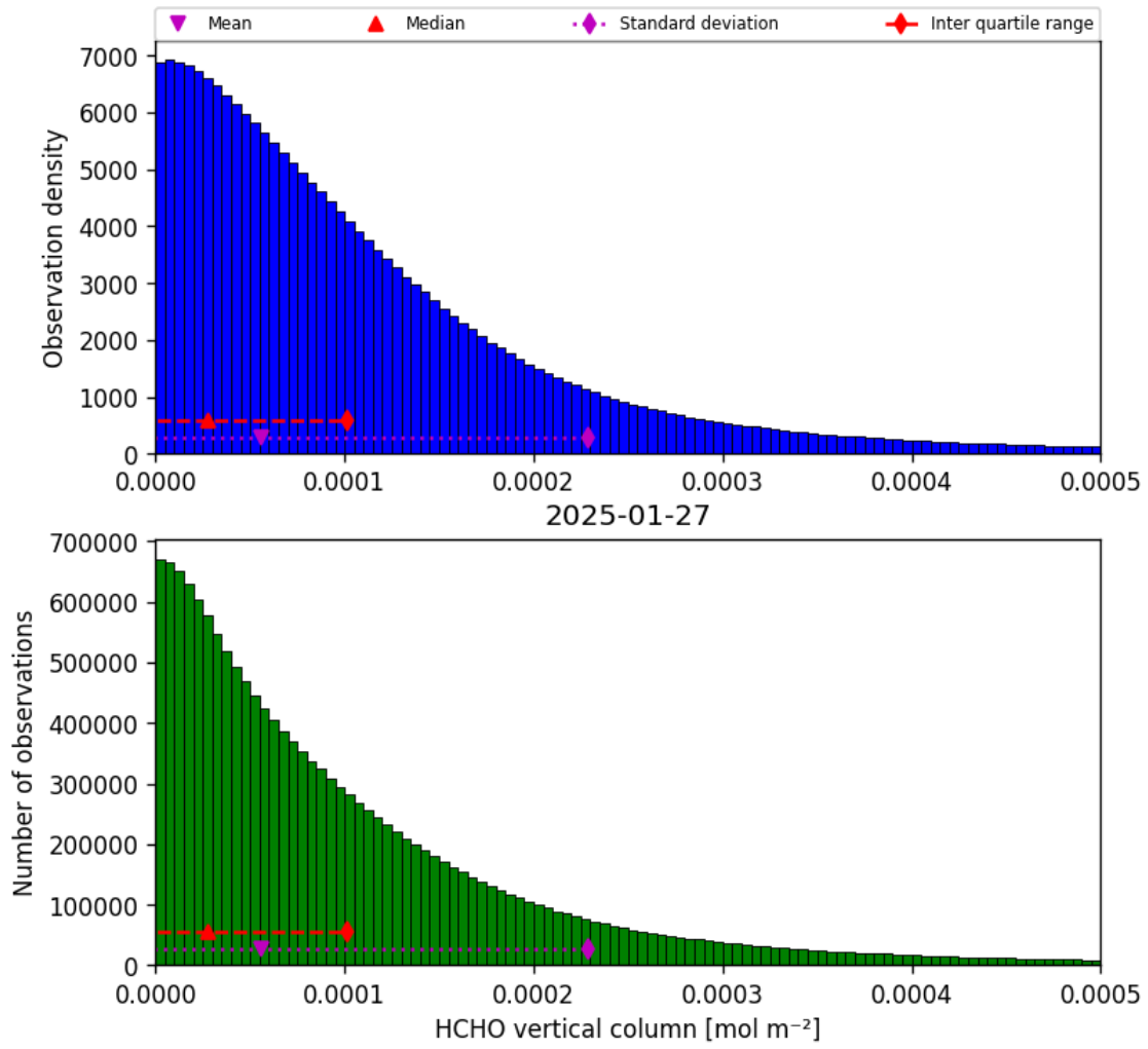
Figure 33: Histogram of “HCHO vertical column” for 2025-01-27 to 2025-01-28
