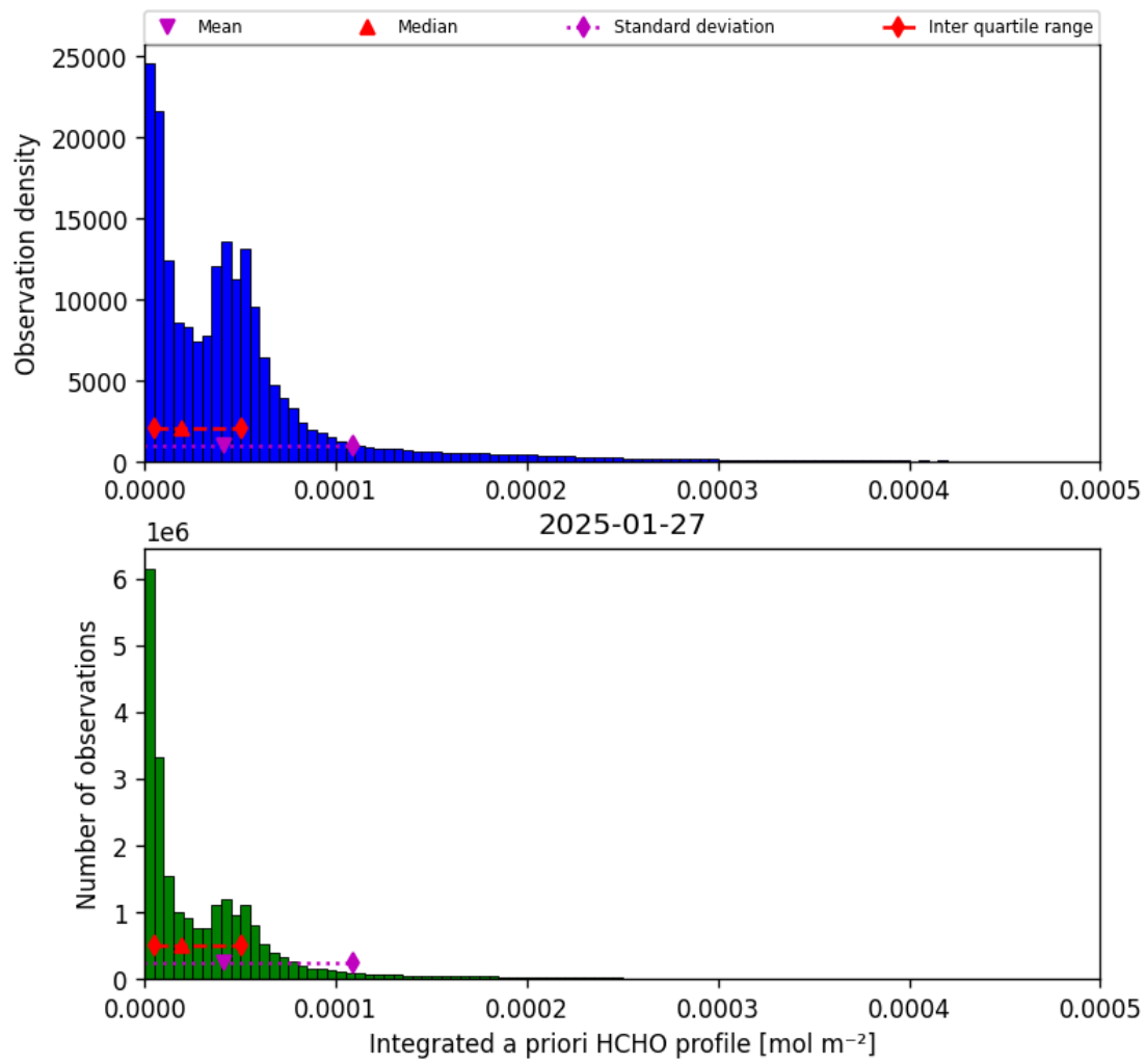
Figure 41: Histogram of “Integrated a priori HCHO profile” for 2025-01-27 to 2025-01-28
