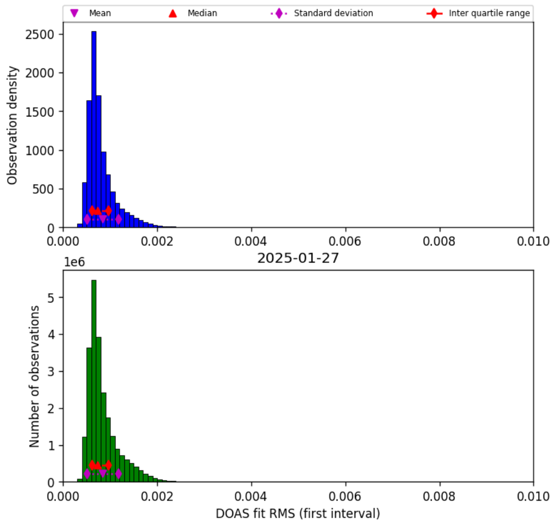
Figure 44: Histogram of “DOAS fit RMS (first interval)” for 2025-01-27 to 2025-01-28
