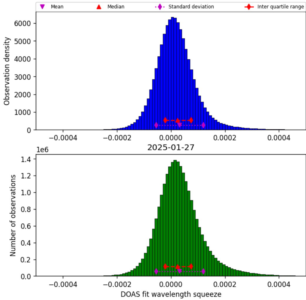
Figure 43: Histogram of “DOAS fit wavelength squeeze” for 2025-01-27 to 2025-01-28
