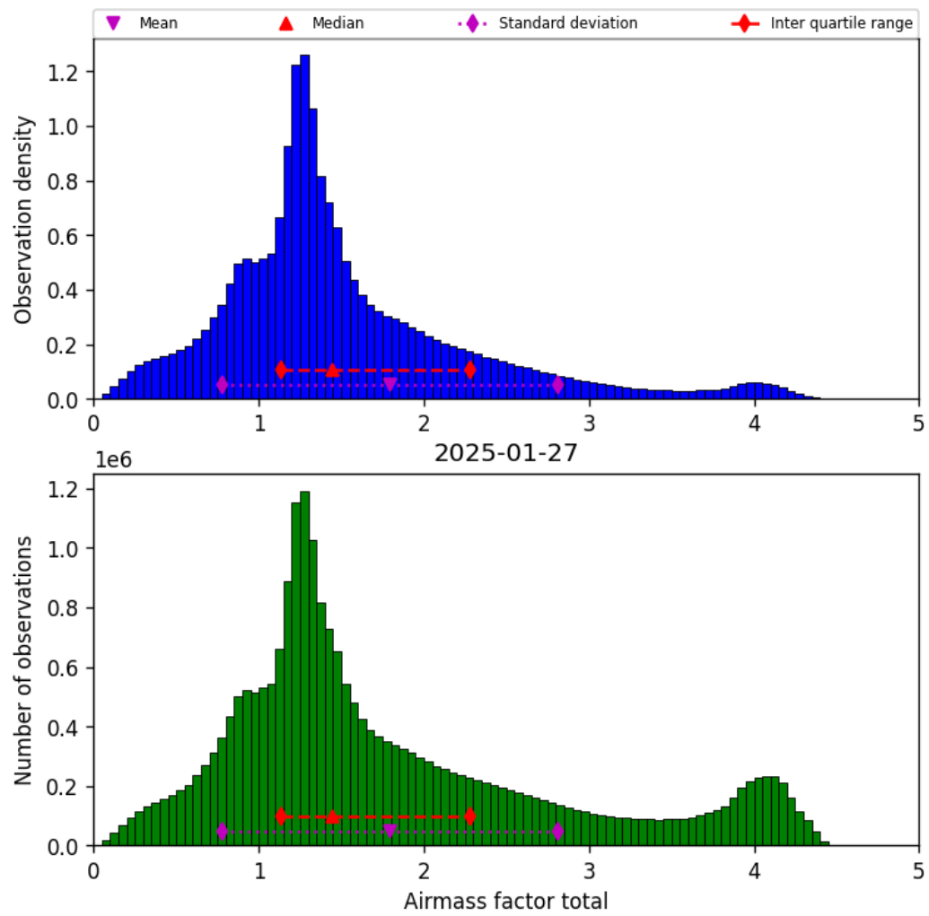
Figure 38: Histogram of “Airmass factor total” for 2025-01-27 to 2025-01-28
