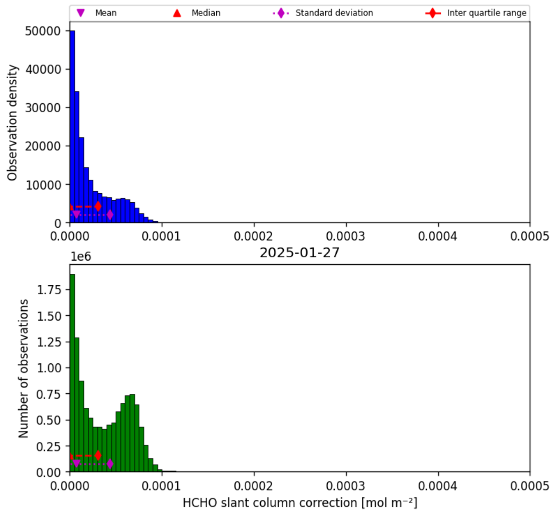
Figure 45: Histogram of “HCHO slant column correction” for 2025-01-27 to 2025-01-28
