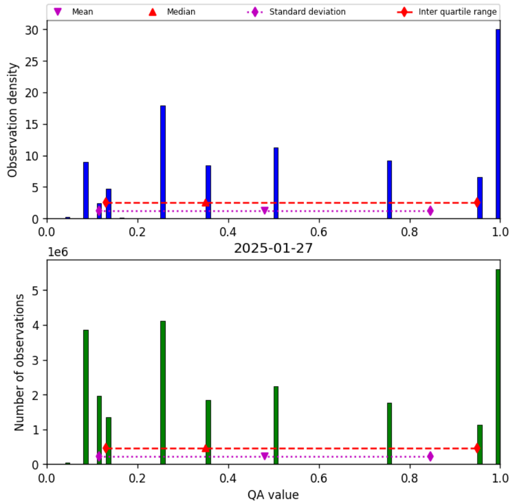
Figure 32: Histogram of “QA value” for 2025-01-27 to 2025-01-28
