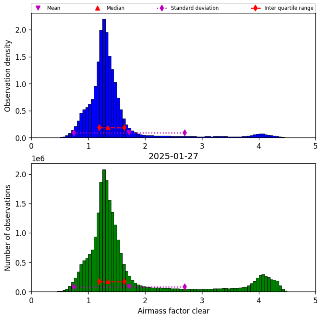
Figure 40: Histogram of “Airmass factor clear” for 2025-01-27 to 2025-01-28
