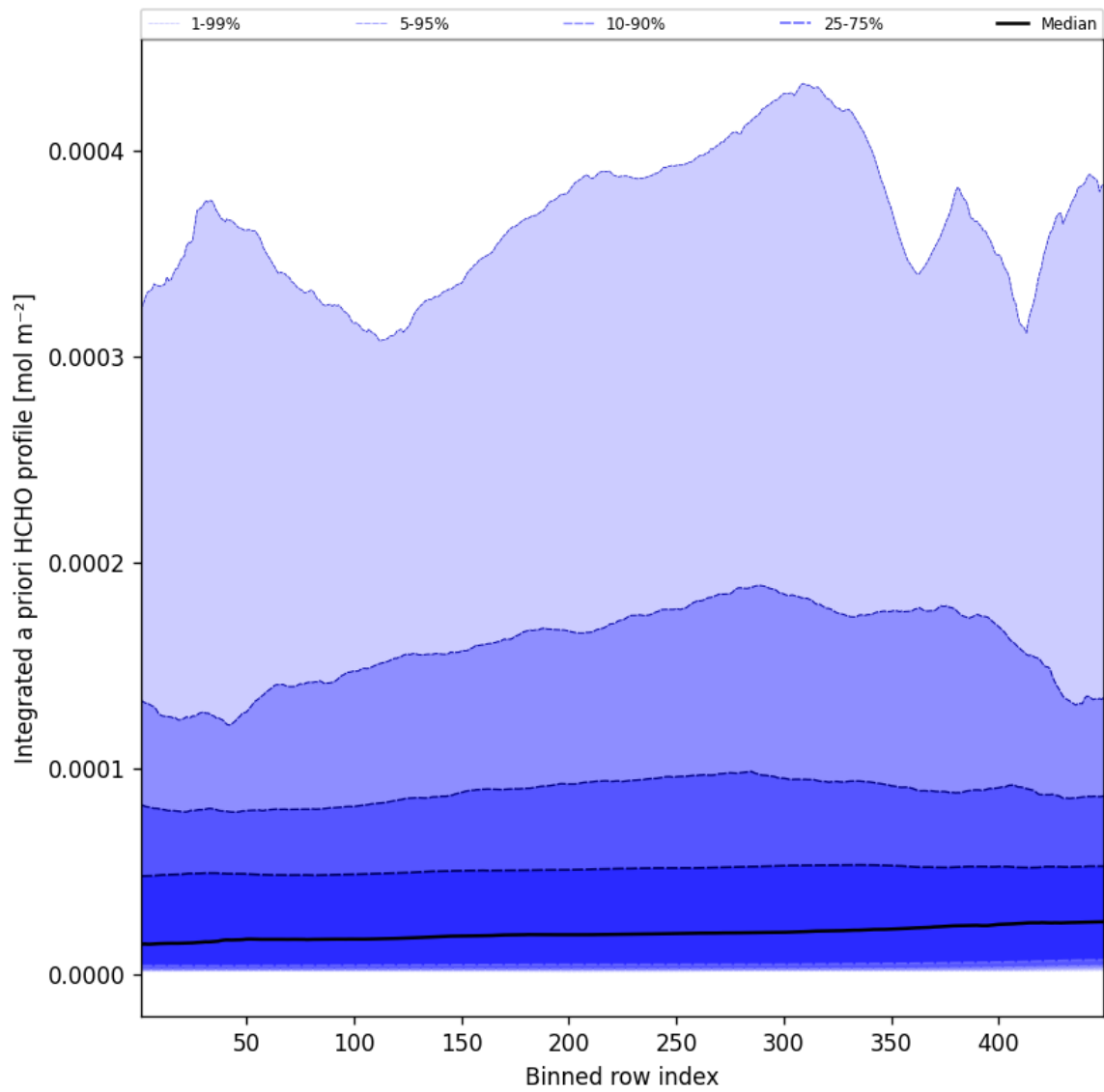
Figure 55: Along track statistics of "Integrated a priori HCHO profile" for 2025-01-27 to 2025-01-28
