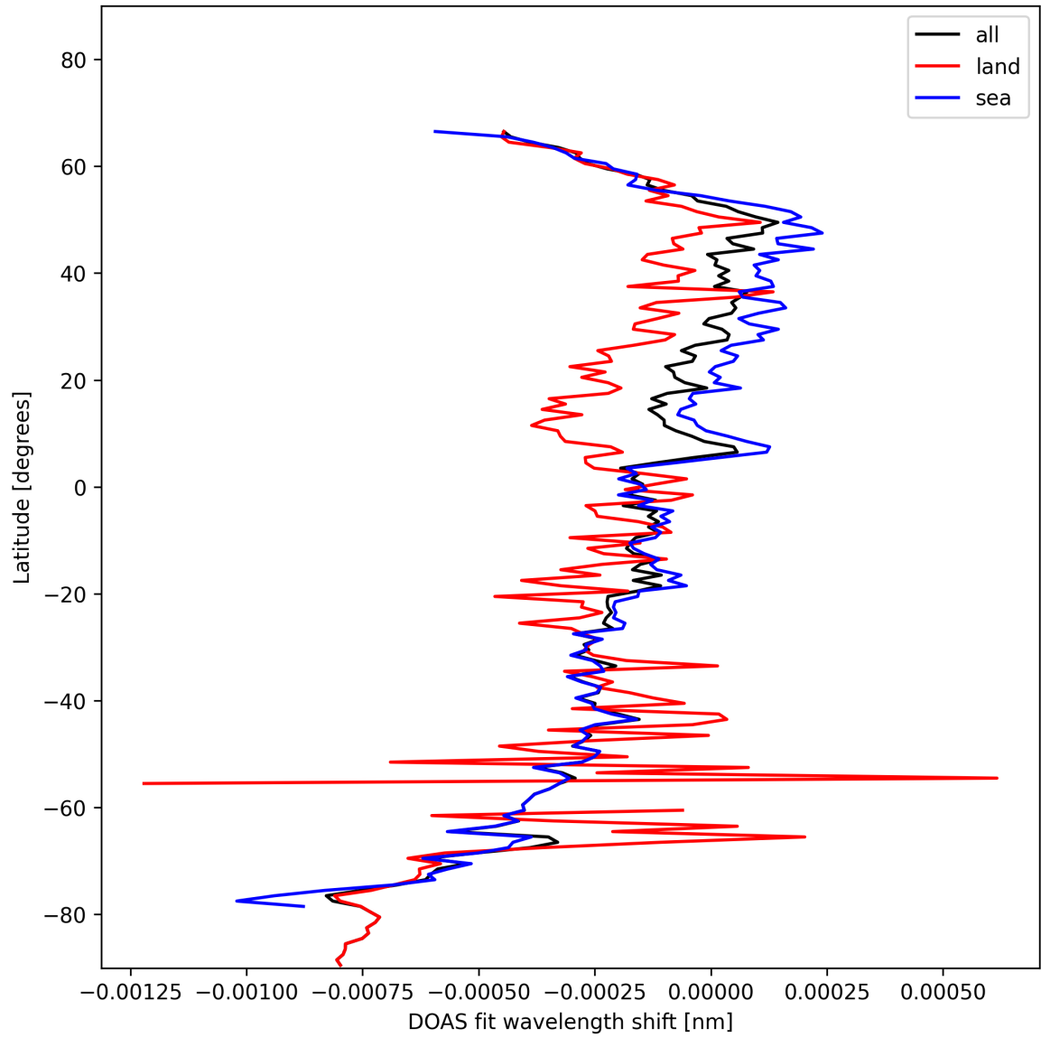
Figure 28: Zonal average of “DOAS fit wavelength shift” for 2025-01-27 to 2025-01-28.
