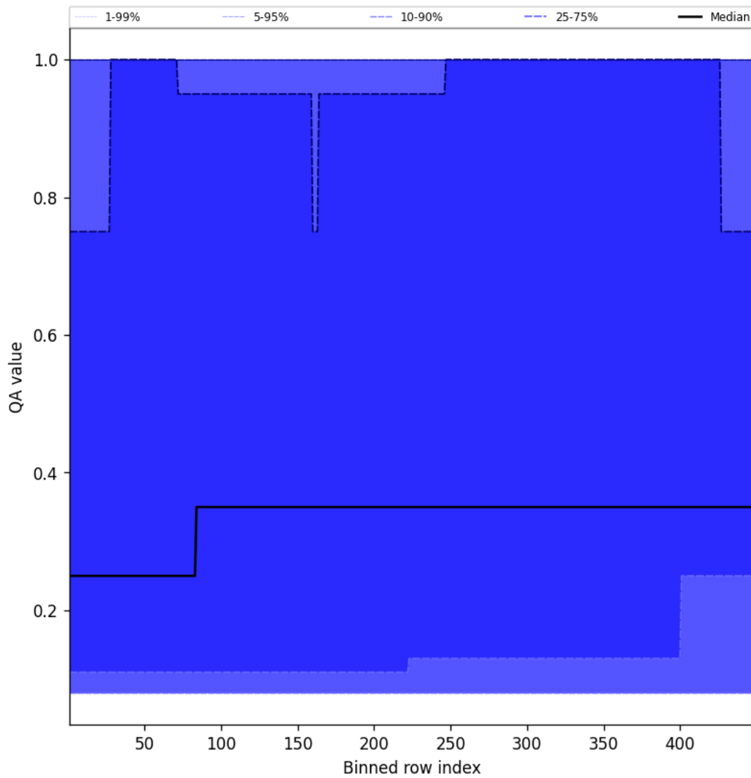
Figure 46: Along track statistics of “QA value” for 2025-01-27 to 2025-01-28
