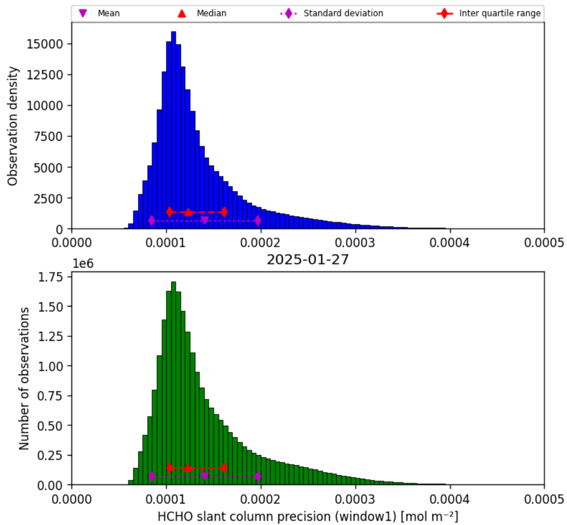
Figure 37: Histogram of “HCHO slant column precision (window1)” for 2025-01-27 to 2025-01-28
