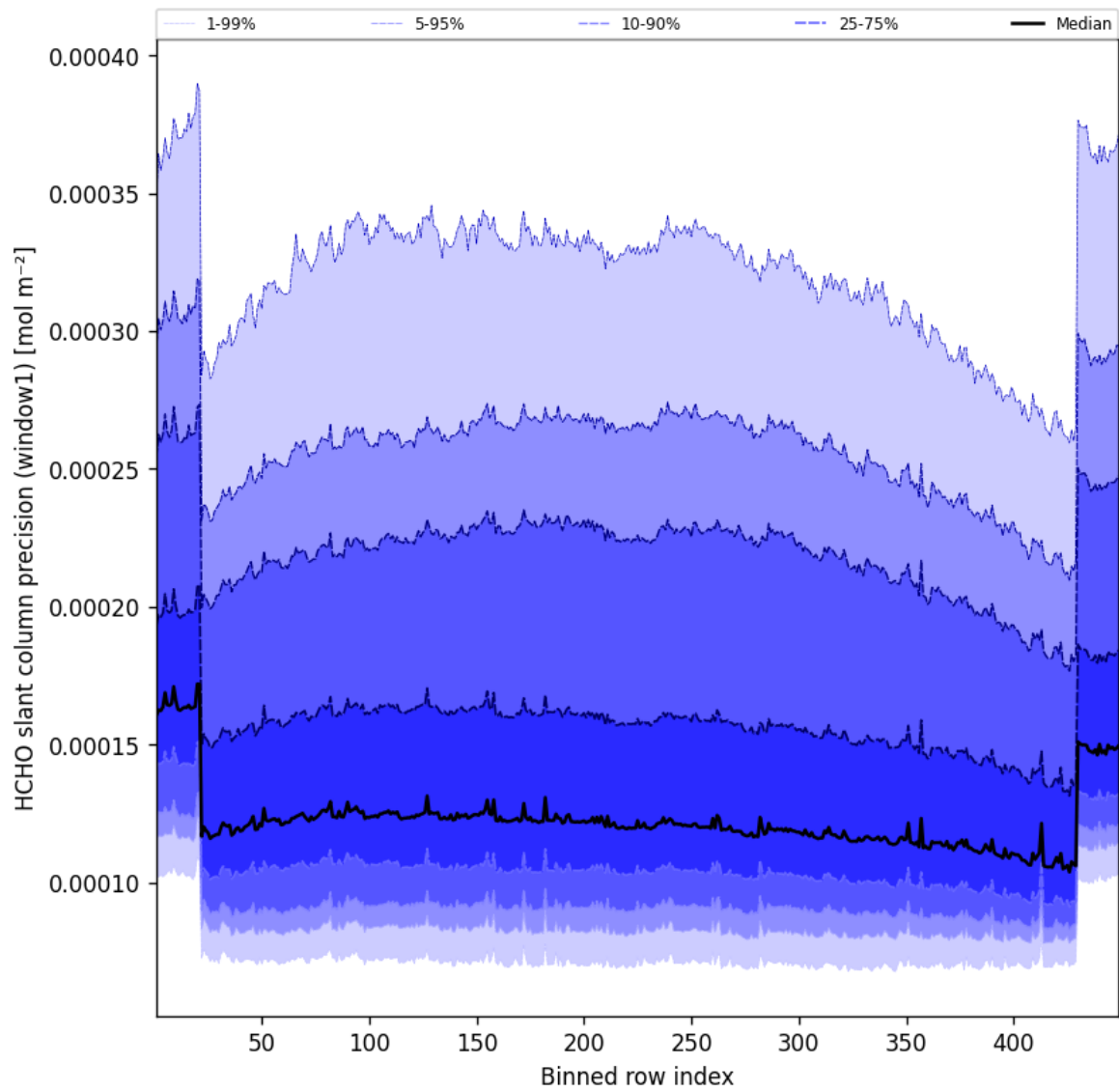
Figure 51: Along track statistics of “HCHO slant column precision (window1)” for 2025-01-27 to 2025-01-28
