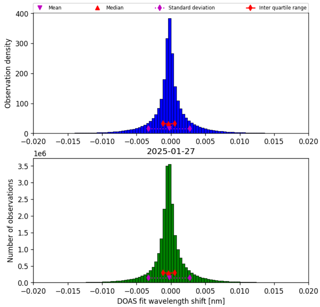
Figure 42: Histogram of “DOAS fit wavelength shift” for 2025-01-27 to 2025-01-28
