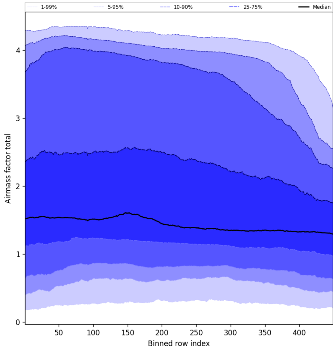
Figure 52: Along track statistics of “Airmass factor total” for 2025-01-27 to 2025-01-28
