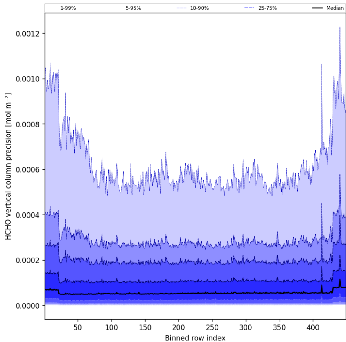
Figure 48: Along track statistics of “HCHO vertical column precision” for 2025-01-27 to 2025-01-28
