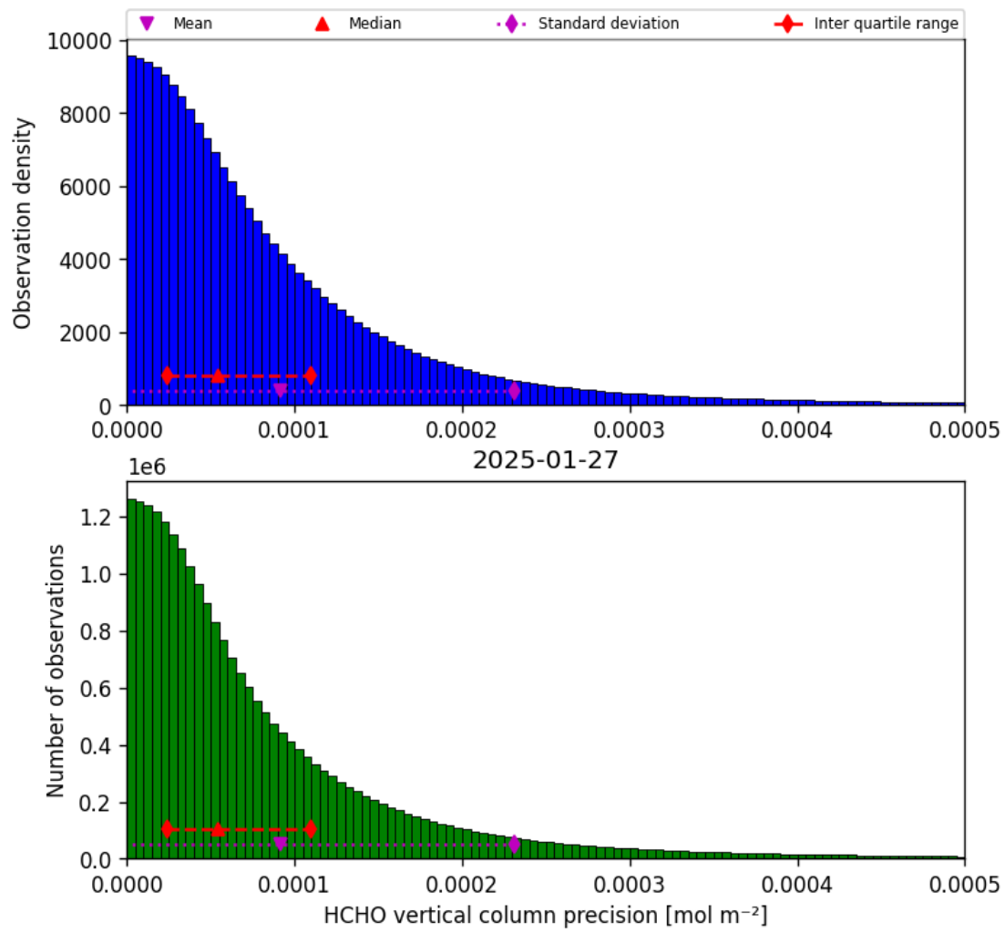
Figure 34: Histogram of “HCHO vertical column precision” for 2025-01-27 to 2025-01-28
