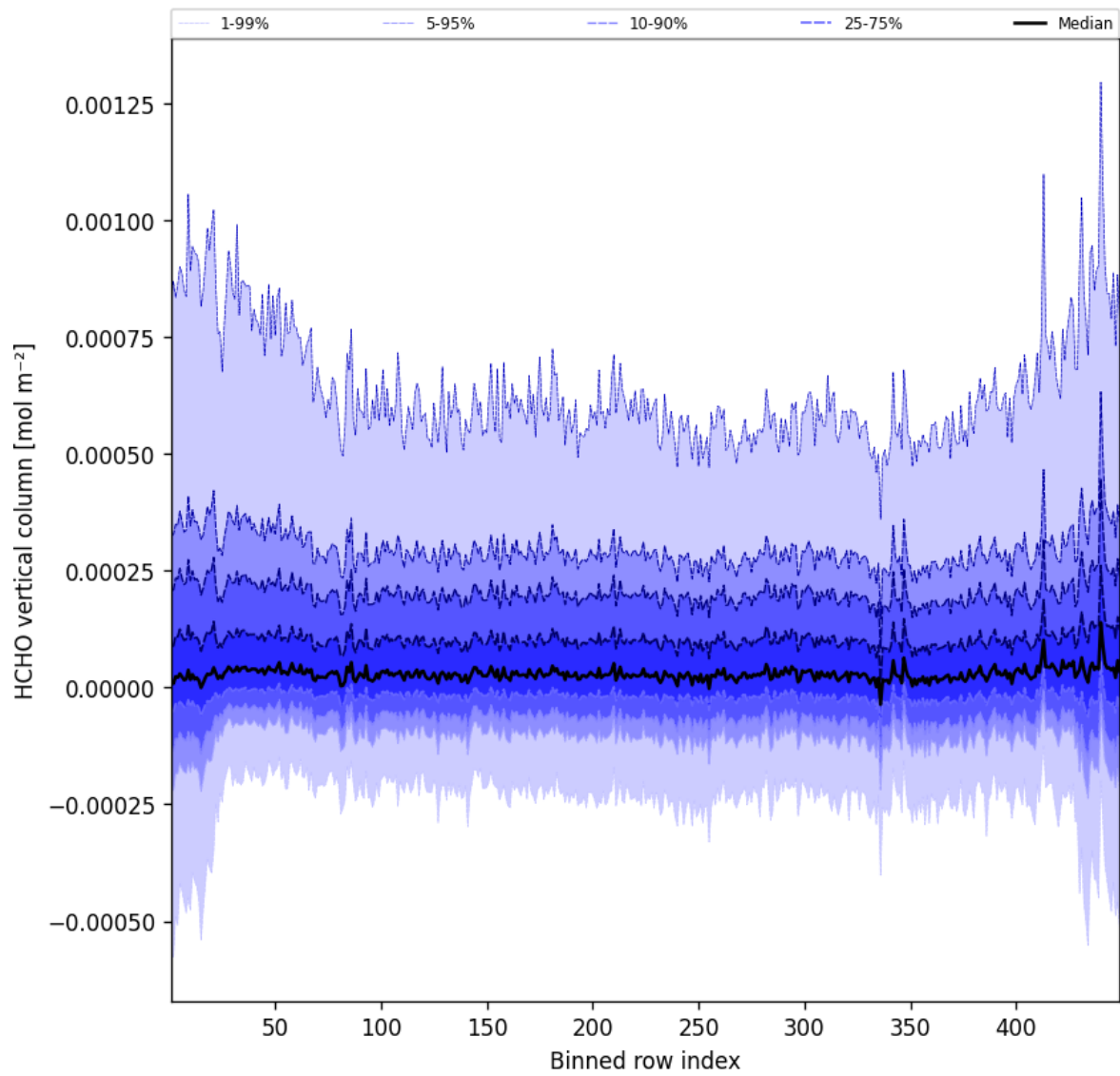
Figure 47: Along track statistics of “HCHO vertical column” for 2025-01-27 to 2025-01-28
