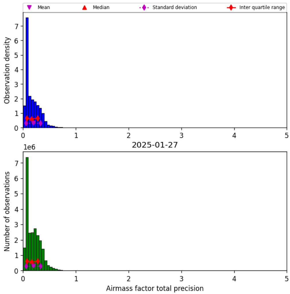
Figure 39: Histogram of “Airmass factor total precision” for 2025-01-27 to 2025-01-28
