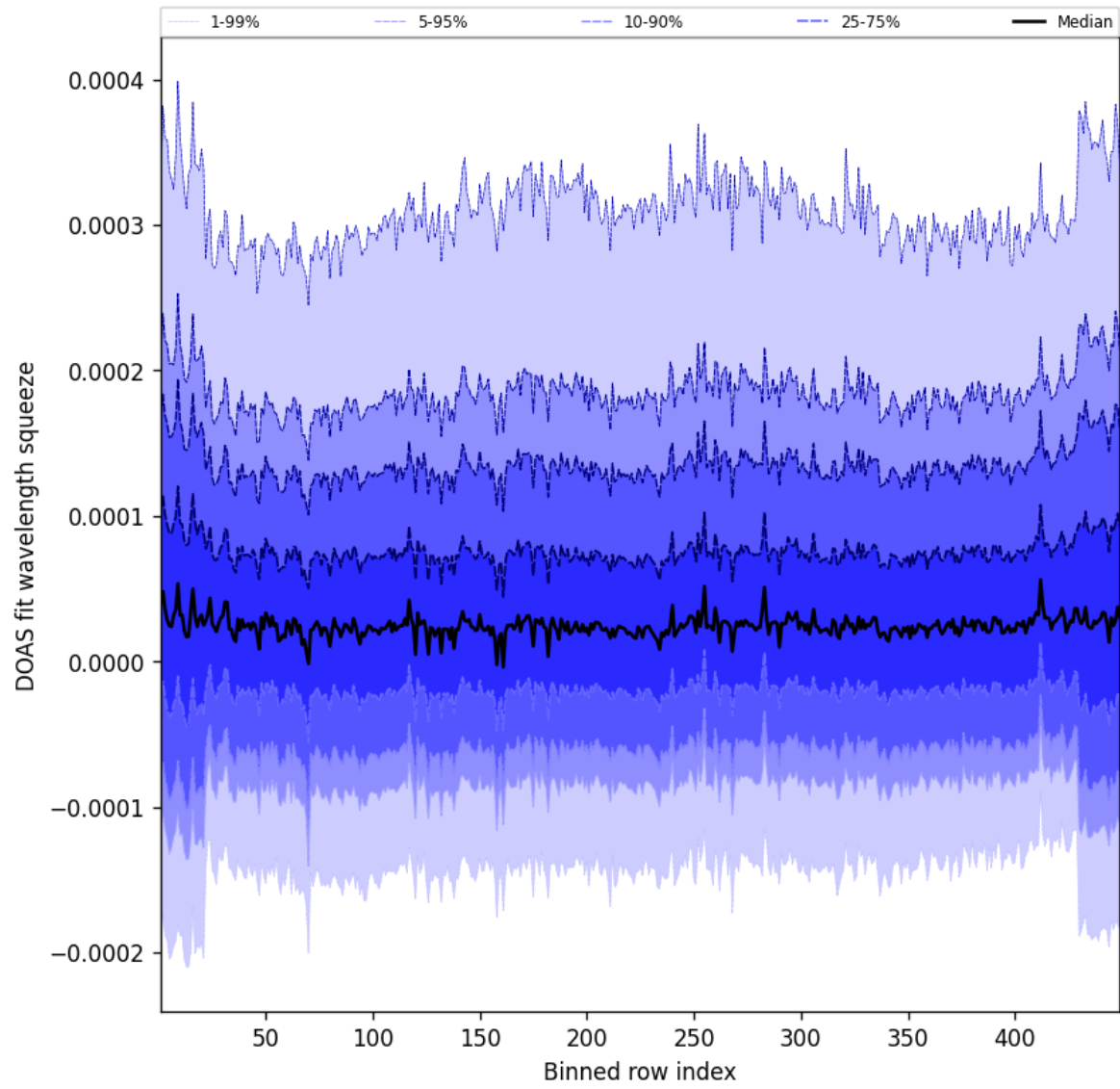
Figure 57: Along track statistics of “DOAS fit wavelength squeeze” for 2025-01-27 to 2025-01-28
