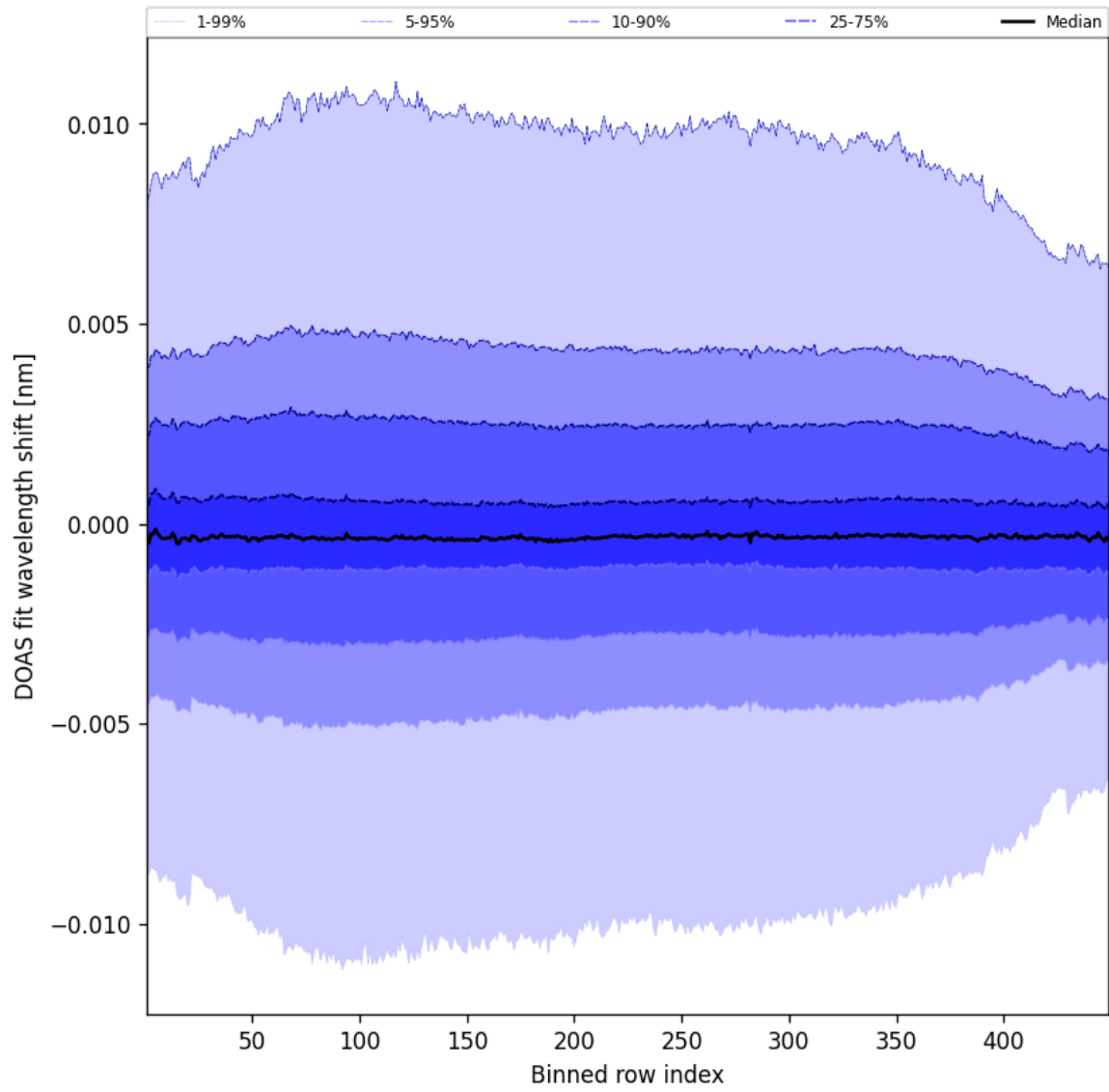
Figure 56: Along track statistics of “DOAS fit wavelength shift” for 2025-01-27 to 2025-01-28
