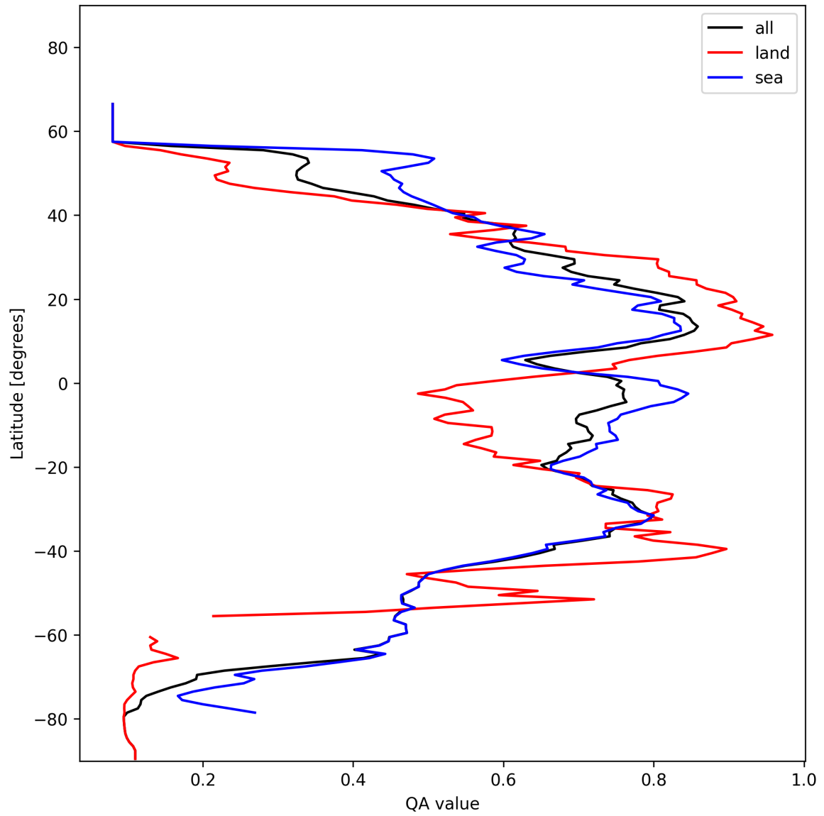
Figure 18: Zonal average of “QA value” for 2025-01-27 to 2025-01-28.
