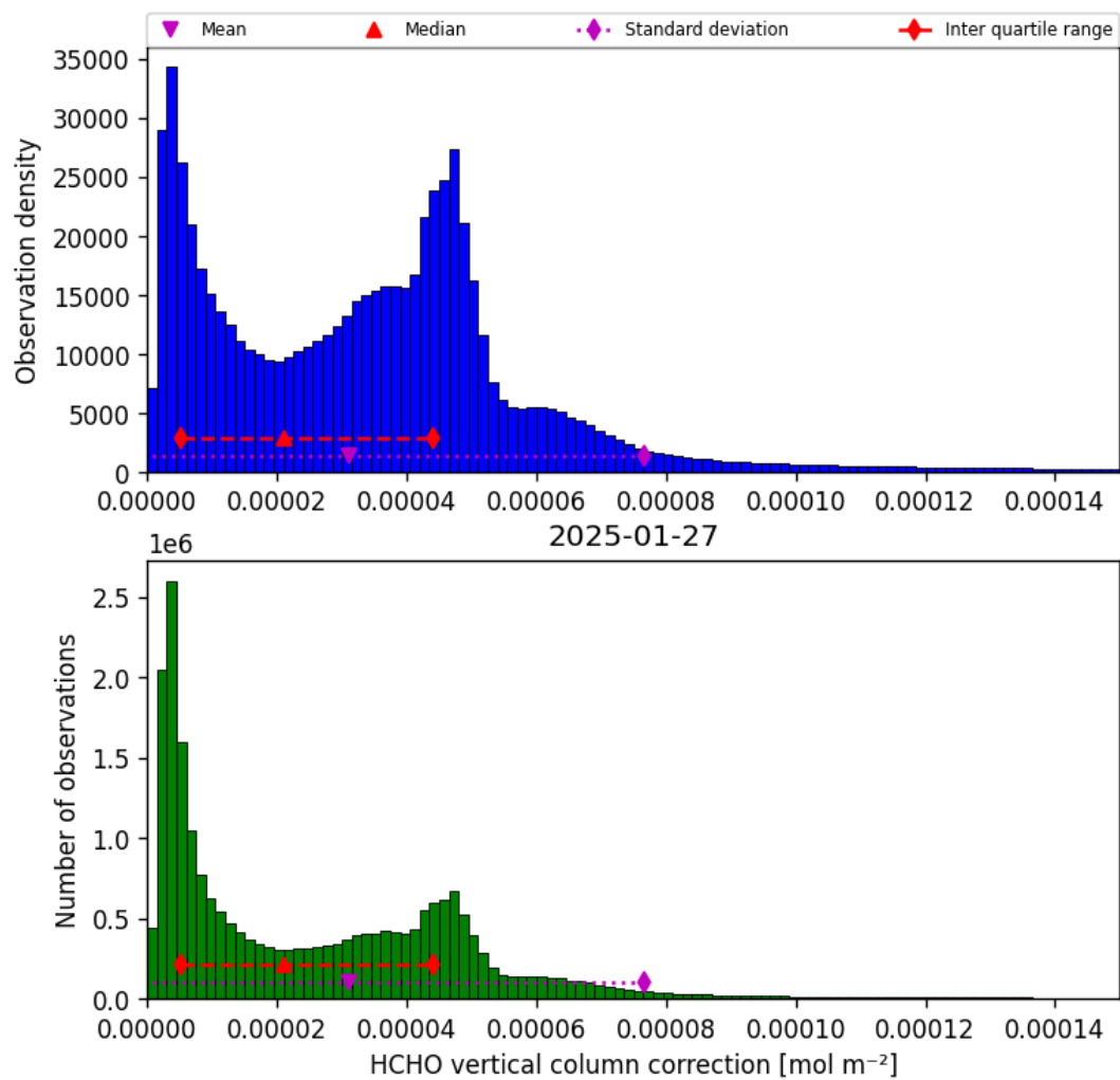
Figure 35: Histogram of “HCHO vertical column correction” for 2025-01-27 to 2025-01-28
