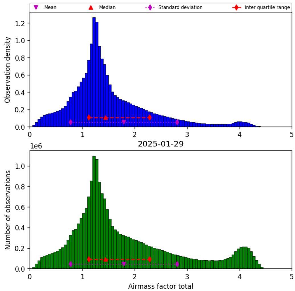
Figure 38: Histogram of “Airmass factor total” for 2025-01-29 to 2025-01-30
