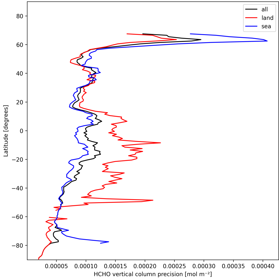
Figure 20: Zonal average of “HCHO vertical column precision” for 2025-01-29 to 2025-01-30.
