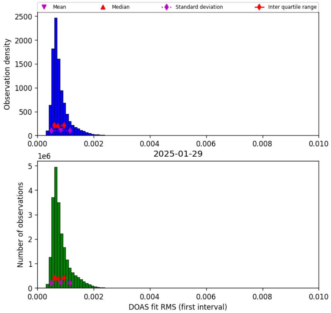
Figure 44: Histogram of “DOAS fit RMS (first interval)” for 2025-01-29 to 2025-01-30
