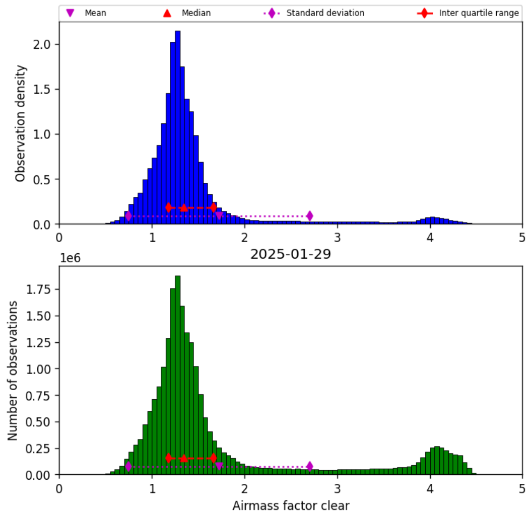
Figure 40: Histogram of “Airmass factor clear” for 2025-01-29 to 2025-01-30
