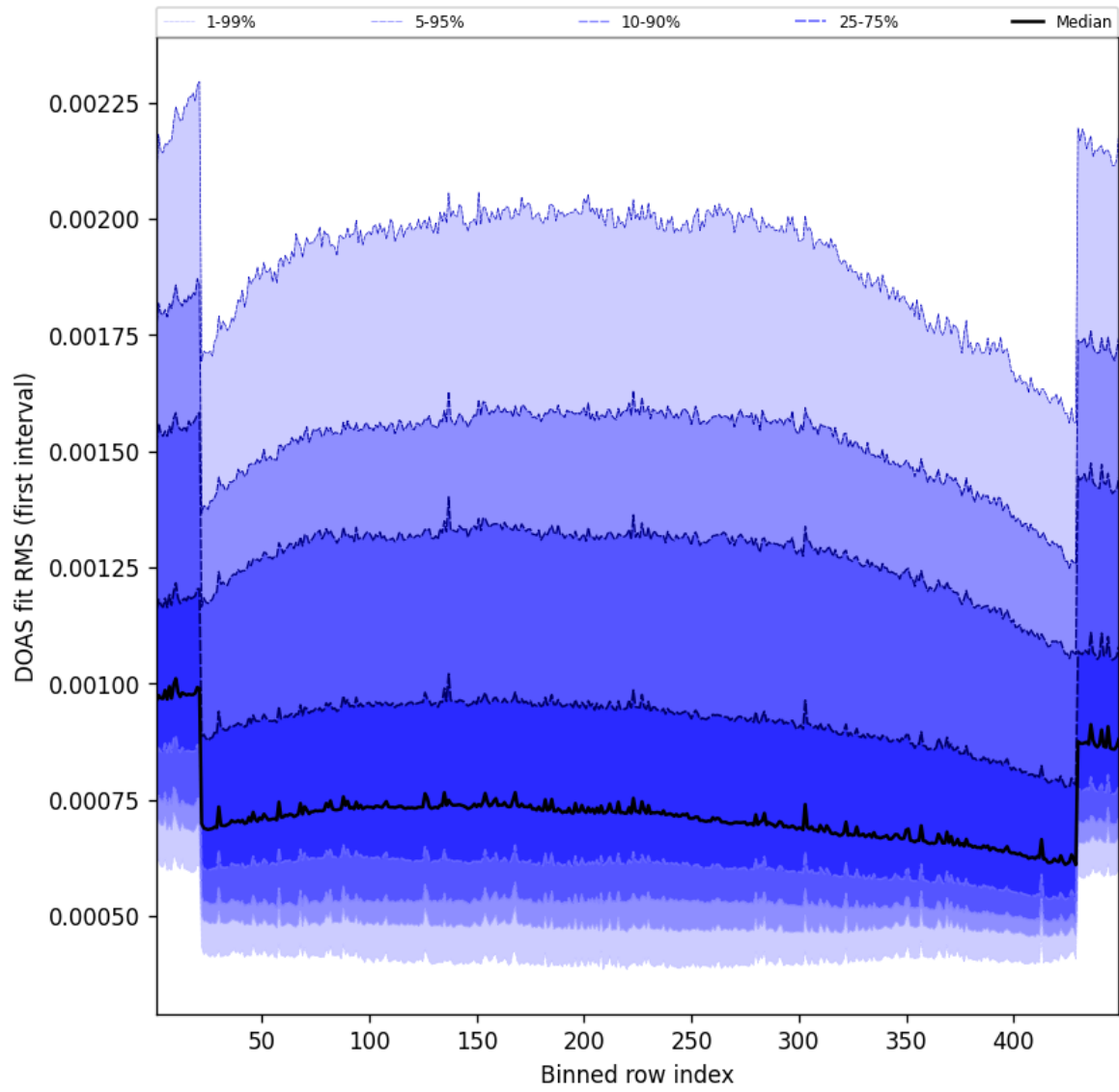
Figure 58: Along track statistics of “DOAS fit RMS (first interval)” for 2025-01-29 to 2025-01-30
