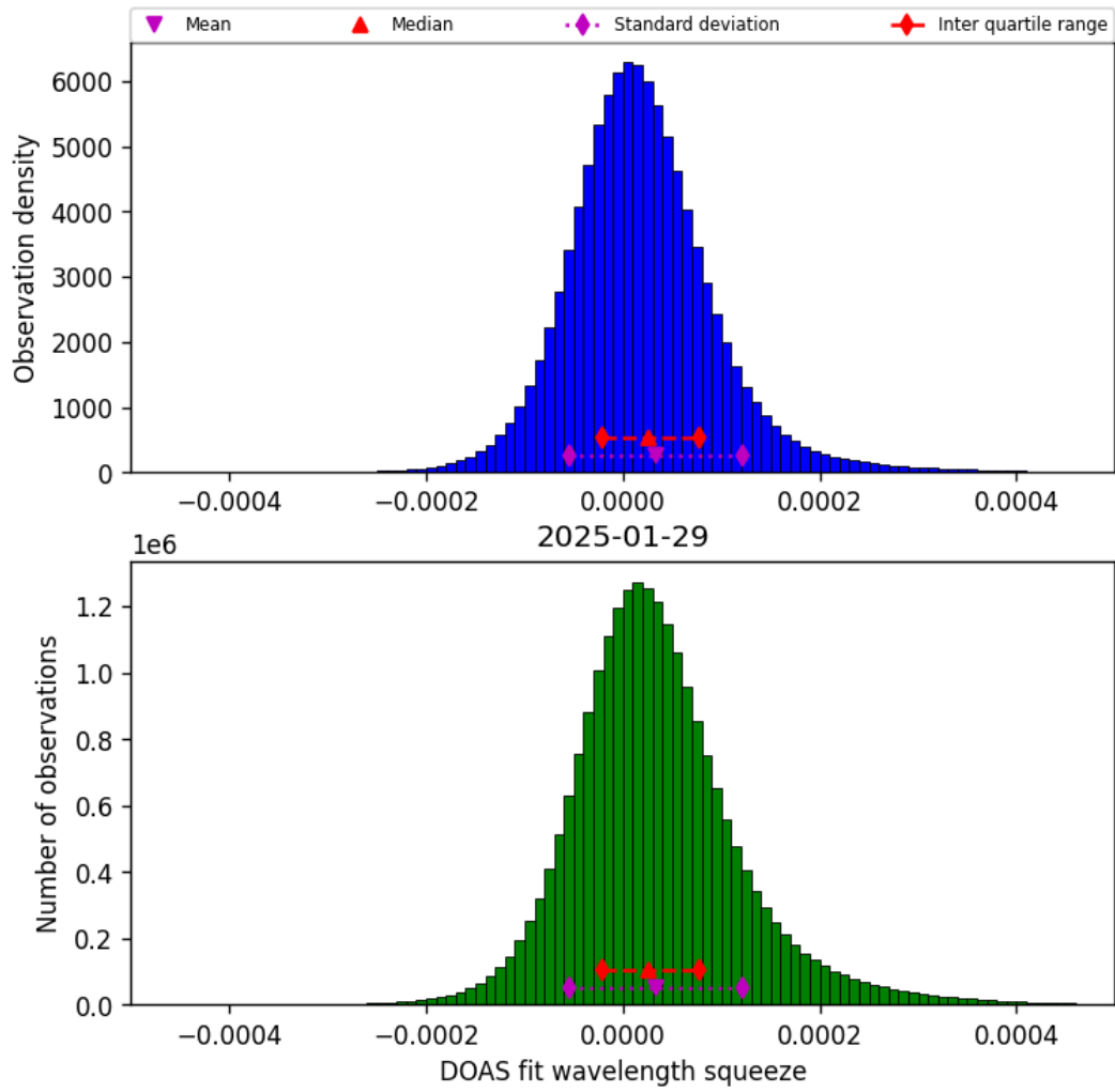
Figure 43: Histogram of “DOAS fit wavelength squeeze” for 2025-01-29 to 2025-01-30
