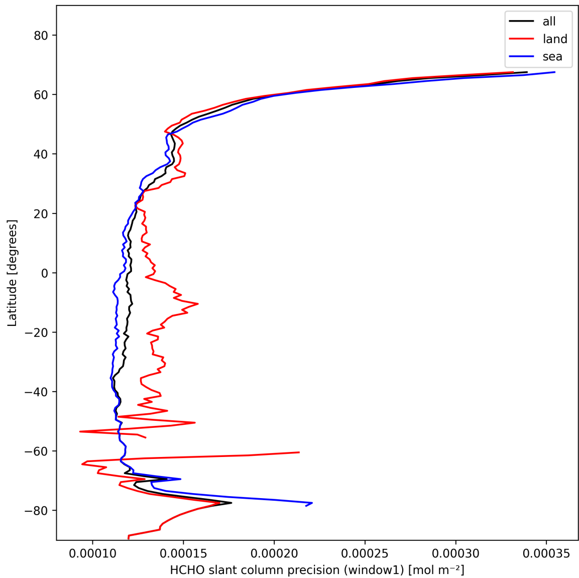
Figure 23: Zonal average of “HCHO slant column precision (window1)” for 2025-01-29 to 2025-01-30.
