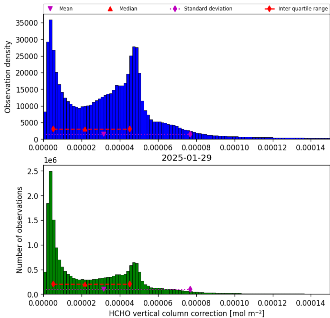
Figure 35: Histogram of “HCHO vertical column correction” for 2025-01-29 to 2025-01-30
