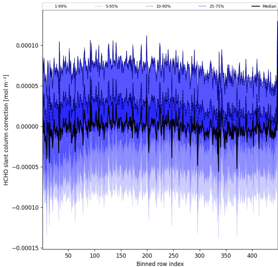
Figure 59: Along track statistics of “HCHO slant column correction” for 2025-01-29 to 2025-01-30
