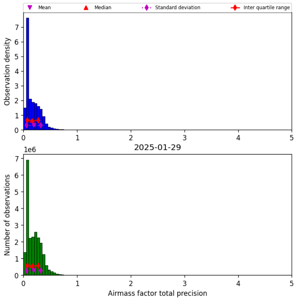
Figure 39: Histogram of “Airmass factor total precision” for 2025-01-29 to 2025-01-30
