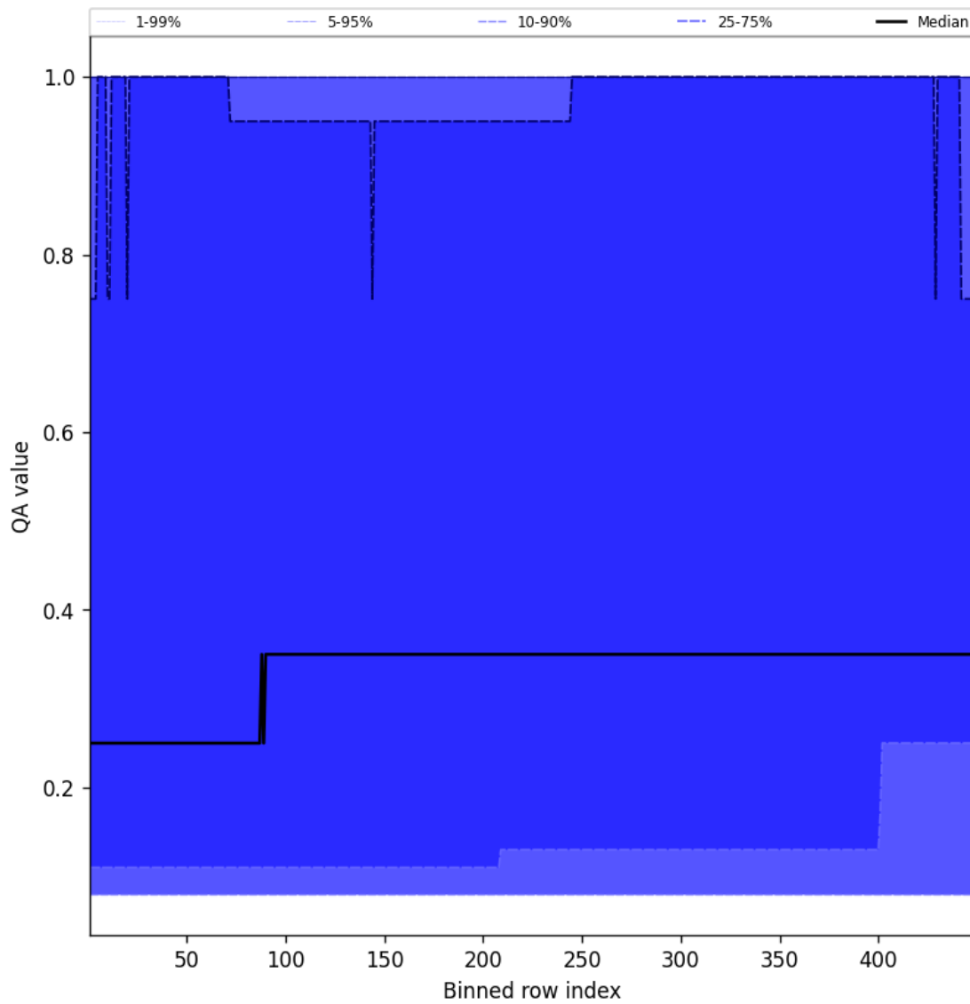
Figure 46: Along track statistics of “QA value” for 2025-01-29 to 2025-01-30
