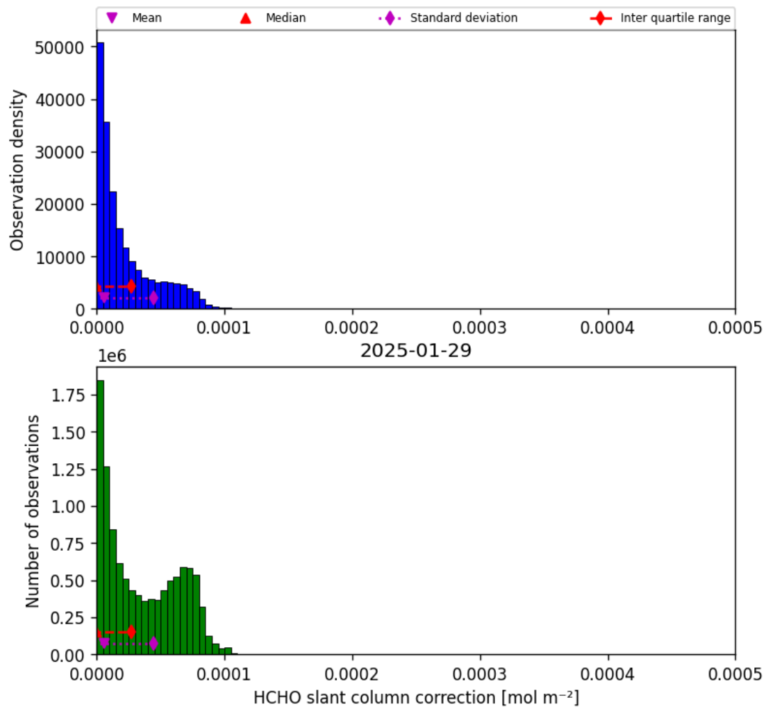
Figure 45: Histogram of “HCHO slant column correction” for 2025-01-29 to 2025-01-30
