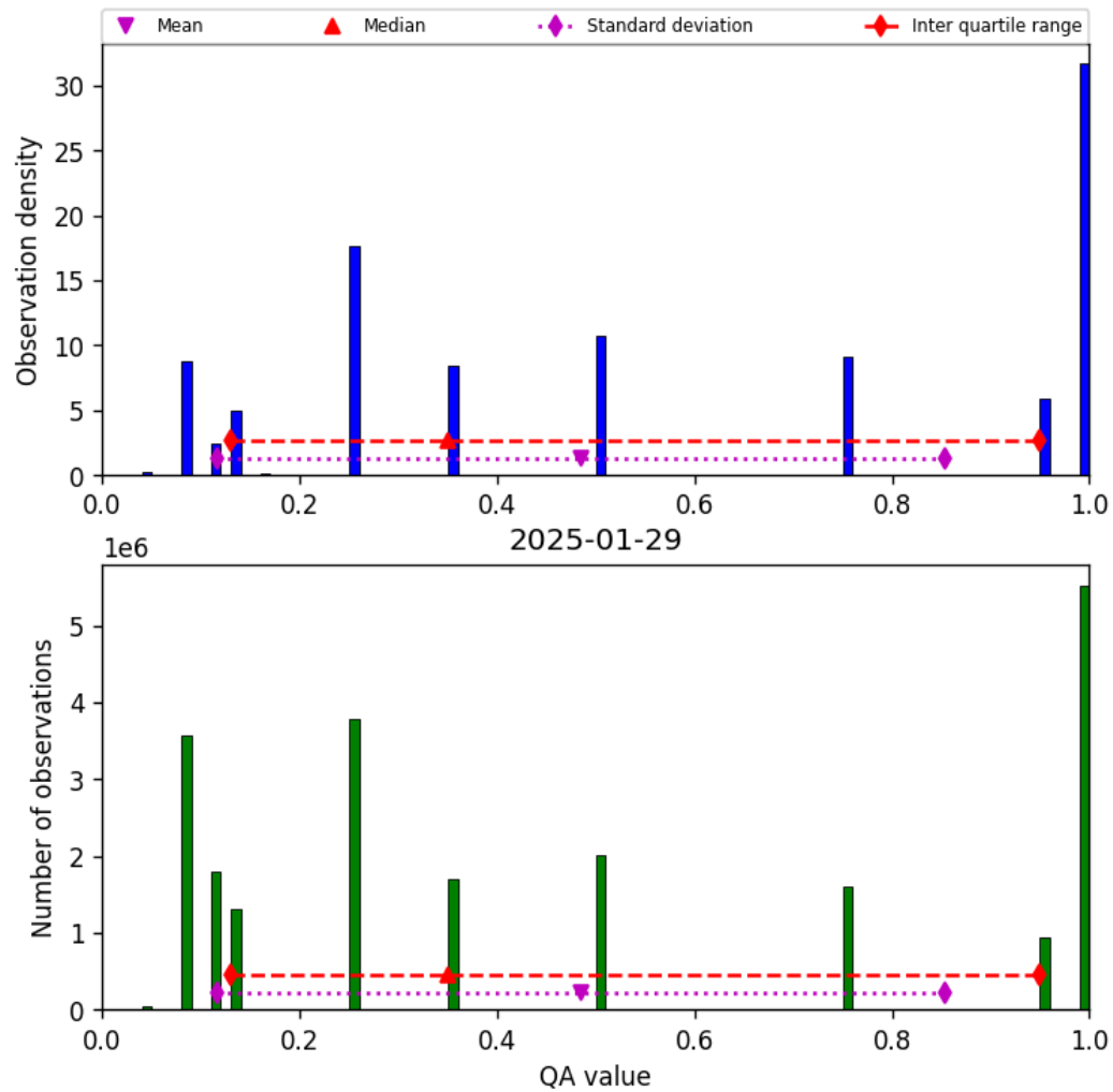
Figure 32: Histogram of “QA value” for 2025-01-29 to 2025-01-30
