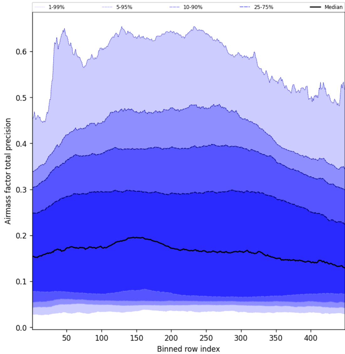
Figure 53: Along track statistics of “Airmass factor total precision” for 2025-01-29 to 2025-01-30
