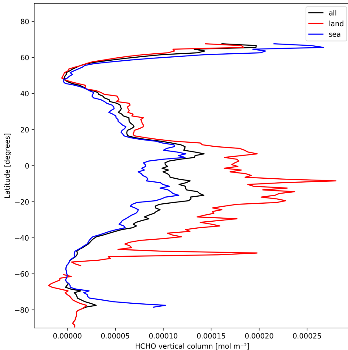
Figure 19: Zonal average of “HCHO vertical column” for 2025-01-29 to 2025-01-30.
