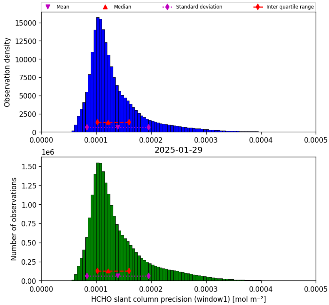
Figure 37: Histogram of “HCHO slant column precision (window1)” for 2025-01-29 to 2025-01-30
