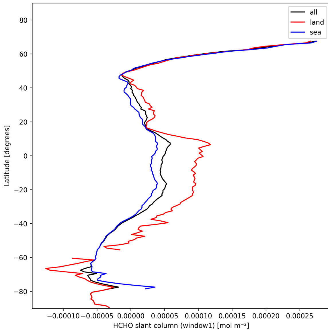
Figure 22: Zonal average of “HCHO slant column (window1)” for 2025-01-29 to 2025-01-30.
