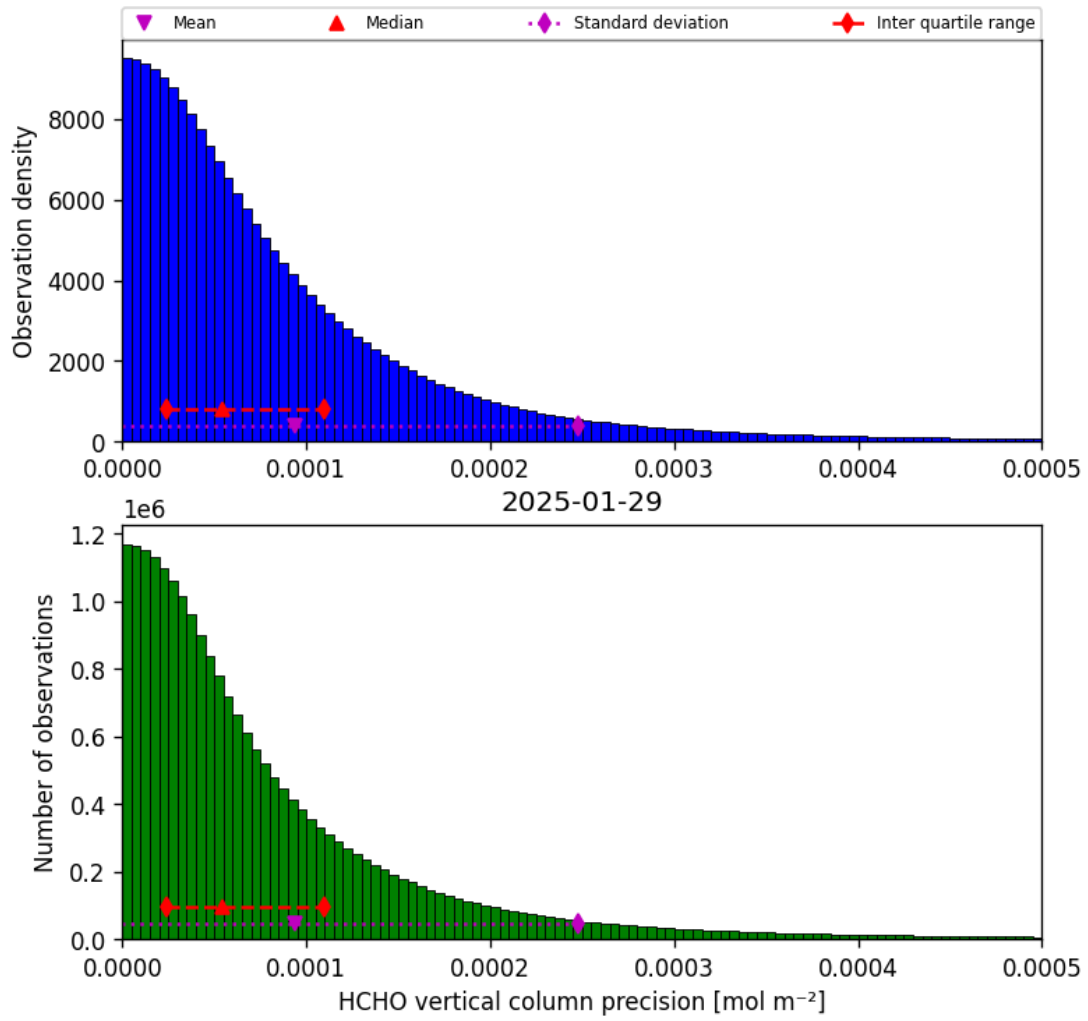
Figure 34: Histogram of “HCHO vertical column precision” for 2025-01-29 to 2025-01-30
