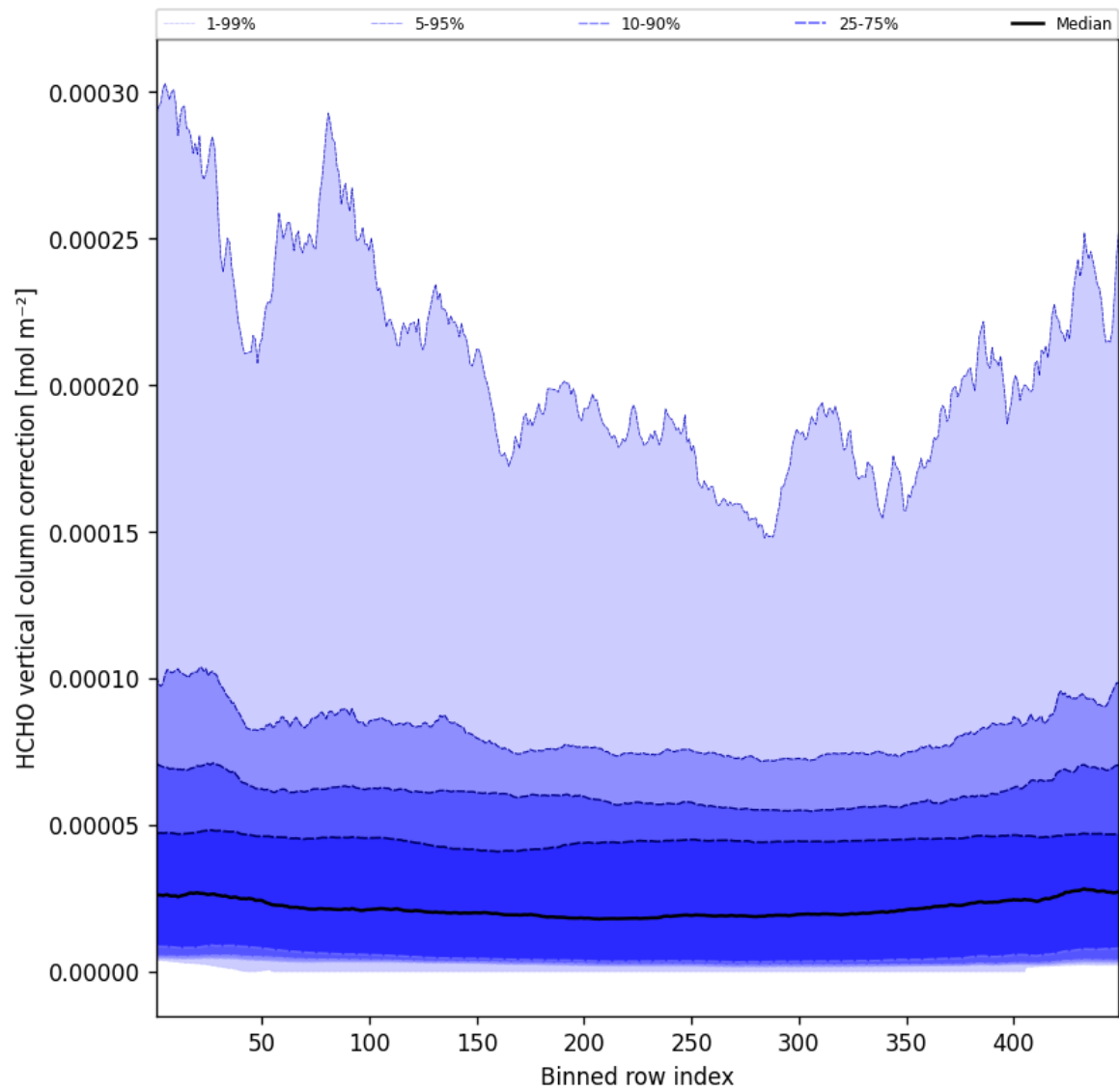
Figure 49: Along track statistics of “HCHO vertical column correction” for 2025-01-29 to 2025-01-30
