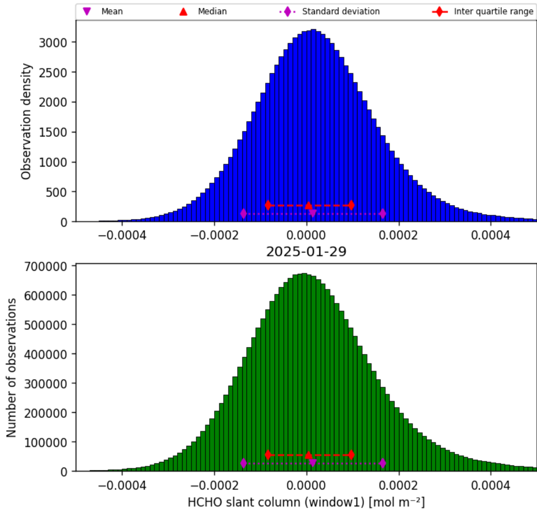
Figure 36: Histogram of “HCHO slant column (window1)” for 2025-01-29 to 2025-01-30
