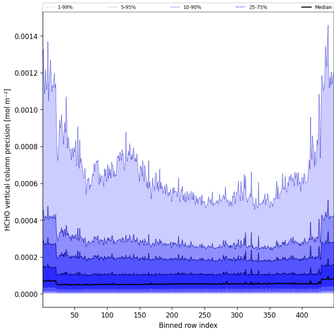
Figure 48: Along track statistics of “HCHO vertical column precision” for 2025-01-29 to 2025-01-30
