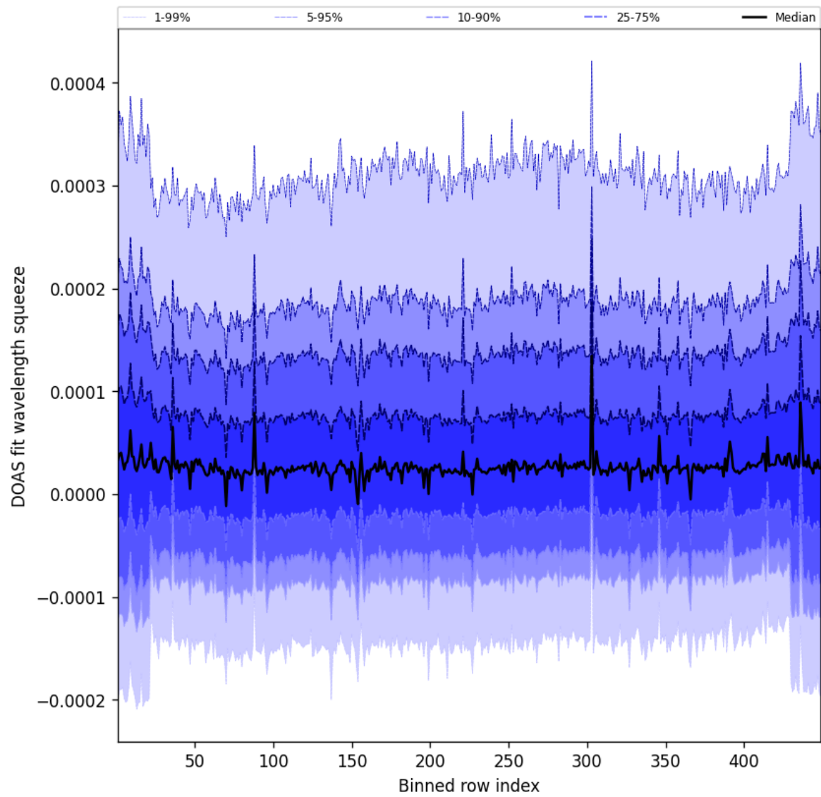
Figure 57: Along track statistics of “DOAS fit wavelength squeeze” for 2025-01-29 to 2025-01-30
