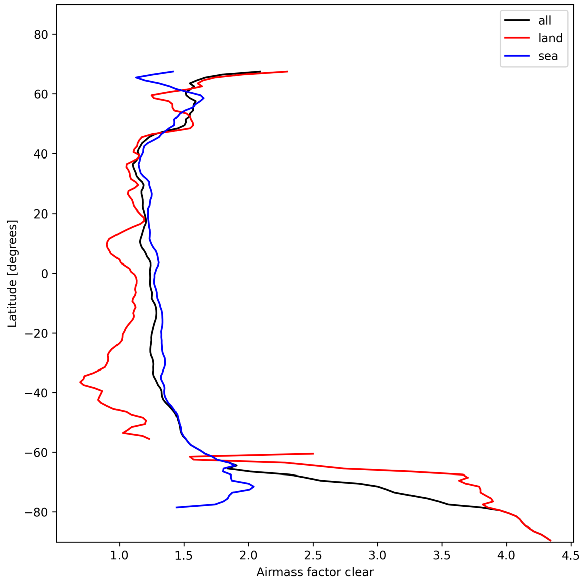
Figure 26: Zonal average of “Airmass factor clear” for 2025-01-29 to 2025-01-30.
