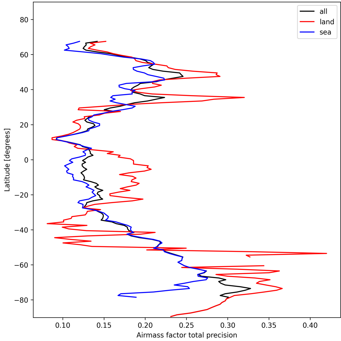
Figure 25: Zonal average of “Airmass factor total precision” for 2025-01-29 to 2025-01-30.
