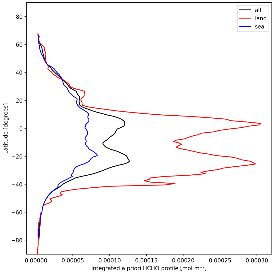
Figure 27: Zonal average of “Integrated a priori HCHO profile” for 2025-01-29 to 2025-01-30.
