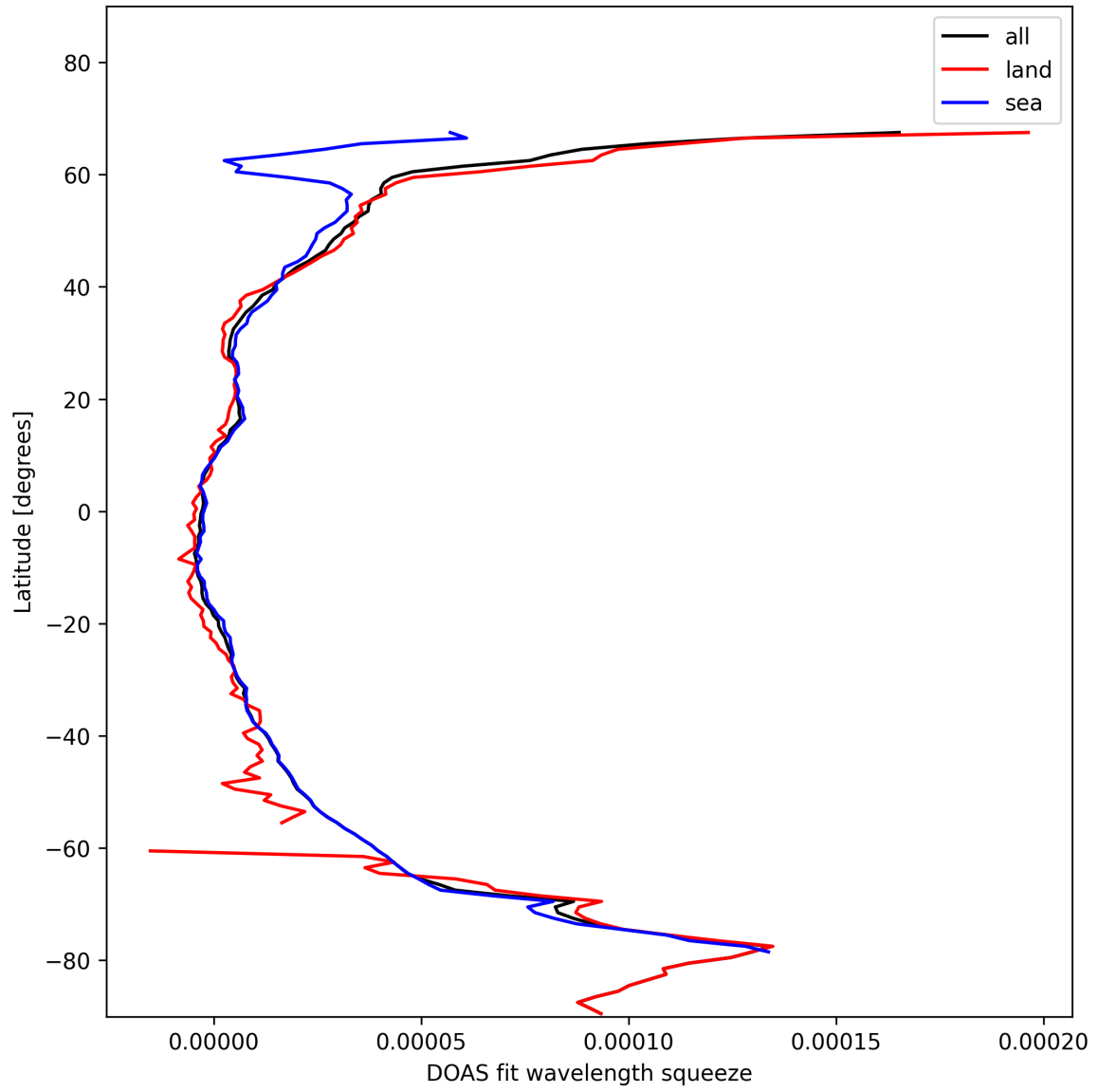
Figure 29: Zonal average of “DOAS fit wavelength squeeze” for 2025-01-29 to 2025-01-30.
