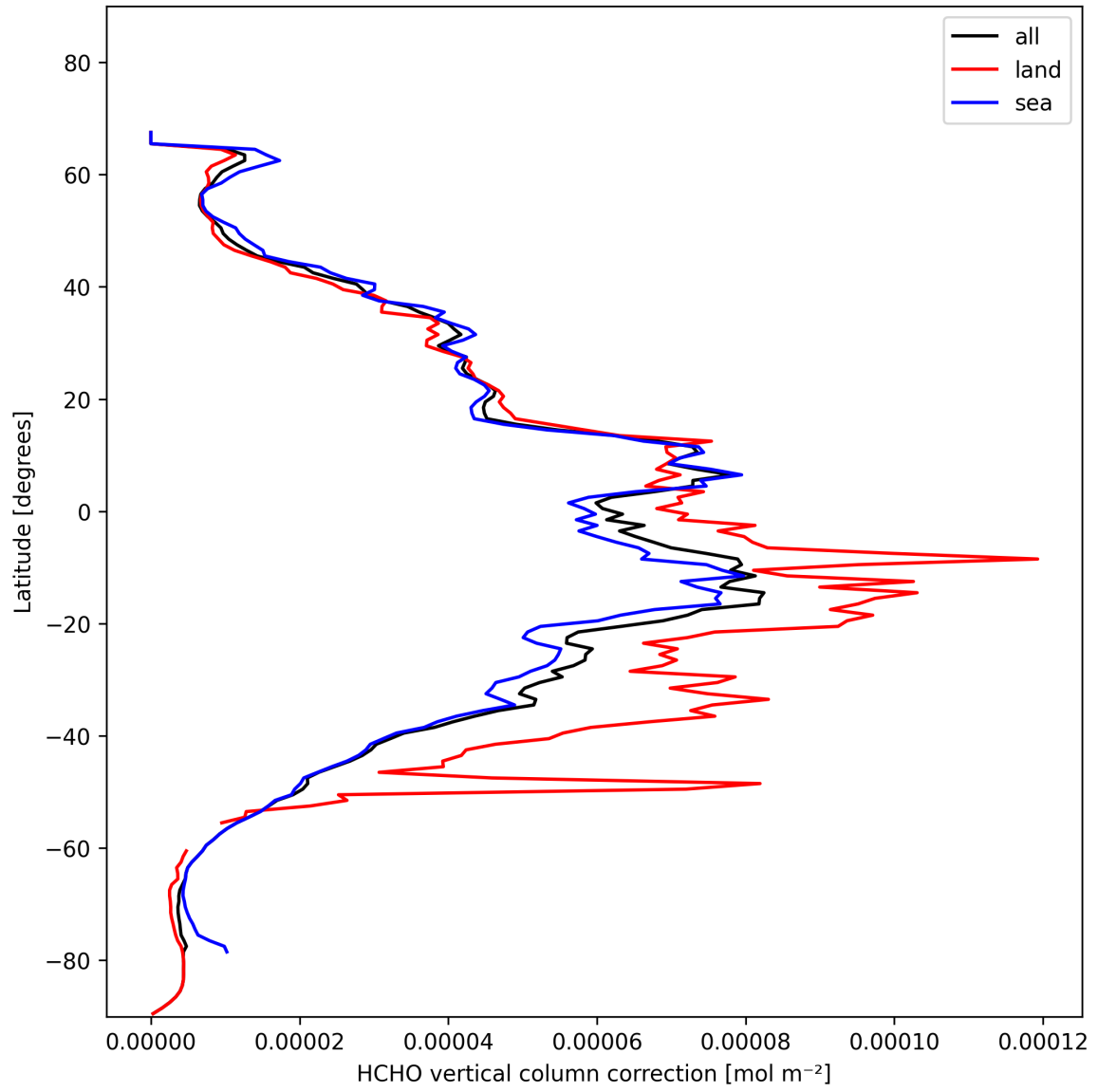
Figure 21: Zonal average of “HCHO vertical column correction” for 2025-01-29 to 2025-01-30.
