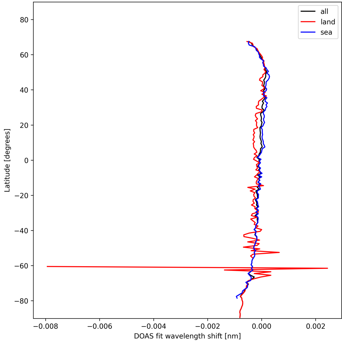
Figure 28: Zonal average of “DOAS fit wavelength shift” for 2025-01-29 to 2025-01-30.
