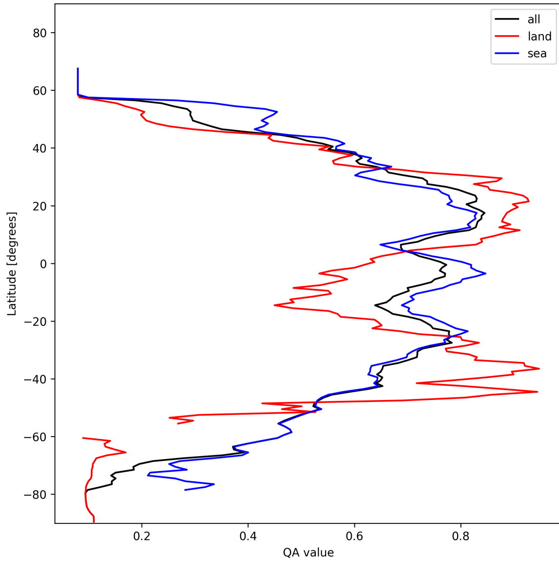
Figure 18: Zonal average of “QA value” for 2025-01-29 to 2025-01-30.
