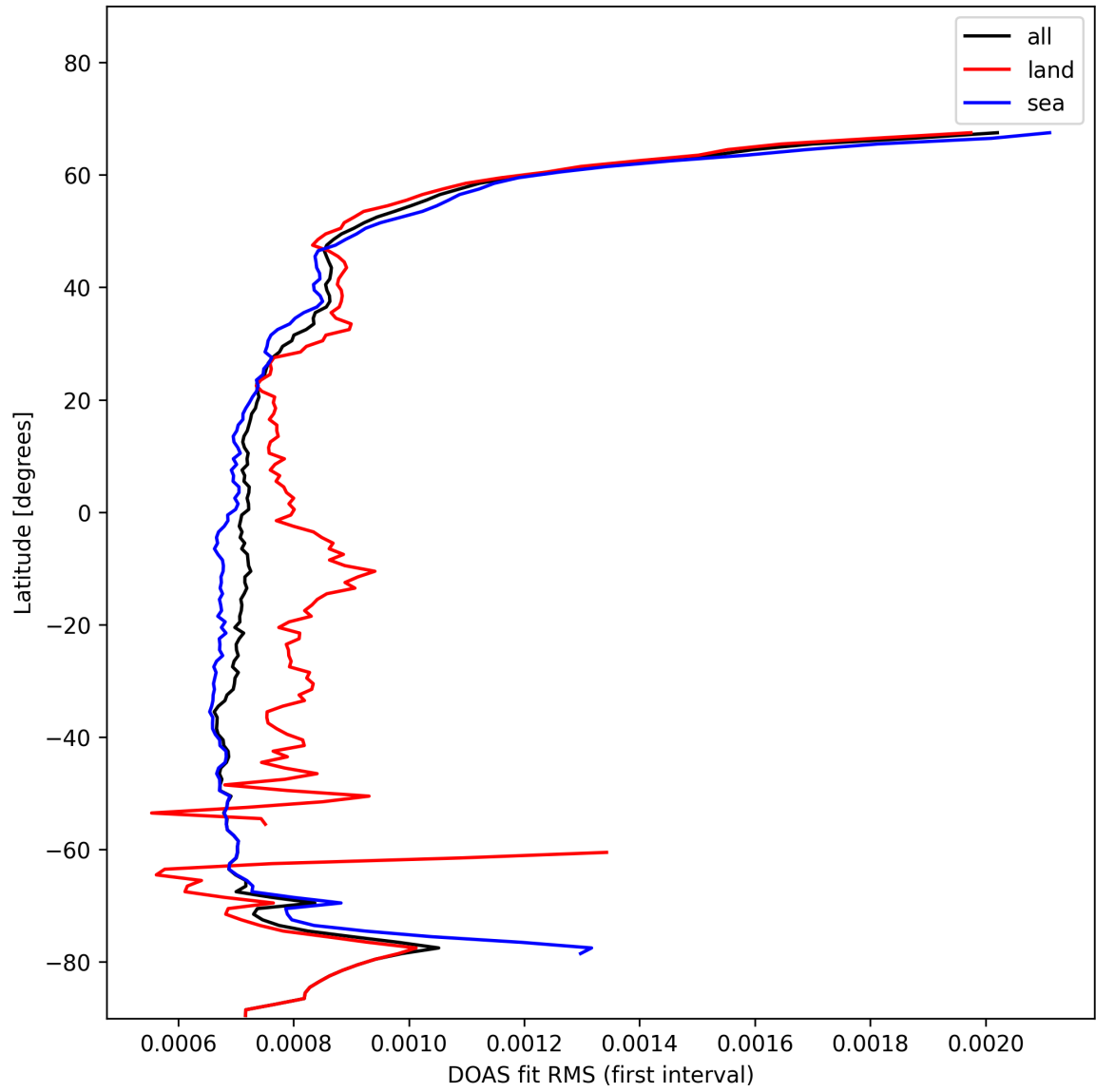
Figure 30: Zonal average of “DOAS fit RMS (first interval)” for 2025-01-29 to 2025-01-30.
