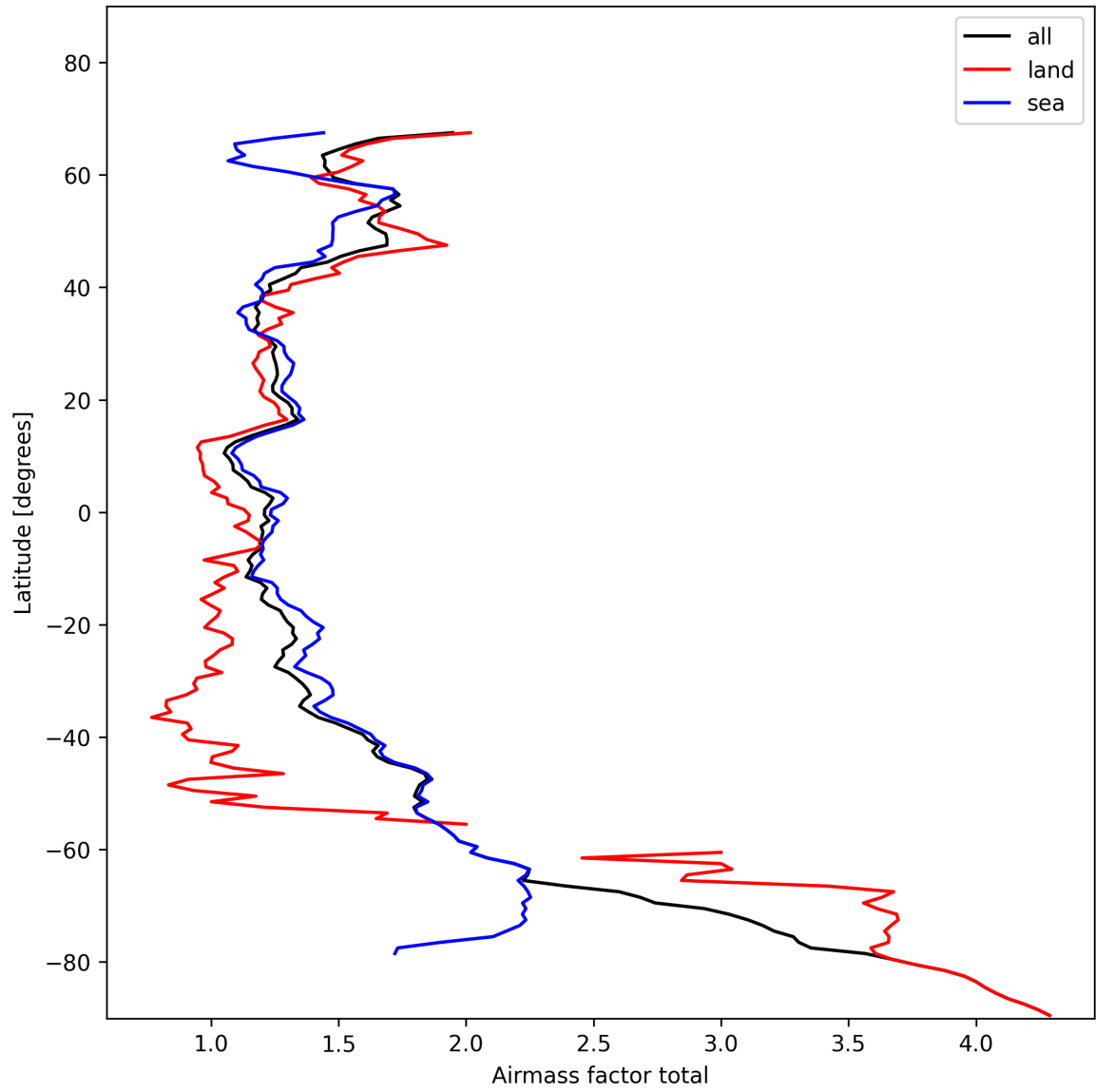
Figure 24: Zonal average of “Airmass factor total” for 2025-01-29 to 2025-01-30.
