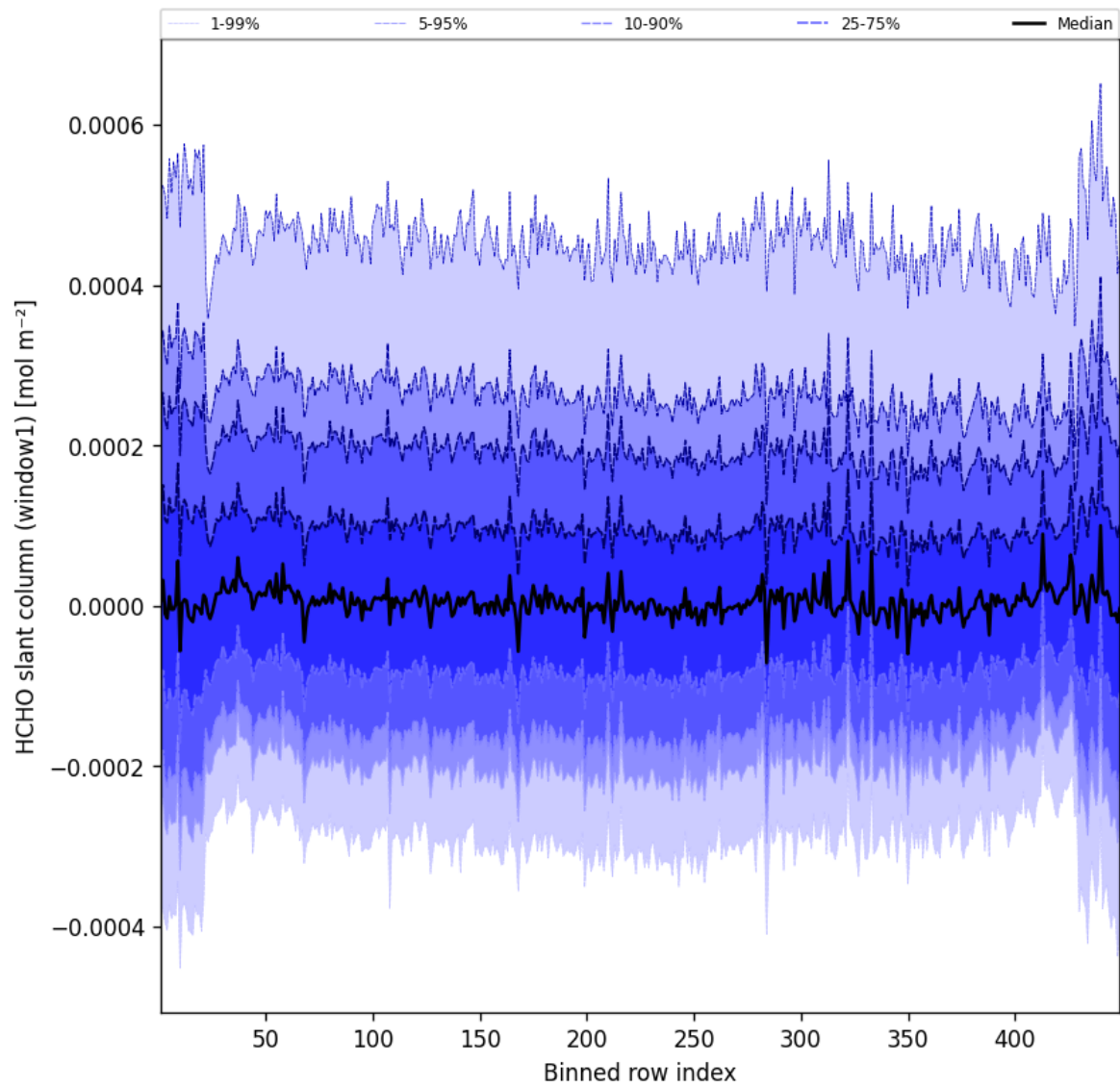
Figure 50: Along track statistics of “HCHO slant column (window1)” for 2025-01-29 to 2025-01-30
