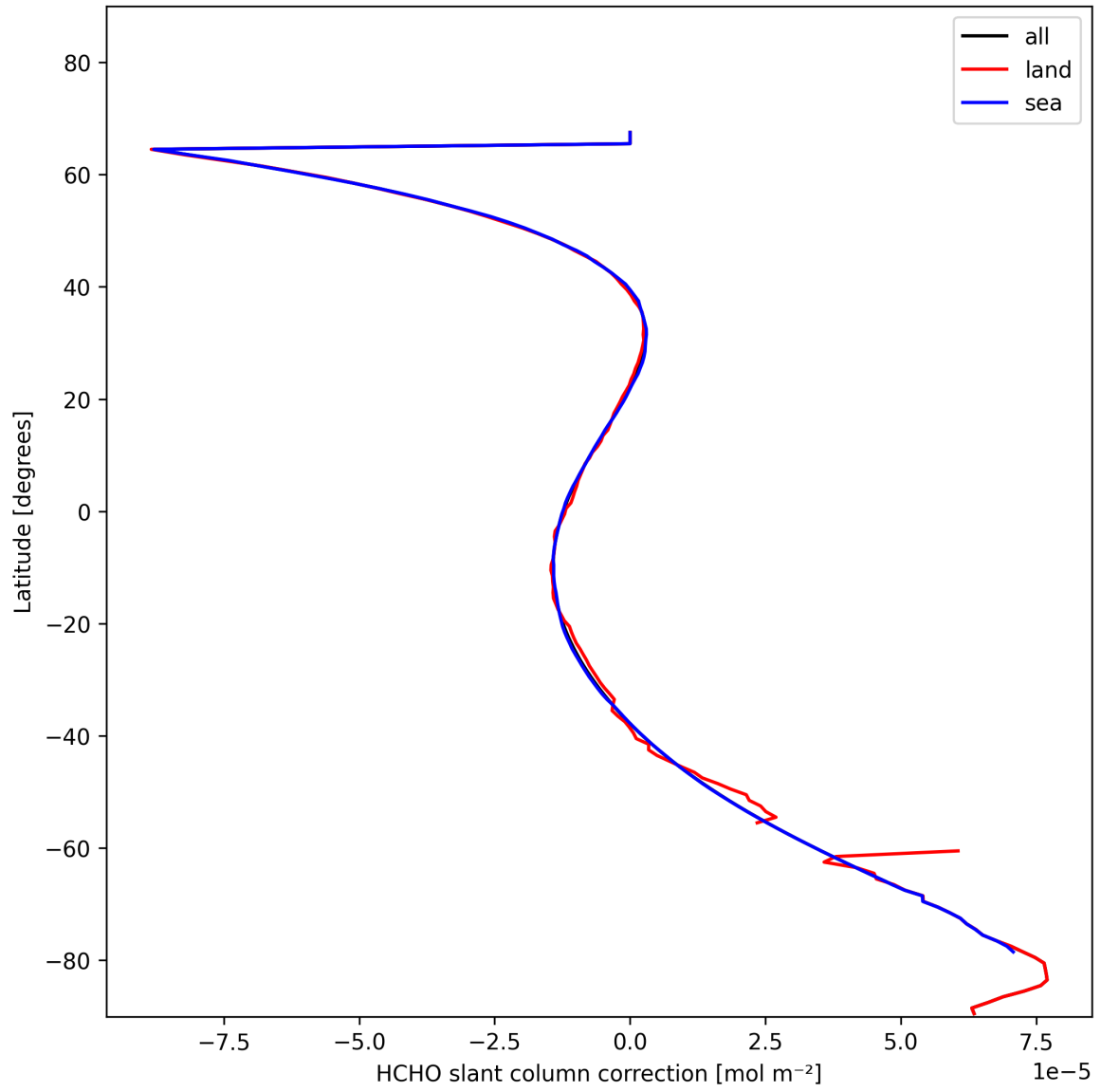
Figure 31: Zonal average of “HCHO slant column correction” for 2025-01-29 to 2025-01-30.
