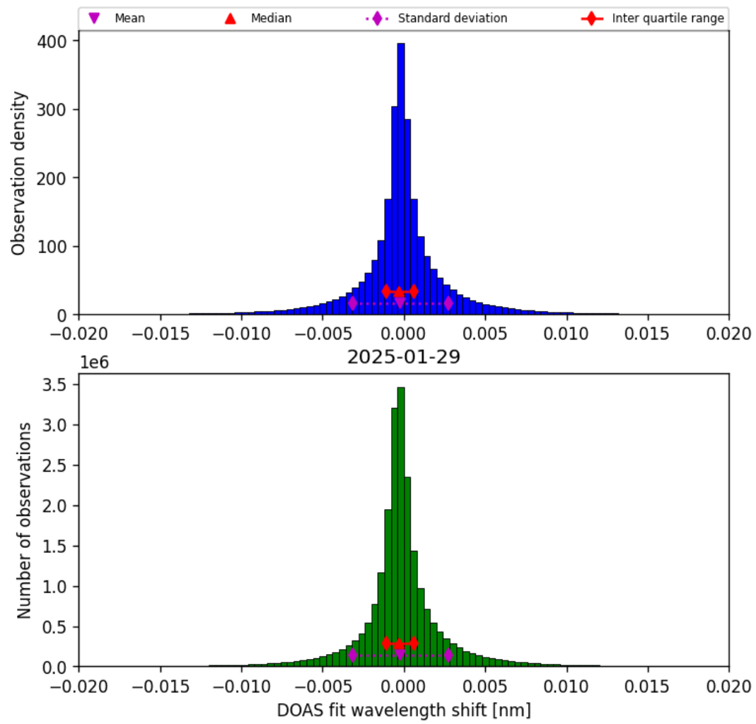
Figure 42: Histogram of “DOAS fit wavelength shift” for 2025-01-29 to 2025-01-30
