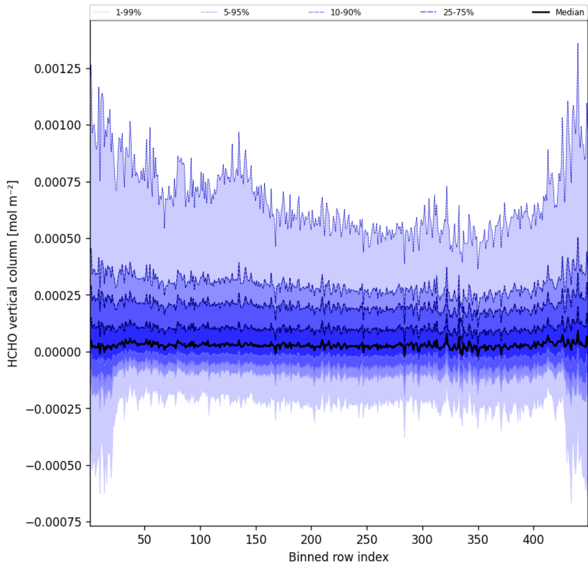
Figure 47: Along track statistics of “HCHO vertical column” for 2025-01-29 to 2025-01-30
