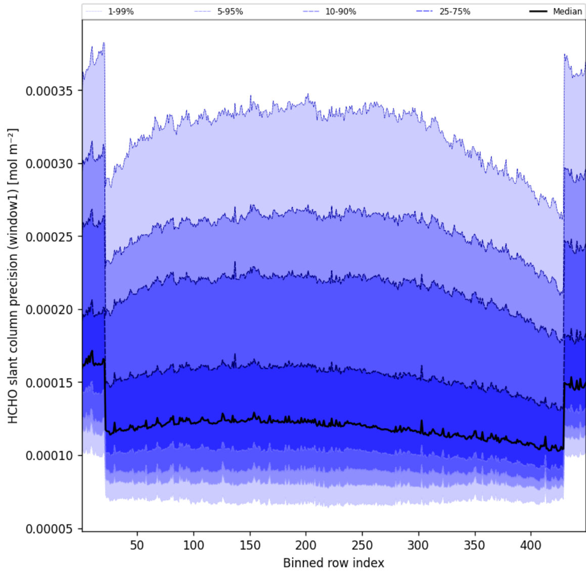
Figure 51: Along track statistics of “HCHO slant column precision (window1)” for 2025-01-29 to 2025-01-30
