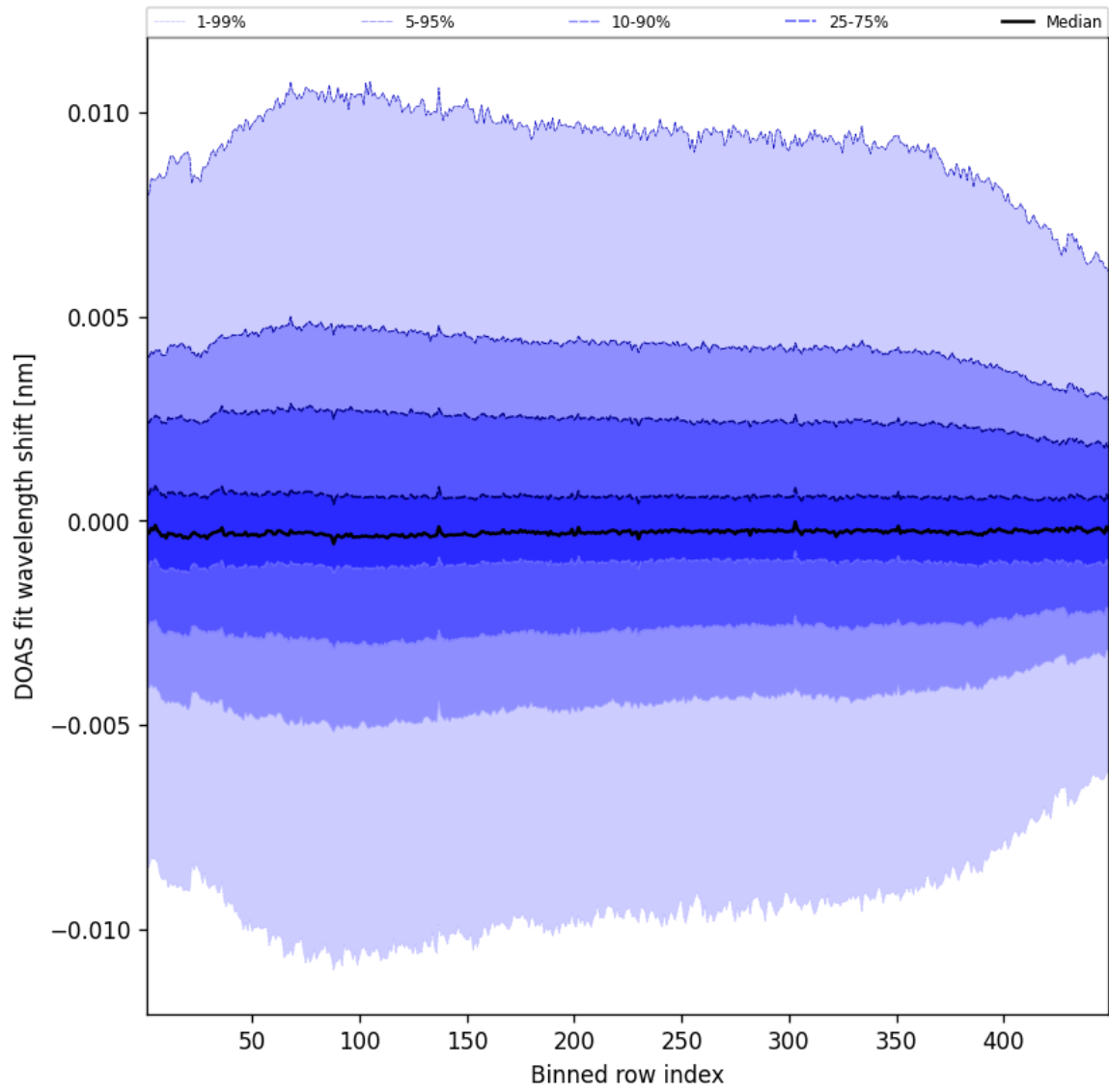
Figure 56: Along track statistics of “DOAS fit wavelength shift” for 2025-01-29 to 2025-01-30
