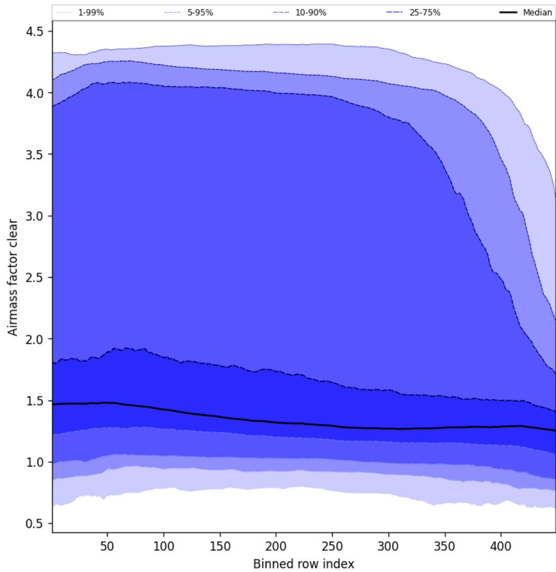
Figure 54: Along track statistics of “Airmass factor clear” for 2025-01-29 to 2025-01-30
