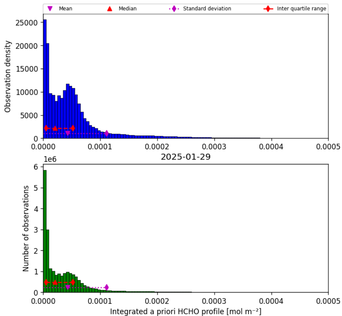
Figure 41: Histogram of “Integrated a priori HCHO profile” for 2025-01-29 to 2025-01-30
