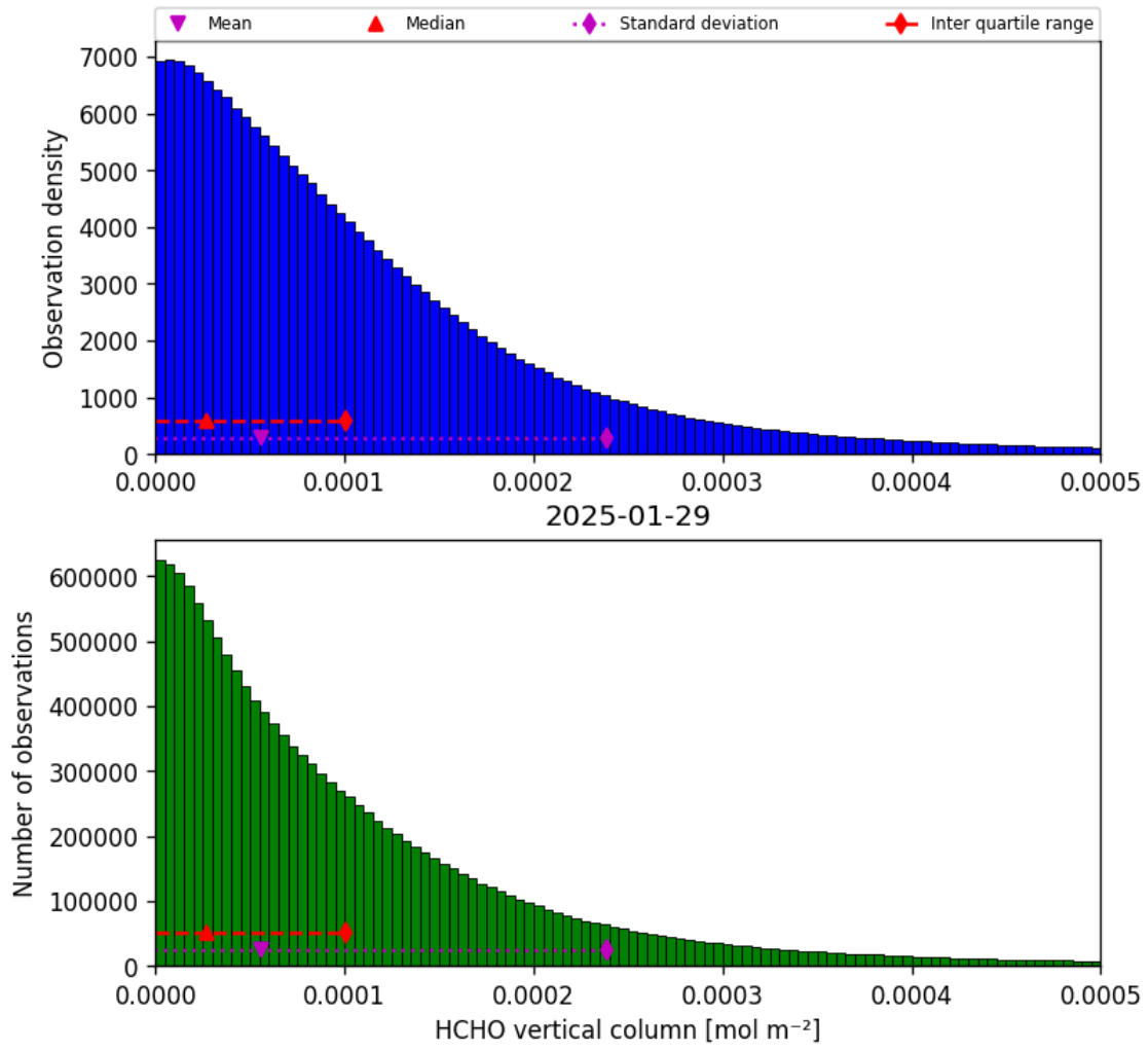
Figure 33: Histogram of “HCHO vertical column” for 2025-01-29 to 2025-01-30
