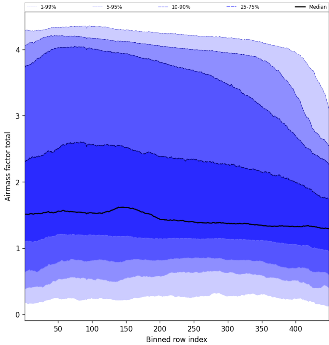
Figure 52: Along track statistics of “Airmass factor total” for 2025-01-29 to 2025-01-30
