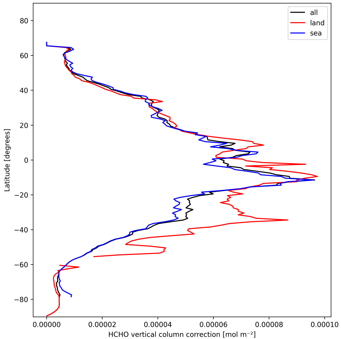
Figure 21: Zonal average of “HCHO vertical column correction” for 2025-01-30 to 2025-01-31.
