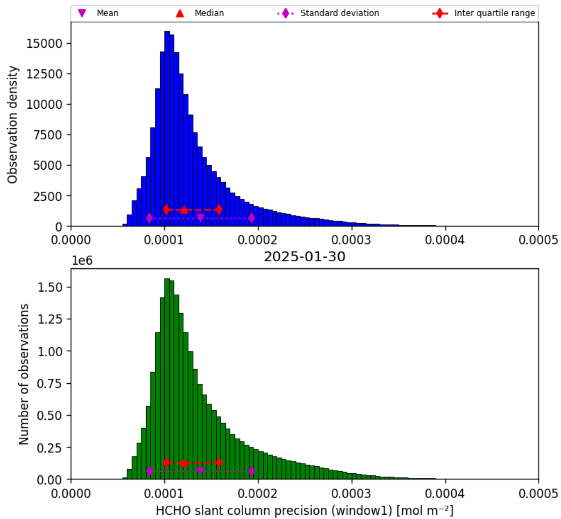
Figure 37: Histogram of “HCHO slant column precision (window1)” for 2025-01-30 to 2025-01-31
