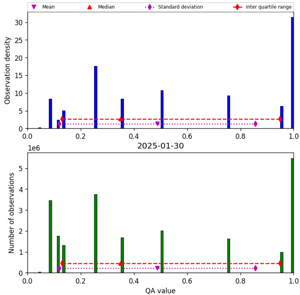
Figure 32: Histogram of “QA value” for 2025-01-30 to 2025-01-31
