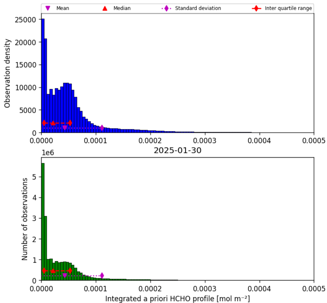
Figure 41: Histogram of “Integrated a priori HCHO profile” for 2025-01-30 to 2025-01-31
