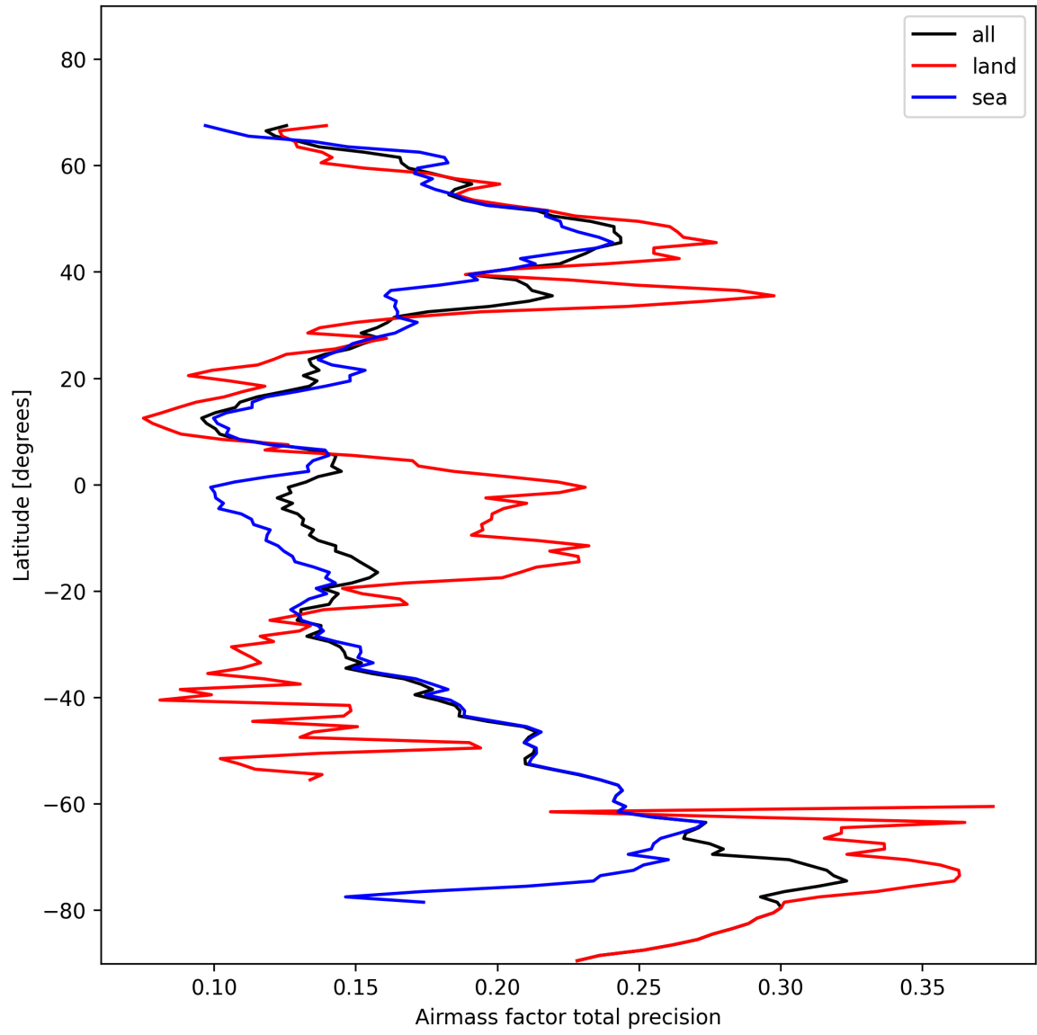
Figure 25: Zonal average of “Airmass factor total precision” for 2025-01-30 to 2025-01-31.
