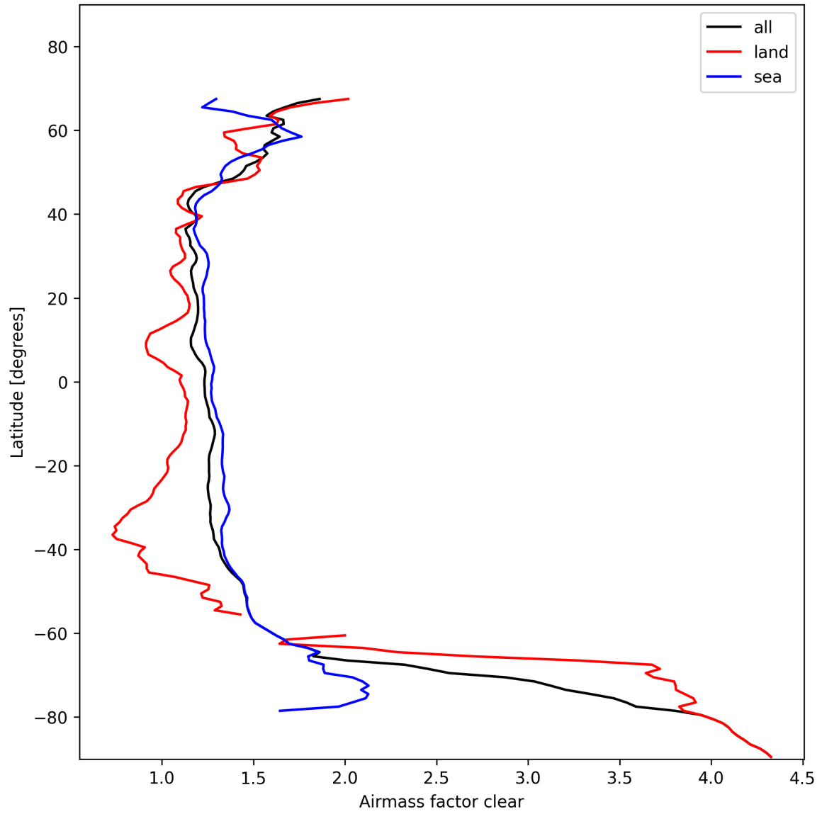
Figure 26: Zonal average of “Airmass factor clear” for 2025-01-30 to 2025-01-31.
