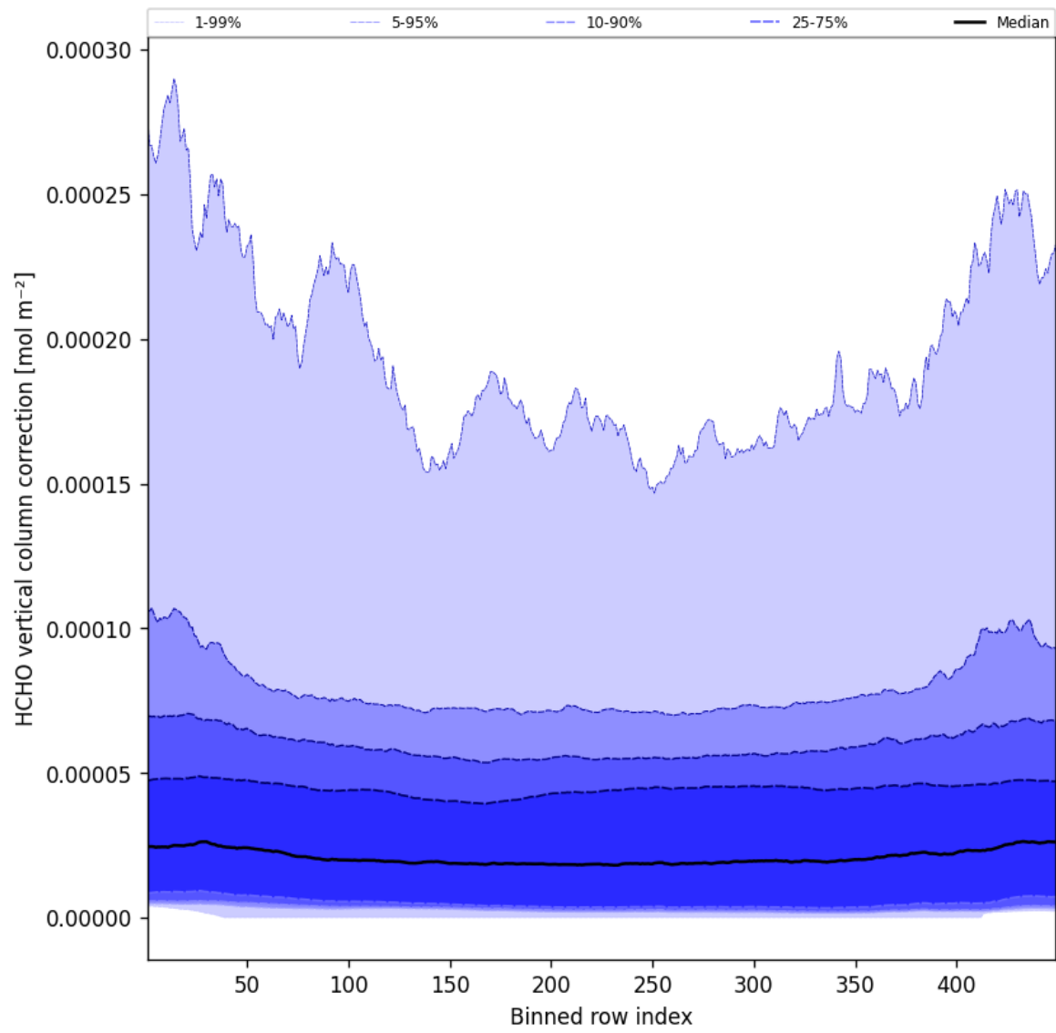
Figure 49: Along track statistics of “HCHO vertical column correction” for 2025-01-30 to 2025-01-31
