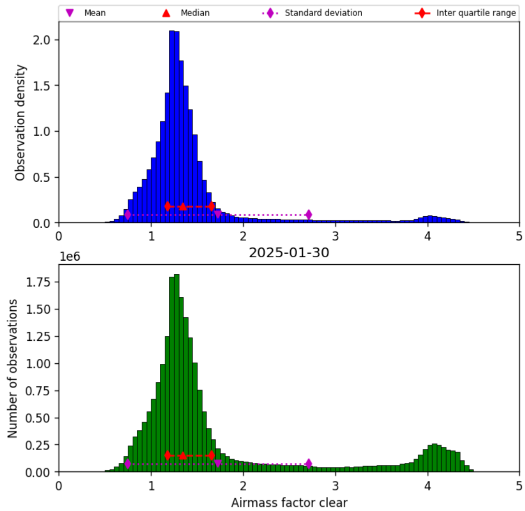
Figure 40: Histogram of “Airmass factor clear” for 2025-01-30 to 2025-01-31
