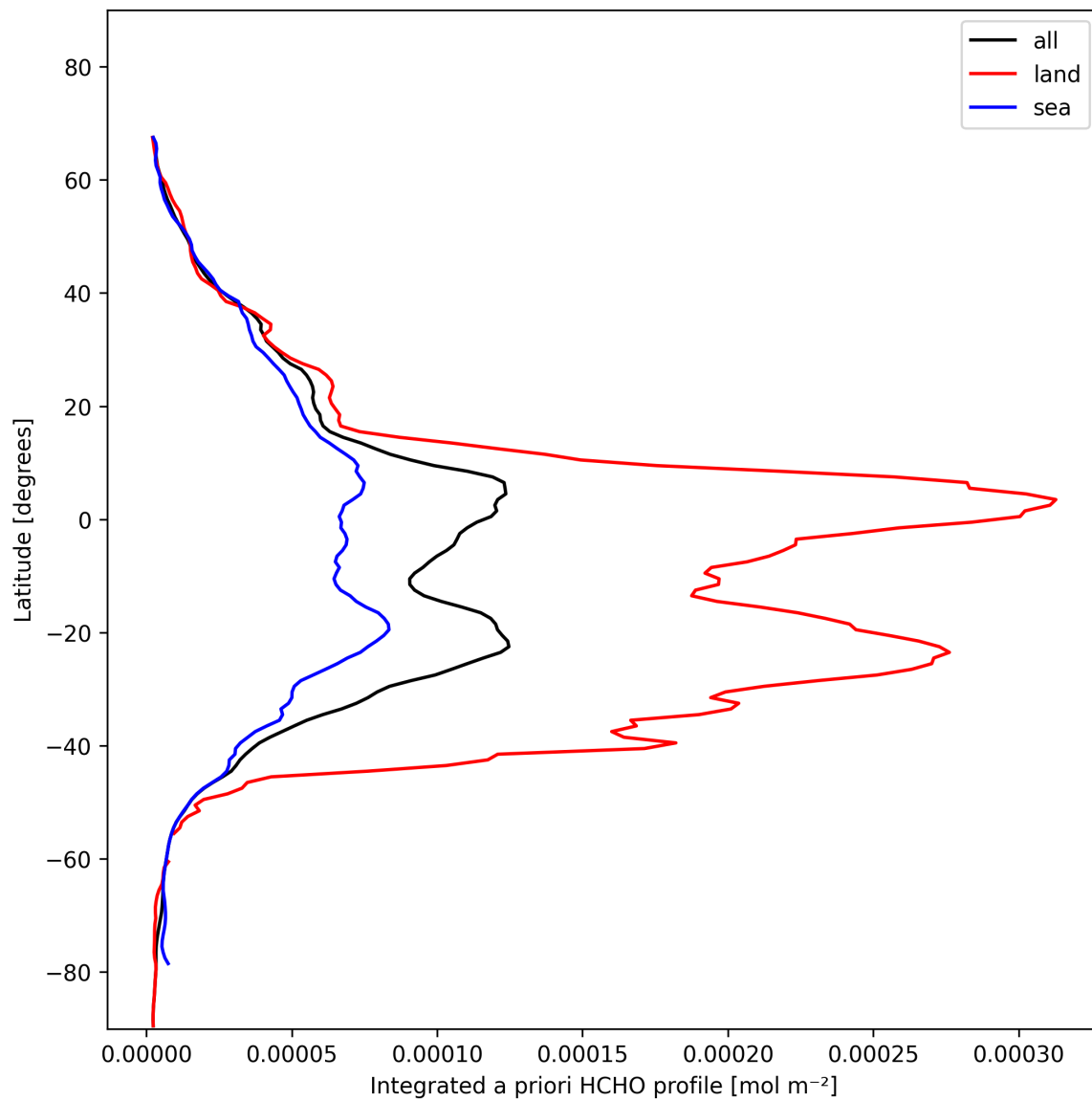
Figure 27: Zonal average of “Integrated a priori HCHO profile” for 2025-01-30 to 2025-01-31.
