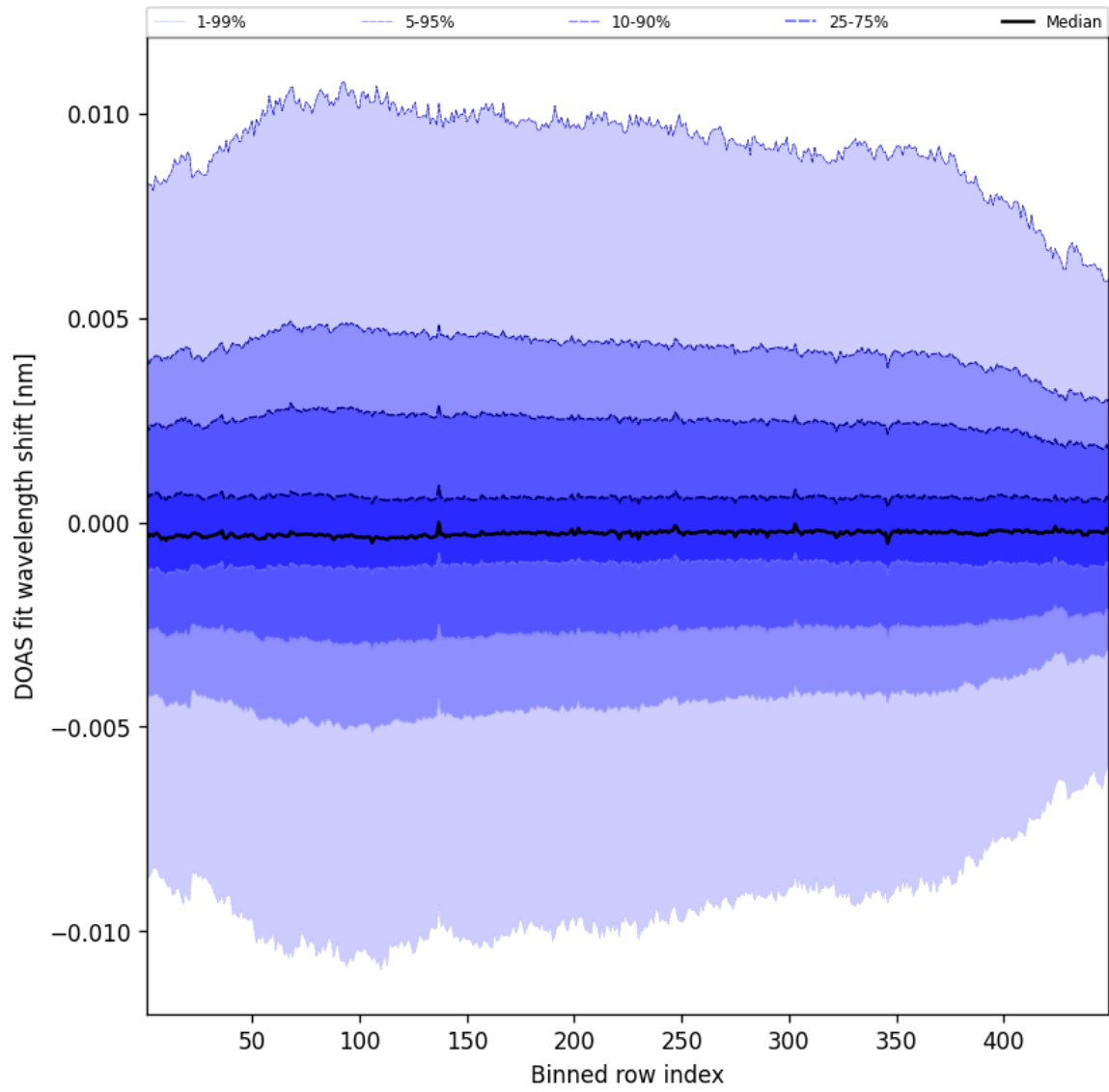
Figure 56: Along track statistics of “DOAS fit wavelength shift” for 2025-01-30 to 2025-01-31
