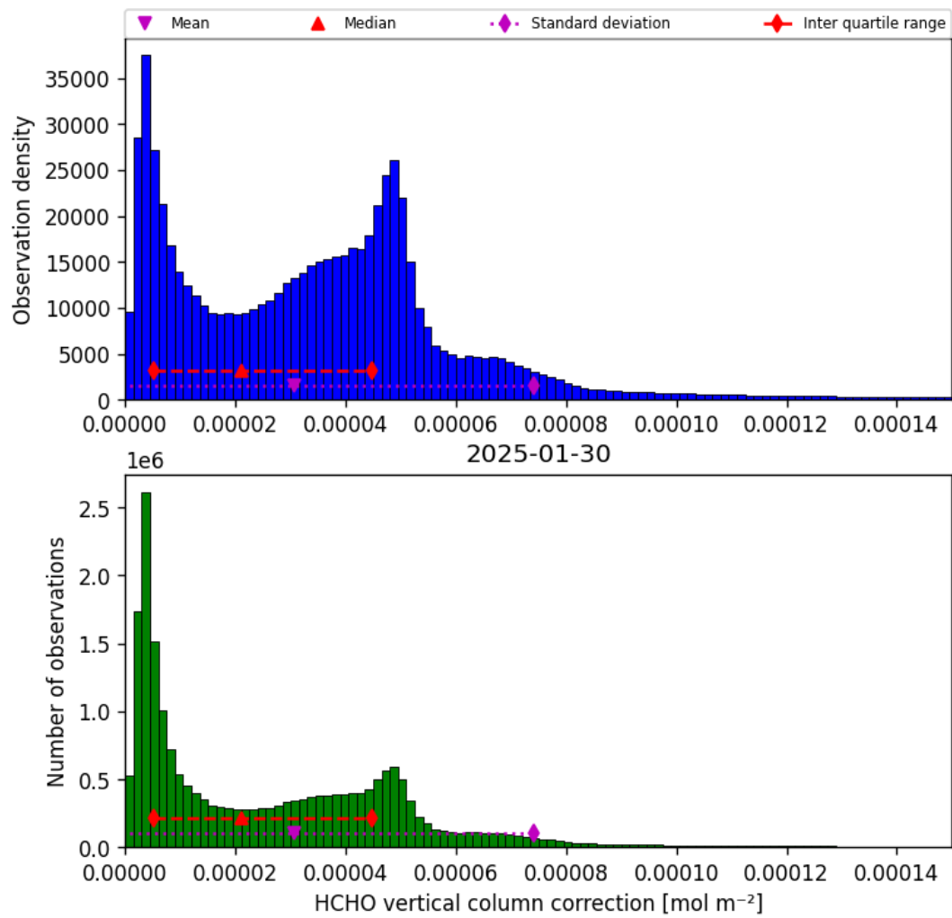
Figure 35: Histogram of “HCHO vertical column correction” for 2025-01-30 to 2025-01-31
