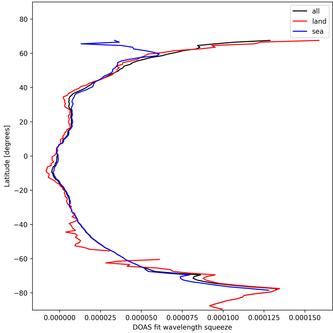
Figure 29: Zonal average of “DOAS fit wavelength squeeze” for 2025-01-30 to 2025-01-31.
