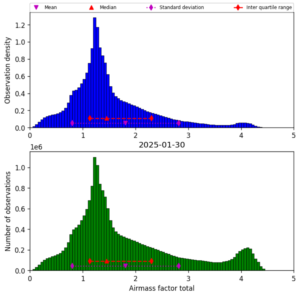
Figure 38: Histogram of “Airmass factor total” for 2025-01-30 to 2025-01-31
