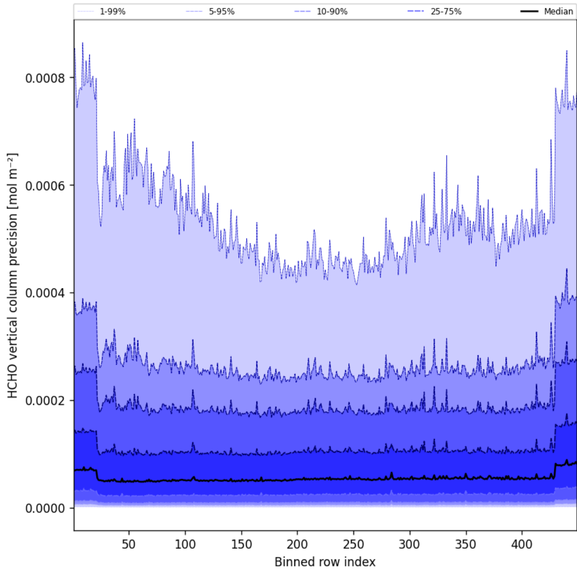
Figure 48: Along track statistics of “HCHO vertical column precision” for 2025-01-30 to 2025-01-31
