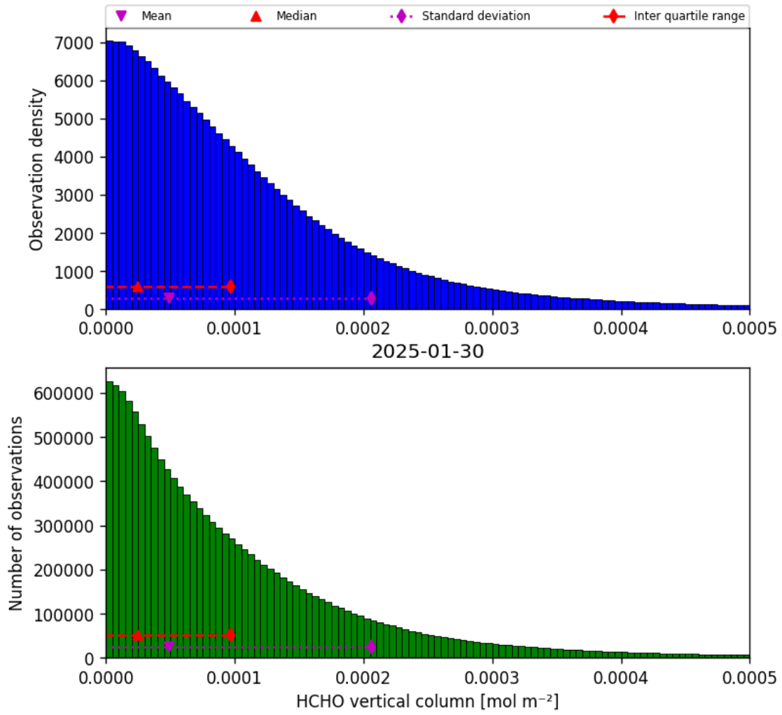
Figure 33: Histogram of “HCHO vertical column” for 2025-01-30 to 2025-01-31
