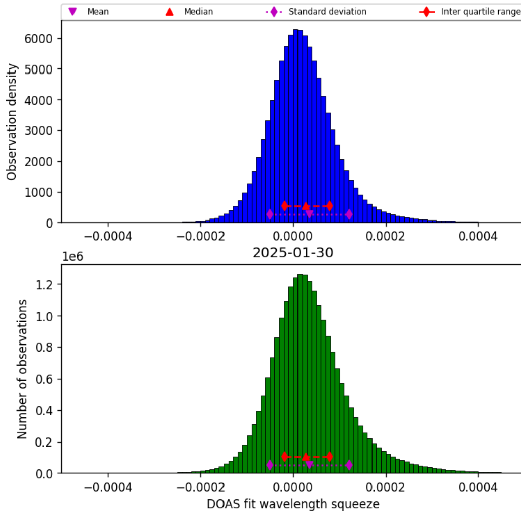
Figure 43: Histogram of “DOAS fit wavelength squeeze” for 2025-01-30 to 2025-01-31
