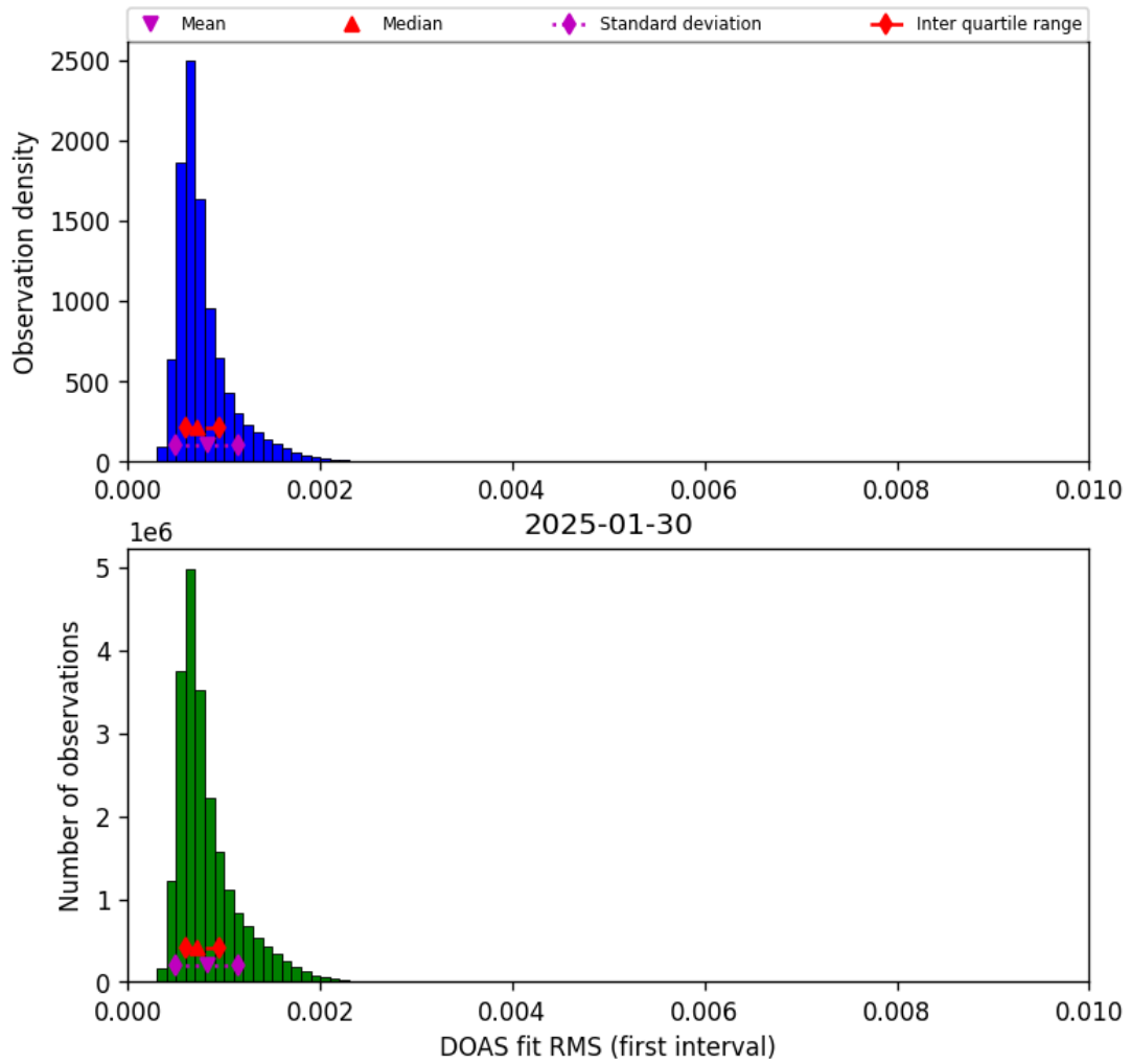
Figure 44: Histogram of “DOAS fit RMS (first interval)” for 2025-01-30 to 2025-01-31
