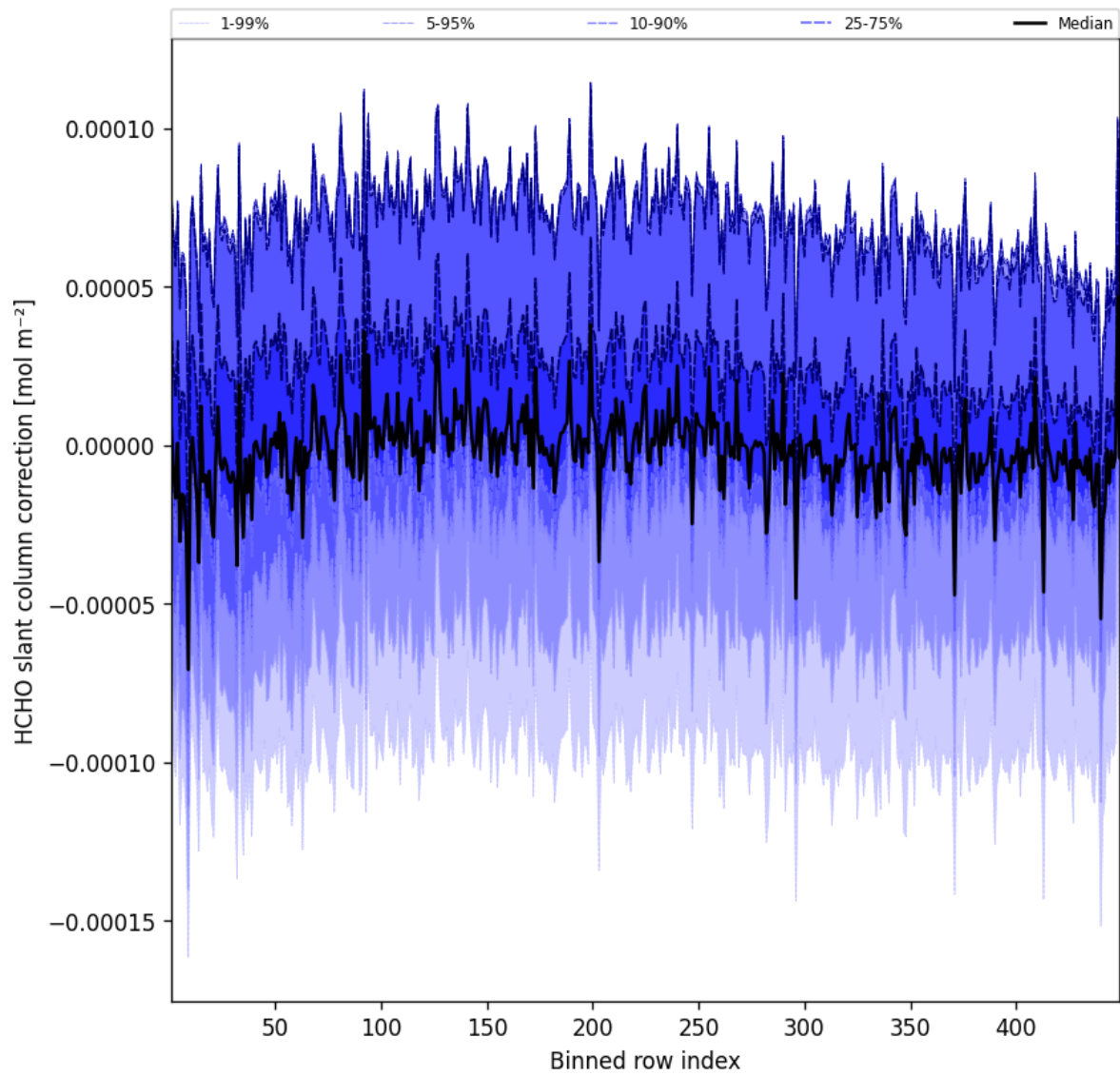
Figure 59: Along track statistics of “HCHO slant column correction” for 2025-01-30 to 2025-01-31
