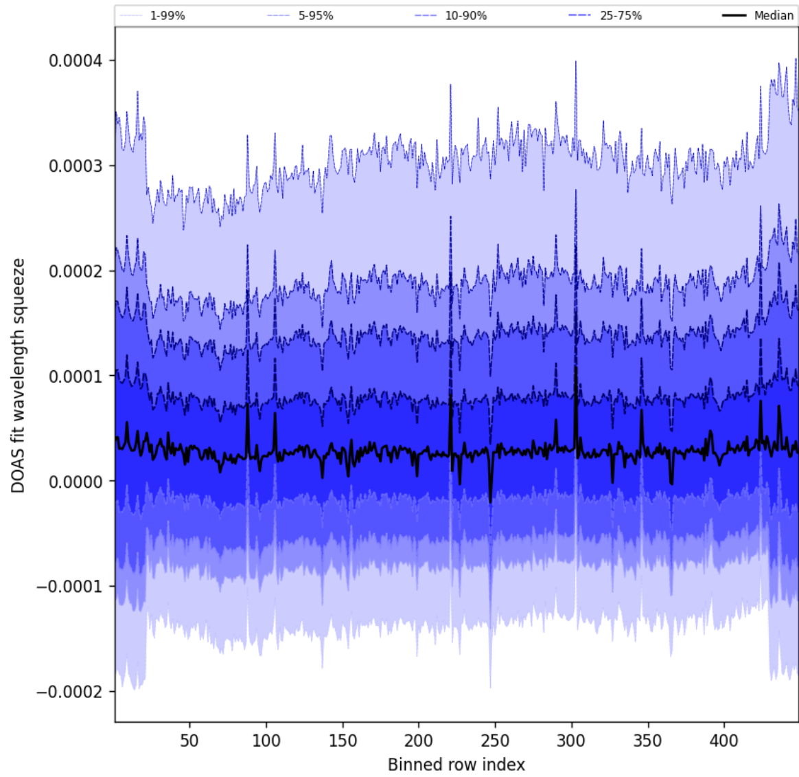
Figure 57: Along track statistics of “DOAS fit wavelength squeeze” for 2025-01-30 to 2025-01-31
