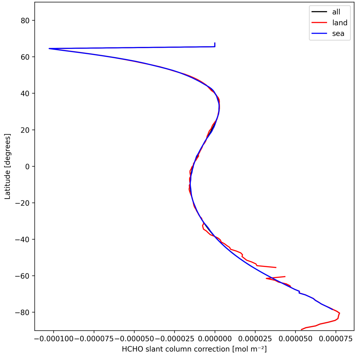
Figure 31: Zonal average of “HCHO slant column correction” for 2025-01-30 to 2025-01-31.
