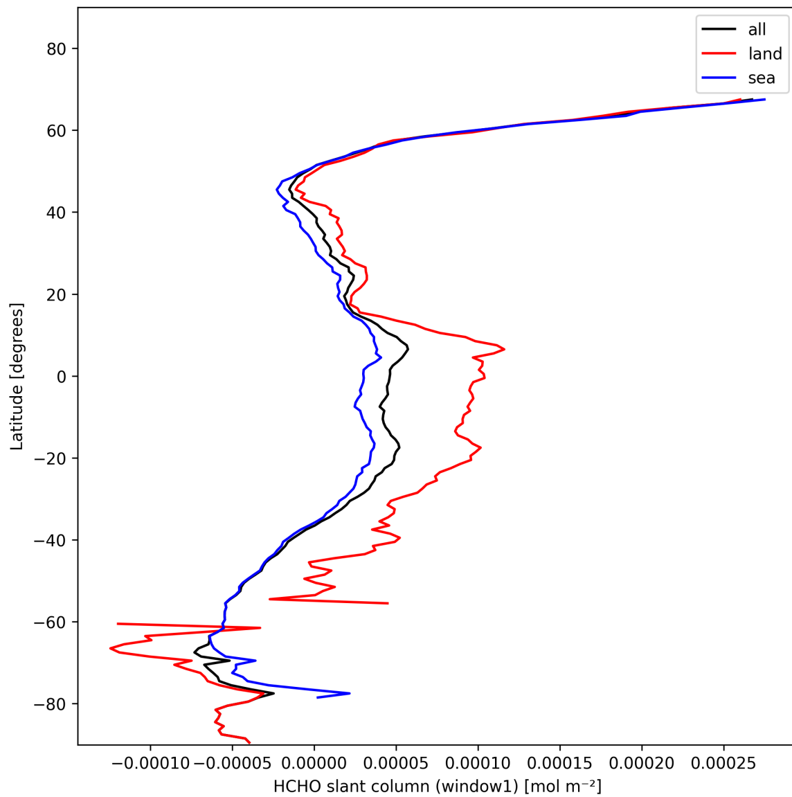
Figure 22: Zonal average of “HCHO slant column (window1)” for 2025-01-30 to 2025-01-31.
