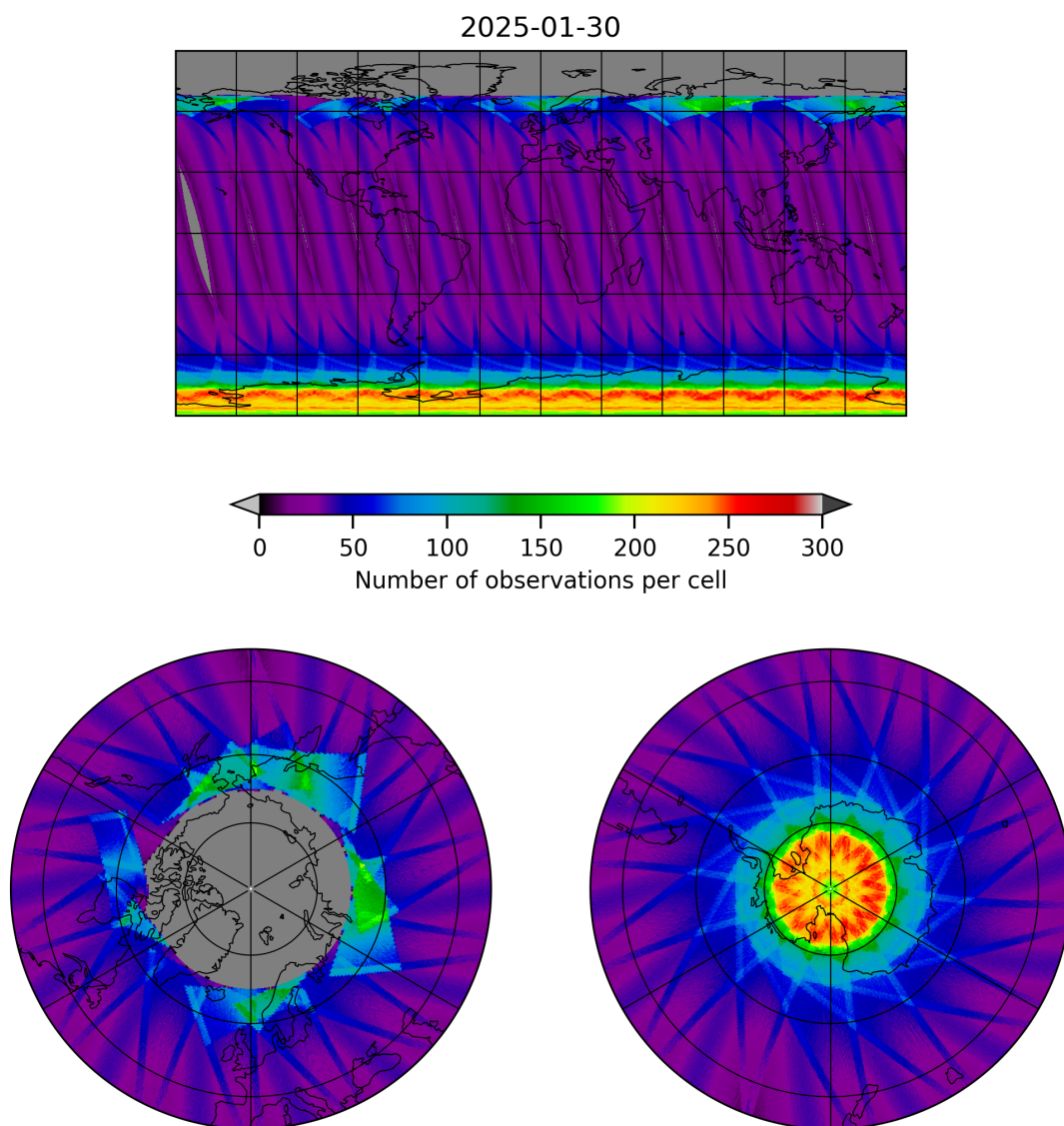
Figure 17: Map of the number of observations for 2025-01-30 to 2025-01-31
