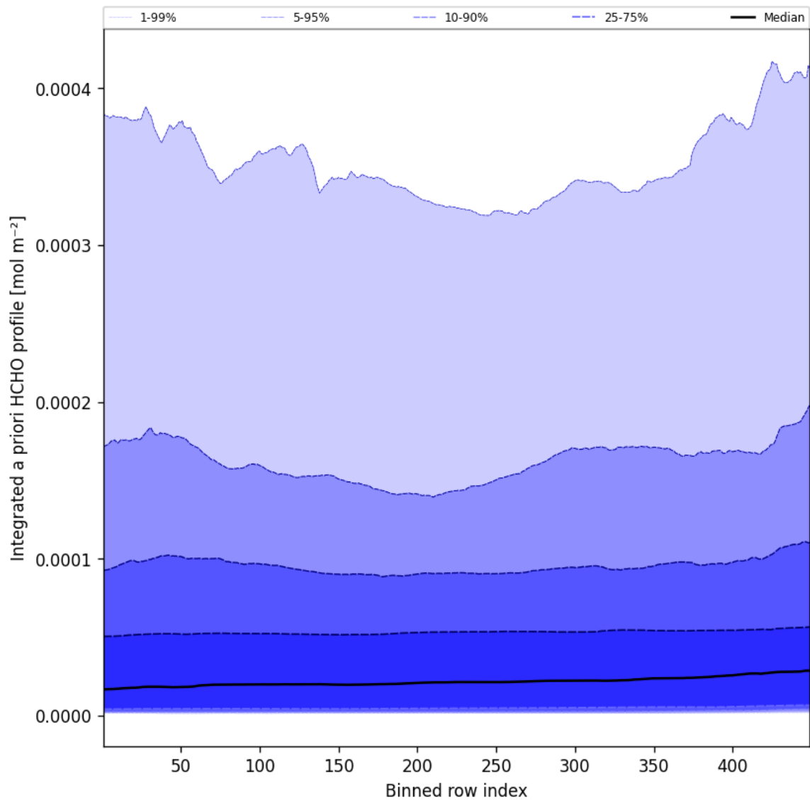
Figure 55: Along track statistics of “Integrated a priori HCHO profile” for 2025-01-30 to 2025-01-31
