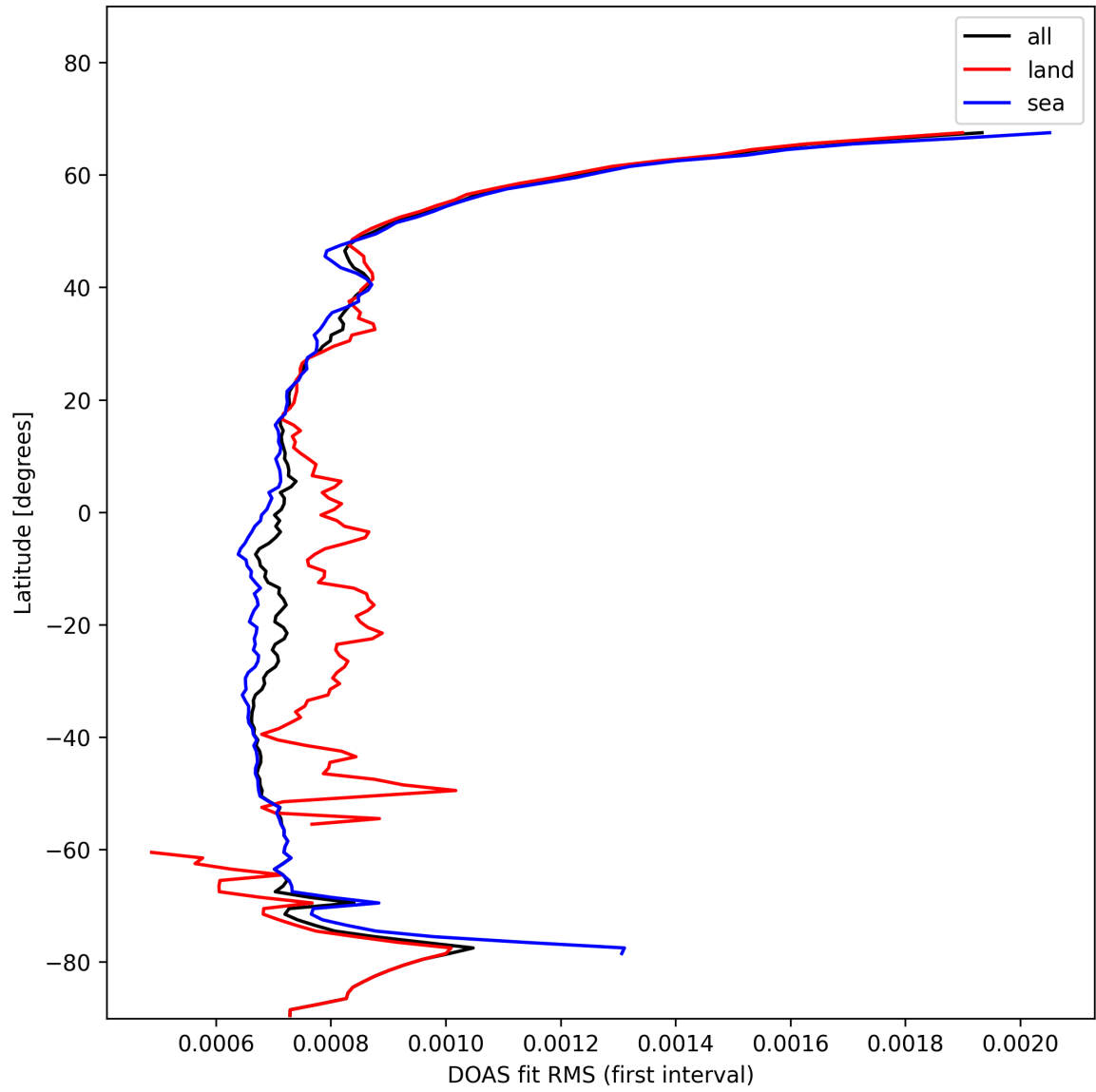
Figure 30: Zonal average of “DOAS fit RMS (first interval)” for 2025-01-30 to 2025-01-31.
