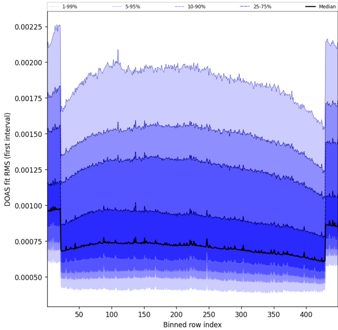
Figure 58: Along track statistics of “DOAS fit RMS (first interval)” for 2025-01-30 to 2025-01-31
