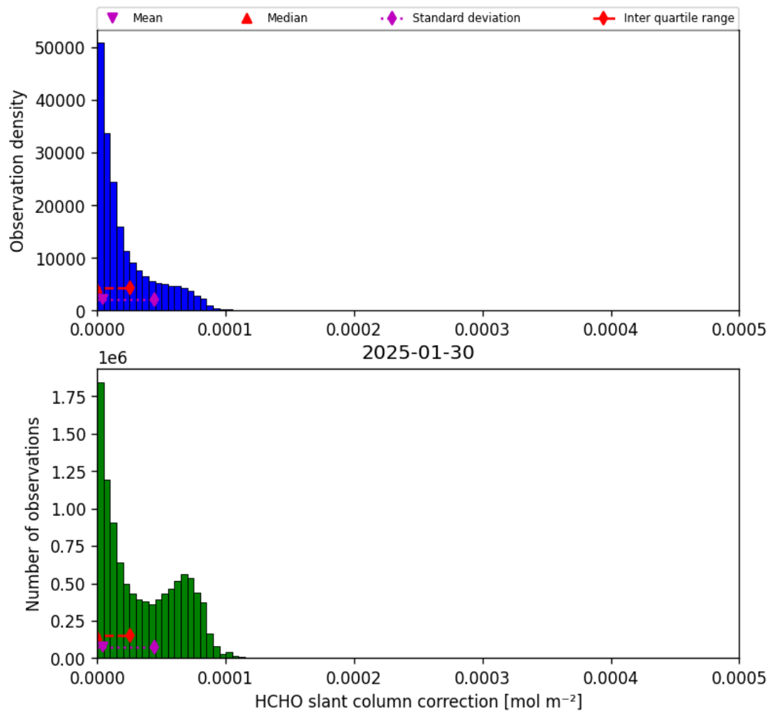
Figure 45: Histogram of “HCHO slant column correction” for 2025-01-30 to 2025-01-31
