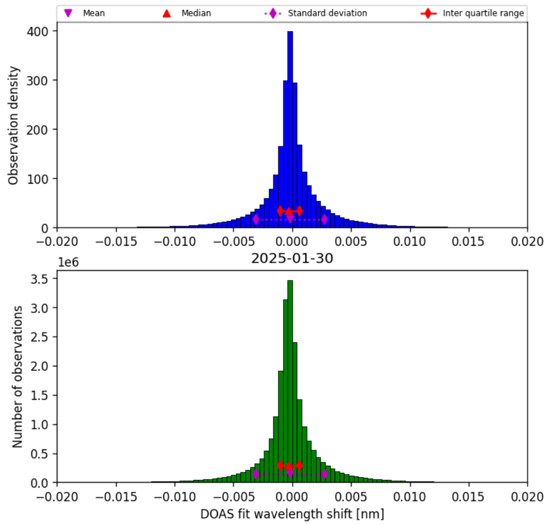
Figure 42: Histogram of “DOAS fit wavelength shift” for 2025-01-30 to 2025-01-31
