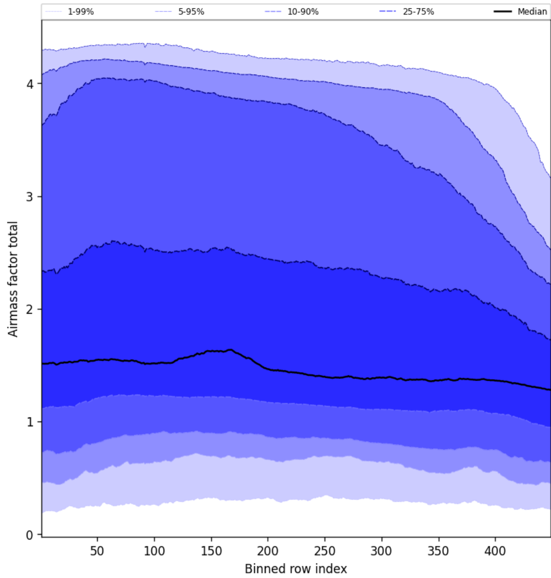
Figure 52: Along track statistics of “Airmass factor total” for 2025-01-30 to 2025-01-31
