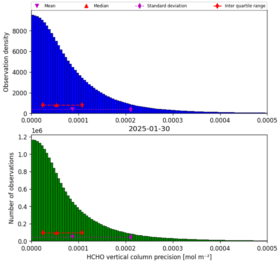
Figure 34: Histogram of “HCHO vertical column precision” for 2025-01-30 to 2025-01-31
