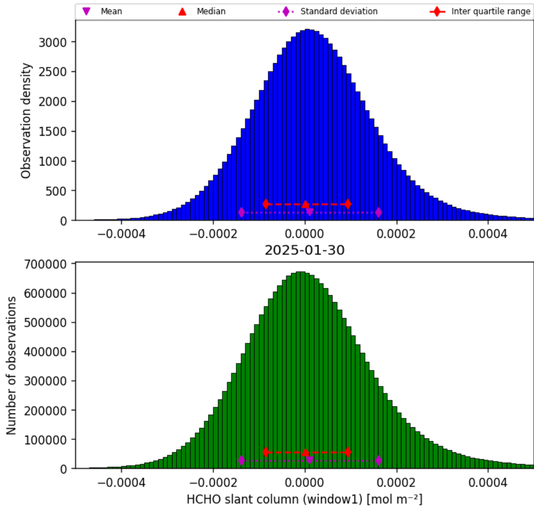
Figure 36: Histogram of “HCHO slant column (window1)” for 2025-01-30 to 2025-01-31
