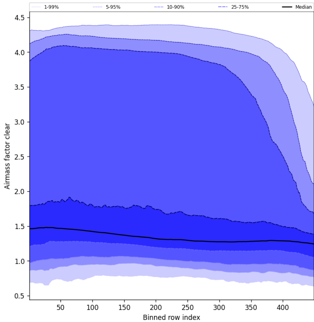
Figure 54: Along track statistics of “Airmass factor clear” for 2025-01-30 to 2025-01-31
