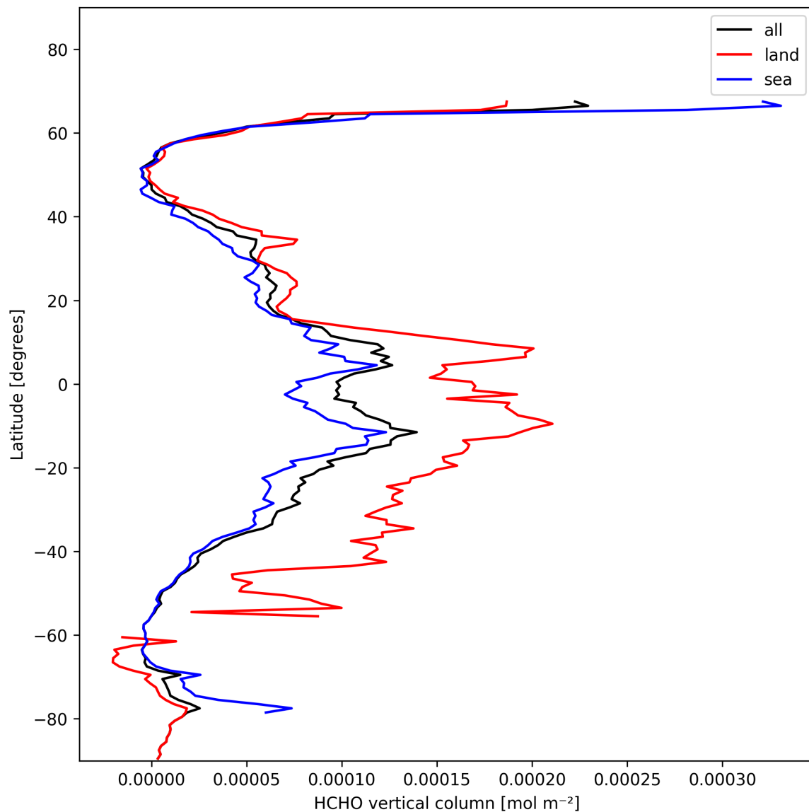
Figure 19: Zonal average of “HCHO vertical column” for 2025-01-30 to 2025-01-31.
