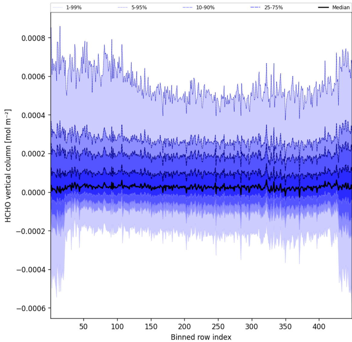
Figure 47: Along track statistics of “HCHO vertical column” for 2025-01-30 to 2025-01-31
