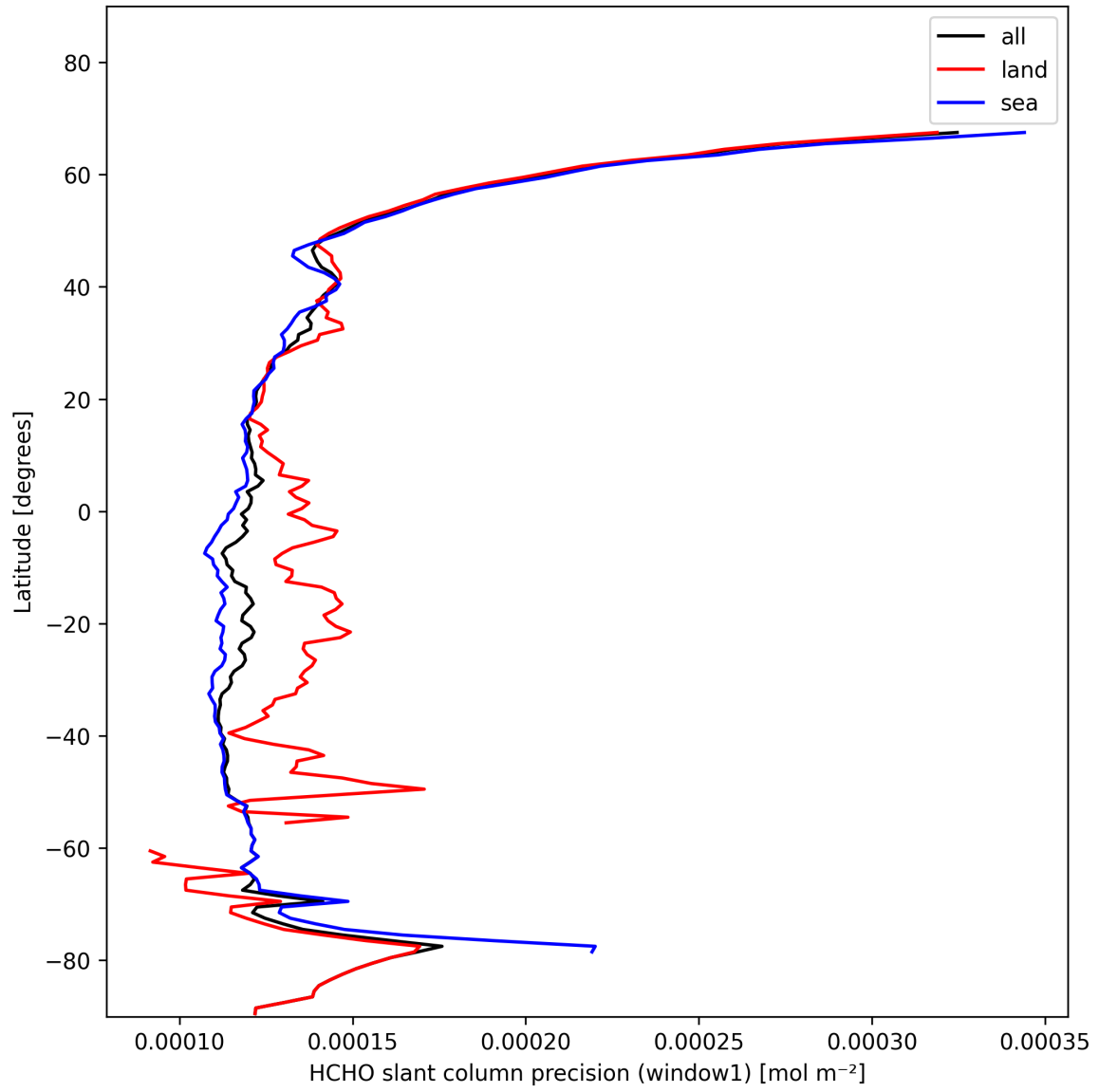
Figure 23: Zonal average of “HCHO slant column precision (window1)” for 2025-01-30 to 2025-01-31.
