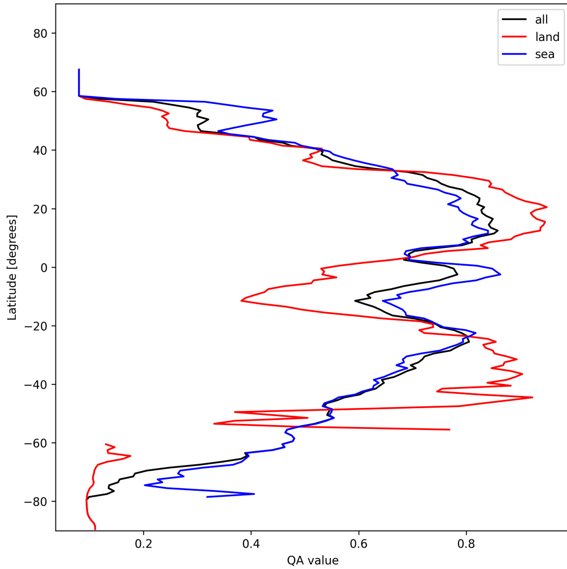
Figure 18: Zonal average of “QA value” for 2025-01-30 to 2025-01-31.
