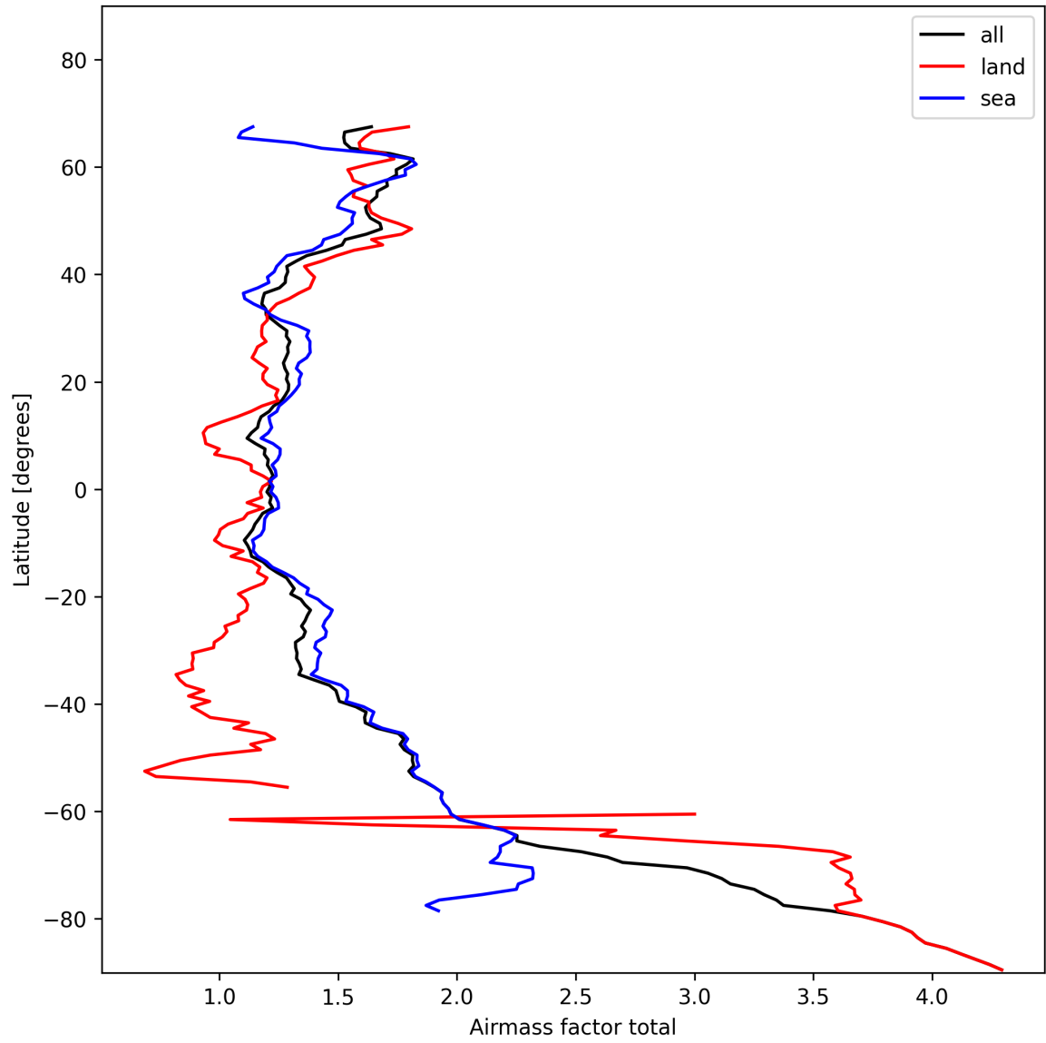
Figure 24: Zonal average of “Airmass factor total” for 2025-01-30 to 2025-01-31.
