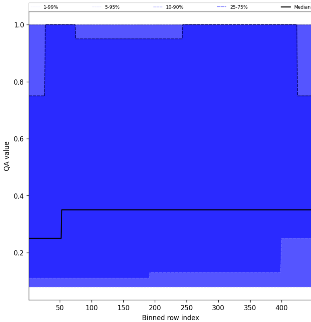
Figure 46: Along track statistics of “QA value” for 2025-01-30 to 2025-01-31
