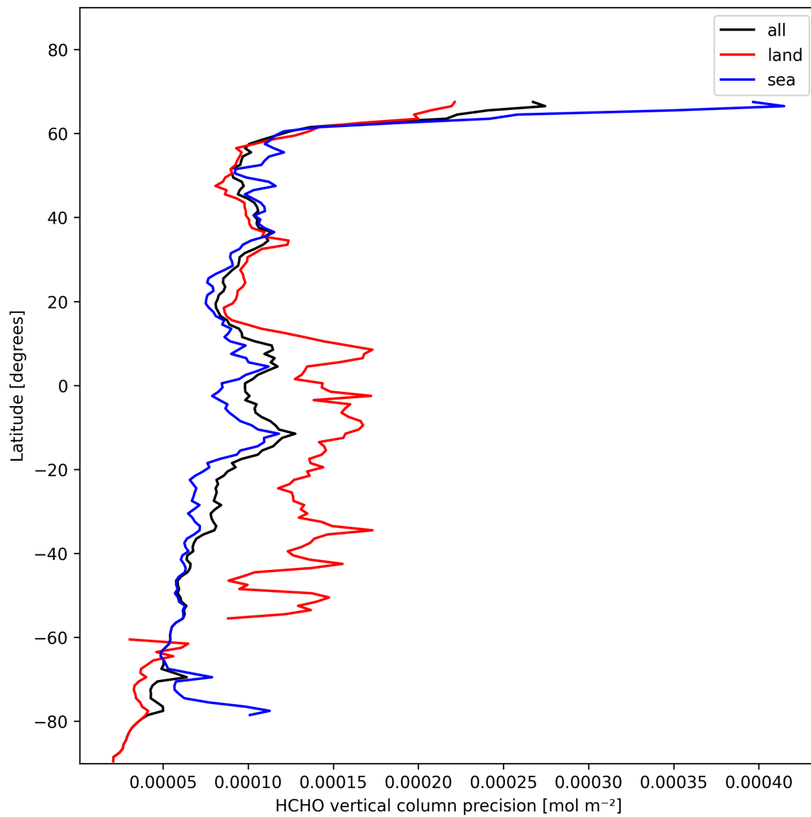
Figure 20: Zonal average of “HCHO vertical column precision” for 2025-01-30 to 2025-01-31.
