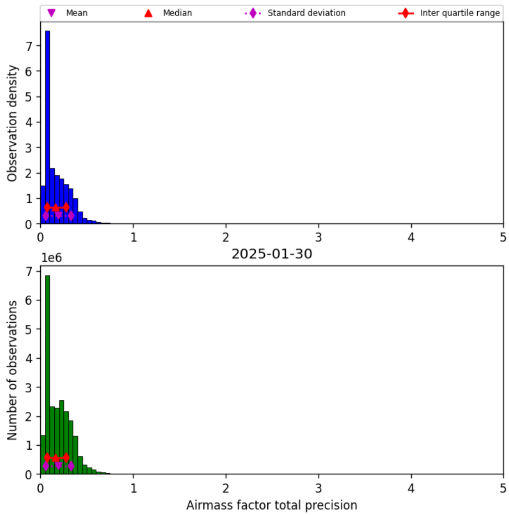
Figure 39: Histogram of “Airmass factor total precision” for 2025-01-30 to 2025-01-31
