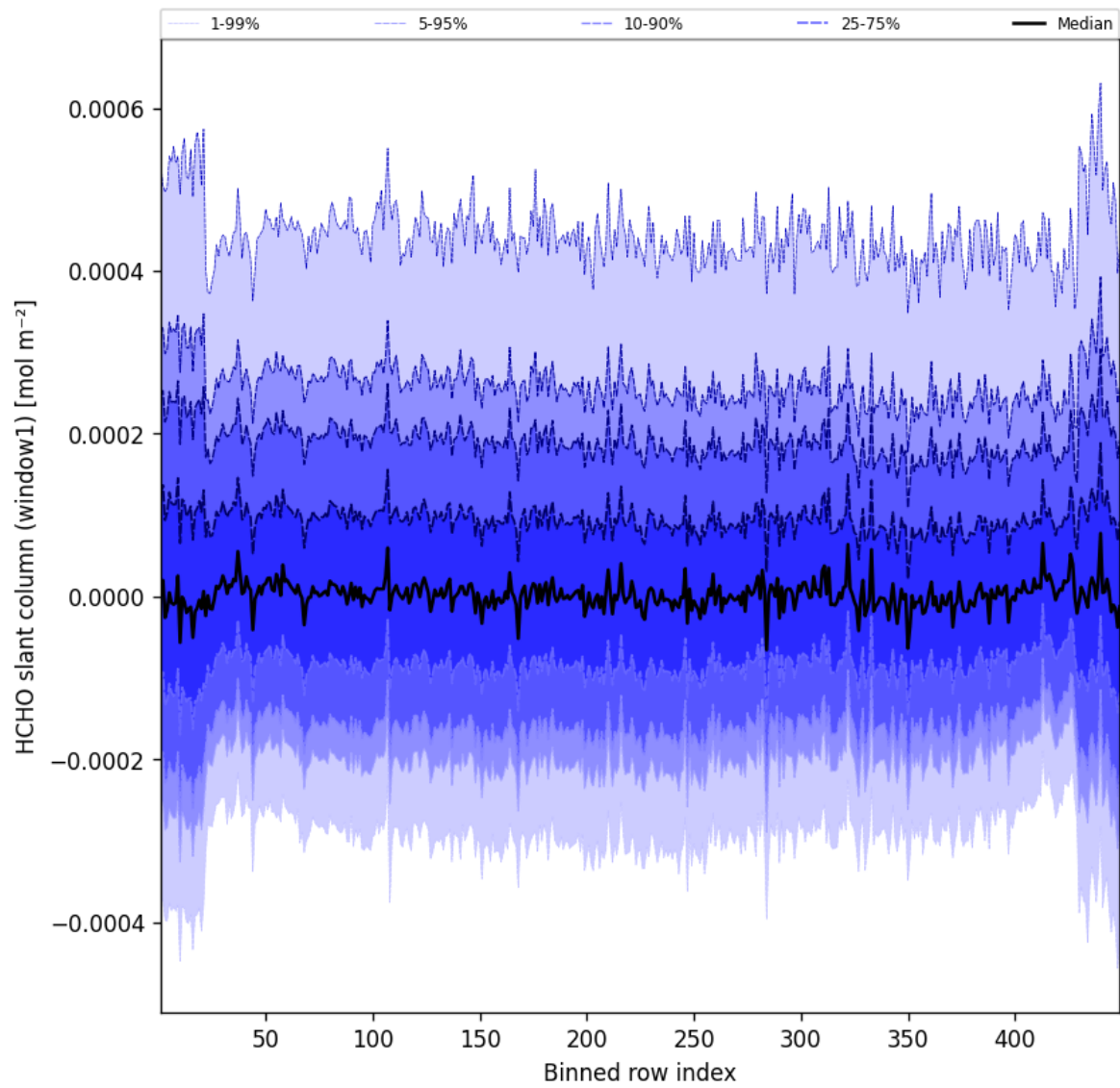
Figure 50: Along track statistics of “HCHO slant column (window1)” for 2025-01-30 to 2025-01-31
