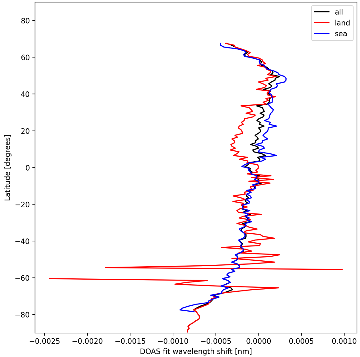
Figure 28: Zonal average of "DOAS fit wavelength shift" for 2025-01-30 to 2025-01-31.
