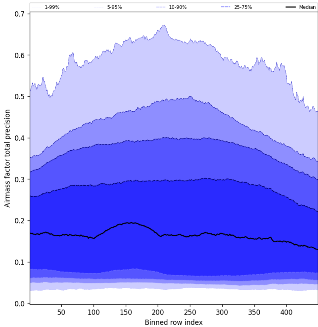
Figure 53: Along track statistics of “Airmass factor total precision” for 2025-01-30 to 2025-01-31
