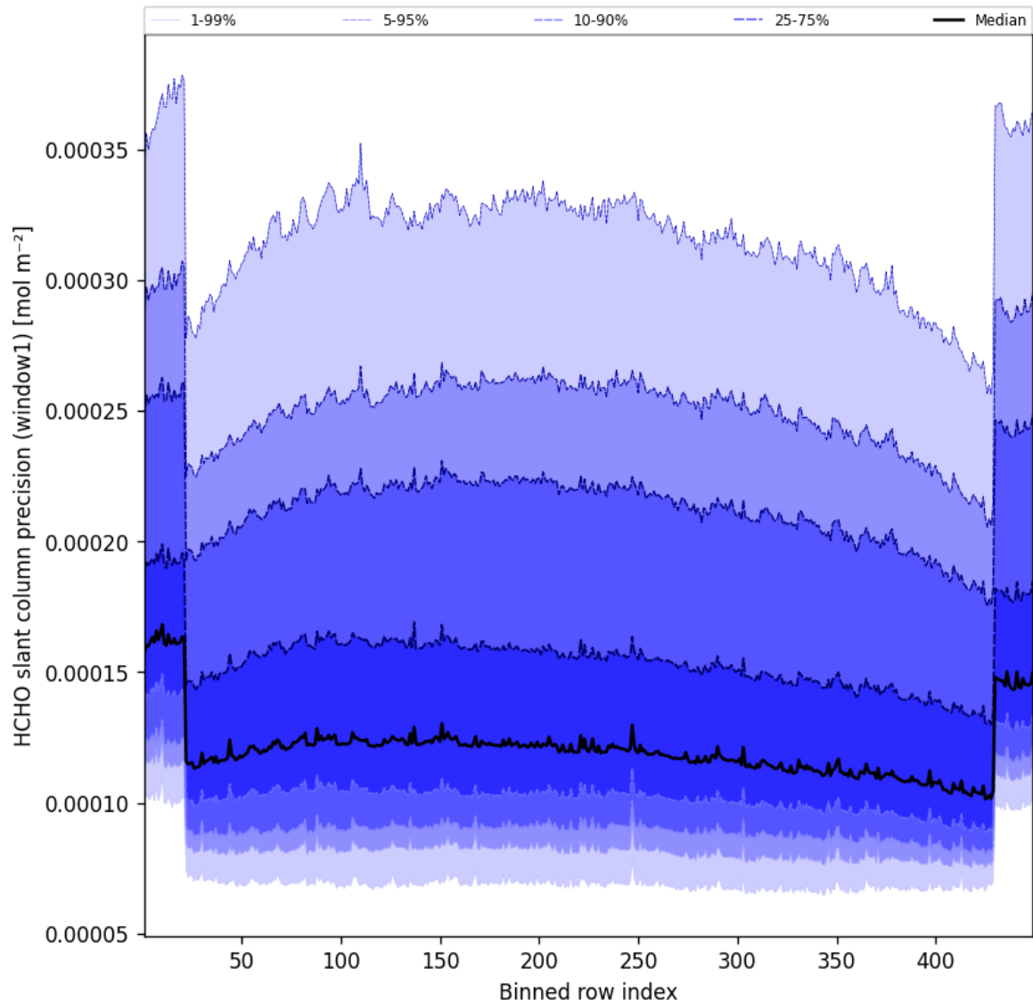
Figure 51: Along track statistics of “HCHO slant column precision (window1)” for 2025-01-30 to 2025-01-31
